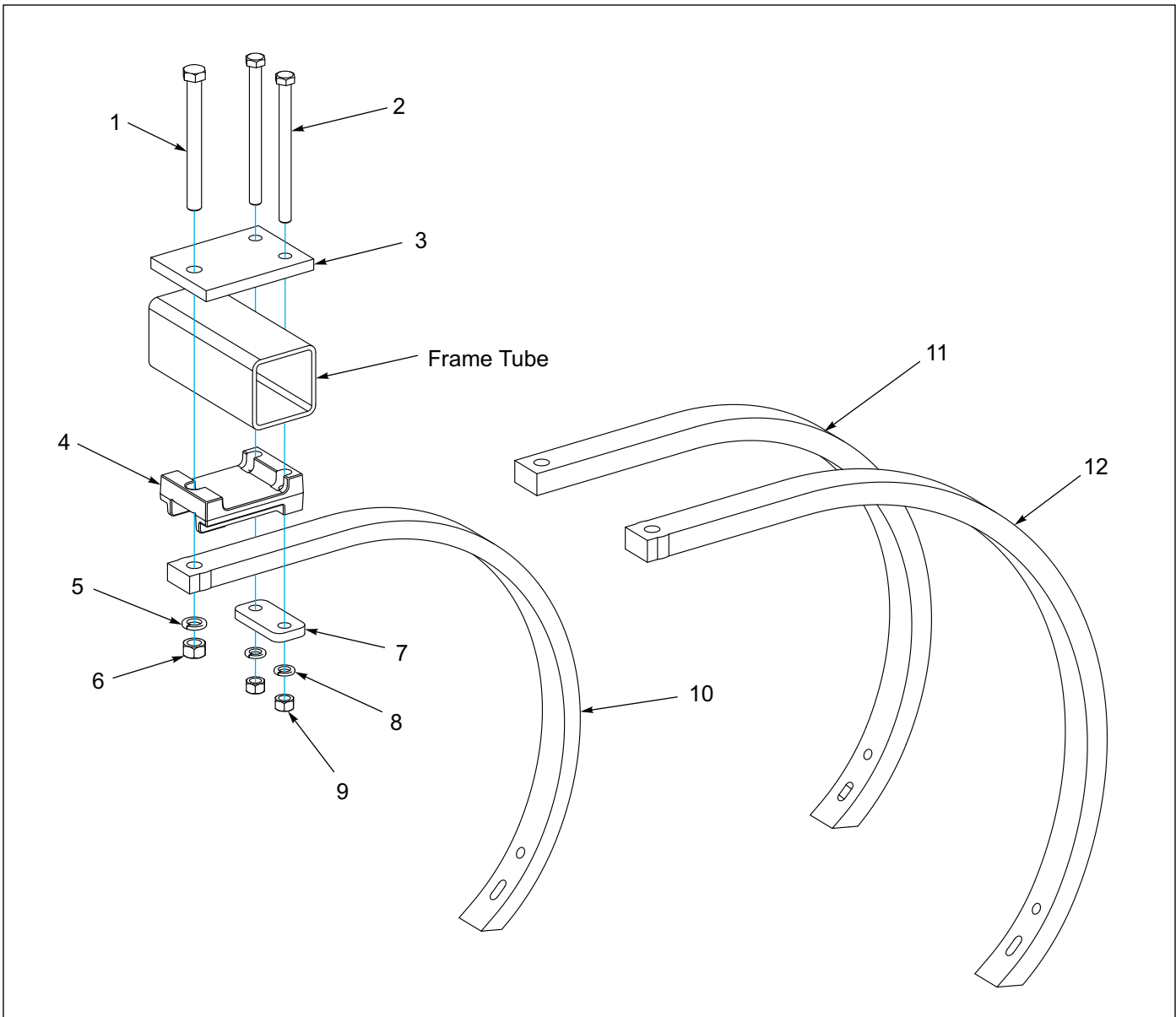
Figure 1-7: Rigid Shank Assembly
