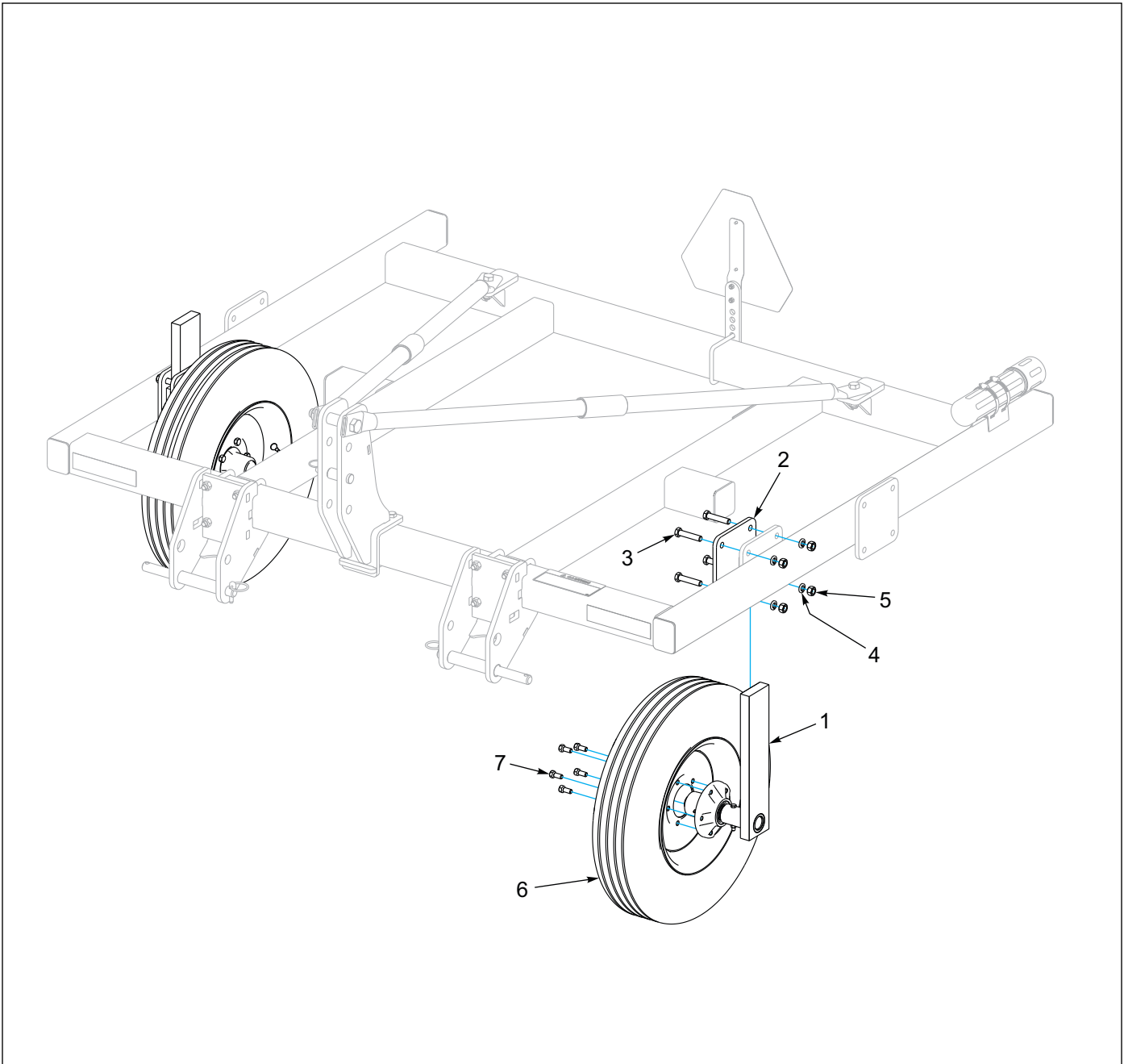
Figure 1-16: Optional Gauge Wheel Kit 26"
