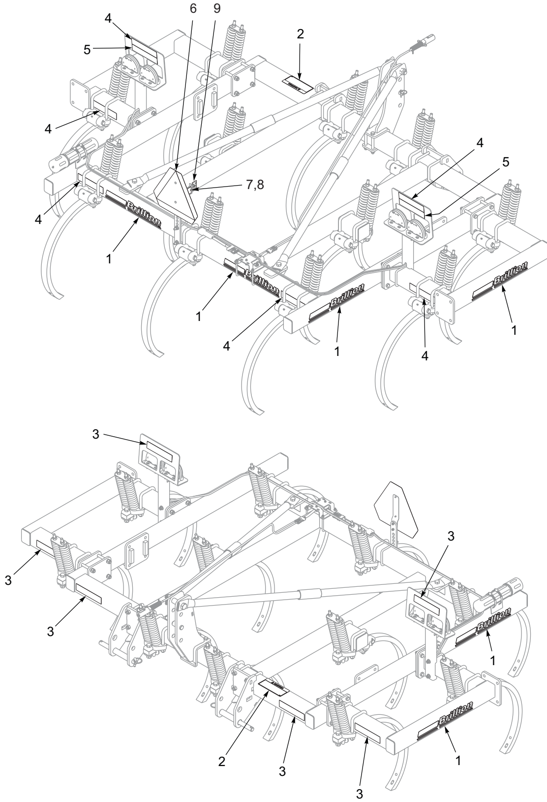
Figure 1-24: Decals (11 Shank Models)
