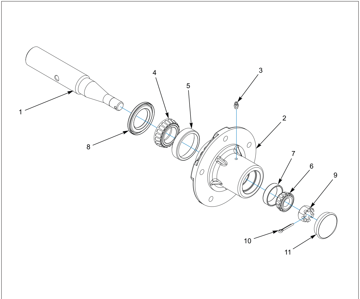
Figure 1-19: Hub and Spindle Assembly
