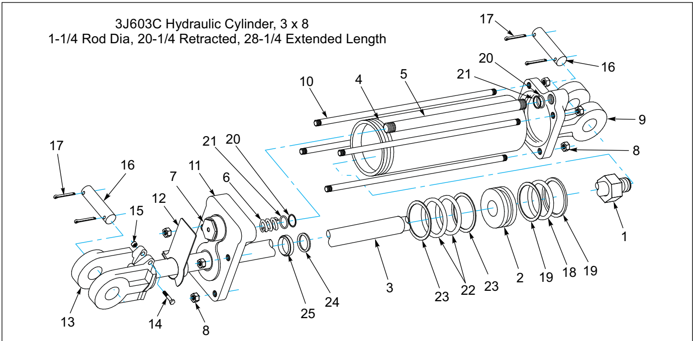
Figure 1-29: Hydraulic Cylinder, 3 X 8 - Cross
