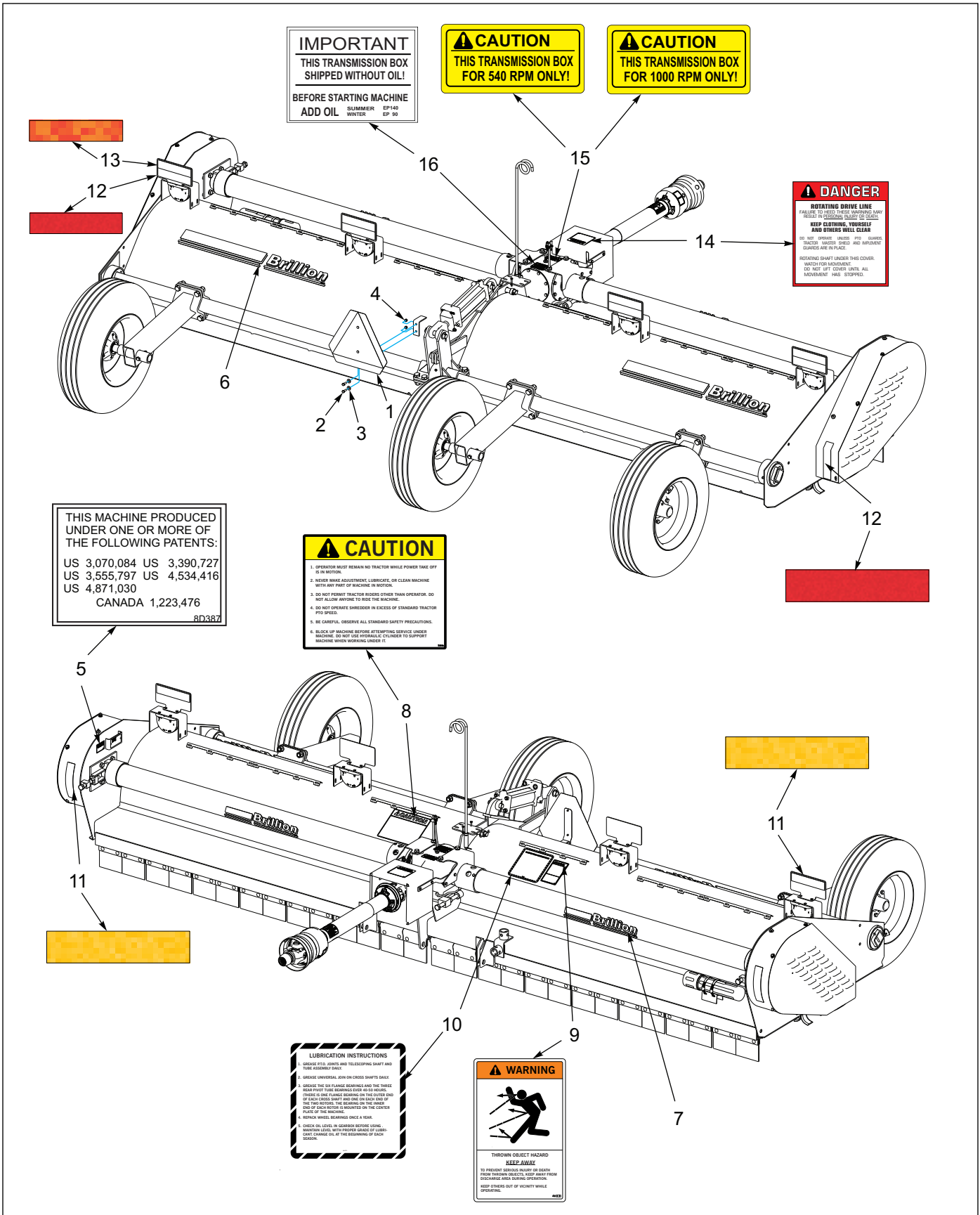
Figure 1-2: Decals
