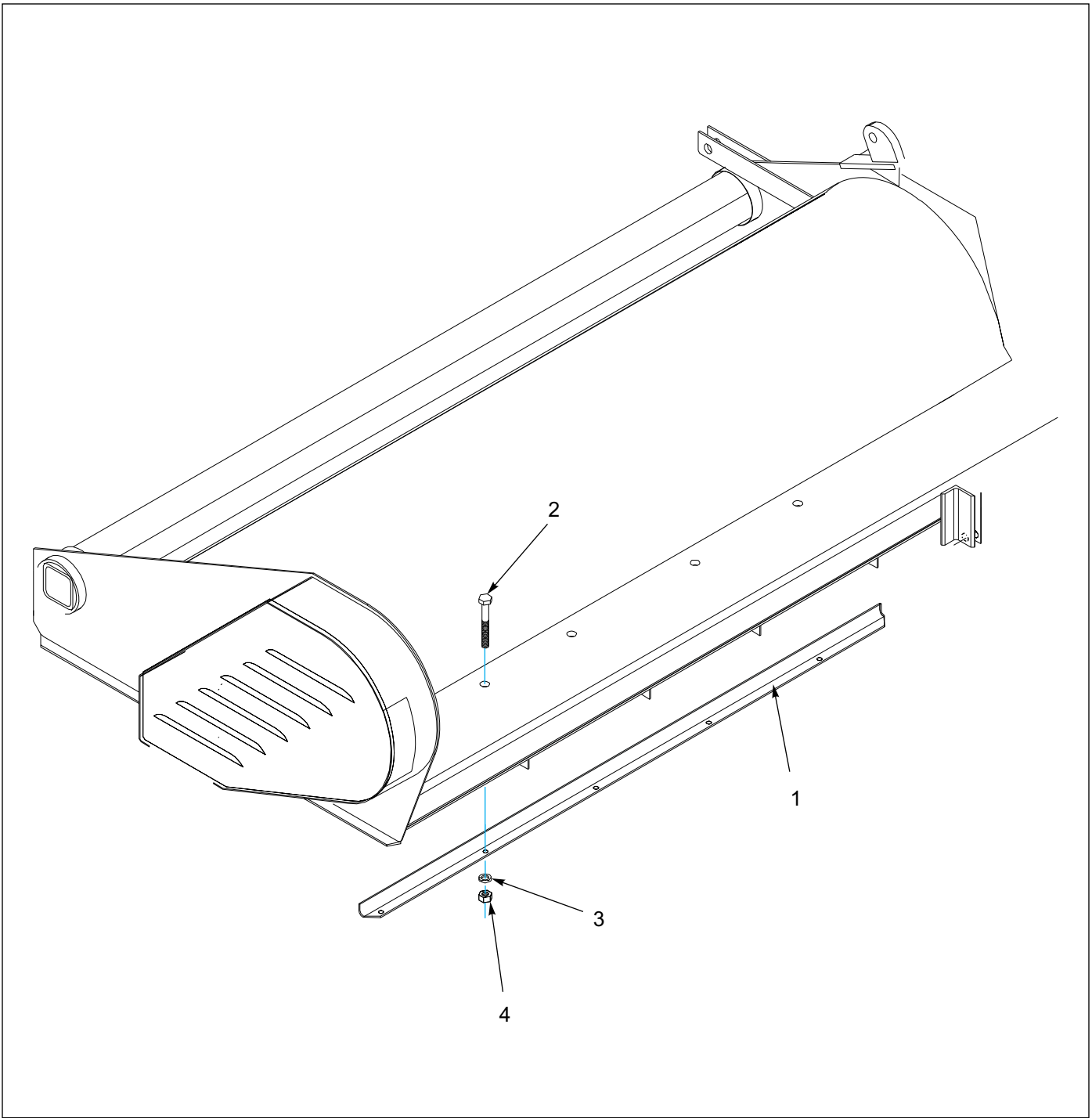
Figure 1-4: Wear Plate - 01/25/2008 and Prior
