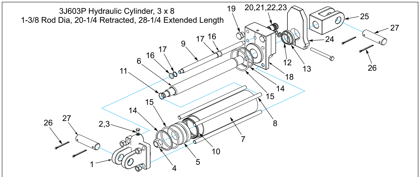
Figure 1-30: Hydraulic Cylinder, 3" X 8 - Prince
