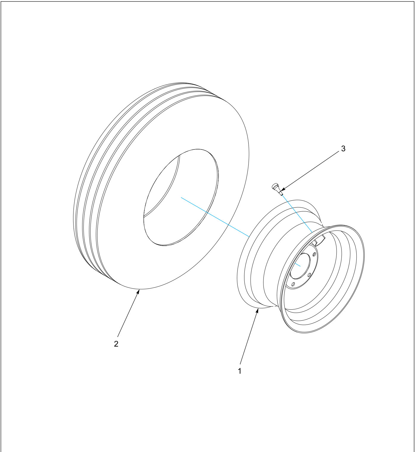
Figure 1-25: Wheel and Tire Assembly
