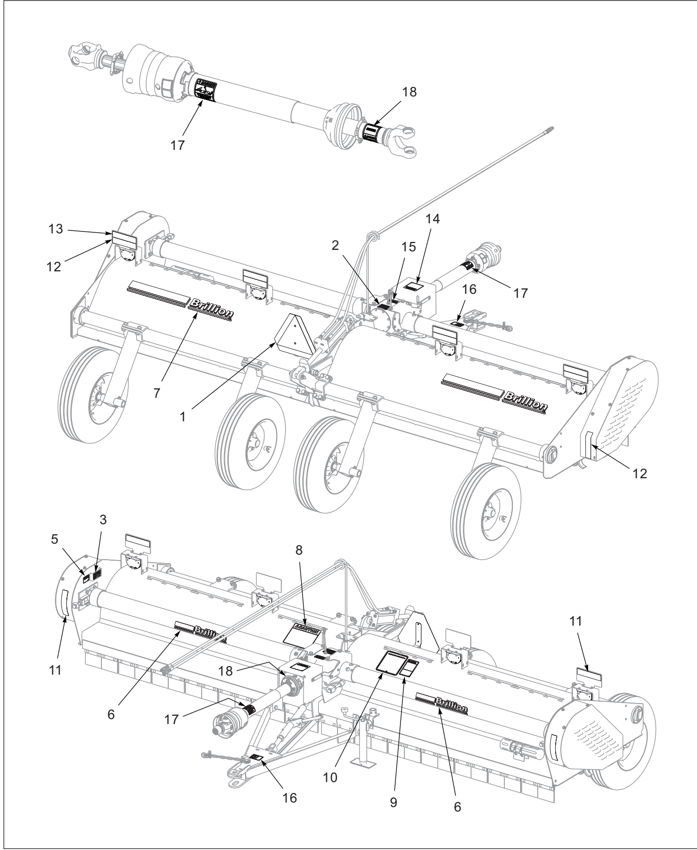
Figure 1-31: Decal Locations
