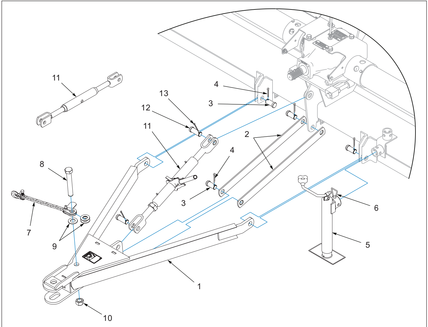
Figure 1-4: Drawbar
