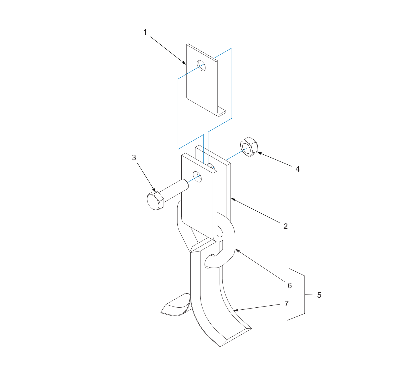
Figure 1-12: Knife Assembly, Slice
