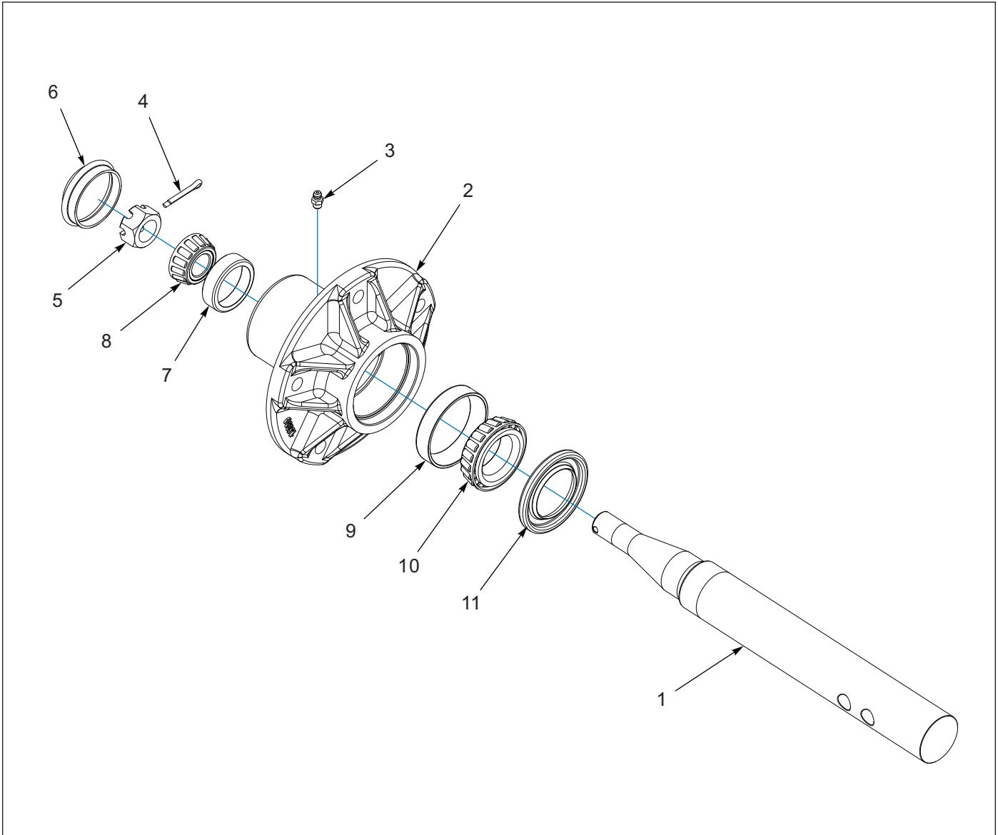
Figure 1-16: Hub and Spindle Assembly
