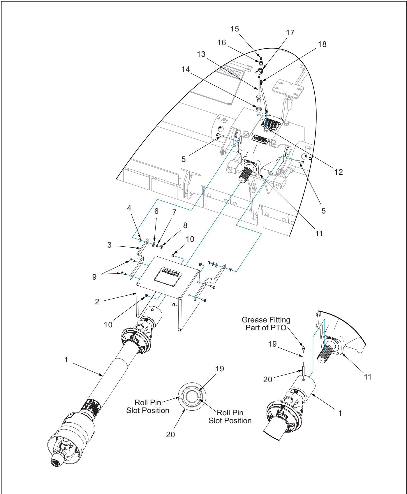
Figure 1-19: PTO Guard
