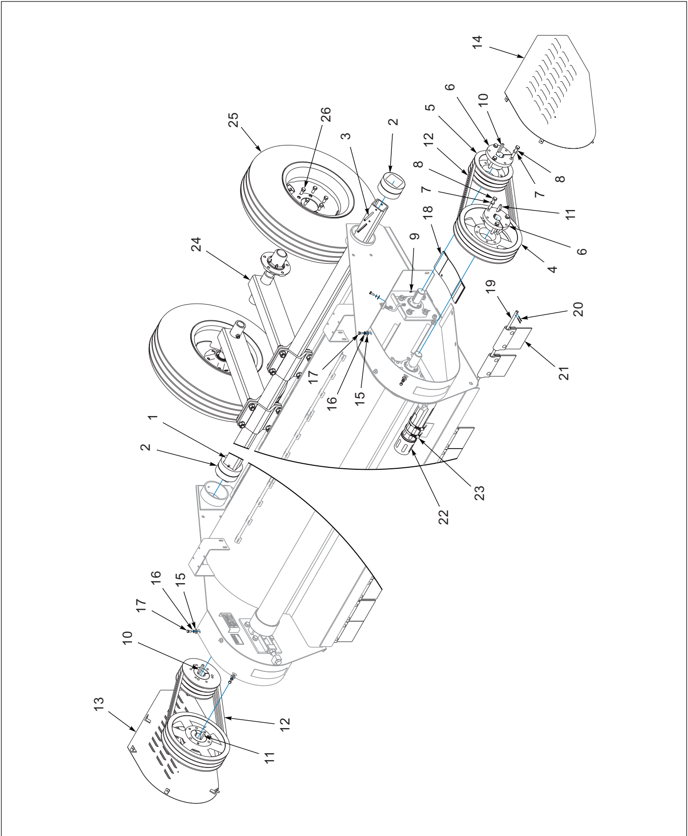
Figure 1-14: Pulley Guards
