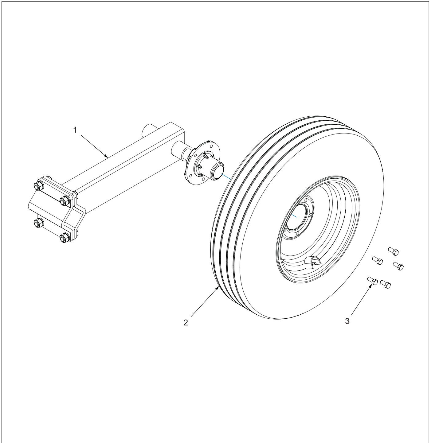
Figure 1-18: Wheel Kit, Auxiliary - Optional
