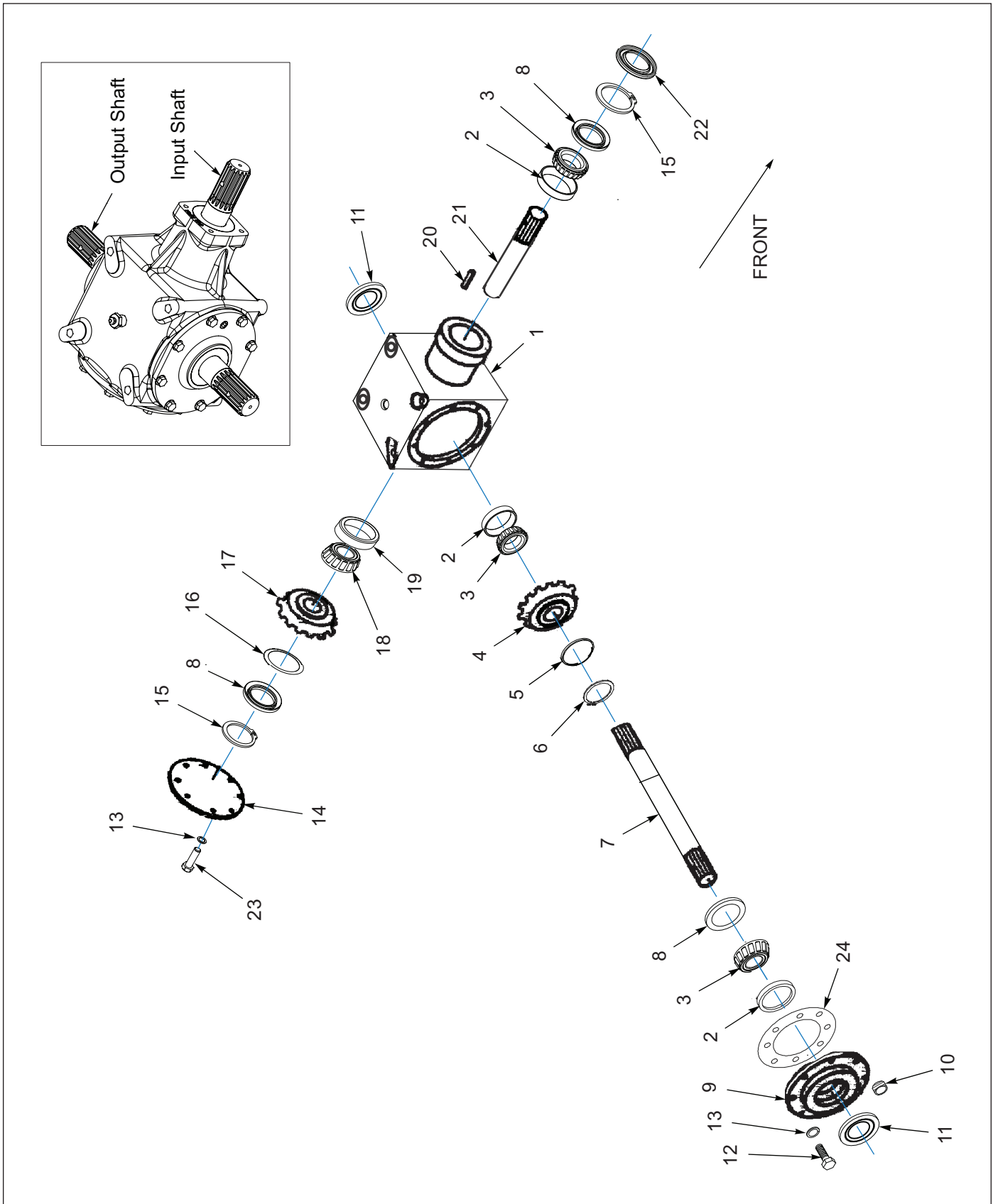
Figure 1-21: Gearbox Assembly, 540 RPM
