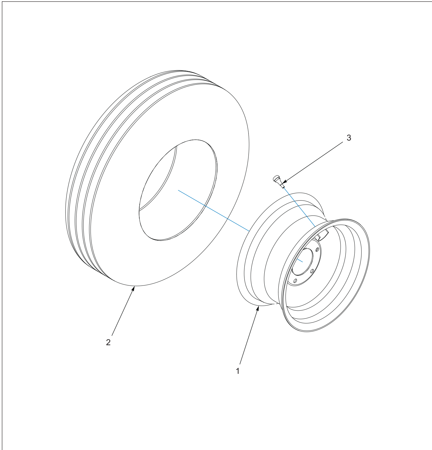
Figure 1-17: Wheel and Tire Assembly
