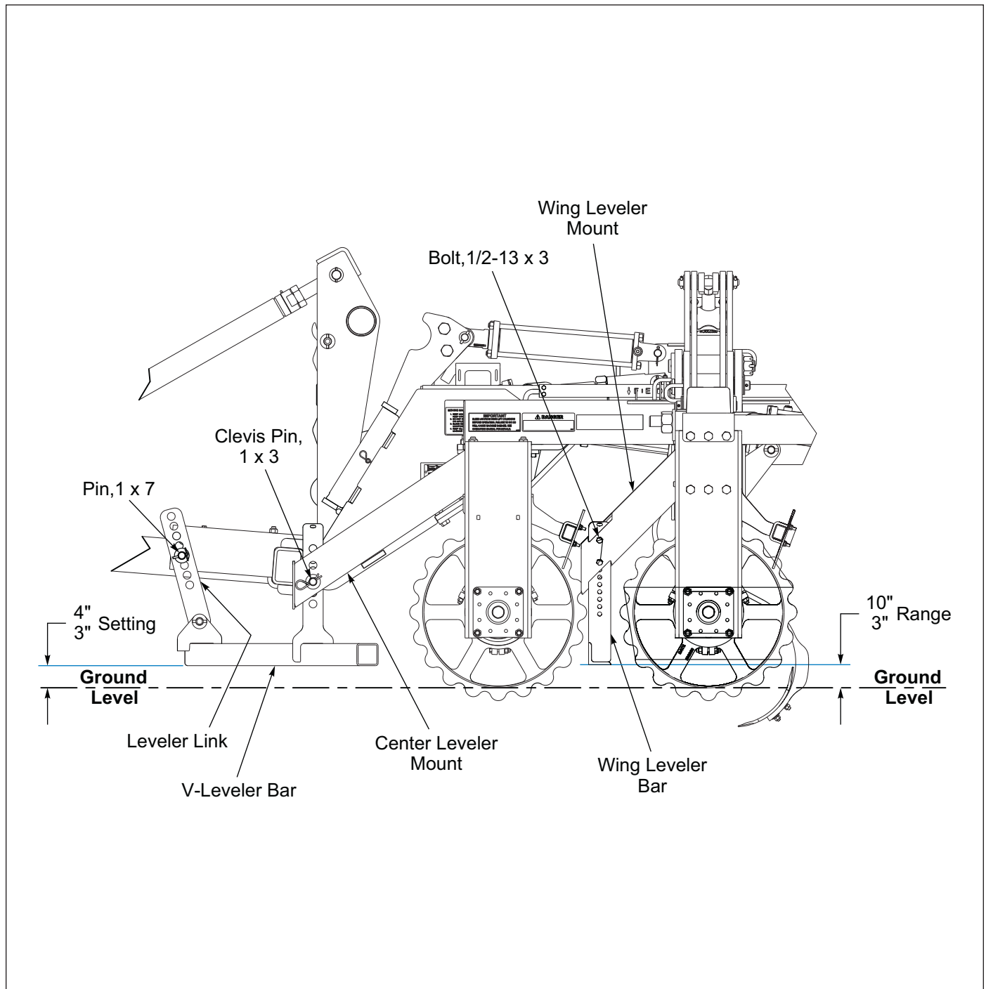
Figure 3-9: V-Leveler Adjustment
