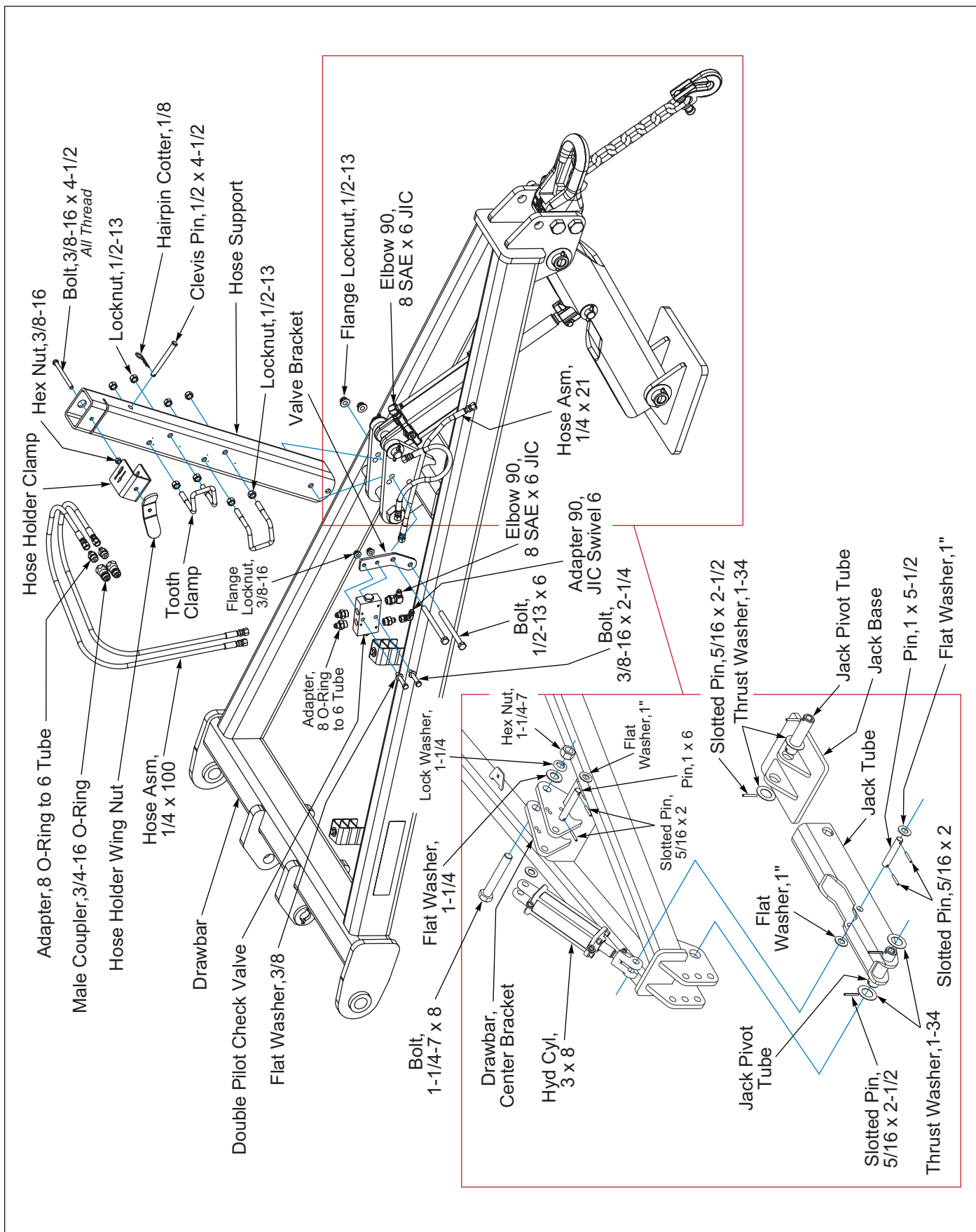
Figure 2-11: Drawbar w/ Hydraulic Jack Installation
