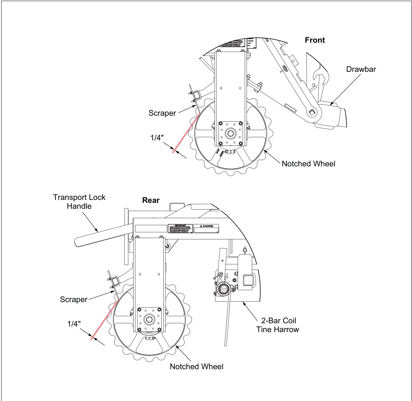
Figure 3-10: Scraper Adjustment
