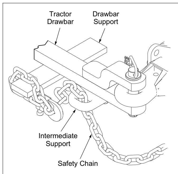
Figure 3-12: Safety Chain
