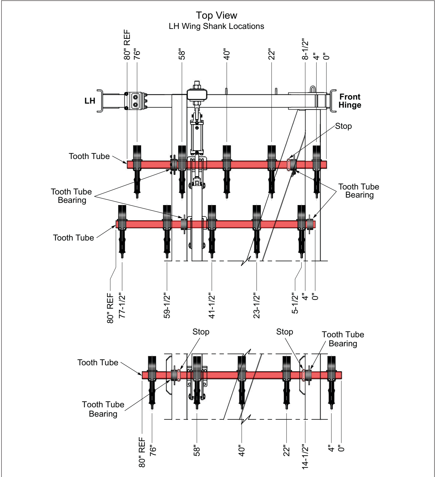
Figure 2-53: Left Hand Wing Shank Mounting Dimensions
