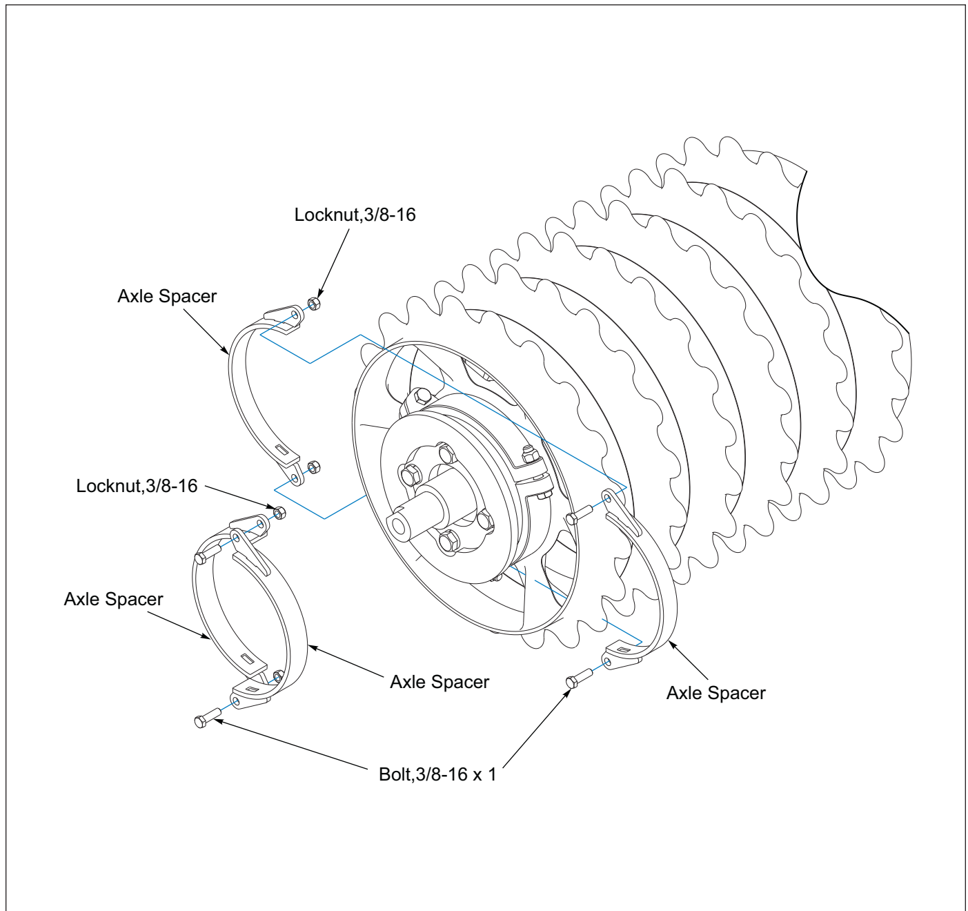
Figure 4-6: Clamp End Spacer Kit - Optional (2 of 2)
