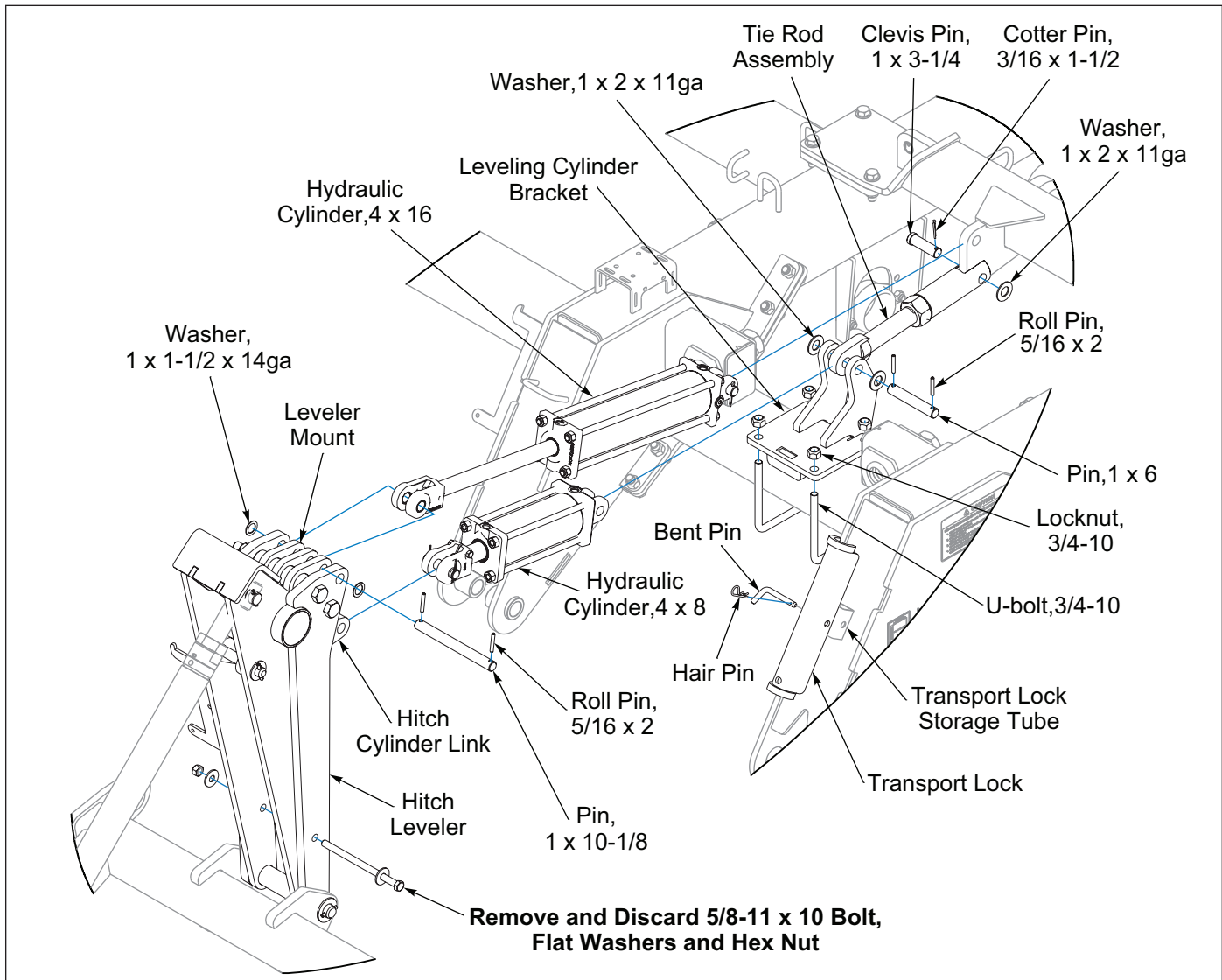
Figure 2-12: Drawbar Leveler
