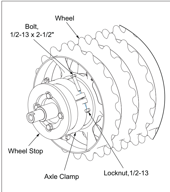
Figure 4-3: Roller Axle Assembly
