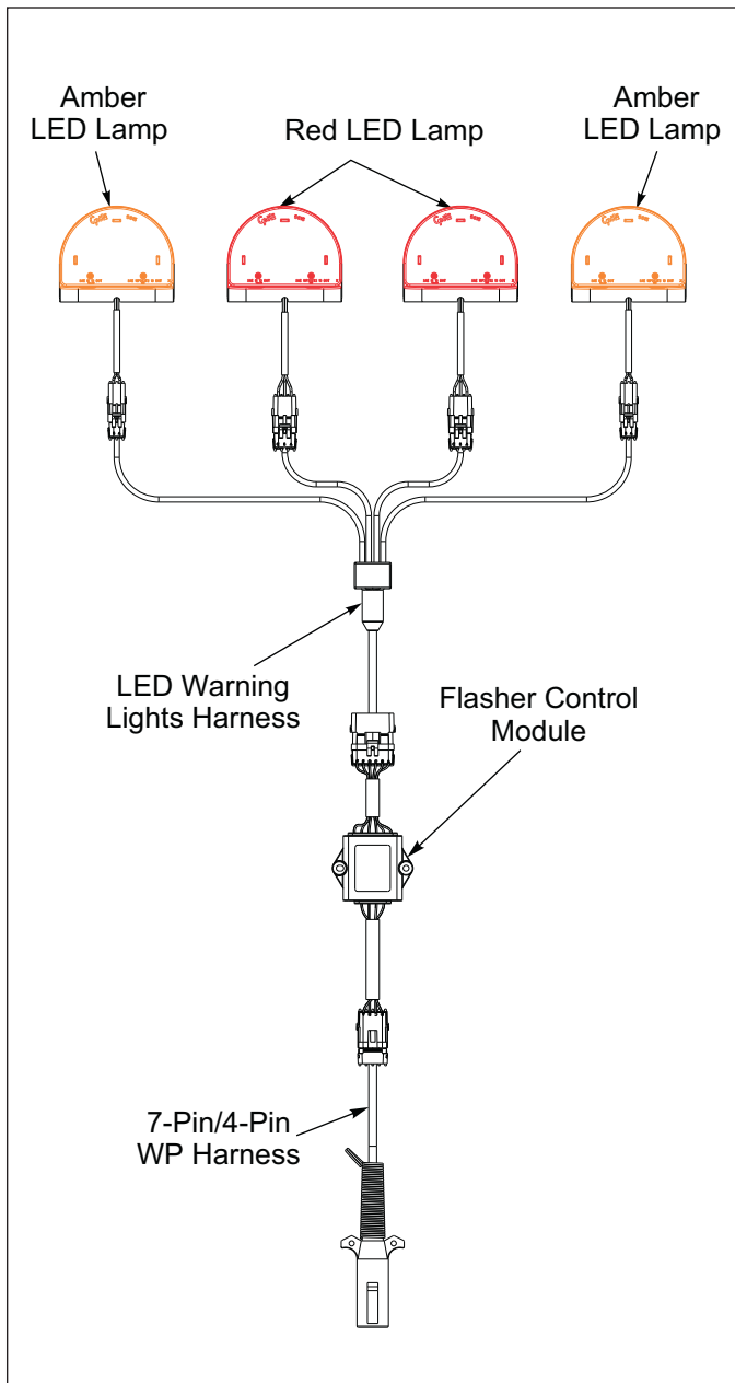
Figure 4-7: LED Warning Lamps
