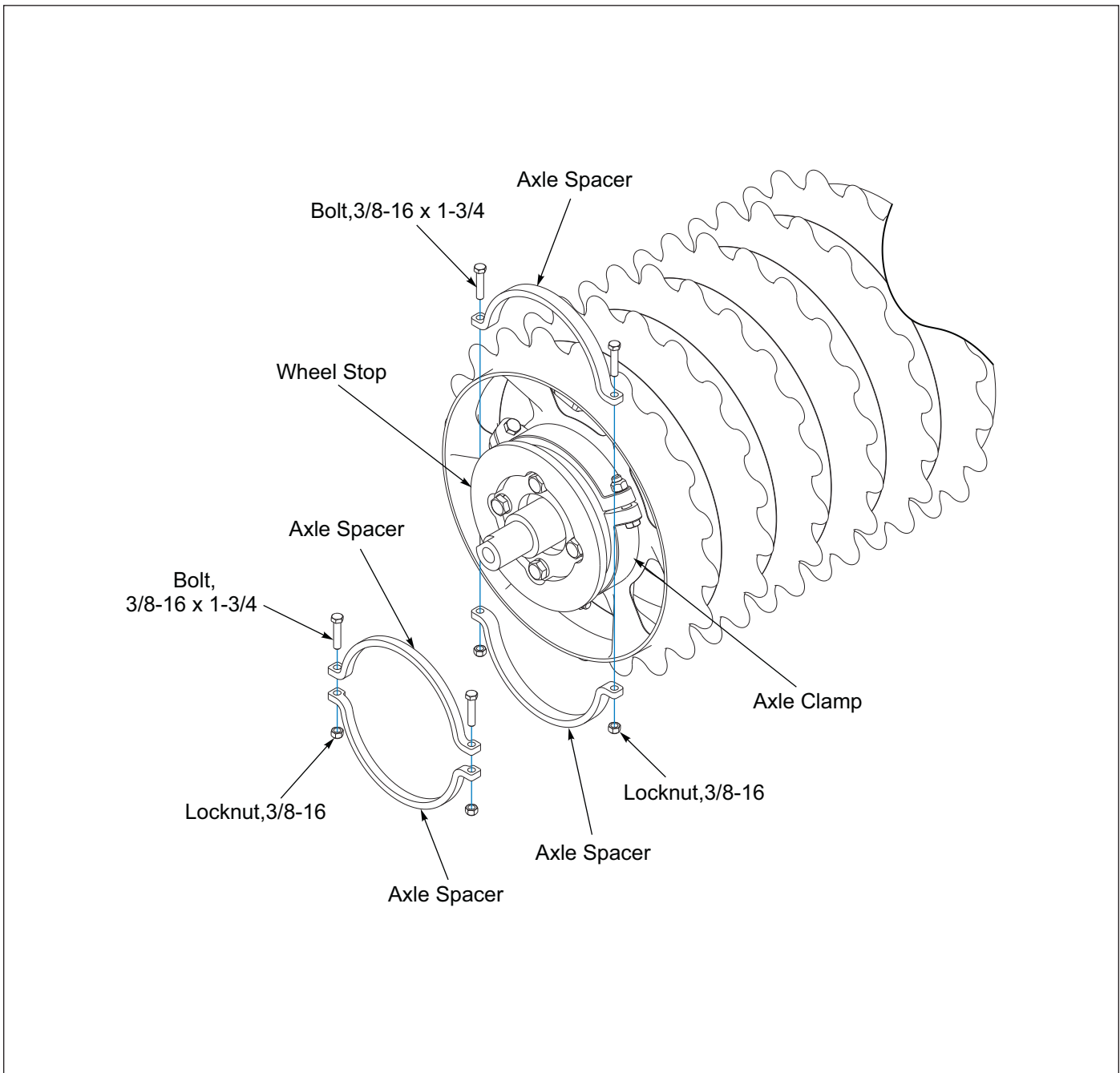
Figure 4-5: Clamp End Spacer Kit - Optional (1 of 2)
