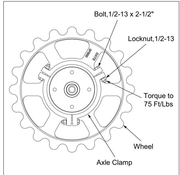
Figure 4-4: Clamp Tightening
