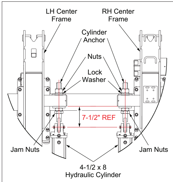
Figure 2-17: Center Frame Distance
