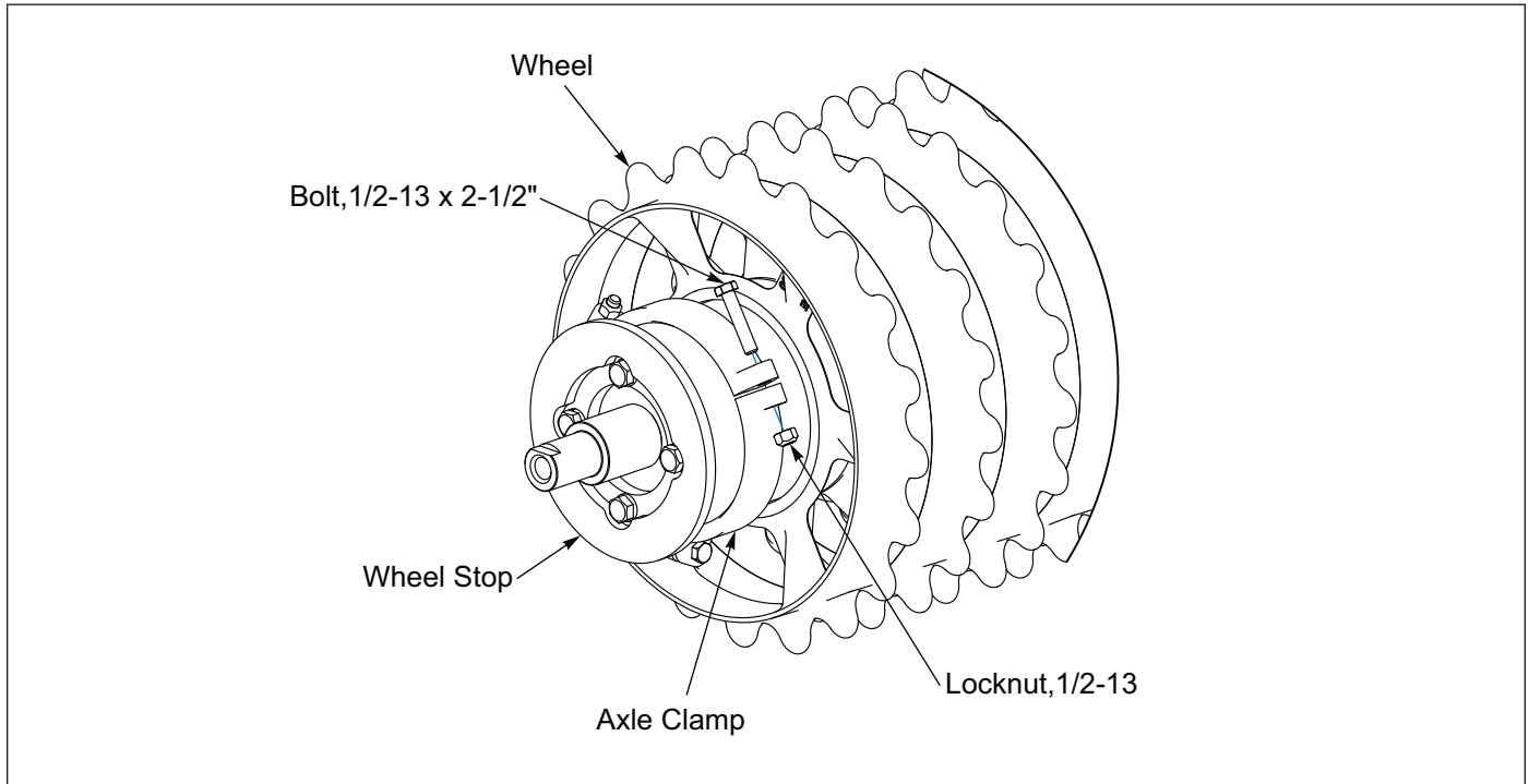
Figure 4-3: Roller Axle Assembly
