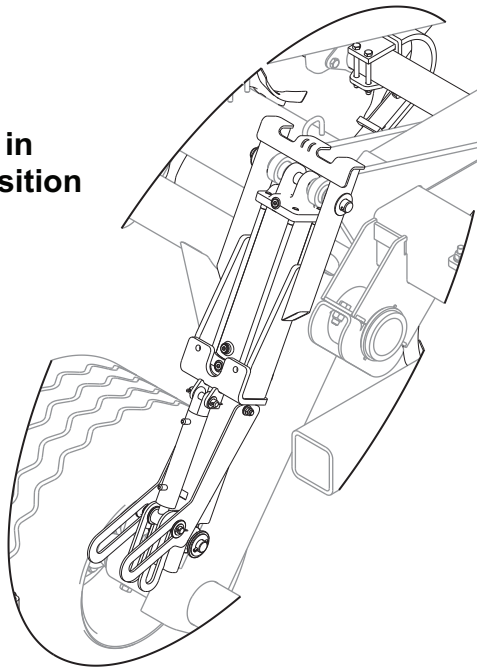
Figure 3-7: Rockshaft Transport Lock Position (Hydraulic/Automatic Locks)
