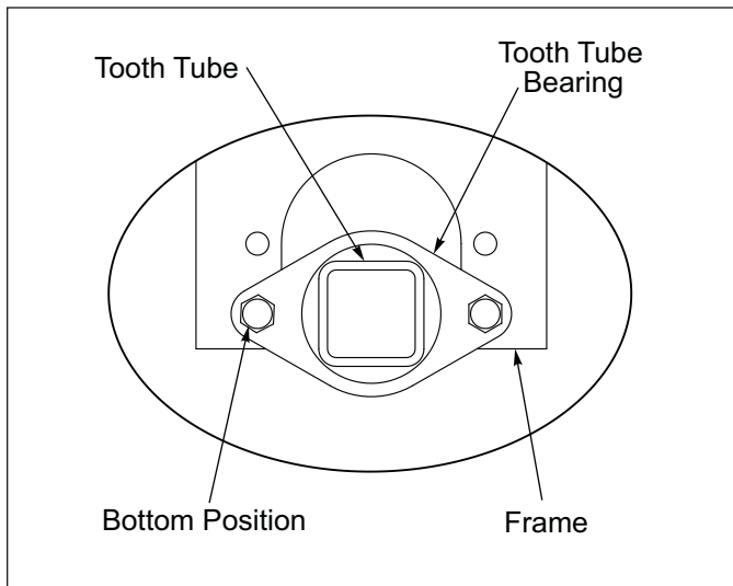
Figure 2-36: Tooth Tube Bearing Position for Roller with 24" Wheels
