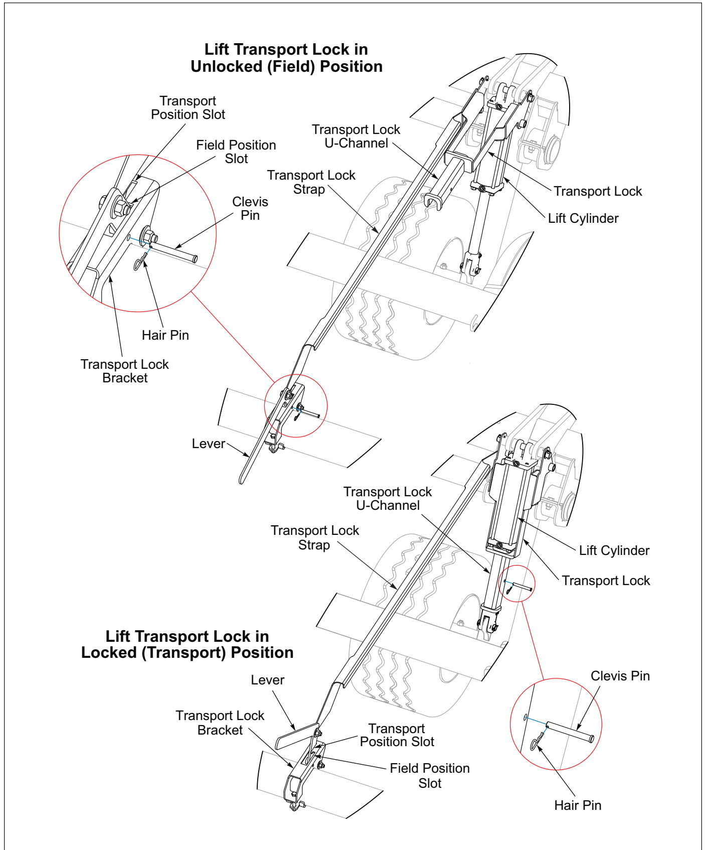
Figure 3-5: Rockshaft Transport Lock Position (Manual Locks)
