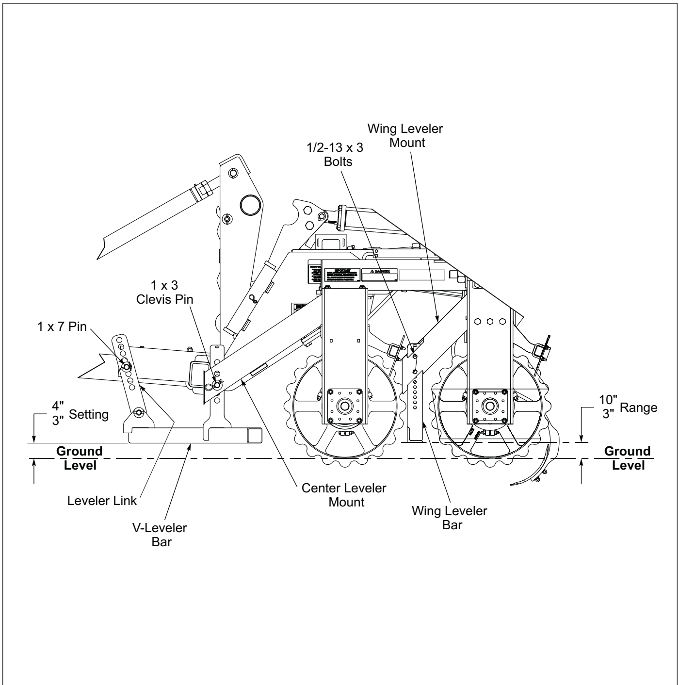
Figure 3-11: V-Leveler Adjustment
