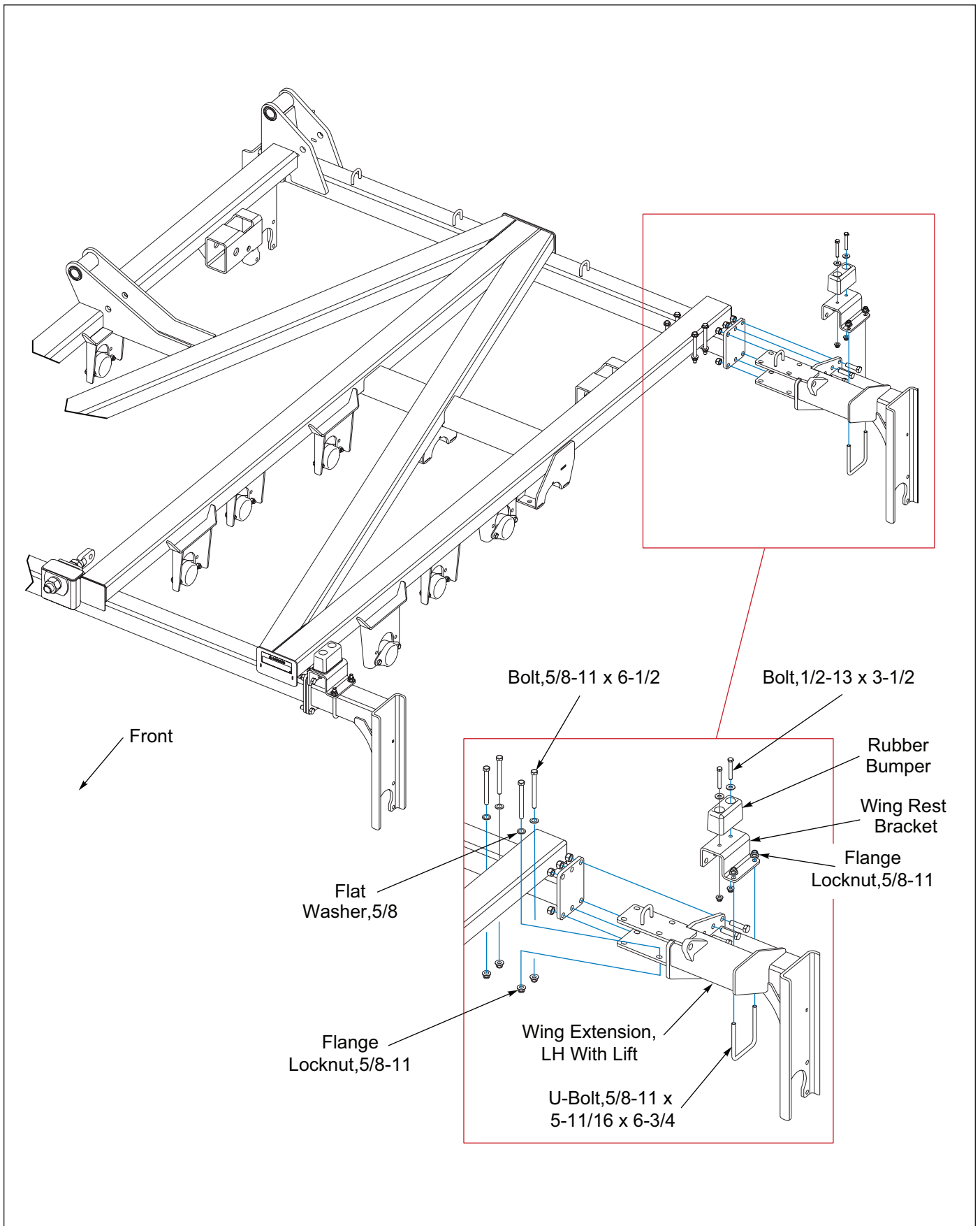
Figure 2-50: Left Right Wing Rest and Bearing Hanger
