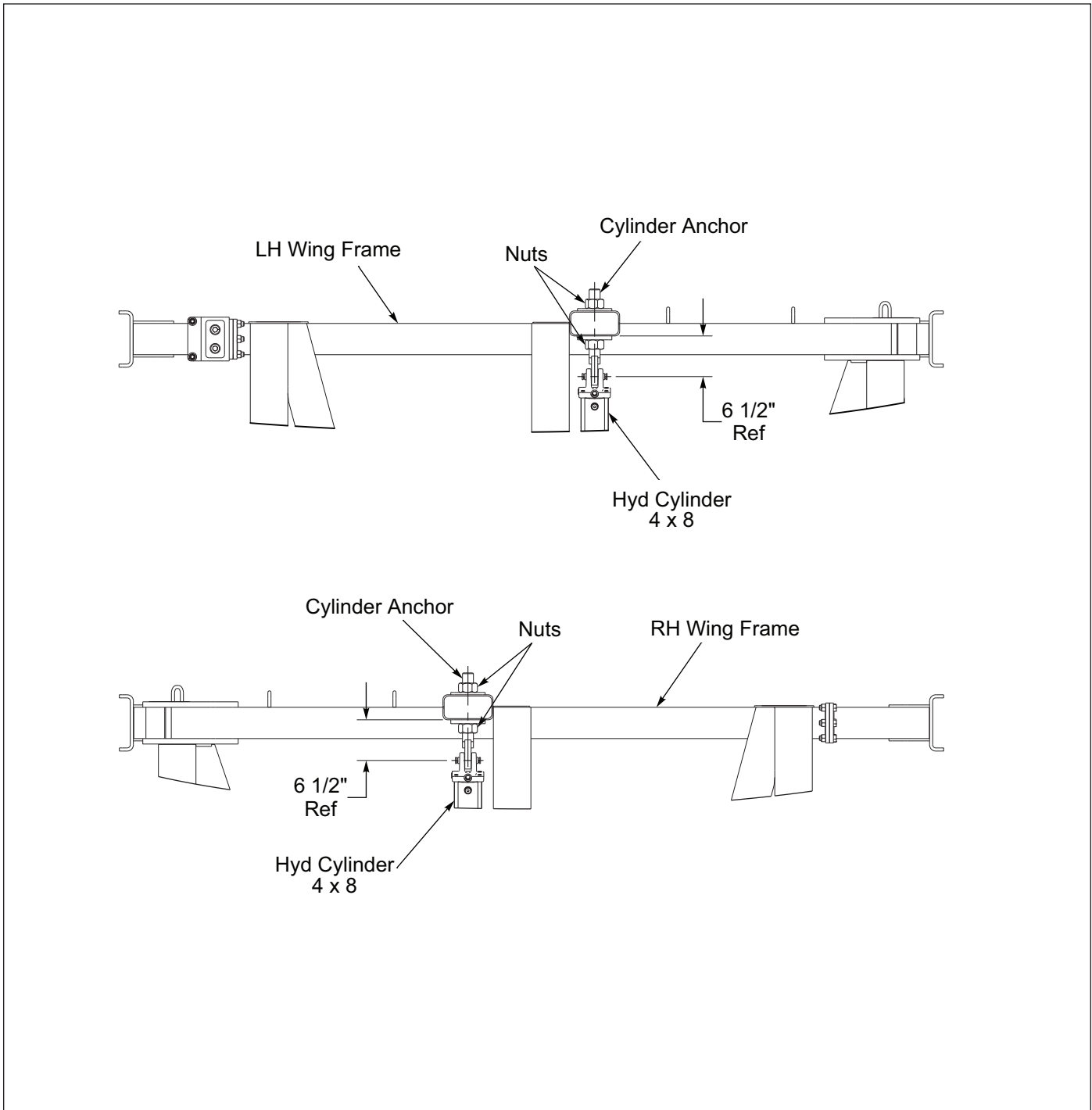
Figure 2-58: Wing Tooth Control Cylinder Installation
