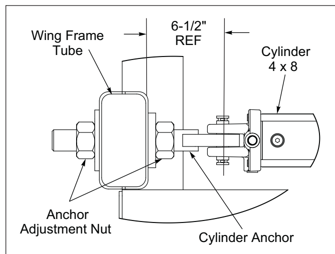
Figure 3-3: Wing Frame Hyd Cyl Spacing
