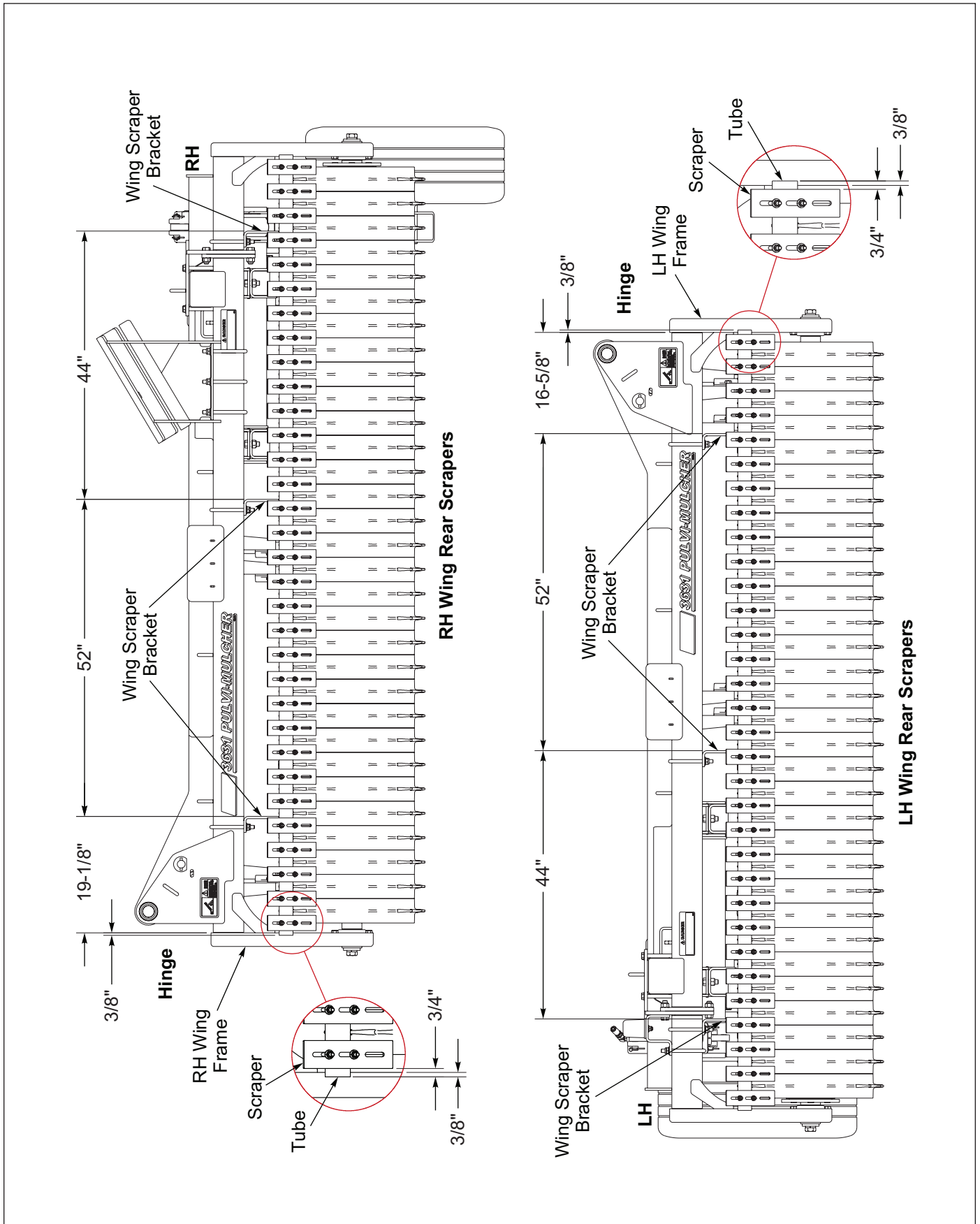
Figure 2-77: Wing Rear Scraper Mounting Dimensions
