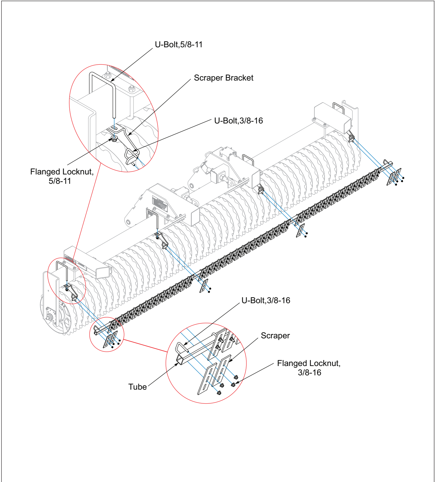
Figure 2-78: Center Front Scrapers Installation - Optional
