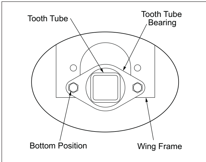
Figure 2-59: Wing Tooth Tube Bearing Position for Roller with 24" Wheels
