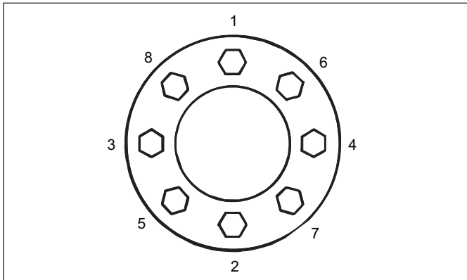
Figure 4-1: Stud Tightening Sequence
