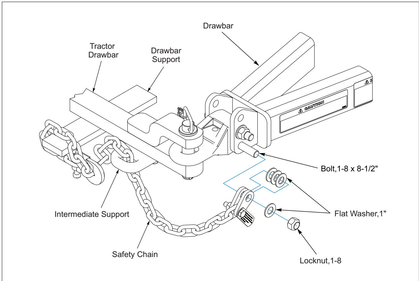
Figure 1-2: Safety Chain
