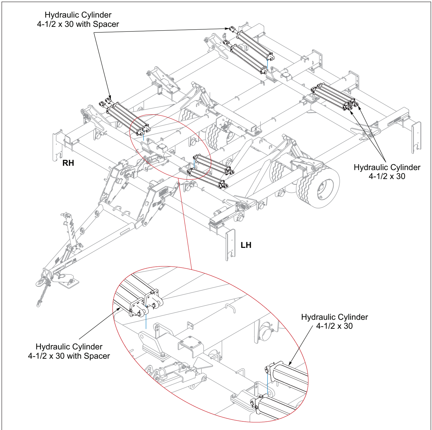
Figure 2-16: Wing Fold Hydraulic Cylinder Installation
