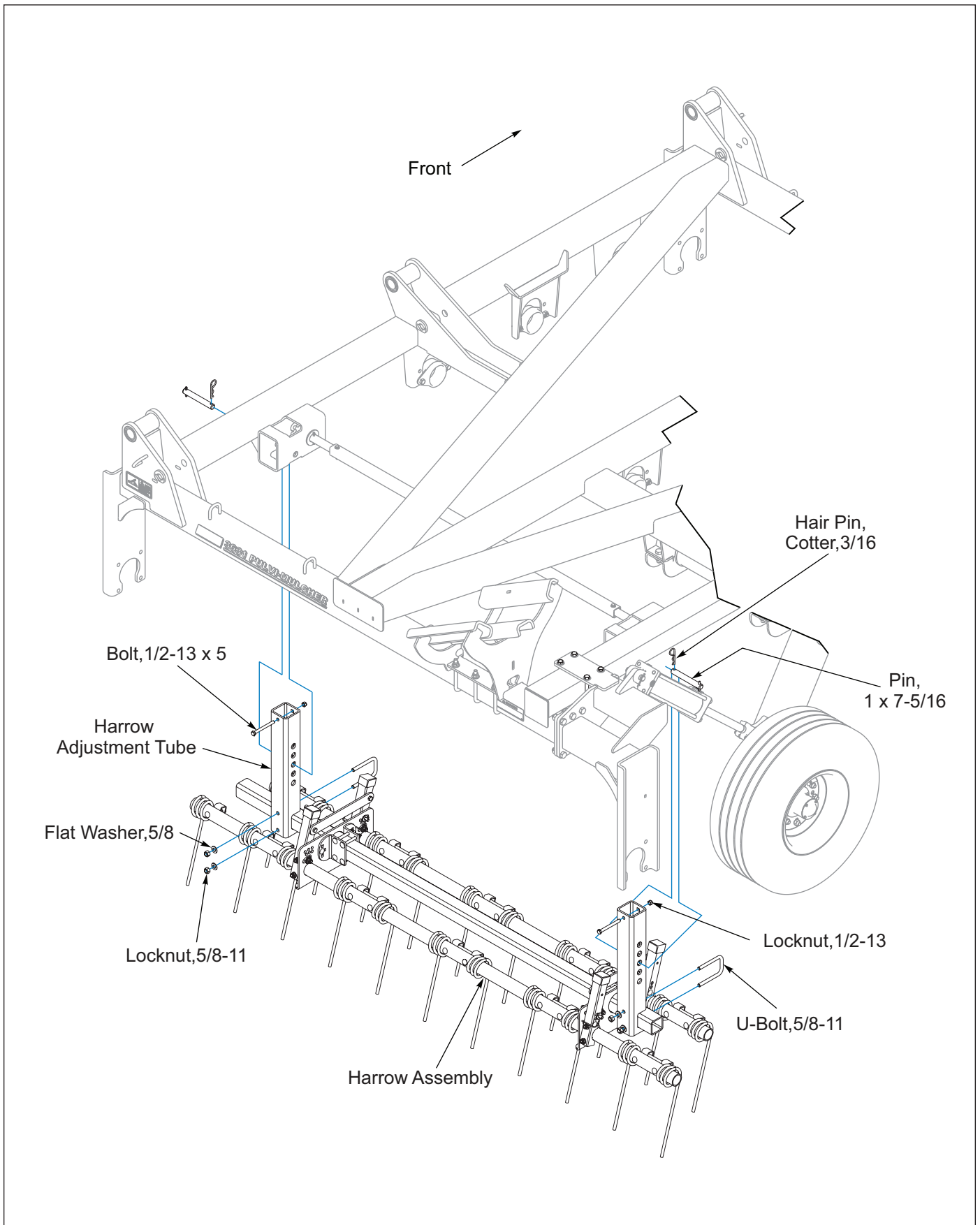
Figure 2-70: Right Hand Wing Harrow
