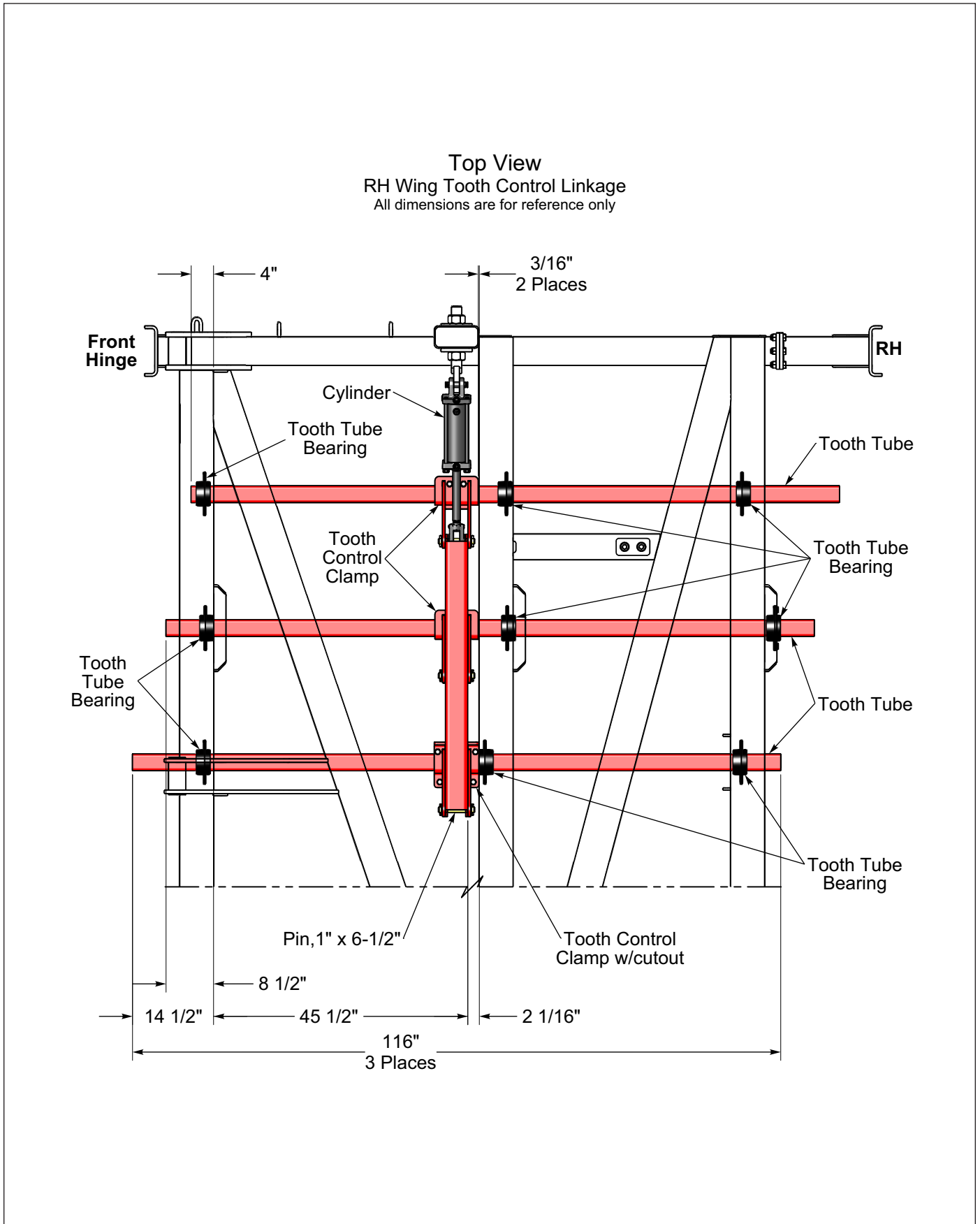
Figure 2-64: Right Hand Wing Tooth Control Linkage
