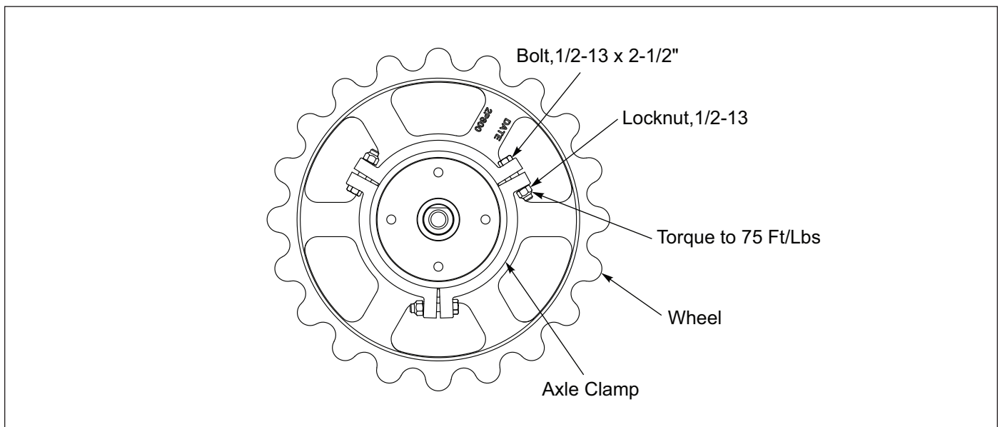
Figure 4-4: Clamp Tightening
