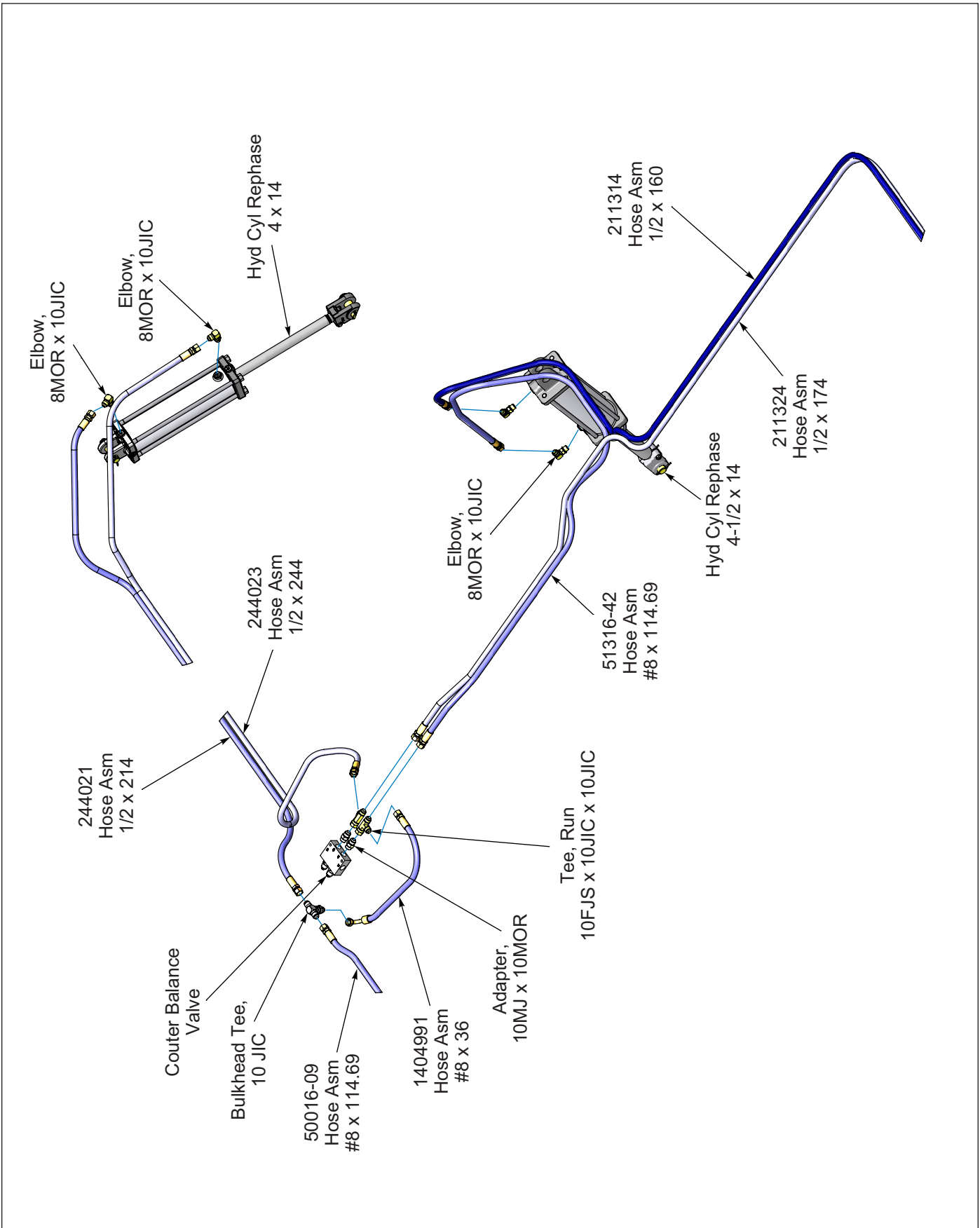
Figure 2-31: Hydraulic Lift Schematic (Series Cylinders w/ Wing Lift Wheels) (LH)
