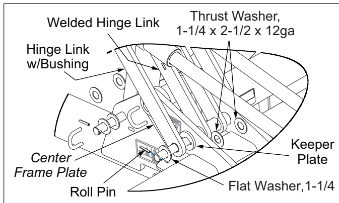
Figure 2-51: Center Frame Hinge Assembly
