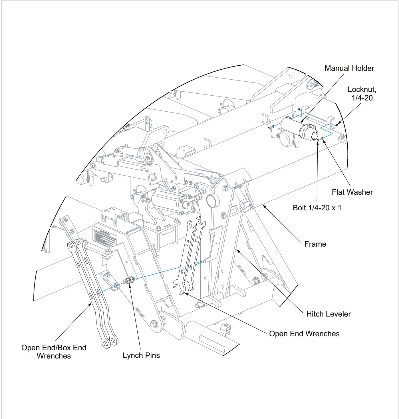
Figure 2-15: Manual Holder and Wrenches
