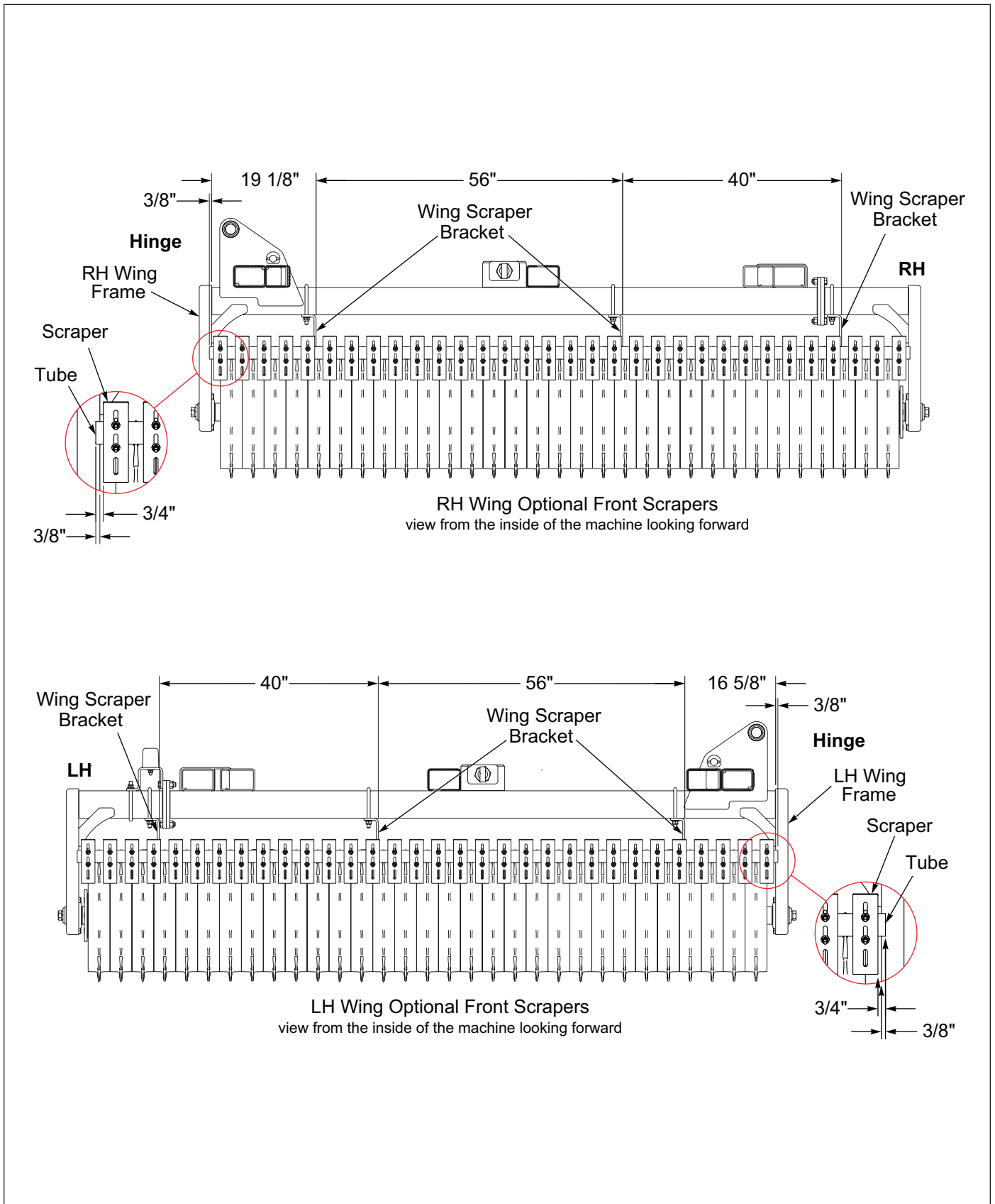
Figure 2-81: Wing Front Scraper Mounting Dimensions
