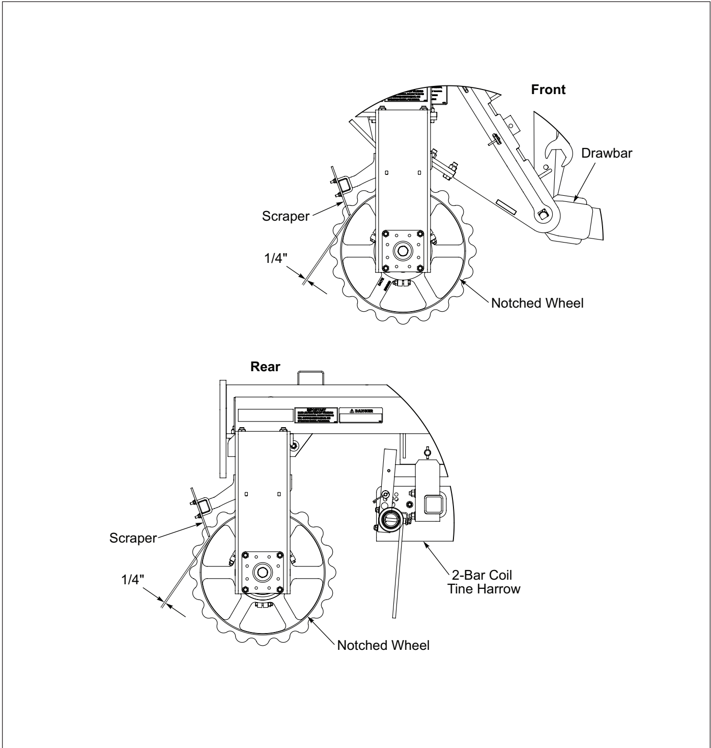
Figure 3-12: Scraper Adjustment
