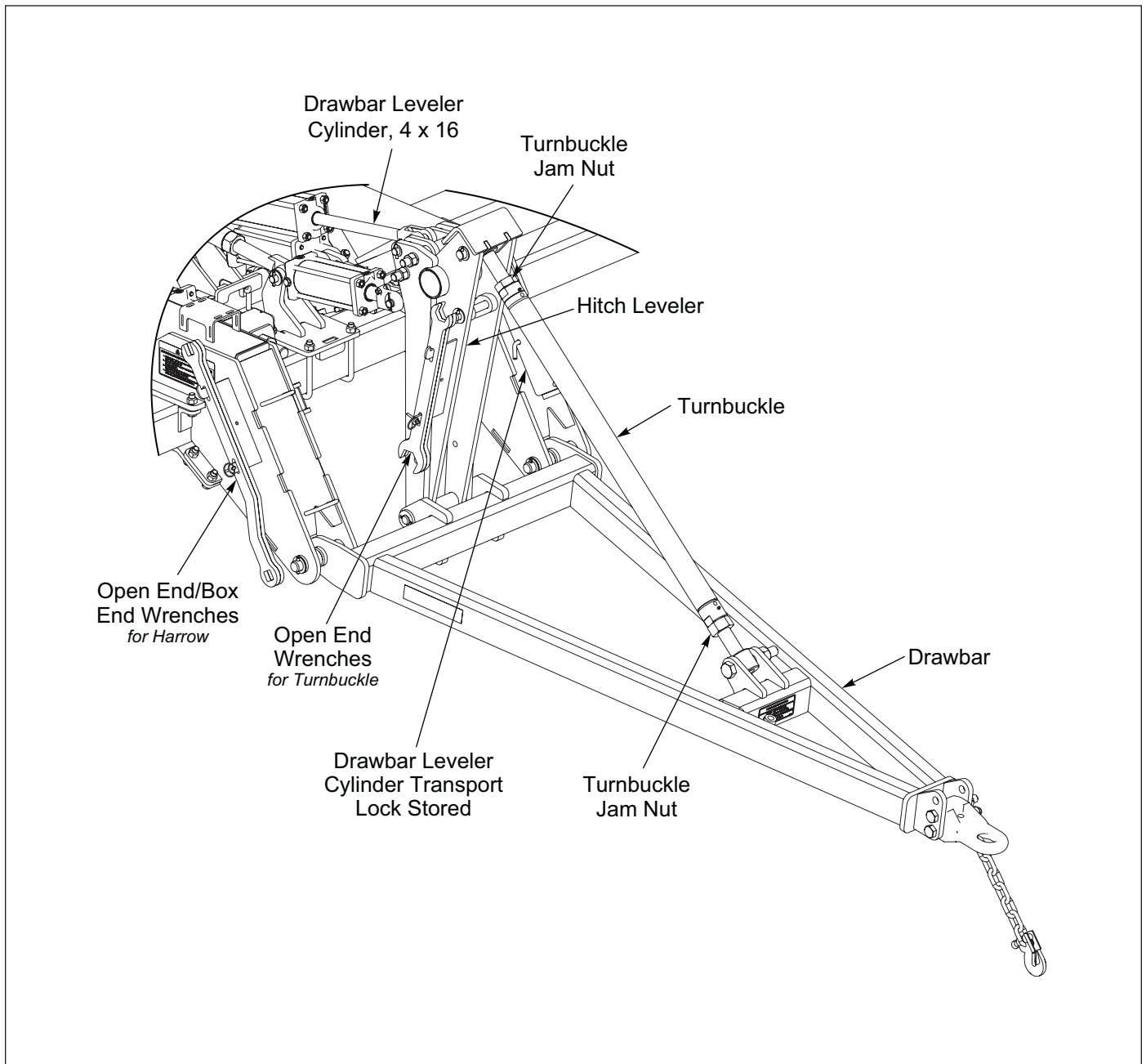
Figure 3-9: Drawbar Turnbuckle Adjustment
