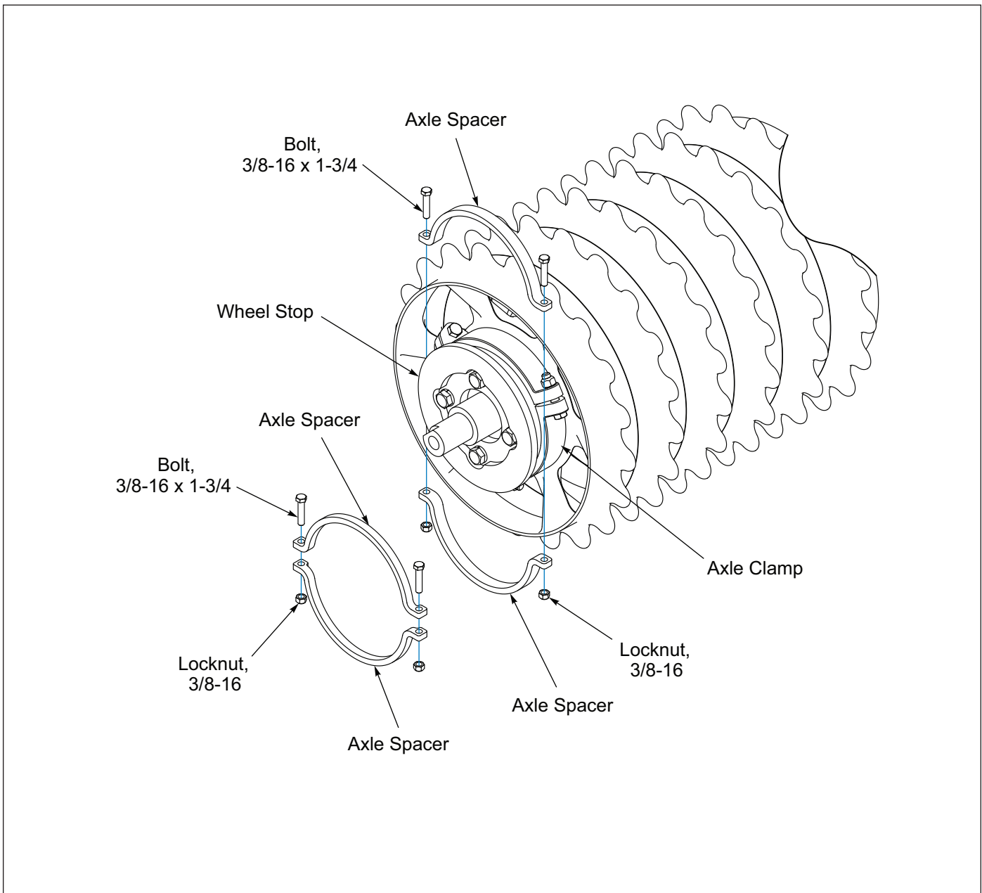
Figure 4-5: Clamp End Spacer Kit 1 of 2 - Optional
