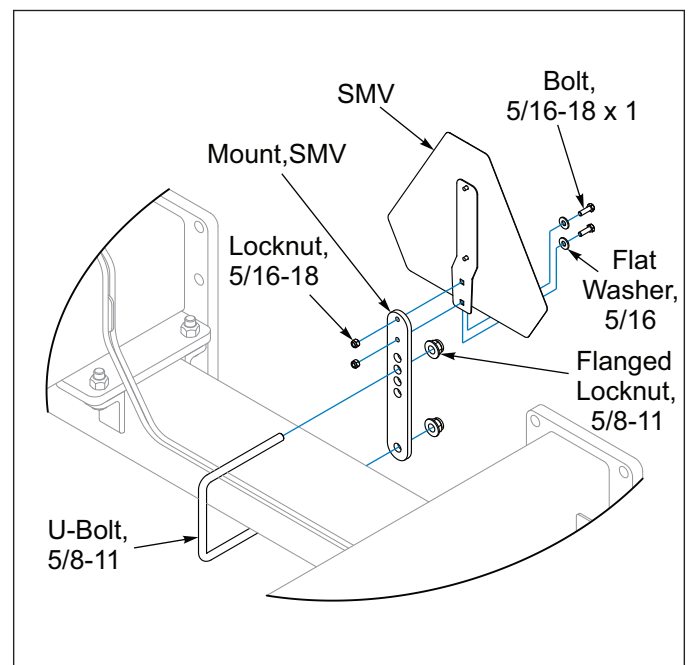
Figure 2-46: SMV Sign Installation
