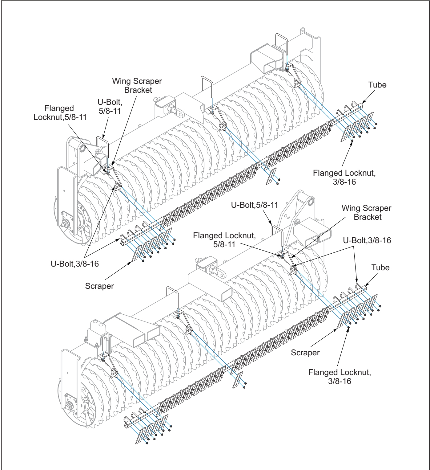
Figure 2-80: Wing Front Scraper Installation - Optional
