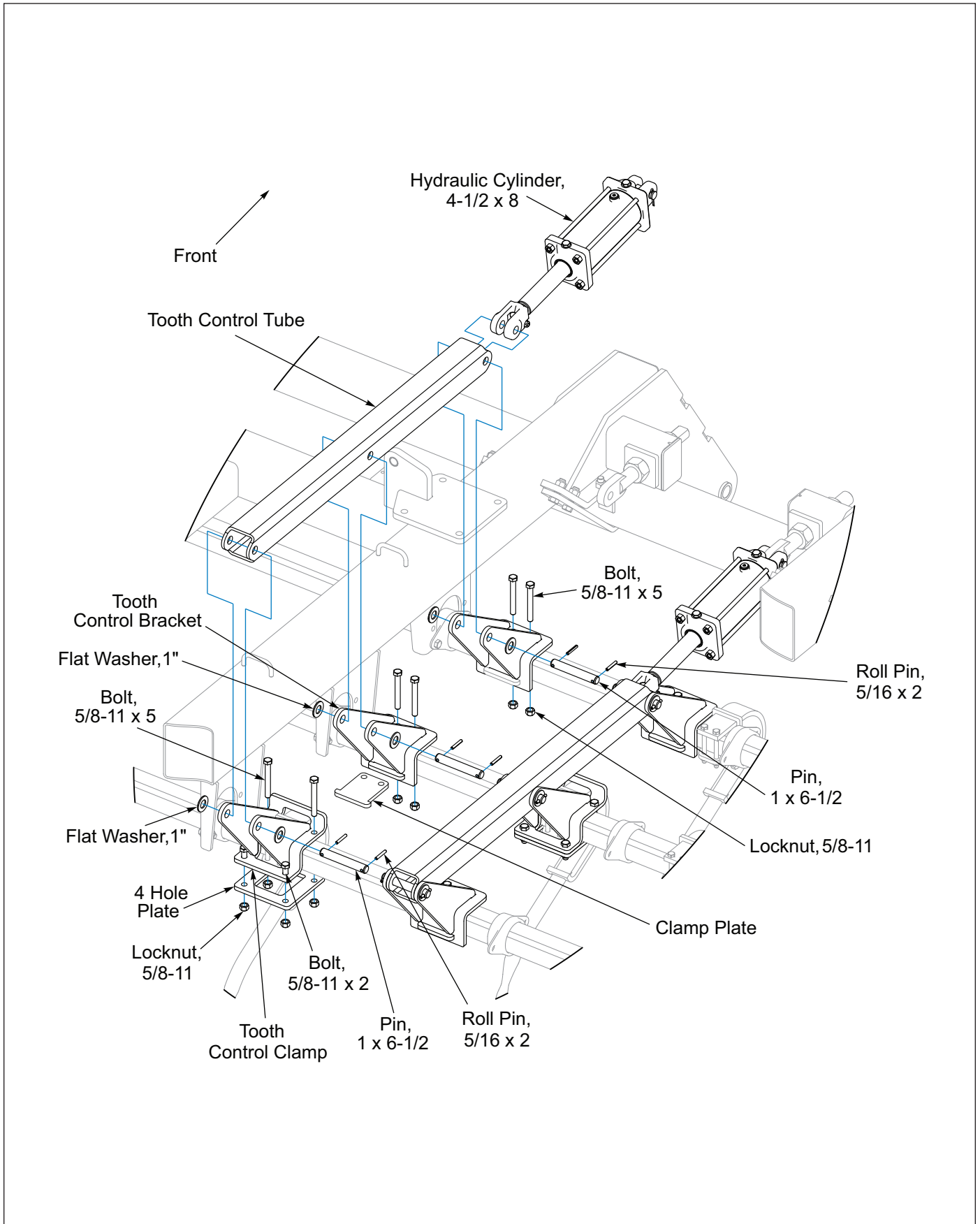
Figure 2-39: Center Frame Tooth Control Linkage
