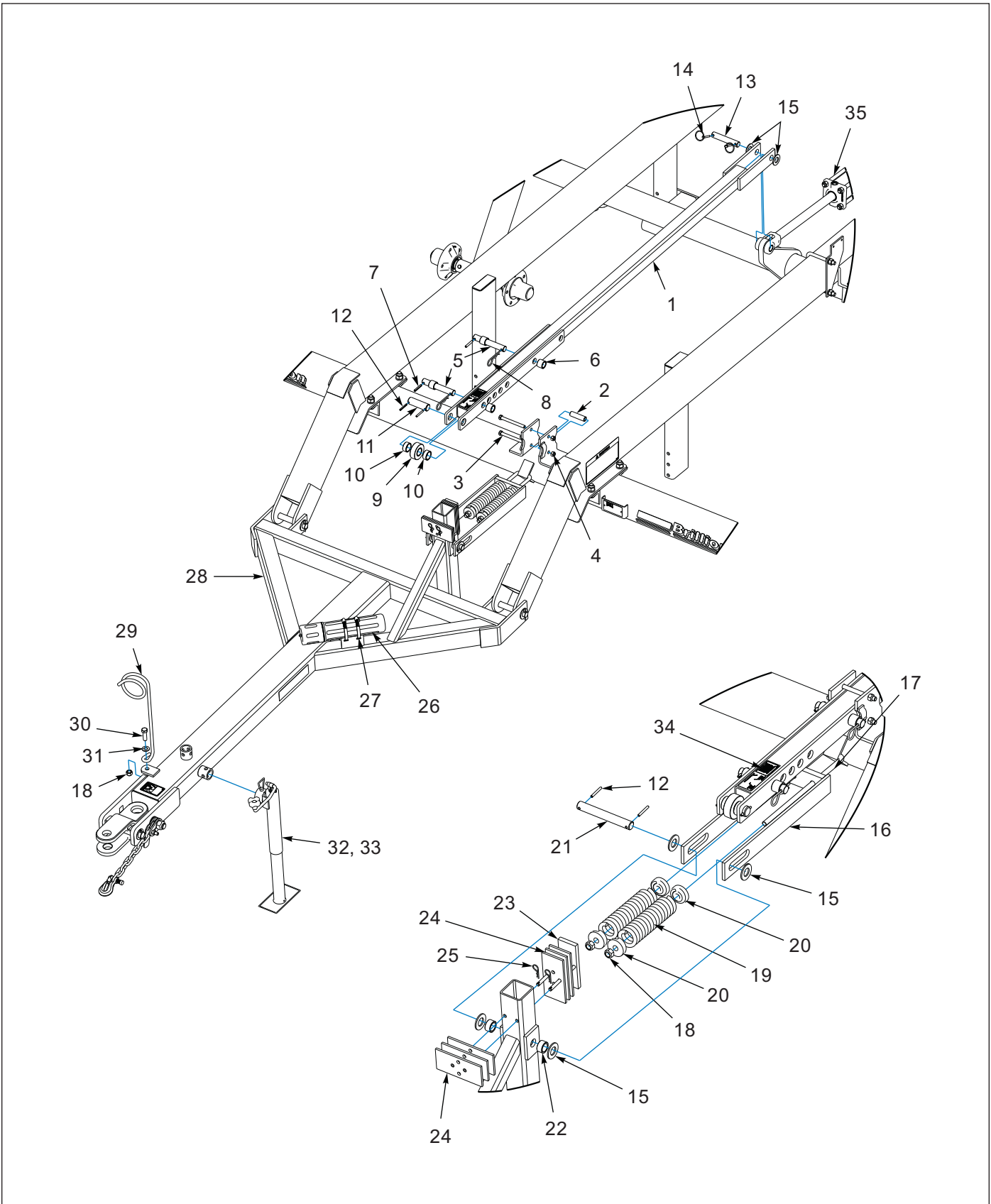
Figure 1-4: Drawbar (Before 07/2016)
