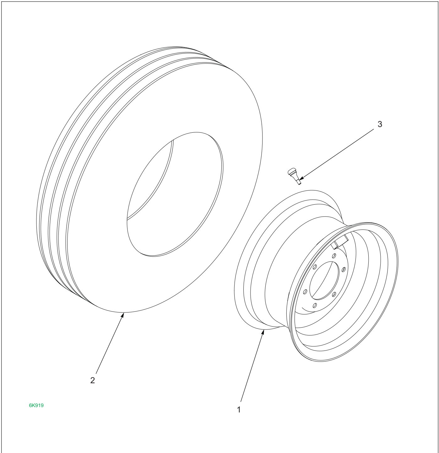
Figure 1-9: Wheel Assembly
