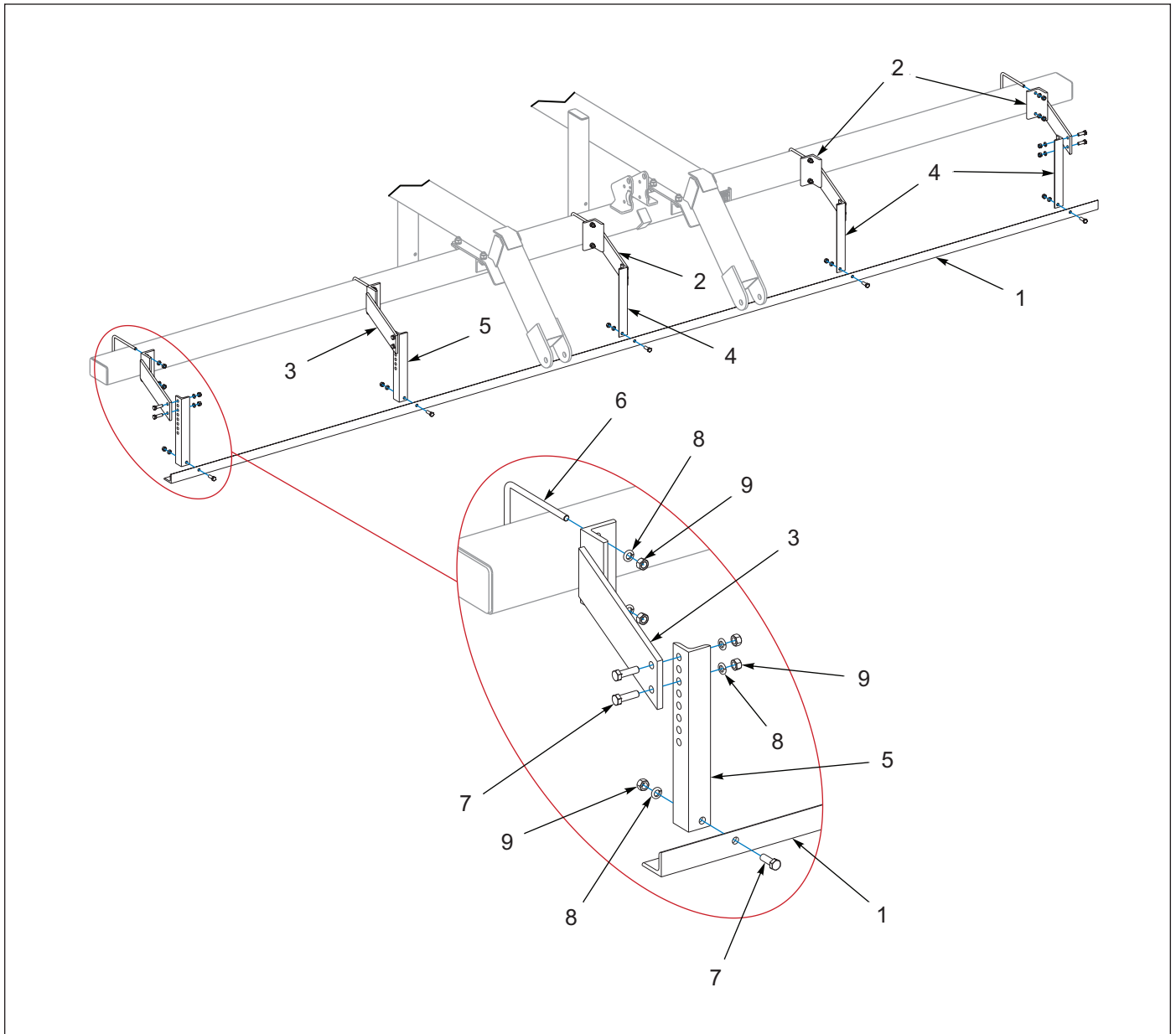
Figure 1-33: Land Leveler Kit - Optional
