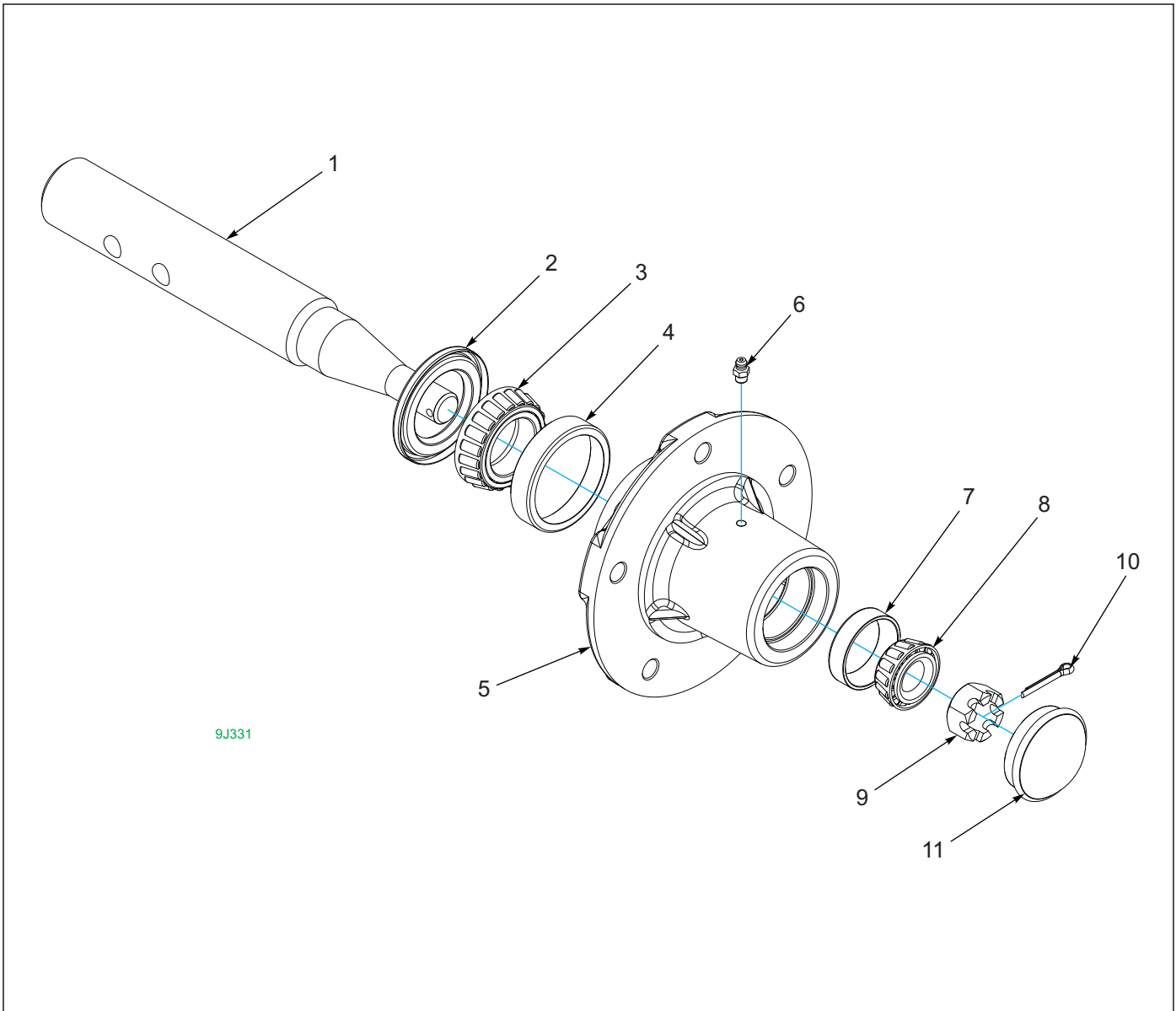
Figure 1-3: Hub and Spindle
