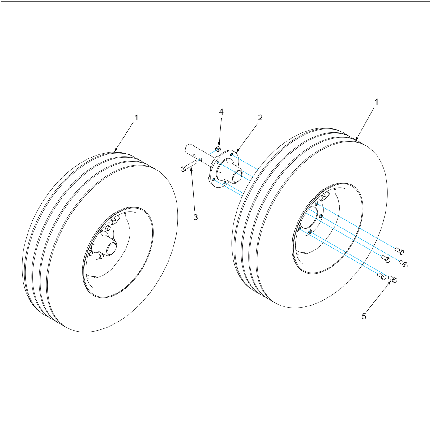
Figure 1-5: Dual Wheel Kit - Optional
