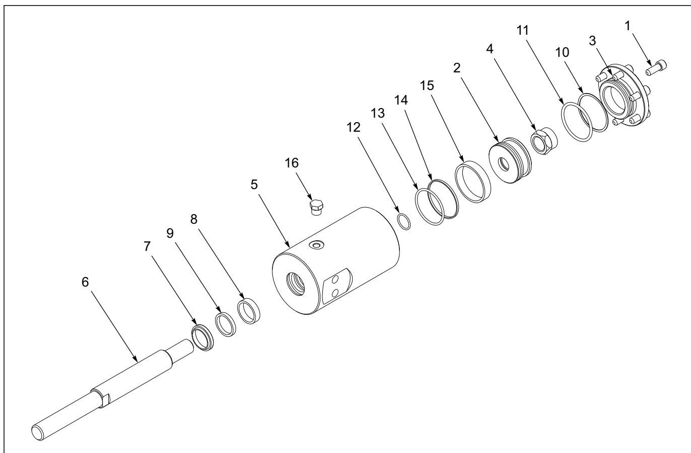
Figure 1-37: Cylinder 2-1/2" X 2-1/2"
