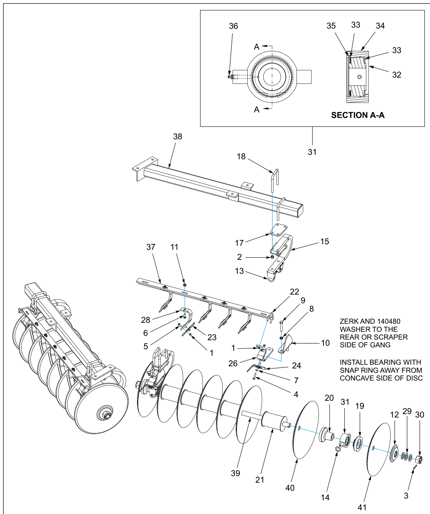
Figure 1-13: Disc Gang Assembly 22", 24" & 26" (8-3/4" Spacing)
