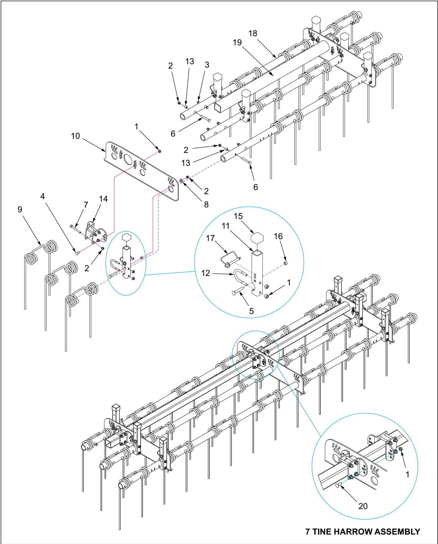
Figure 1-26: Harrow Center Assembly
