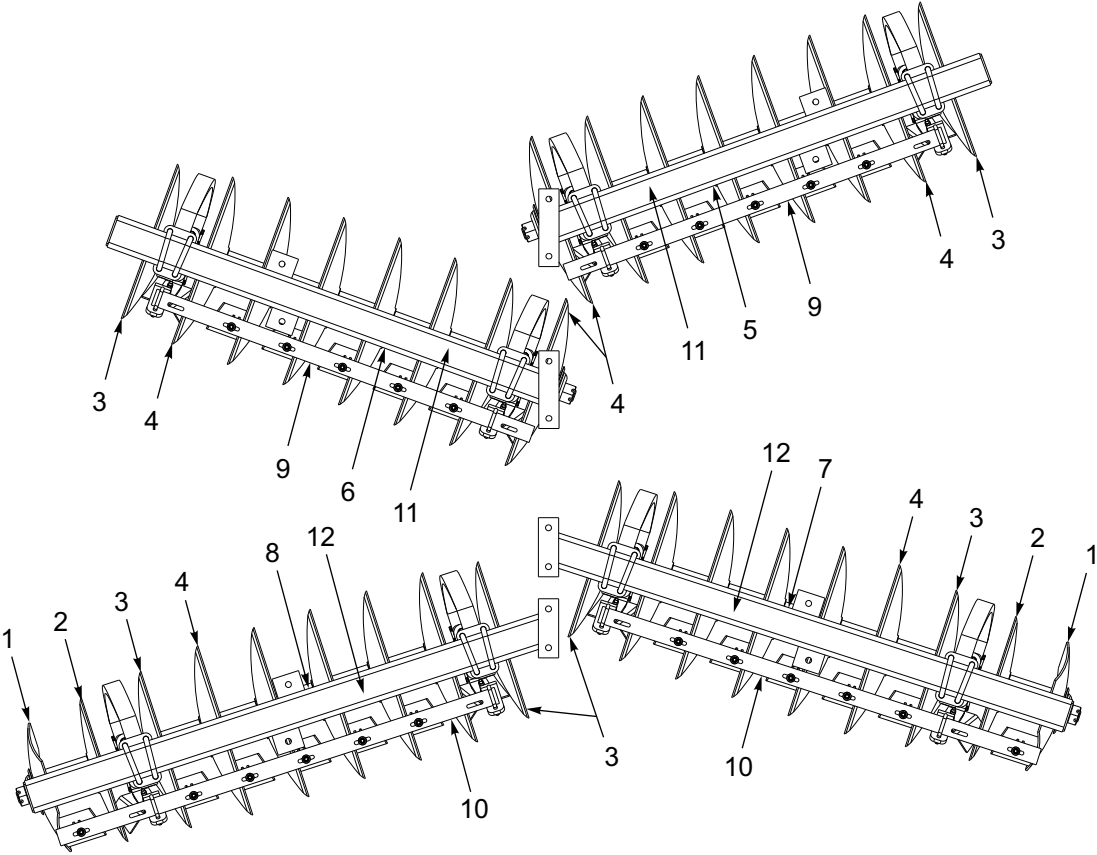
6211-12 26" 4GA DISC BLADES (201794)
