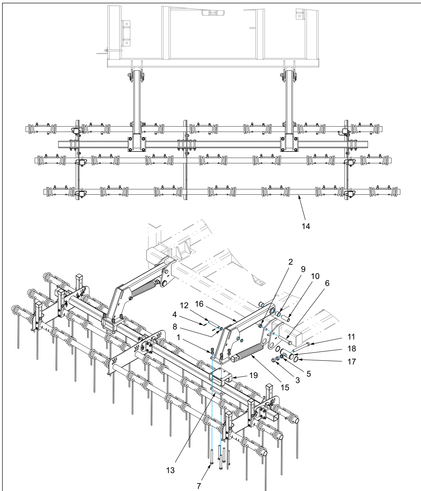
Figure 1-24: 3 Row Coil Tine Harrow Assembly - 12'
