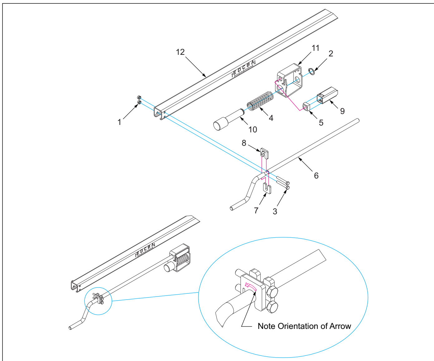
Figure 1-9: Depth Stop Assembly
