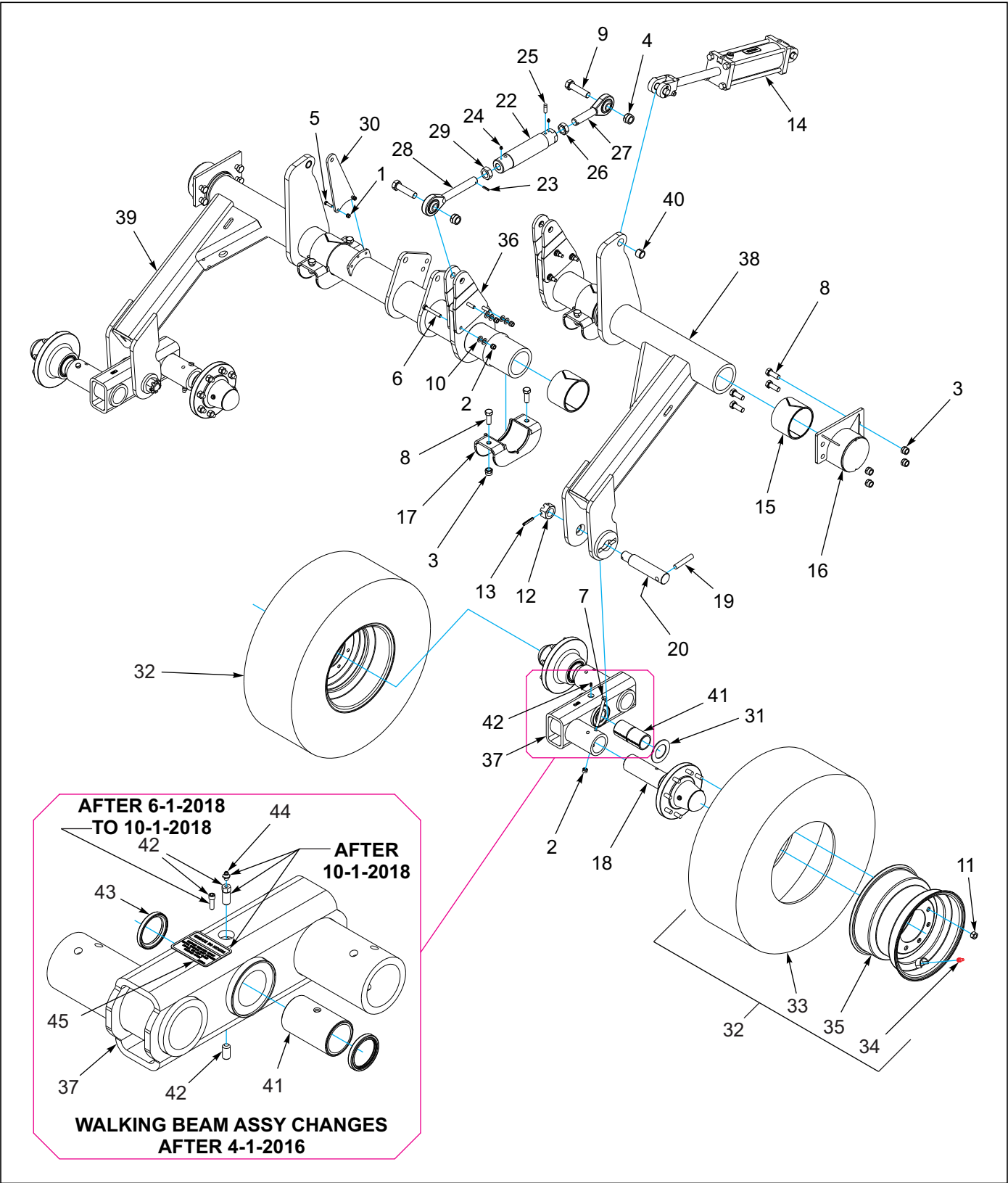
Figure 1-3: Lift Wheel Assembly
