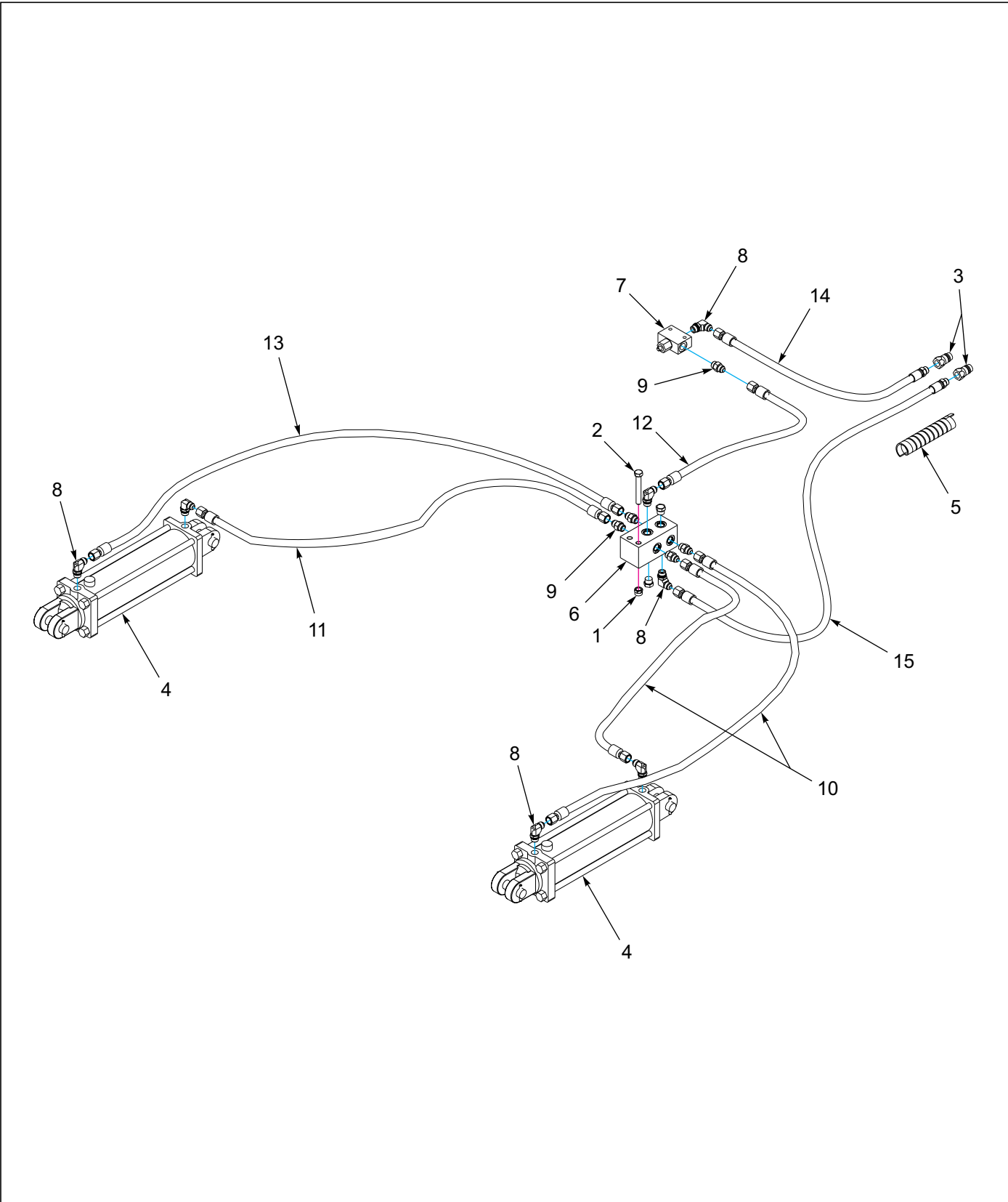
Figure 1-32: Lift Hydraulic Assembly - 12'-15'
