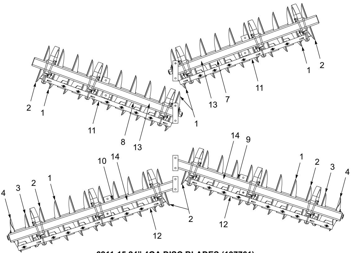
6211-15 24" 4GA DISC BLADES (197761)
