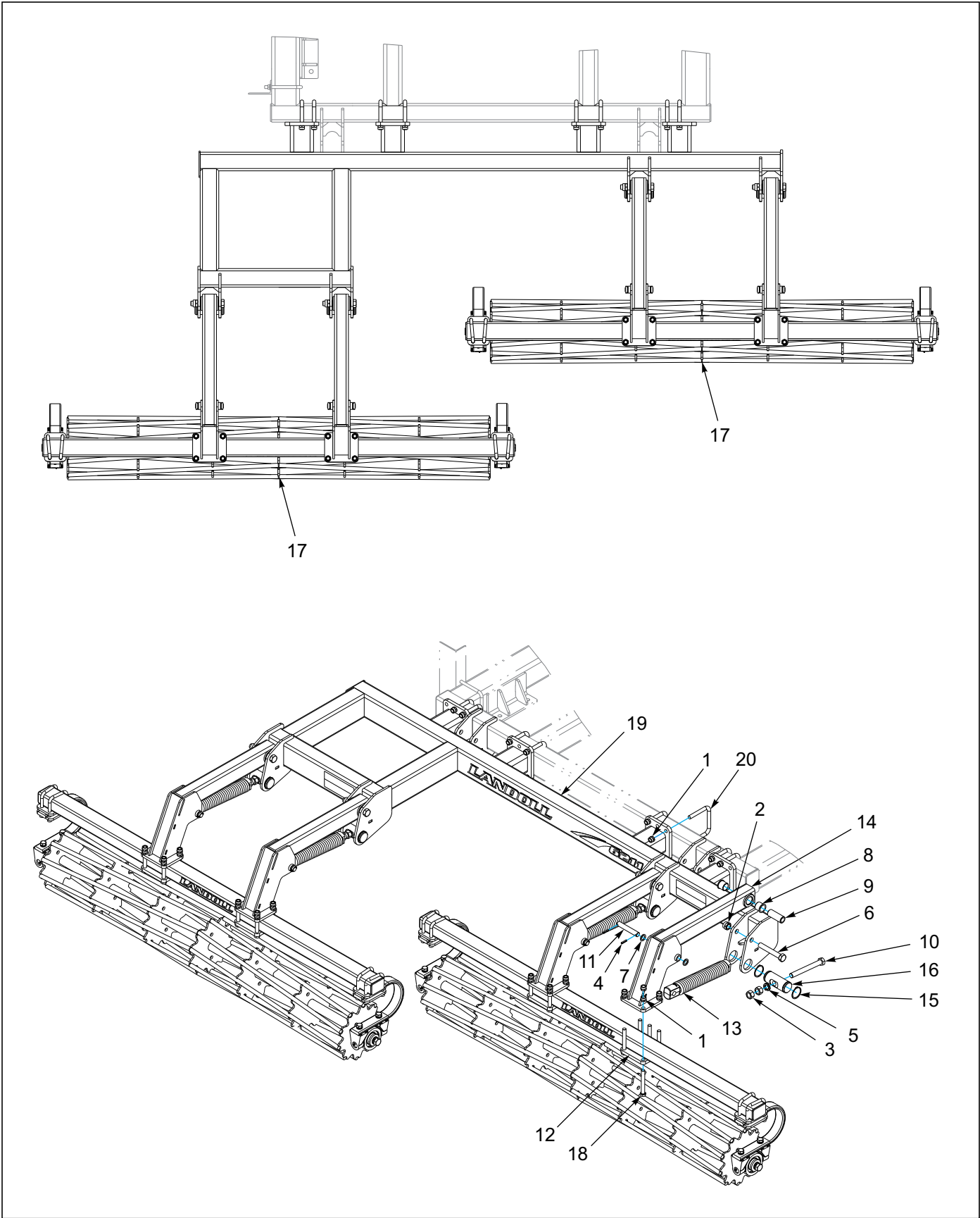
Figure 1-28: Conditioner Reel Assembly - 14' & 15'
