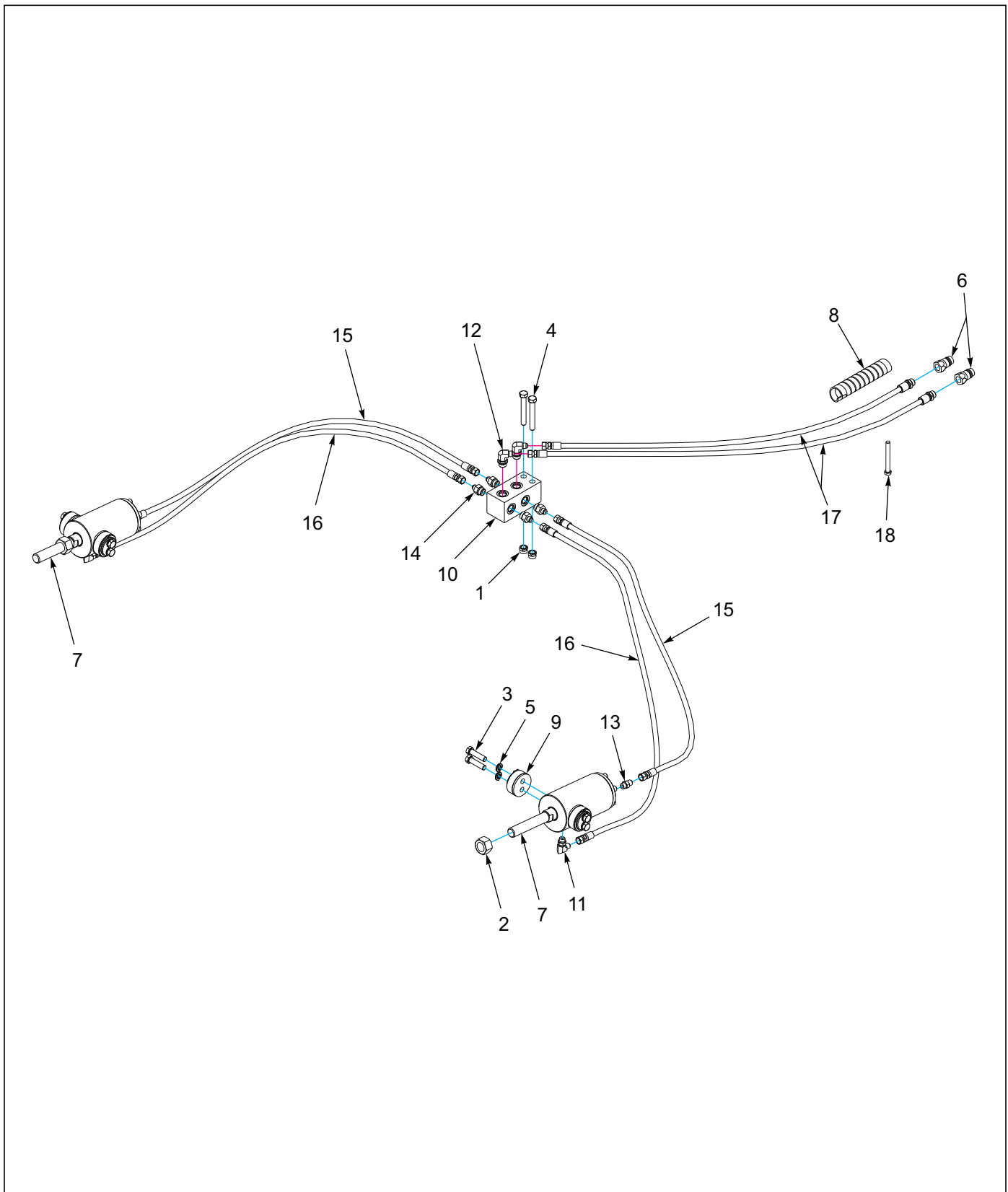
Figure 1-33: Reel Hydraulic Assembly - 12'
