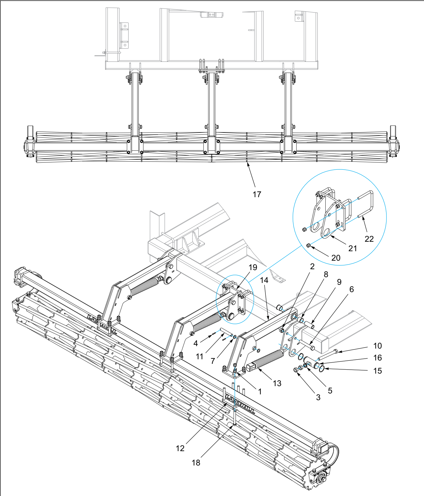
Figure 1-27: Conditioner Reel Assembly - 12'
