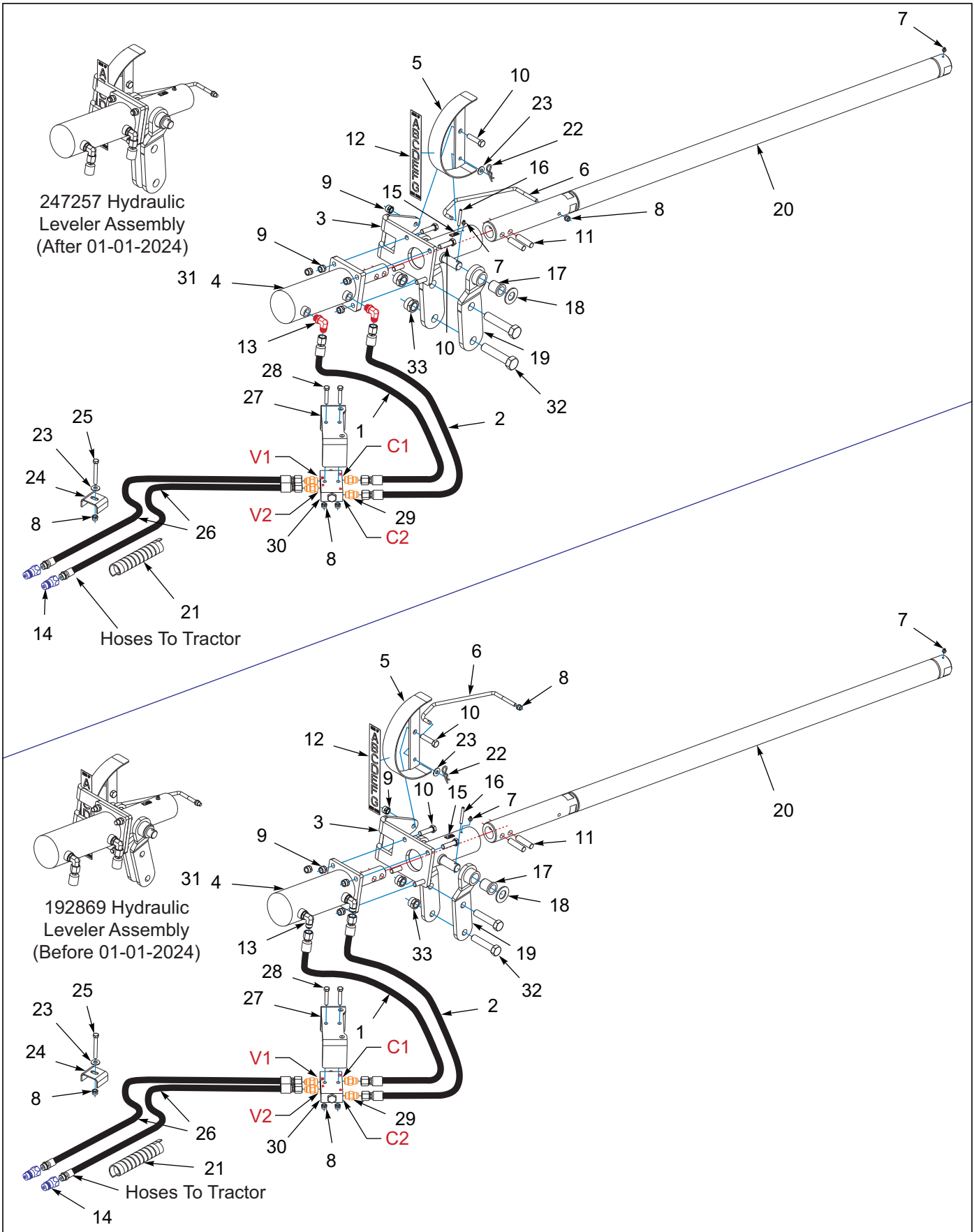
Figure 1-11: Hydraulic Leveler Assembly
