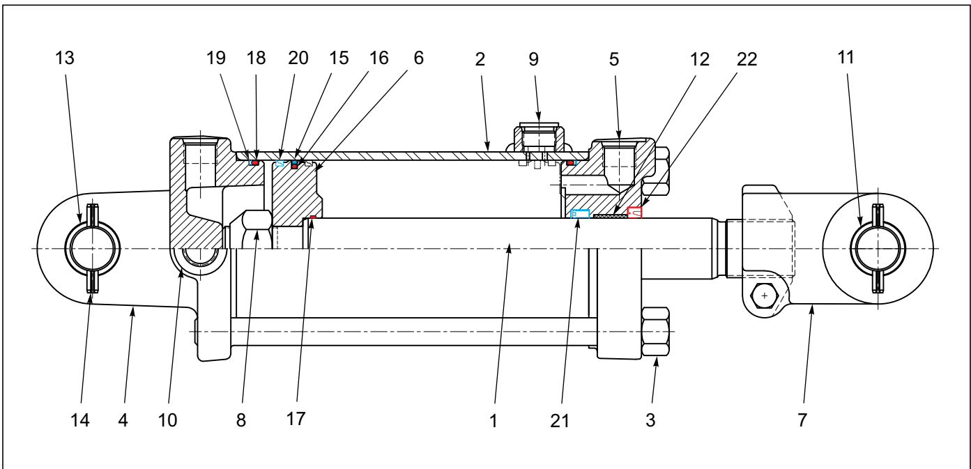
Figure 1-35: Rephase Cylinder 4" X 10"
