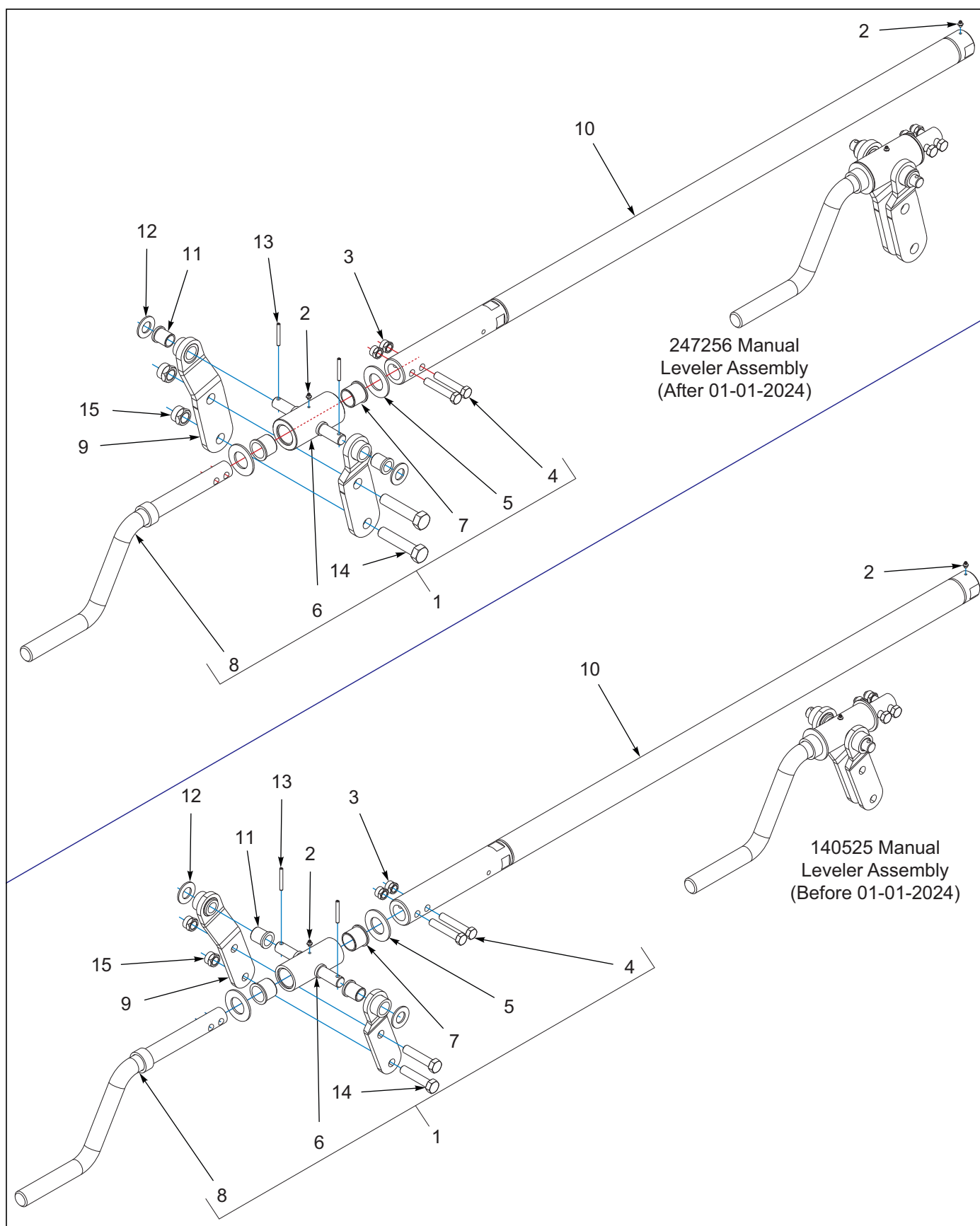
Figure 1-10: Manual Leveler Assembly
