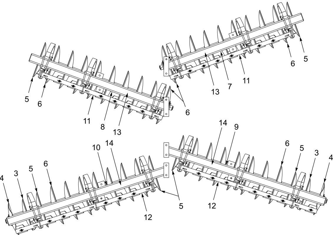
6211-15 24" 4GA DISC BLADES - ROLLABLE (197767)
