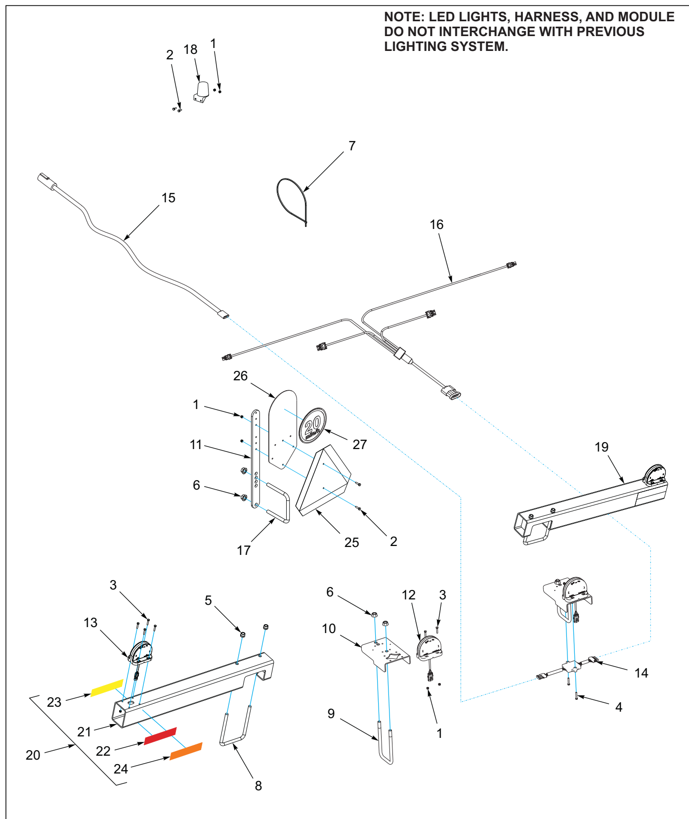
Figure 1-38: Electrical Assembly W/ LED Lights (1 of 2)
