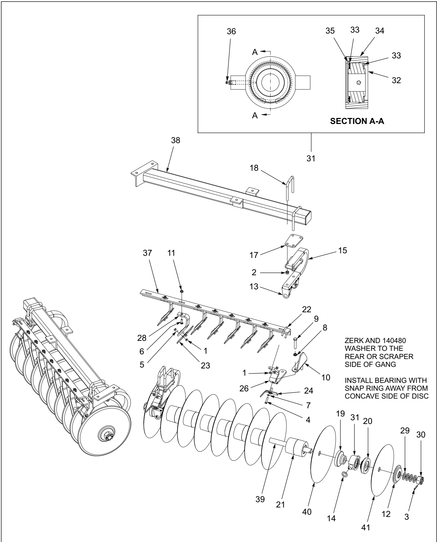
Figure 1-14: Disc Gang Assembly 22" (7" Spacing)
