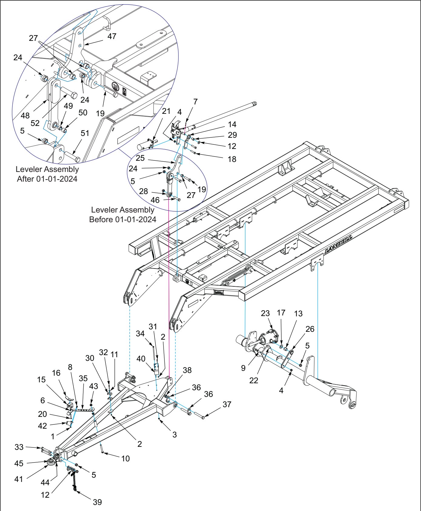
Figure 1-5: Hitch and Leveling Linkage Assembly
