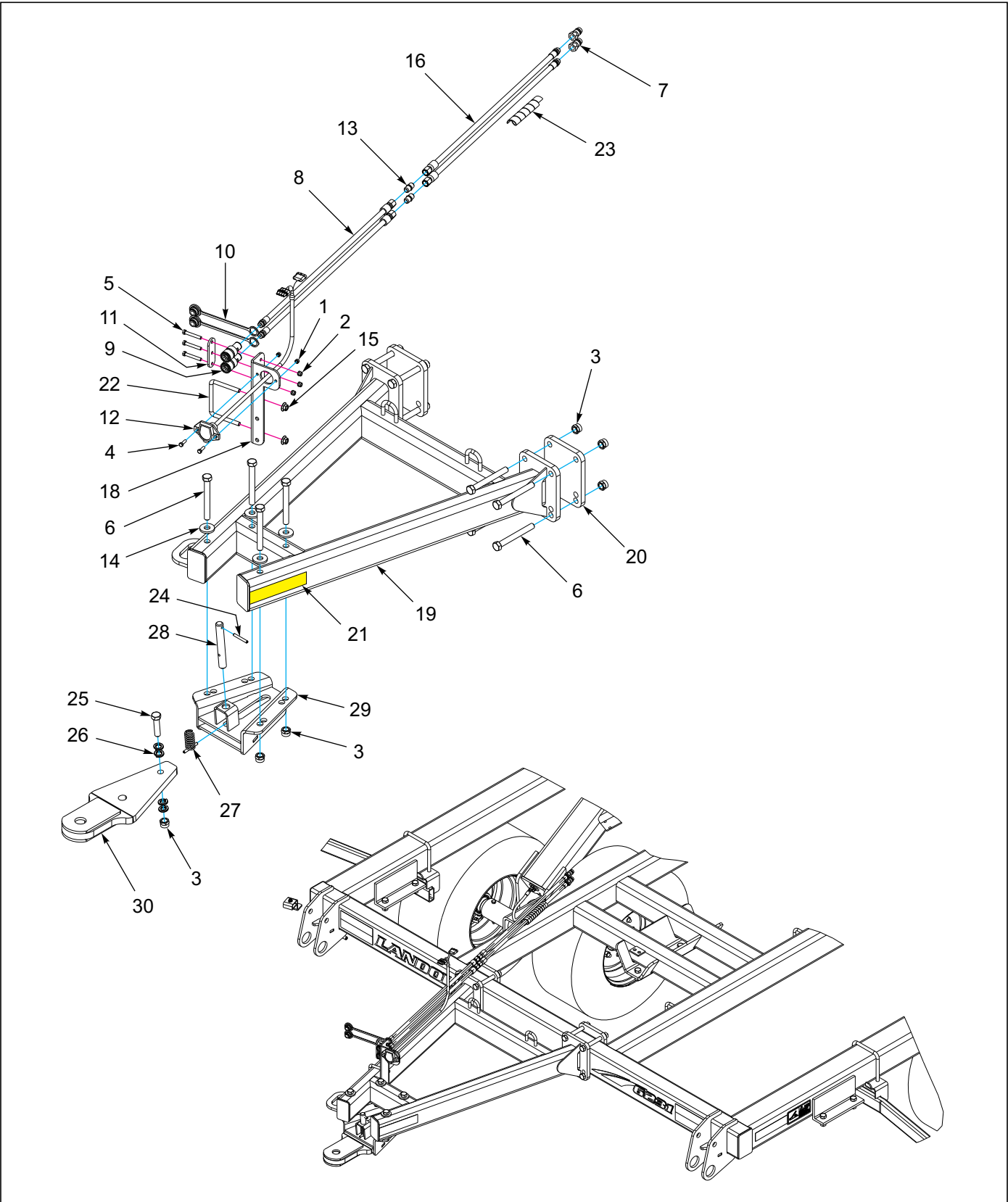
Figure 1-12: Straight Rear Tow Hitch
