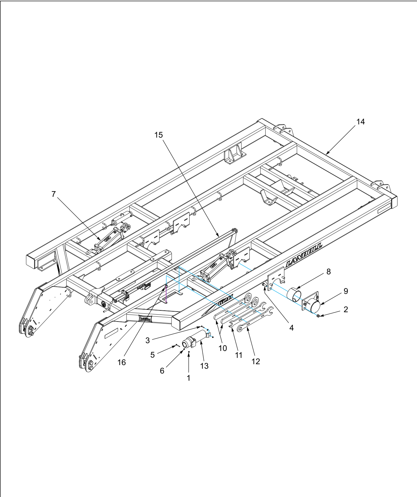
Figure 1-2: Frame Assembly
