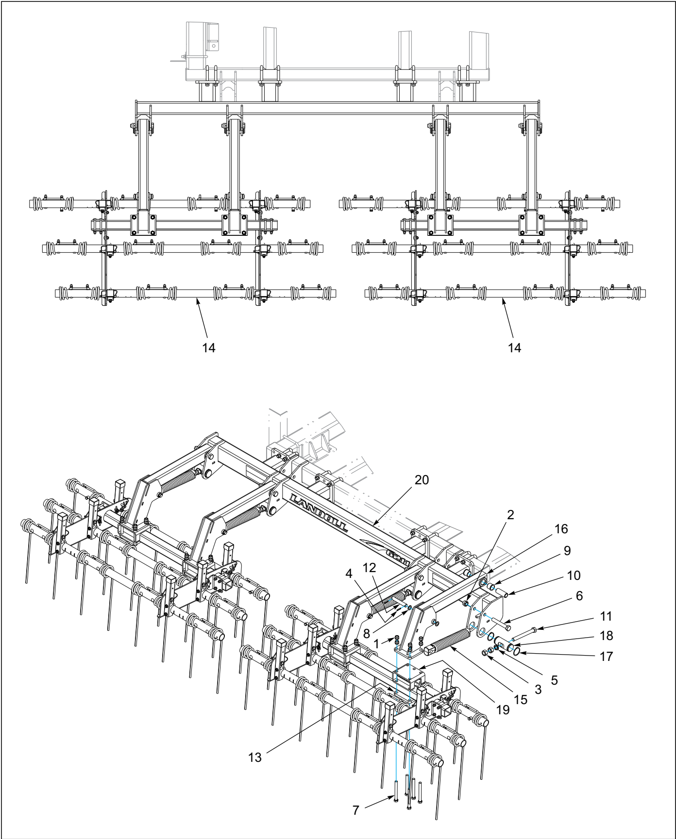
Figure 1-25: 3 Row Coil Tine Harrow Assembly - 14' & 15'
