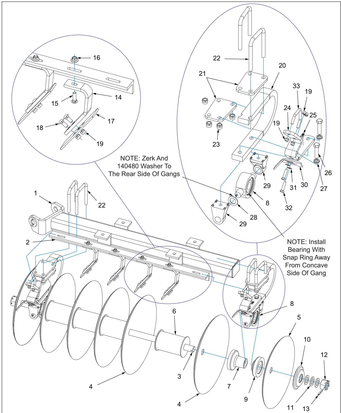
Figure 3-11: Disc Gang Assembly 24" 8-3/4SP Rollable 4 GA
