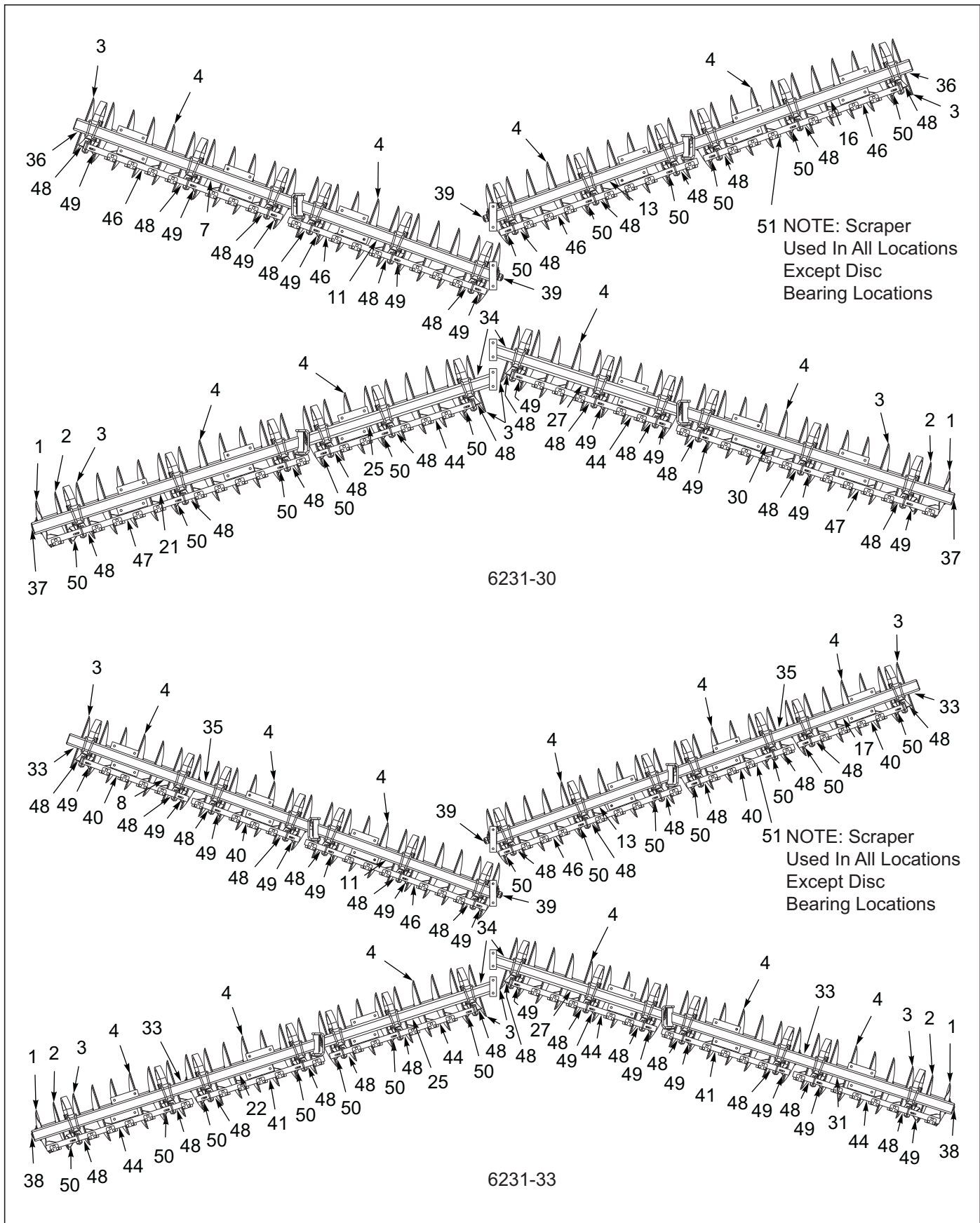
Figure 3-34: Disc Gang Assembly 6231 26" 8-3/4SP HDS 4 GA (Heavy Duty Scraper) (3 of 4)
