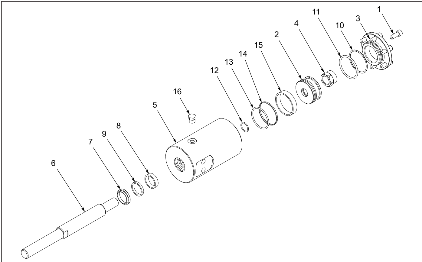
Figure 5-9: Cylinder Assembly 2-1/2 x 2-1/2
