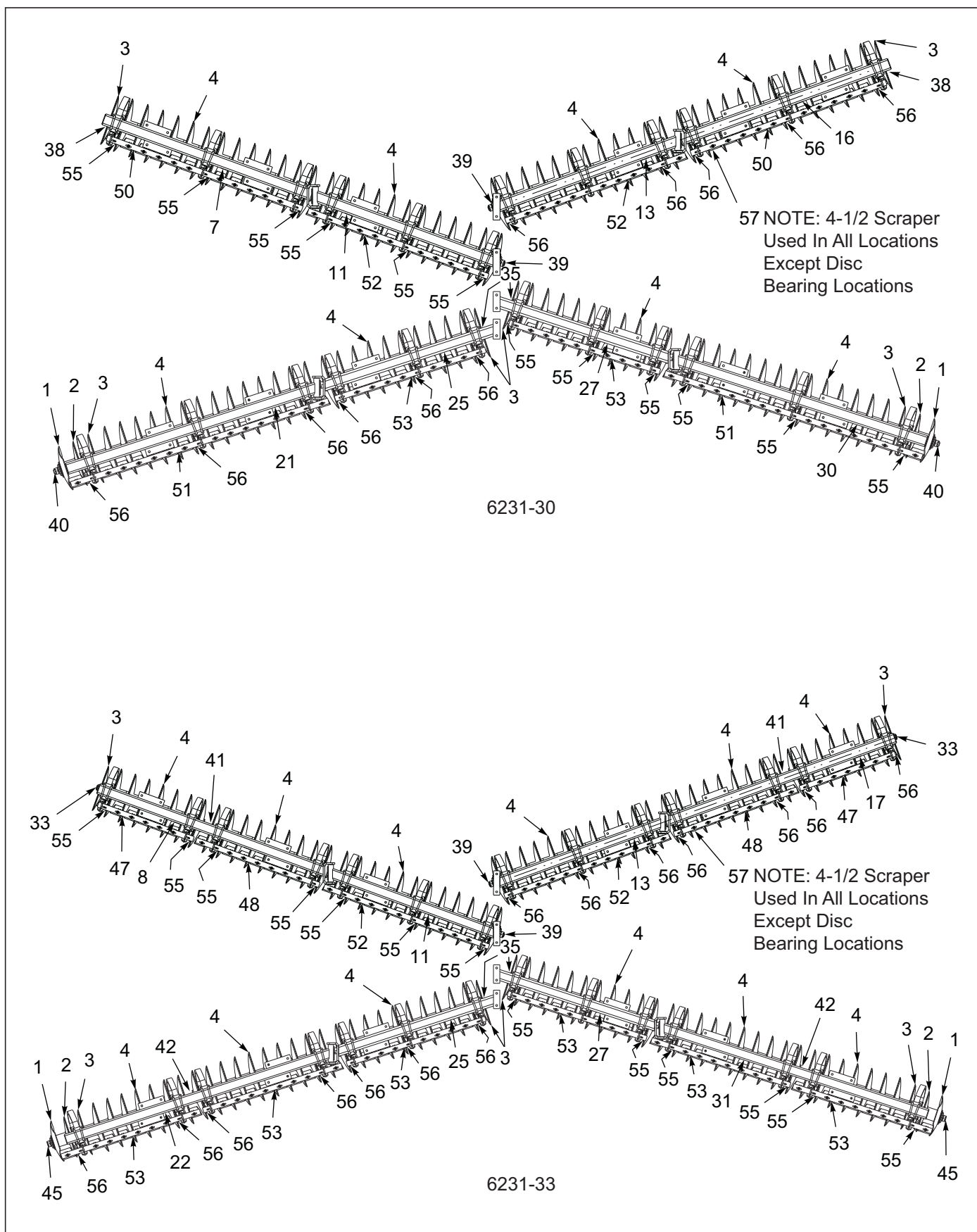
Figure 3-4: Disc Gang Assembly 6231 24" 7SP Rollable 4 GA (3 of 4)
