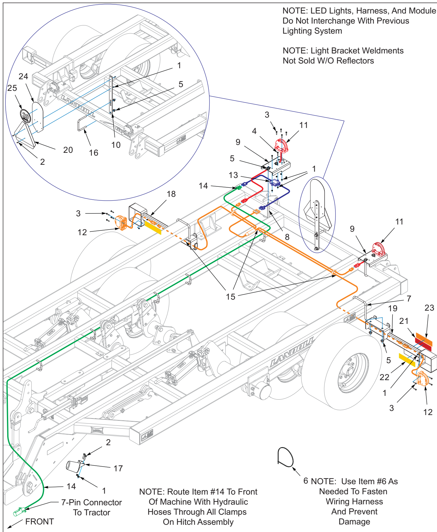
Figure 6-2: Electrical Assembly W/LED Lights
