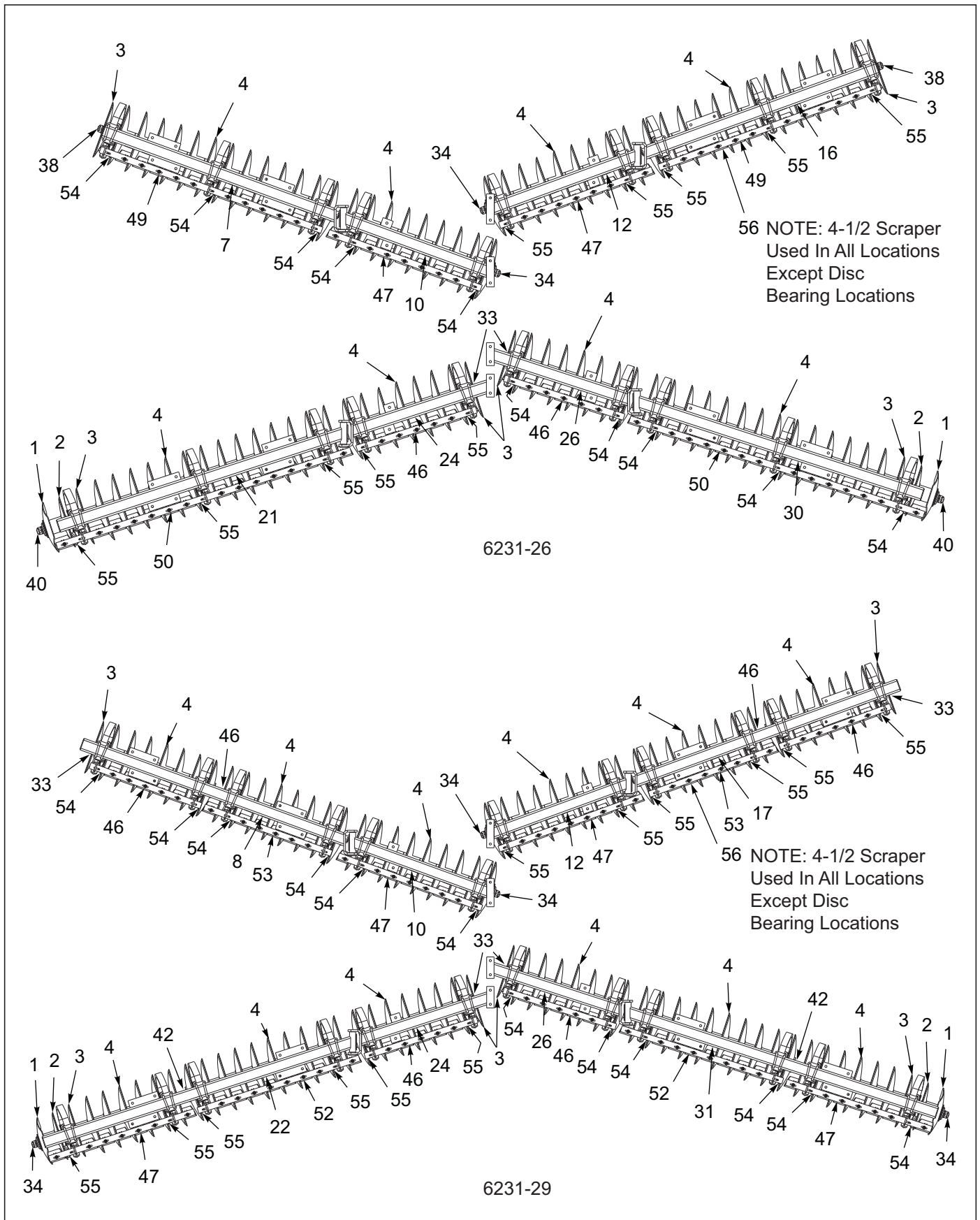
Figure 3-8: Disc Gang Assembly 6231 24' 7SP 4 GA (Non-Rollable) (2 of 4)
