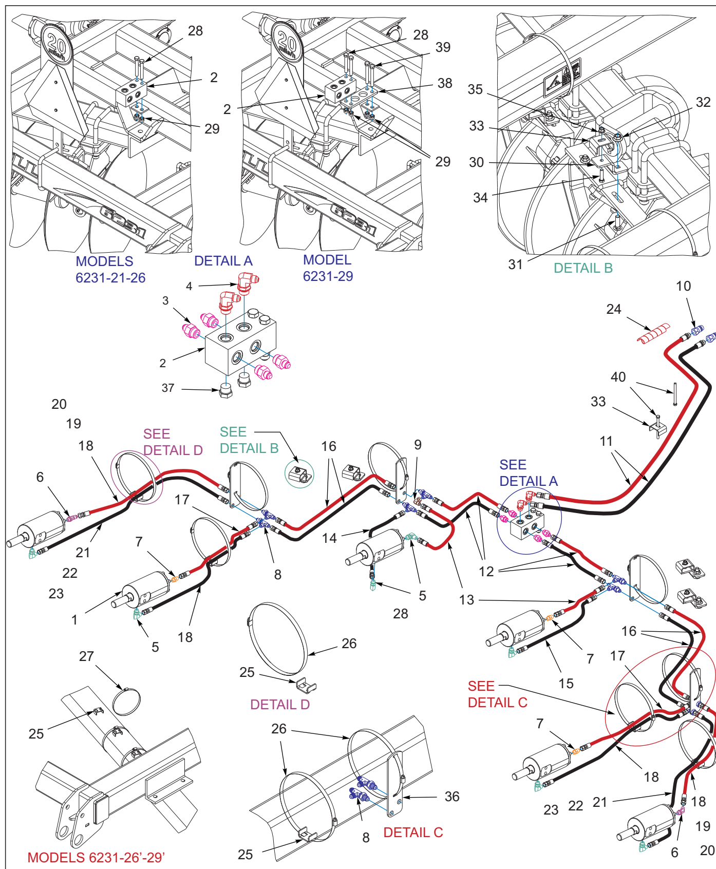
Figure 8-30: Hydraulic Double Reel Assembly 6231-21-26-29
