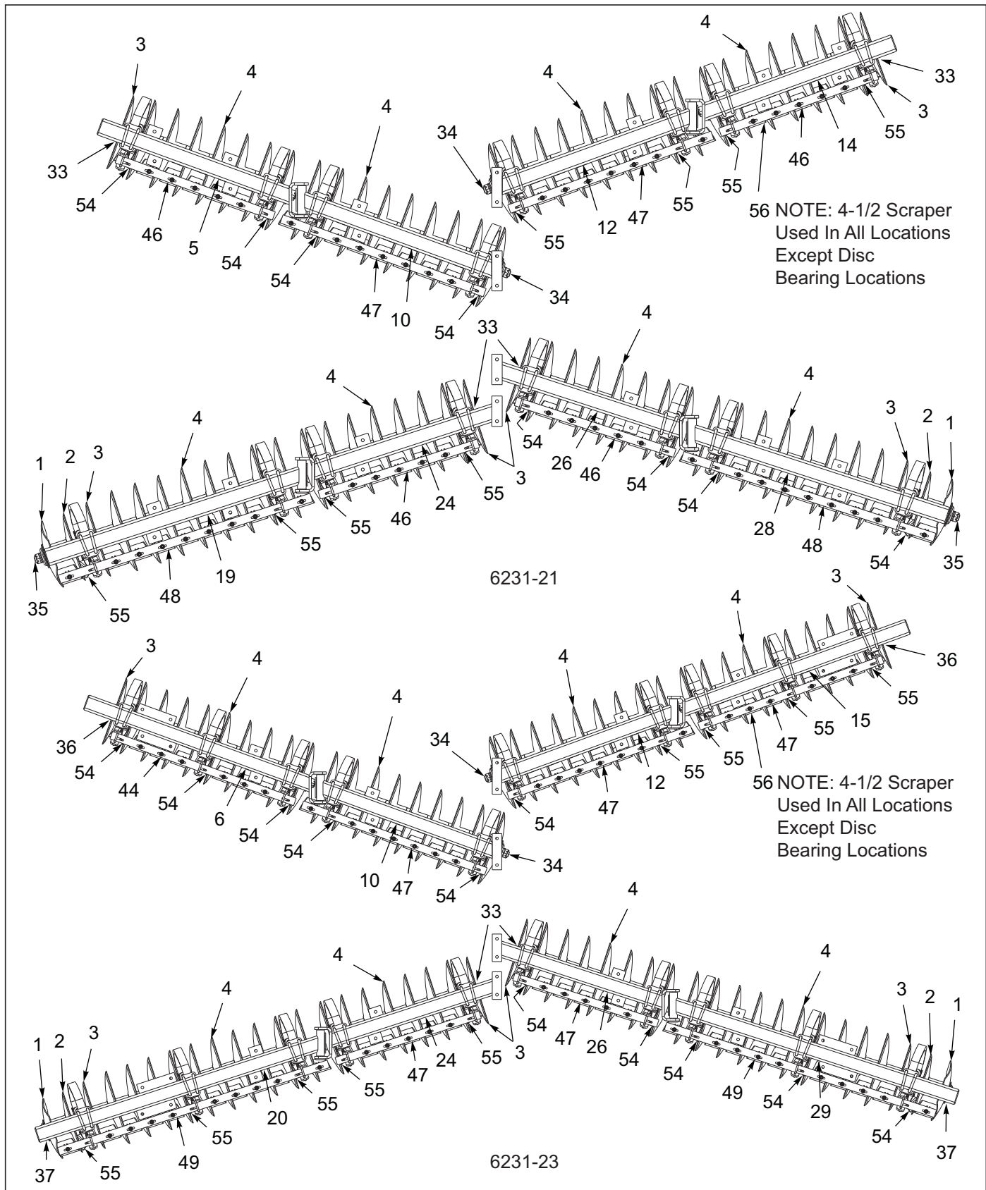
Figure 3-7: Disc Gang Assembly 6231 24" 7SP 4 GA (Non-Rollable) (1 of 4)
