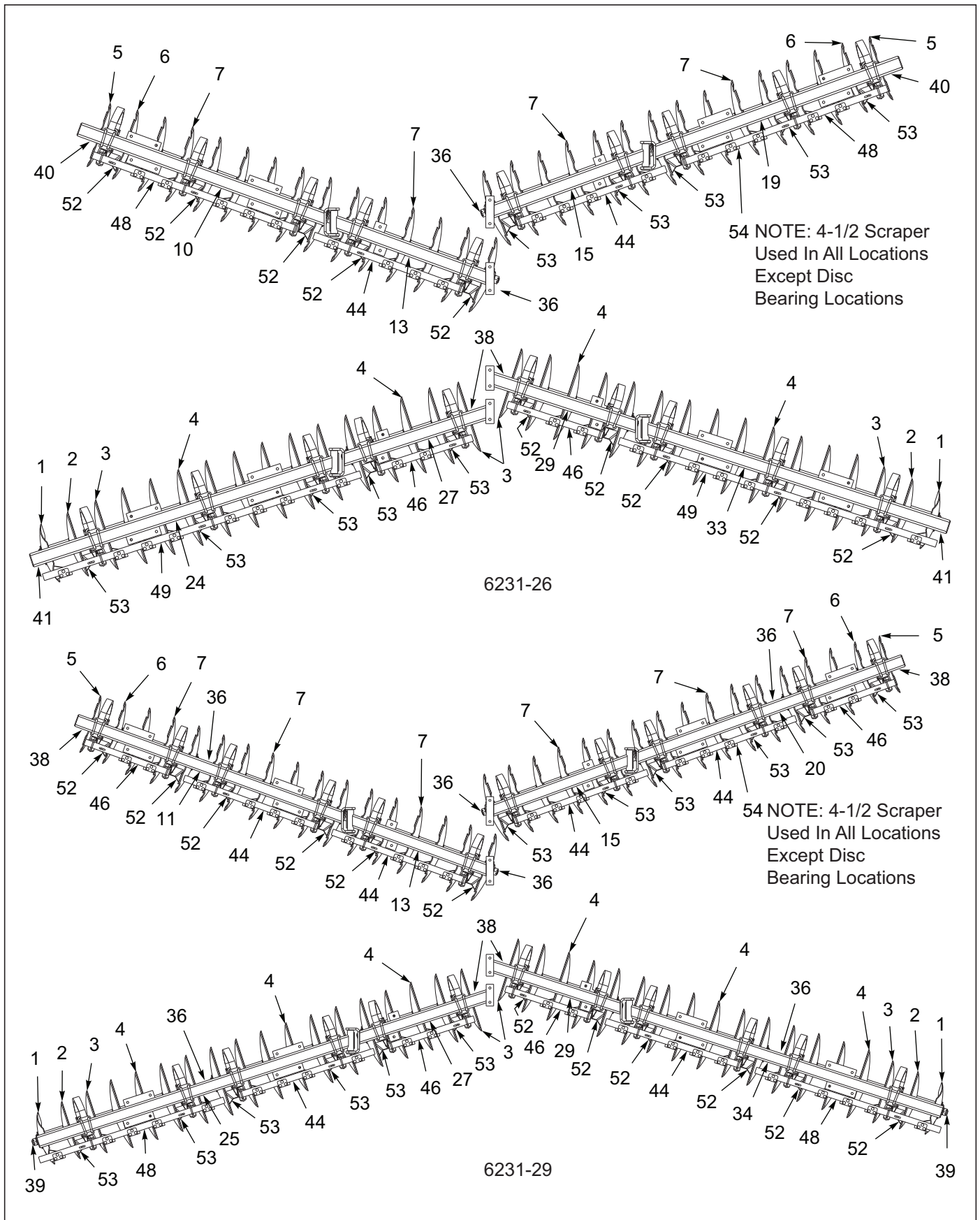
Figure 3-49: Disc Gang Assembly 6231 28" 10-1/2SP NF 5/16" (Notched Front) (2 of 4)
