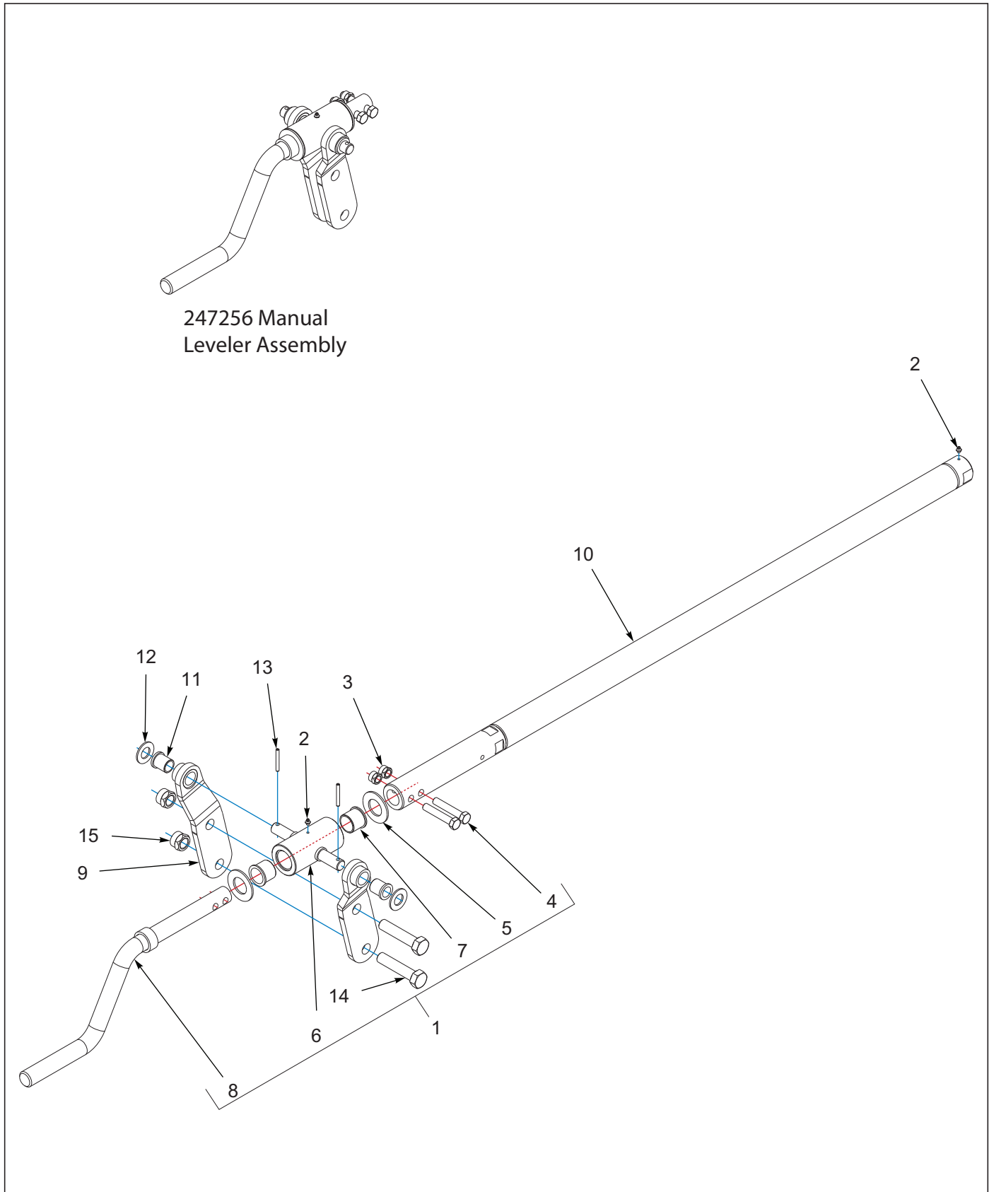
Figure 2-6: Leveler Assembly Manual (After 01-01-2024)
