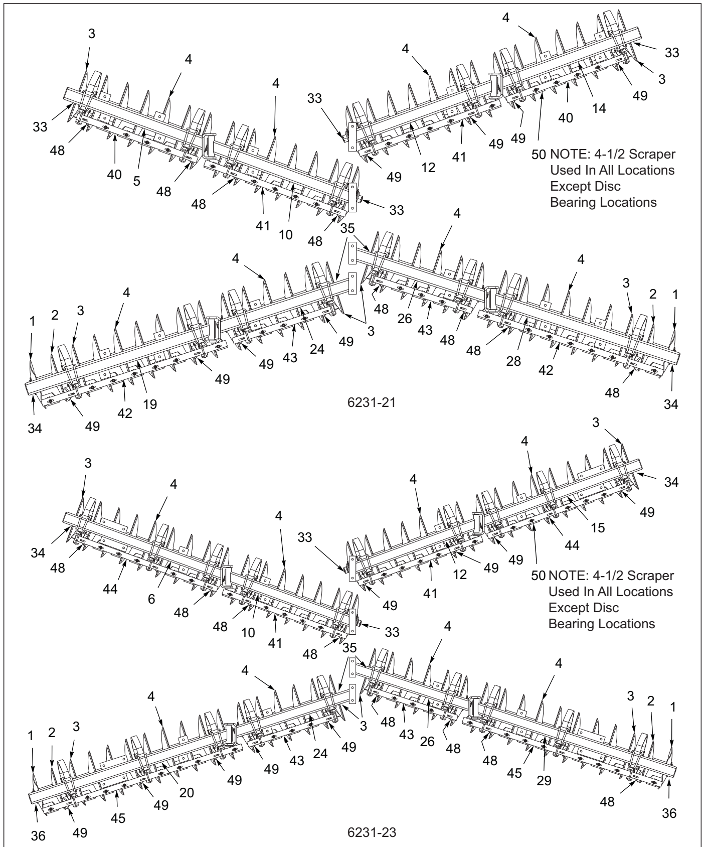
Figure 3-12: Disc Gang Assembly 6231 24" 8-3/4SP Rollable 4 GA (1 of 4)
