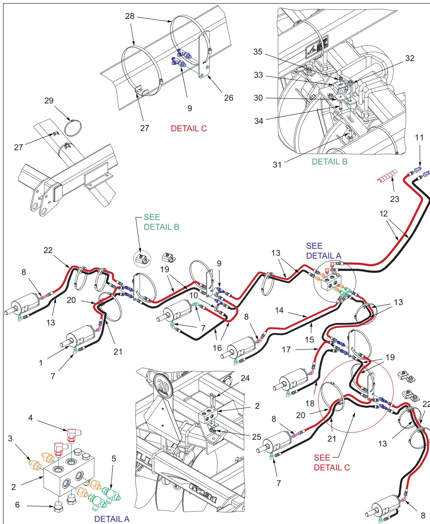
Figure 8-31: Hydraulic Double Reel Assembly 6231-30
