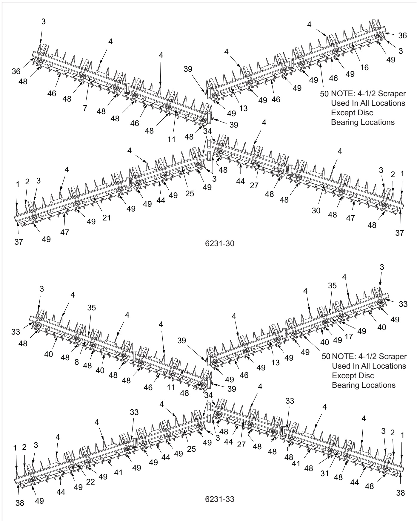
Figure 3-19: Disc Gang Assembly 6231 24' 8-3/4SP 4 GA (Non-Rollable) (3 of 4)
