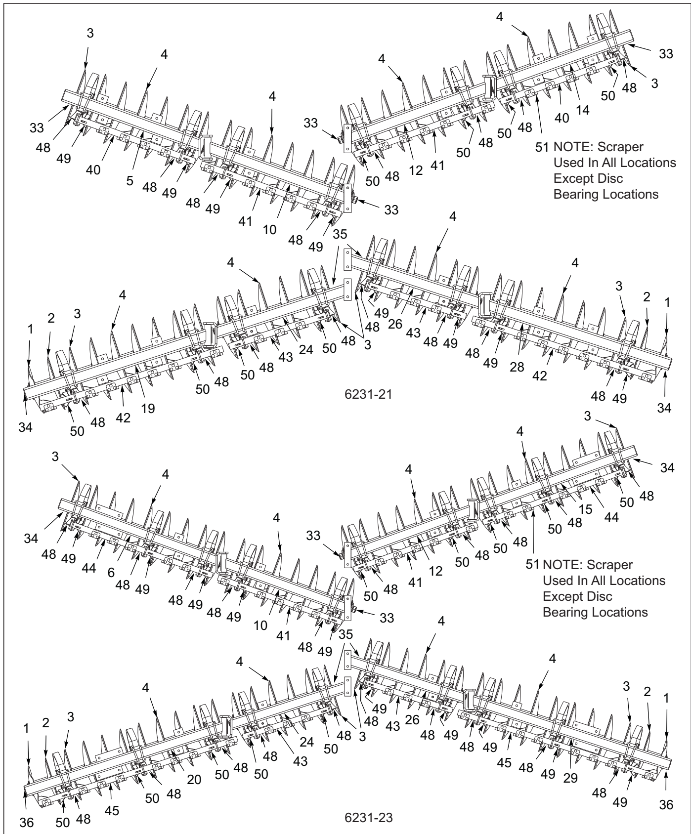
Figure 3-32: Disc Gang Assembly 6231 26" 8-3/4SP HDS 4 GA (Heavy Duty Scraper) (1 of 4)
