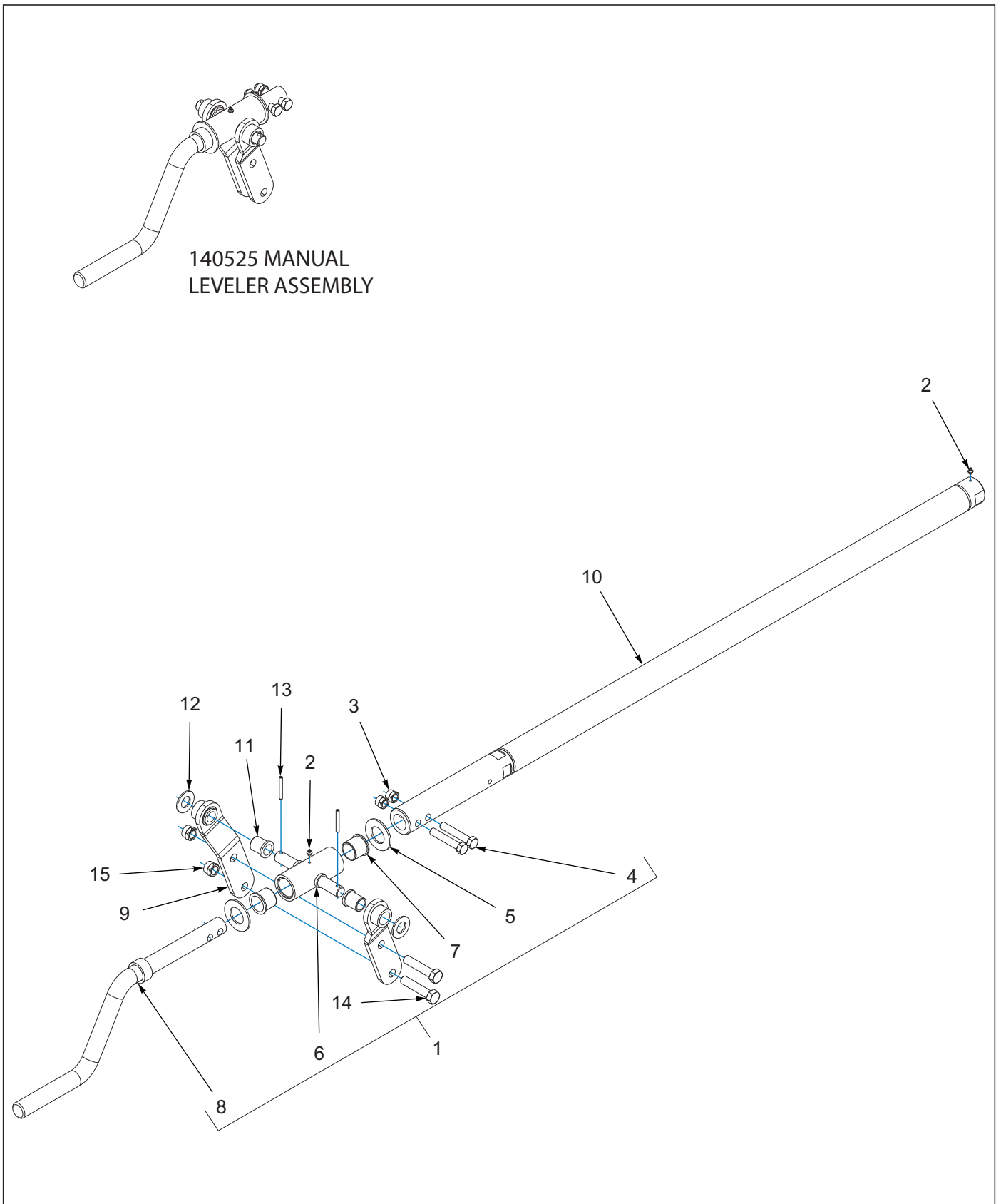
Figure 2-5: Leveler Assembly Manual (Before 01-01-2024)
