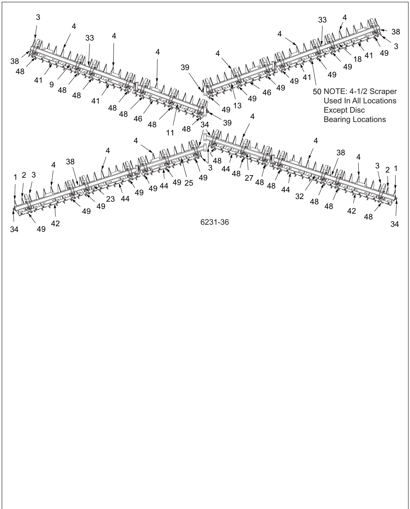
Figure 3-20: Disc Gang Assembly 6231 24" 8-3/4SP4 GA (Non-Rollable) (4 of 4)
