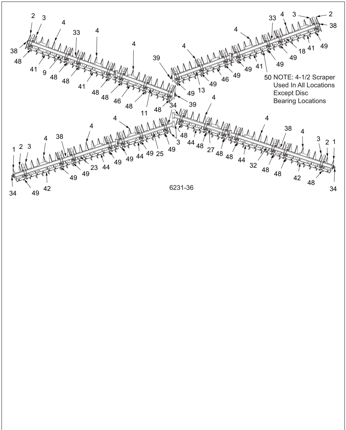
Figure 3-40: Disc Gang Assembly 6231 26" 8-3/4SP 5/16" (4 of 4)
