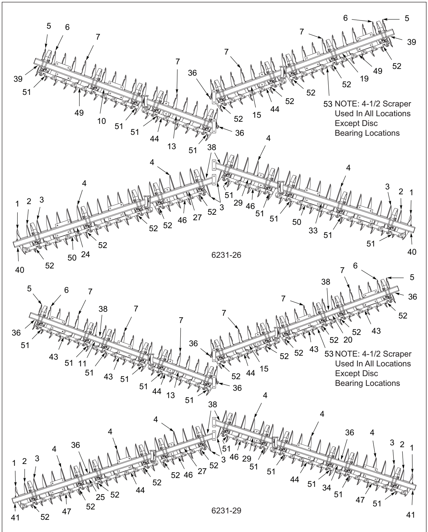
Figure 3-43: Disc Gang Assembly 6231 28" 8-3/4SP NF 5/16"(Notched Front) (2 of 4)
