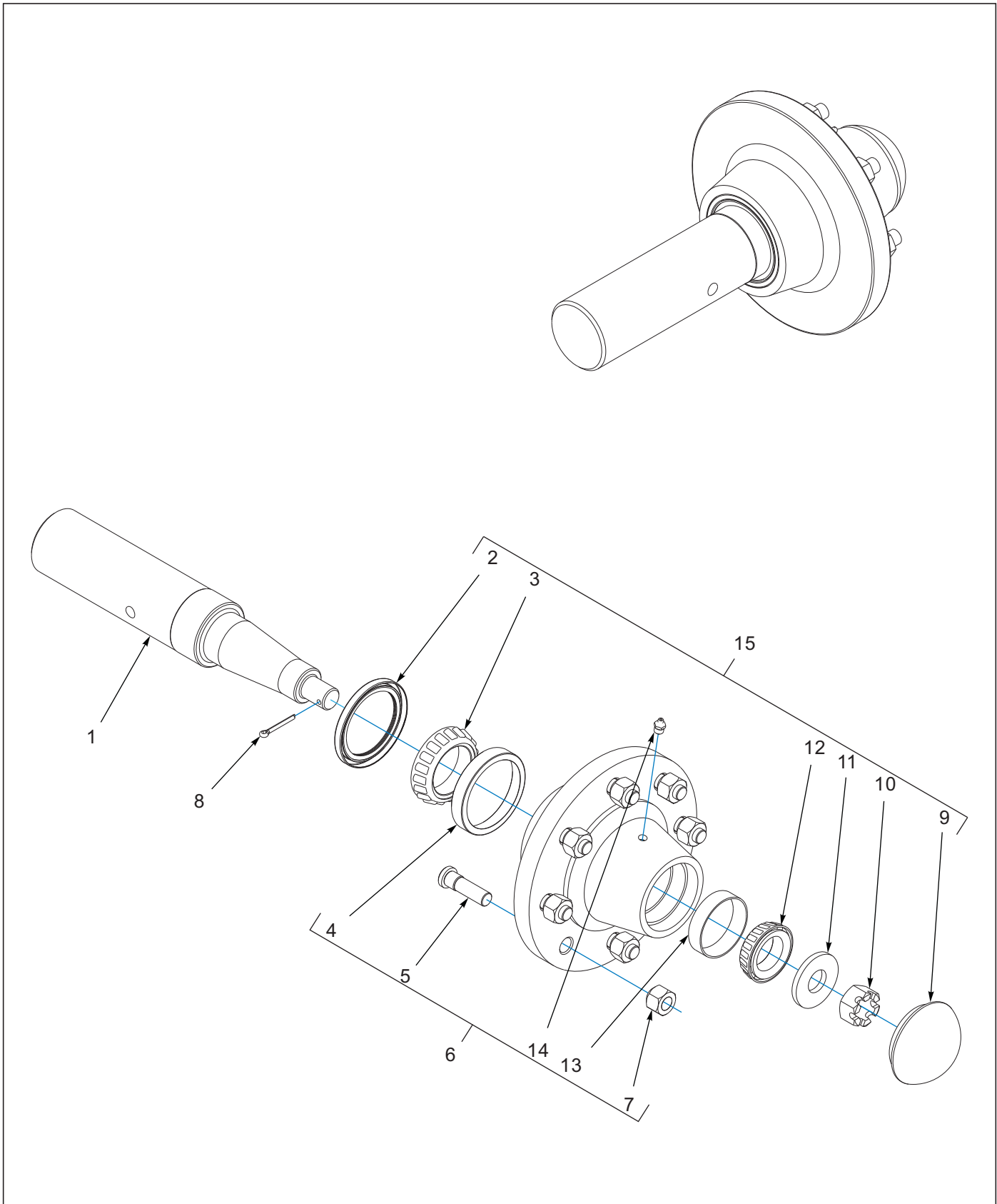
Figure 1-9: Hub/Spindle Assembly 156972
