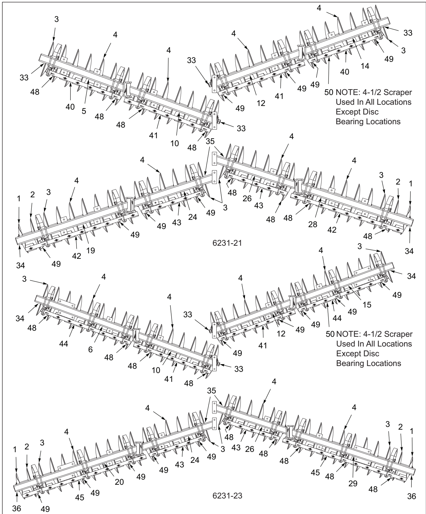
Figure 3-27: Disc Gang Assembly 6231 26" 8-3/4SP 4 GA (1 of 4)
