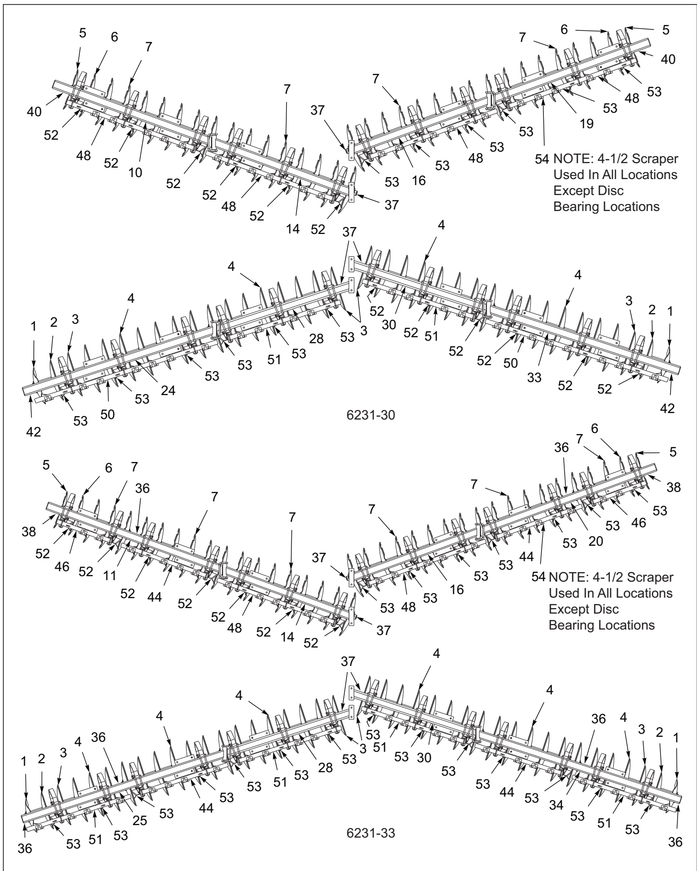
Figure 3-50: Disc Gang Assembly 6231 28" 10-1/2SP NF 5/16" (Notched Front) (3 of 4)
