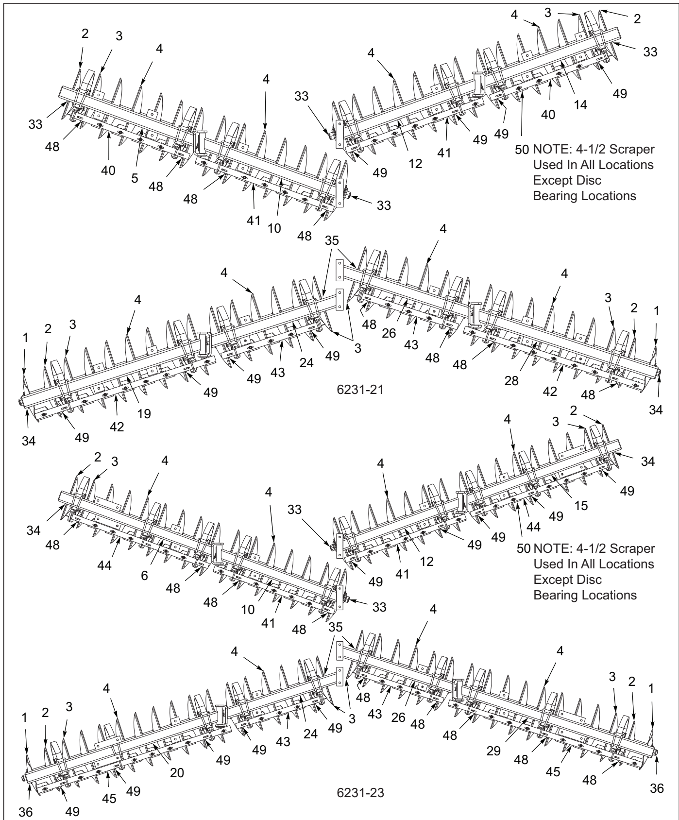
Figure 3-37: Disc Gang Assembly 6231 26" 8-3/4SP 5/16" (1 of 4)
