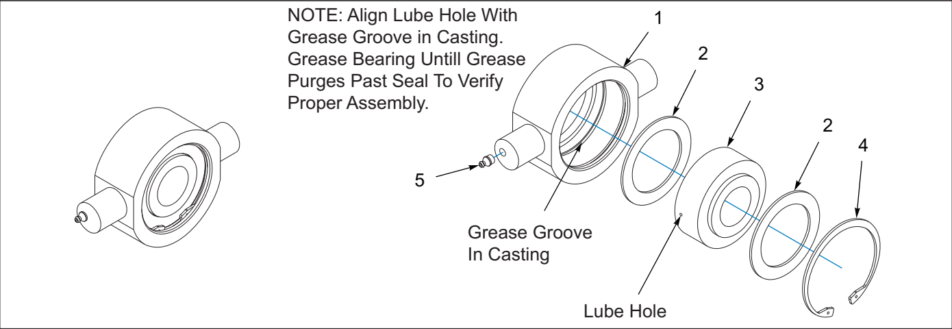
Figure 3-52: Disc Bearing Assembly
