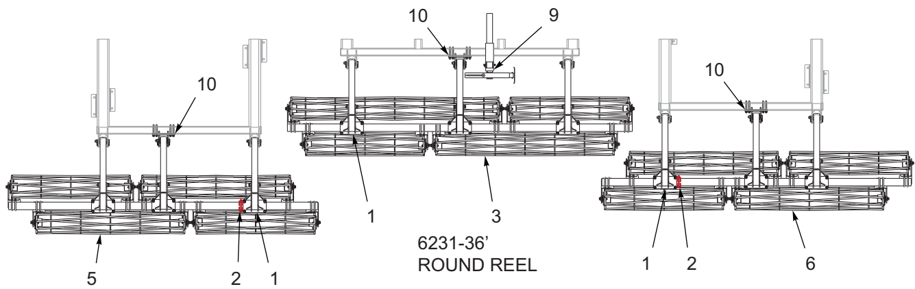
6231-36' - 135"/135" ROUND REEL
