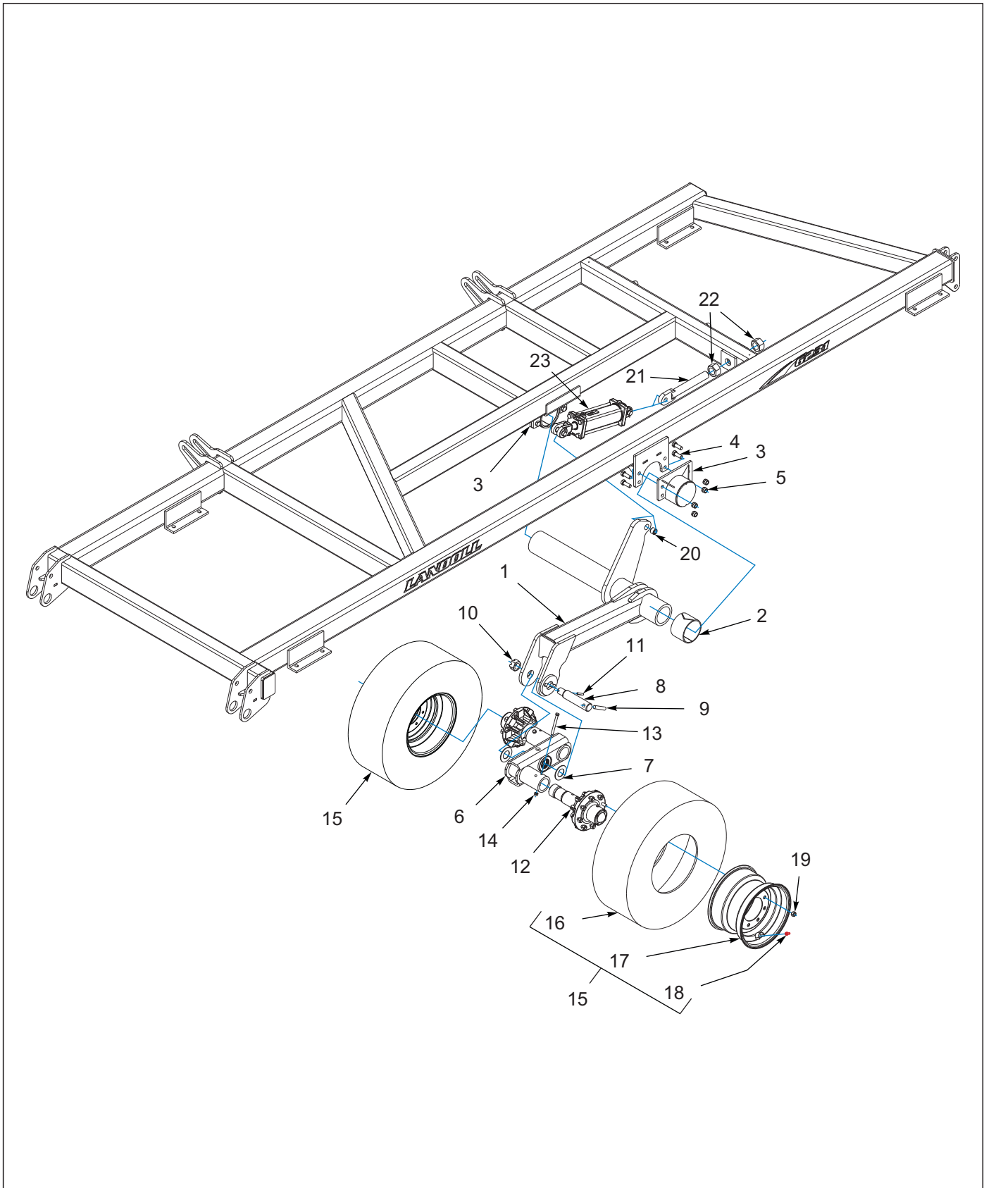
Figure 1-6: Wing Lift Assembly 6231-23'-29', 30'-36' (BEFORE 02-15-2020)
