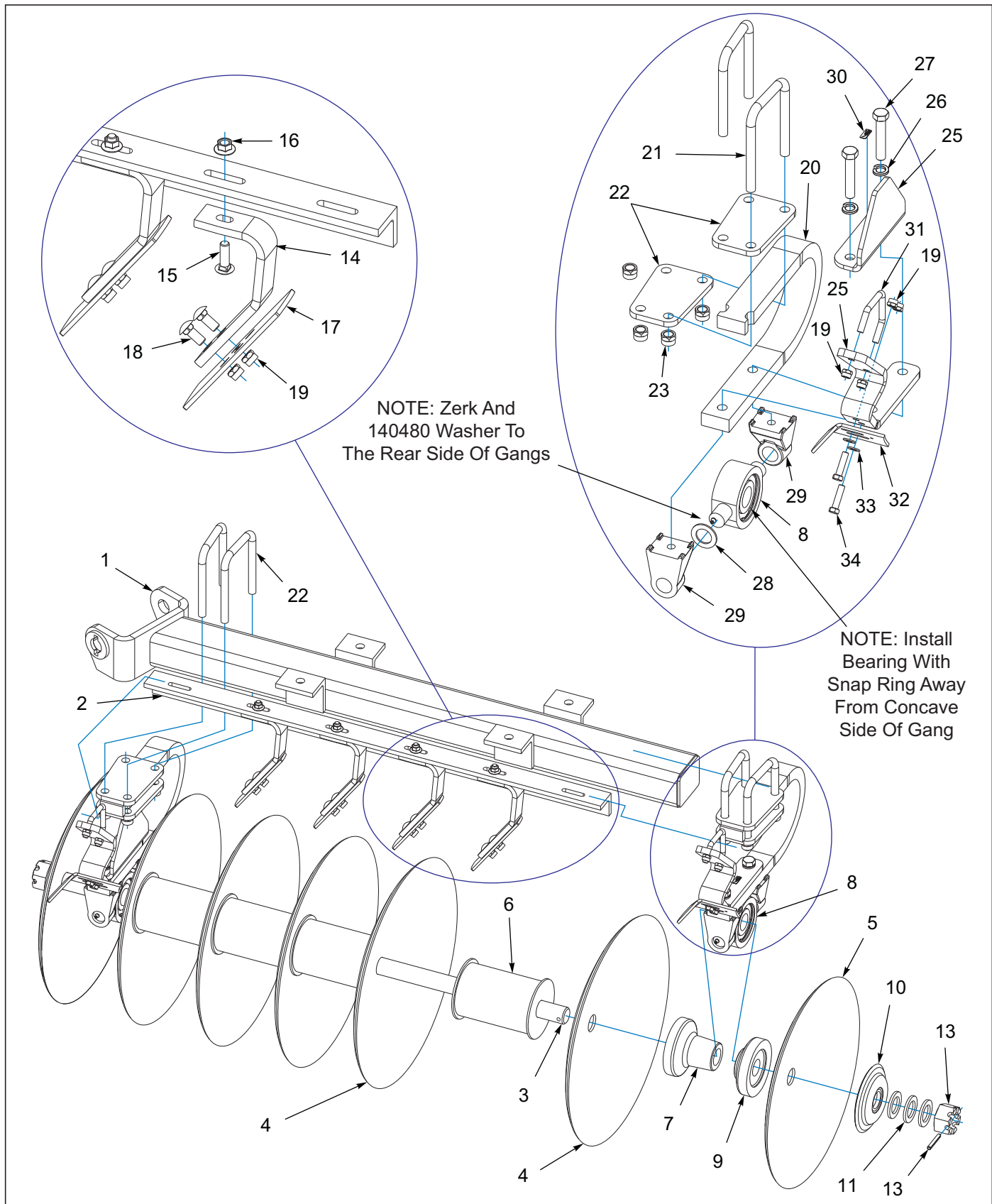
Figure 3-16: Disc Gang Assembly 24" 8-3/4SP 4 GA (Non-Rollable)
