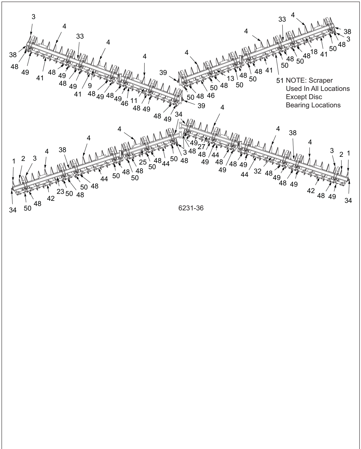
Figure 3-25: Disc Gang Assembly 6231 24" 8-3/4SP HDS 4 GA (Heavy Duty Scraper) (4 of 4)
