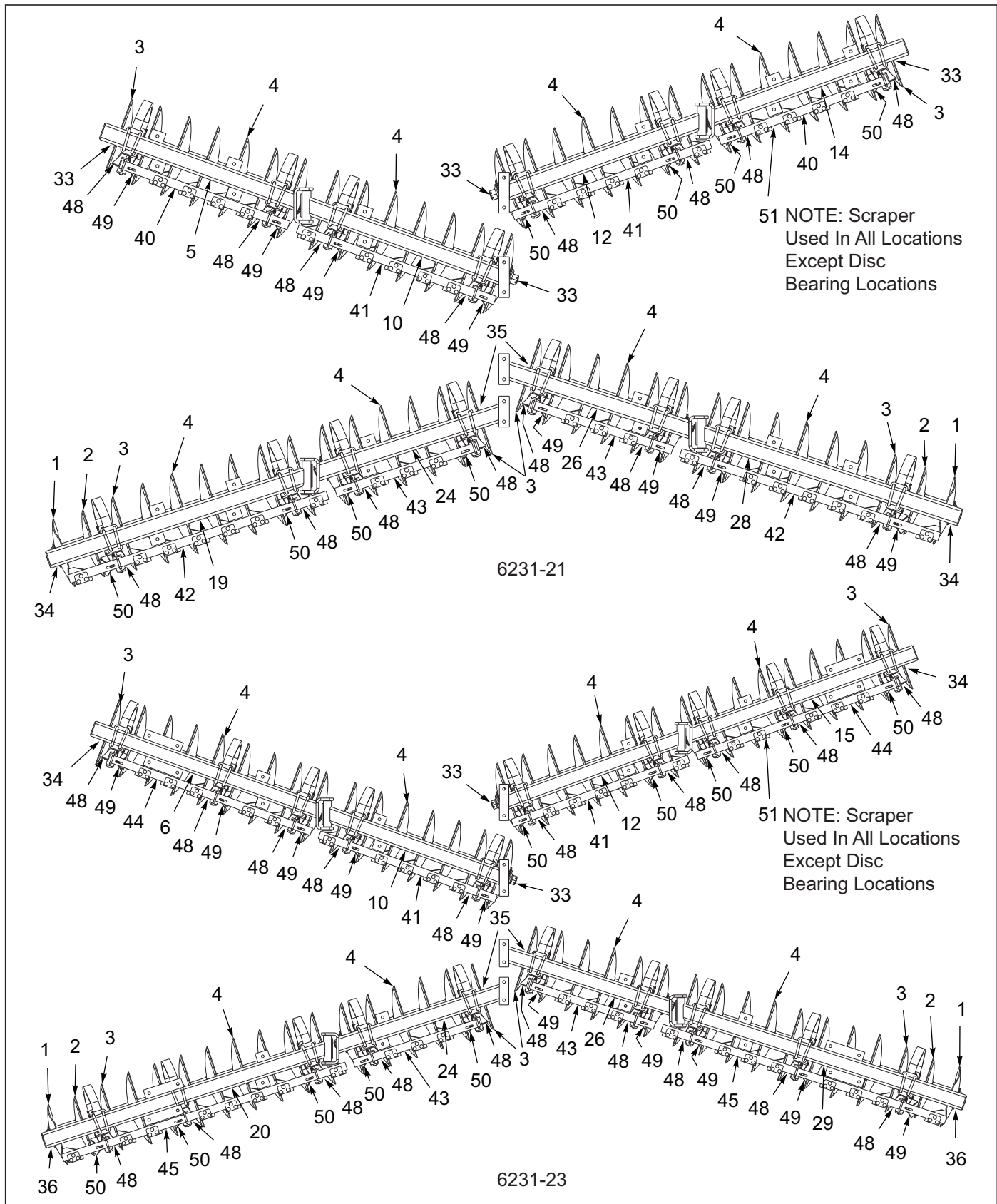
Figure 3-22: Disc Gang Assembly 6231 24" 8-3/4SP HDS 4 GA (Heavy Duty Scraper) (1 of 4)
