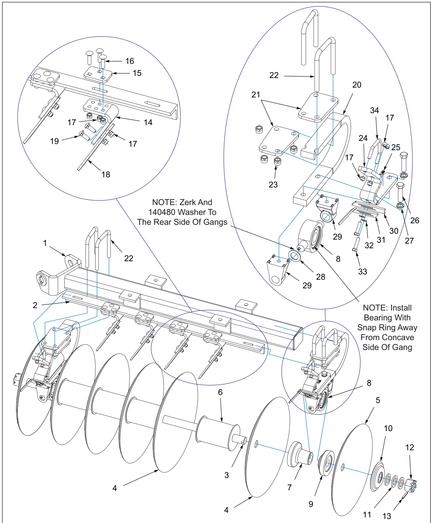
Figure 3-21: Disc Gang Assembly 24" 8-3/4SP HDS 4 GA (Heavy Duty Scraper)
