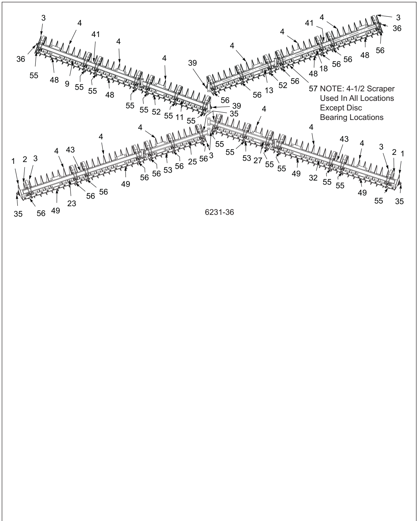
Figure 3-5: Disc Gang Assembly 6231 24" 7SP Rollable 4 GA (4 of 4)
