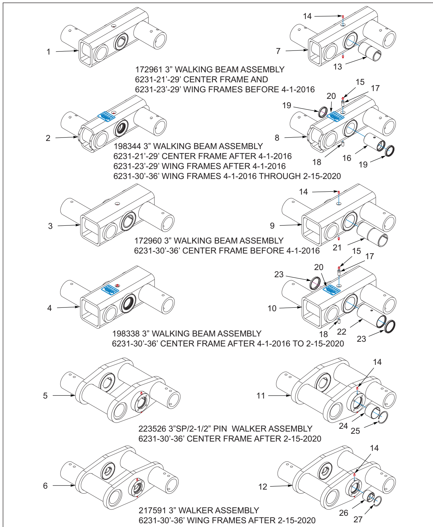
Figure 1-8: Walking Beam Assemblies
