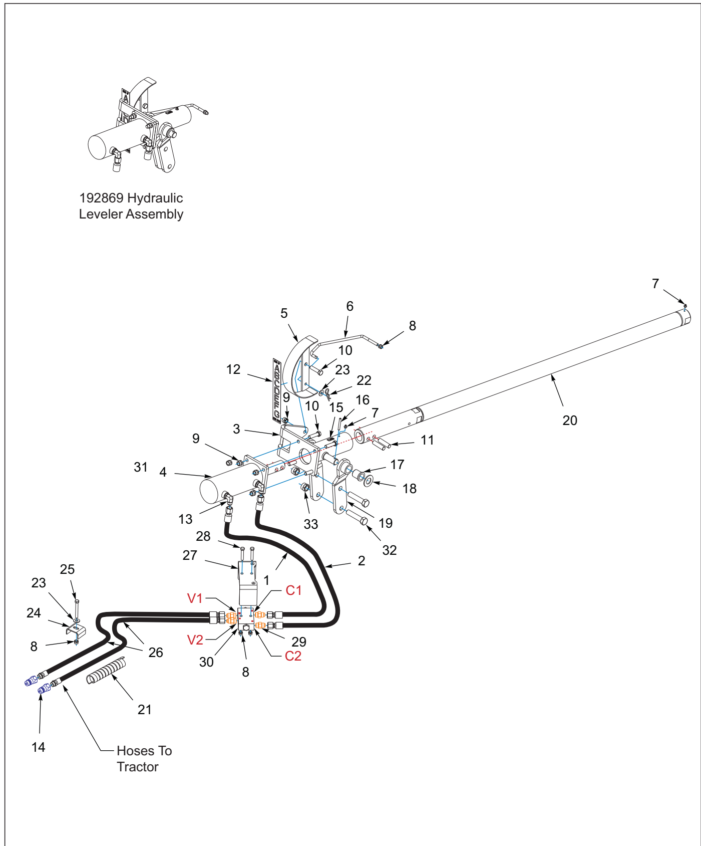
Figure 2-7: Leveler Assembly Hydraulic (Before 01-01-2024)
