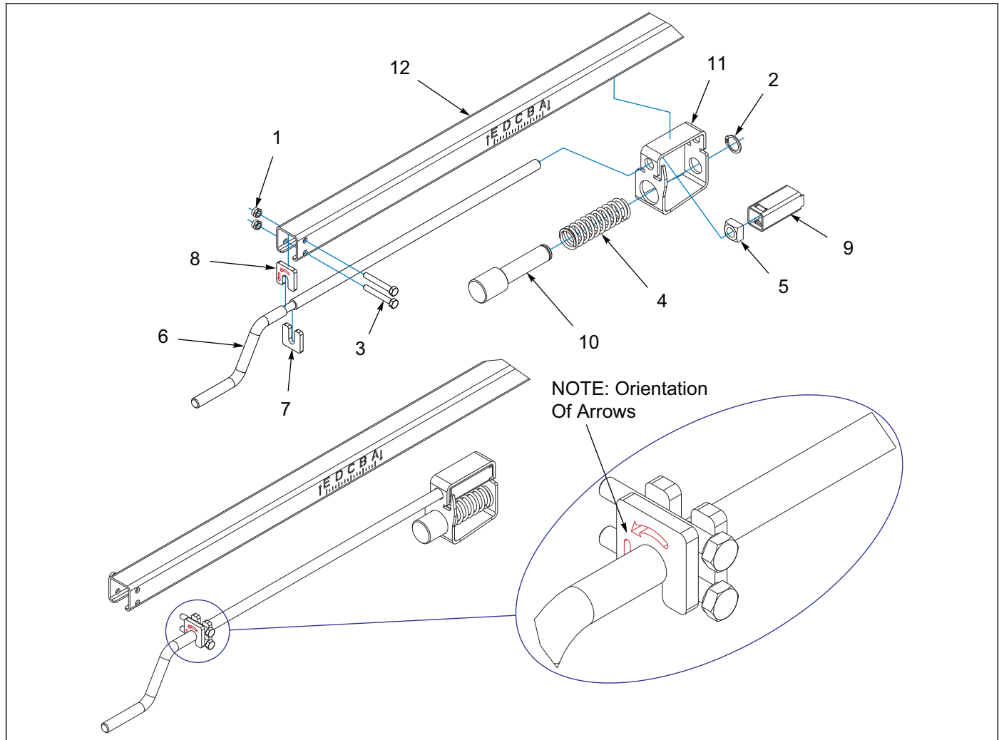
Figure 2-4: Depth Stop Tube Assembly
