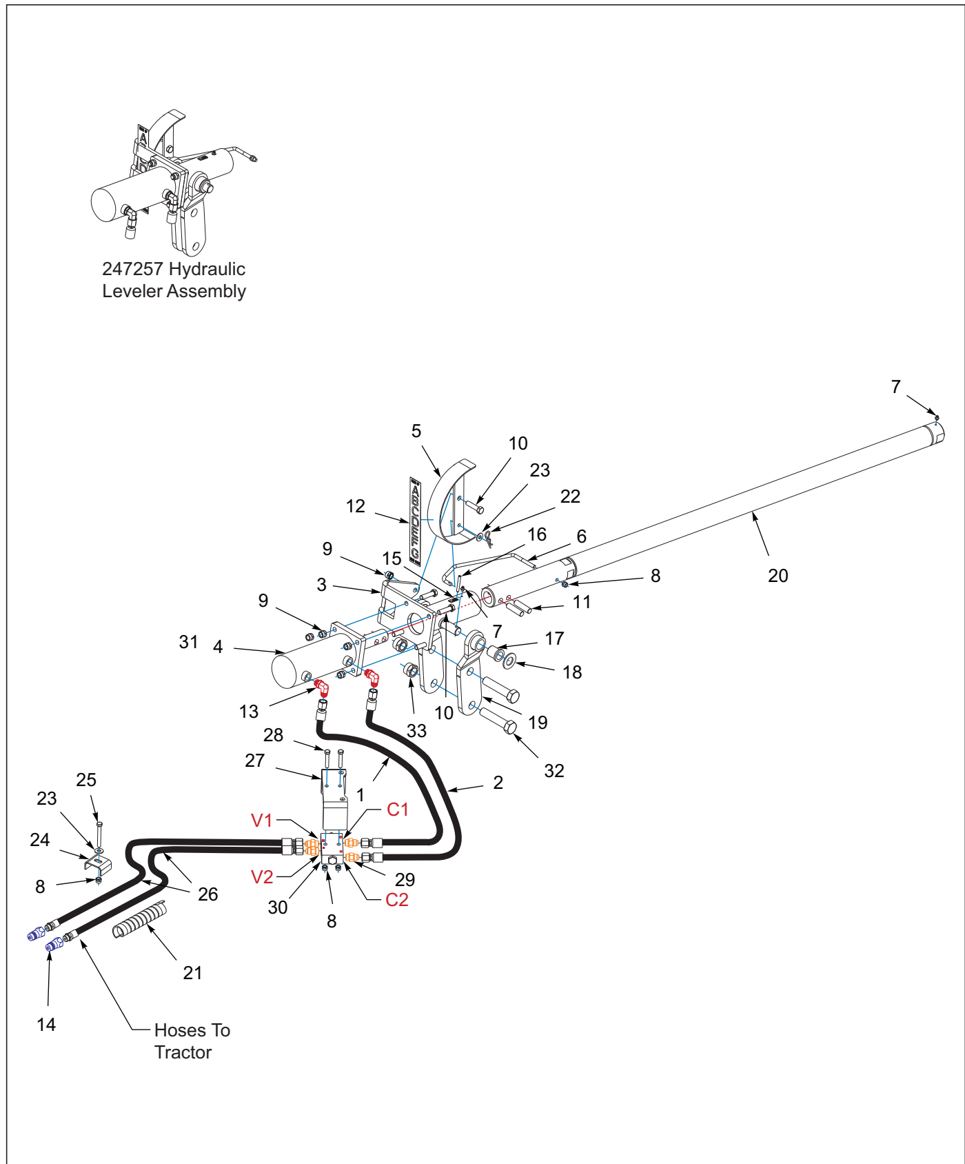
Figure 2-8: Leveler Assembly Hydraulic (After 01-01-2024)
