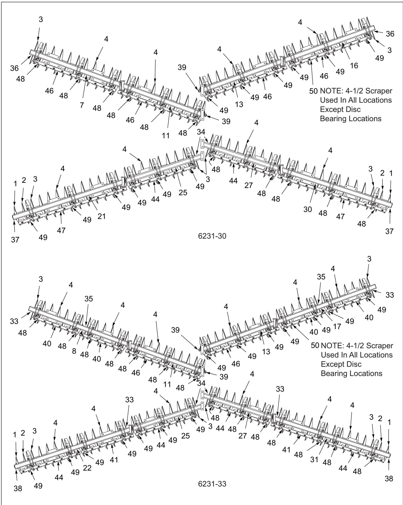
Figure 3-29: Disc Gang Assembly 6231 26" 8-3/4SP 4 GA (3 of 4)
