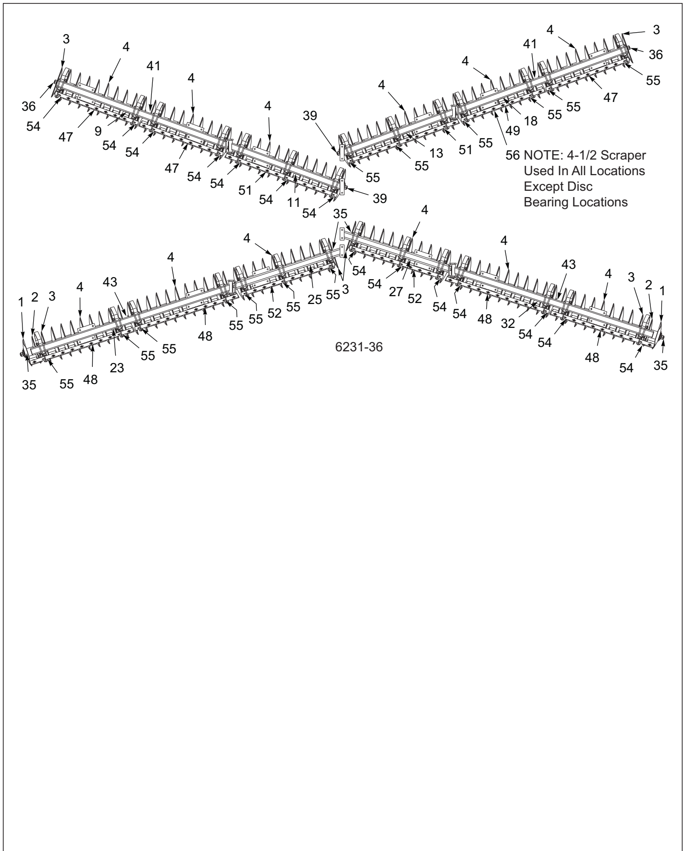
Figure 3-10: Disc Gang Assembly 6231 24" 7SP 4 GA (Non-Rollable) (4 of 4)
