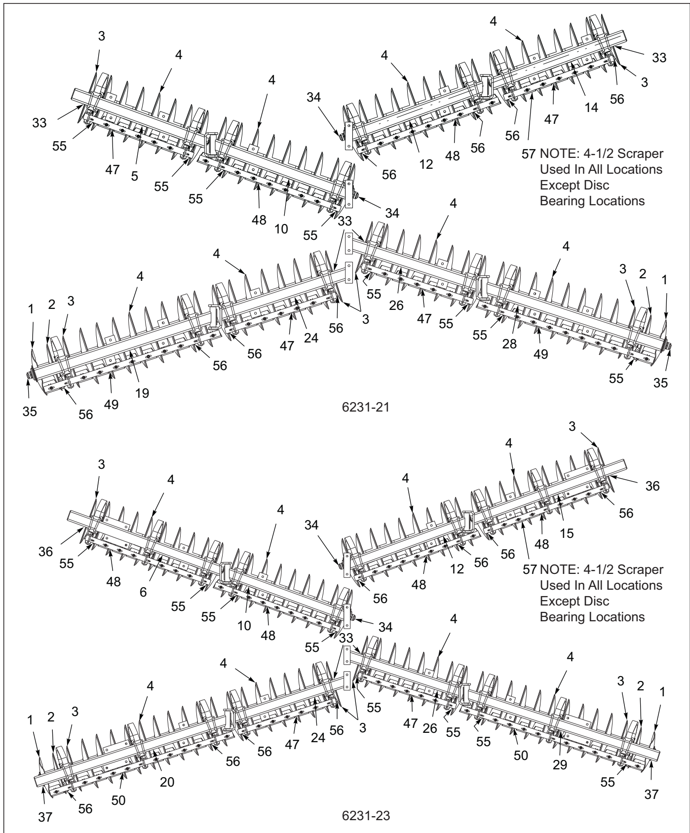
Figure 3-2: Disc Gang Assembly 6231 24" 7SP Rollable 4 GA (1 of 4)
