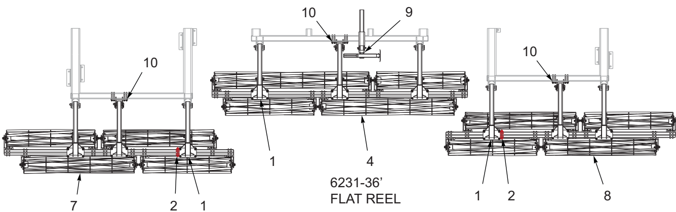
6231-36' - 135"/135" FLAT REEL
