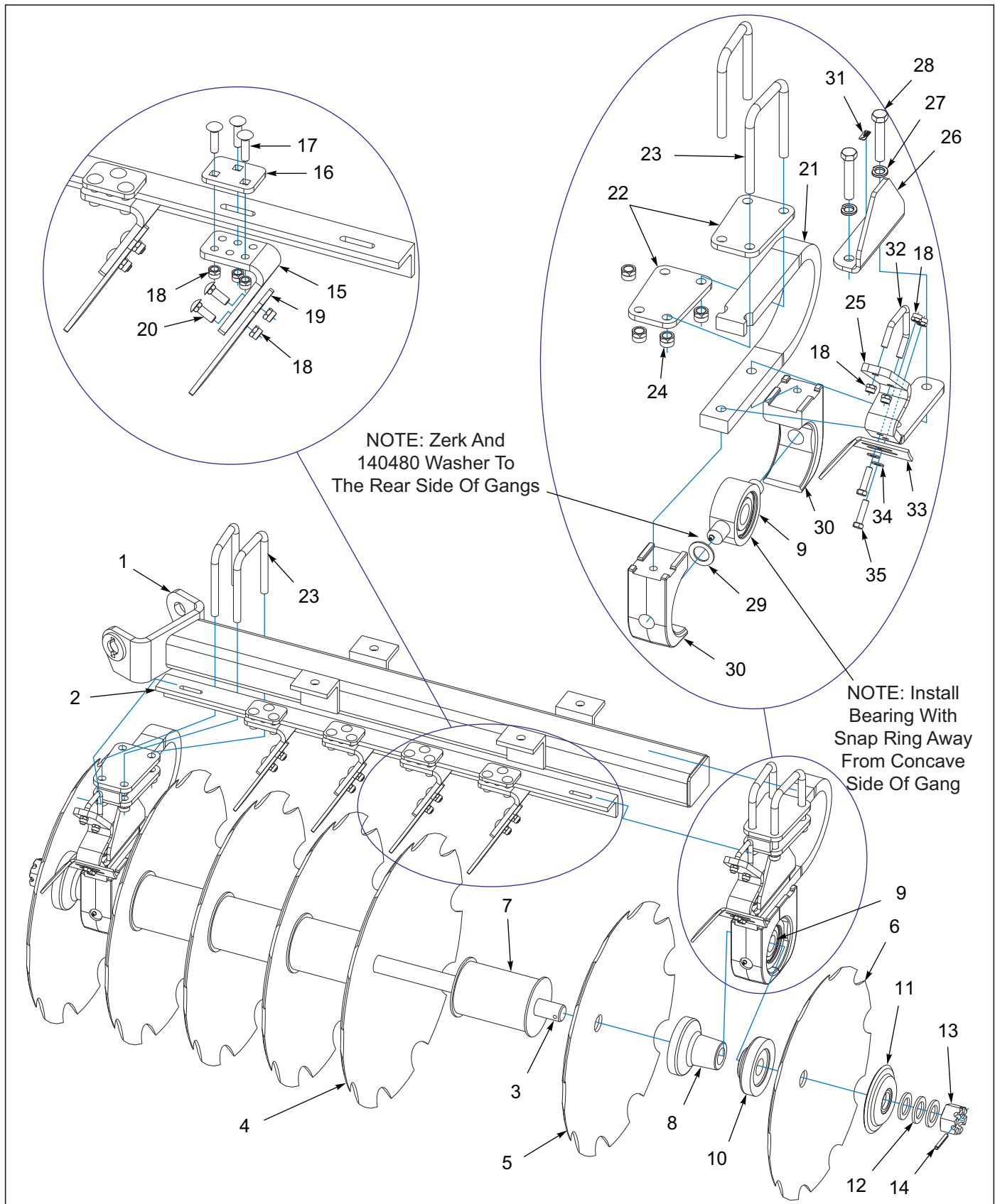
Figure 3-41: Disc Gang Assembly 28" 8-3/4SP NF 5/16" (Notched Front)
