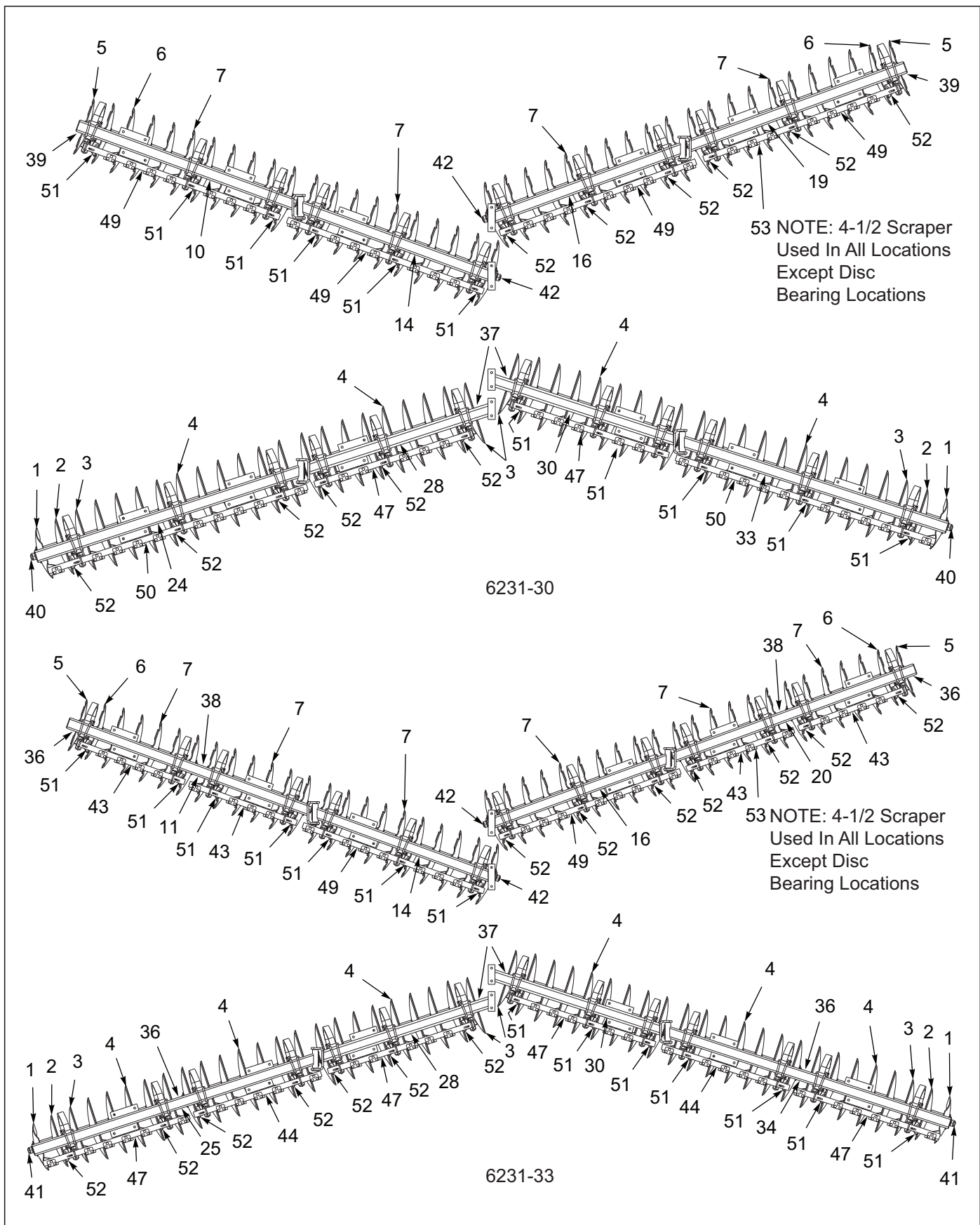
Figure 3-44: Disc Gang Assembly 6231 28' 8-3/4SP NF 5/16" (Notched Front) (3 of 4)
