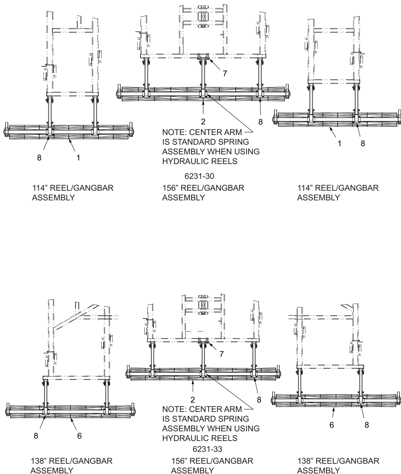
Figure 8-10: Conditioner Reel Layout 6231-30-33
