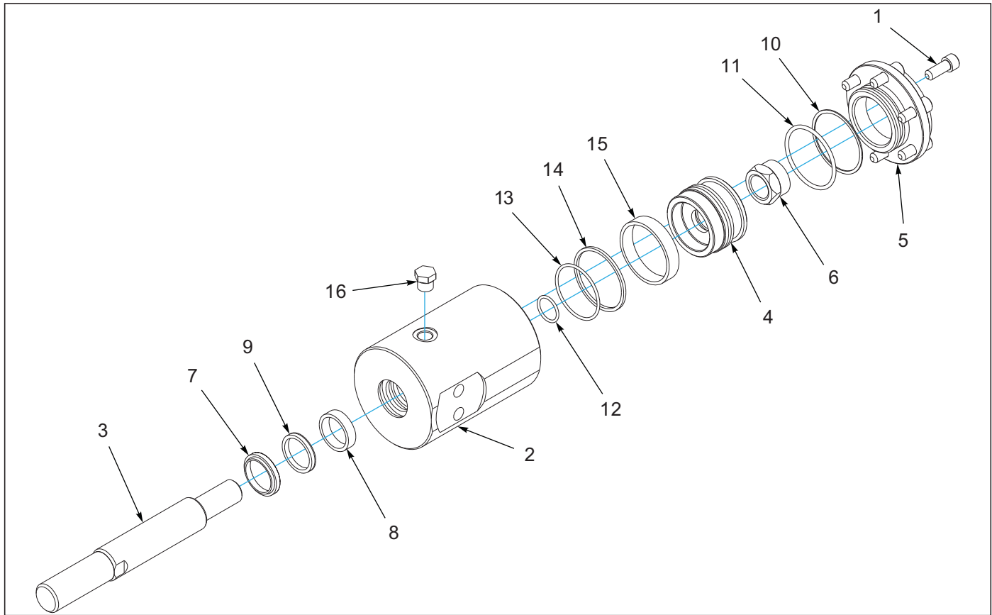
Figure 5-10: Cylinder Assembly 2-1/2 x 2-1/2 1-1/8 Threads
