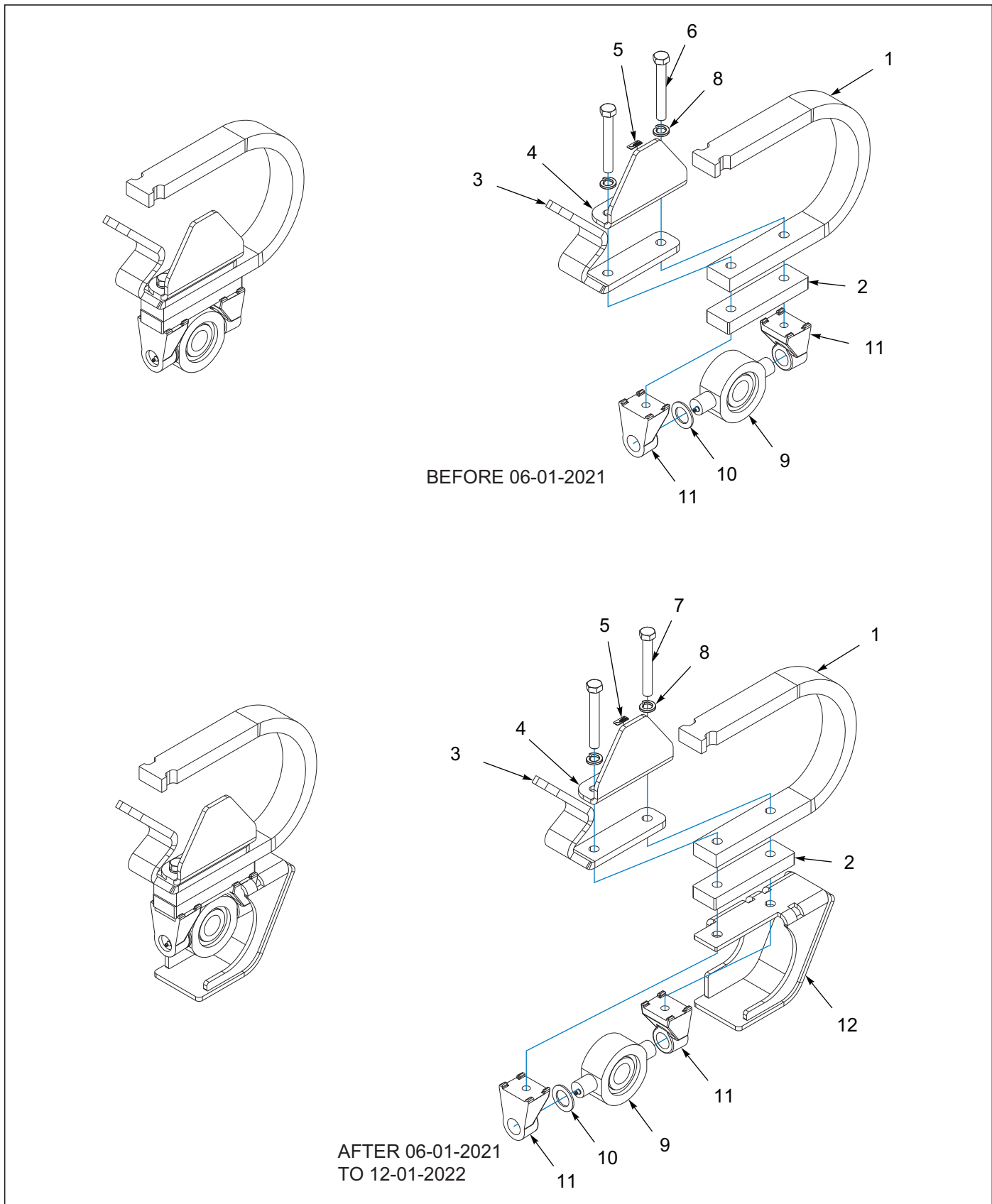
Figure 3-47: Shank & Bearing Assembly 28" NF Before 12-01-2022
