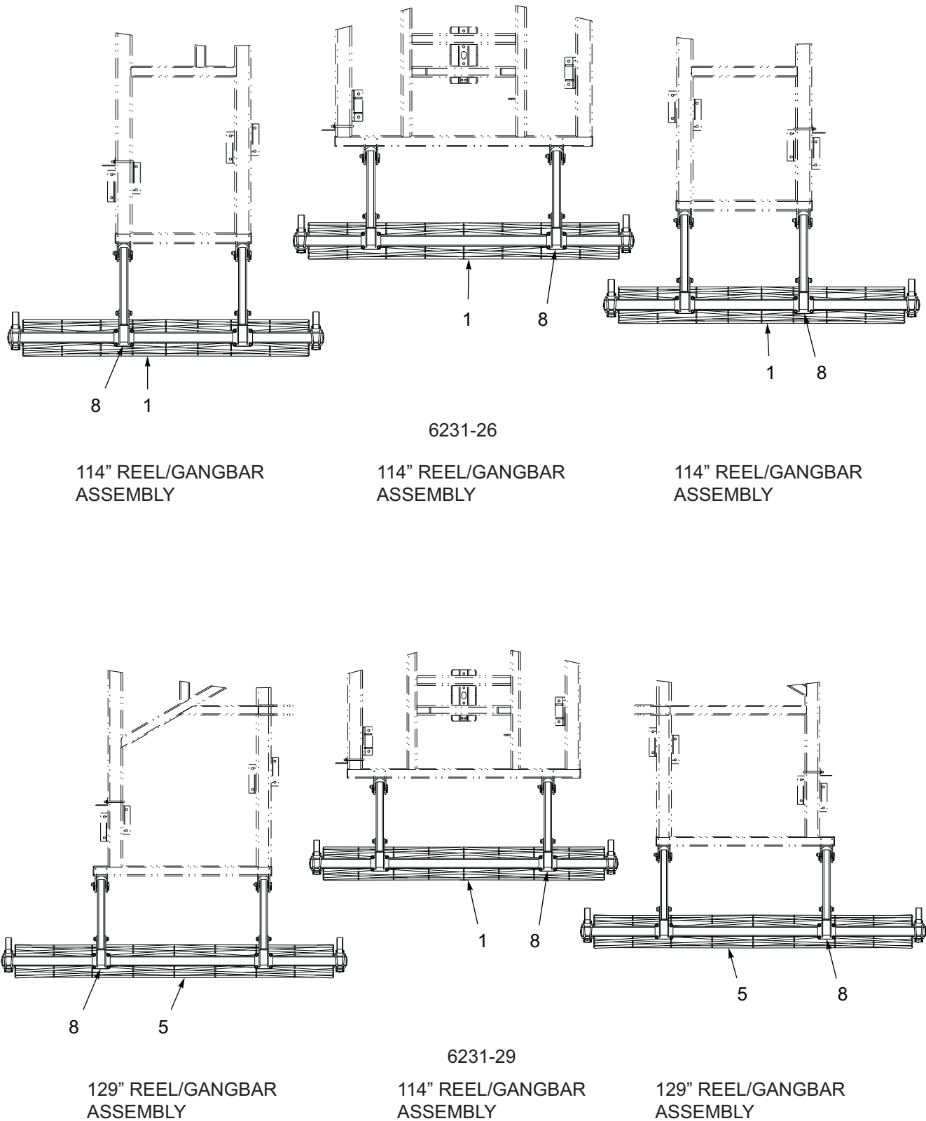
Figure 8-9: Conditioner Reel Layout 6231-26-29
