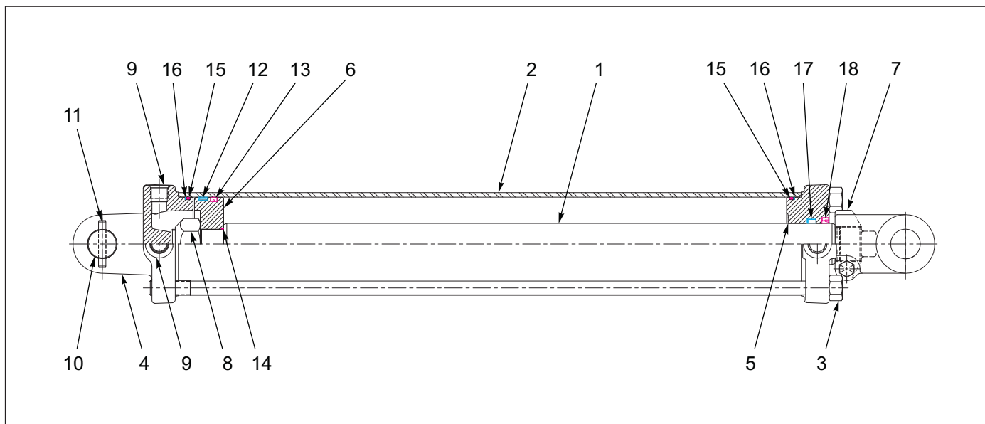
Figure 5-7: Cylinder Assembly 4-1/2 x 30
