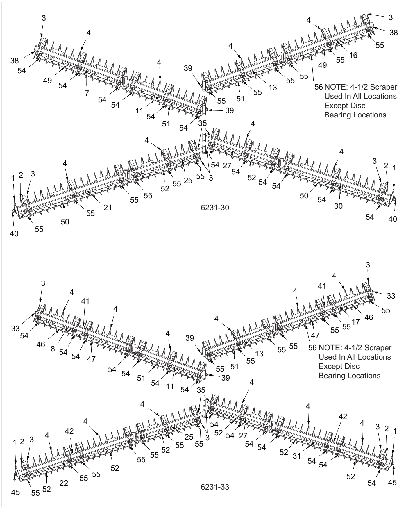
Figure 3-9: Disc Gang Assembly 6231 24" 7SP 4 GA (Non-Rollable) (3 of 4)
