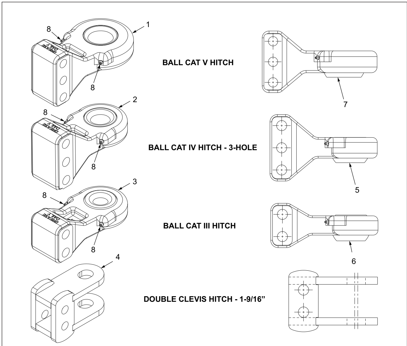
Figure 2-9: Hitch Assemblies
