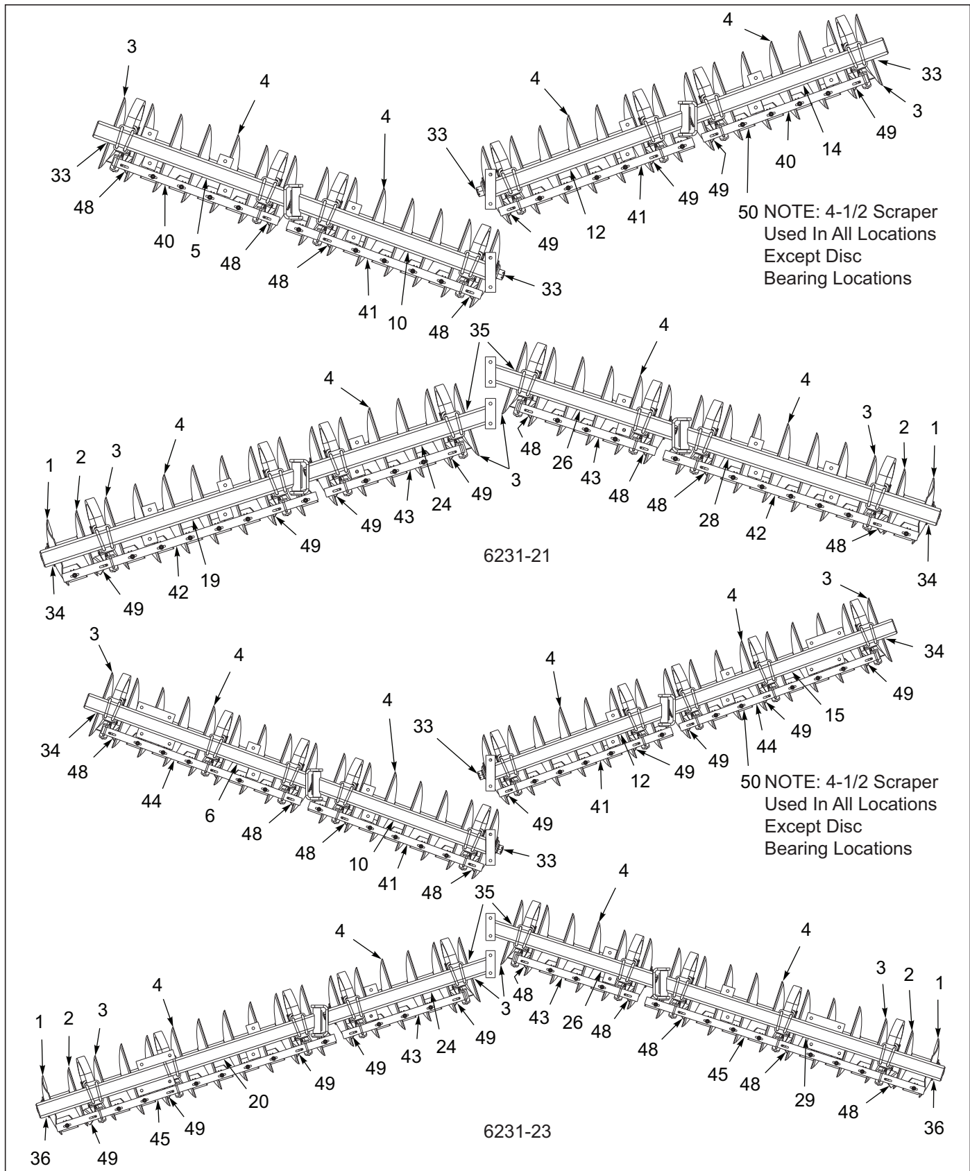
Figure 3-17: Disc Gang Assembly 6231 24" 8-3/4SP 4 GA (Non-Rollable) (1 of 4)
