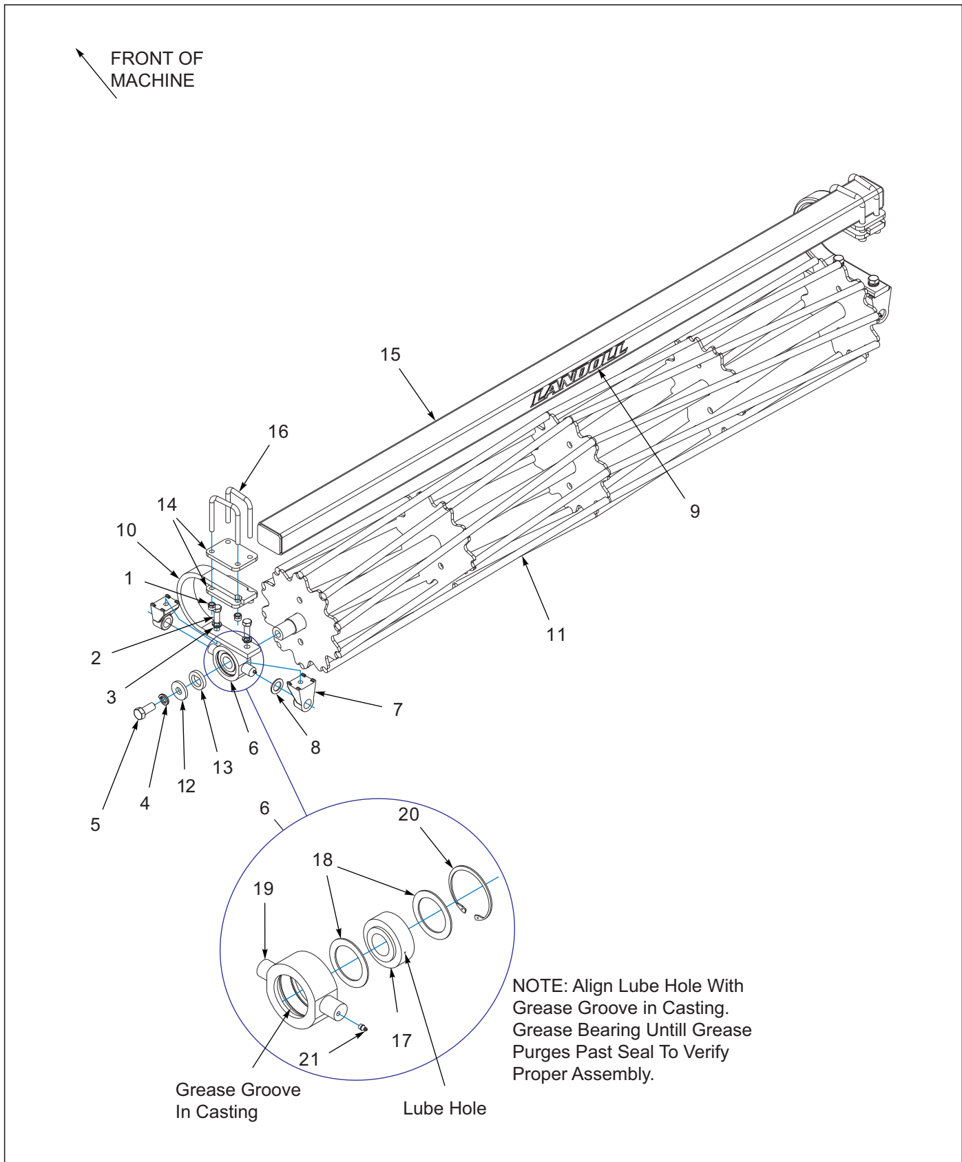
Figure 8-14: Conditioner Reel/Gangbar Assembly
