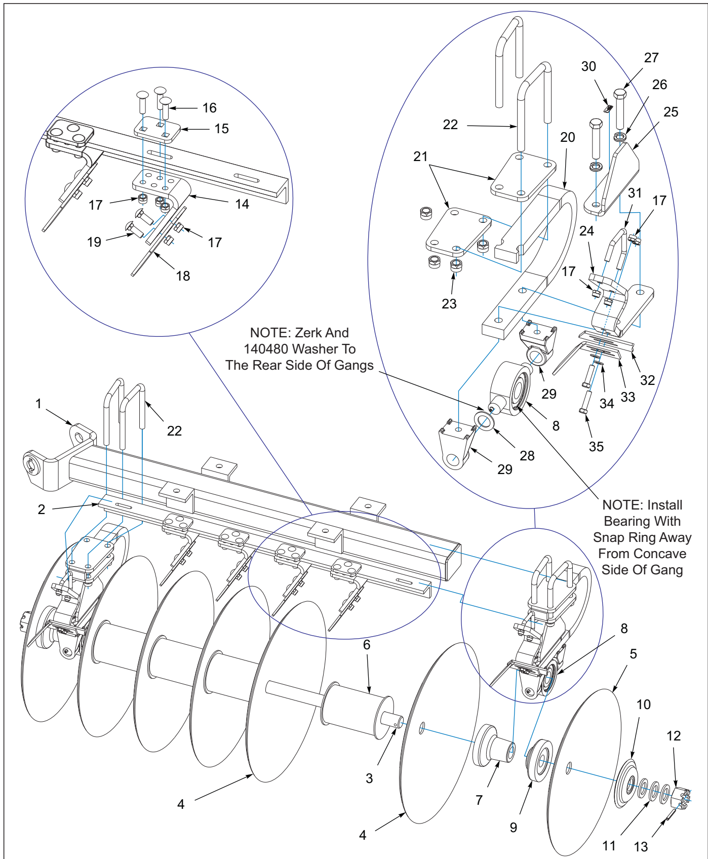
Figure 3-31: Disc Gang Assembly 26" 8-3/4SP HDS 4 GA (Heavy Duty Scraper)
