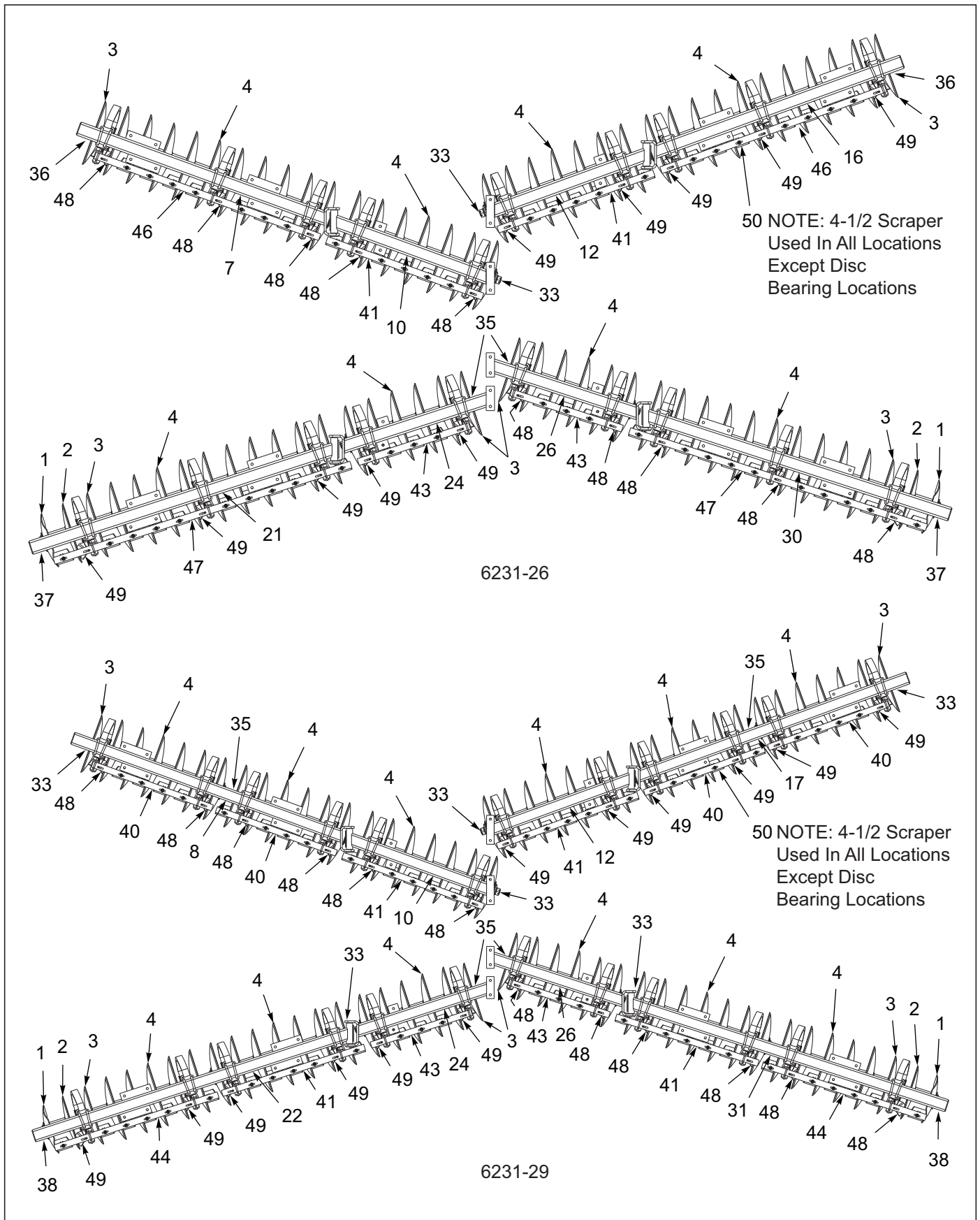
Figure 3-28: Disc Gang Assembly 6231 26" 8-3/4SP 4 GA (2 of 4)
