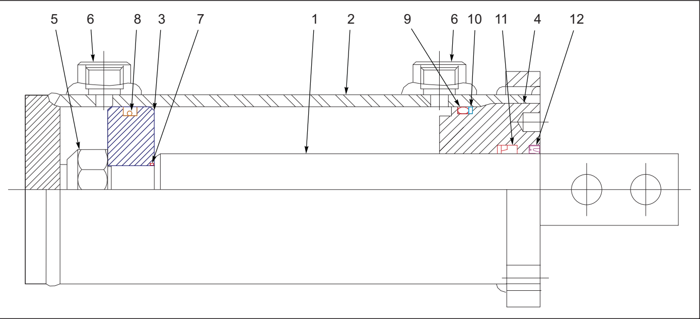
Figure 5-8: Cylinder Assembly 3-1/2 x 6
