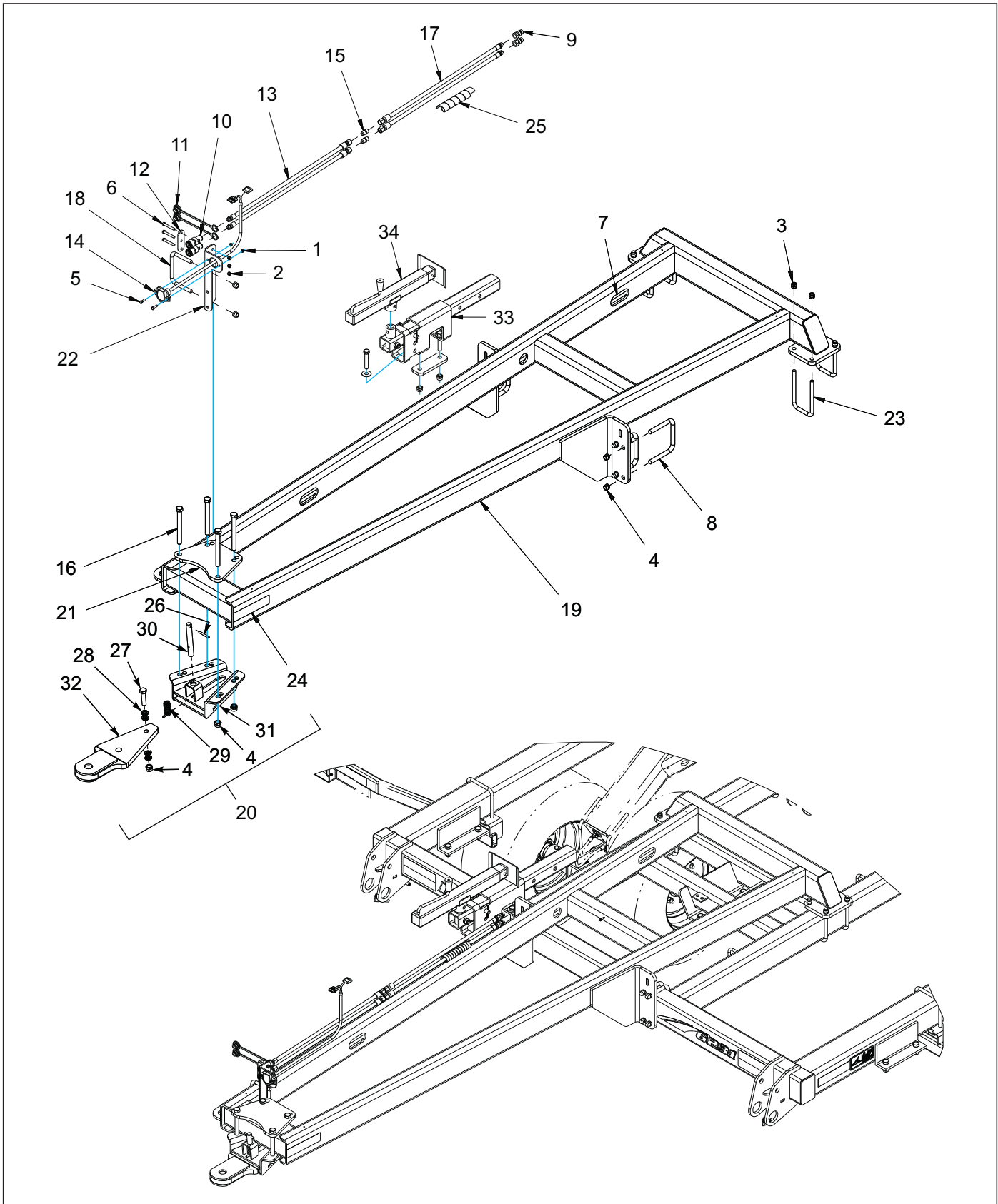
Figure 8-44: Rear Hitch Assembly Long
