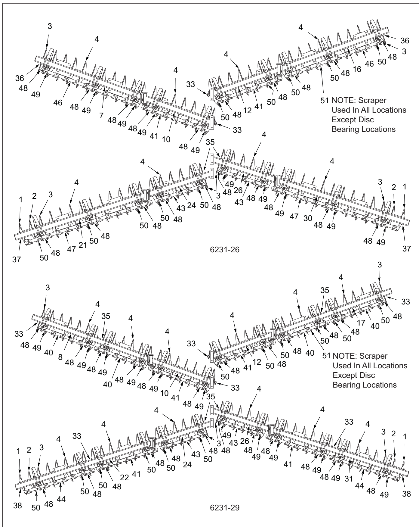
Figure 3-23: Disc Gang Assembly 6231 24" 8-3/4SP HDS 4 GA (Heavy Duty Scraper) (2 of 4)
