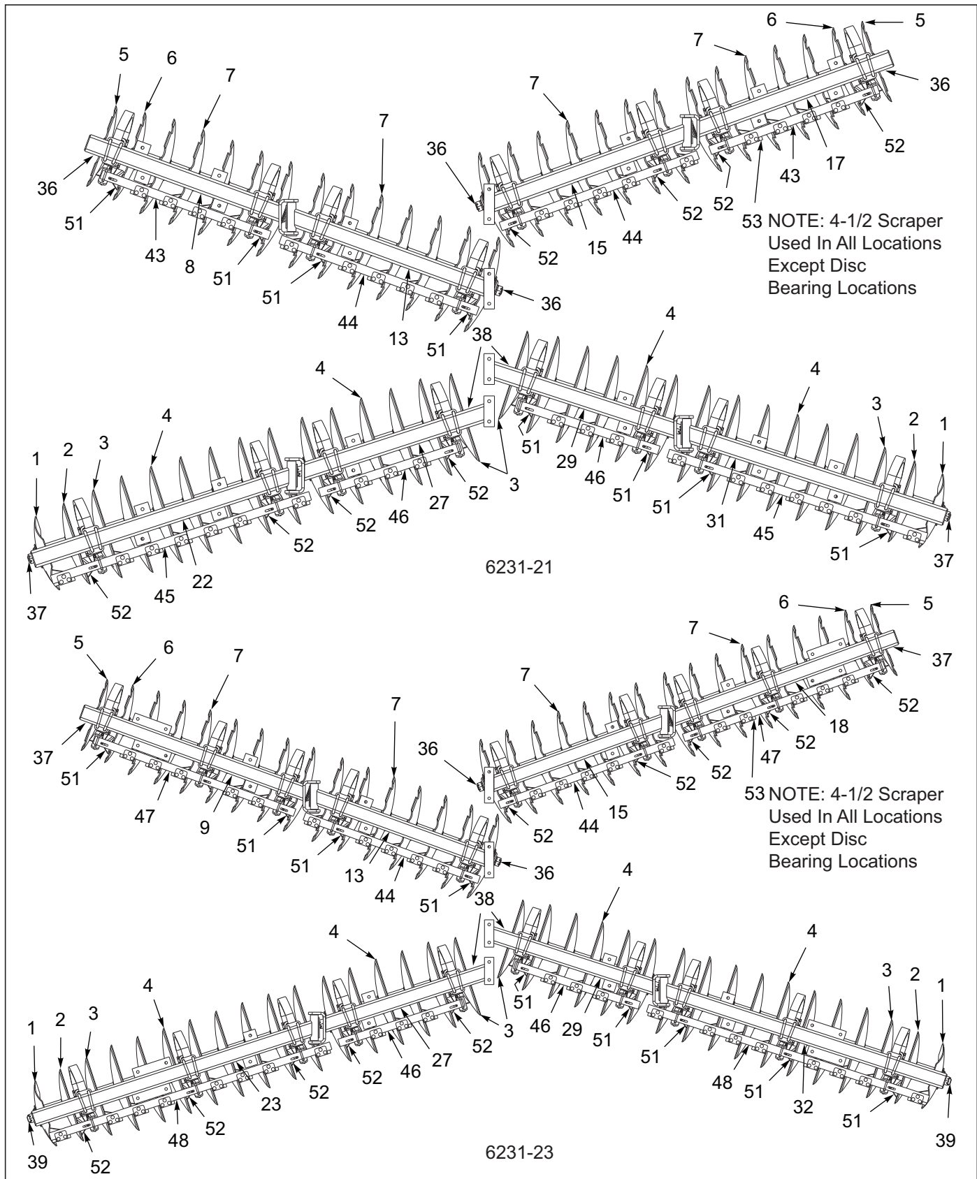
Figure 3-42: Disc Gang Assembly 6231 28" 8-3/4SP NF 5/16"(Notched Front) (1 of 4)
