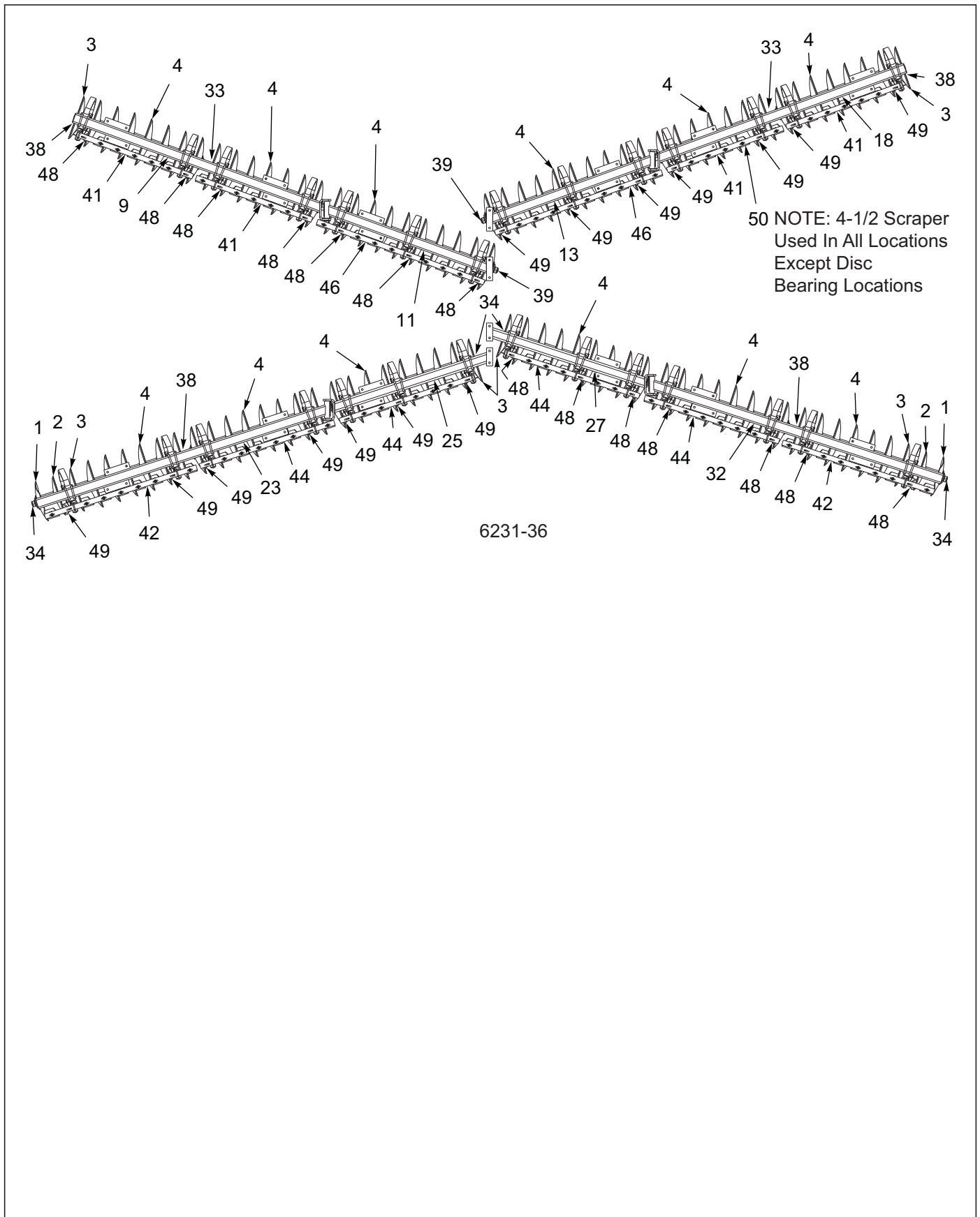
Figure 3-15: Disc Gang Assembly 6231 24" 8-3/4SP Rollable 4 GA (4 of 4)
