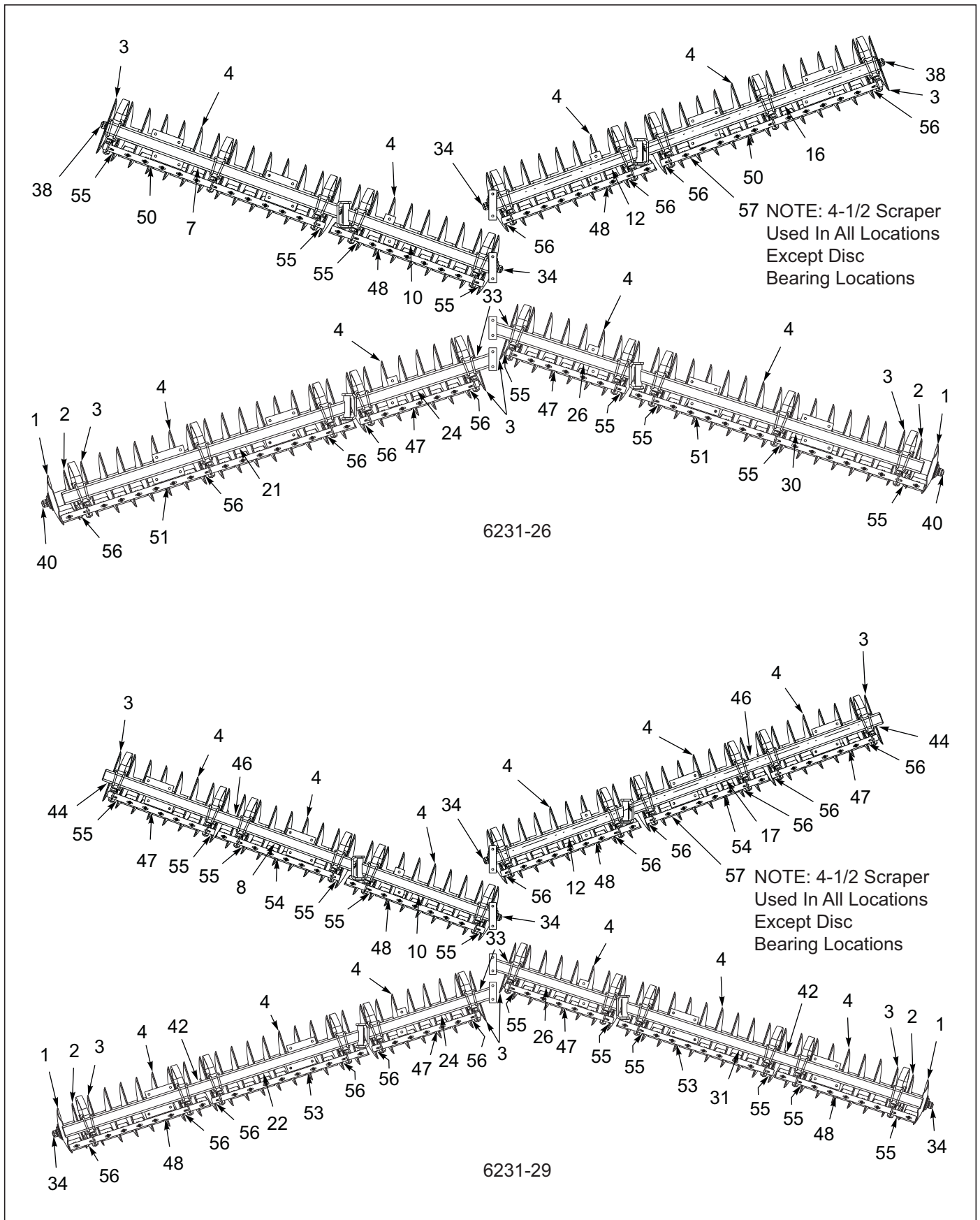
Figure 3-3: Disc Gang Assembly 6231 24" 7SP Rollable 4 GA (2 of 4)
