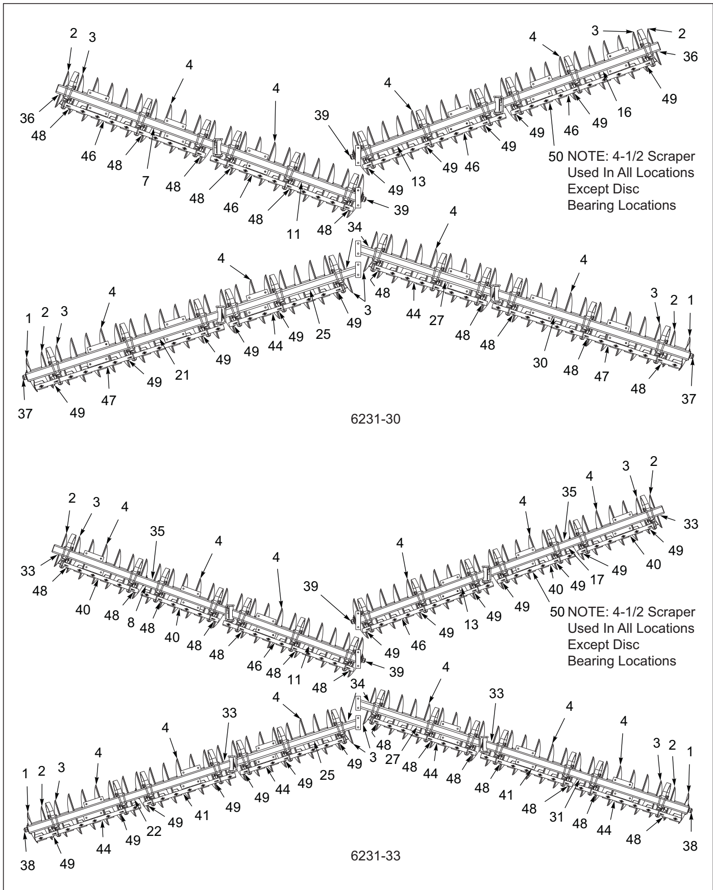
Figure 3-39: Disc Gang Assembly 6231 26" 8-3/4SP 5/16" (3 of 4)
