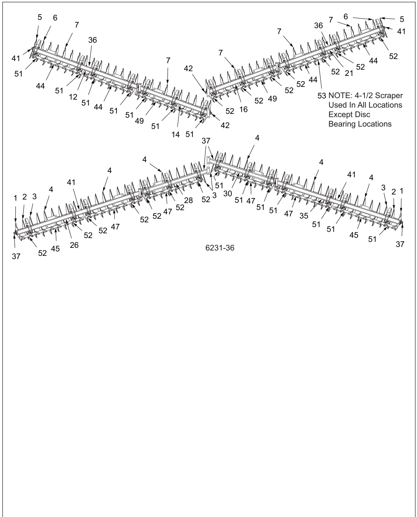
Figure 3-45: Disc Gang Assembly 6231 28" 8-3/4SP NF 5/16" (Notched Front) (4 of 4)
