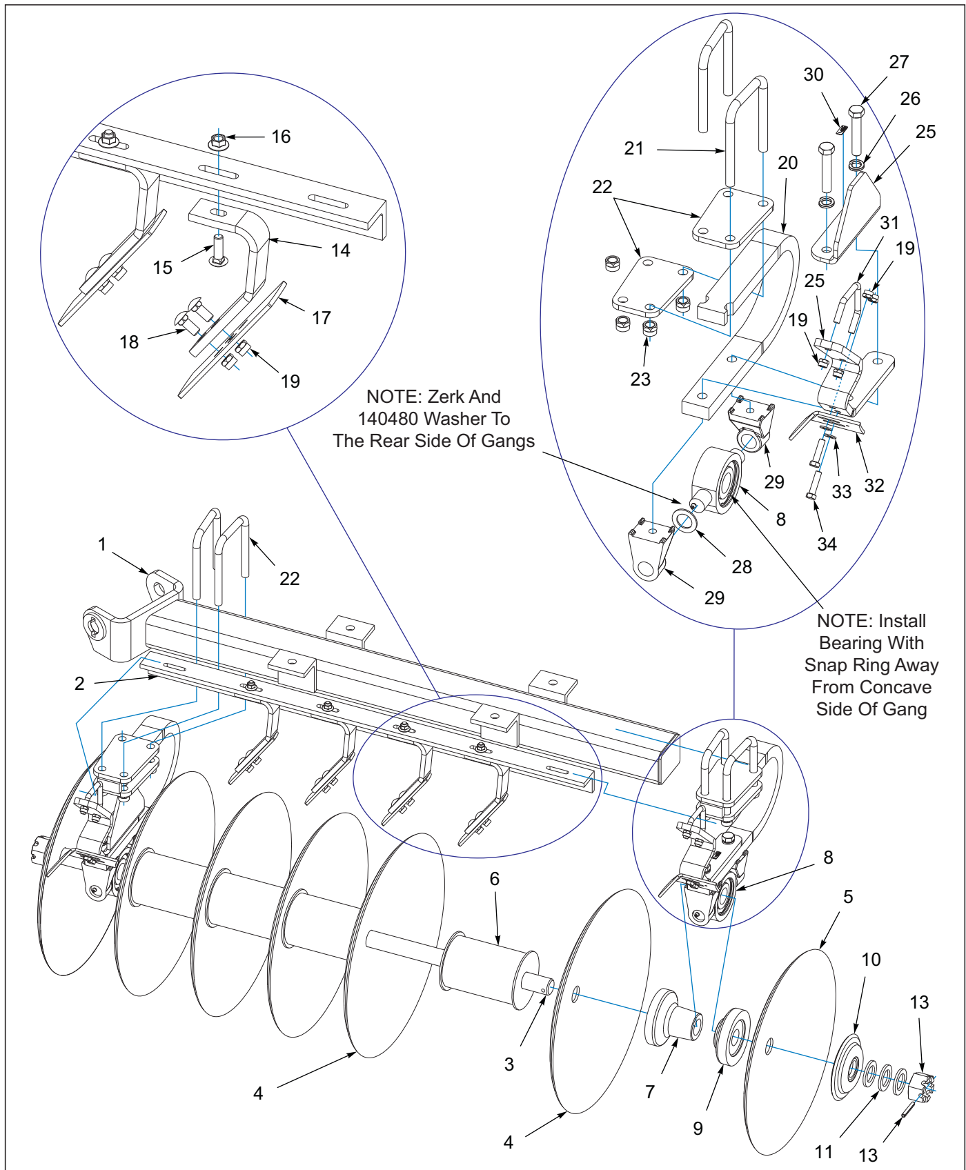
Figure 3-36: Disc Gang Assembly 26" 8-3/4SP 5/16"
