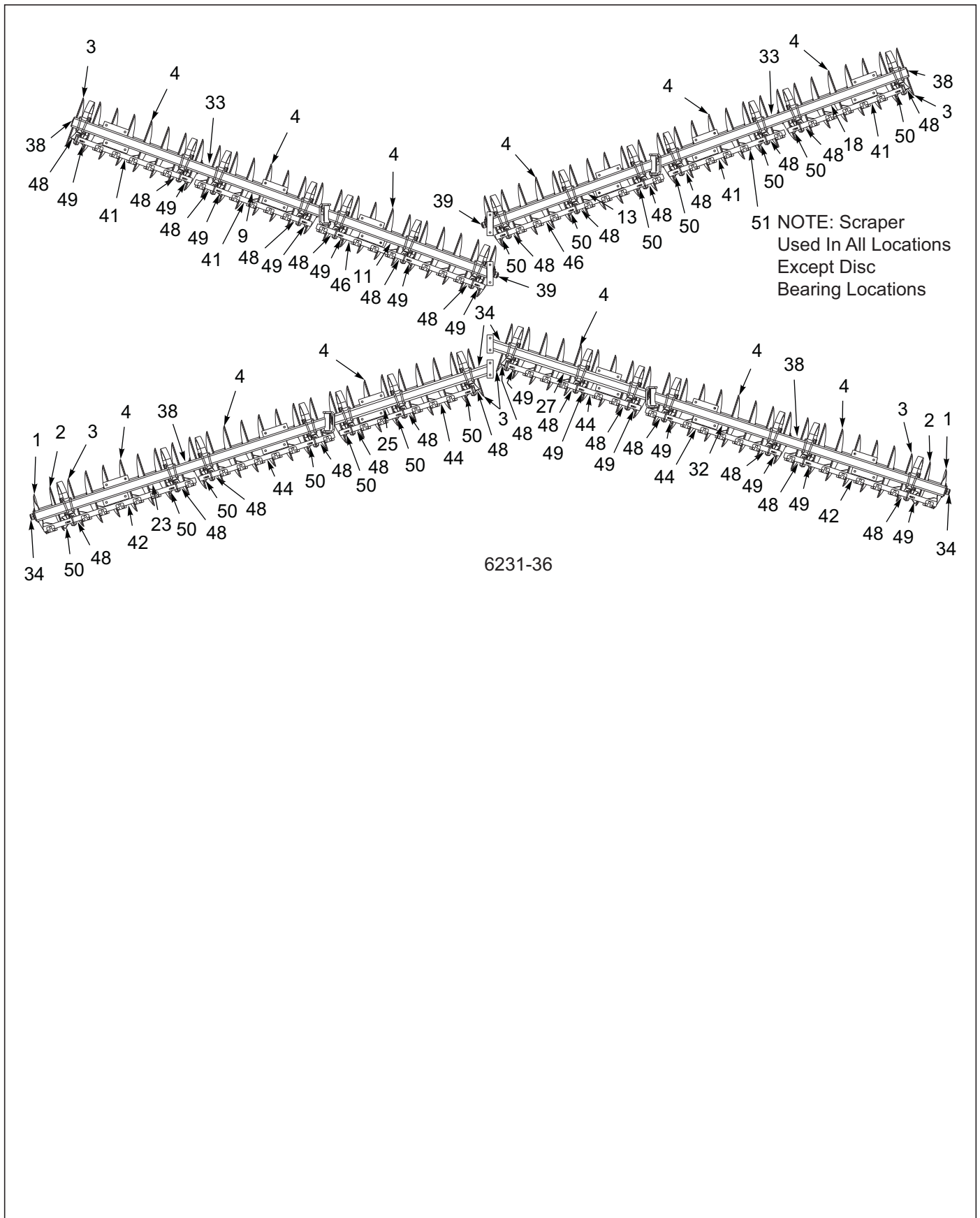
Figure 3-35: Disc Gang Assembly 6231 26" 8-3/4SP HDS 4 GA (Heavy Duty Scraper) (4 of 4)
