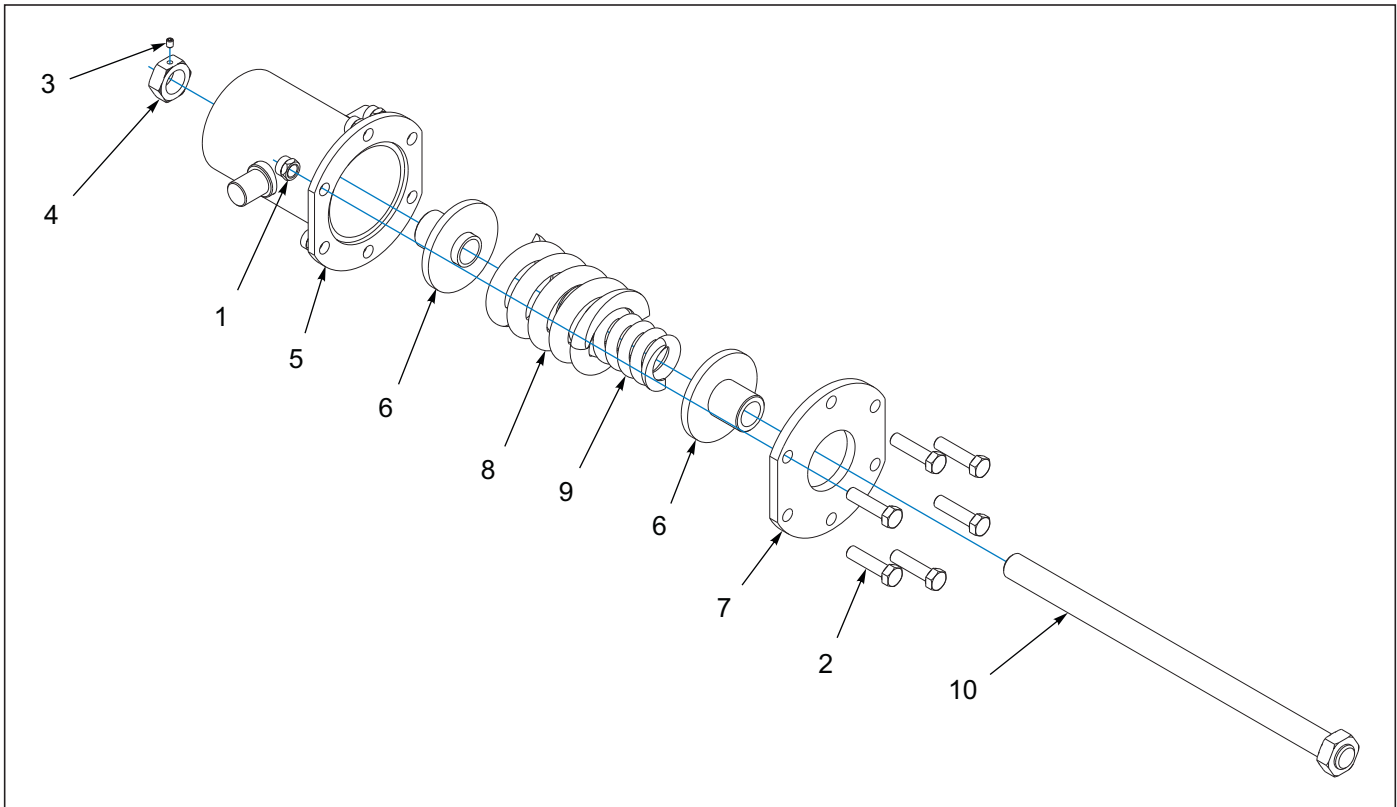
Figure 2-3: Leveler Spring Tube Assembly
