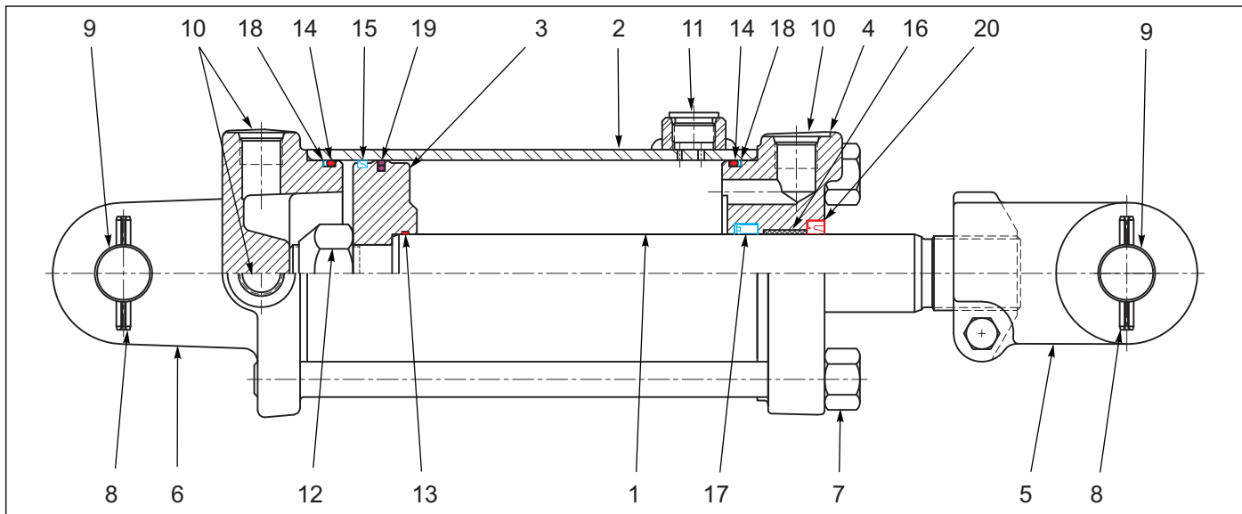
Figure 5-5: Cylinder Assembly 3-3/4 x 10, Rephase
