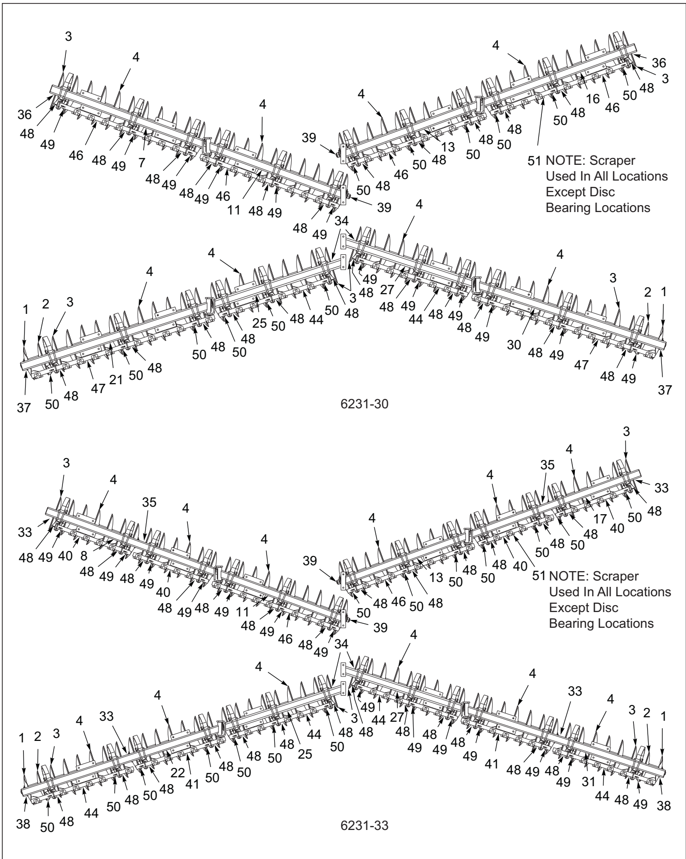
Figure 3-24: Disc Gang Assembly 6231 24" 8-3/4SP HDS 4 GA (Heavy Duty Scraper) (3 of 4)
