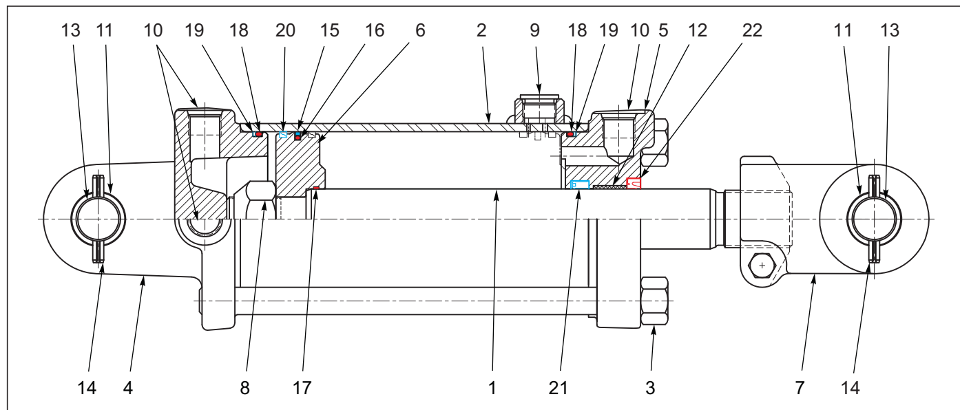
Figure 5-6: Cylinder Assembly 3-3/4, x 10, Rephase
