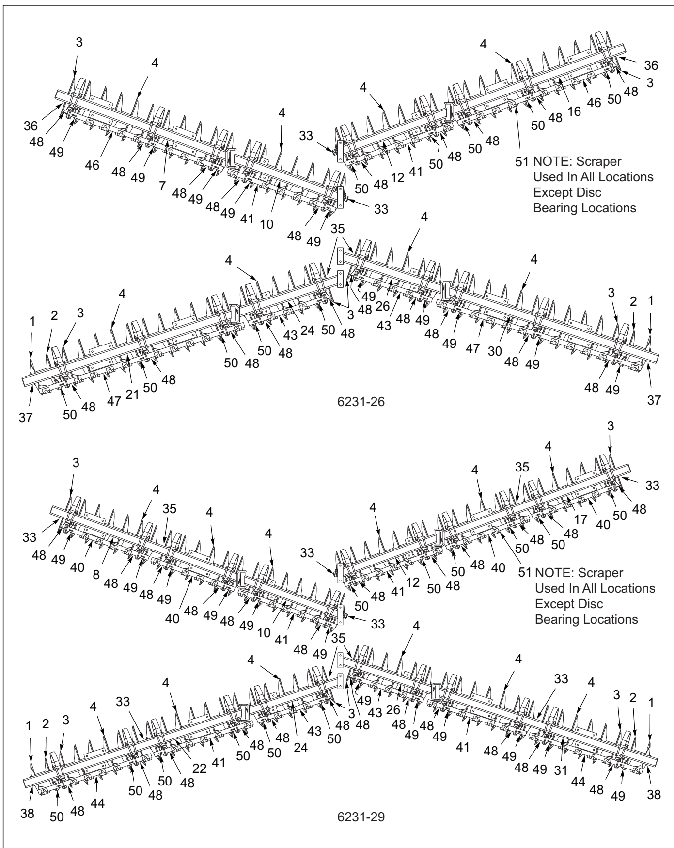
Figure 3-33: Disc Gang Assembly 6231 26" 8-3/4SP HDS 4 GA (Heavy Duty Scraper) (2 of 4)
