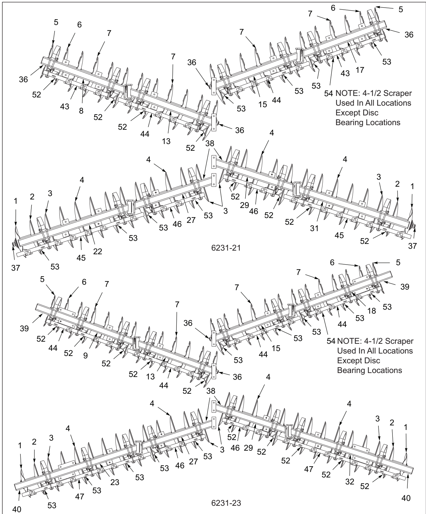
Figure 3-48: Disc Gang Assembly 6231 28" 10-1/2SP NF 5/16" (Notched Front)(1 of 4)
