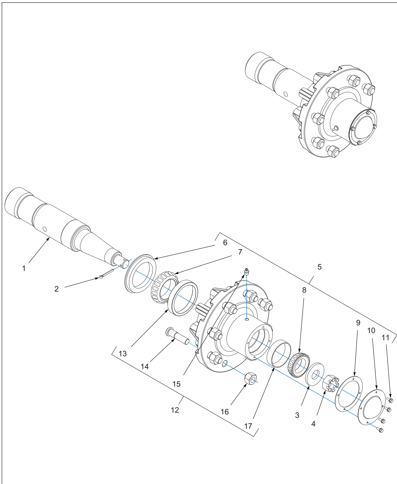
Figure 1-10: Hub/Spindle Assembly 223440
