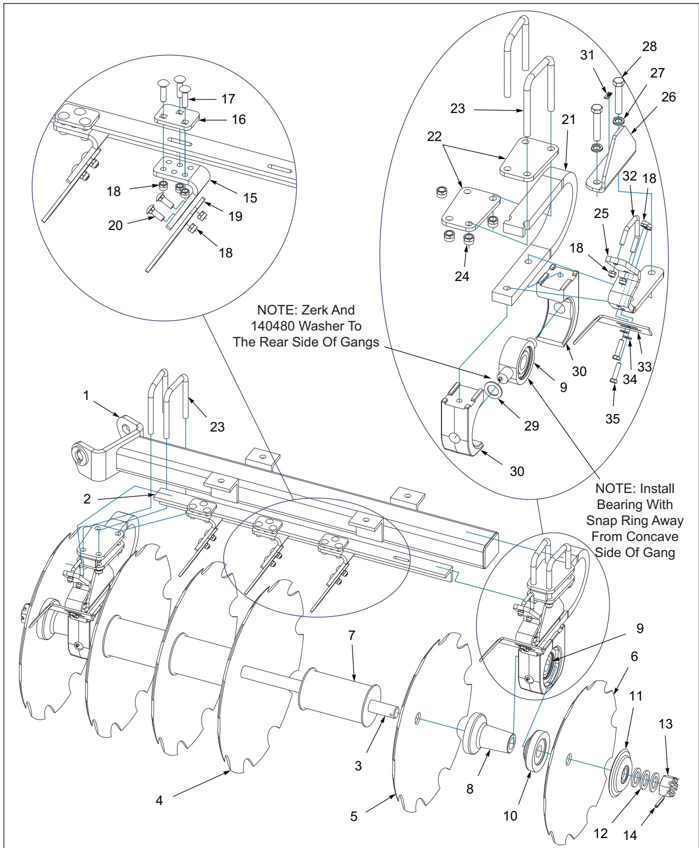
Figure 3-46: Disc Gang Assembly 28" 10-1/2SP NF 5/16" (Notched Front)
