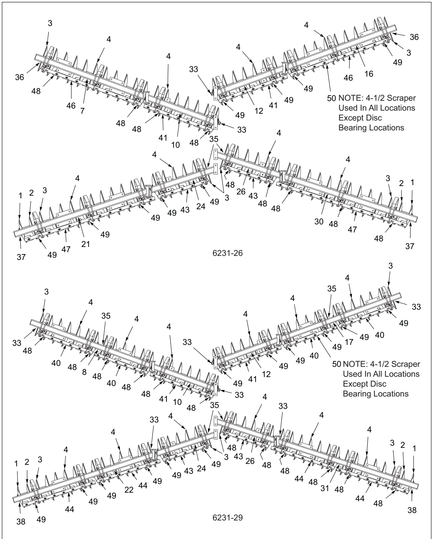
Figure 3-13: Disc Gang Assembly 6231 24" 8-3/4SP Rollable 4 GA (2 of 4)
