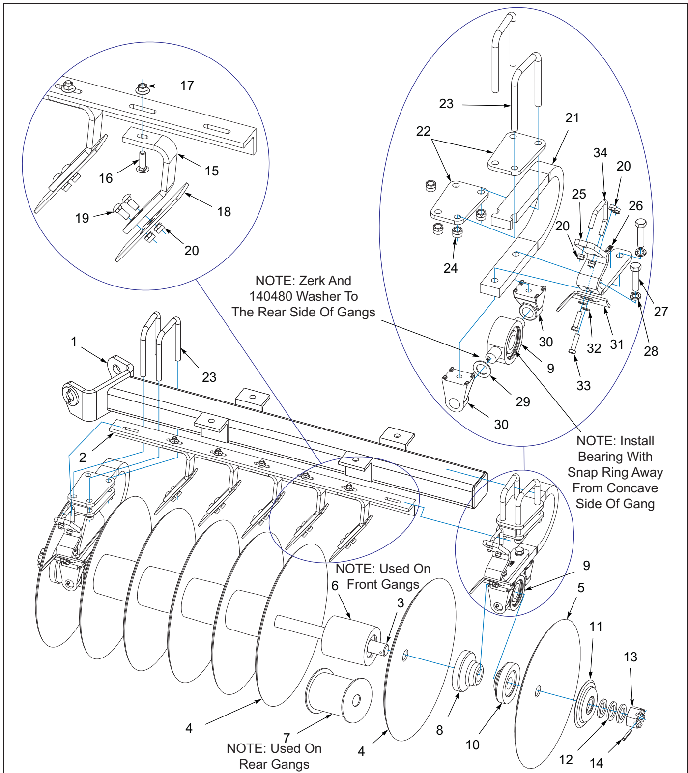
Figure 3-1: Disc Gang Assembly 24" 7SP Rollable 4 GA
