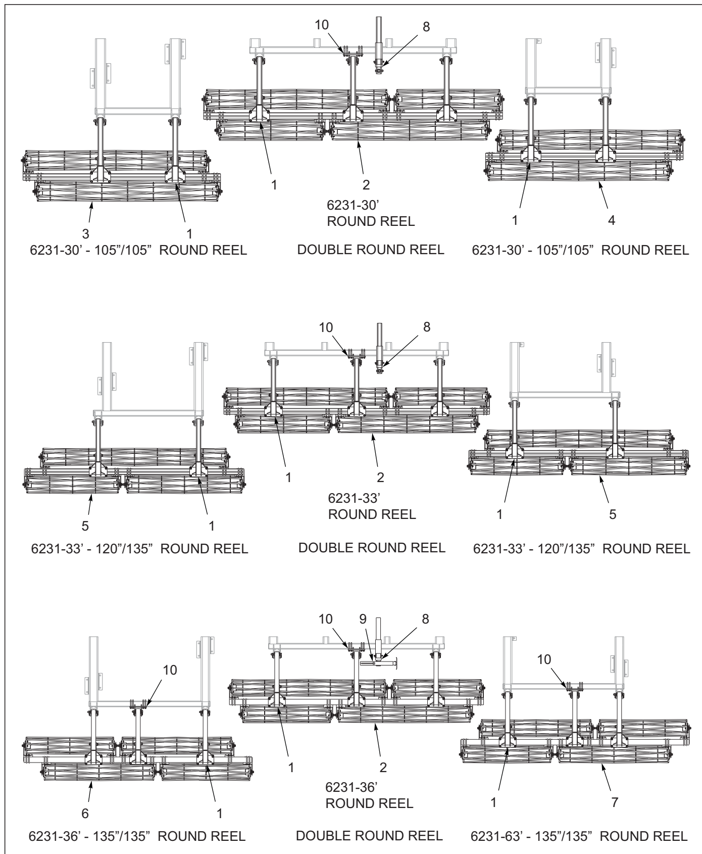
Figure 8-29: Hydraulic Double Reel Layout 6231-30-33-36
