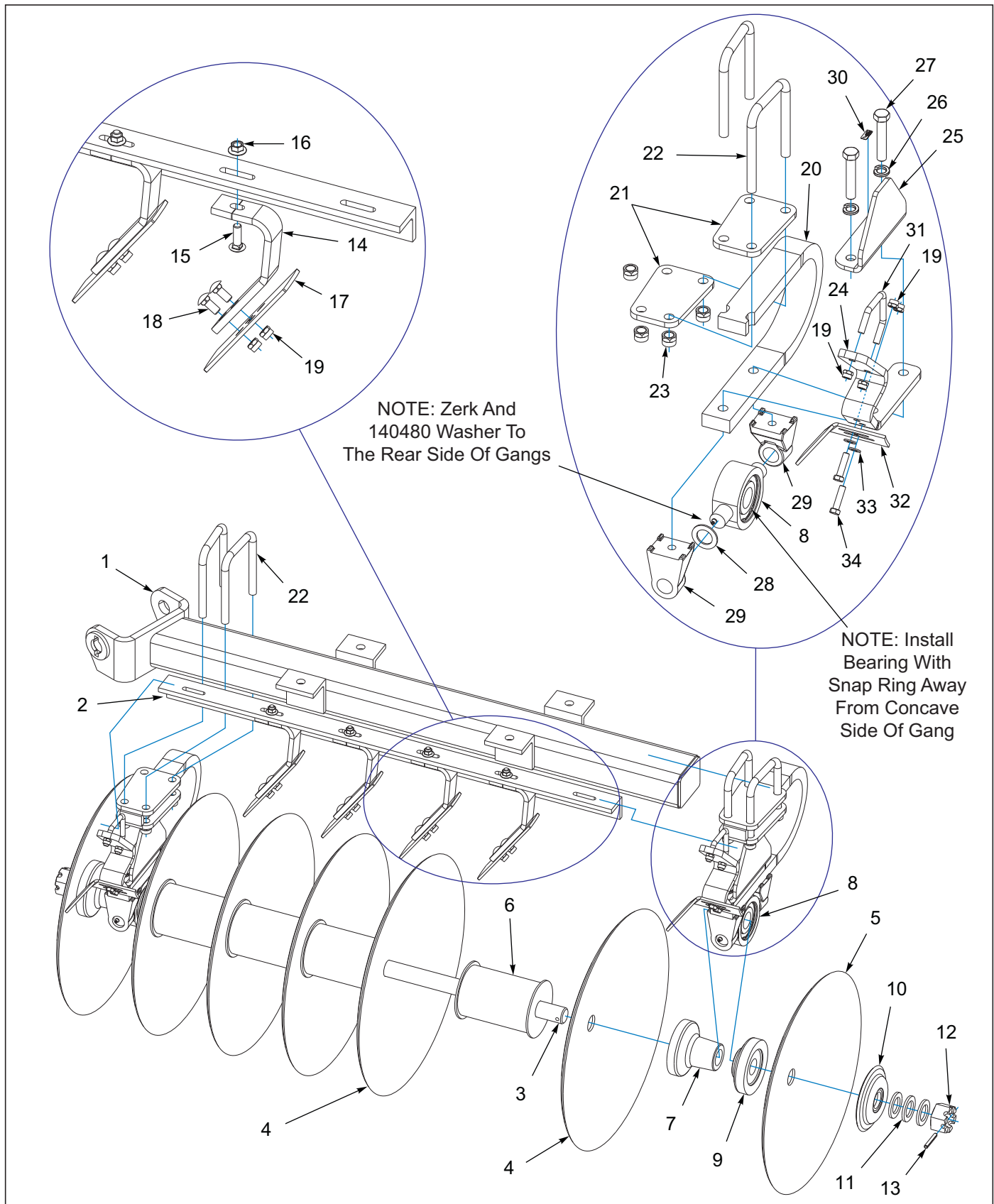
Figure 3-26: Disc Gang Assembly 26" 8-3/4SP 4 GA
