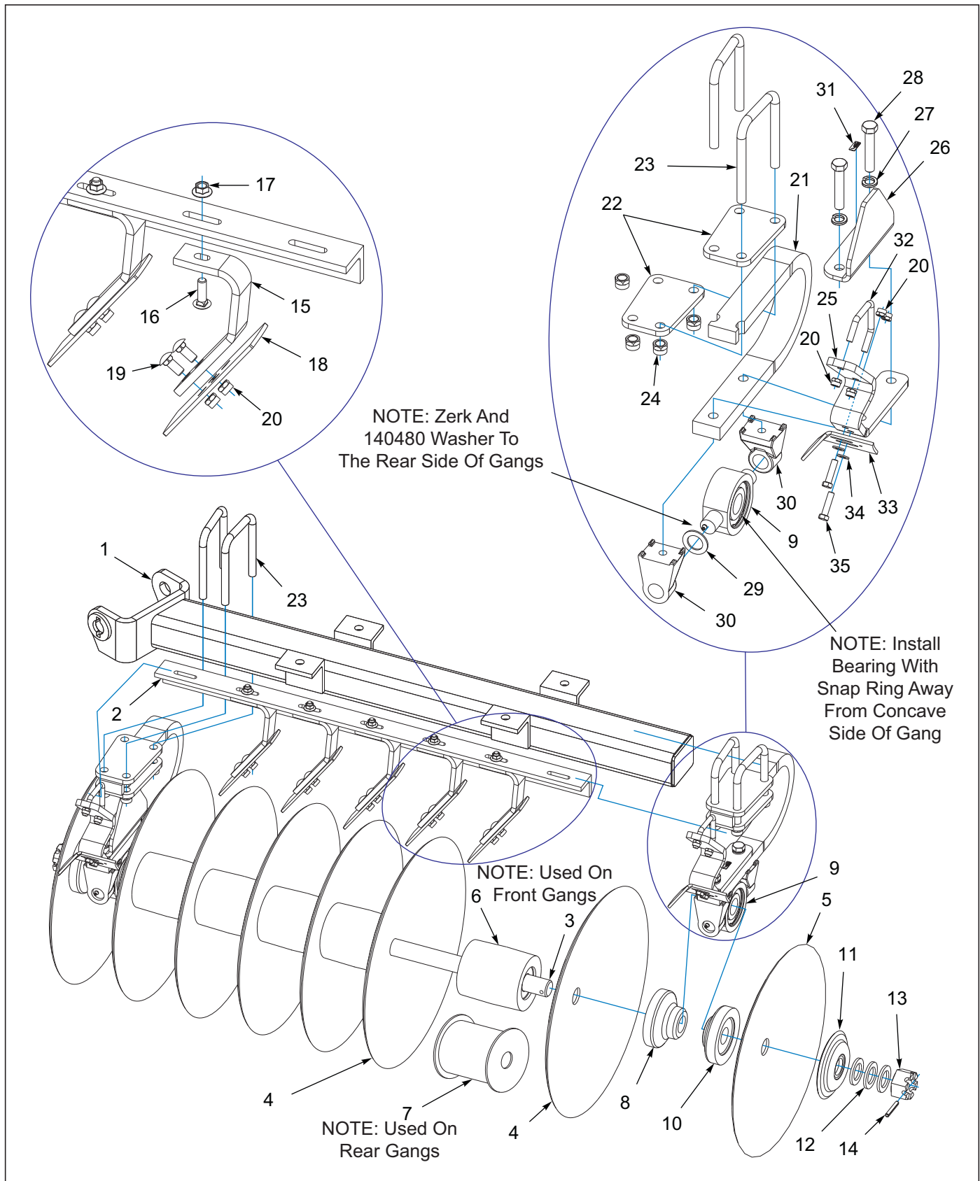
Figure 3-6: Disc Gang Assembly 24" 7SP 4 GA _Non-Rollable)
