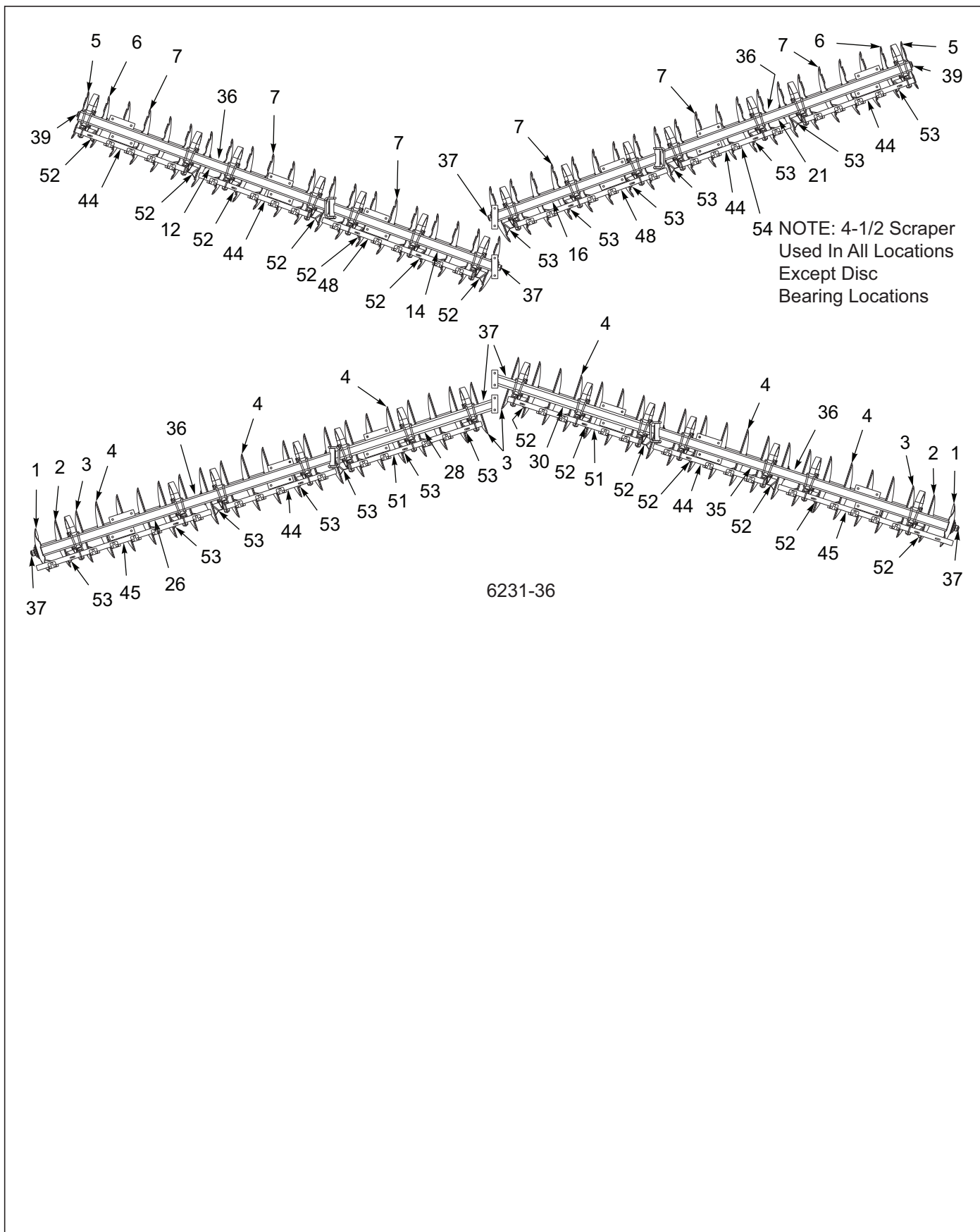
Figure 3-51: Disc Gang Assembly 6231 28" 10-1/2SP NF 5/16" (Notched Front) (4 of 4)
