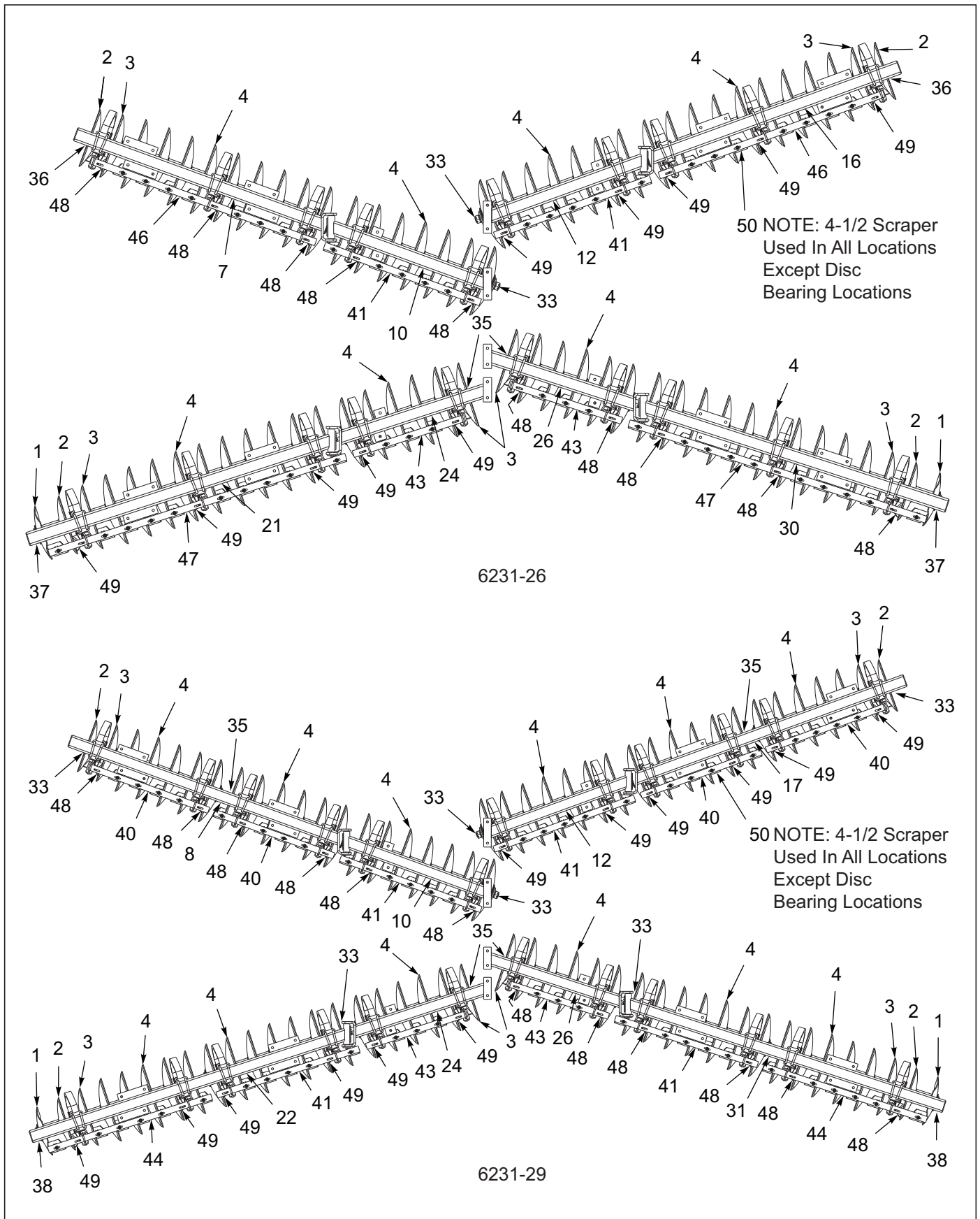
Figure 3-38: Disc Gang Assembly 6231 26" 8-3/4SP 5/16" (2 of 4)
