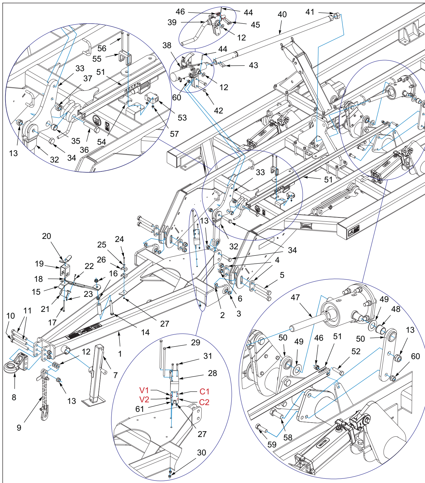
Figure 2-1: Hitch/Leveler Assembly (Before 01-01-2021)
