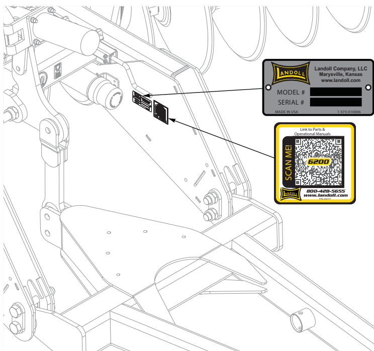
Figure 11-1: Identification Plate and Location
