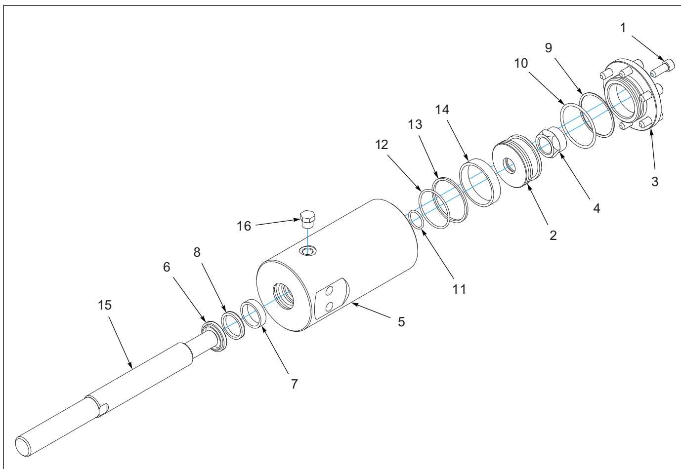
Figure 1-37: Cylinder - 2-1/2" X 3-1/2"
