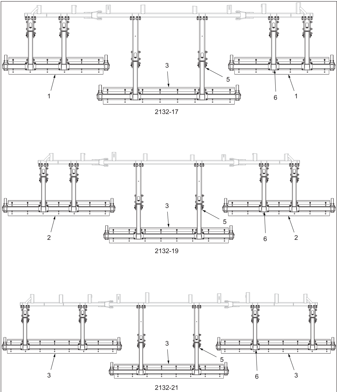
Figure 1-56: Hyd Chopper Reel Layout (1 of 2)
