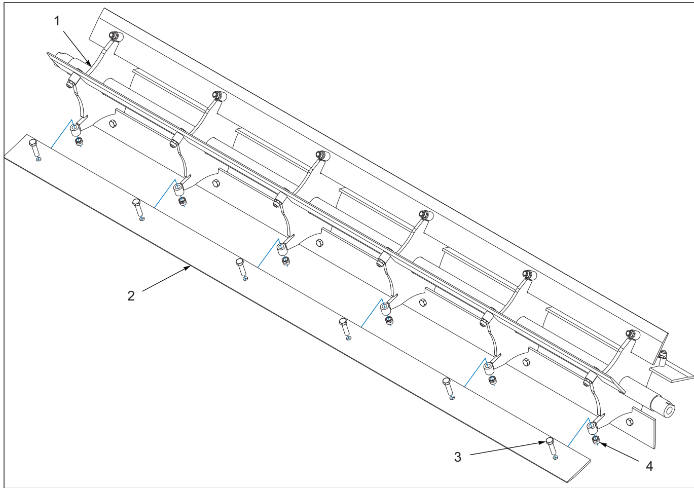
Figure 1-61: Reel Blade Assembly
