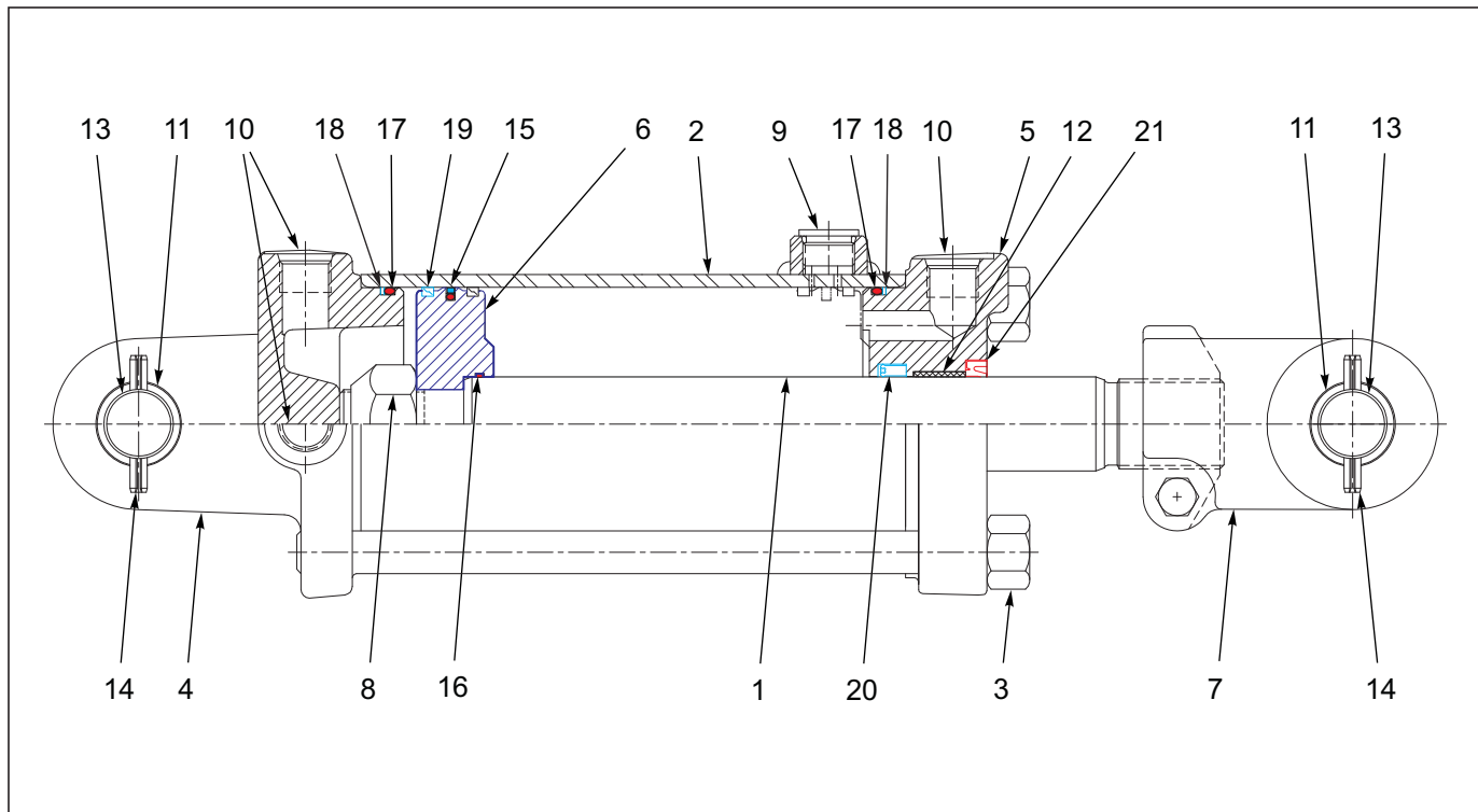
Figure 1-31: Cylinder - Rephase Assembly 3-3/4 X 8
