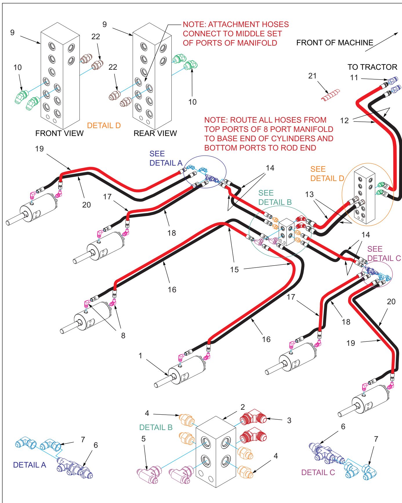
Figure 1-51: 3BCT/Chopper Hydraulic Assembly
