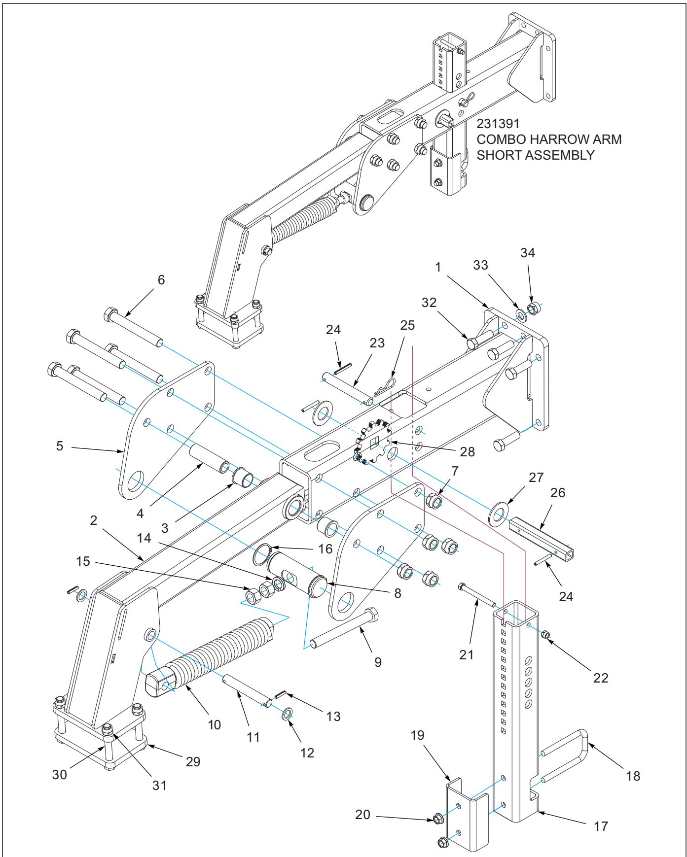
Figure 1-45: Std Combo Harrow Arm Short Assembly
