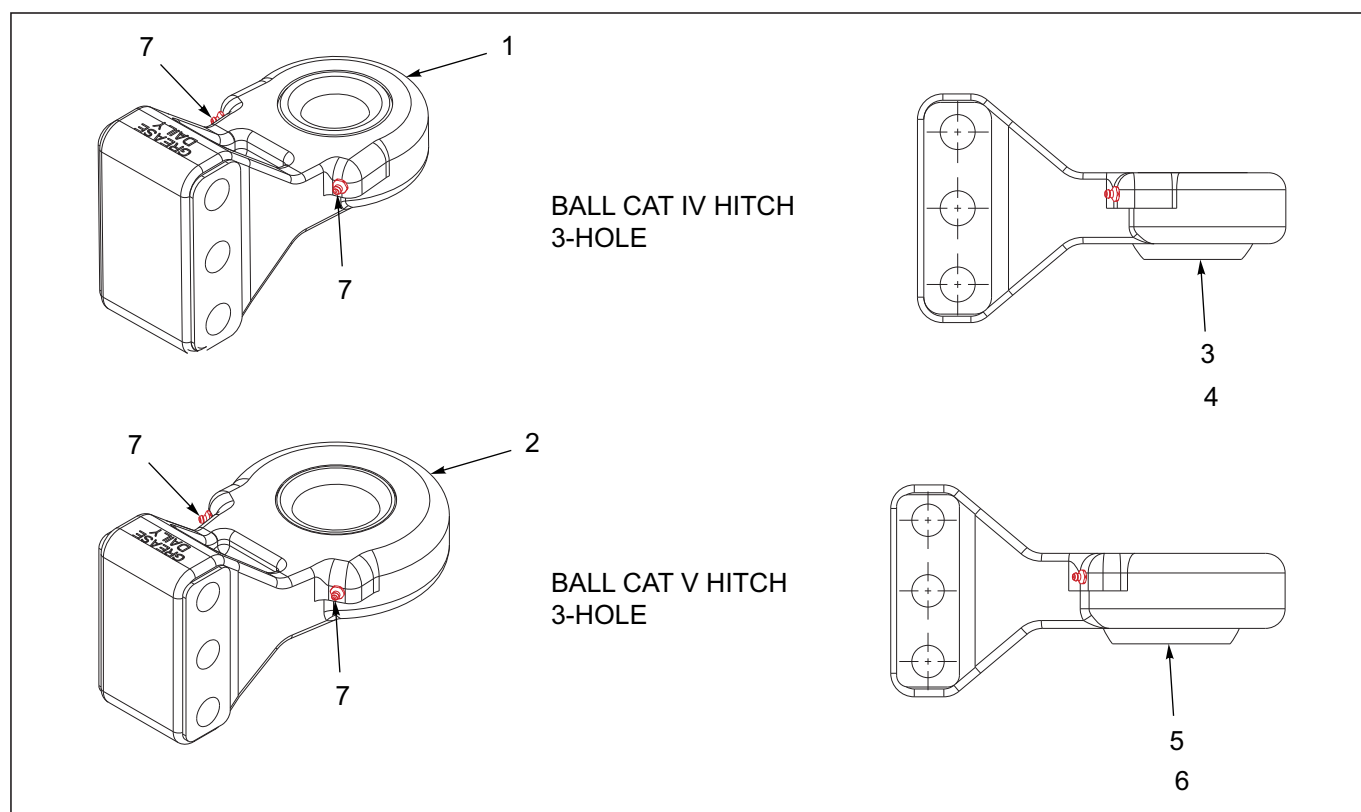
Figure 1-7: Ball &amp; Clevis Hitches
