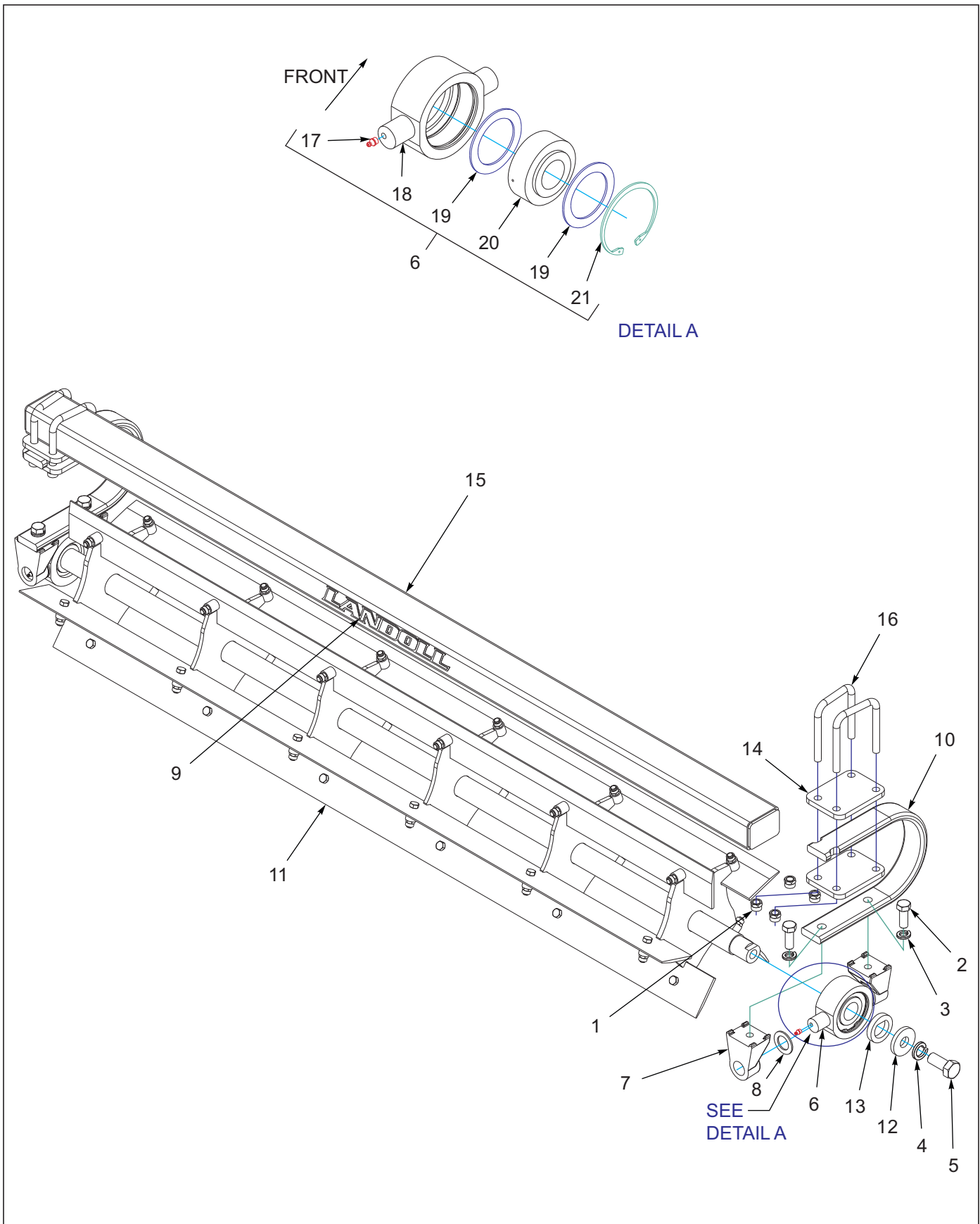
Figure 1-60: Reel/Gangbar Assembly
