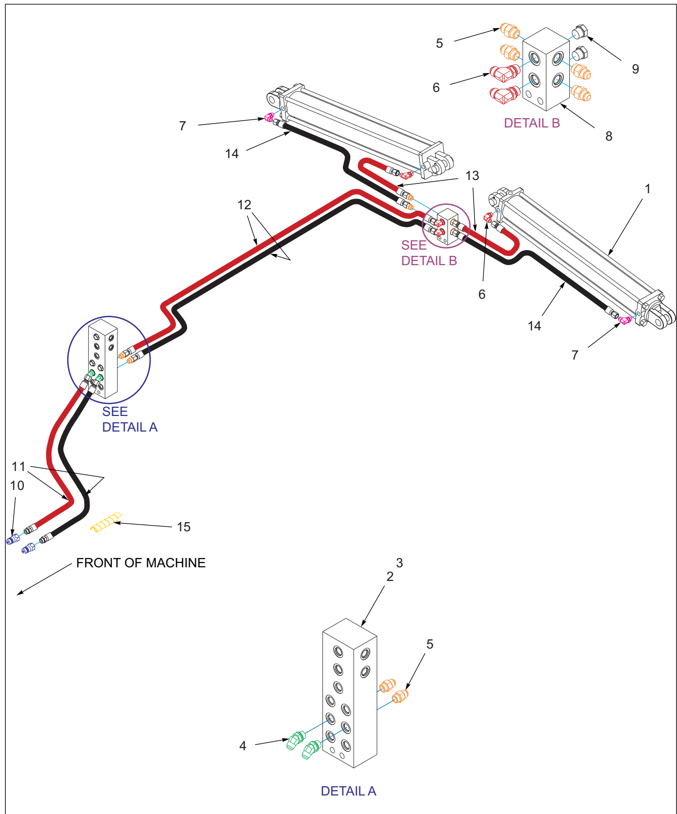
Figure 1-21: Fold Assembly 2132-17-19
