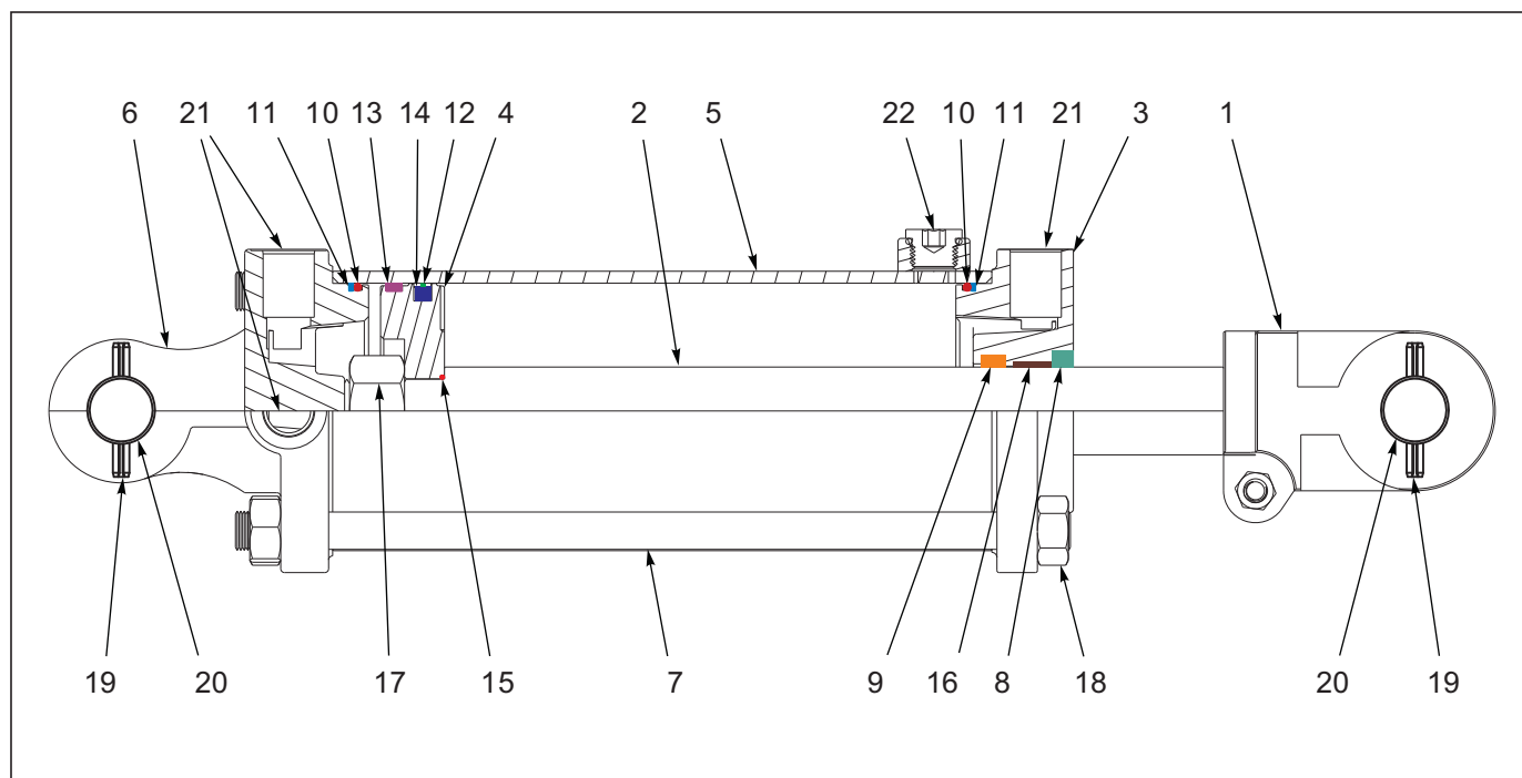
Figure 1-30: Cylinder - Rephase Assembly 4 X 8
