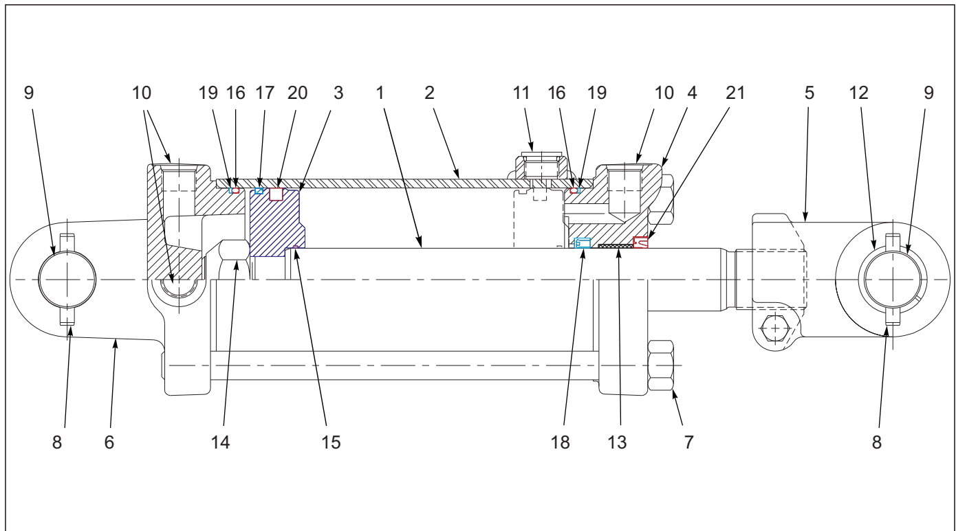
Figure 1-26: Cylinder - Rephase Assembly - 4 X 16
