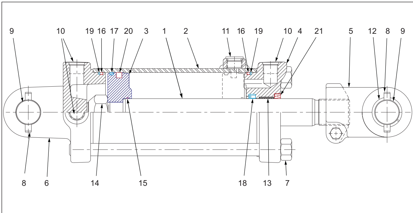
Figure 1-25: Cylinder - Rephase Assembly - 4 X 16
