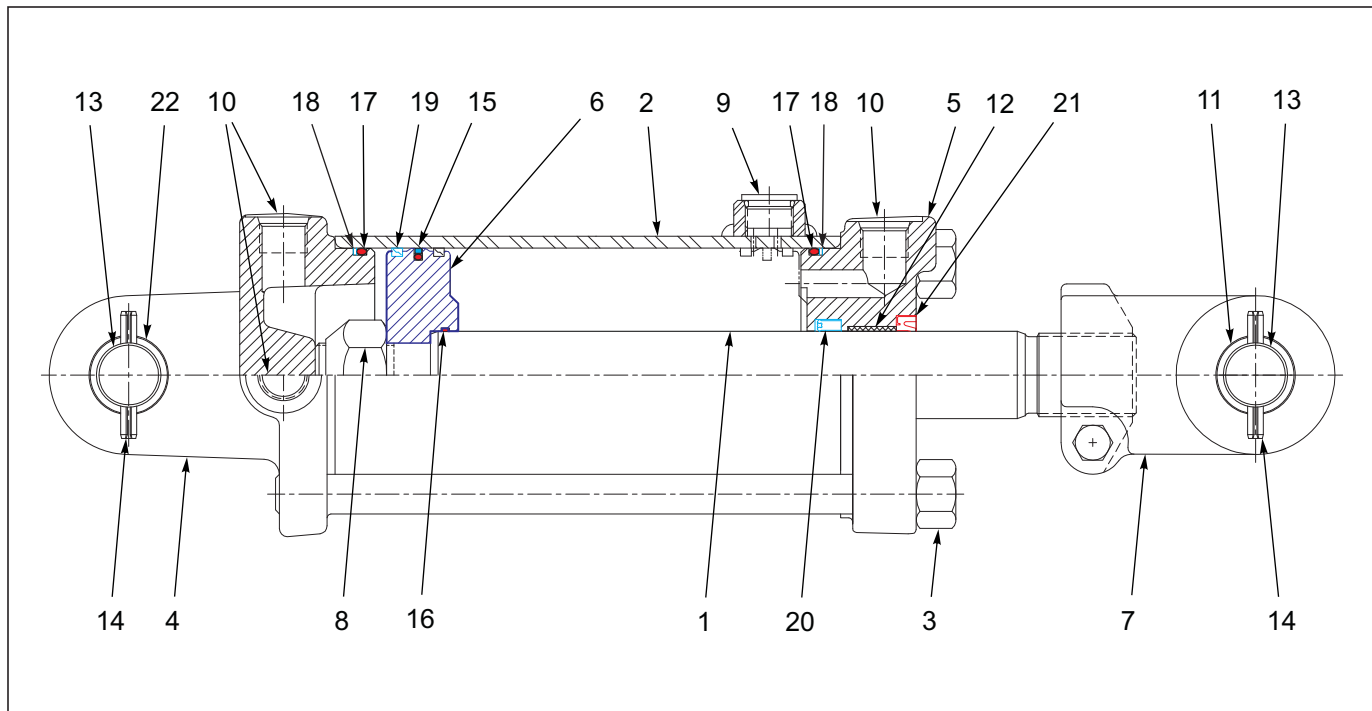
Figure 1-35: Cylinder - Rephase Assembly - 3-1/4 X 8
