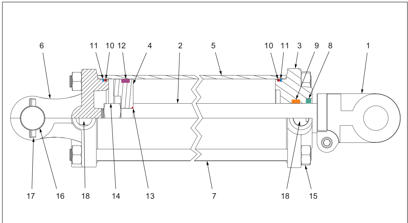
Figure 1-28: Hydraulic Cylinder 4 X 30 (Midway)
