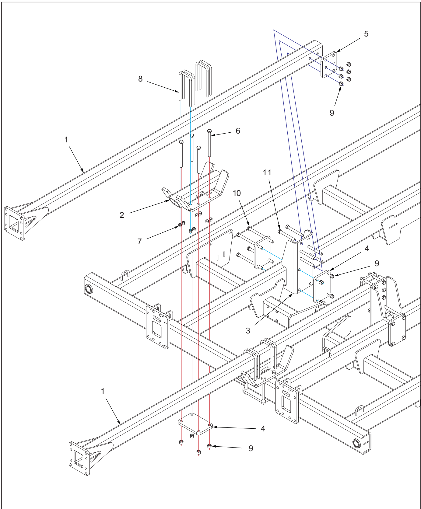
Figure 1-63: Rear Tow Hitch Assembly (1 of 2)
