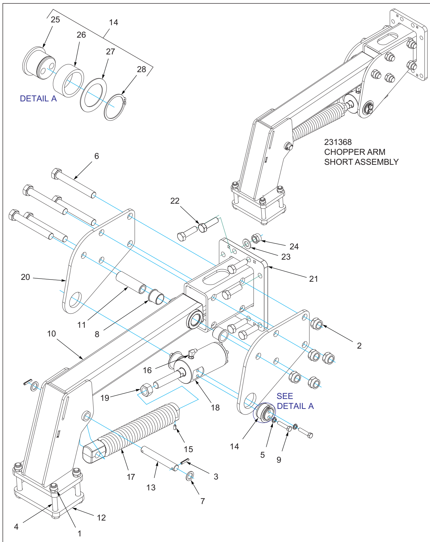
Figure 1-59: Hyd Chopper Arm Short Assembly
