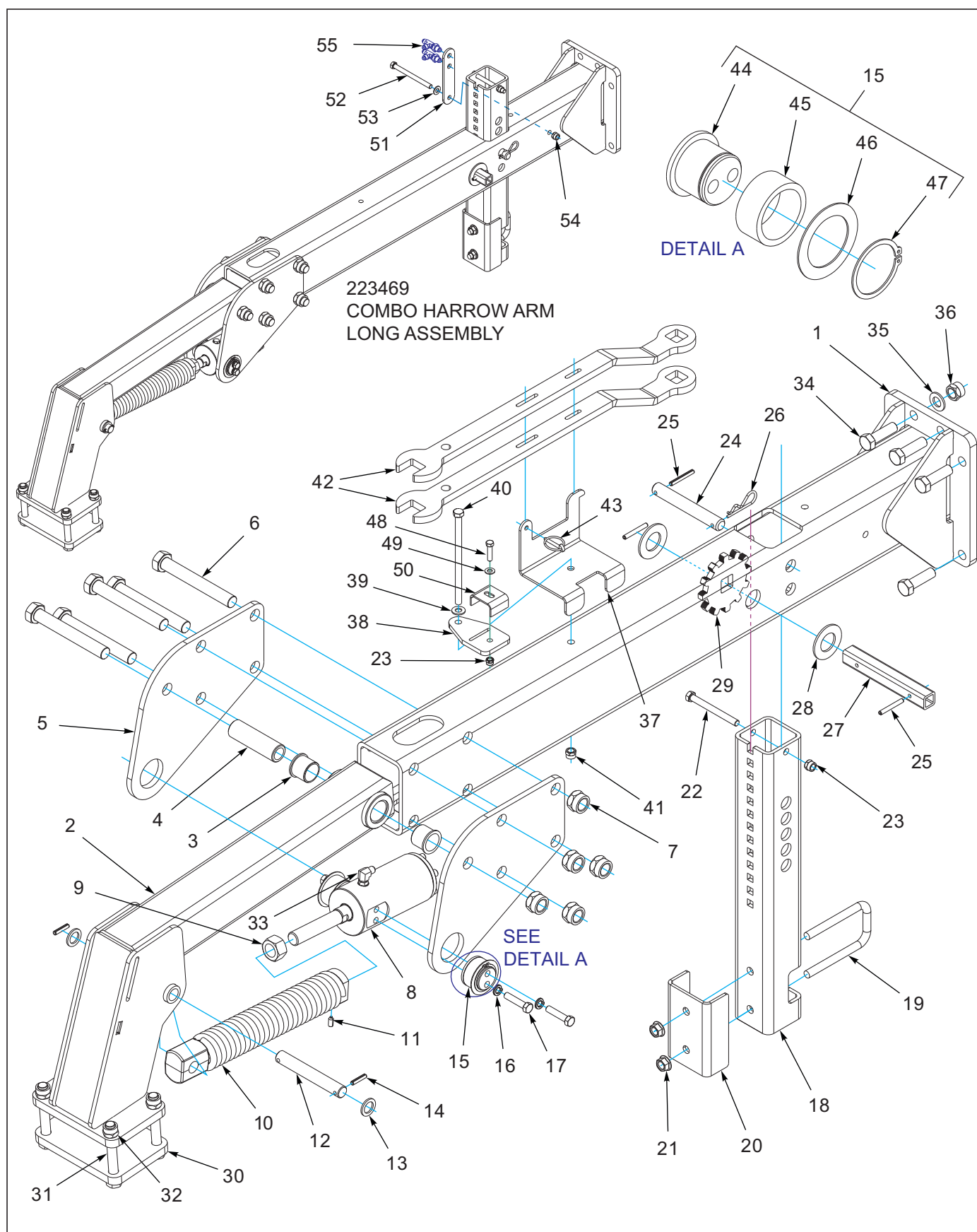
Figure 1-48: Hyd Combo Harrow Arm Long Assembly
