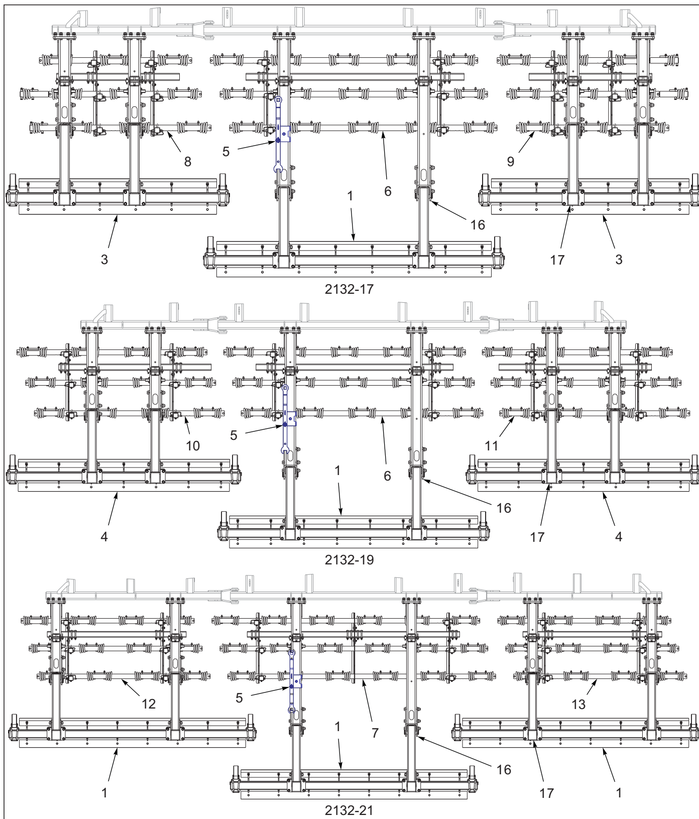
Figure 1-42: Std 3BCT/Chopper Layout (1 of 2)
