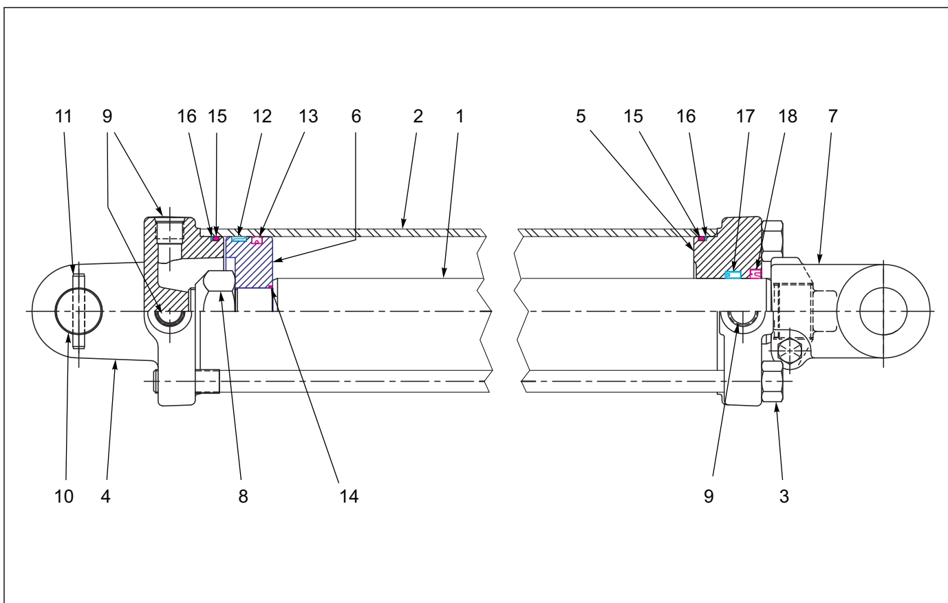
Figure 1-27: Hydraulic Cylinder 4 X 30 (Prince)
