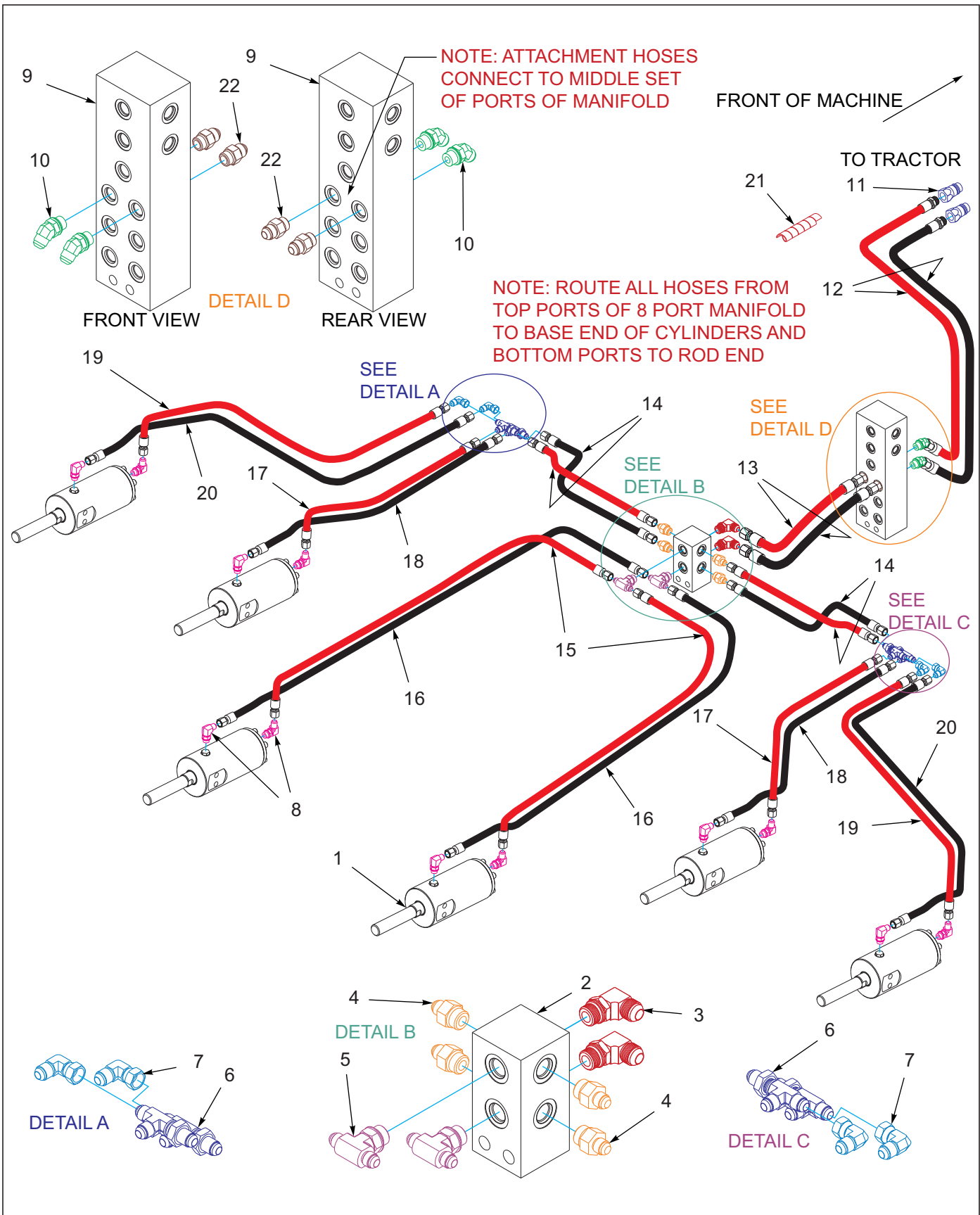
Figure 1-62: Chopper Reel Hydraulic Assembly
