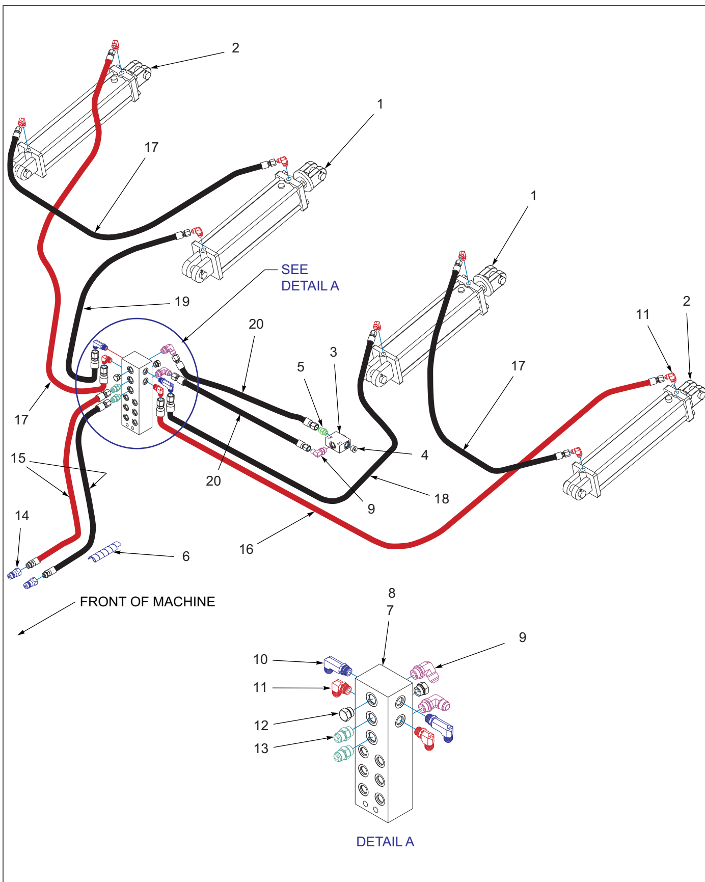
Figure 1-20: Lift Hydraulic Assembly 2132-17-19 After 01-01-2024 &amp; 21-23-25 After 10-03-2023
