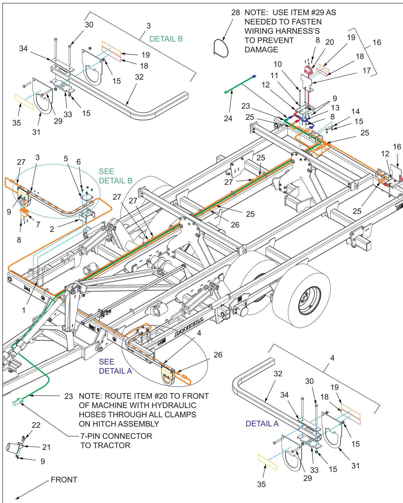
Figure 1-39: Electrical Assembly W/ LED Lights (2 of 2)
