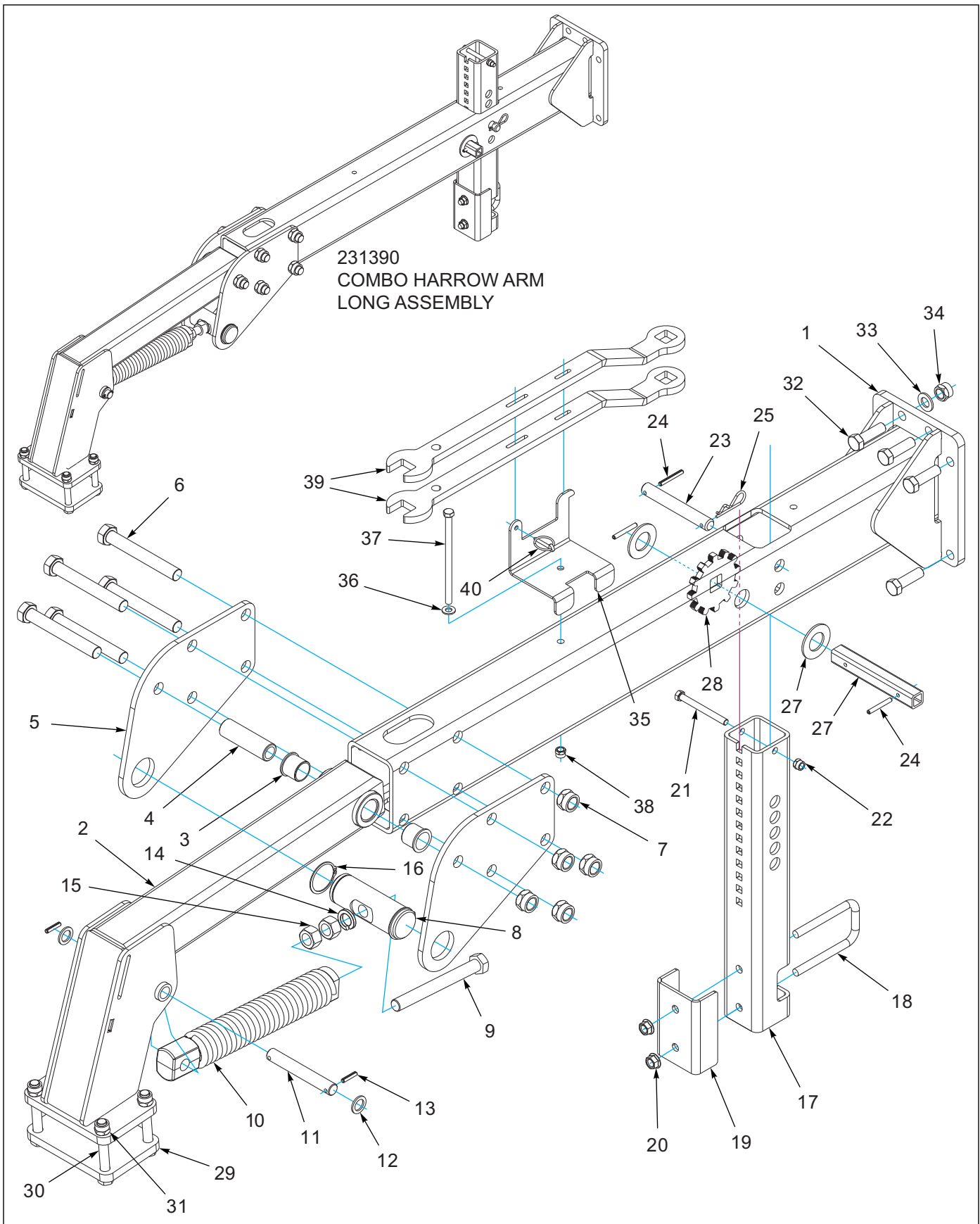
Figure 1-44: Std Combo Harrow Arm Long Assembly
