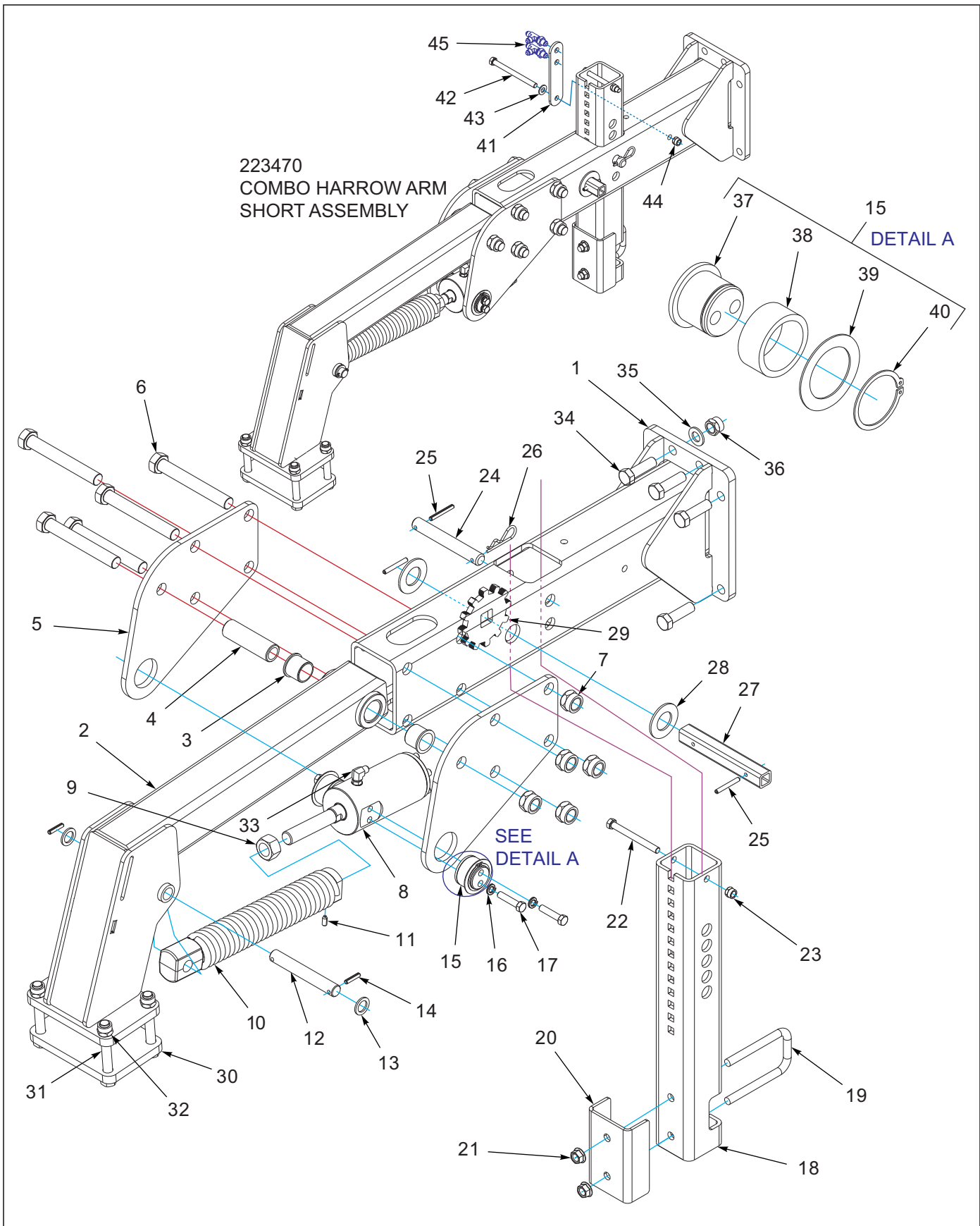
Figure 1-49: Hyd Combo Harrow Arm Short Assembly
