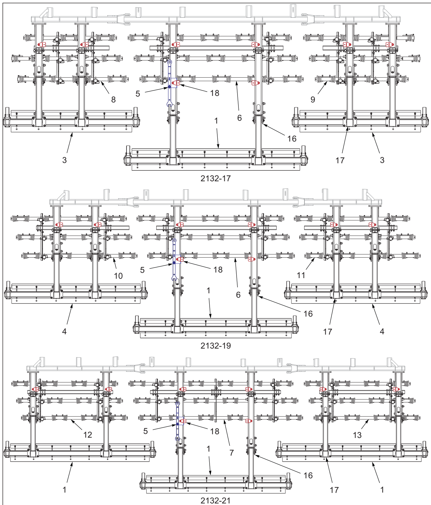
Figure 1-46: Hyd 3BCT/Chopper Layout (1 of 2)
