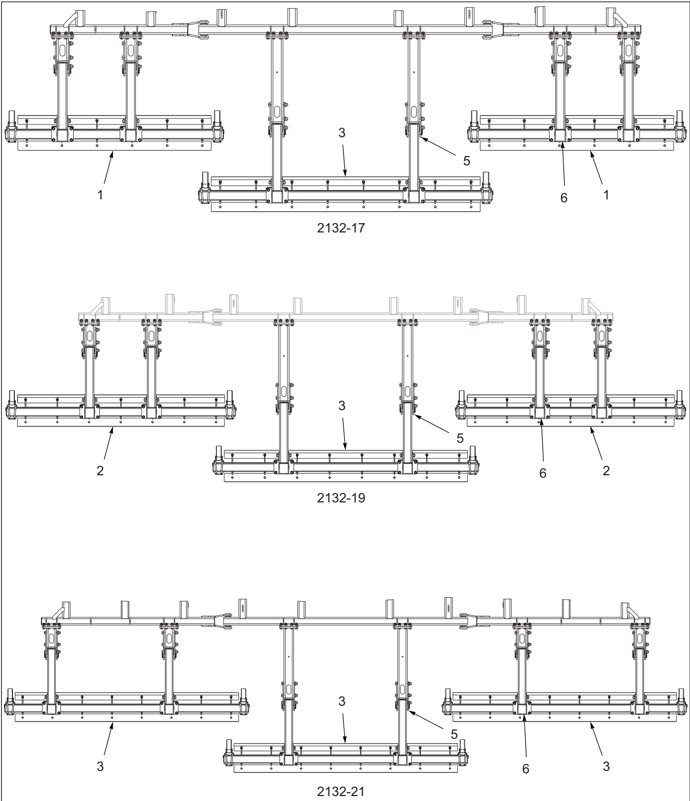
Figure 1-52: Std Chopper Reel Layout (1 of 2)
