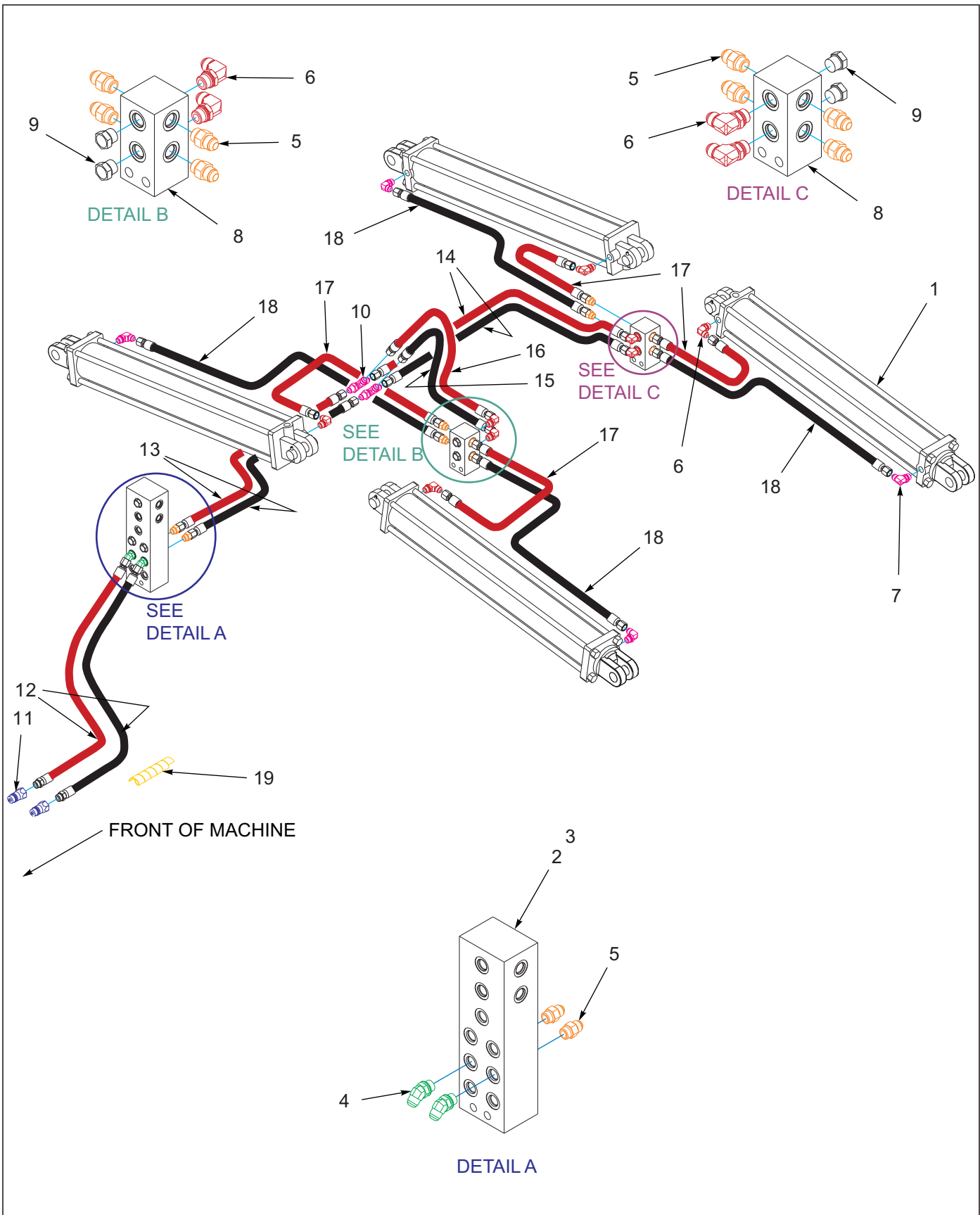
Figure 1-22: Fold Hydraulic Assembly 2132-21-23-25
