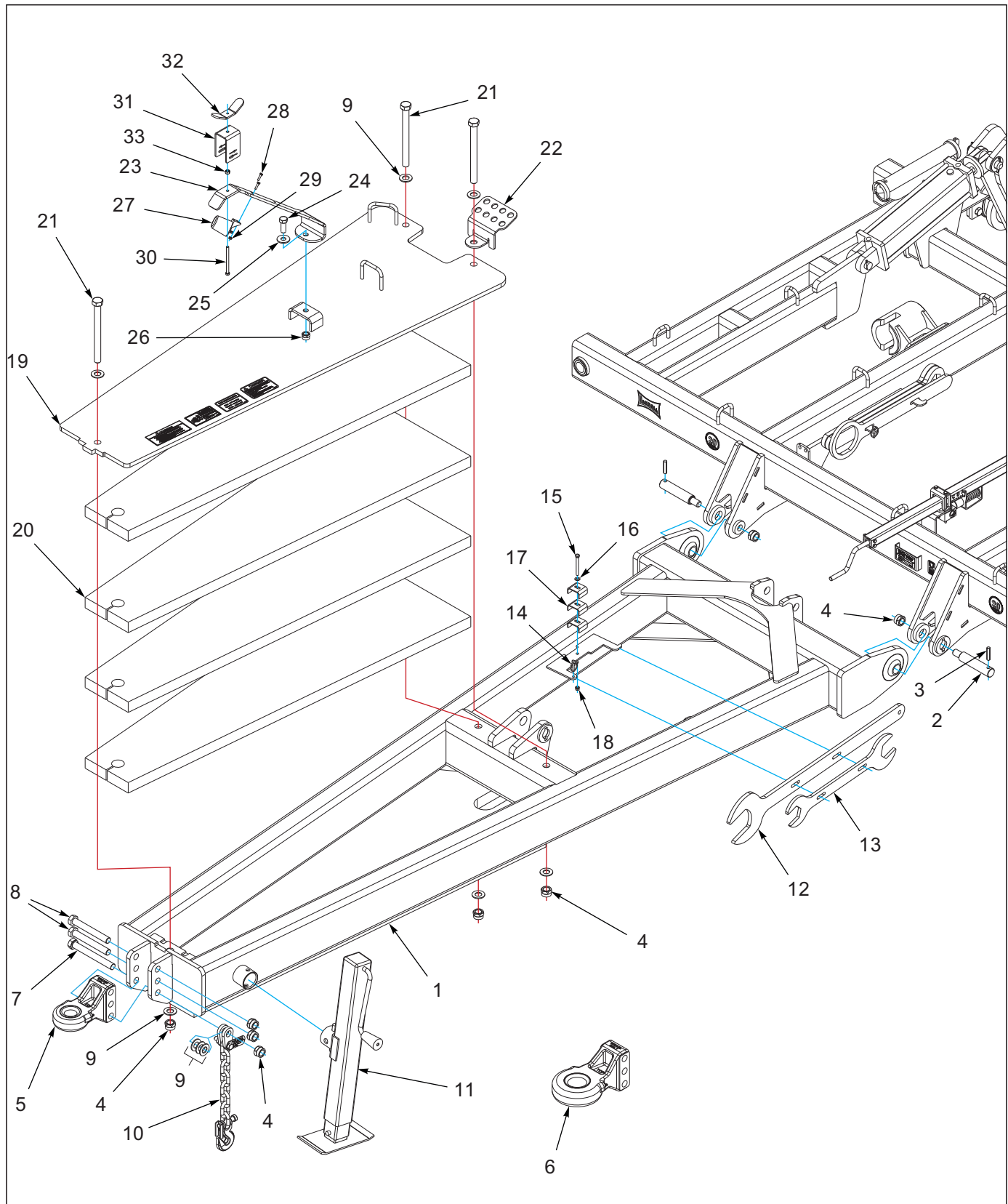
Figure 1-5: Hitch Assembly
