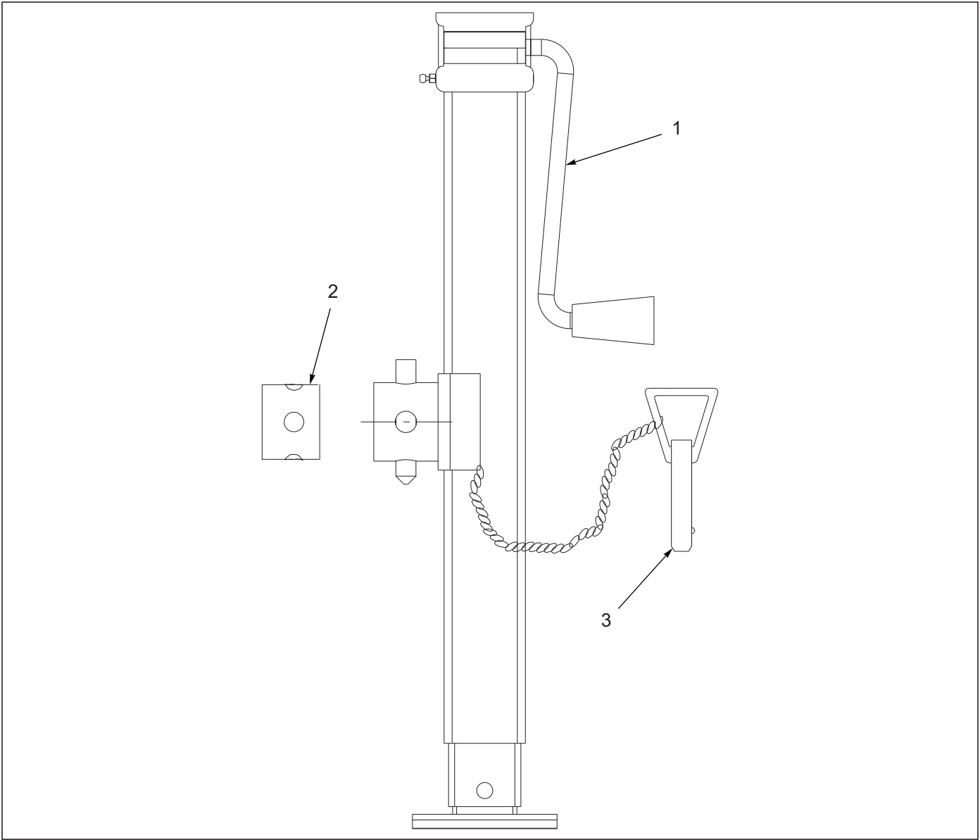
Figure 1-8: 7,000 Lb. Sidewind Jack Assembly
