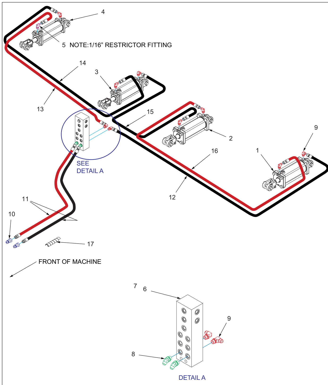
Figure 1-23: Coulter Gang Assembly
