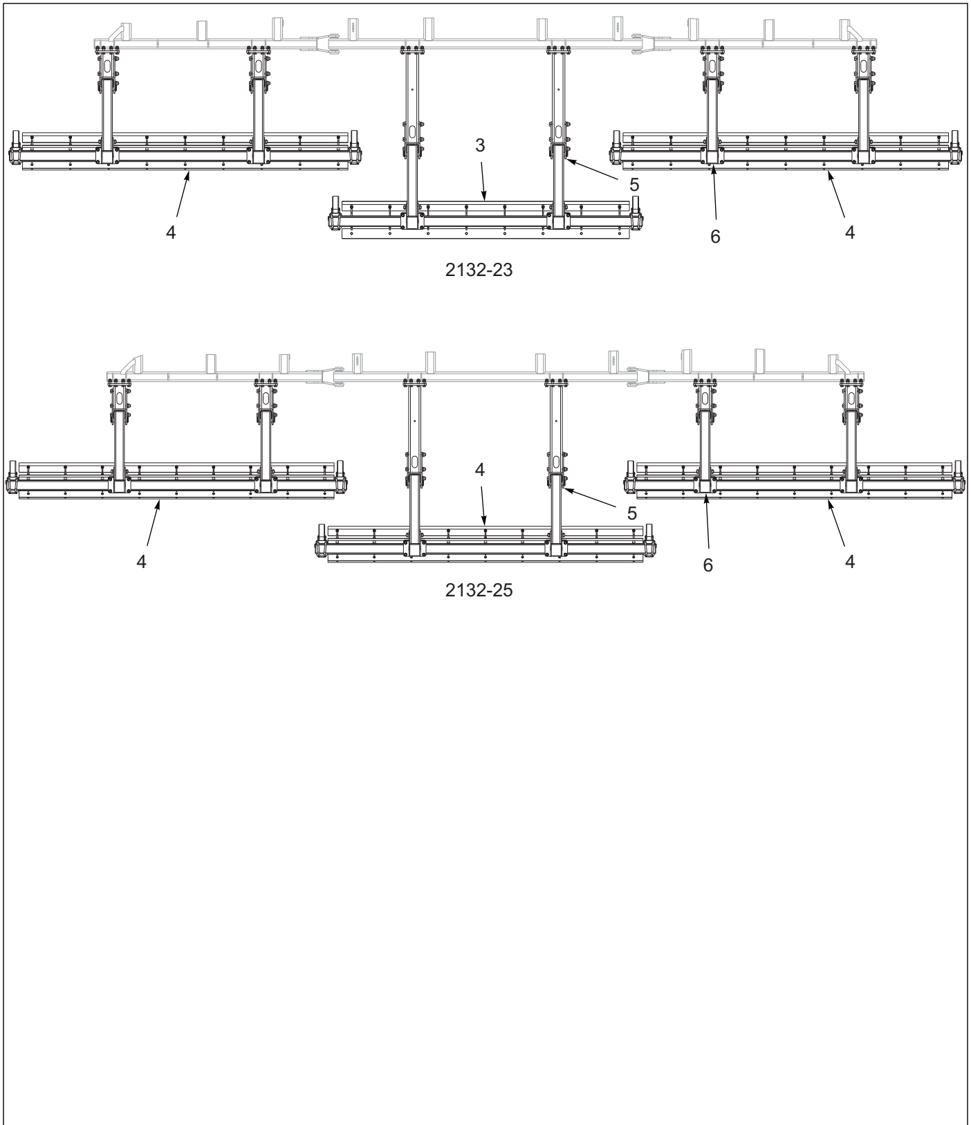
Figure 1-53: Std Chopper Reel Layout (2 of 2)
