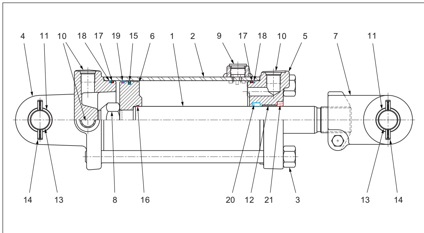
Figure 1-29: Cylinder - Rephase Assembly 4 X 8
