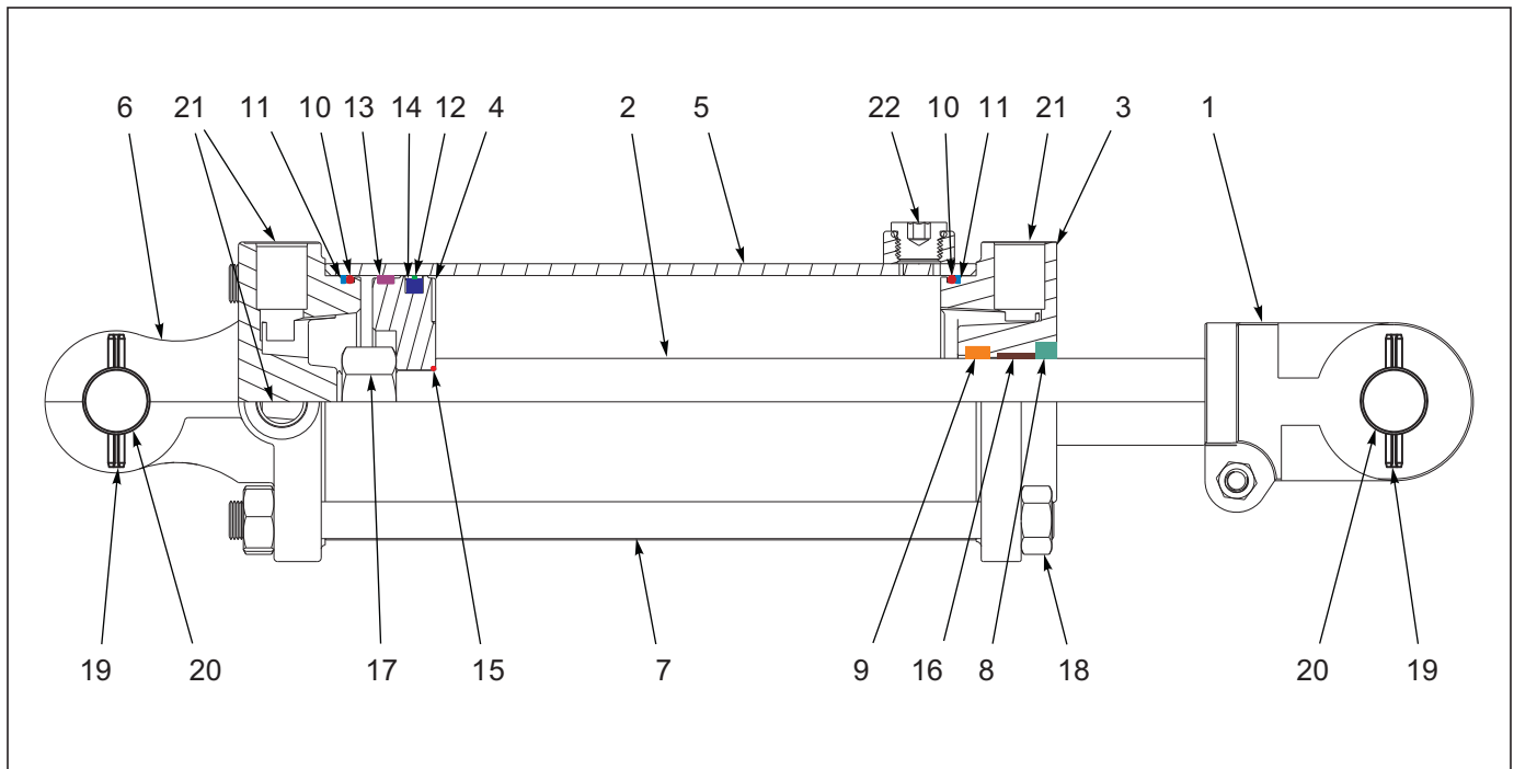
Figure 1-32: Cylinder - Rephase Assembly 3-3/4 X 8
