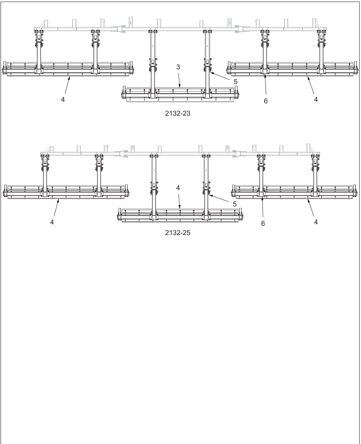
Figure 1-57: Hyd Chopper Reel Layout (2 of 2)
