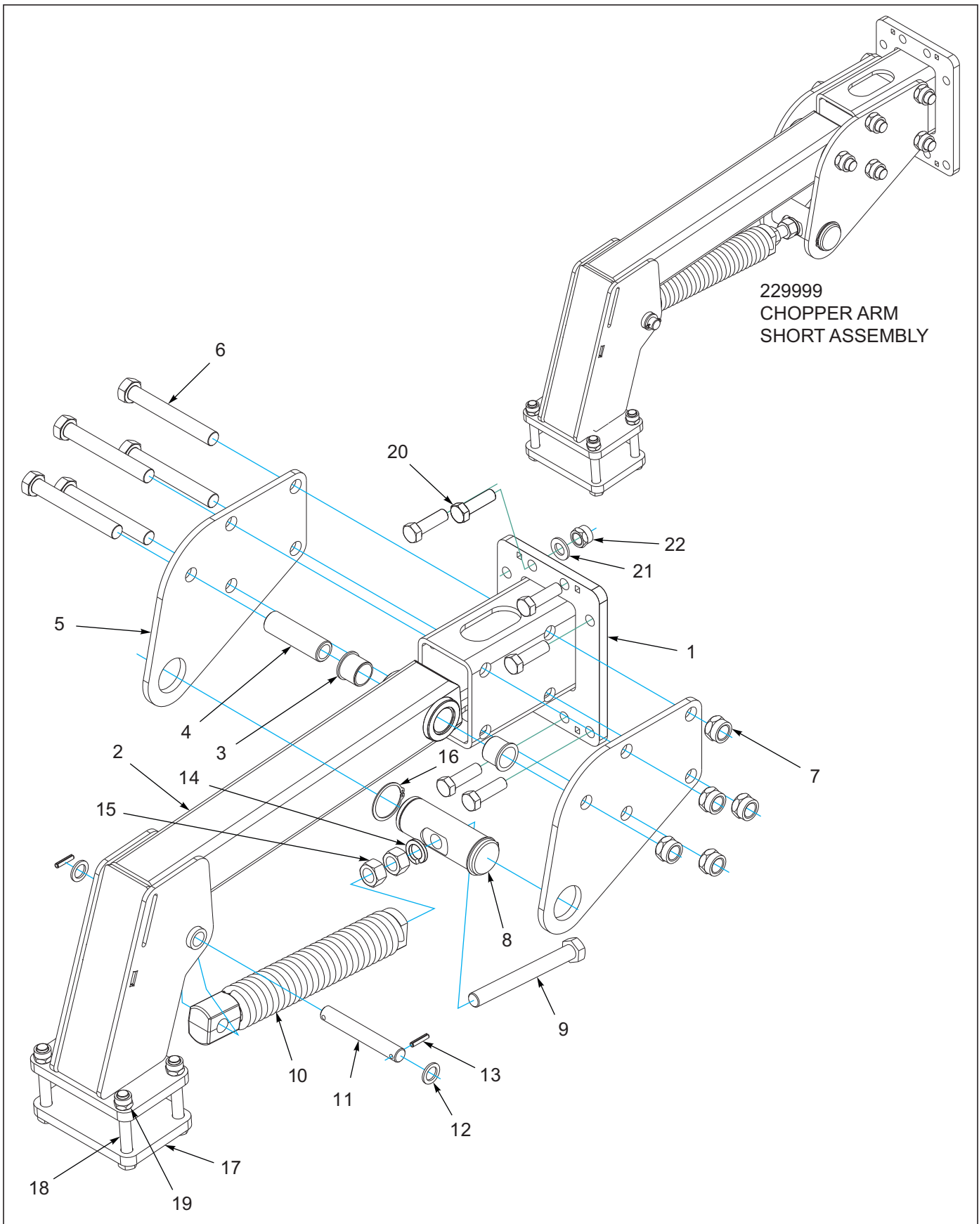
Figure 1-55: Std Chopper Arm Short Assembly
