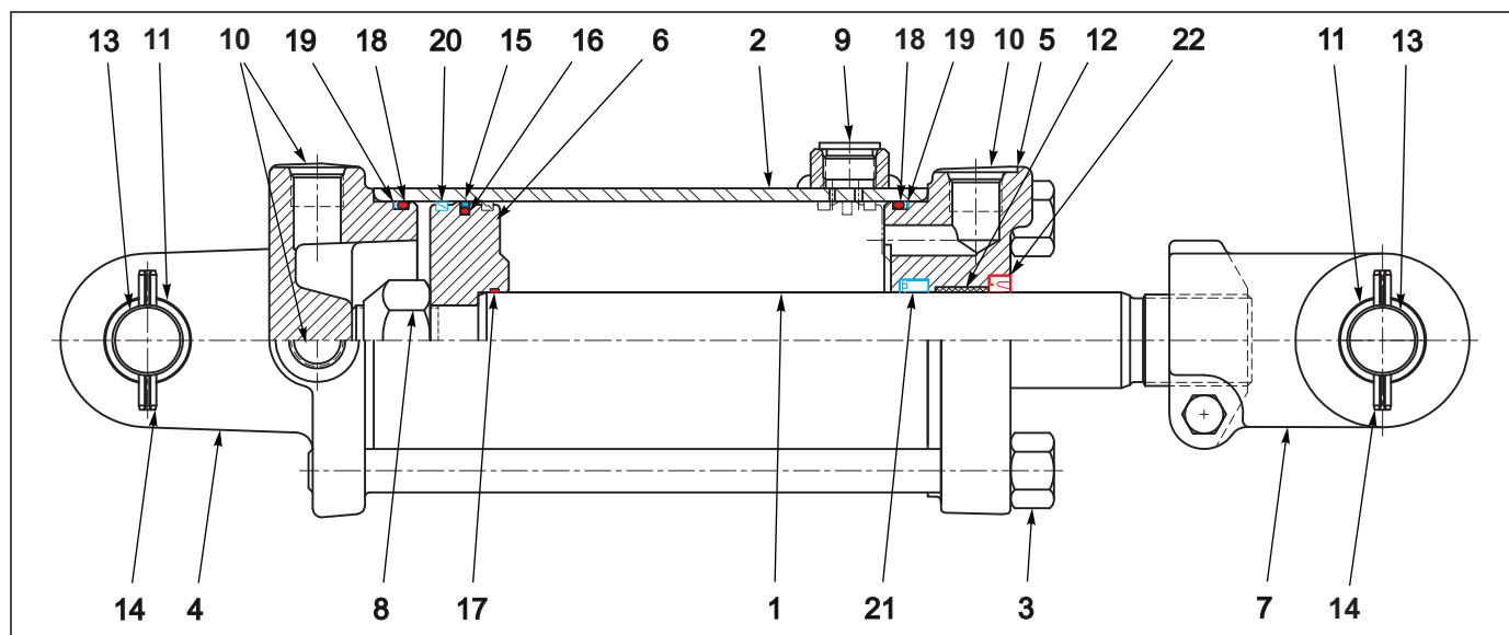
Figure 1-33: Cylinder Assembly Rephase 4 X 8
