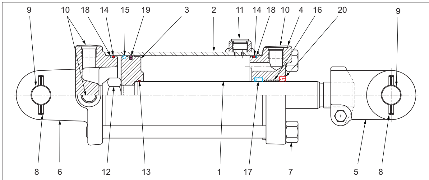
Figure 1-32: Cylinder Assembly Rephase 4 X 8
