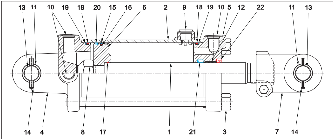
Figure 1-35: Cylinder Assembly Rephase 4-1/2 X 8
