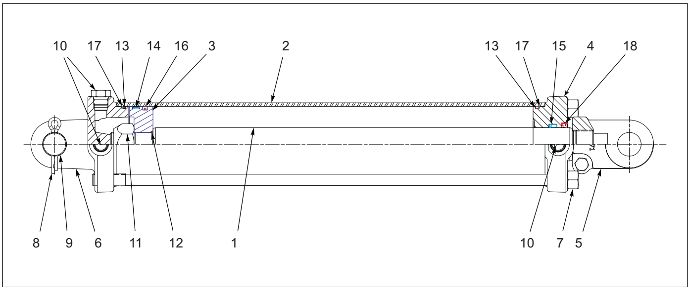
Figure 1-37: Cylinder - Assembly 4-1/2 X 16
