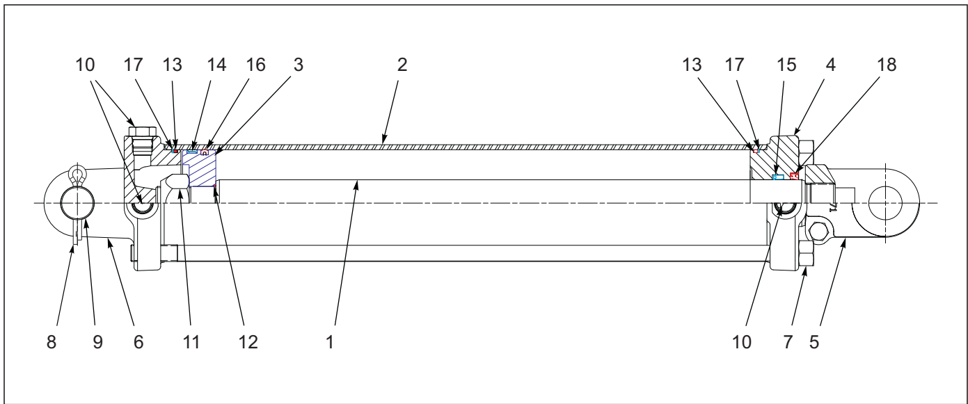
Figure 1-38: Cylinder - Assembly 4-1/2 X 20
