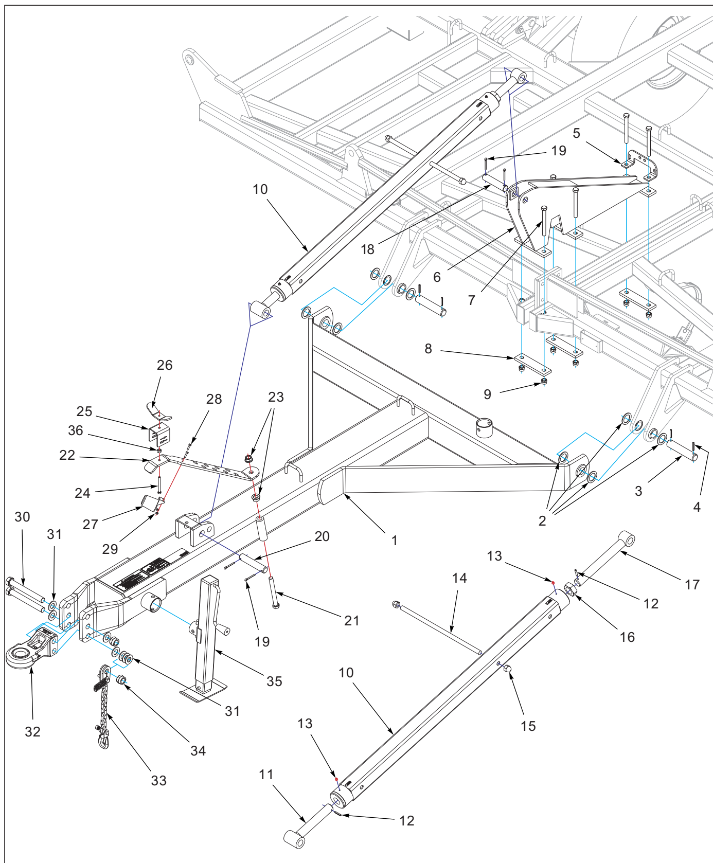
Figure 1-10: Hitch Assembly
