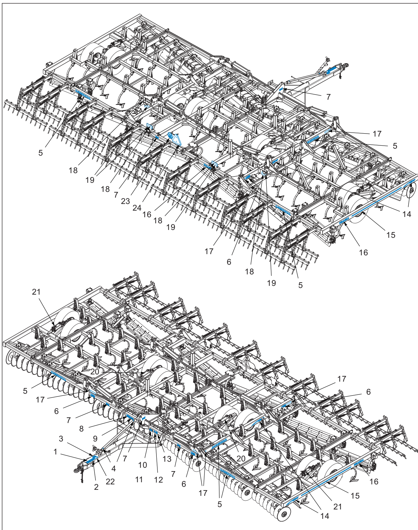
Figure 1-43: Decal Locations
