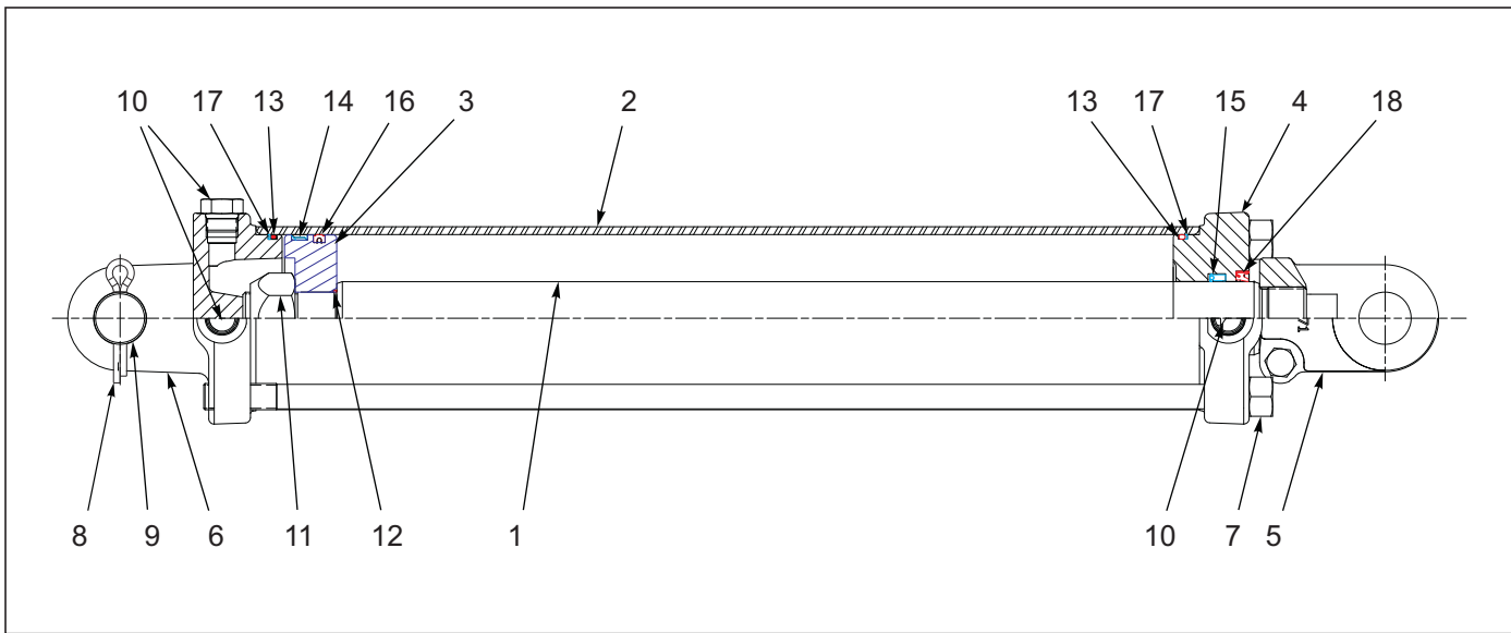
Figure 1-36: Cylinder - Assembly 3-1/2 X 16
