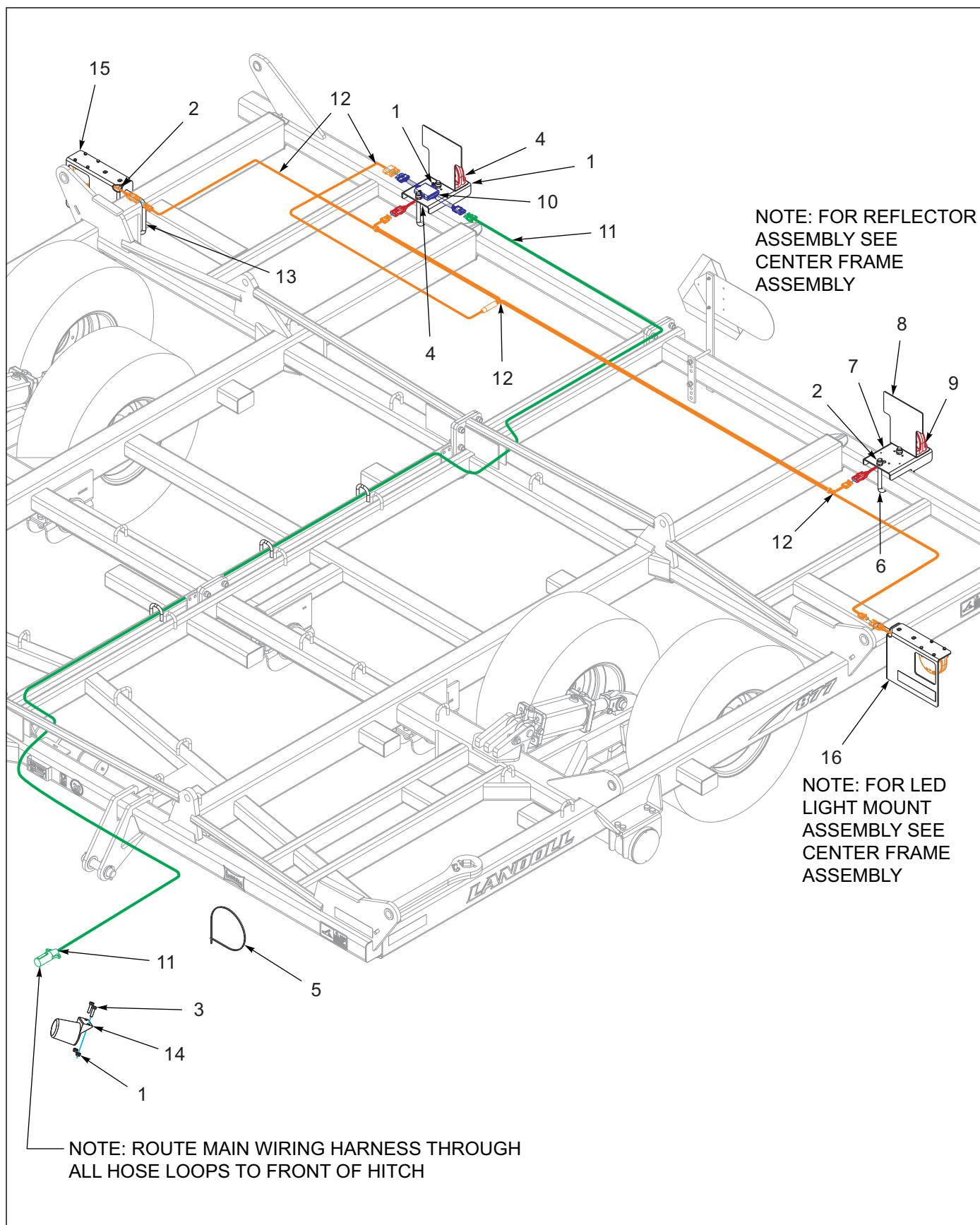
Figure 1-40: Electrical Assembly W/ LED Lights (2 of 2)
