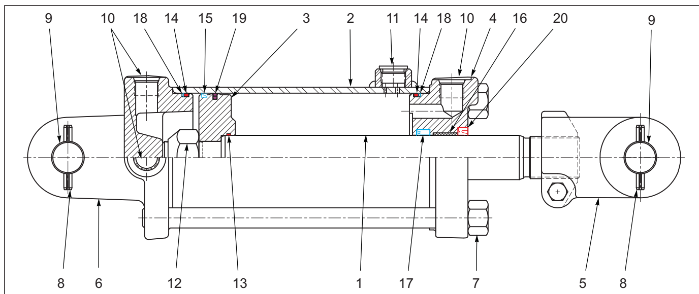
Figure 1-34: Cylinder Assembly Rephase 4-1/2 X 8
