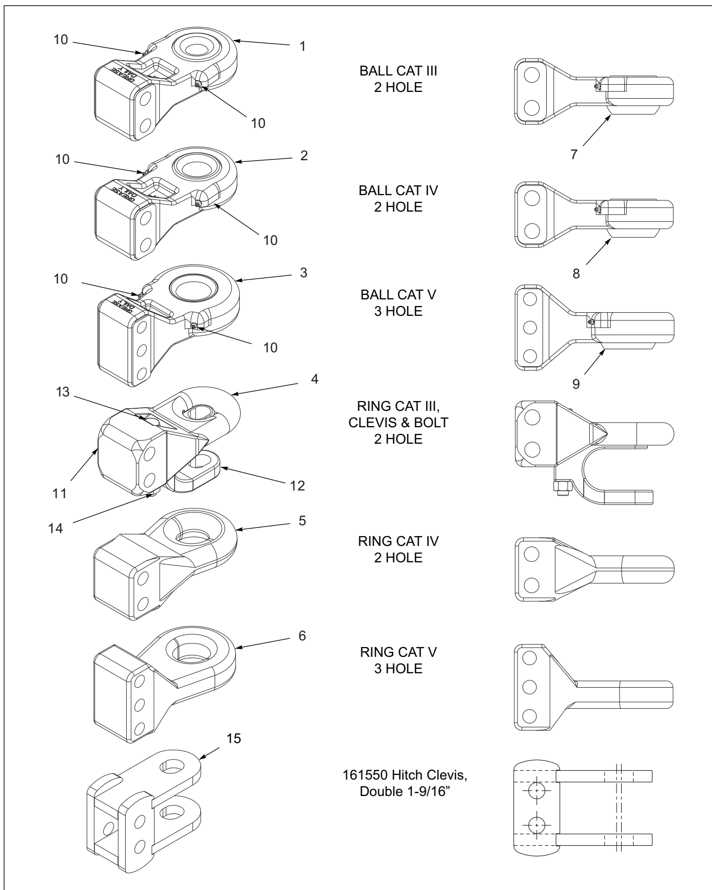
Figure 1-12: Ball &amp; Ring Hitches
