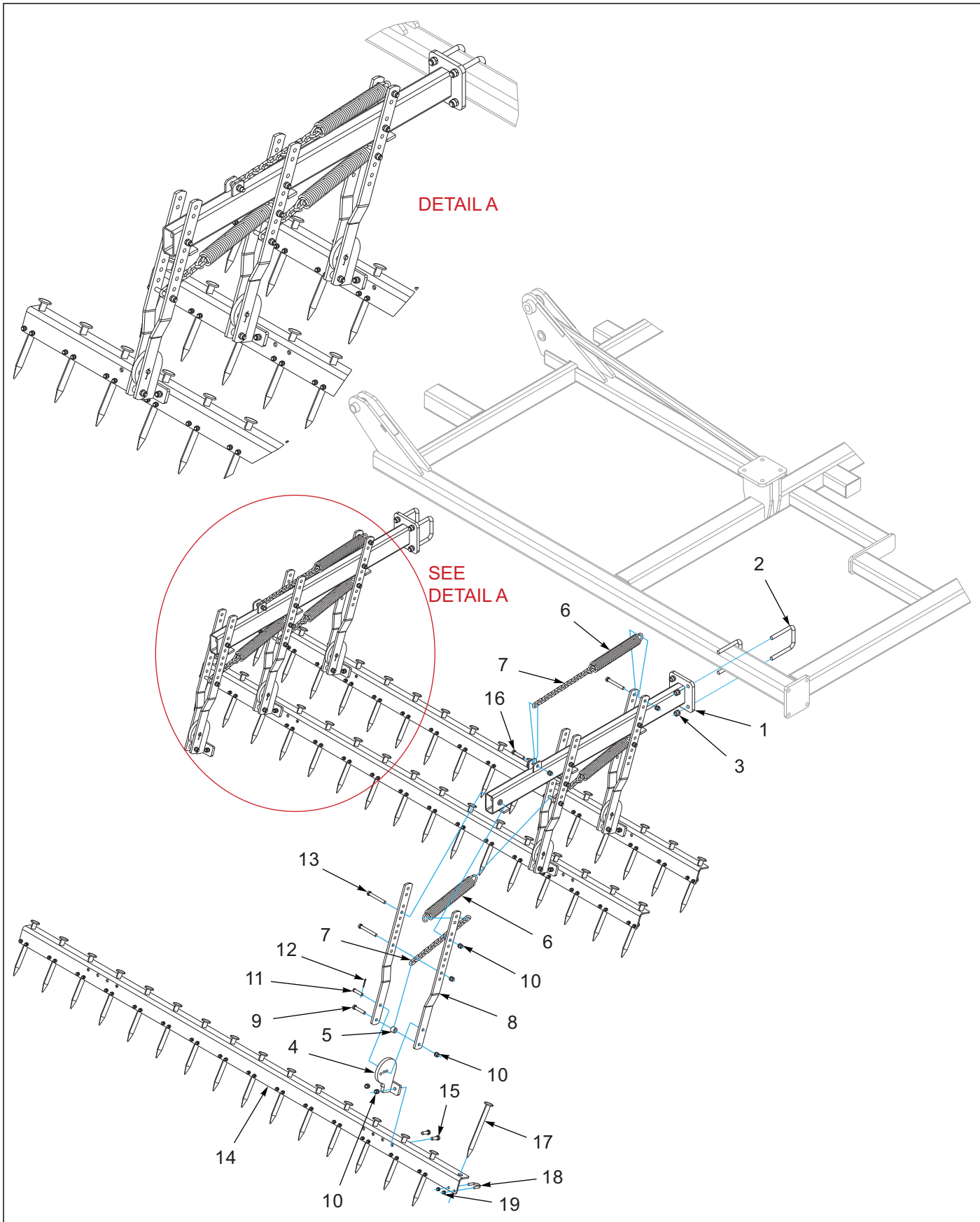
Figure 1-27: Harrow Assembly
