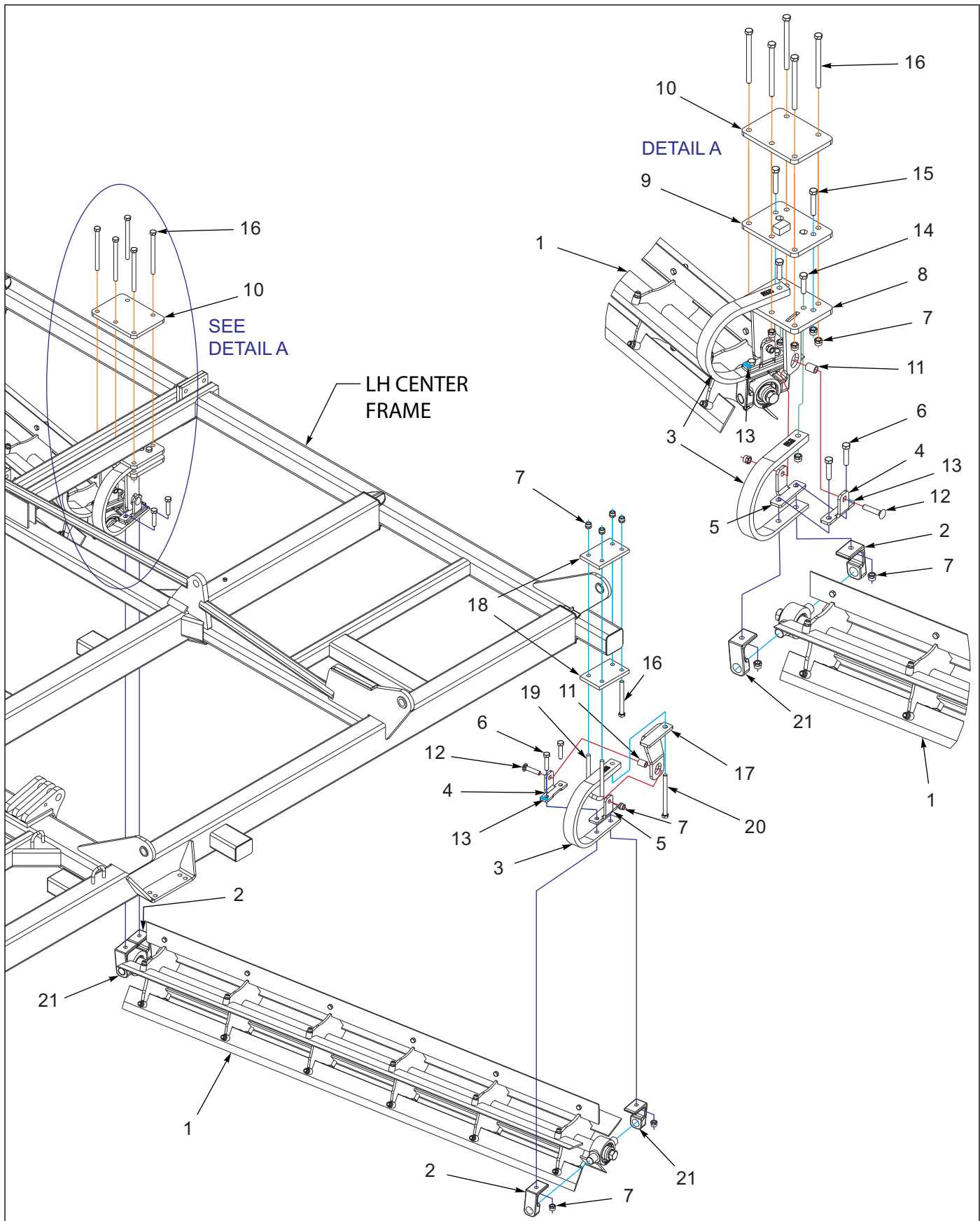
Figure 1-25: Reel Assembly
