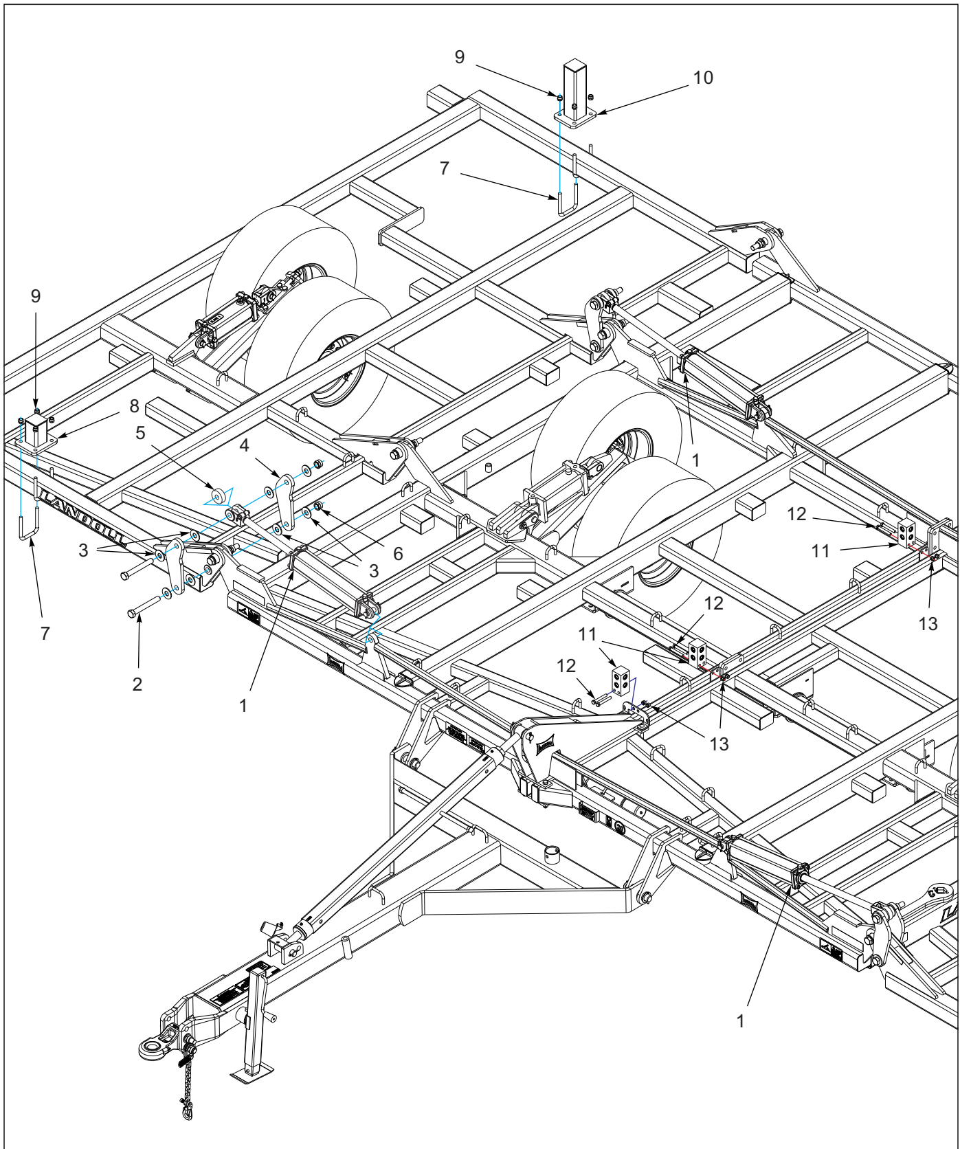
Figure 1-13: Fold Assembly 877-30'
