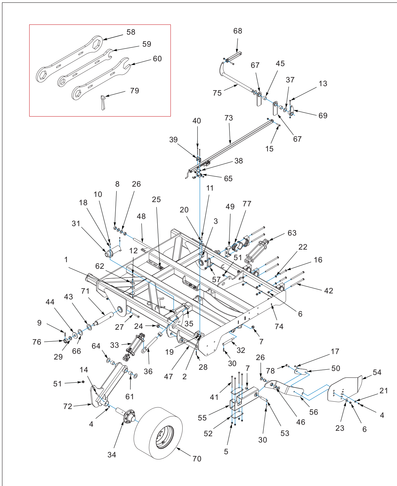
Figure 2-2: Wing Assembly - Left Hand 17'
