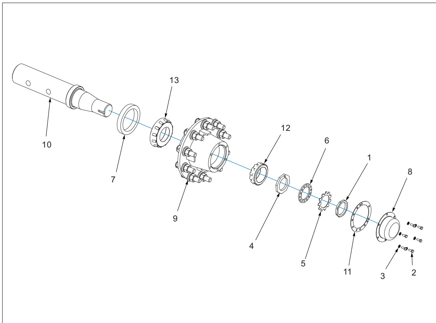
Figure 3-3: Hub and Spindle Assembly, 10 Bolt - 193814 (BEFORE 05/27/2020)
