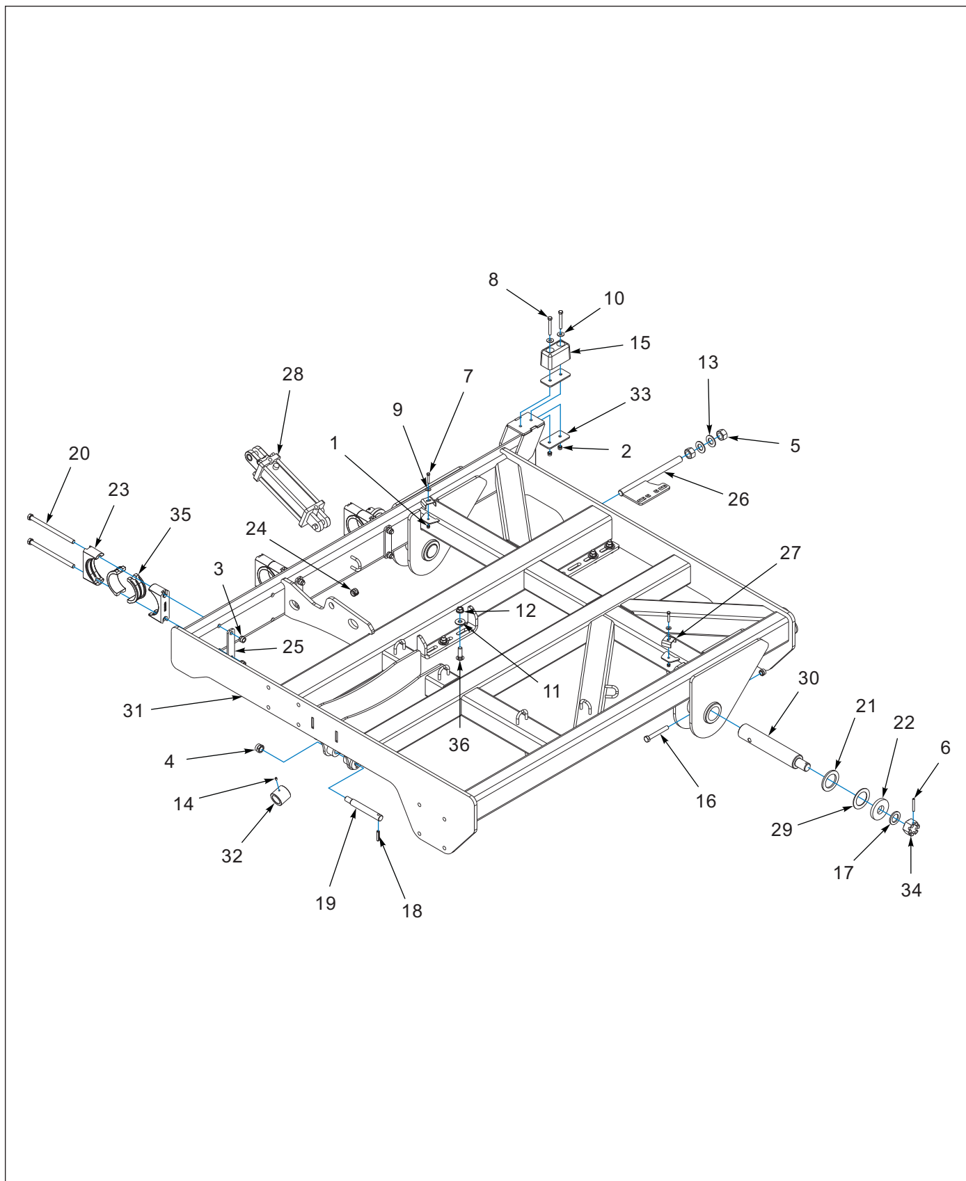
Figure 2-6: Wing Assembly - Right Hand 15'
