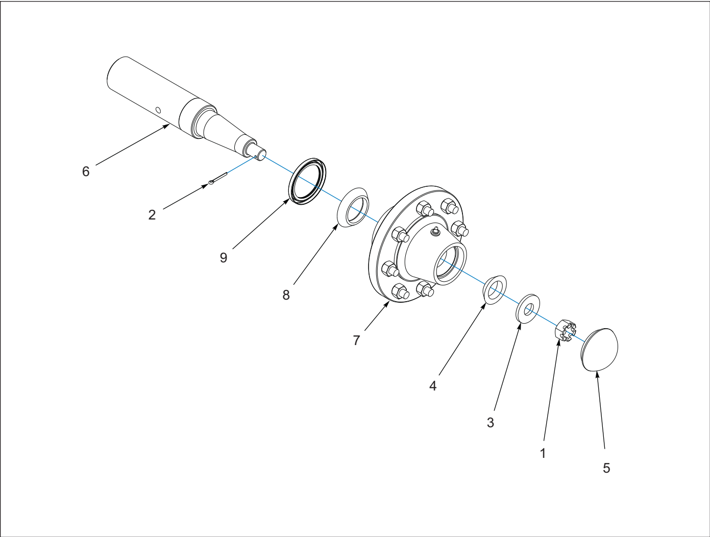
Figure 3-1: Hub and Spindle Assembly, 8 Bolt
