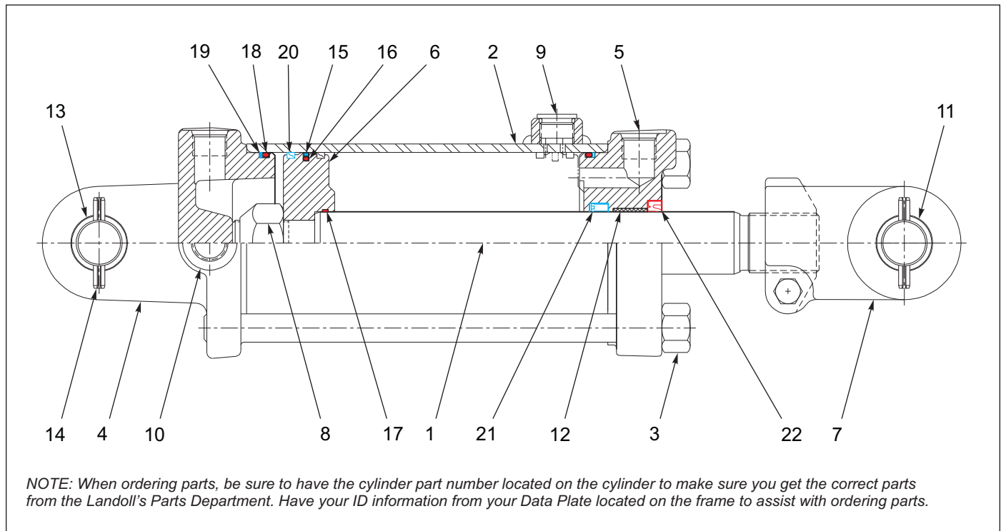
Figure 12-15: Hydraulic Cylinder, 4 x 10 - 201275
