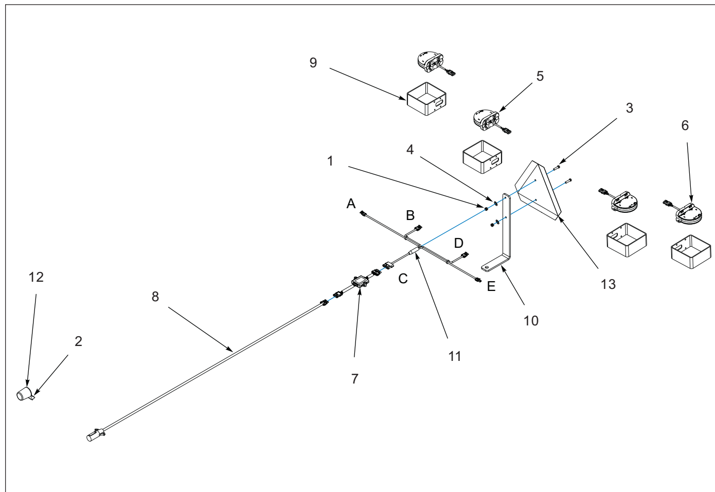
Figure 13-2: Electrical Assembly (2 of 2)
