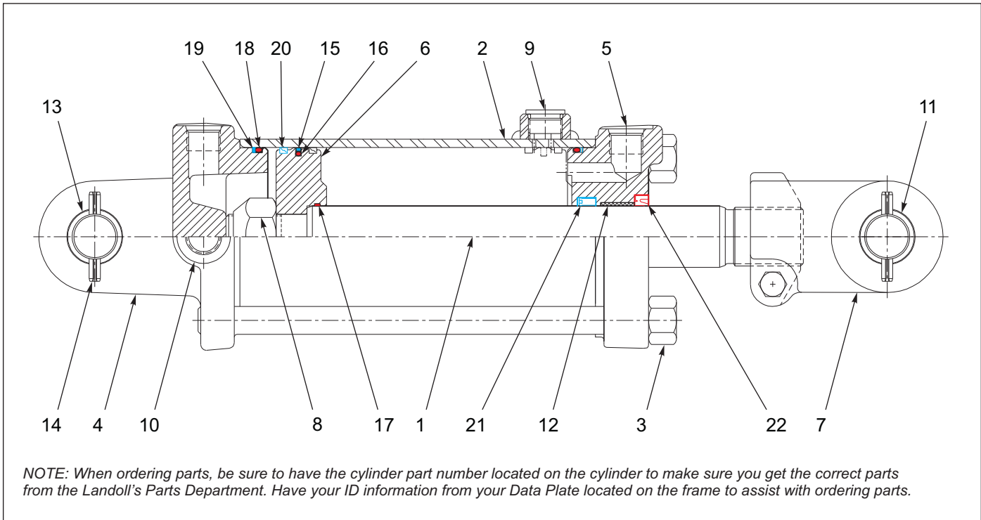
Figure 12-12: Hydraulic Cylinder, 3-3/4 x 10 - 201276
