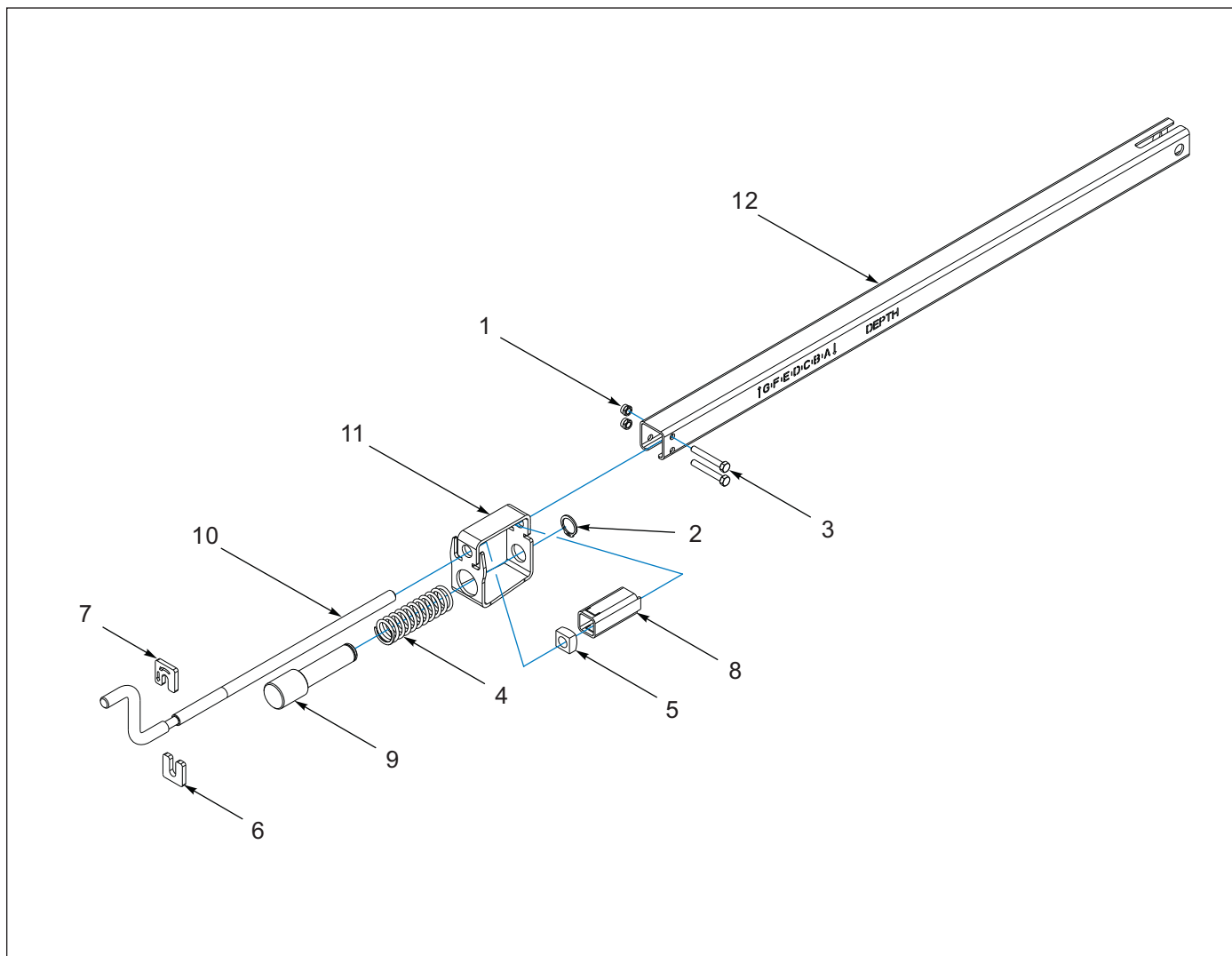
Figure 4-5: Depth Control Assembly - 218749
