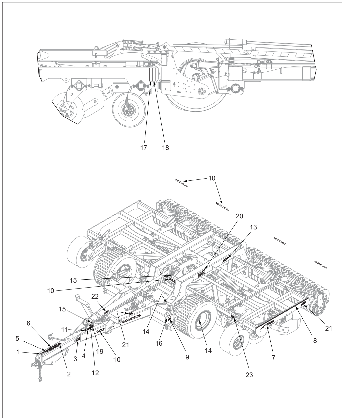
Figure 14-2: Decal Placement
