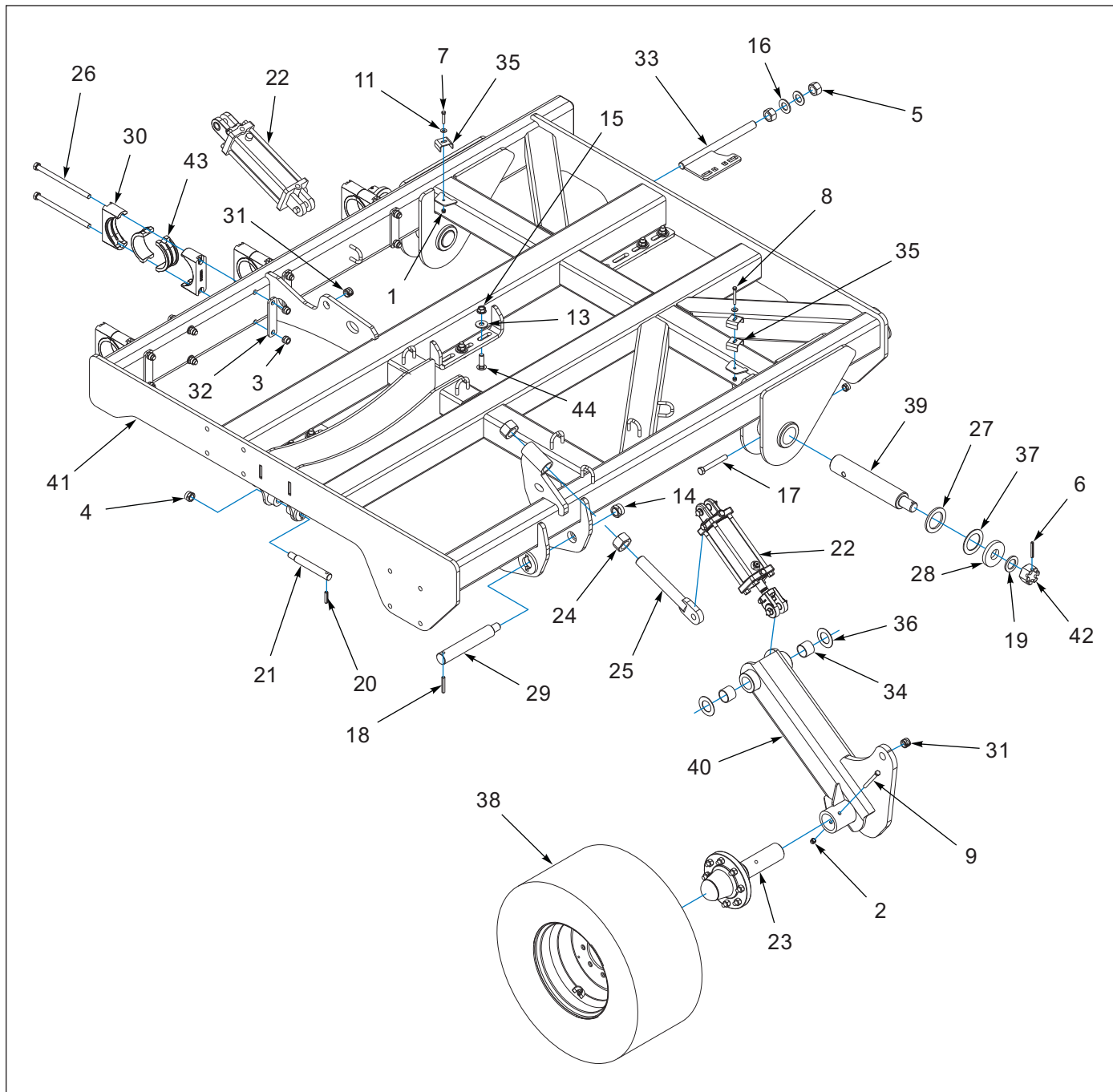
Figure 2-7: Wing Assembly - Right Hand 17'
