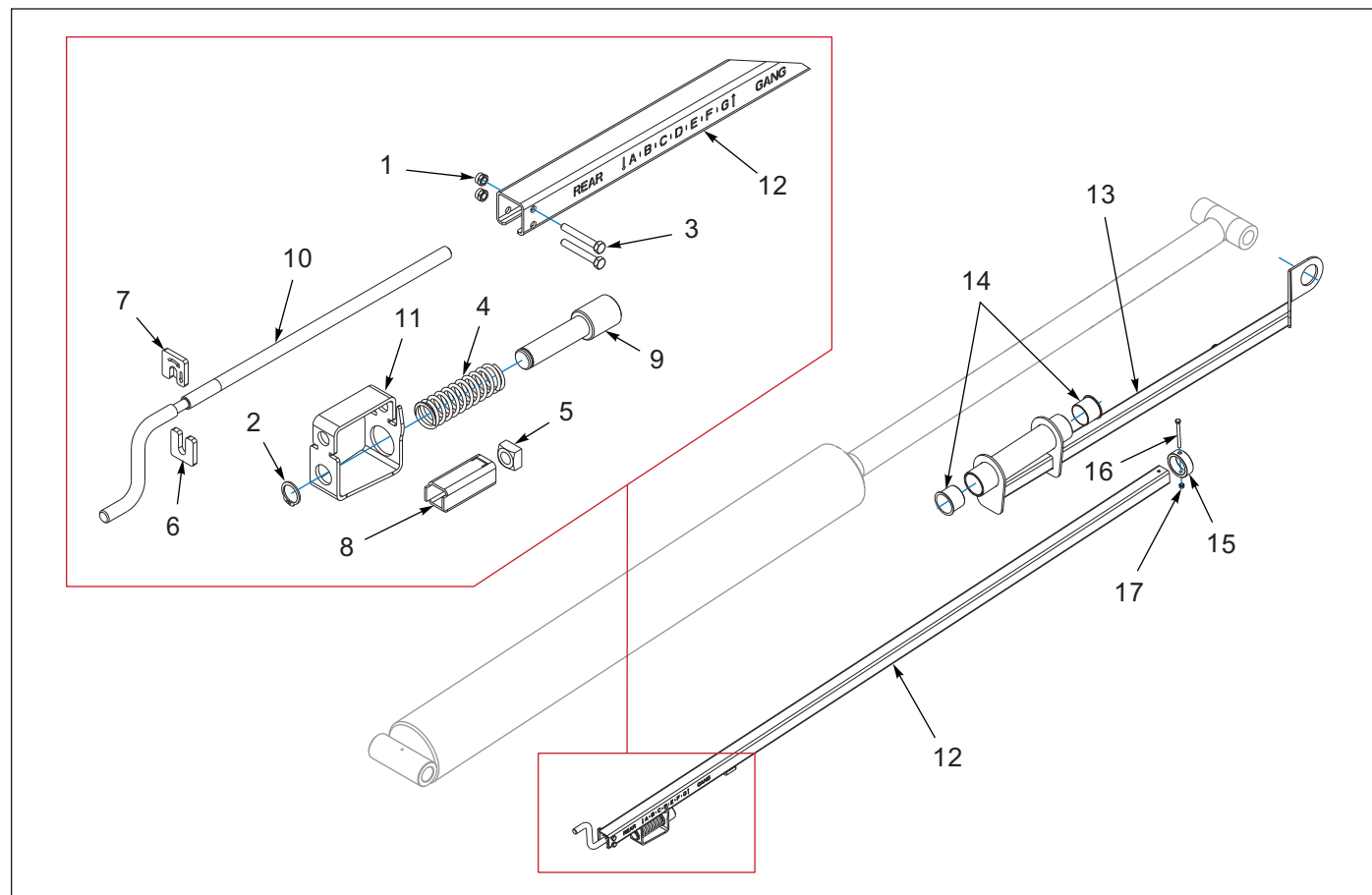
Figure 4-6: Tilt Stop Assembly (AFTER 05/2024)
