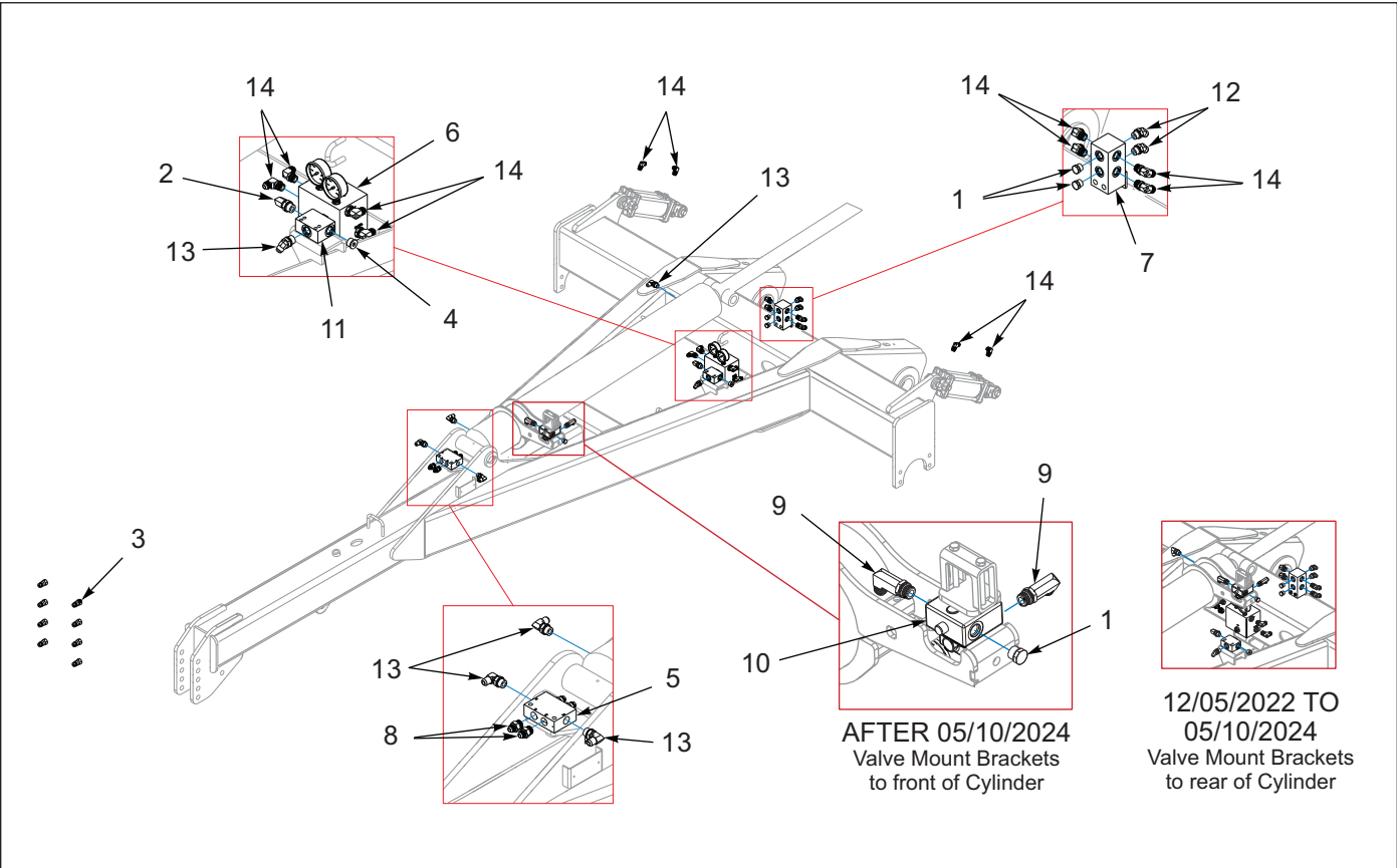
Figure 12-1: Hydraulic Hitch Kit (AFTER 12/05/2022)
