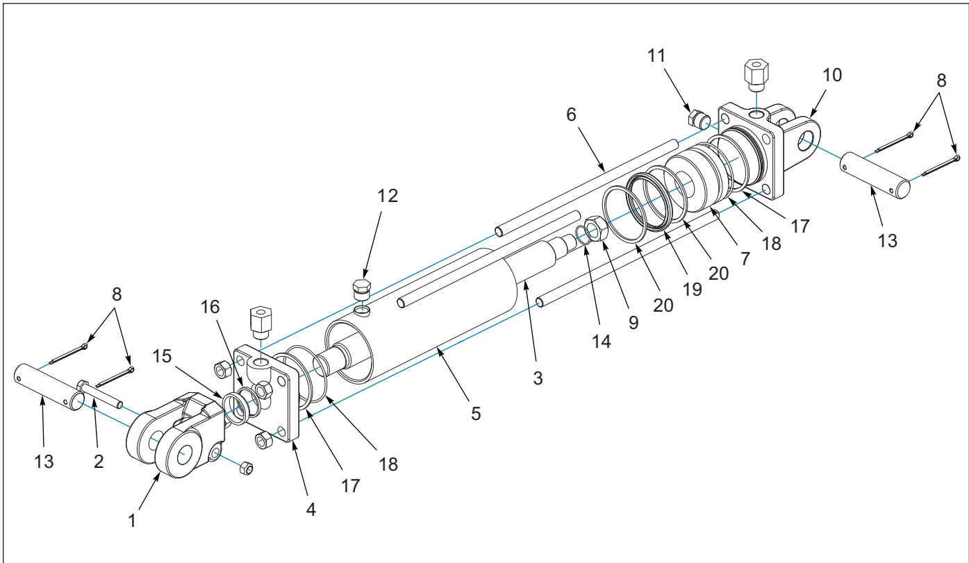
Figure 12-18: Hydraulic Cylinder, 4-1/2 x 8 - 177389
