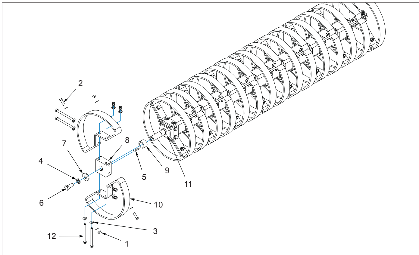
Figure 9-10: Hemi Spring Reel Assembly
