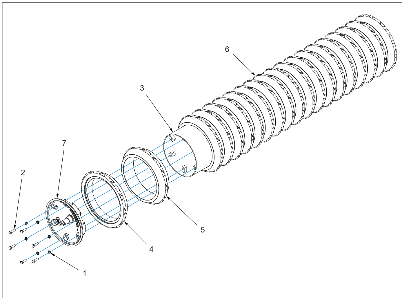
Figure 11-7: Rubber Roller Assemblies
