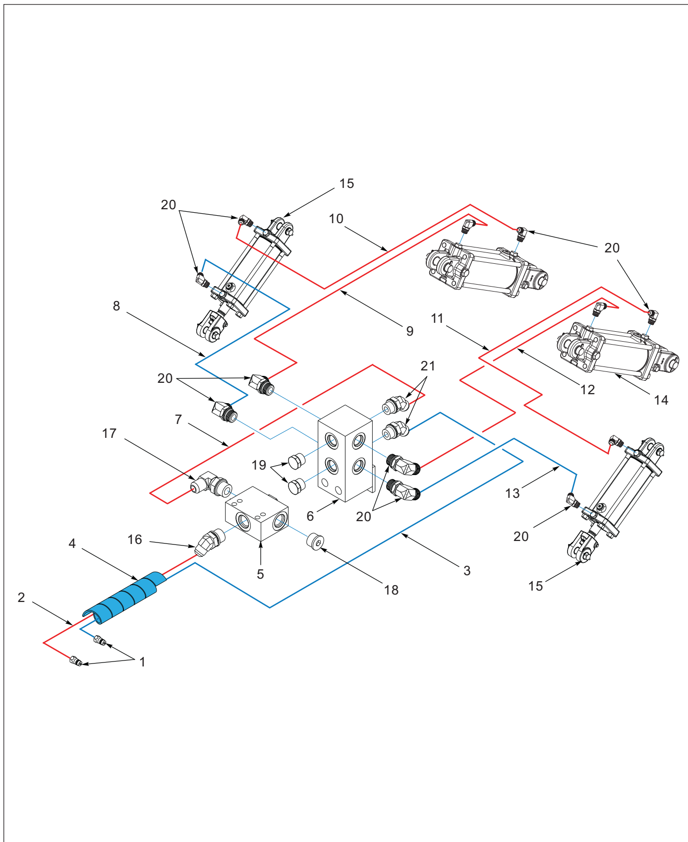
Figure 12-6: Hydraulic System - Front Gauge - 17', 20', 23'
