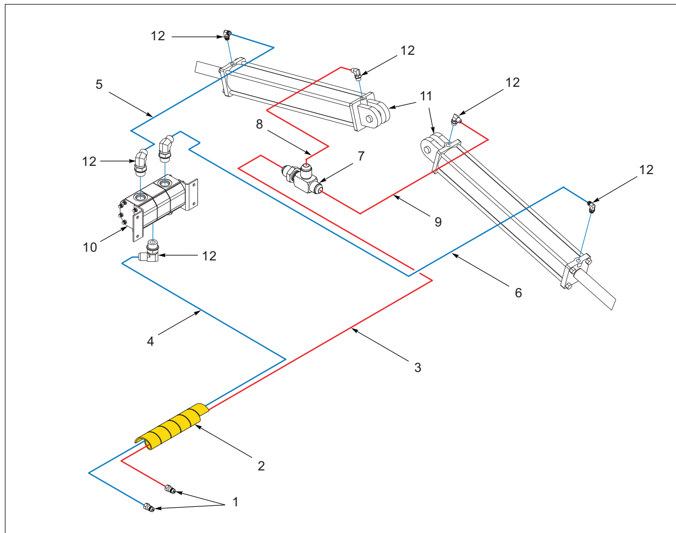
Figure 12-8: Hydraulic System - Wing Fold Down Circuit - 15'
