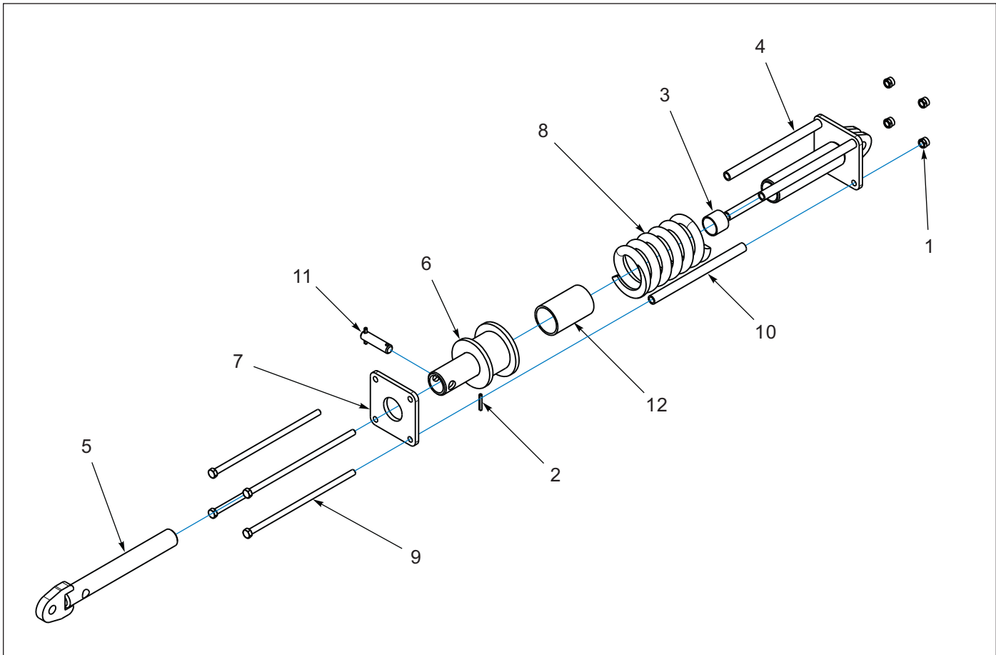
Figure 9-13: Link Spring Cylinder Assemblies
