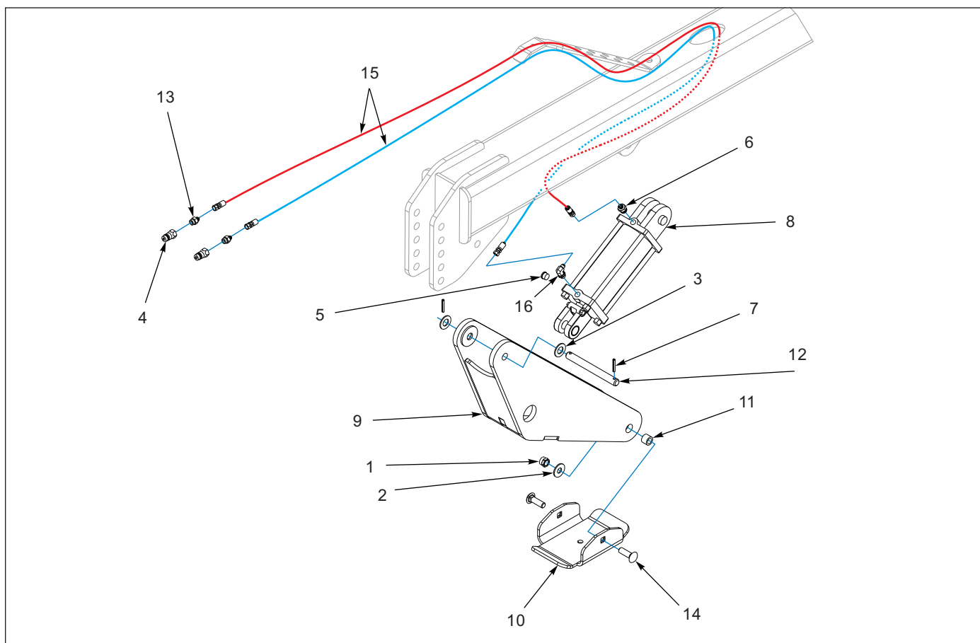
Figure 12-10: Hydraulic Jack Assembly
