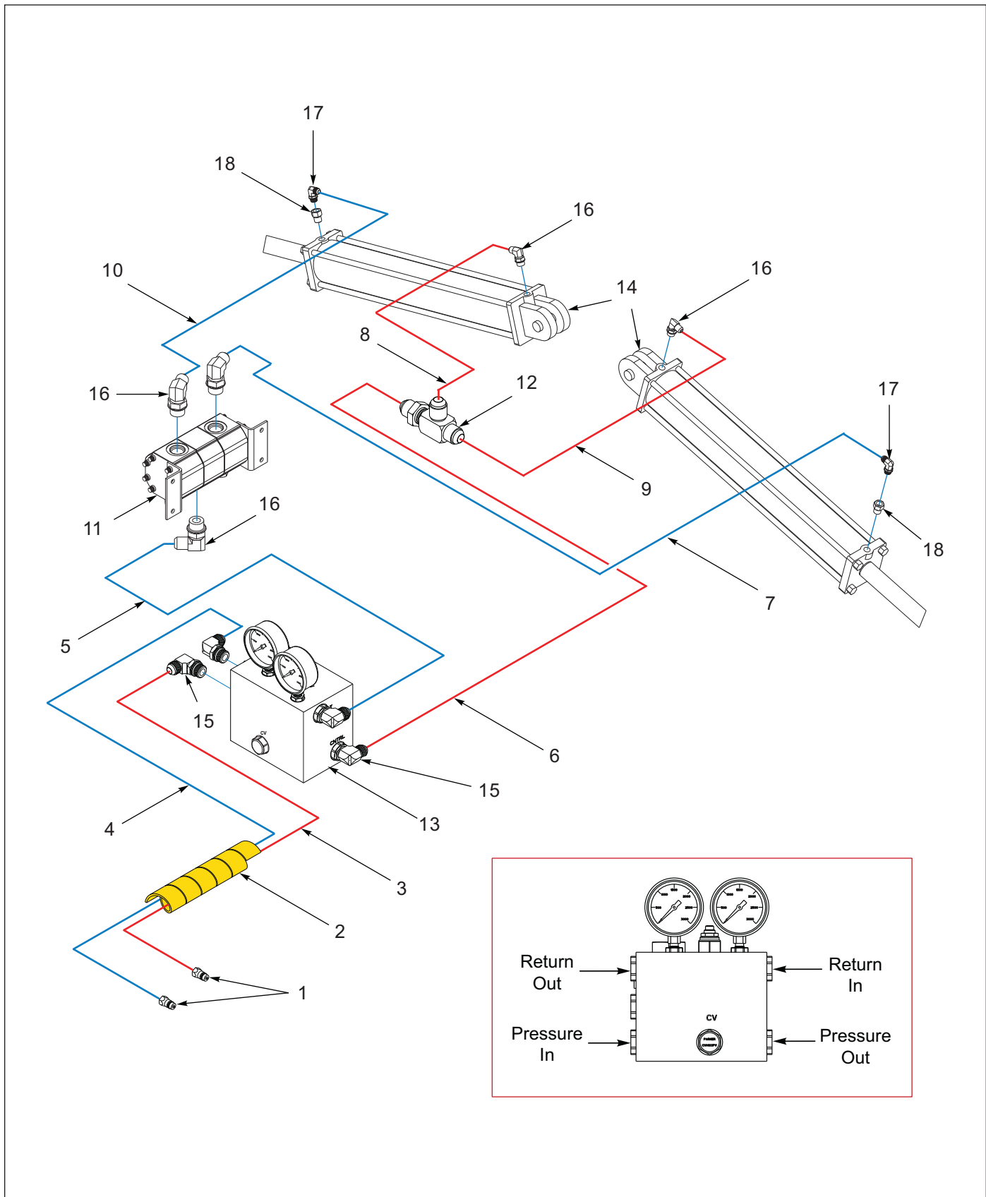
Figure 12-9: Hydraulic System - Wing Fold Down Circuit - 17', 20', 23'
