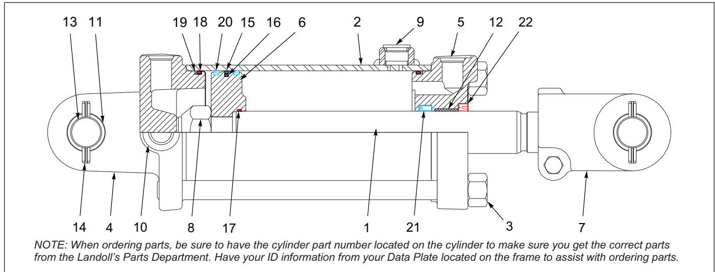
Figure 12-11: Hydraulic Cylinder, 3-3/4 x 8 - 145202
