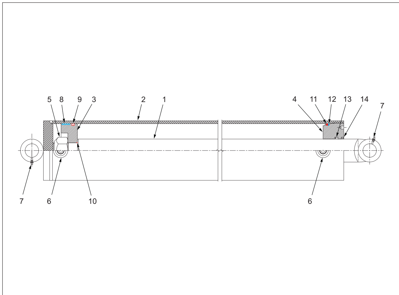
Figure 12-19: Hydraulic Cylinder, 7 x 60 - 187436
