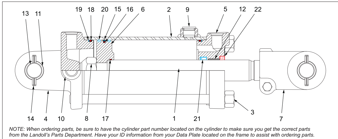
Figure 12-14: Hydraulic Cylinder, 4 x 8 - 145201
