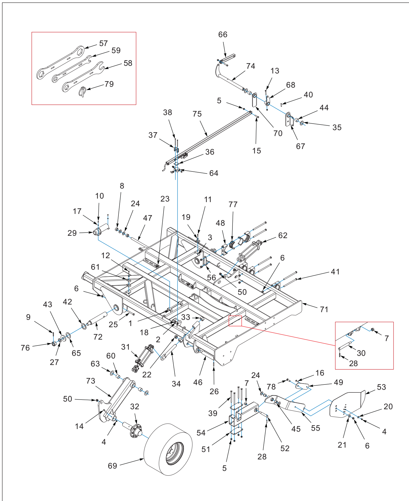
Figure 2-3: Wing Assembly - Left Hand 20'
