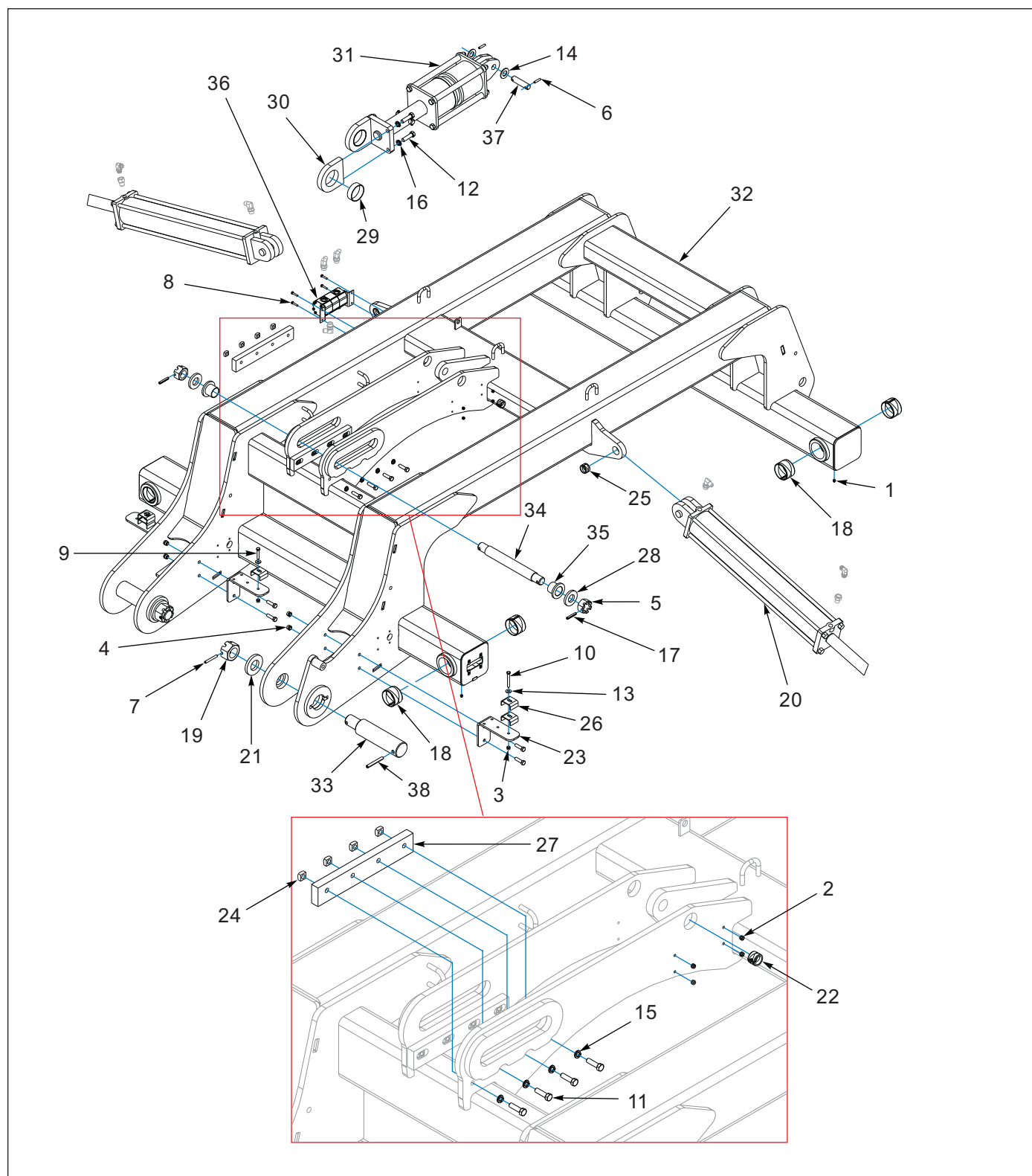
Figure 1-1: Center Frame Assembly
