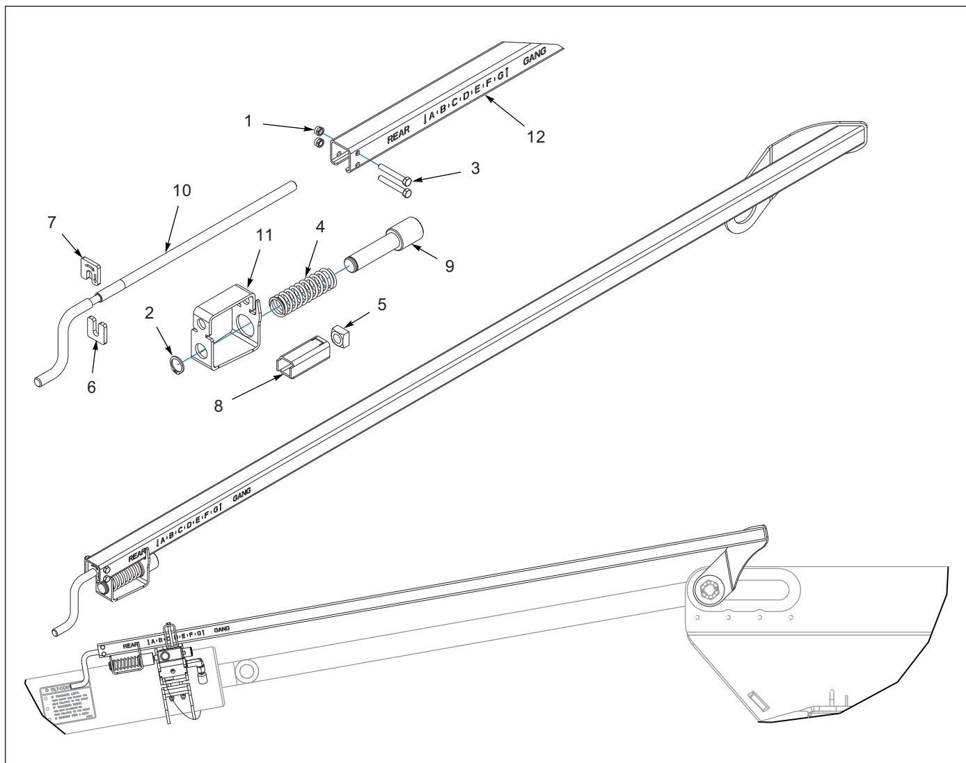
Figure 4-7: Tilt Stop Assembly (12/2022 TO 05/2024)
