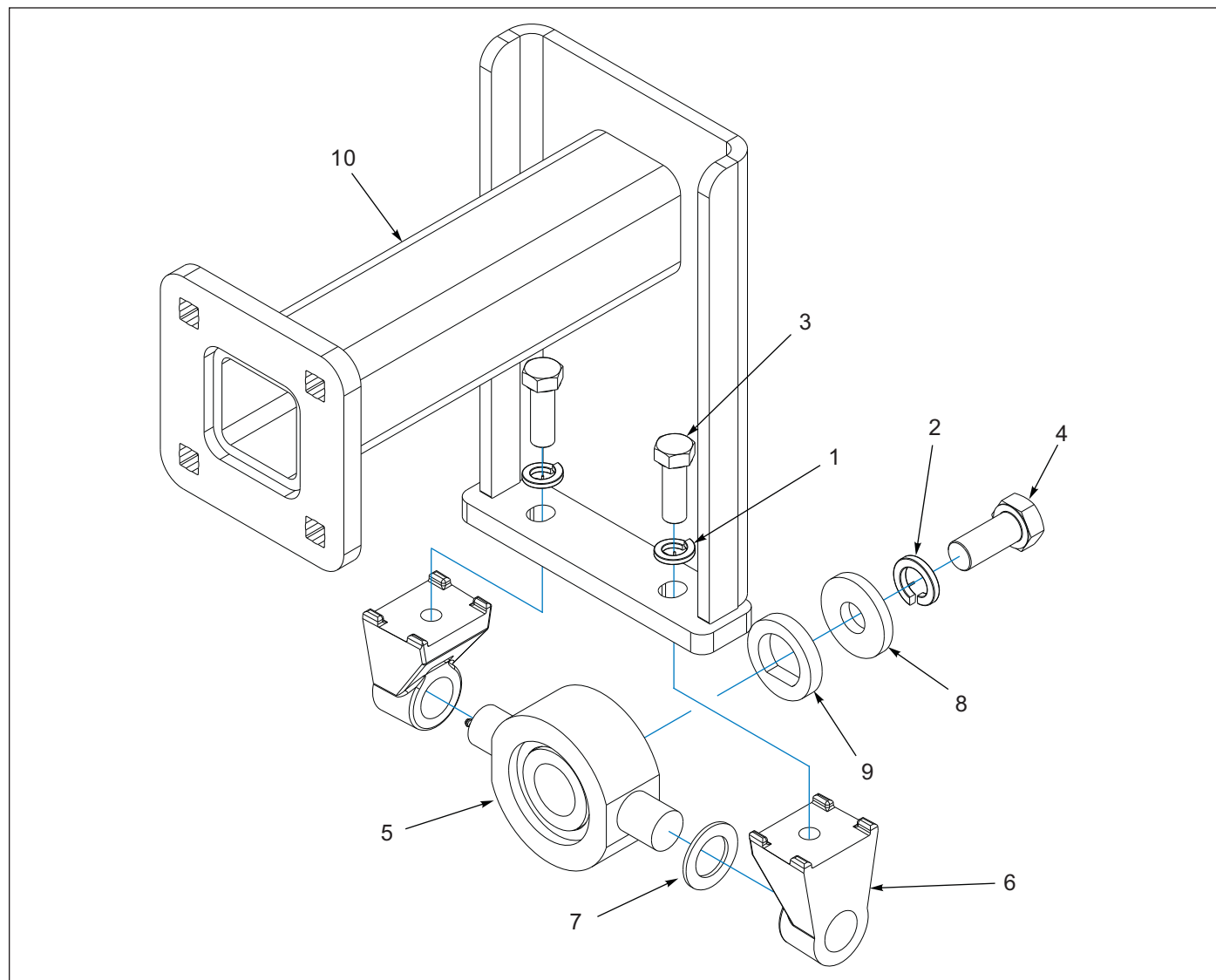
Figure 9-12: Spring Reel Extension Assemblies
