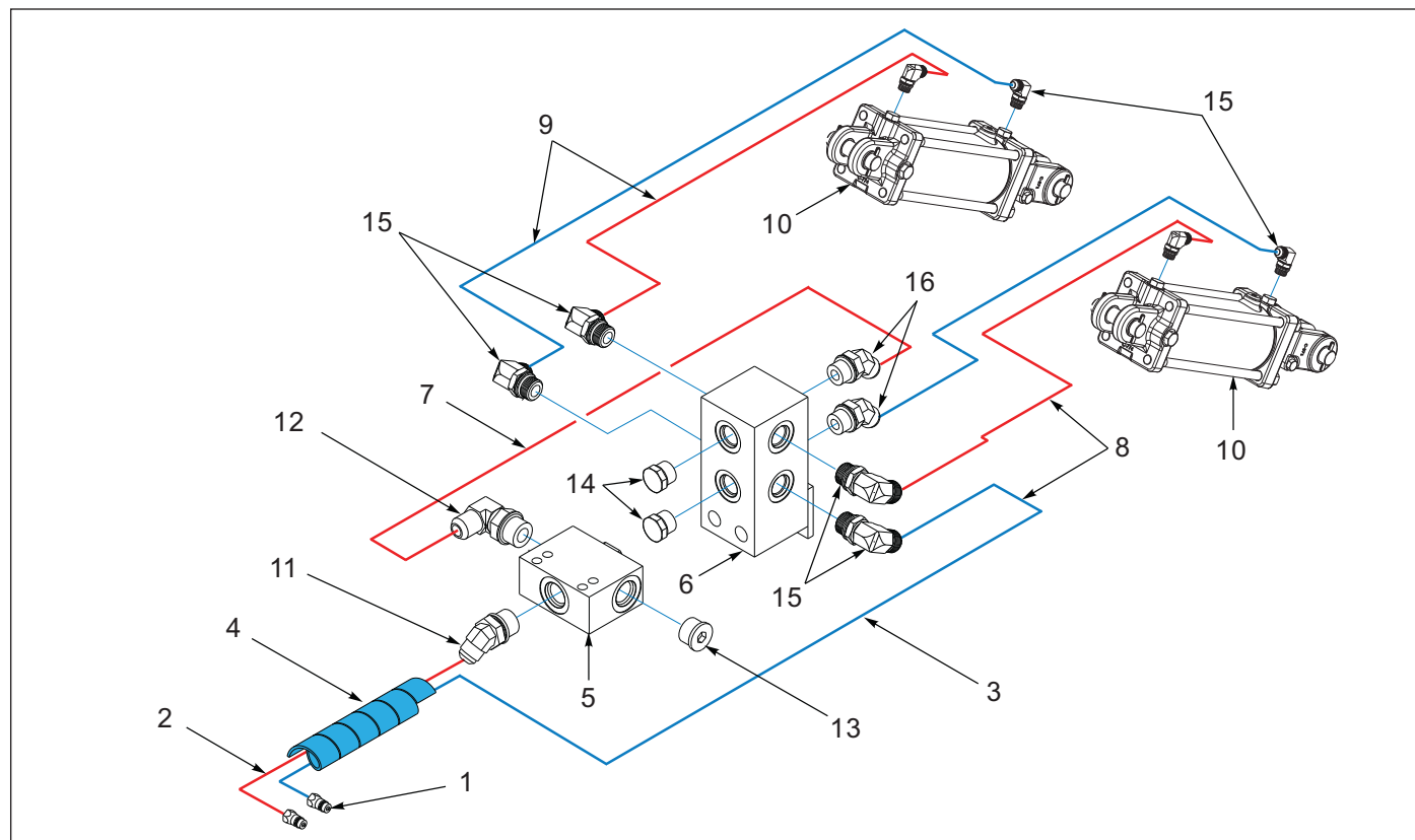
Figure 12-5: Hydraulic System - Front Gauge - 15'
