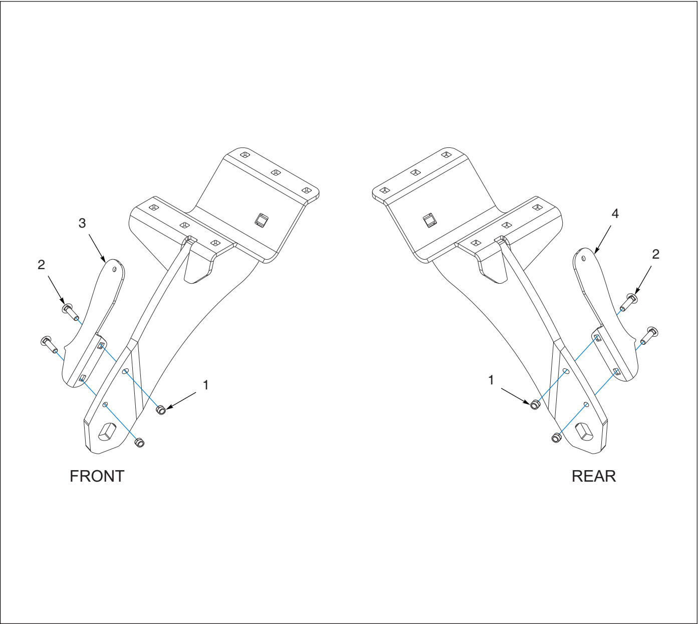
Figure 8-1: Scraper, Disc Blade
