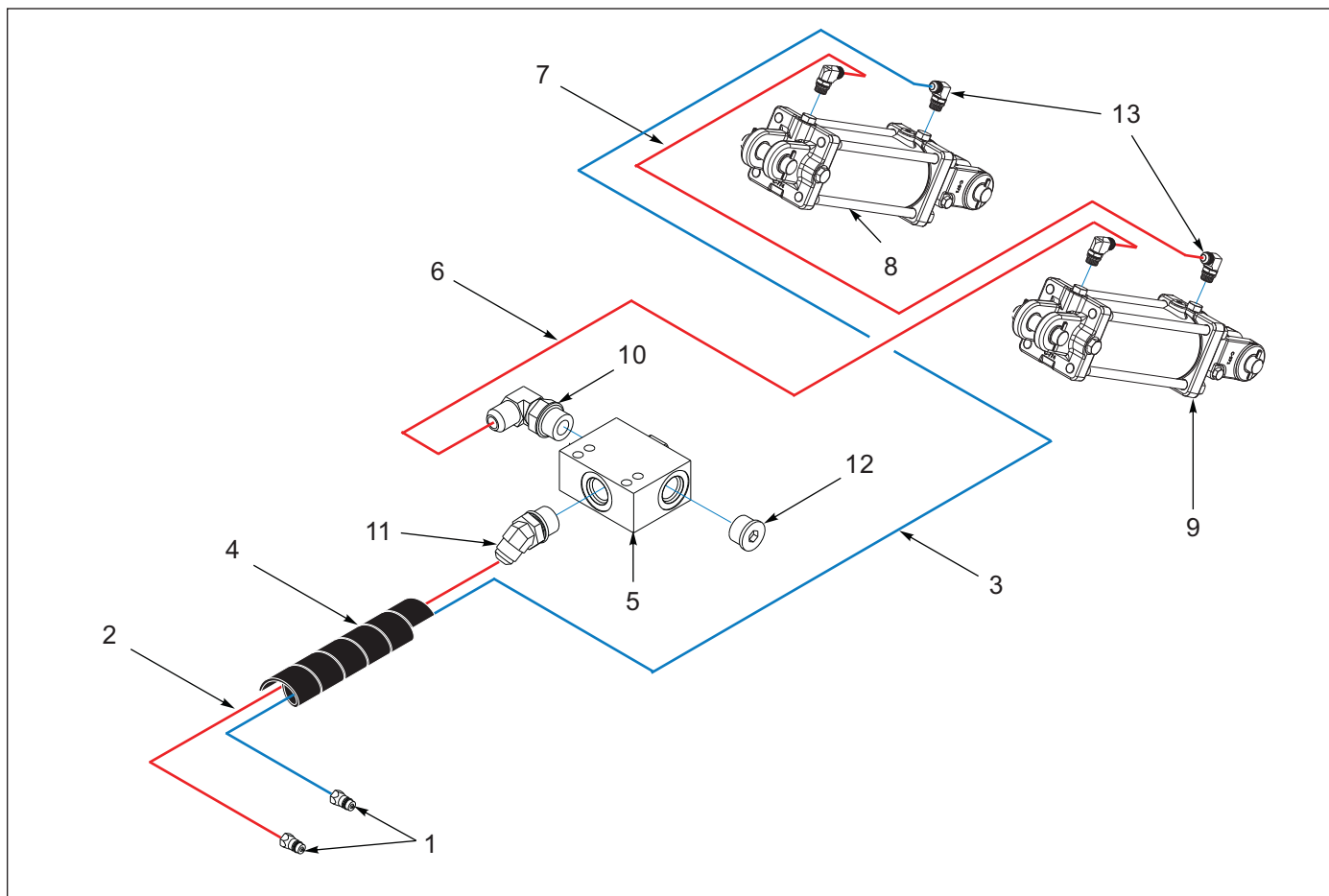
Figure 12-7: Hydraulic System - Rear Reel/Roller Circuit
