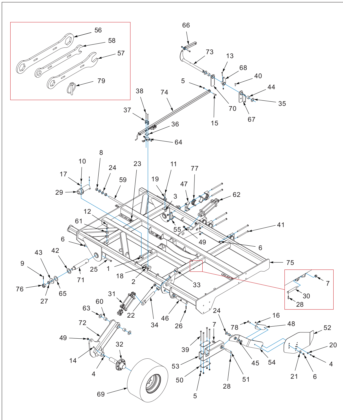
Figure 2-4: Wing Assembly - Left Hand 23'
