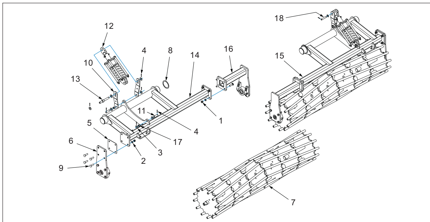
Figure 10-1: Chevron Single Reel Assembly - 15'
