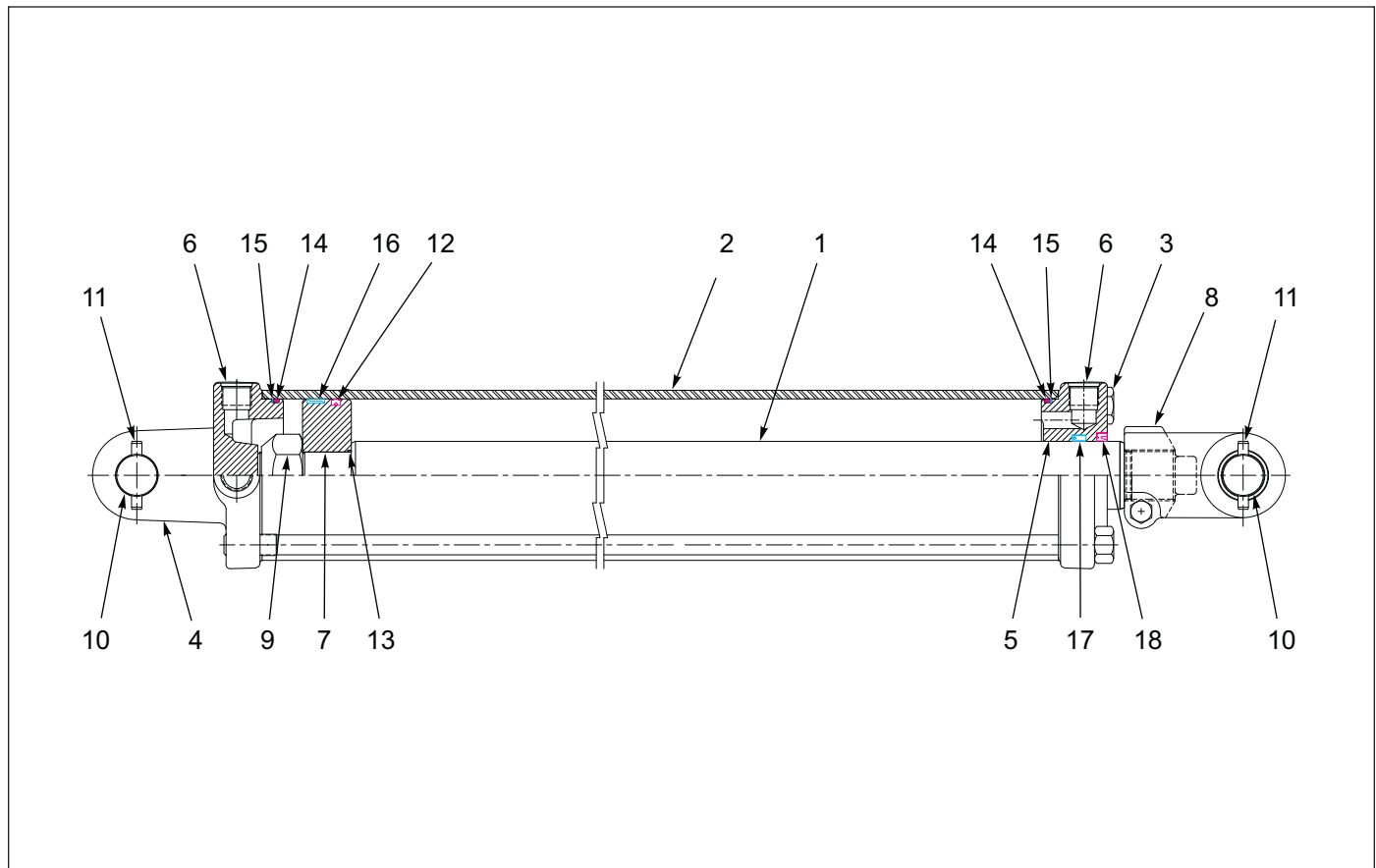
Figure 12-17: Hydraulic Cylinder, 4-1/2 x 30 - 176035
