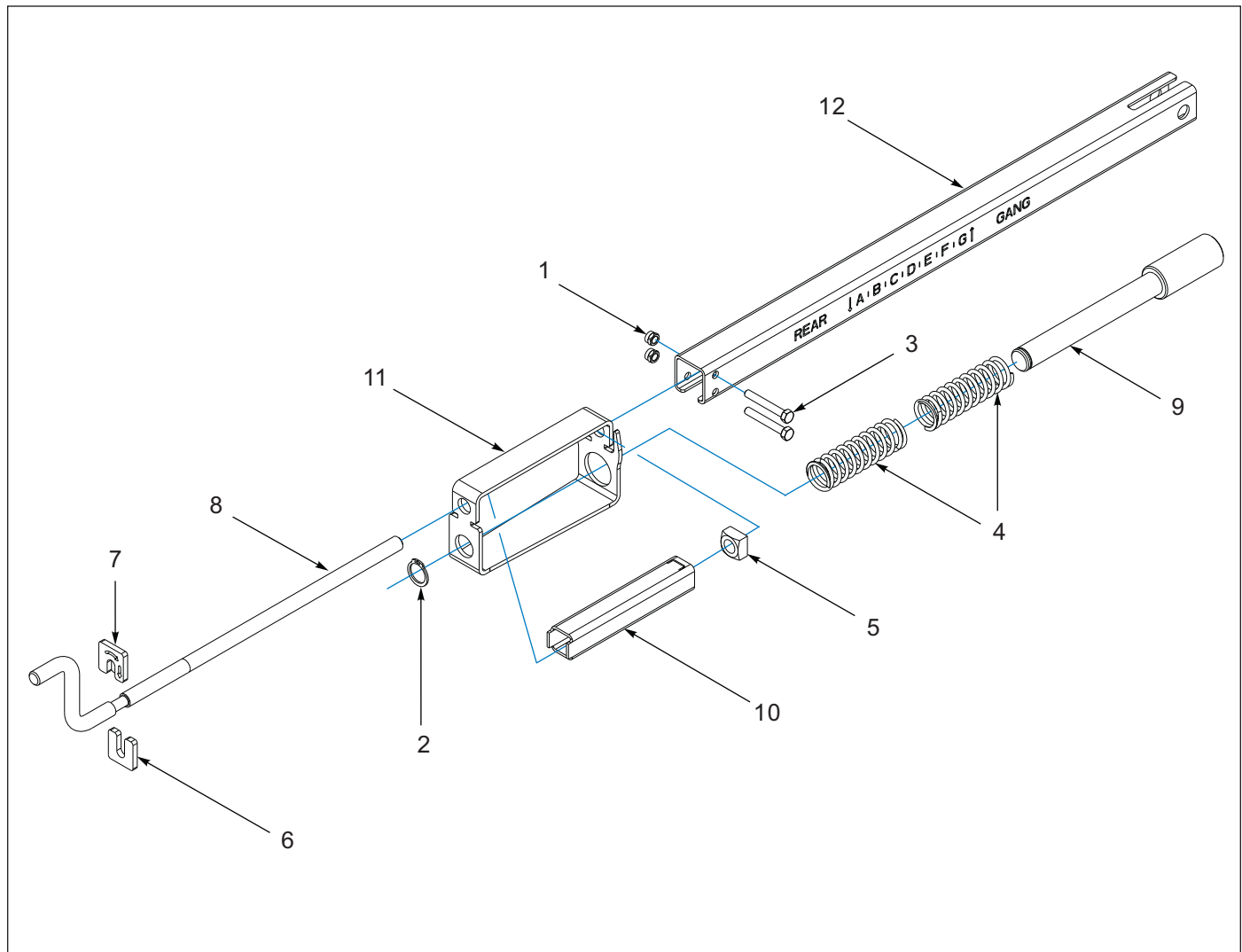
Figure 4-8: Tilt Stop Assembly (BEFORE 12/2022)
