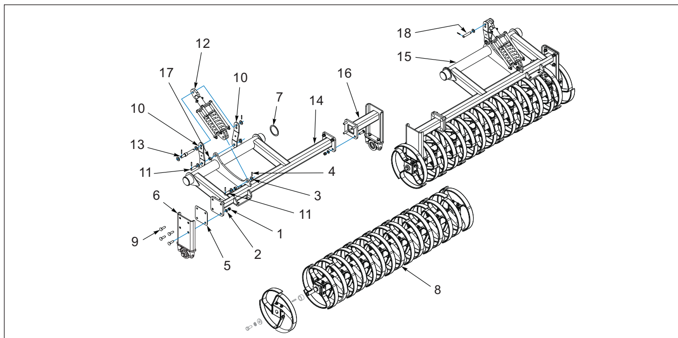
Figure 9-1: Spring Reel Assembly - 15'
