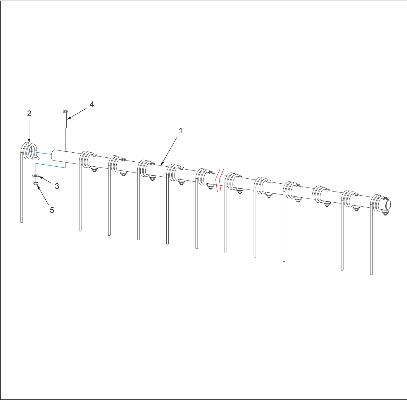
Figure 1-8: Coil Tine Harrow, 75-1/8"
