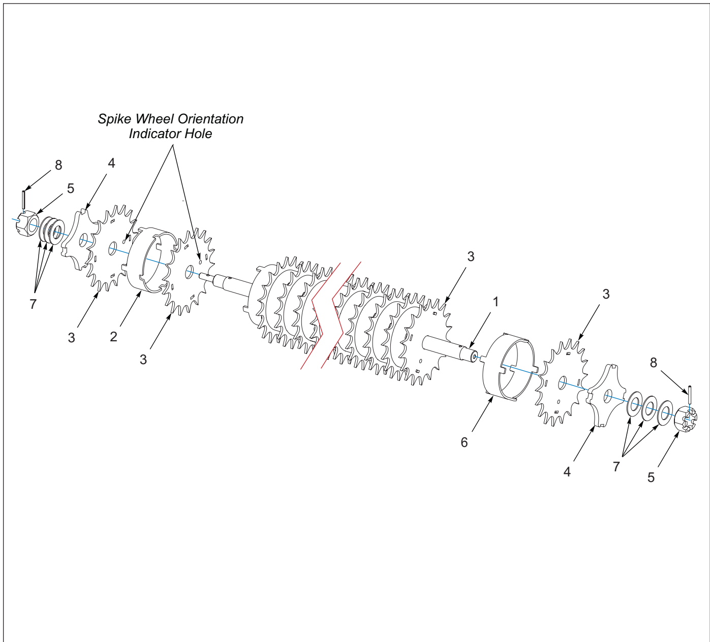
Figure 1-13: Front Spike Roller Assembly (6FT Only)
