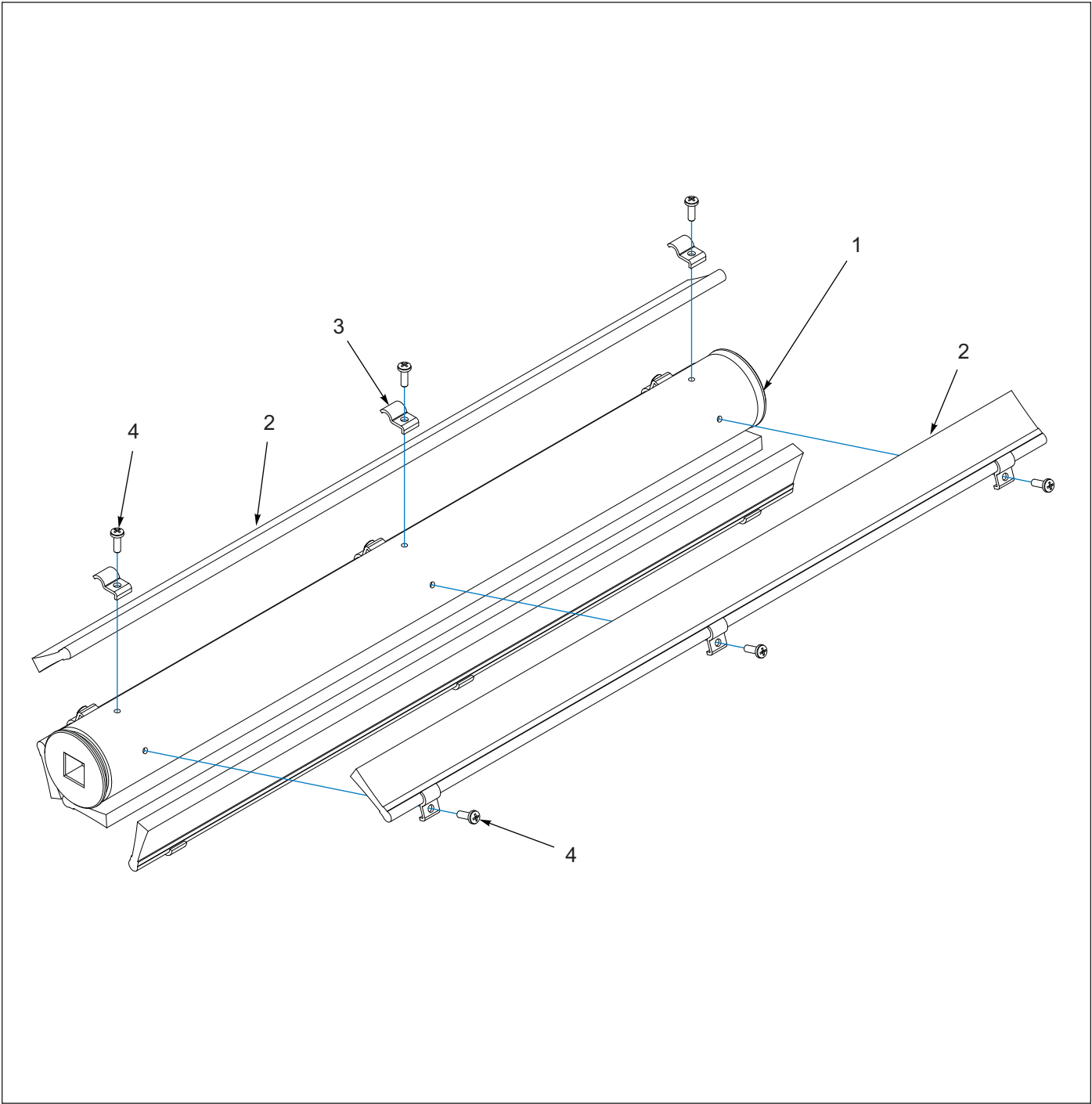
Figure 1-23: Brush Agitator Assembly - 22-1/2"
