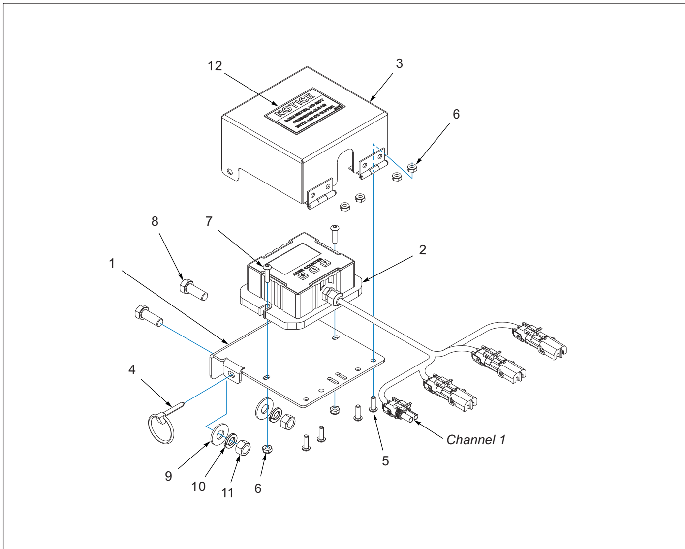
Figure 1-27: Acre Meter Assembly (After 06/01/2025)
