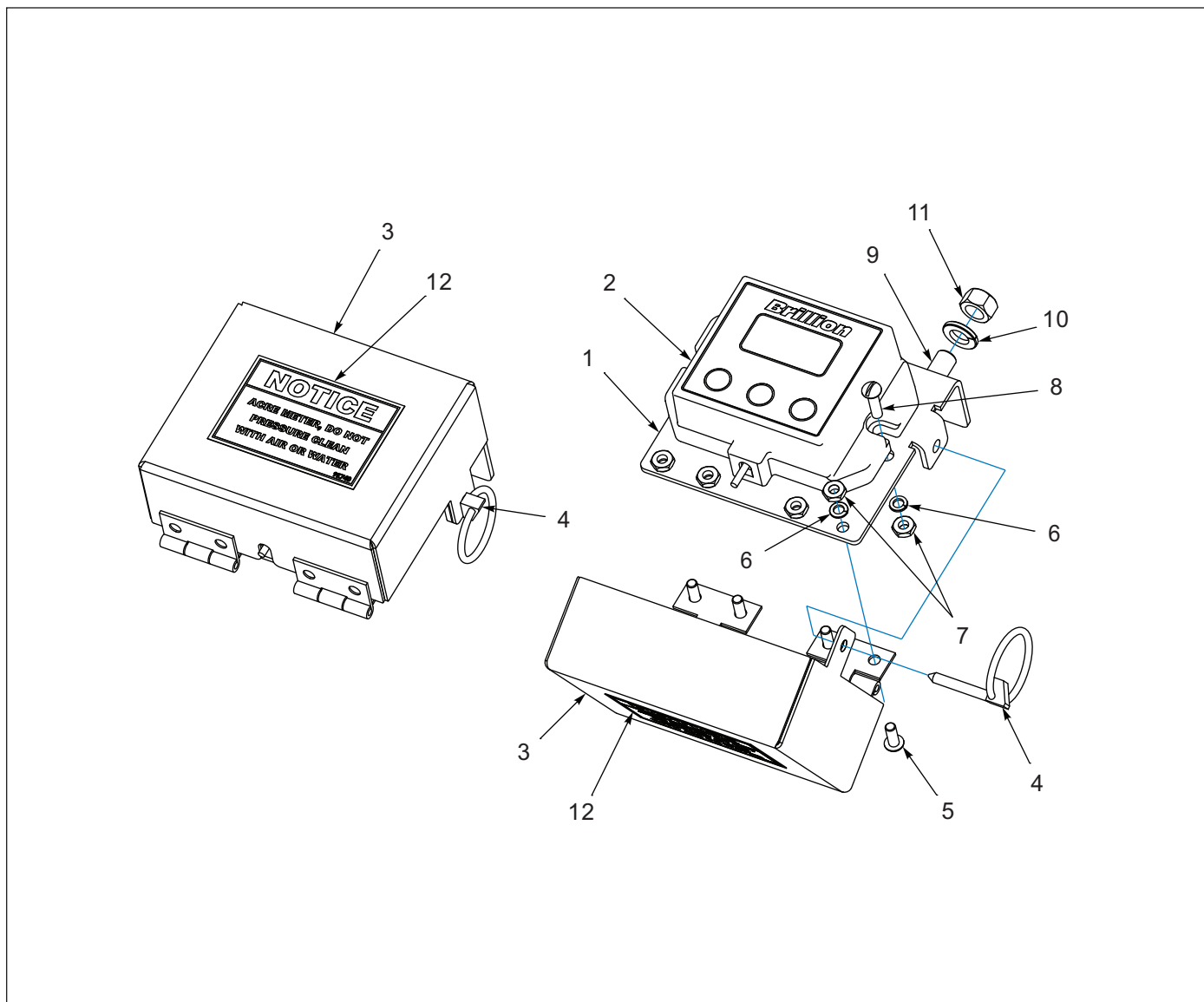
Figure 1-29: Acre Meter Assembly (Before 05/15/2012)
