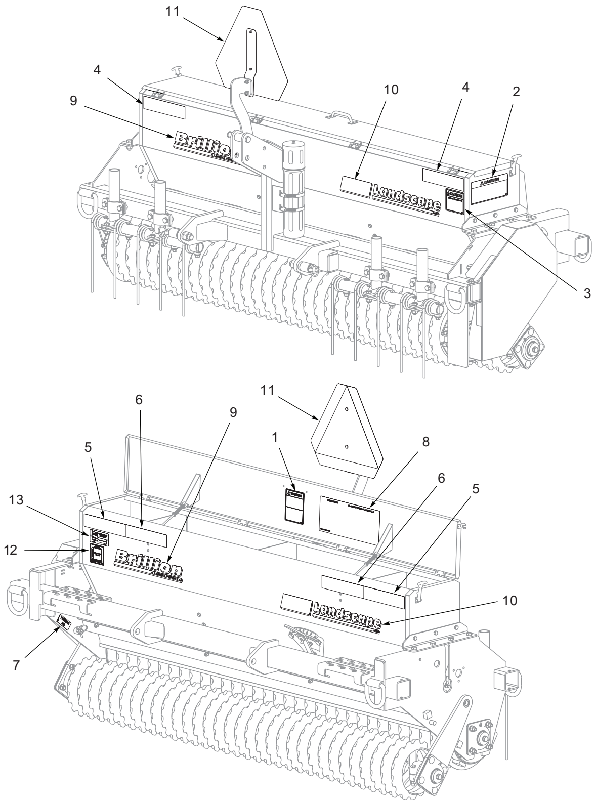
Figure 1-34: LSS6 Decal Locations (After 12/2023)
