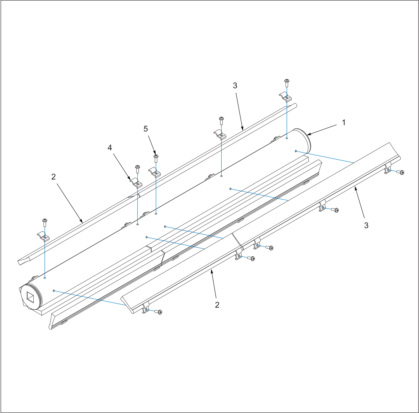
Figure 1-22: Brush Agitator Assembly - 28"
