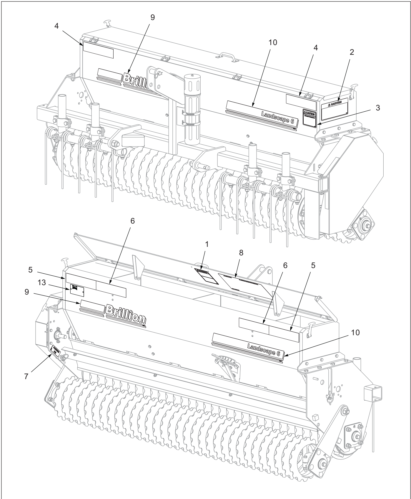
Figure 1-35: LSP Decal Locations (Before 12/2023)
