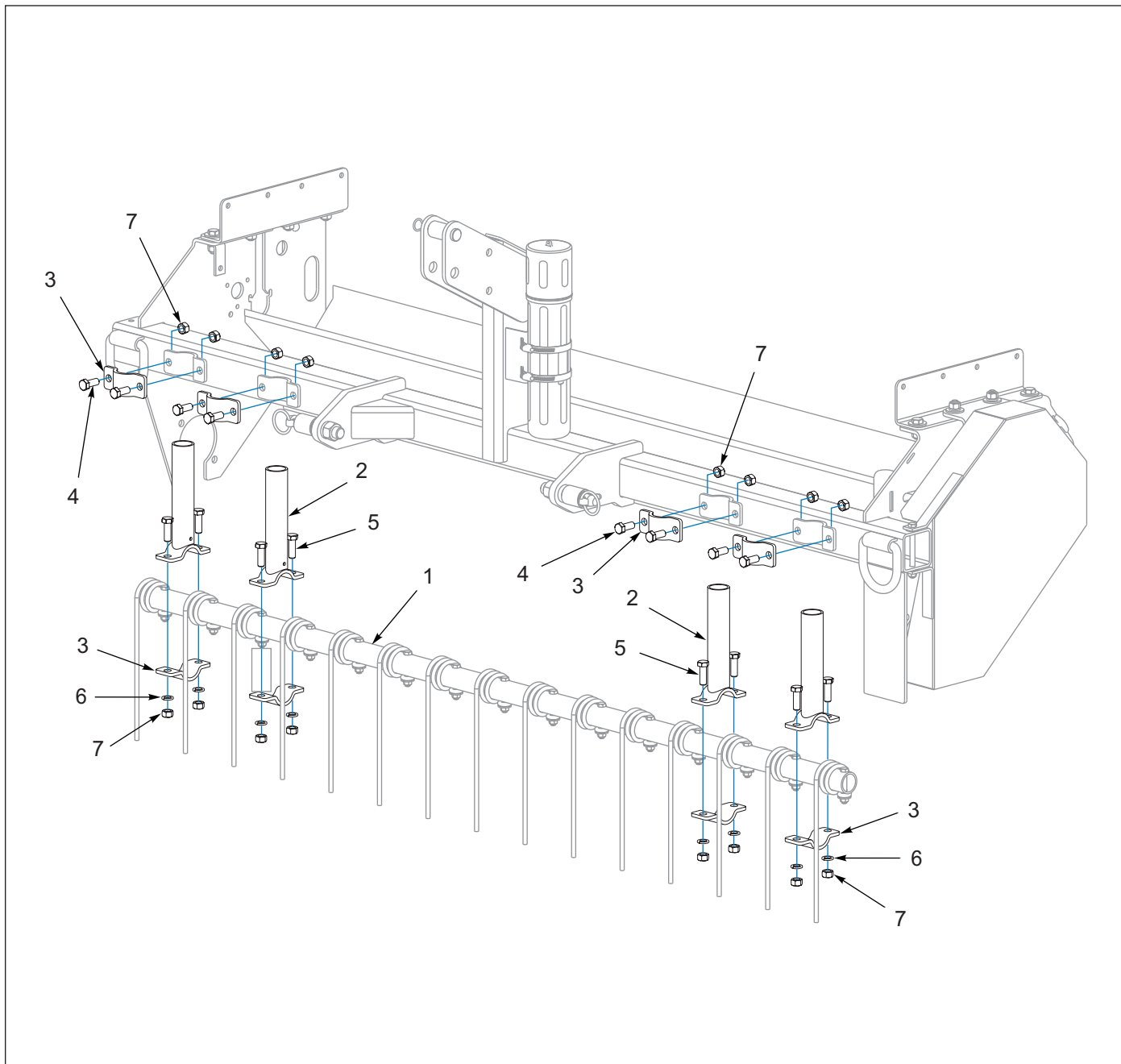
Figure 1-5: Coil Tine Harrow, 6FT (Full Width)
