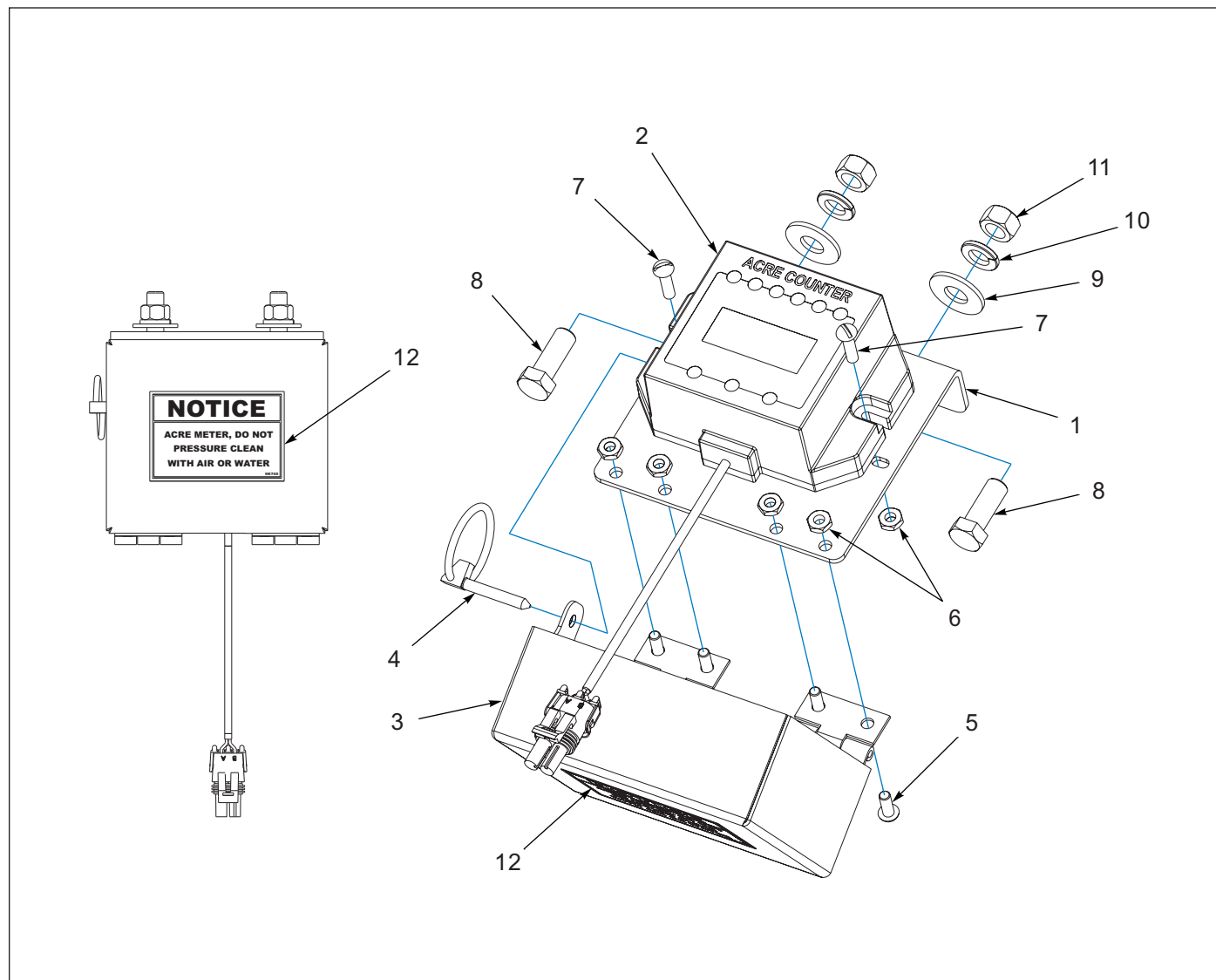
Figure 1-28: Acre Meter Assembly (05/15/2012 TO 06/01/2025)
