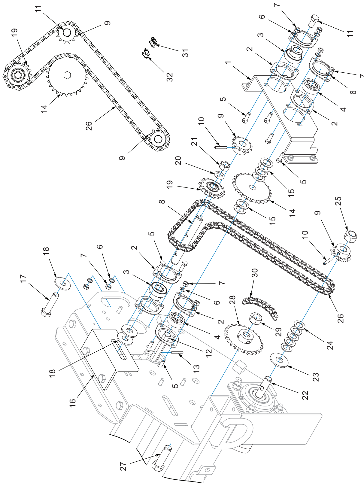
Figure 1-18: Transmission Assembly
