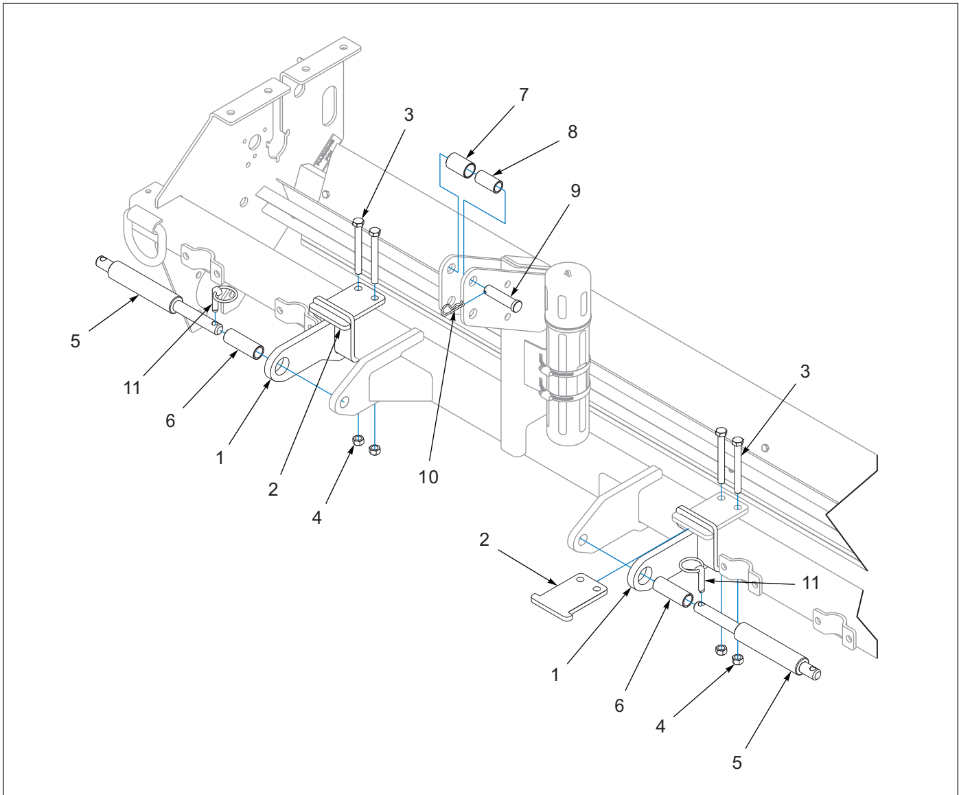
Figure 1-30: CAT2 Quick Hitch Adapter Kit - Optional
