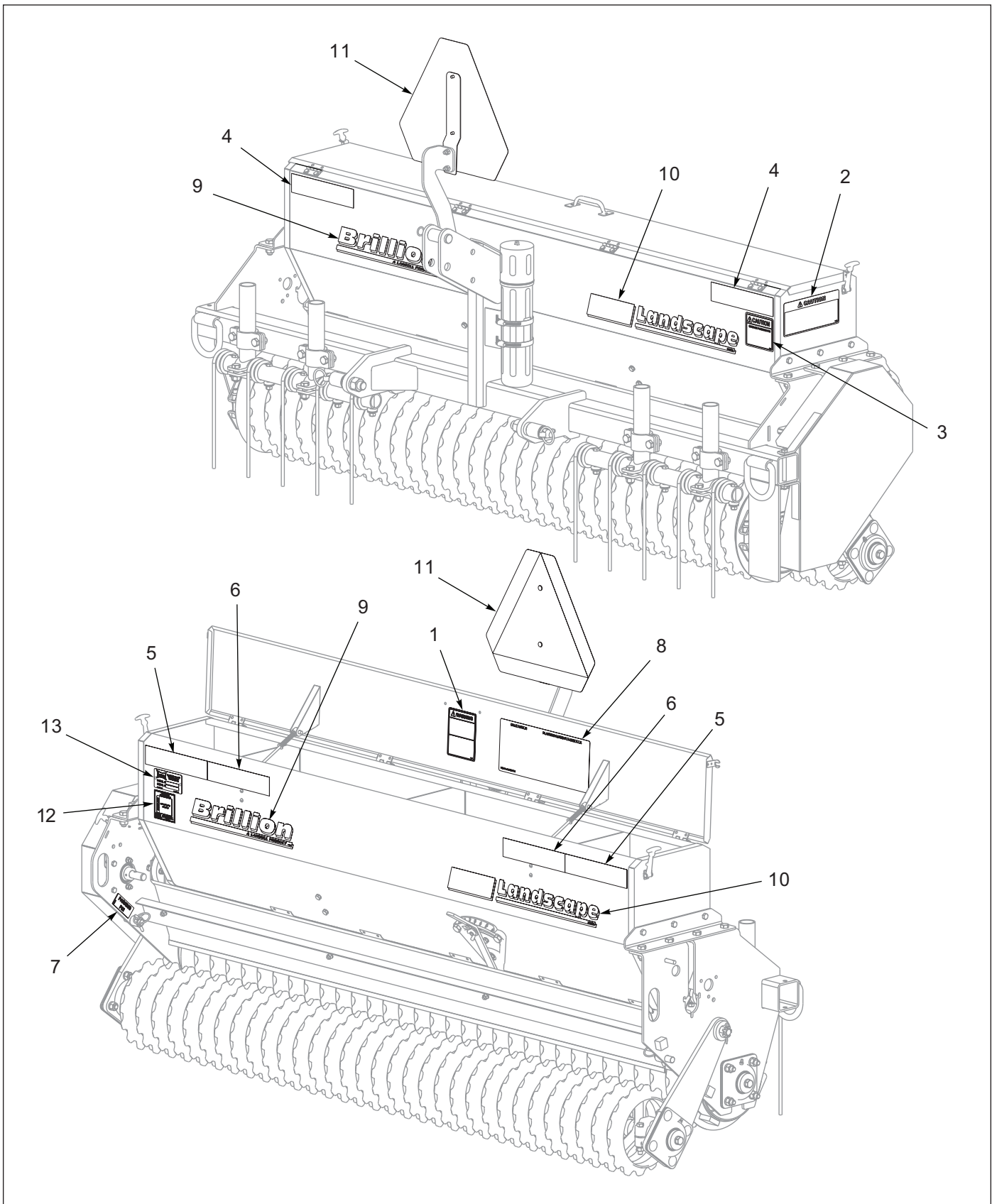
Figure 1-33: LSP Decal Locations (After 12/2023)
