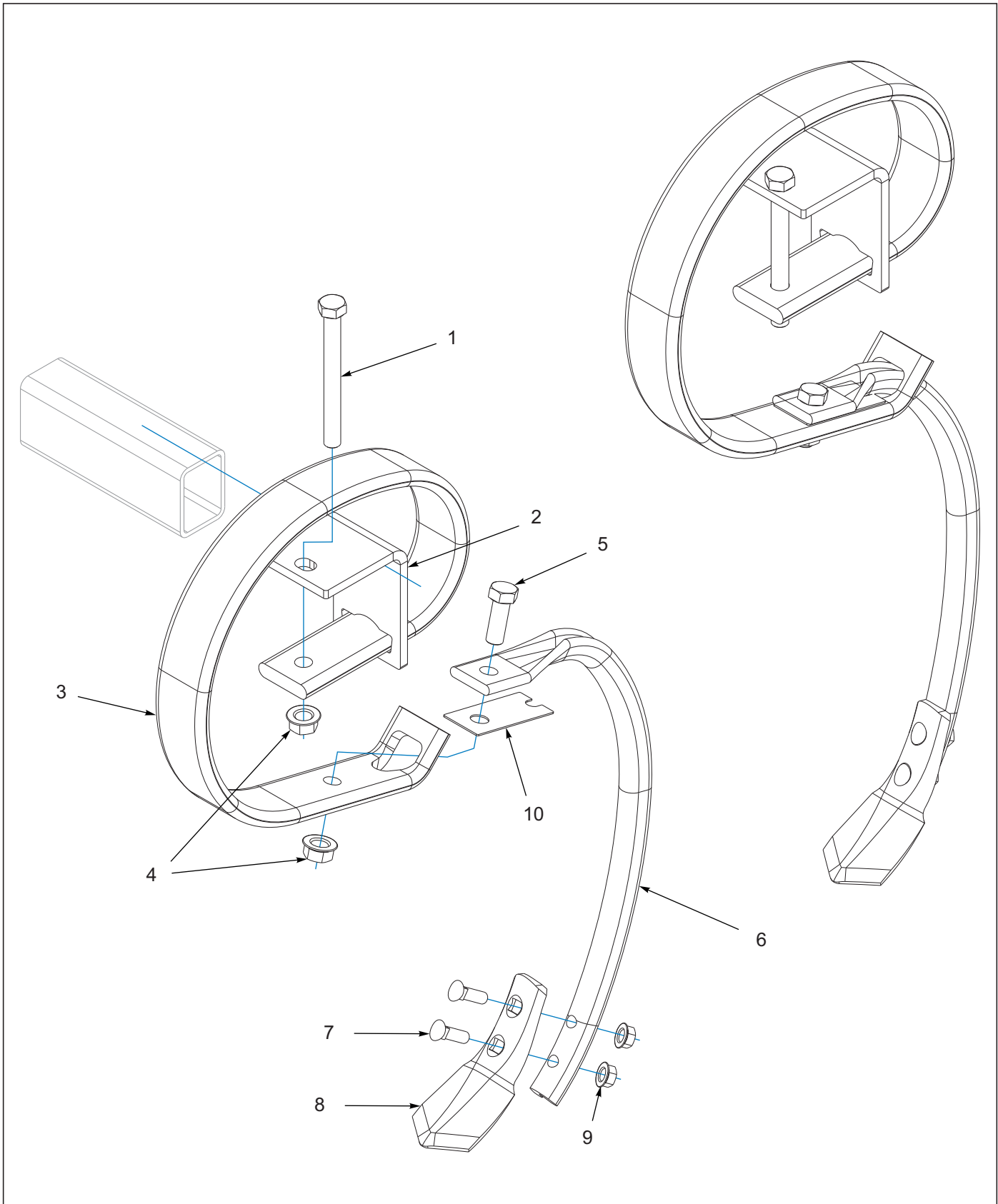
Figure 5-2: HD Tine Assembly
