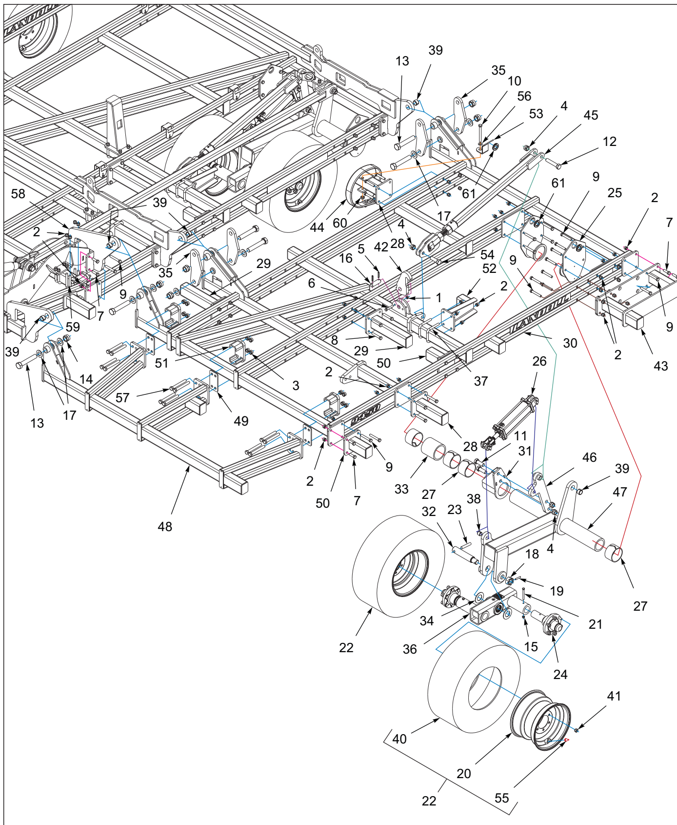
Figure 3-7: 8' Outer Wing Assembly 9450FH-46'-50'
