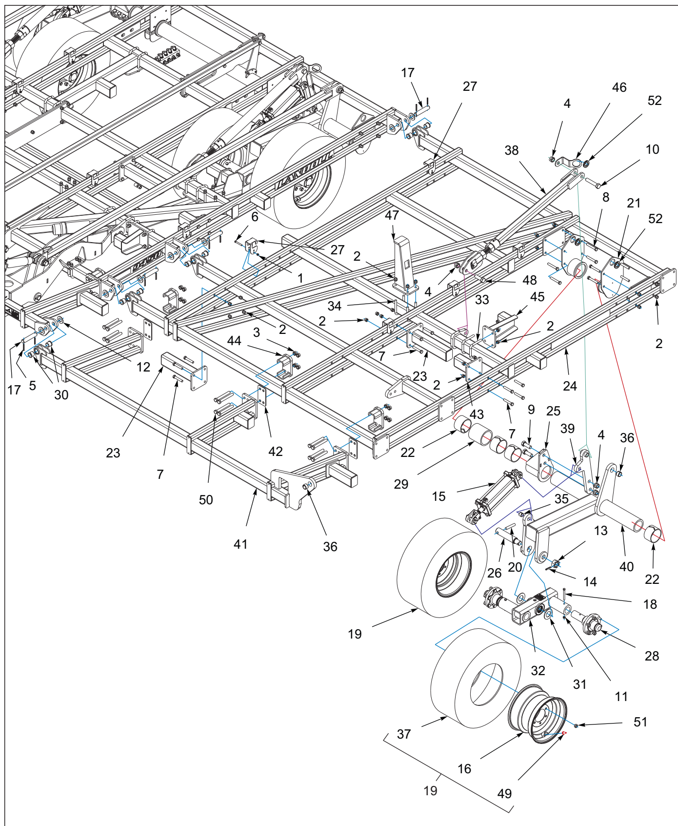
Figure 3-3: 10' Inner Wing Assembly 9450FH-46'-50'
