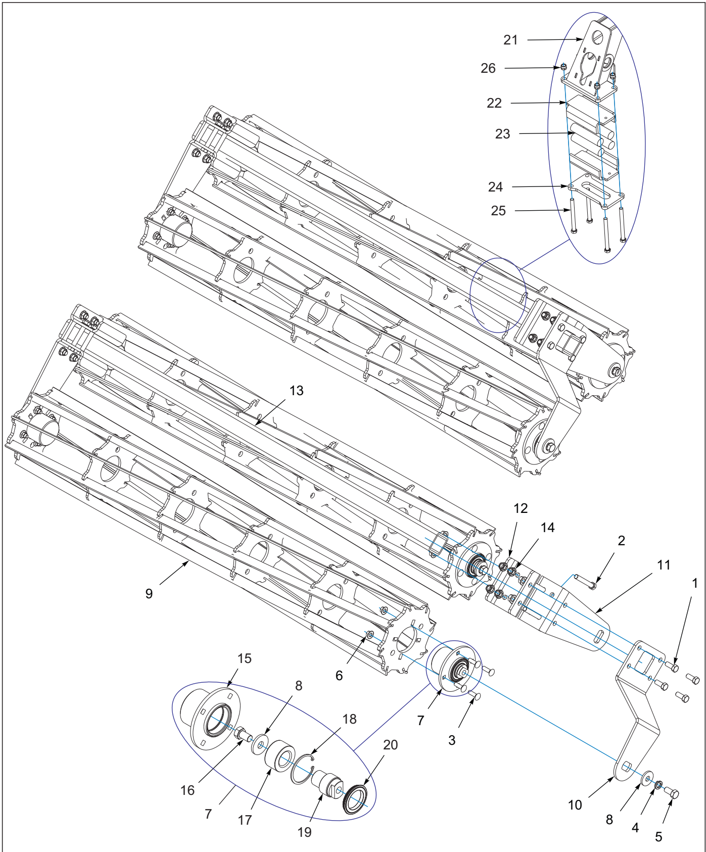
Figure 10-23: Double Flat Reel Assembly
