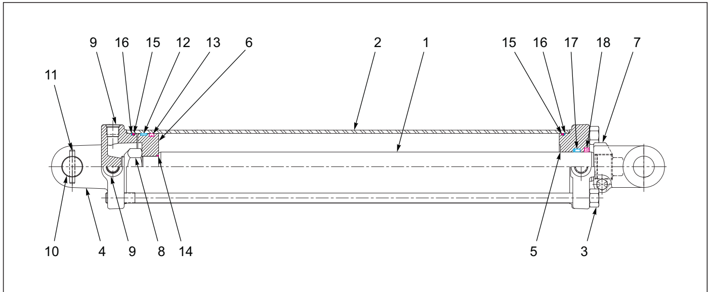
Figure 7-11: Cylinder Assembly 4-1/2 x 30 9450-38'-42'
