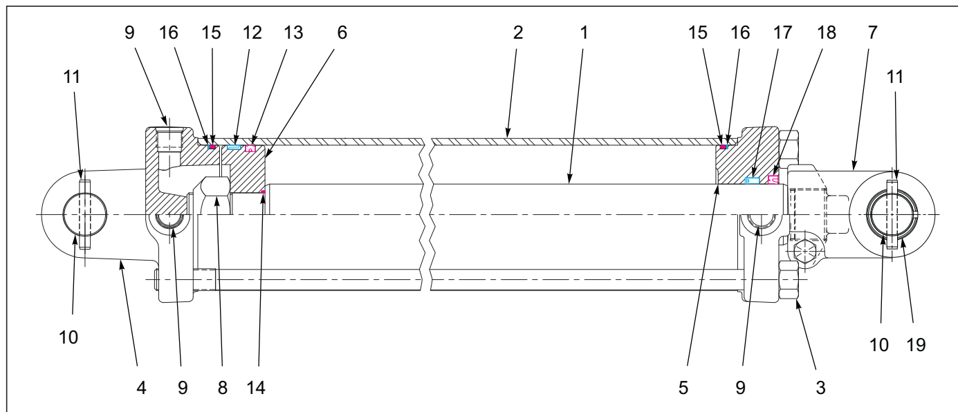
Figure 7-14: Cylinder Assembly 4 x 16 9450-46'-50'
