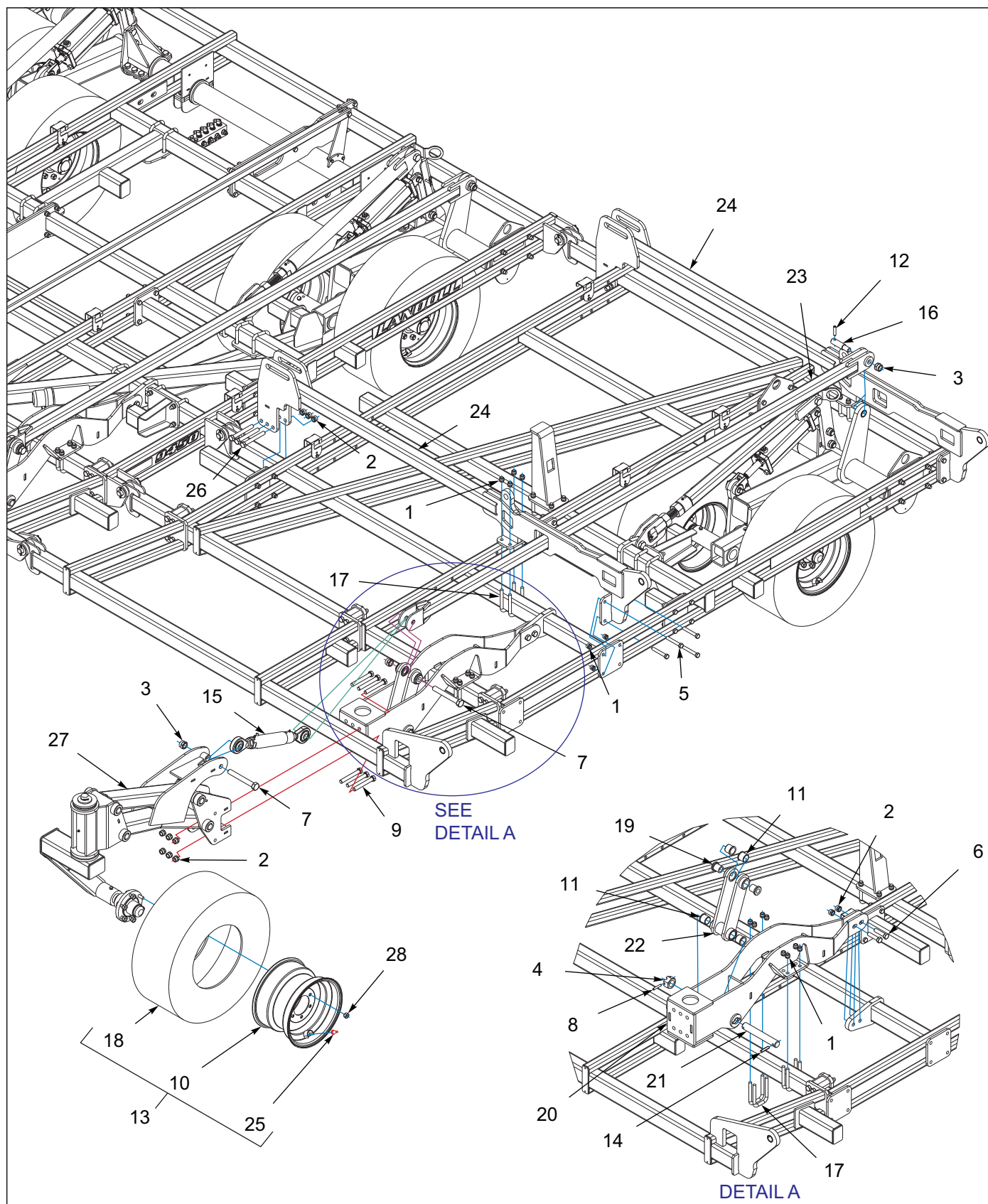
Figure 3-4: 10' Inner Wing Gauge Wheel Assembly 9450FH-46'-50'
