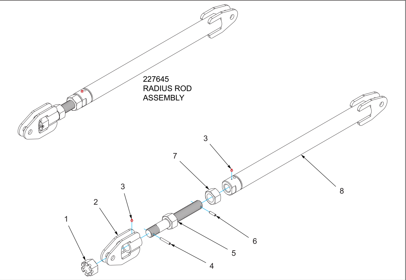
Figure 1-5: Radius Rod Assembly
