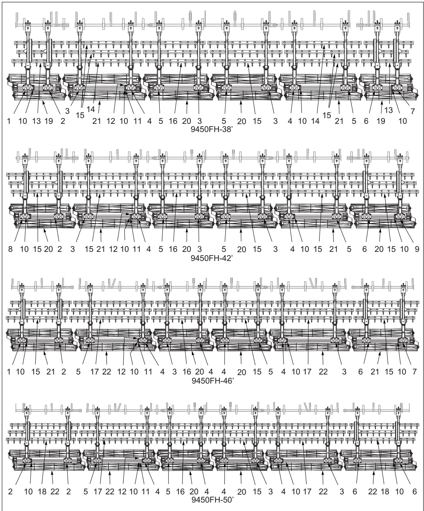
Figure 10-19: 3RS DBL Flat Reel Layout
