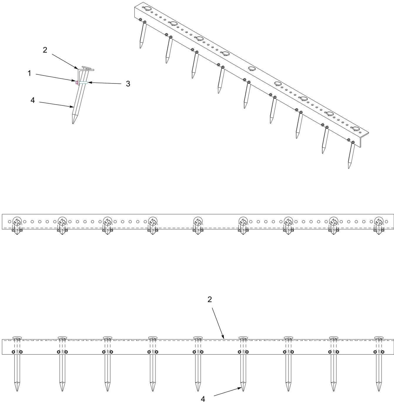
Figure 10-24: Spike Bar Assembly, 11L 9 SP
