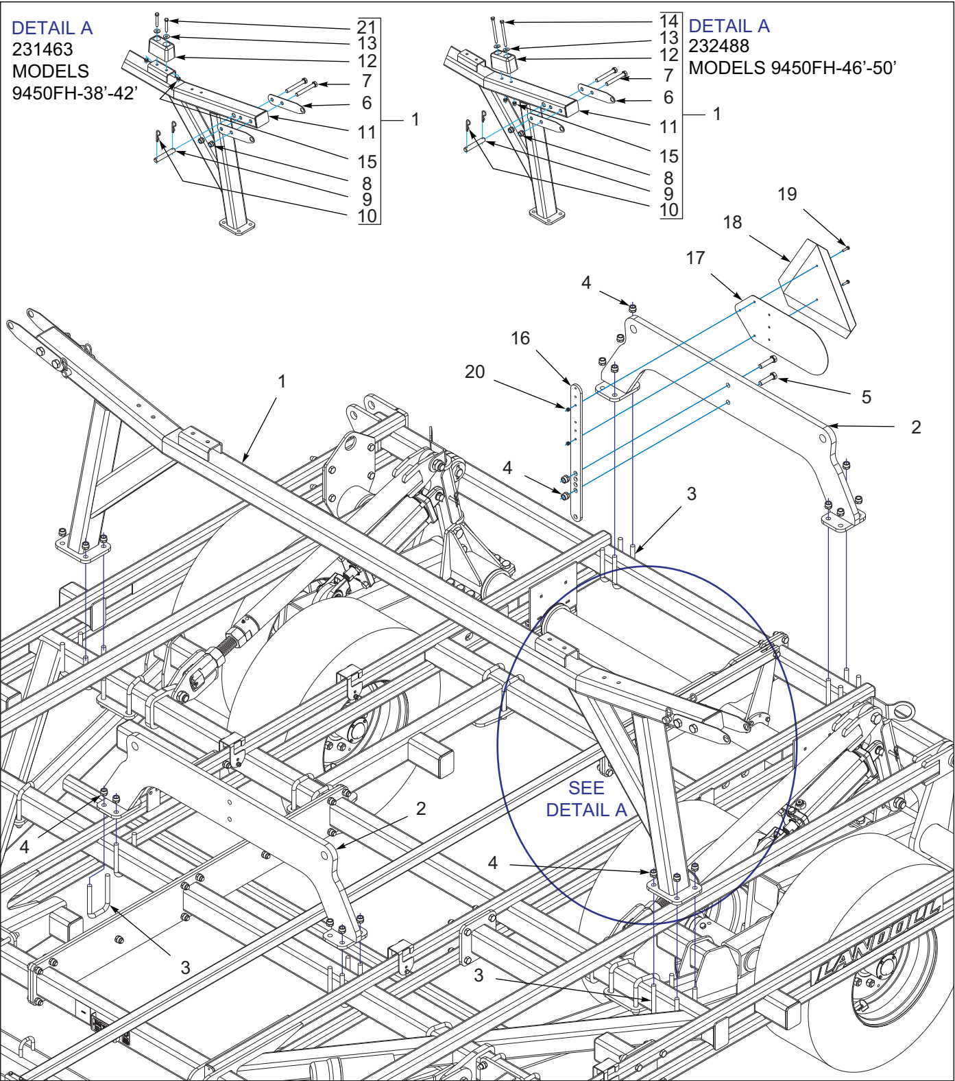
Figure 4-1: Center Frame Fold Bracket Assembly
