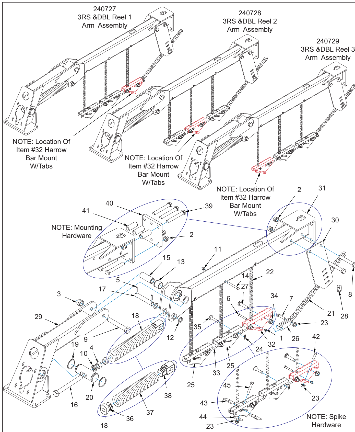
Figure 10-20: Arm Assembly 3RS and Double Reel
