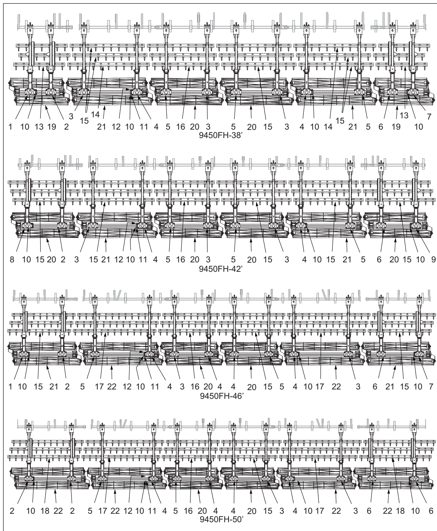
Figure 10-18: 3RS DBL Conditioner Reel Layout
