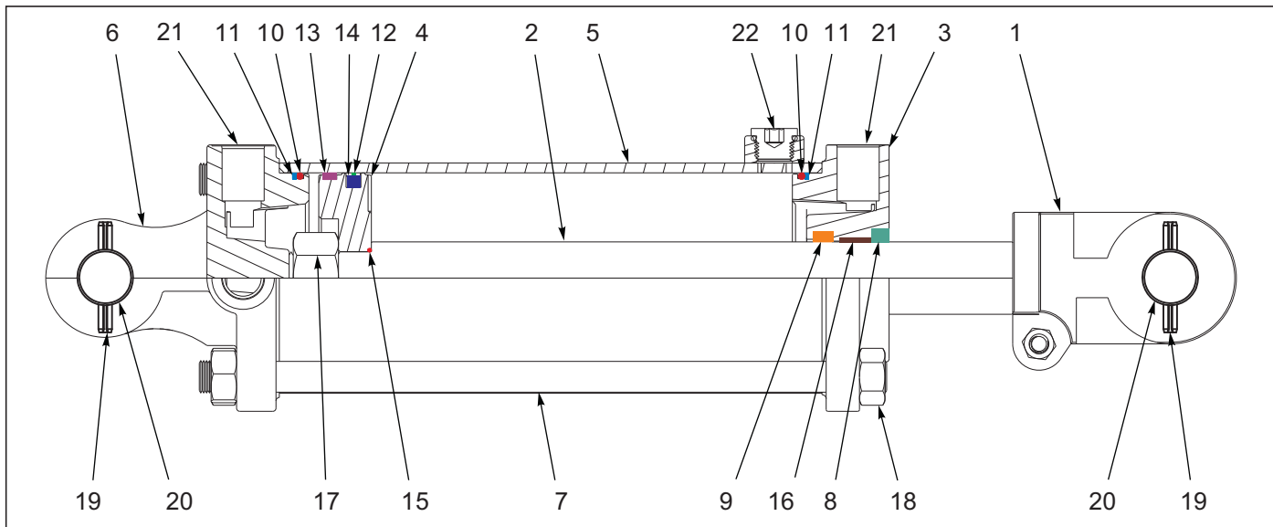
Figure 7-5: Cylinder Assembly Rephase 3-1/2 x 10 (Midway)
