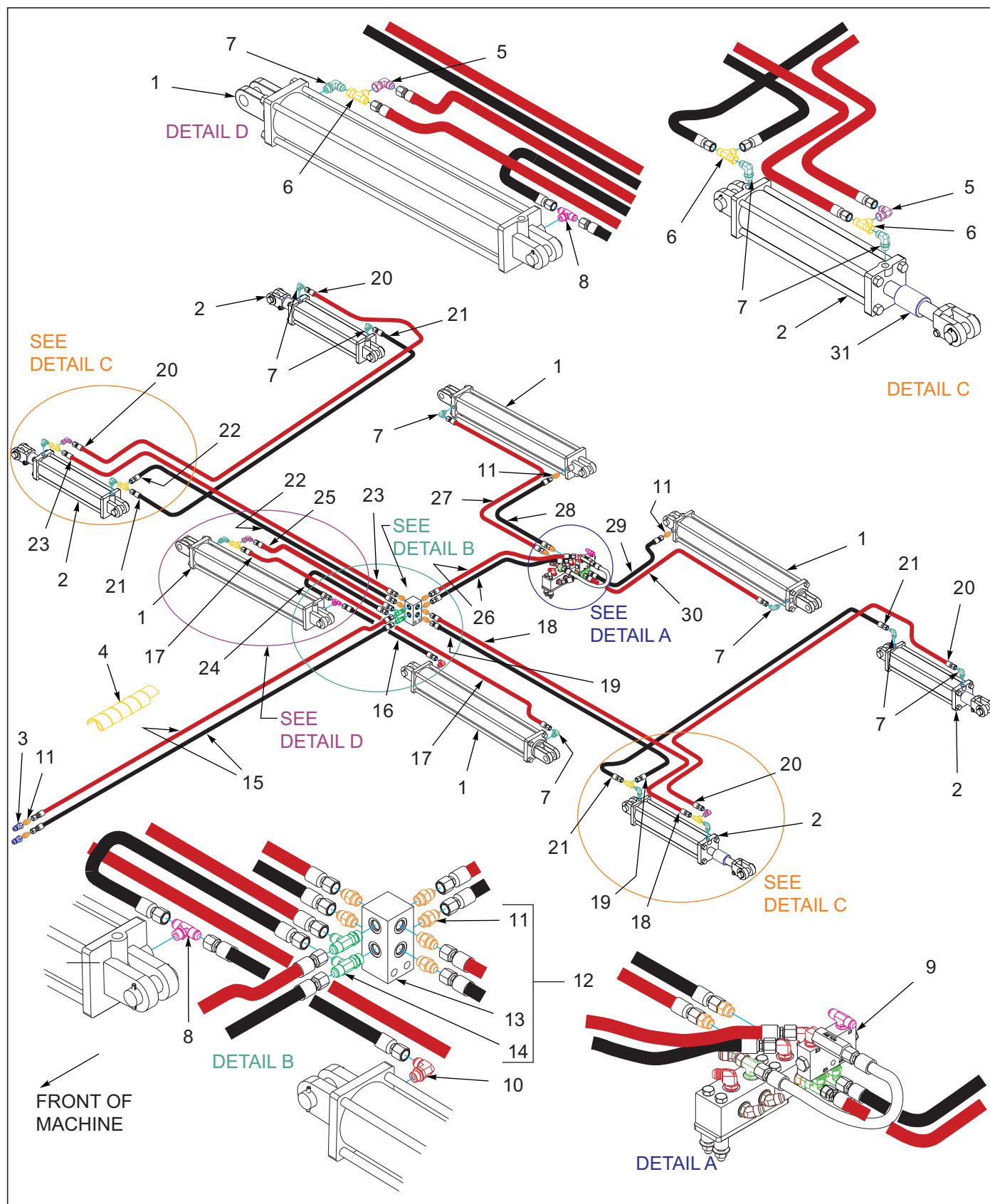
Figure 6-3: Hydraulic Assembly Fold 9450-38'-42'
