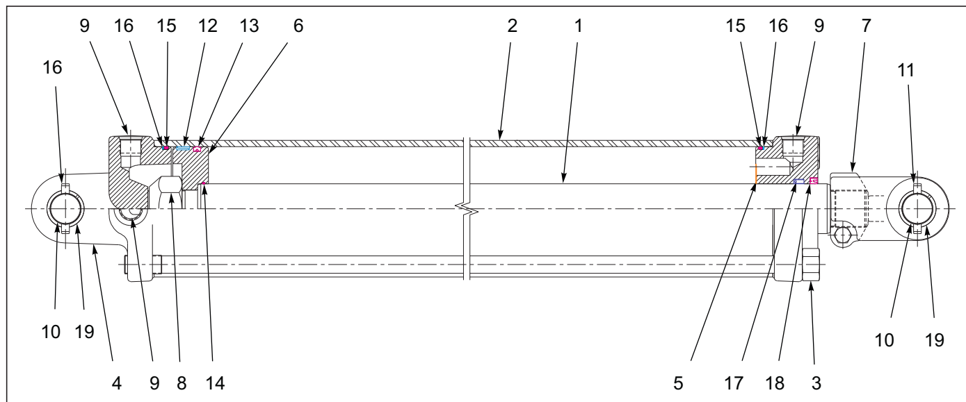
Figure 7-12: Cylinder Assembly 5 x 30 9450-46'-50'
