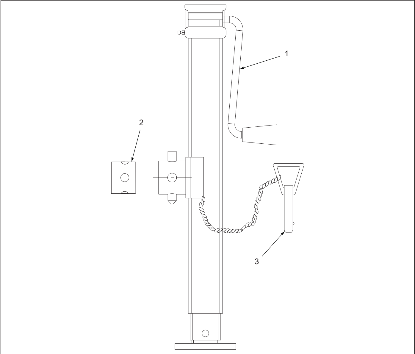
Figure 2-3: Jack Assembly
