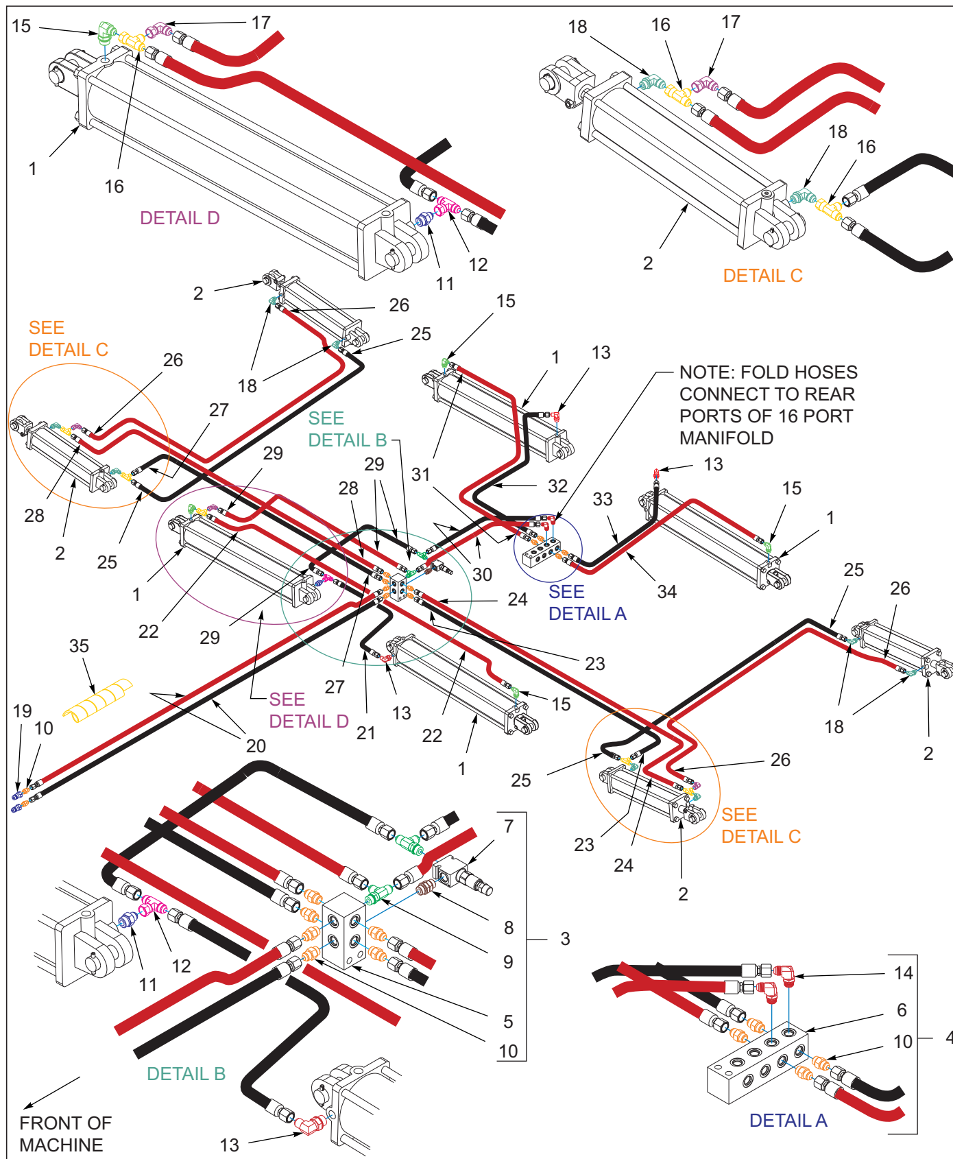
Figure 6-5: Hydraulic Assembly Fold 9450-46'-50'
