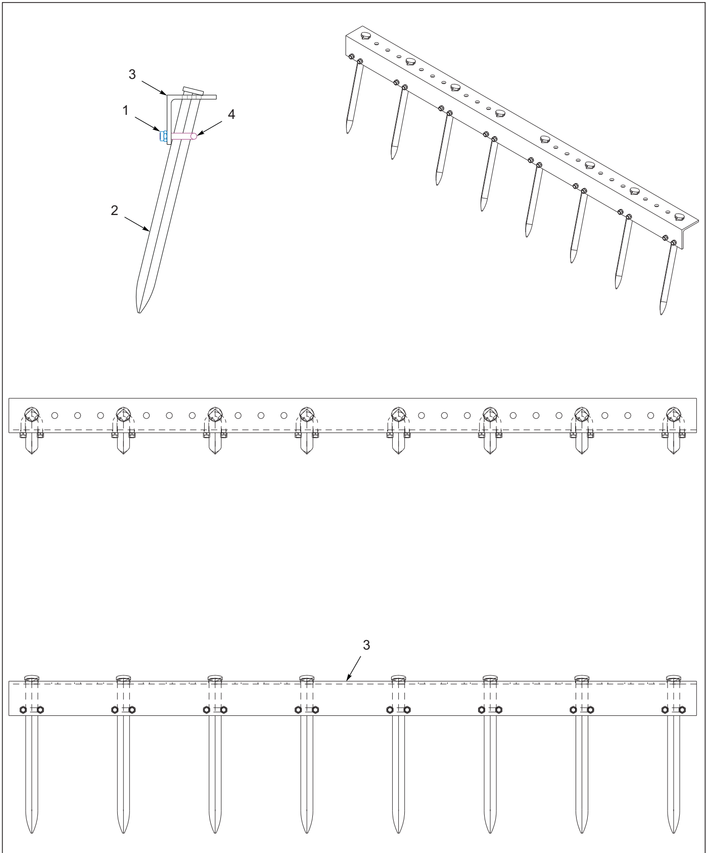
Figure 10-17: Spike Bar Assembly 8SP
