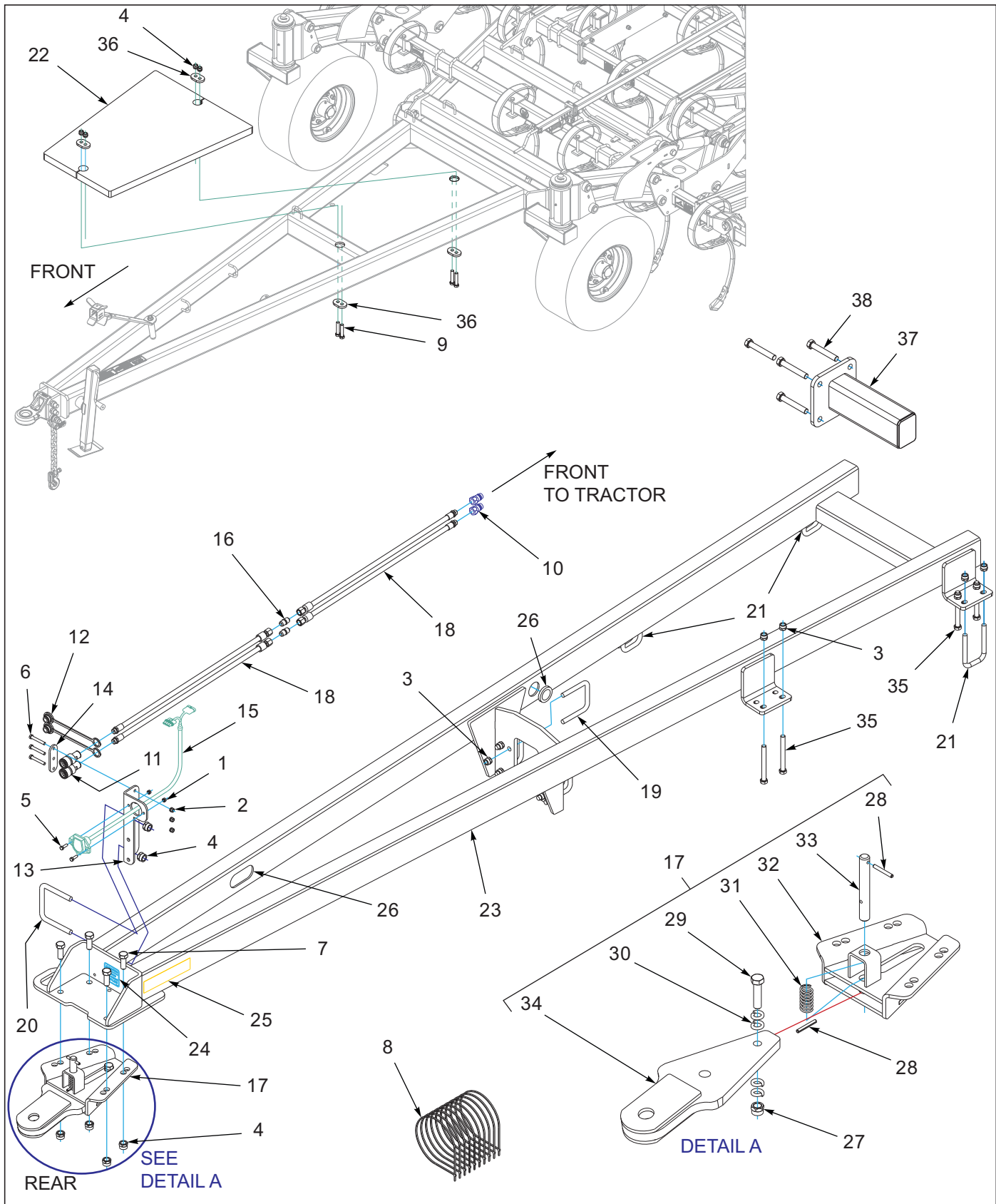
Figure 10-25: Rear Tow Hitch Assembly
