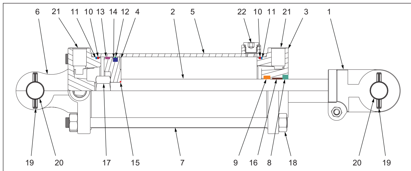
Figure 7-6: Cylinder Assembly Rephase 3-1/2 x 10( Midway)
