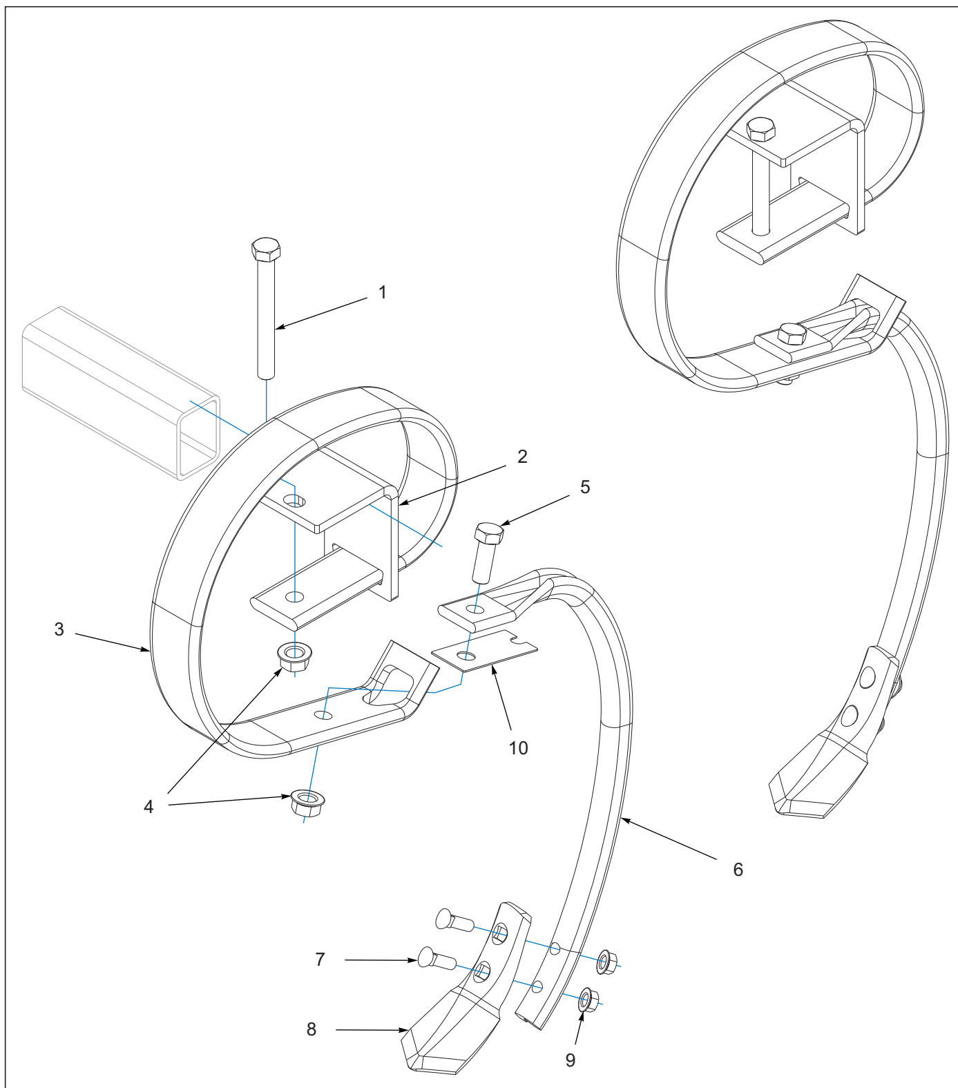
Figure 5-1: Tine Assembly
