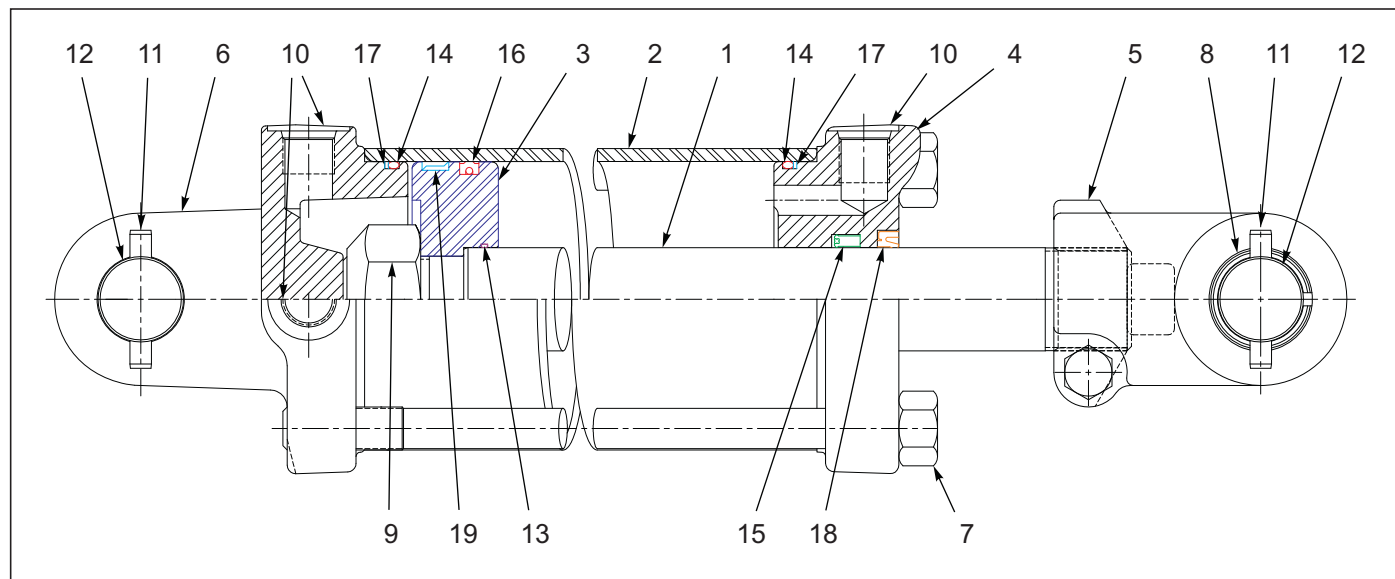
Figure 7-13: Cylinder Assembly 4 x 16 9450-38'-42'
