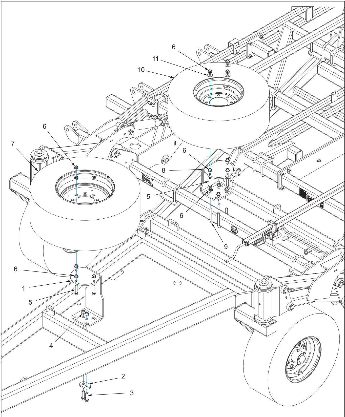
Figure 10-26: Spare Tire Assembly
