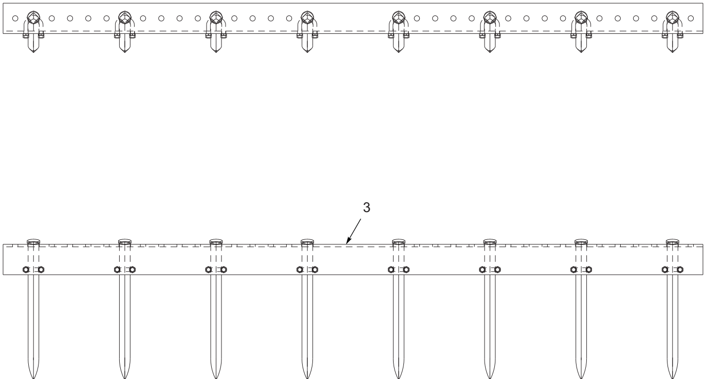
Figure 10-11: Spike Bar Assembly 9SP
