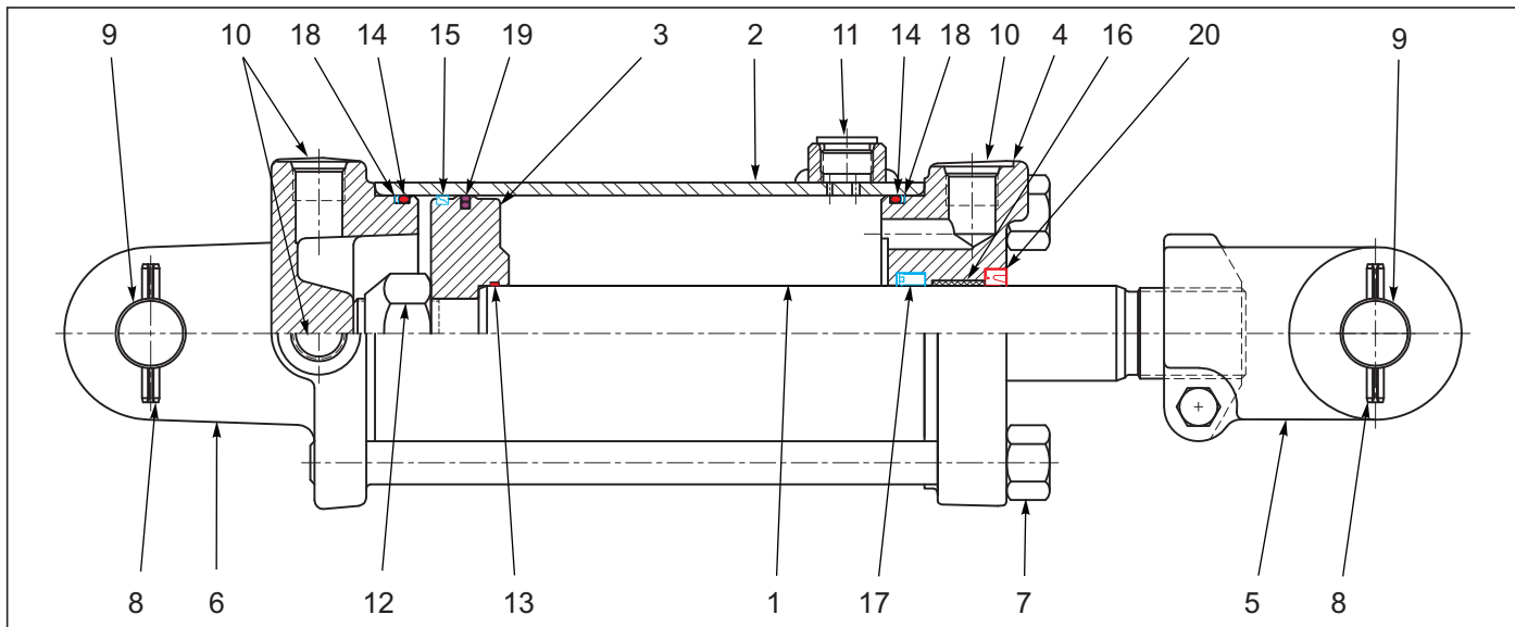
Figure 7-3: Cylinder Assembly Rephase 3-1/2 x 10 (Prince)
