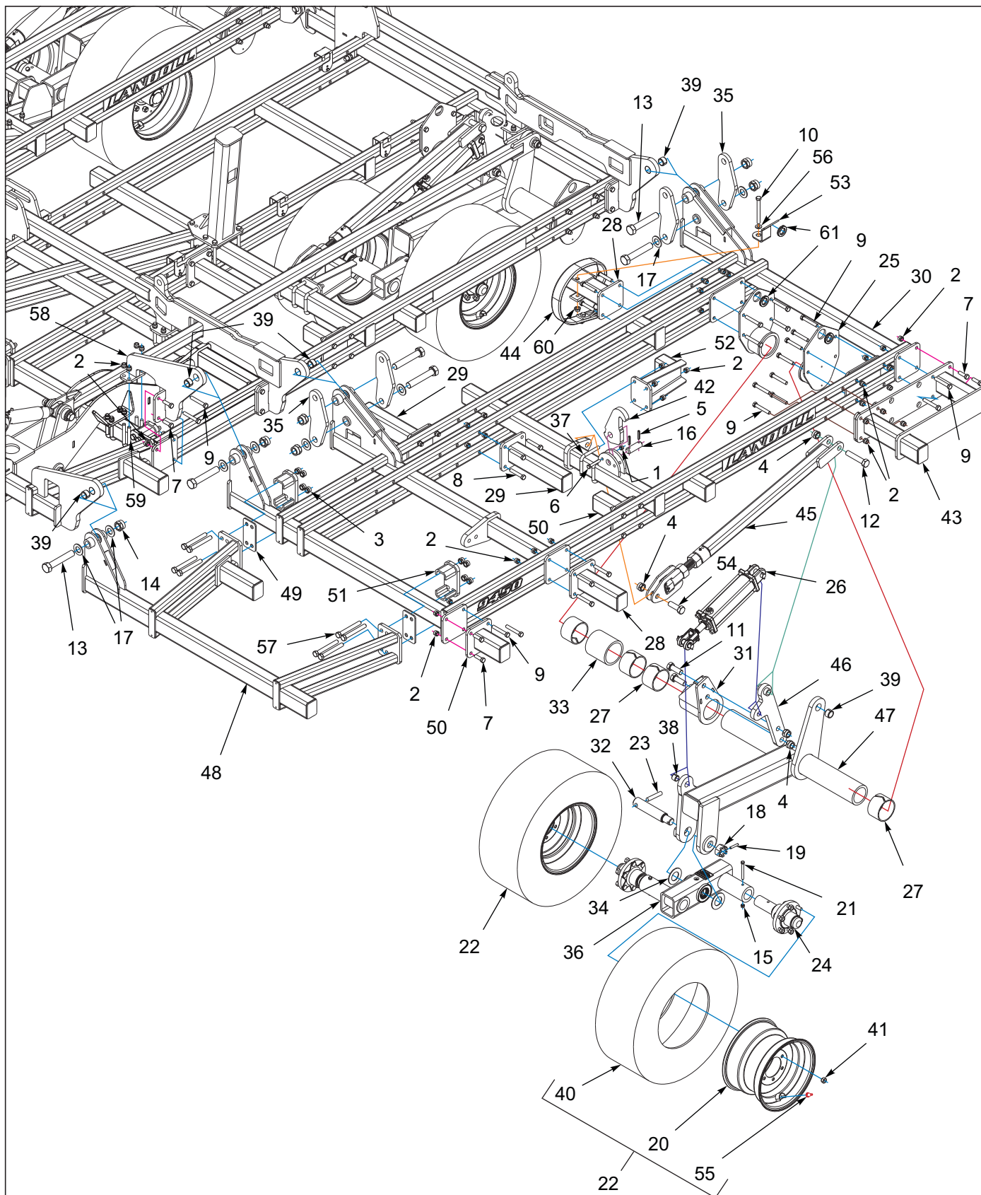
Figure 3-5: 6' Outer Wing Assembly 9450FH-38'-42'
