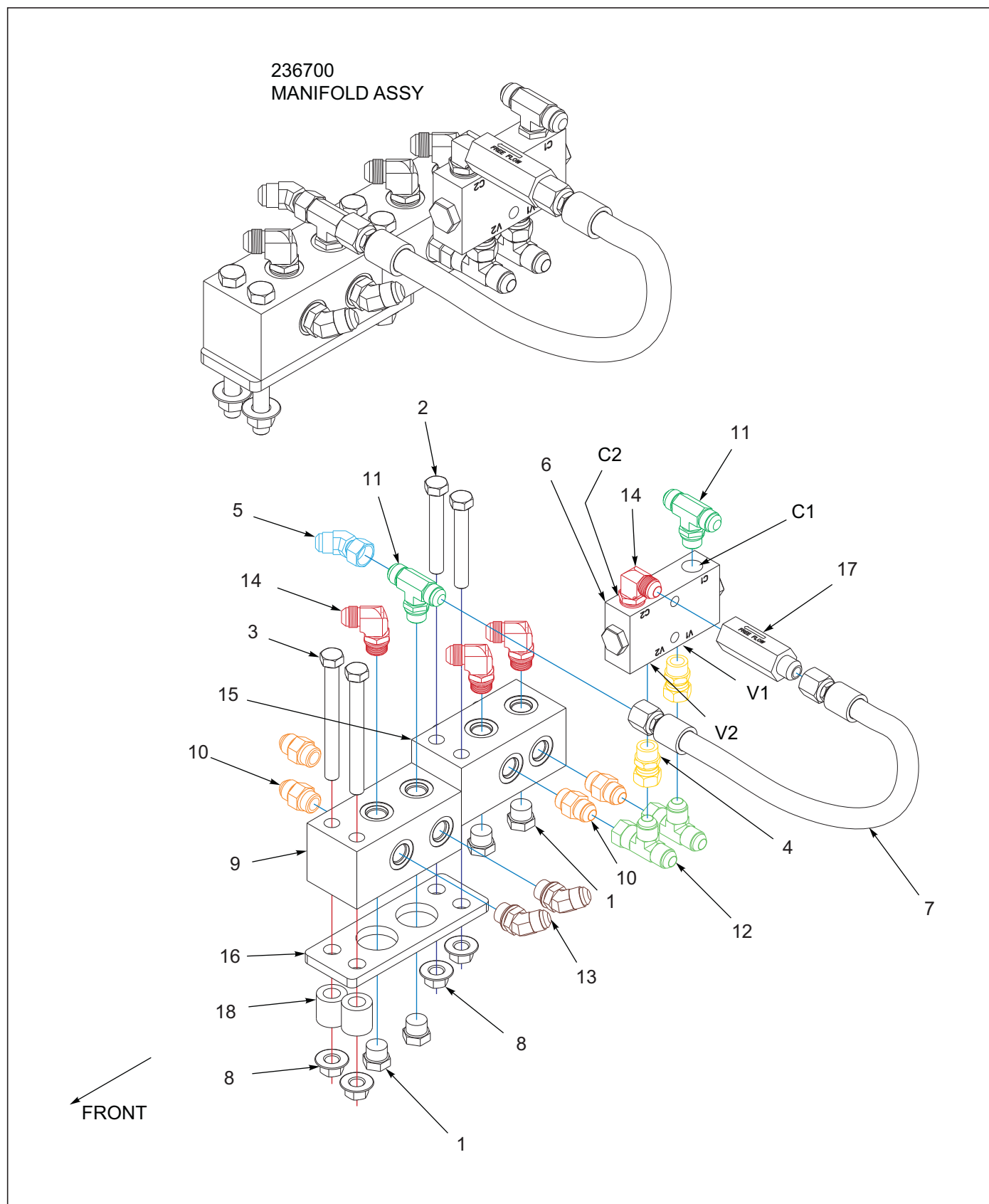
Figure 6-4: Manifold Assembly 9450-38'-42'
