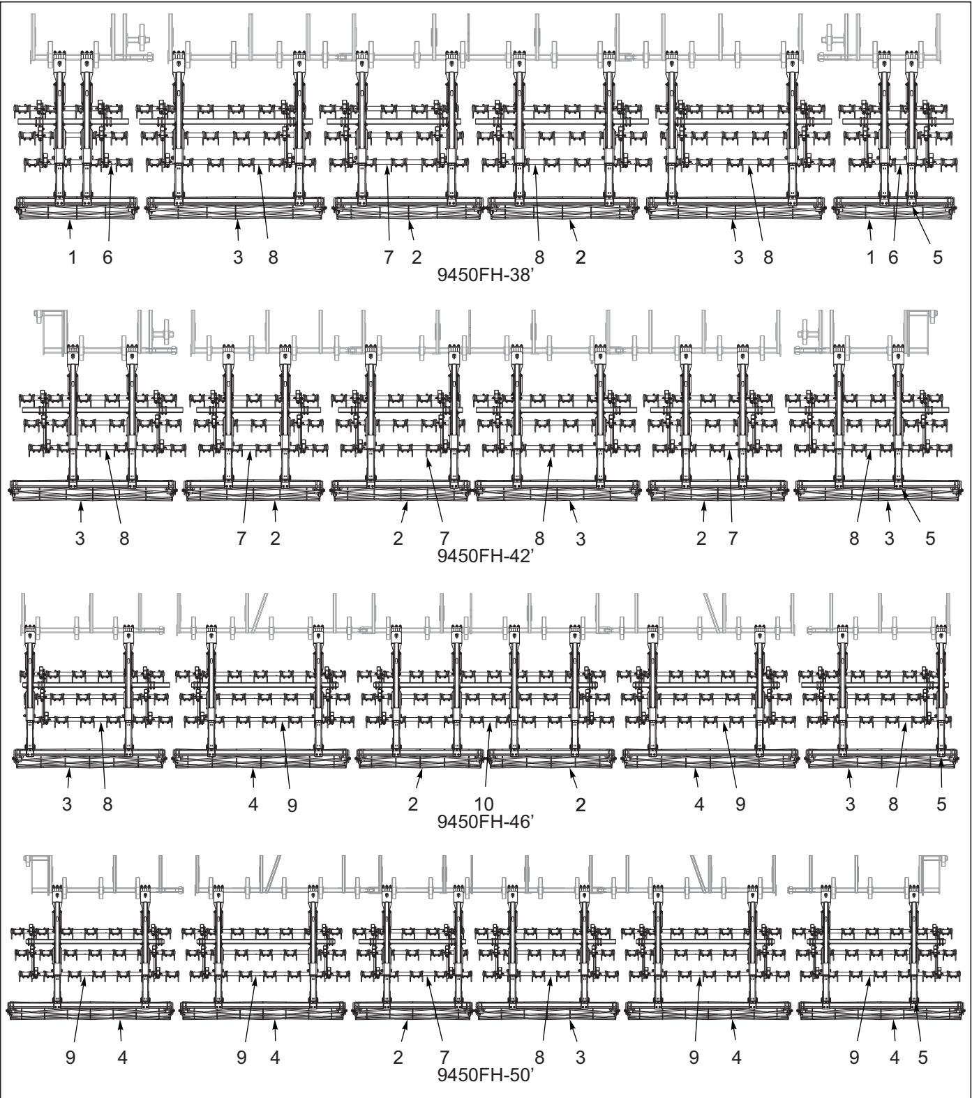
Figure 10-1: 3 Row Tine and Reel Harrow Layout
