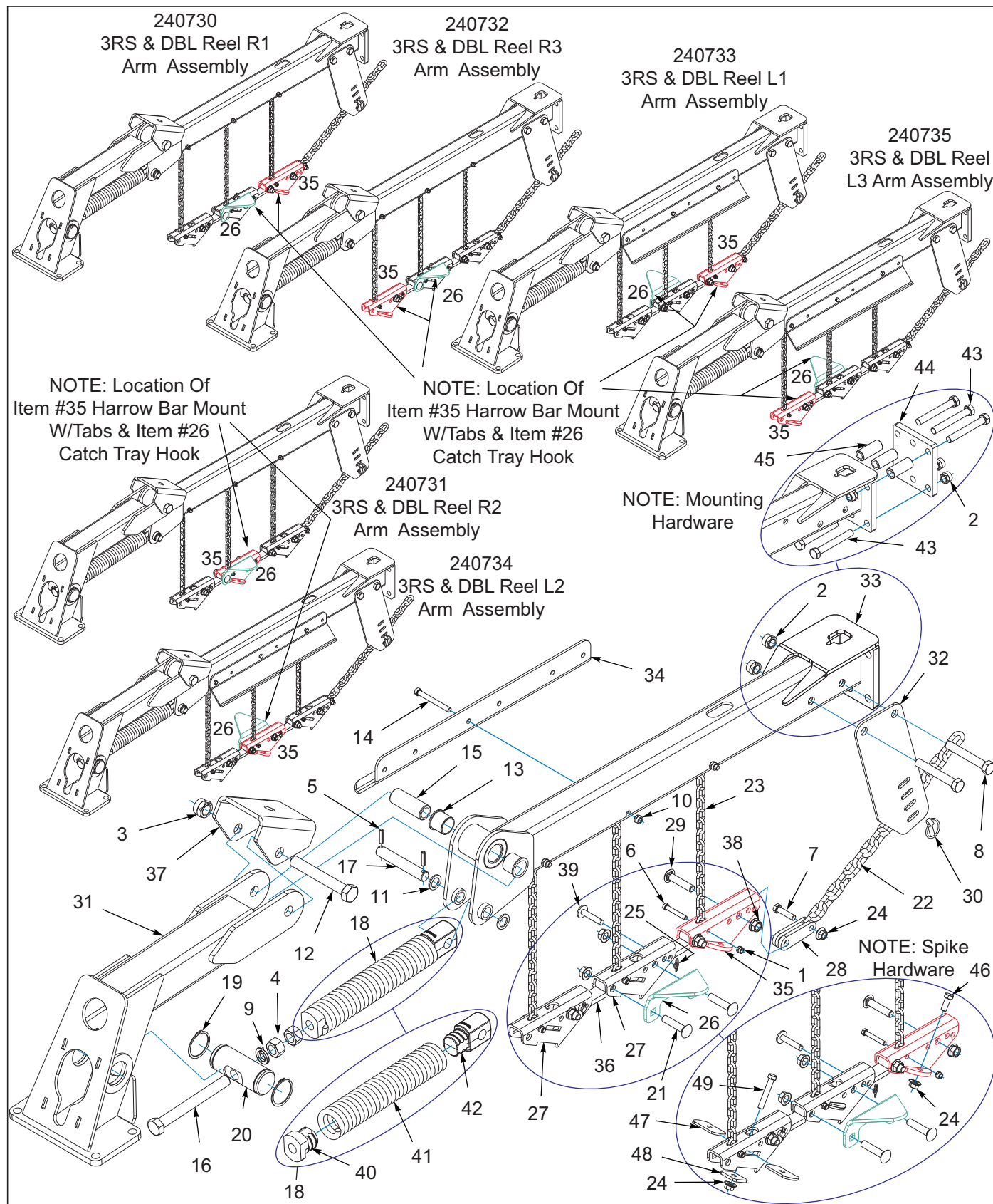
Figure 10-21: Arm Assembly 3RS and Double Reel W/Tray
