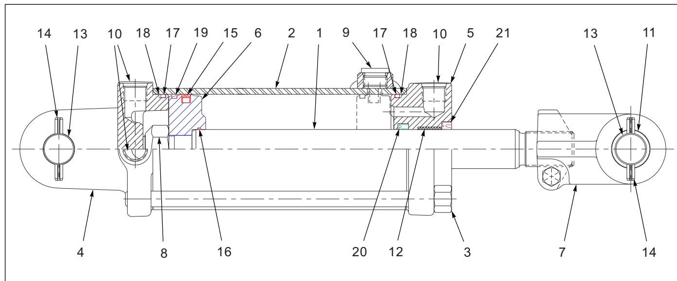
Figure 7-4: Cylinder Assembly Rephase 3-1/2 x 10 (Prince)
