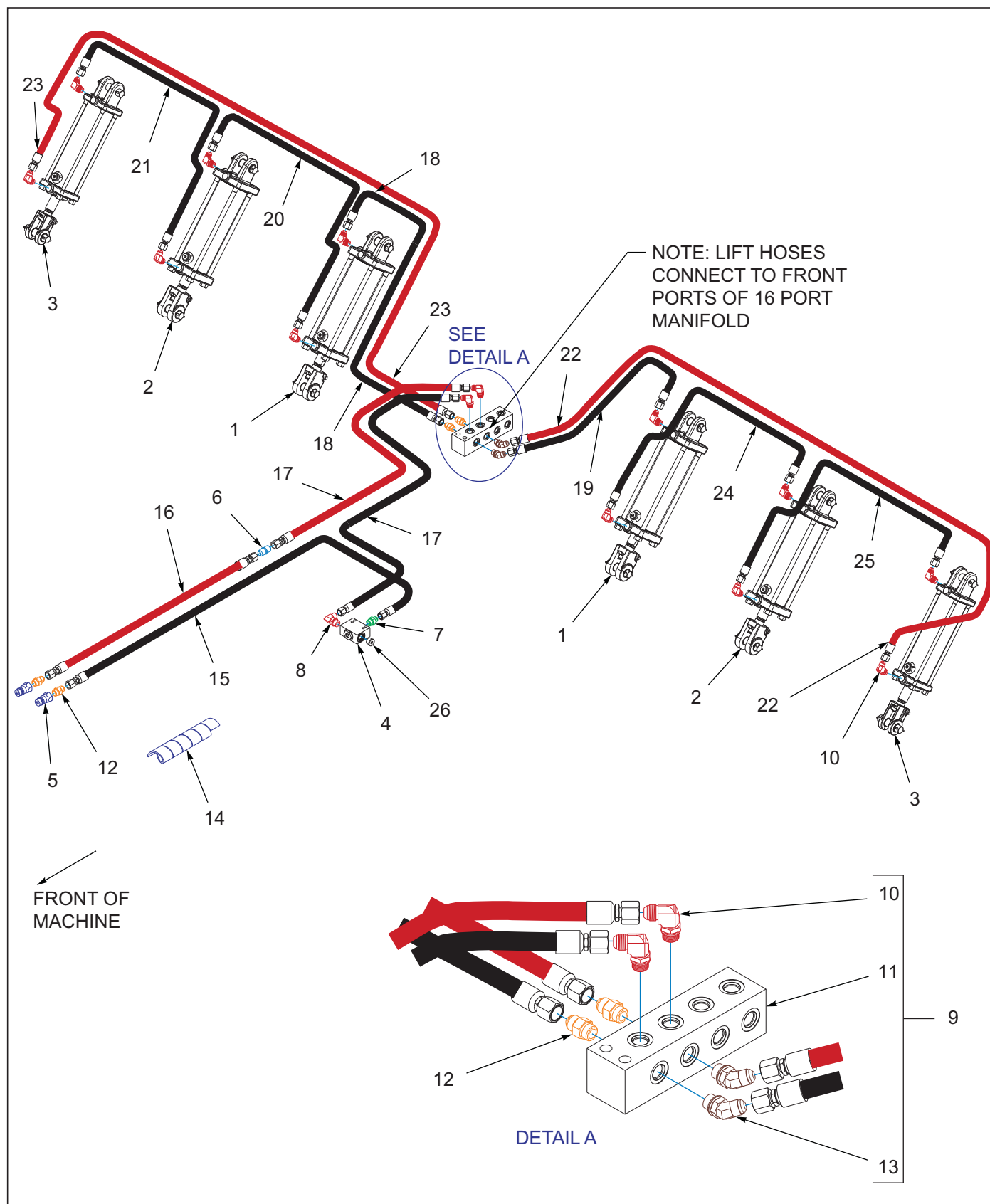
Figure 6-2: Hydraulic Assembly Lift 9450-46'-50'
