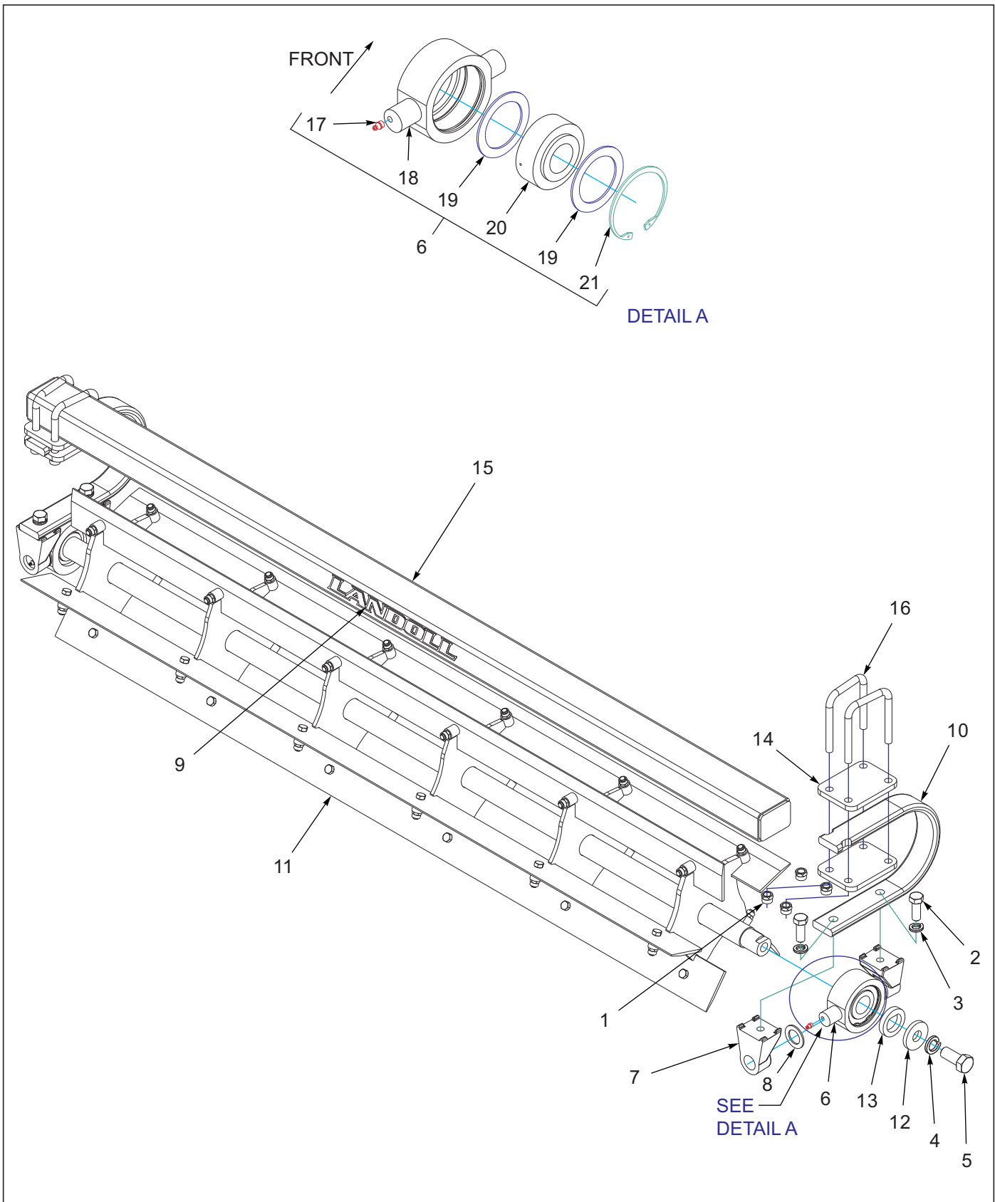
Figure 9-5: 3BCT ChopperReel/ Gangbar Assembly
