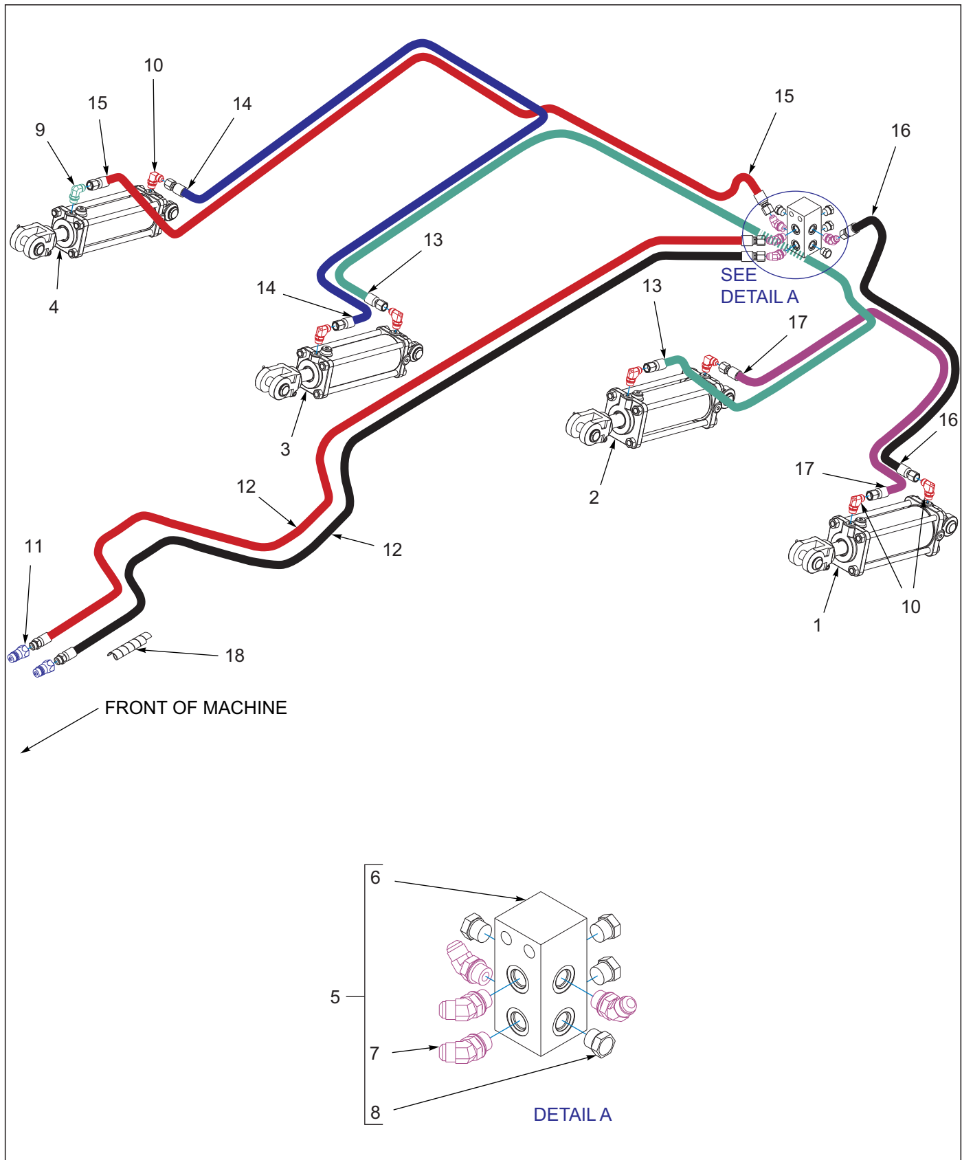
Figure 5-3: Gang Lift Assembly
