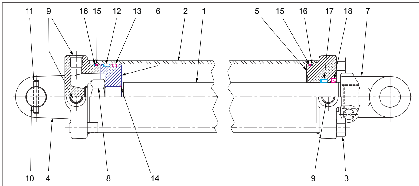
Figure 6-11: Cylinder Assembly 4 x30 (Prince)
