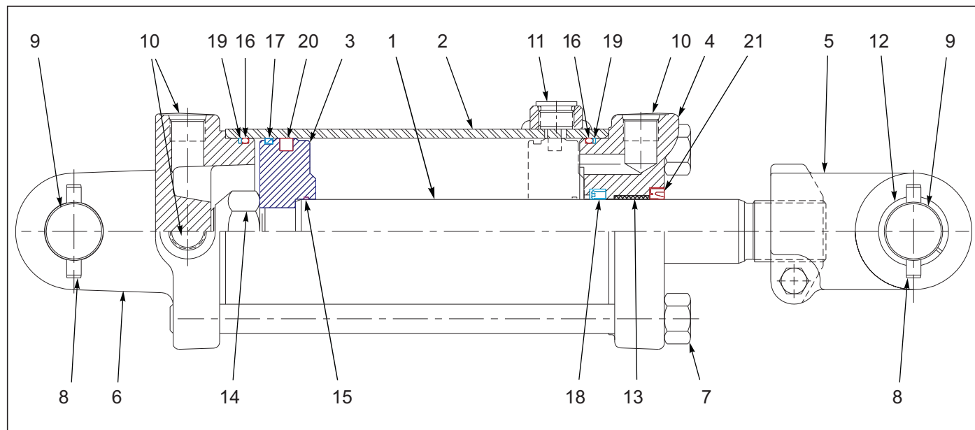
Figure 6-2: Cylinder Assembly 4 x 16 Rephase
