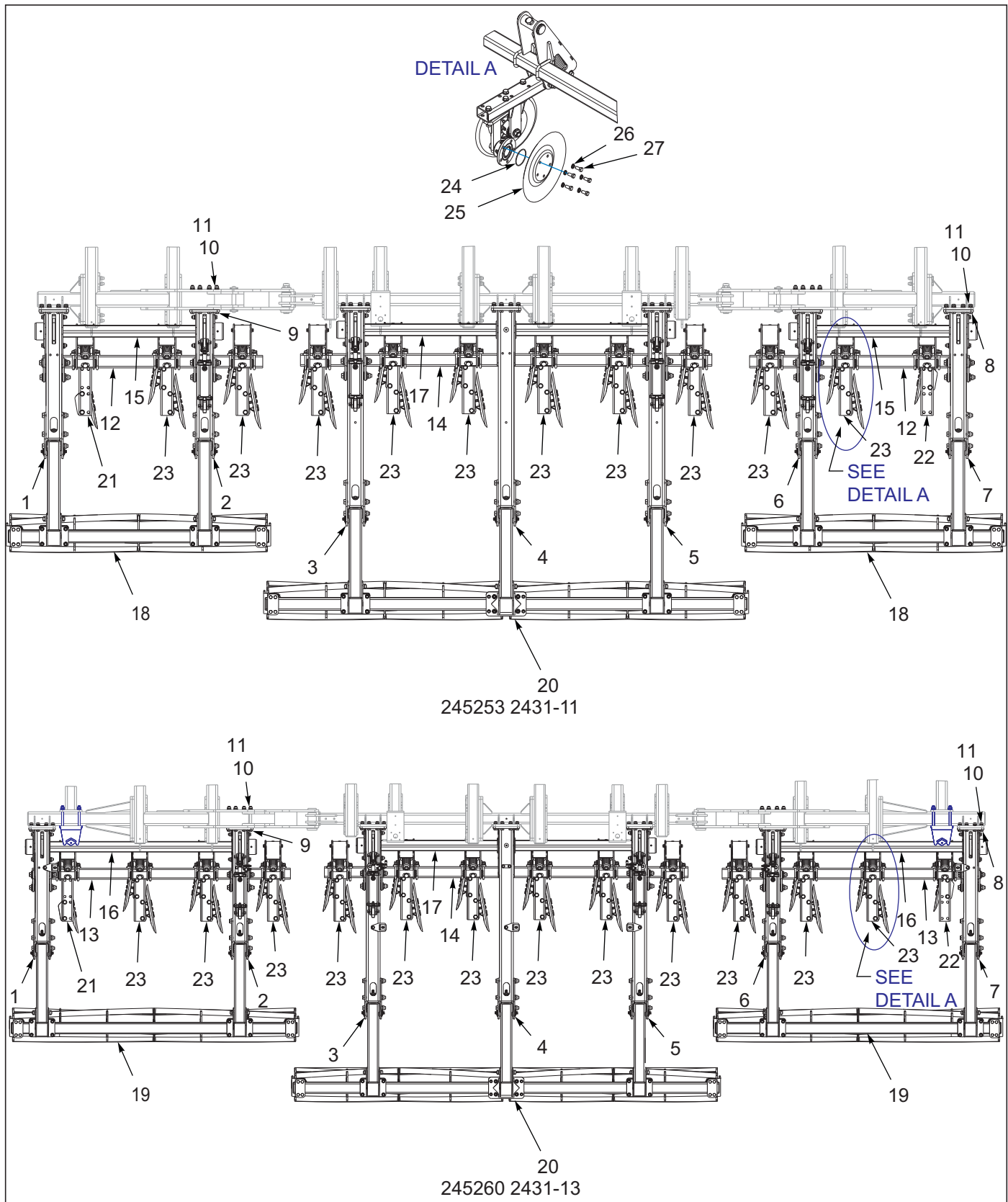
Figure 9-9: Disc Lev/Hyd Flat RL W/Bearing Layout
