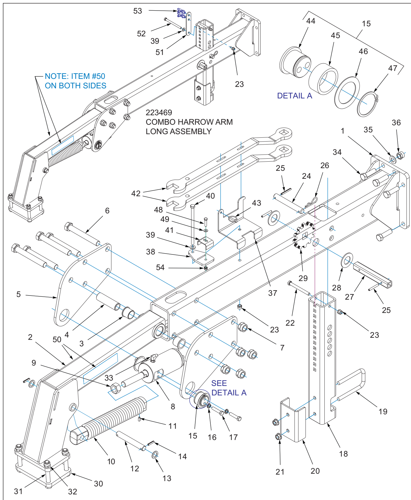
Figure 9-2: Harrow Arm Assembly Combo Hydraulic Long
