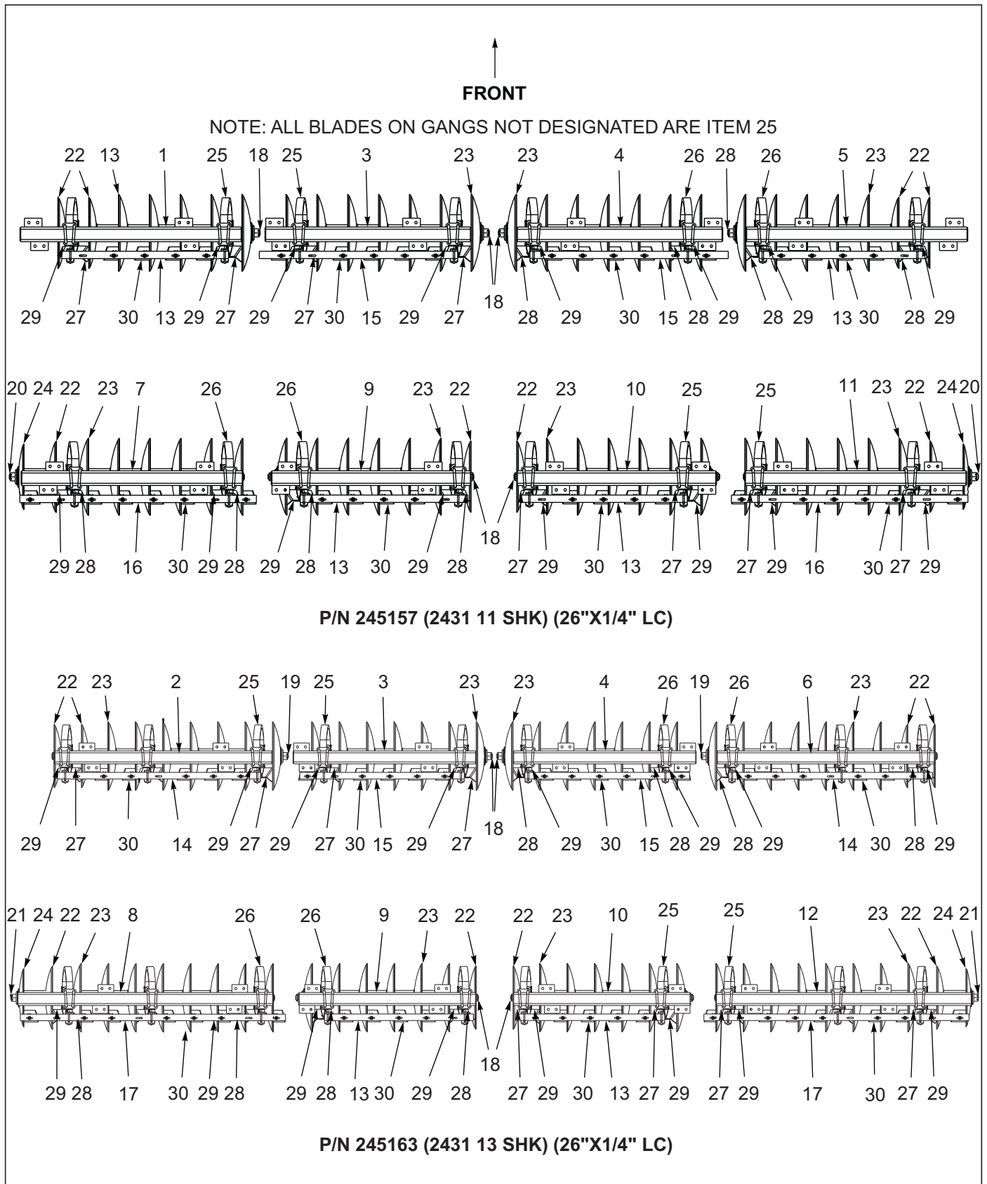
Figure 3-2: Disc Gang Placement 26" Blade
