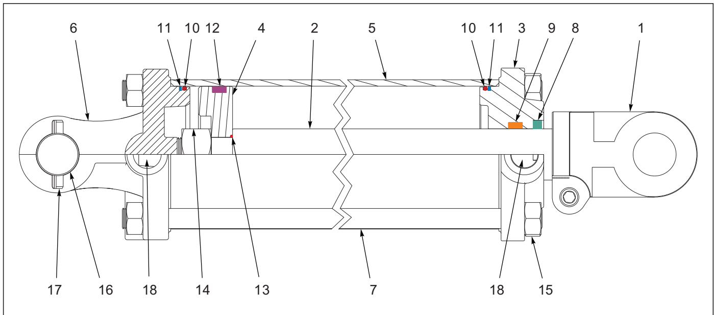
Figure 6-12: Cylinder Assembly 4 x30 (Midway)
