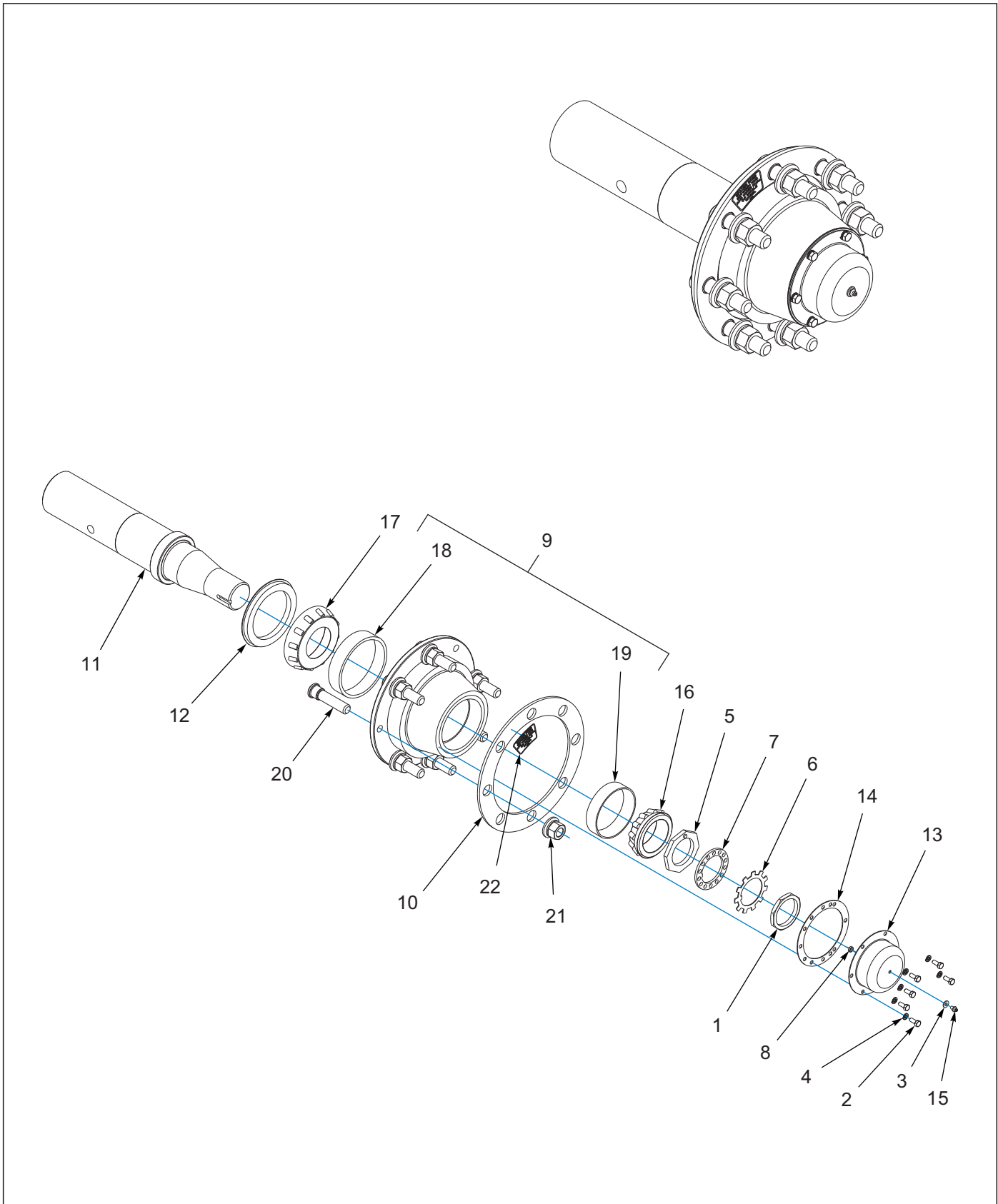
Figure 1-5: Hub and Spindle Assembly 191974
