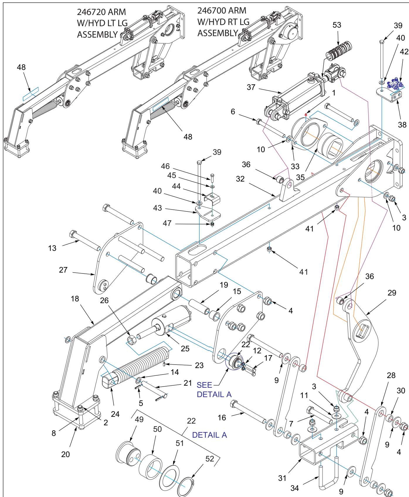
Figure 9-12: Arm With/Hyd LG Assembly
