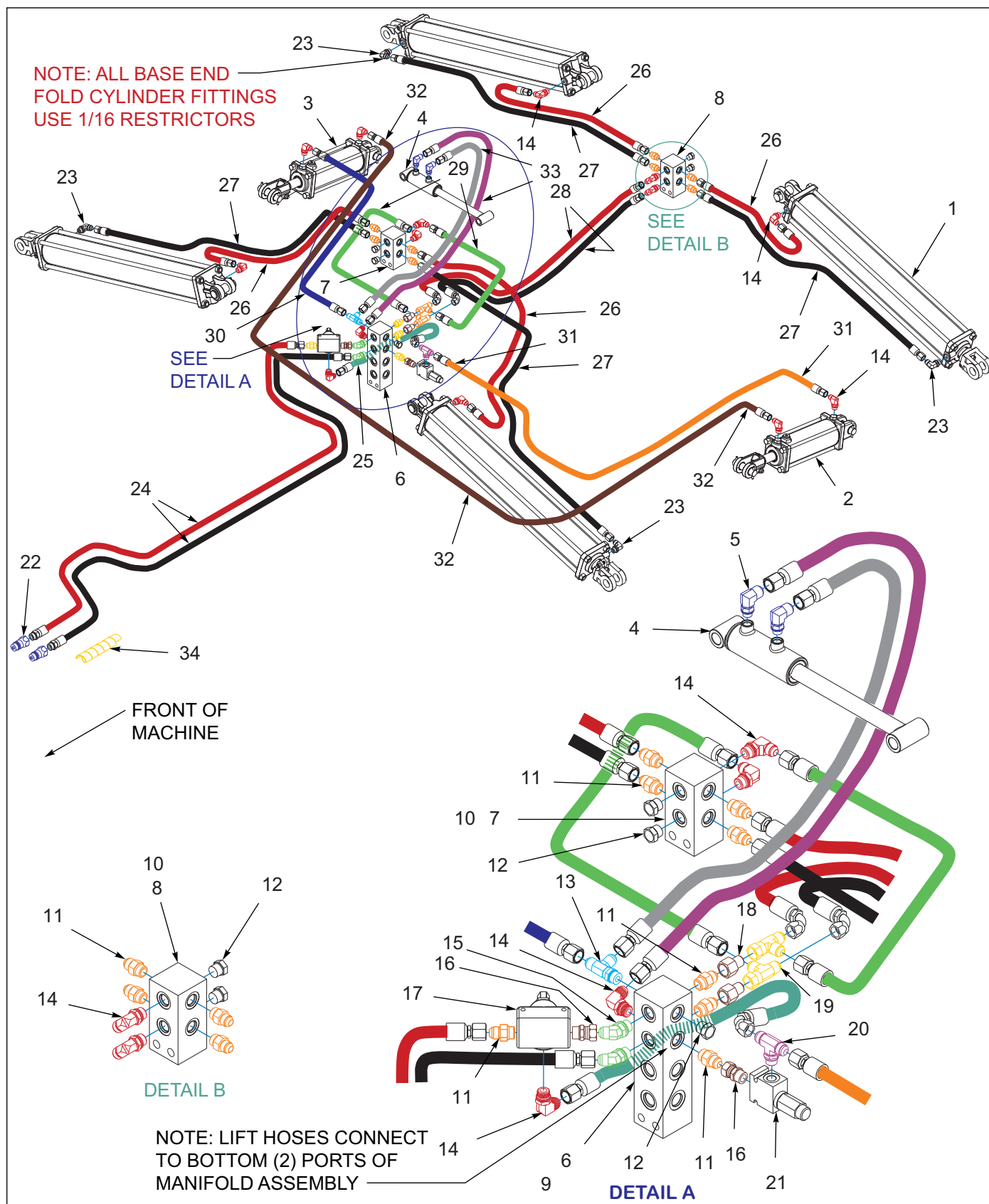
Figure 5-2: Fold Assembly
