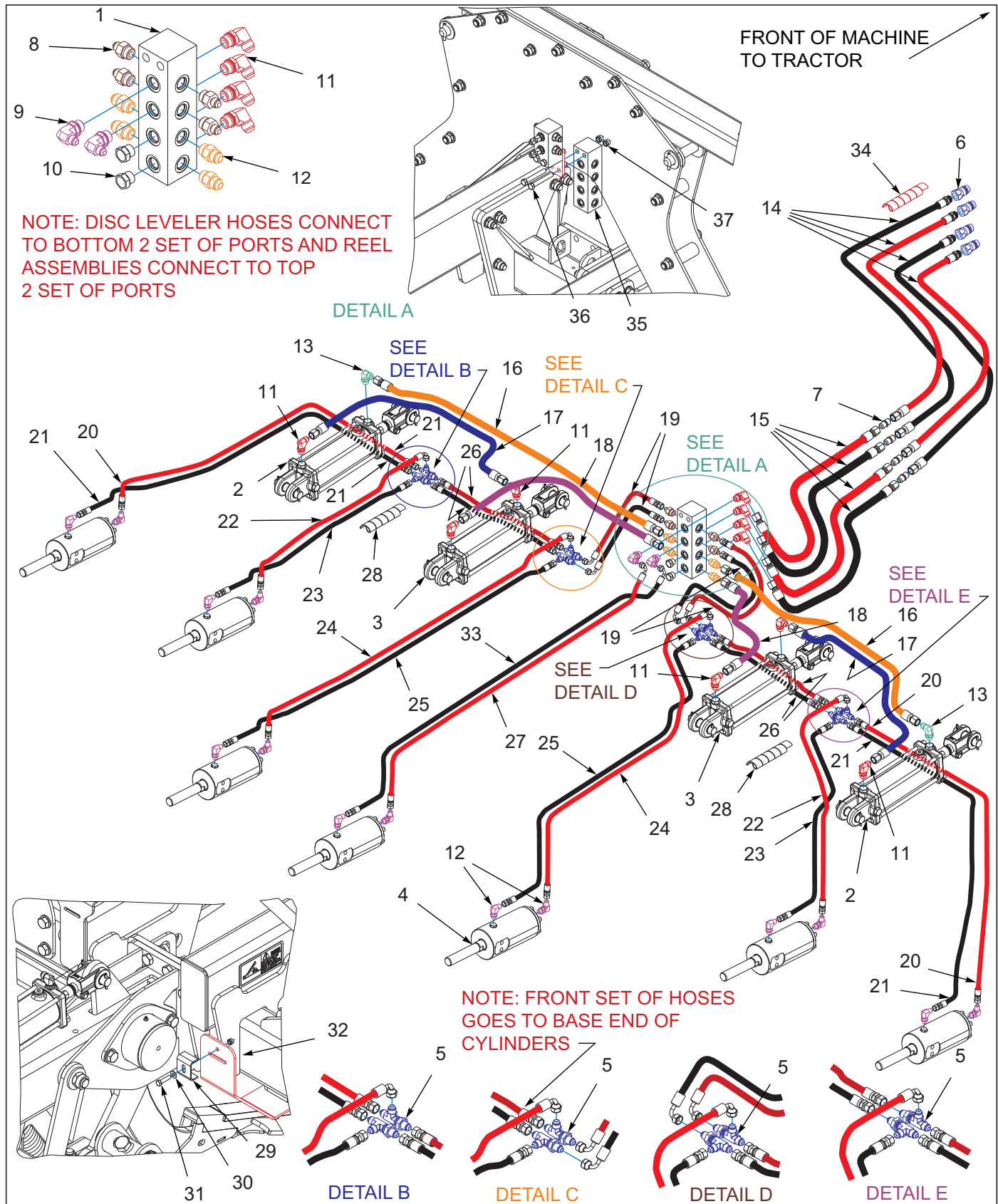
Figure 9-16: Disc Lev/Hyd RL Assembly
