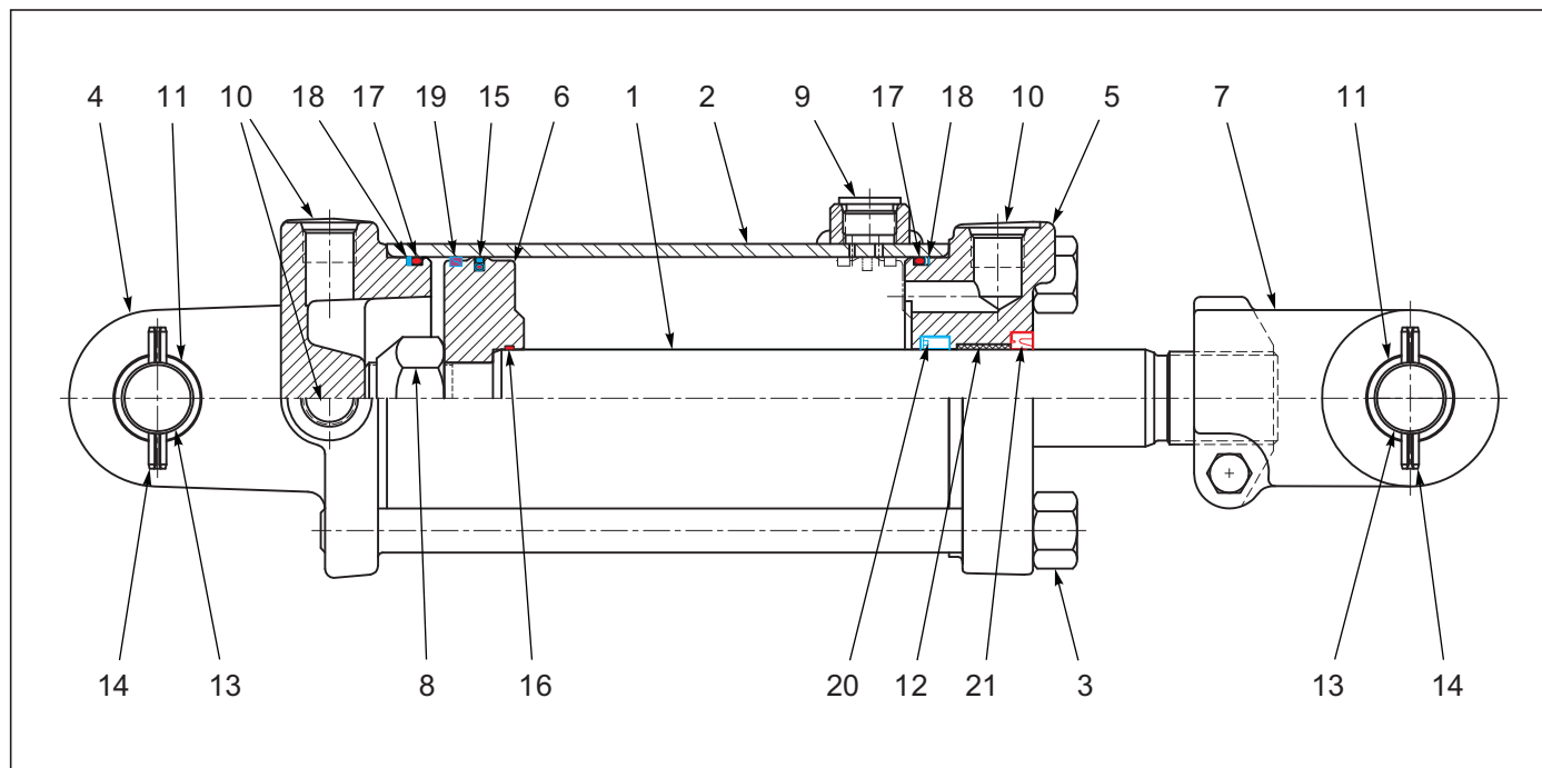
Figure 6-3: Cylinder Assembly 4 x 8, Rephase (Prince)
