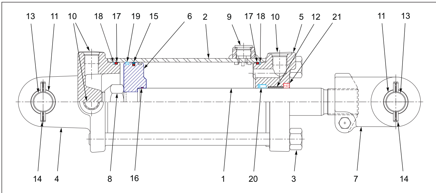
Figure 6-5: Cylinder Assembly 3-3/4 x 8, Rephase (Prince)
