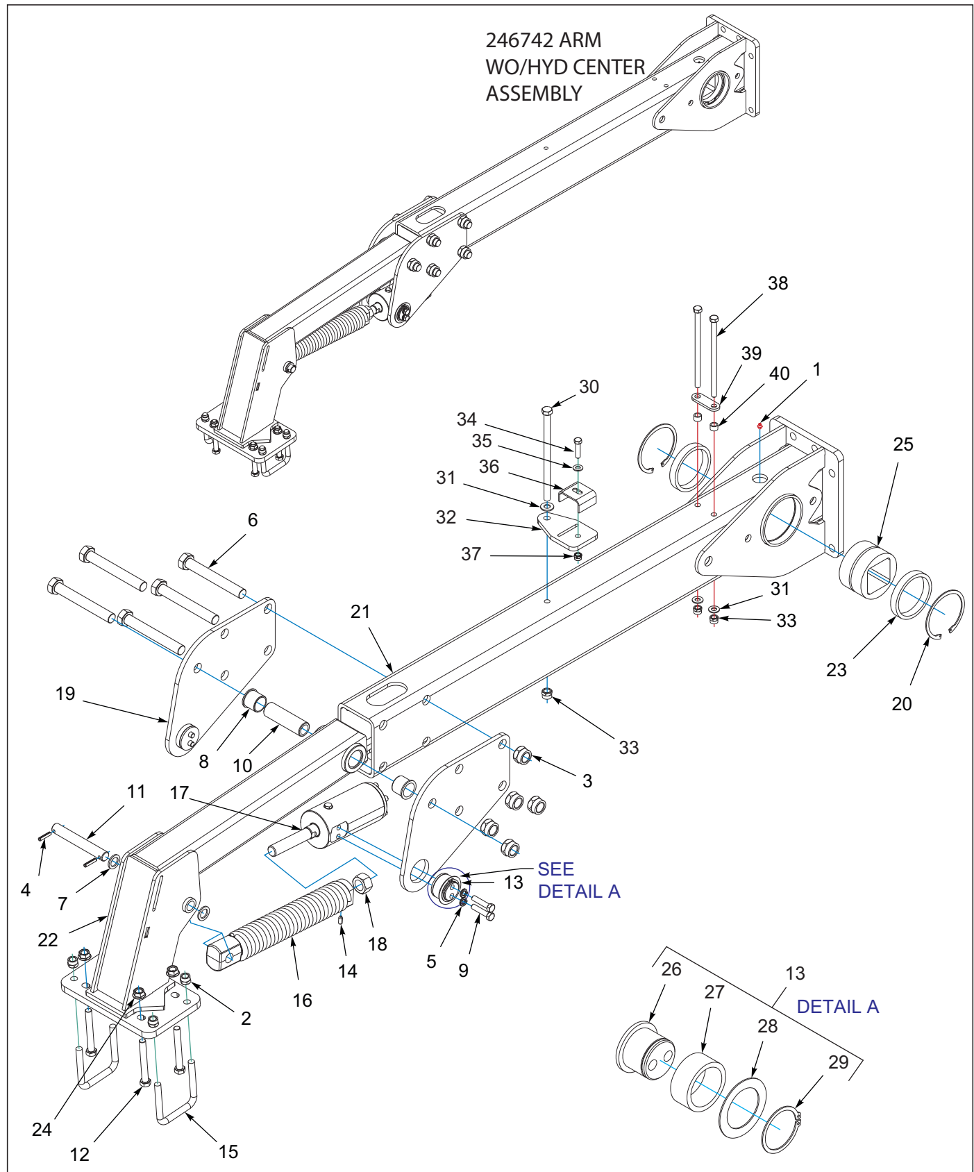
Figure 9-13: Arm No/Hyd Center Assembly
