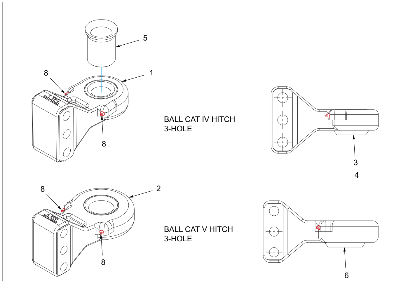
Figure 2-4: Hitch & Ball Assemblies
