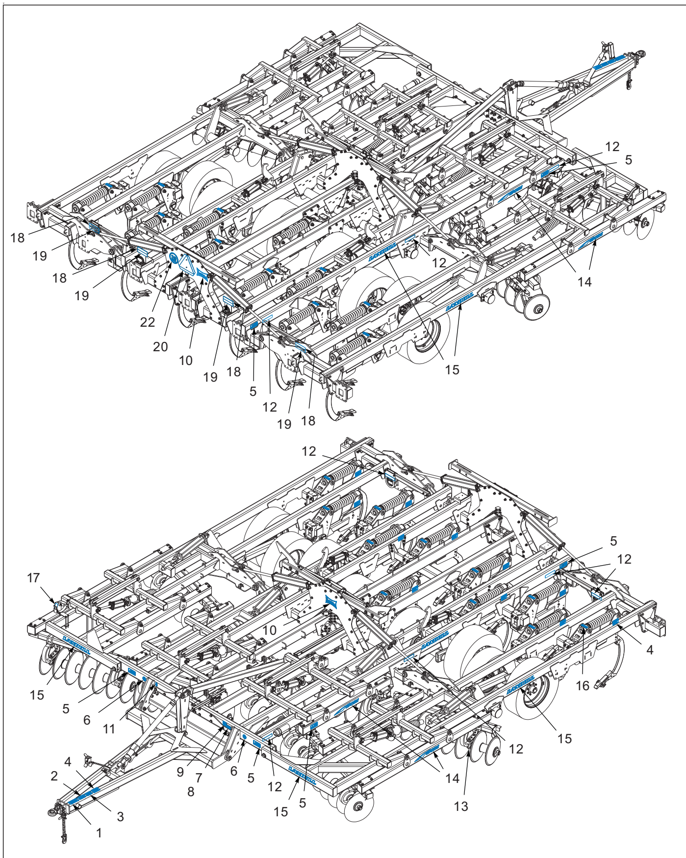
Figure 8-2: Decal Installation 2411AFG-07-09
