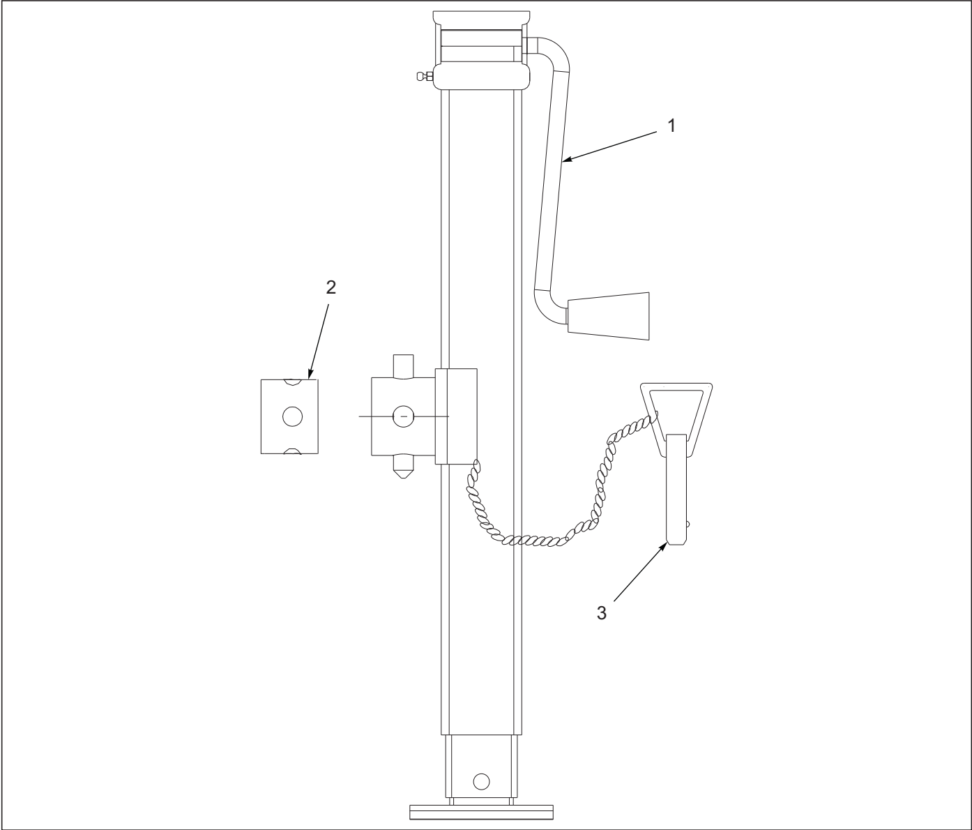
Figure 2-5: 7,000 Lb. Sidewind Jack Assembly
