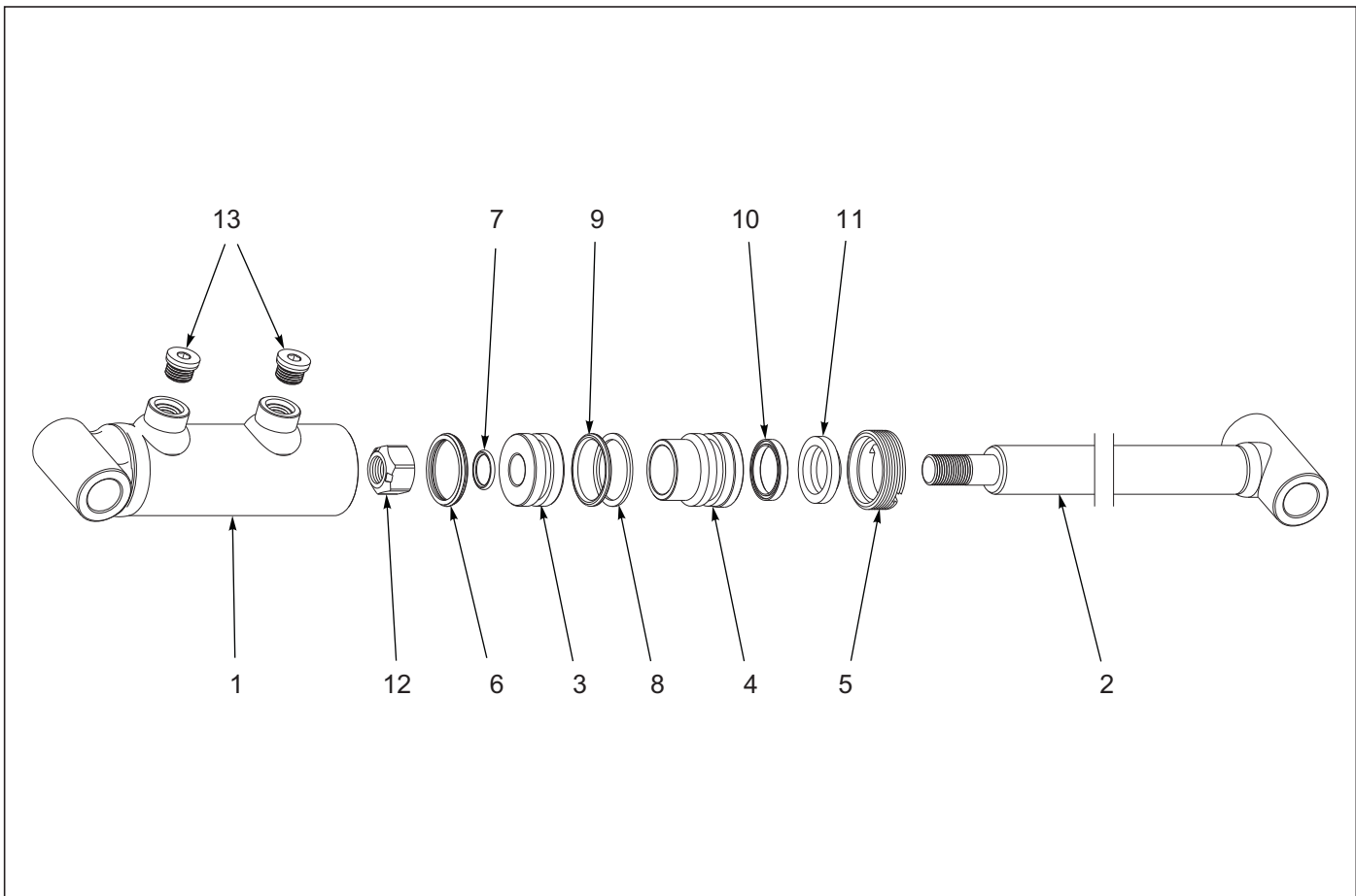
Figure 6-13: Cylinder Assembly 1-1/2 x -1-1/2
