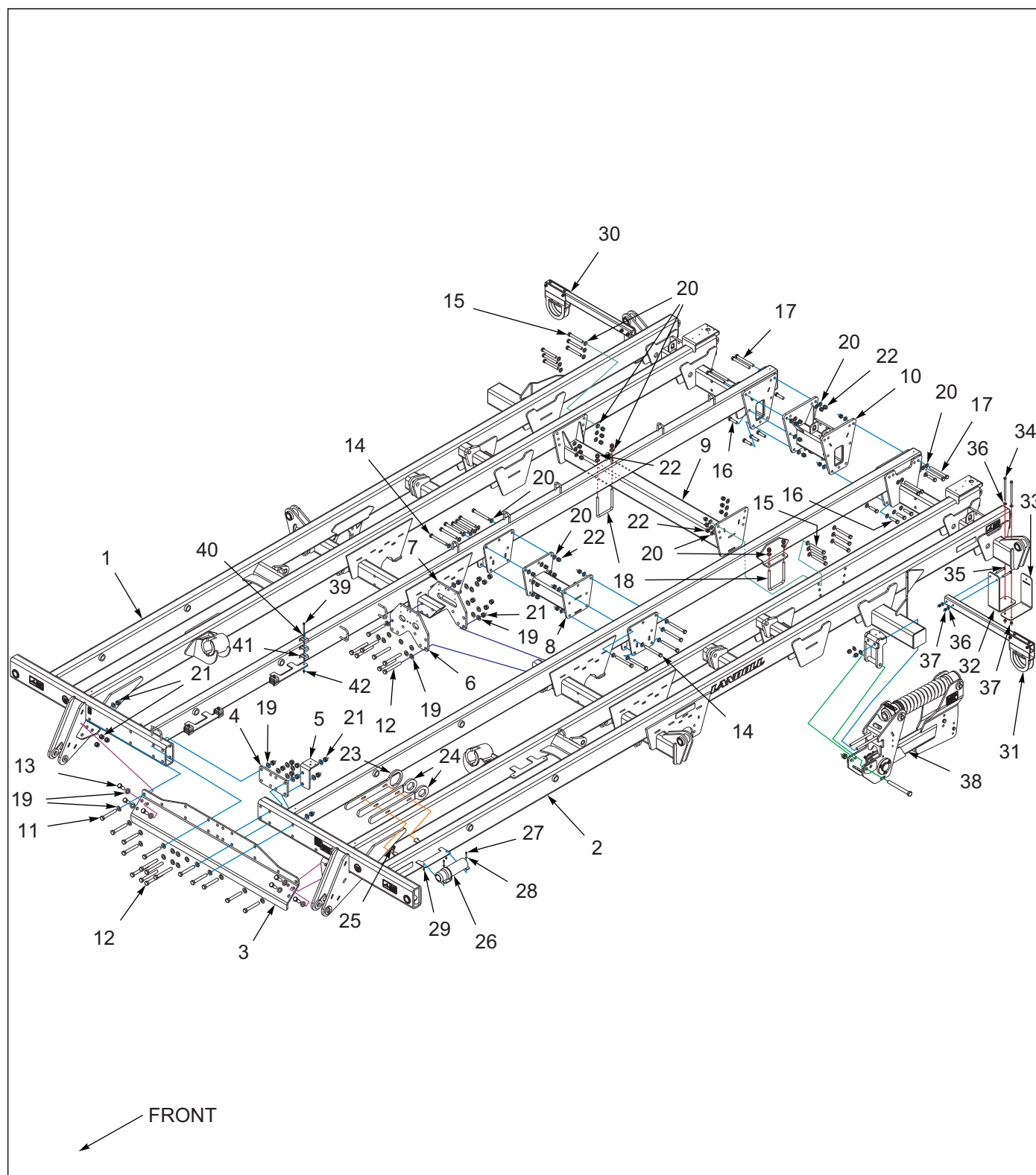
Figure 1-1: Frame Assembly Center
