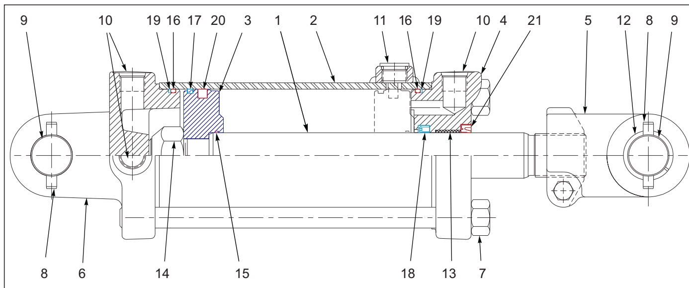
Figure 6-1: Cylinder Assembly 4-1/2 x 16, Rephase
