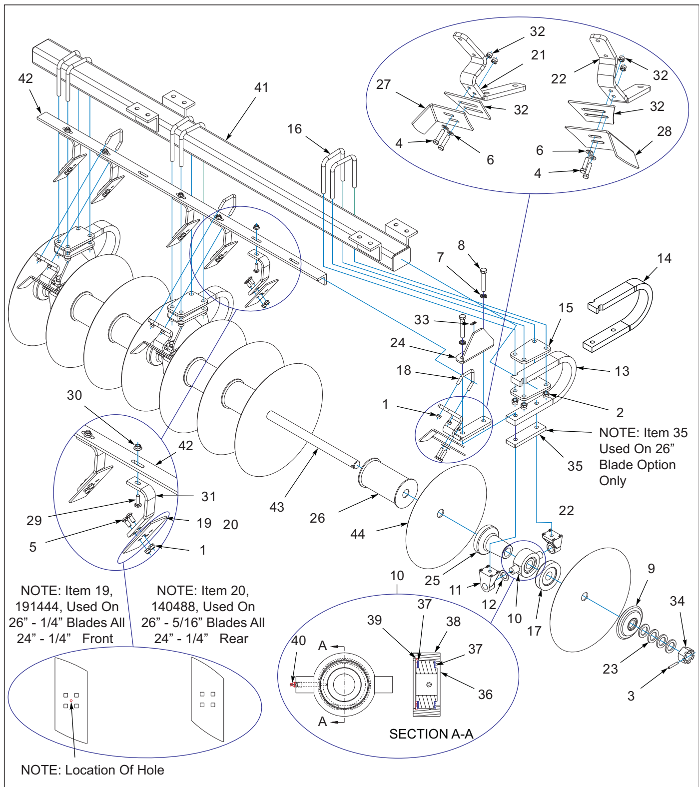
Figure 3-1: Disc Gang Assembly (2431-11/13 Shank)
