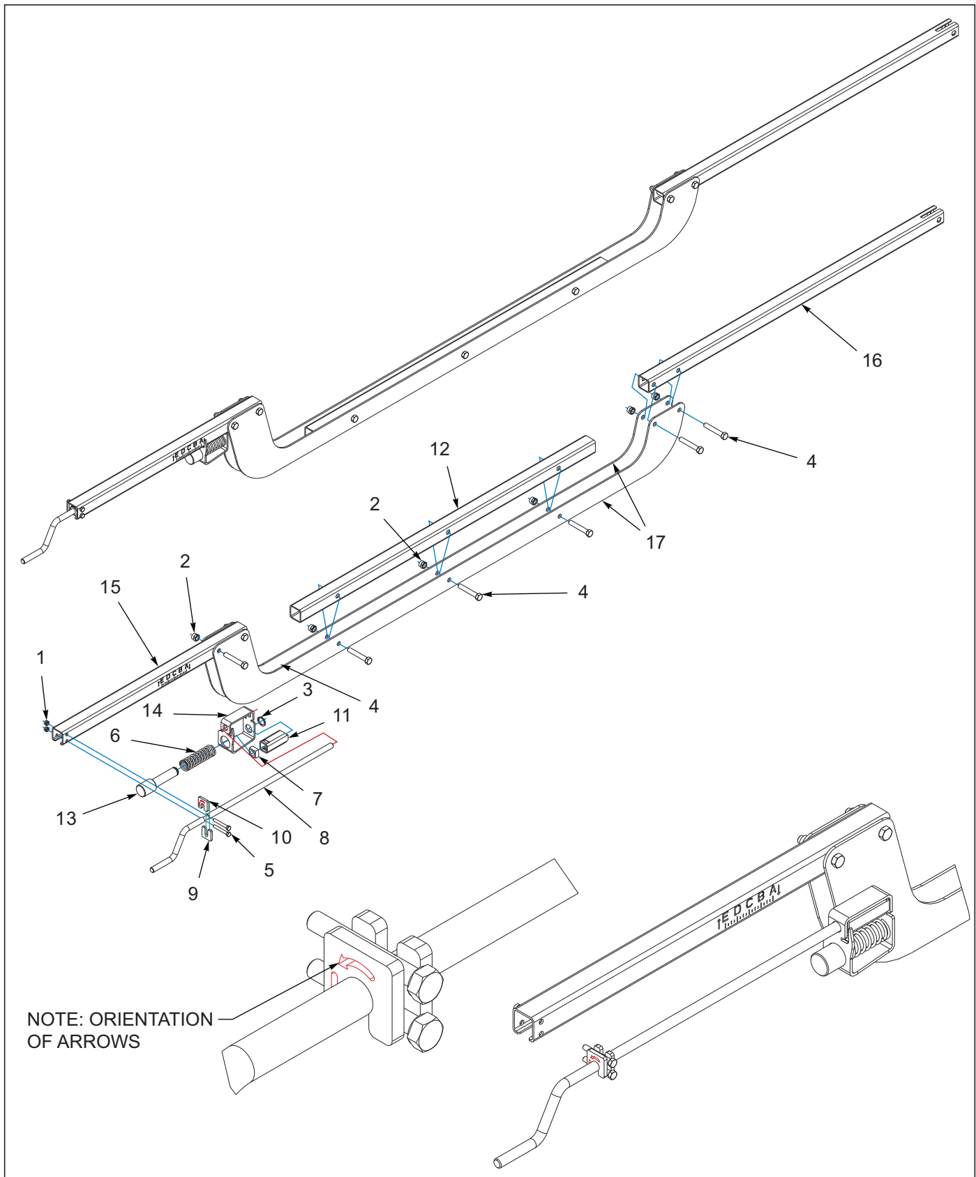
Figure 1-7: Depth Stop Assembly 2431
