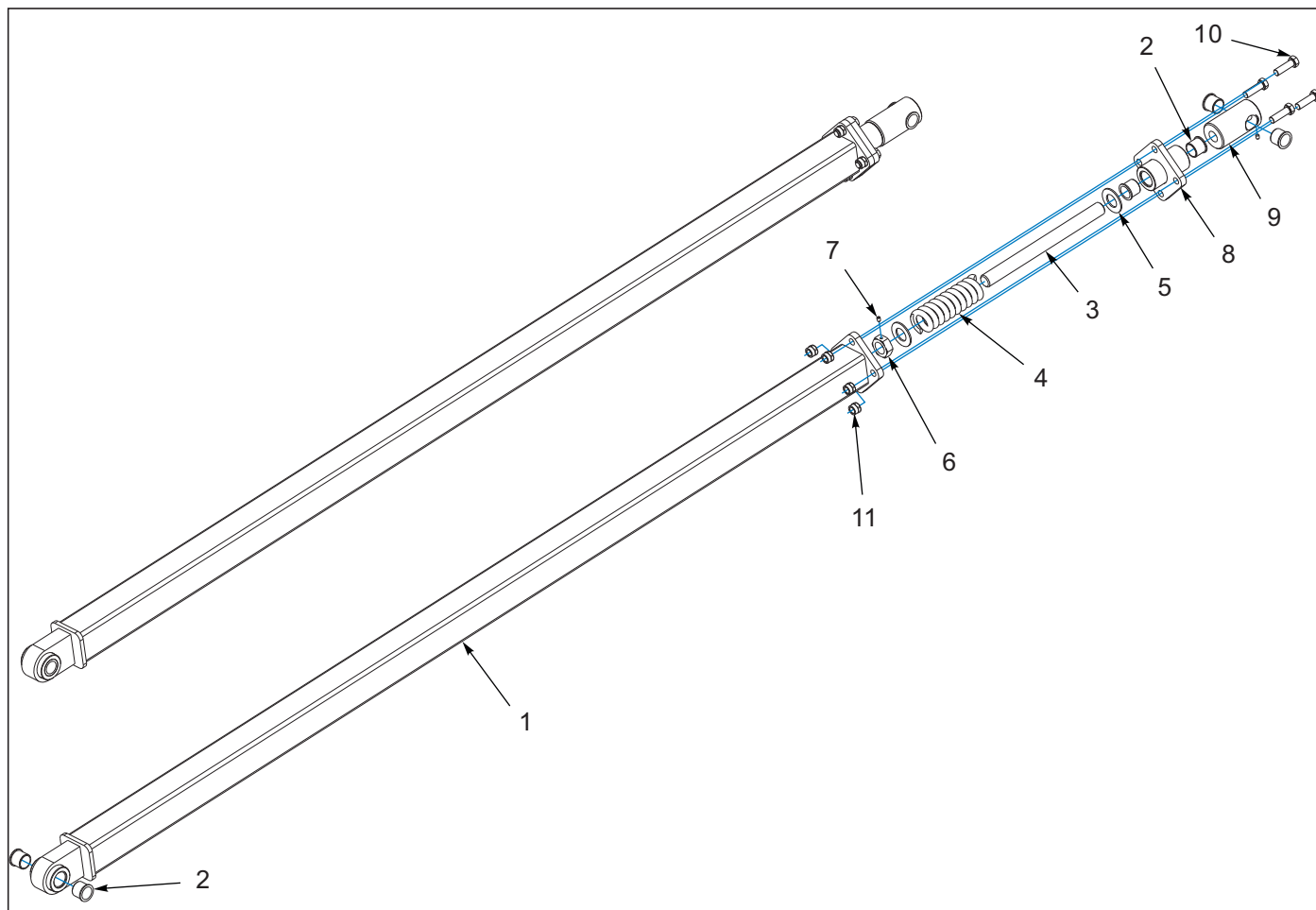
Figure 2-3: Leveler Assembly
