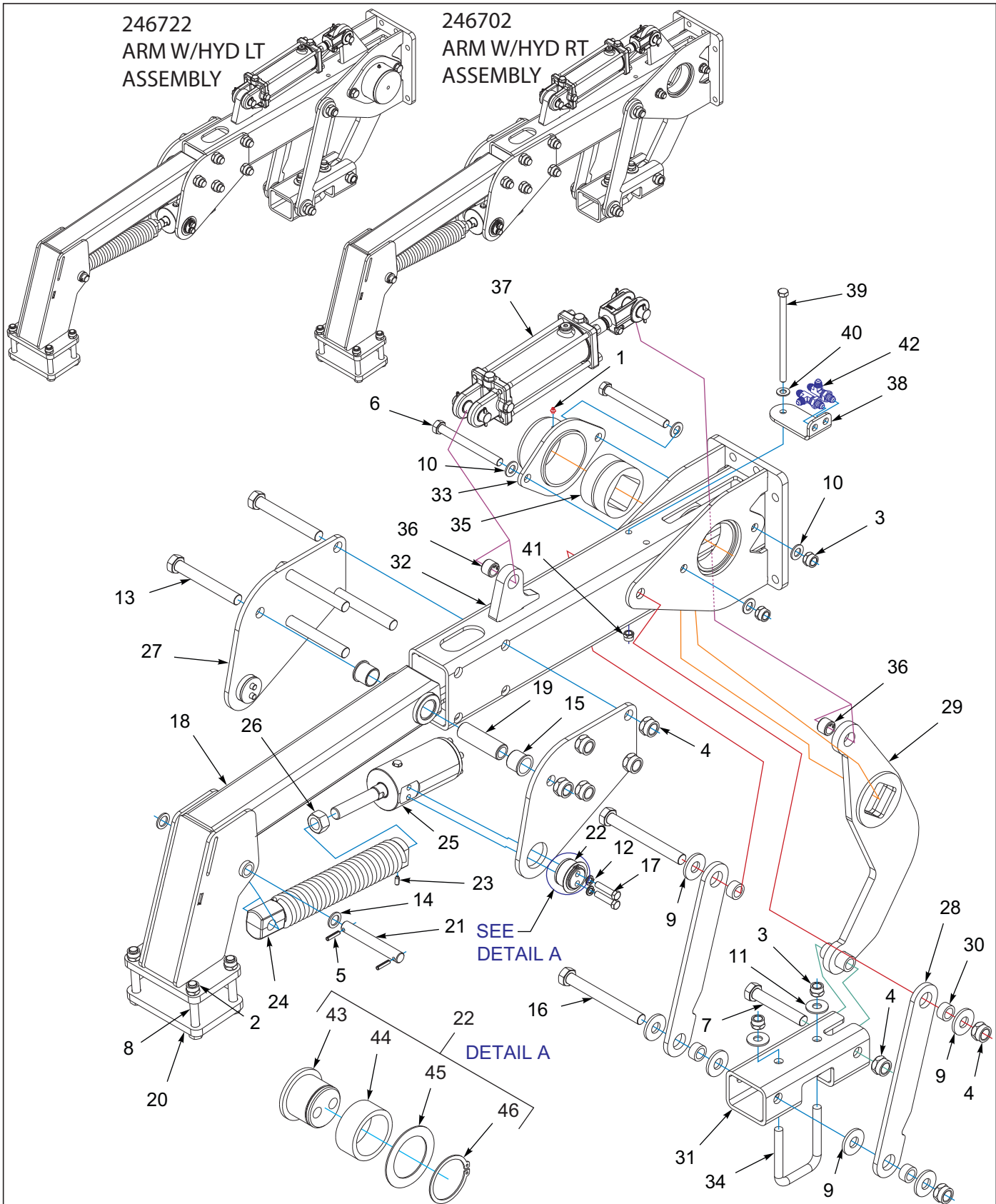
Figure 9-11: Arm With/Hyd Assembly
