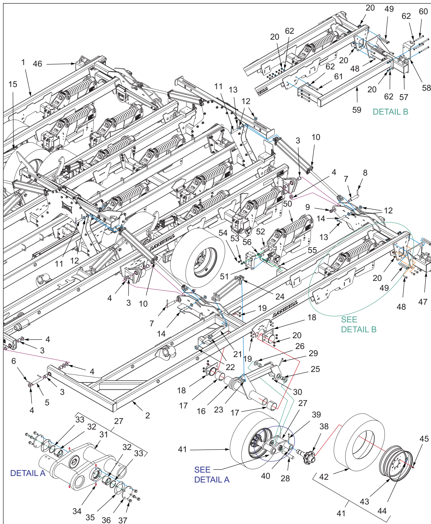
Figure 1-4: Wing Frame Assembly 2431-11/13
