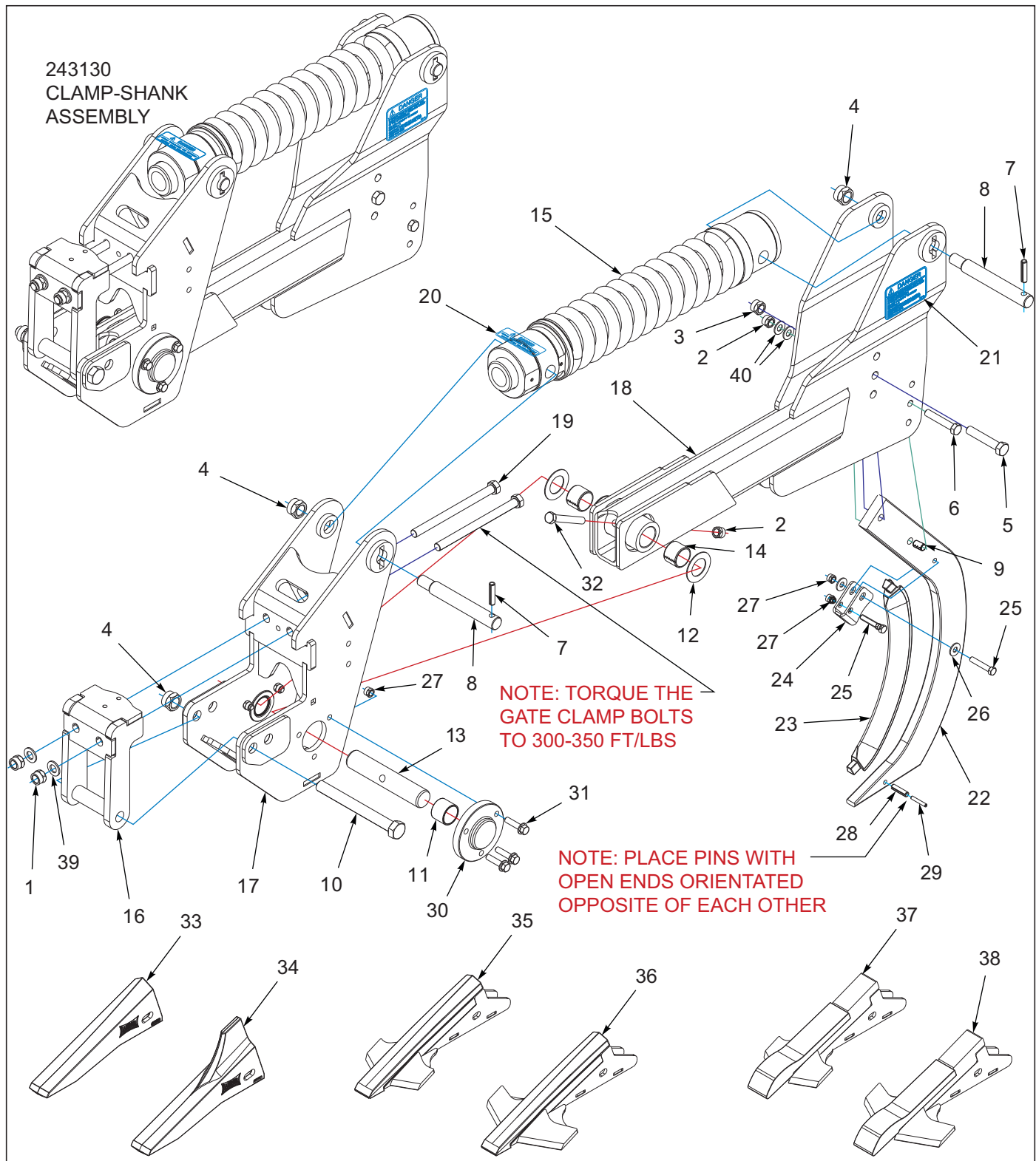
Figure 4-1: Shank Assembly
