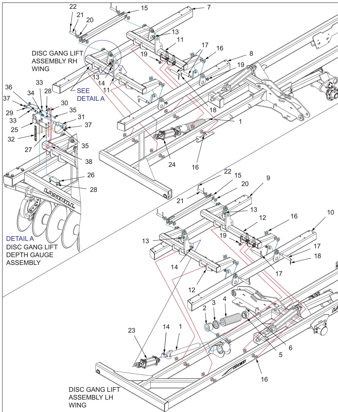
Figure 3-6: Disc Gang Lift Assembly Wing
