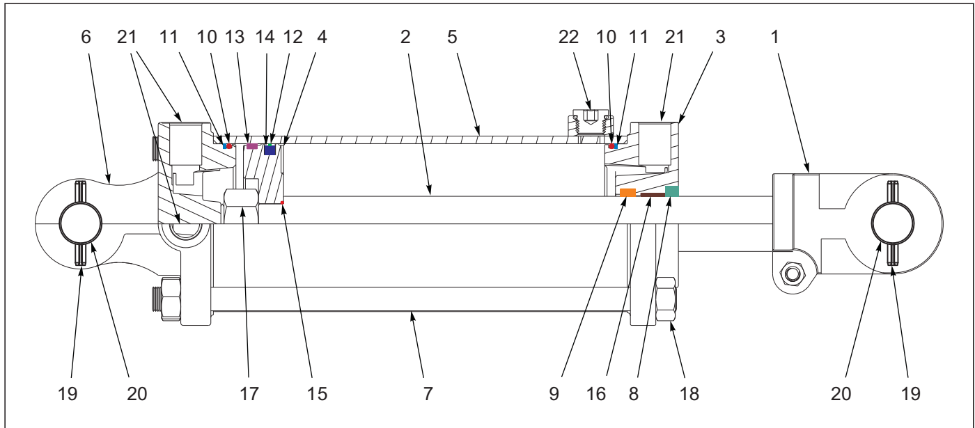
Figure 6-6: Cylinder Assembly 3-3/4 x 8, Rephase (Midway)
