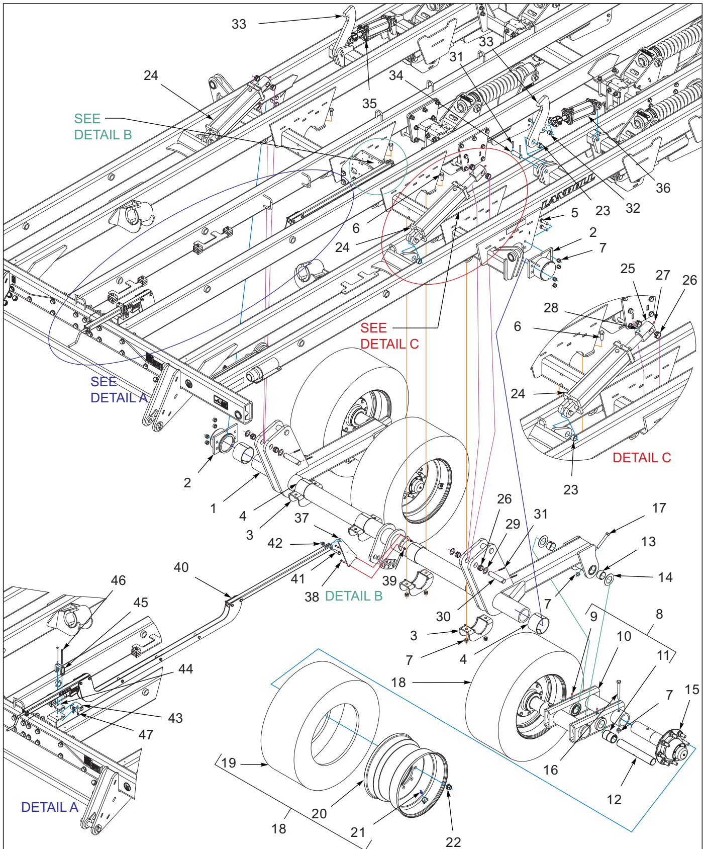
Figure 1-3: Frame Assembly Center Lift
