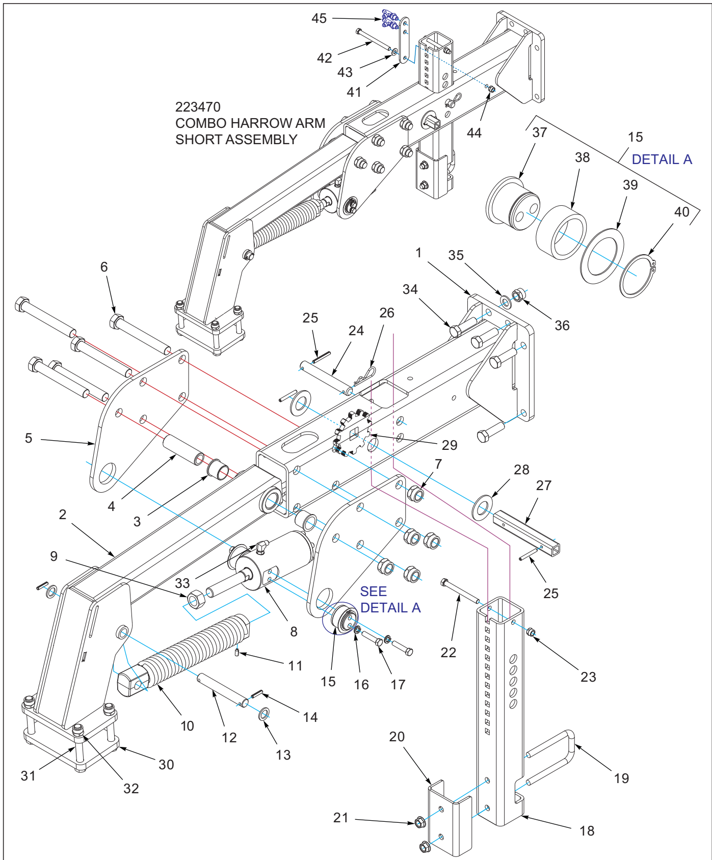
Figure 9-3: Harrow Arm Assembly Combo Hydraulic Short
