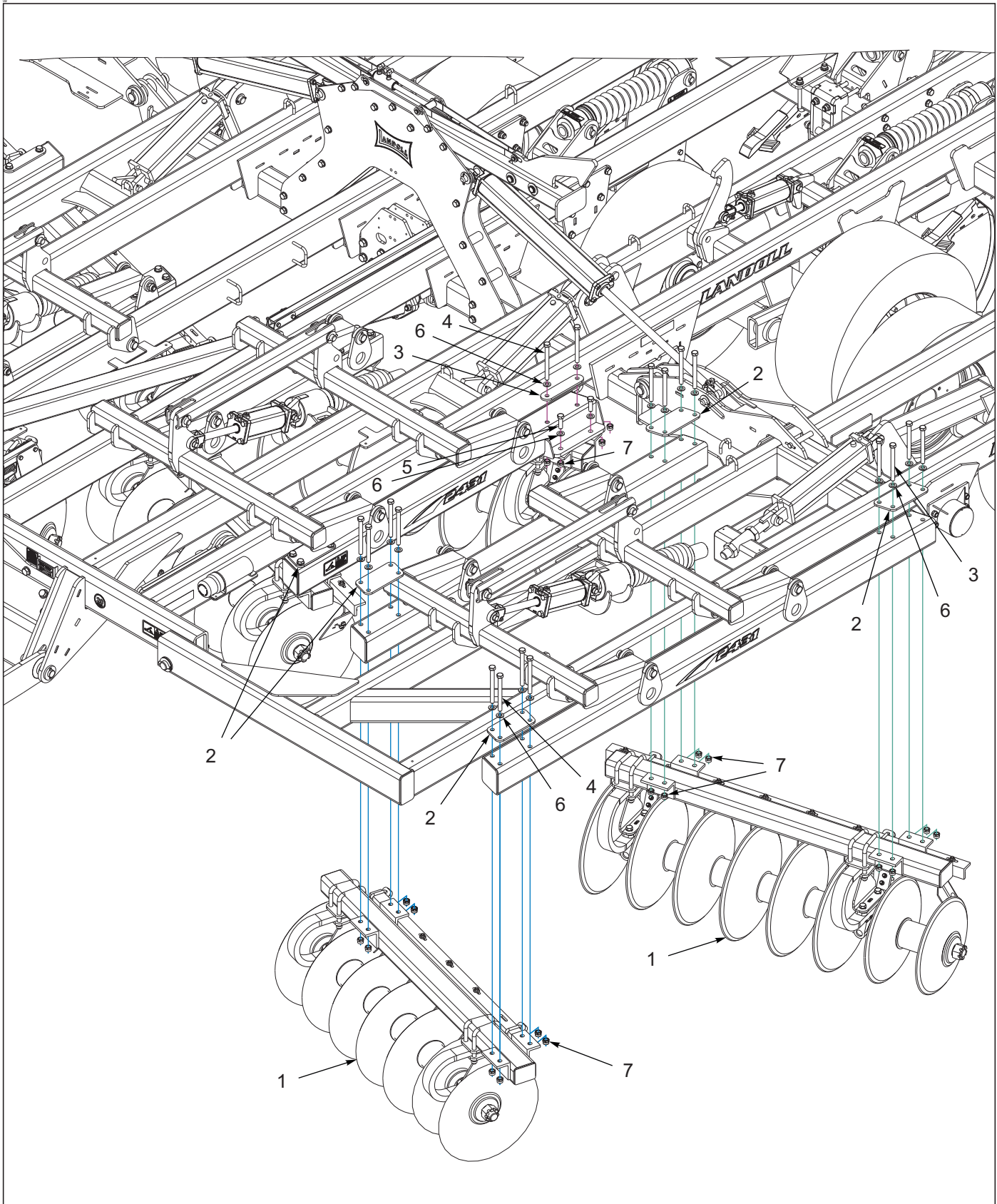
Figure 3-7: Disc Gang To Frame Assembly
