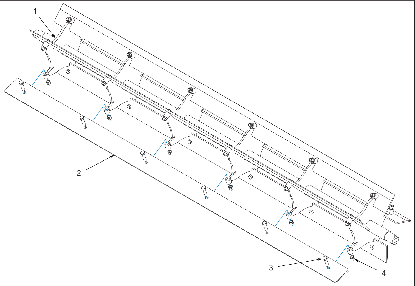
Figure 9-6: Reel Blade Assembly
