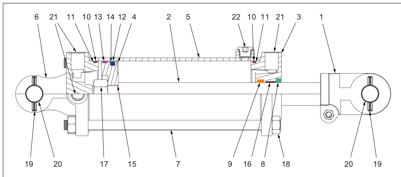
Figure 6-8: Cylinder Assembly 3-1/2 x 8, Rephase (Midway)
