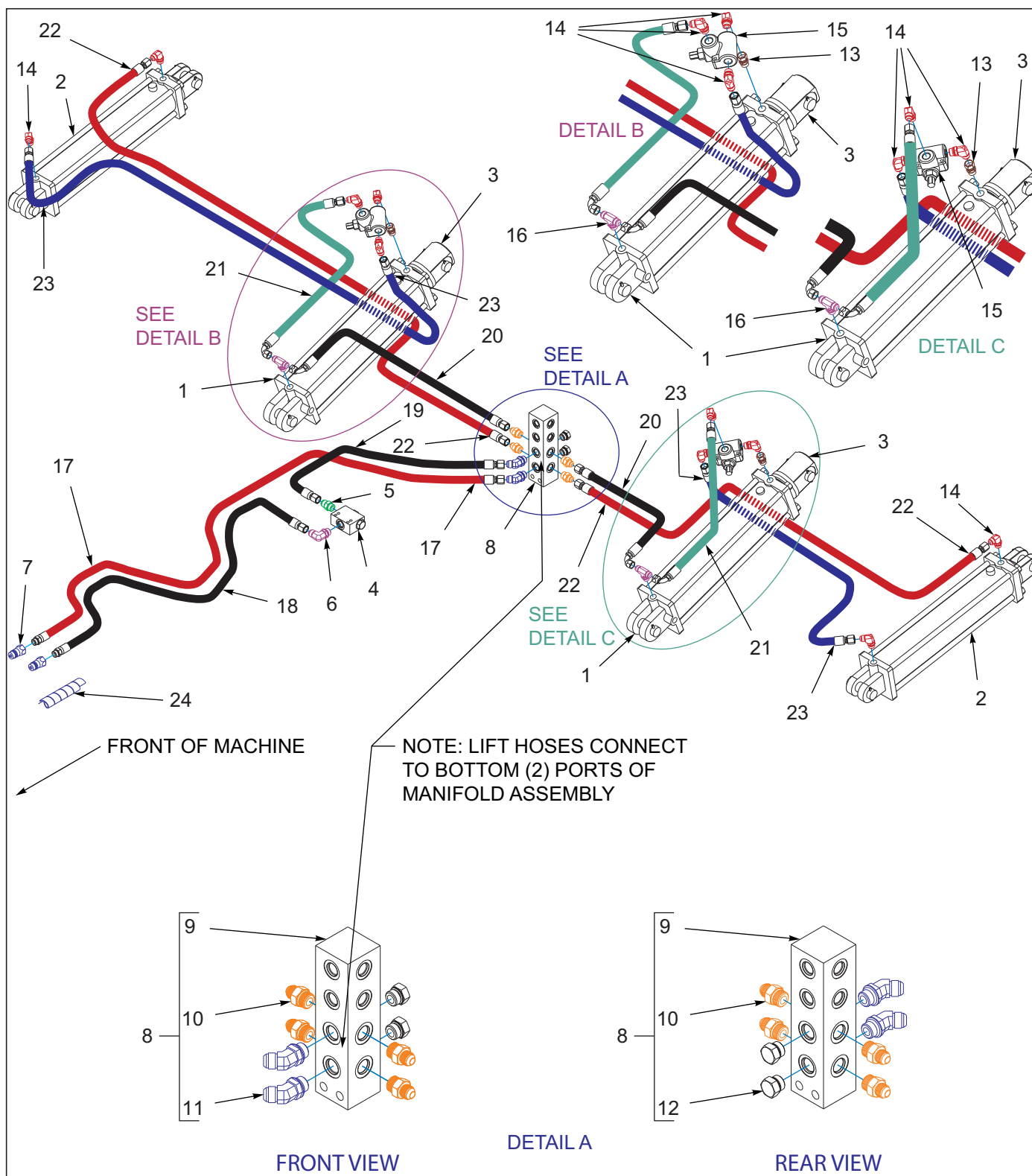
Figure 5-1: Lift Assembly
