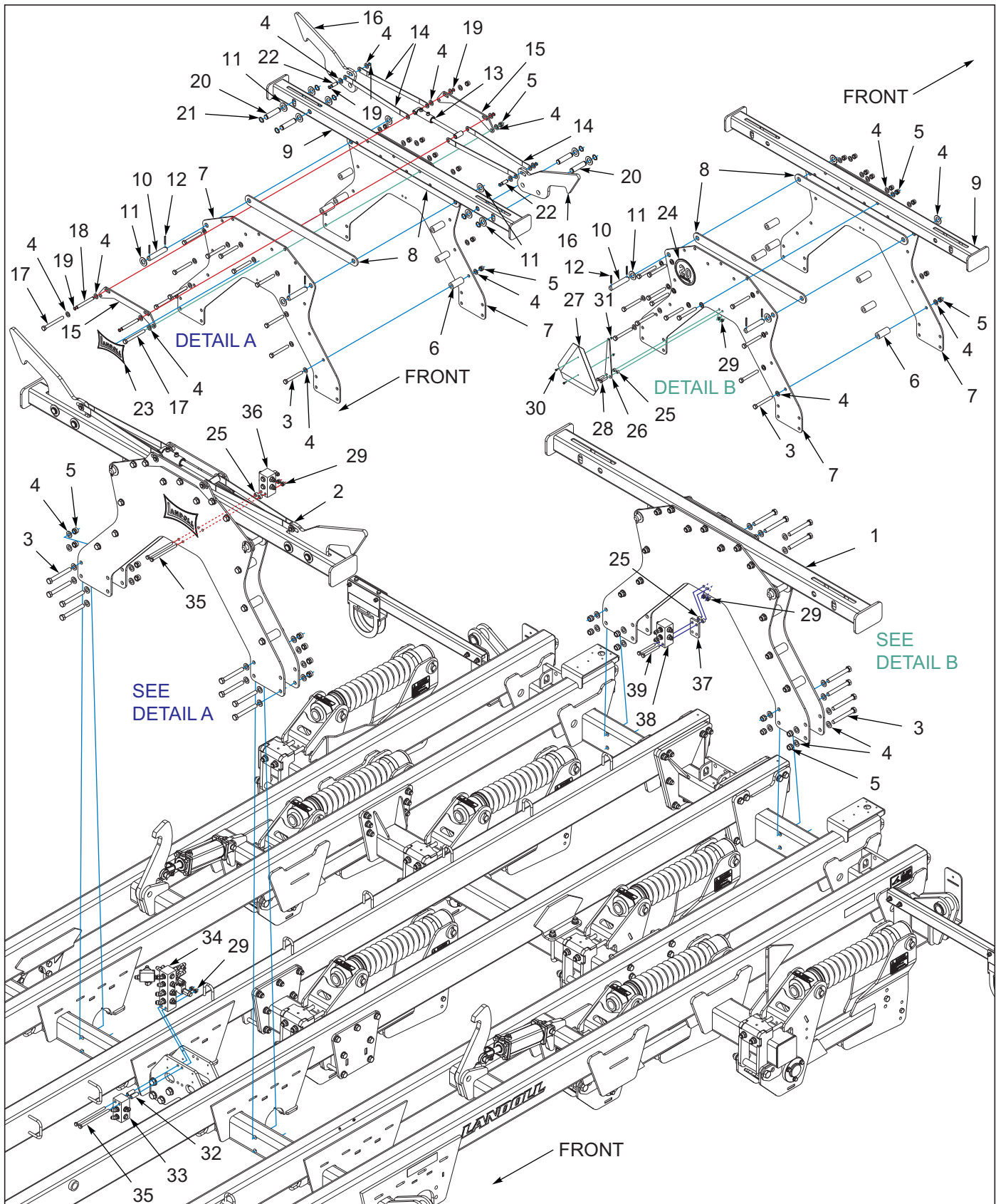
Figure 1-2: Frame Assembly Center Fold
