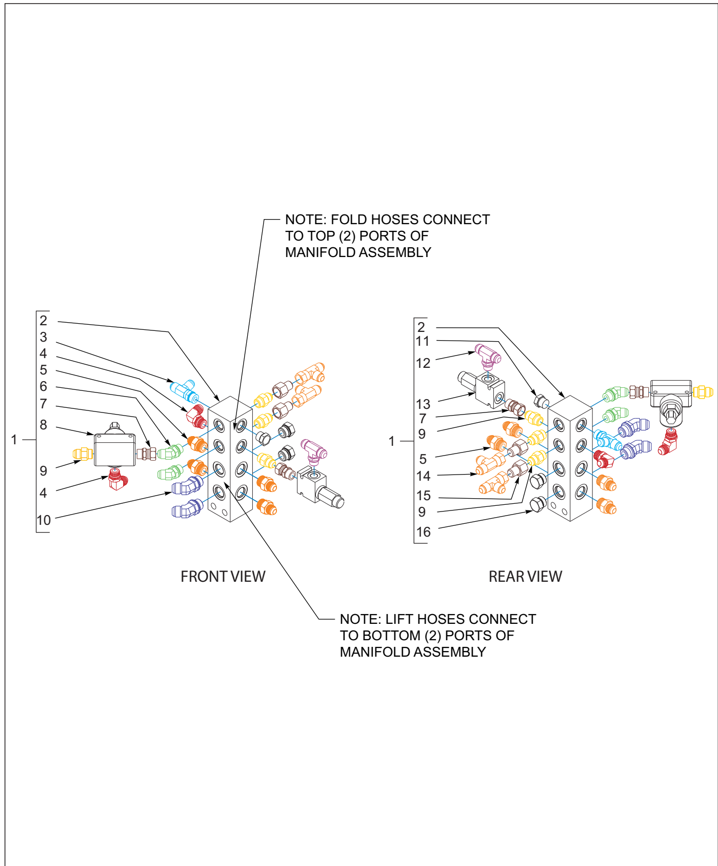
Figure 5-4: Manifold Assembly 246765
