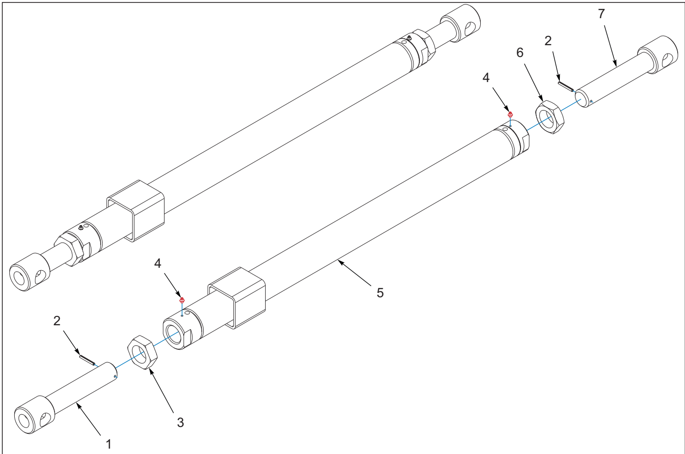
Figure 2-2: Radius Assembly
