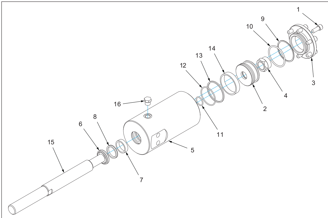
Figure 6-14: Cylinder Assembly 2-1/2 x 3-1/2
