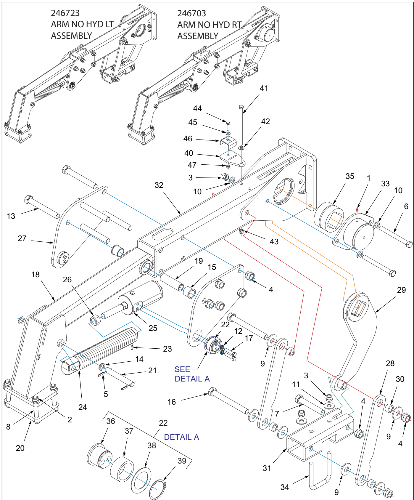
Figure 9-10: Arm No/Hyd Assembly
