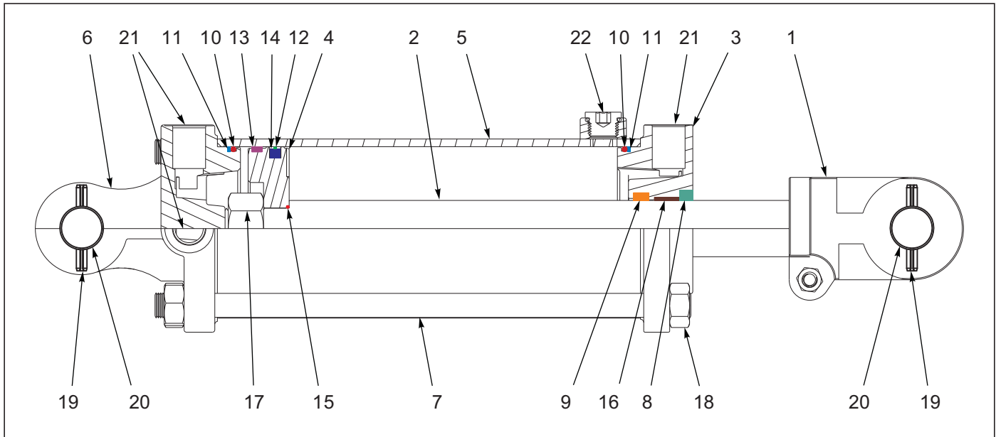
Figure 6-4: Cylinder Assembly 4 x 8, Rephase (Midway)
