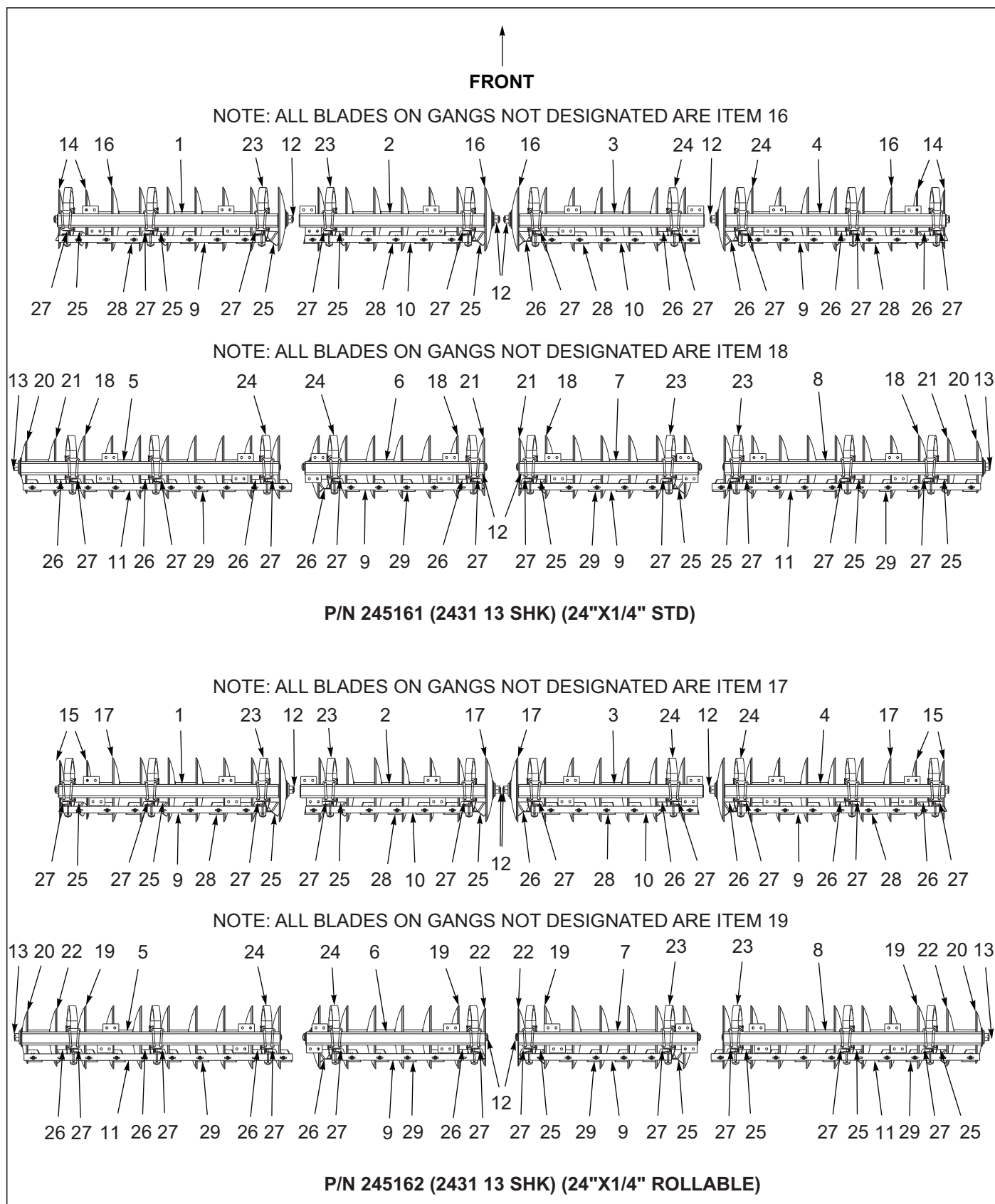
Figure 3-4: Disc Gang Placement 24" Blade (2431-13 Shank)
