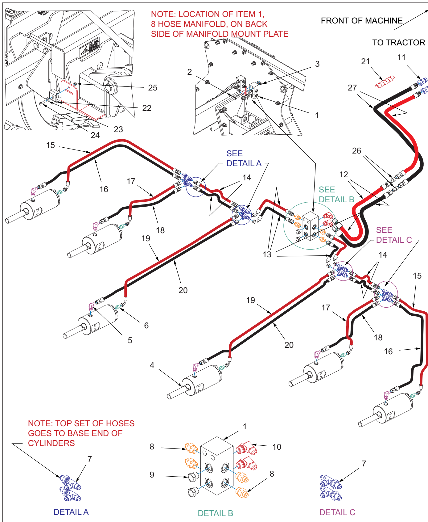
Figure 9-7: 3BCT/Chopper Hydraulic Assembly
