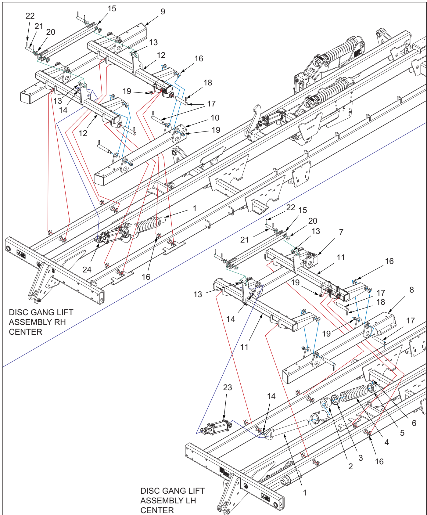
Figure 3-5: Disc Gang Lift Assembly Center
