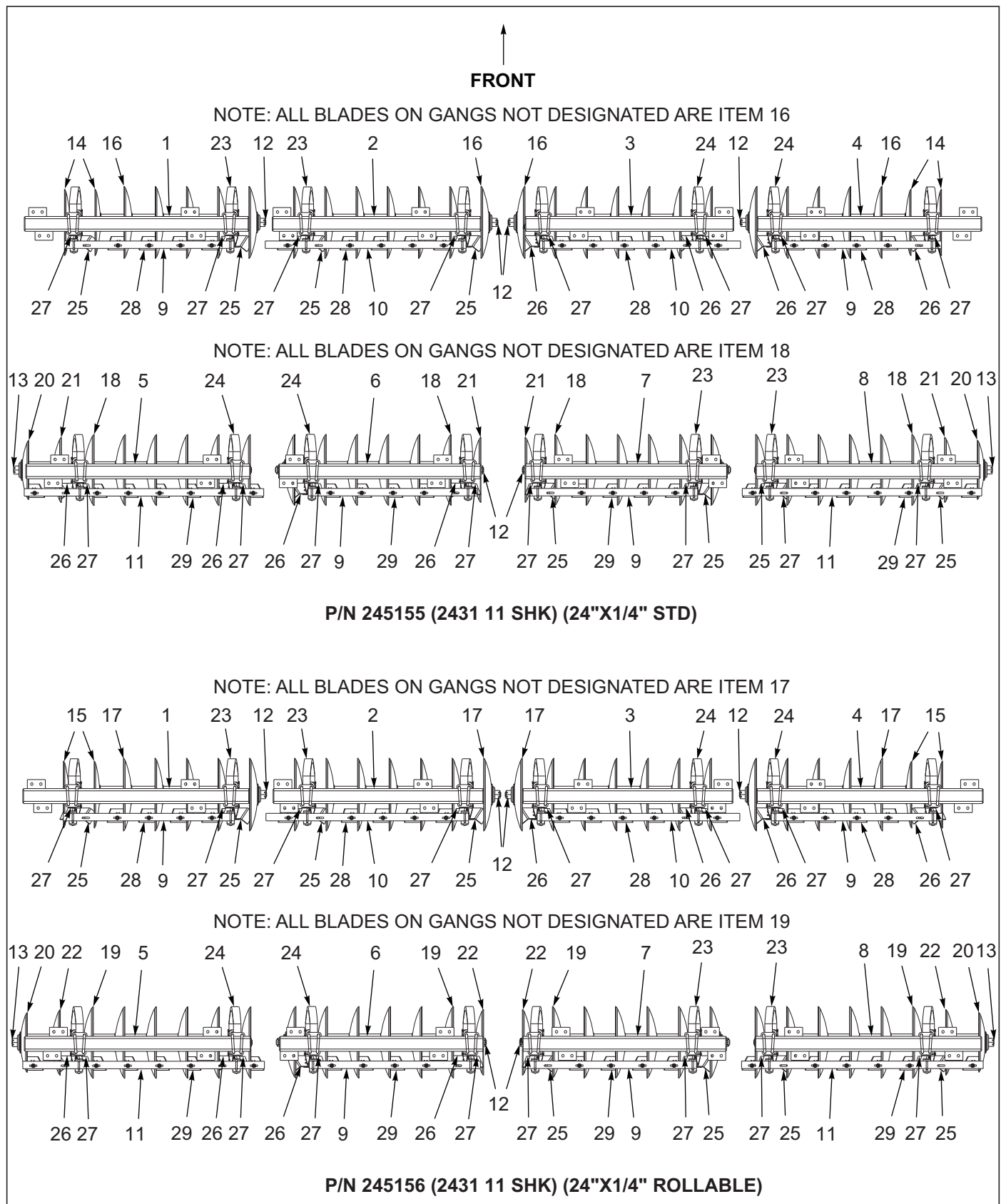
Figure 3-3: Disc Gang Placement 24" Blade (2431-11 Shank)
