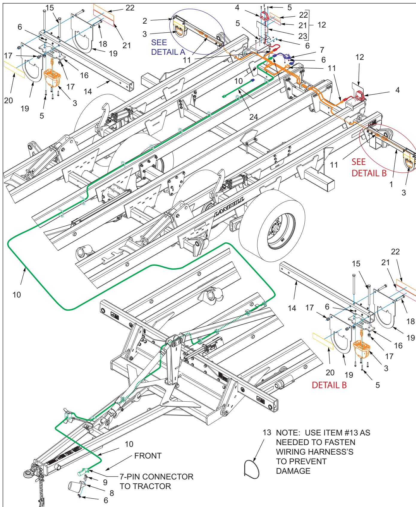
Figure 7-2: Electrical Assembly W/LED Lights
