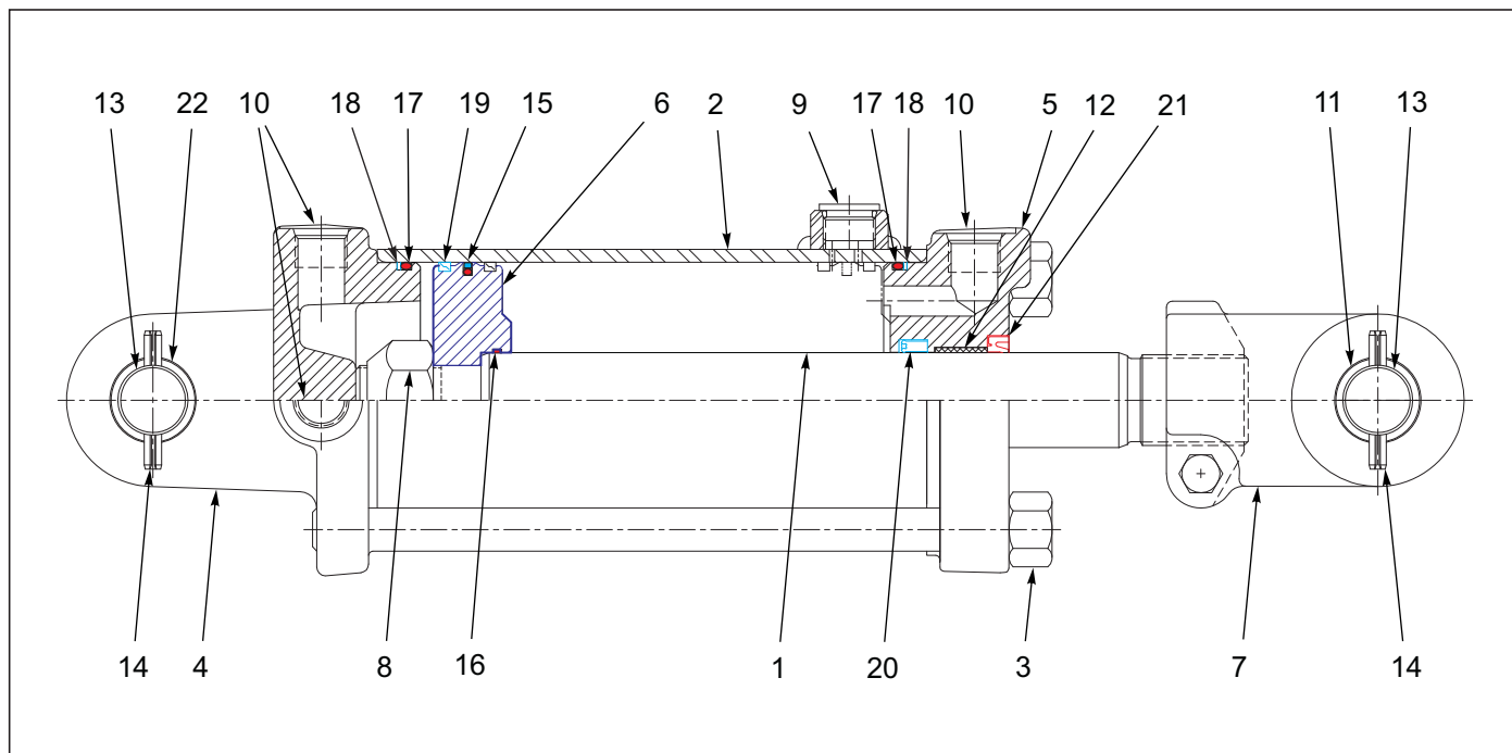
Figure 6-7: Cylinder Assembly 3-1/2 x 8, Rephase (Prince)
