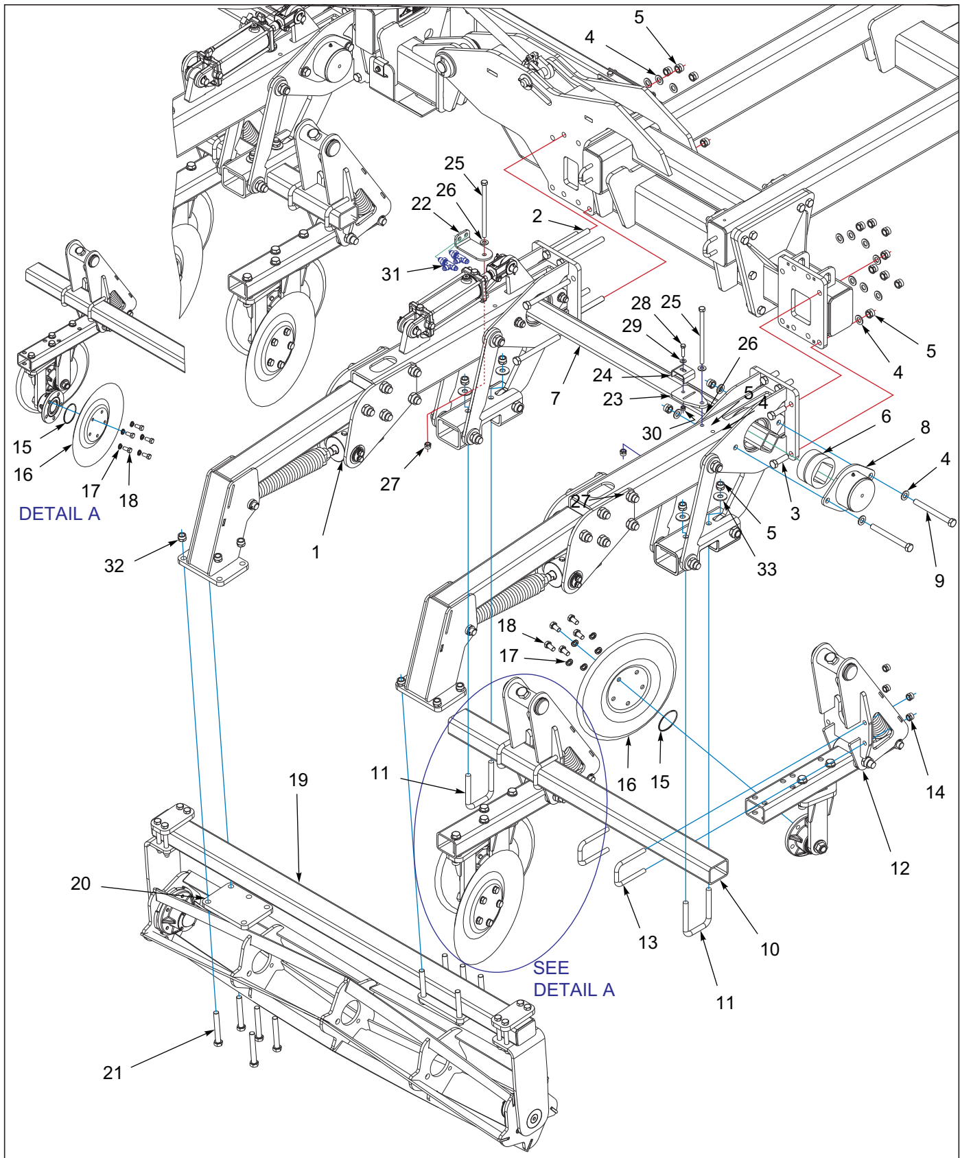
Figure 9-8: Disc Lev/Hyd RL W/Bearing Assembly
