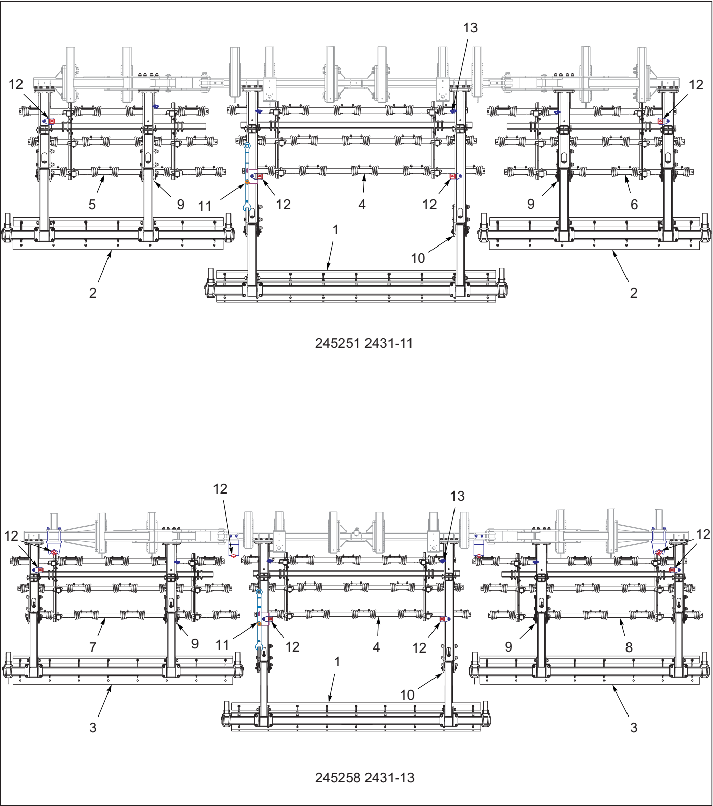
Figure 9-1: 3BCT W/Hydraulic Chopper Layout
