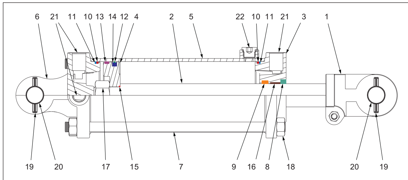
Figure 6-10: Cylinder Assembly 3-1/4 x 8, Rephase (Midway)
