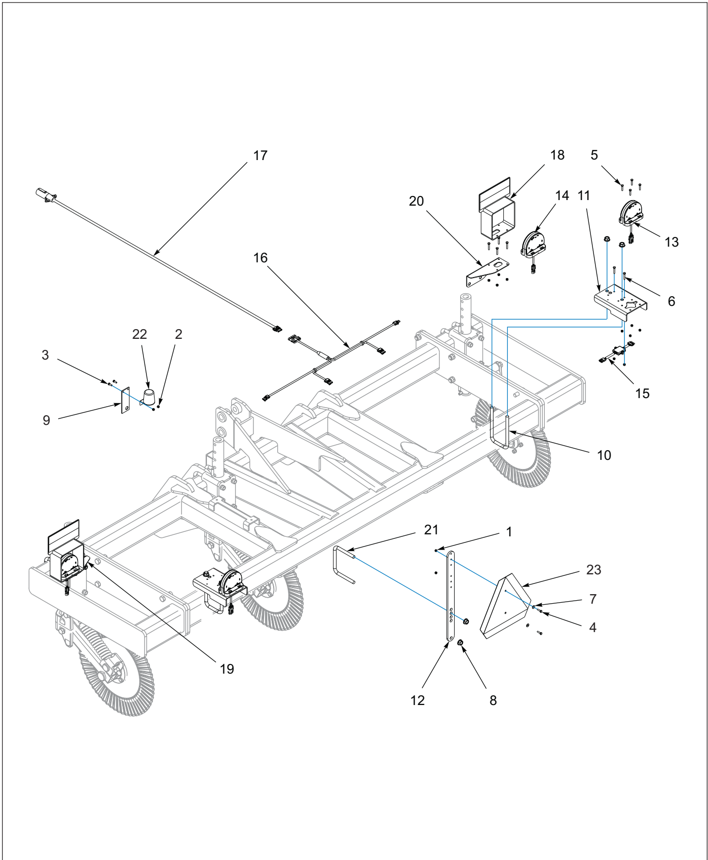
Figure 4-2: Electrical - 5 Shanks
