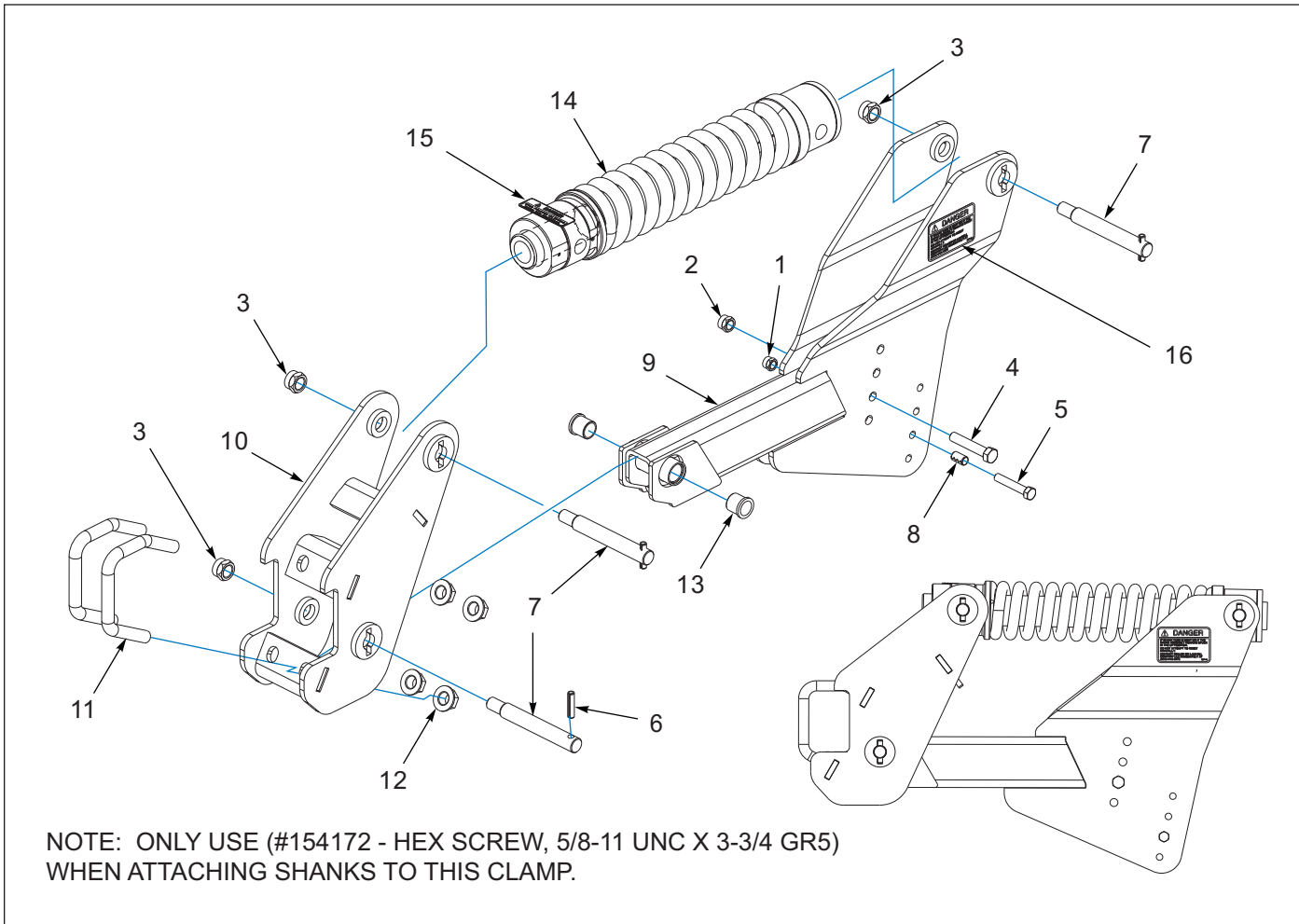
Figure 1-3: Auto Reset Clamp Assembly
