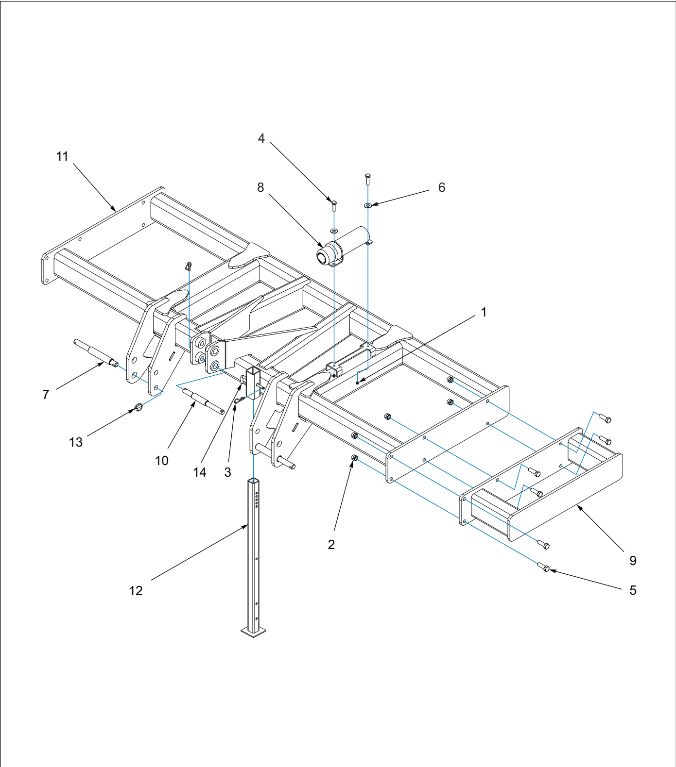
Figure 1-1: Narrow Frame
