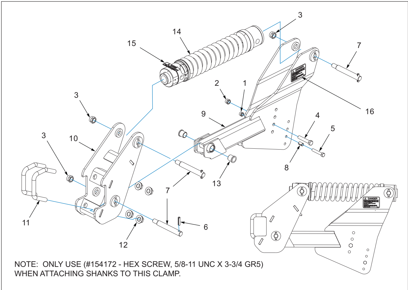
Figure 1-3: Auto Reset Clamp Assembly
