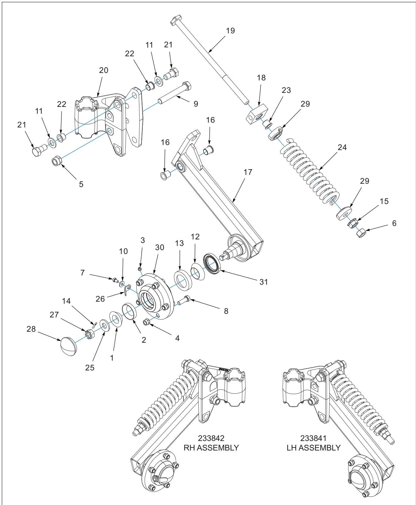
Figure 3-3: Heavy Duty Coulter (AFTER 02/2022)
