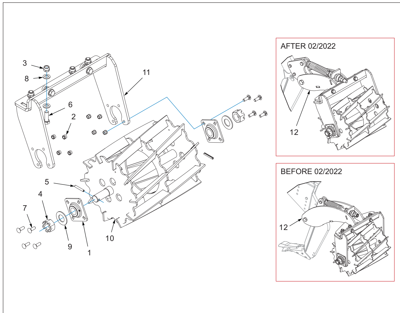
Figure 5-8: Flat Bar Basket - 20"
