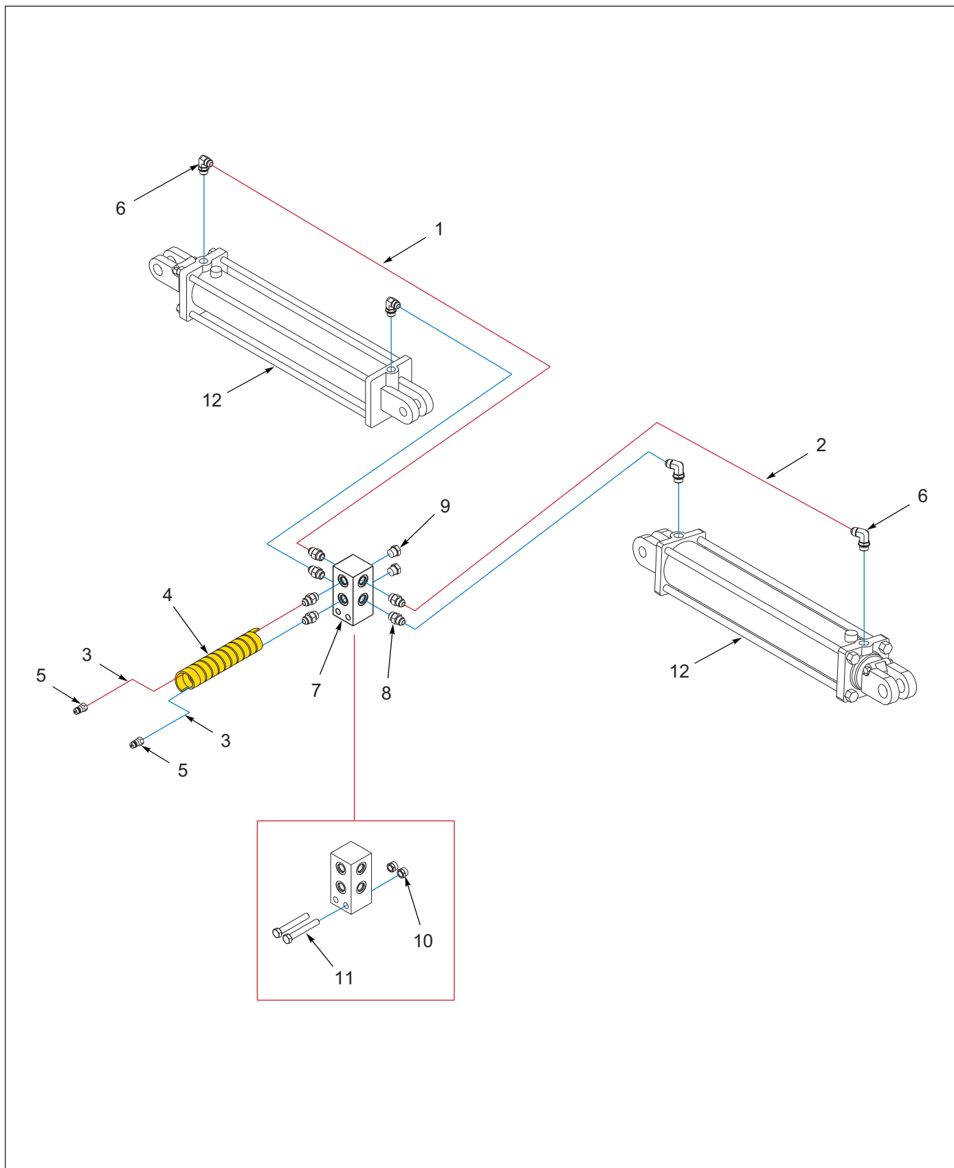
Figure 4-2: Folding Frame Hydraulic Diagram (BEFORE 11/01/2021)
