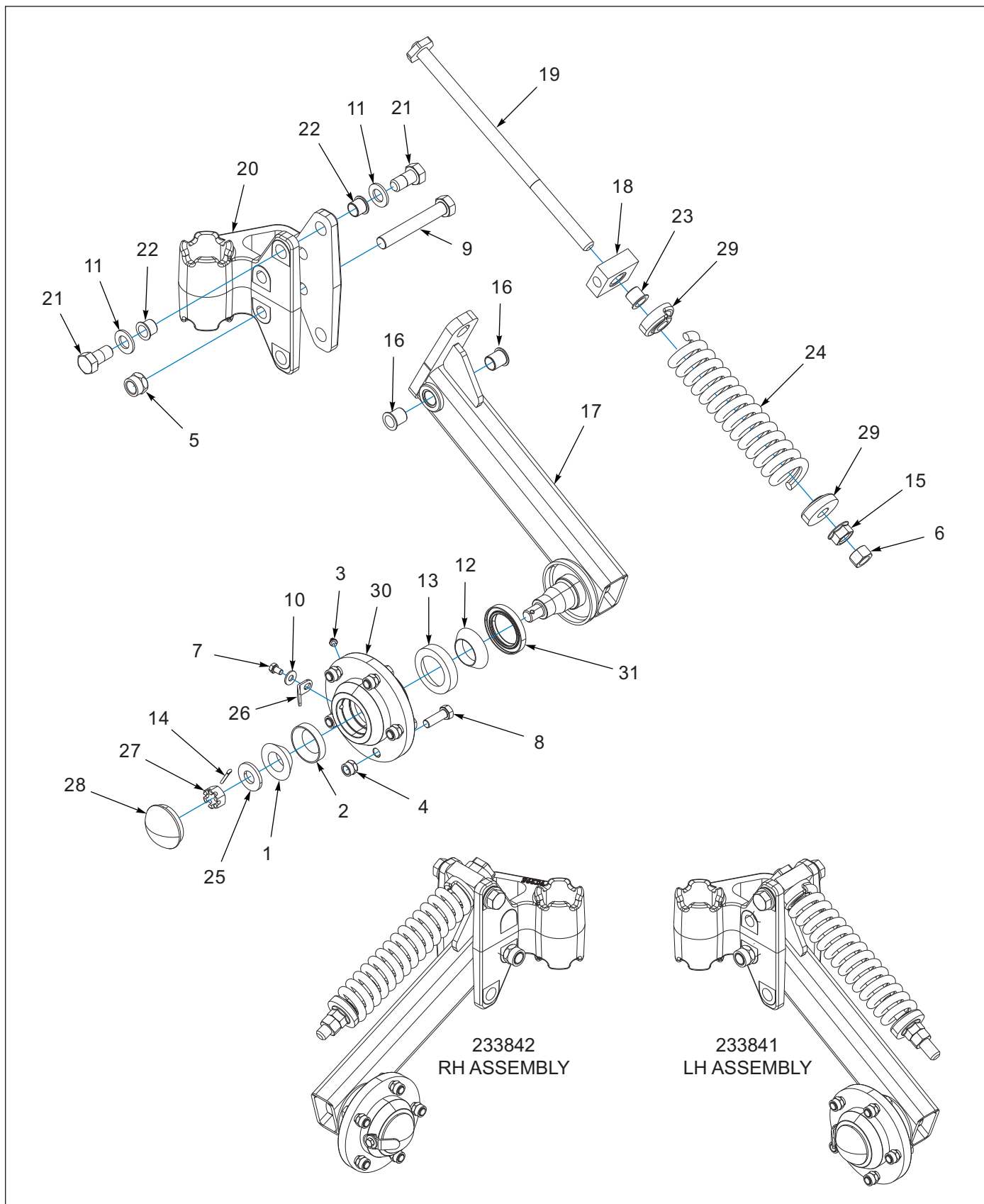
Figure 2-3: Heavy Duty Coulter (AFTER 02/2022)
