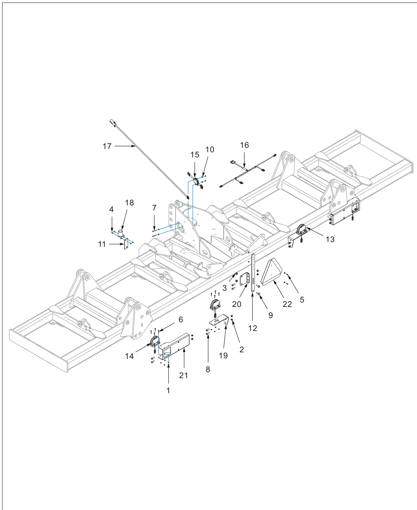
Figure 3-3: Lighting and Reflectors (Folding)
