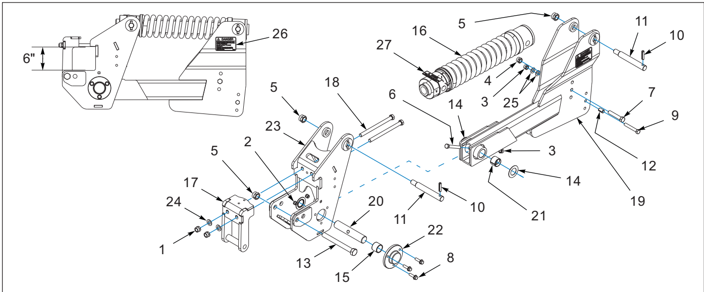
Figure 1-5: Auto Reset Shank Clamp, Spring (AFT. 01/01/2024)
