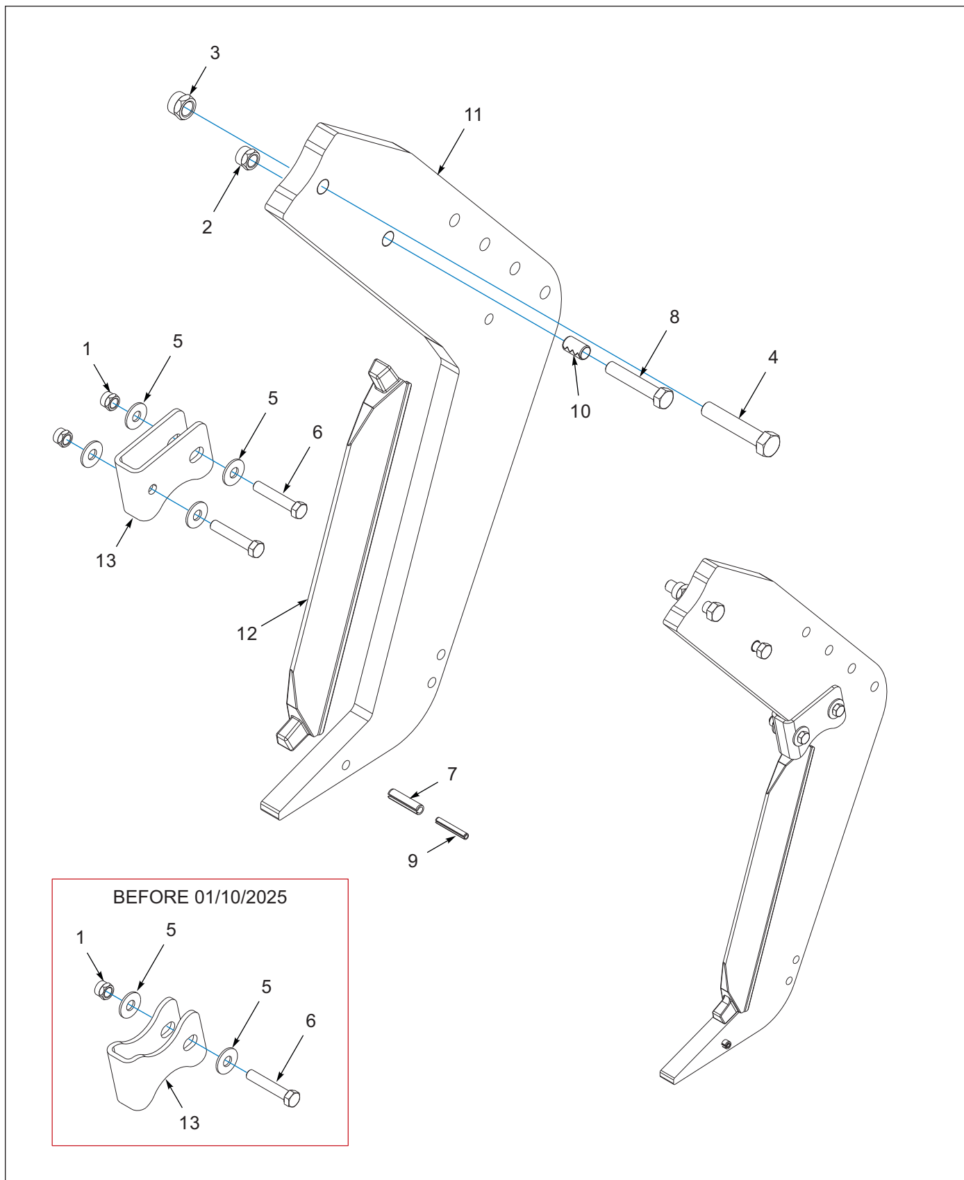
Figure 5-2: Straight Leg Shank, 1-1/4
