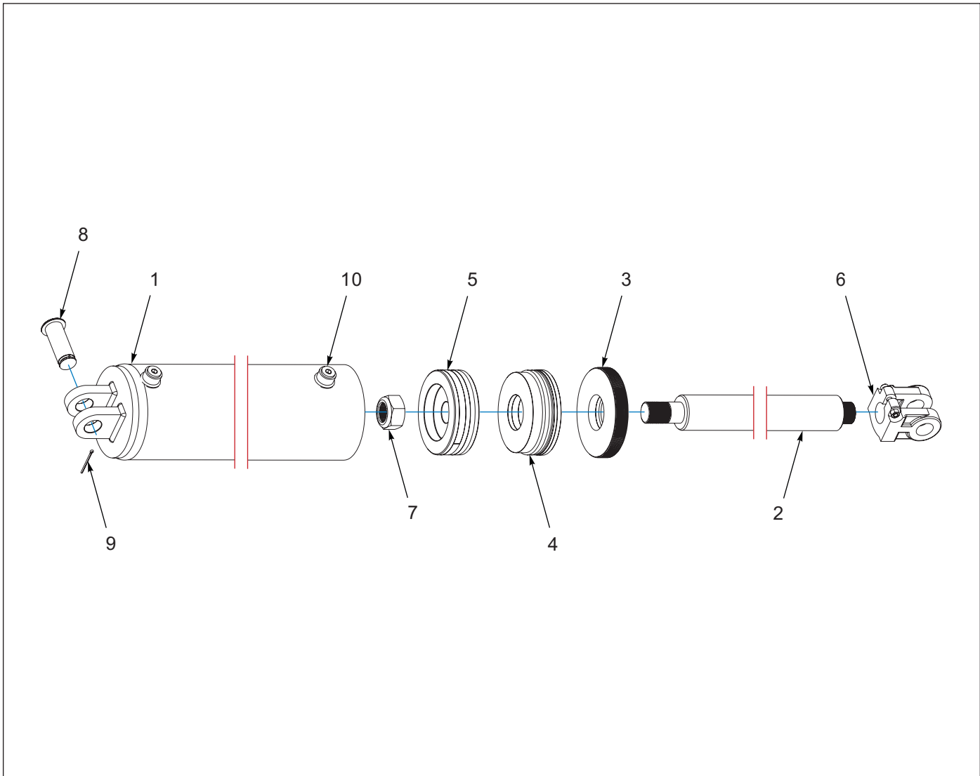
Figure 4-21: Hydraulic Cylinder, 6 x 30 - 233833
