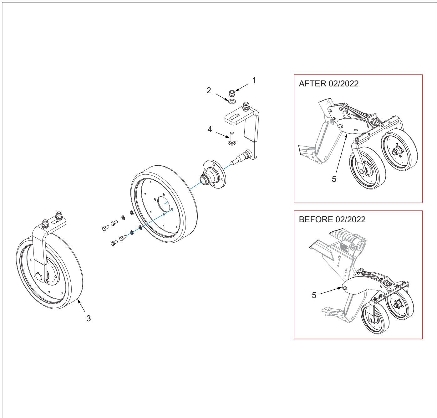
Figure 7-7: Closer Wheel
