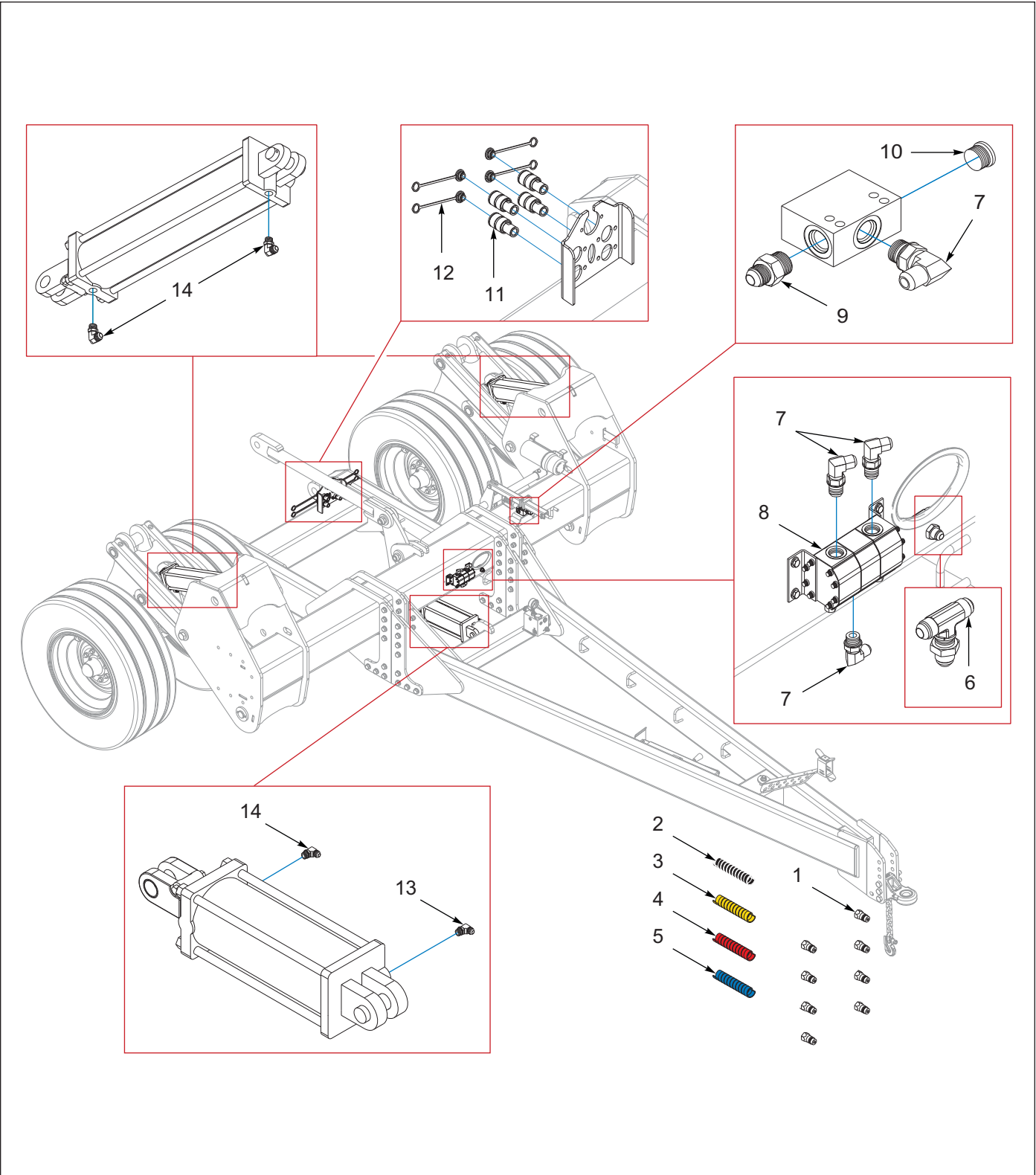
Figure 4-1: Hydraulic Kit
