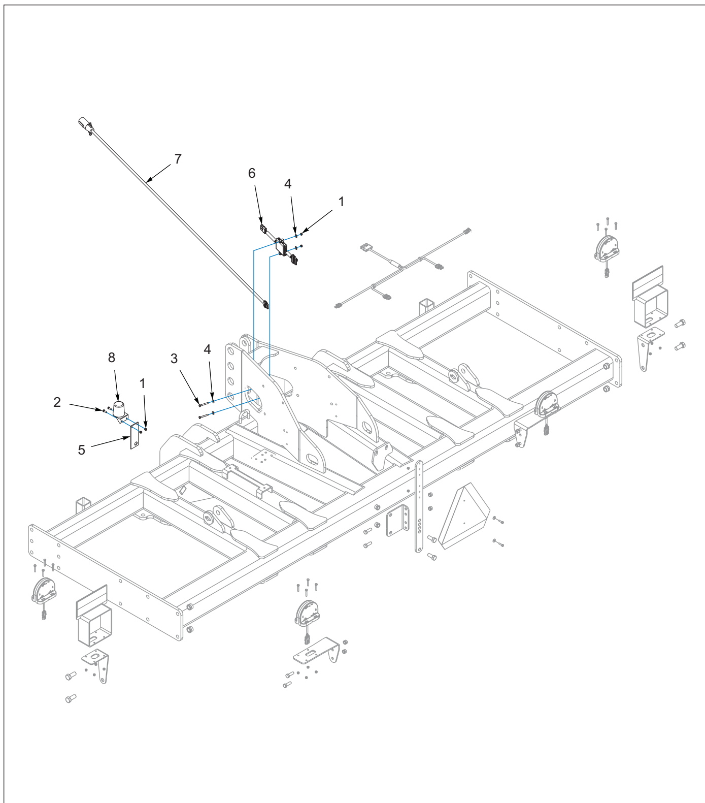
Figure 2-1: Wiring Components
