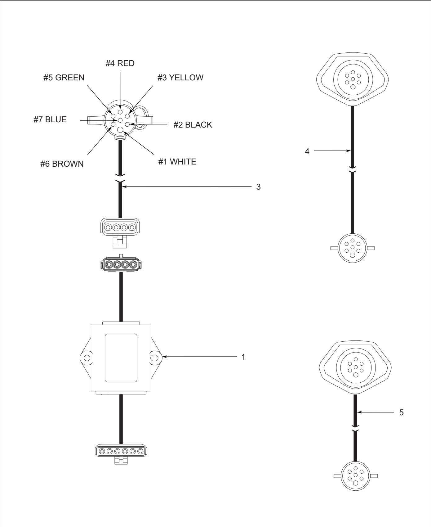
Figure 2-2: Wiring Diagram
