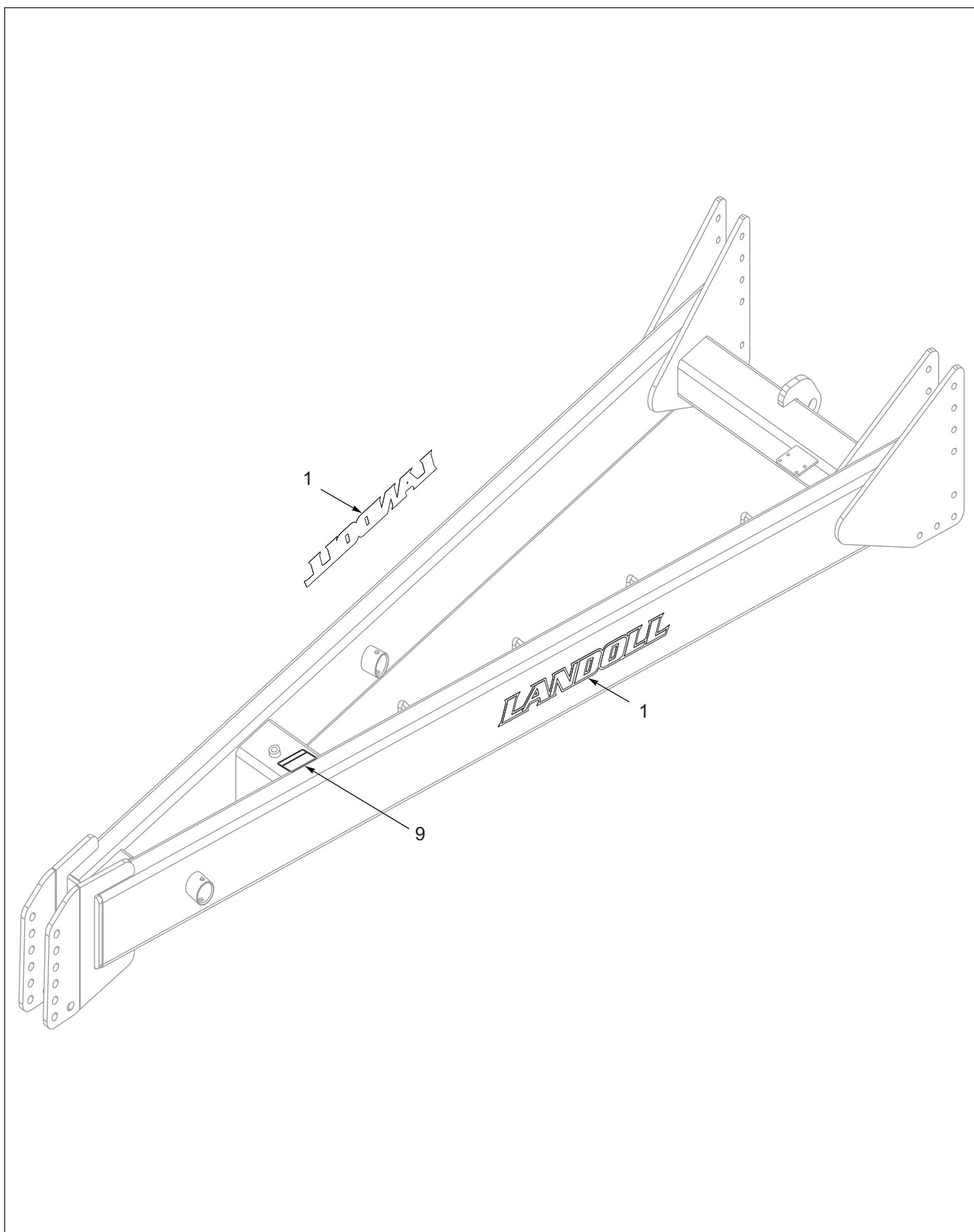
Figure 5-3: Decal Placement - Caddy (2 of 2)
