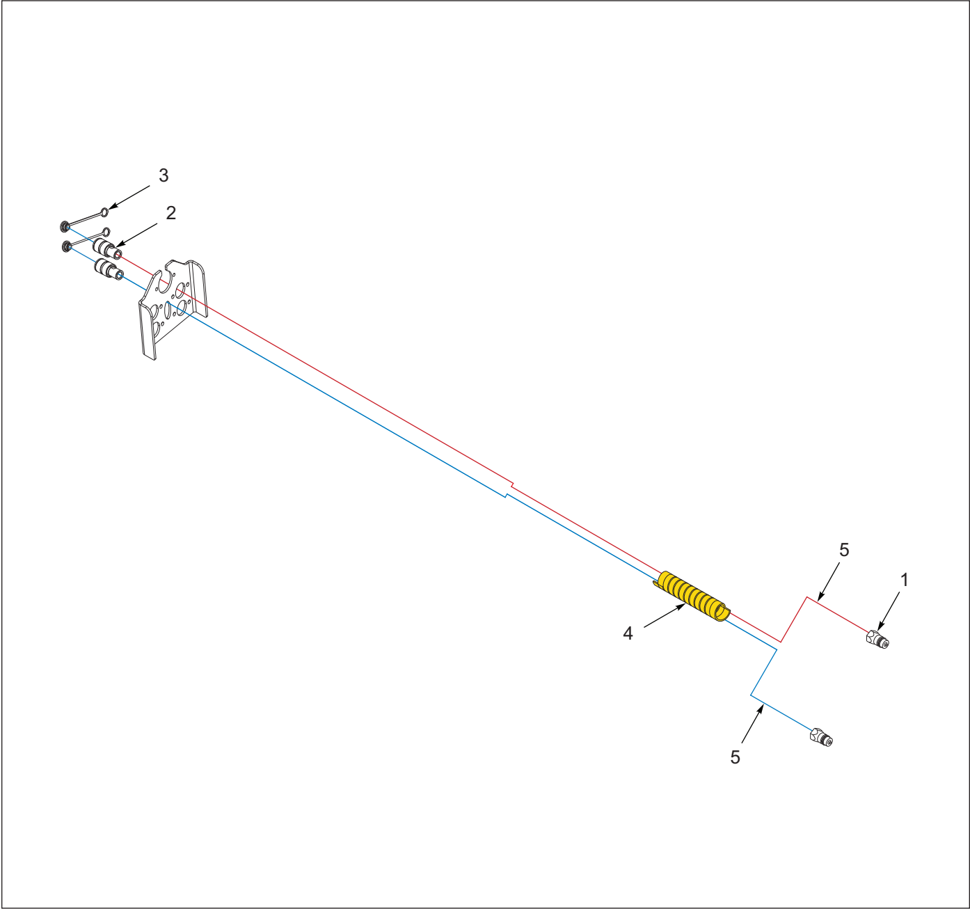
Figure 4-4: Caddy Wing Circuit
