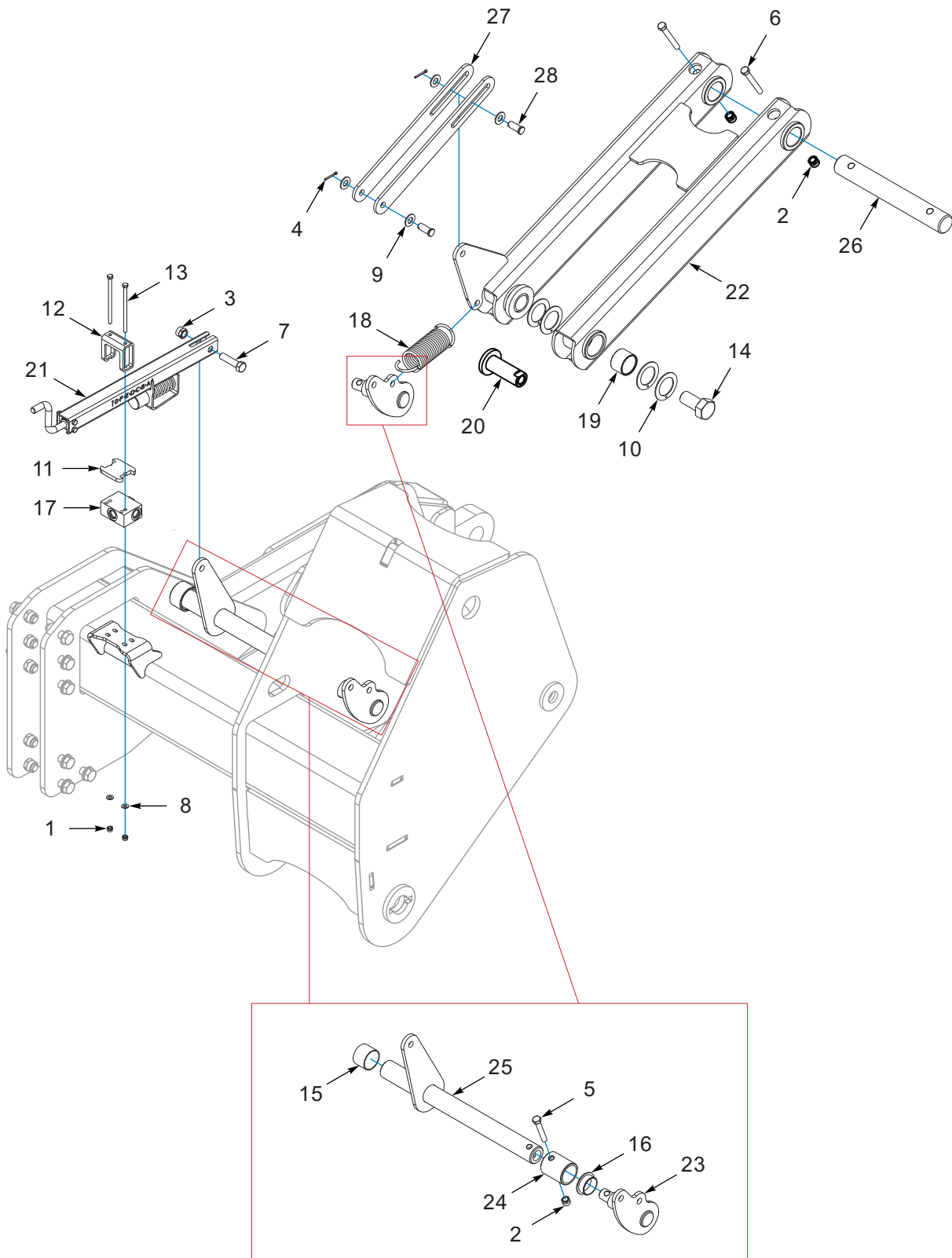
Figure 3-5: Standard Caddy Depth Control Assembly
