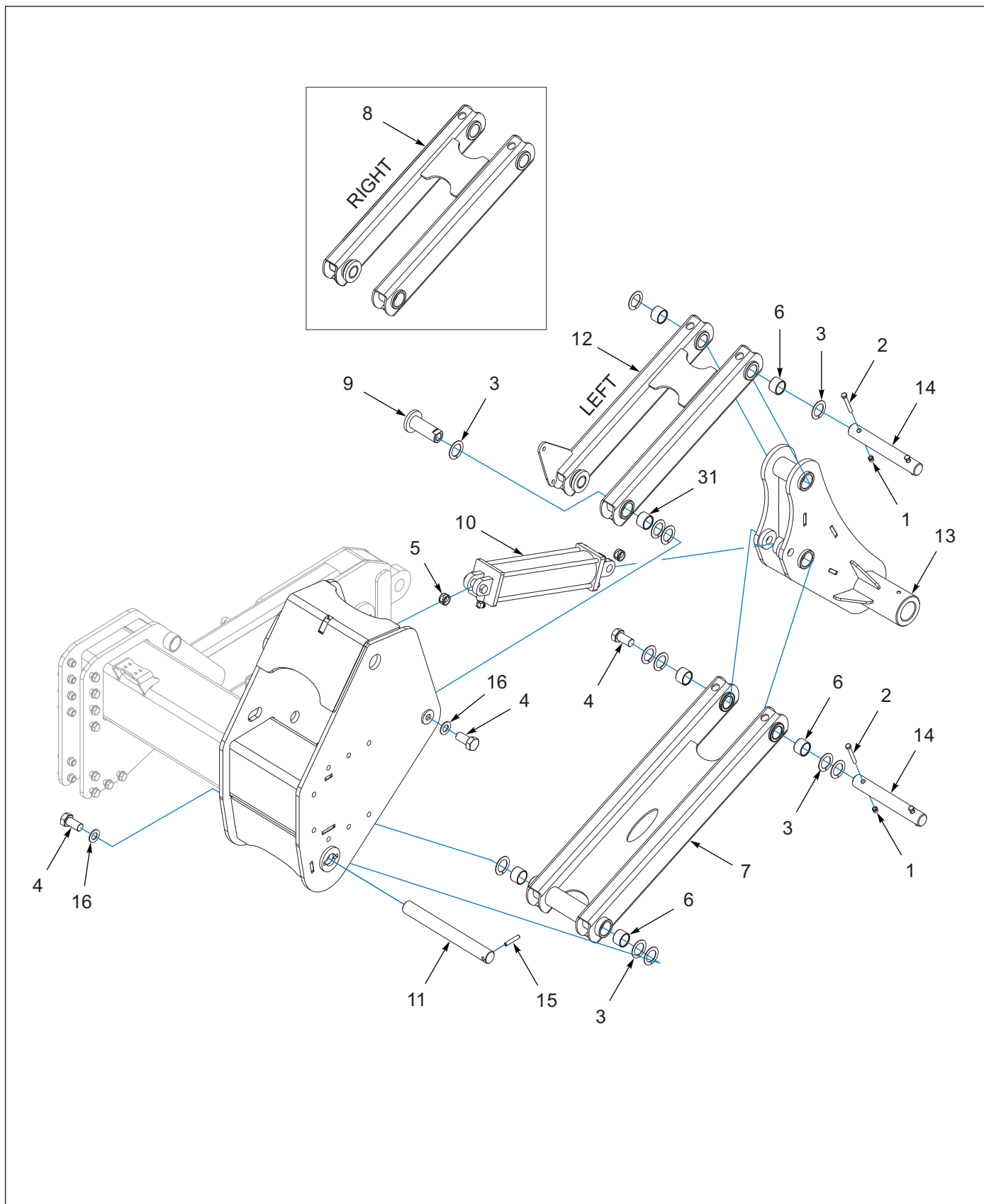
Figure 3-3: Standard Axle Lift Assembly
