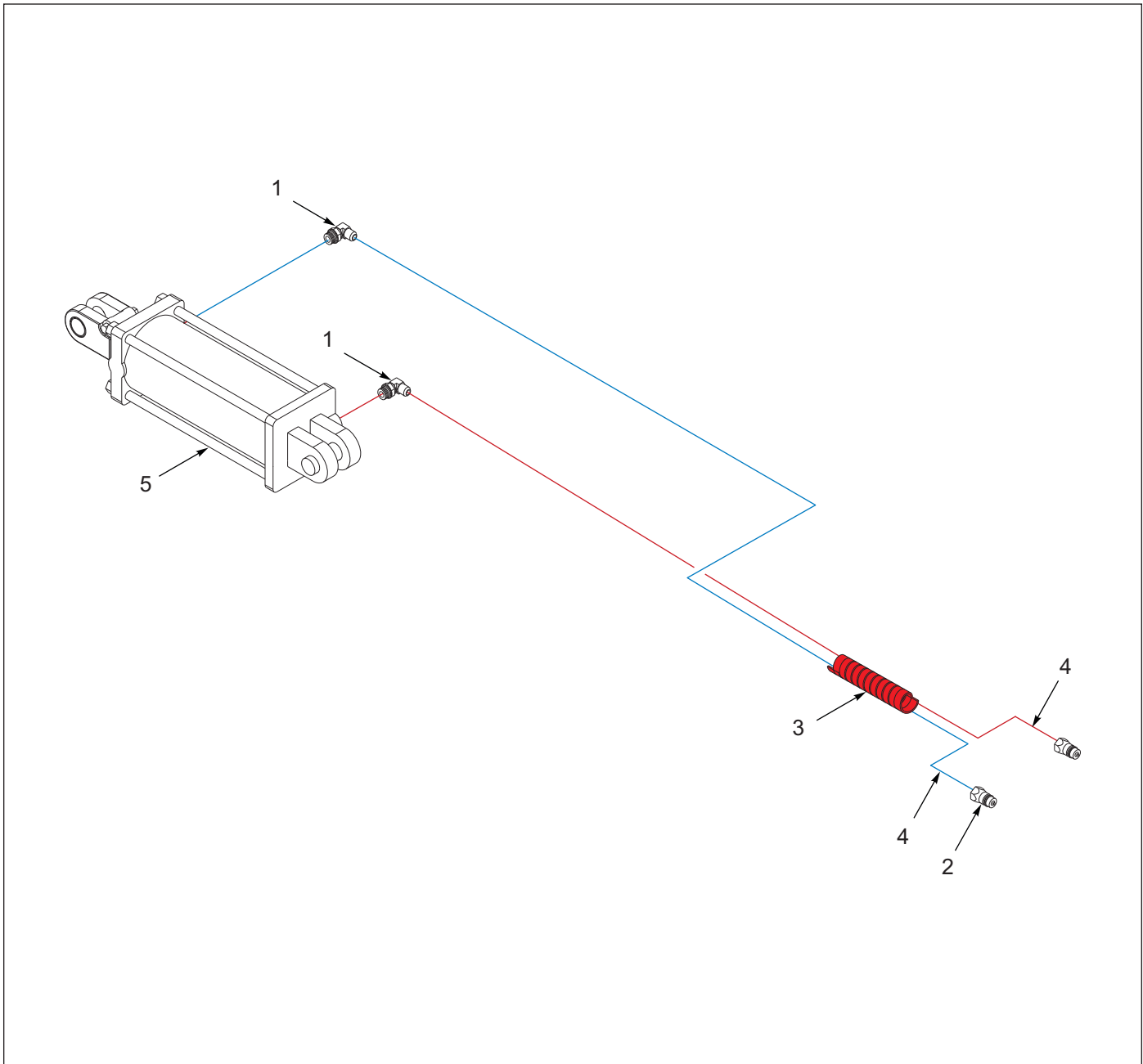
Figure 4-5: Caddy Top Link Circuit
