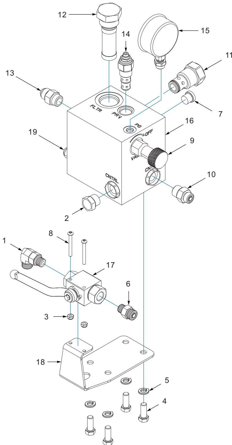
Figure 4-2: Manifold-Draft Assembly
