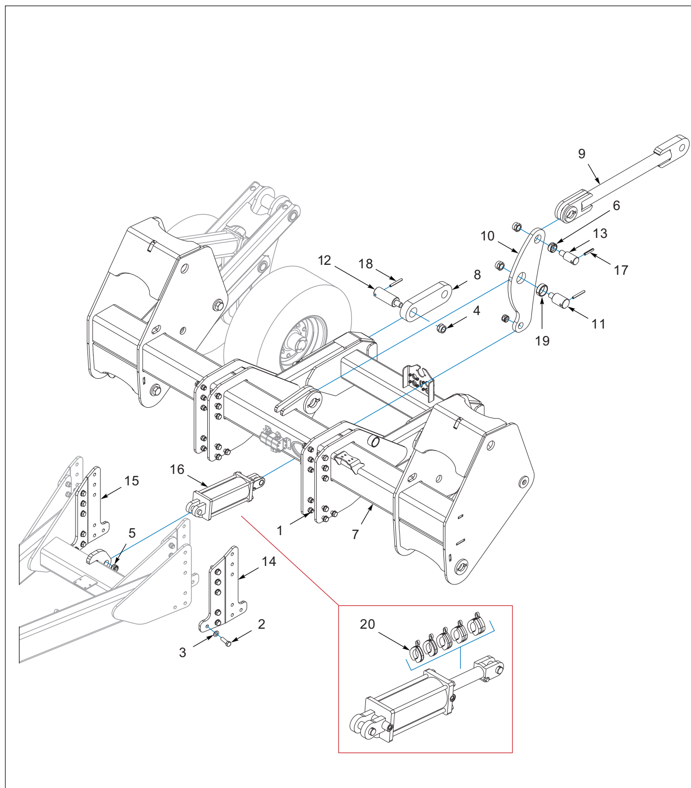
Figure 3-1: Standard Caddy Bottom and Top Link Assembly
