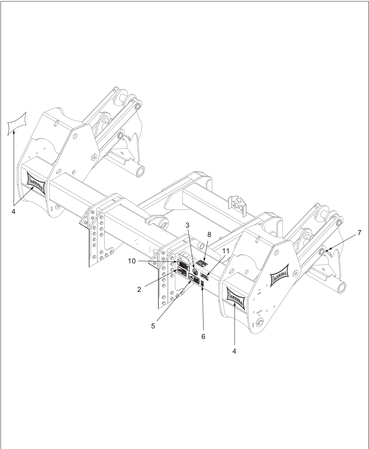
Figure 5-2: Decal Placement - Caddy (1 of 2)
