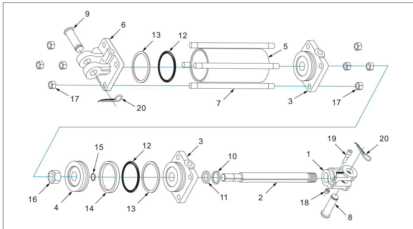
Figure 4-8: Lift Cylinder, 4-1/2 x 20 (Before 03/2021)
