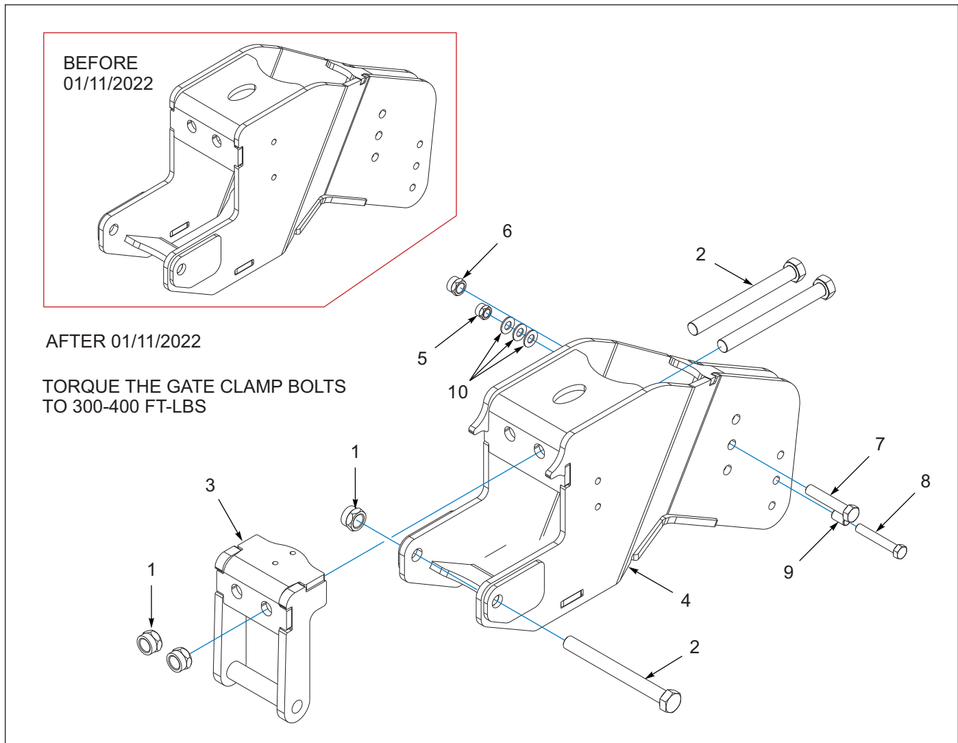
Figure 1-17: RSB Shank Clamp Assembly (Rigid Shear Bolt)
