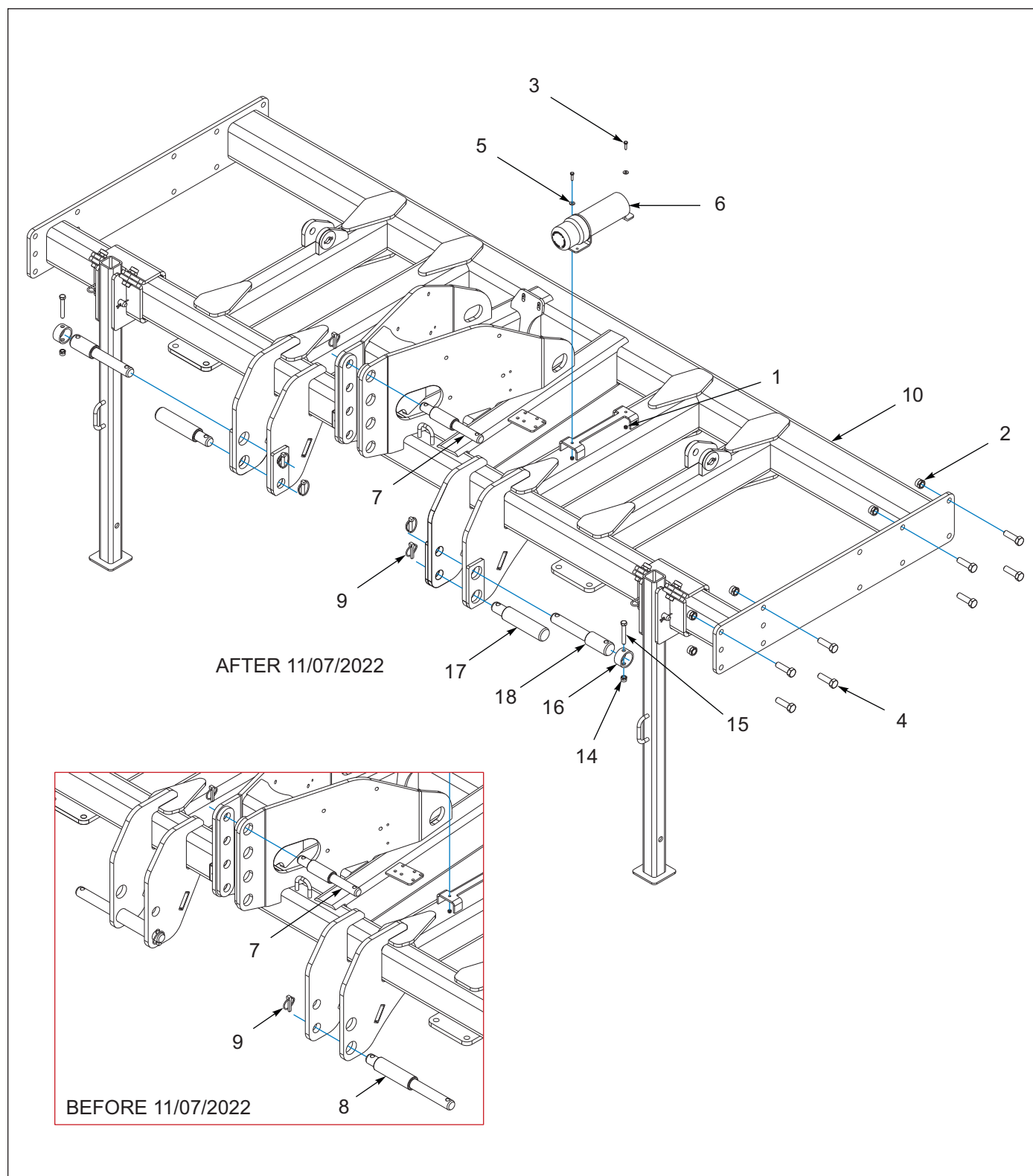
Figure 1-1: Rigid Frame (1 of 2)
