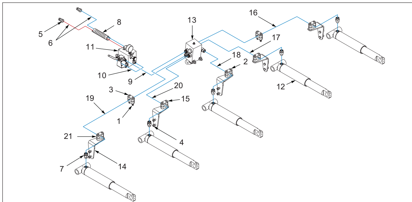
Figure 4-5: 2512 Hydraulics, 5 Shank
