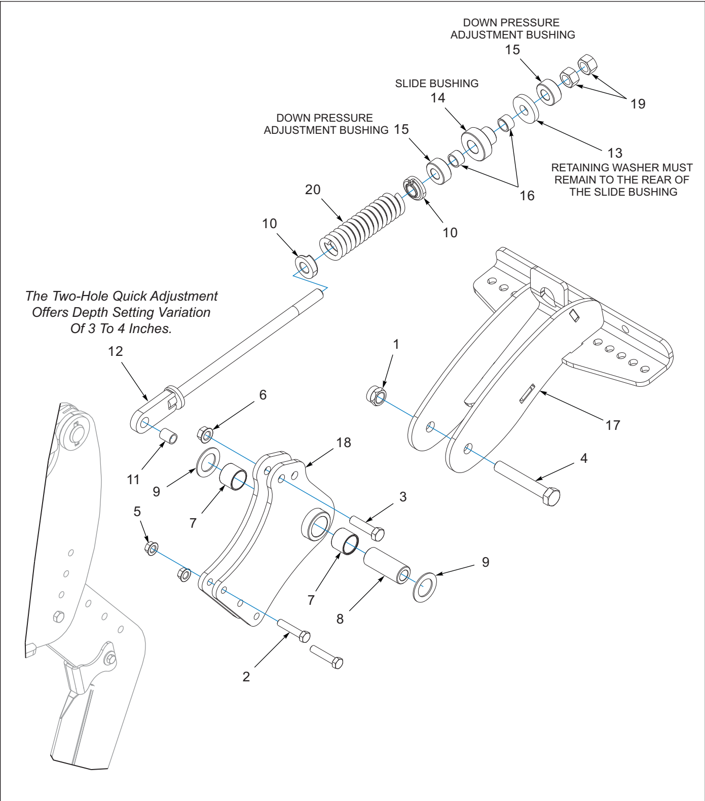
Figure 7-1: Closing Platform (AFTER 04/2024) (1 of 2)
