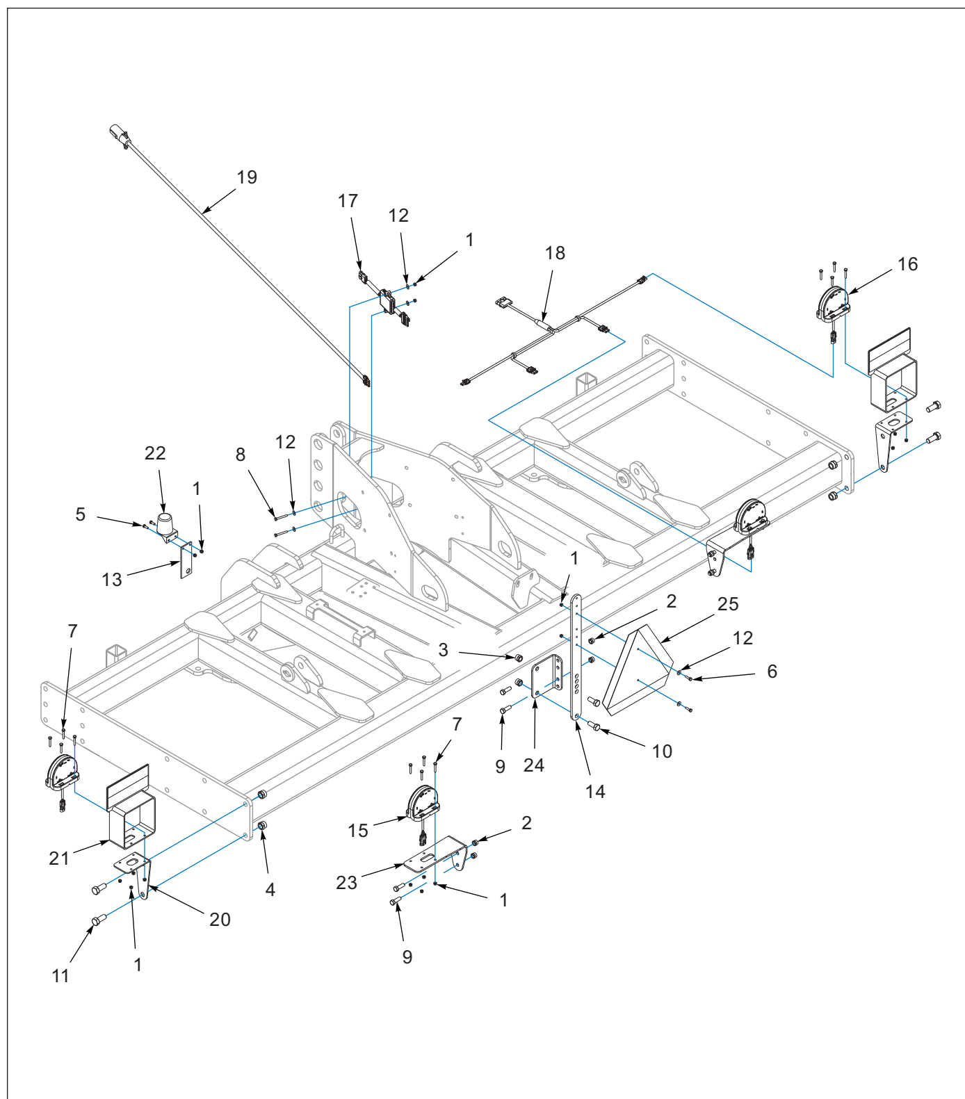
Figure 3-1: Lighting and Reflectors (Rigid 4 Shank)
