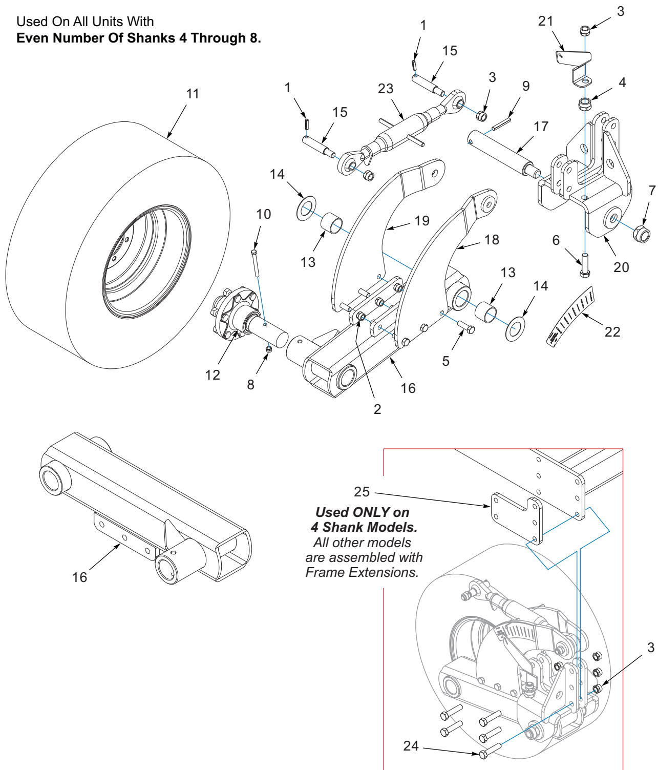
Figure 1-23: Gauge Wheel Assembly - Vertical Mount (Left and Right)
