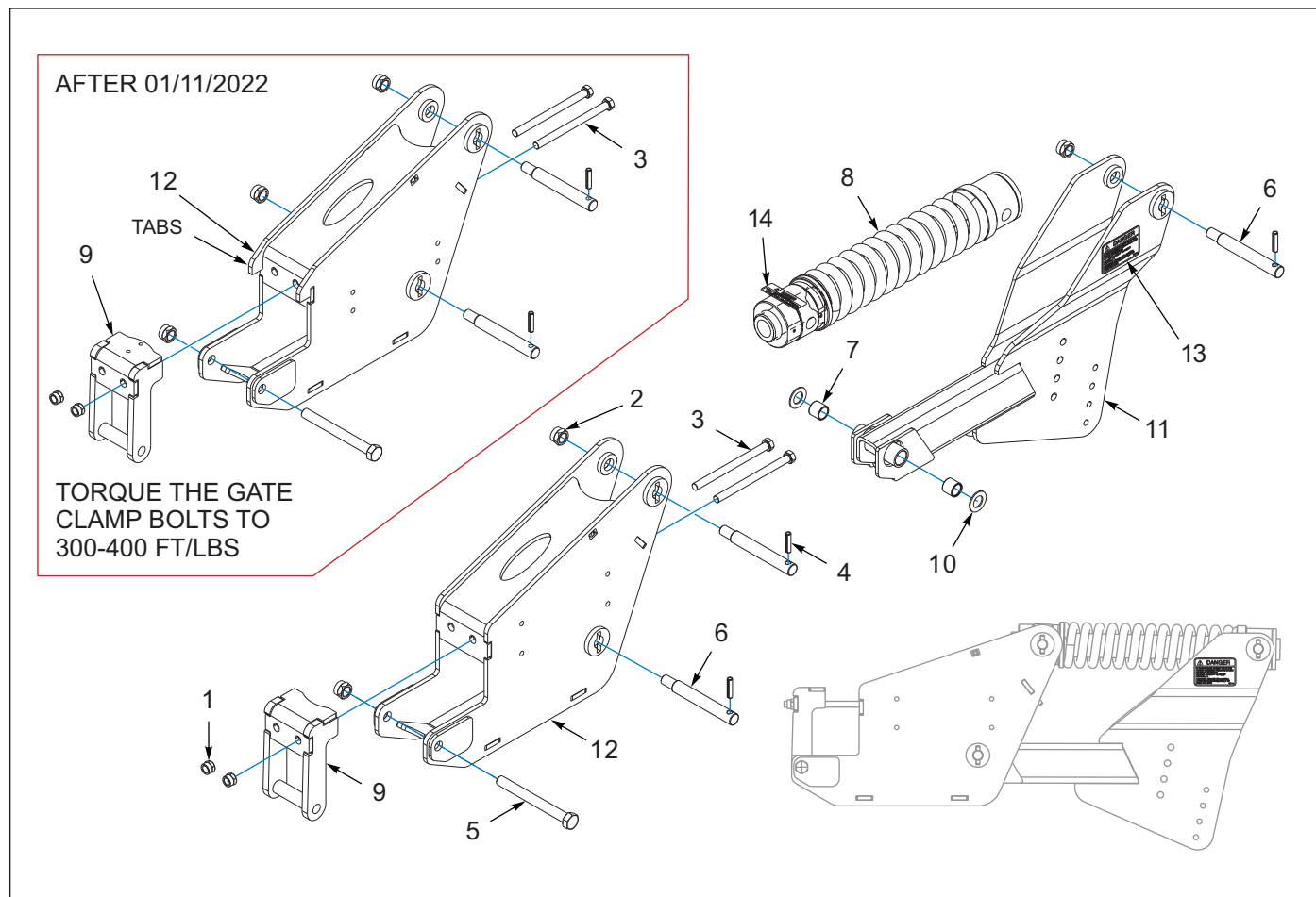
Figure 1-10: 2512 Auto Reset Shank Clamp, Spring - Setback (BEFORE 01/16/2023)
