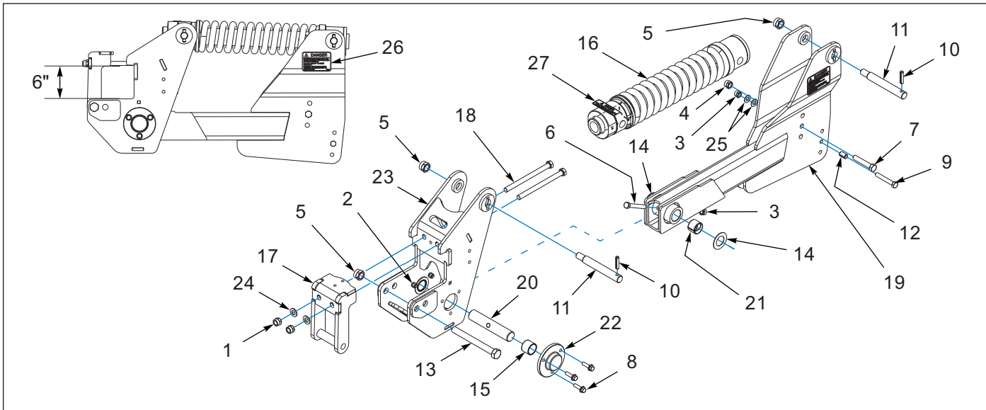
Figure 1-5: Auto Reset Shank Clamp, Spring (AFT. 01/01/2024)
