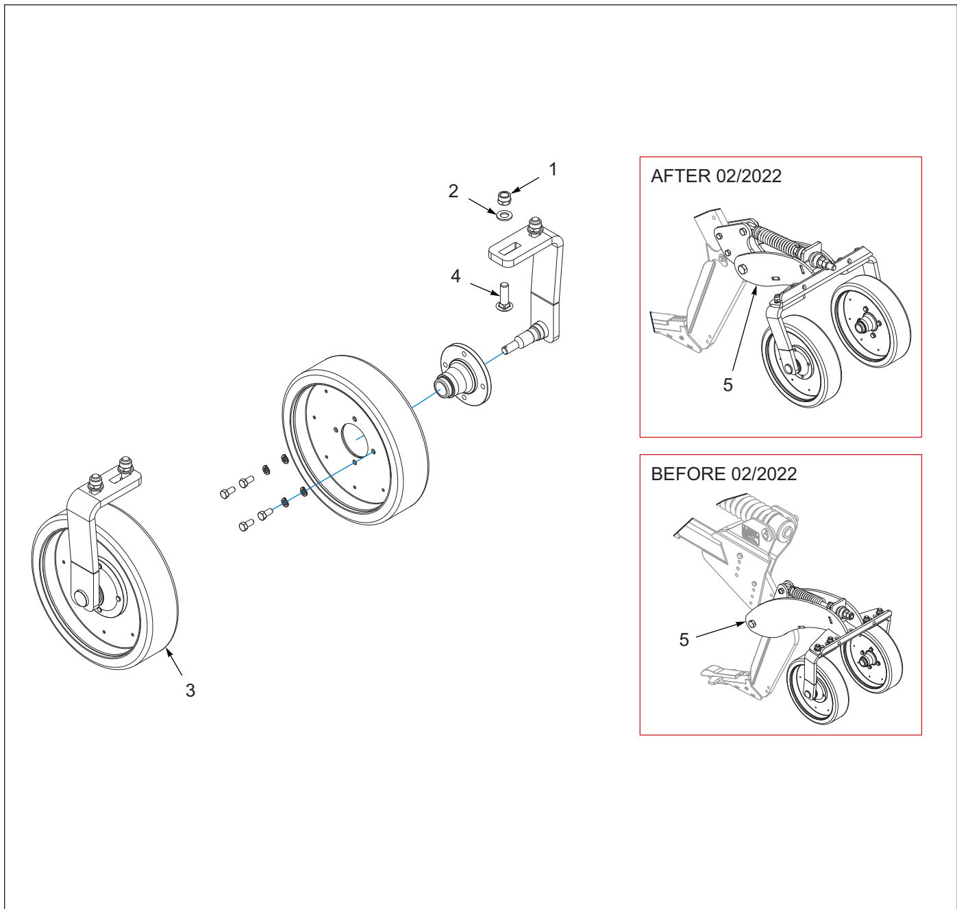
Figure 7-7: Closer Wheel
