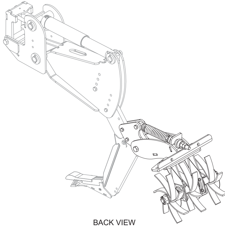
Figure 7-4: Closing Platform (02/2022 TO 04/2024) (2 of 2)
