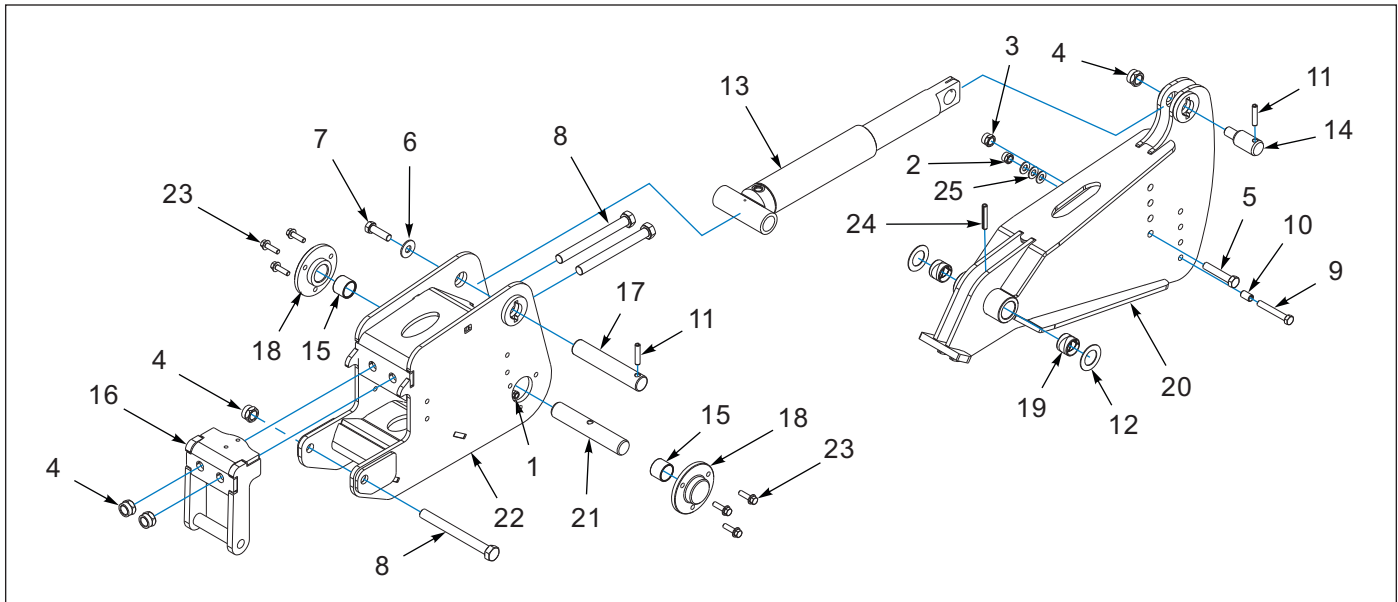
Figure 1-12: Auto Reset Shank Clamp, Hydraulic - Setback (AFT. 12/12/2023)
