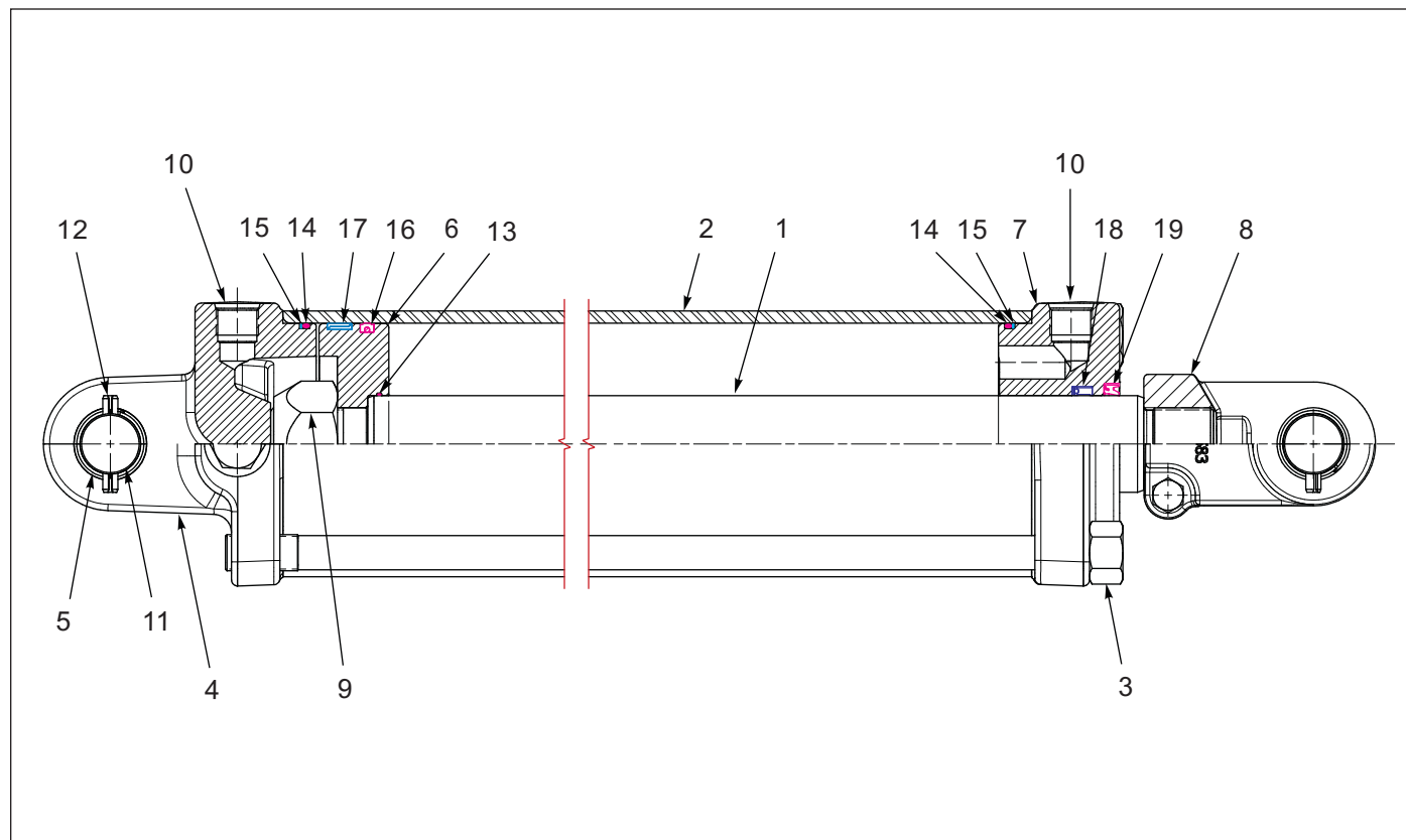
Figure 4-20: Hydraulic Cylinder, 5 x 30 - 233870
