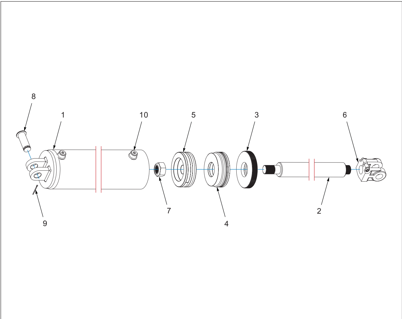
Figure 4-21: Hydraulic Cylinder, 6 x 30 - 233833
