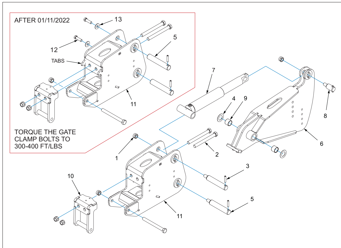
Figure 1-16: Auto Reset Shank Clamp, Hydraulic - Setback (BEF. 12/12/2023)
