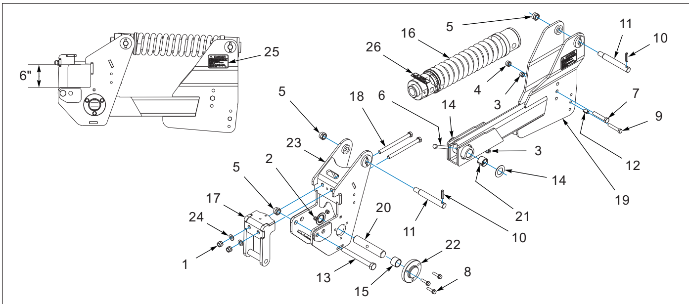
Figure 1-7: Auto Reset Shank Clamp, Spring (01/16/2023 TO 01/01/2024)
