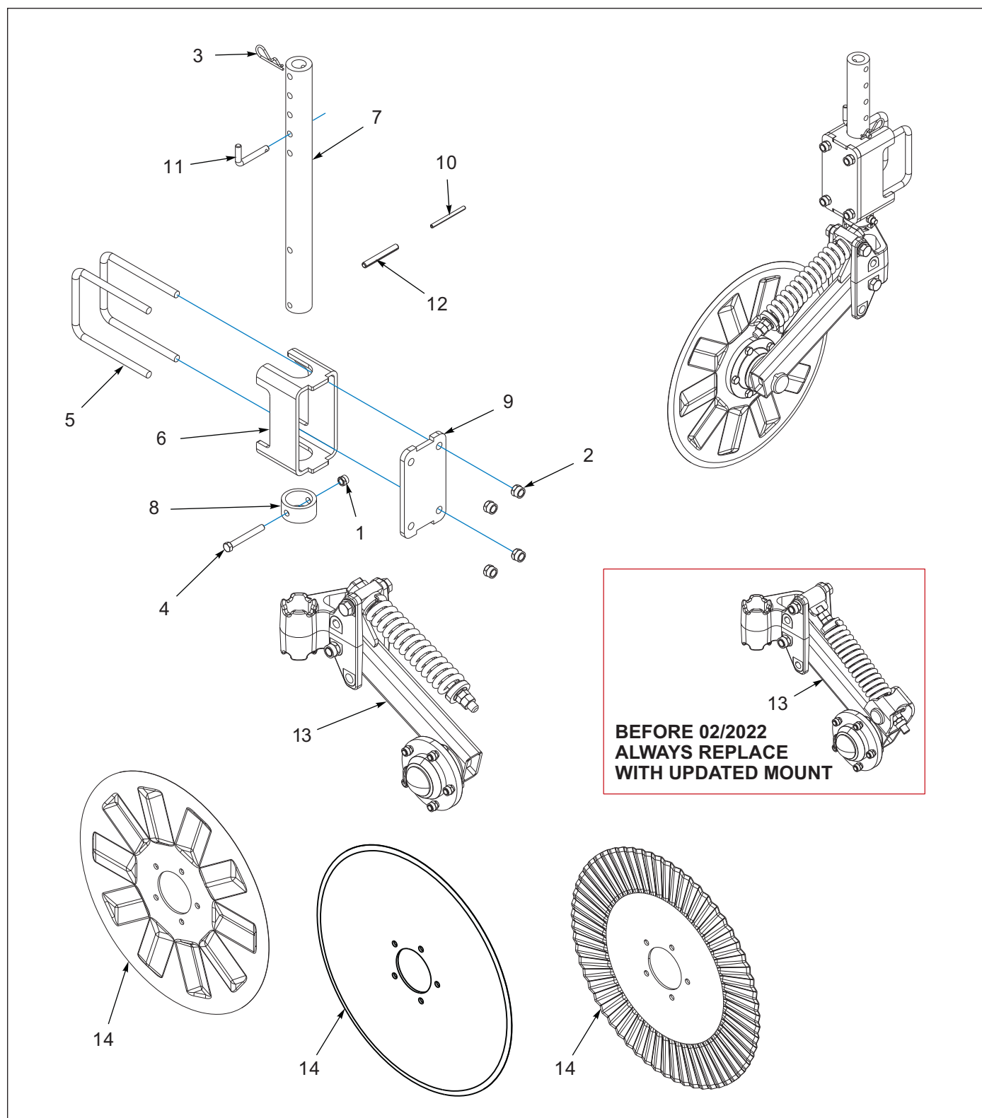
Figure 2-1: Blade Coulter - Straight, Rippled & Pyramid Option (Left Hand)
