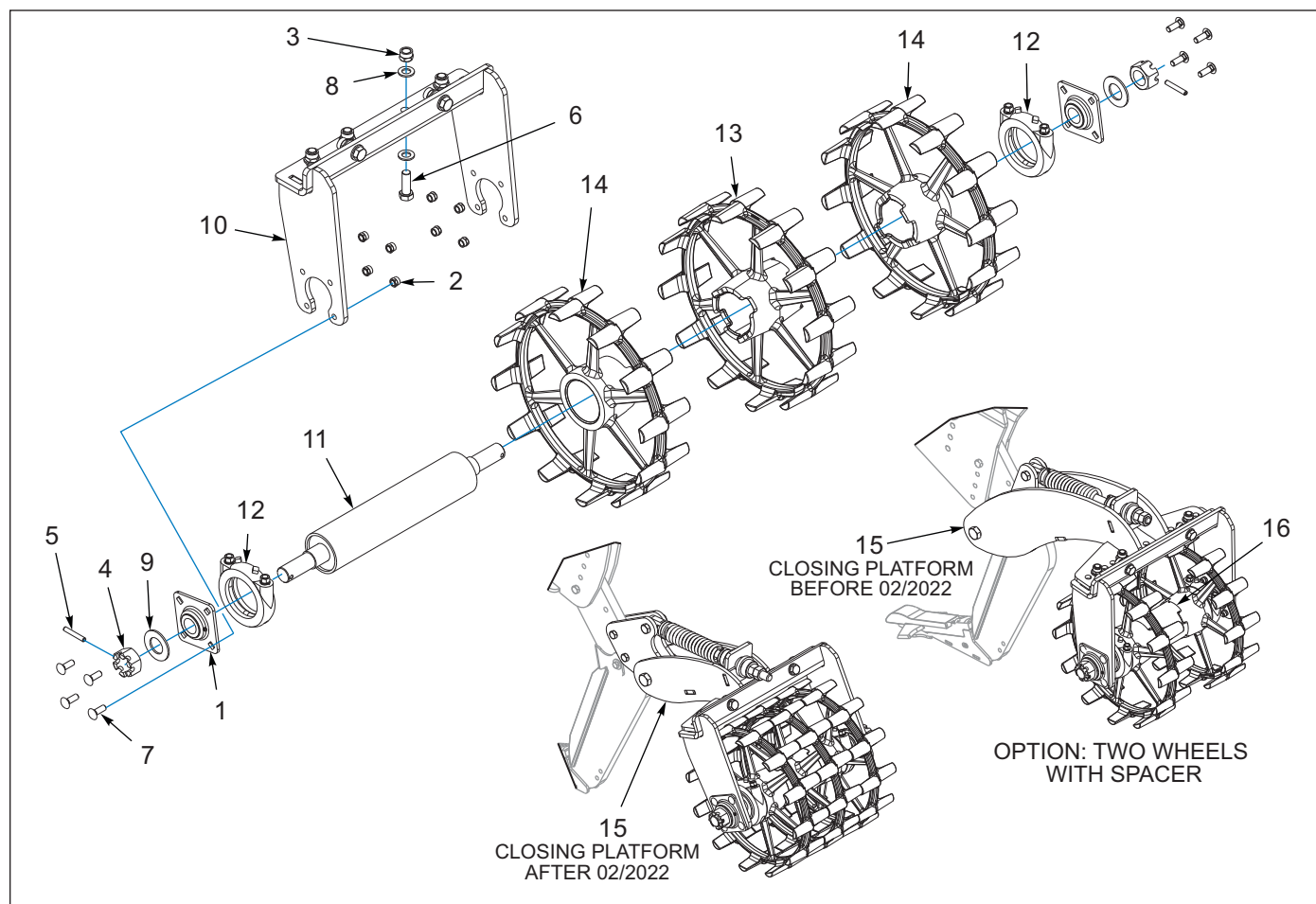
Figure 7-10: Crumbler Reel
