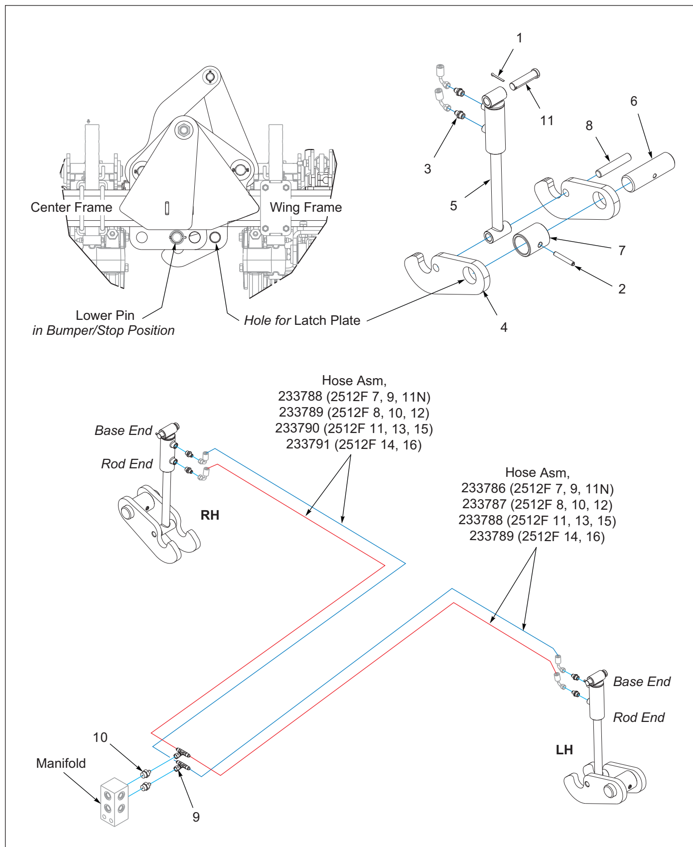
Figure 4-16: Wing Lock Kit - Optional
