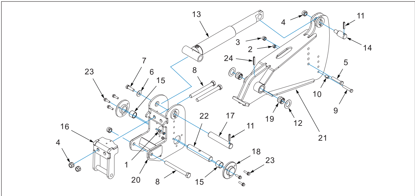
Figure 1-13: Auto Reset Shank Clamp, Hydraulic (12/12/23 TO 02/07/25)
