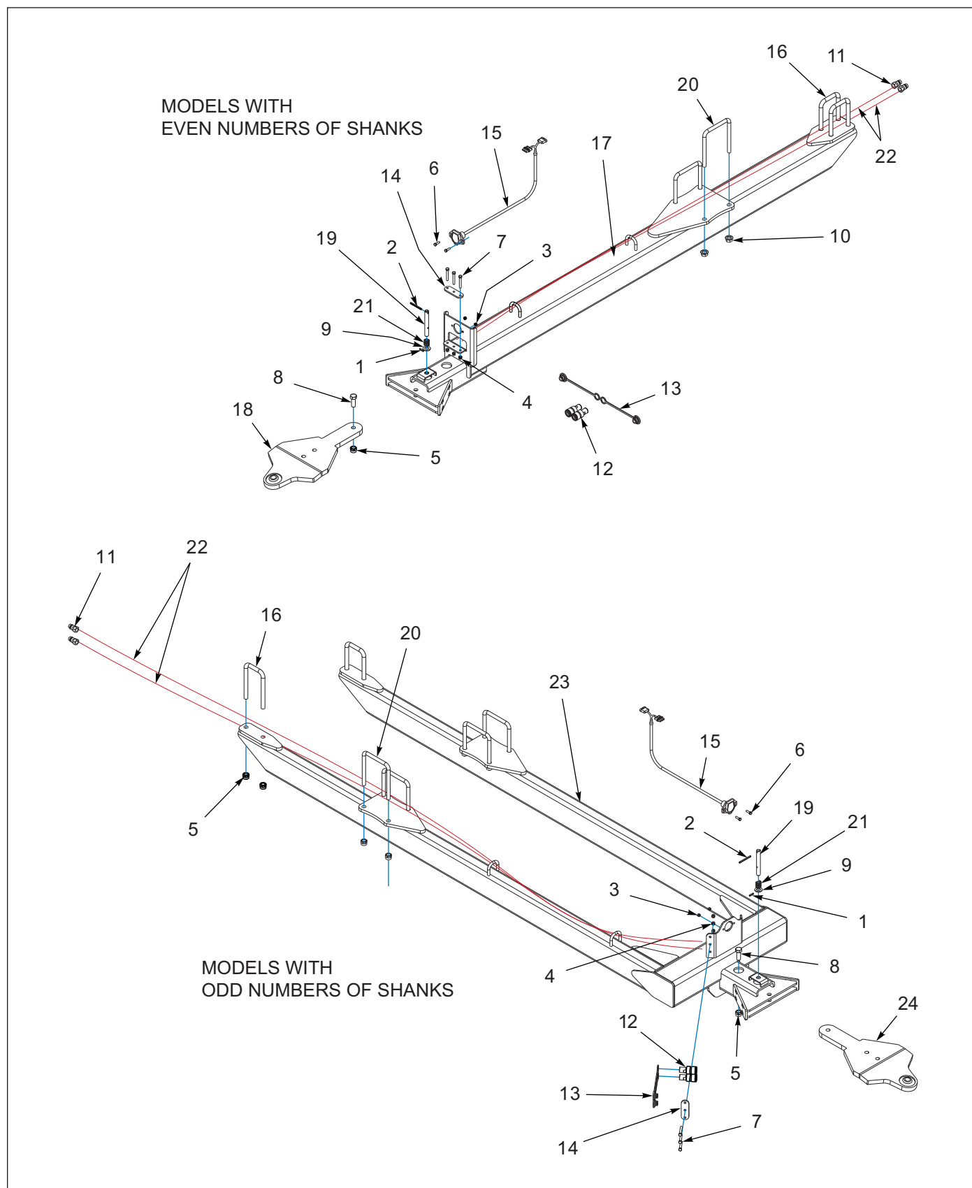
Figure 1-25: Rear Tow Bar Hitch - Optional
