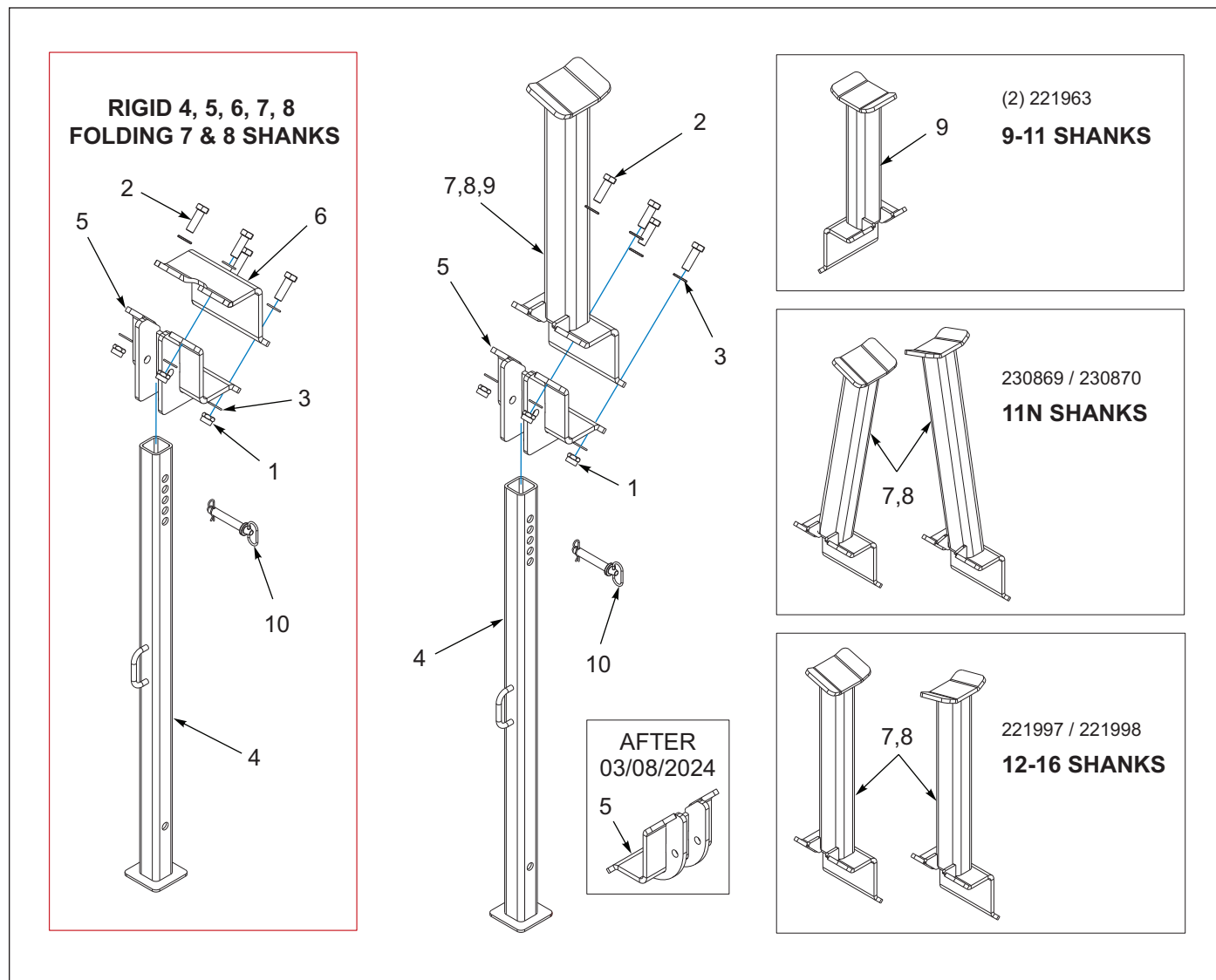
Figure 1-18: 2512 Jack Stand and Wing Rest (AFTER 06/07/2023)
