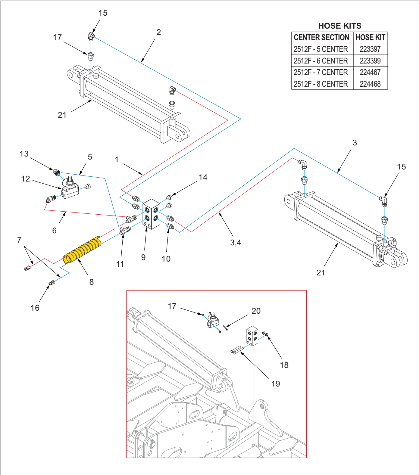
Figure 4-1: Folding Frame Hydraulic Diagram (AFTER 11/01/2021)
