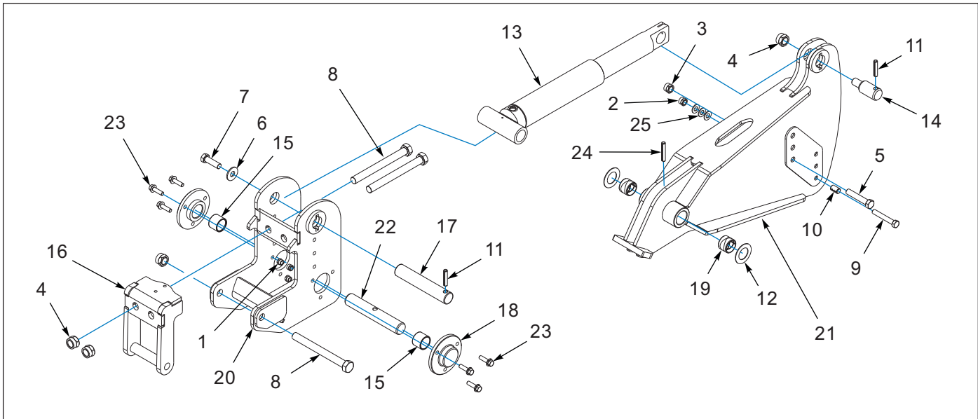
Figure 1-11: Auto Reset Shank Clamp, Hydraulic (AFT. 02/07/2025)
