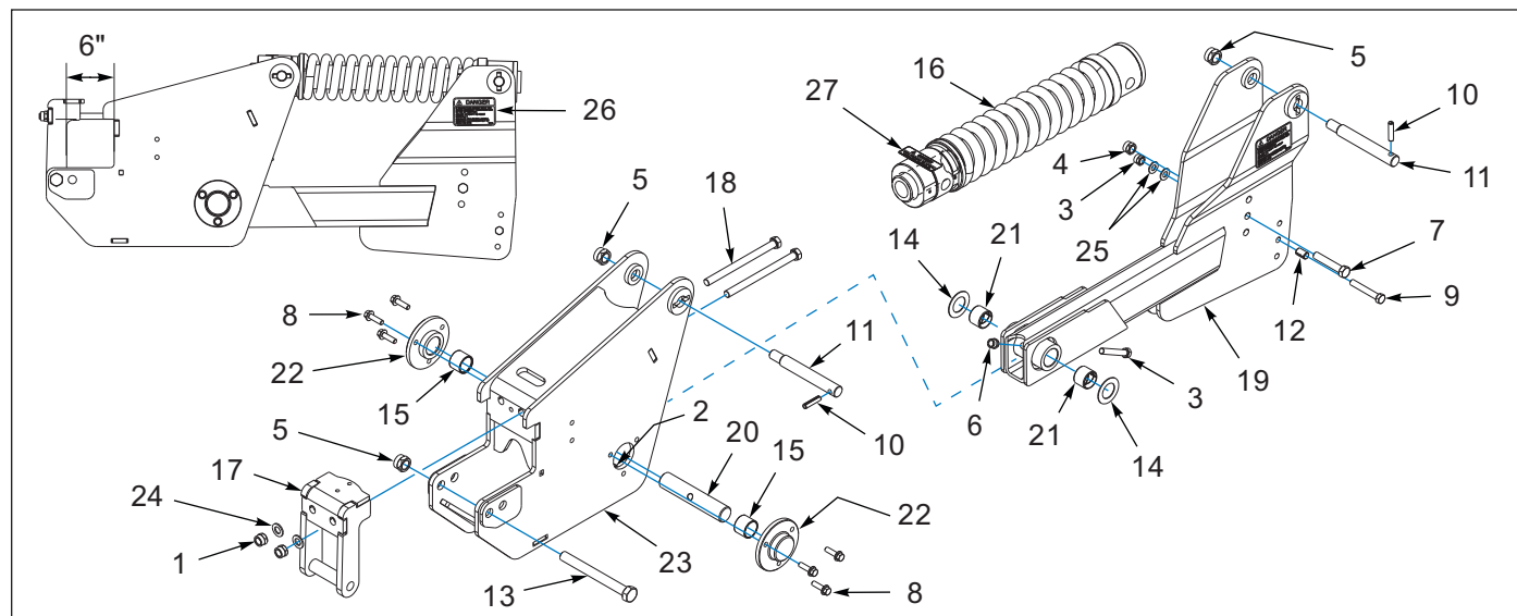
Figure 1-6: 2512 Auto Reset Shank Clamp, Spring - Setback (AFTER 01/01/2024)
