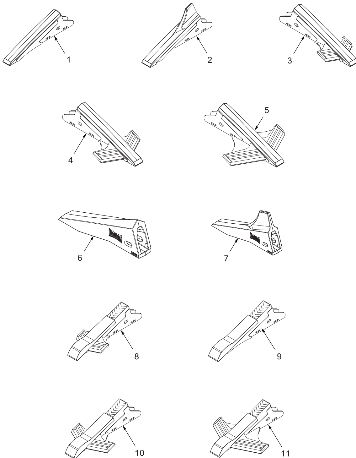
Figure 6-1: Points for 1-1/4 Shank
