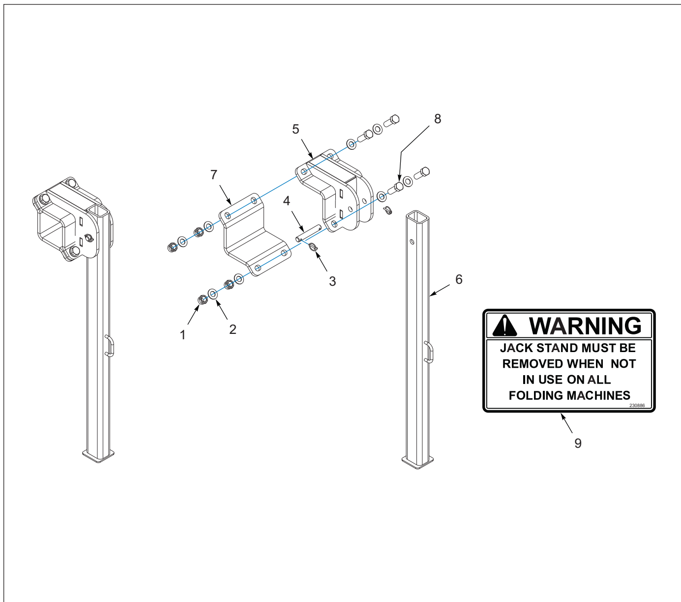
Figure 1-21: Jack Stand, Rear - Optional
