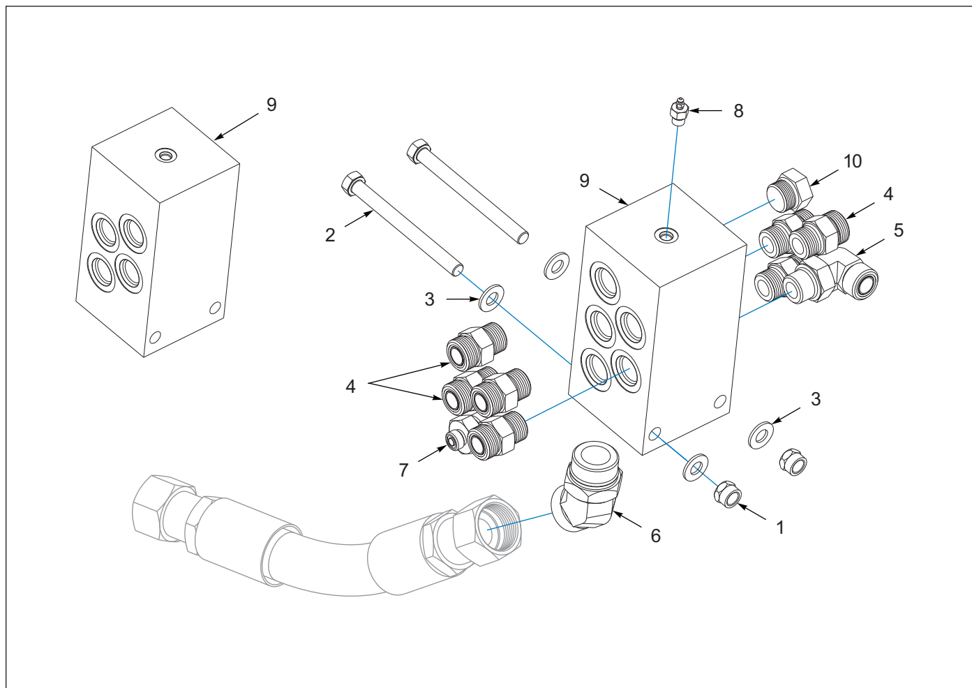
Figure 4-15: Manifold-Shank Cylinder Assembly
