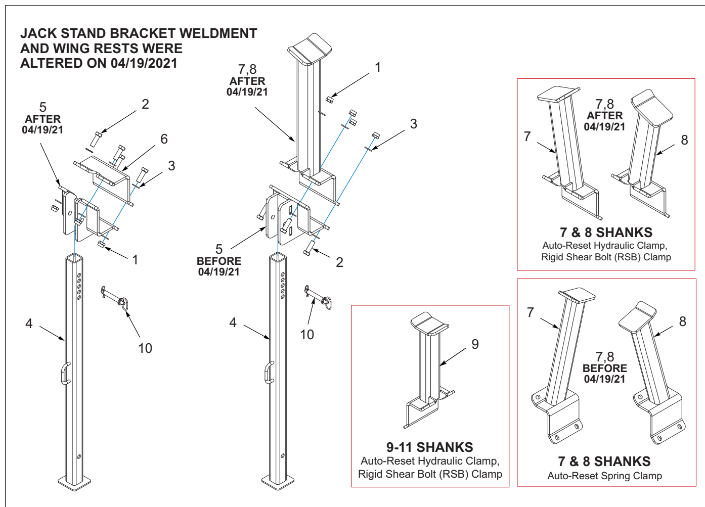
Figure 1-20: 2512 Jack Stand and Wing Rest (BEFORE 11/01/2021)
