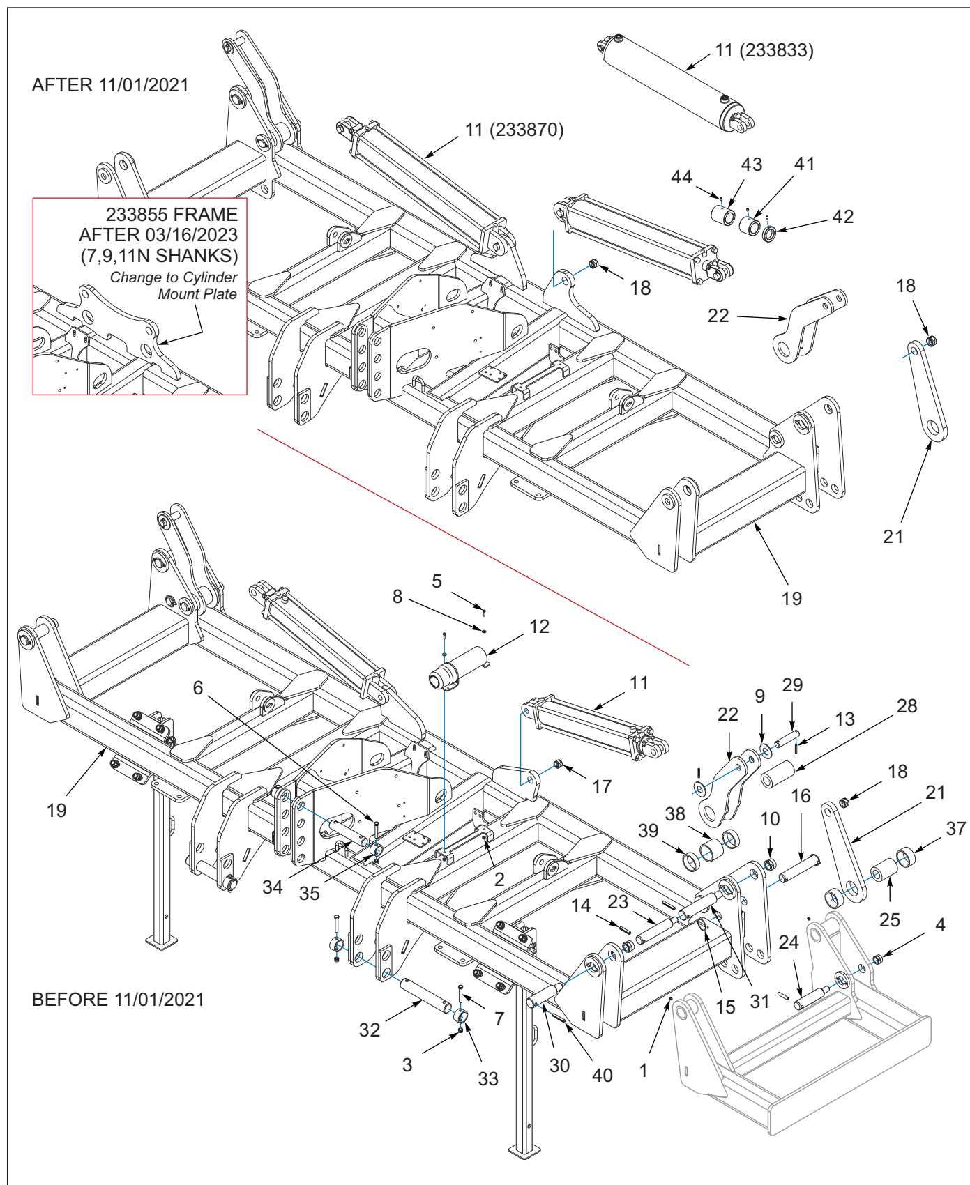
Figure 1-3: 2512 Folding Frame (1 of 2)
