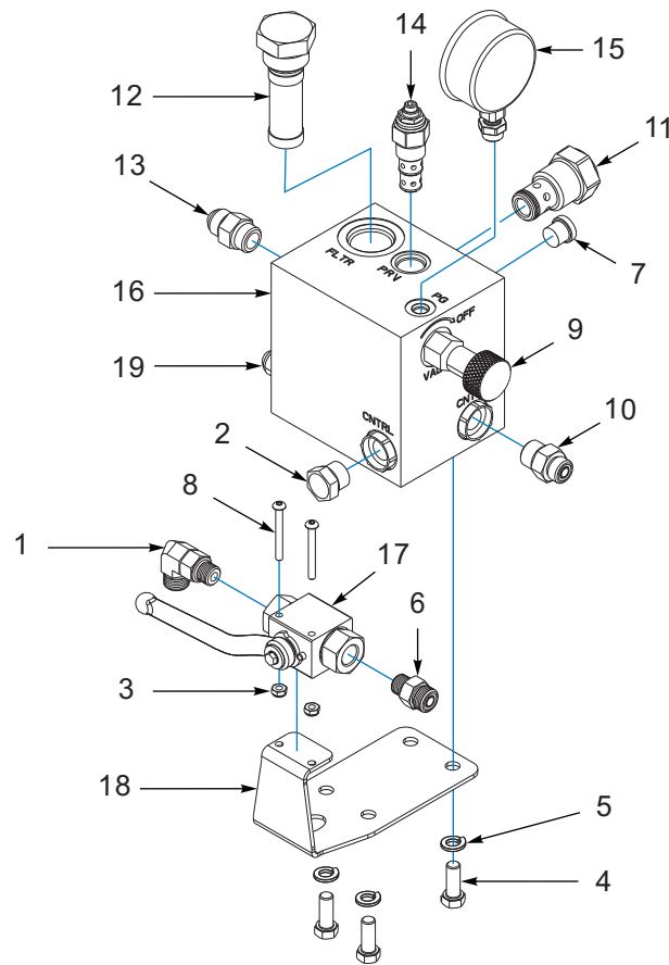
Figure 4-14: Manifold-Draft Assembly
