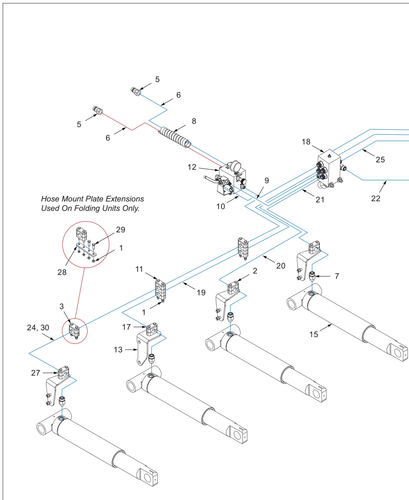
Figure 4-10: 2512 Hydraulics, 8 Shank (Rigid and Folding) (1 of 2)
