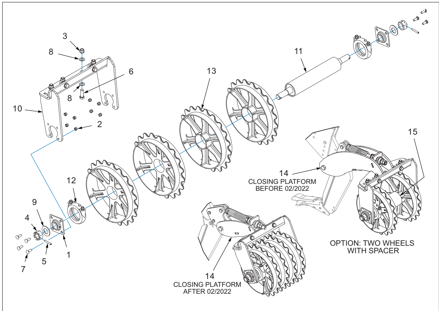
Figure 7-11: Packer Reel
