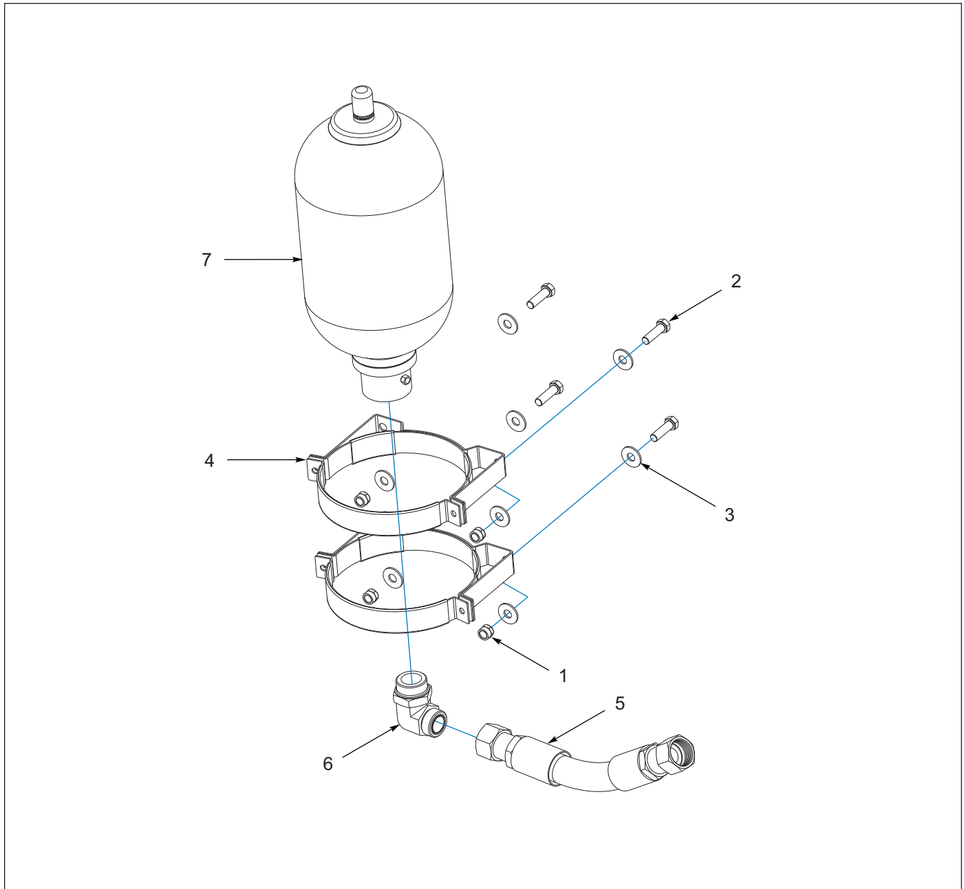
Figure 4-3: 2512 Accumulator Bladder
