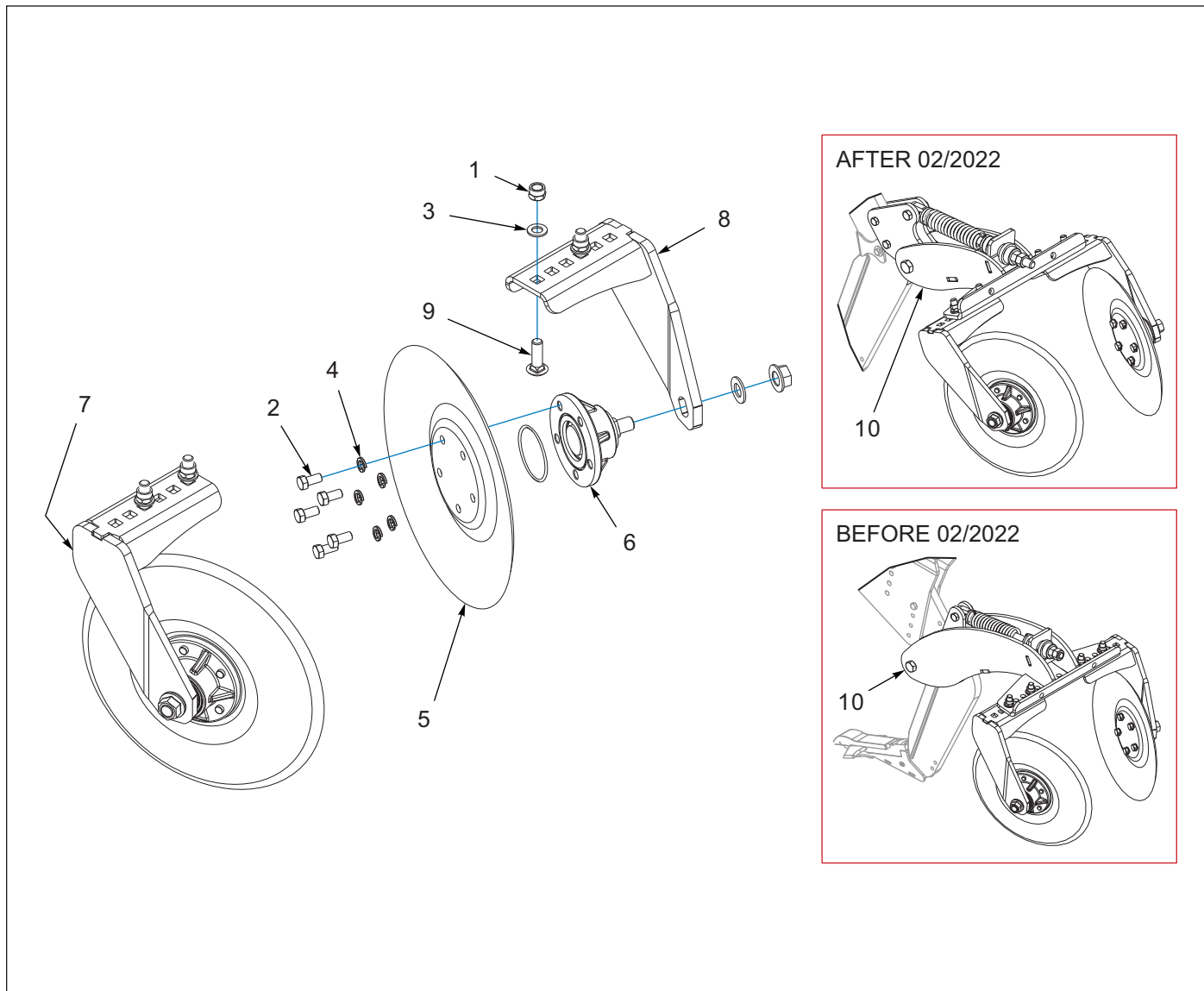
Figure 7-9: Closer Disc
