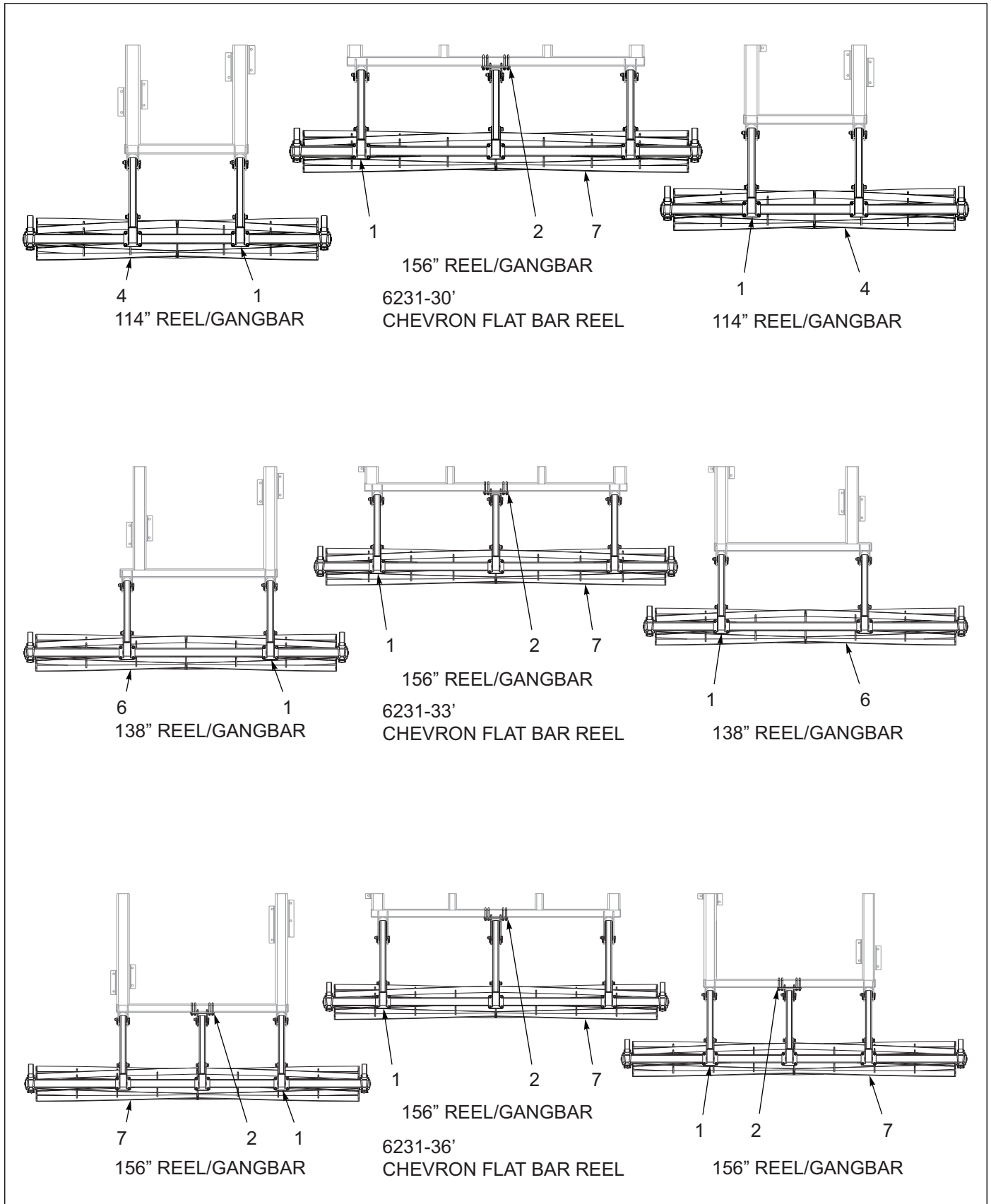
Figure 8-21: Chevron Flat Bar Reel Assembly 6231-30-33-36
