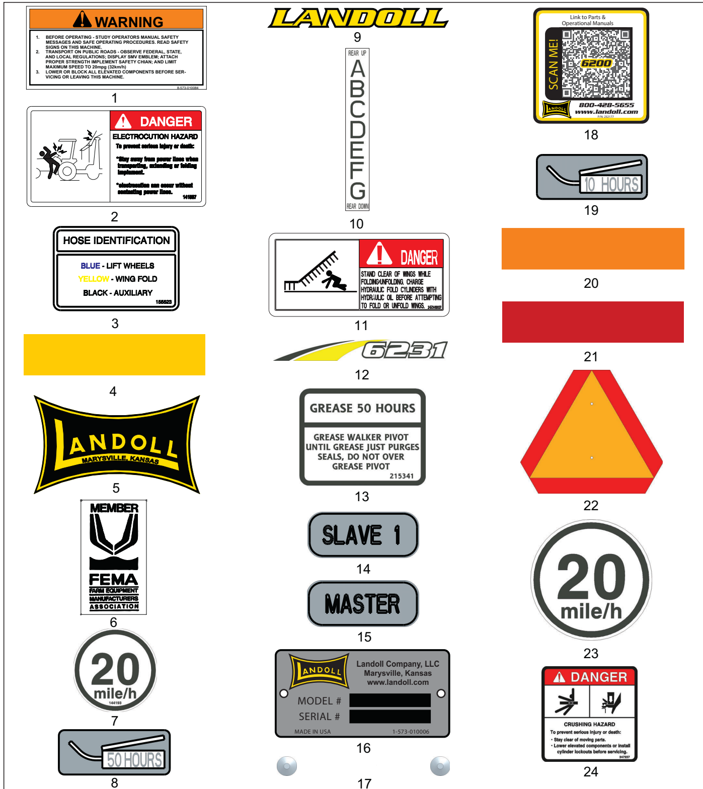
Figure 7-1: Decals (1 of 2)
