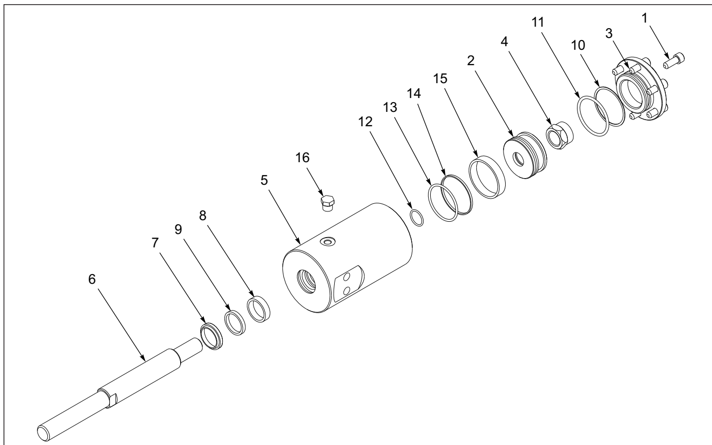
Figure 5-9: Cylinder Assembly 2-1/2 x 2-1/2
