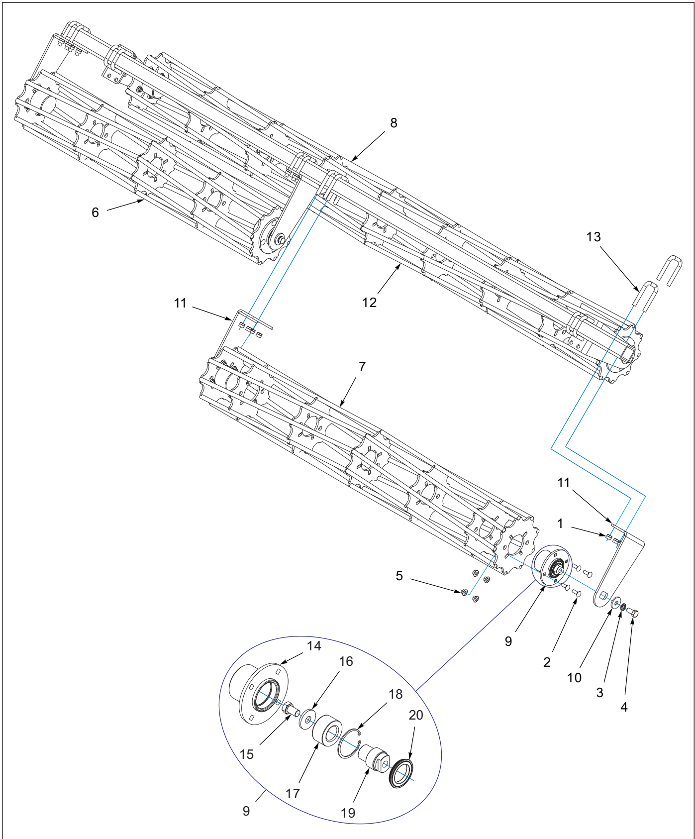
Figure 8-41: Double Reel Assembly Wing 6231-33
