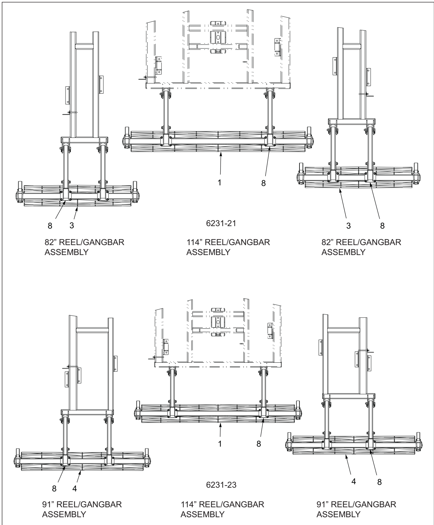
Figure 8-8: Conditioner Reel Assembly 6231-21-23
