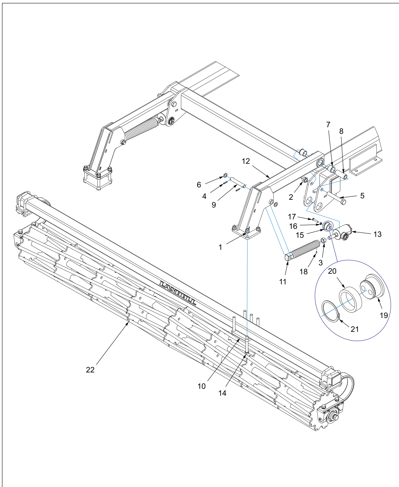
Figure 8-13: Conditioner Reel Assembly Hydraulic
