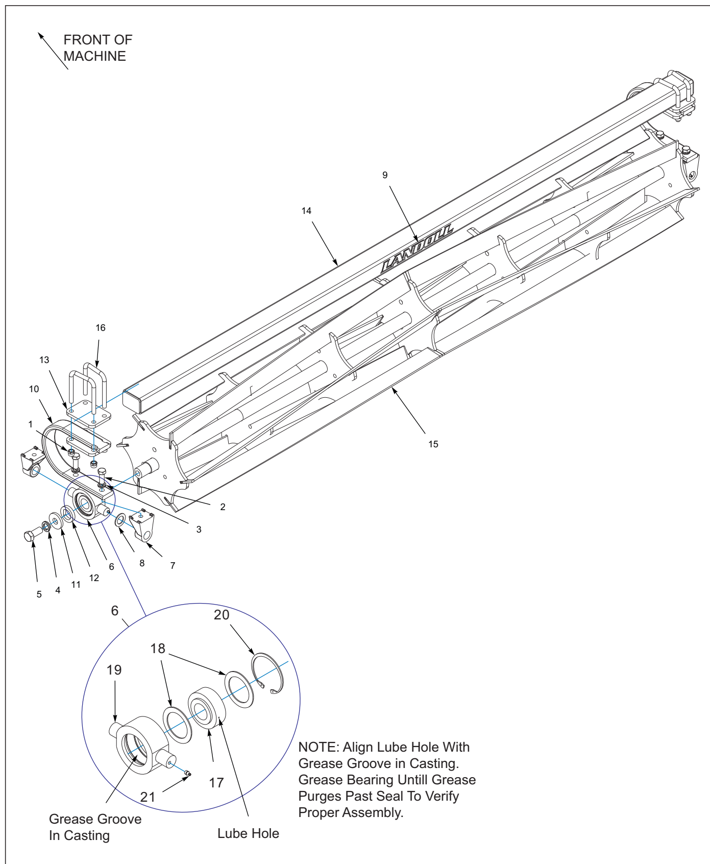
Figure 8-23: Chevron Flat Bar Reel/Gangbar Assembly
