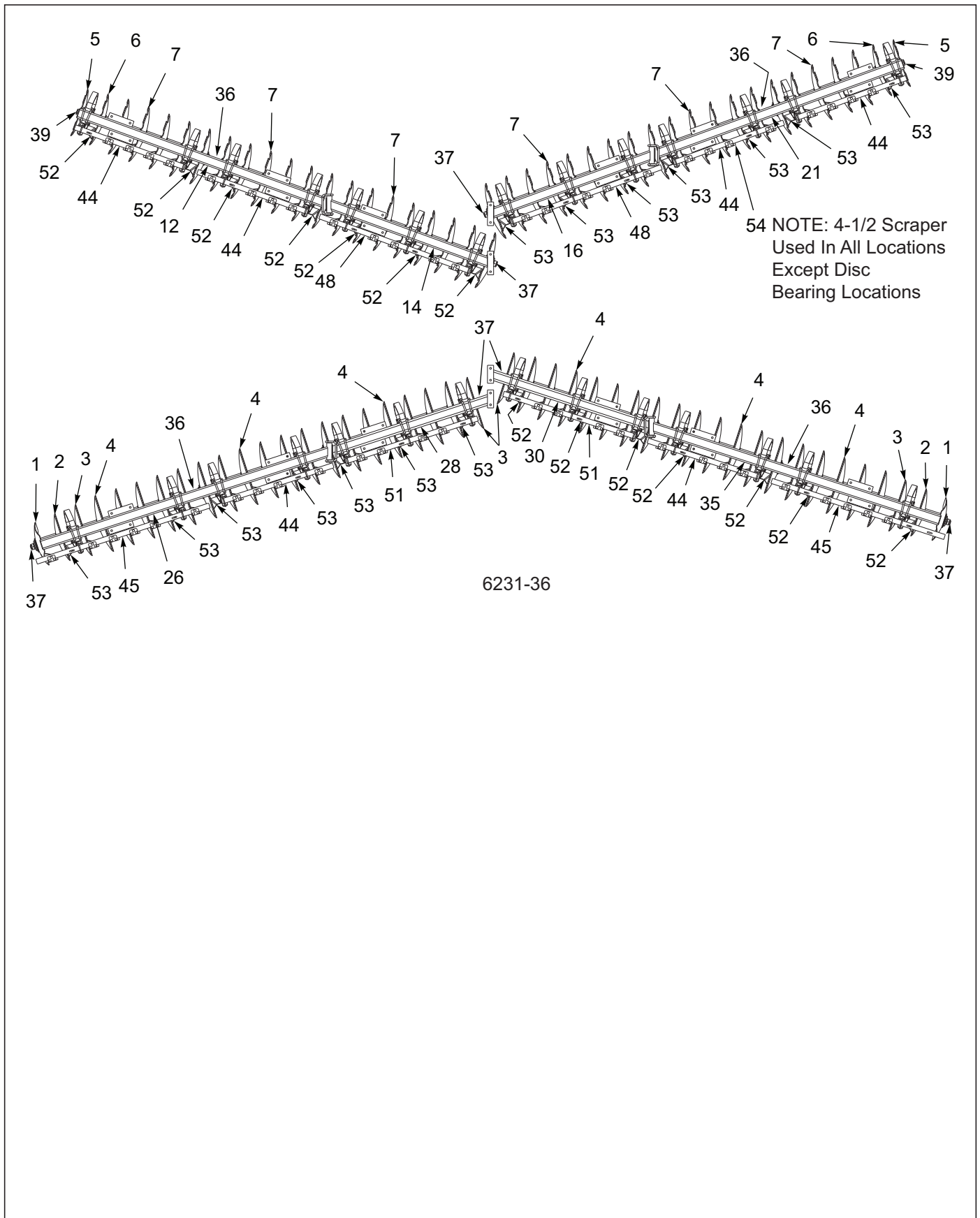
Figure 3-51: Disc Gang Assembly 6231 28" 10-1/2SP NF 5/16" (Notched Front) (4 of 4)
