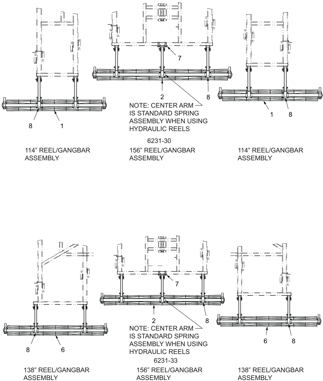
Figure 8-10: Conditioner Reel Assembly 6231-30-33
