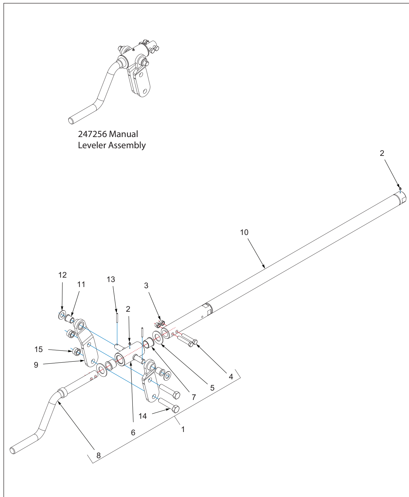
Figure 2-6: Leveler Assembly Manual (After 01-01-2024)
