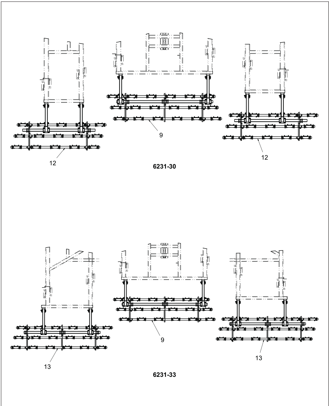
Figure 8-3: 3 Row Coil Tine Harrow Assembly 6231-30-33
