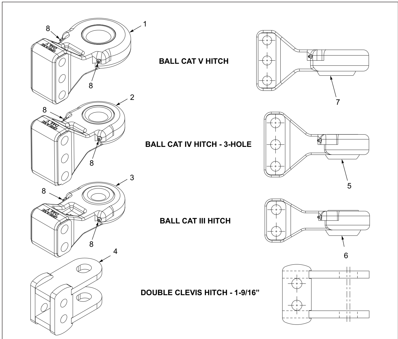
Figure 2-9: Hitch Assemblies
