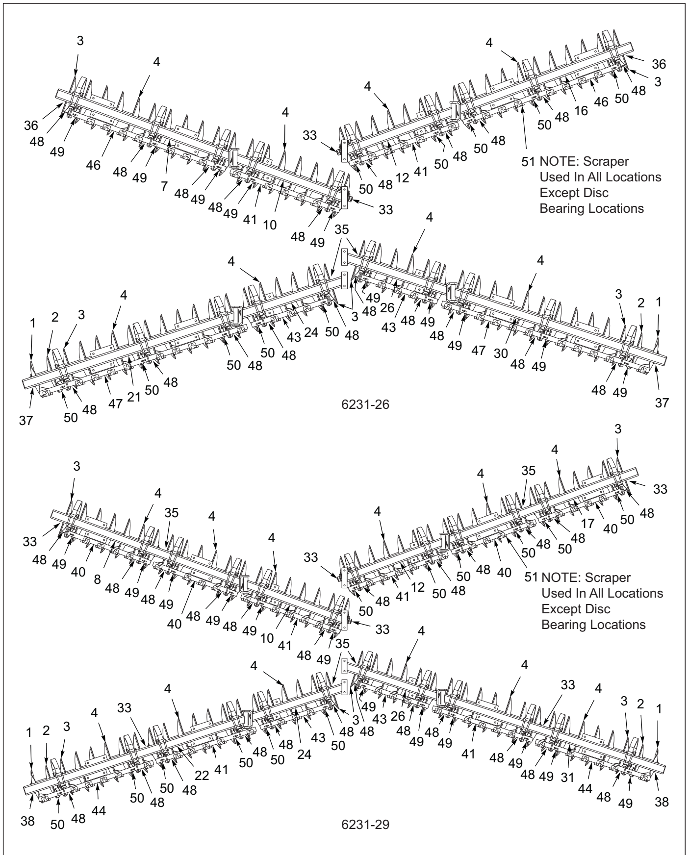
Figure 3-33: Disc Gang Assembly 6231 26" 8-3/4SP HDS 4 GA (Heavy Duty Scraper) (2 of 4)
