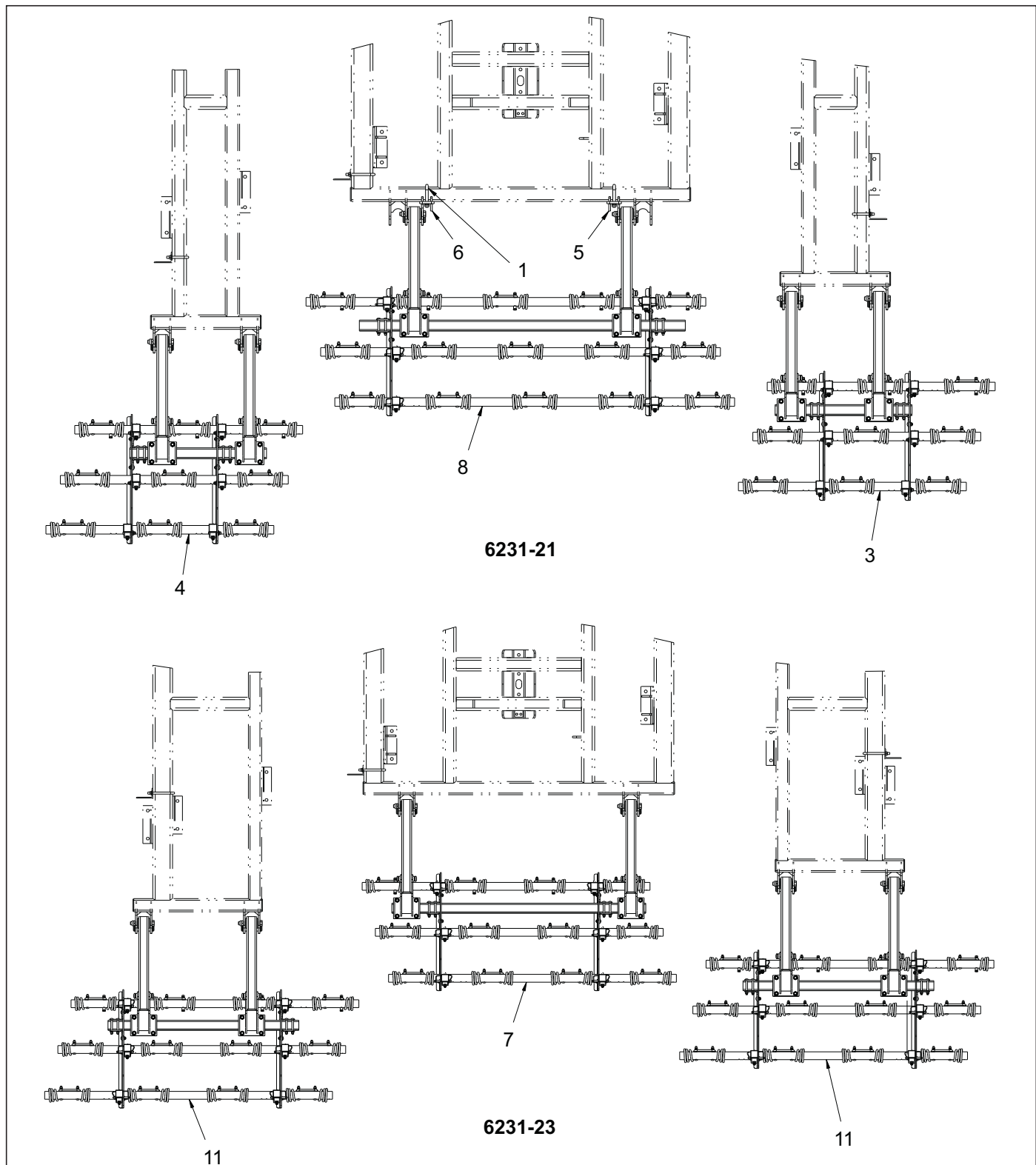
Figure 8-1: 3 Row Coil Tine Harrow Assembly 6231-21-23
