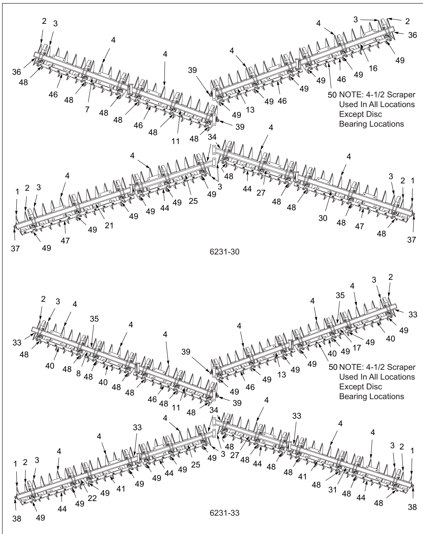
Figure 3-39: Disc Gang Assembly 6231 26" 8-3/4SP 5/16" (3 of 4)
