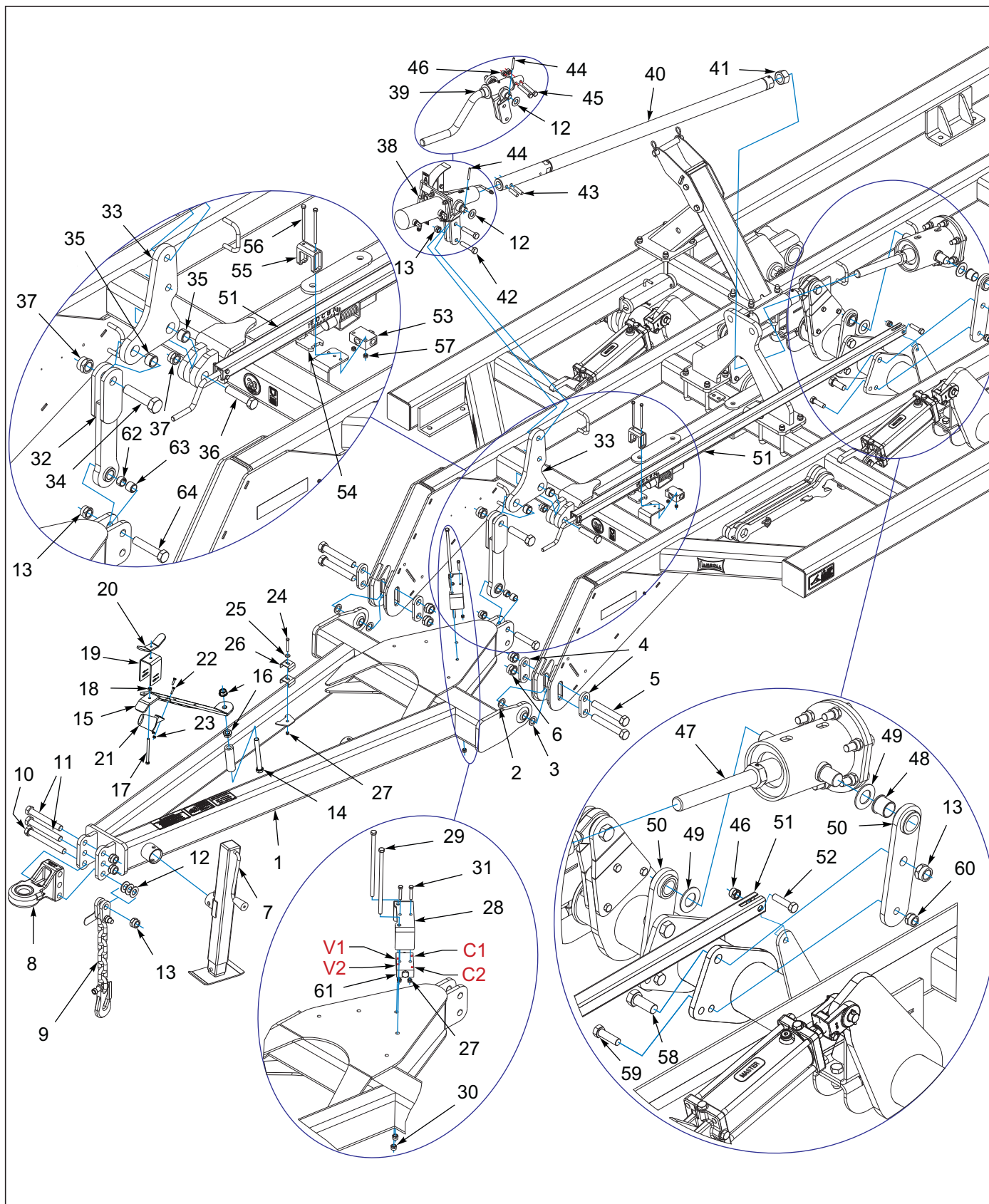
Figure 2-2: Hitch/Leveler Assembly (After 01-01-2021)
