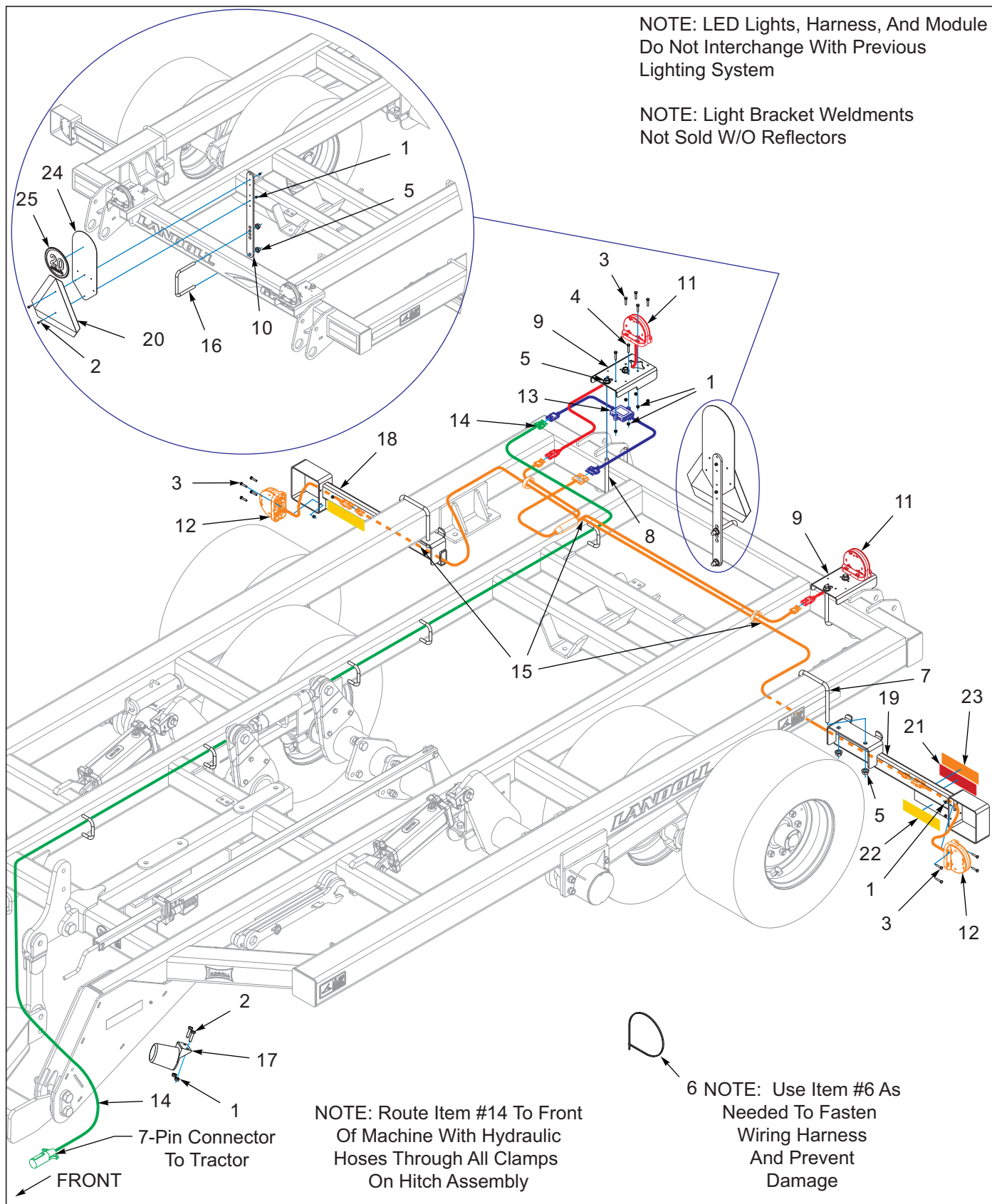
Figure 6-2: Electrical Assembly W/LED Lights (2 of 2)
