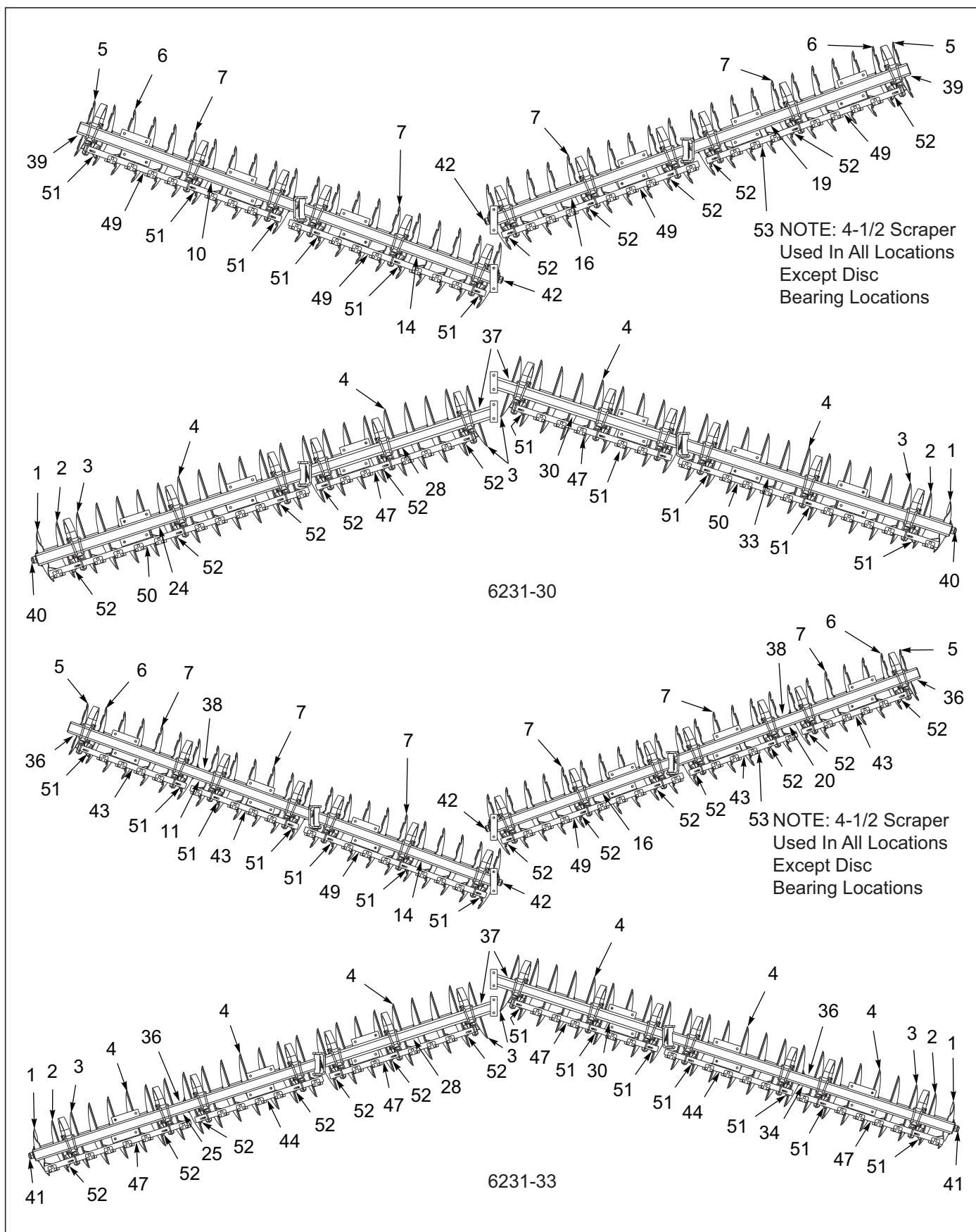
Figure 3-44: Disc Gang Assembly 6231 28' 8-3/4SP NF 5/16' (Notched Front) (3 of 4)
