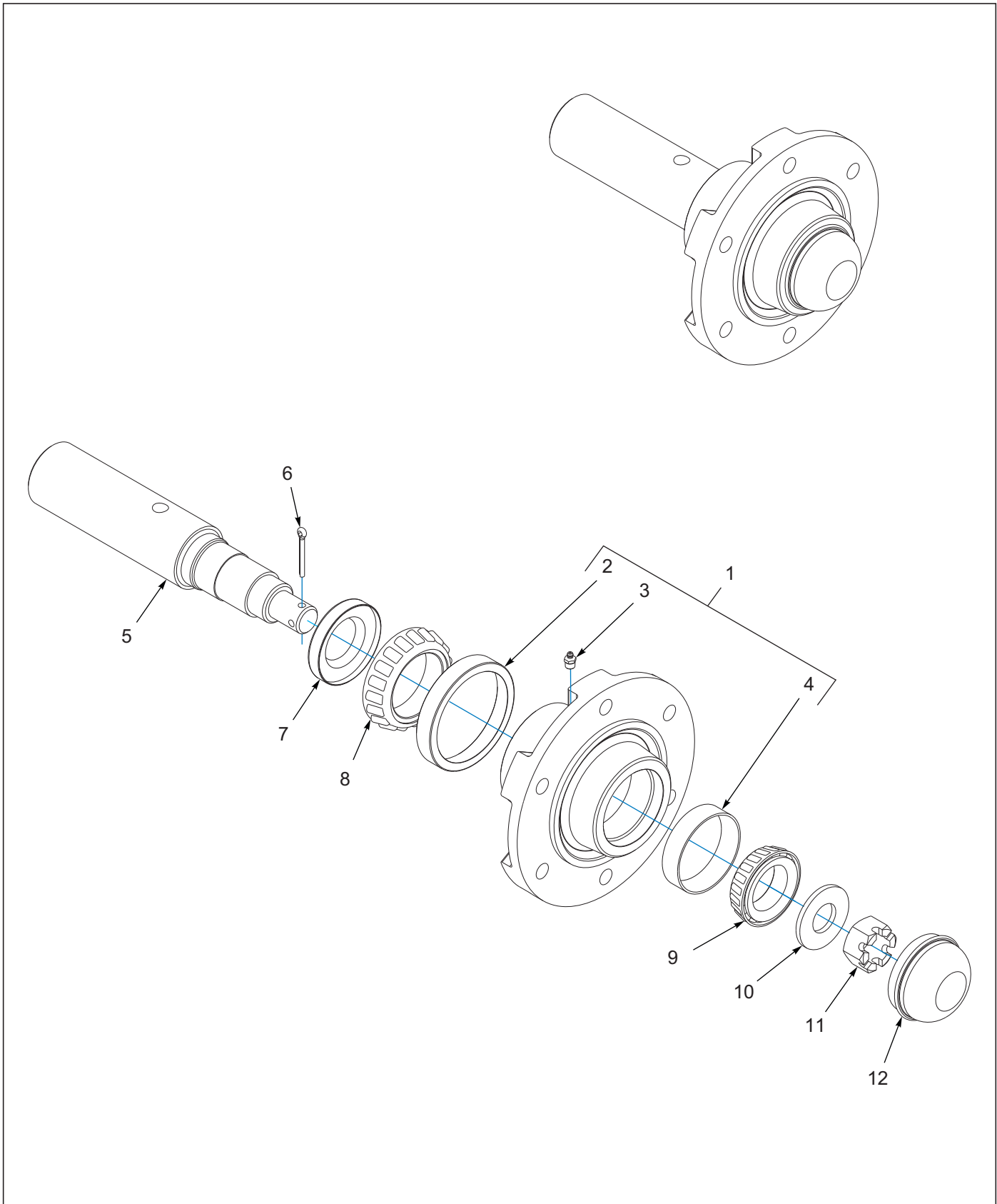
Figure 1-13: Hub/Spindle Assembly 224600
