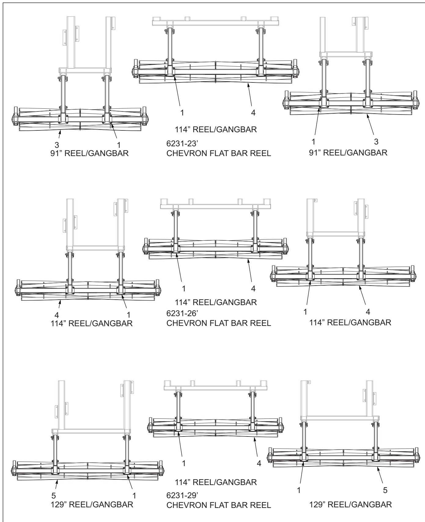
Figure 8-20: Chevron Flat Bar Reel Assembly 6231-26-29
