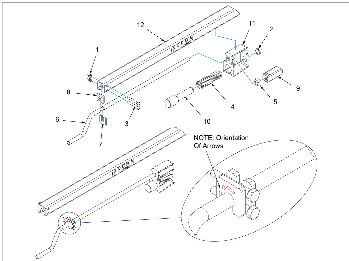
Figure 2-4: Depth Stop Tube Assembly
