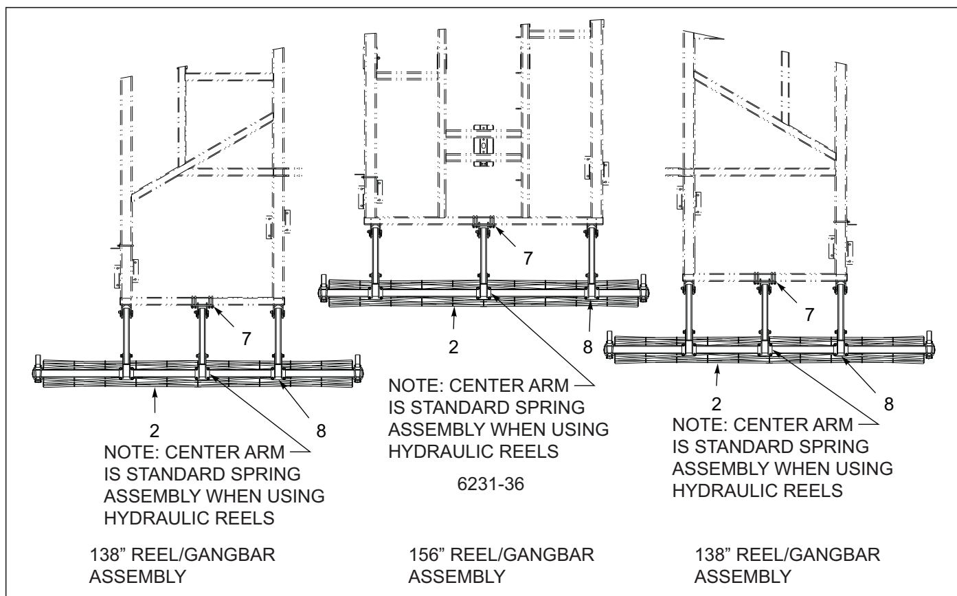
Figure 8-11: Conditioner Reel Assembly 6231-36
