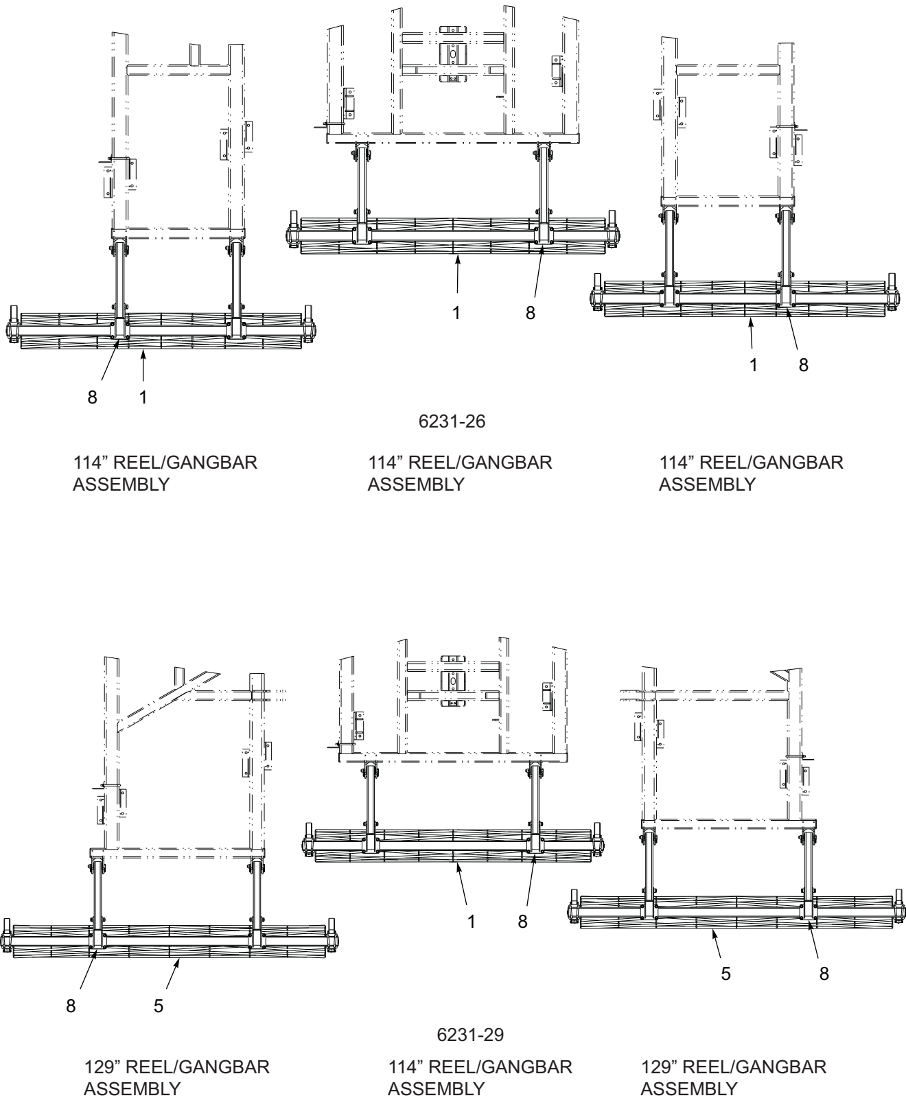
Figure 8-9: Conditioner Reel Assembly 6231-26-29
