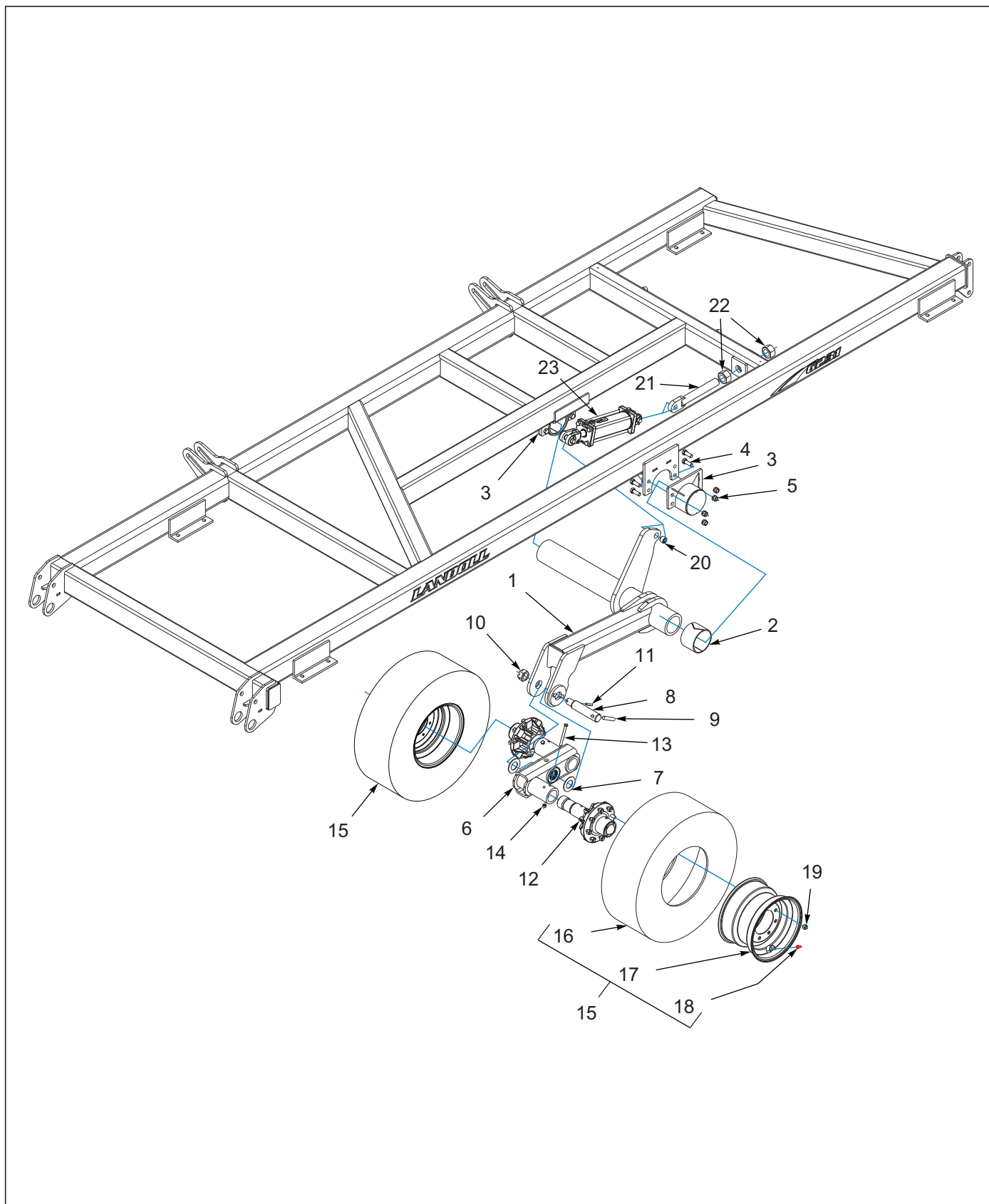
Figure 1-6: Wing Lift Assembly 6231-23'-29', 30'-36' (BEFORE 02-15-2020)
