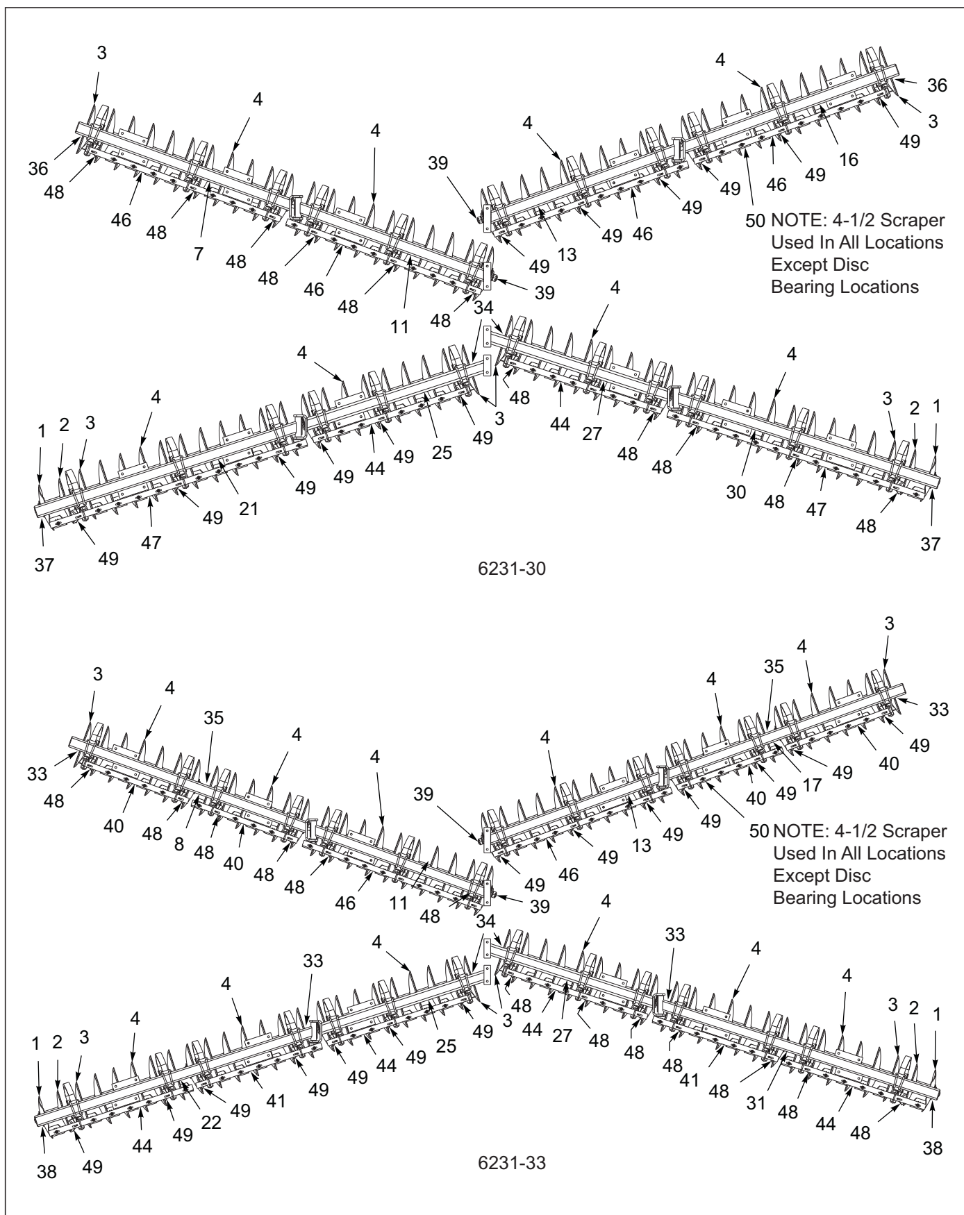
Figure 3-19: Disc Gang Assembly 6231 24' 8-3/4SP 4 GA (Non-Rollable) (3 of 4)
