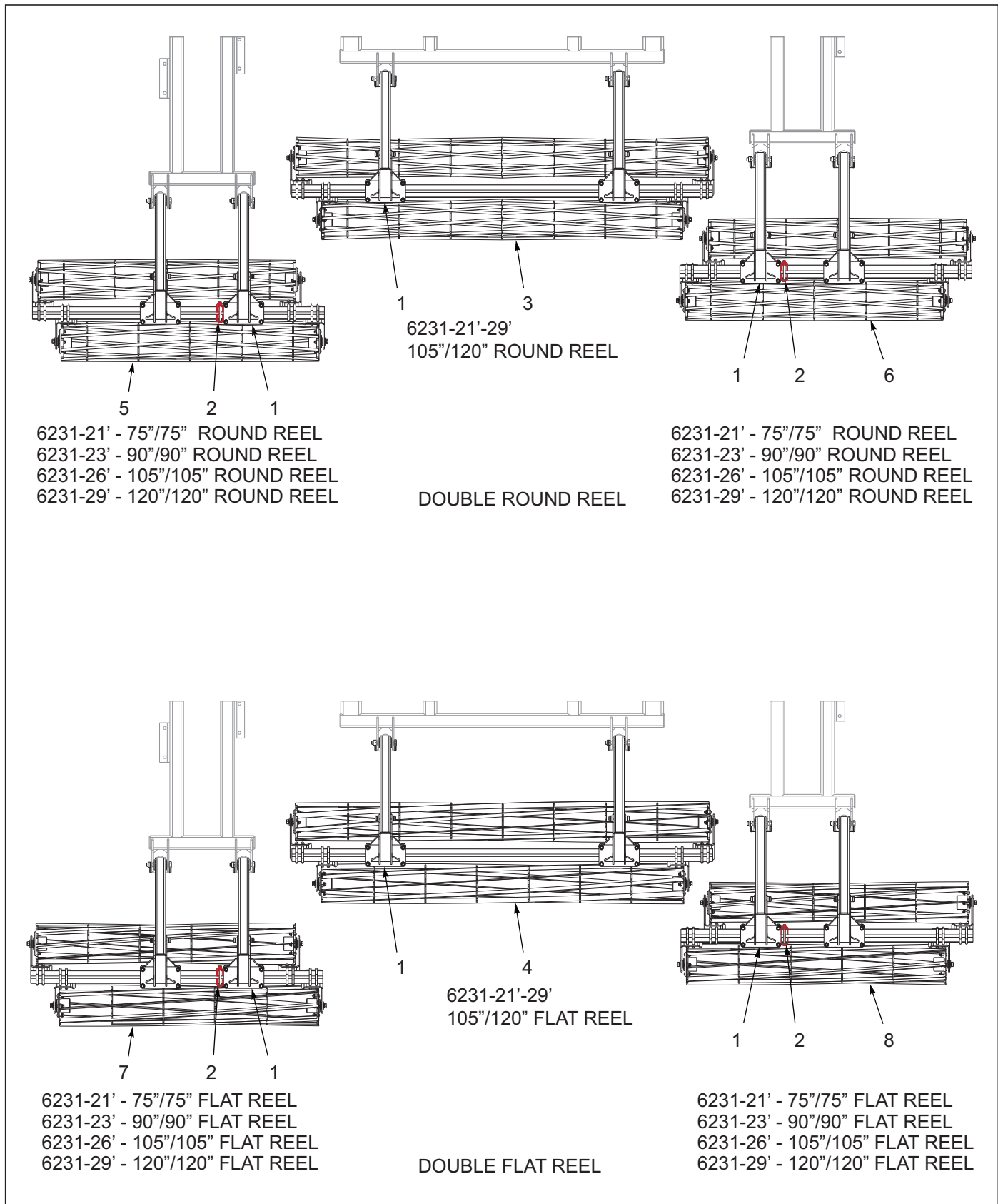
Figure 8-24: Double Reel Assembly 6231-21-23-26-29
