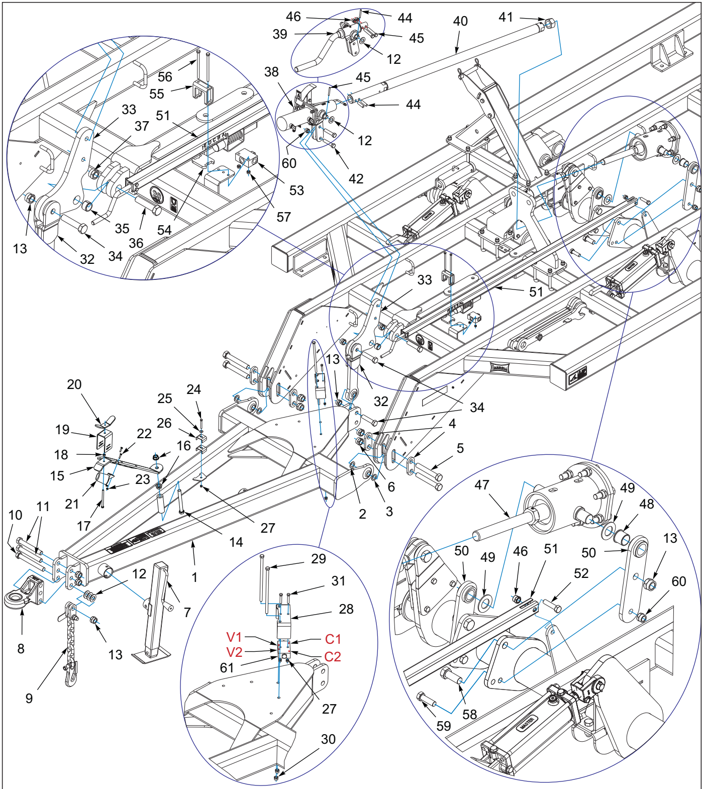
Figure 2-1: Hitch/Leveler Assembly (Before 01-01-2021)
