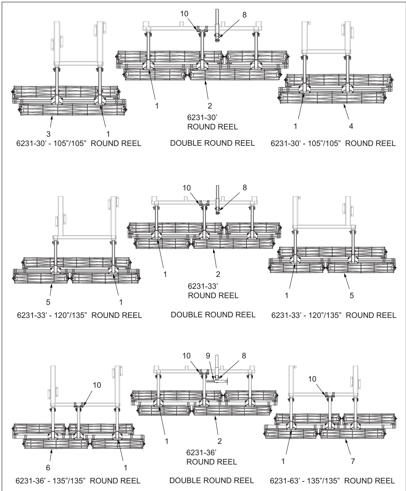
Figure 8-29: Hydraulic Double Reel Assembly 6231-30-33-36
