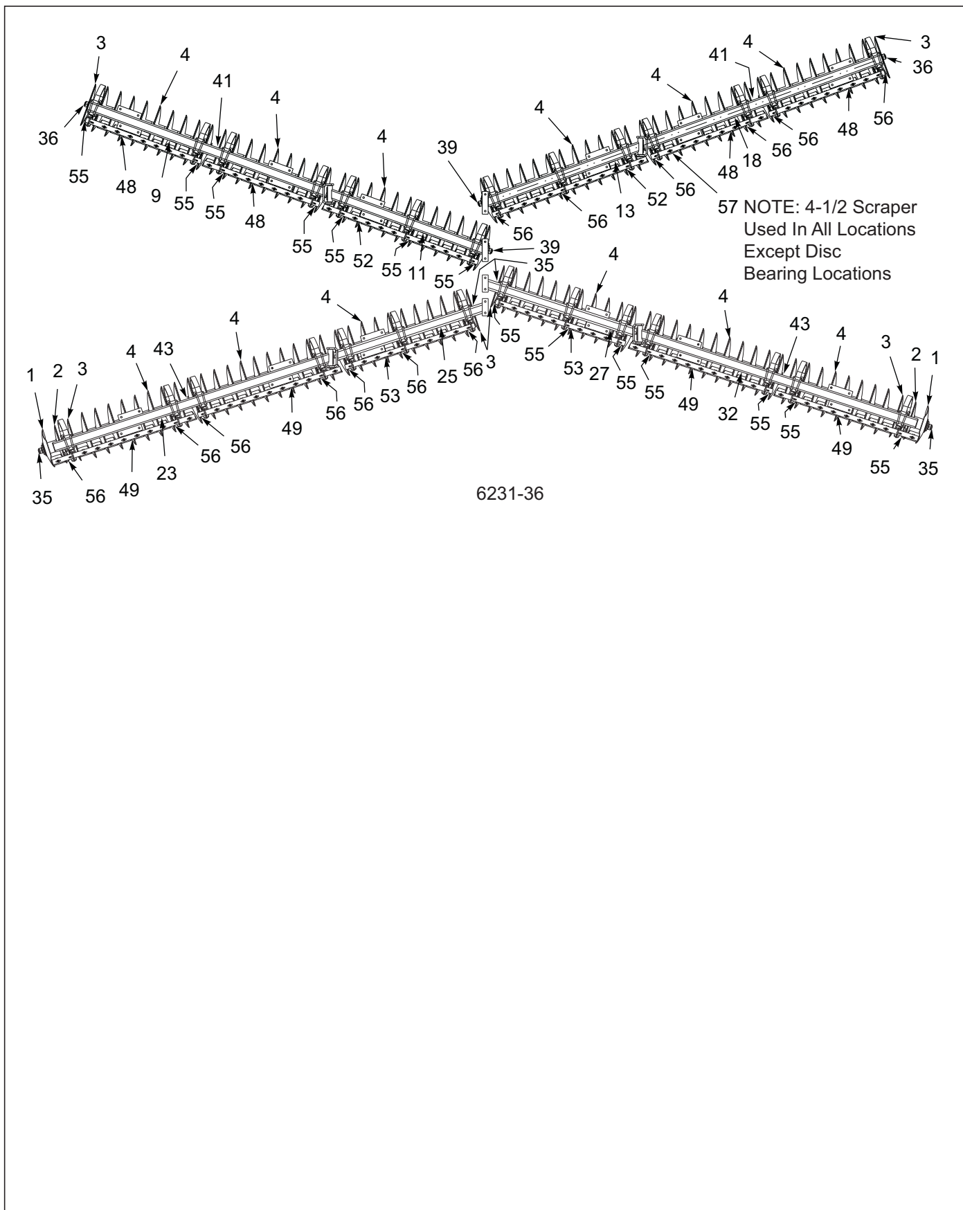
Figure 3-5: Disc Gang Assembly 6231 24" 7SP Rollable 4 GA (4 of 4)
