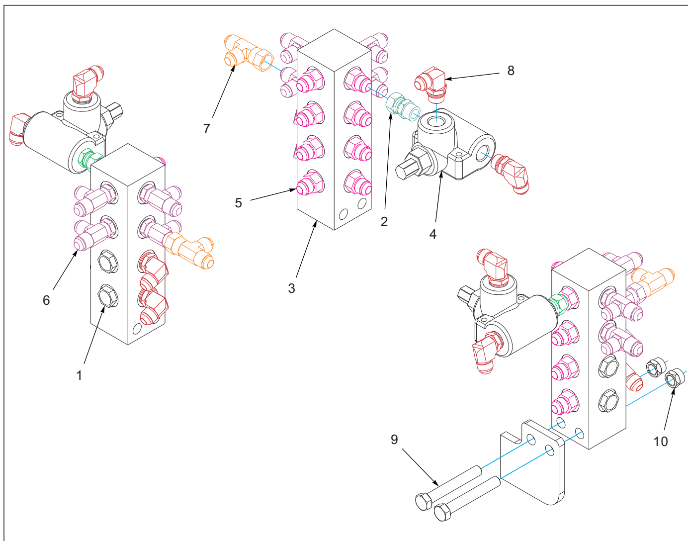
Figure 1-38: Front Manifold Assembly
