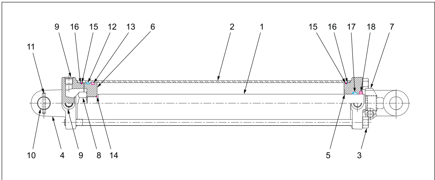
Figure 1-58: Hydraulic Cylinder 4-1/2 X 30
