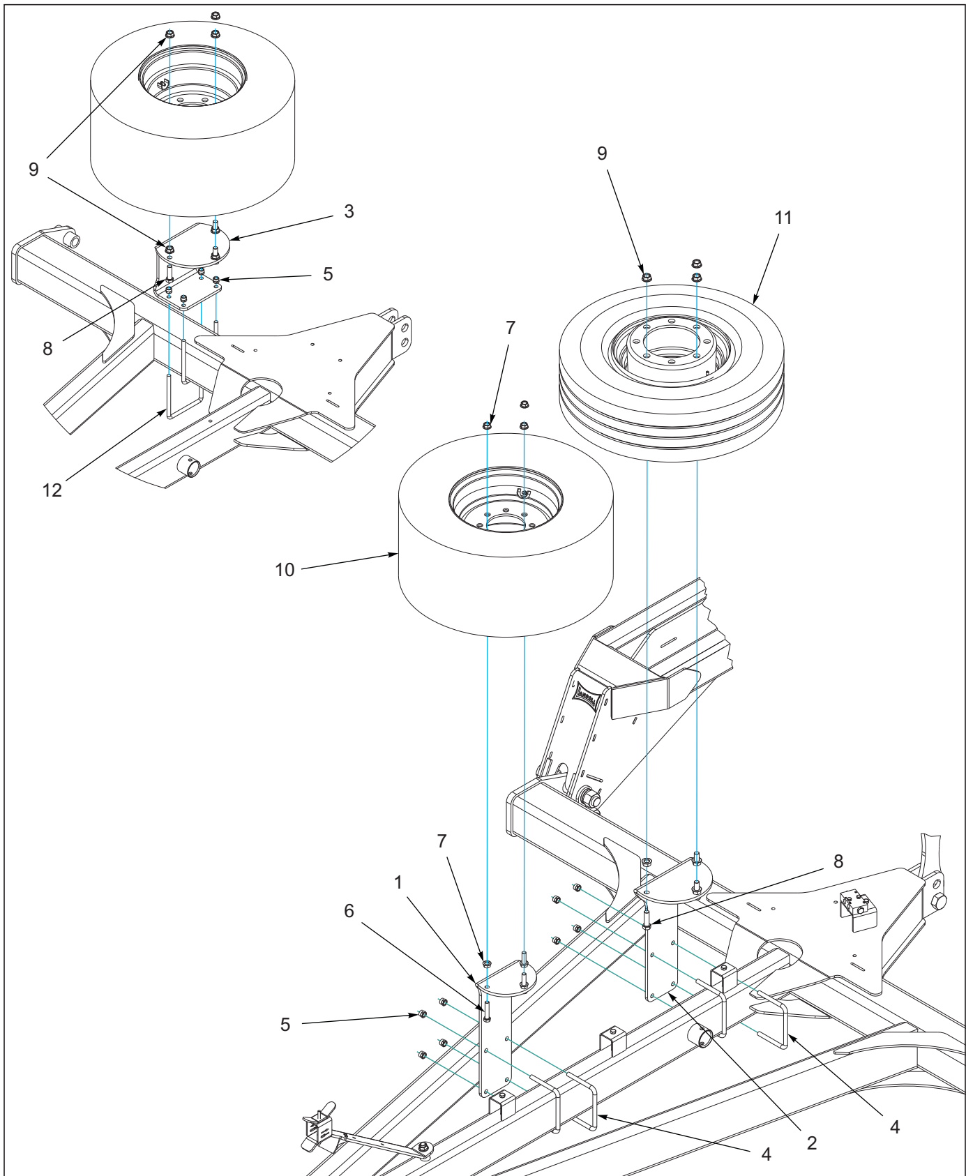
Figure 1-78: Spare Tire Assembly
