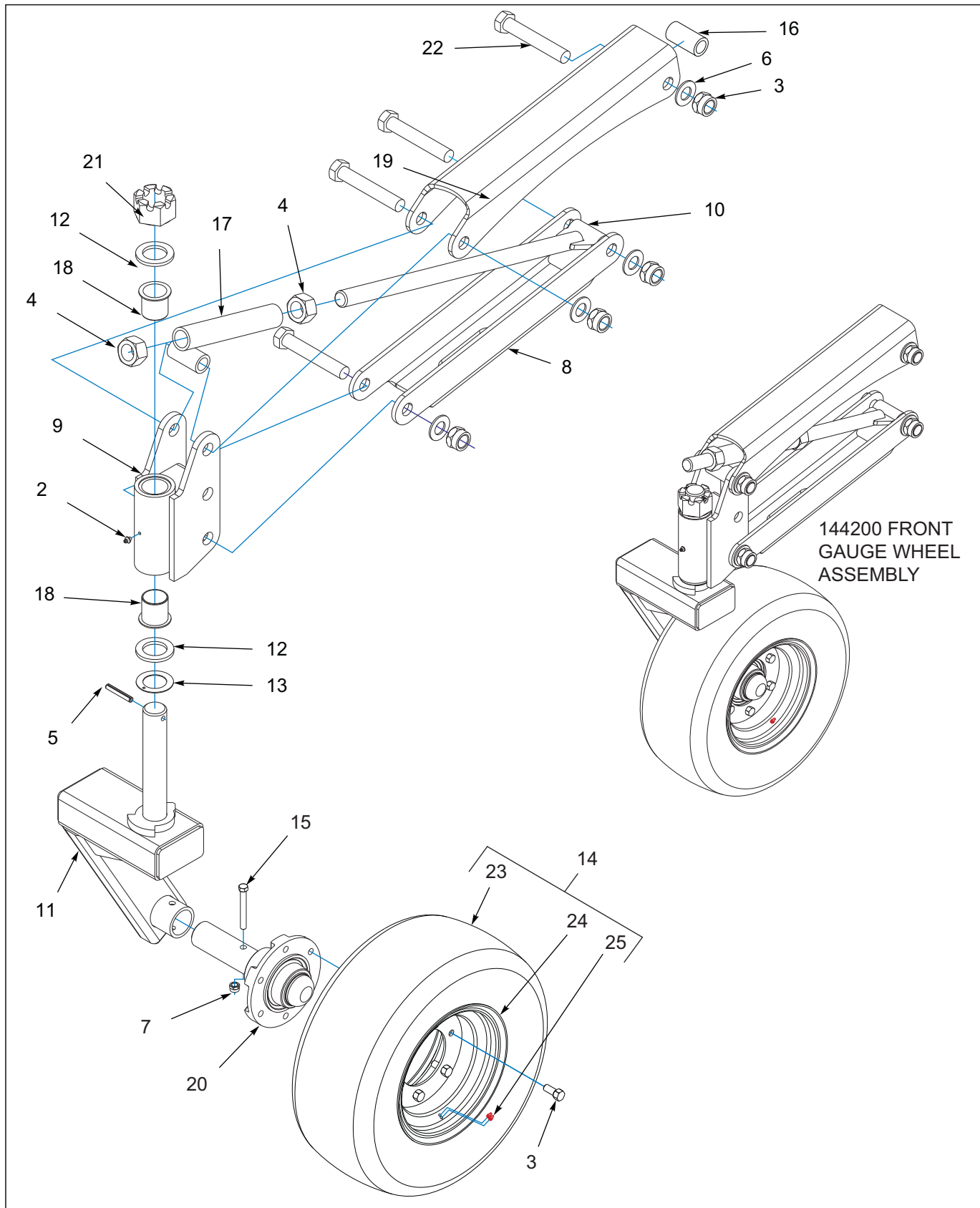
Figure 1-23: Gauge Wheel Assembly
