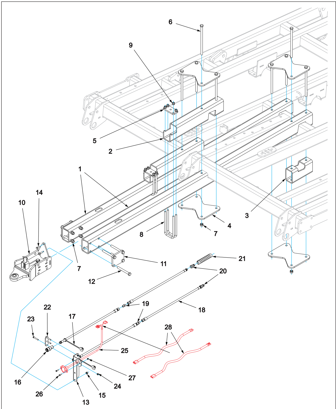
Figure 1-74: Rear Tow Hitch Assembly - Short - Fits all 6250 Models
