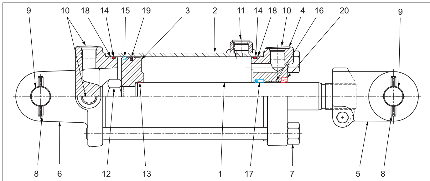
Figure 1-46: Cylinder Assembly Rephase 3-1/2 X 8 (Prince)
