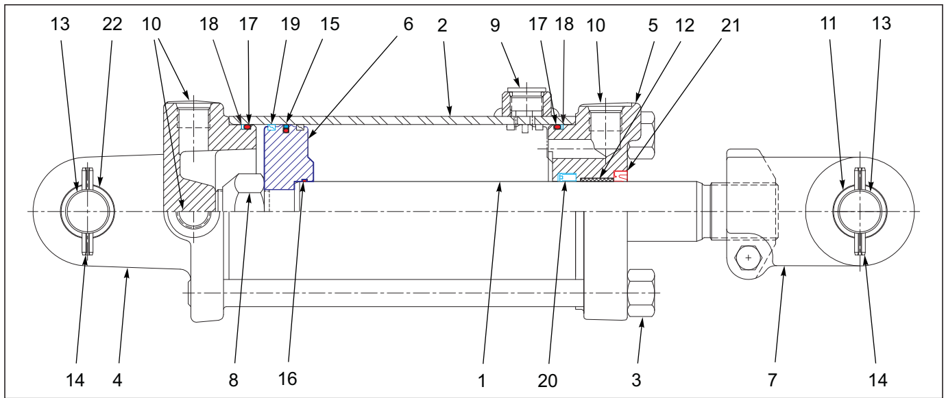
Figure 1-47: Cylinder Assembly Rephase 3-1/2 X 8 (Prince)
