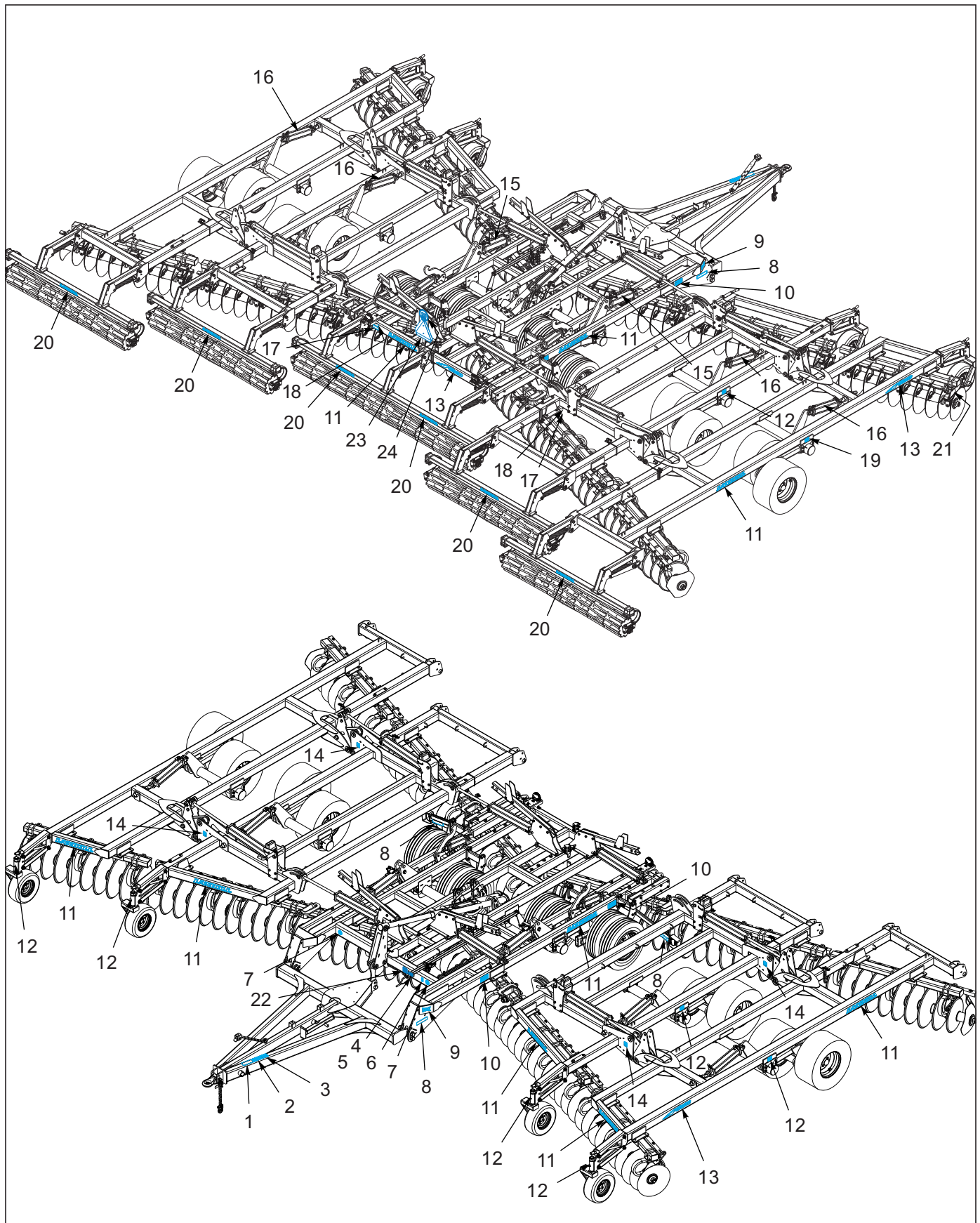
Figure 1-63: Decals (2 of 2)
