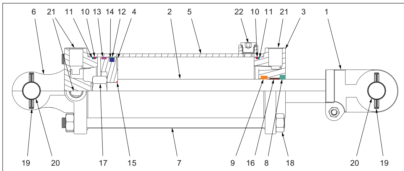
Figure 1-44: Cylinder Assembly Rephase 3-1/4 X 8 (Midway)
