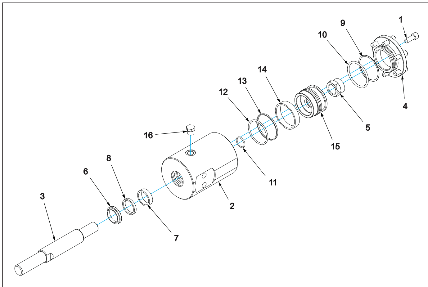
Figure 1-59: Cylinder - 2-1/2" X 1" (1" Thds)
