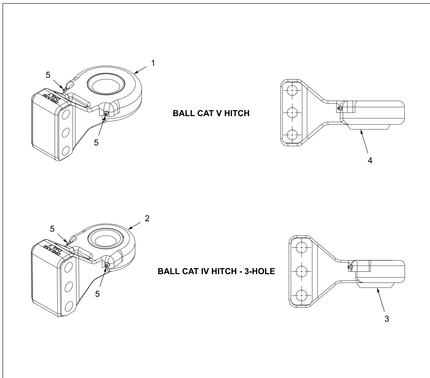
Figure 1-21: Hitch Assemblies
