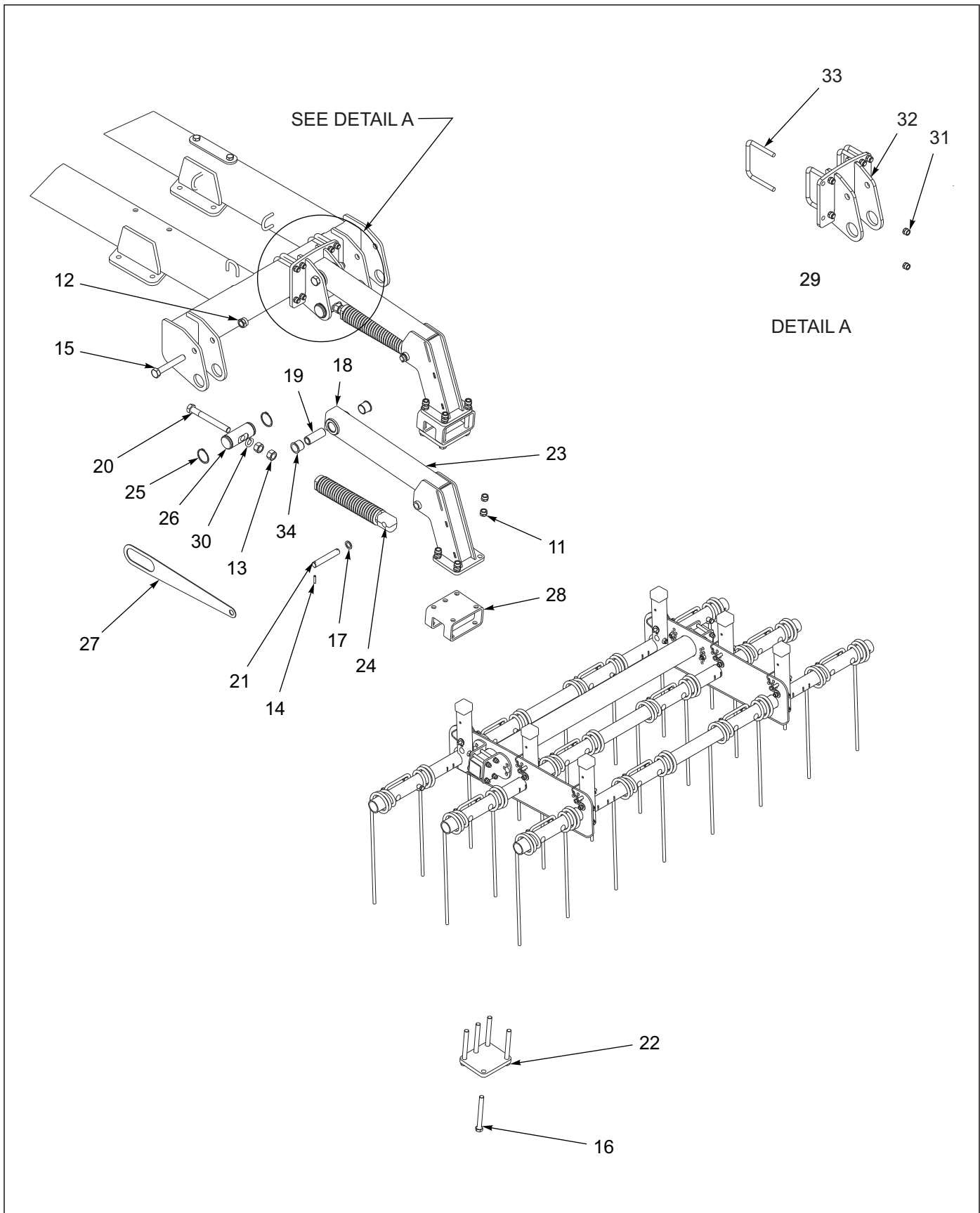
Figure 1-70: Coil Tine Harrow Assembly (3 of 3)
