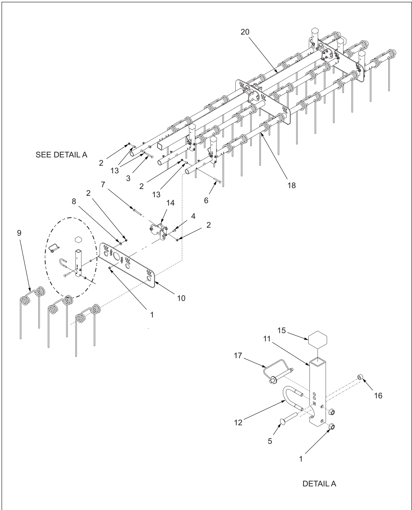
Figure 1-71: Harrow Center Assembly
