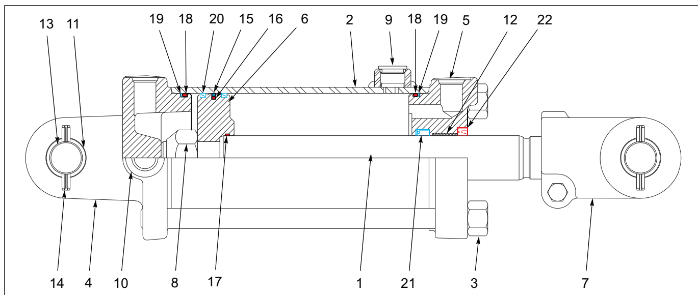
Figure 1-43: Cylinder Assembly Rephase 3-1/4 X 8 (Prince)
