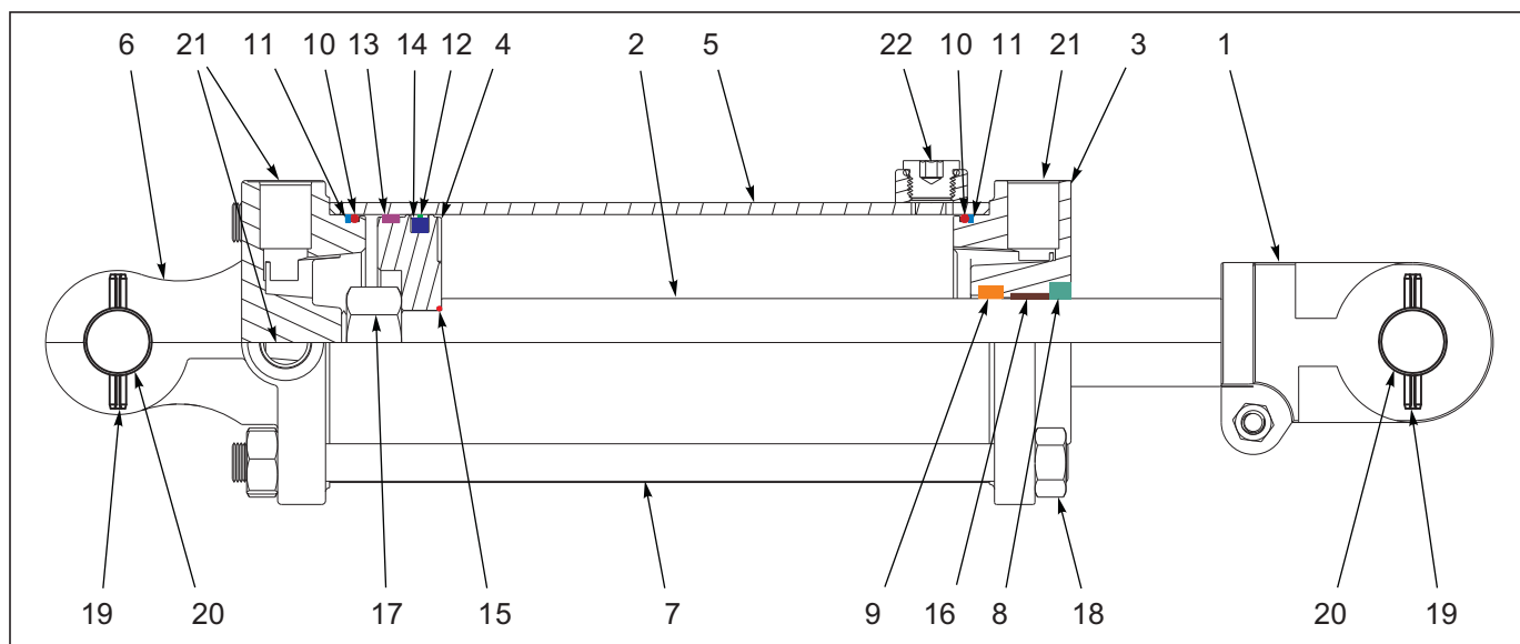
Figure 1-49: Cylinder Assembly Rephase 3-1/2 X 8 (Midway)
