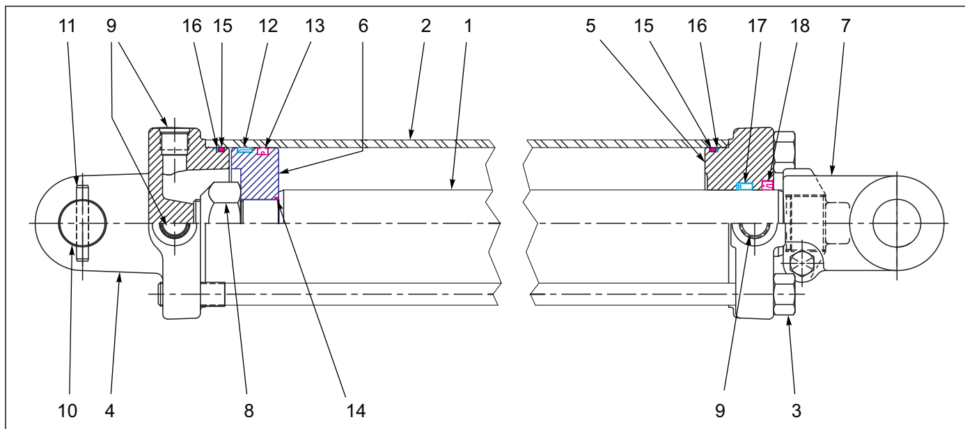
Figure 1-57: Hydraulic Cylinder 4 X 30
