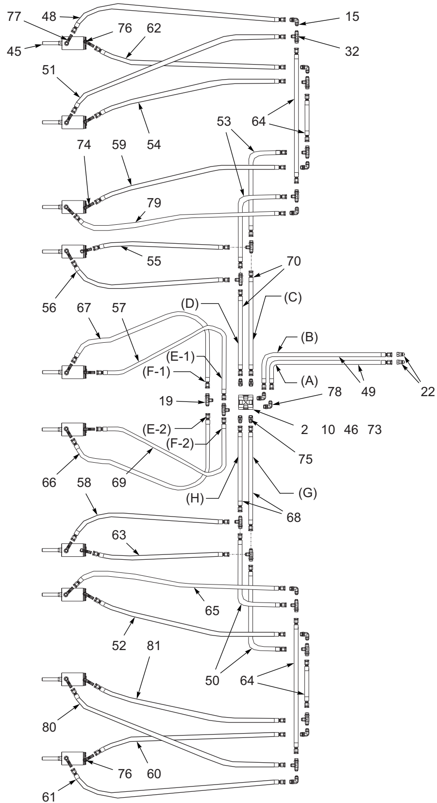
Figure 1-65: Hydraulic Conditioner Reel Assembly (2 of 3)
