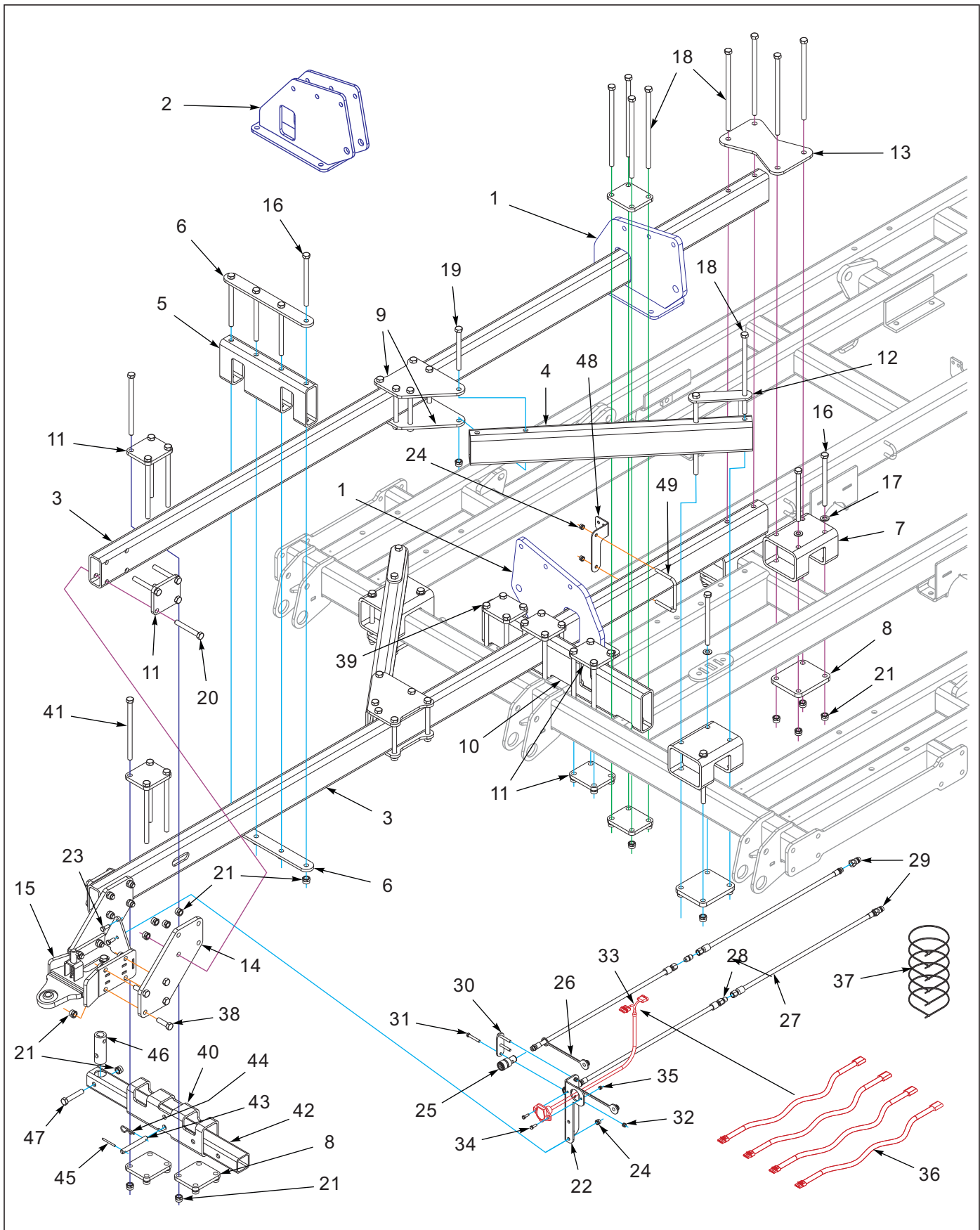
Figure 1-75: Rear Tow Hitch Assembly - Long
