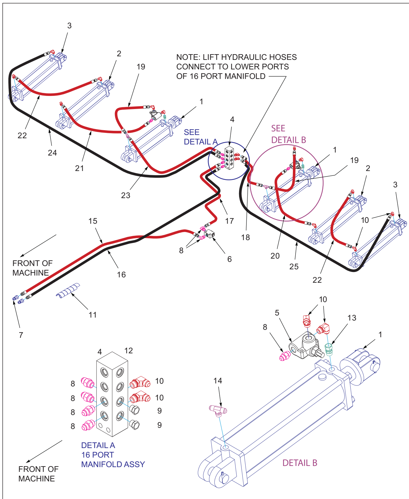
Figure 1-35: Lift Hydraulic Assembly
