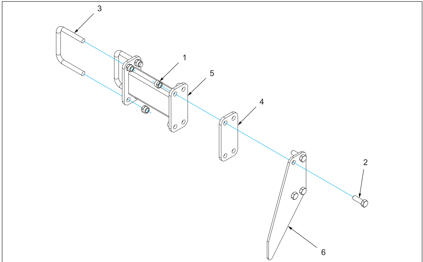
Figure 1-6: Leveler Assembly
