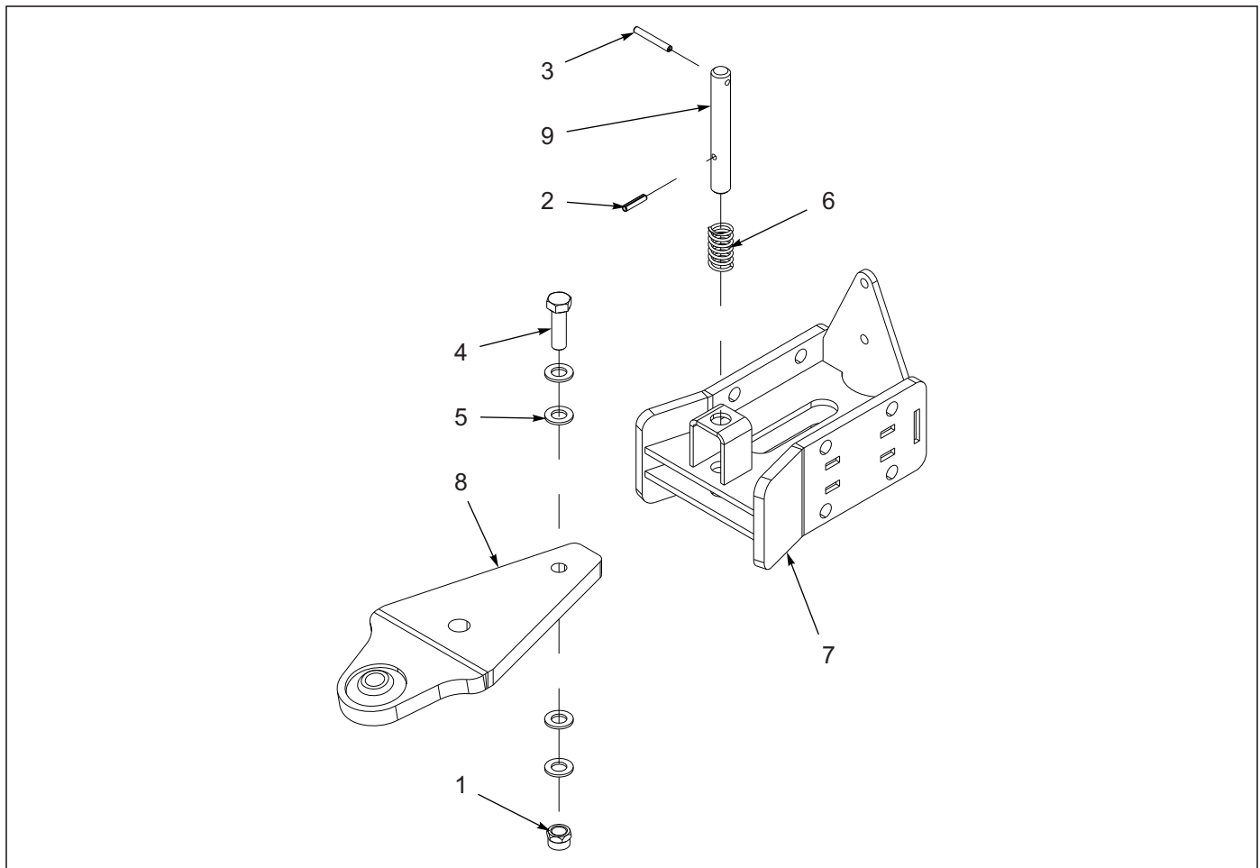
Figure 1-76: Rear Tow Hitch Assembly
