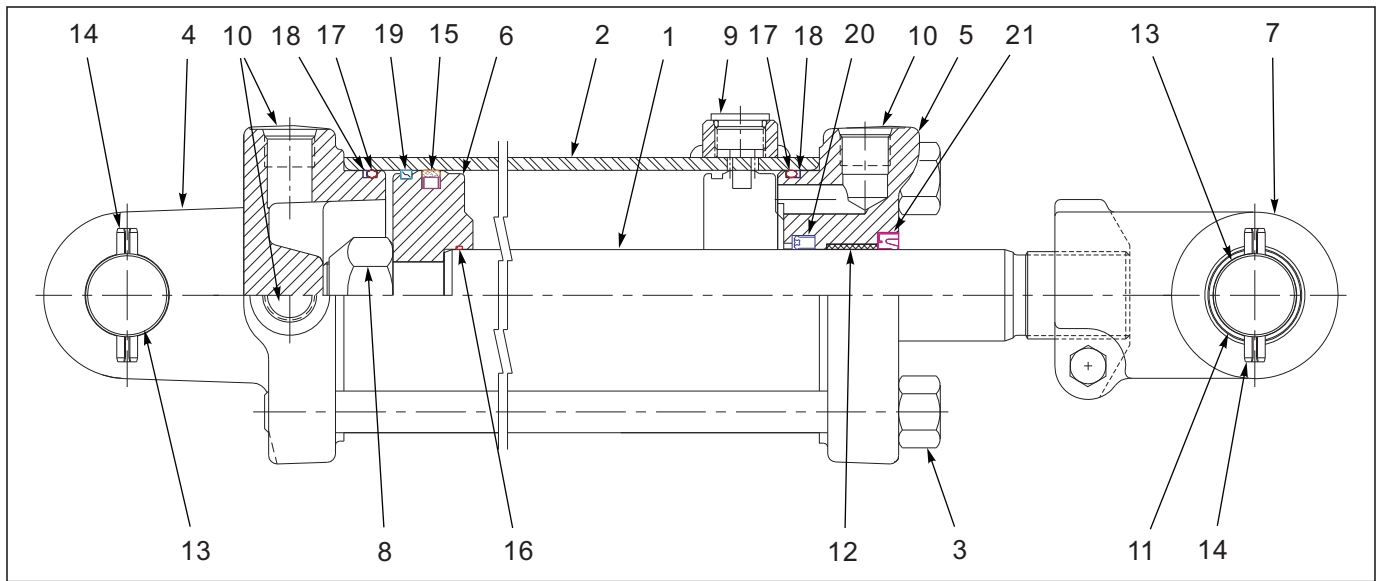
Figure 1-51: Cylinder Assembly Rephase 3-3/4 X 16 (Prince)
