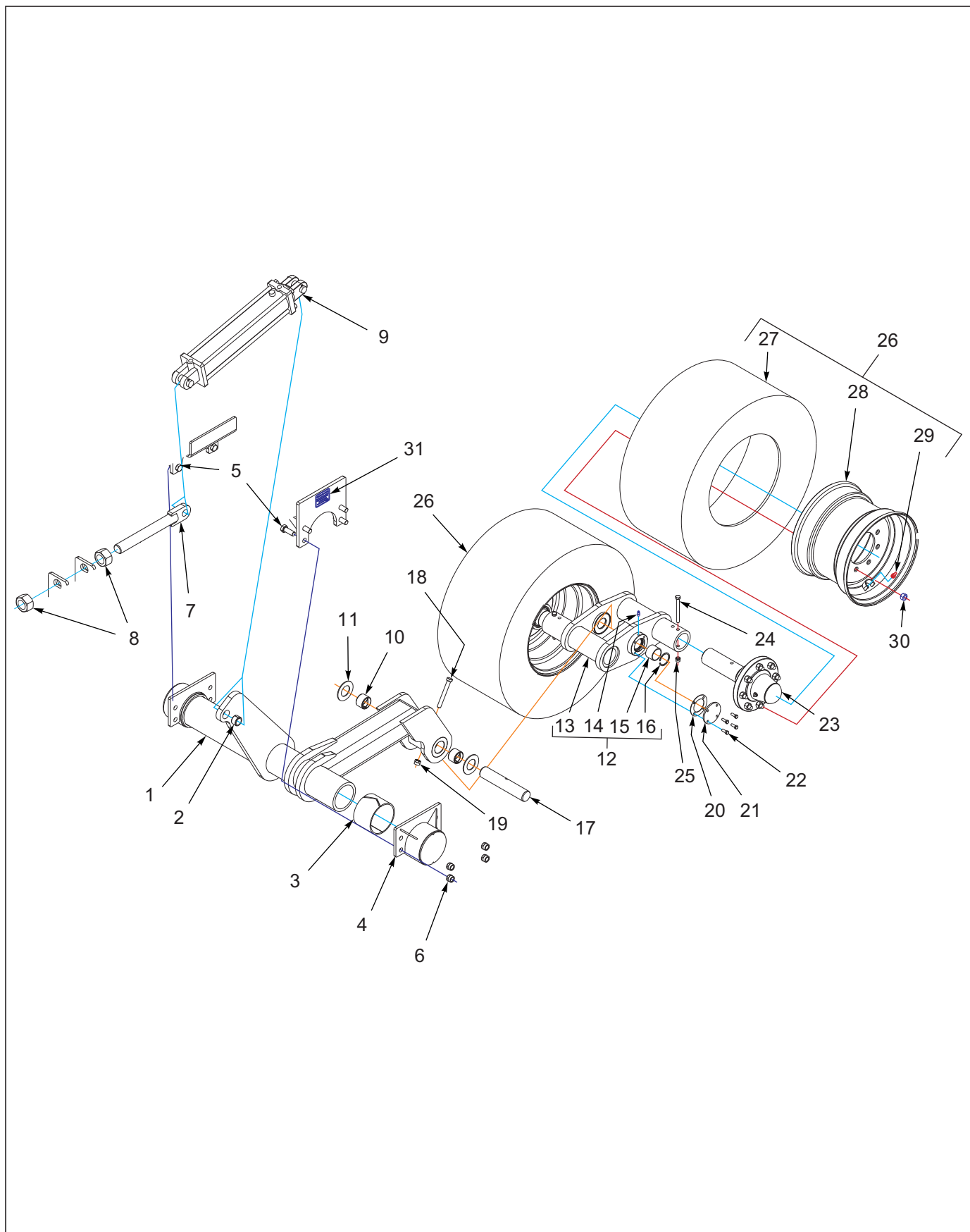
Figure 1-17: Outer Wing Lift Wheel Assembly 6250-45'-50' (After 02-01-2019)
