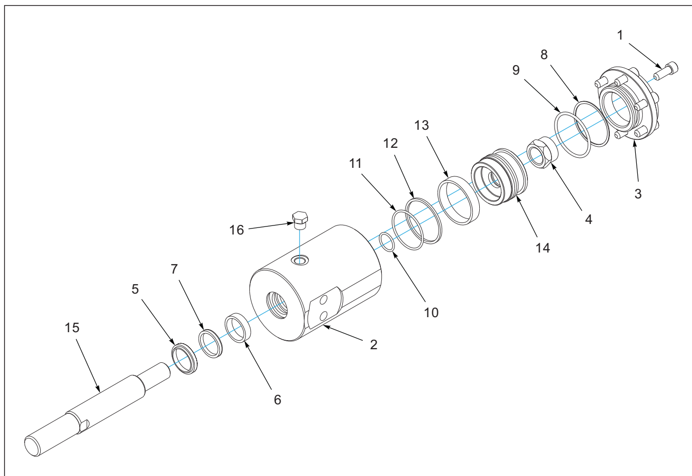
Figure 1-60: Cylinder - 2-1/2" X 1" (1-1/8" Thds)
