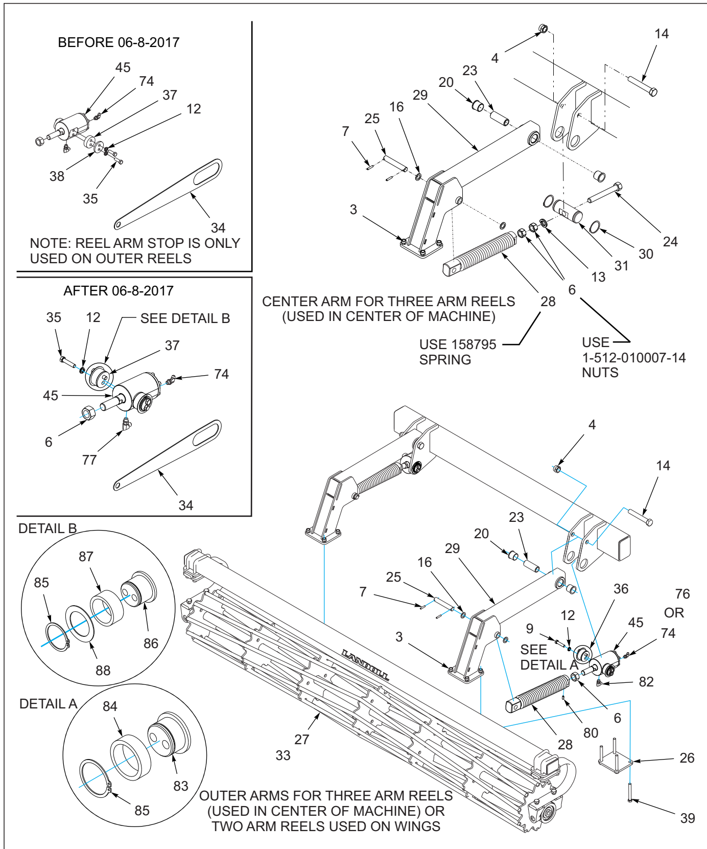
Figure 1-64: Hydraulic Conditioner Reel Assembly (1 of 3)
