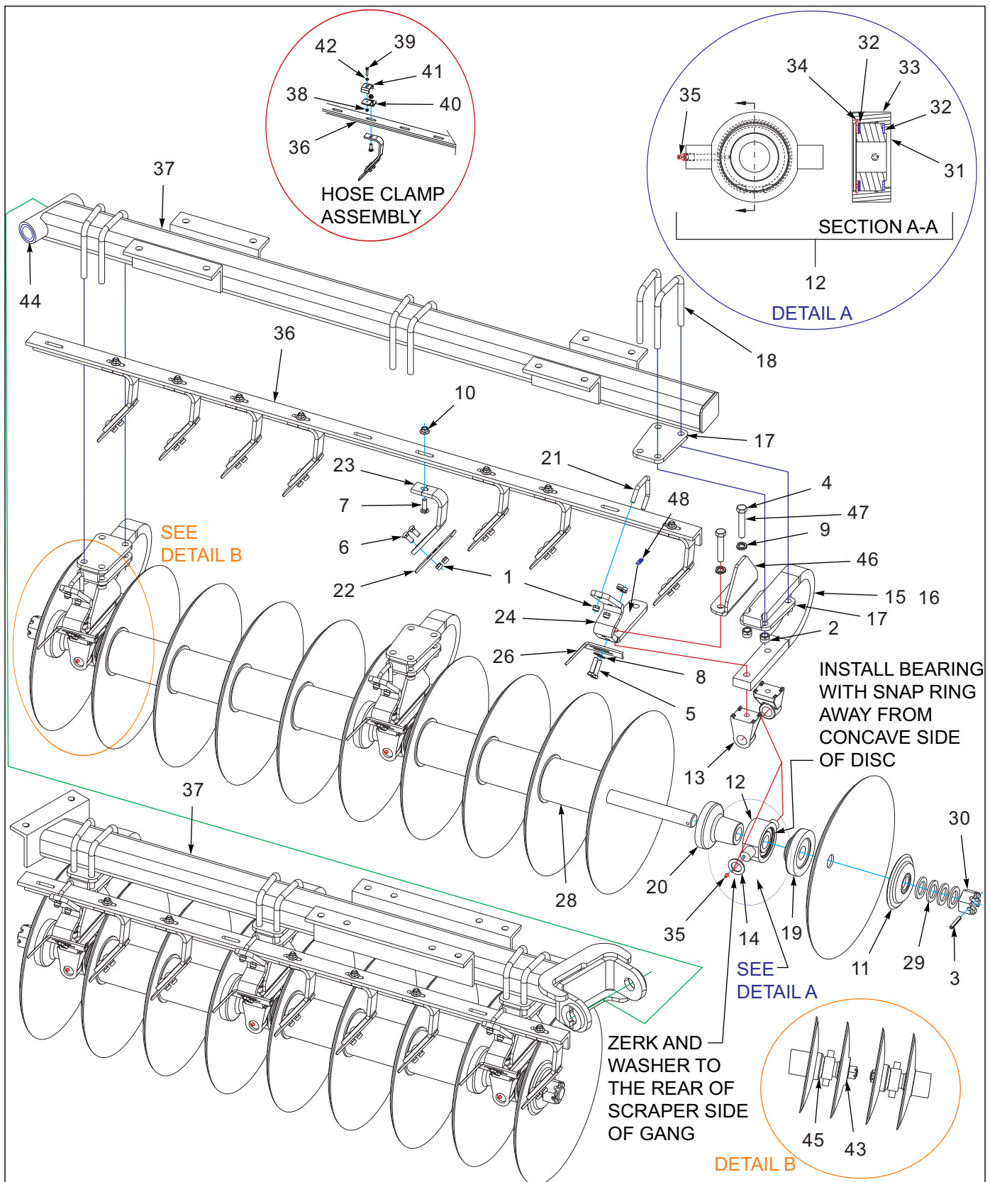
Figure 1-25: Disc Gang Assembly
