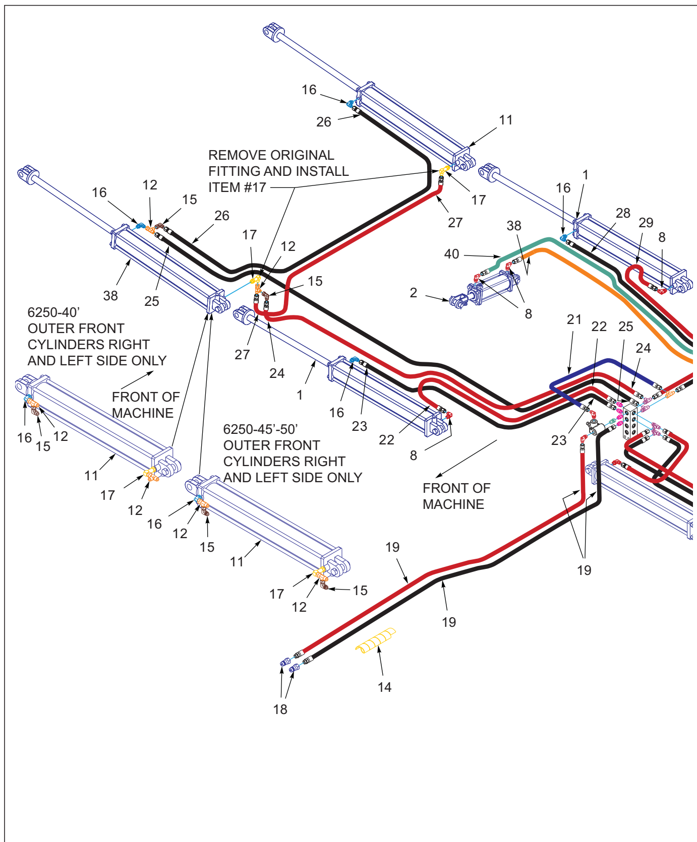
Figure 1-36: Fold Hydraulic Assembly RH
