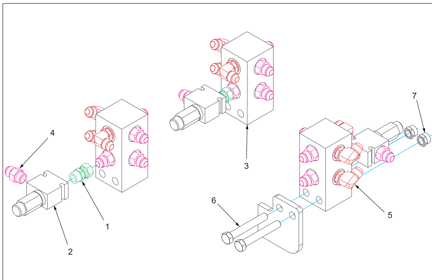
Figure 1-39: Rear Manifold Assembly
