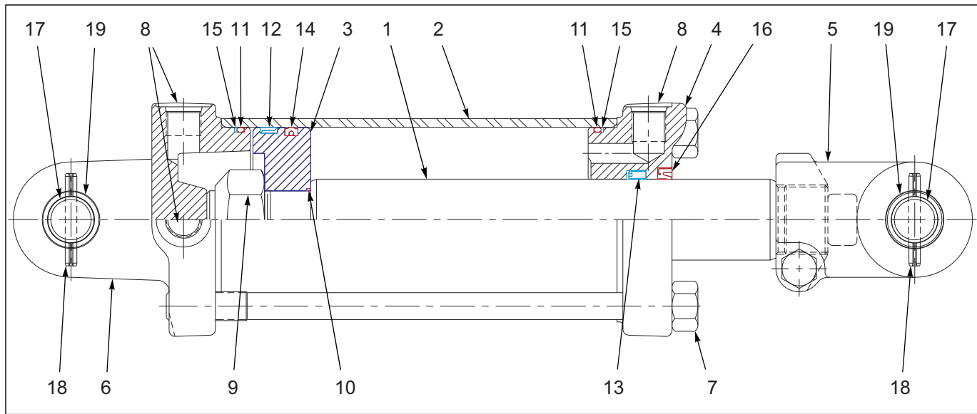
Figure 1-56: Cylinder Assembly 4 X 8
