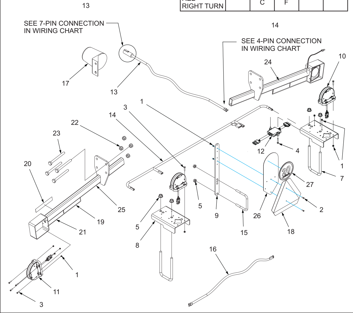
Figure 1-61: Electrical Assembly
