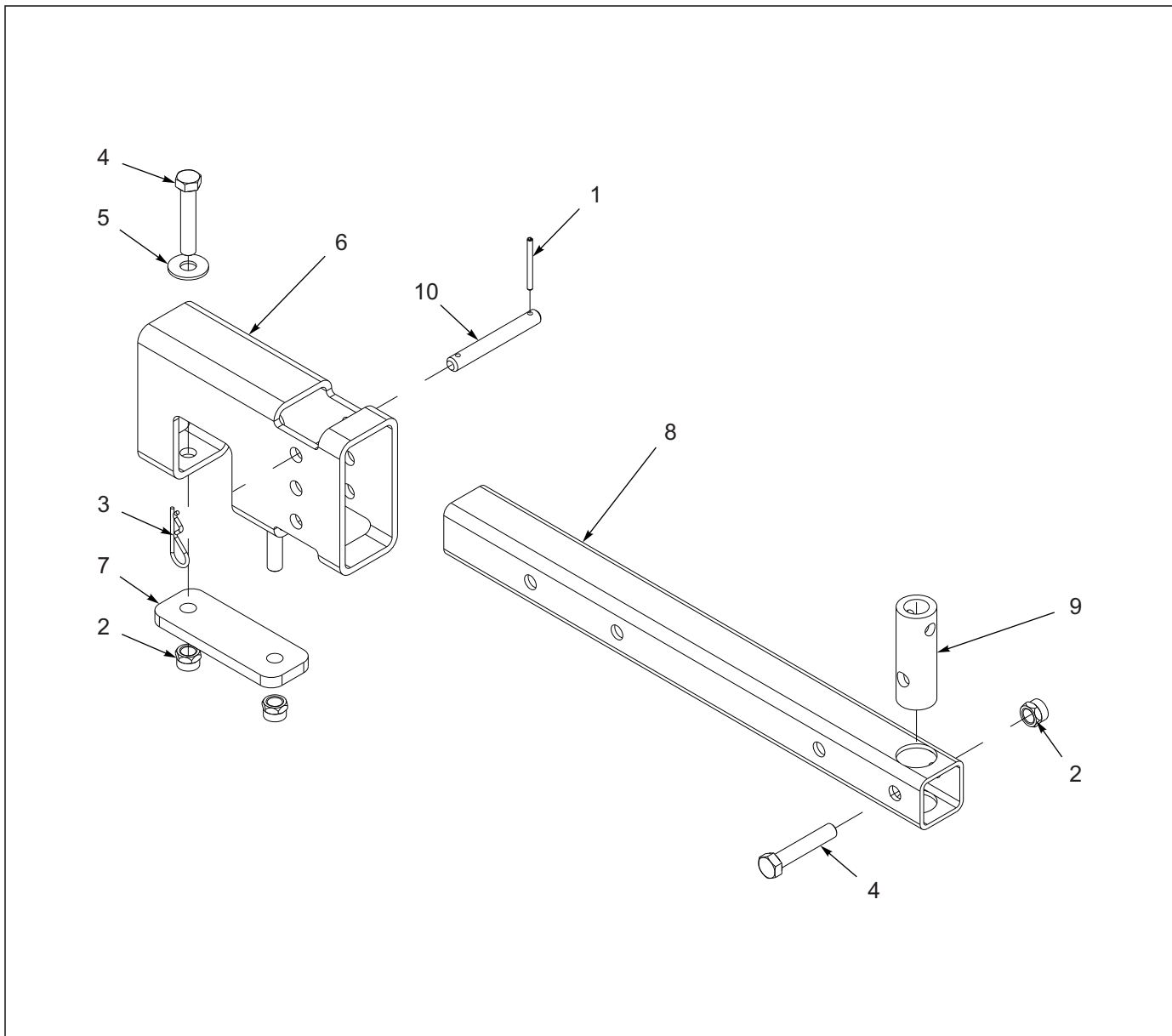
Figure 1-77: Rear Jack Assembly
