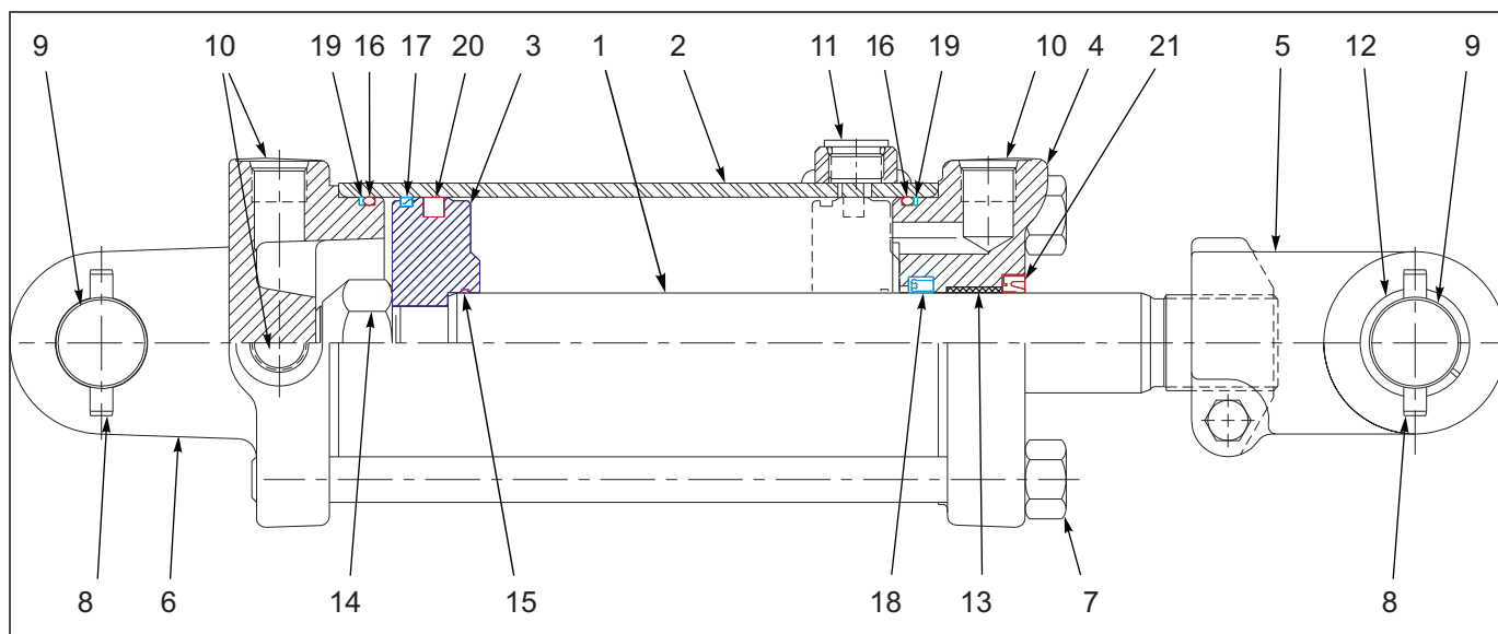
Figure 1-53: Cylinder Assembly Rephase 4 X 16 (Prince)
