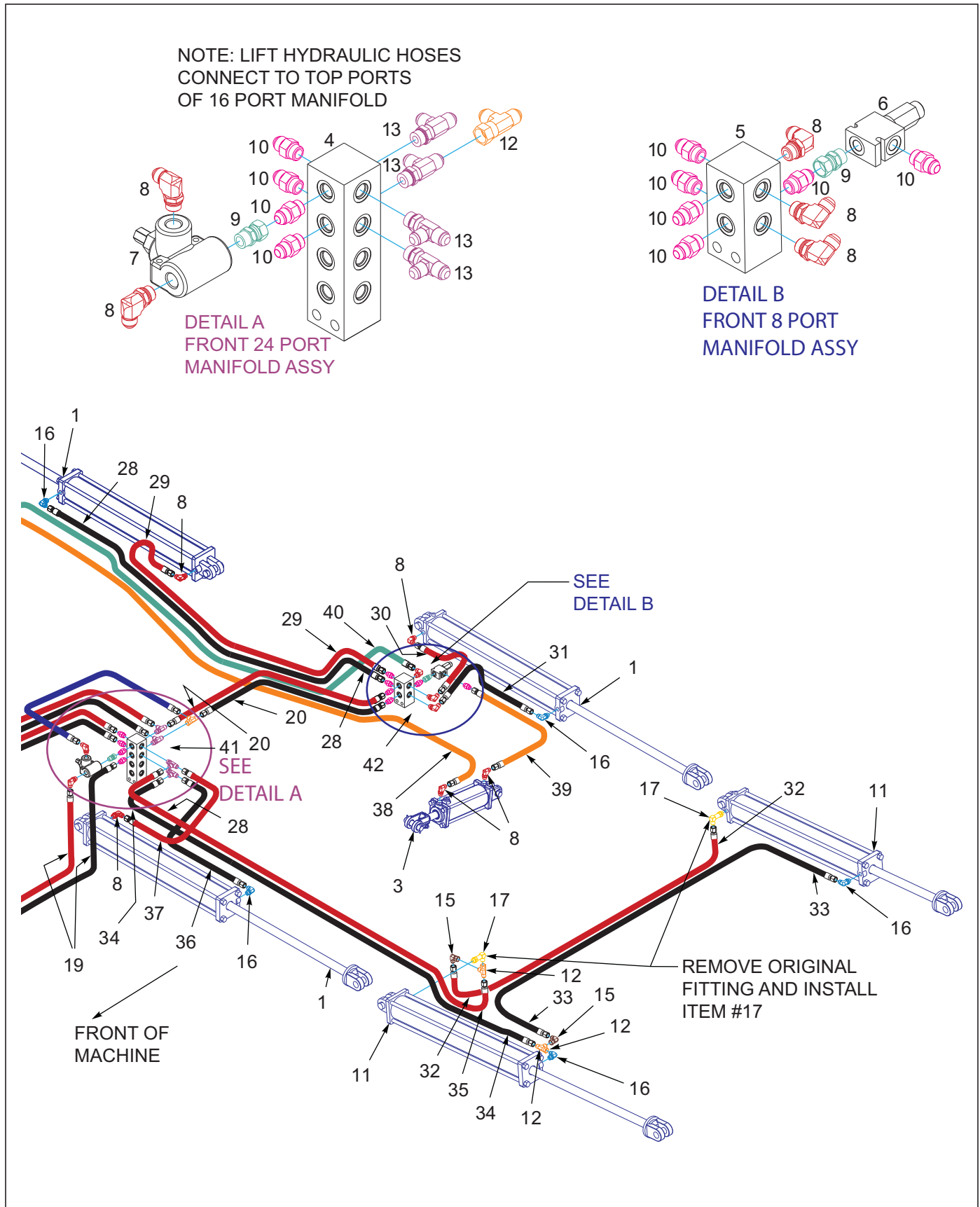
Figure 1-37: Fold Hydraulic Assembly LH
