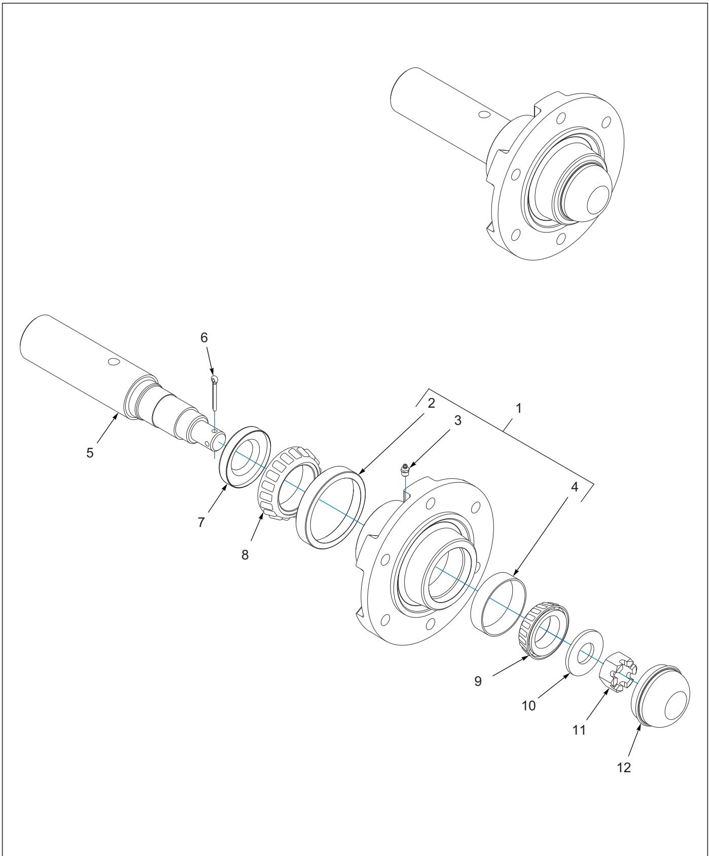
Figure 1-24: Hub/Spindle Assembly 224600
