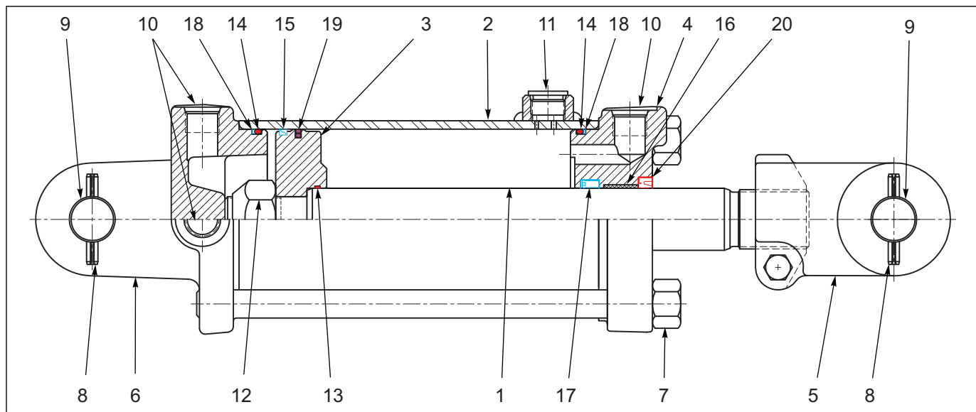
Figure 1-42: Cylinder Assembly Rephase 3-1/4 X 8 (Prince)
