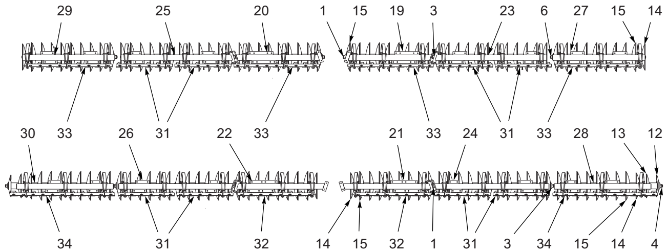
6250-45 8-3/4"-26" 4 GA LC BLADES (180062) (ALL DISC BLADES NOT BALLOONED ARE ITEM 15)
