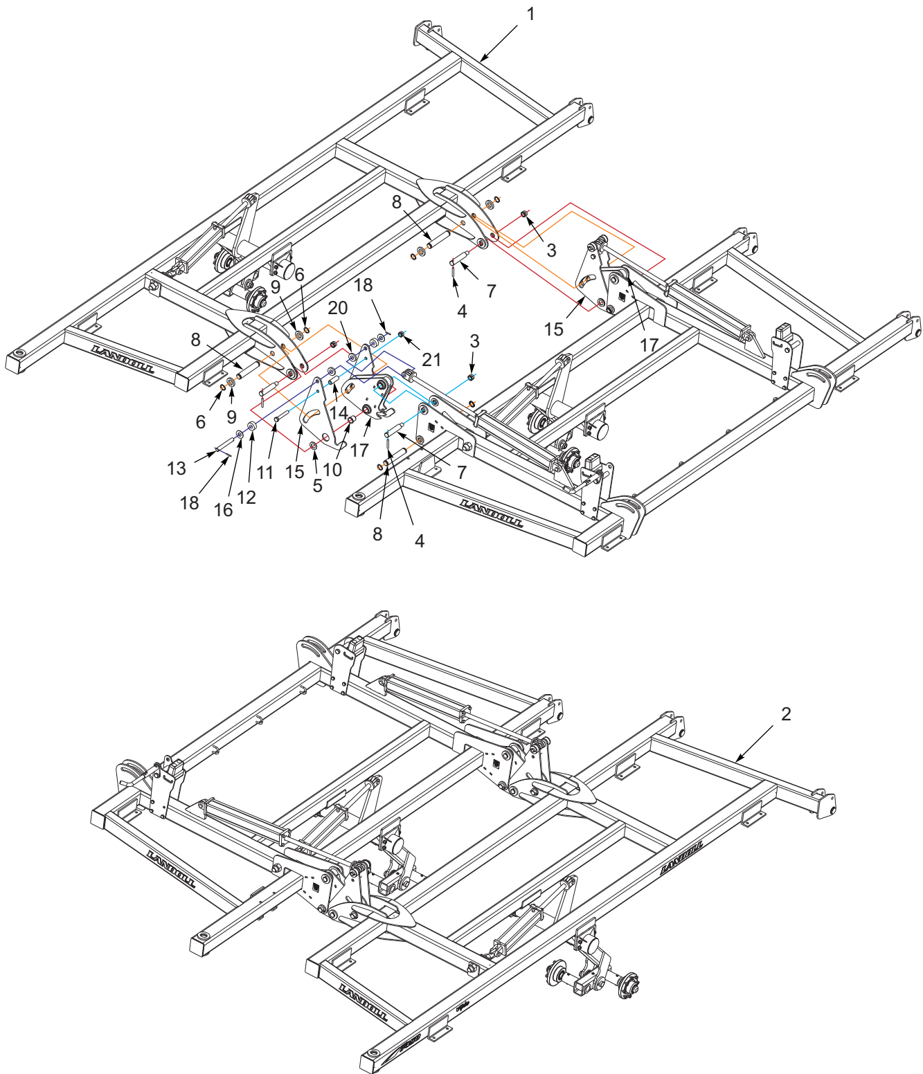
Figure 1-15: Outer Wing Frame and Fold Lock Assembly
