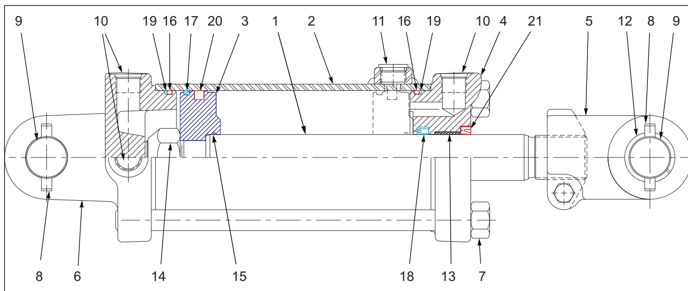
Figure 1-55: Cylinder Assembly Rephase 4-1/2 X 16 (Prince)
