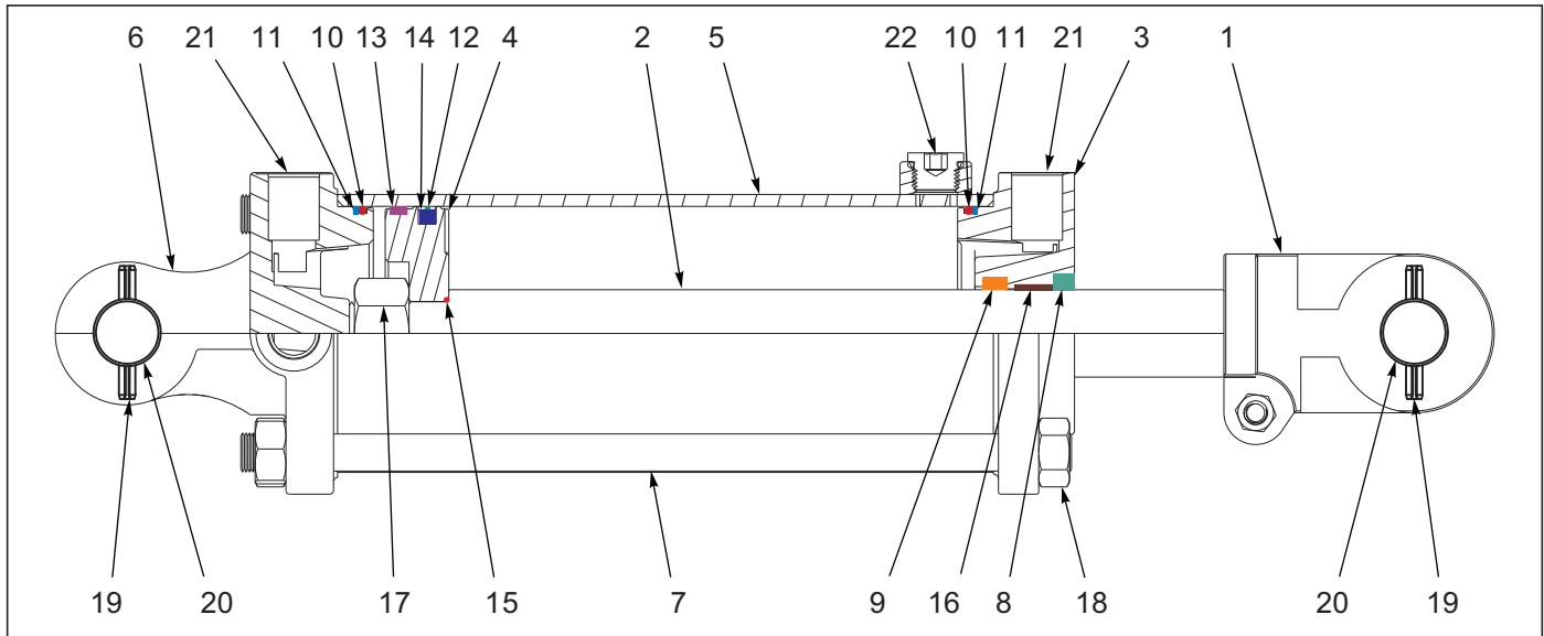
Figure 6-2: Cylinder Assembly 4 x 10 Rephase (Midway)
