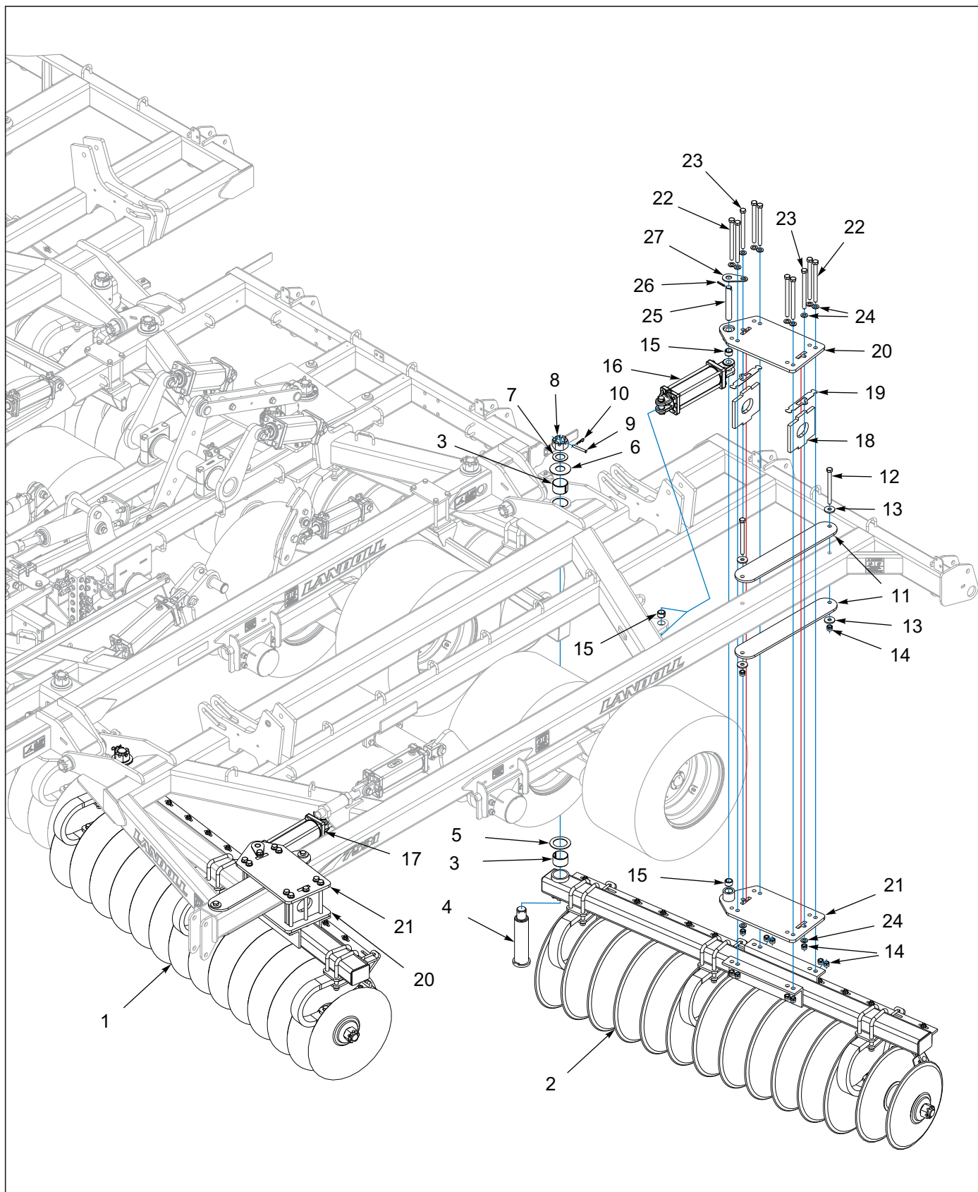
Figure 4-5: Gang Assembly Wing 7531-26'-35'
