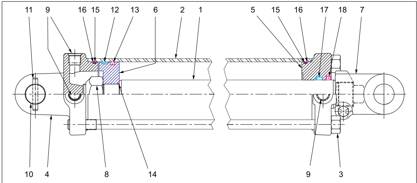
Figure 6-22: Cylinder Assembly 4 x 30 (Prince)
