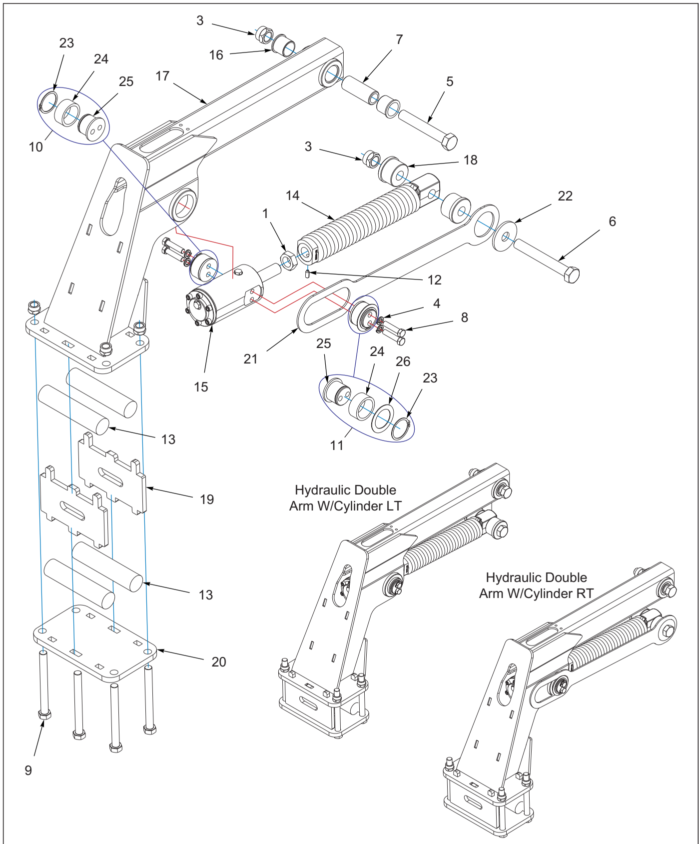
Figure 9-17: Hydraulic Double Arm W/Stop Assembly
