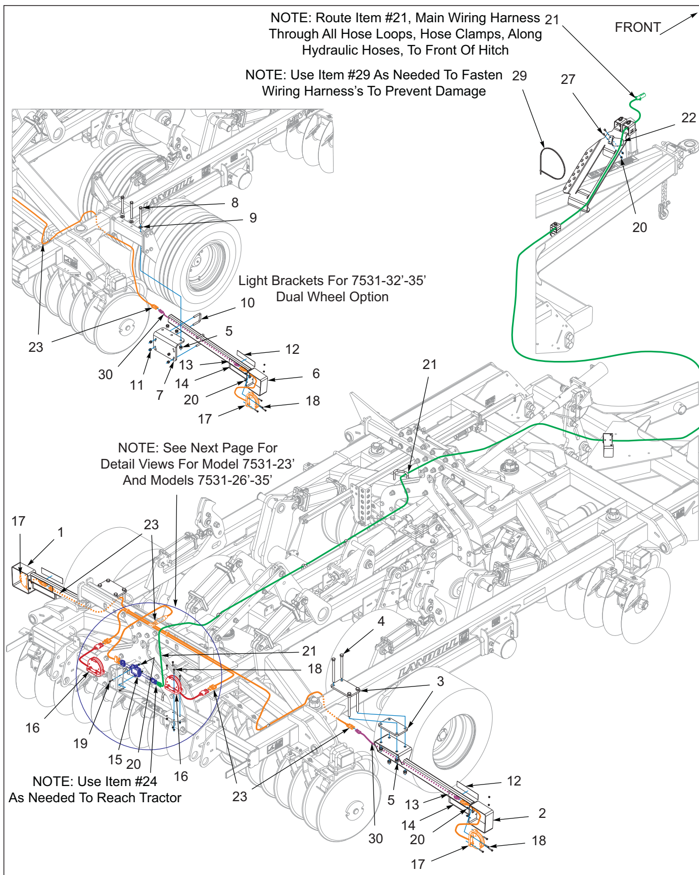
Figure 7-2: Electrical Assembly W/LED Lights (2 of 3)
