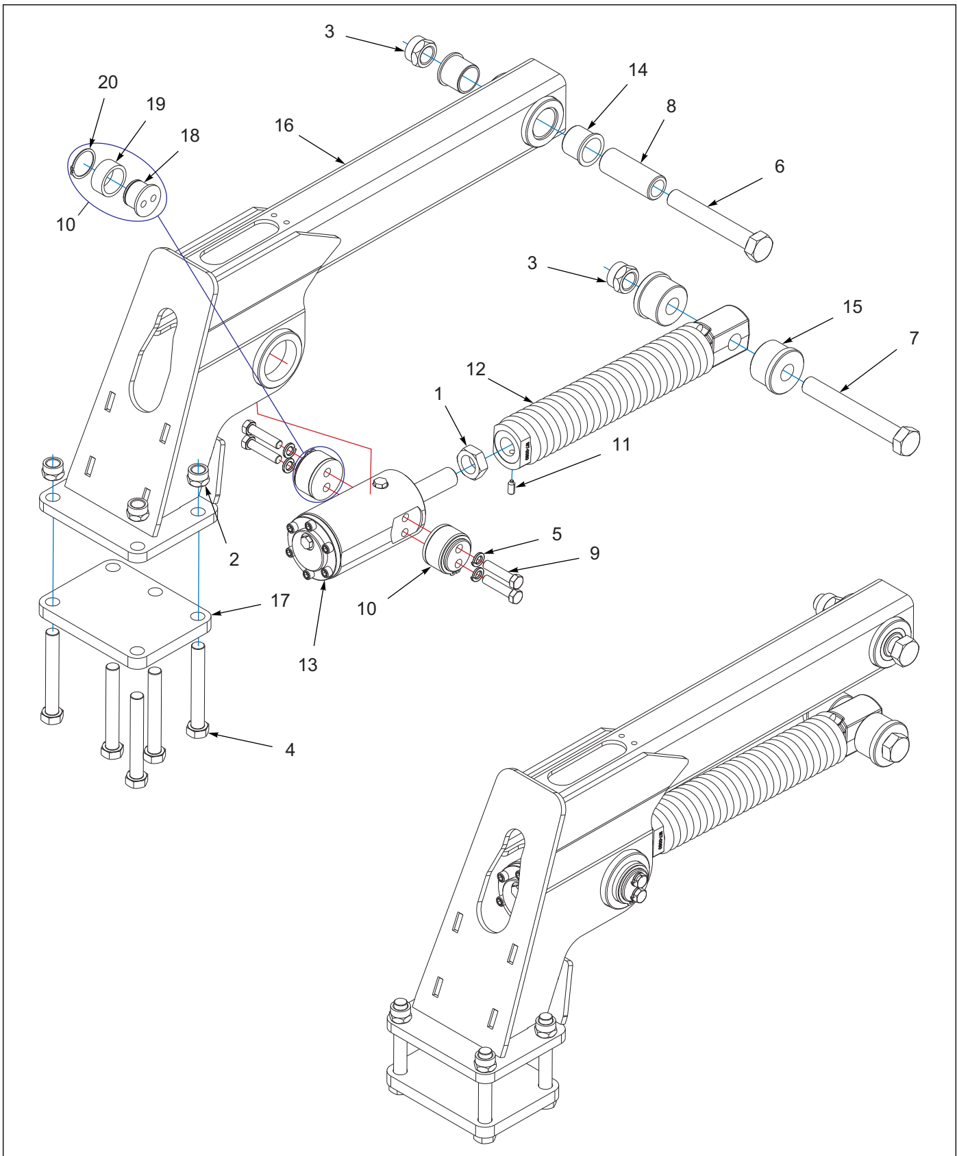
Figure 9-12: Hydraulic Single Arm Assembly
