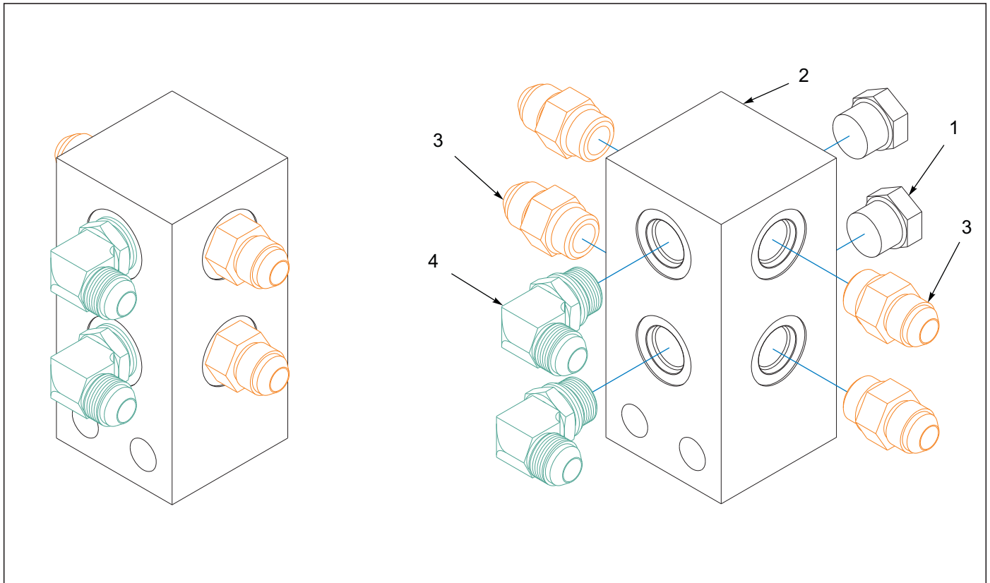
Figure 5-23: Manifold Assembly Front 7531-26'/29' After
