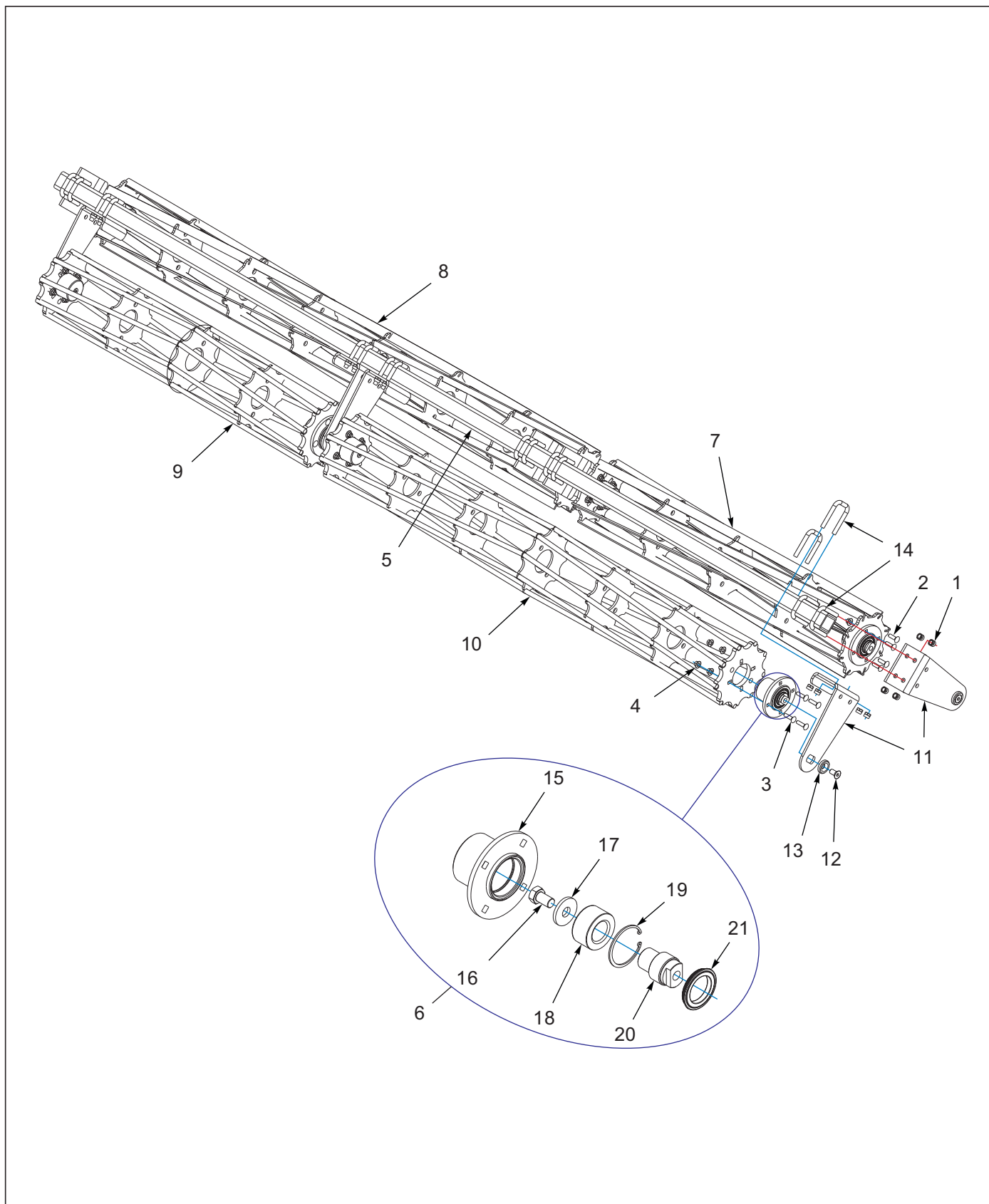
Figure 9-22: Double Flat/RD Reel Assembly 7531-32'-35' Center
