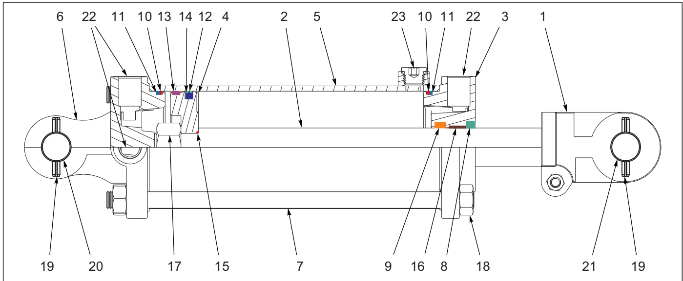
Figure 6-4: Cylinder Assembly 4-1/2 x 10 Rephase (Midway)
