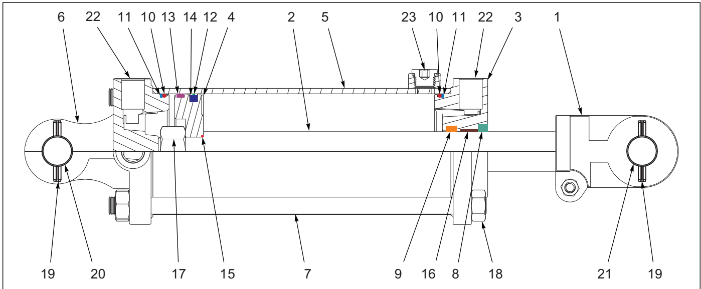
Figure 6-6: Cylinder Assembly 4-1/2 x 8 Rephase (Midway)
