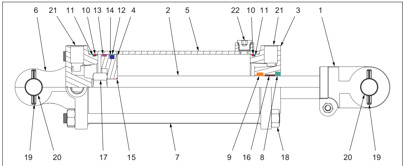
Figure 6-8: Cylinder Assembly 3-3/4 x 30 Rephase
