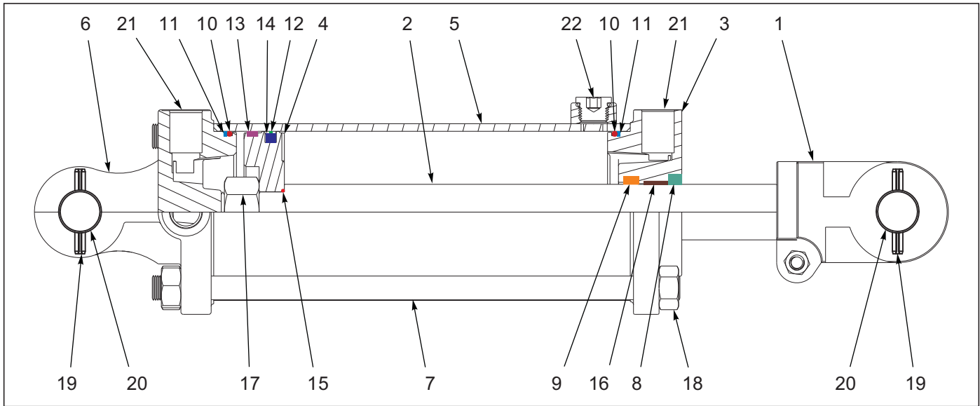
Figure 6-10: Cylinder Assembly 3-1/4 x 8 Rephase (Midway)
