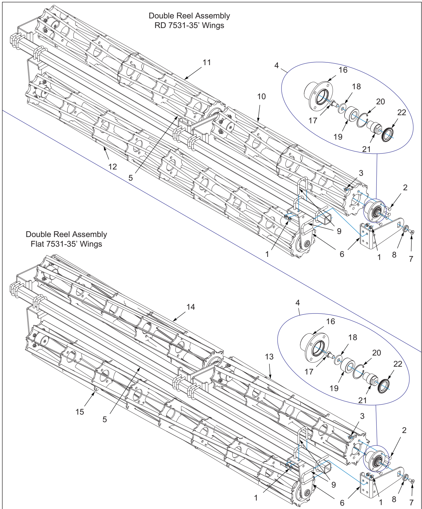
Figure 9-25: Double Reel Assembly 7531-35' Wings
