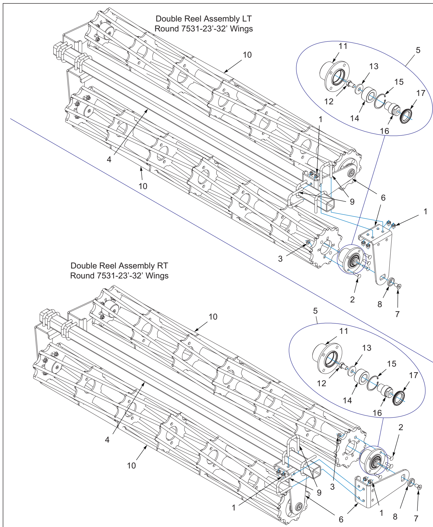
Figure 9-23: Double Round Reel Assembly 7531-23'-32' Wings
