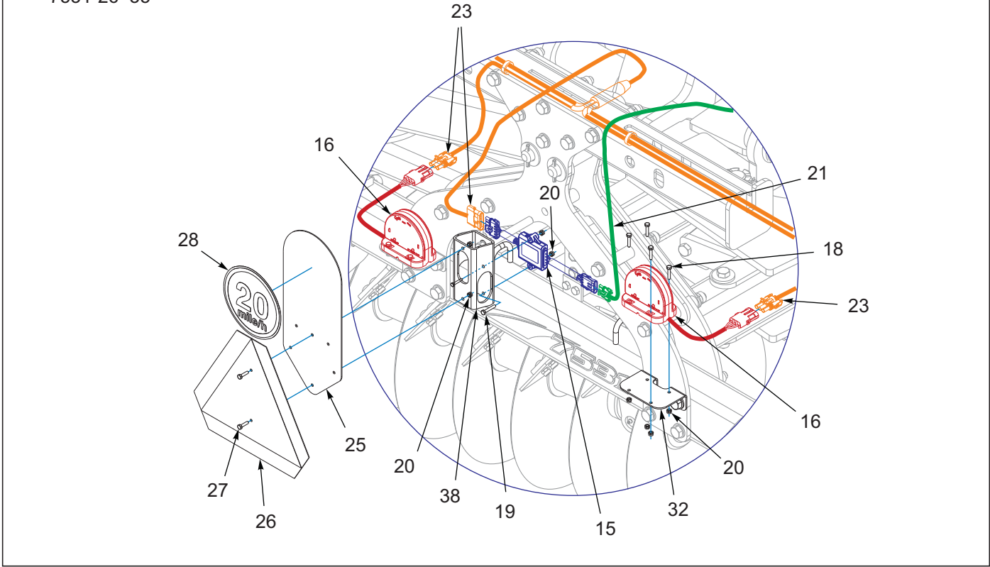
Figure 7-3: Electrical Assembly W/LED Lights (3 of 3)
