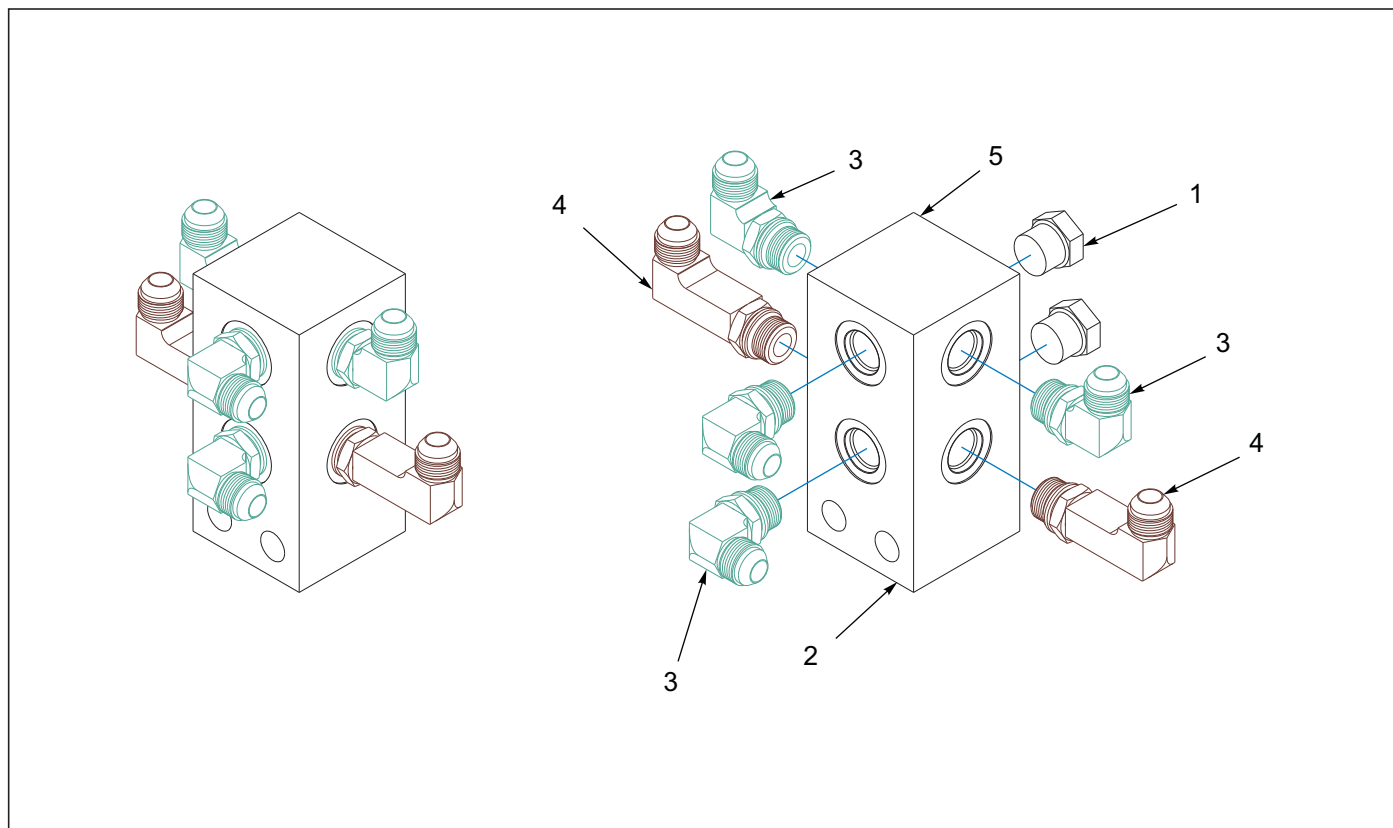
Figure 5-28: Manifold Assembly Rear 7531-32'-35' After
