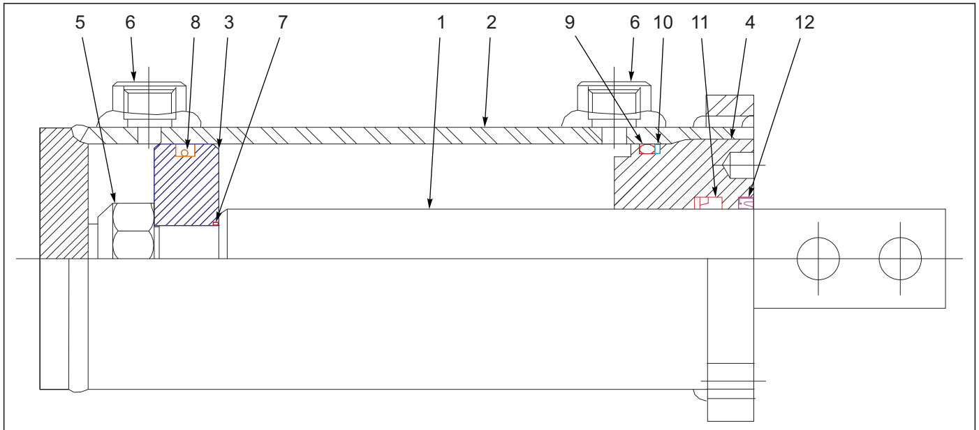
Figure 6-24: Cylinder Assembly 3-1/2 x 6
