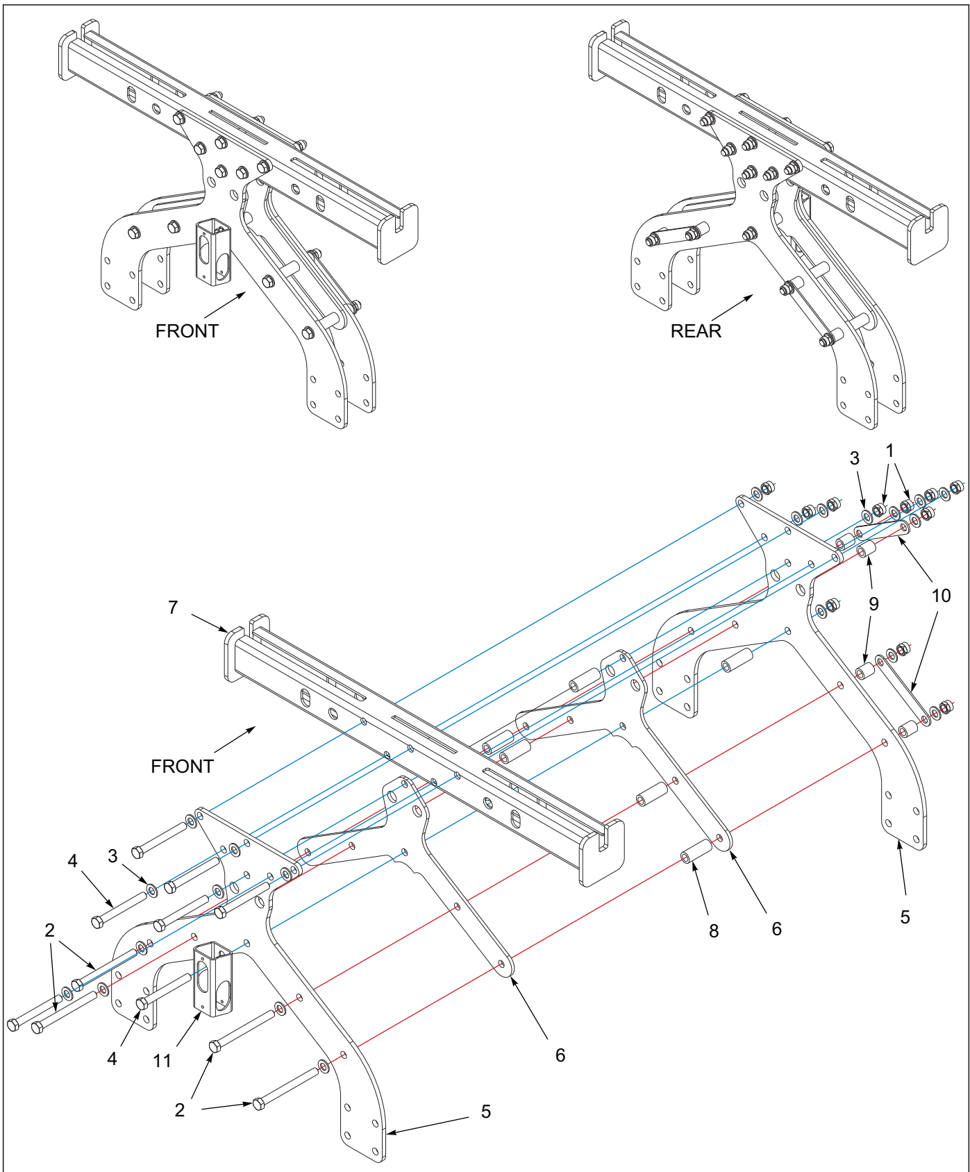
Figure 5-7: Wing Fold Stabilizer Assembly 7531-26'-29' Rear
