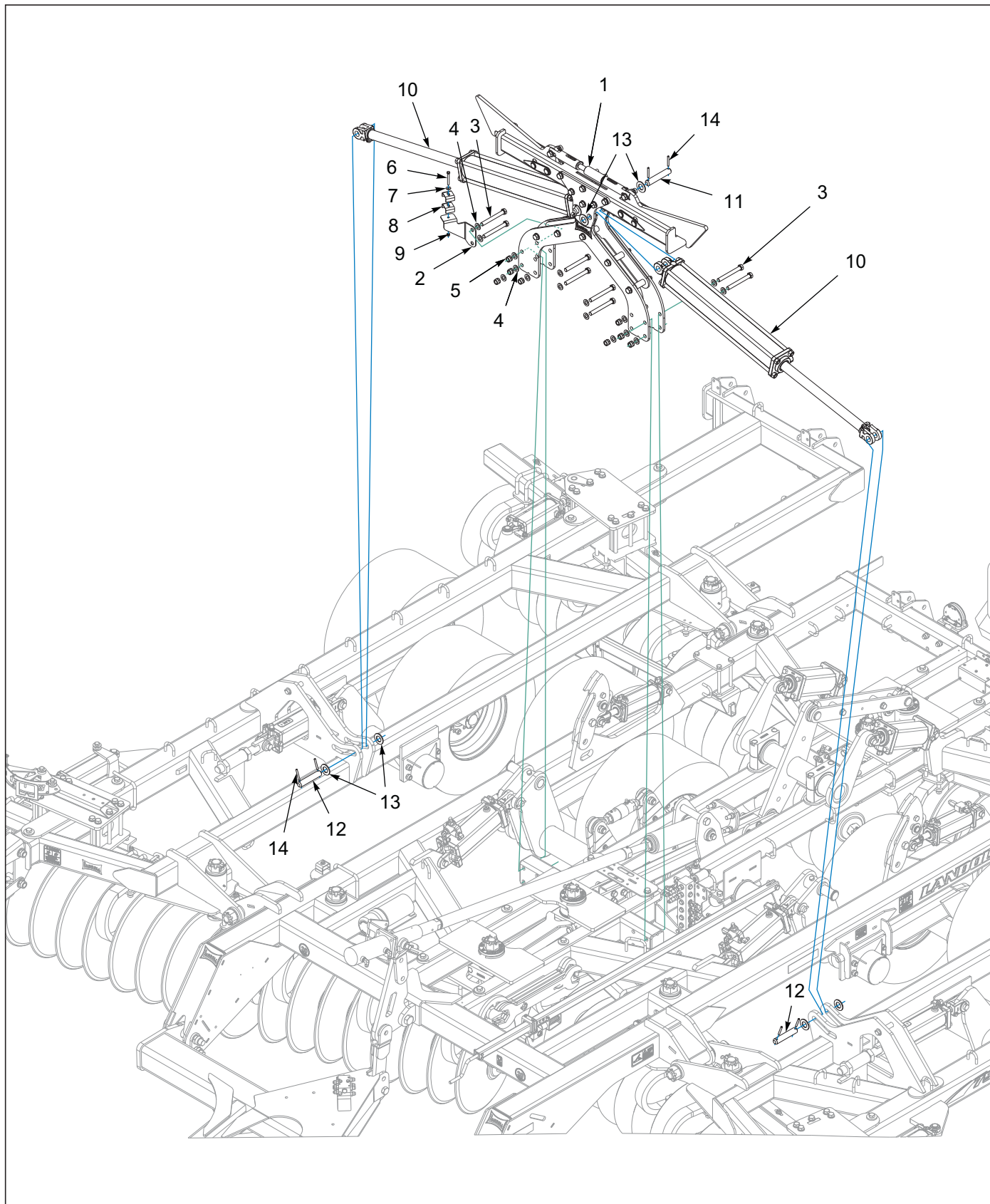
Figure 5-3: Fold Stabilizer Assembly 7531-23'
