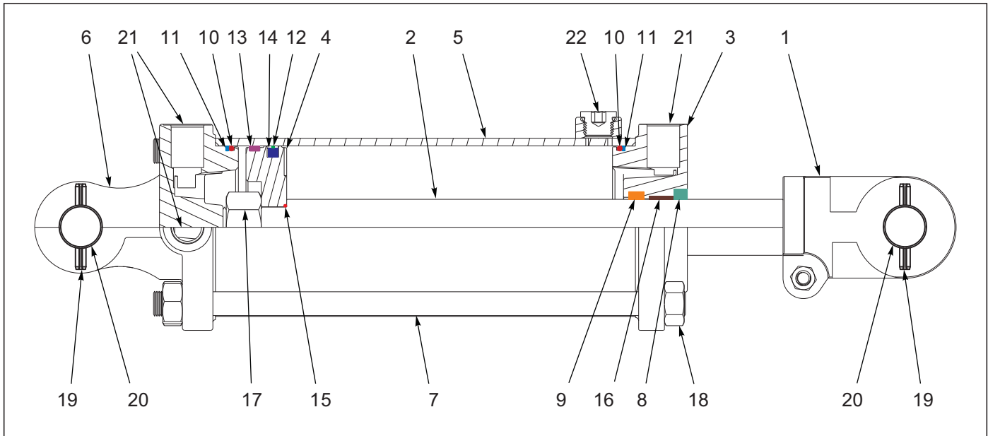
Figure 6-16: Cylinder Assembly 3-1/2 x 8, Rephase (Midway)
