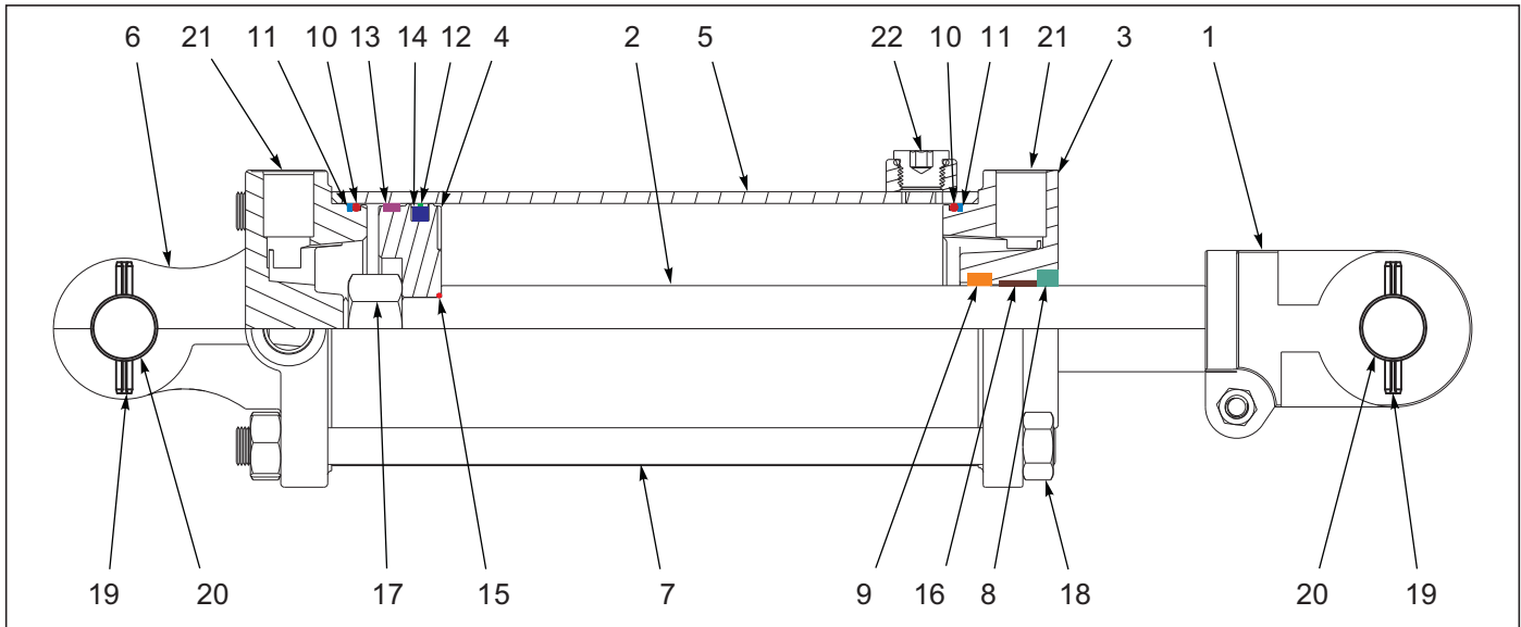
Figure 6-12: Cylinder Assembly 3-1/2 x 8 Rephase (Midway)
