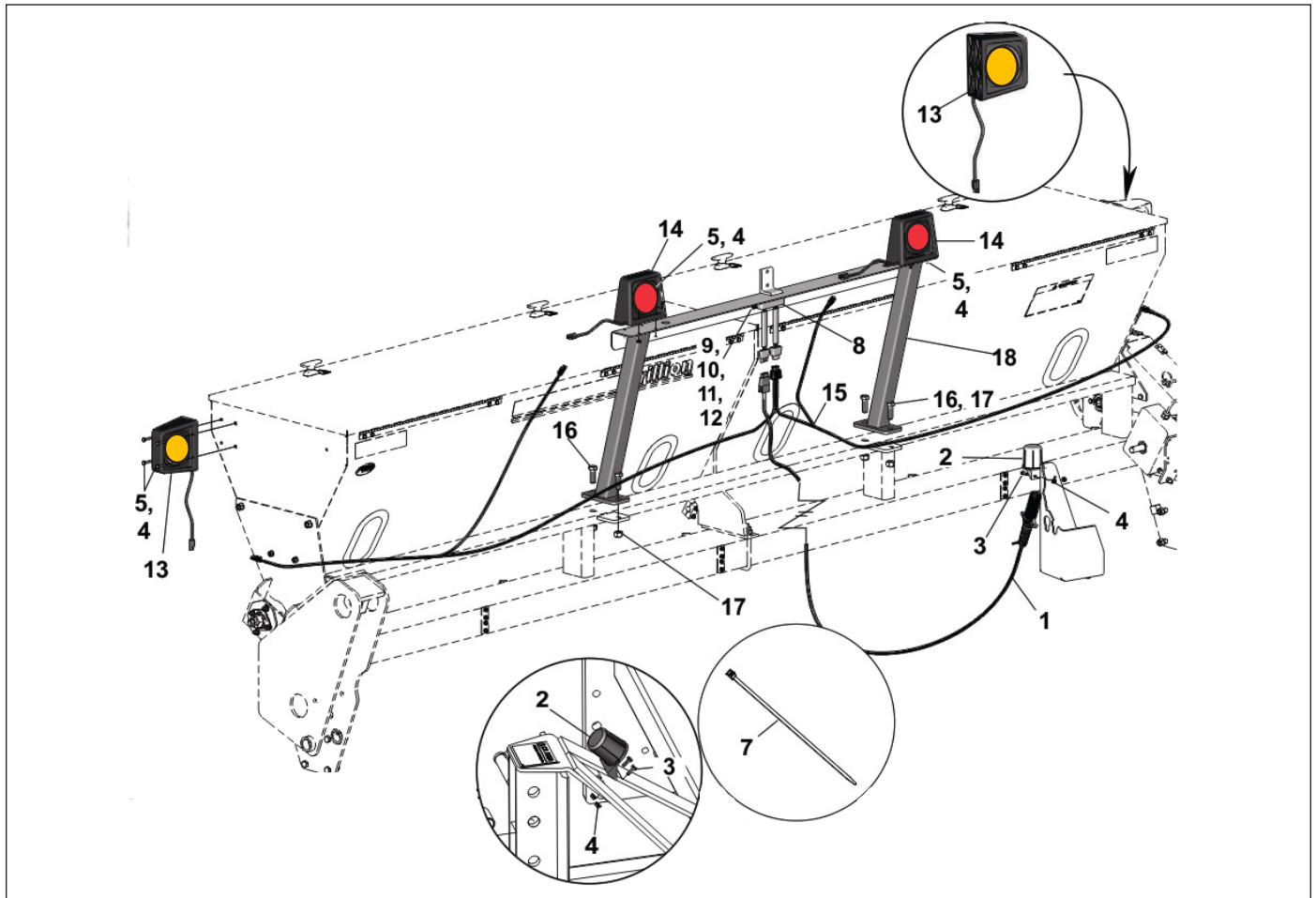
Figure 1-39: Warning Lamp Kit, 12FT (BEFORE 09/2013)
