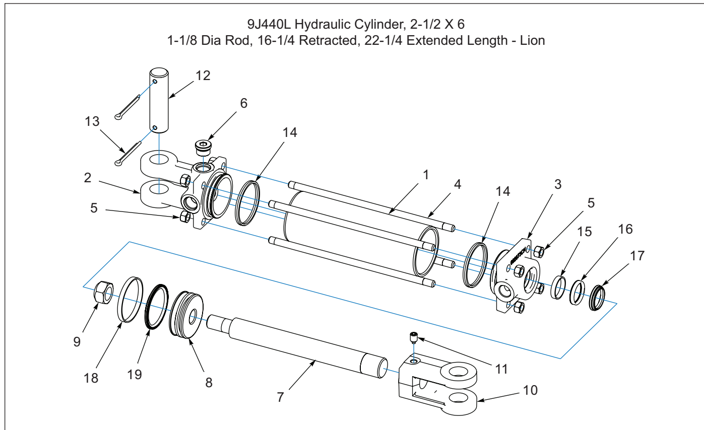
Figure 1-57: Hydraulic Cylinder, 2-1/2 x 6 - Lion (AFTER 01/15/2008)
