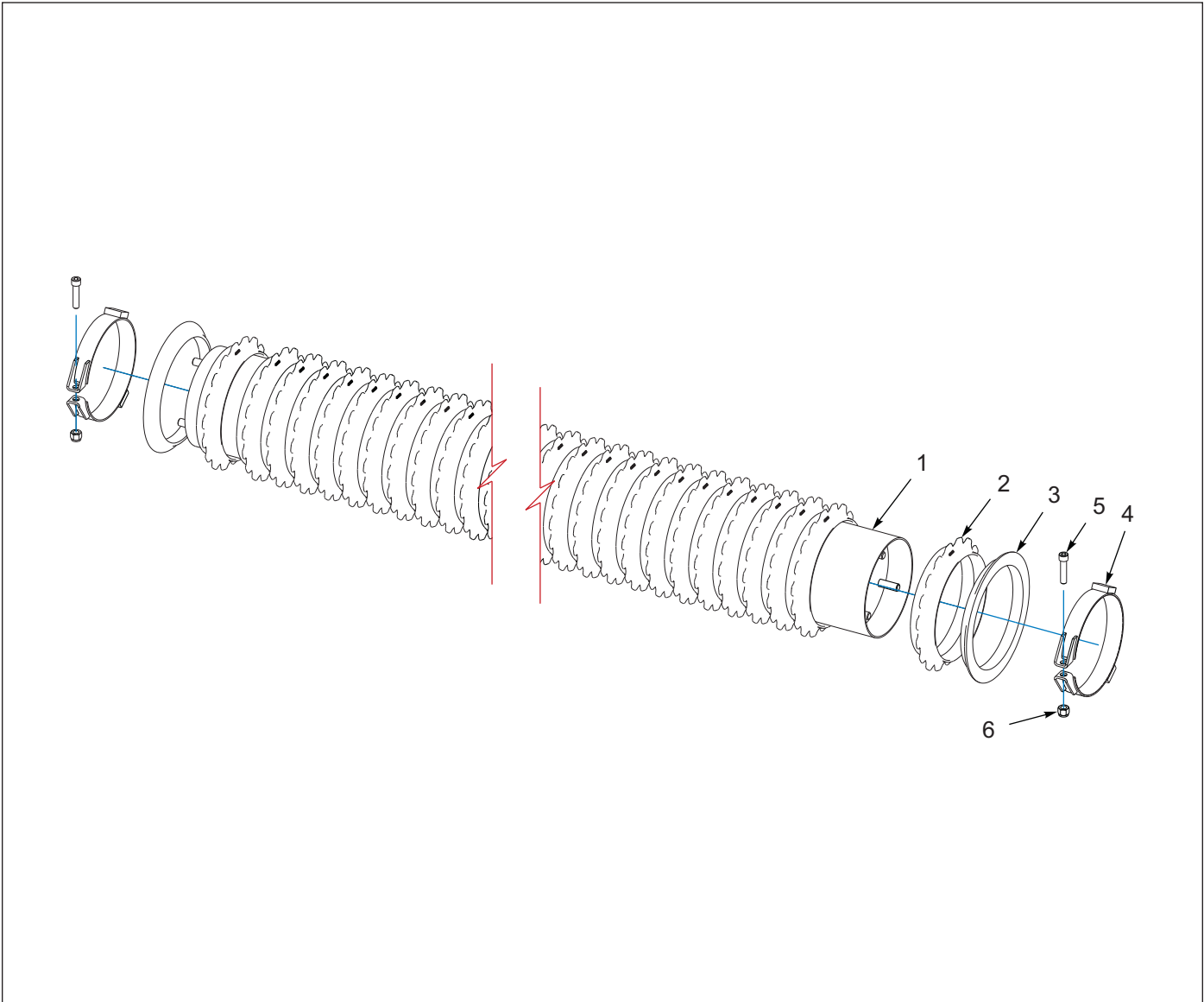
Figure 1-20: Rear Roller Assembly
