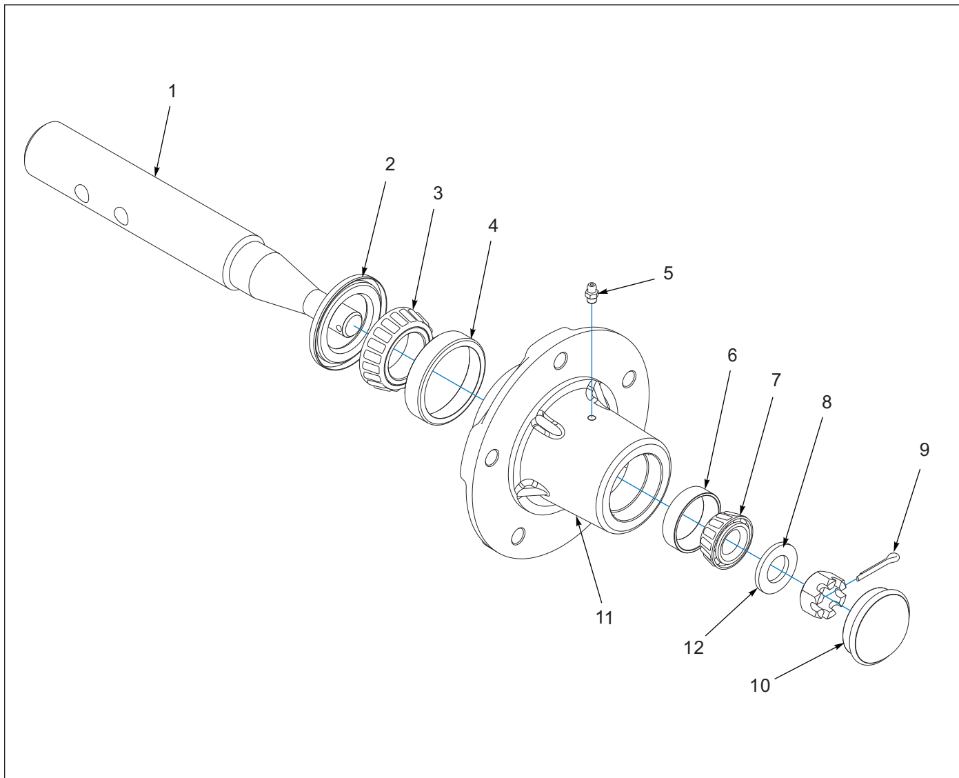
Figure 1-11: Hub and Spindle Assembly - 5 Bolt (BEFORE 05/2021)
