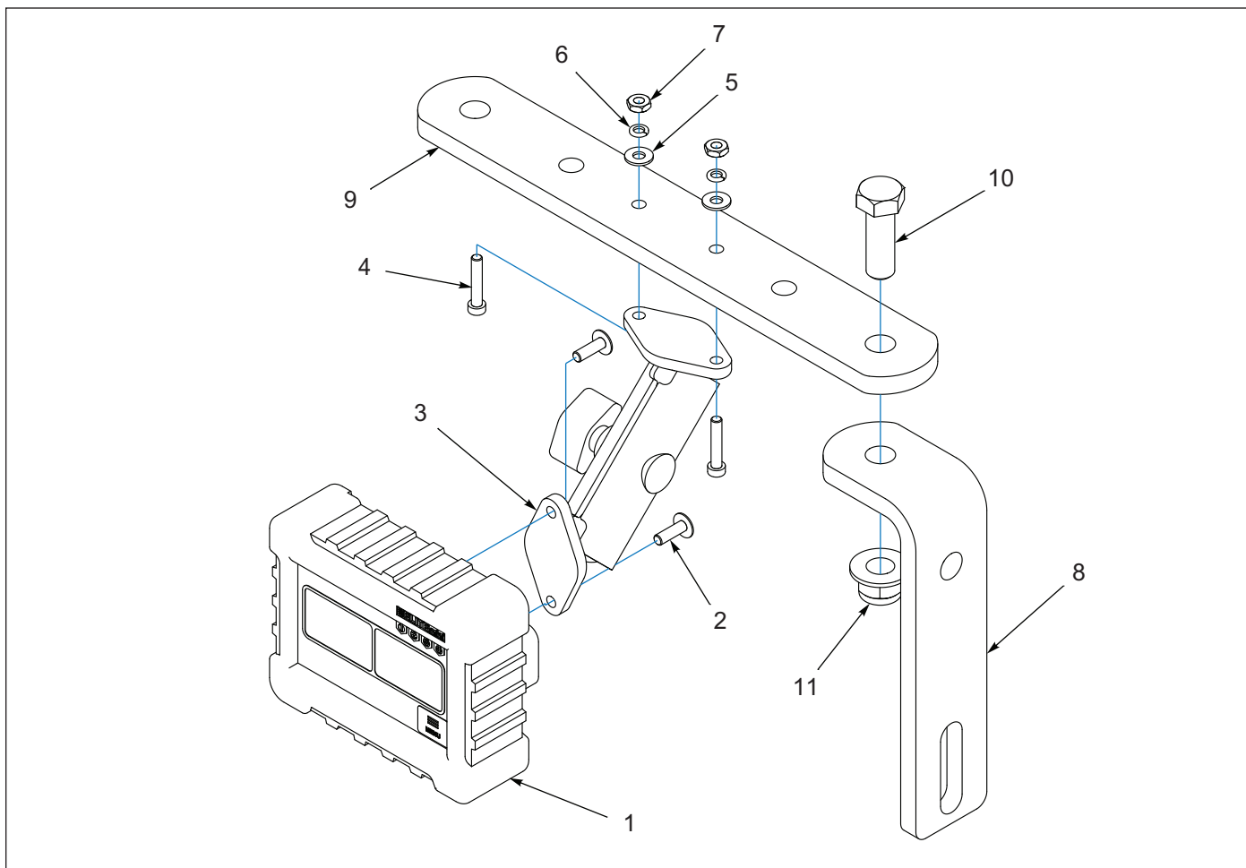
Figure 1-51: Brillion Elite Mini Monitor Tractor Mount
