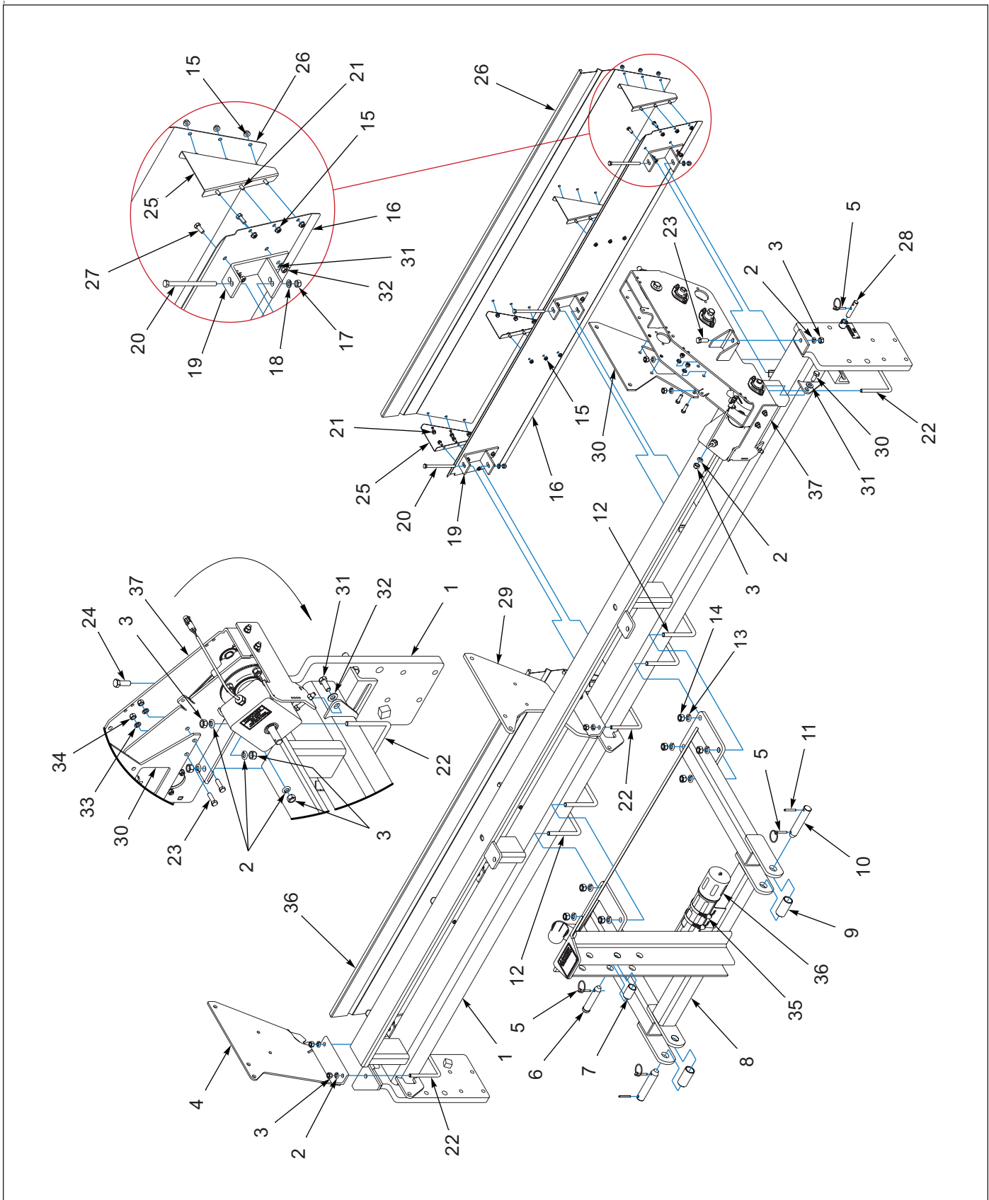
Figure 1-7: 3-PT - Frame, Deflectors, Seed box Mounts - 12FT (AFTER 03/2012)
