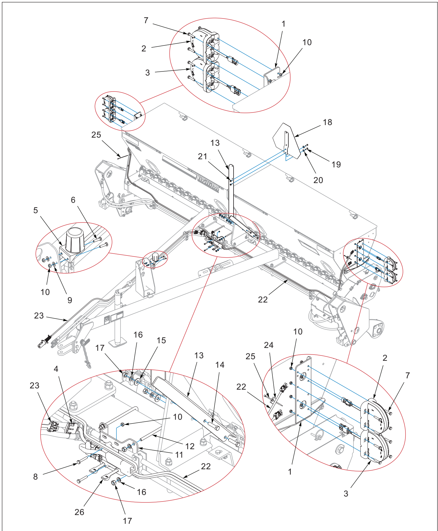
Figure 1-36: LED Warning Lamps, 8FT and 10FT (AFTER 09/2013)
