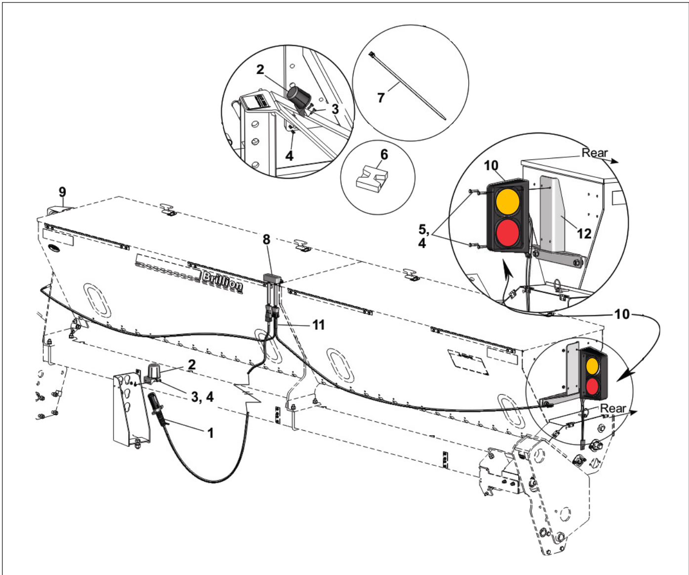
Figure 1-38: Warning Light Kit, 8FT and 10FT (BEFORE 09/2013)
