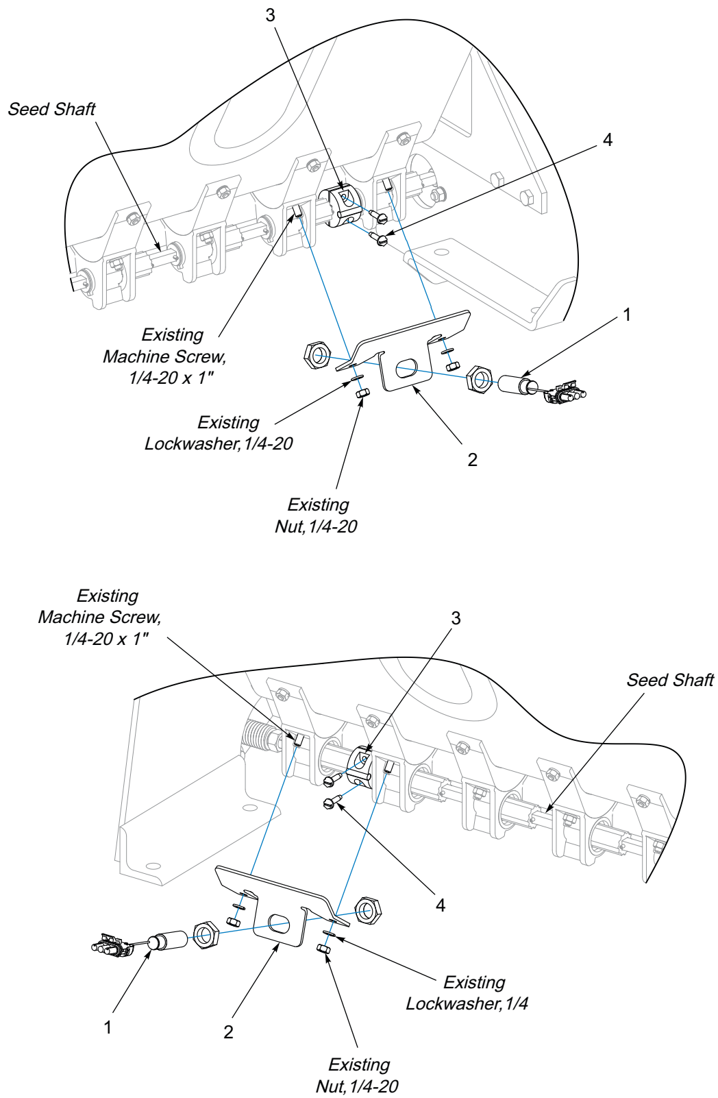
Figure 1-55: Console w/Clutch Control - Seed Shaft Sensor
