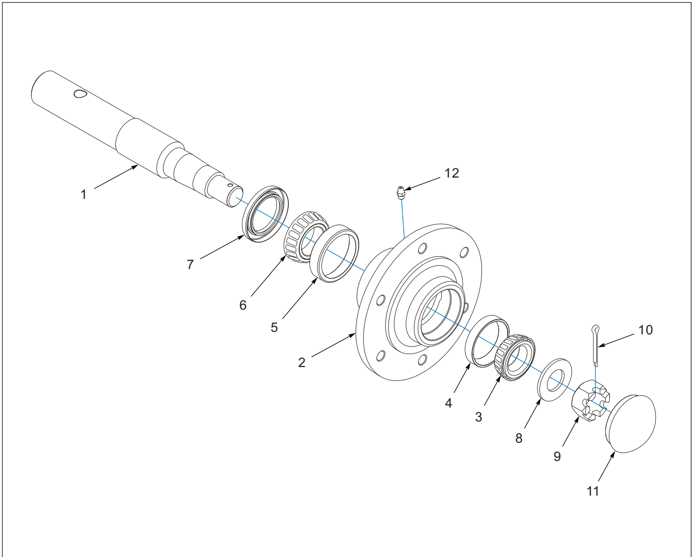
Figure 1-10: Hub and Spindle Assembly - 6 Bolt (AFTER 05/2021)
