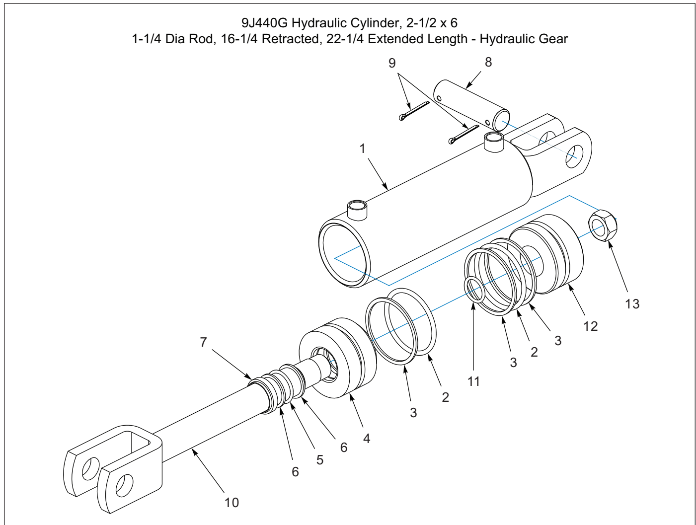
Figure 1-58: Hydraulic Cylinder, 2-1/2 x 6 - Hydraulic Gear (BEFORE 01/14/2008)
