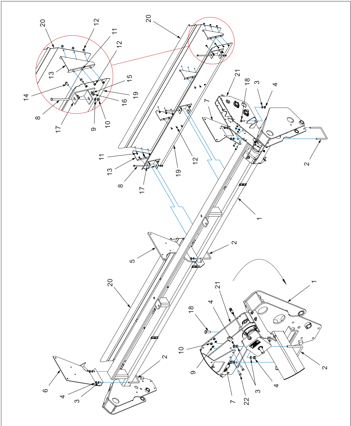
Figure 1-3: Drawbar Frame, Deflectors, Seed Box Mounts - 12FT (AFTER 03/2012)
