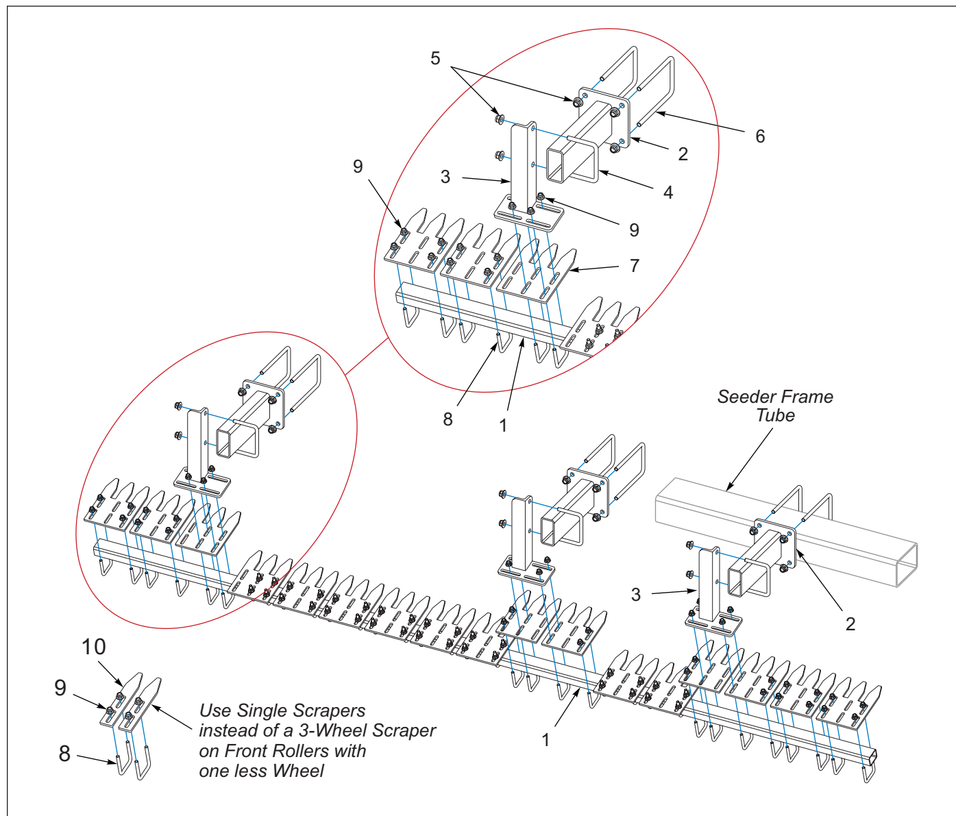
Figure 1-41: Scraper Kit, 10FT Tube Mounted - Optional
