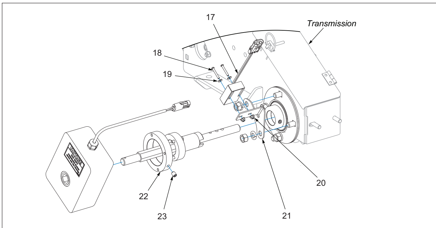
Figure 1-52: Brillion Elite Mini Monitor by Loup - Ground Speed
