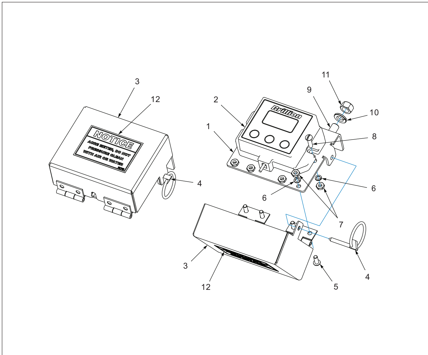
Figure 1-49: Acre Meter Assembly (BEFORE 05/15/2012)
