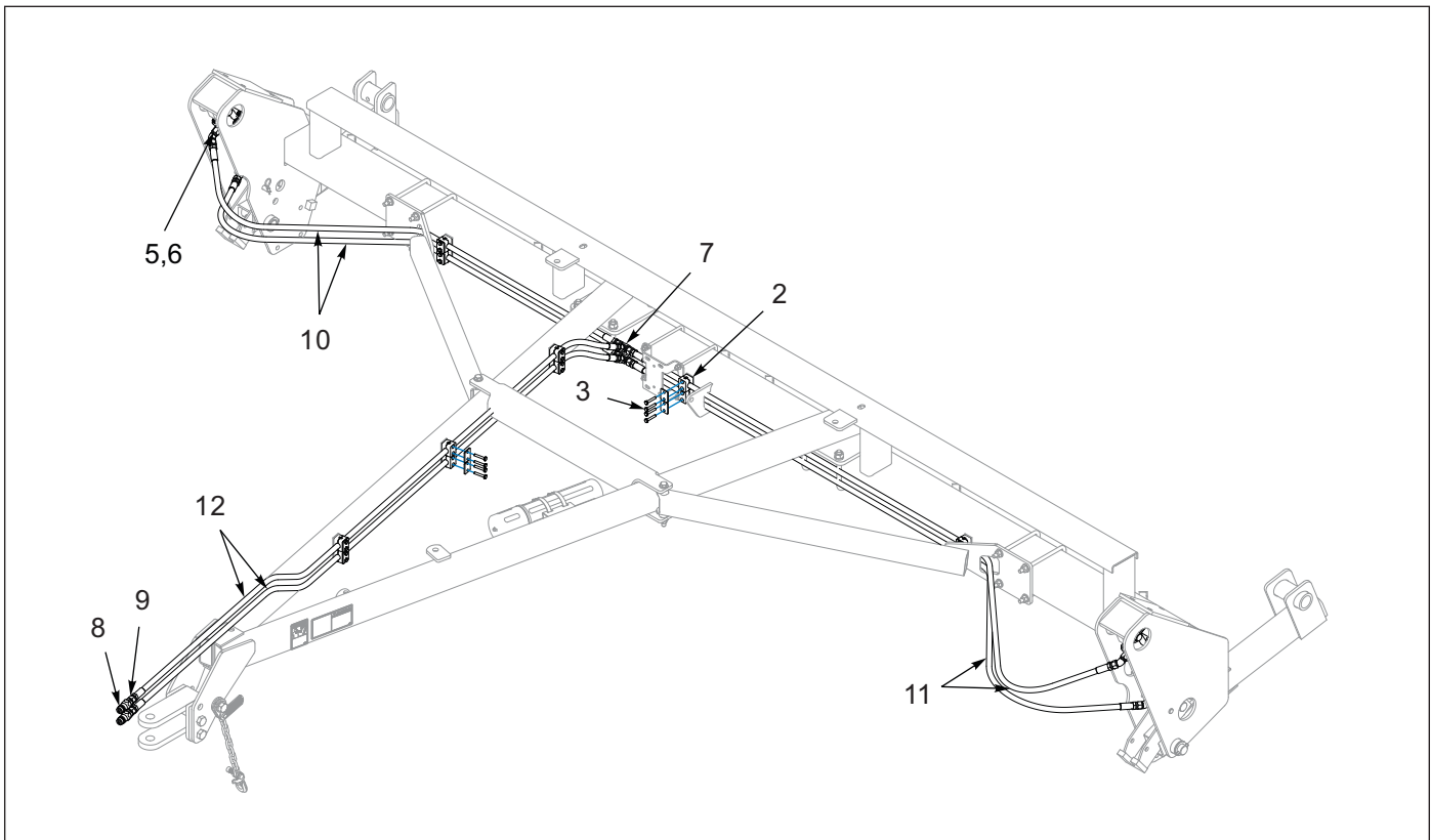
Figure 1-15: Hydraulic Layout - 12FT
