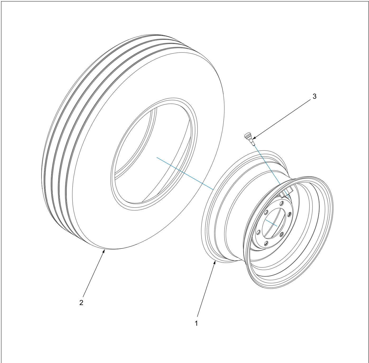
Figure 1-12: Tire and Wheel Assembly - 6 Bolt (AFTER 05/2021)
