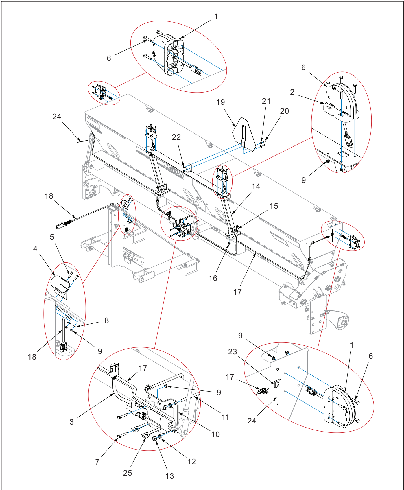
Figure 1-37: LED Warning Lamps, 12FT (AFTER 09/2013)
