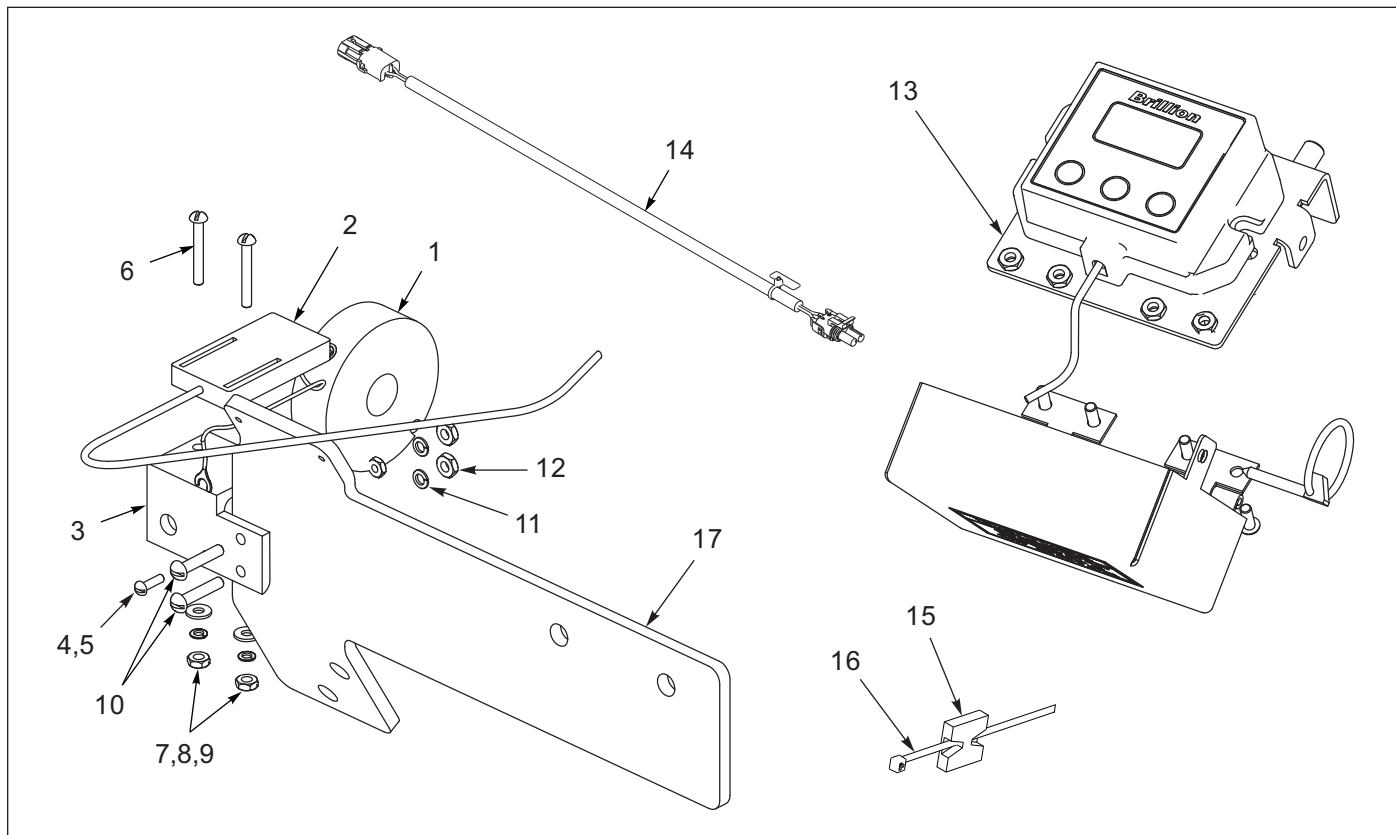
Figure 1-46: Electronic Acre Meter Kit with Clutch - Optional
