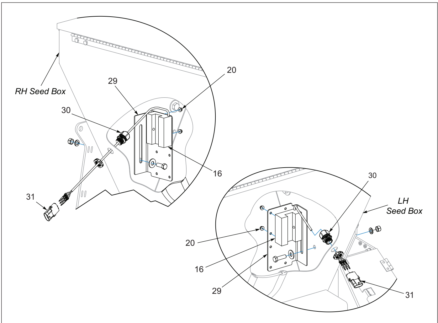
Figure 1-54: Brillion Elite Mini Monitor - Bin Level Sensor
