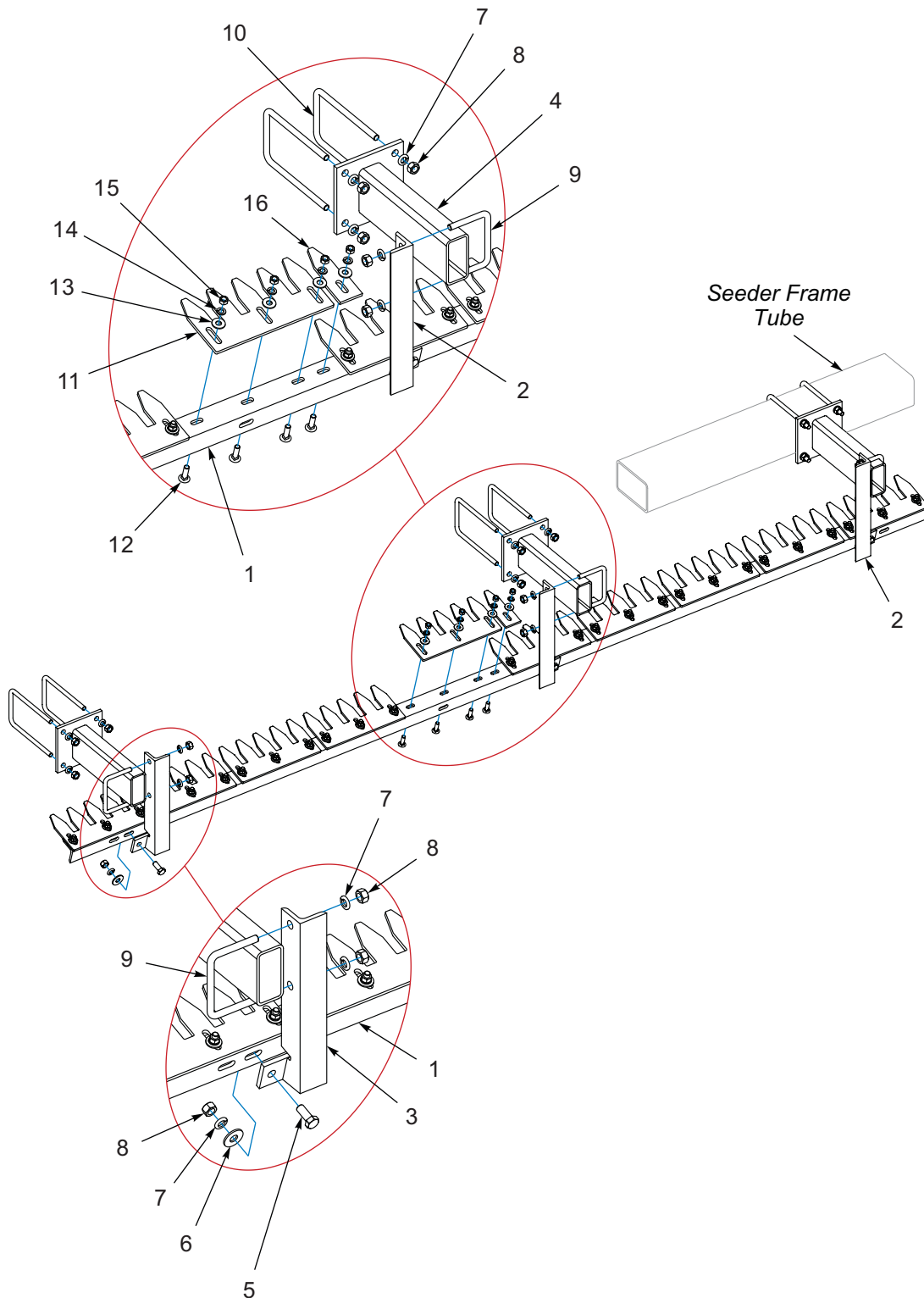
Figure 1-43: Scraper Kit, Angle Mounted - Optional
