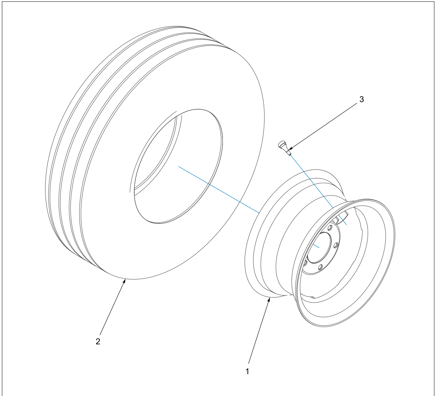
Figure 1-13: Tire and Wheel Assembly - 5 Bolt (BEFORE 05/2021)
