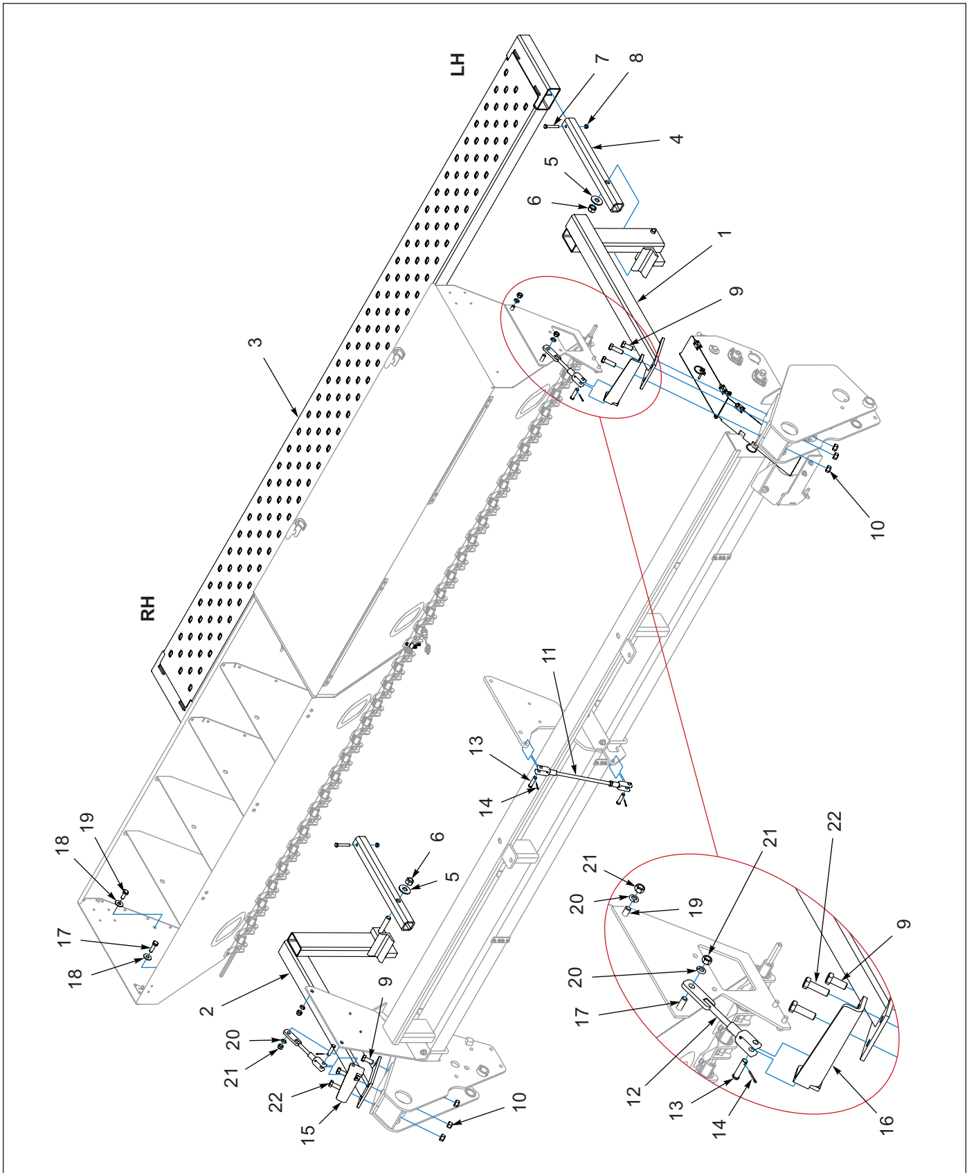
Figure 1-27: Drawbar Walk Board - 12FT
