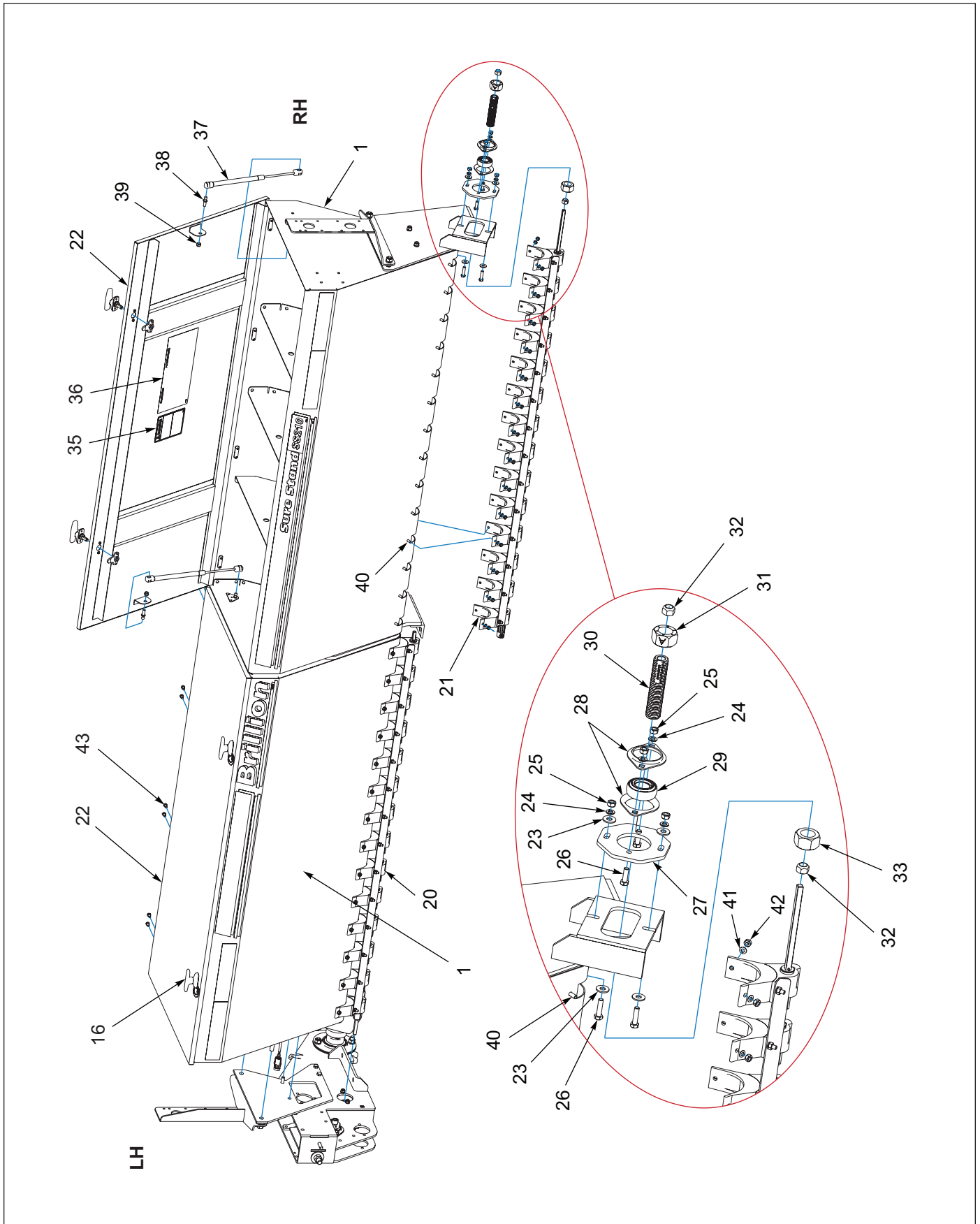
Figure 1-33: Seed Box and Mounting Brackets (2 of 2)
