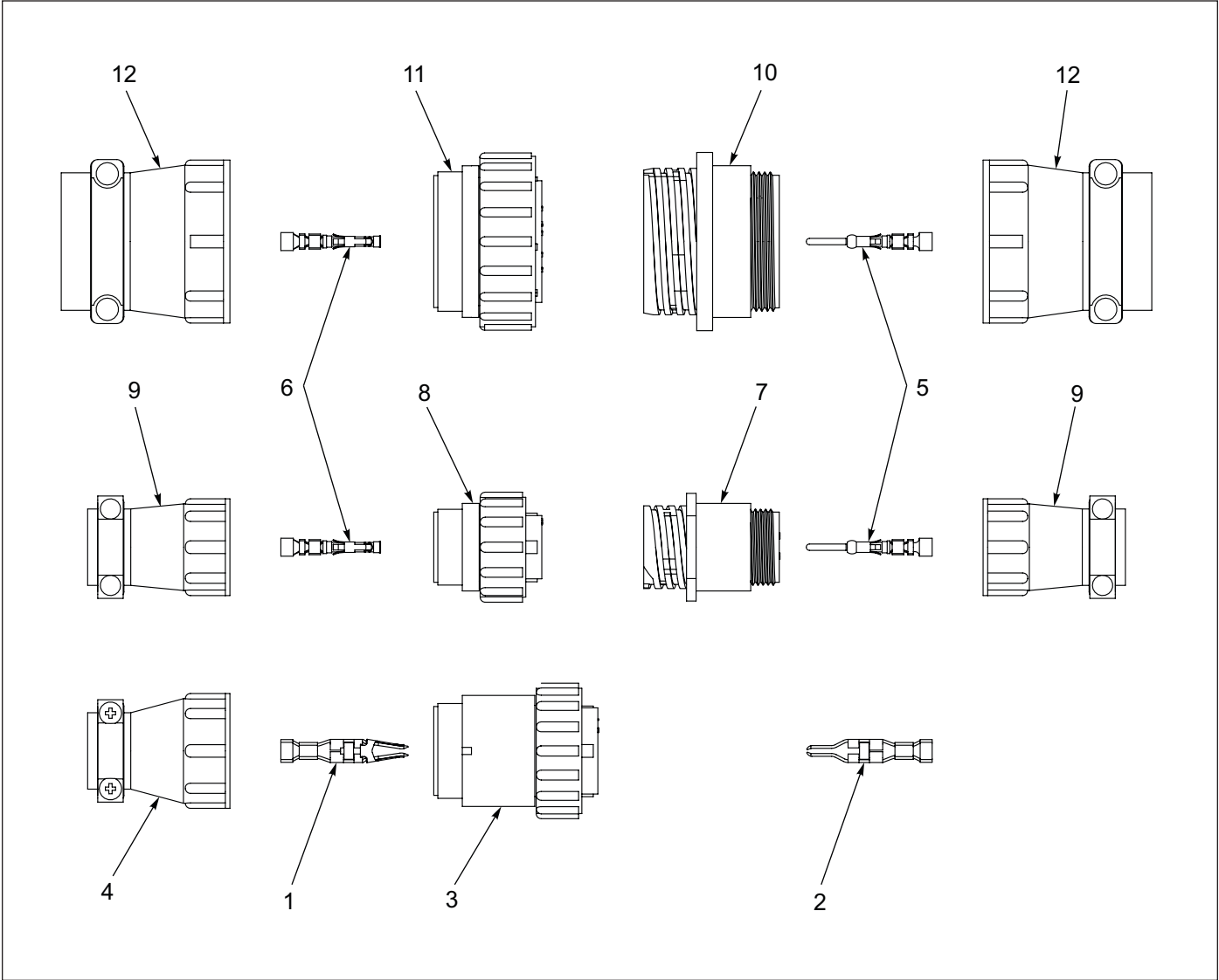
Figure 1-60: AMP Connectors
