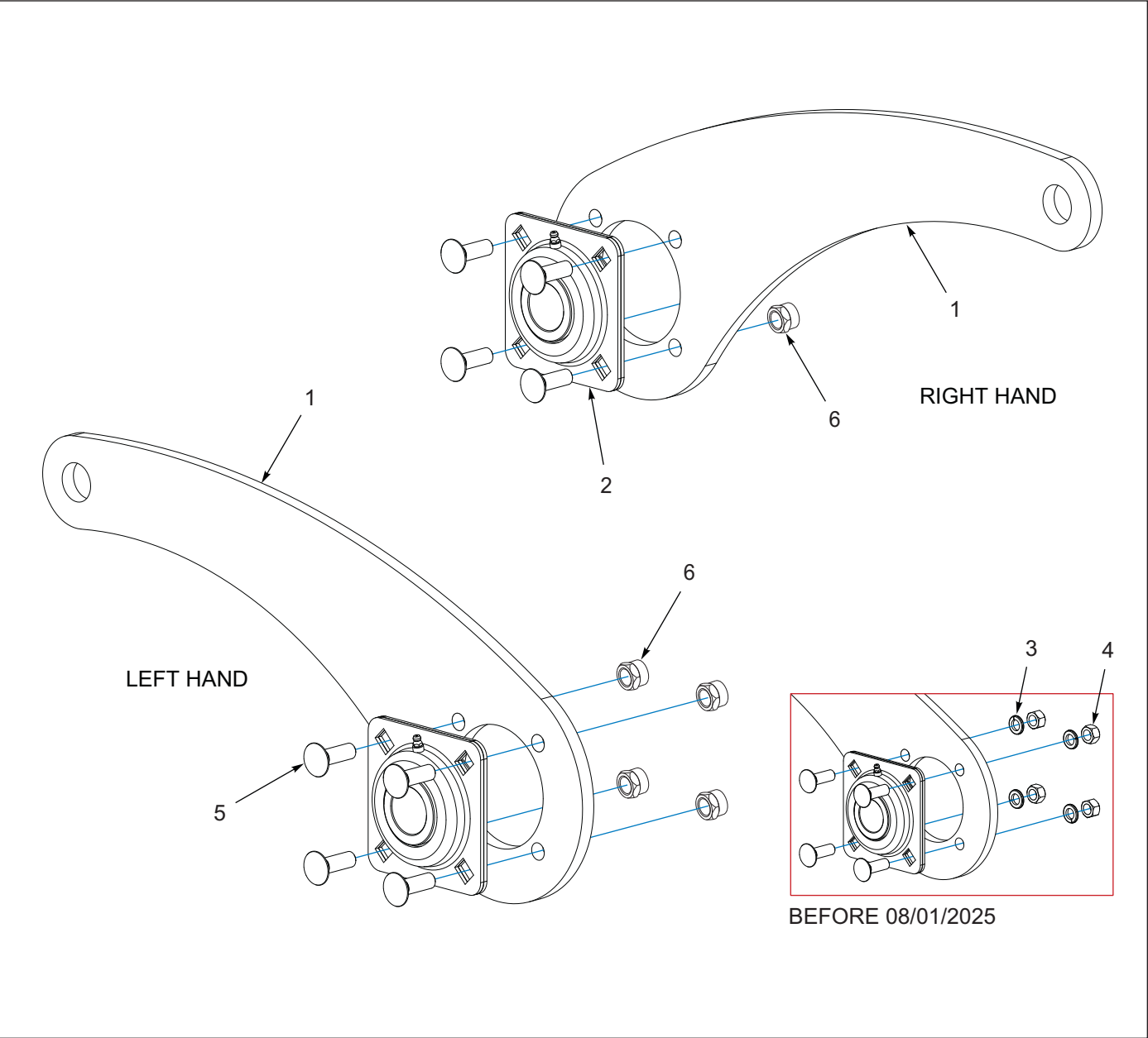
Figure 1-21: Rear Arm Assemblies
