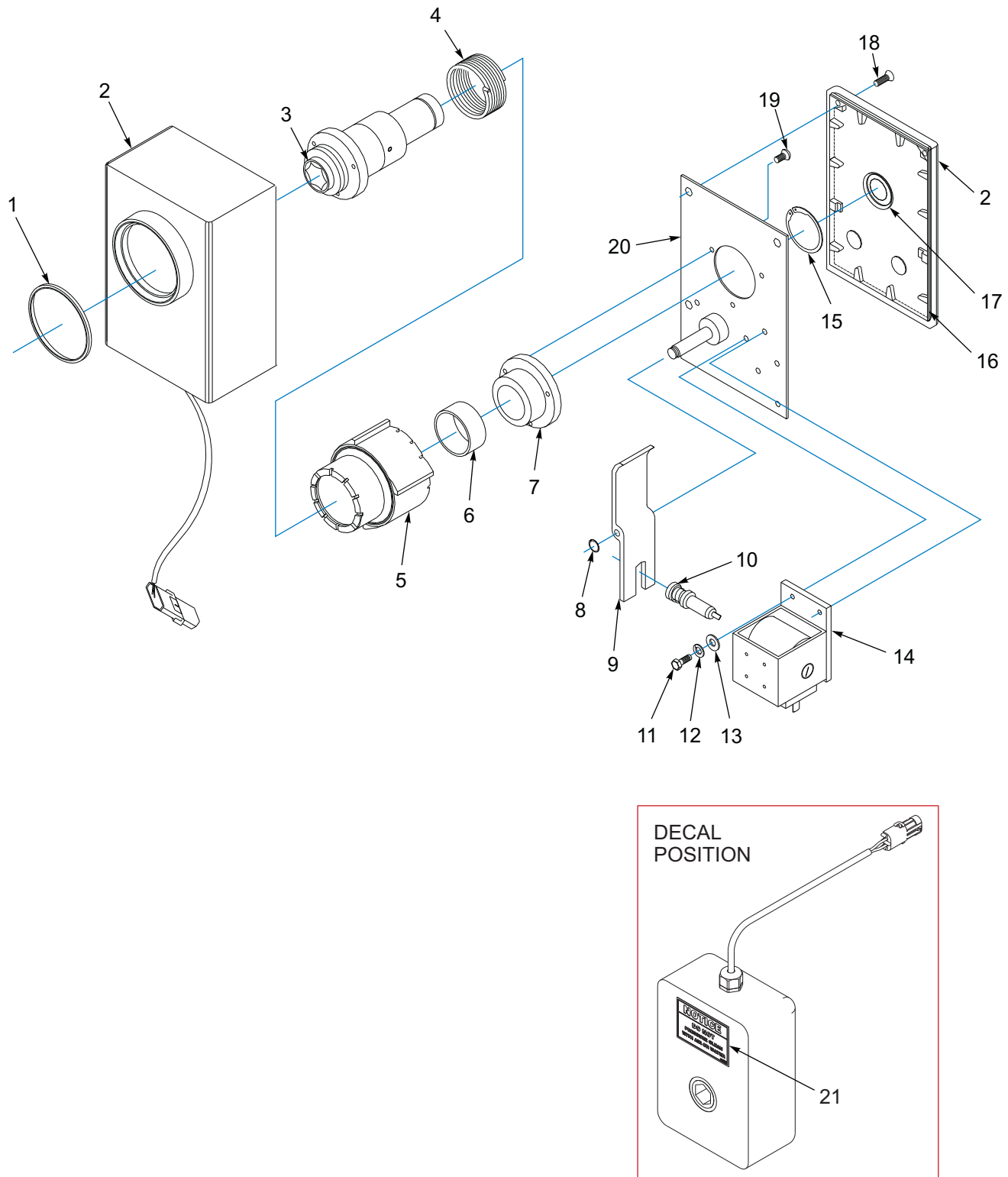
Figure 1-24: Electric Clutch
