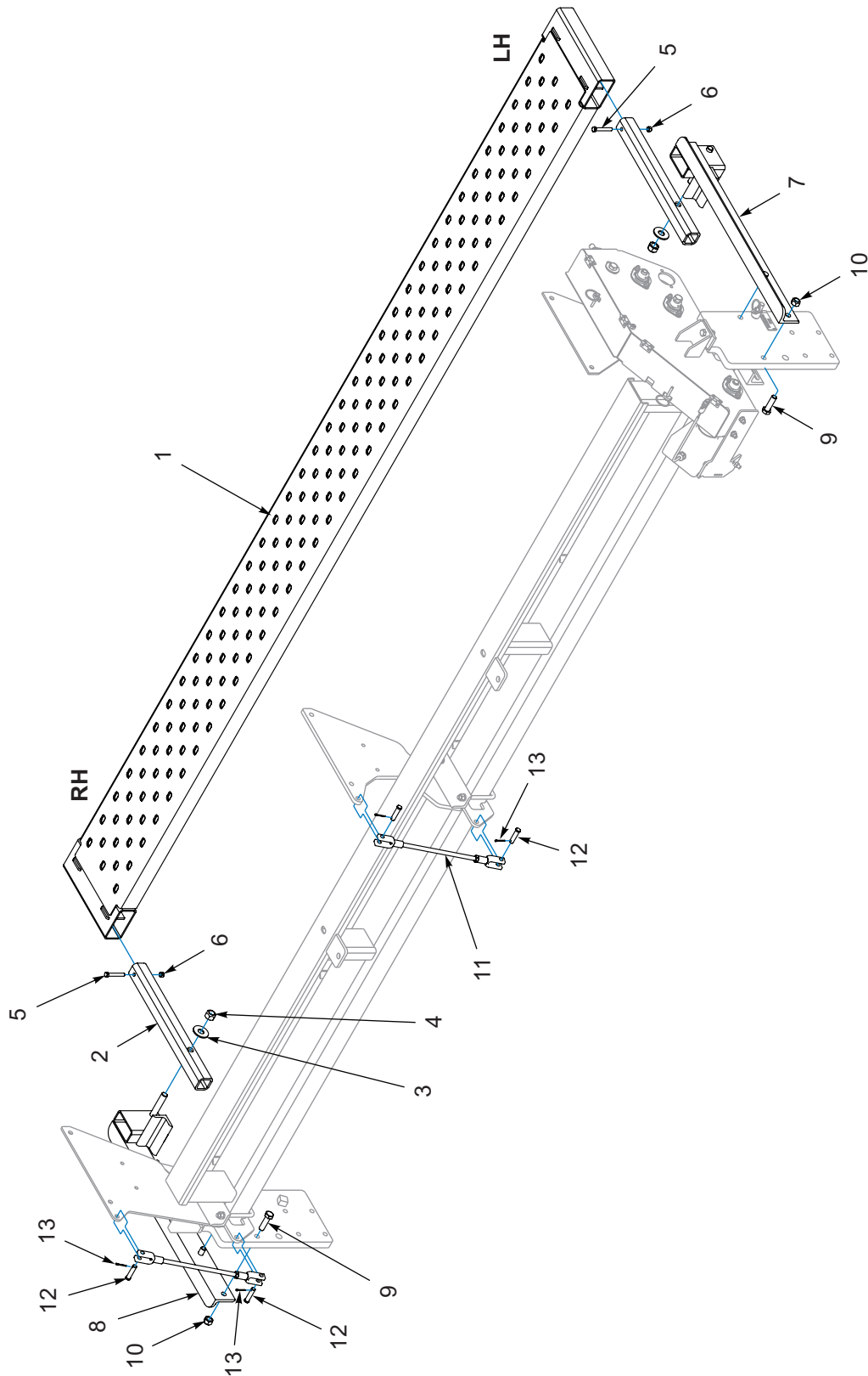
Figure 1-29: 3-PT Walk Board - 12FT
