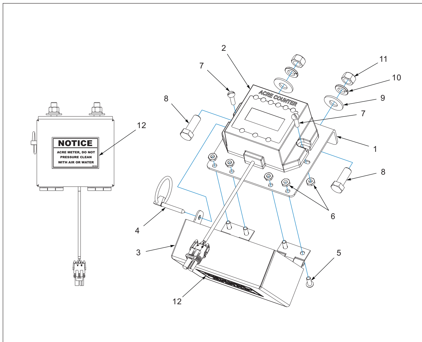
Figure 1-48: Acre Meter Assembly (05/15/2012 TO 06/01/2025)
