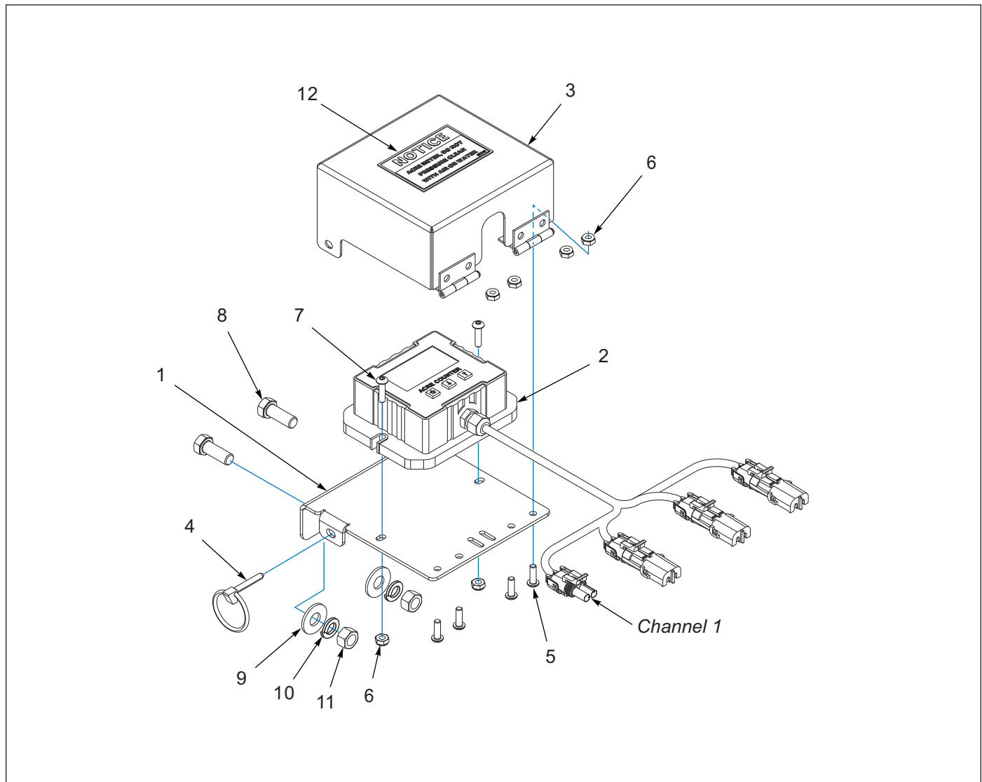
Figure 1-47: Acre Meter Assembly (AFTER 06/01/2025)
