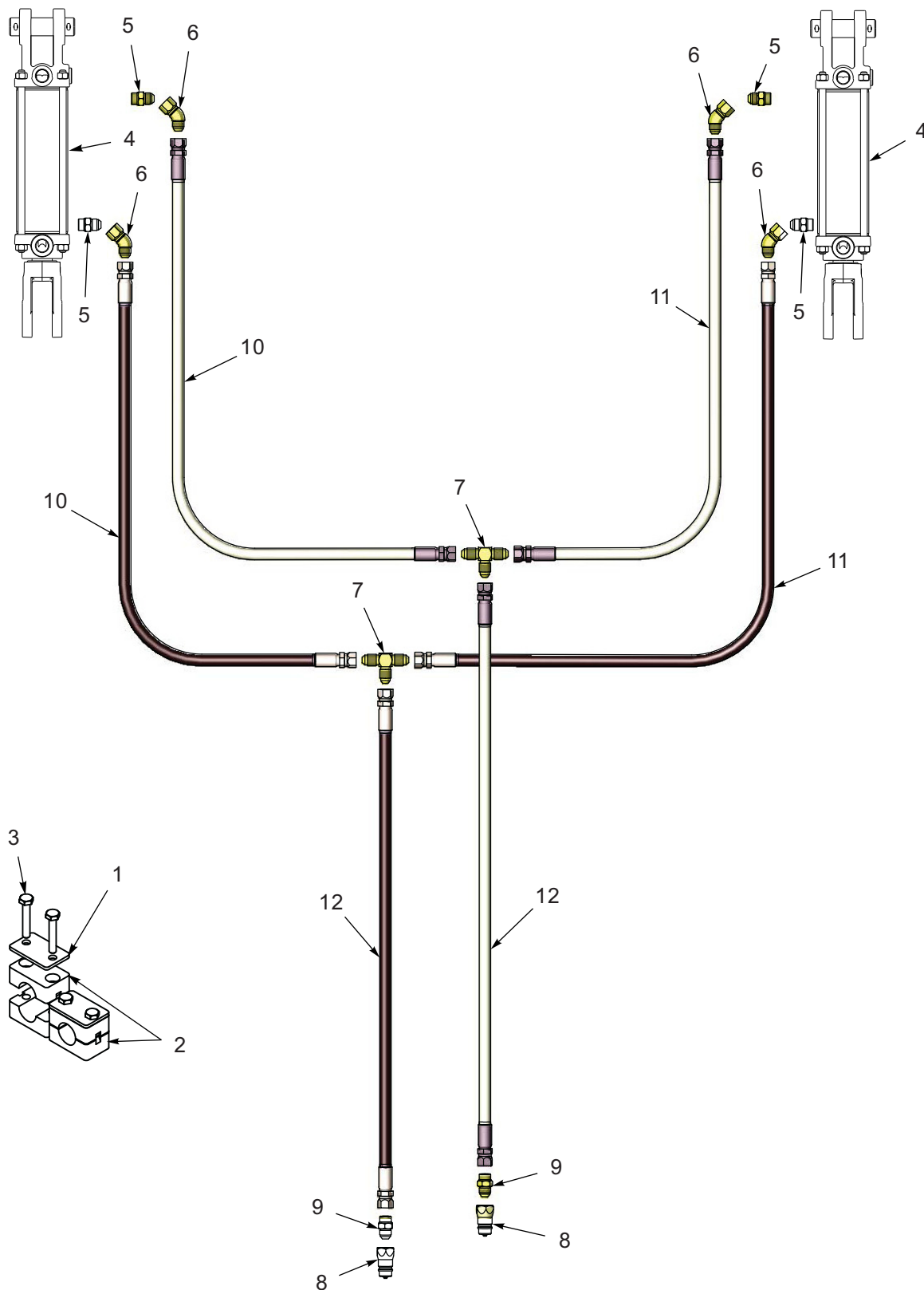
Figure 1-16: Hydraulic Schematic
