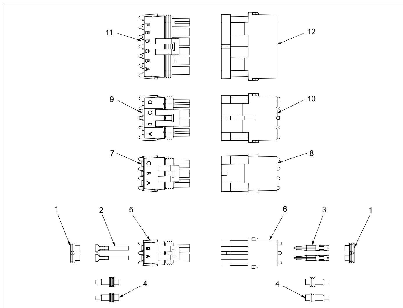
Figure 1-59: Weather Pack Connectors
