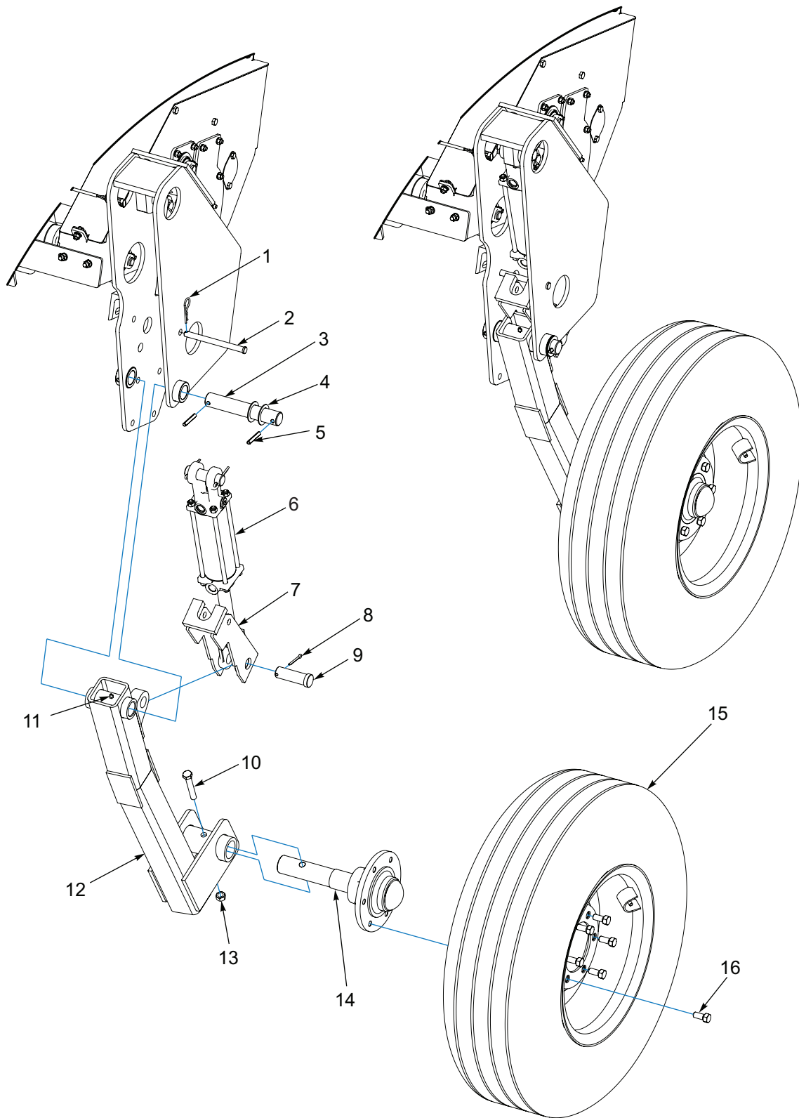
Figure 1-9: Wheel Arm Assembly
