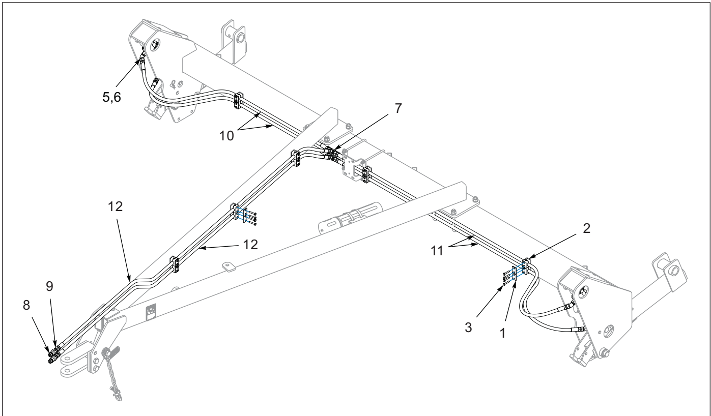
Figure 1-14: Hydraulic Layout - 8FT and 10FT
