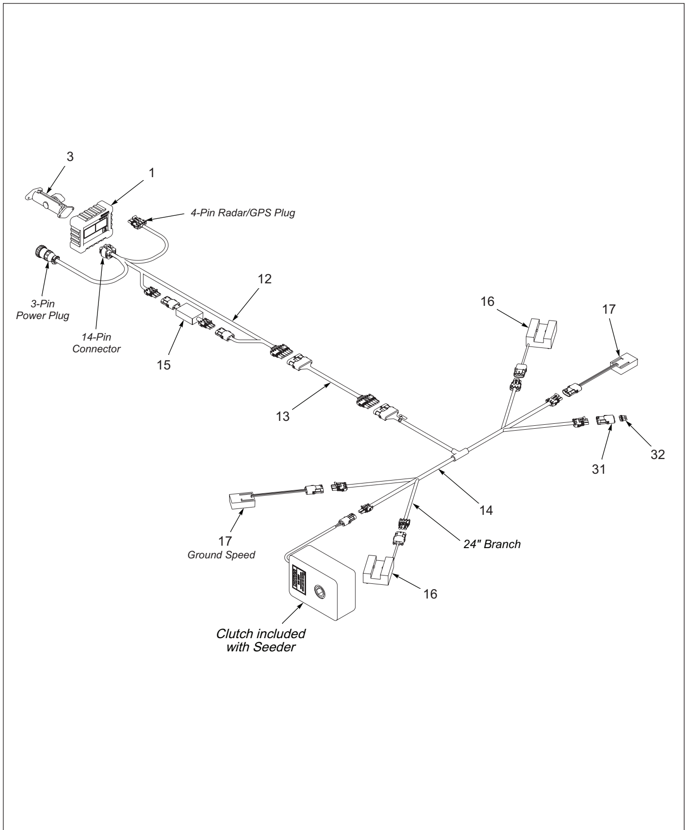
Figure 1-50: Brillion Elite Mini Monitor Electrical Schematic
