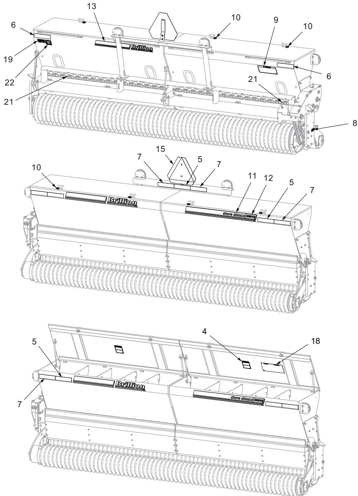
Figure 1-64: Decal Placement, 12FT
