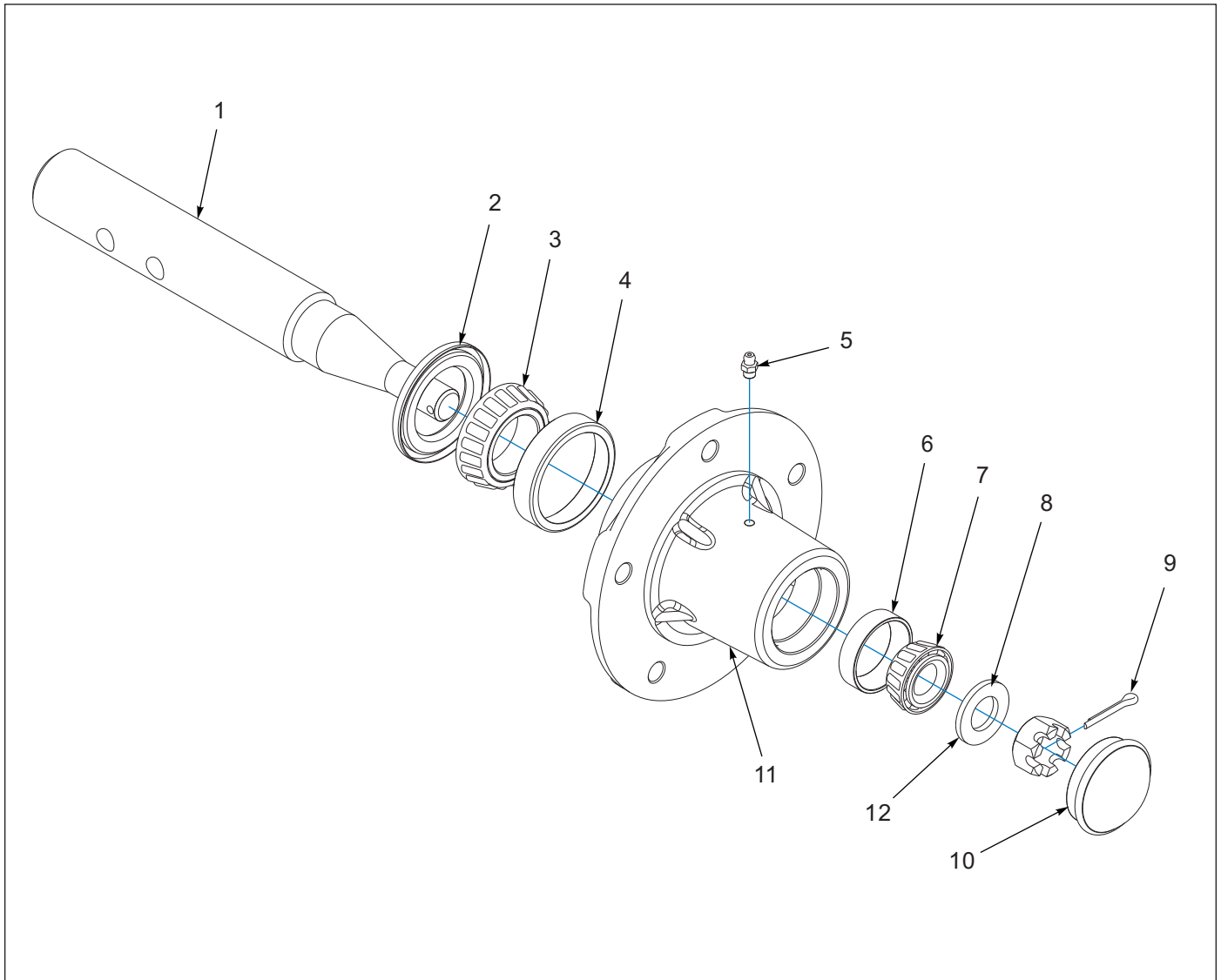
Figure 1-12: Hub and Spindle Assembly - 5 Bolt (BEFORE 05/2021)
