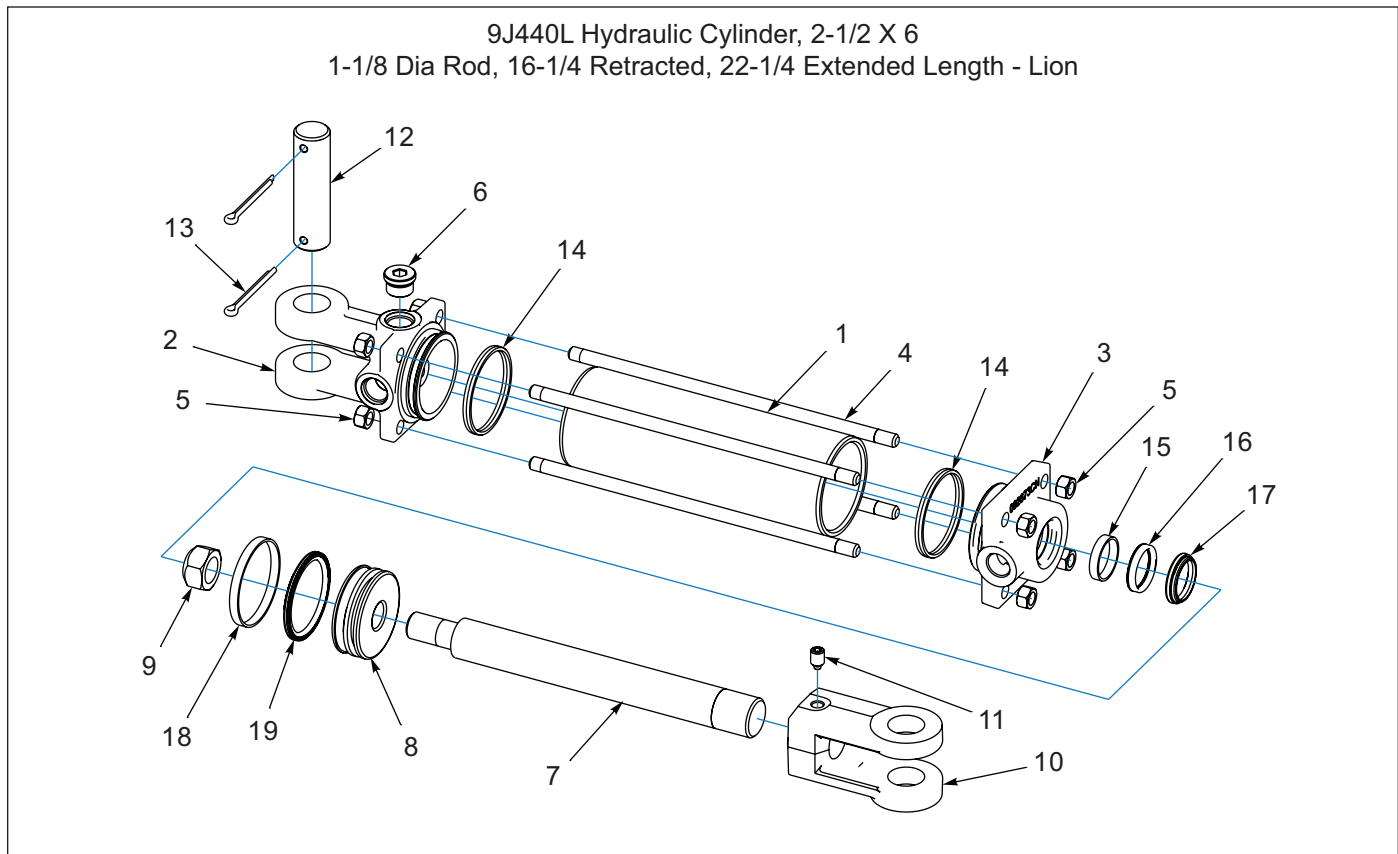
Figure 1-62: Hydraulic Cylinder, 2-1/2 x 6 - Lion (AFTER 01/15/2008)
