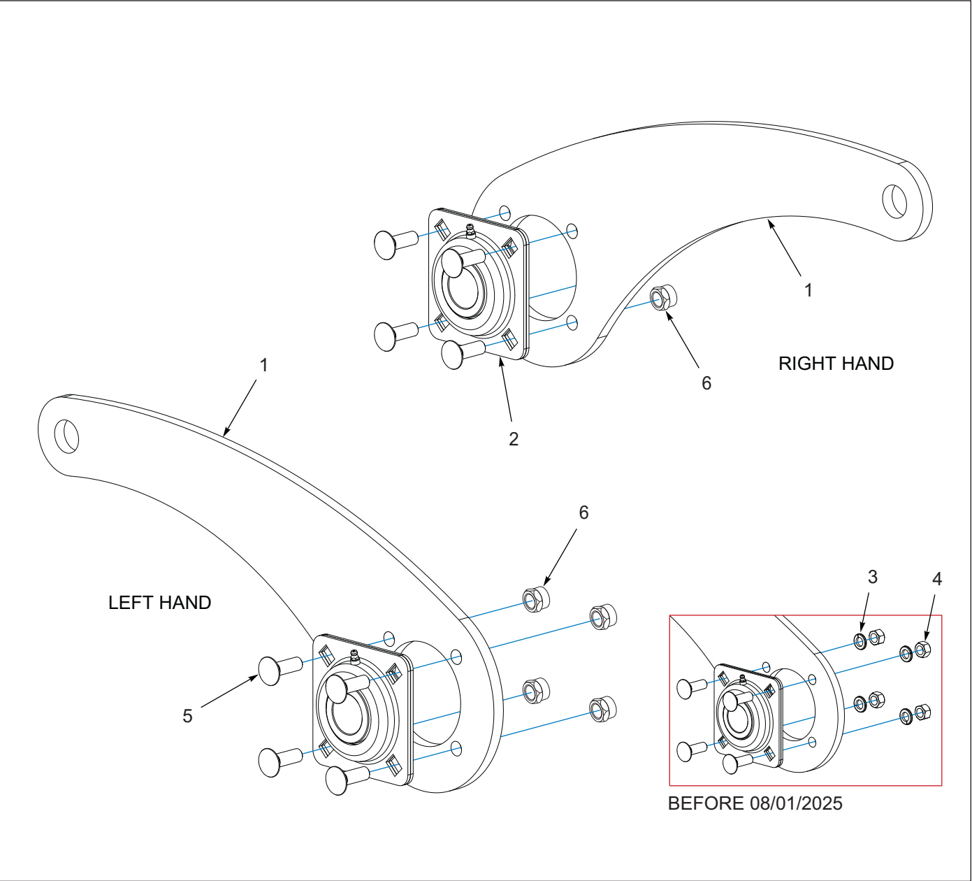
Figure 1-22: Rear Arm Assemblies
