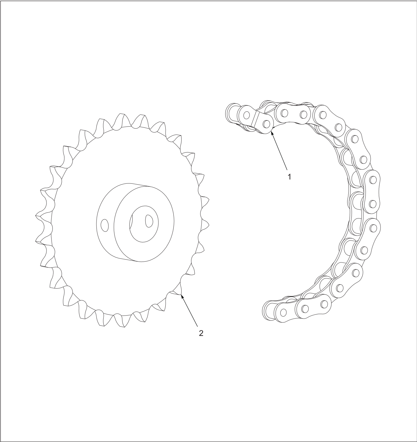
Figure 1-60: Speed-Up Kit - Optional
