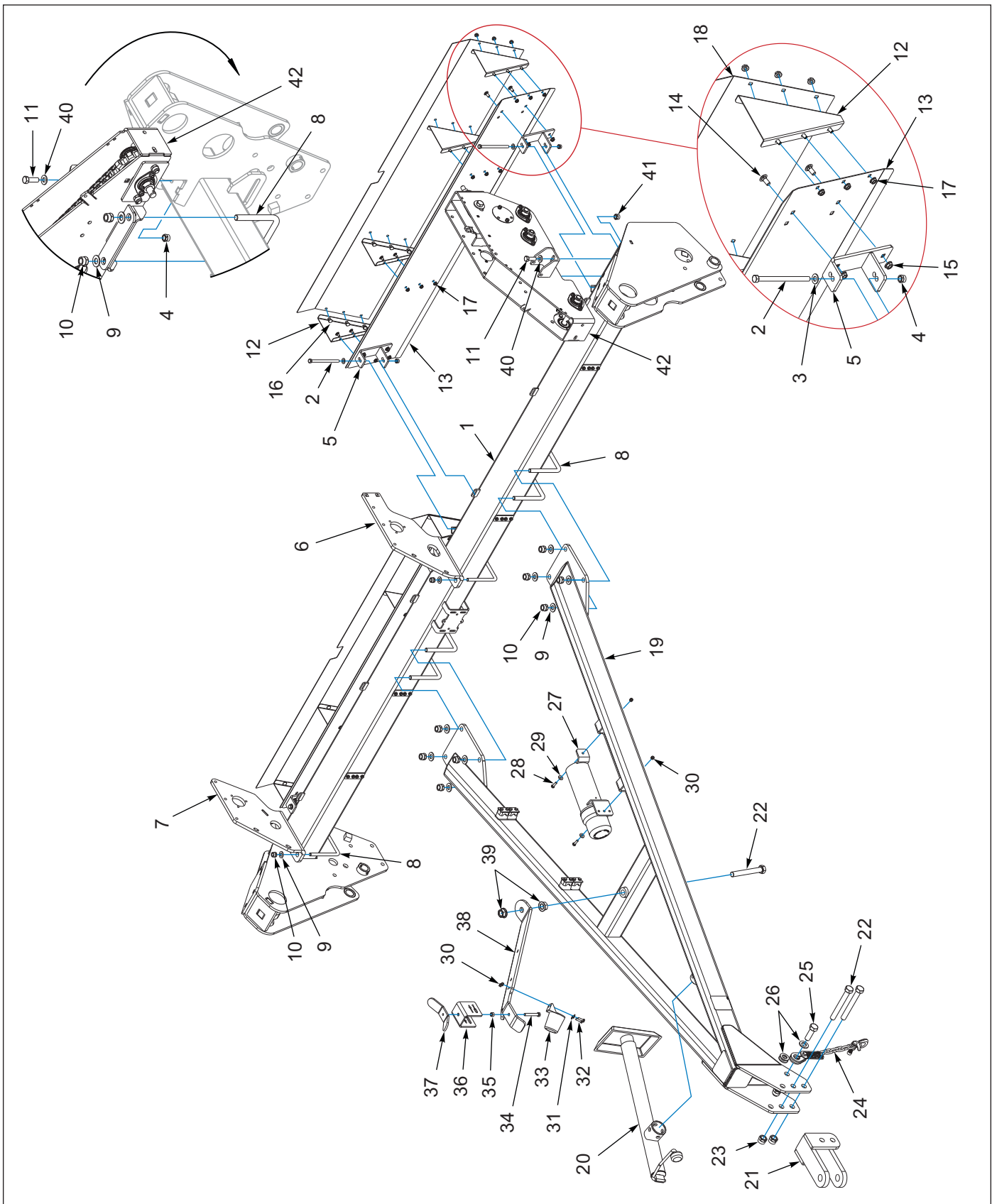
Figure 1-4: Drawbar Frame, Deflectors & Mounting - 10FT, 12FT (AFT. 08/2025)
