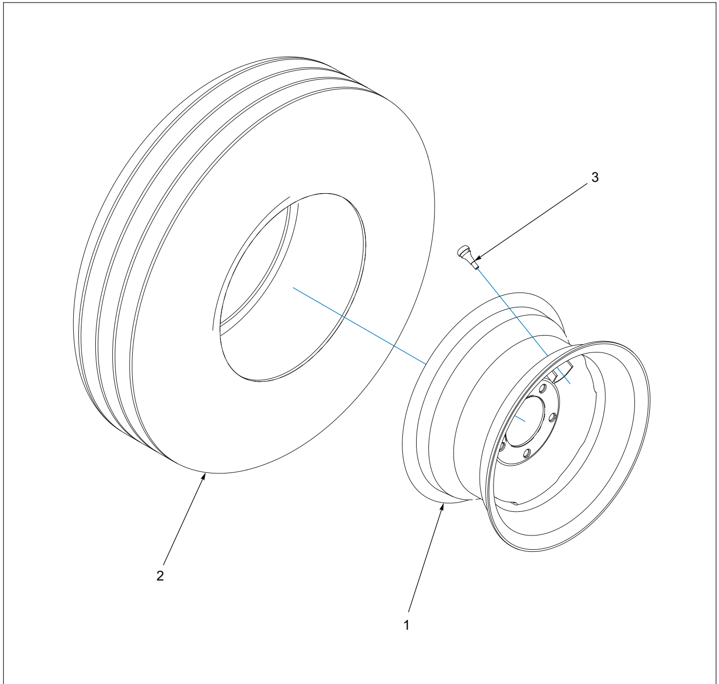
Figure 1-14: Tire and Wheel Assembly - 5 Bolt (BEFORE 05/2021)
