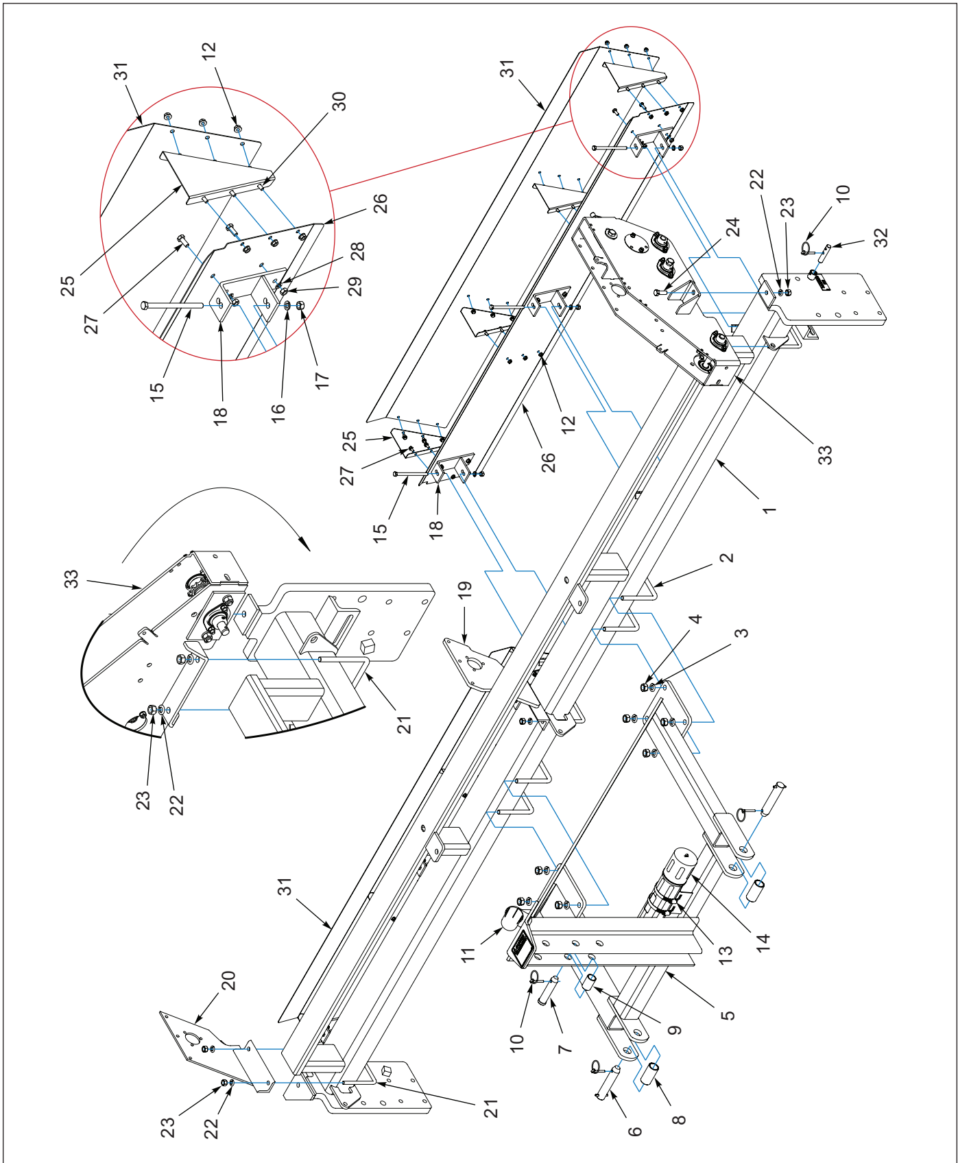
Figure 1-9: 3-PT Frame, Deflectors & Mounting - 10FT, 12FT (BEF. 08/2025)
