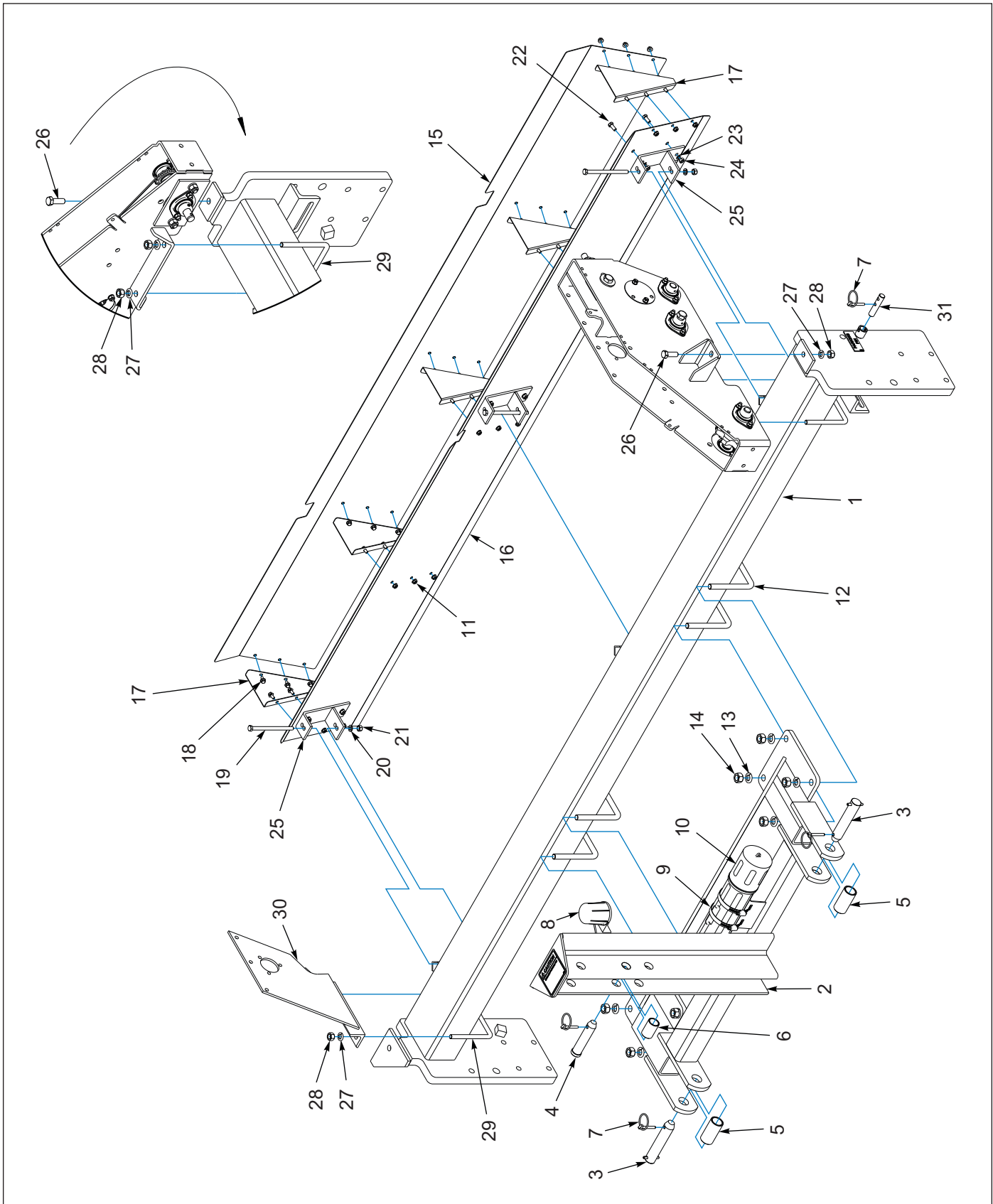
Figure 1-7: 3-PT Frame, Deflector & Mounting - 8FT (BEF. 08/2025)
