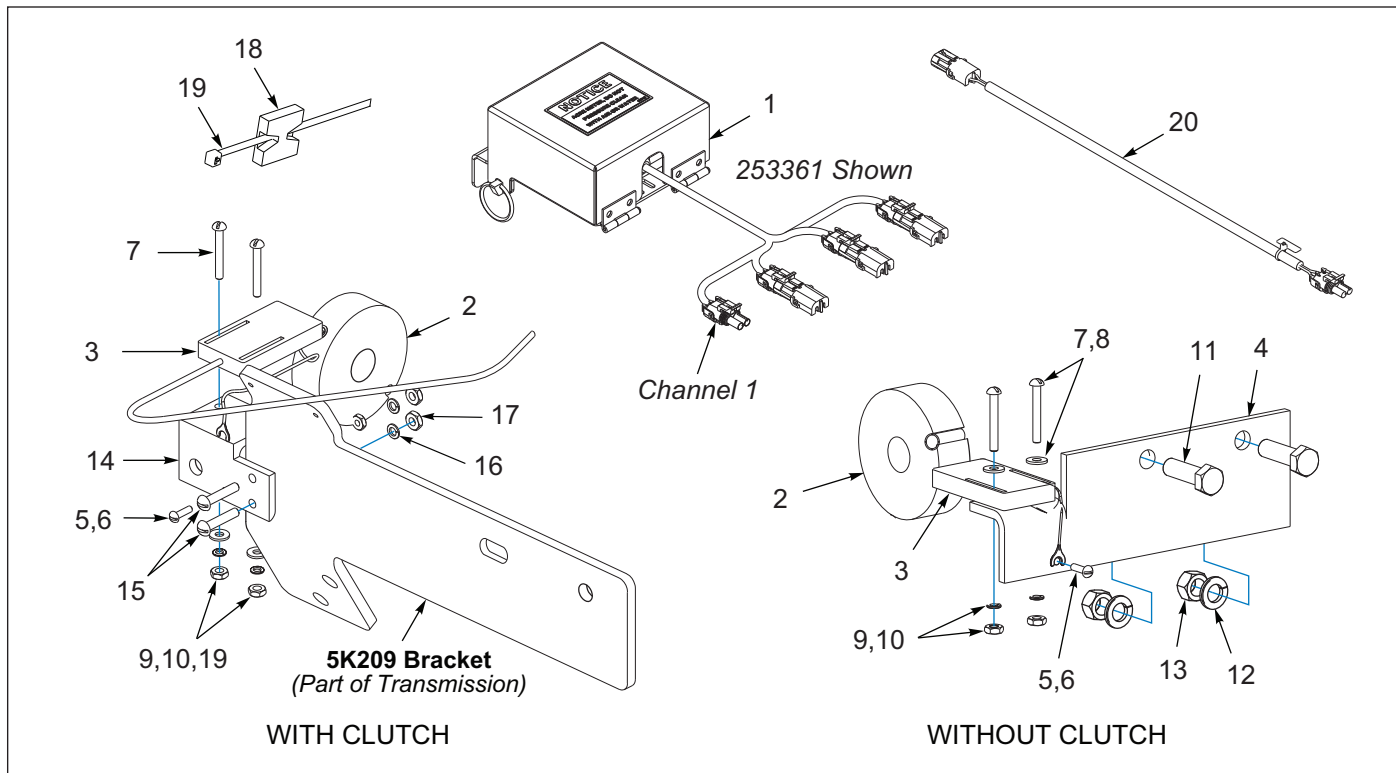
Figure 1-56: Electronic Acre Meter Assembly - Optional
