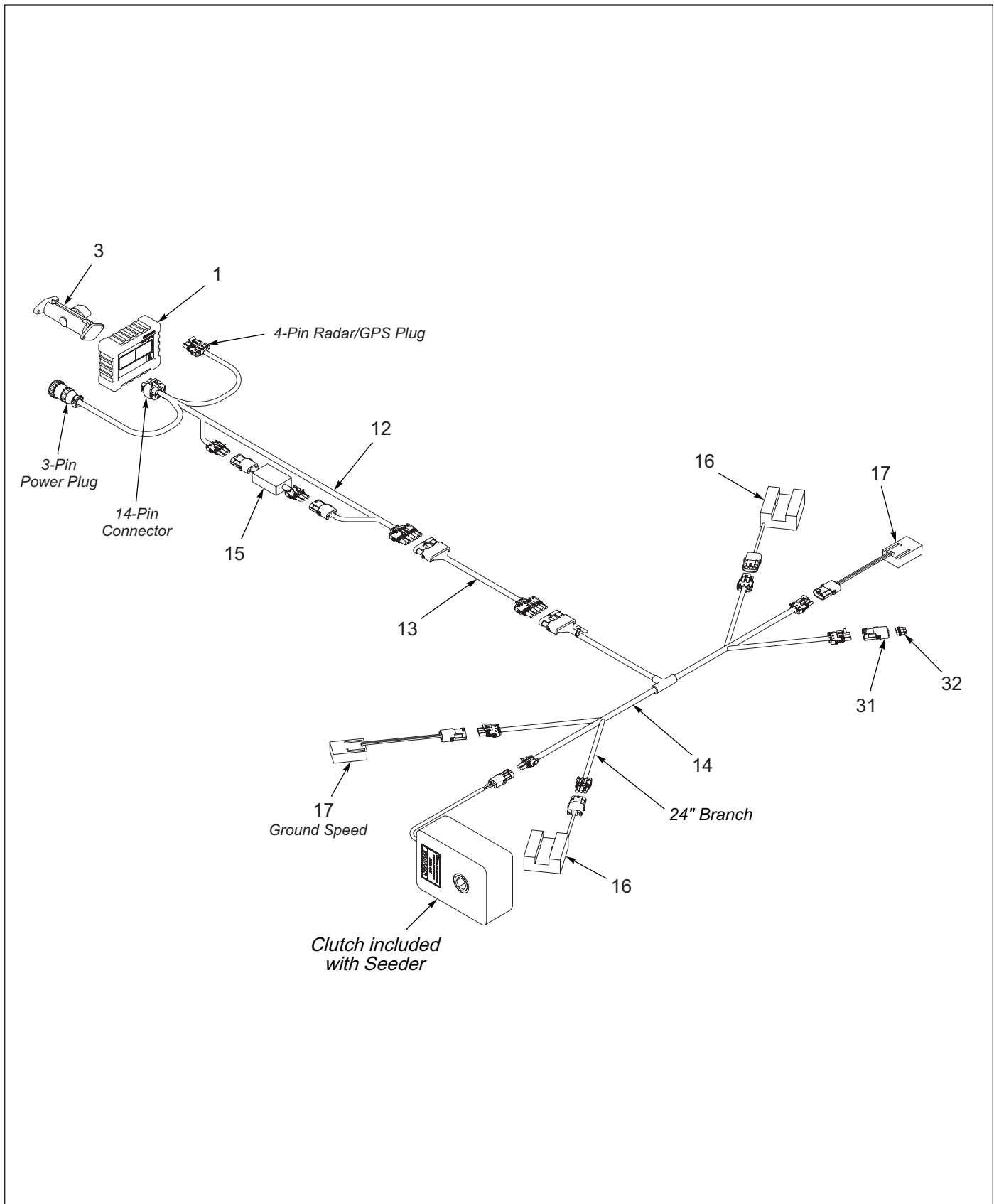
Figure 1-49: Brillion Elite Mini Monitor Electrical Schematic
