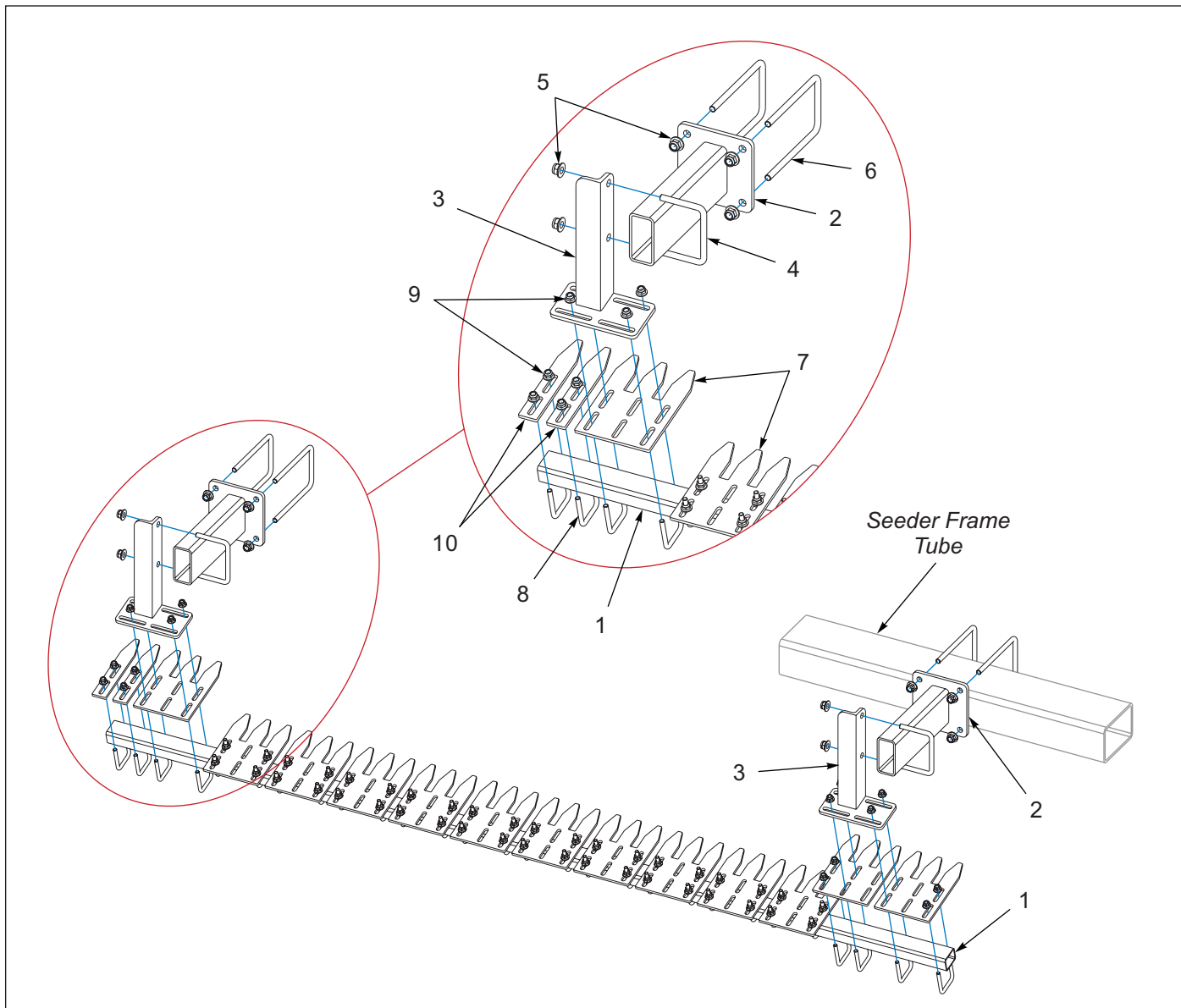
Figure 1-43: Scraper Kit, 8FT Tube Mounted - Optional
