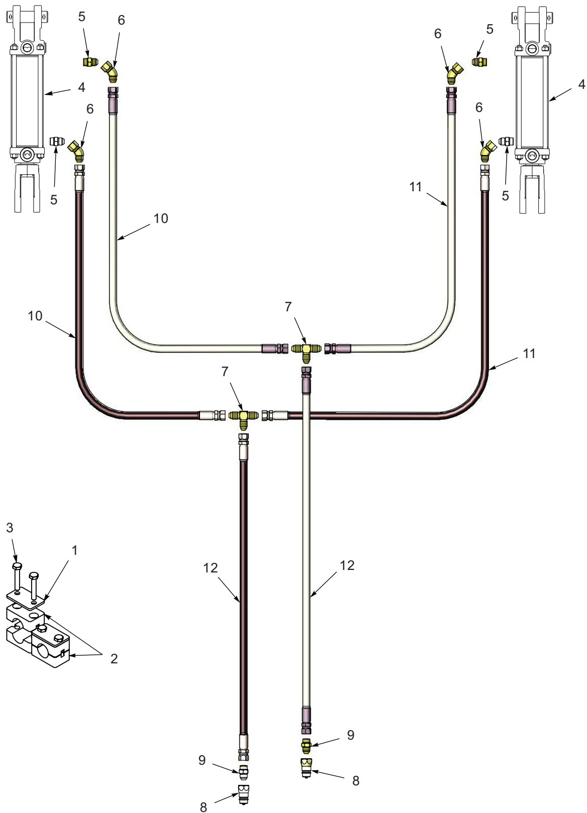
Figure 1-17: Hydraulic Schematic
