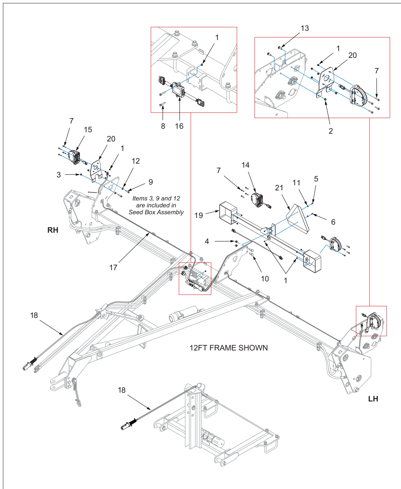
Figure 1-37: LED Warning Lamps - 10FT, 12FT (AFTER 08/2025)
