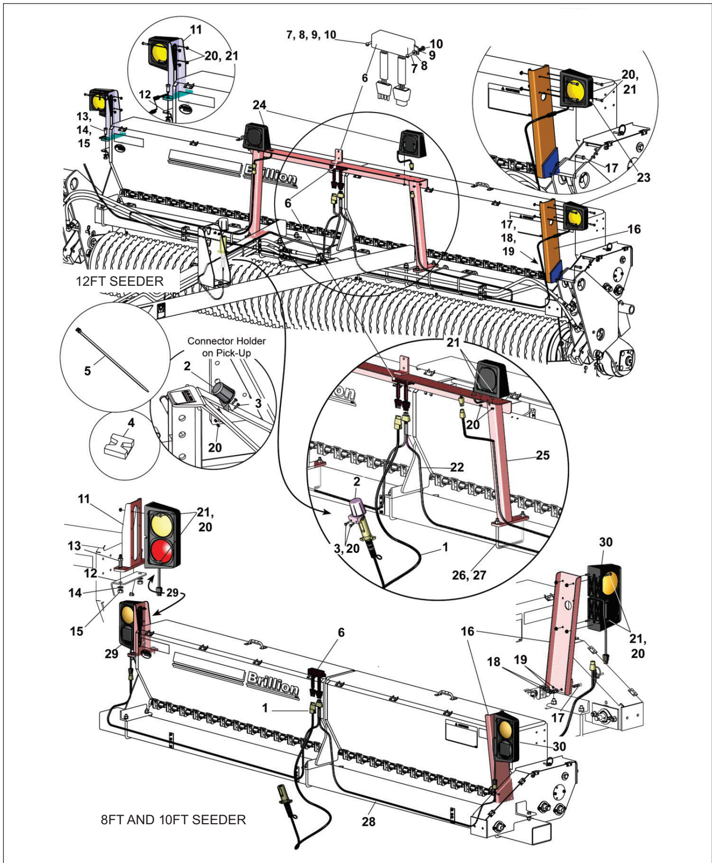
Figure 1-42: Warning Lamp Assembly (BEFORE 09/2013)
