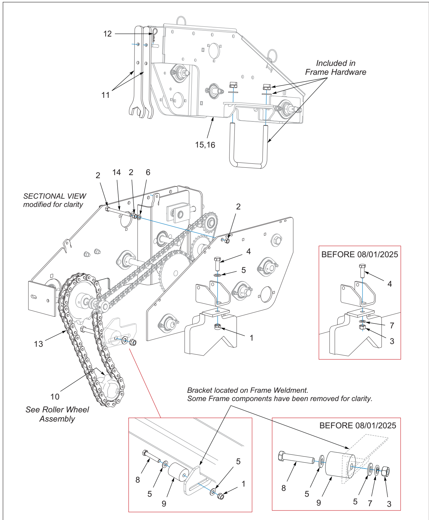
Figure 1-23: Transmission Mounting and Drive
