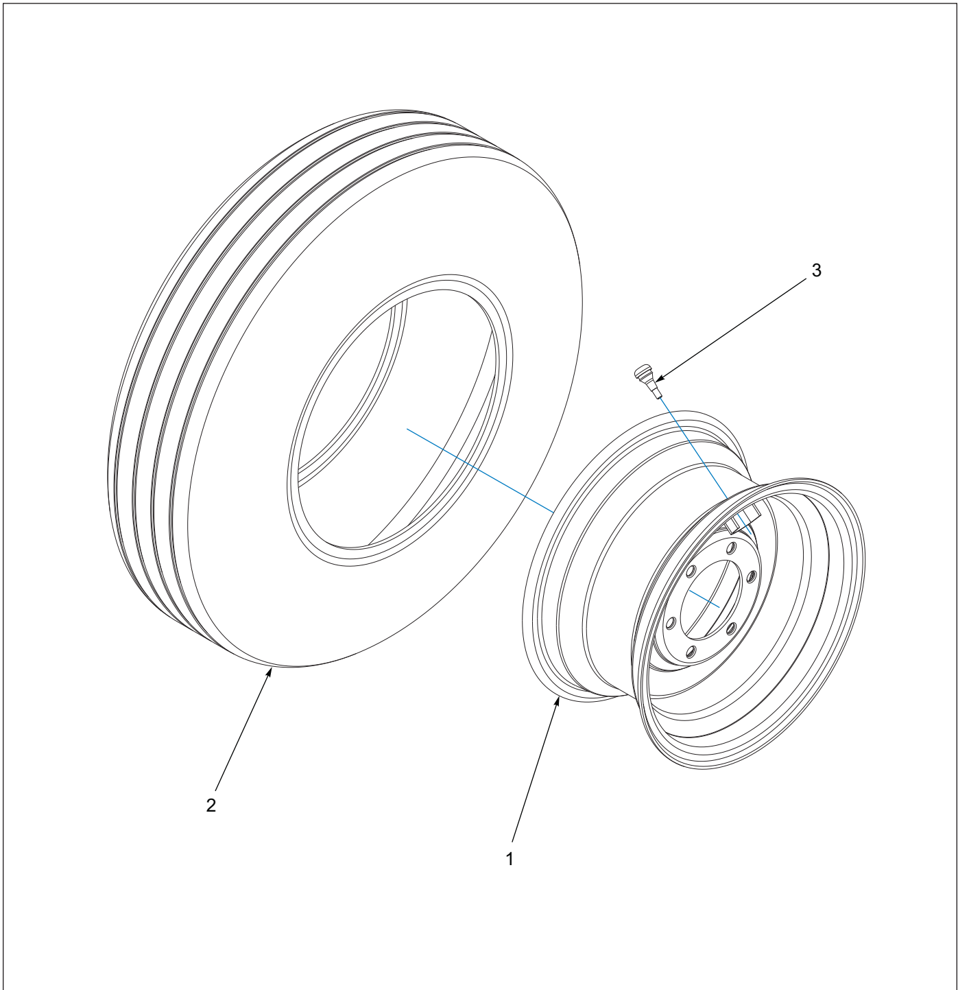
Figure 1-13: Tire and Wheel Assembly - 6 Bolt (AFTER 05/2021)
