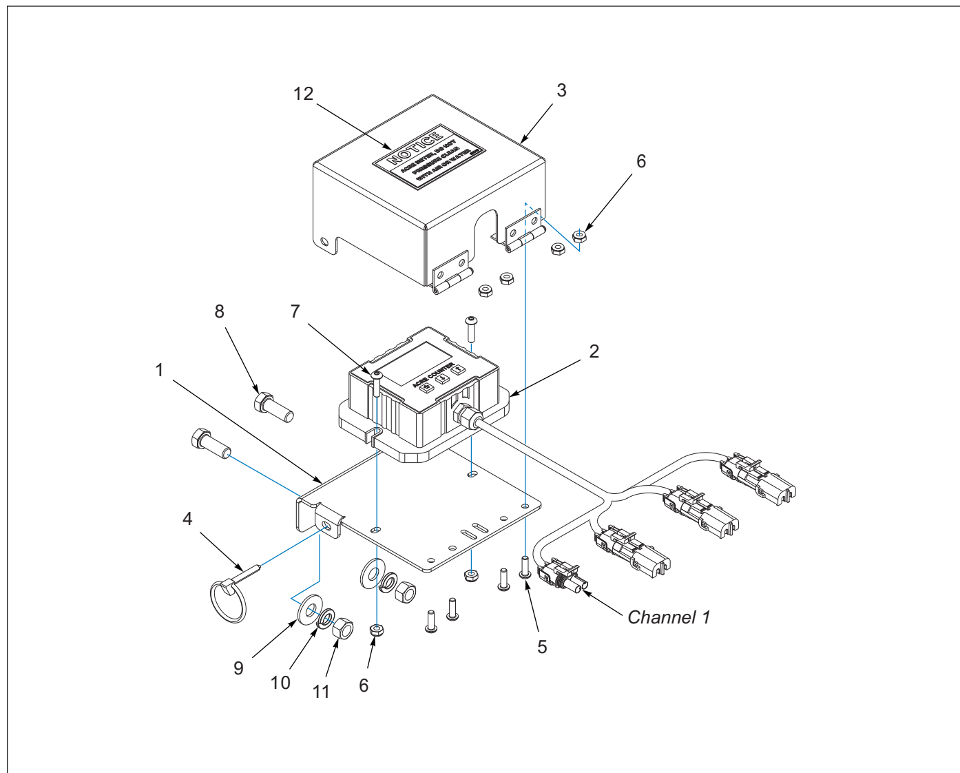
Figure 1-57: Acre Meter Assembly (AFTER 06/01/2025)
