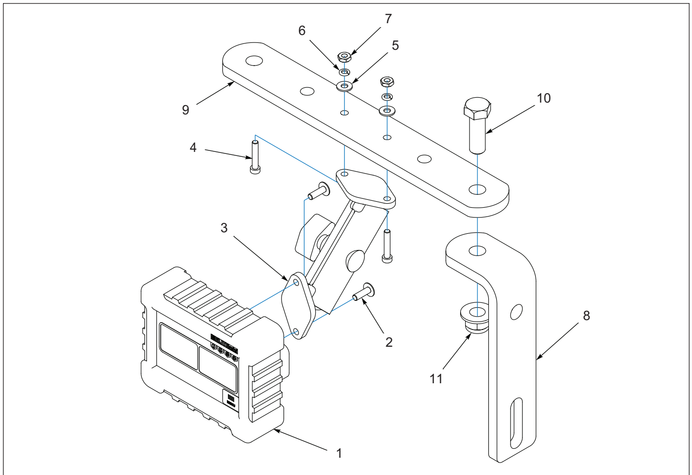
Figure 1-50: Brillion Elite Mini Monitor Tractor Mount
