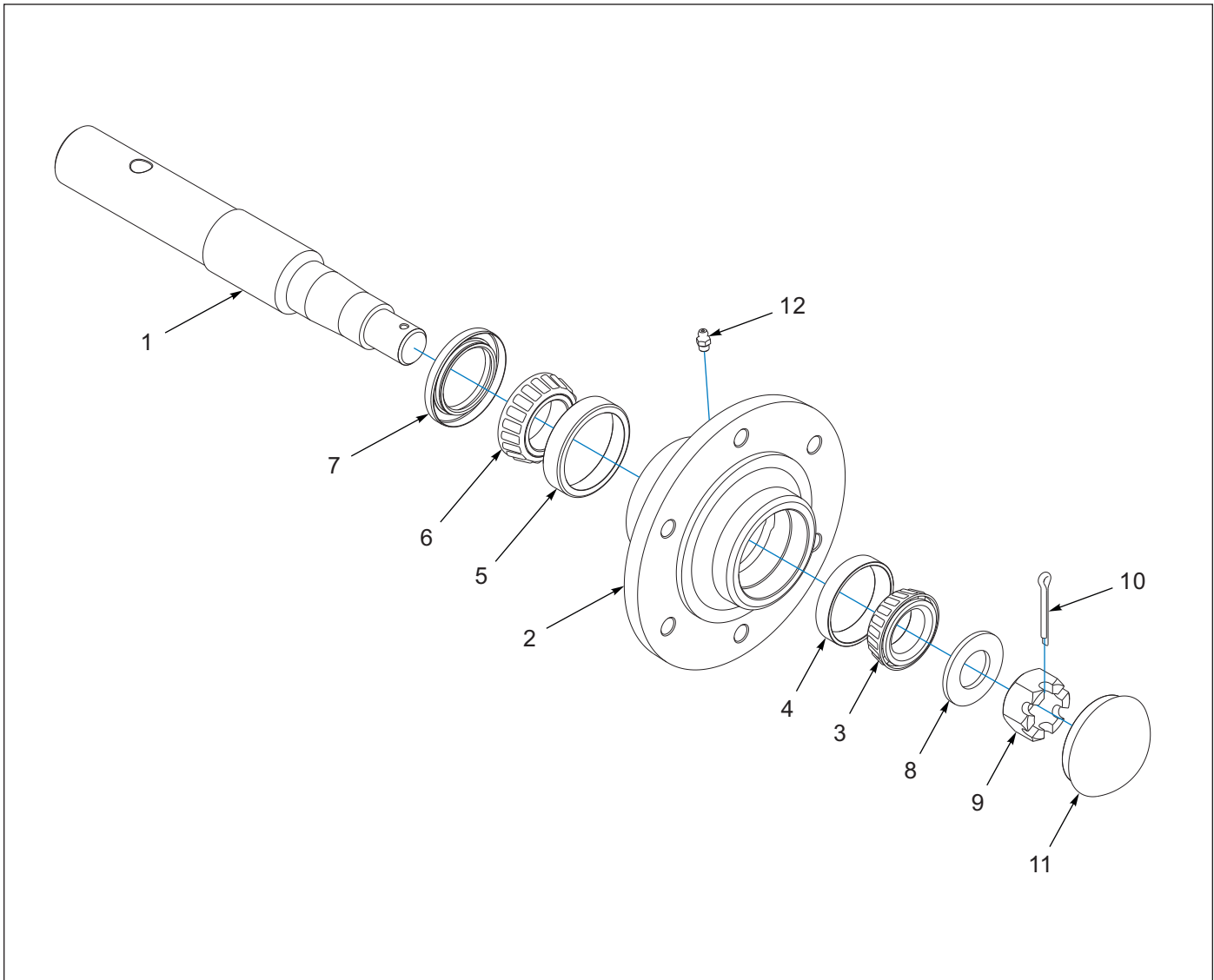
Figure 1-11: Hub and Spindle Assembly - 6 Bolt (AFTER 05/2021)
