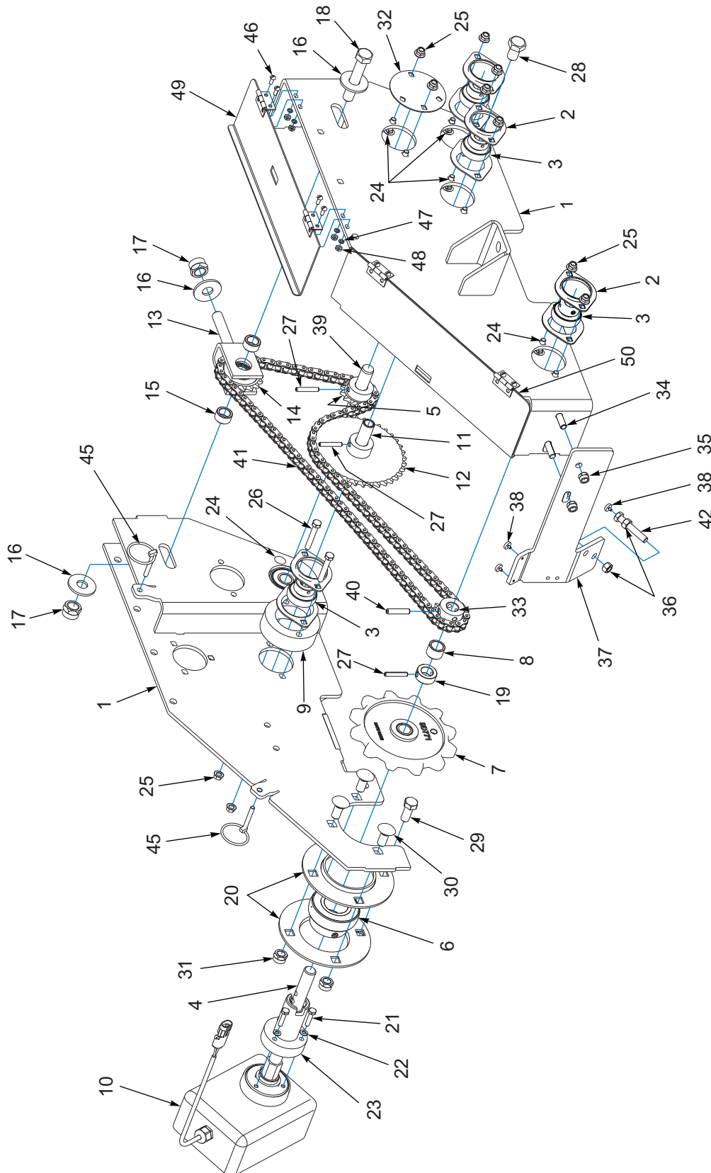
Figure 1-26: Transmission Assembly with Optional Electric Clutch (AFT. 08/2025)
