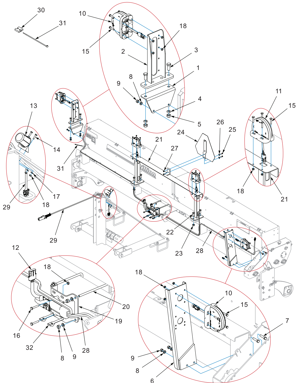
Figure 1-41: LED Warning Lights - 12FT 3-PT Model (09/2013 TO 08/2025)
