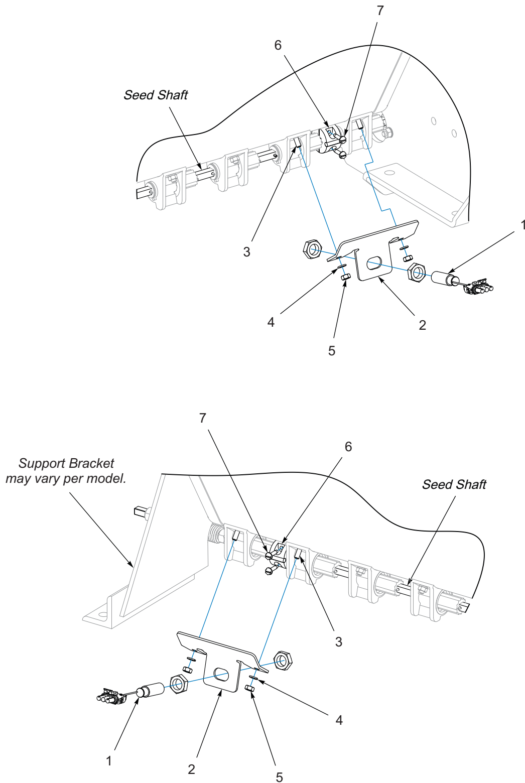
Figure 1-54: Console w/Clutch Control - Seed Shaft Sensor
