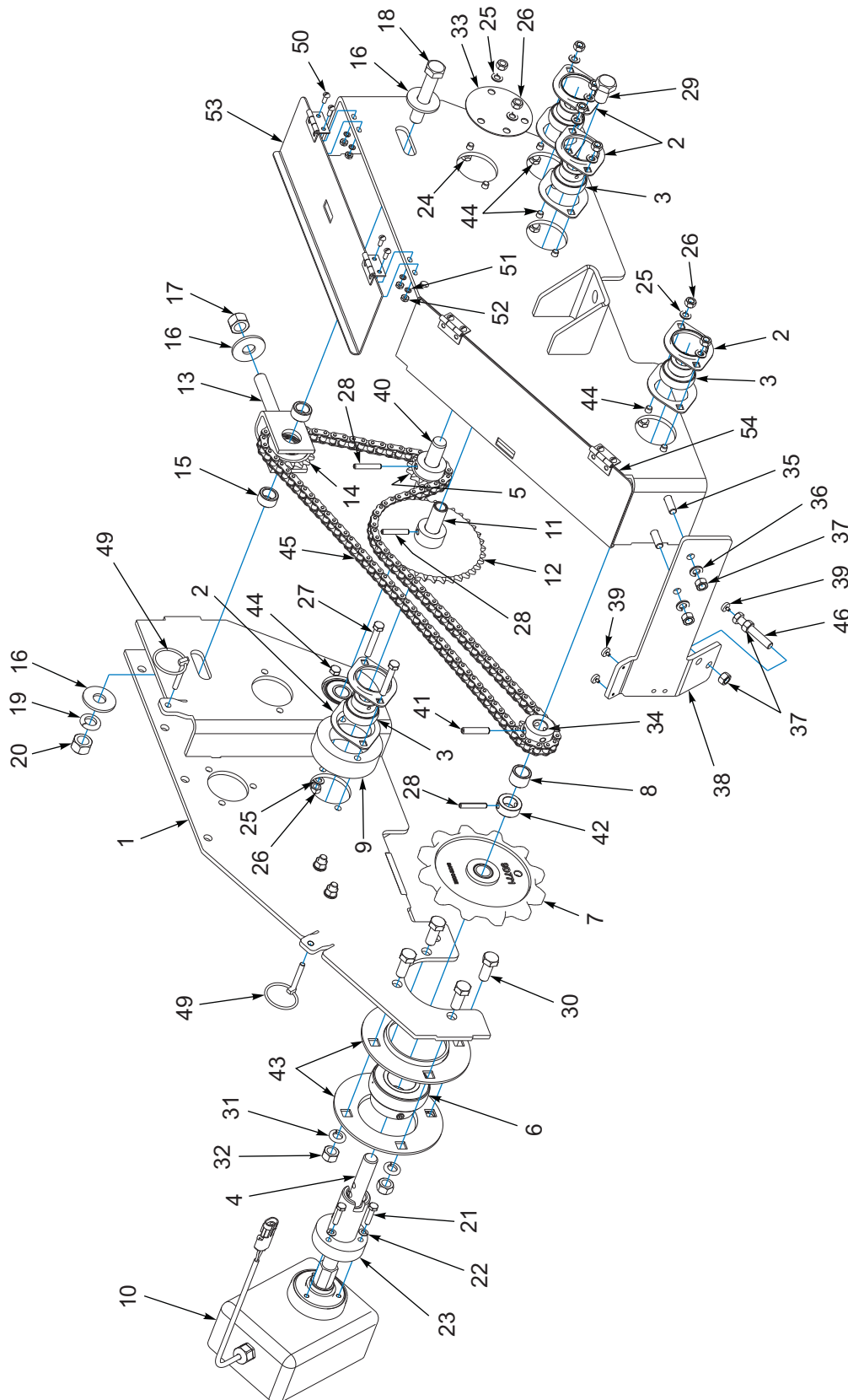
Figure 1-27: Transmission Assembly with Optional Electric Clutch (BEF. 08/2025)
