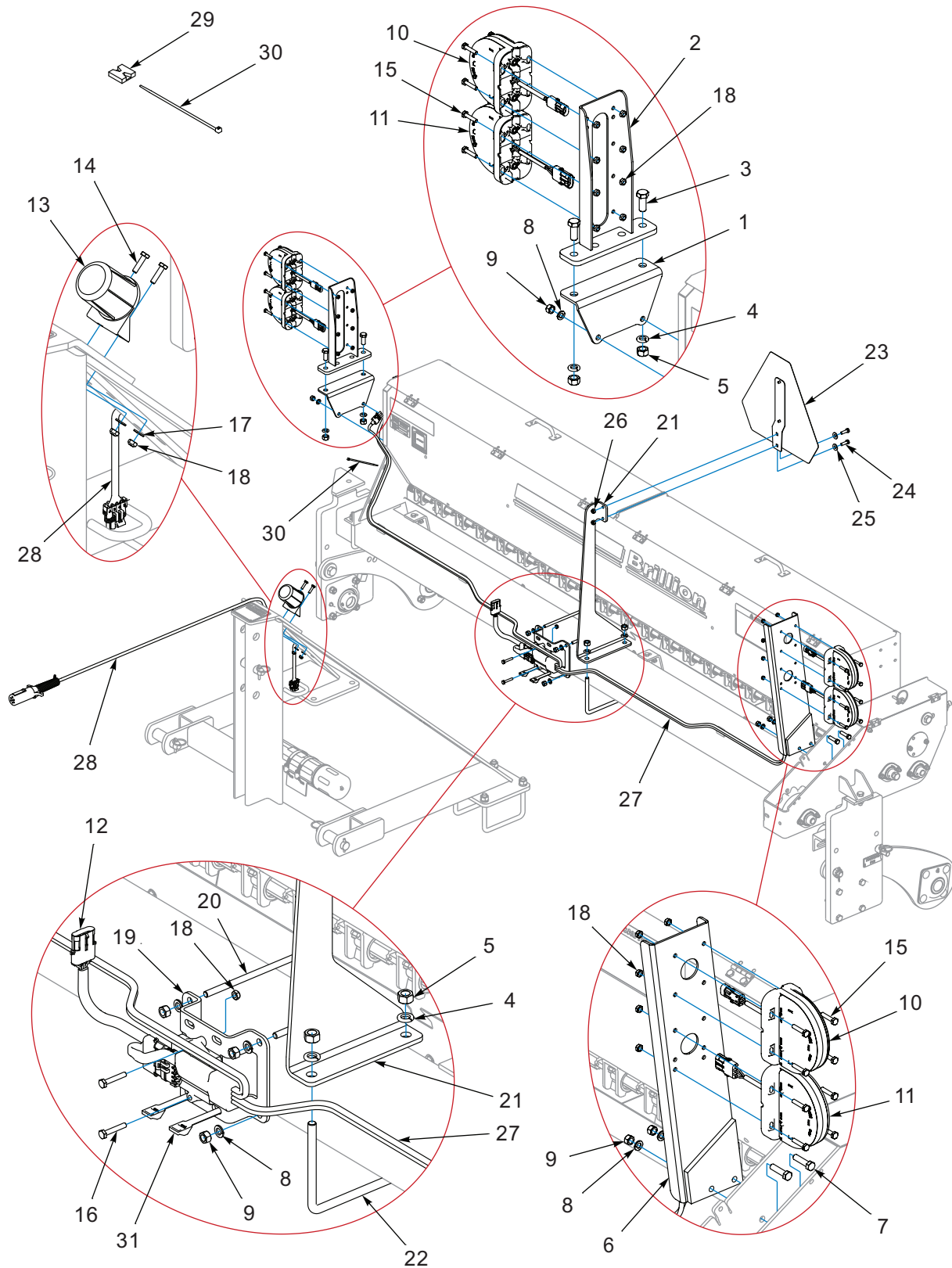
Figure 1-38: LED Warning Lamps - 8FT (09/2013 TO 08/2025)
