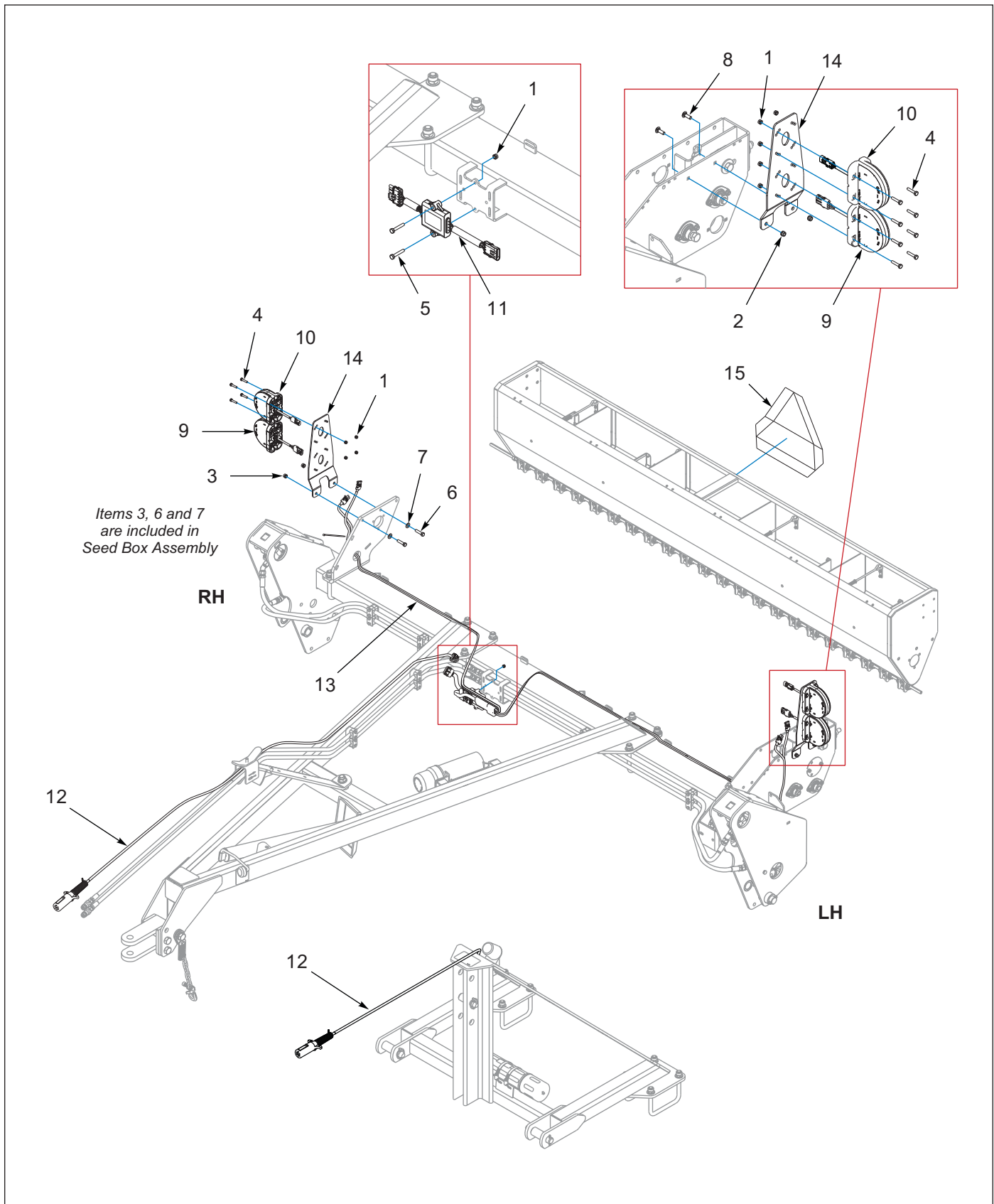
Figure 1-36: LED Warning Lamps - 8FT (AFTER 08/2025)
