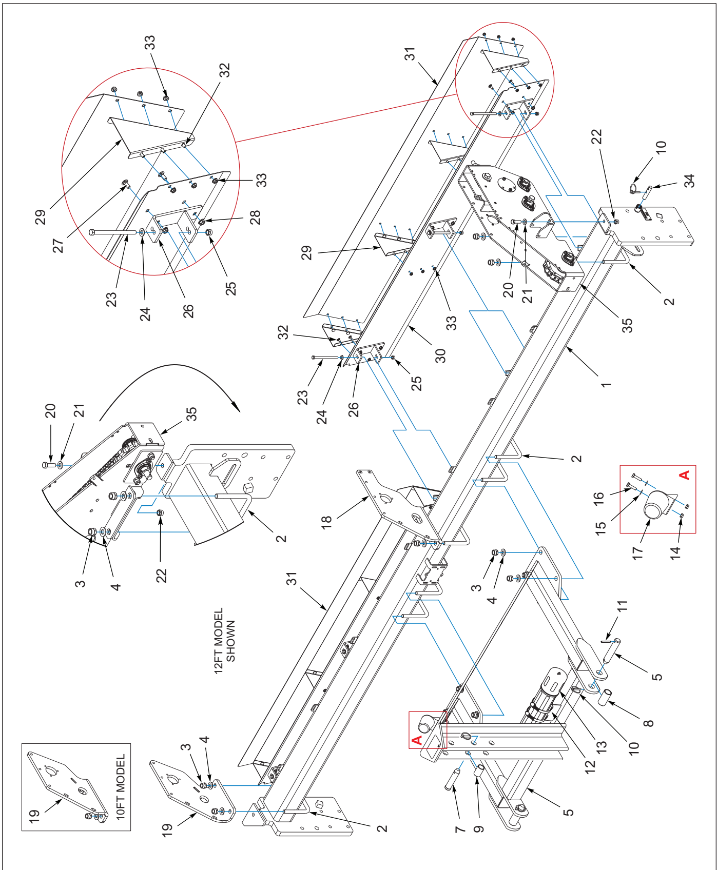
Figure 1-8: 3-PT Frame, Deflectors & Mounting - 10FT, 12FT (AFT. 08/2025)
