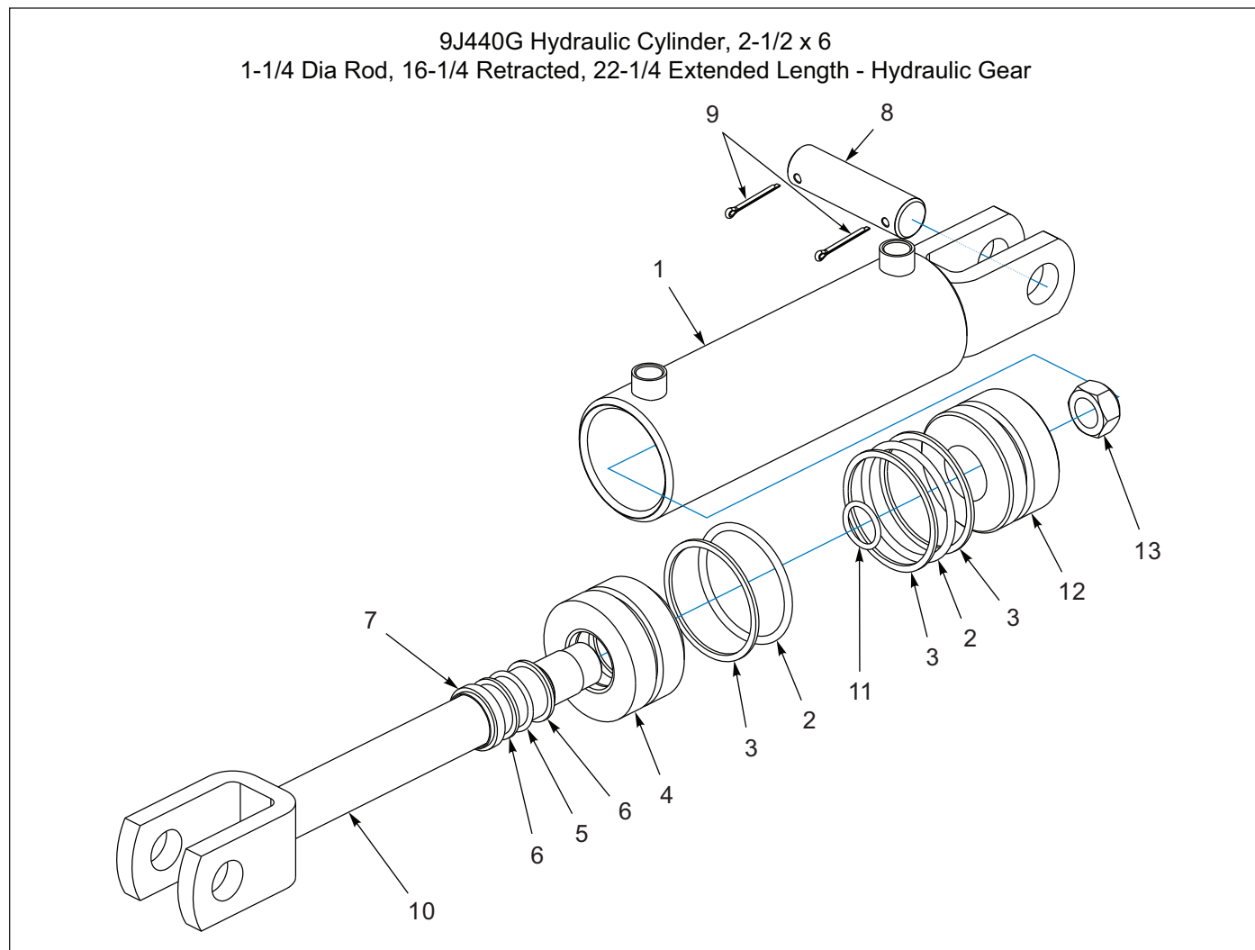
Figure 1-63: Hydraulic Cylinder, 2-1/2 x 6 - Hydraulic Gear (BEFORE 01/14/2008)
