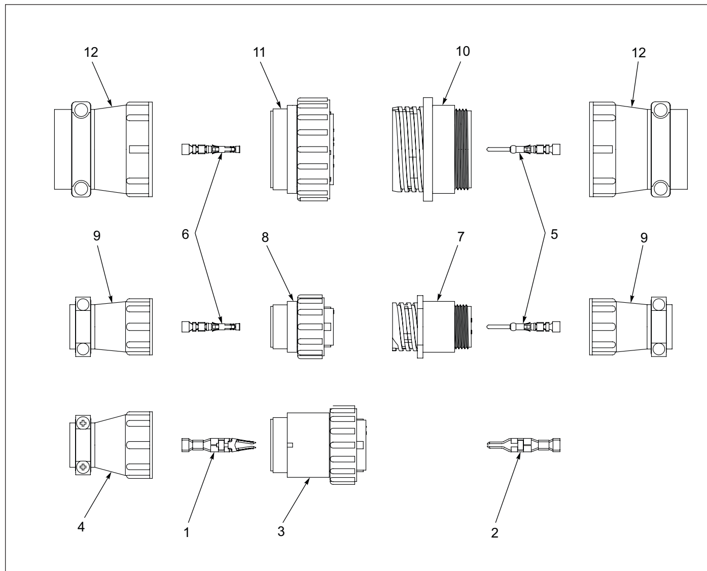
Figure 1-65: AMP Connectors
