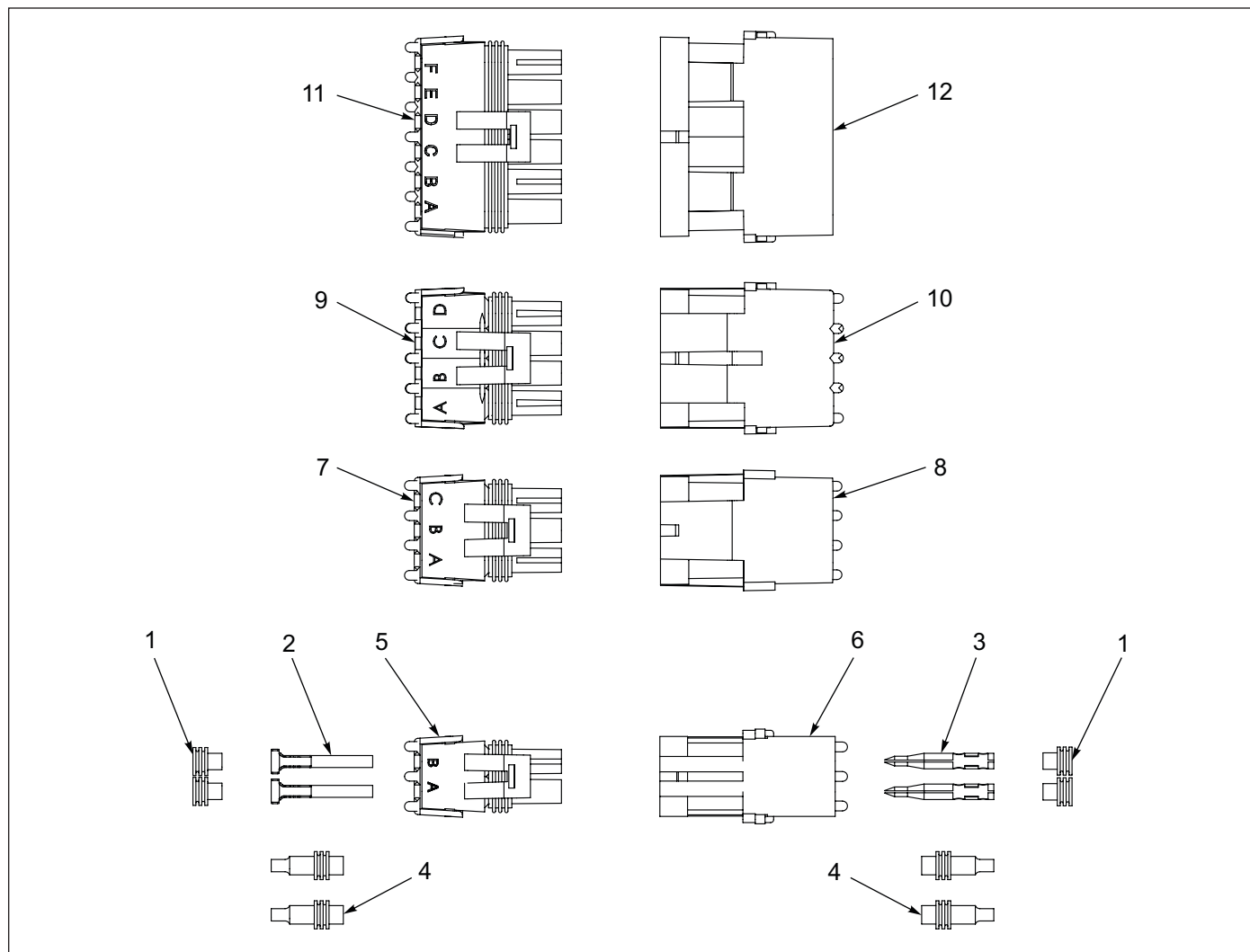
Figure 1-64: Weather Pack Connectors
