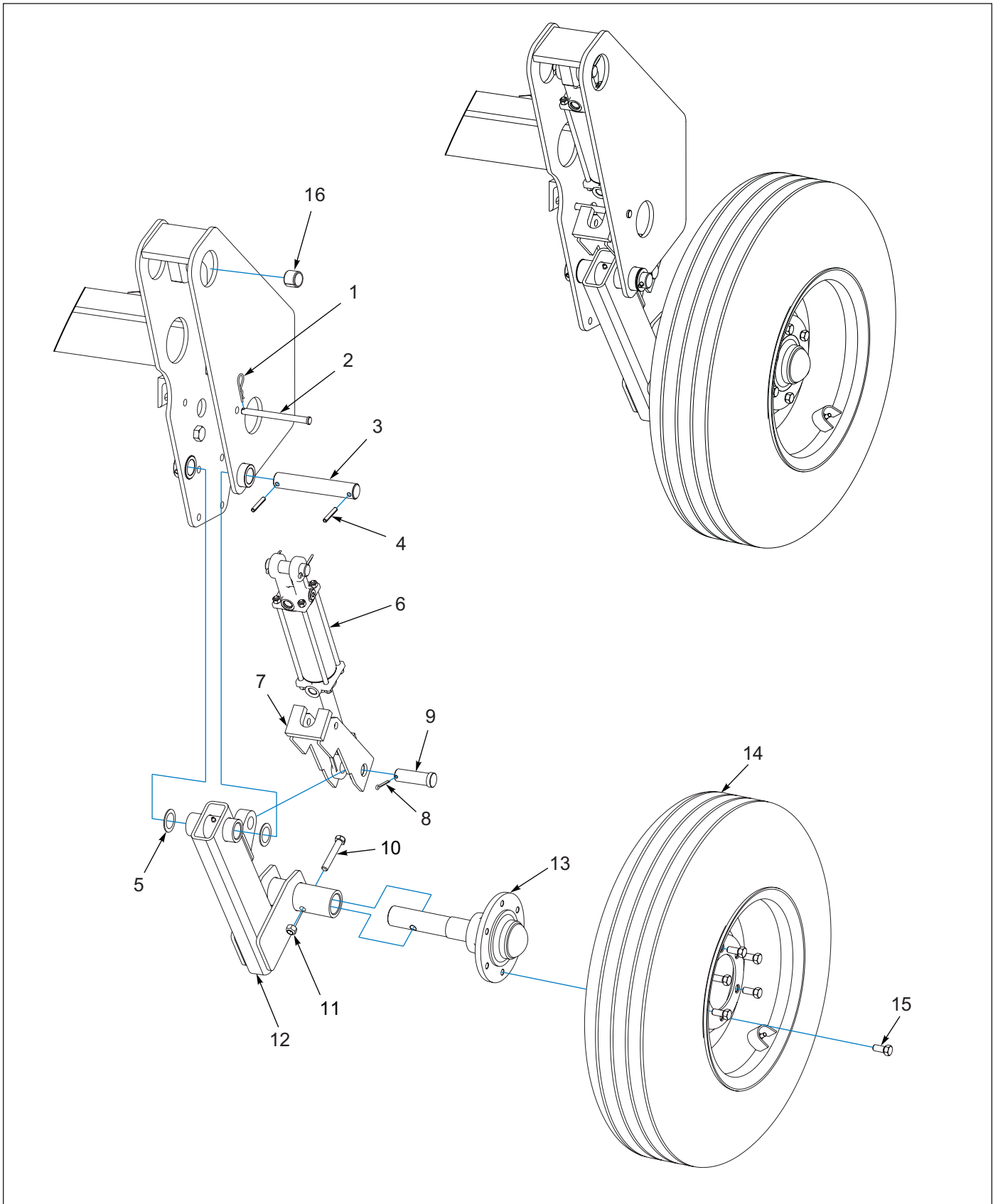
Figure 1-10: Wheel Arm Assembly
