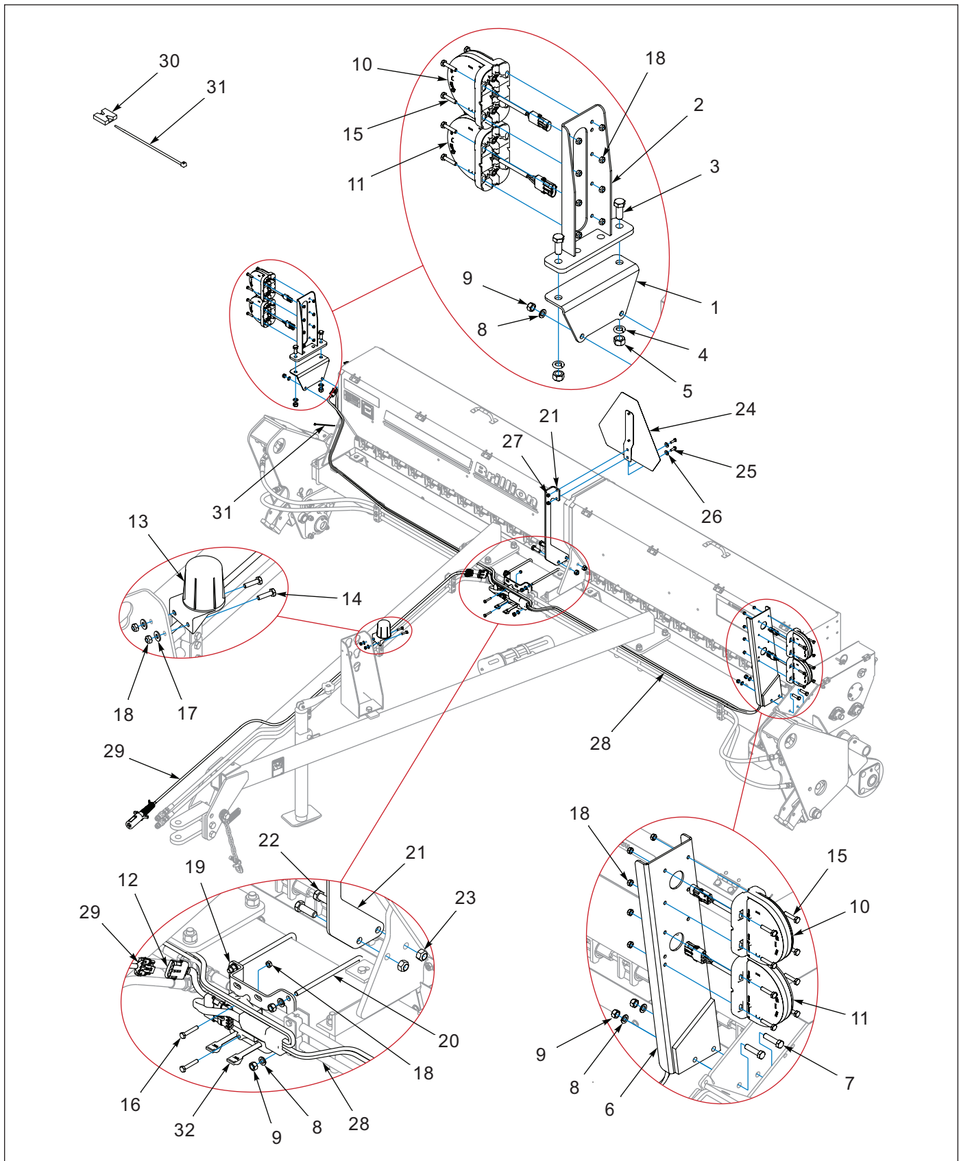
Figure 1-39: LED Warning Lamps - 10FT (09/2013 TO 08/2025)
