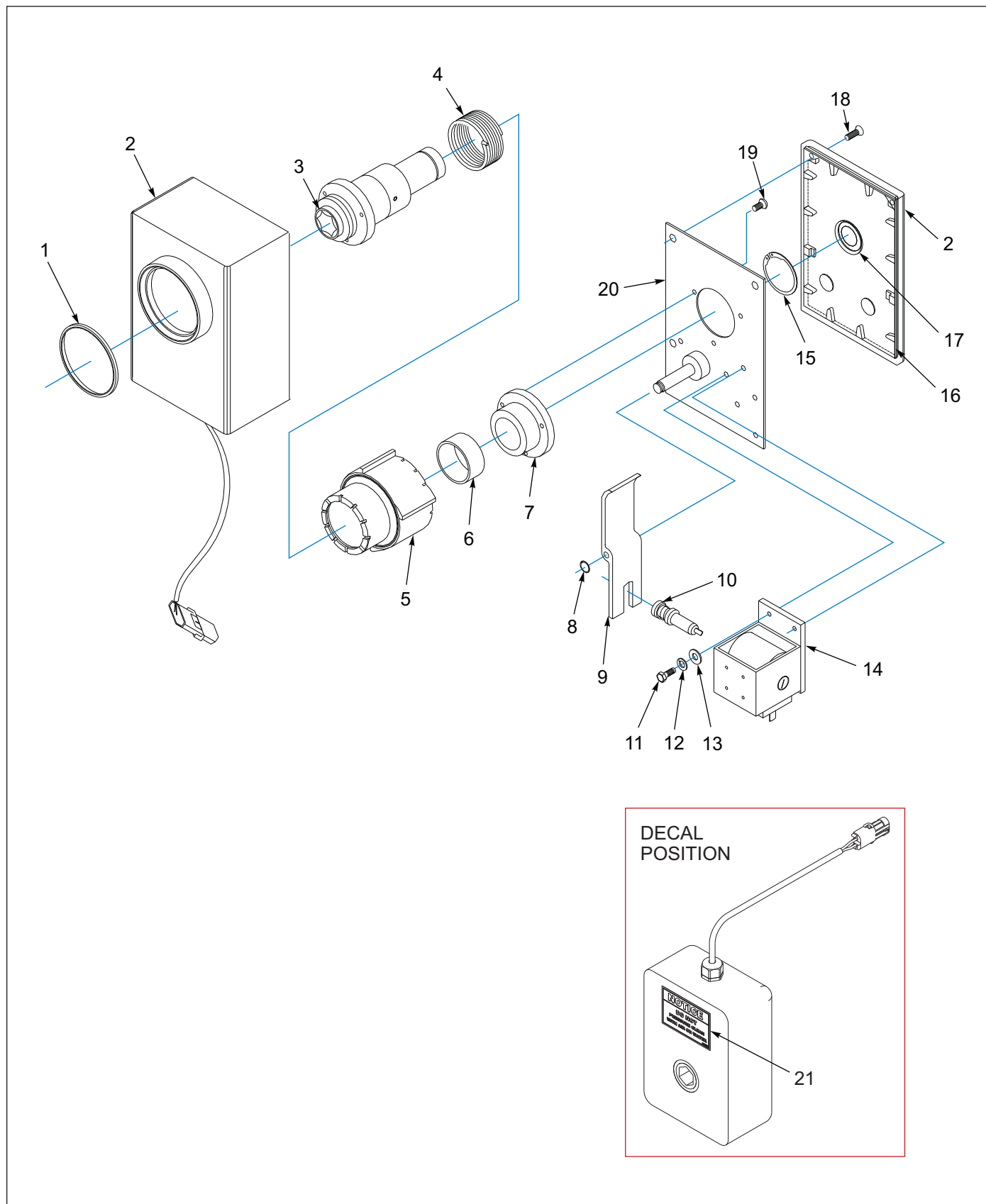
Figure 1-28: Electrical Clutch - Optional
