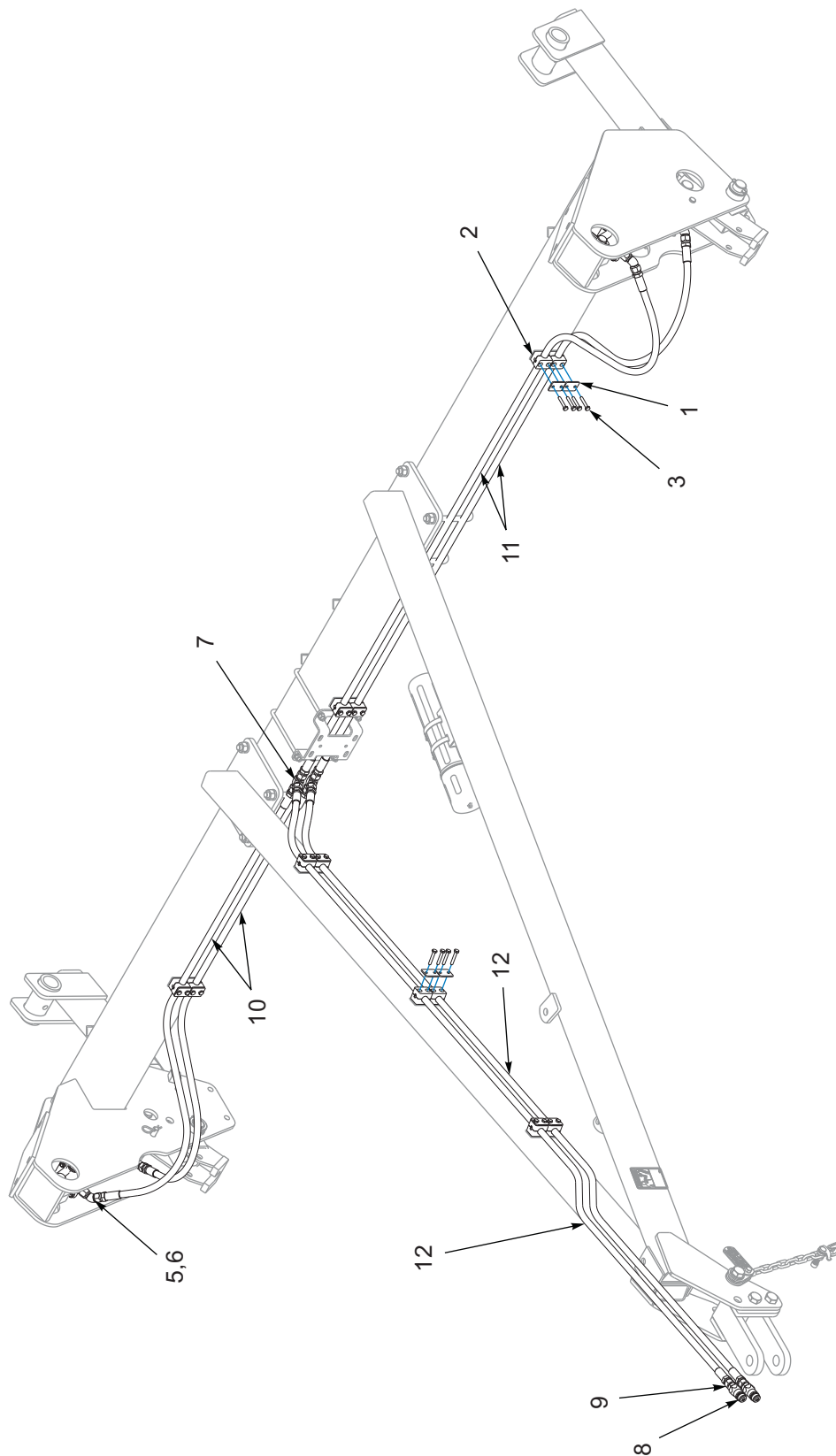
Figure 1-16: Hydraulic Layout (BEFORE 08/2025)
