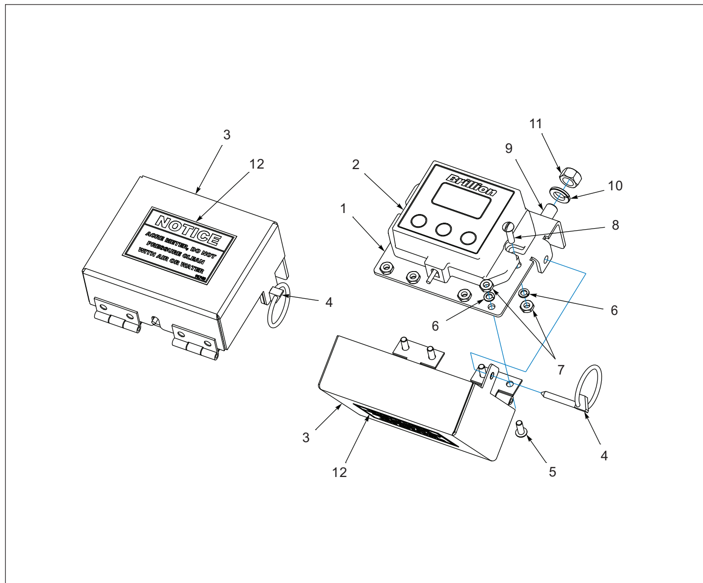
Figure 1-59: Acre Meter Assembly (BEFORE 05/15/2012)
