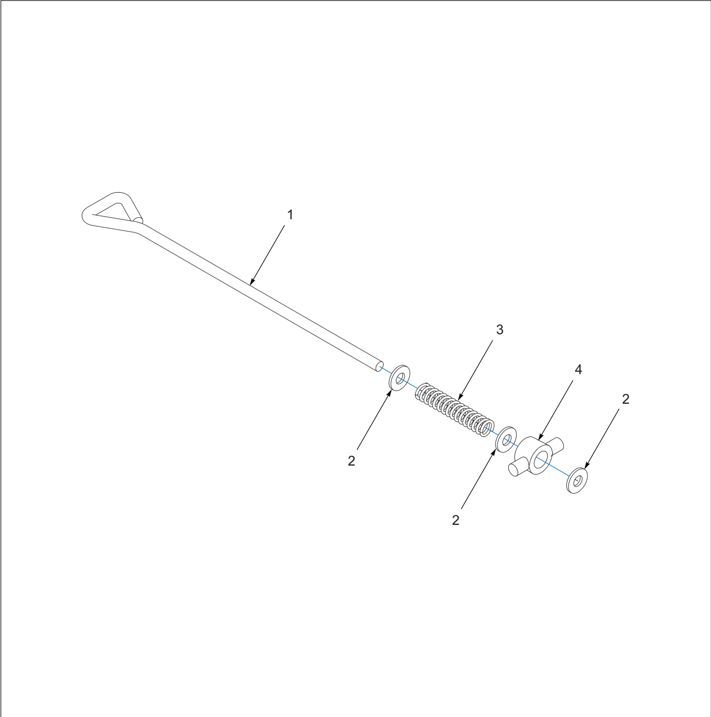
Figure 1-32: Cover Lock
