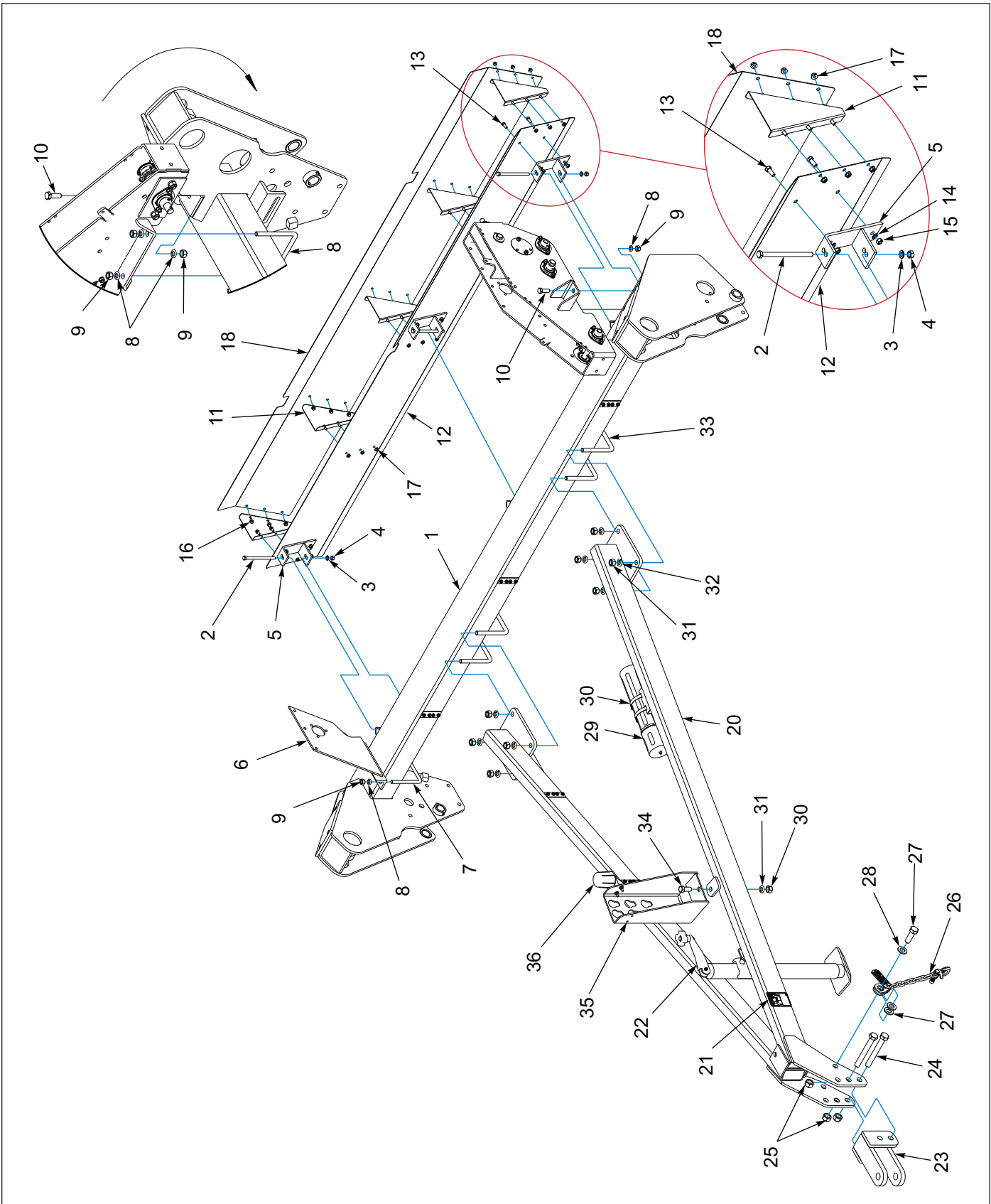
Figure 1-3: Drawbar Frame, Deflectors & Mounting - 8FT (BEF. 08/2025)
