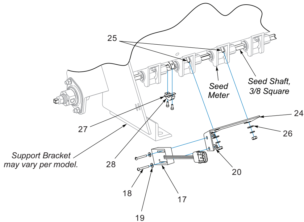
Figure 1-52: Brillion Elite Mini Monitor - Seed Shaft Sensor
