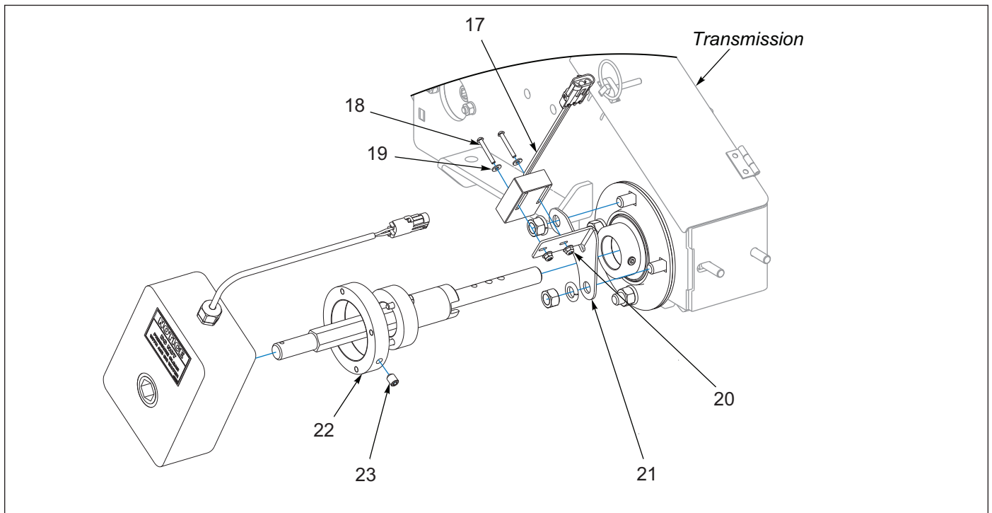
Figure 1-51: Brillion Elite Mini Monitor - Ground Speed
