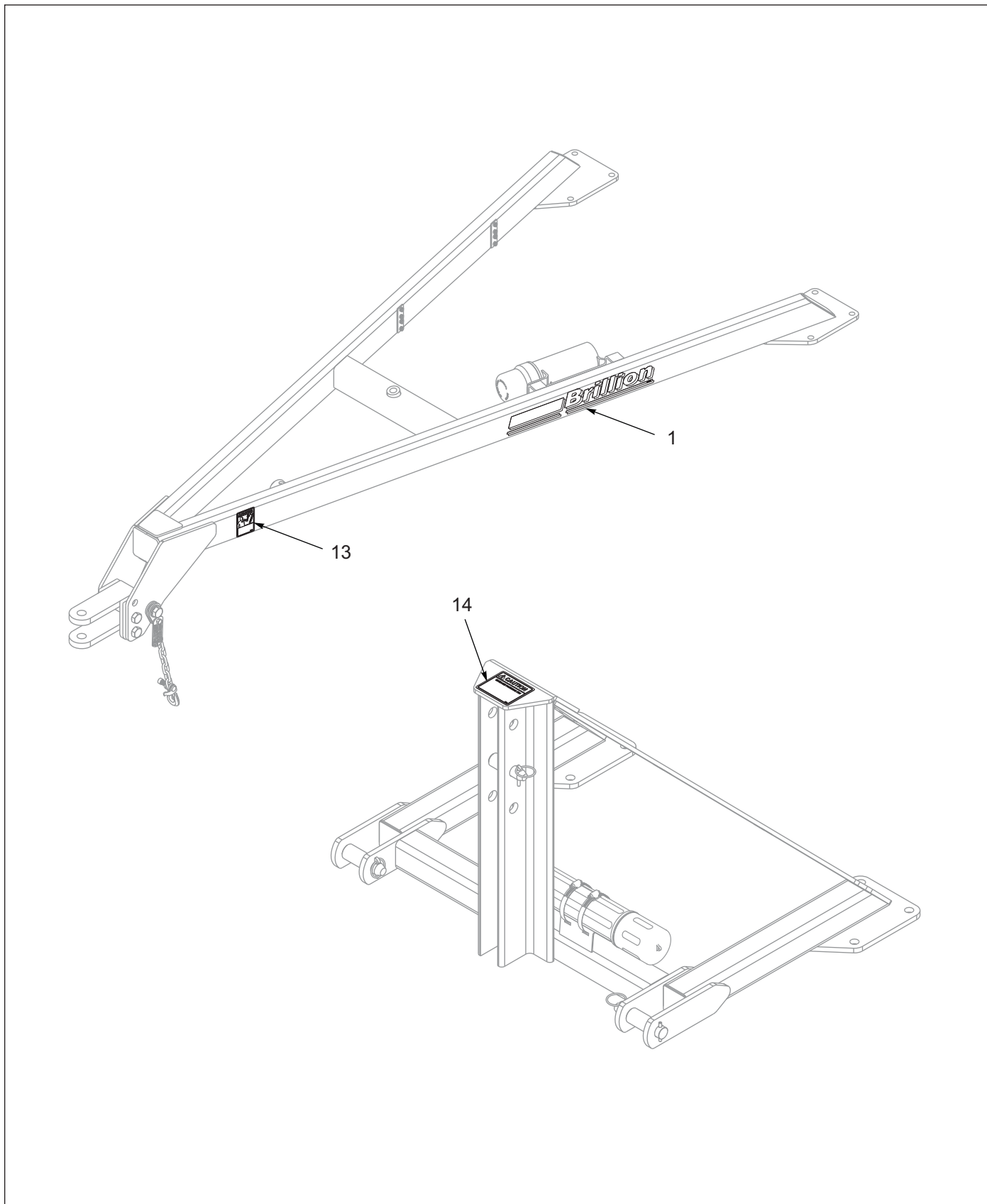
Figure 1-68: Decal Placement - Hitch
