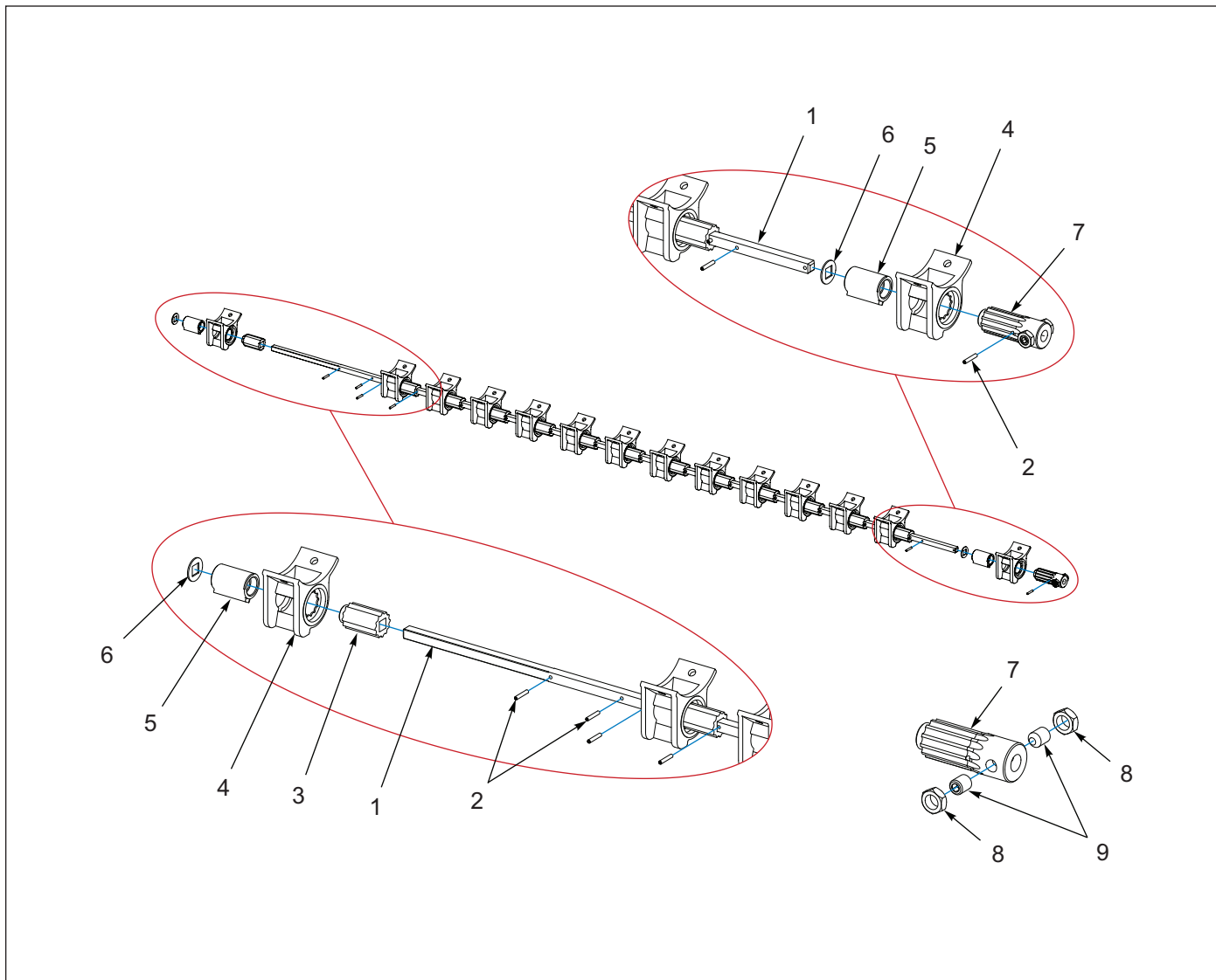
Figure 1-35: Seed Meter Assembly, Right-Hand 10FT and 12FT
