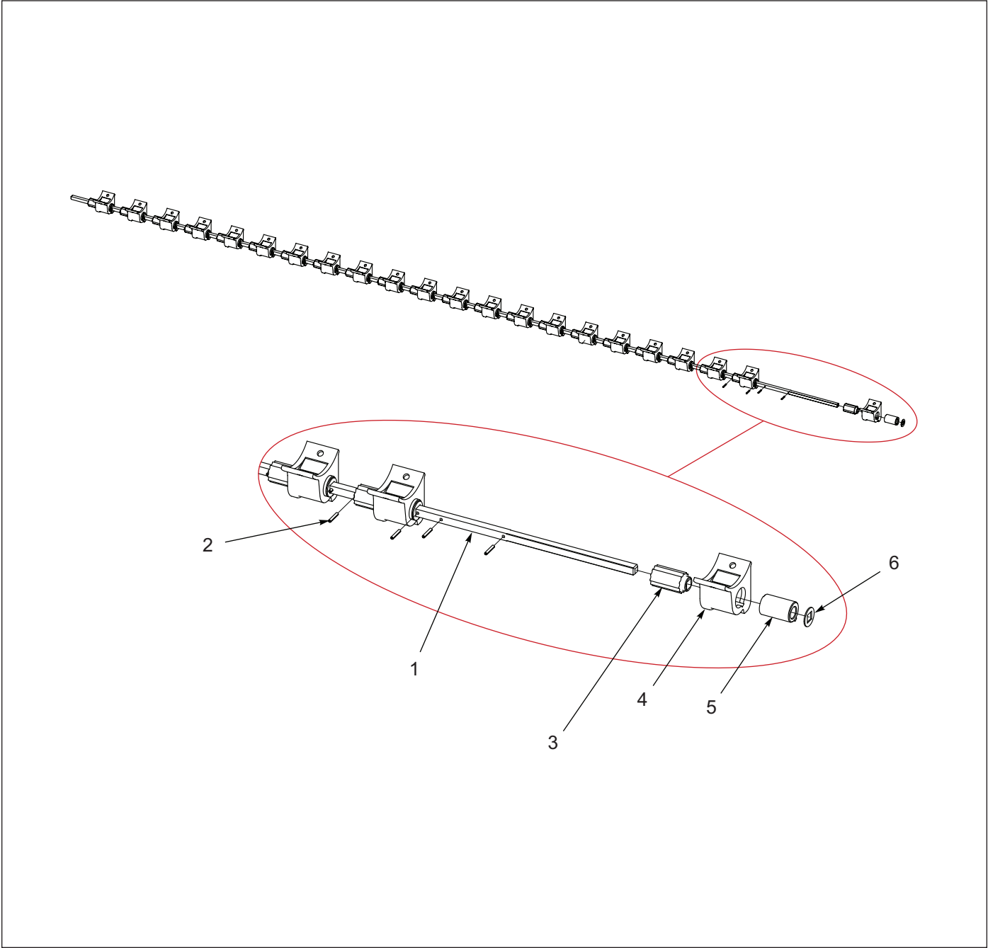
Figure 1-33: Seed Meter Assembly, 8FT
