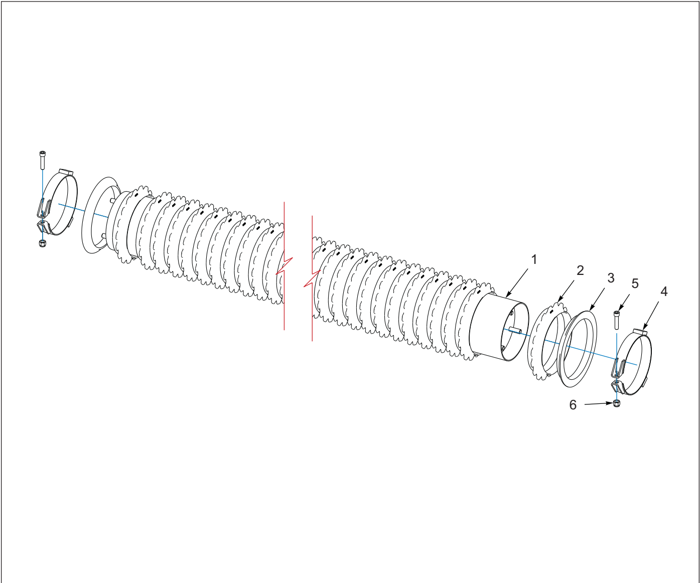
Figure 1-21: Rear Roller Assemblies
