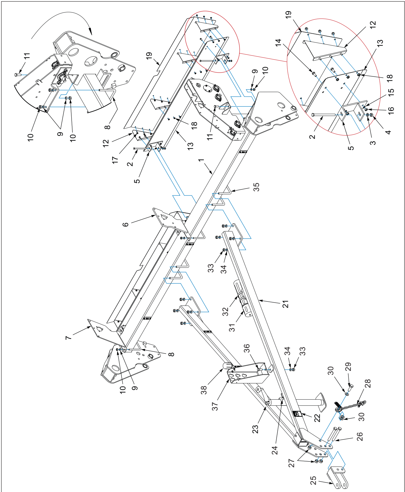
Figure 1-5: Drawbar Frame, Deflectors & Mounting - 10FT, 12FT (BEF. 08/2025)
