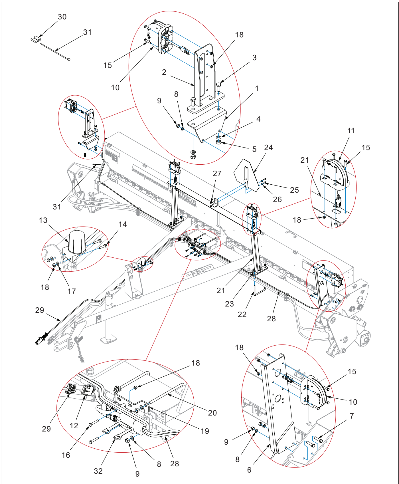
Figure 1-40: LED Warning Lamps - 12FT Drawbar Model (09/2013 TO 08/2025)
