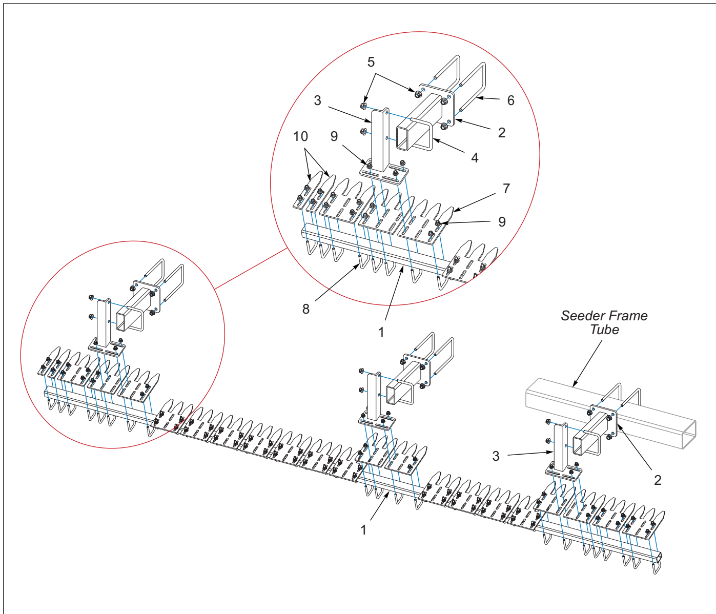
Figure 1-45: Scraper Kit, 12FT Tube Mounted - Optional
