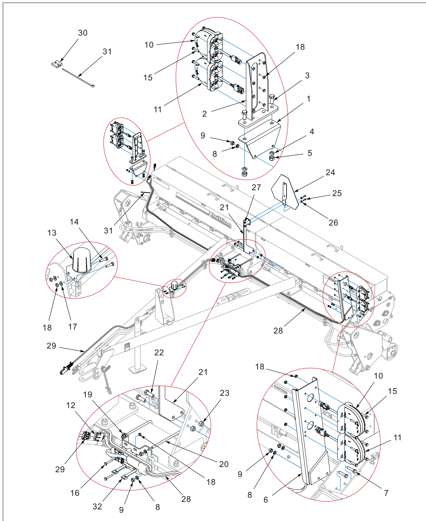
Figure 1-49: LED Warning Lamps - 8FT, 10FT (09/2013 TO 08/2025)
