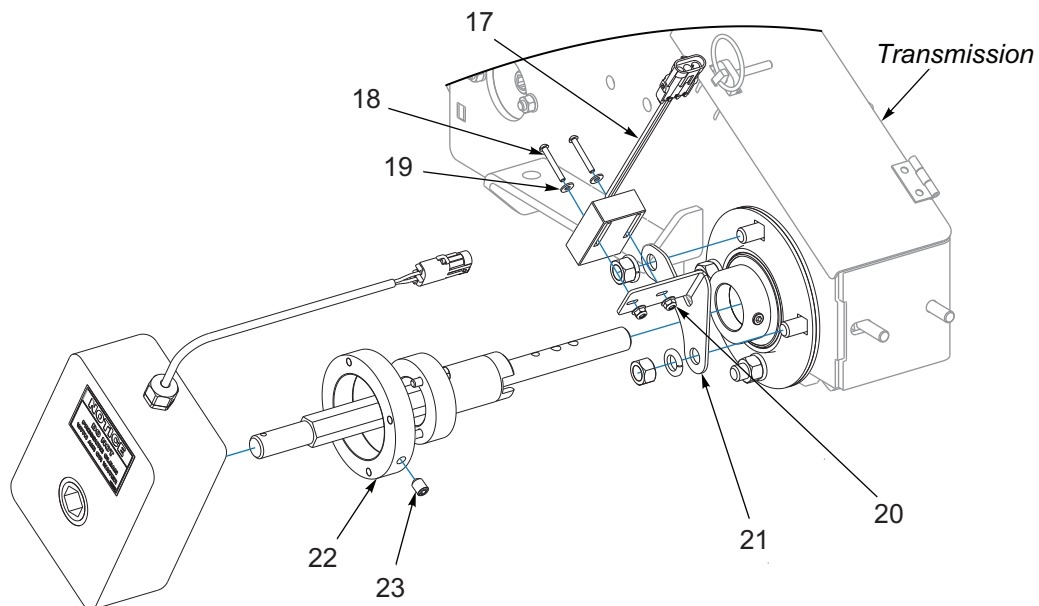
Figure 1-65: Brillion Elite Mini Monitor - Ground Speed
