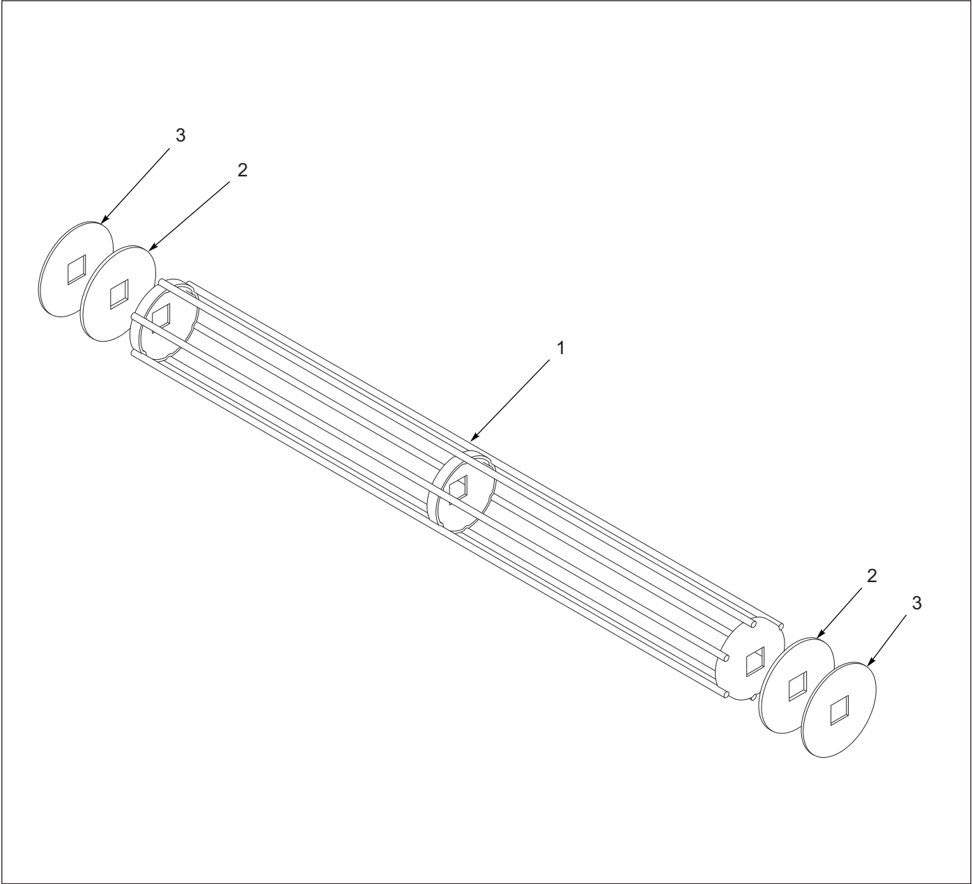
Figure 1-47: Agitator Cage - Optional
