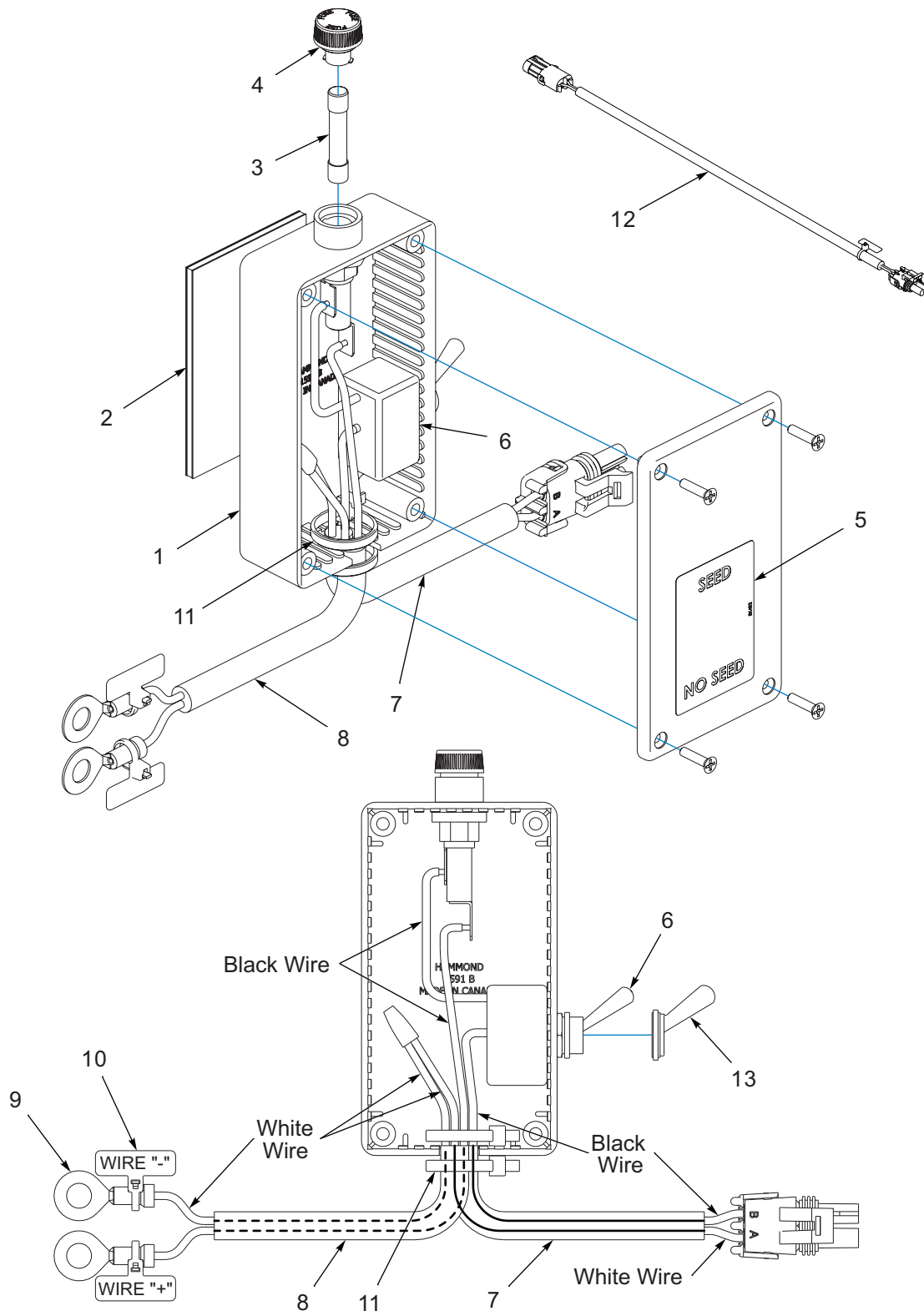
Figure 1-27: Clutch Switch Box - Optional
