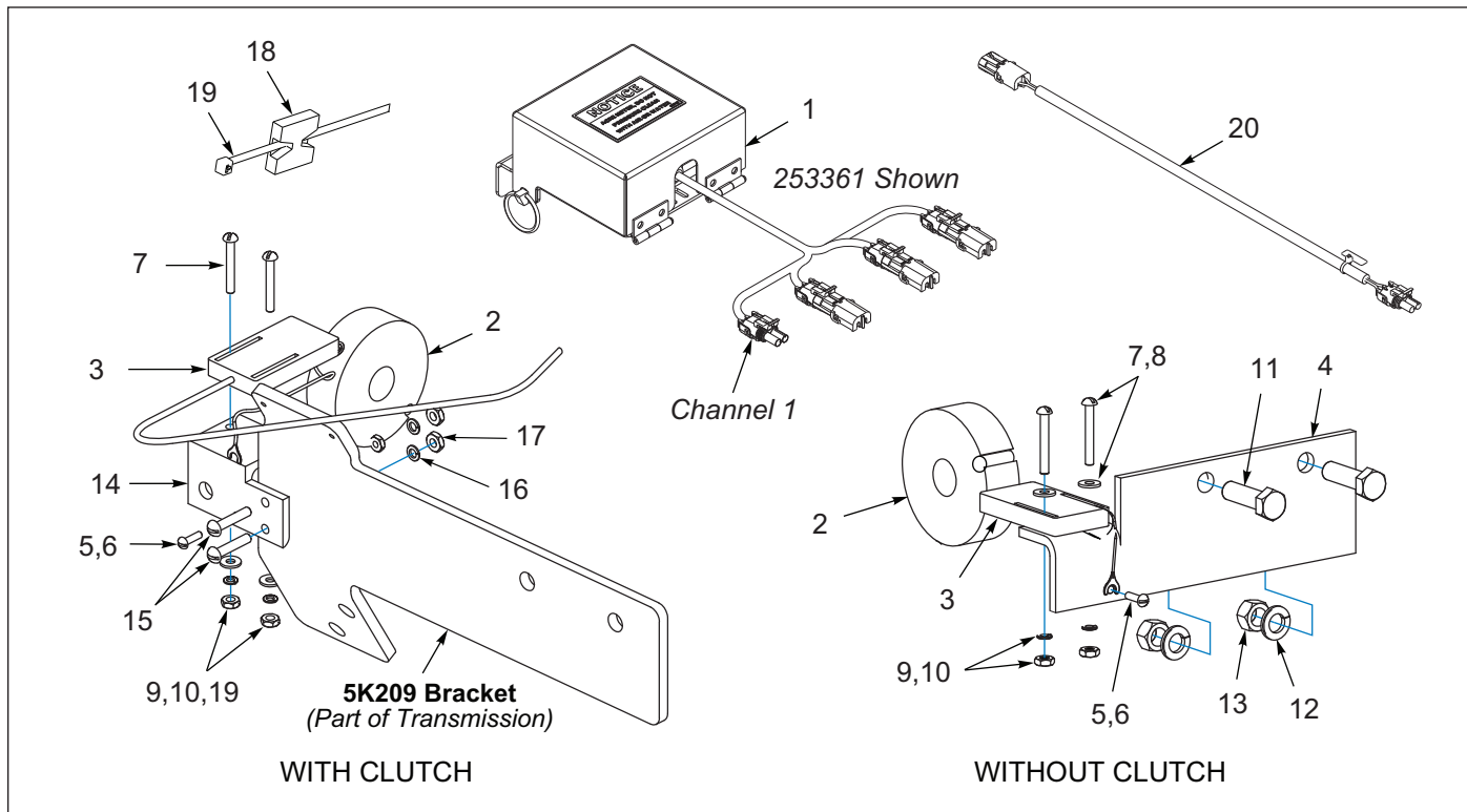
Figure 1-72: Electronic Acre Meter Assembly - Optional
