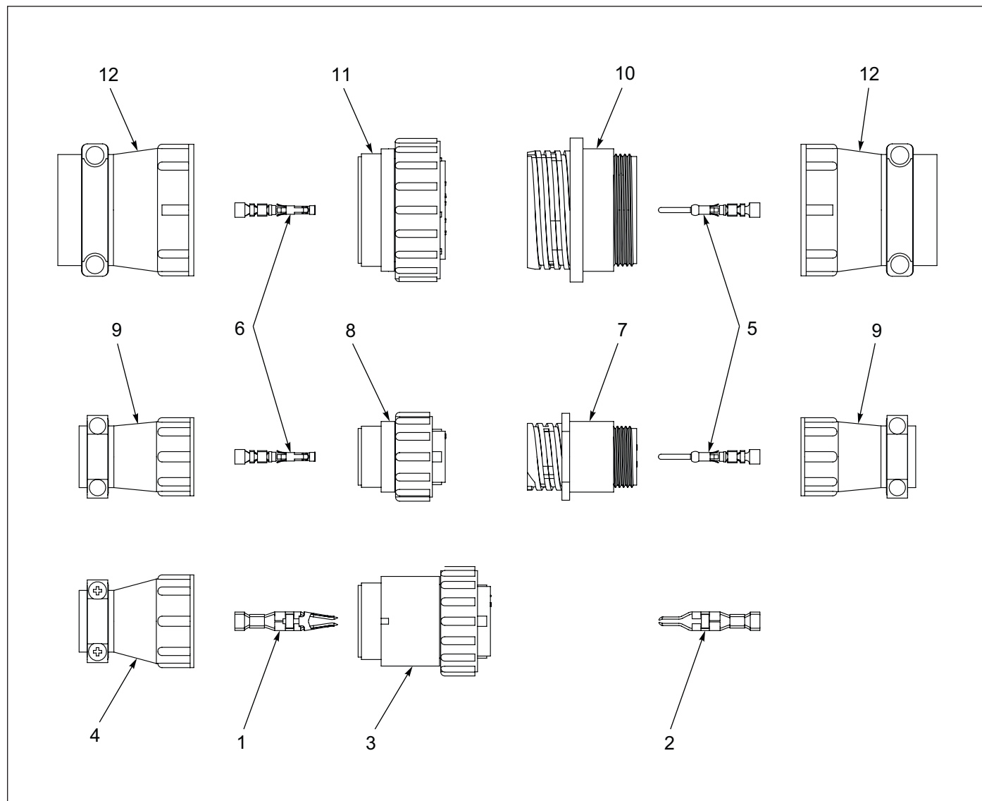
Figure 1-81: AMP Connectors
