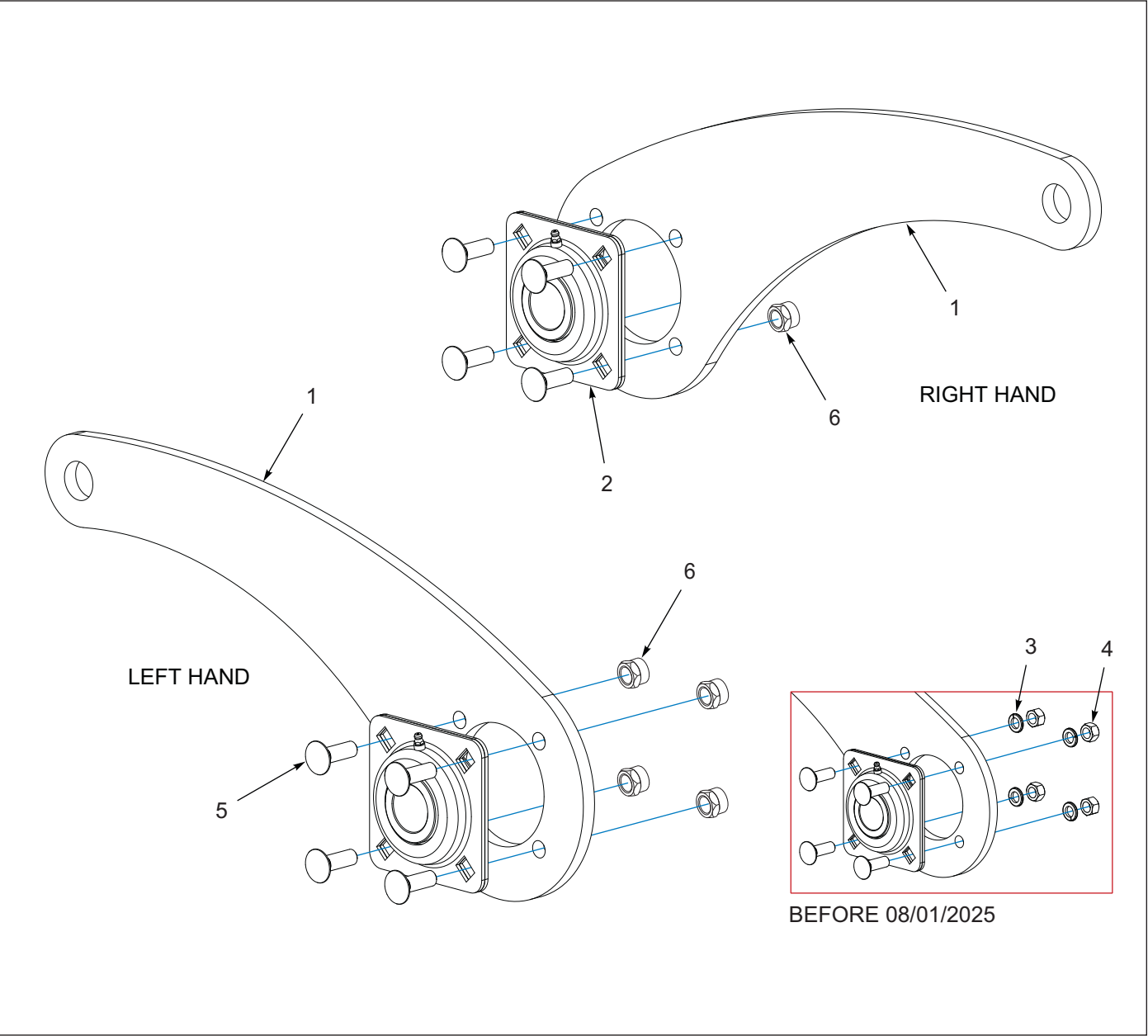
Figure 1-20: Rear Arm Assemblies
