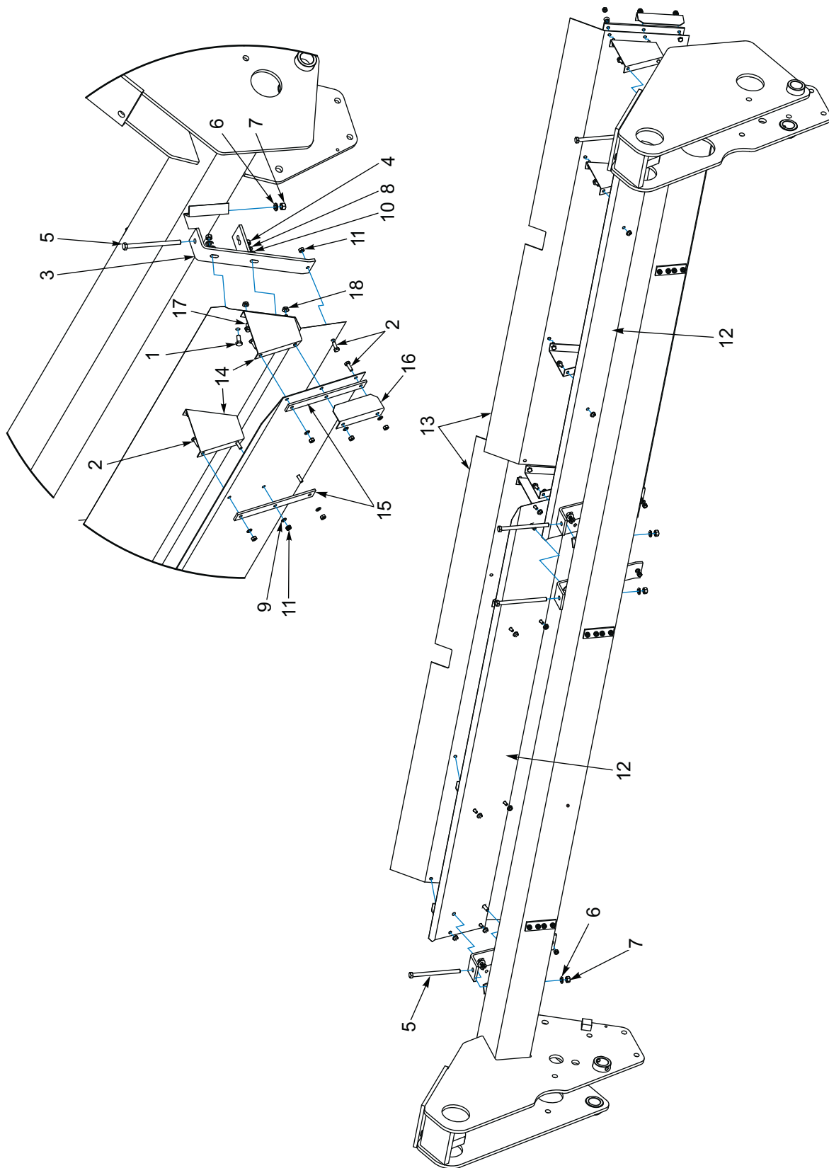
Figure 1-7: Deflectors, Shields, Brackets, and Hardware (BEF. 08/2025)
