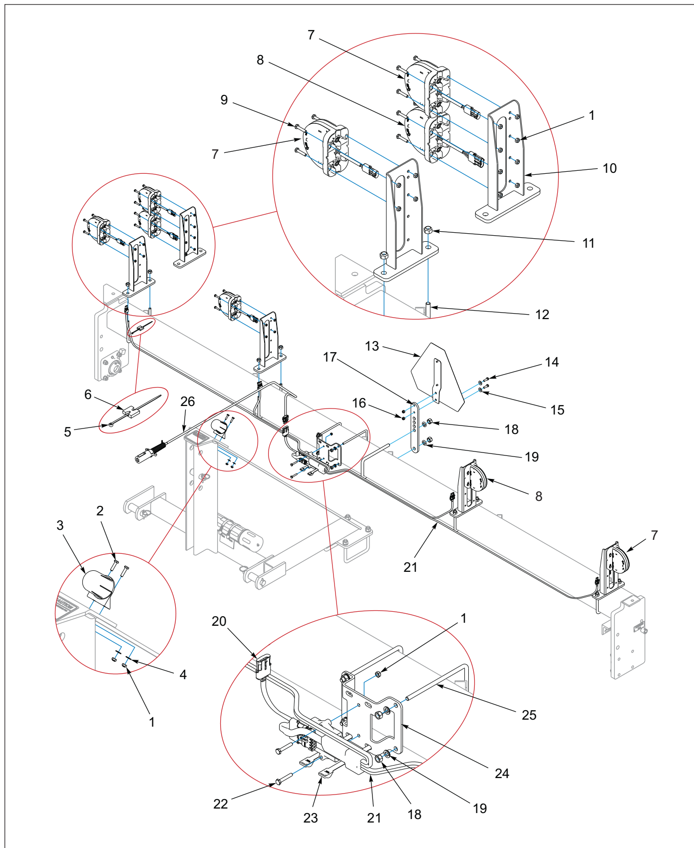
Figure 1-54: LED Warning Lamps - SD, 3-PT (09/2013 TO 08/2025)
