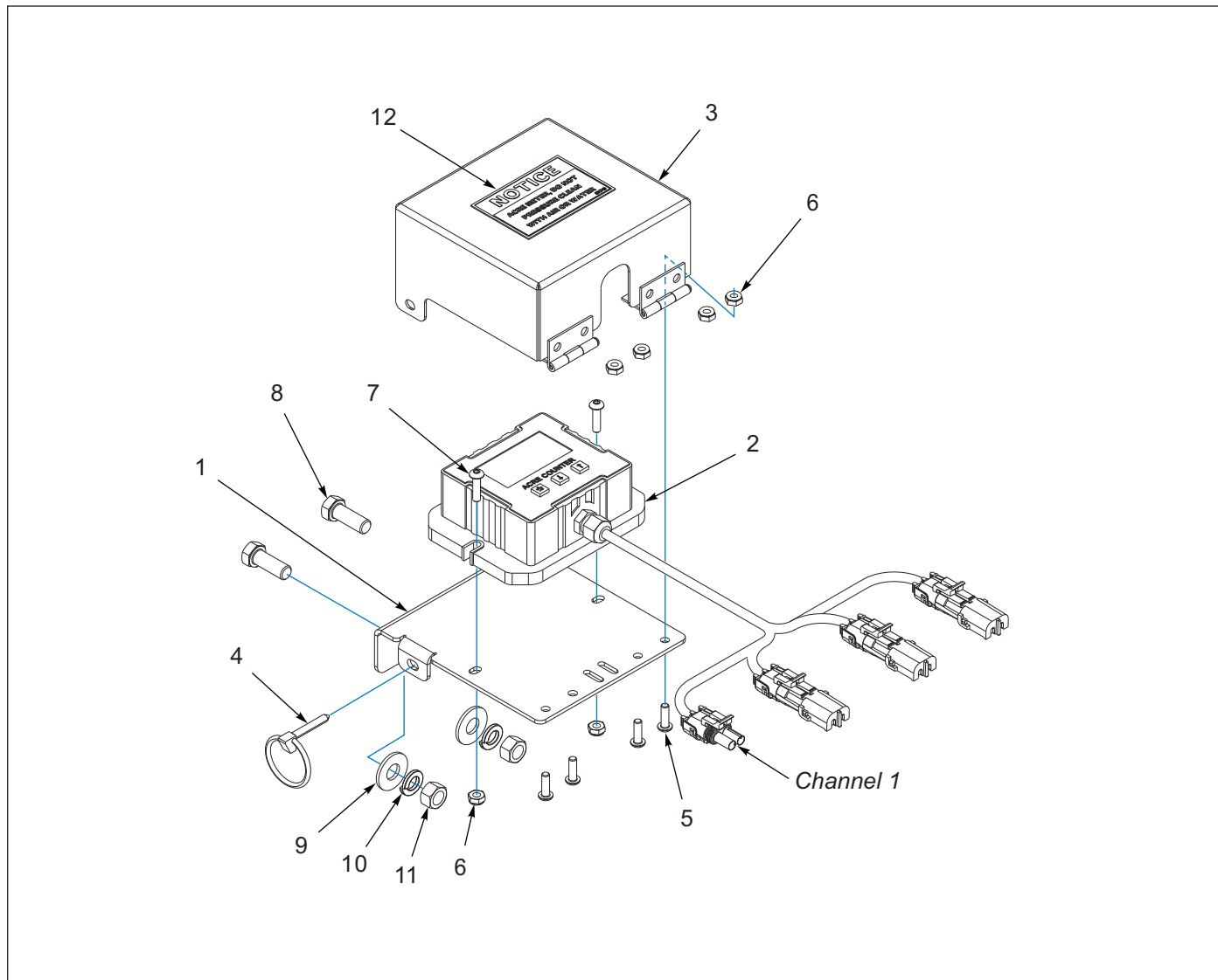
Figure 1-73: Acre Meter Assembly (AFTER 06/01/2025)
