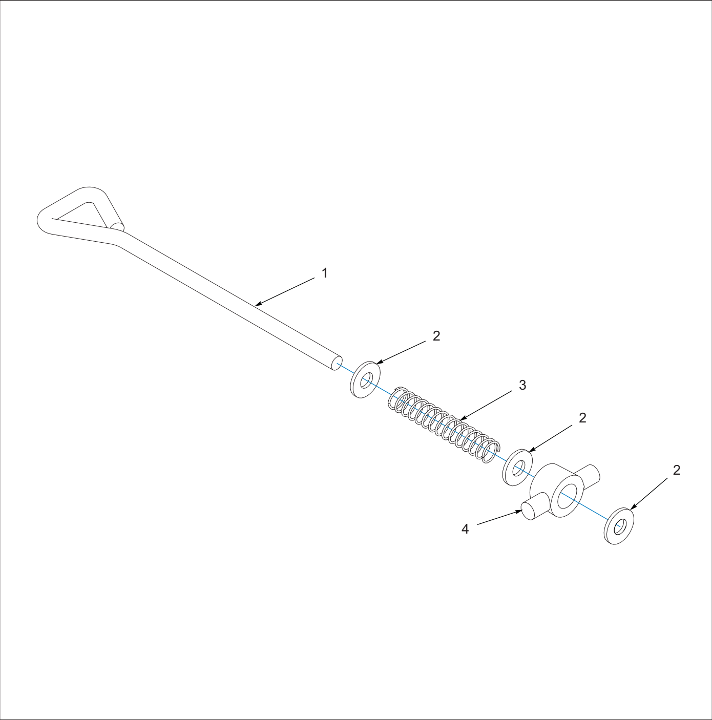
Figure 1-42: Cover Lock
