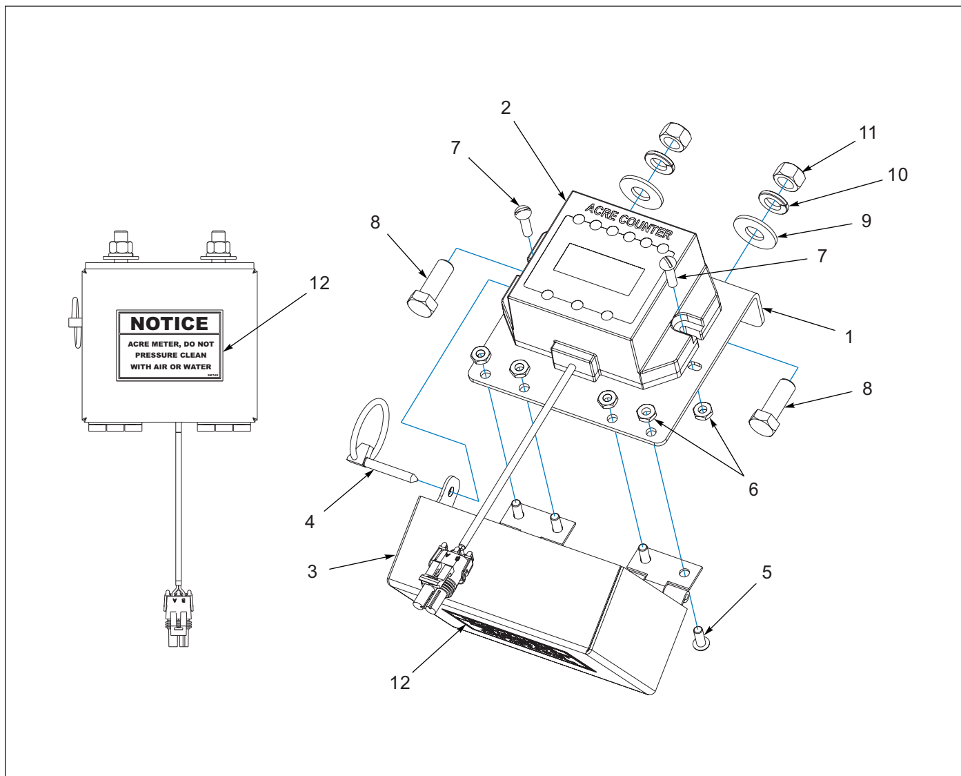
Figure 1-74: Acre Meter Assembly (05/15/2012 TO 06/01/2025)
