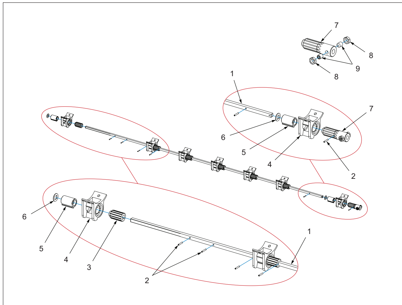
Figure 1-33: Seed Meter Assembly, Right-Hand
