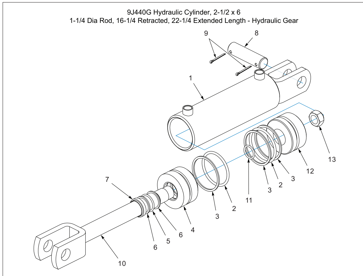
Figure 1-79: Hydraulic Cylinder, 2-1/2 x 6 - Hydraulic Gear (BEF. 01/14/2008)
