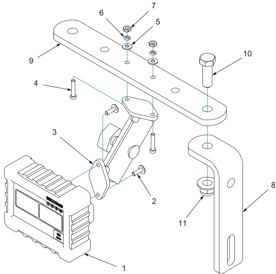
Figure 1-64: Brillion Elite Mini Monitor Tractor Mount
