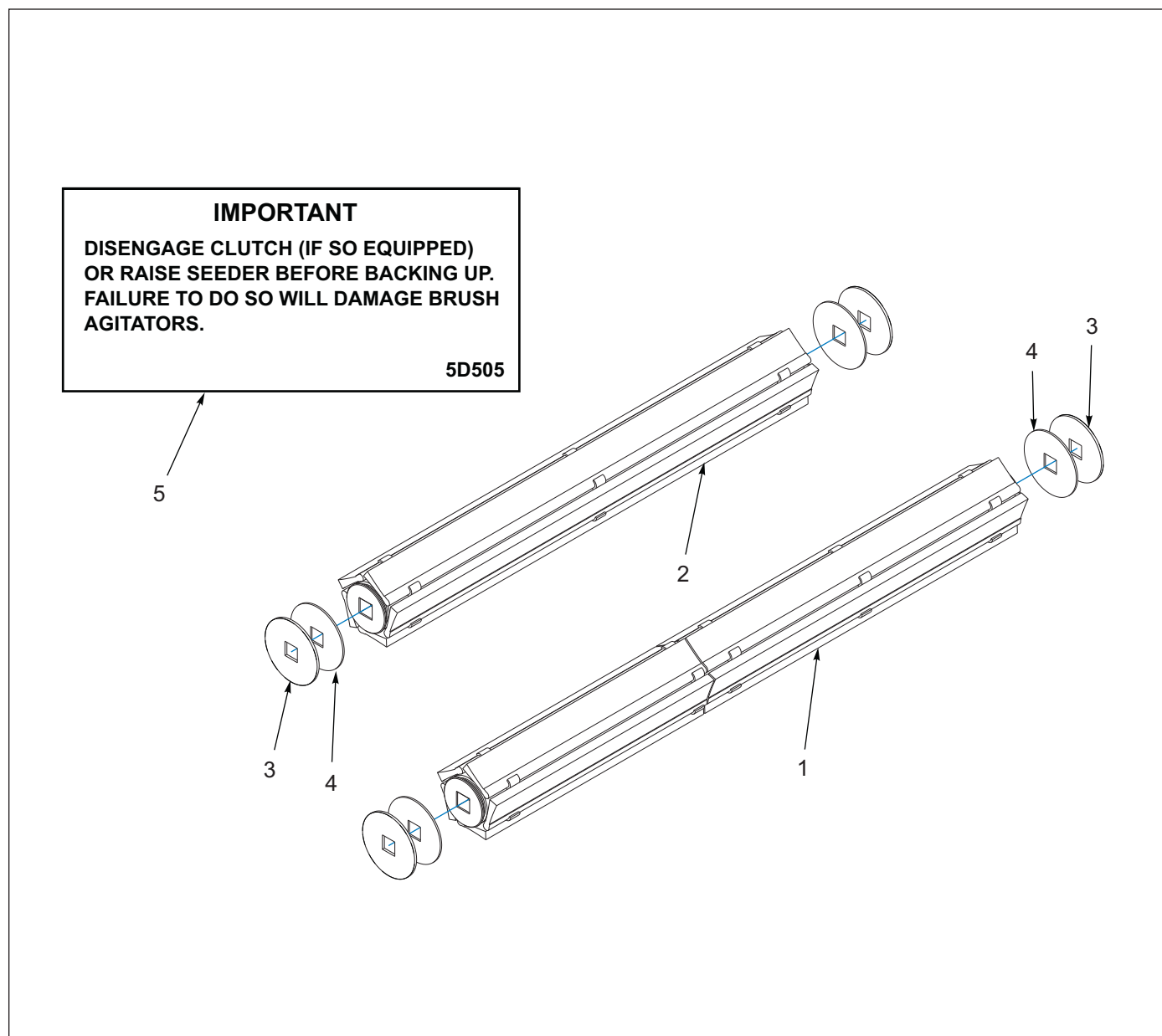
Figure 1-44: 5-Strip Brush Agitator Kit - Optional
