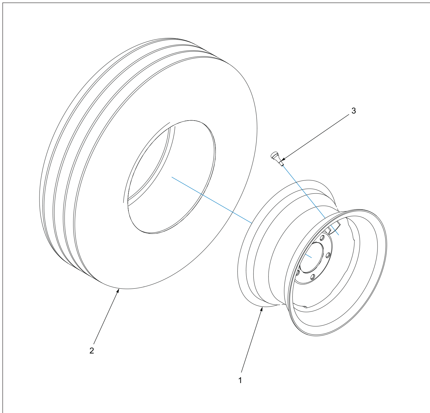
Figure 1-12: Tire and Wheel Assembly - 5 Bolt (BEFORE 05/2021)
