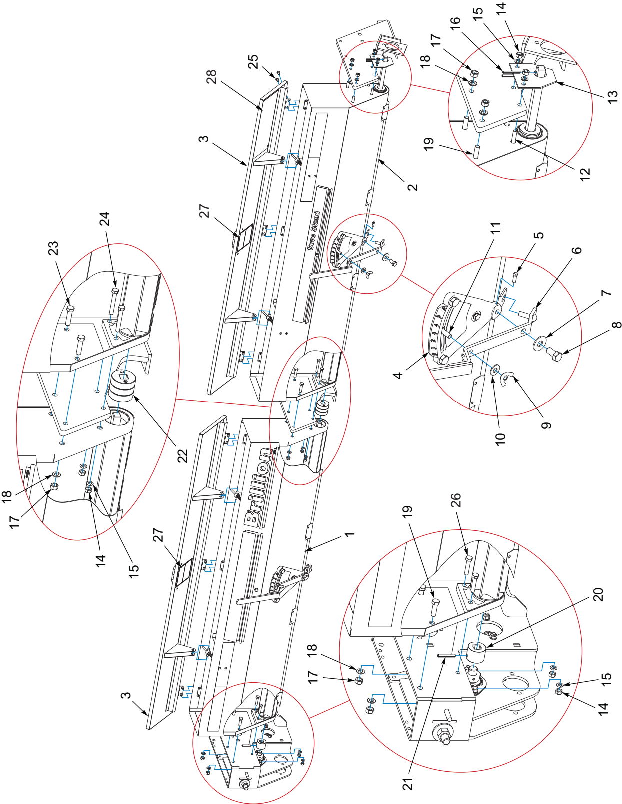
Figure 1-35: Rear Seed Box (Before 08/2025)
