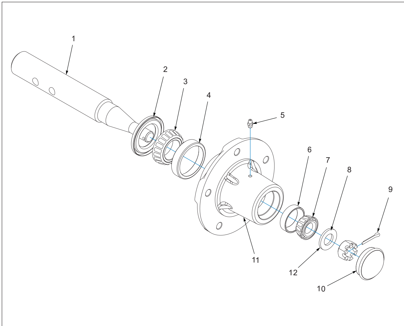
Figure 1-10: Hub and Spindle Assembly - 5 Bolt (BEFORE 05/2021)
