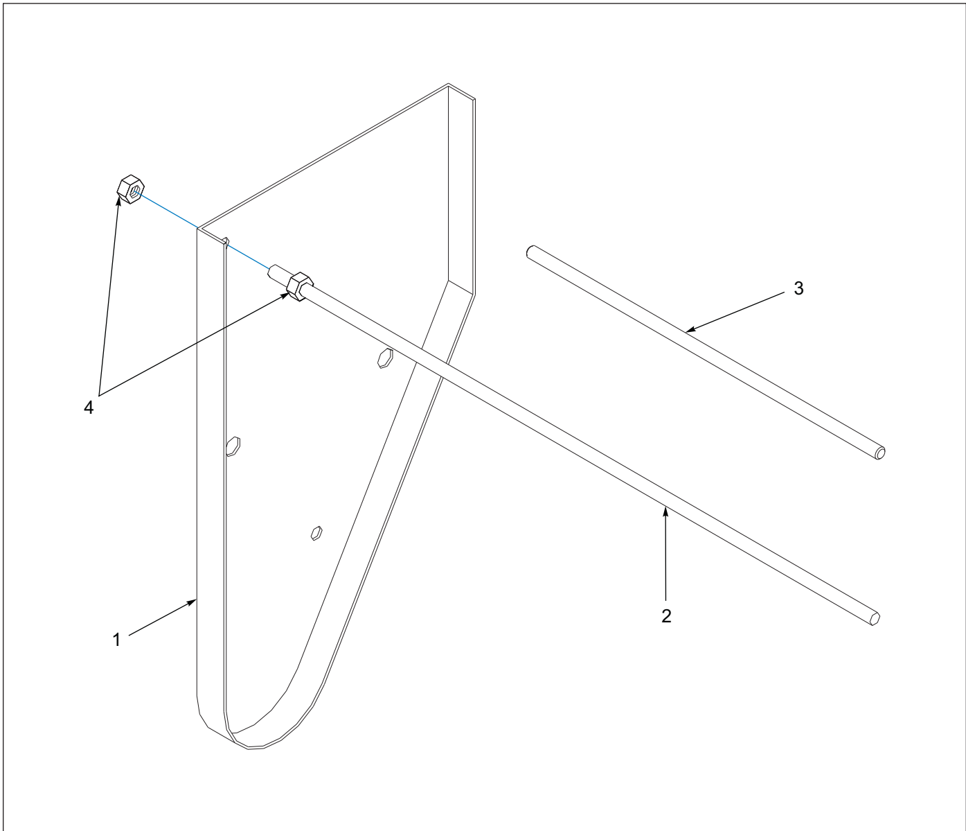
Figure 1-76: Small Meter Seed Box Divider Kit - Optional
