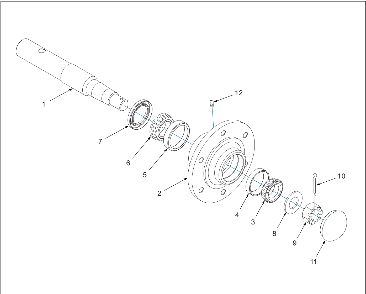
Figure 1-9: Hub and Spindle Assembly - 6 Bolt (AFTER 05/2021)
