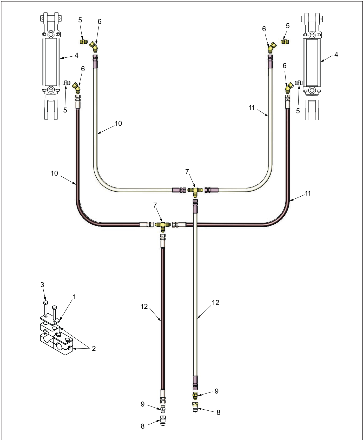
Figure 1-15: Hydraulic Schematic
