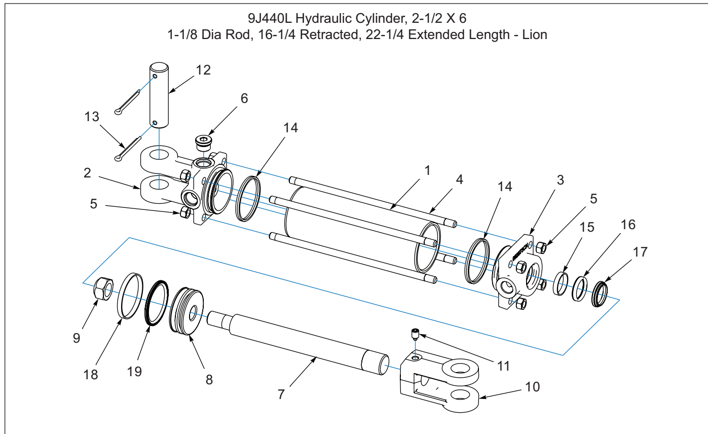
Figure 1-78: Hydraulic Cylinder, 2-1/2 x 6 - Lion (AFT. 01/15/2008)
