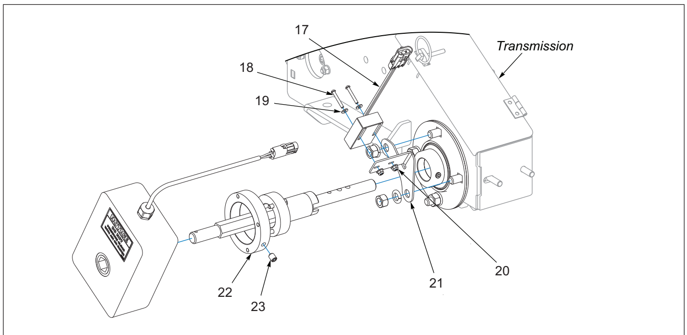
Figure 1-55: Brillion Elite Mini Monitor - Ground Speed
