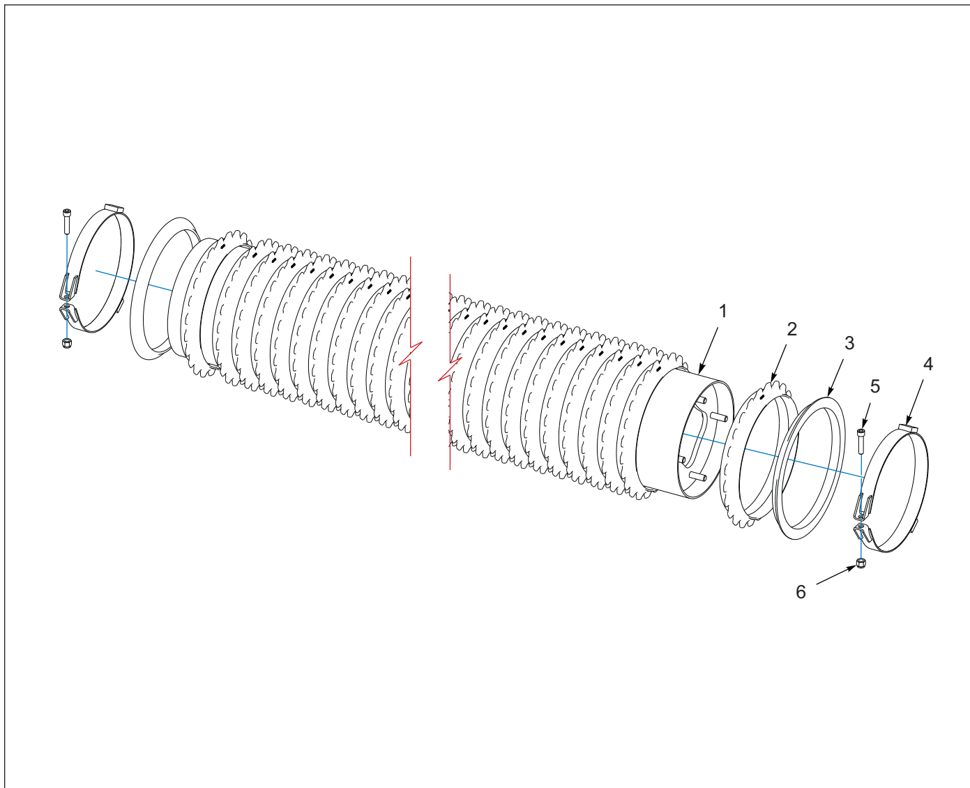
Figure 1-19: Front Roller, 4 - Bolt
