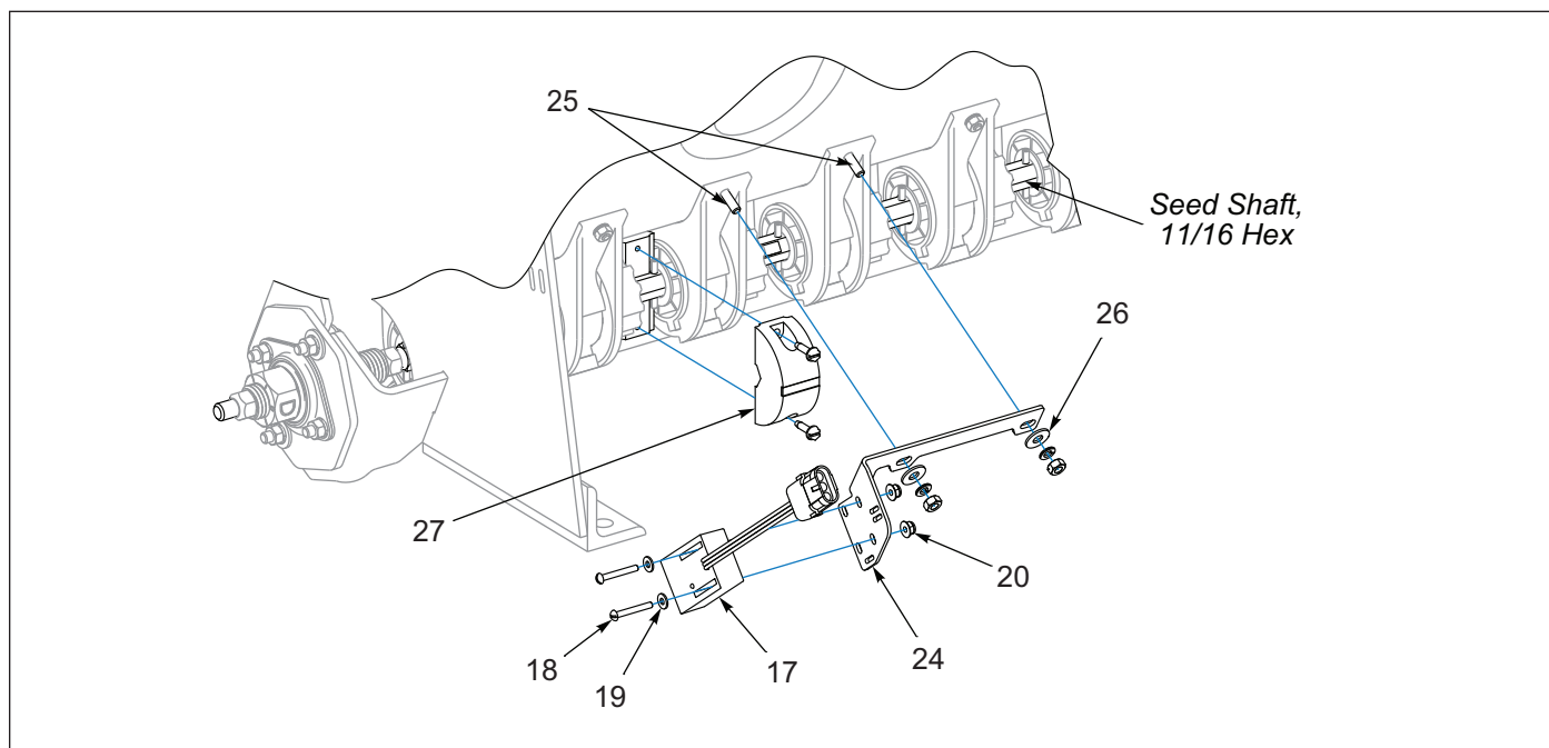
Figure 1-60: Brillion Elite Mini Monitor - Front Seed Box Seed Shaft Sensor
