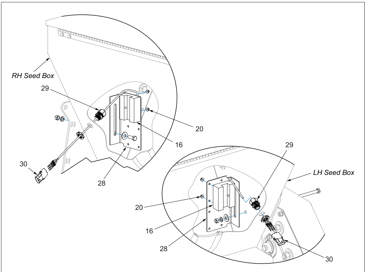
Figure 1-57: Brillion Elite Mini Monitor - Front Seed Box Bin Level Sensor
