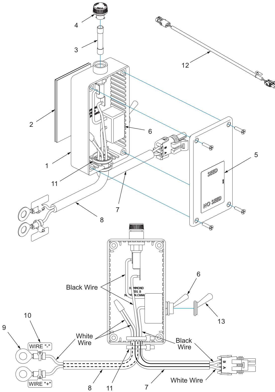
Figure 1-27: Clutch Switch Box
