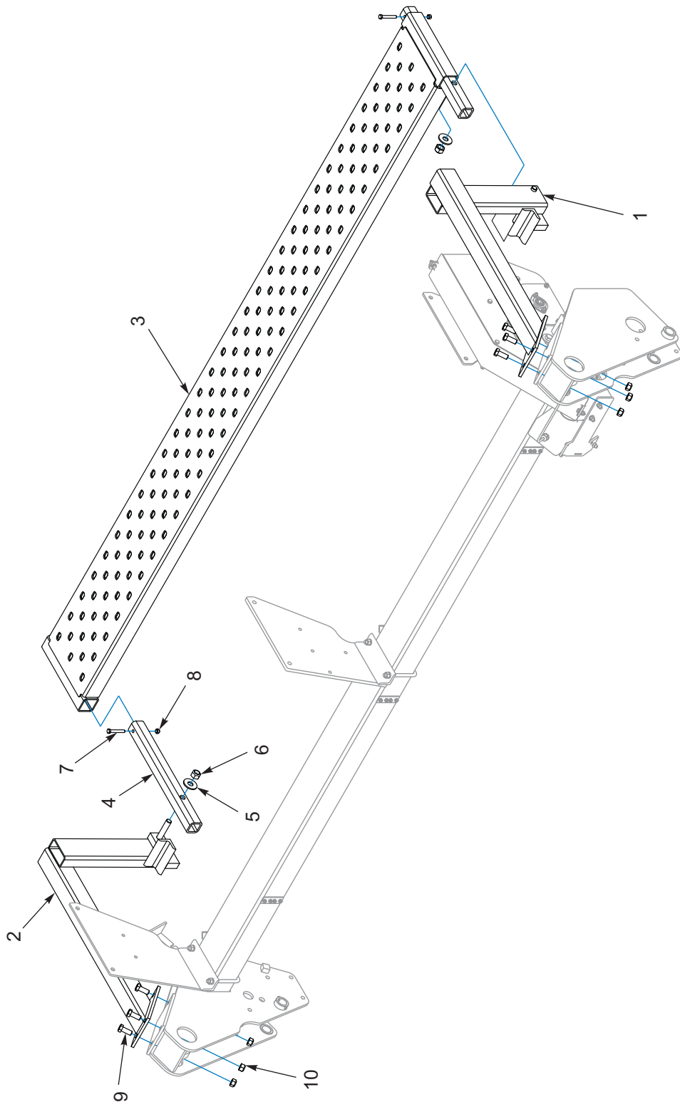
Figure 1-28: Drawbar Walk Board - 8FT and 10FT
