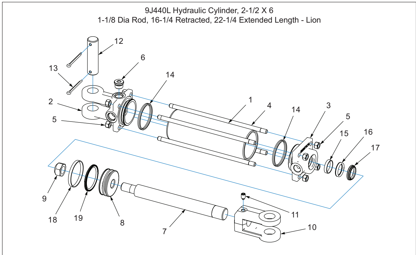
Figure 1-71: Hydraulic Cylinder, 2-1/2 x 6 - Lion (After 01/15/2008)
