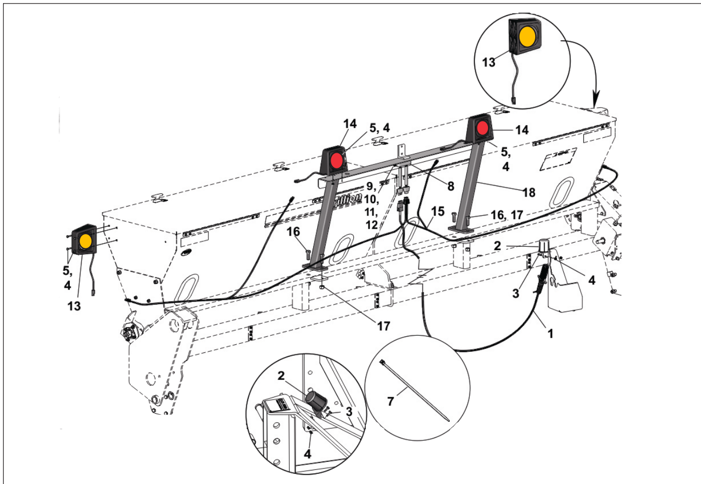
Figure 1-45: Warning Lamp Kit - 12FT (Before 09/2013)
