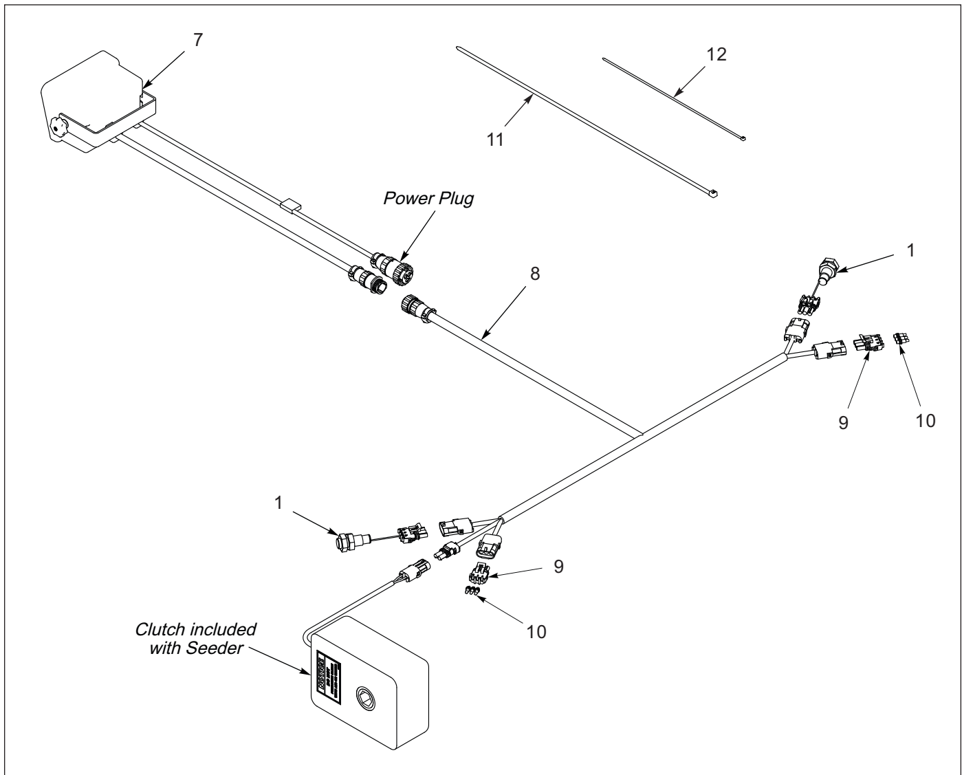
Figure 1-69: Console w/Clutch Control Electrical Schematic - Optional
