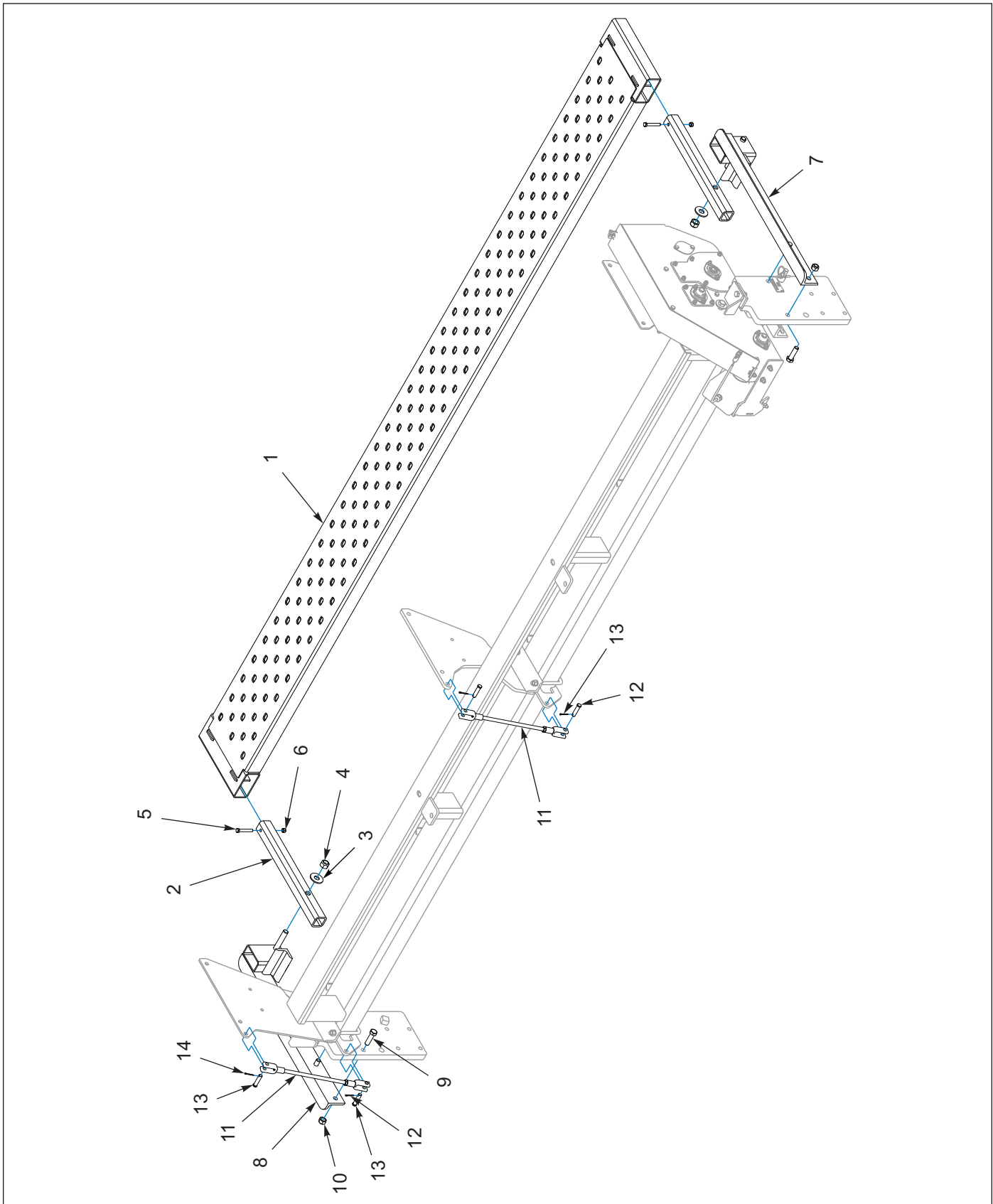
Figure 1-31: 3-PT Walk Board - 12FT
