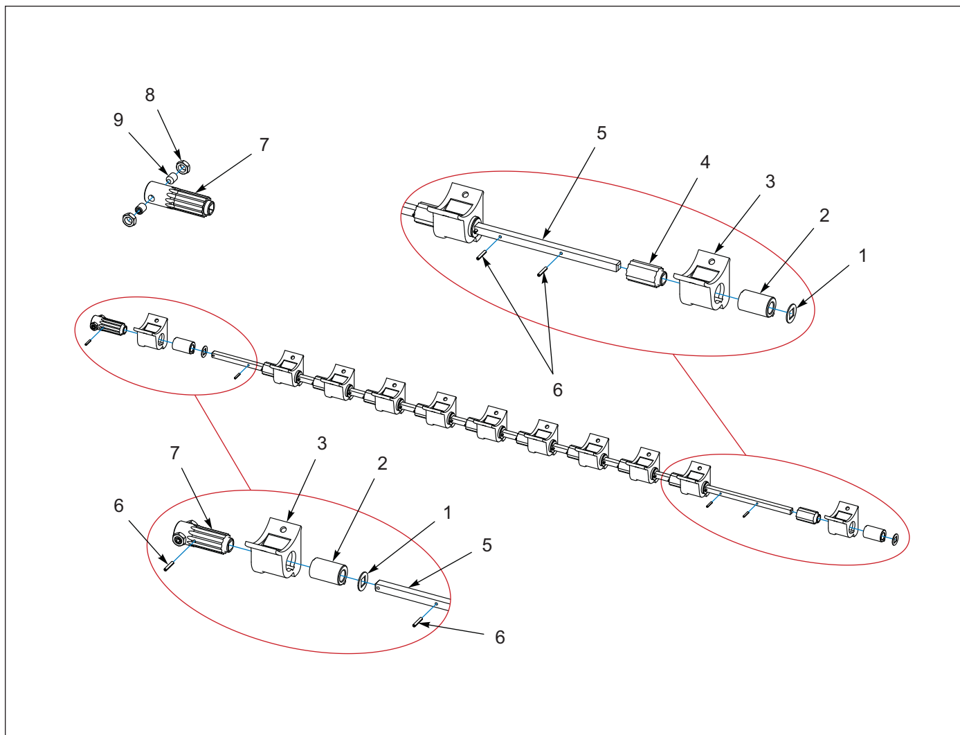
Figure 1-40: Seed Shaft Assembly, Left Hand
