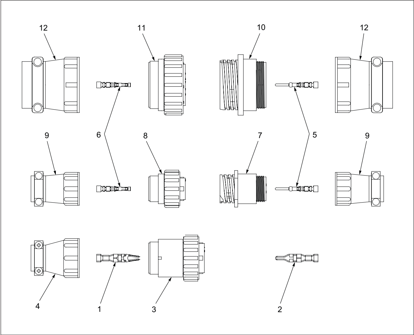
Figure 1-74: AMP Connectors
