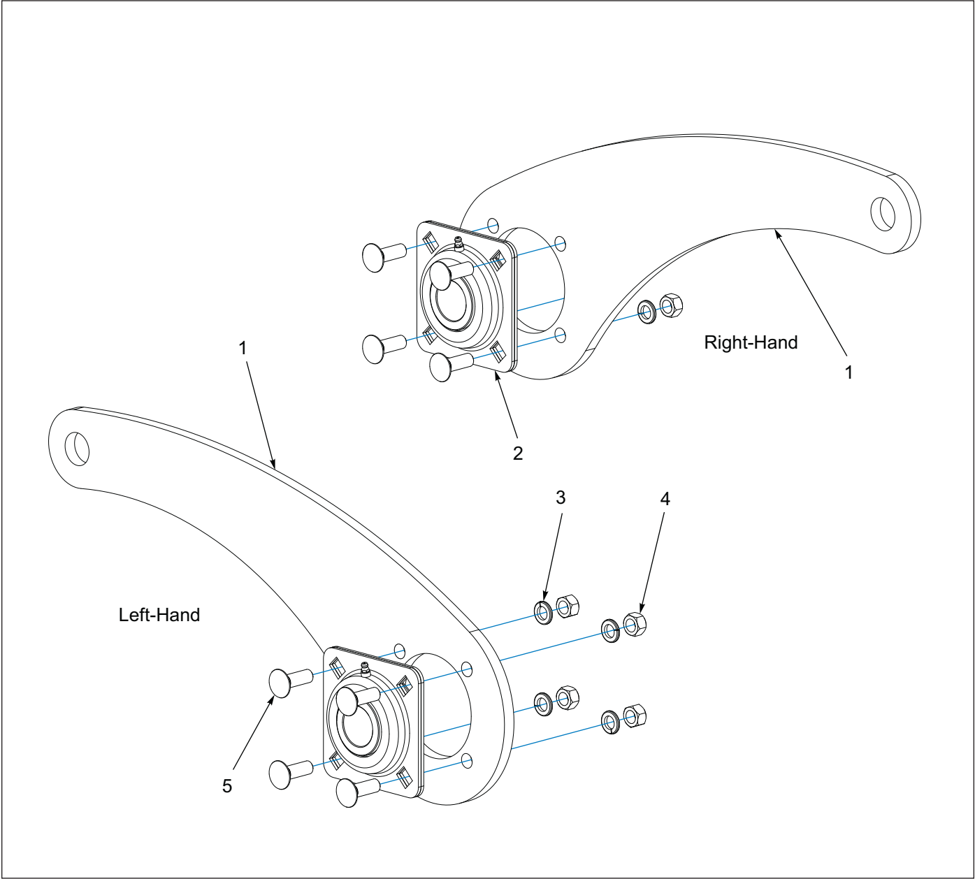
Figure 1-21: Rear Arm Assemblies
