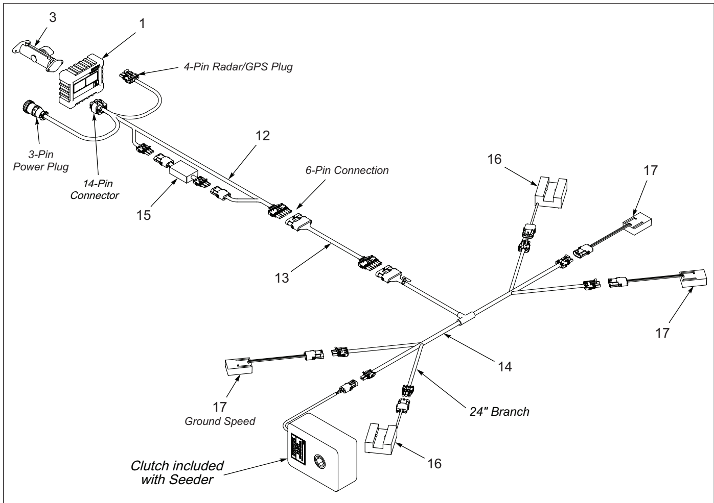
Figure 1-58: Brillion Elite Mini Monitor - Double Seed Box Electrical Schematic
