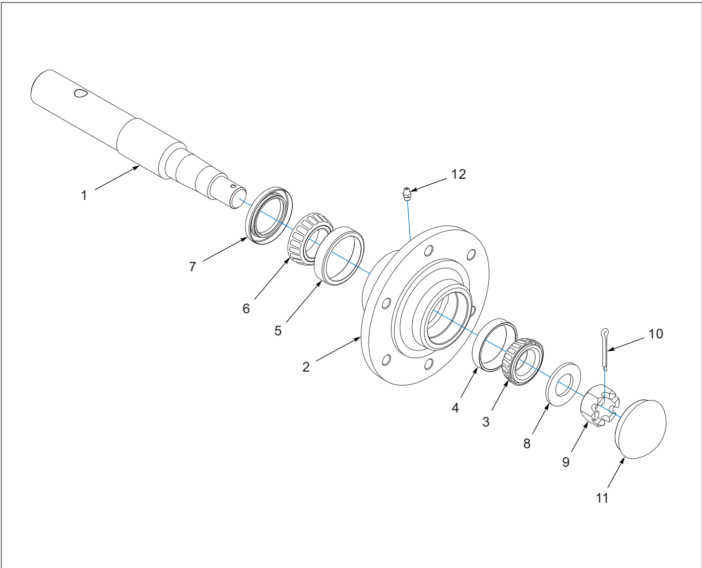
Figure 1-10: Hub and Spindle Assembly - 6 Bolt (After 05/2021)
