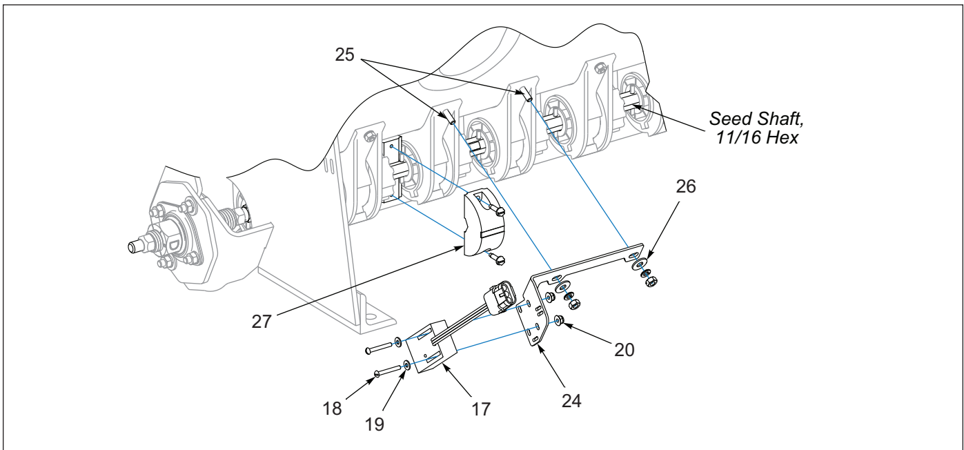
Figure 1-56: Brillion Elite Mini Monitor - Front Seed Box Seed Shaft Sensor
