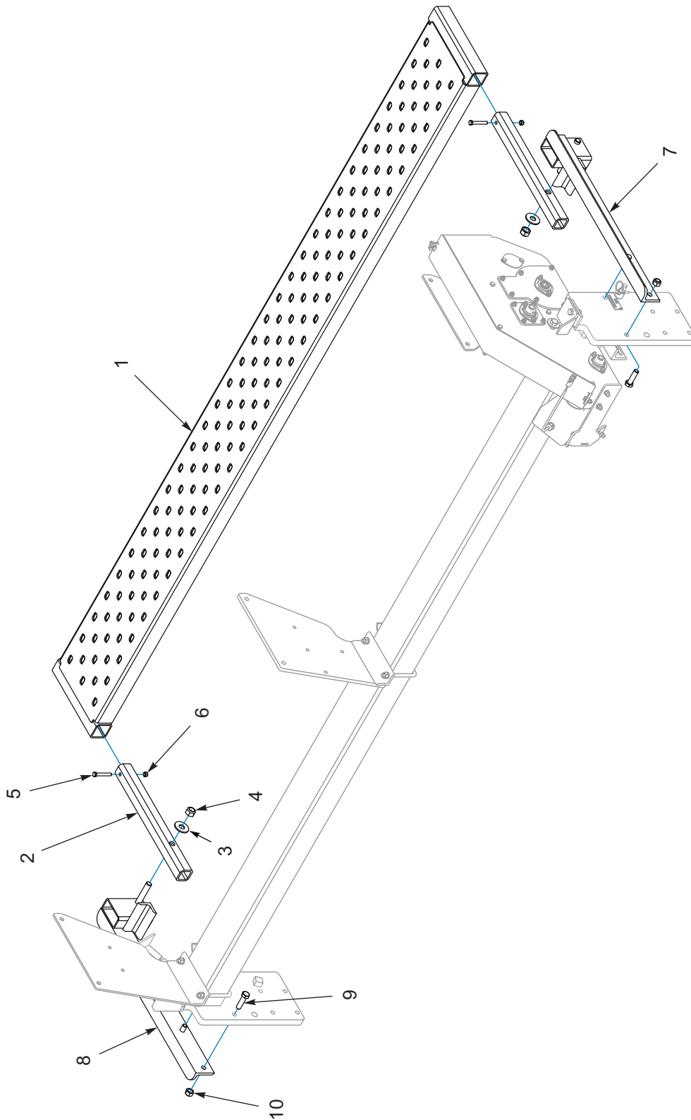
Figure 1-30: 3-PT Walk Board - 8FT and 10FT
