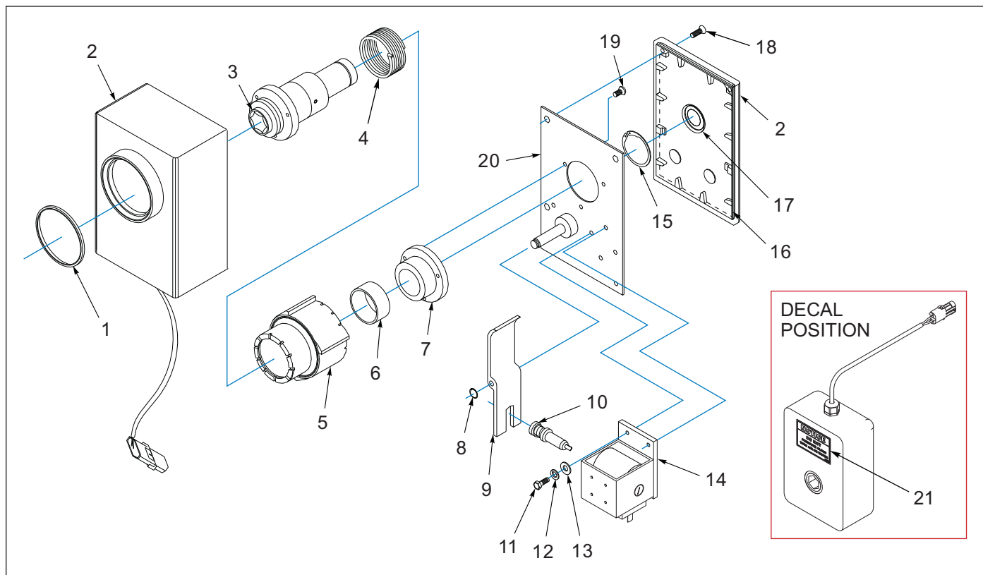
Figure 1-26: Electric Clutch
