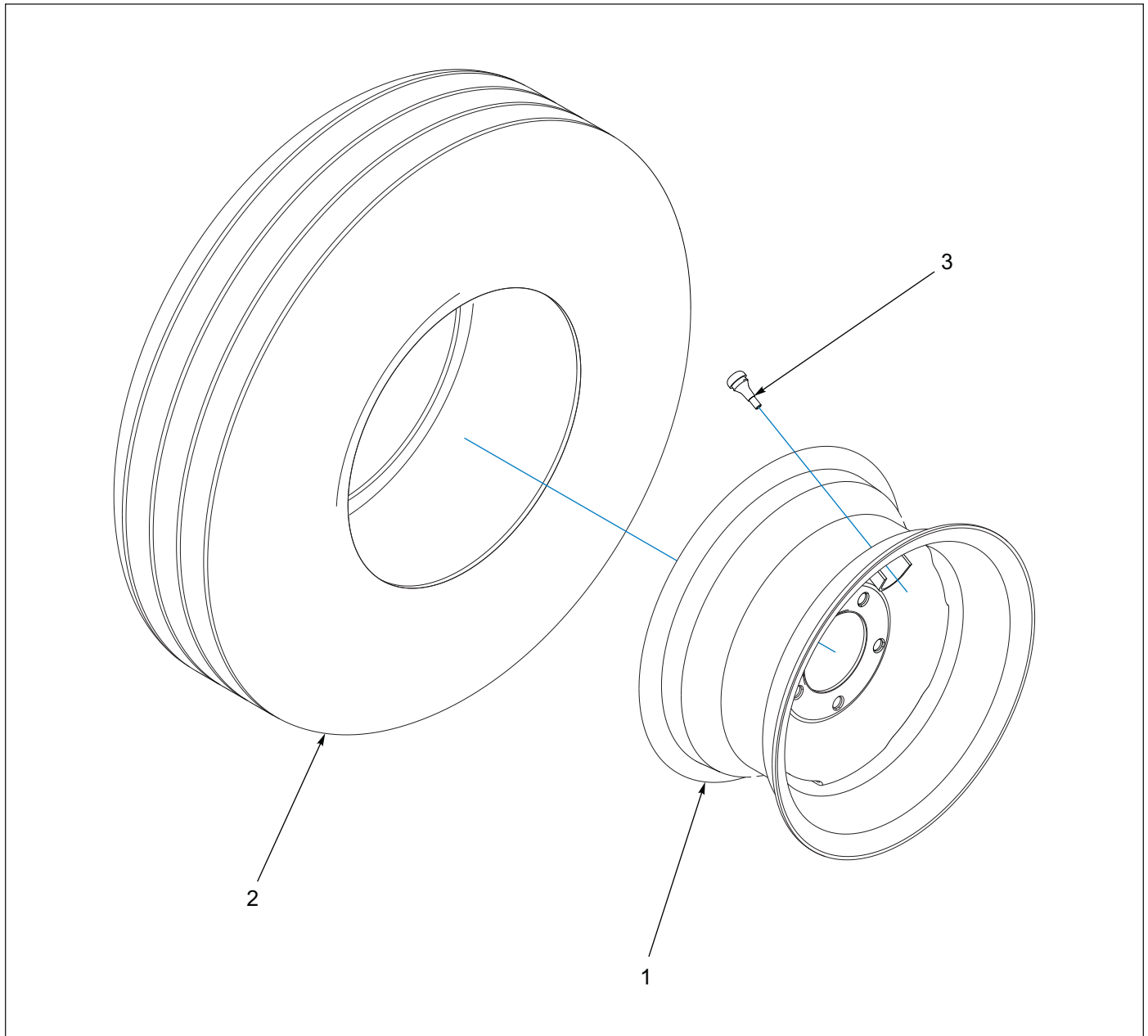
Figure 1-13: Tire and Wheel Assembly - 5 Bolt (Before 05/2021)
