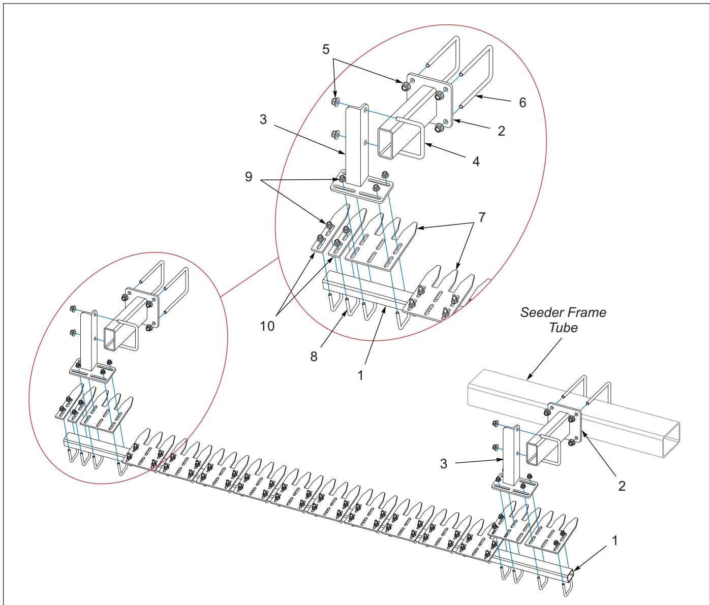
Figure 1-47: Scraper Kit, 8FT Tube Mounted - Optional
