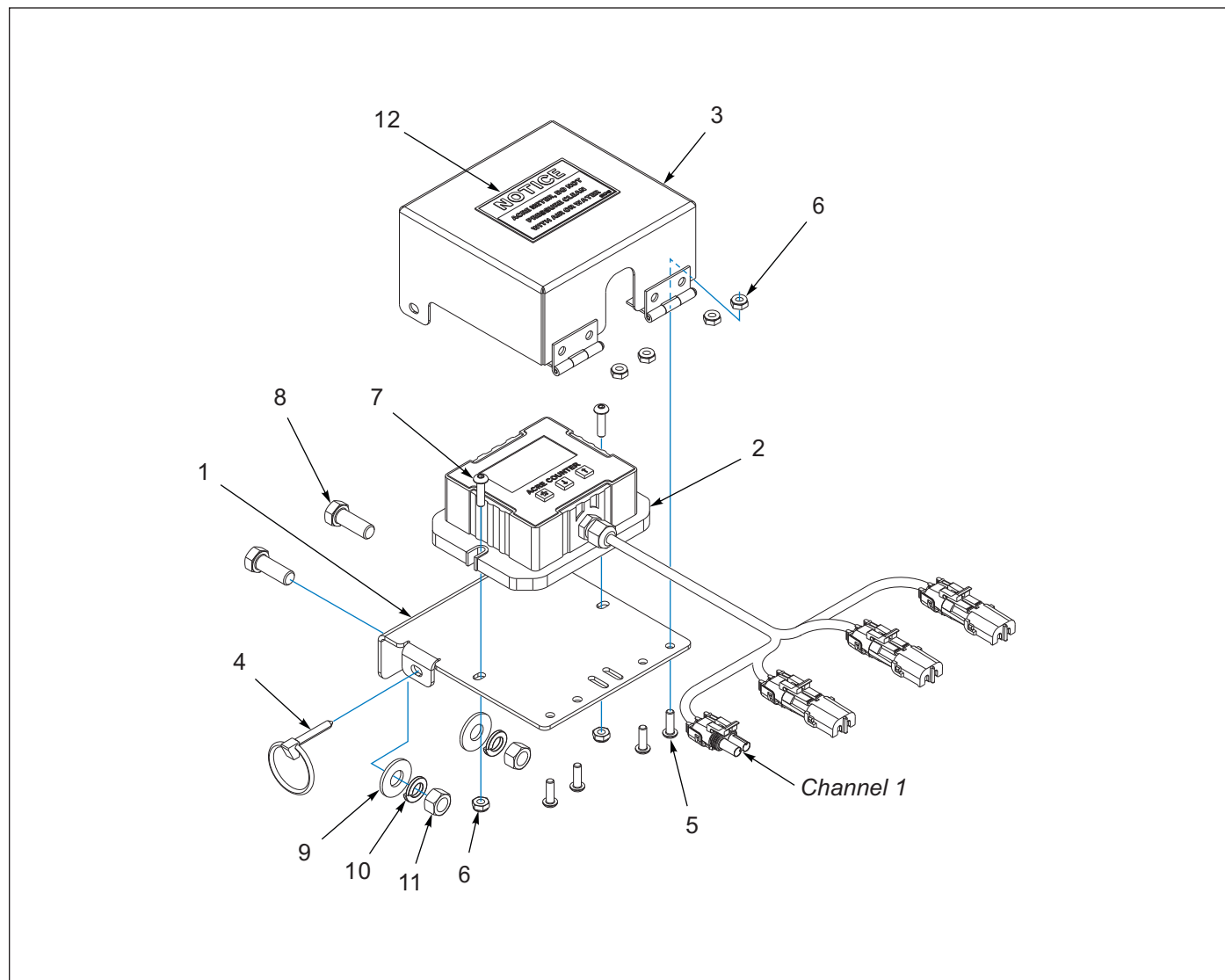
Figure 1-65: Acre Meter Assembly (After 06/01/2025)
