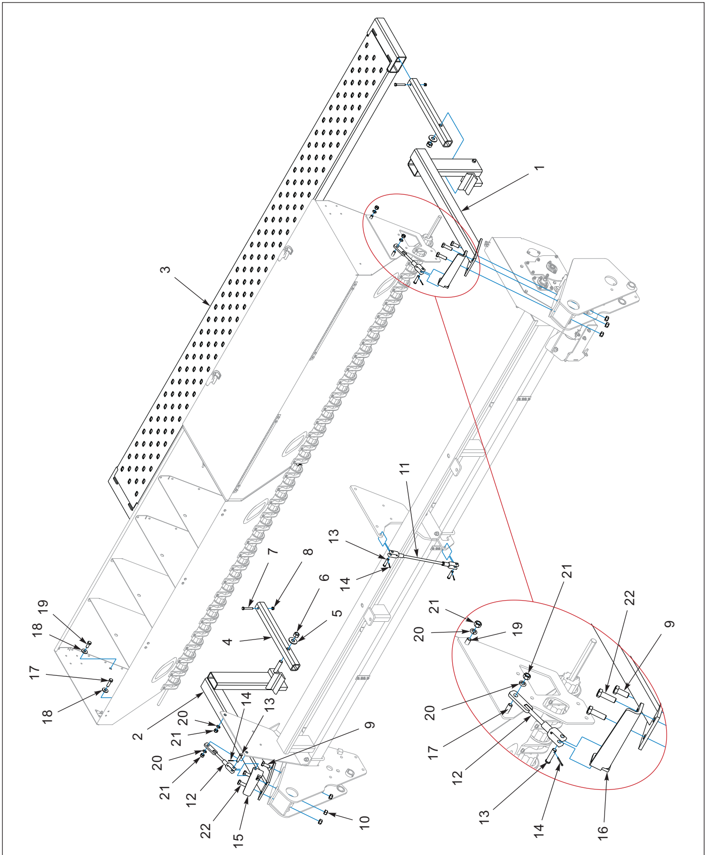
Figure 1-29: Drawbar Walk Board - 12FT
