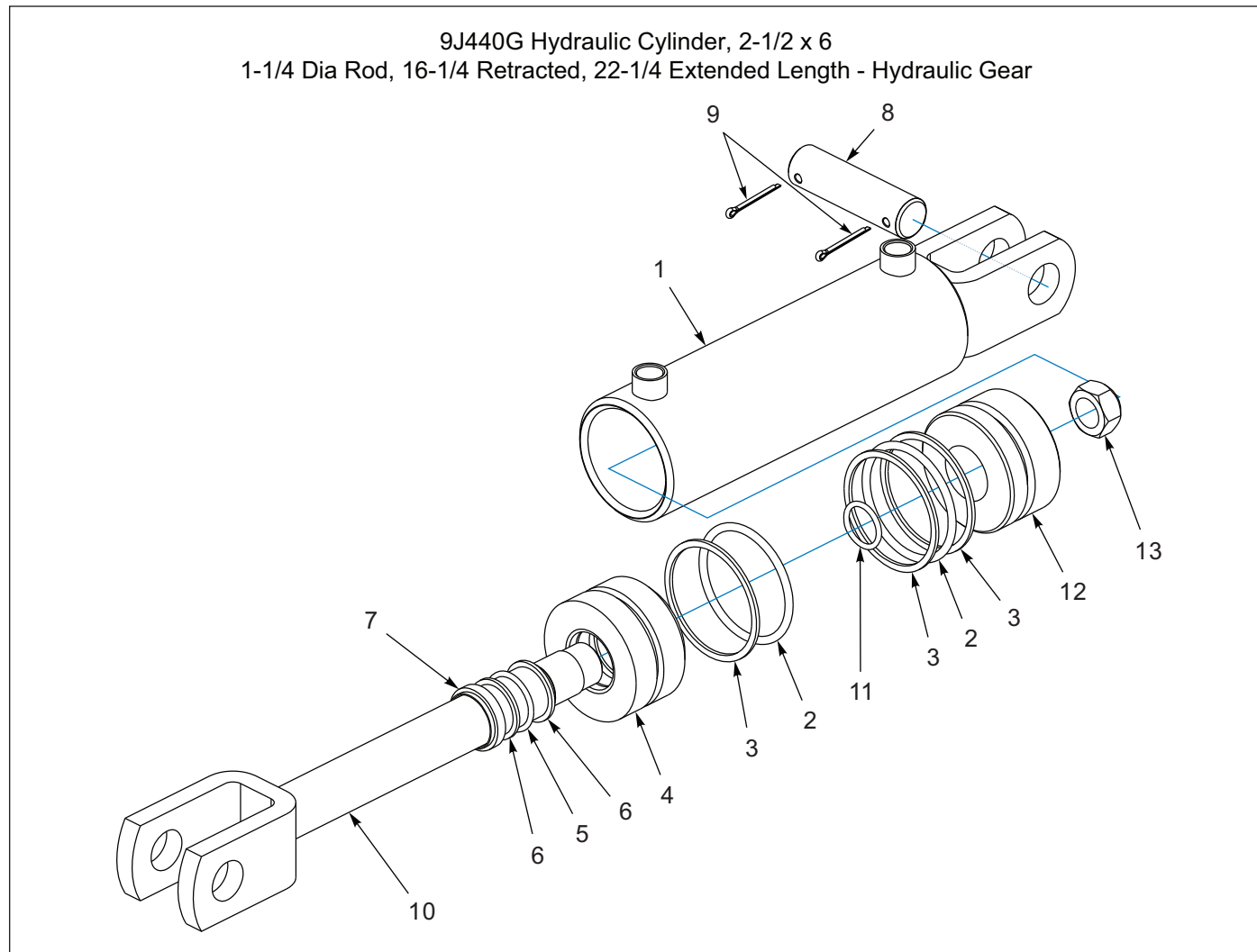
Figure 1-72: Hydraulic Cylinder, 2-1/2 x 6 - Hydraulic Gear (Before 01/14/2008)
