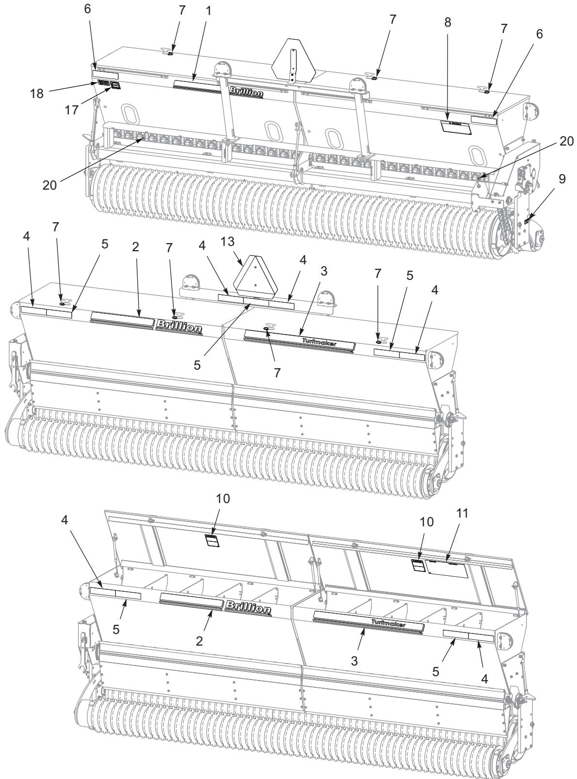
Figure 1-78: Decal Placement - Single Box, 12FT
