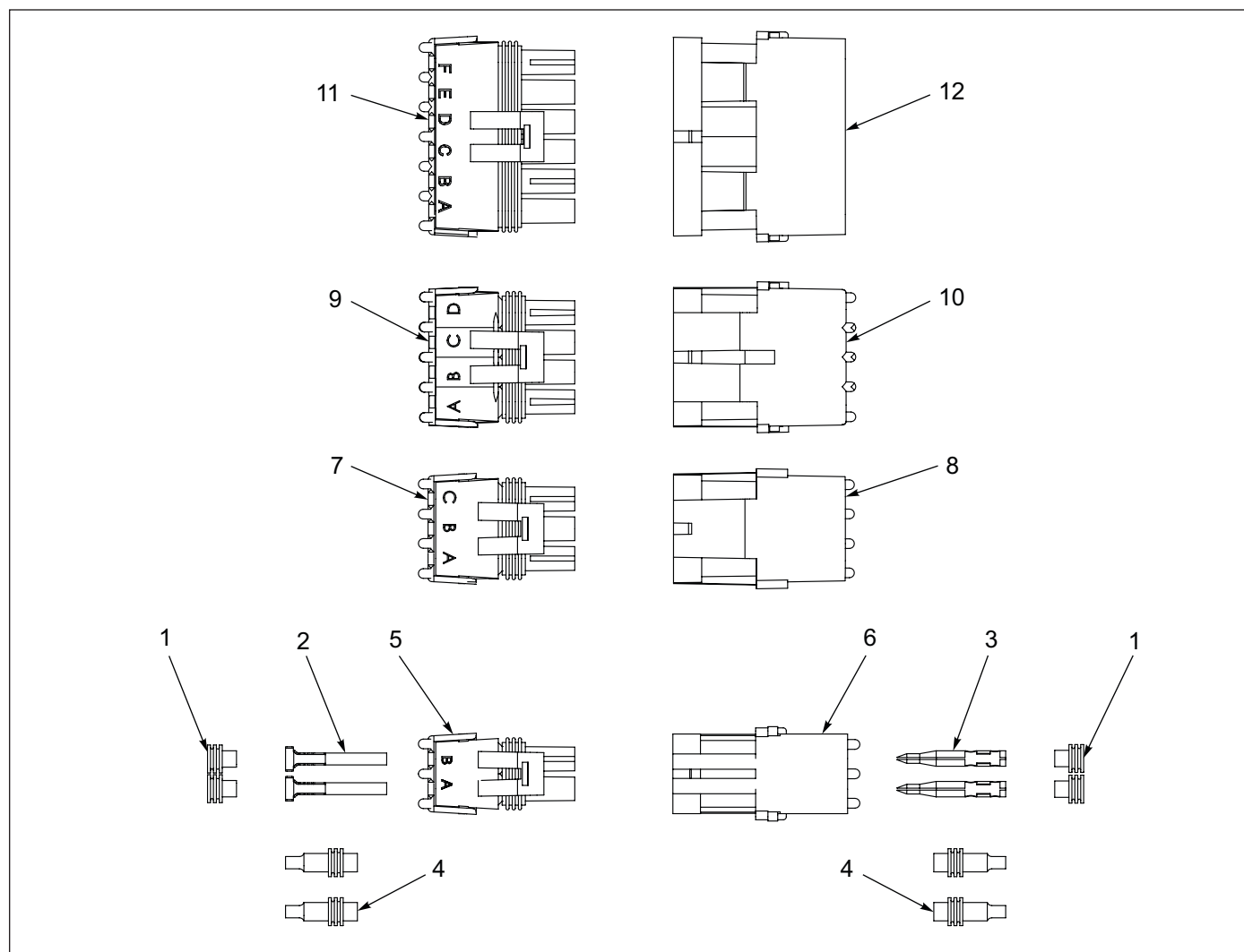
Figure 1-73: Weather Pack Connectors
