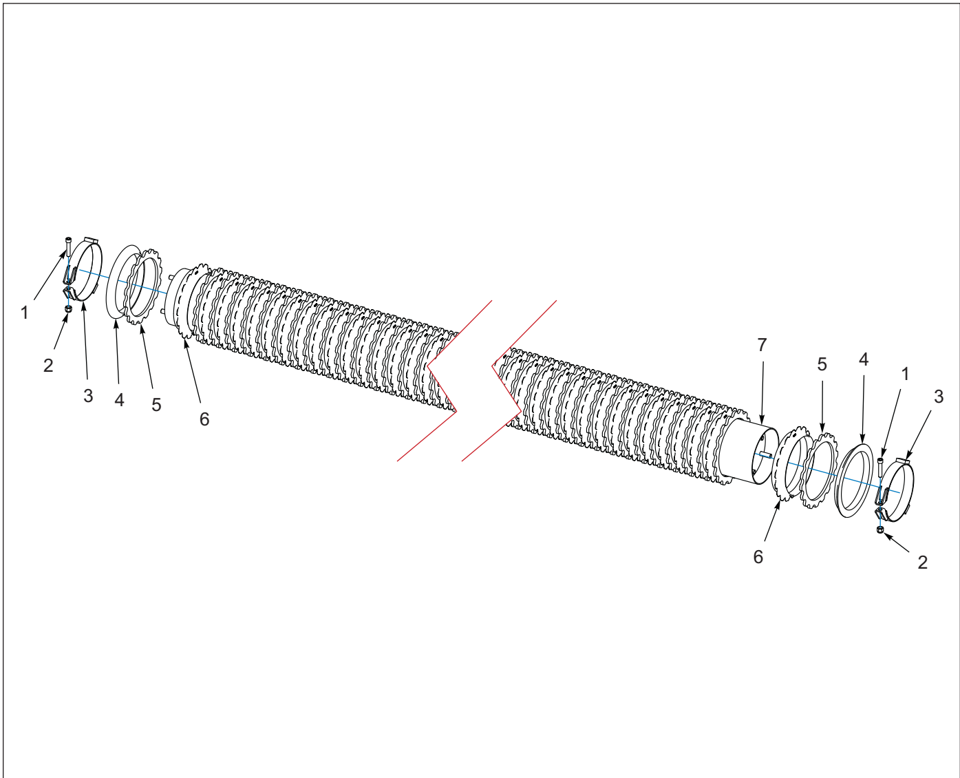
Figure 1-70: Rear Roller Assemblies with Turfmaker Sprockets - Optional
