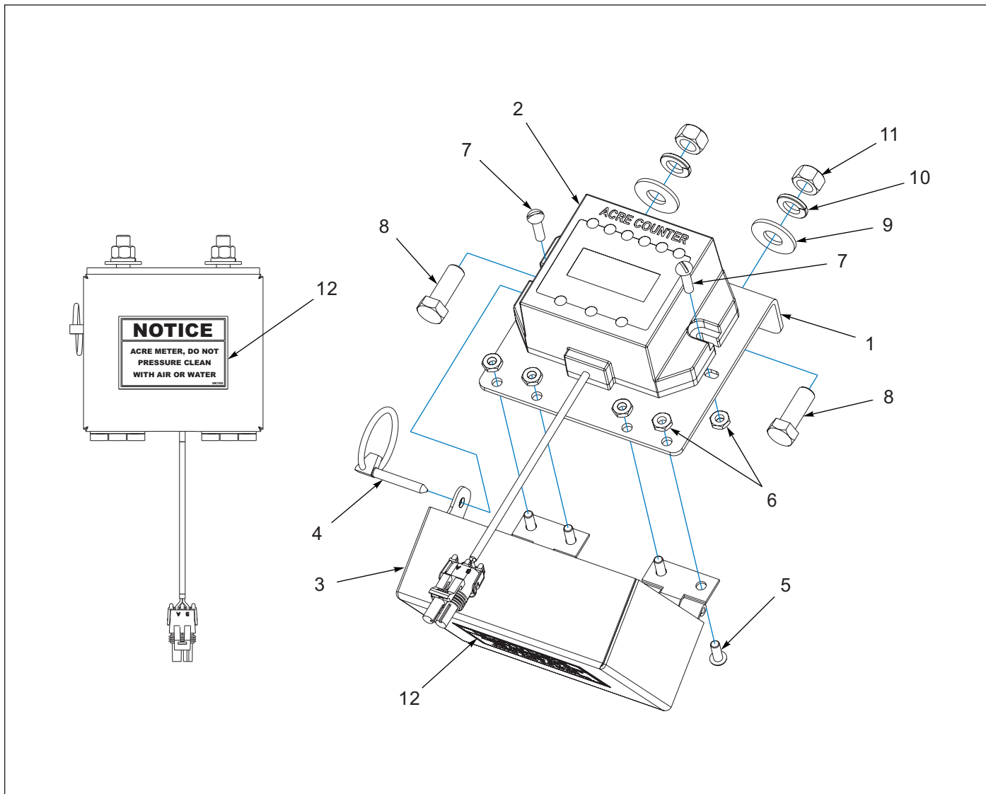
Figure 1-66: Acre Meter Assembly (05/15/2012 TO 06/01/2025)
