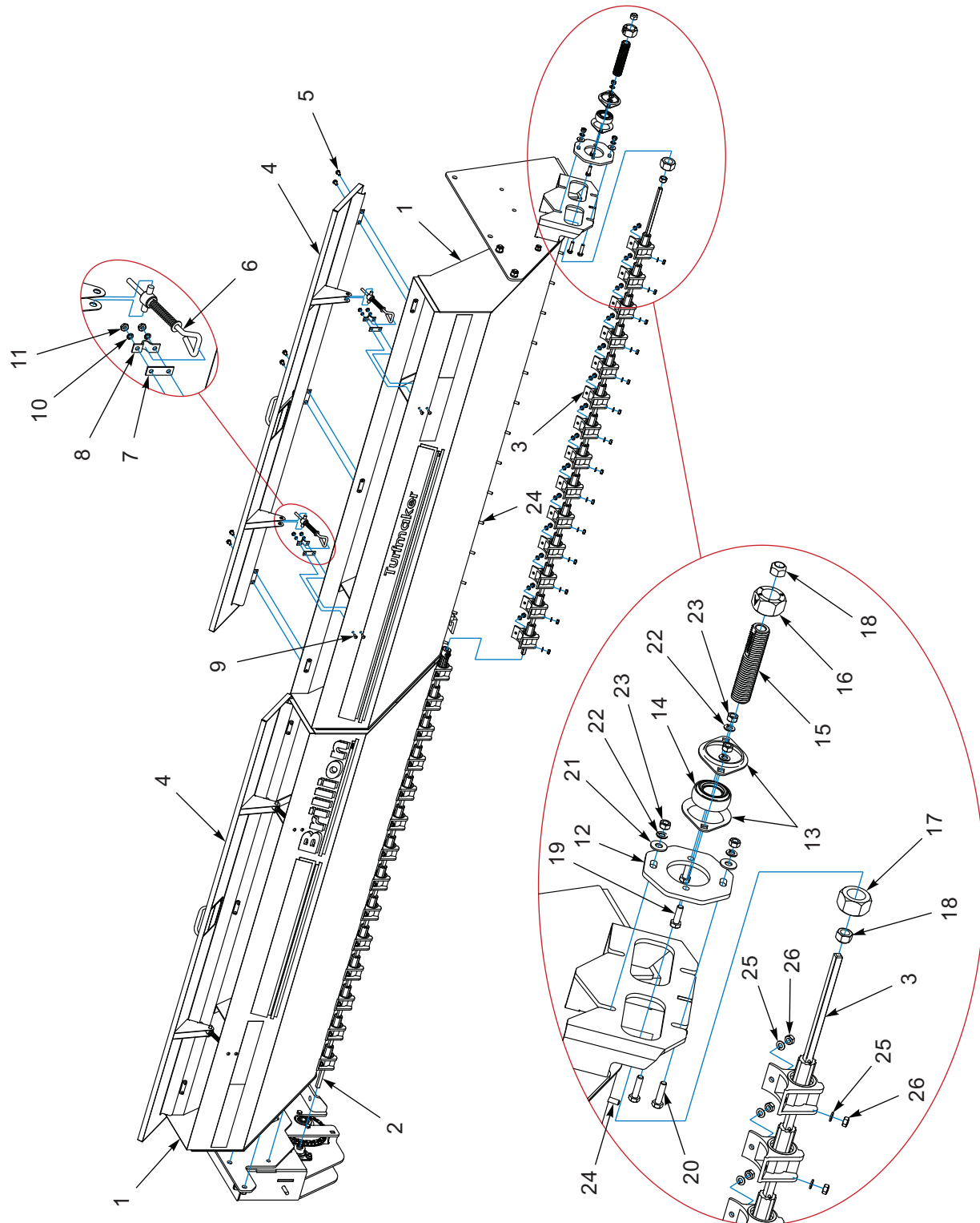
Figure 1-39: Rear Seed Box Assembly
