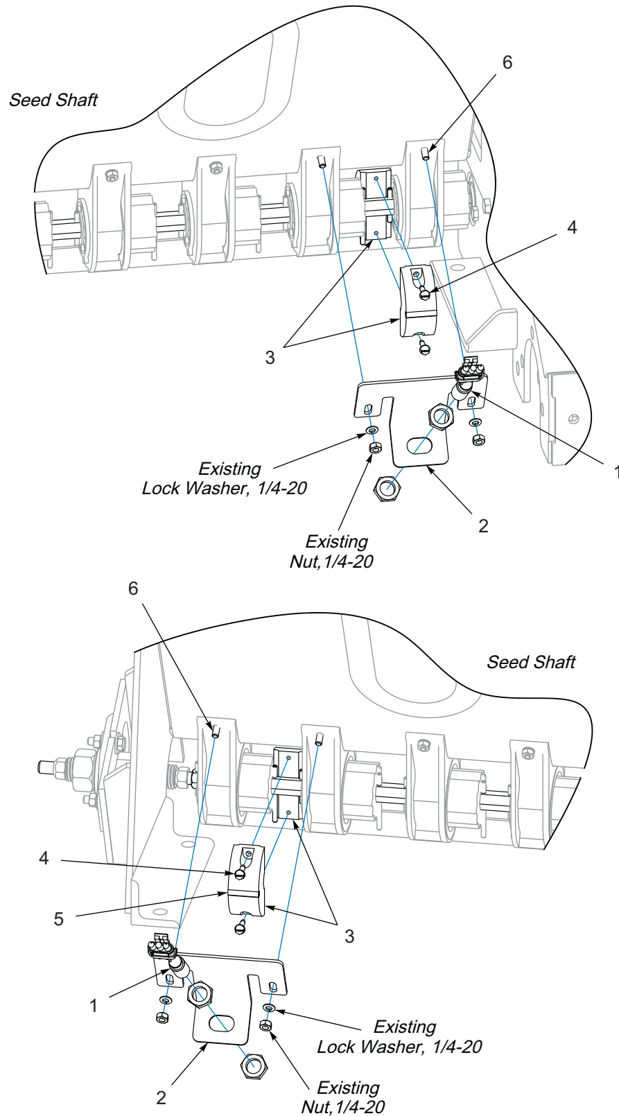
Figure 1-68: Console w/Clutch Control - Seed Shaft Sensor - Optional
