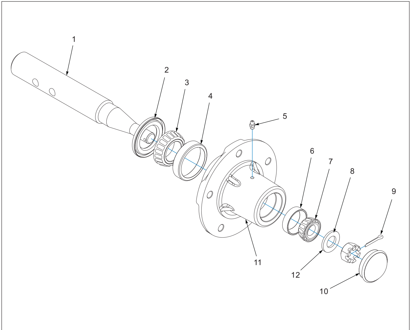
Figure 1-11: Hub and Spindle Assembly - 5 Bolt (Before 05/2021)
