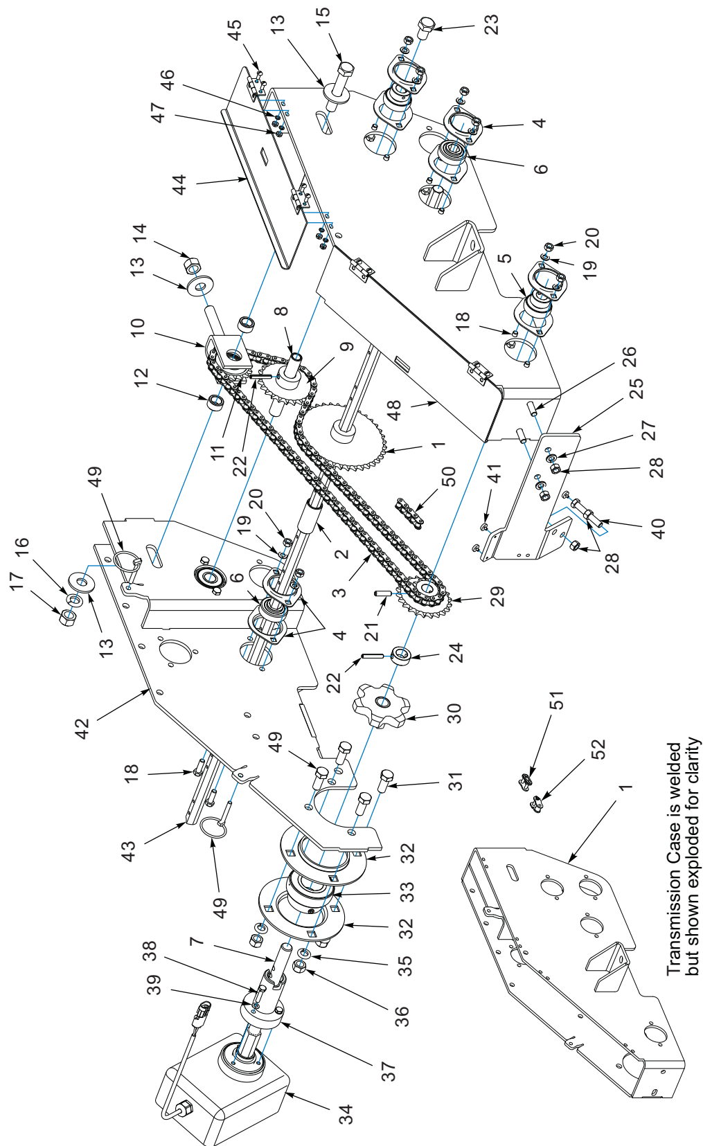
Figure 1-25: Transmission Assembly (Before 01/2020)
