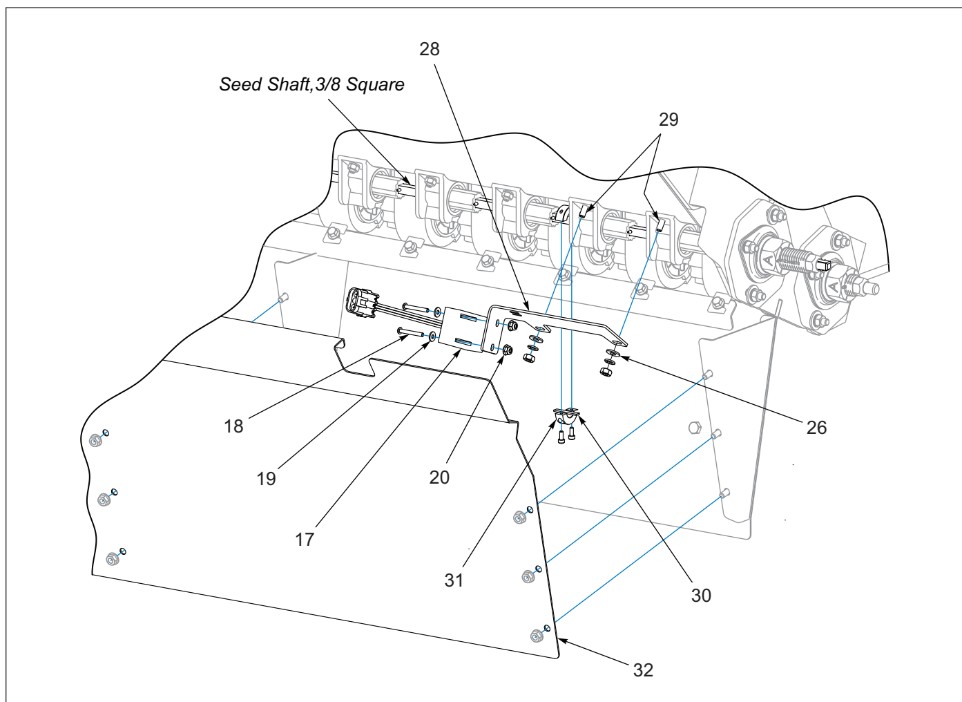
Figure 1-61: Brillion Elite Mini Monitor - Rear Seed Box Seed Shaft Sensor
