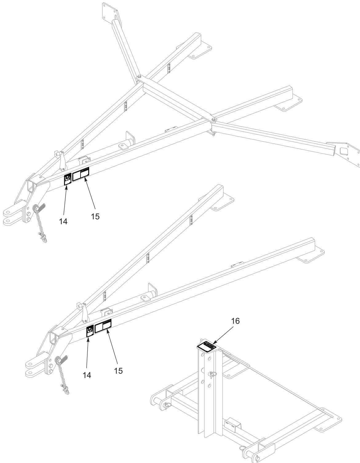
Figure 1-76: Decal Placement - Hitch
