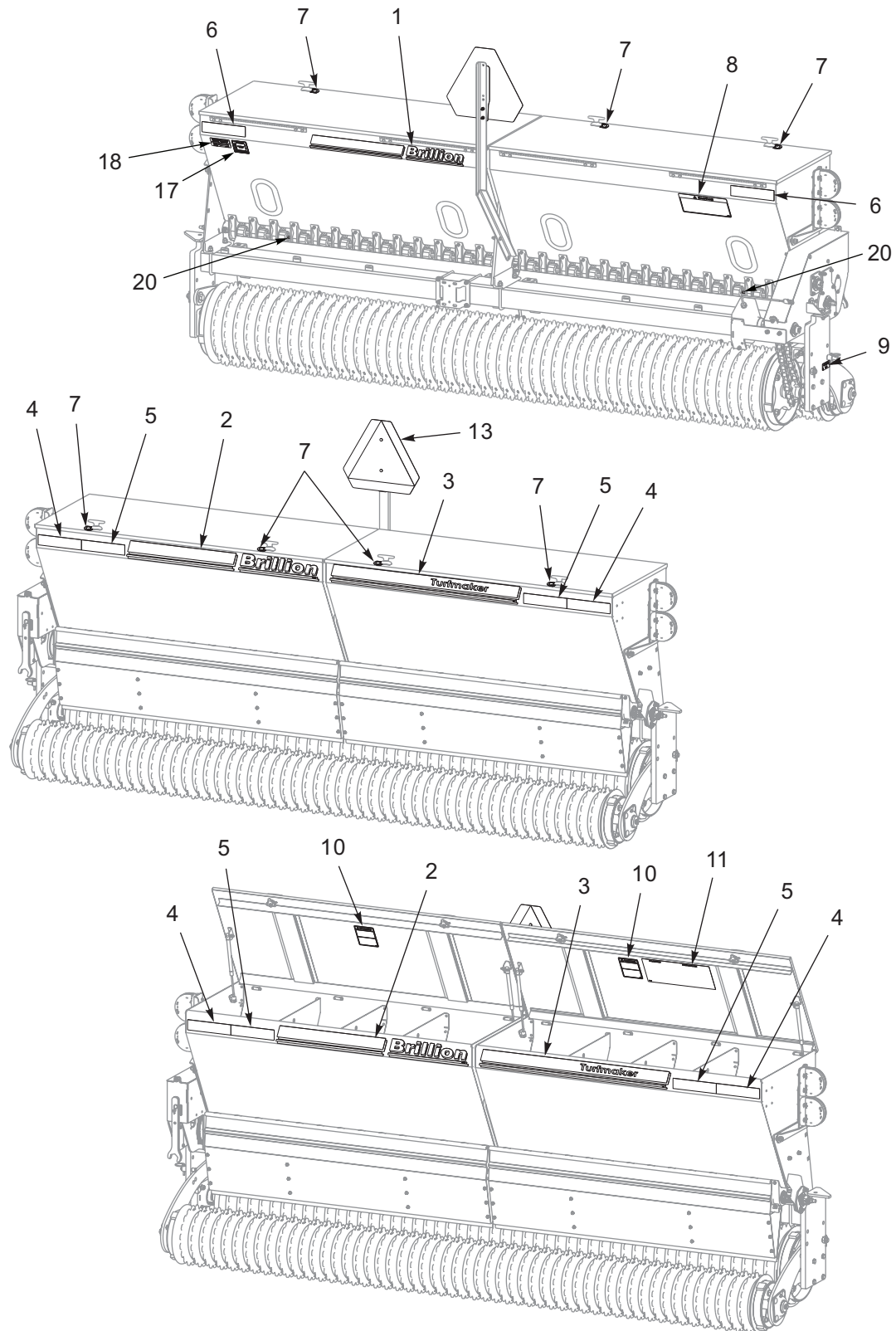
Figure 1-77: Decal Placement - Single Box, 8FT and 10FT
