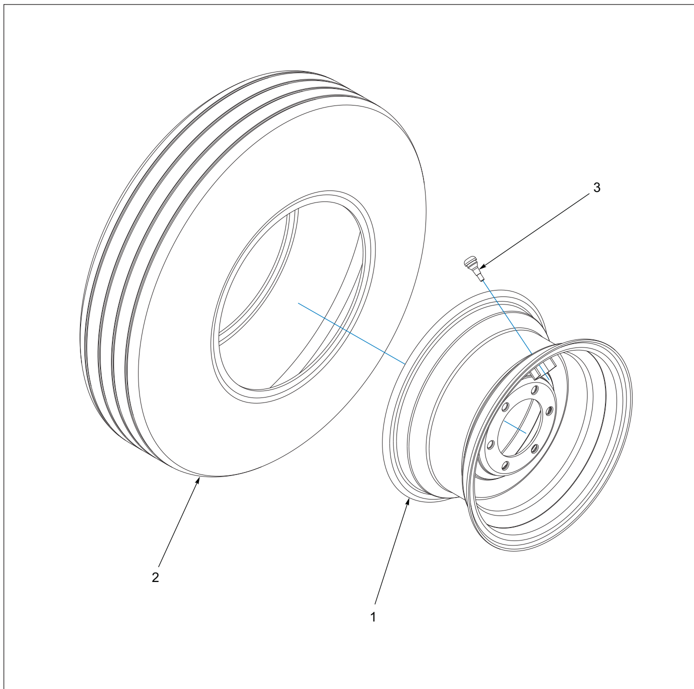
Figure 1-12: Tire and Wheel Assembly - 6 Bolt (After 05/2021)
