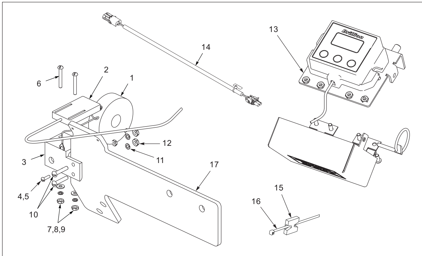
Figure 1-64: Electronic Acre Meter Kit with Clutch - Optional
