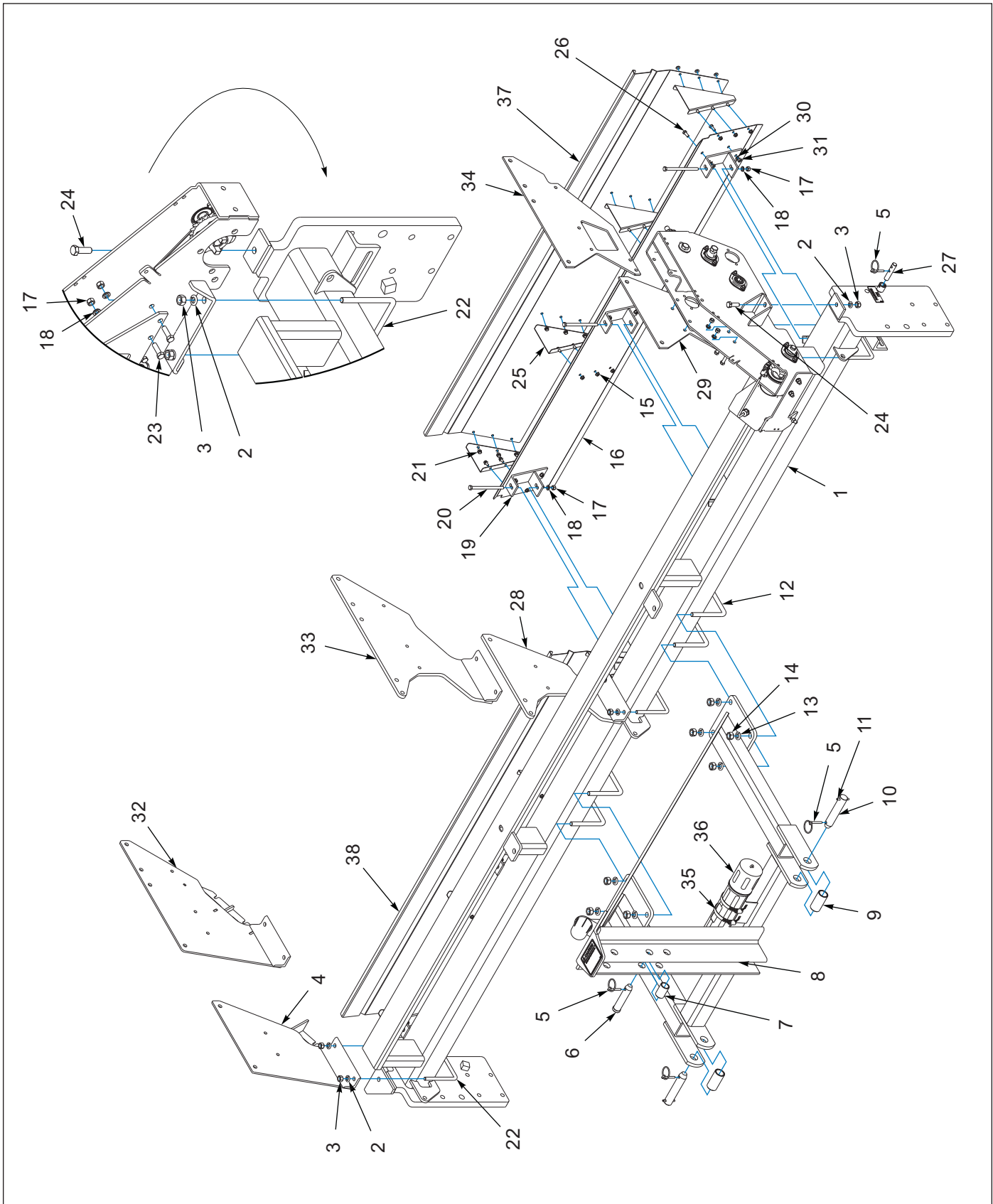
Figure 1-8: 3-PT Hitch - Frame, Deflectors, Seed Box Mounts - 12FT (Before 03/2019)
