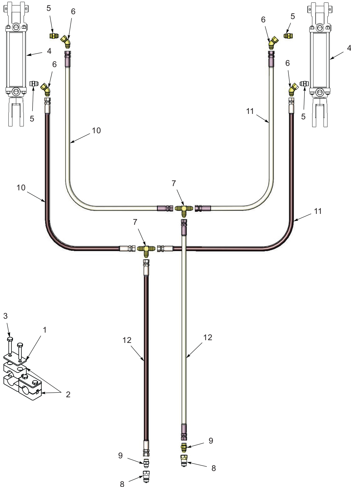
Figure 1-16: Hydraulic Schematic
