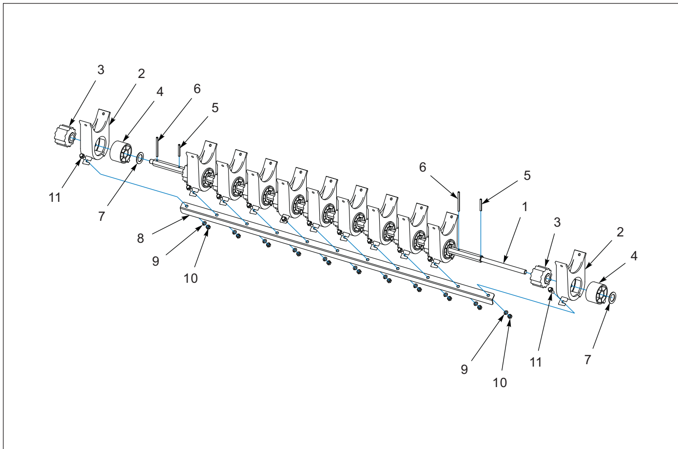
Figure 1-37: Seed Shaft Assembly, Right Hand
