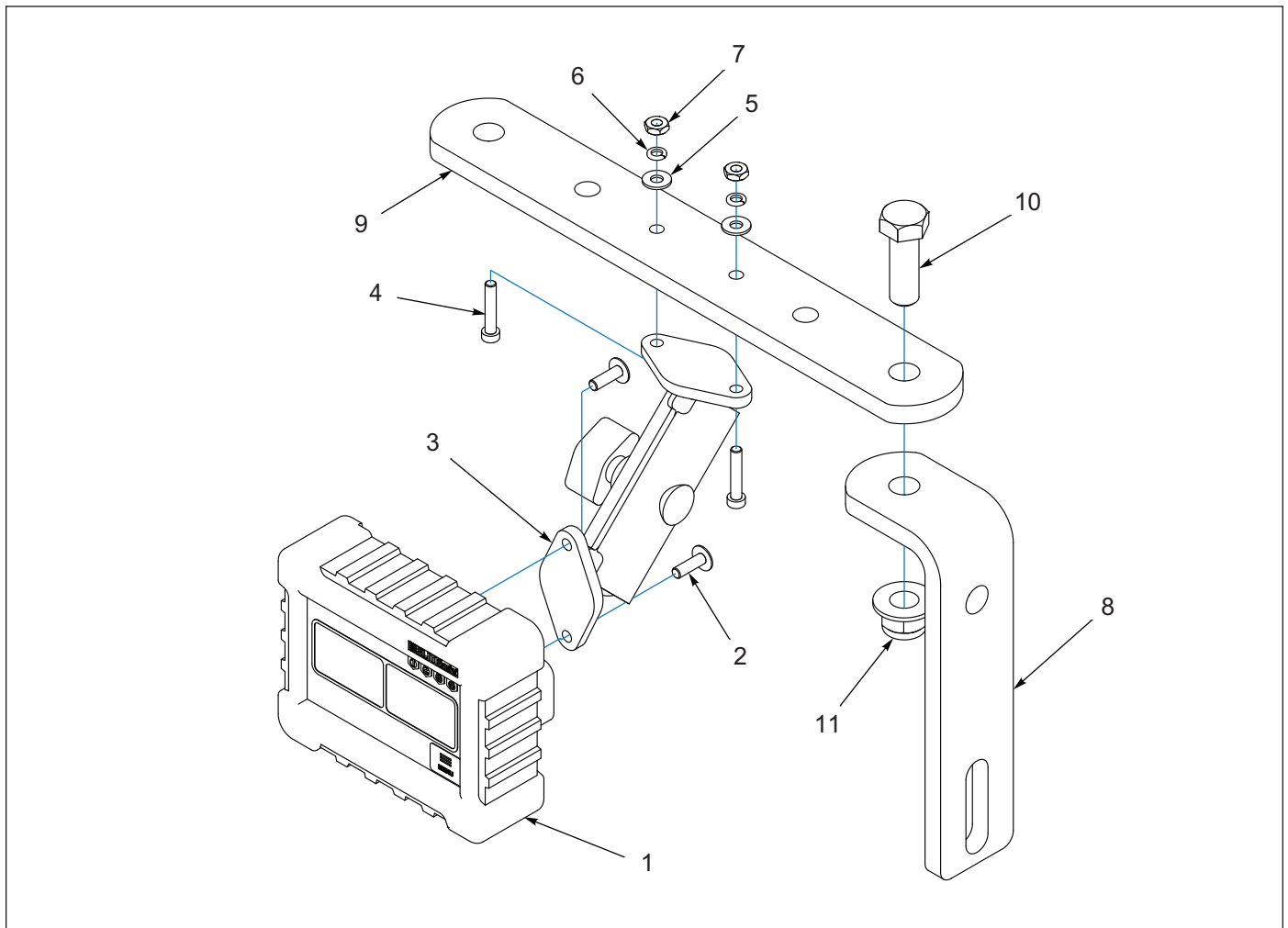
Figure 1-54: Brillion Elite Mini Monitor Tractor Mount
