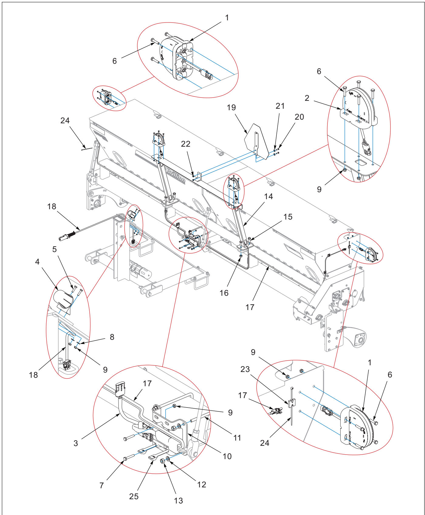
Figure 1-44: LED Warning Lamps - 12FT (After 09/2013)
