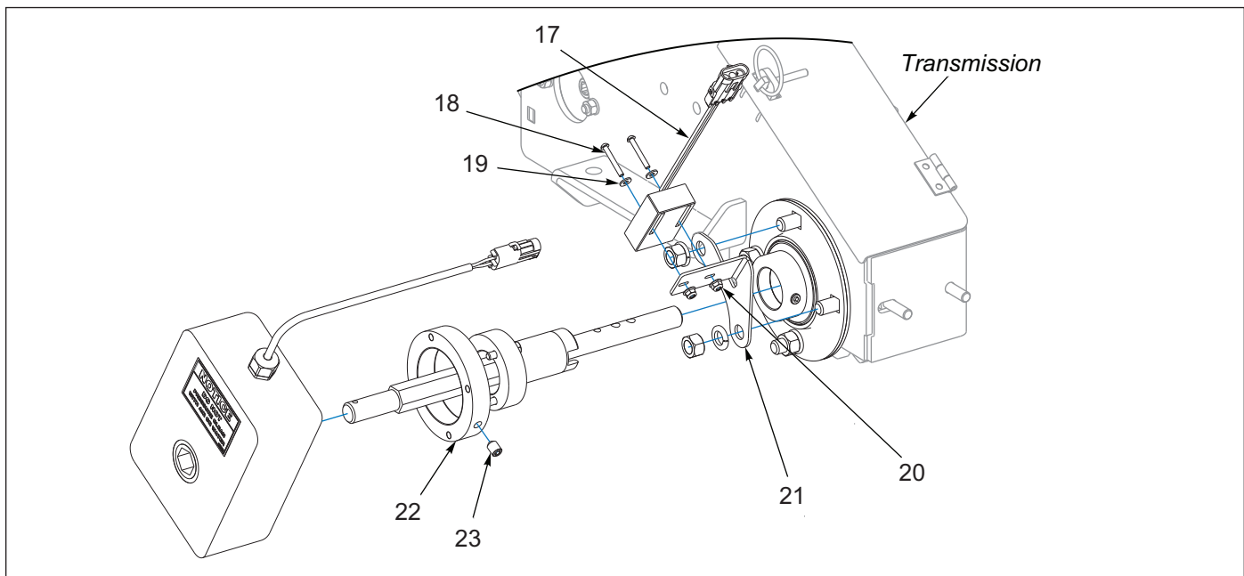
Figure 1-59: Brillion Elite Mini Monitor - Ground Speed
