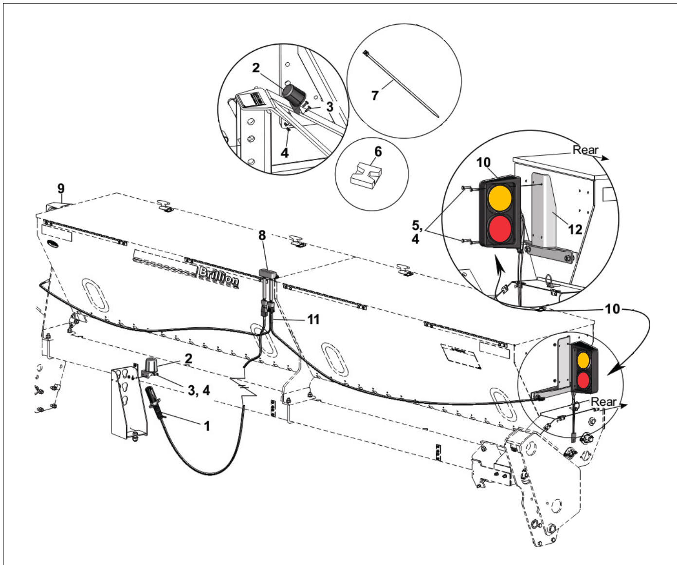
Figure 1-46: Warning Lamp Kit - 8FT and 10FT (Before 09/2013)
