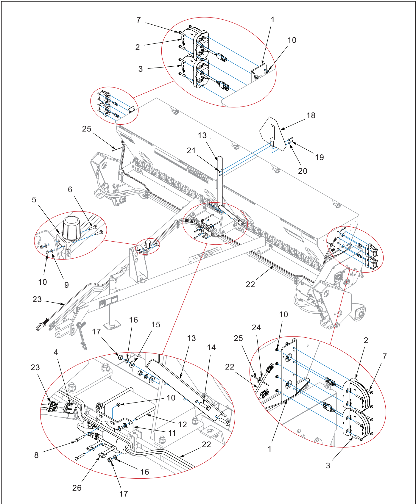
Figure 1-43: LED Warning Lamps - 8FT and 10FT (After 09/2013)
