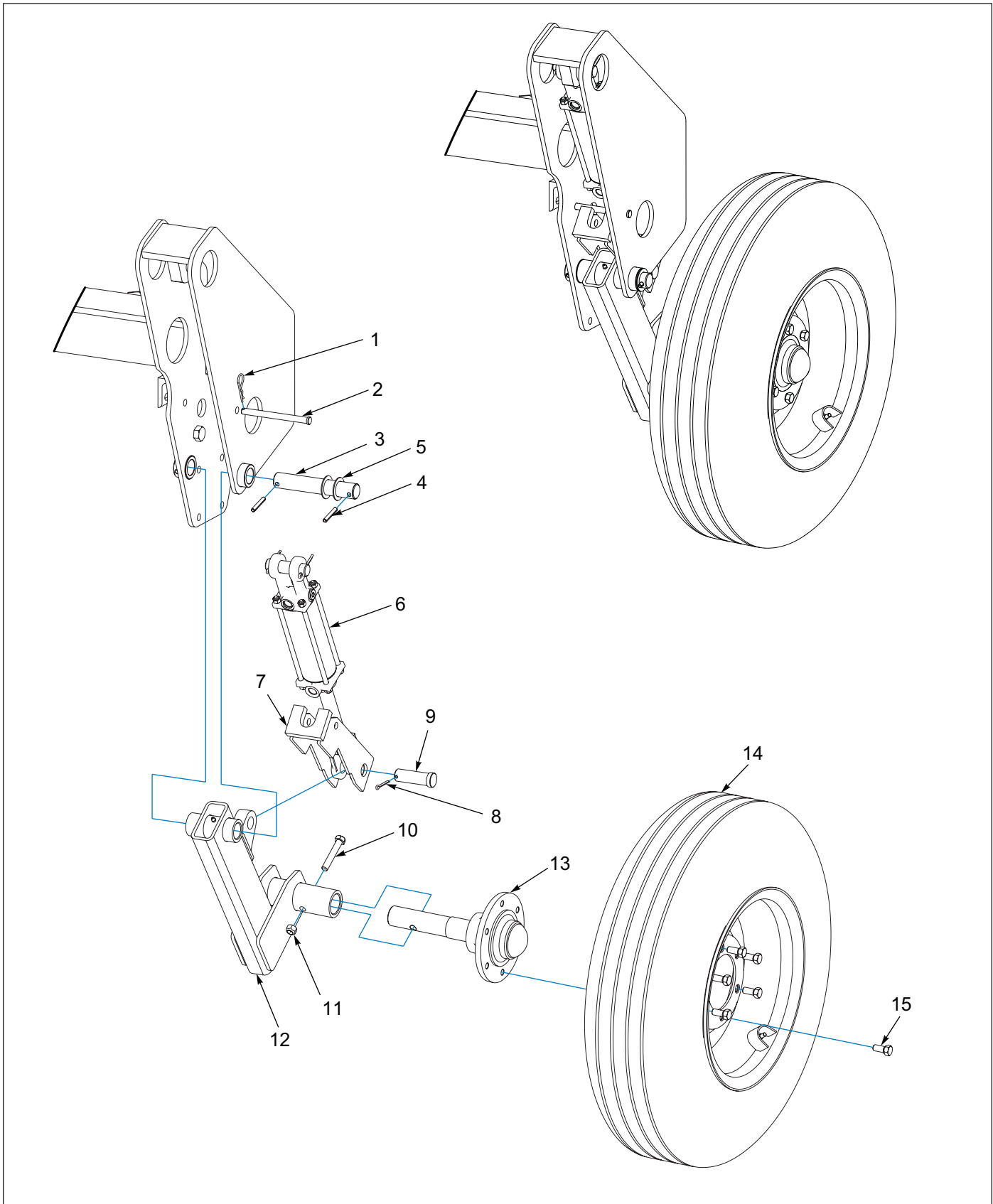
Figure 1-5: Wheel Arm Assembly
