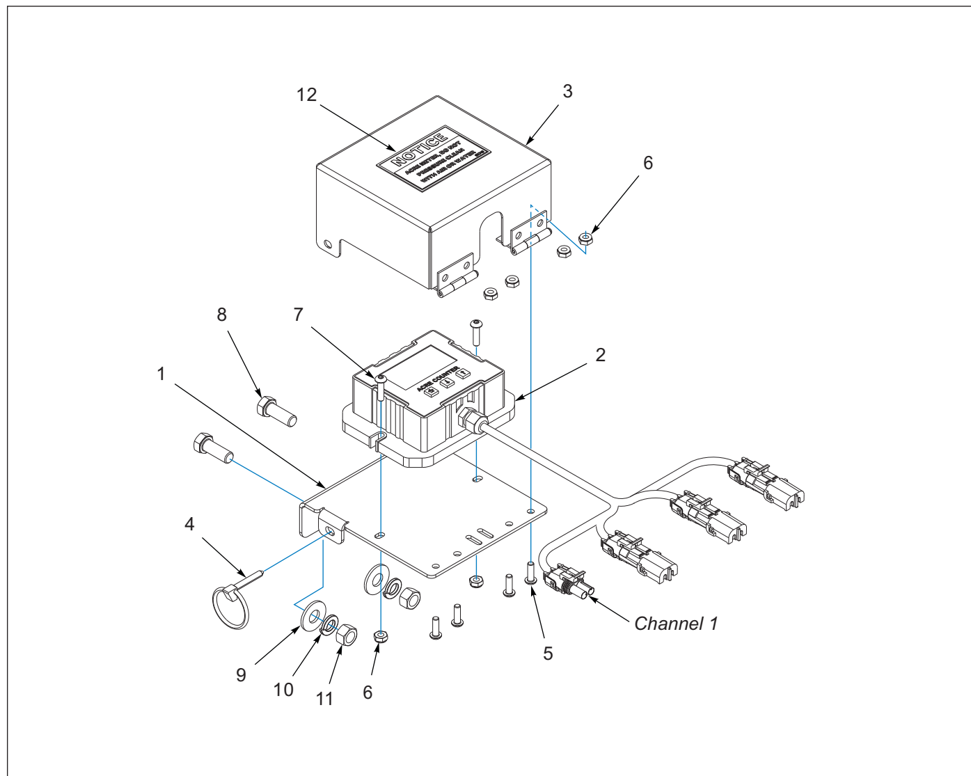
Figure 1-43: Acre Meter Assembly (After 06/01/2025)
