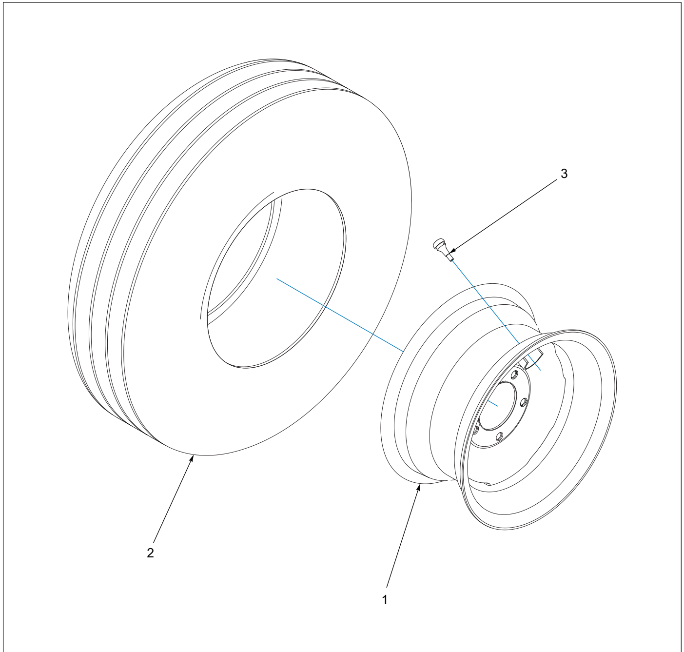
Figure 1-9: Tire and Wheel Assembly - 5 Bolt (Before 05/2021)
