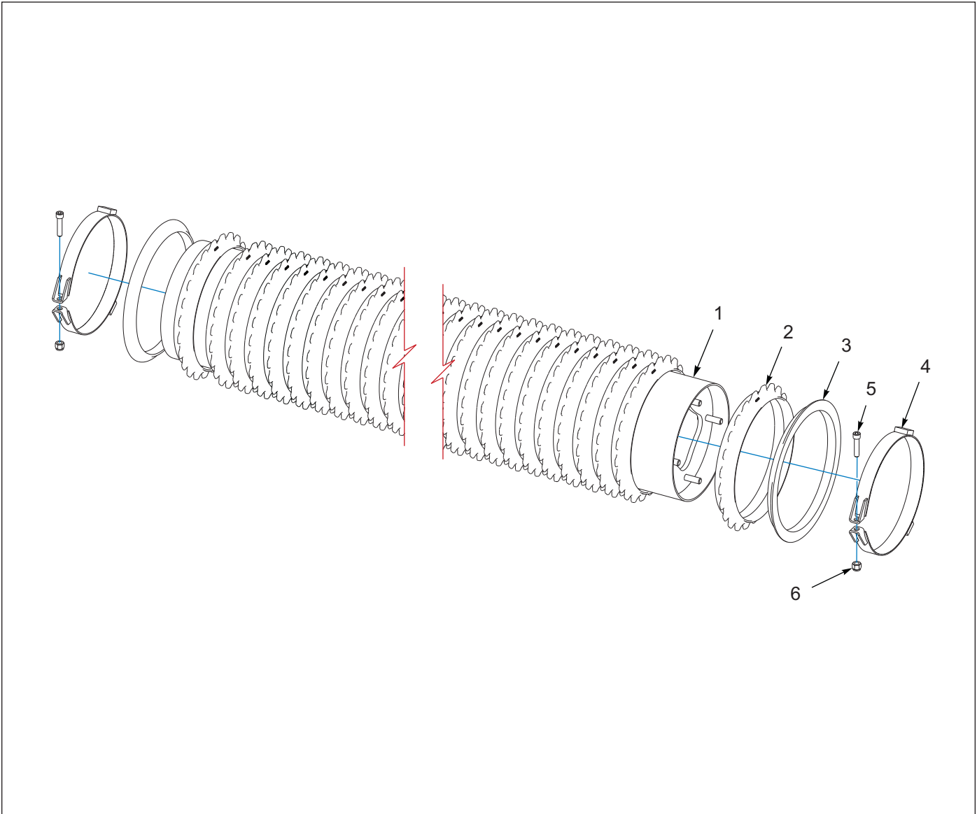
Figure 1-15: Front Roller, 4 - Bolt
