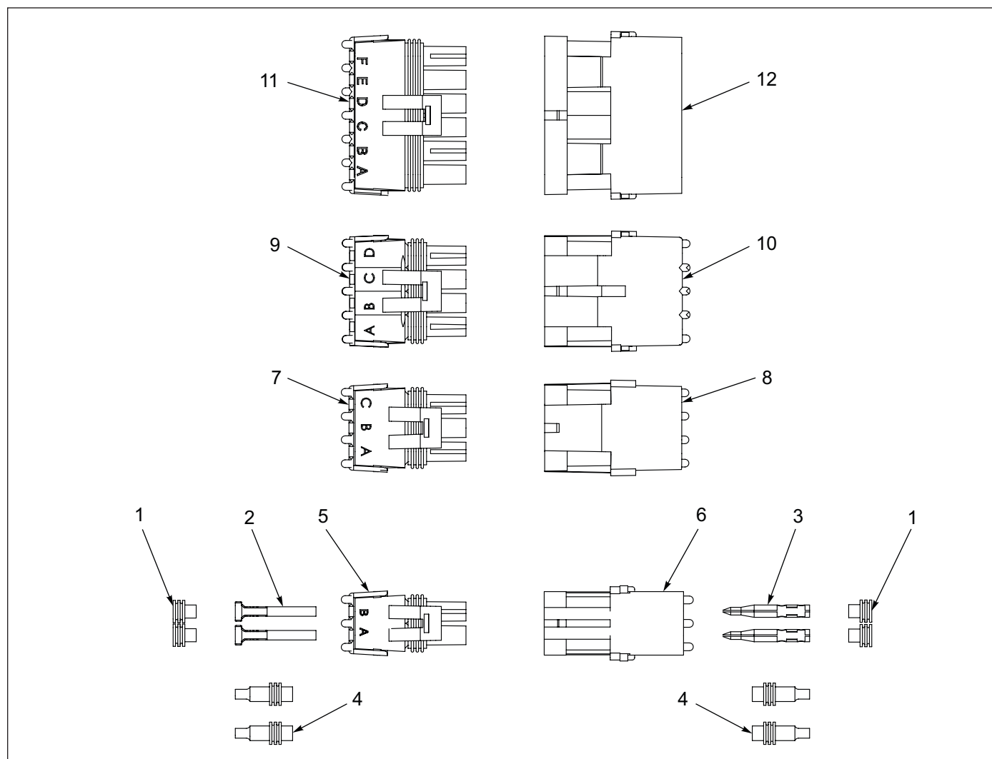
Figure 1-50: Weather Pack Connectors
