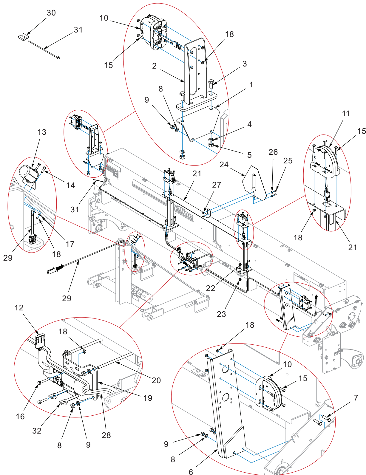
Figure 1-33: LED Warning Lamps, 12FT 3-PT Hitch (After 09/2013)
