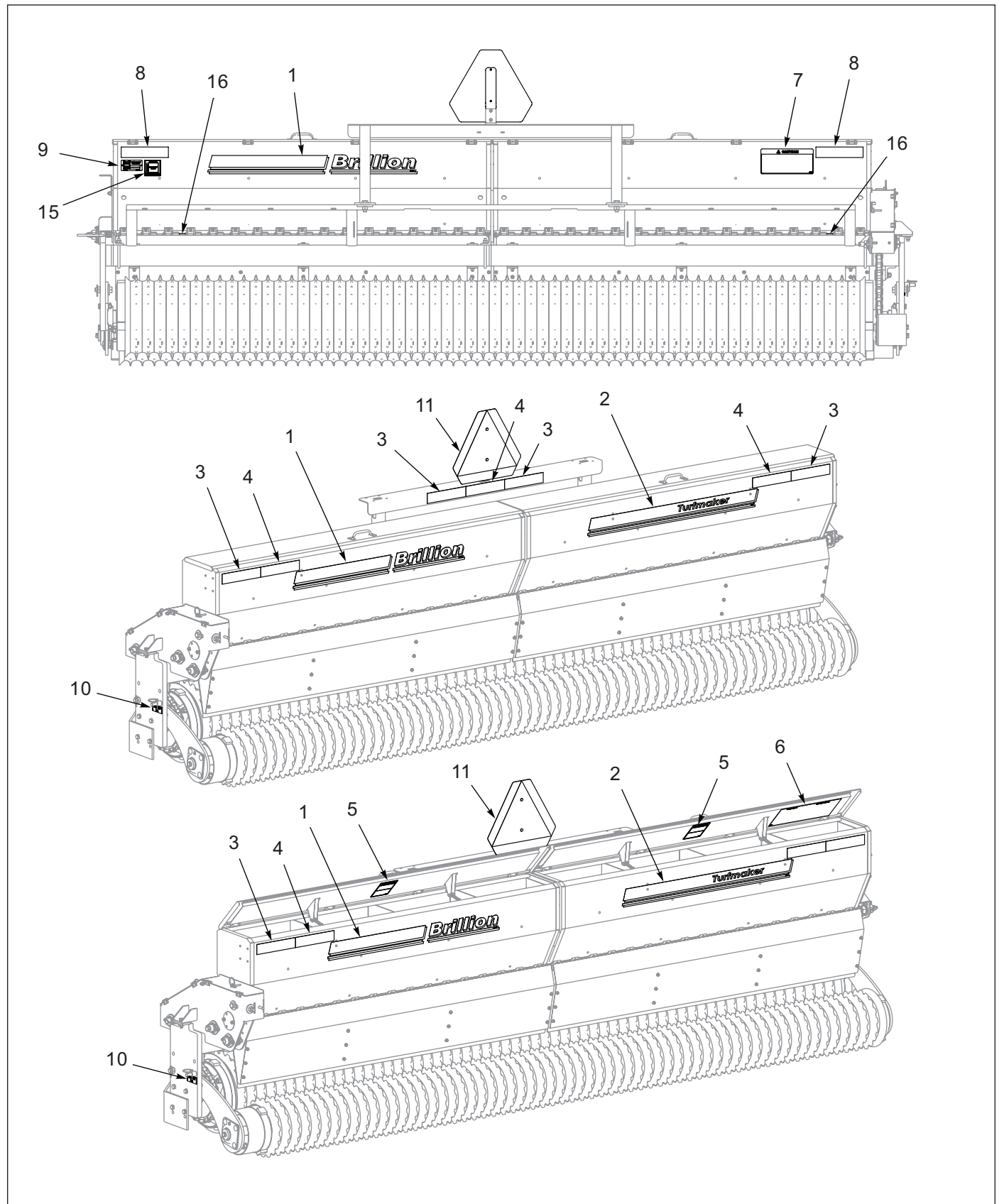
Figure 1-56: Decal Placement - 12FT Models
