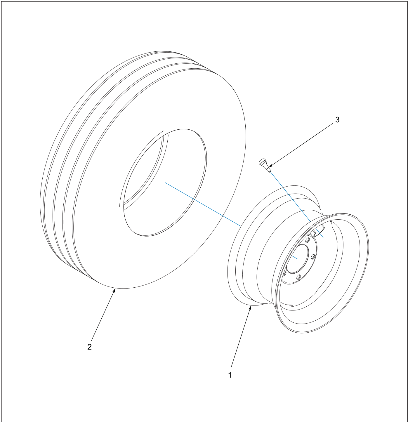
Figure 1-8: Tire and Wheel Assembly - 6 Bolt (After 05/2021)
