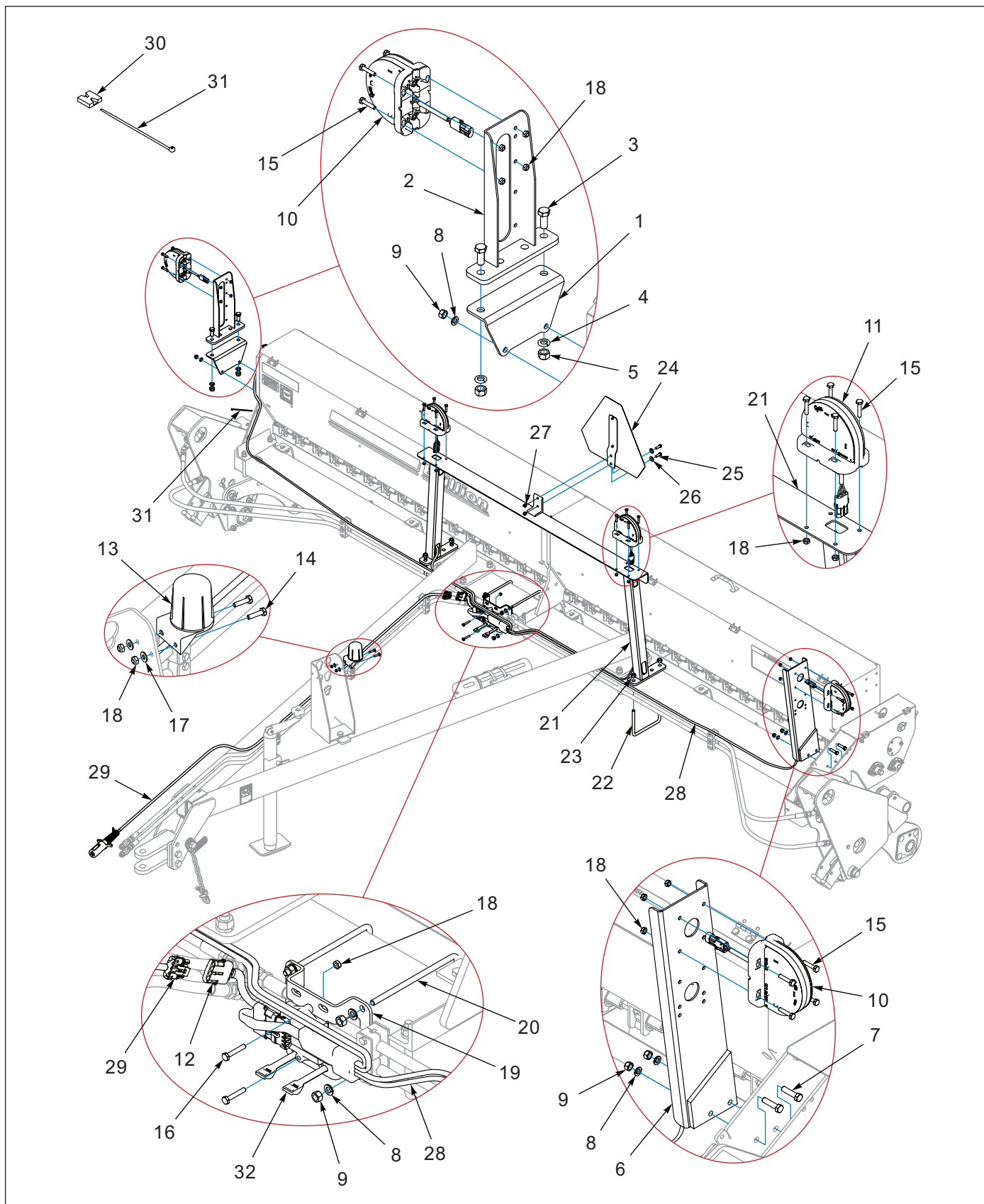
Figure 1-32: LED Warning Lamps, 12FT Drawbar (After 09/2013)
