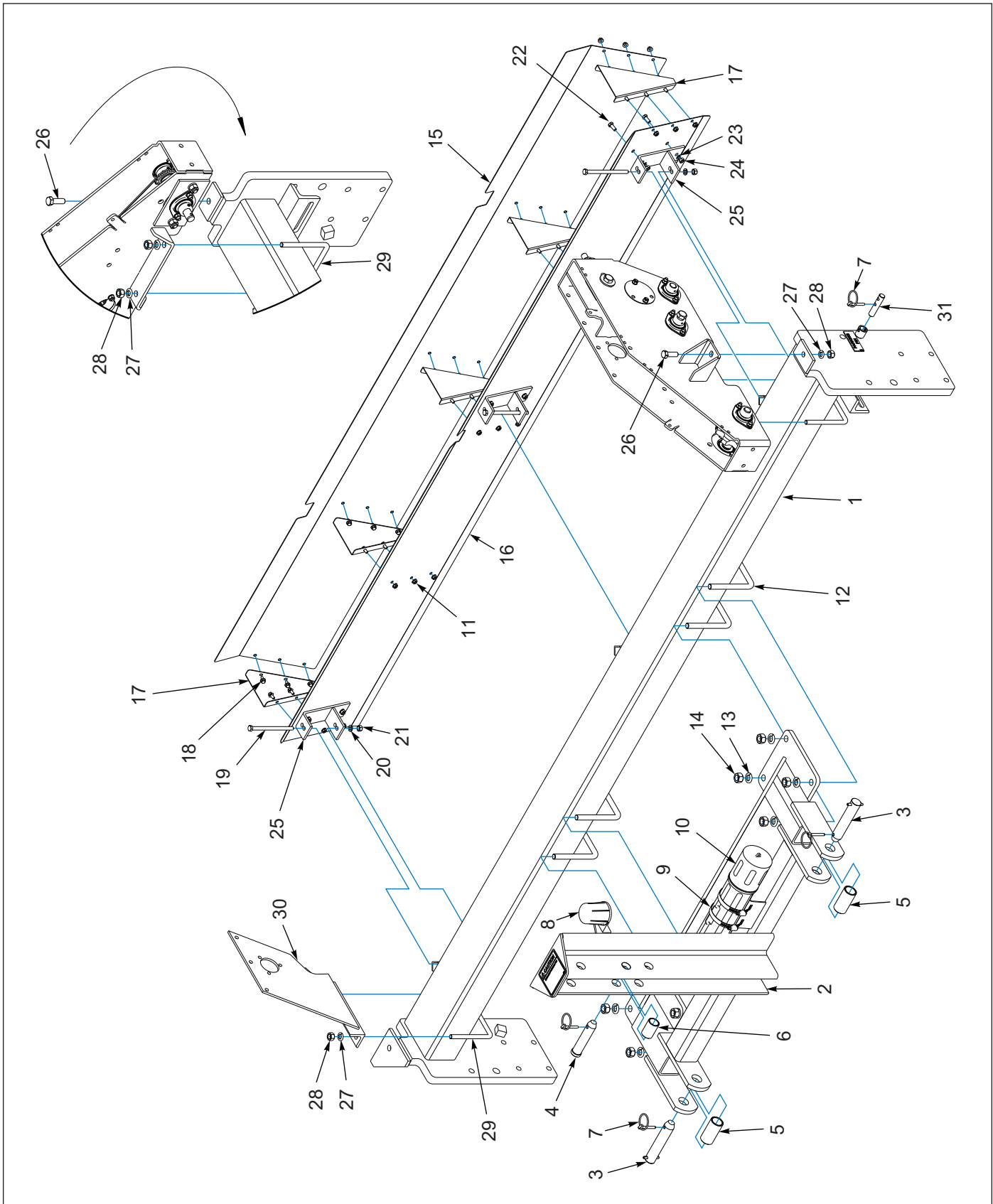
Figure 1-3: 3-PT Frame, Deflector & Mounting - 8FT
