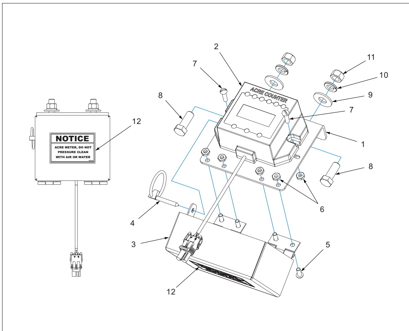
Figure 1-44: Acre Meter Assembly (05/15/2012 TO 06/01/2025)
