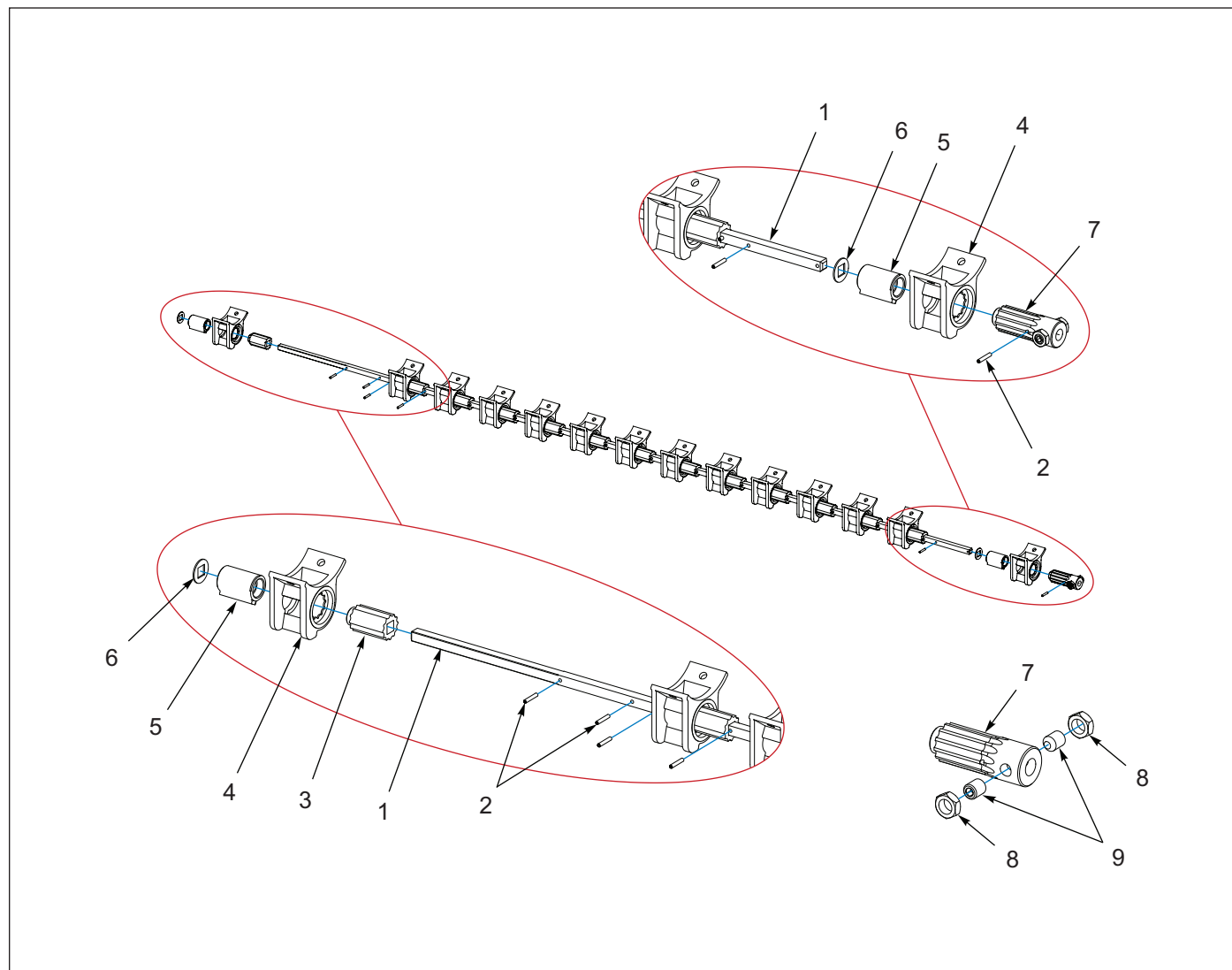
Figure 1-26: Seed Meter Assembly, Right-Hand 10FT and 12FT
