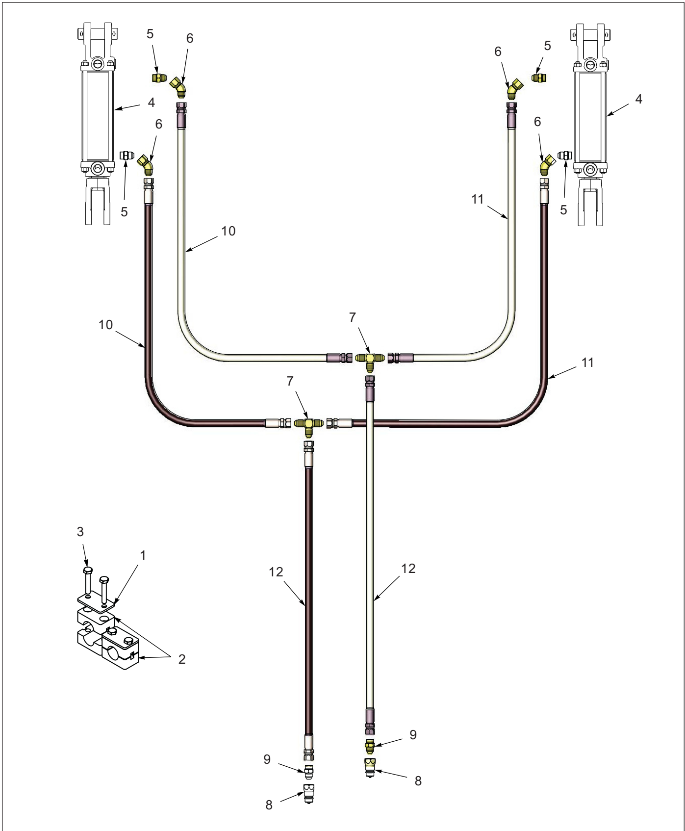
Figure 1-11: Hydraulic Schematic
