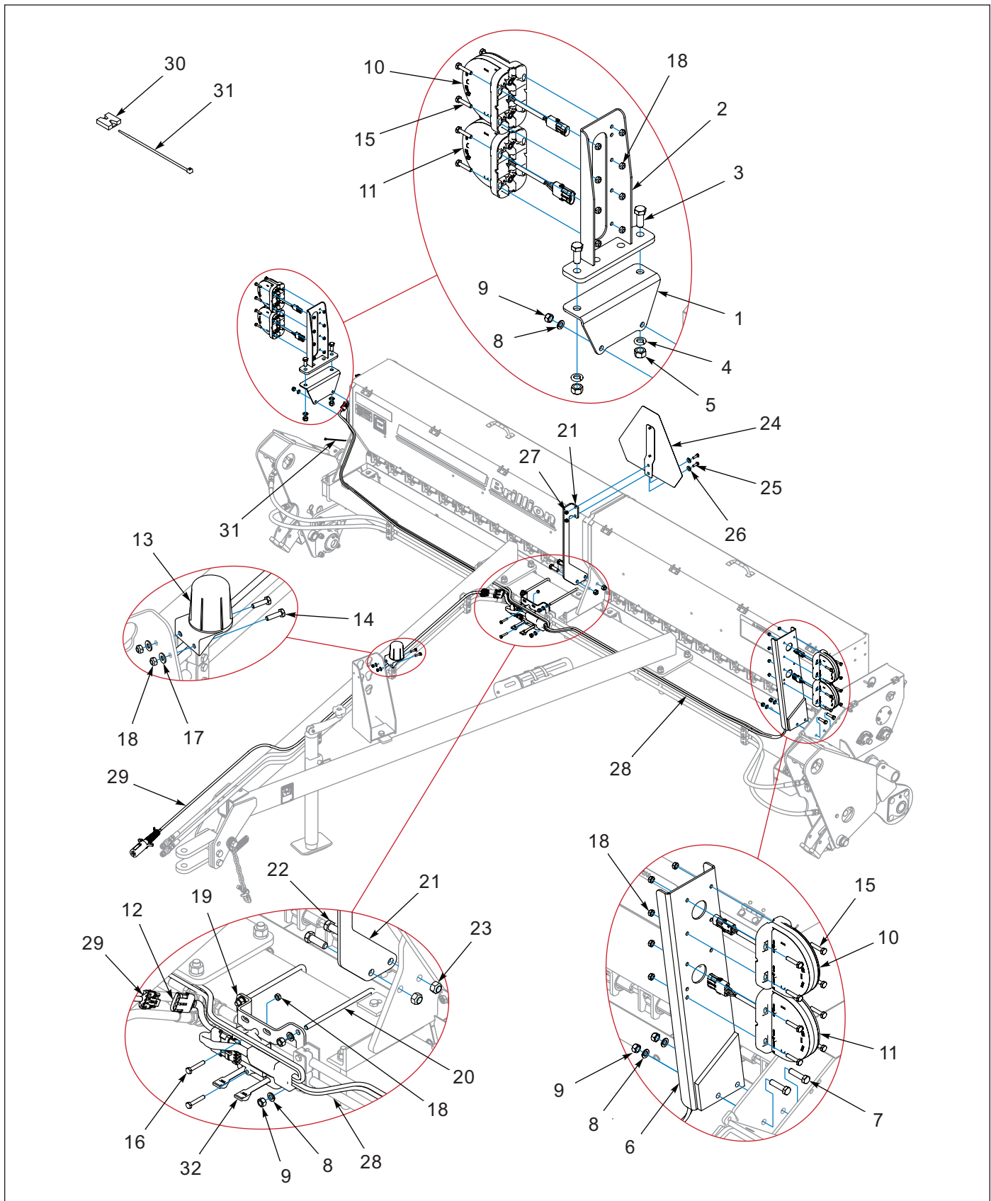
Figure 1-31: LED Warning Lamps, 10FT (After 09/2013)
