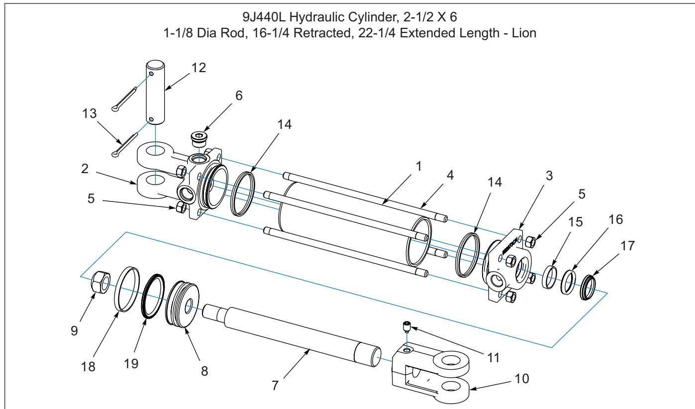
Figure 1-48: Hydraulic Cylinder, 2-1/2 x 6 - Lion (After 01/15/2008)
