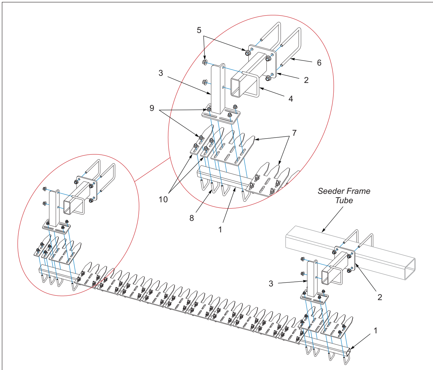
Figure 1-35: Scraper Kit, 8FT Tube Mounted - Optional
