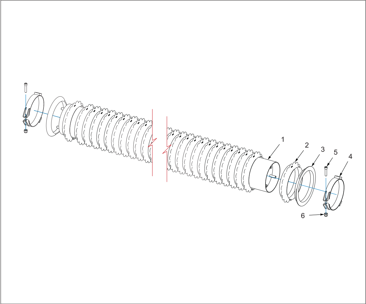
Figure 1-16: Rear Roller Assembly
