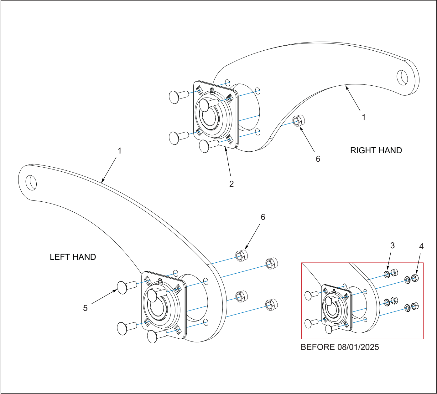
Figure 1-18: Rear Arm Assemblies
