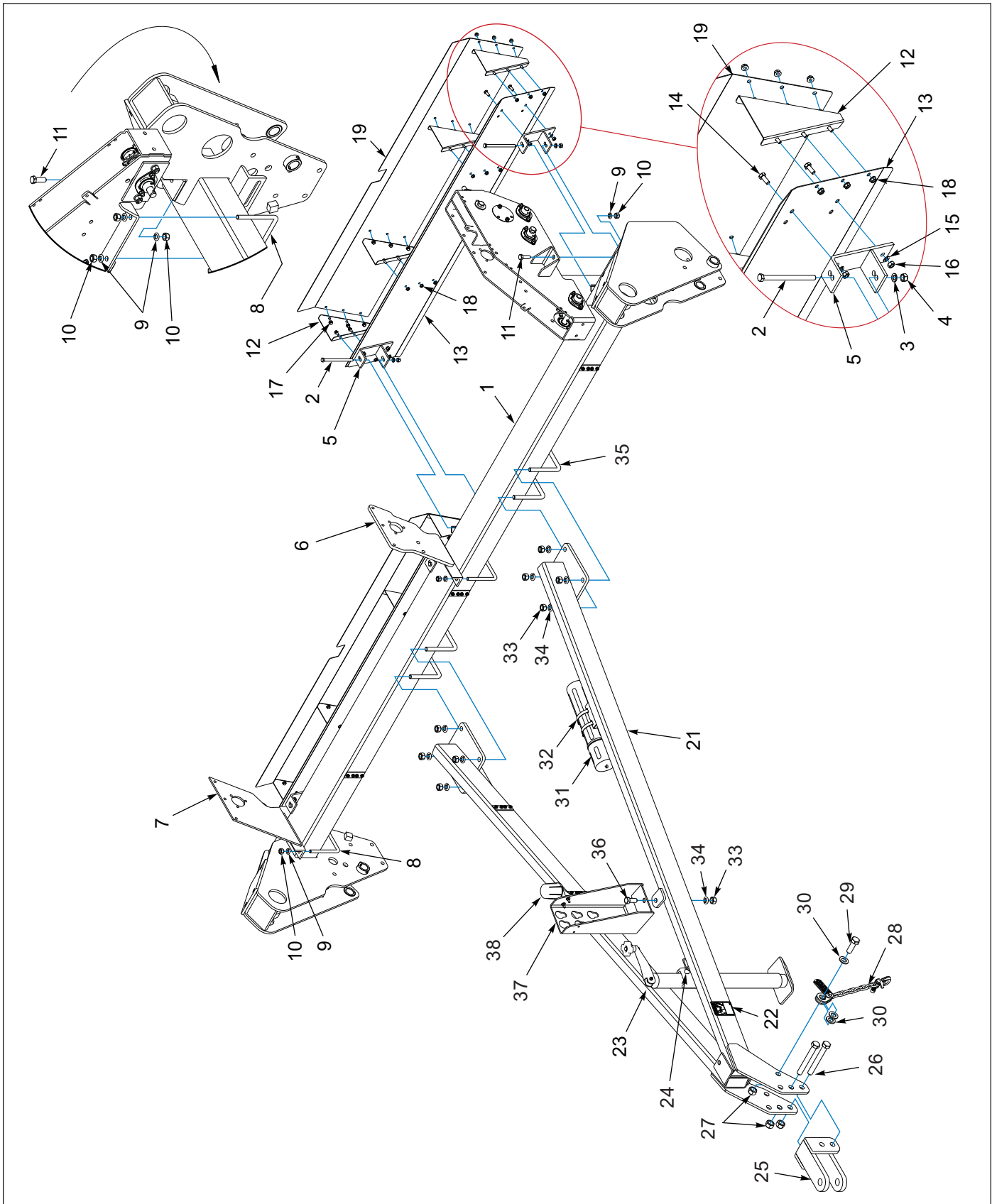
Figure 1-2: Drawbar Frame, Deflectors & Mounting - 10FT and 12FT
