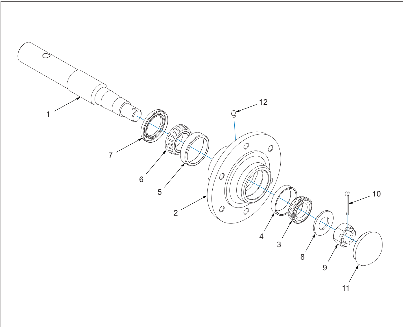
Figure 1-6: Hub and Spindle Assembly - 6 Bolt (After 05/2021)
