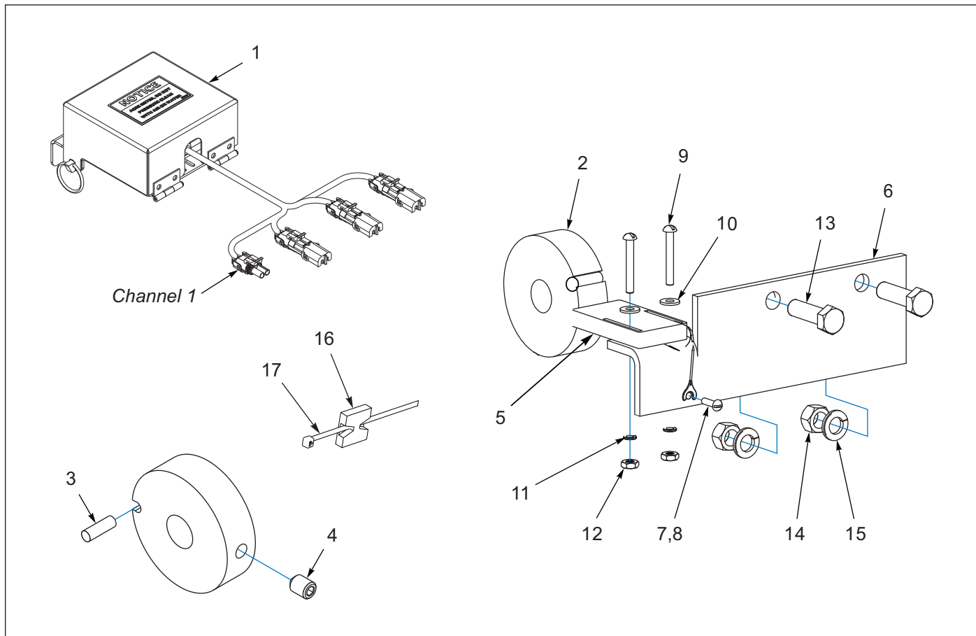
Figure 1-42: Electronic Acre Meter Assembly - Optional
