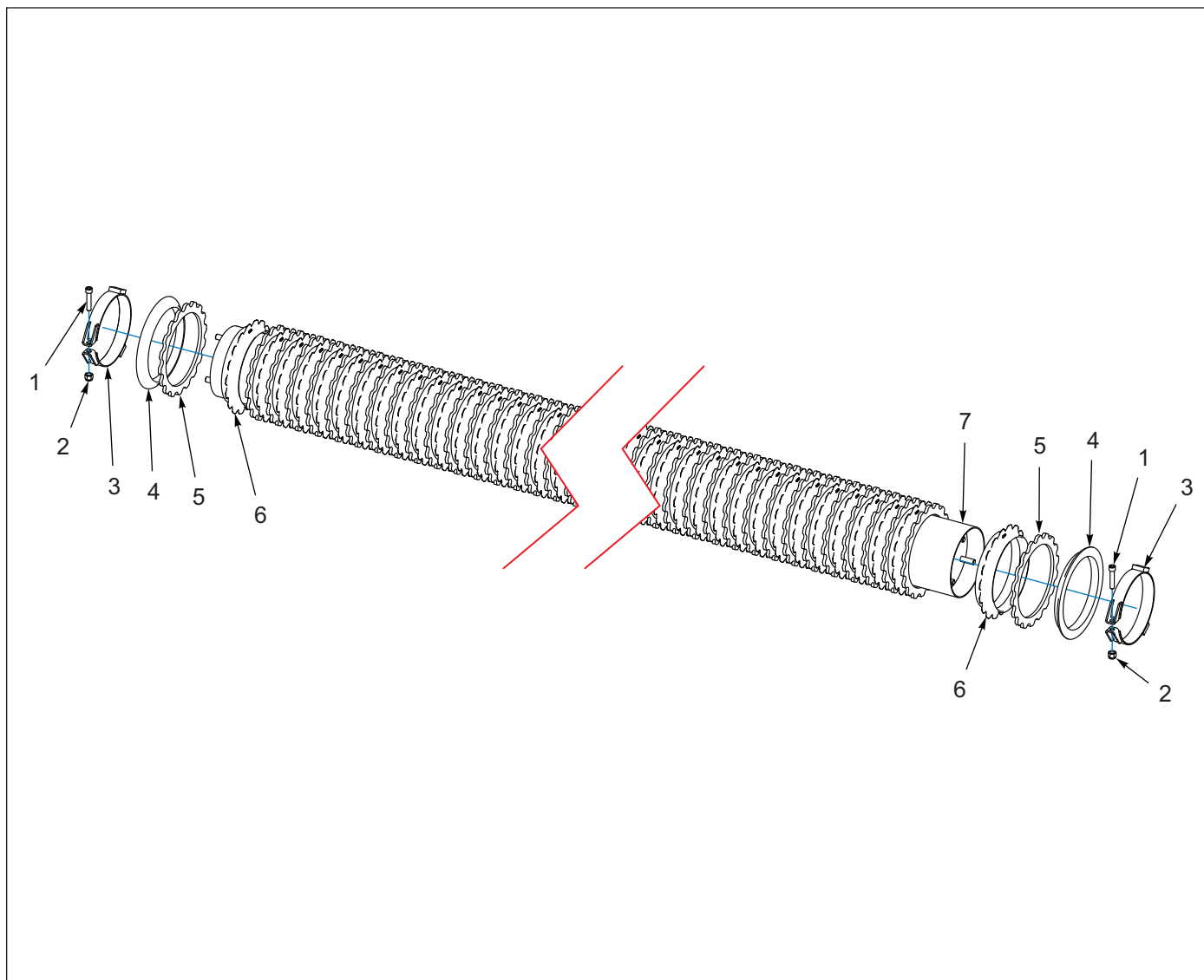
Figure 1-46: Rear Roller Assemblies with Spacers - Optional
