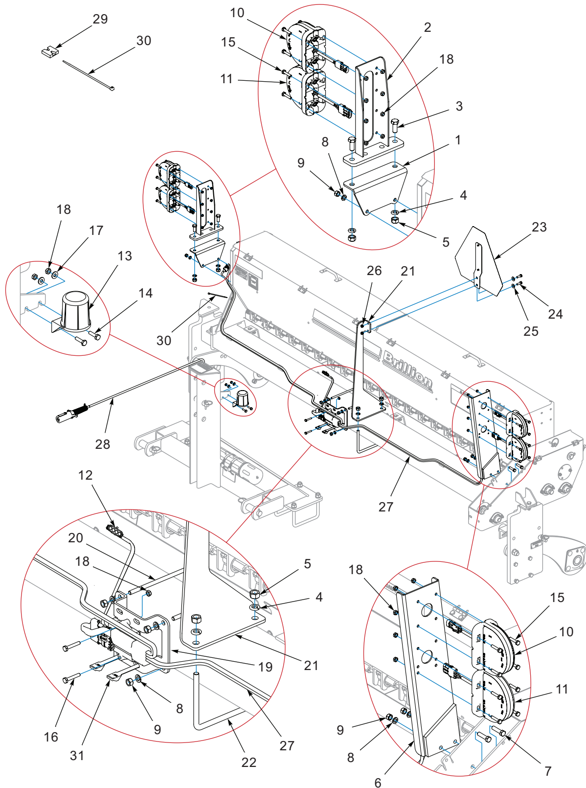
Figure 1-30: LED Warning Lamps, 8FT 3-PT Hitch (After 09/2013)
