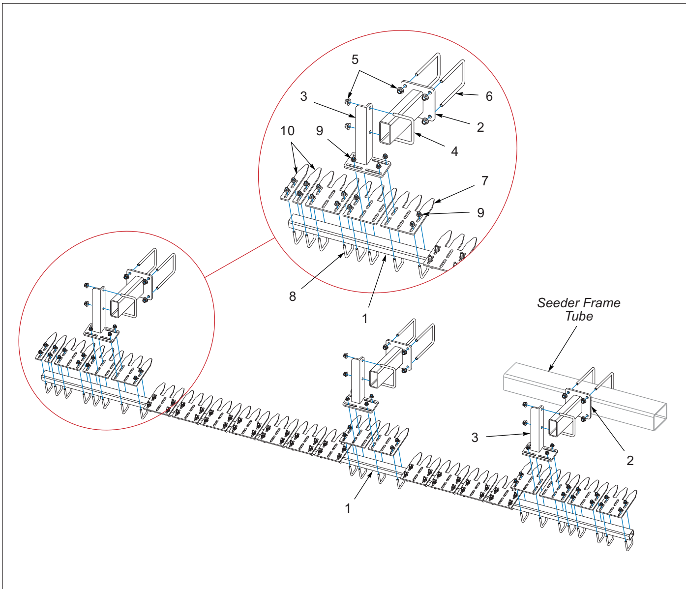
Figure 1-37: Scraper Kit, 12FT Tube Mounted - Optional
