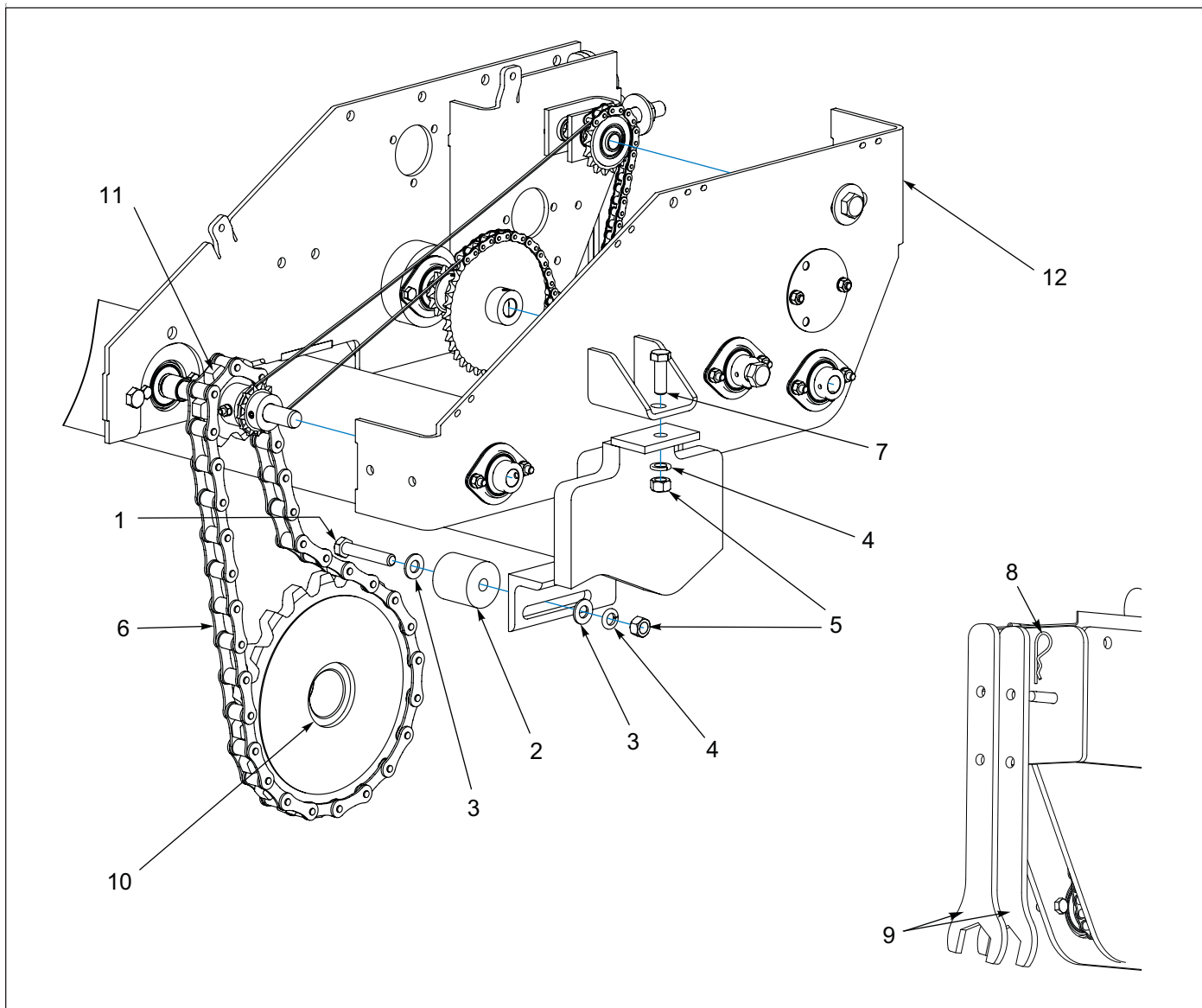
Figure 1-19: Transmission Mounting and Drive
