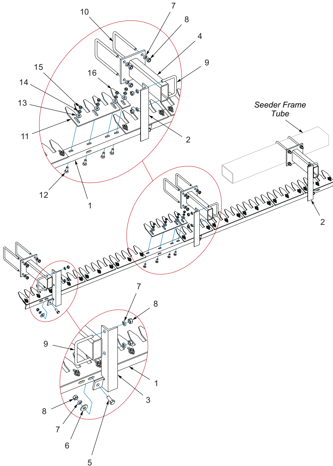
Figure 1-38: Scraper Kit, Angle Mounted - Optional
