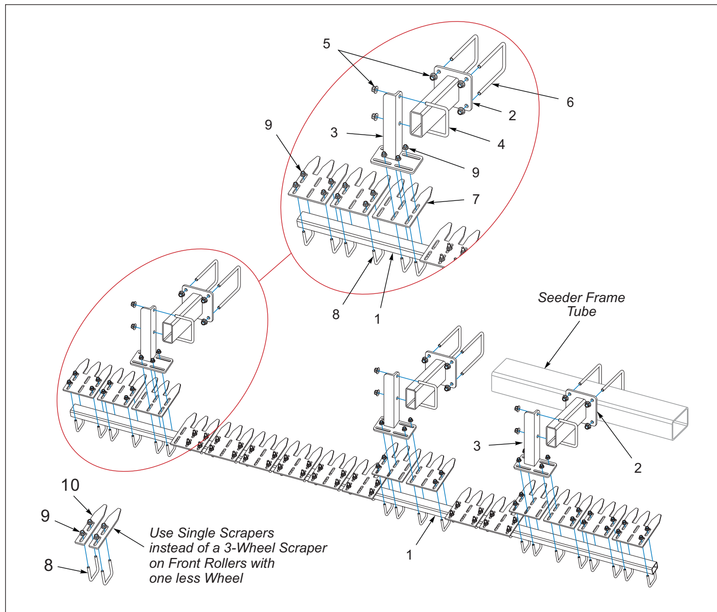
Figure 1-36: Scraper Kit, 10FT Tube Mounted - Optional
