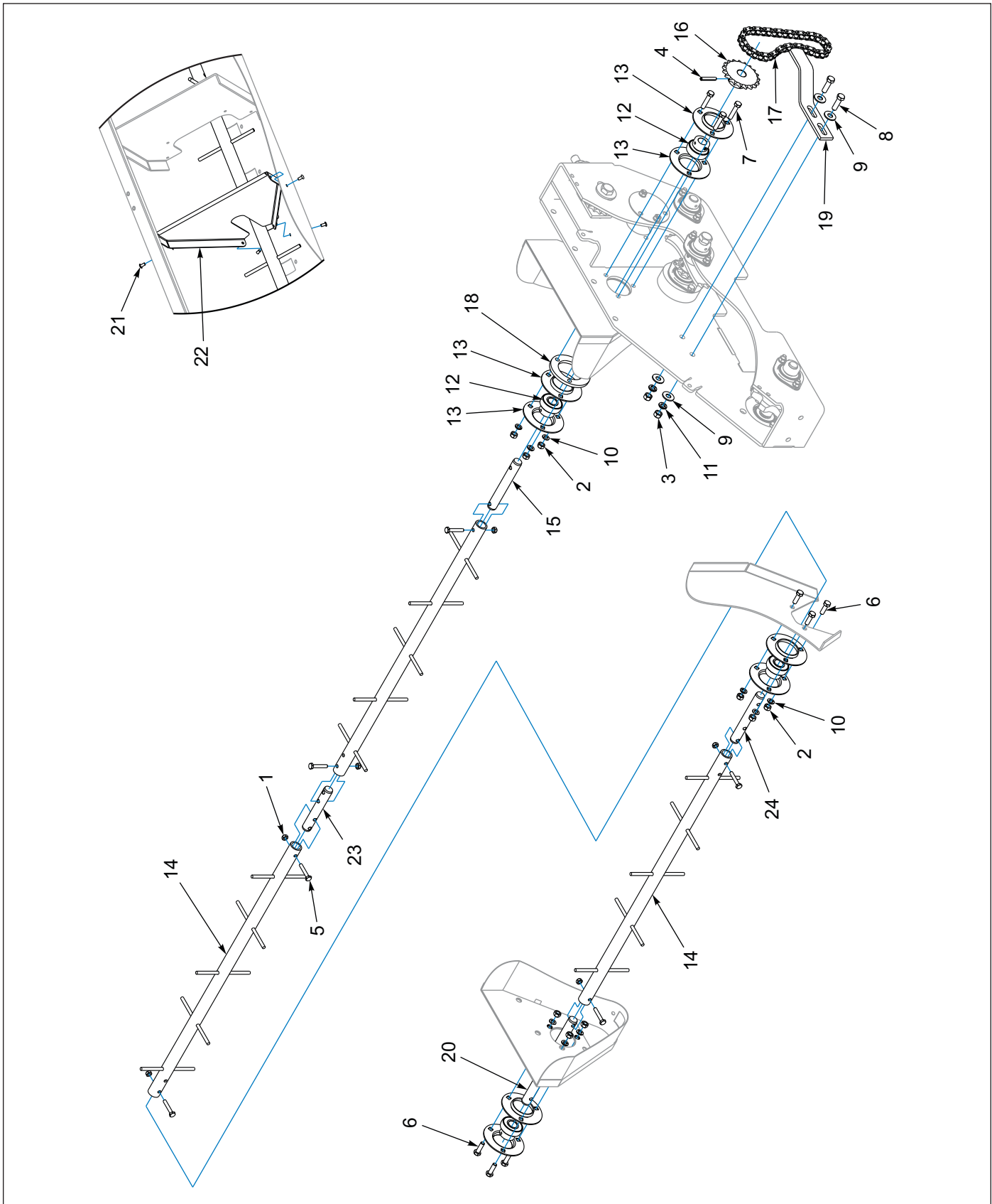
Figure 1-27: Agitator Kit, 8FT - Optional
