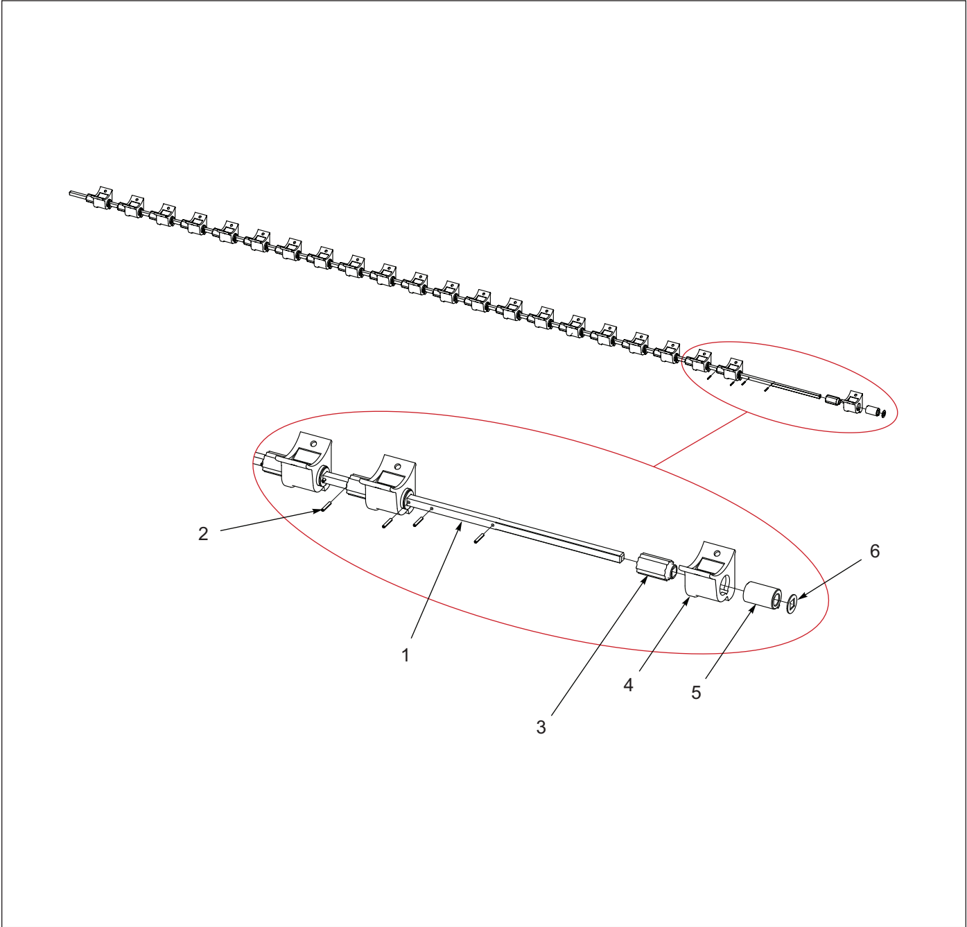
Figure 1-24: Seed Meter Assembly, 8FT
