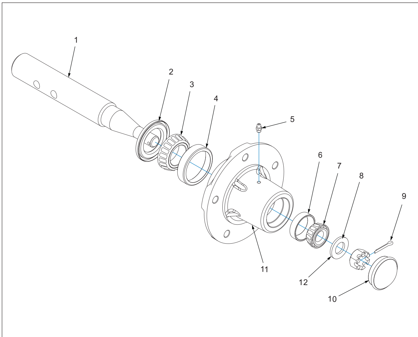
Figure 1-7: Hub and Spindle Assembly - 5 Bolt (Before 05/2021)
