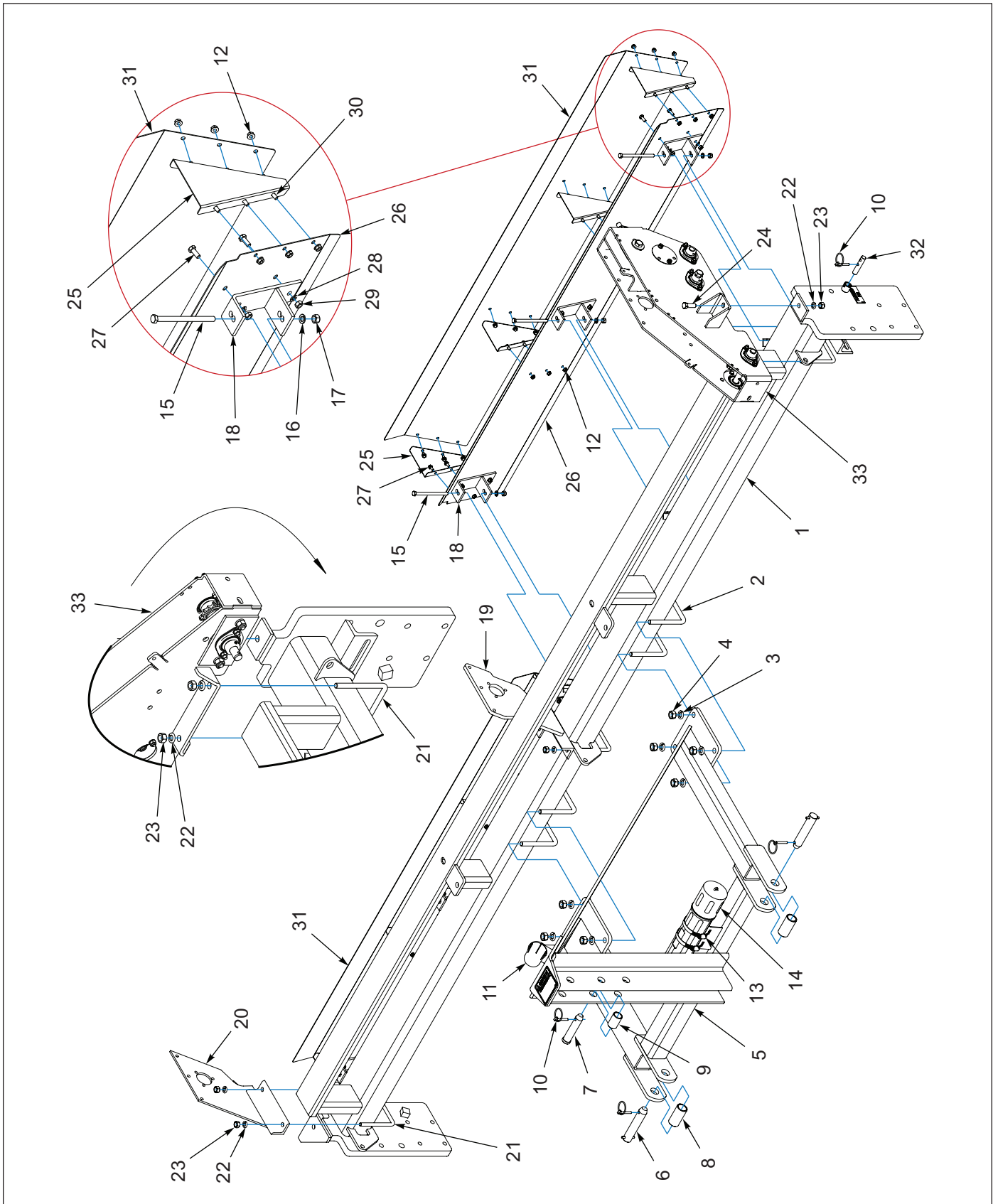
Figure 1-4: 3-PT Frame, Deflectors & Mounting - 10FT and 12FT
