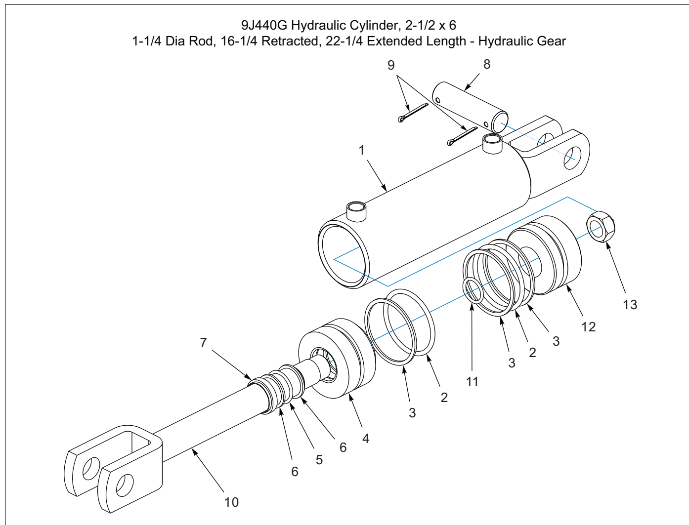
Figure 1-49: Hydraulic Cylinder, 2-1/2 x 6 - Hydraulic Gear (Before 01/14/2008)
