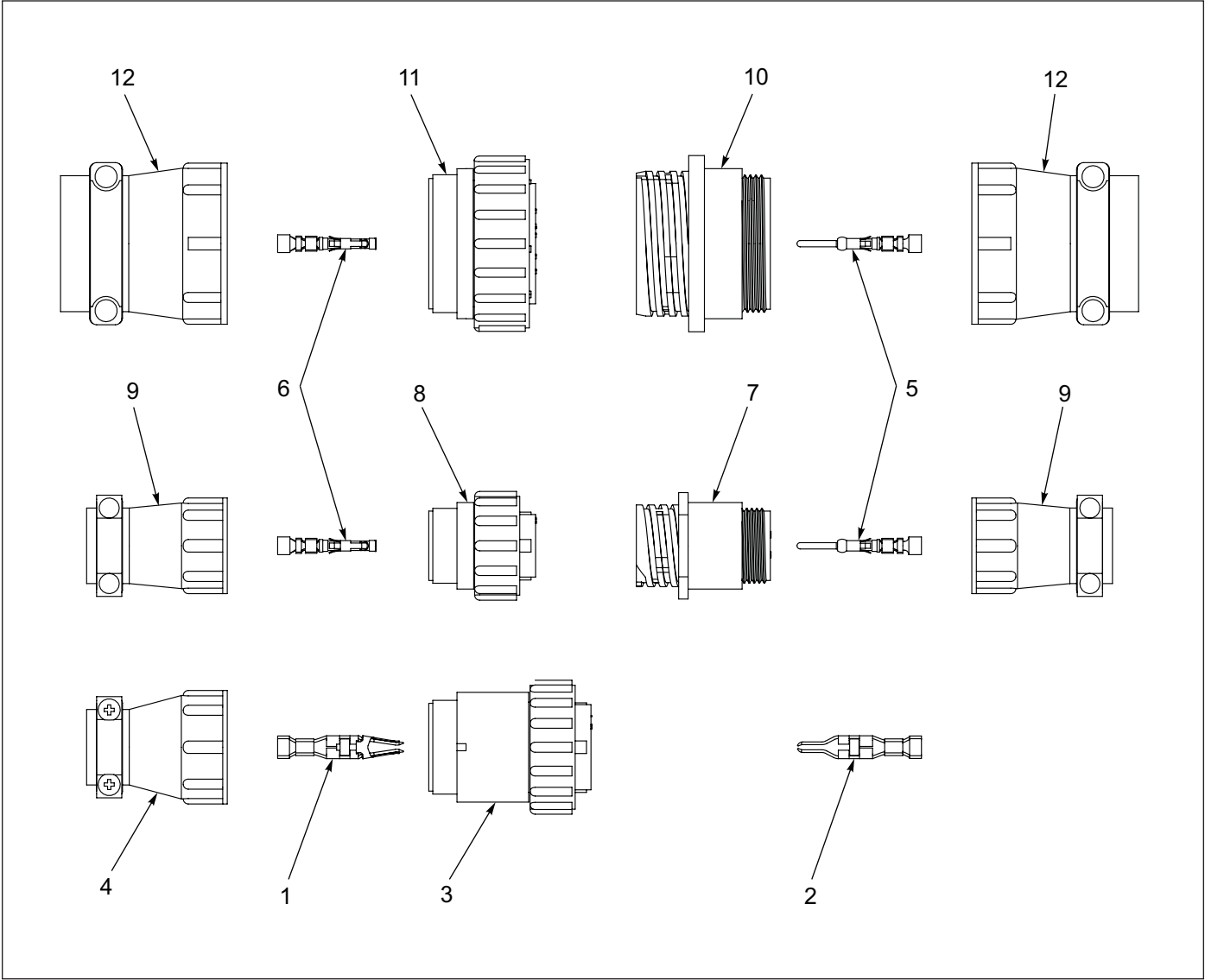
Figure 1-51: AMP Connectors
