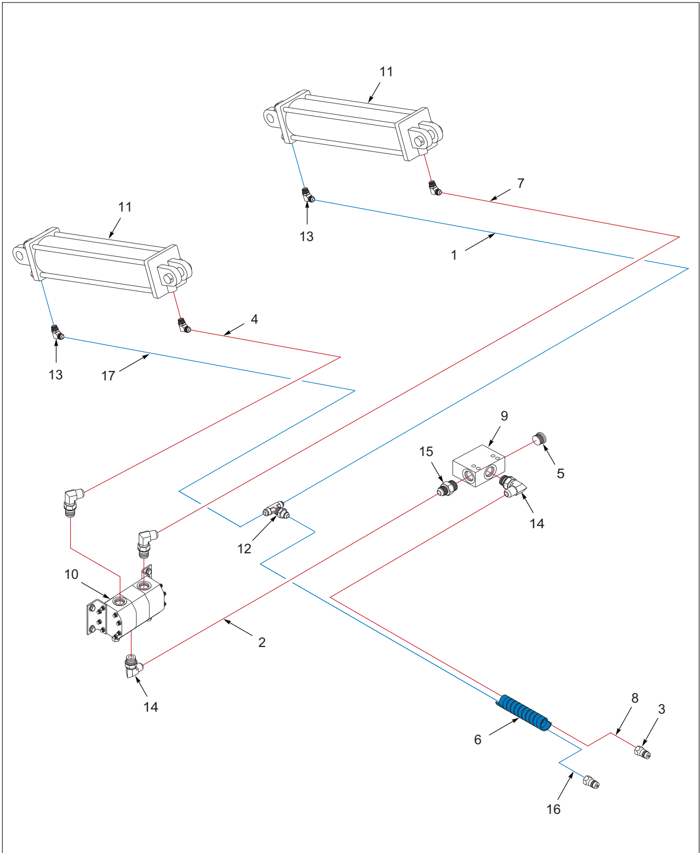
Figure 4-8: Caddy Lift Circuit (BEFORE 09/2025)
