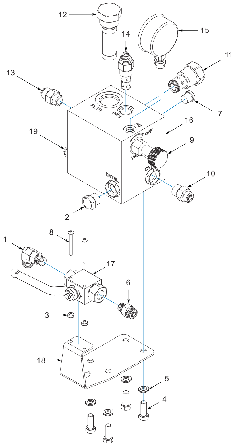
Figure 4-3: Manifold-Draft Assembly
