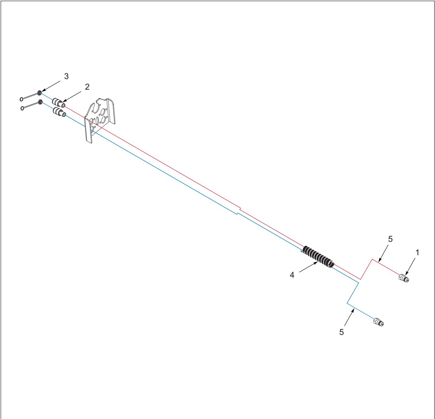
Figure 4-4: Caddy Auxiliary Circuit
