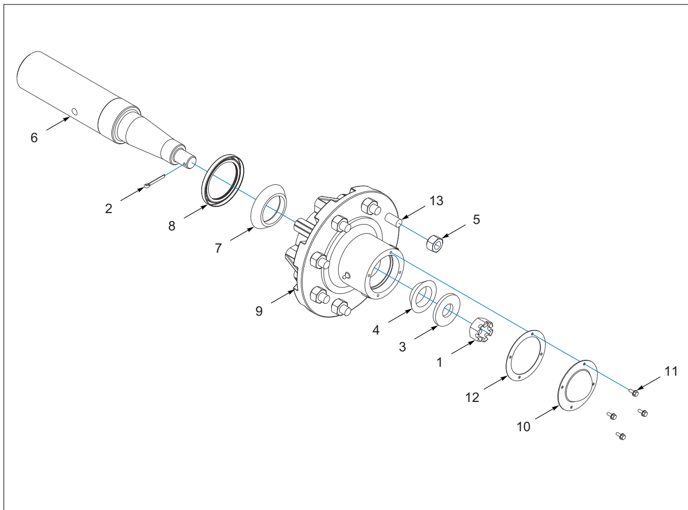
Figure 1-3: Standard Caddy Axle Spindle and Hub Assembly
