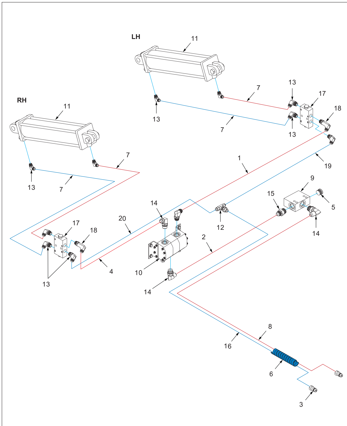
Figure 4-7: Caddy Lift Circuit (AFTER 09/2025)
