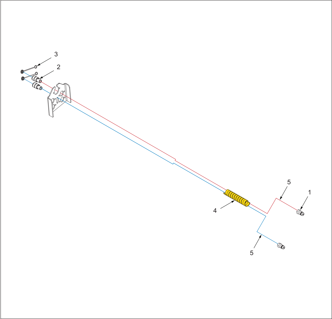
Figure 4-5: Caddy Wing Circuit
