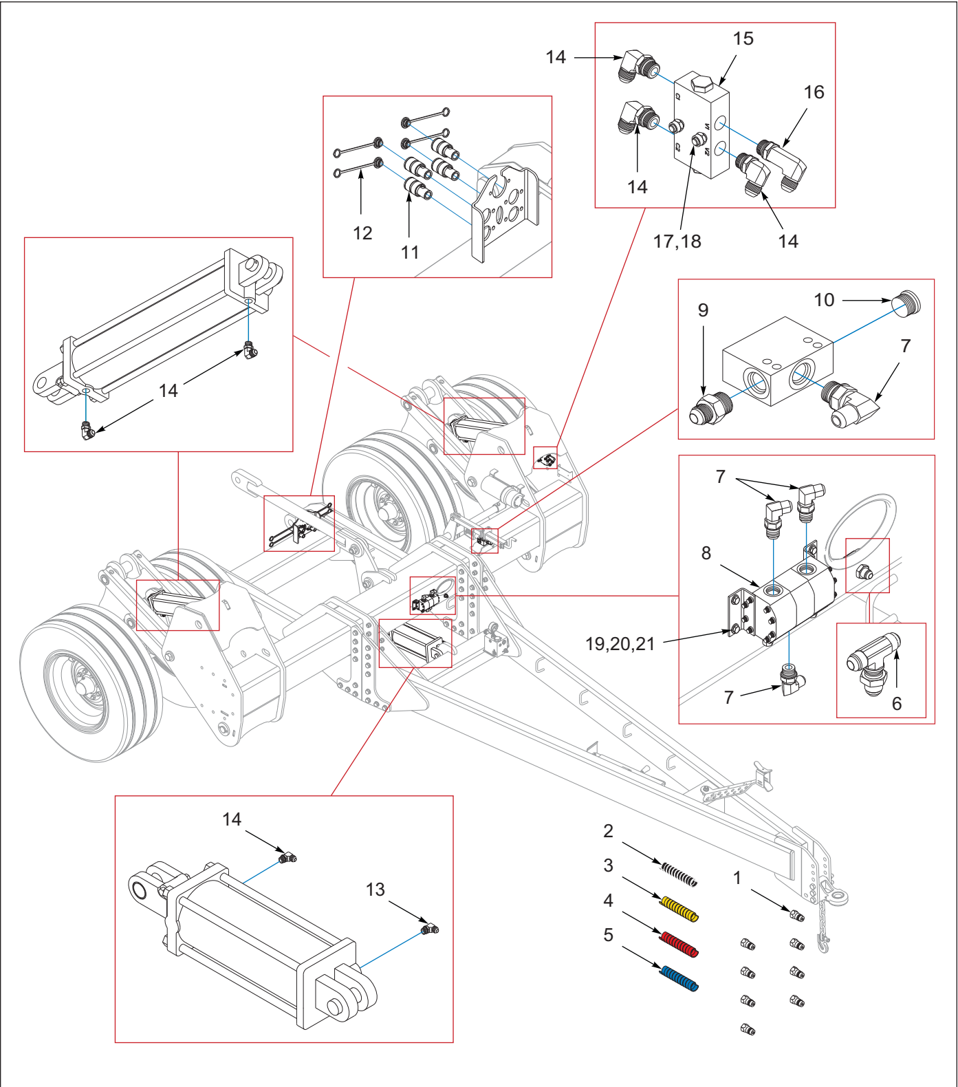
Figure 4-1: Hydraulic Kit (AFTER 09/2025)
