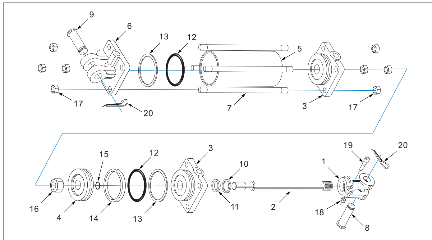
Figure 4-10: Lift Cylinder, 4-1/2 x 20 - 221792
