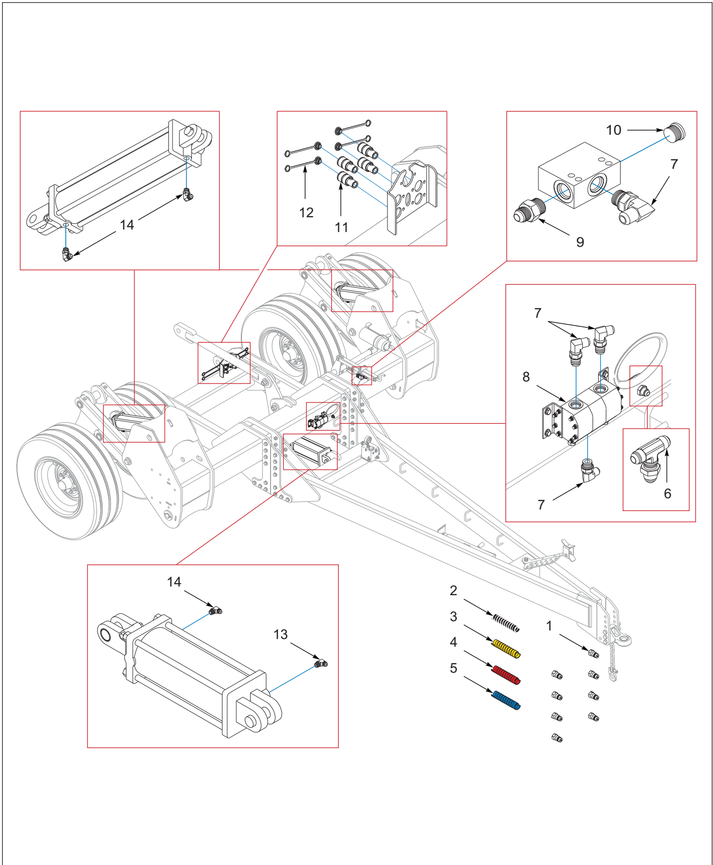
Figure 4-2: Hydraulic Kit (BEFORE 09/2025)
