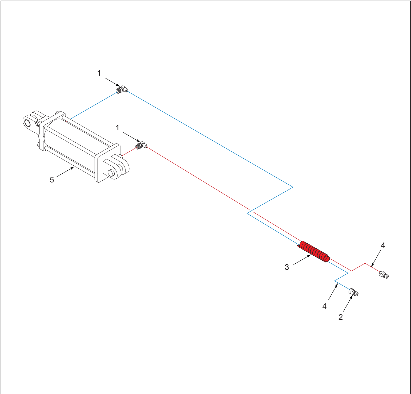
Figure 4-6: Caddy Top Link Circuit
