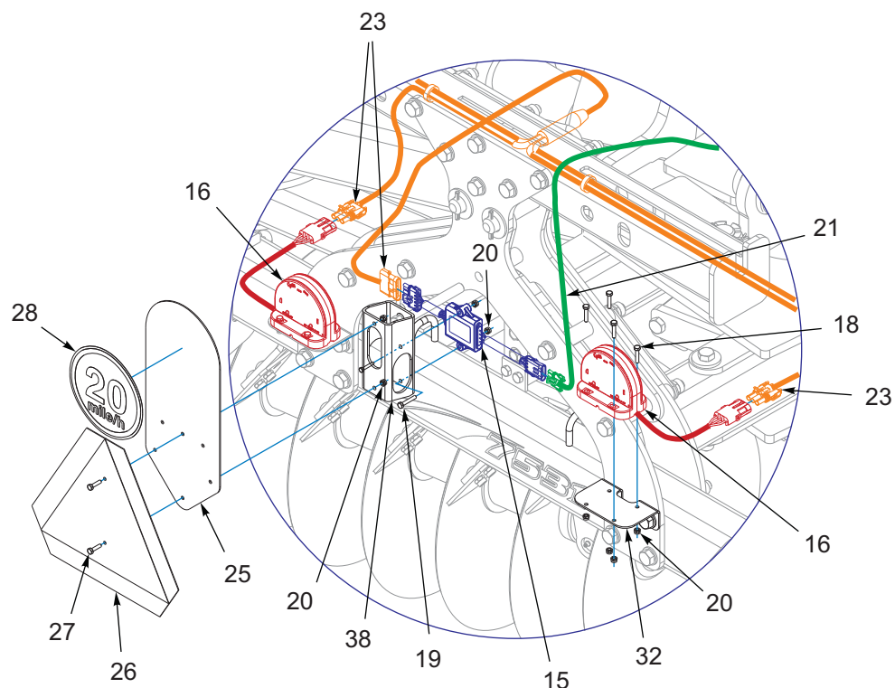
Figure 7-3: Electrical Assembly W/LED Lights (3 of 3)
