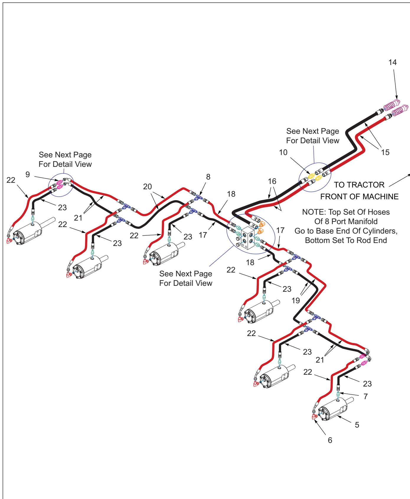
Figure 9-28: Reel Hydraulic Assembly (1 of 2)
