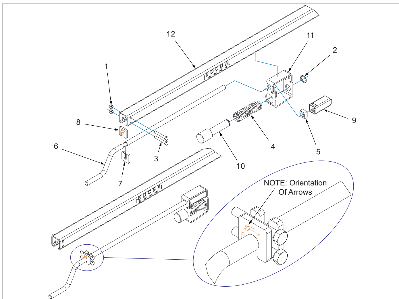
Figure 1-8: Depth Stop Assembly
