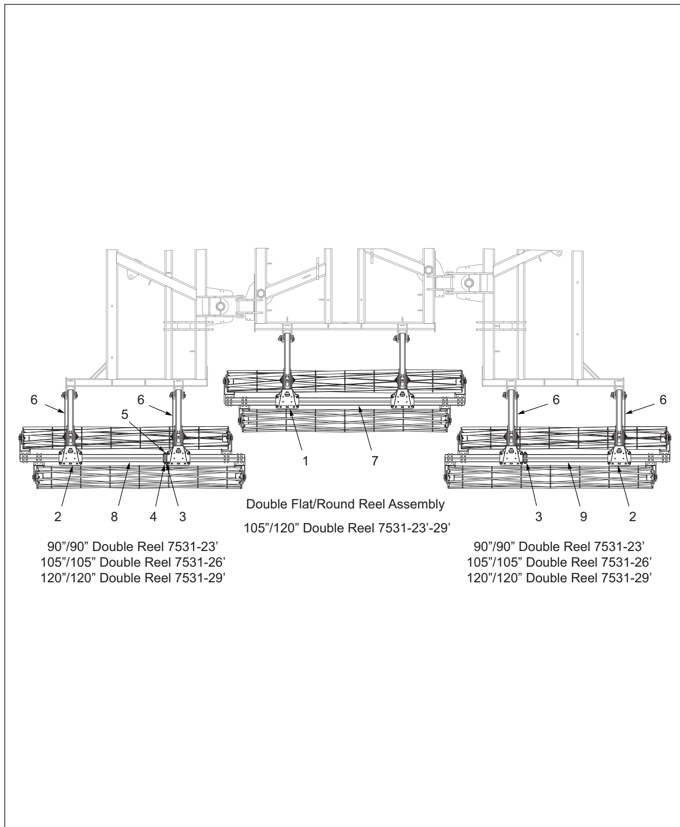
Figure 9-7: Double Flat/ Round Reel Assembly 7531-23'-29'
