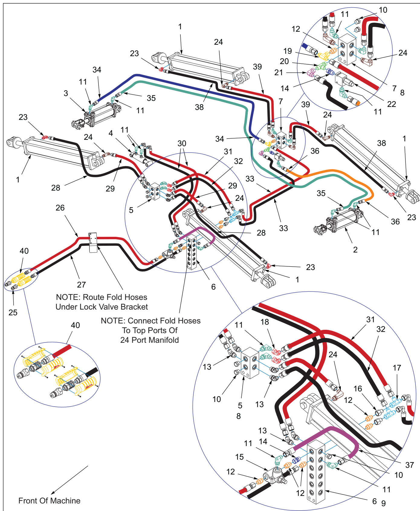
Figure 5-13: Hydraulic Assembly Fold 7531-32'-35' (Before S/N 75K2501921)
