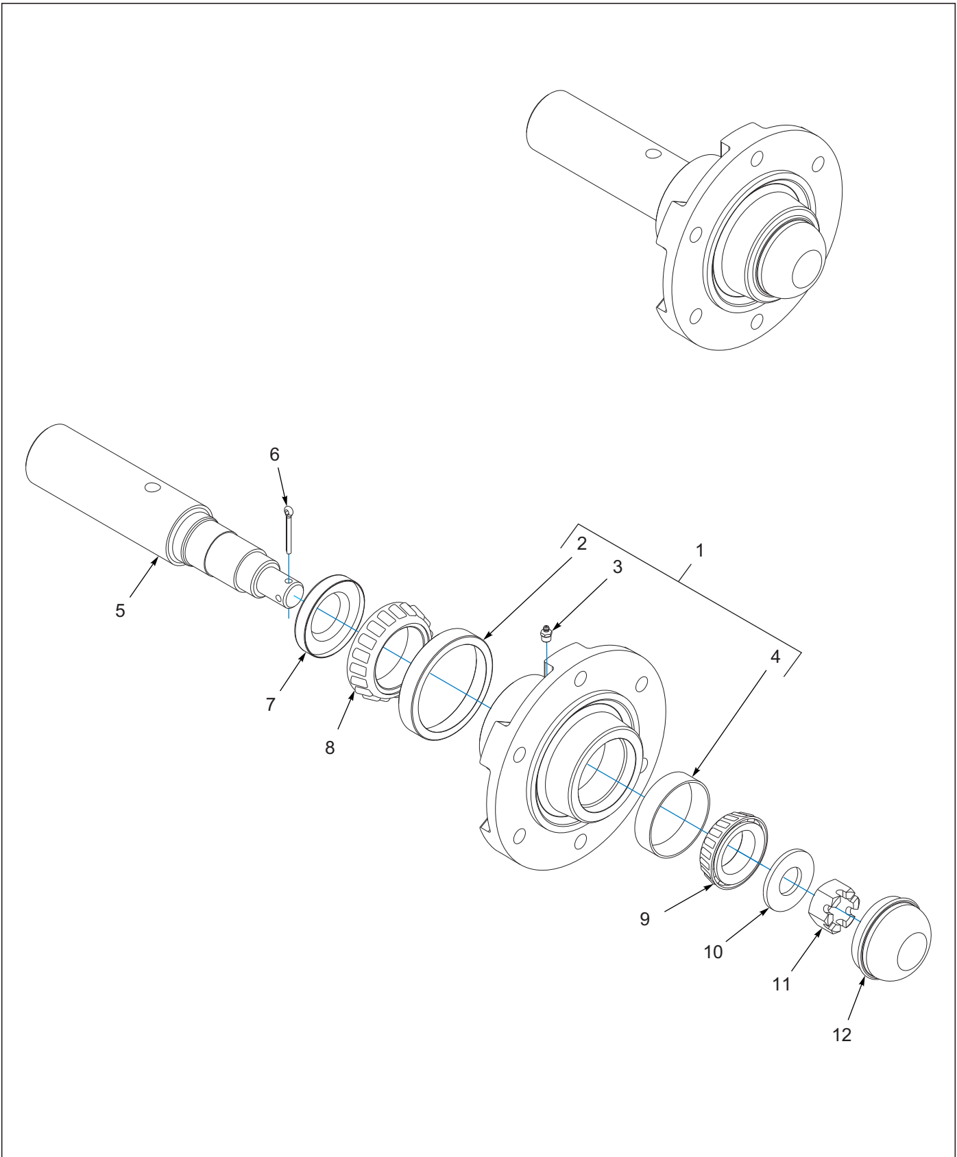
Figure 3-4: Hub/Spindle Assembly 224600
