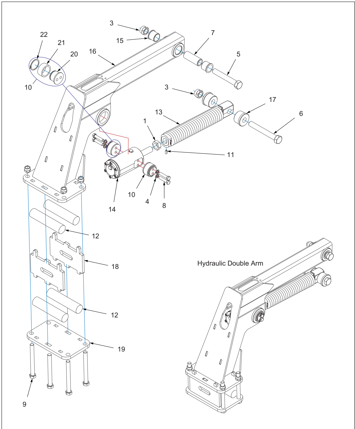
Figure 9-16: Hydraulic Double Arm Assembly
