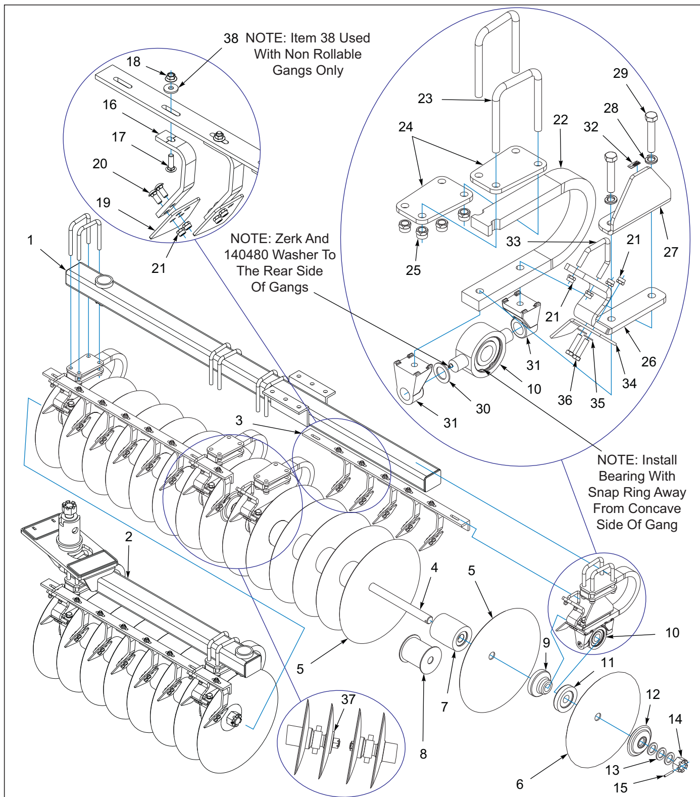
Figure 4-1: Disc Gang Assembly
