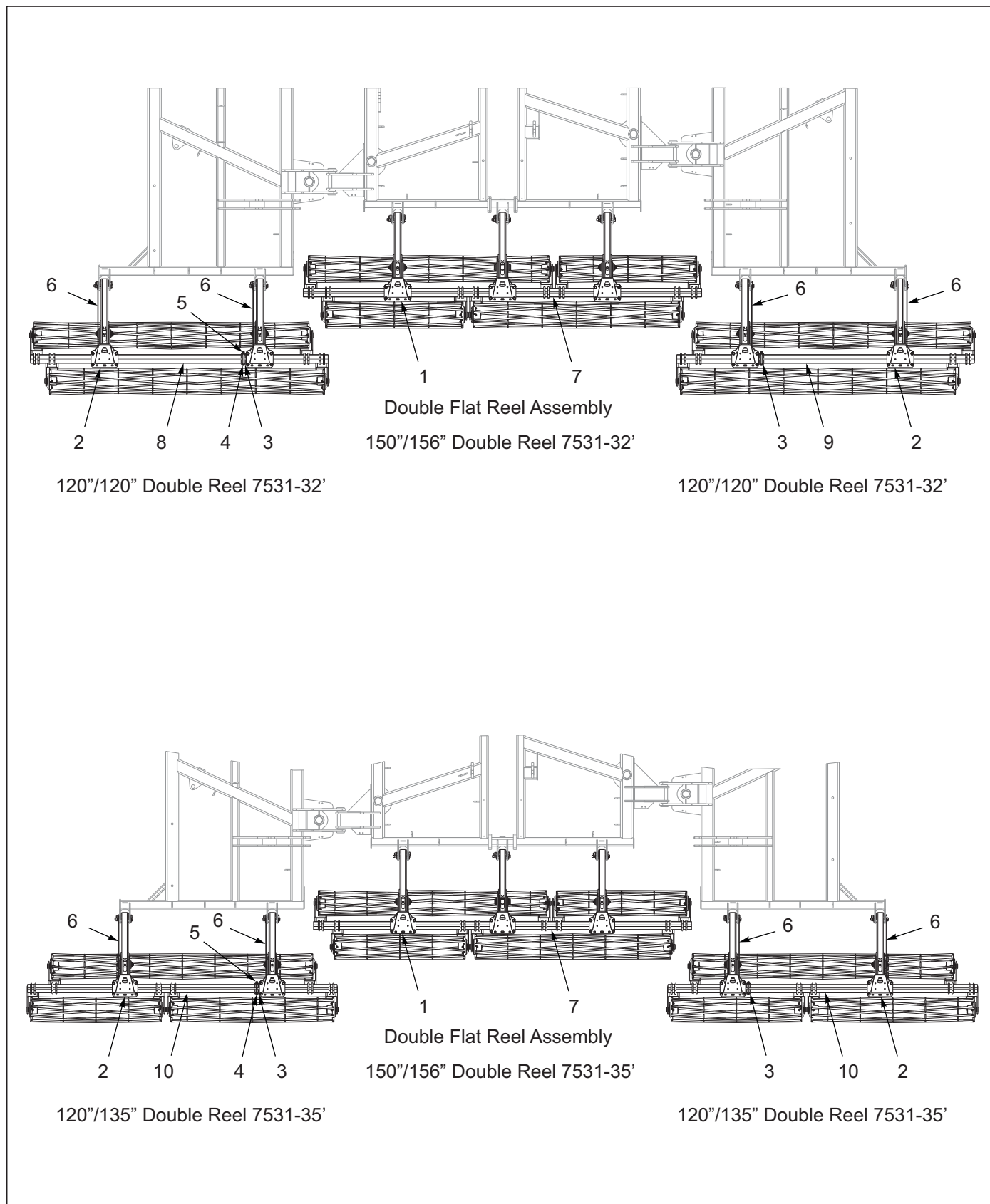
Figure 9-6: Double Flat Reel Assembly 7531-32'-35'
