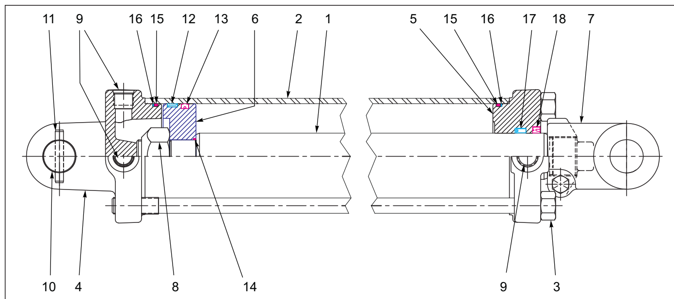
Figure 6-22: Cylinder Assembly 4 x 30 (Prince)
