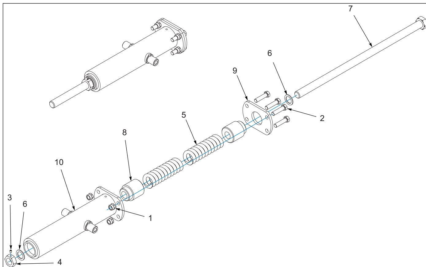
Figure 2-5: Leveler Spring Tube Assembly
