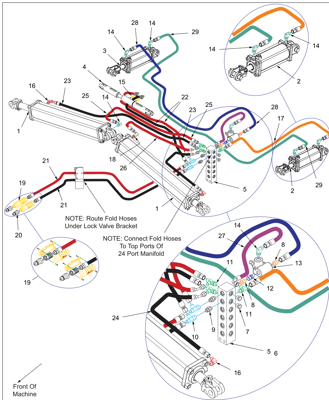
Figure 5-10: Hydraulic Assembly Fold 7531-23'
