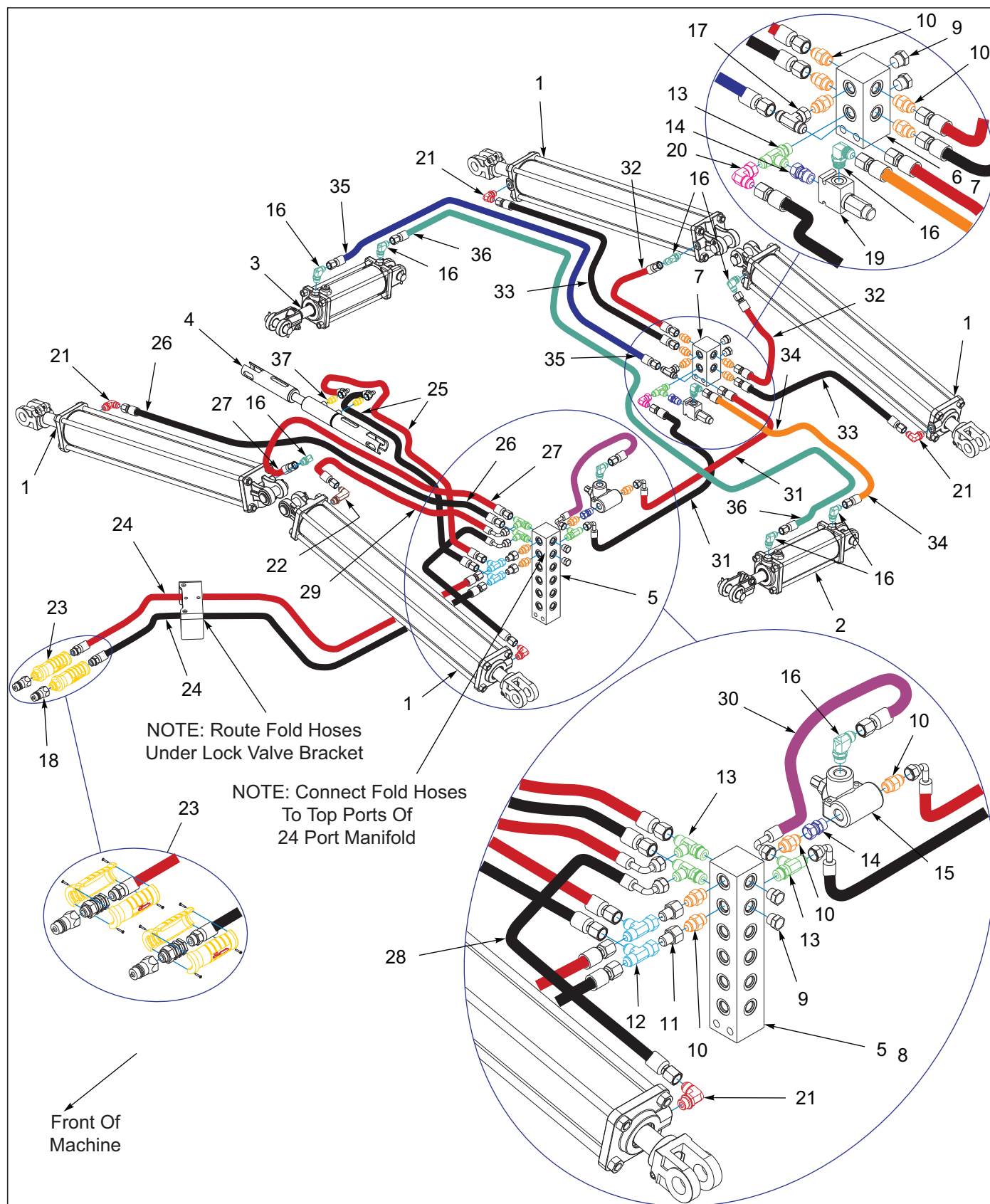
Figure 5-11: Hydraulic Assembly Fold 7531-26'-29' (Before S/N 75K2501921)
