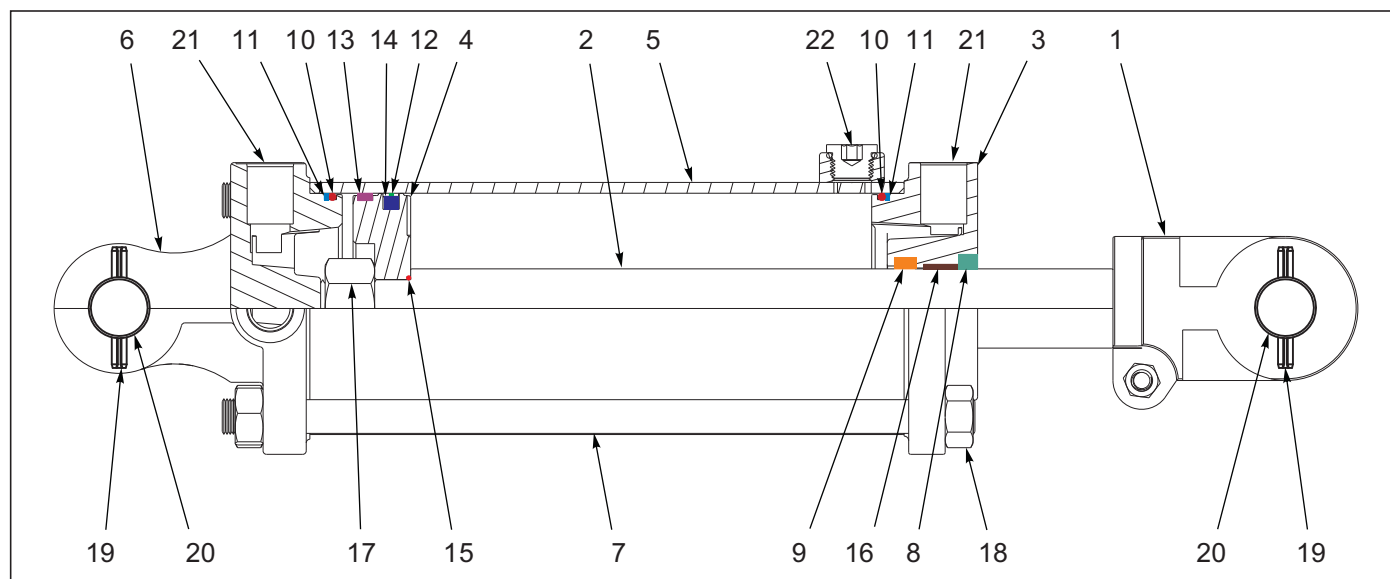
Figure 6-10: Cylinder Assembly 3-1/4 x 8 Rephase (Midway)
