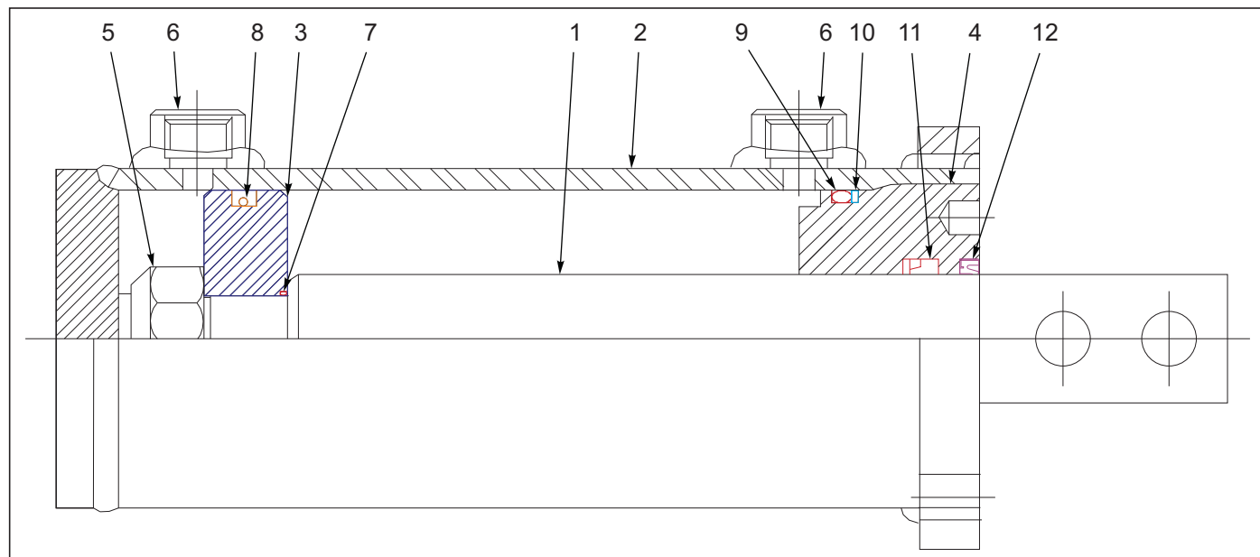
Figure 6-24: Cylinder Assembly 3-1/2 x 6
