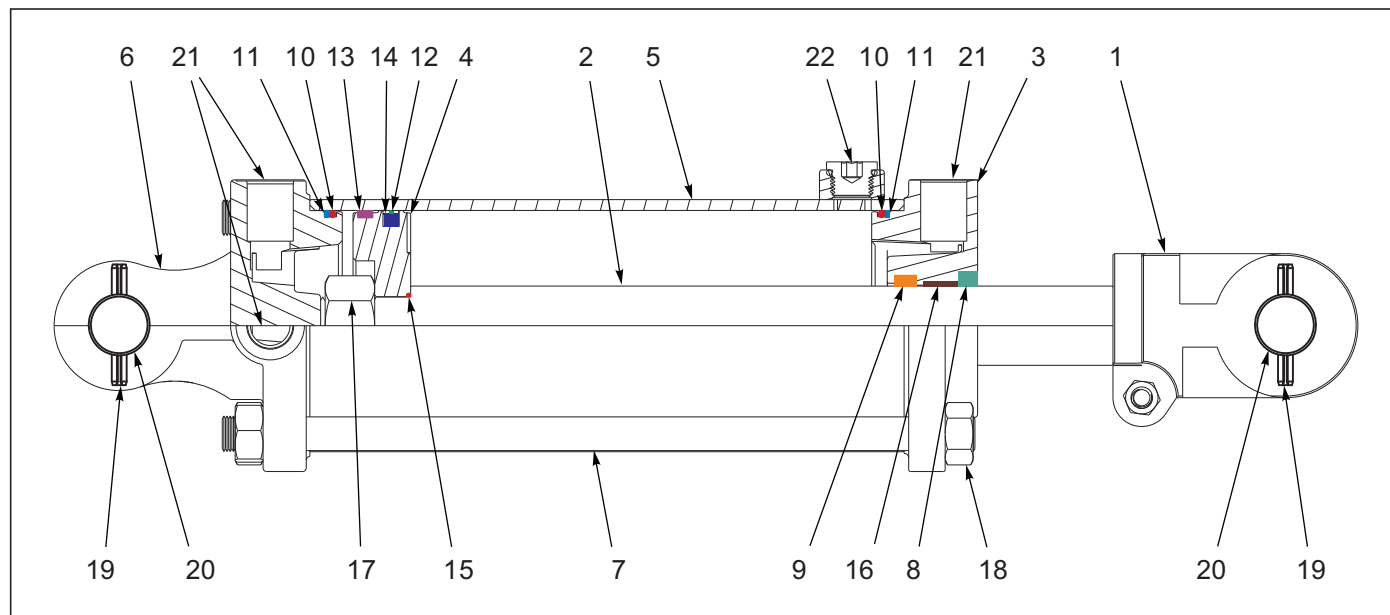
Figure 6-16: Cylinder Assembly 3-1/2 x 8, Rephase (Midway)
