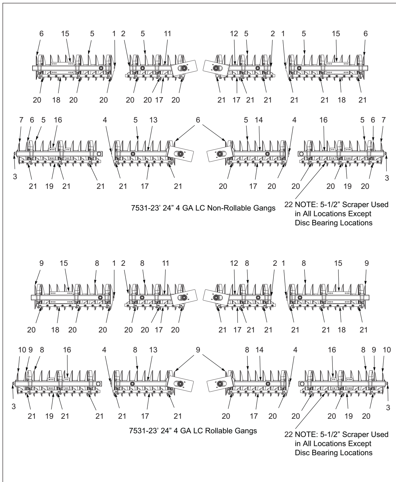
Figure 4-8: Disc Gang Assembly 7531-23'
