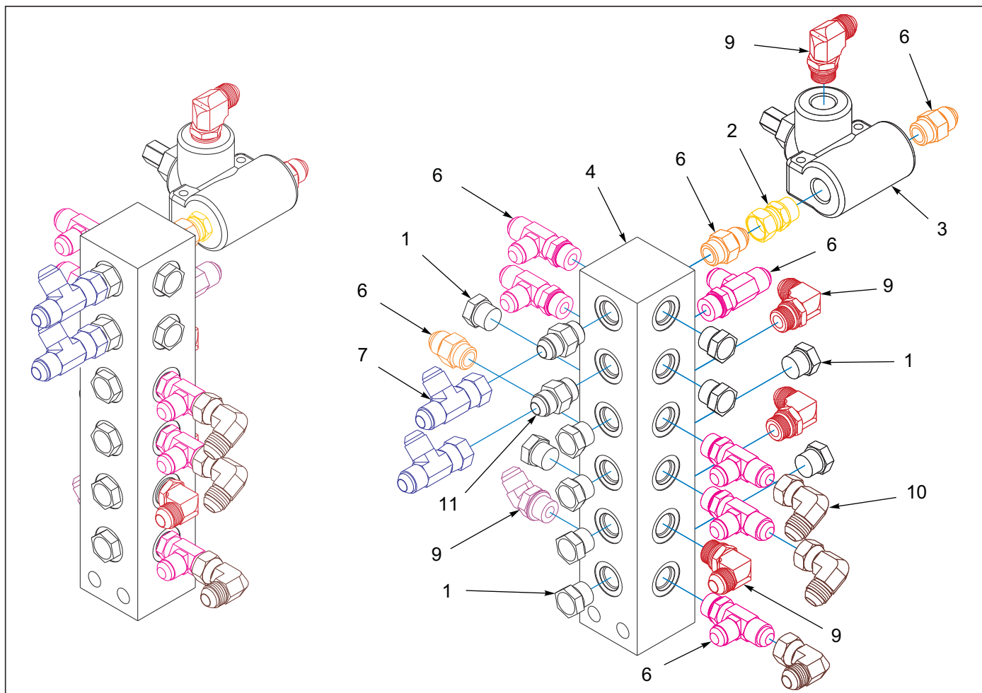
Figure 5-19: Manifold Assembly Front 7531-23'
