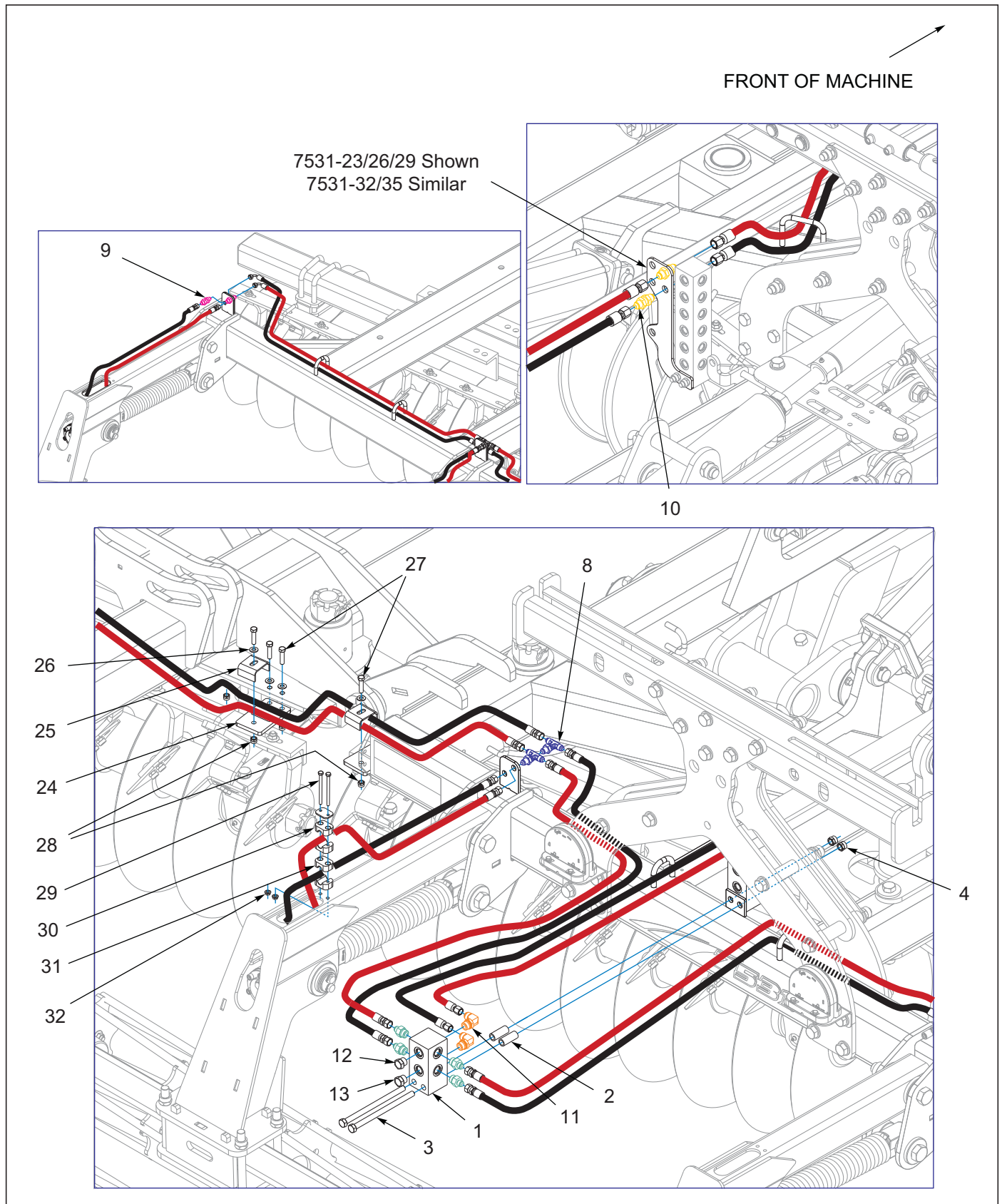
Figure 9-29: Reel Hydraulic Assembly (2 of 2)
