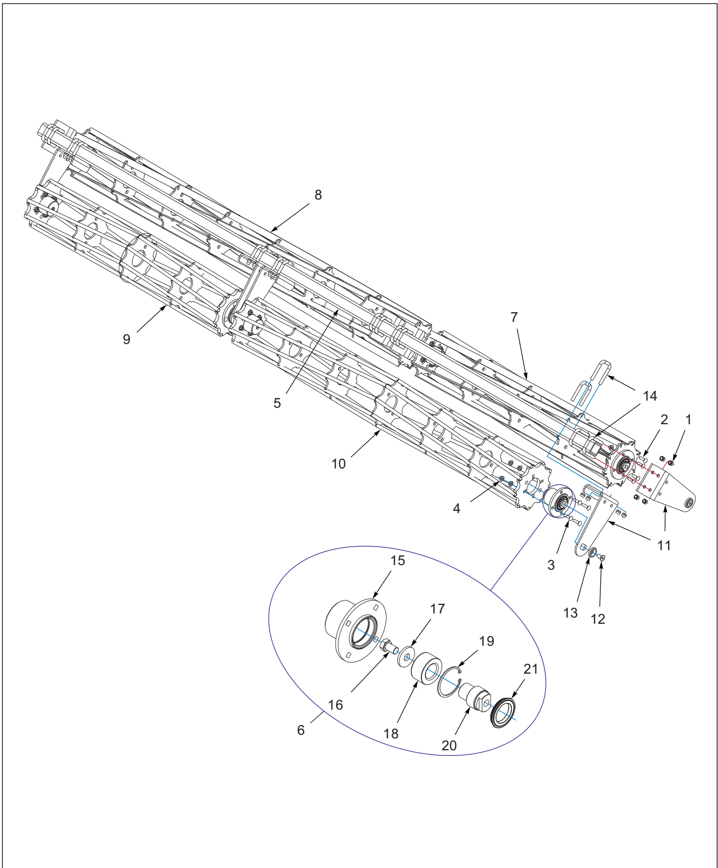
Figure 9-22: Double Flat/RD Reel Assembly 7531-32'-35' Center
