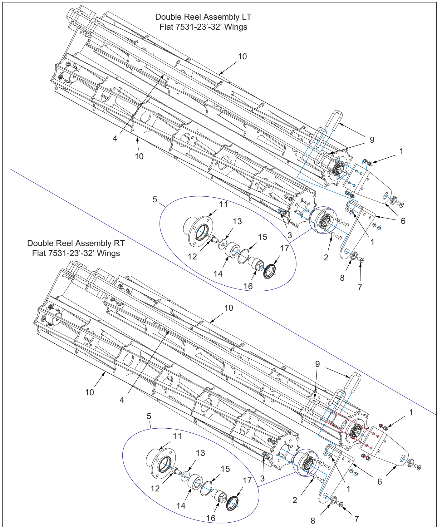
Figure 9-24: Double Flat Reel Assembly 7531-23'-32' Wings
