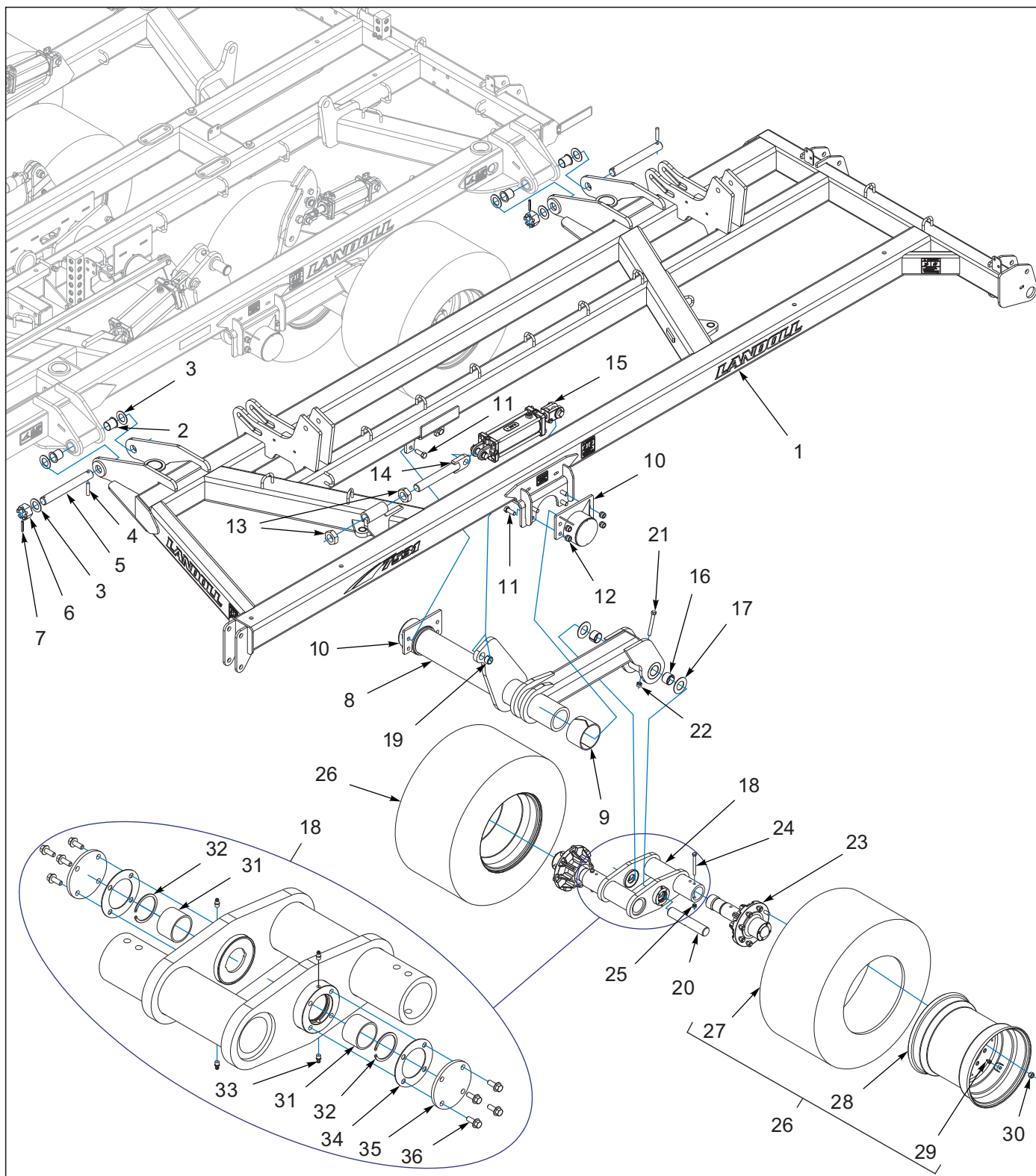
Figure 3-1: Frame Assembly Wing
