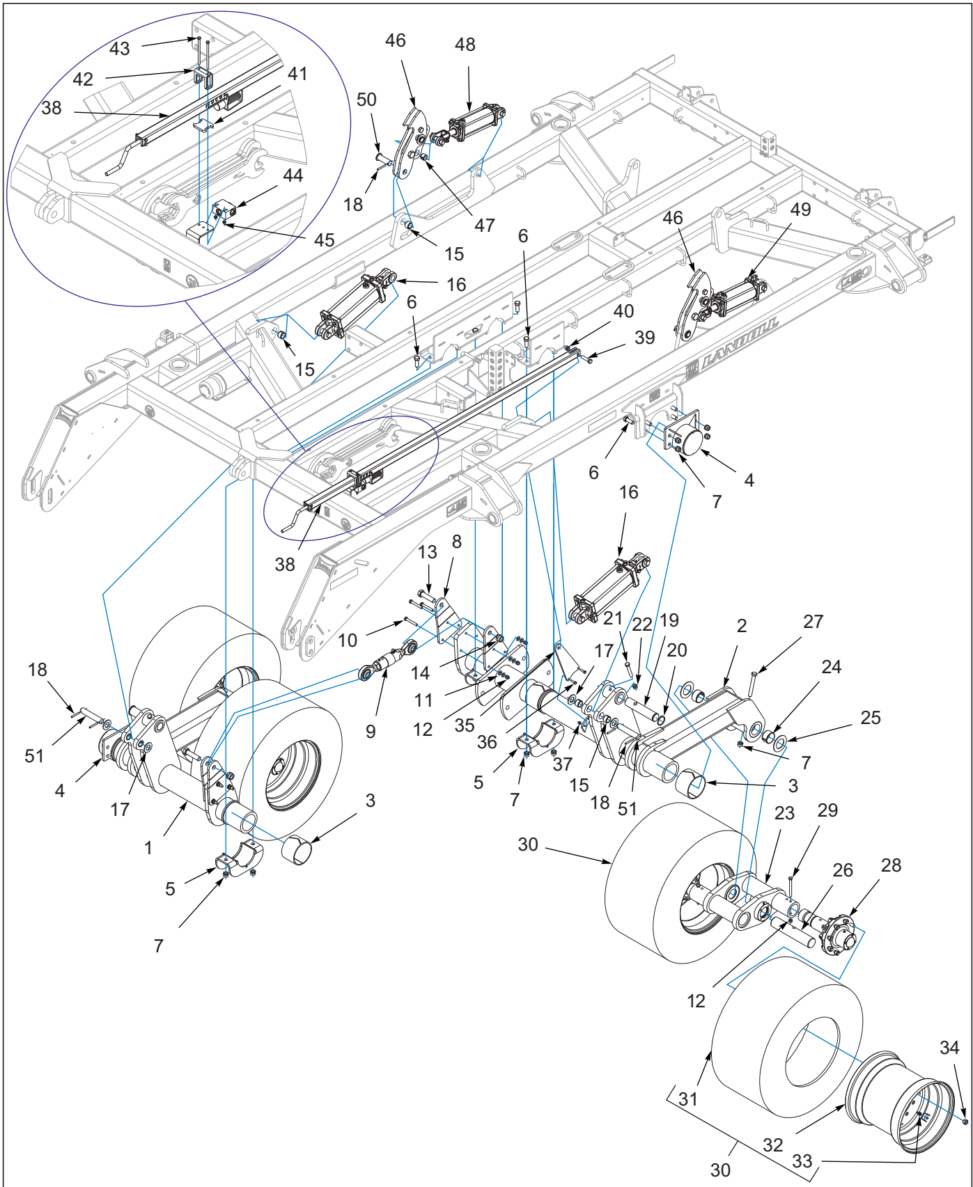
Figure 1-3: Frame Assembly Lift 7531-32'-35'
