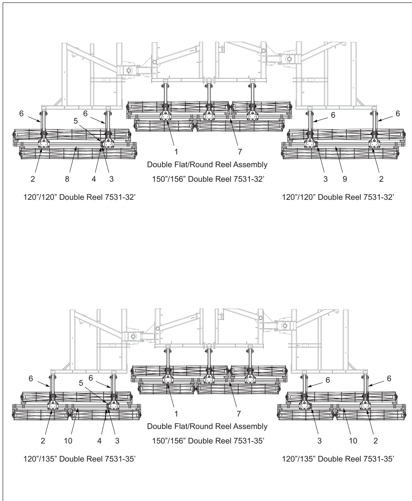
Figure 9-8: Double Flat/Round Reel Assembly 7531-32'-35'
