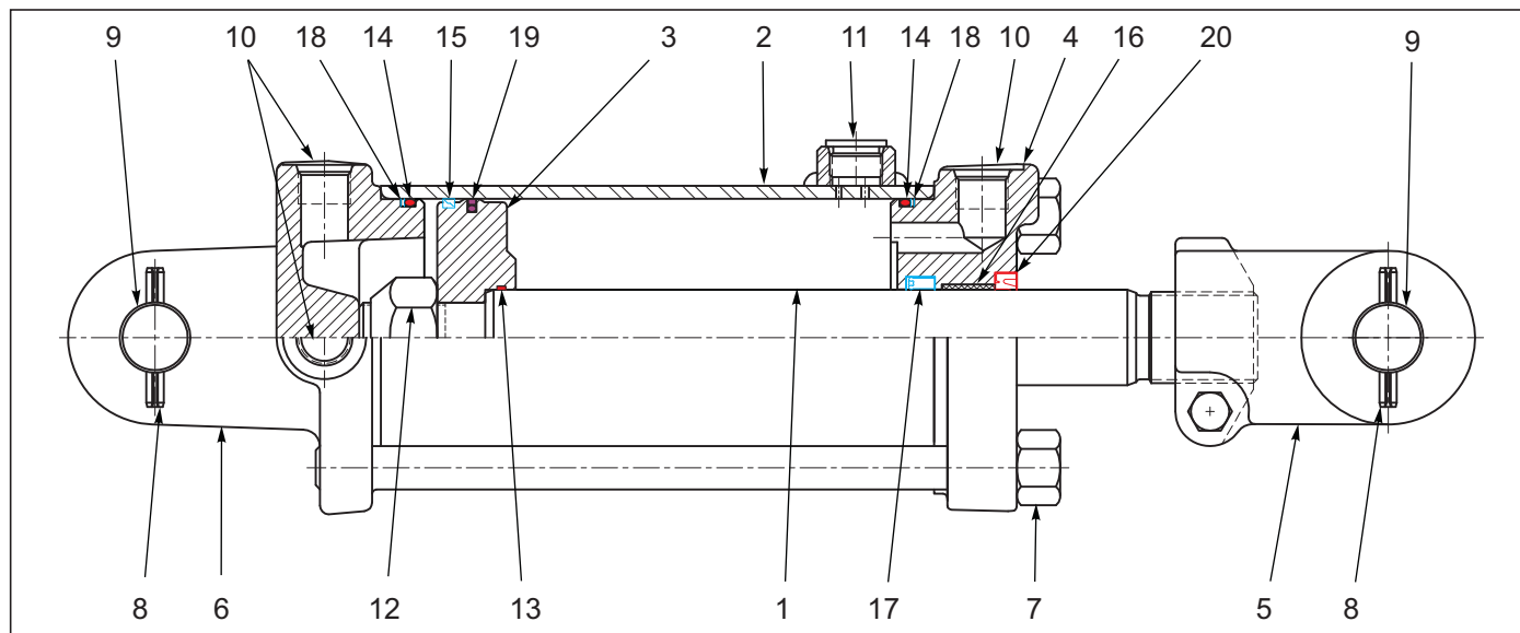
Figure 6-19: Cylinder Assembly 4 x 10 Rephase (Prince) (1-1/4 Clevis Pins)
