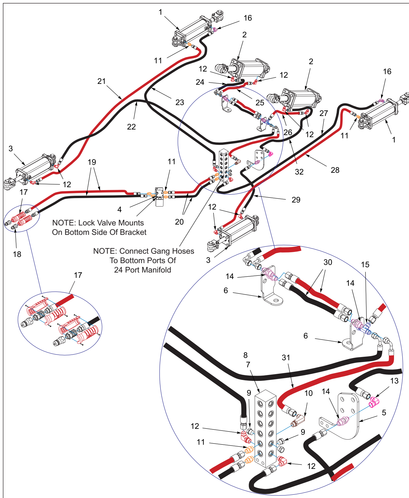
Figure 5-17: Hydraulic Assembly Gang 7531-32'-35'
