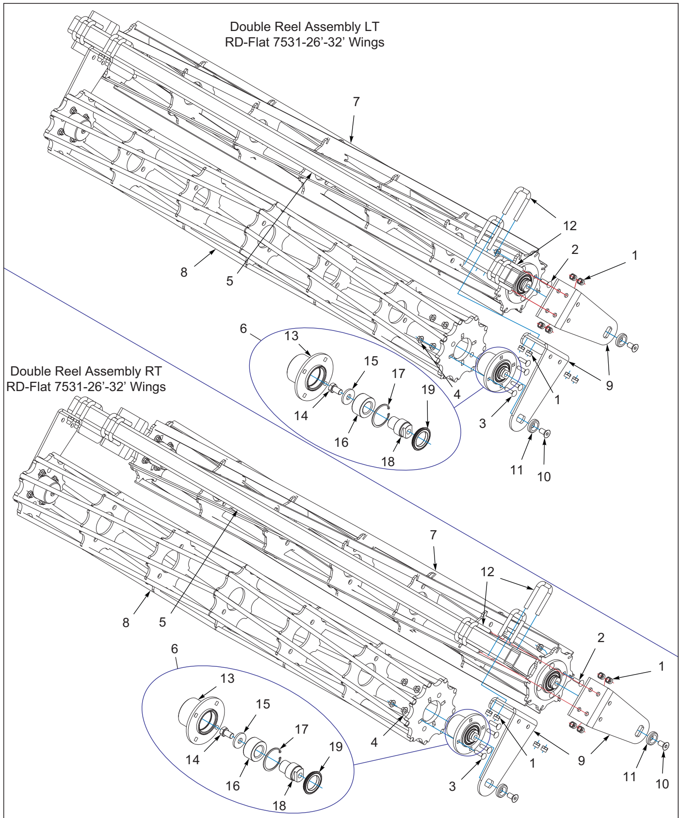
Figure 9-26: Double Flat/RD Reel Assembly 7531-23'-32' Wings
