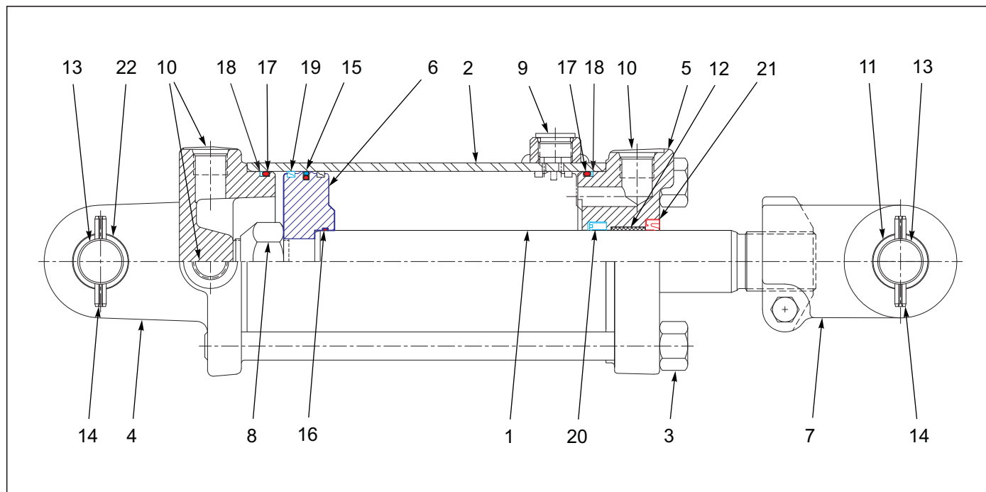
Figure 6-17: Cylinder Assembly 3-1/4 x 8, Rephase (Prince)
