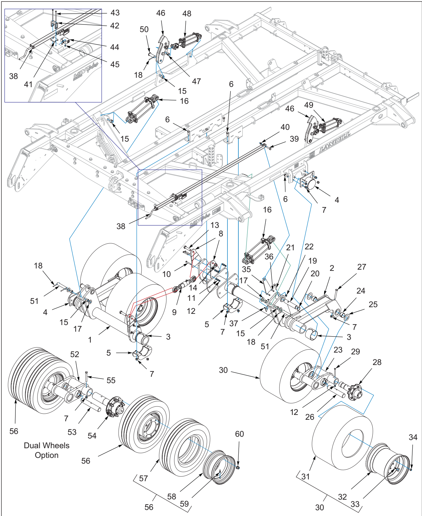
Figure 1-4: Frame Assembly Lift 7531-32'-35'
