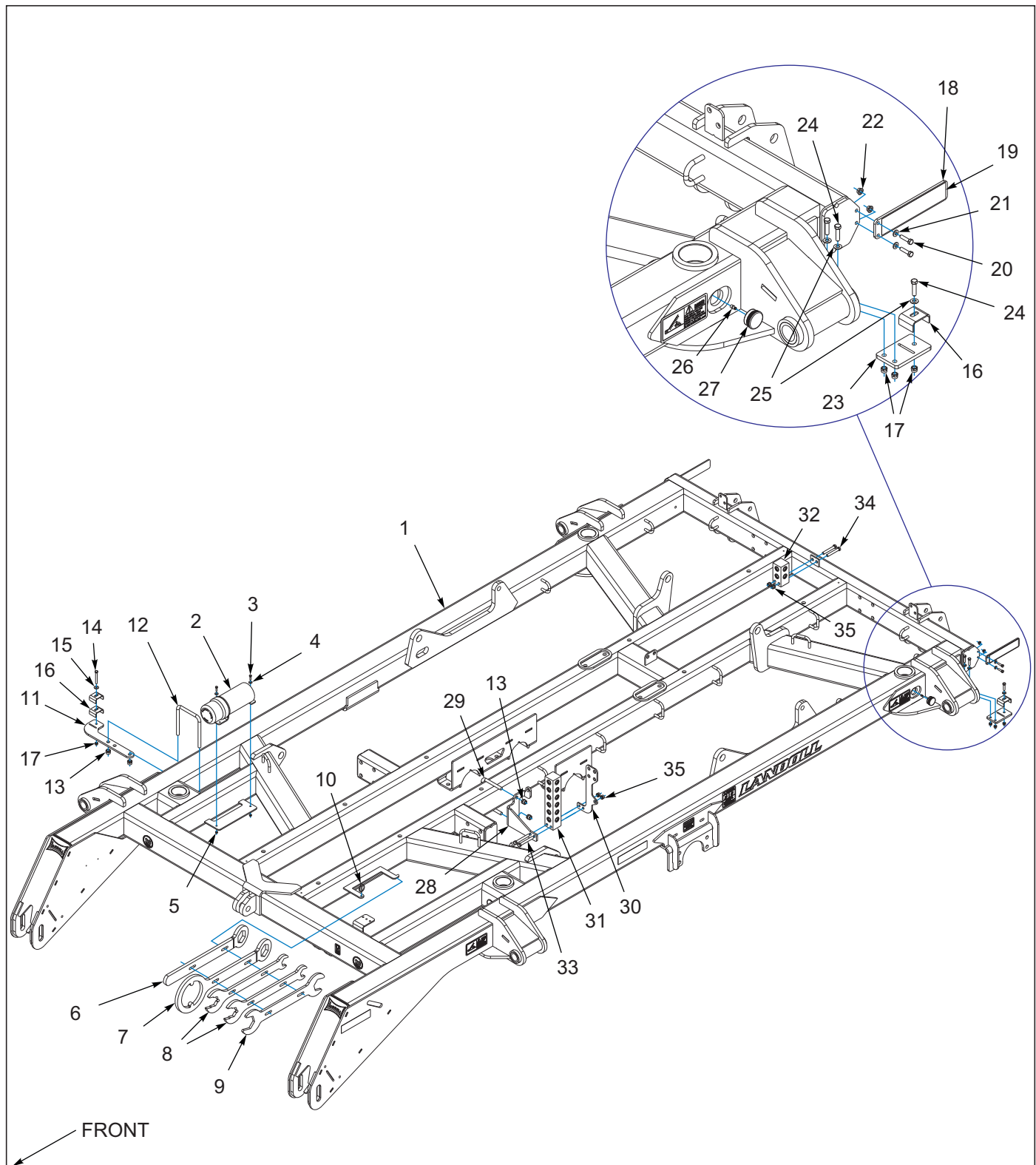
Figure 1-1: Frame Assembly 23'-26'-29'
