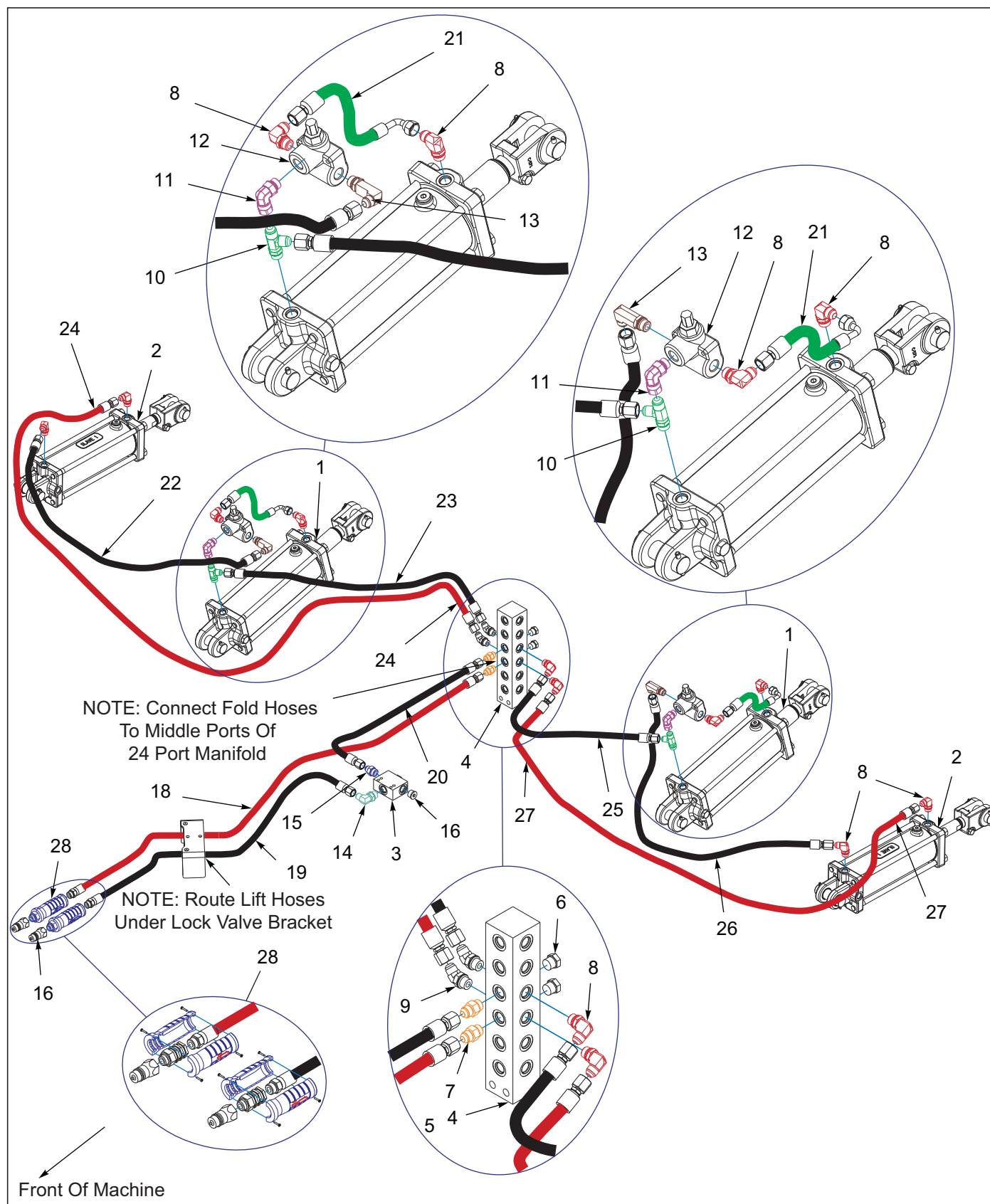
Figure 5-2: Hydraulic Assembly Lift 7531-32'-35'
