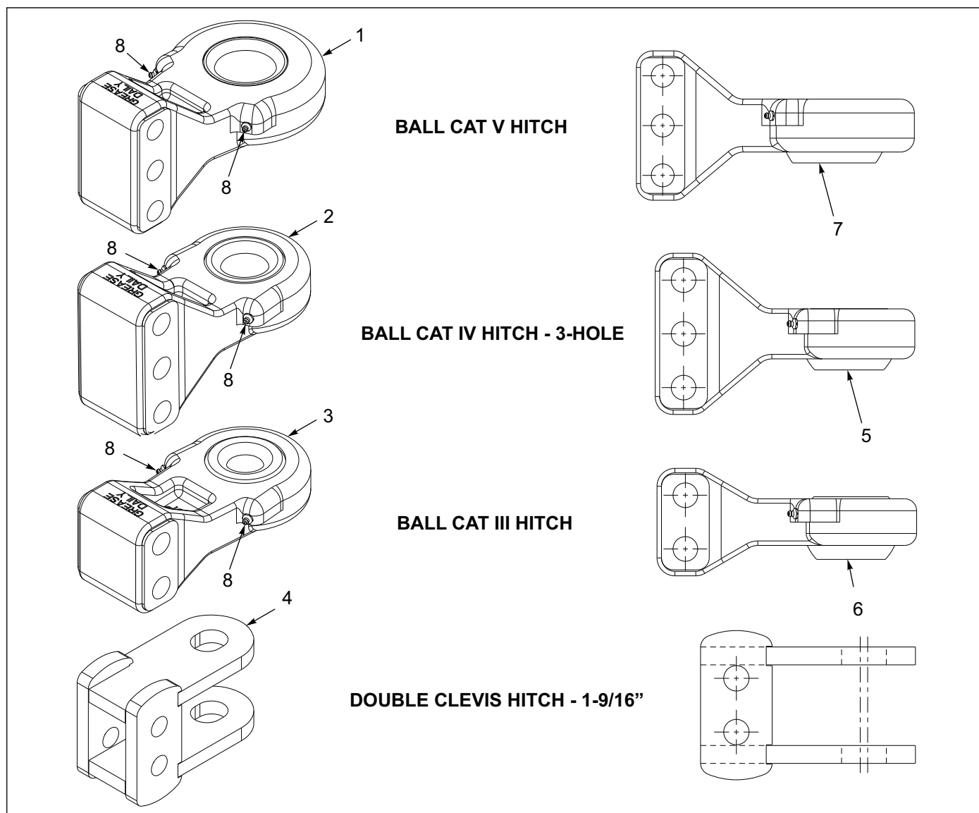
Figure 2-3: Ball & Clevis Assembly
