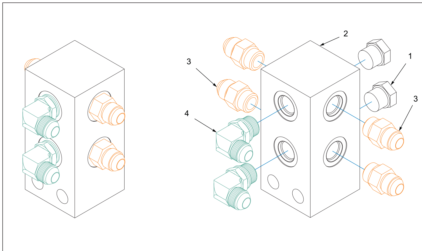
Figure 5-23: Manifold Assembly Front 7531-26'/29' After
