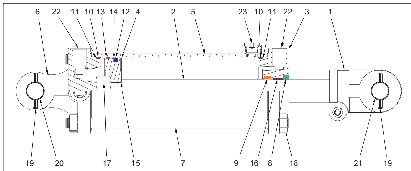
Figure 6-6: Cylinder Assembly 4-1/2 x 8 Rephase (Midway)
