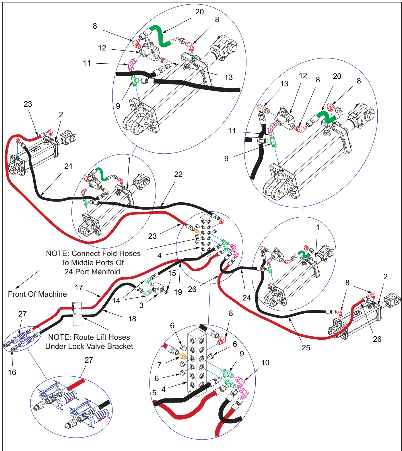
Figure 5-1: Hydraulic Assembly Lift 7531-23'-26'-29'
