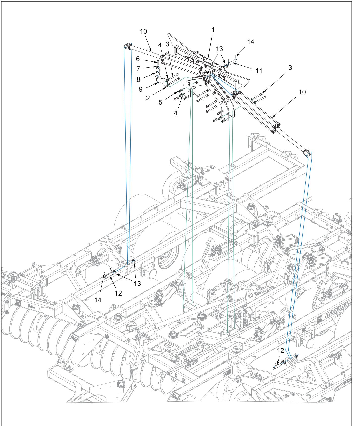
Figure 5-3: Fold Stabilizer Assembly 7531-23'
