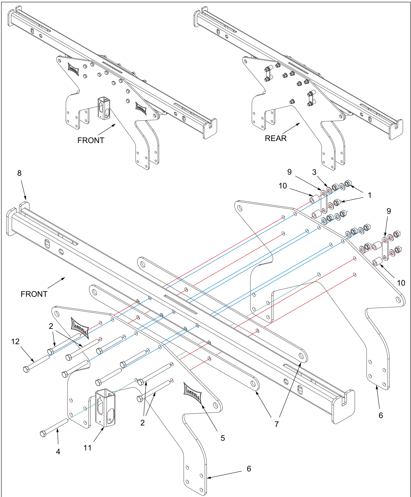
Figure 5-9: Wing Fold Stabilizer Assembly 7531-32'-35' Rear
