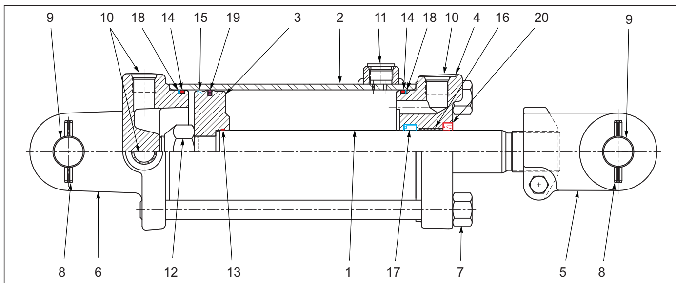
Figure 6-1: Cylinder Assembly 4 x 10 Rephase (Prince)
