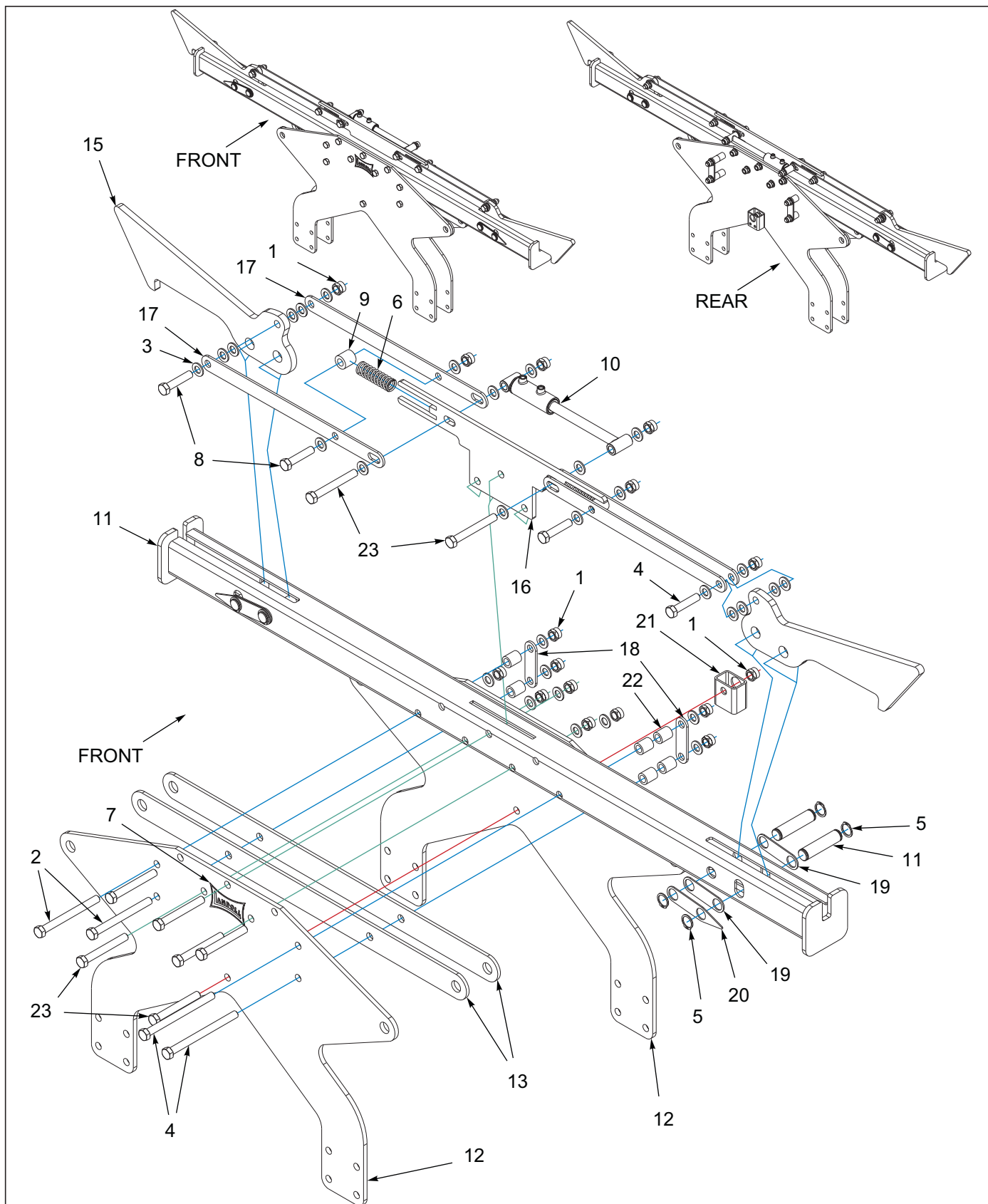
Figure 5-8: Wing Fold Stabilizer Assembly 7531-32'-35' Front
