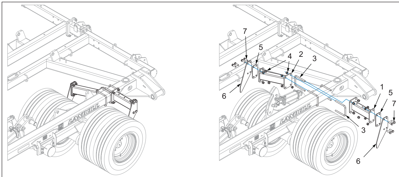
Figure 1-6: Dual Wheel Scraper Assembly
