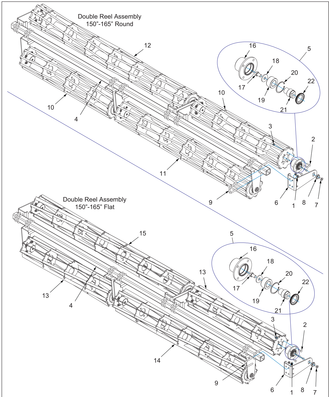
Figure 9-20: Double Reel Assembly 7531-32'-35' Center
