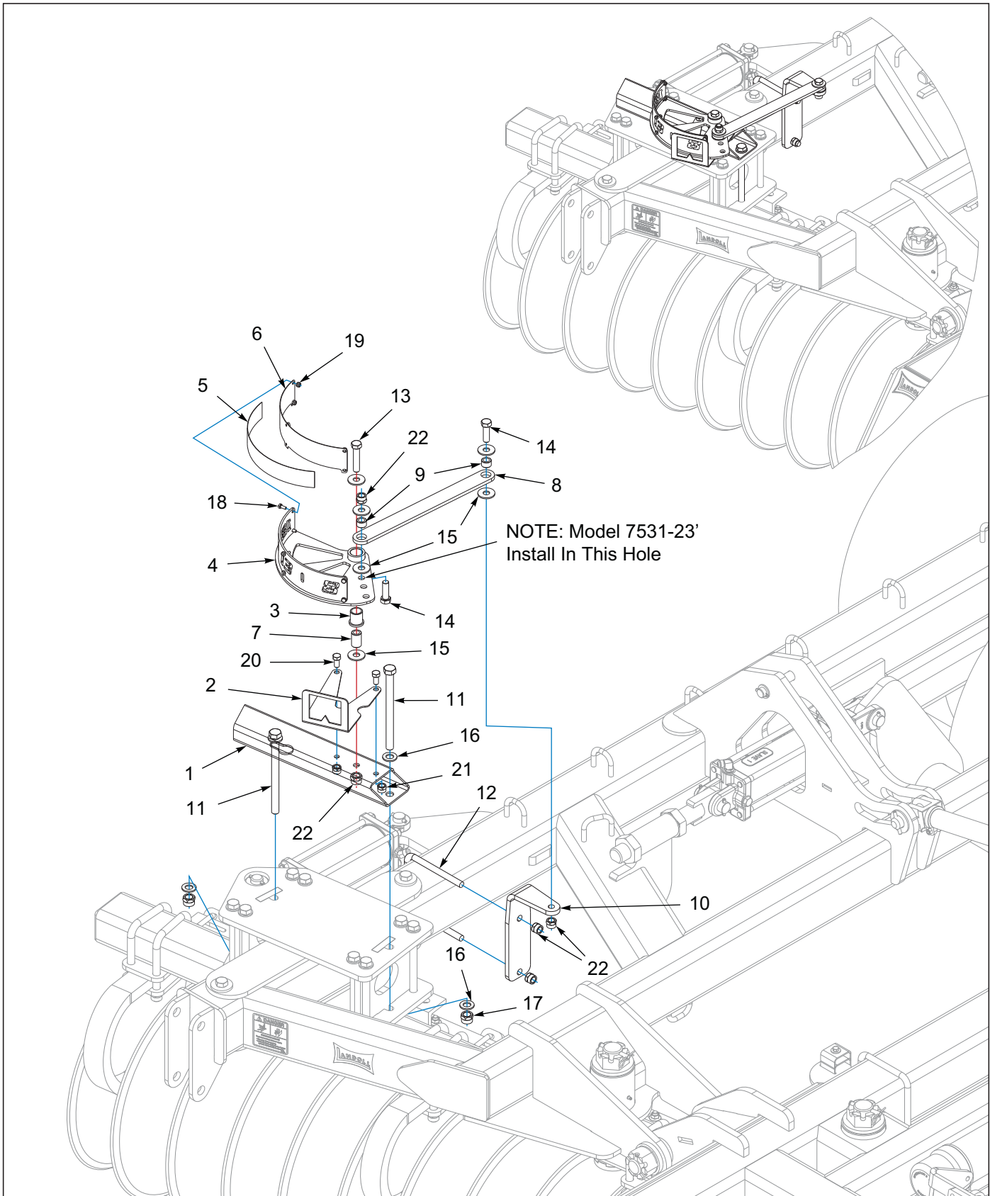
Figure 4-6: Gang Wing Gauge Assembly 7531-23'
