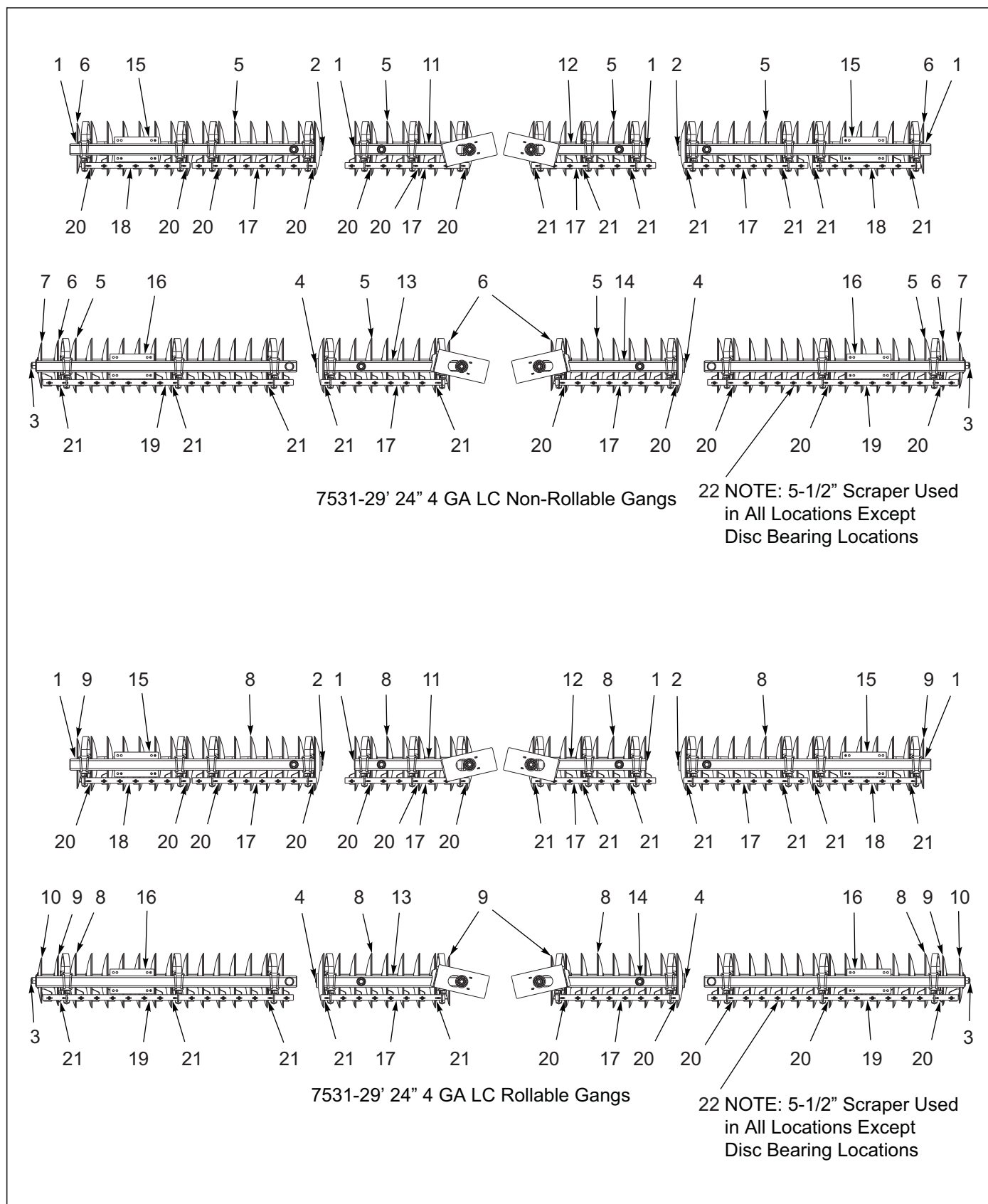
Figure 4-10: Disc Gang Assembly 7531-29'
