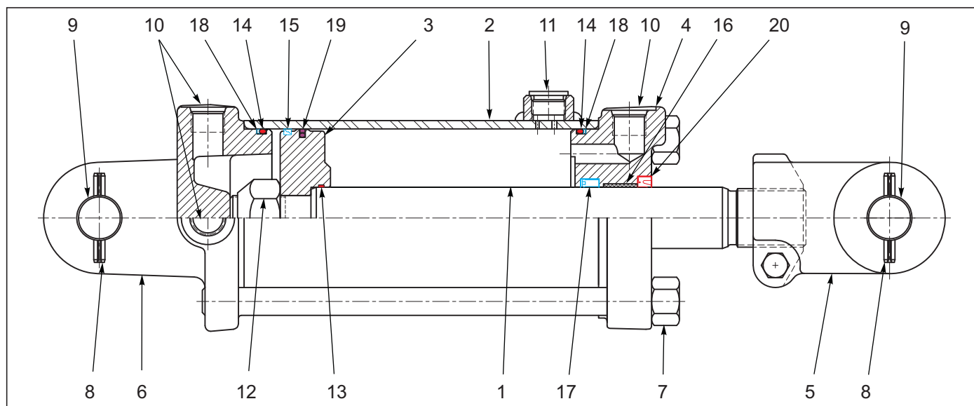
Figure 6-5: Cylinder Assembly 4-1/2 x 8 Rephase (Prince)
