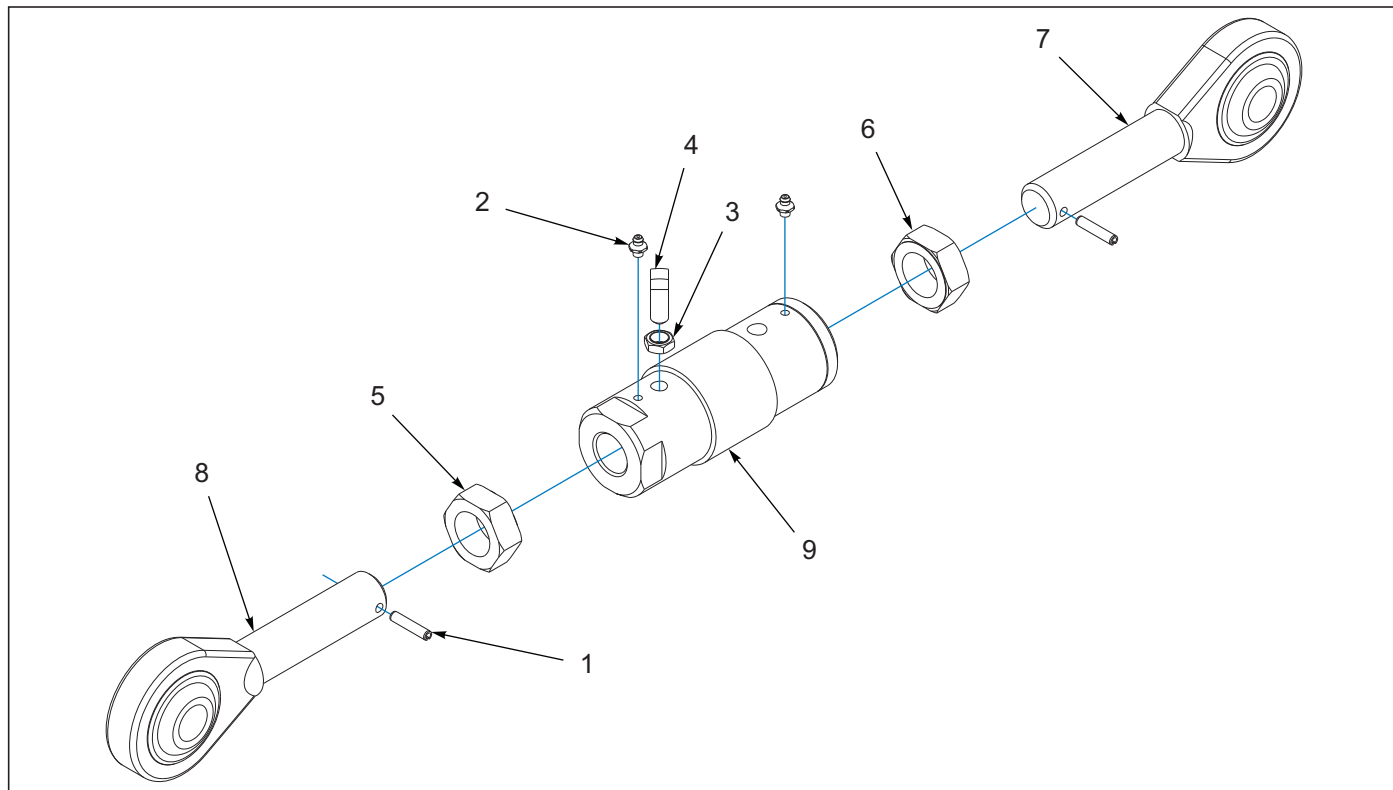
Figure 1-7: Radius Rod Lift Assembly
