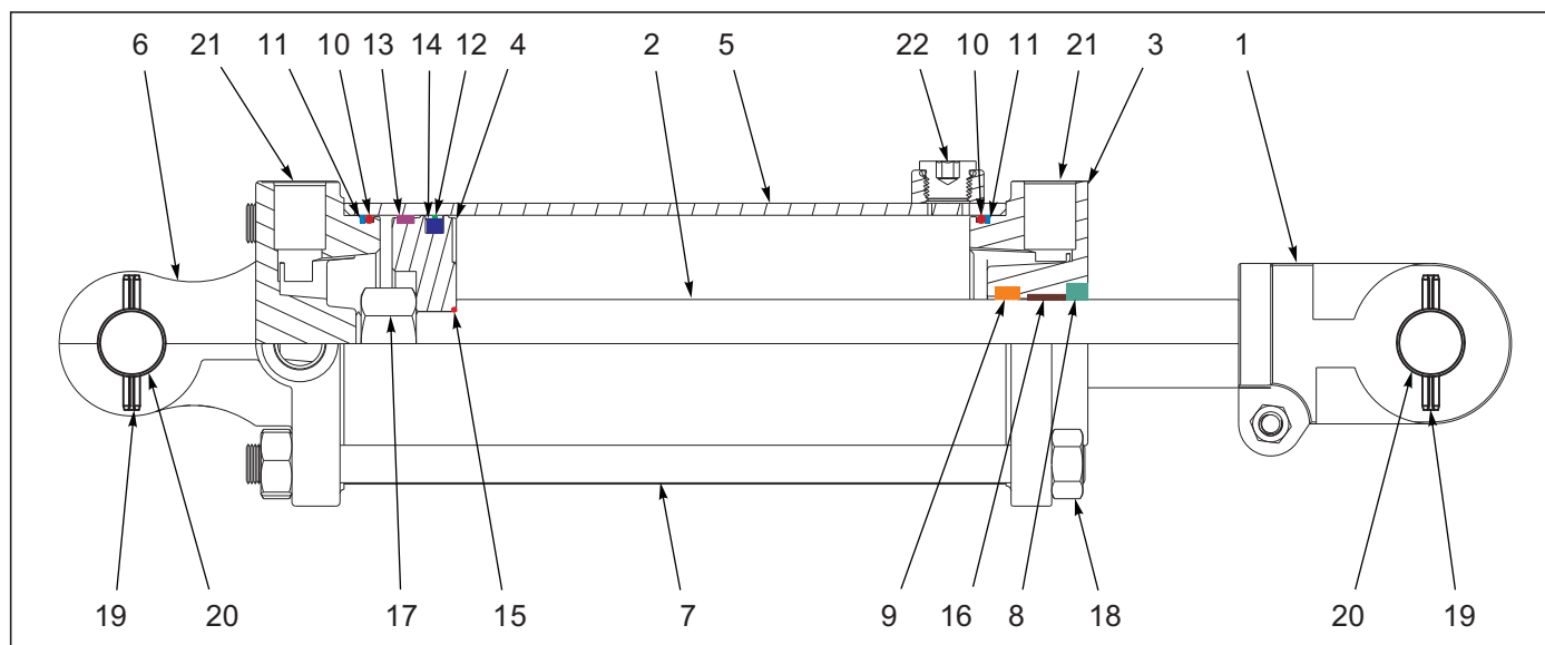
Figure 6-7: Cylinder Assembly x 30 Rephase
