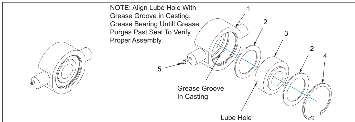
Figure 4-13: Disc Bearing Assembly
