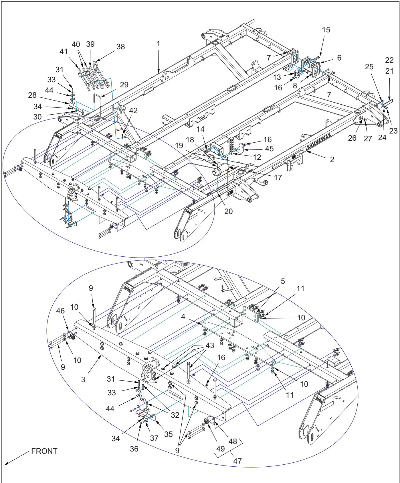
Figure 1-2: Frame Assembly 32'-35'
