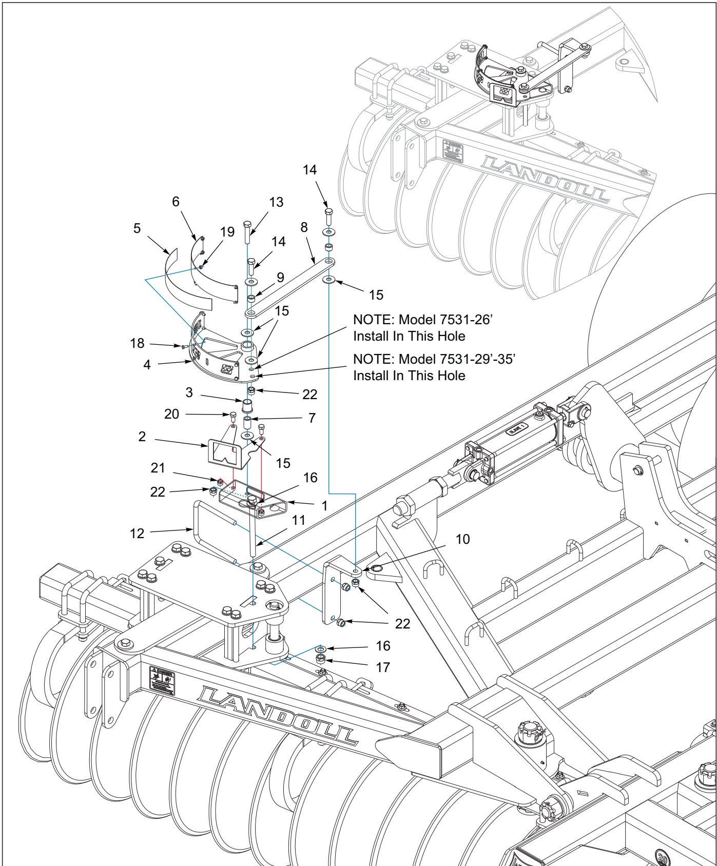
Figure 4-7: Gang Wing Gauge Assembly 7531-26'-35'
