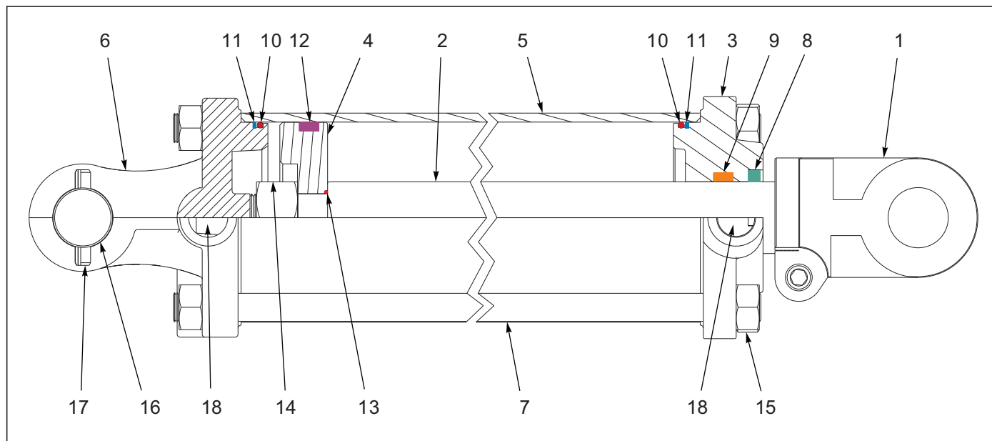
Figure 6-23: Cylinder Assembly 4 x 30 (Midway)
