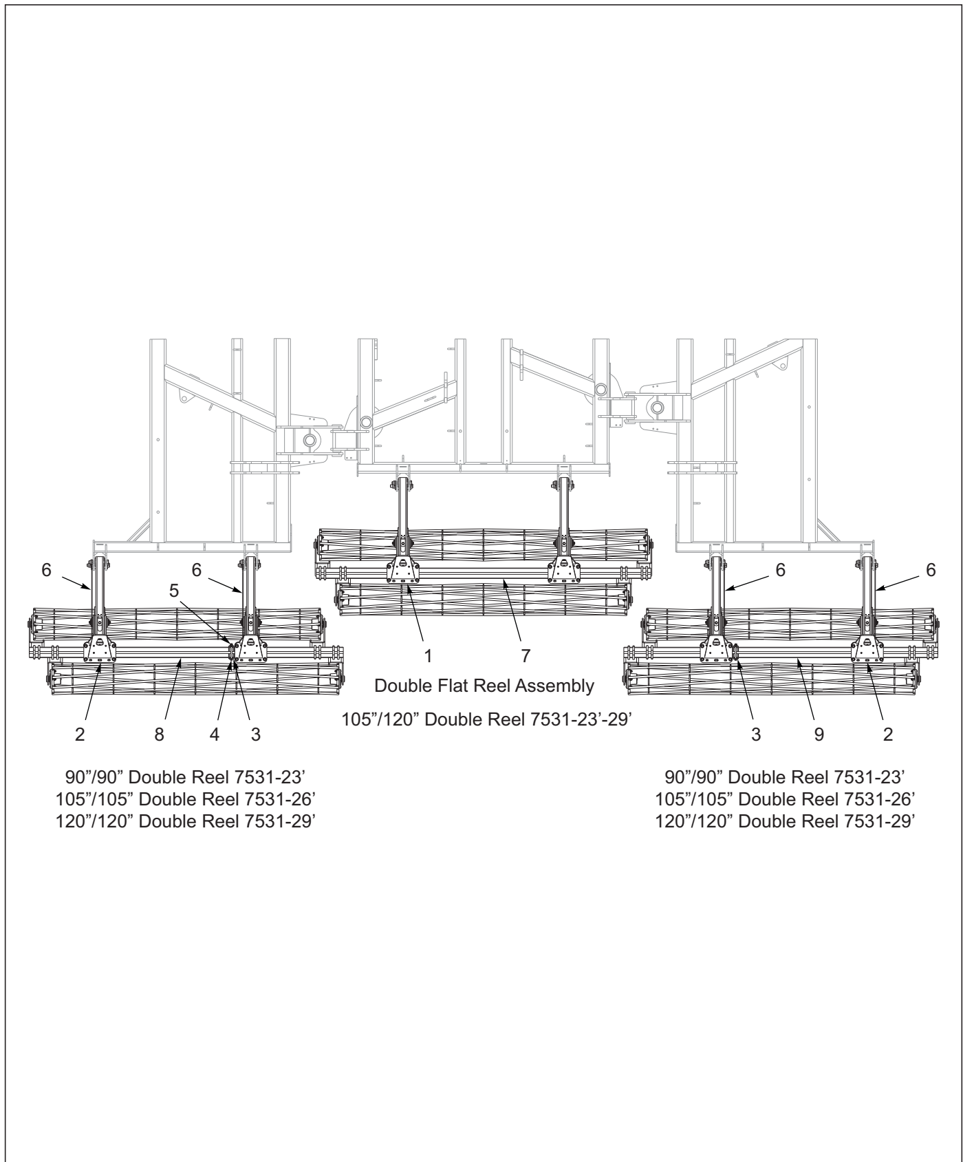
Figure 9-4: Double Flat Reel Assembly 7531-23'-29'
