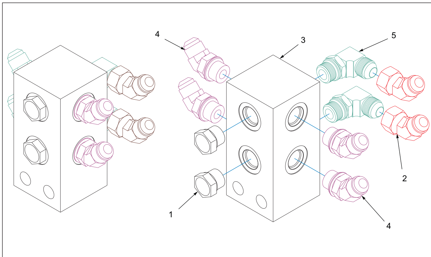
Figure 5-26: Manifold Assembly Front7531-32'-35'
