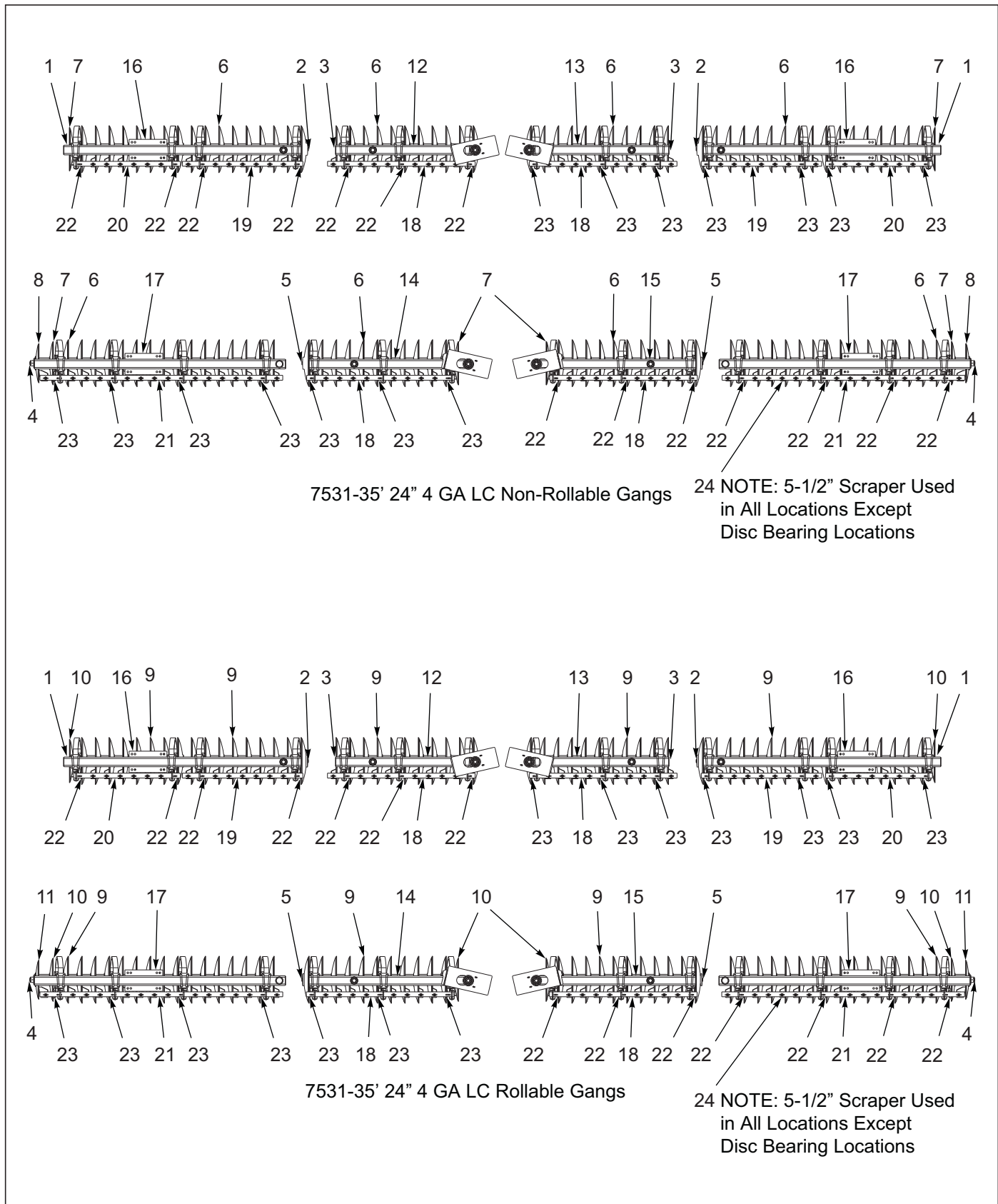
Figure 4-12: Disc Gang Assembly 7531-35'
