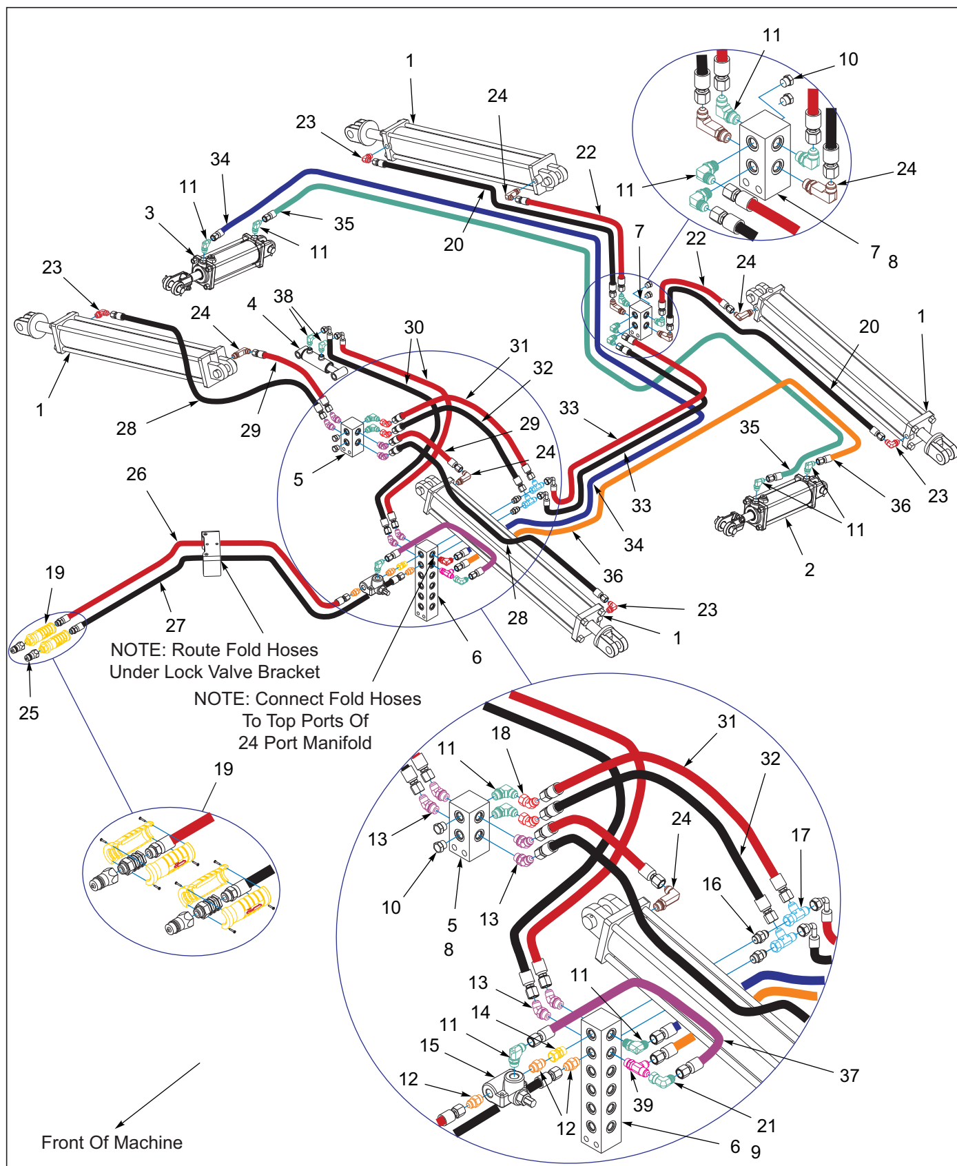
Figure 5-14: Hydraulic Assembly Fold 7531-32'-35' (After S/N 75K2501921)
