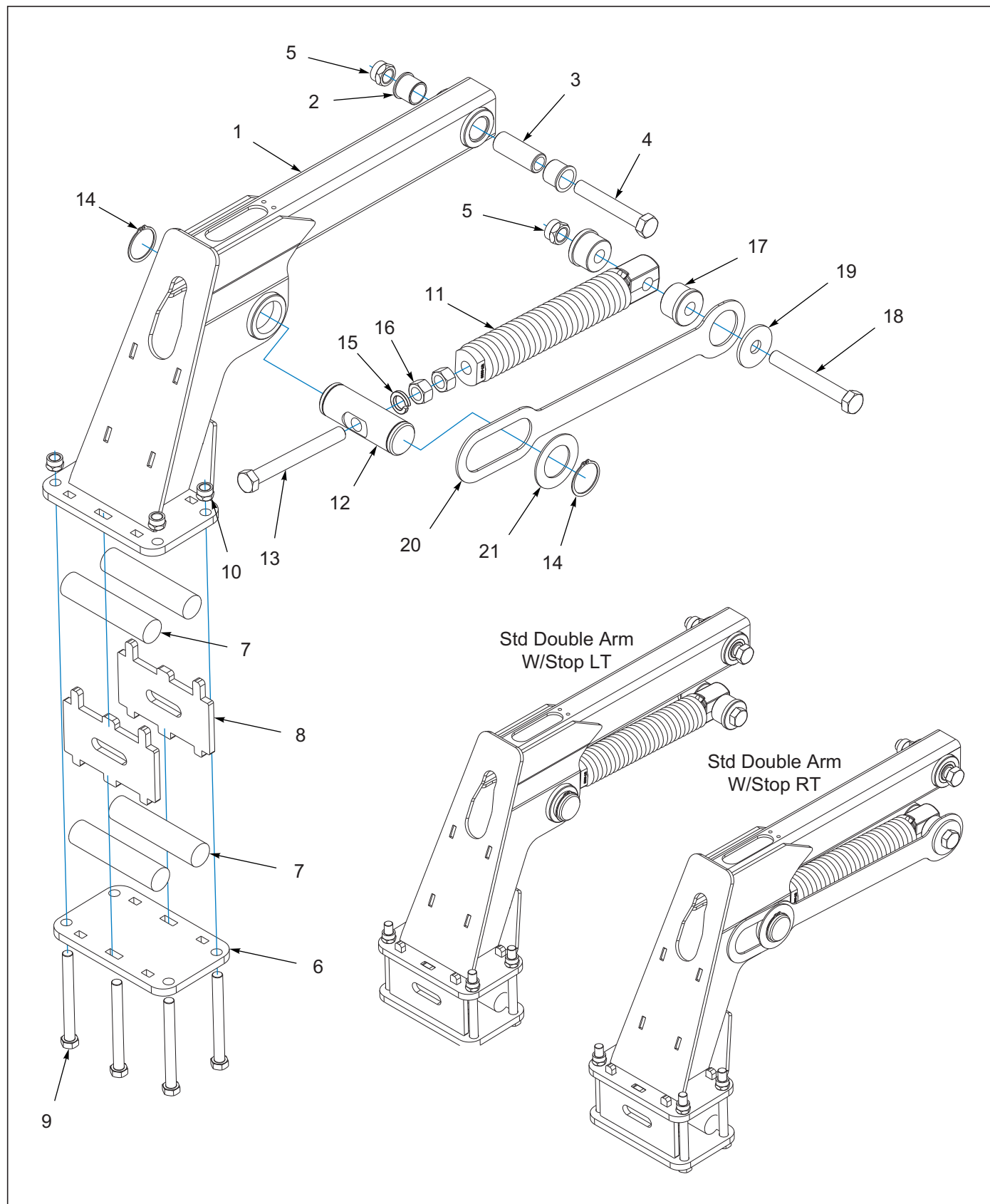
Figure 9-15: STD Double Arm W/Stop Assembly
