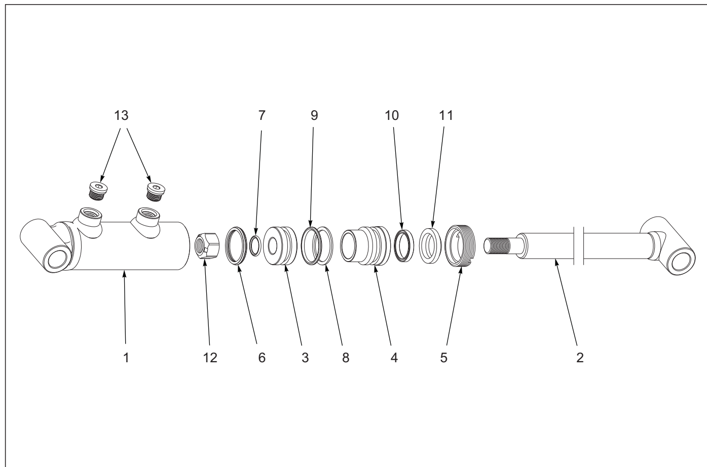
Figure 6-26: Cylinder Assembly 1-1/2 x -1-1/2
