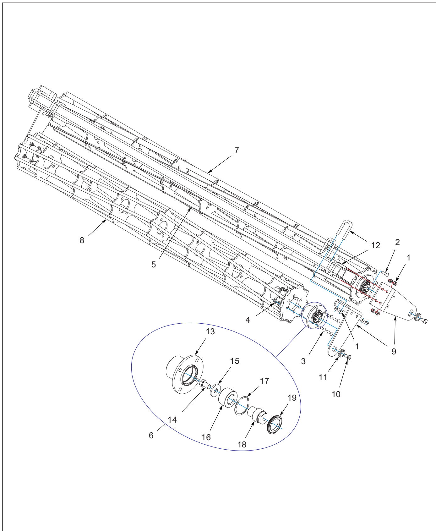
Figure 9-21: Double Flat/RD Reel Assembly 7531-23'-29' Center
