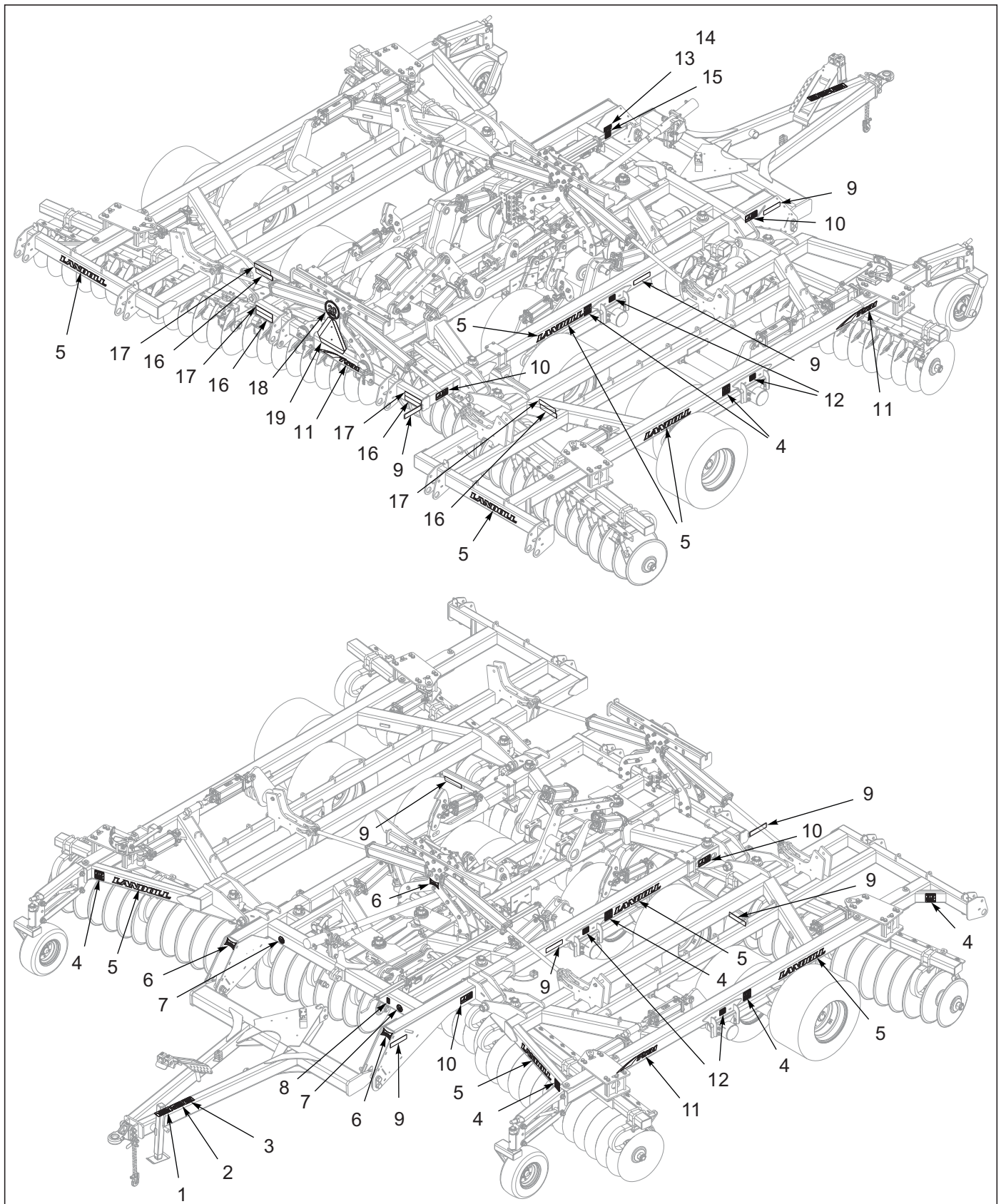
Figure 8-2: Decals (2 of 2)
