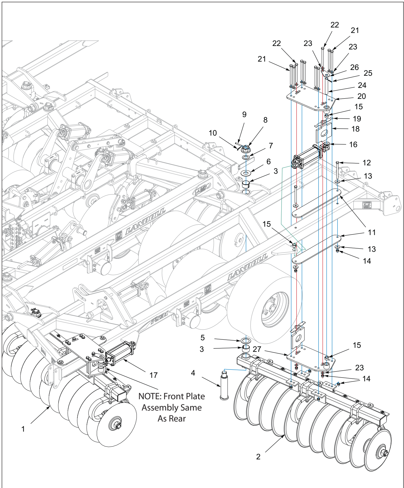
Figure 4-4: Gang Assembly Wing 23'
