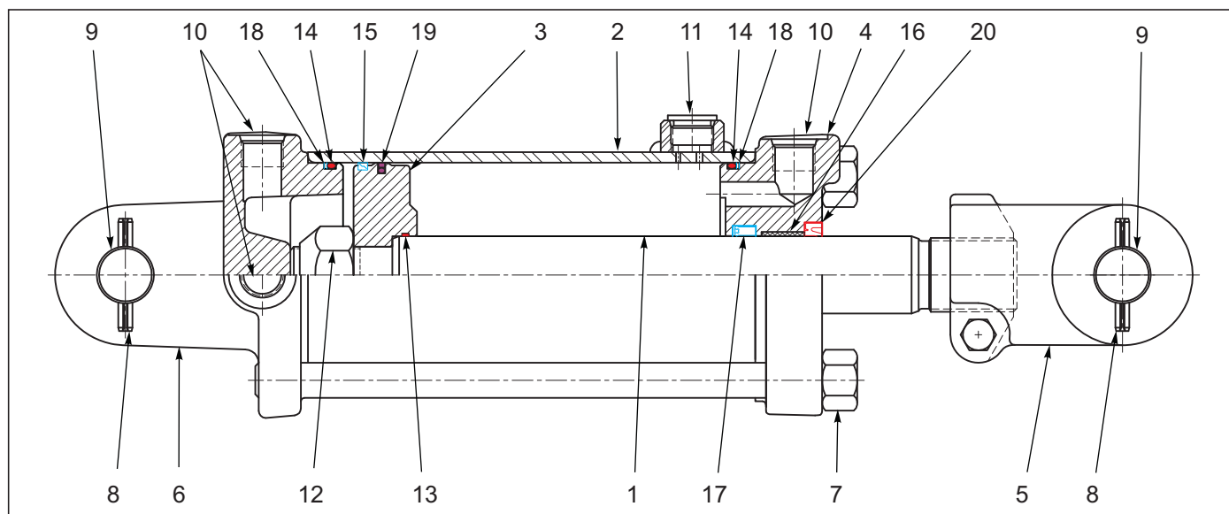
Figure 6-13: Cylinder Assembly 3-3/4 x 10 Rephase (Prince)
