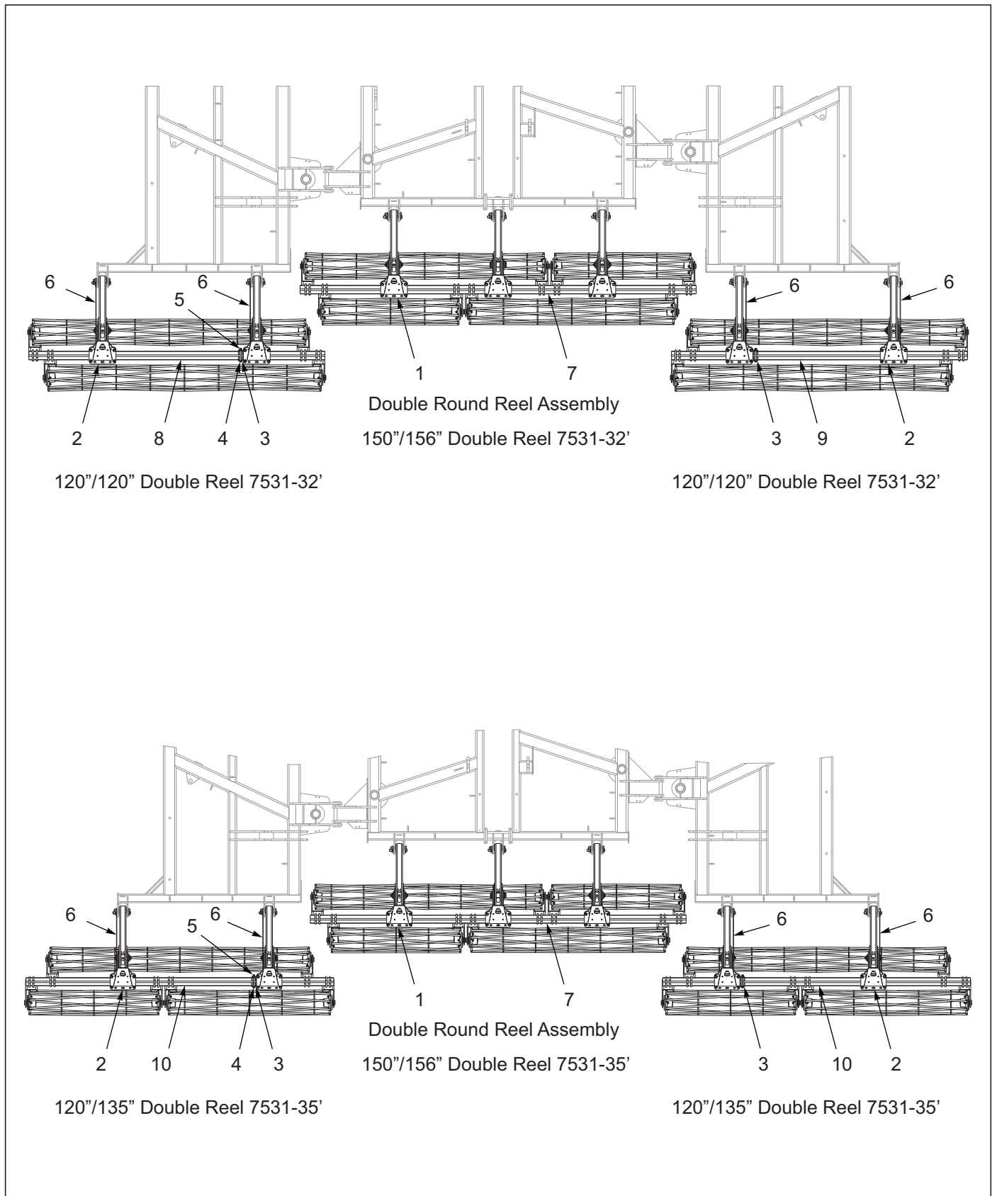
Figure 9-5: Double Round Reel Assembly 7531-32'-35'
