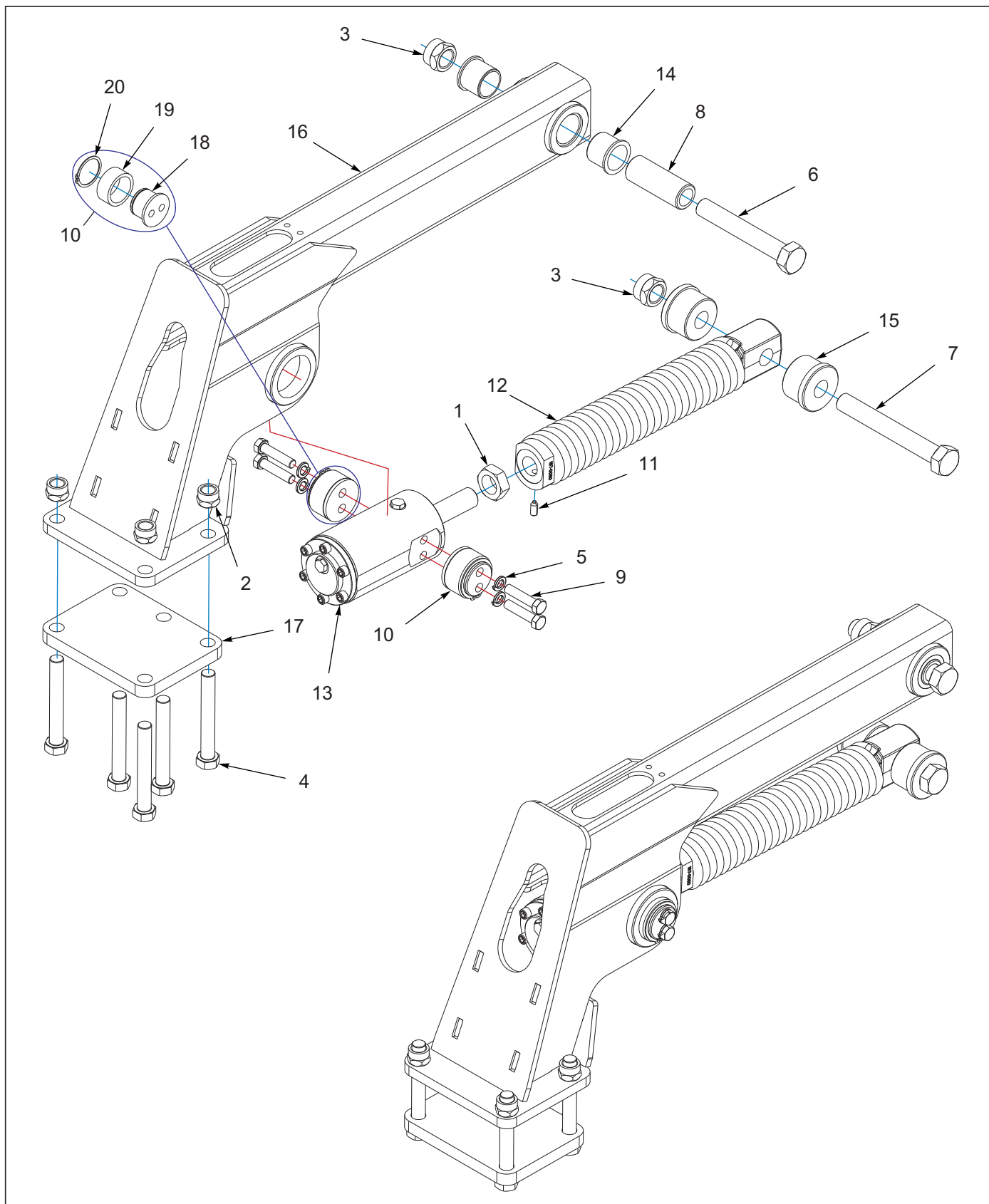
Figure 9-12: Hydraulic Single Arm Assembly
