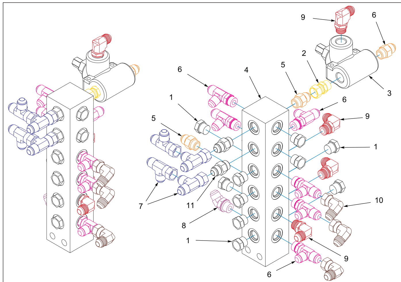
Figure 5-21: Manifold Assembly Front 7531-26'/29' After
