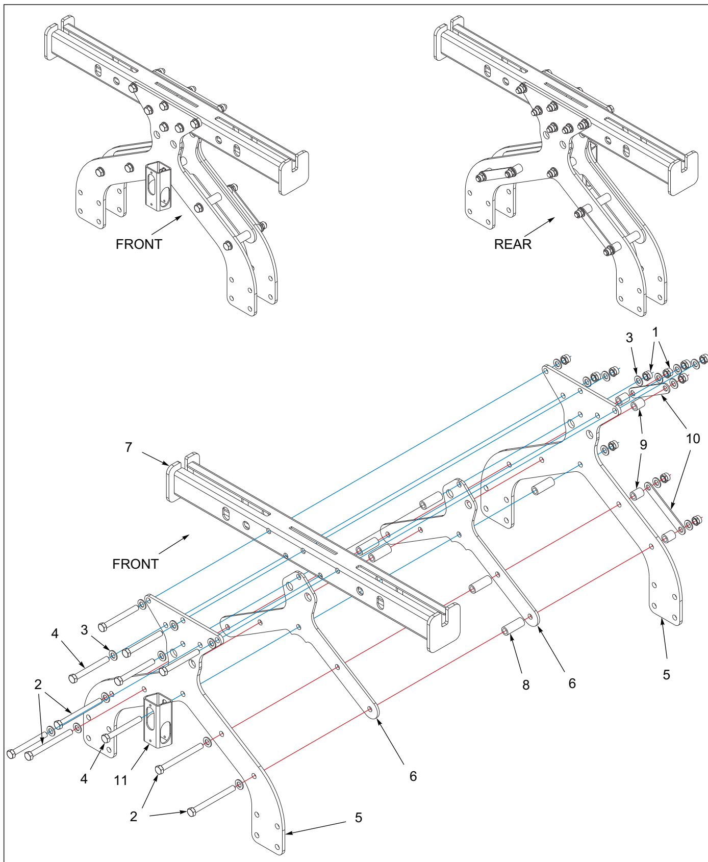
Figure 5-7: Wing Fold Stabilizer Assembly 7531-26'-29' Rear
