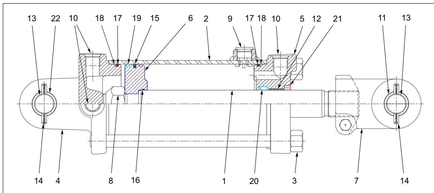
Figure 6-15: Cylinder Assembly 3-1/2 x 8, Rephase (Prince)
