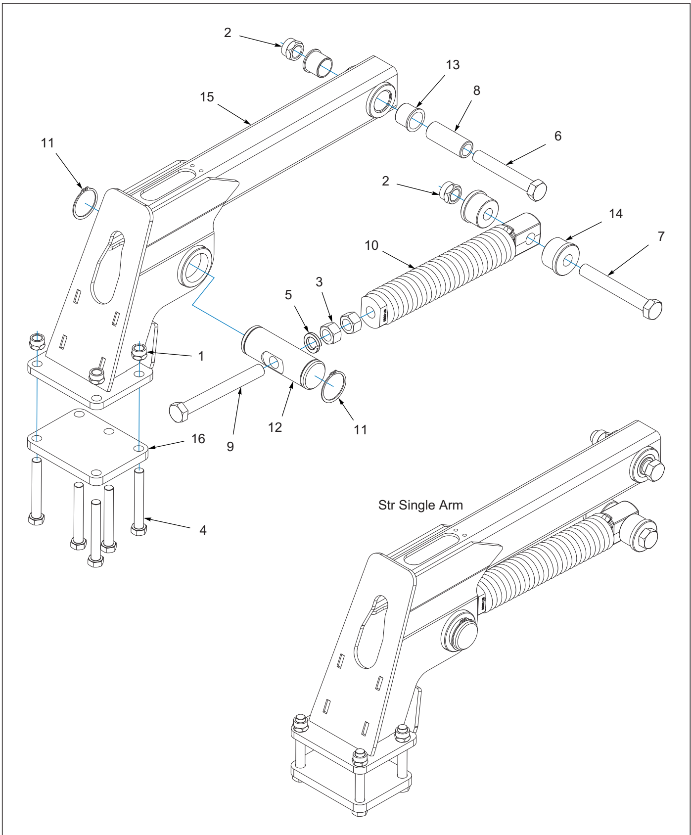
Figure 9-9: Std Single Arm Assembly
