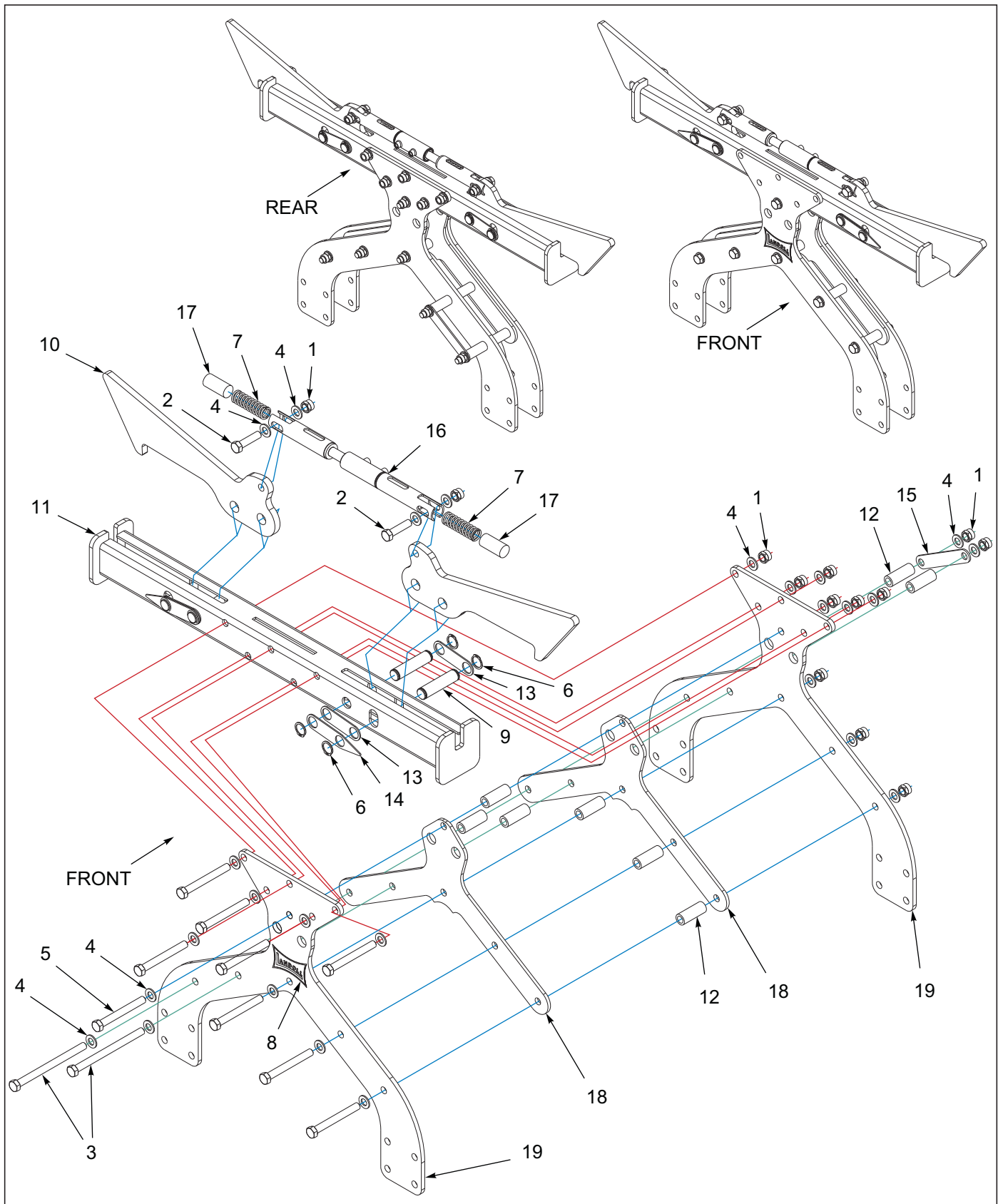
Figure 5-6: Wing Fold Stabilizer Assembly 7531-26'-29' Front
