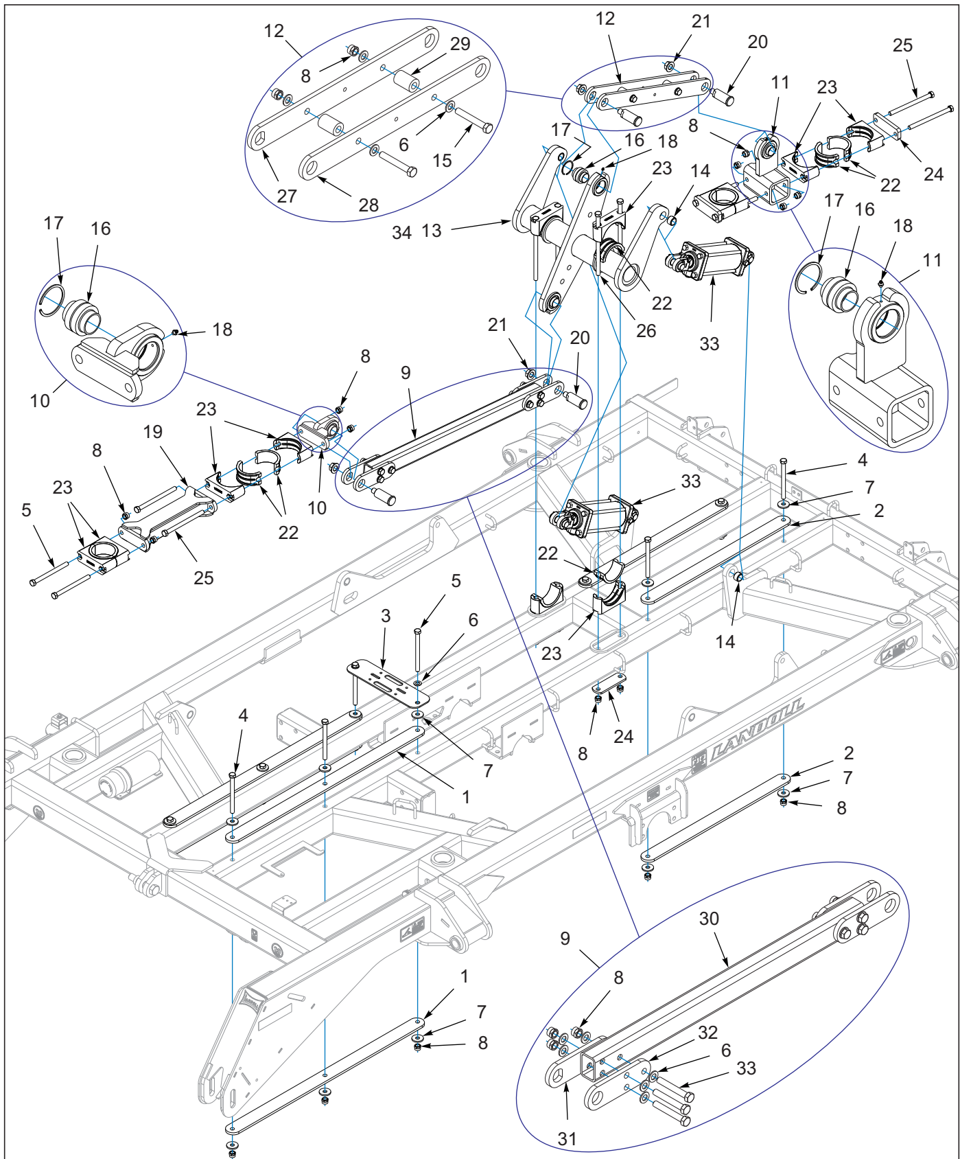
Figure 4-2: Gang Adjust Assembly Center
