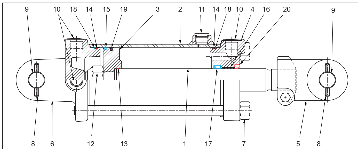
Figure 6-11: Cylinder Assembly 3-1/2 x 8 Rephase (Prince)
