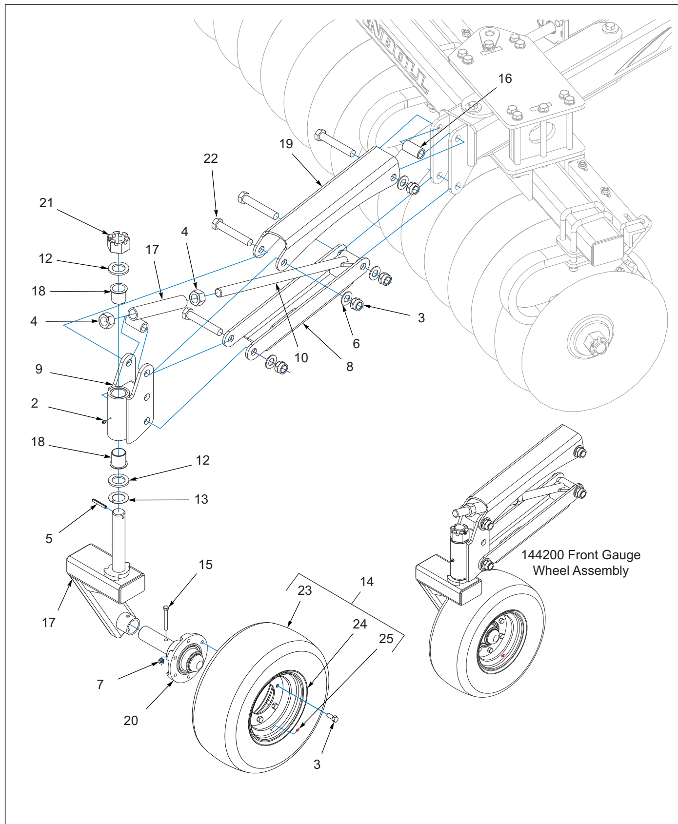
Figure 3-3: Gauge Wheel Assembly
