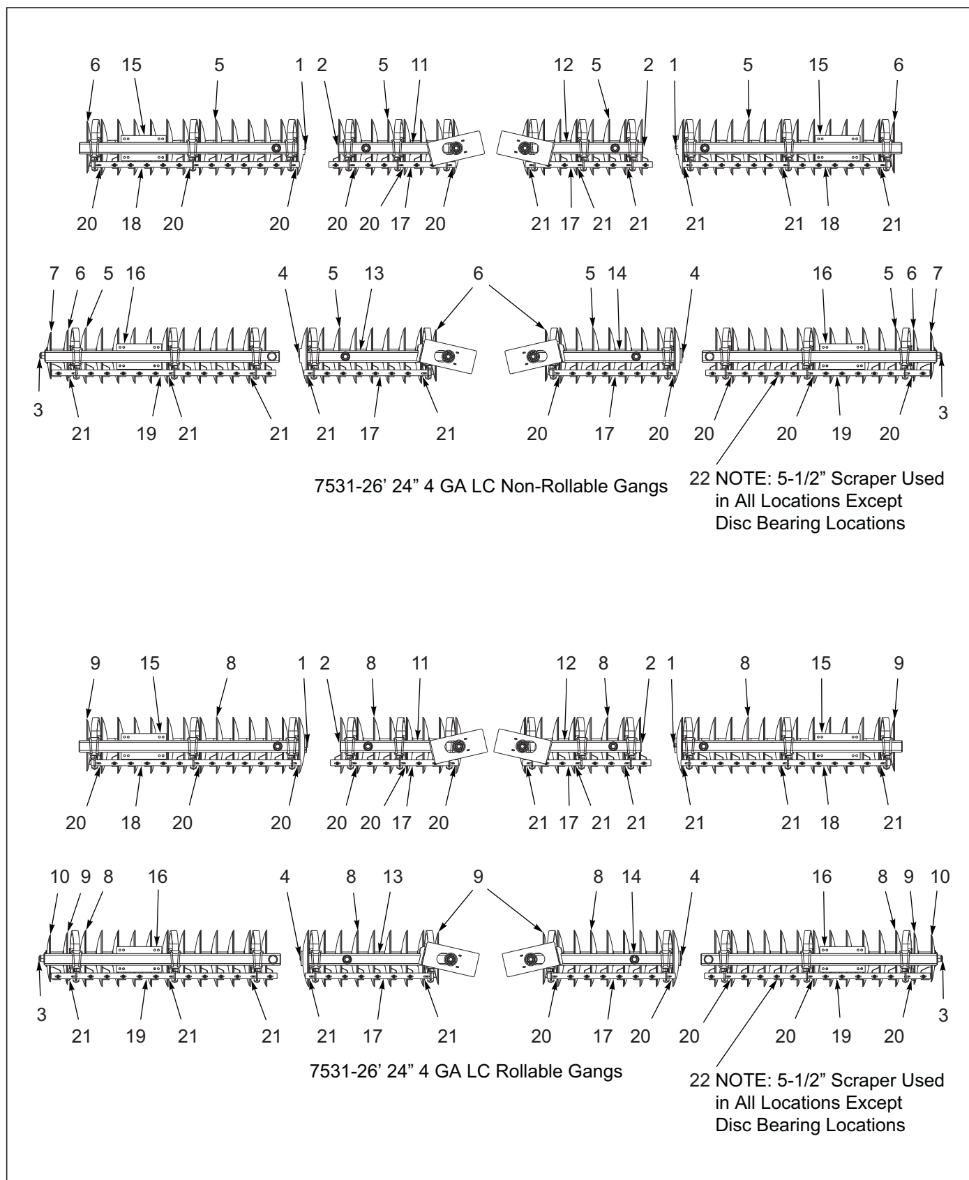
Figure 4-9: Disc Gang Assembly 7531-26'
