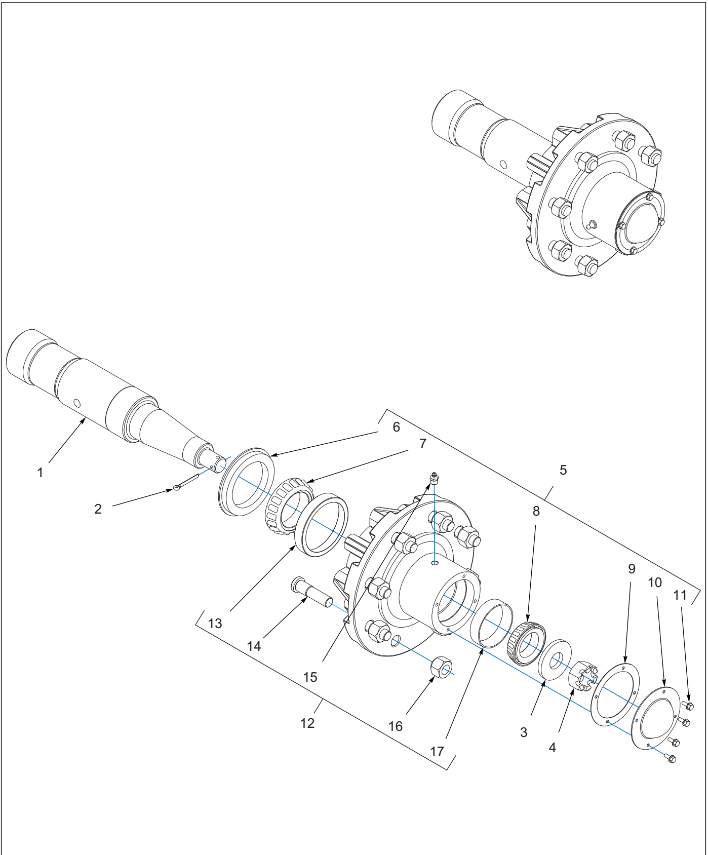
Figure 1-10: Hub/Spindle Assembly, Center
