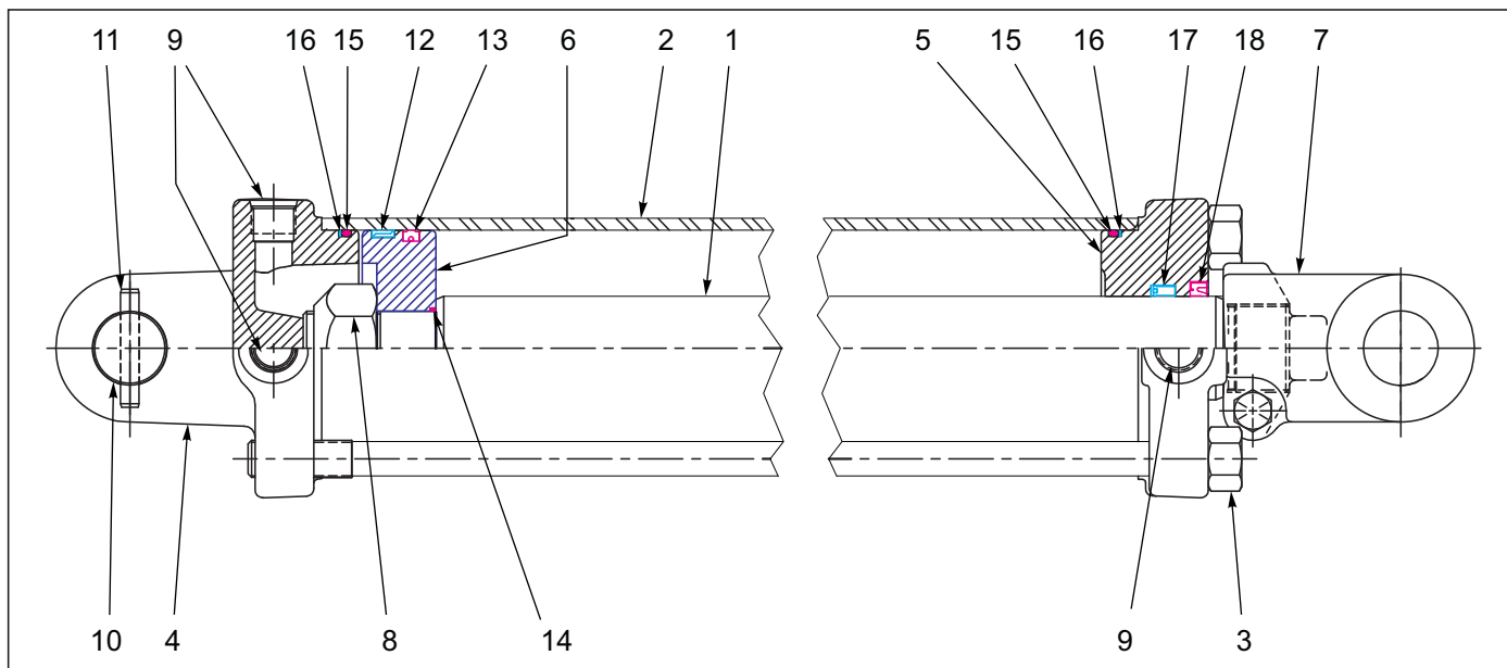
Figure 6-21: Cylinder Assembly 4-1/2 x 30
