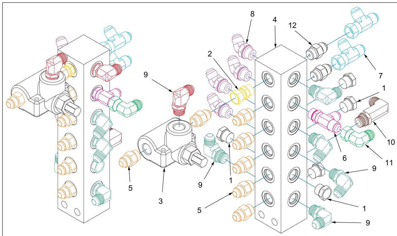
Figure 5-25: Manifold Assembly Front 7531-32'-35' After
