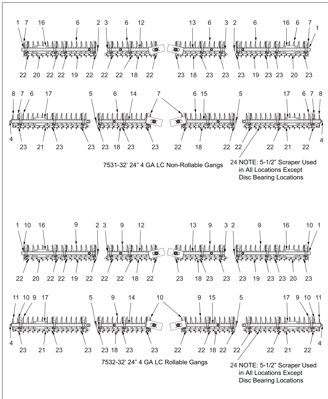
Figure 4-11: Disc Gang Assembly 7531-32'
