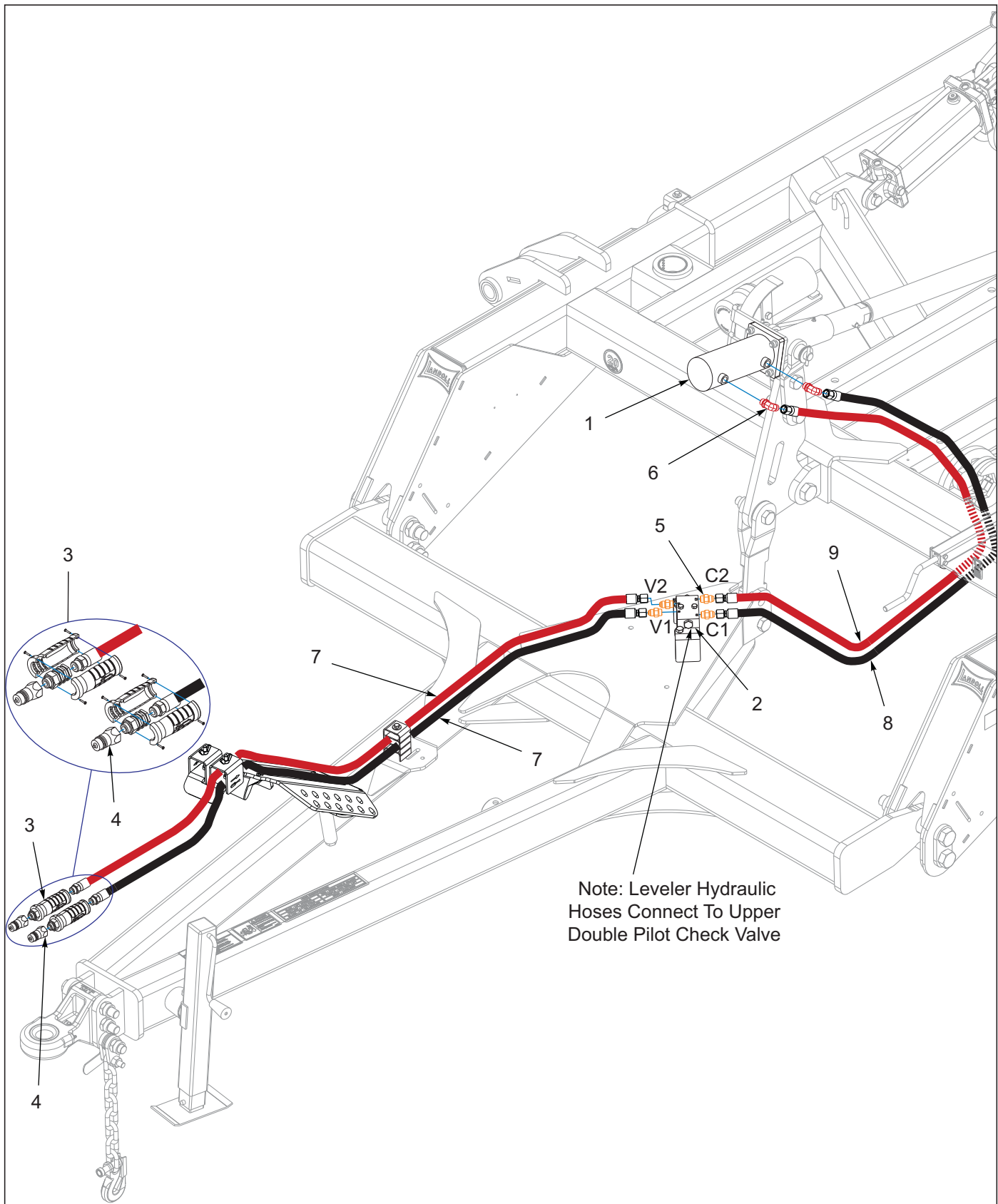
Figure 5-18: Hydraulic Assembly Leveler
