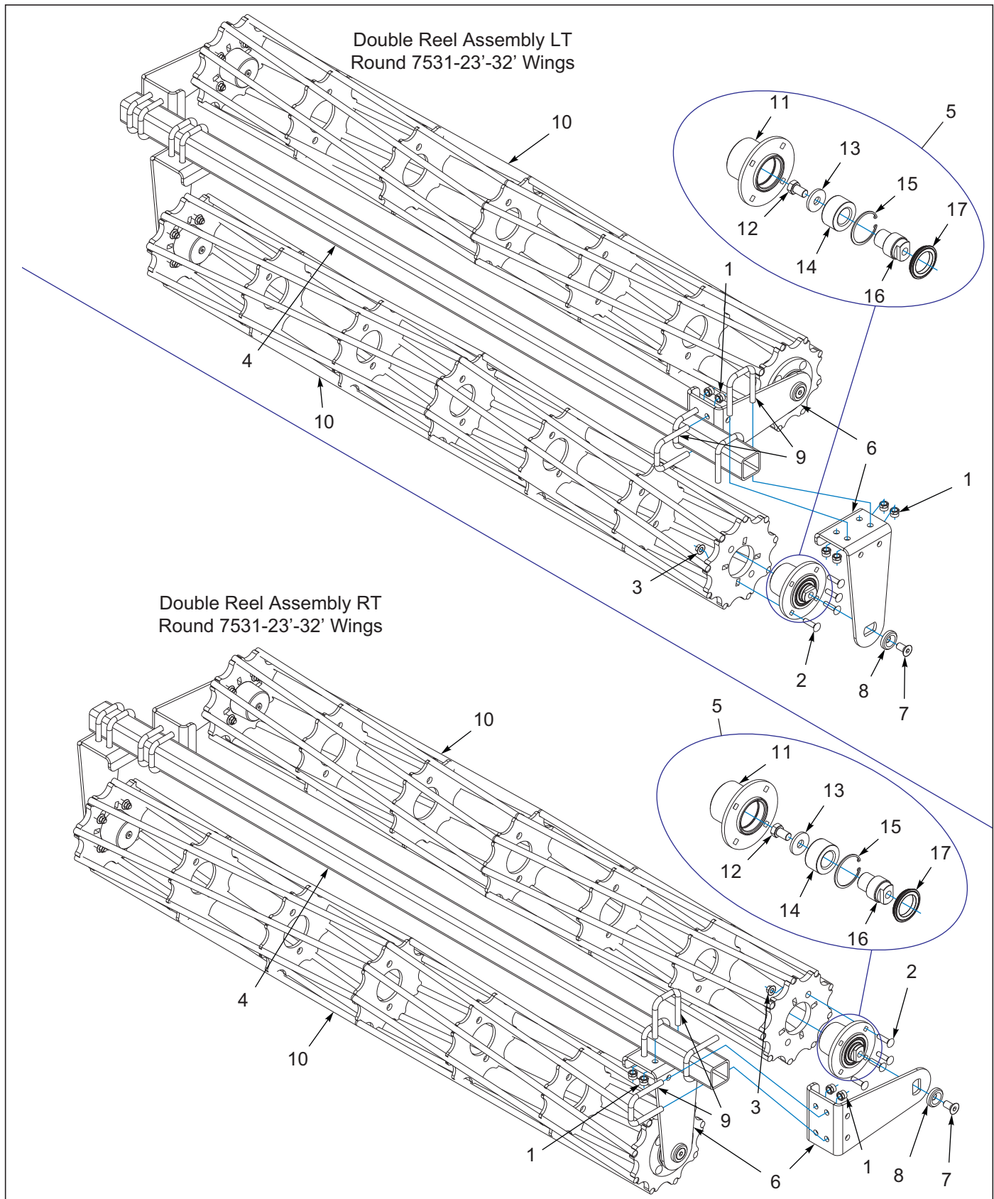
Figure 9-23: Double Round Reel Assembly 7531-23'-32' Wings
