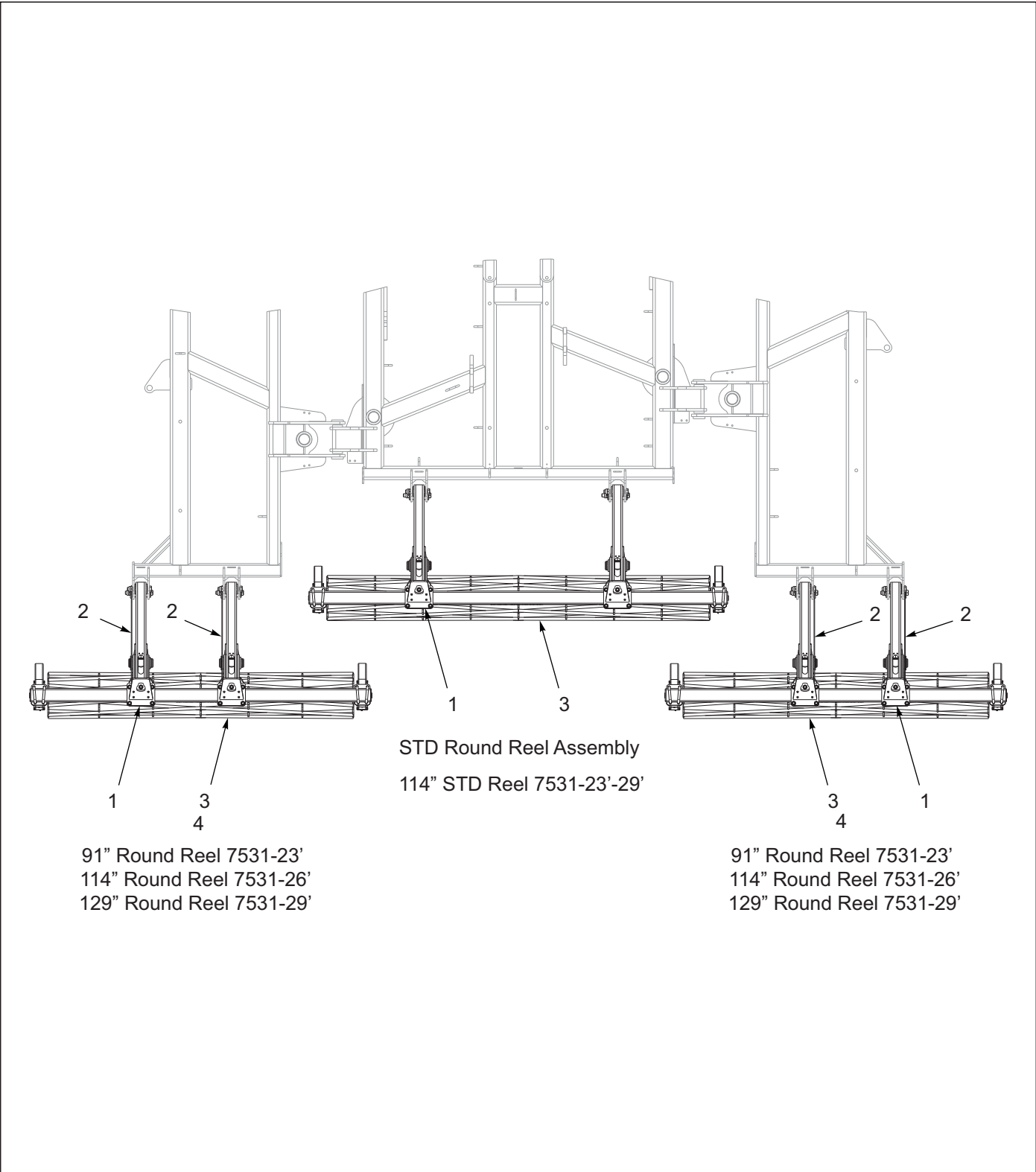
Figure 9-1: STD Round Reel Assembly 7531-23'-29'
