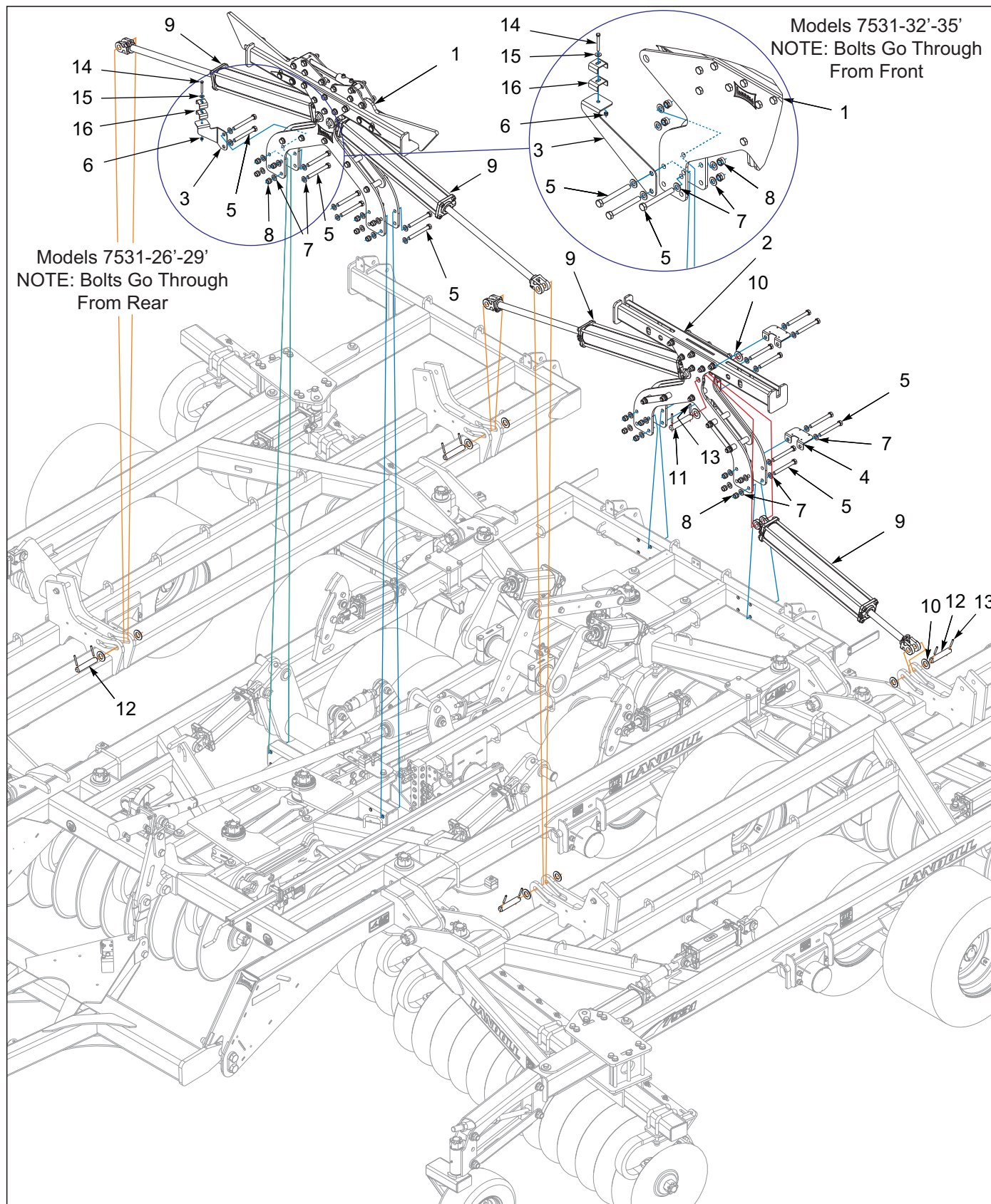
Figure 5-5: Fold Stabilizer Assembly 7531-26'-35'
