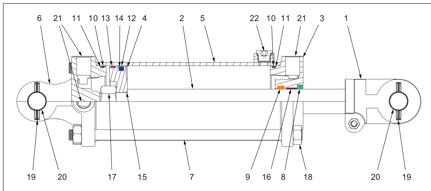
Figure 6-18: Cylinder Assembly 3-1/4 x 8, Rephase (Midway)
