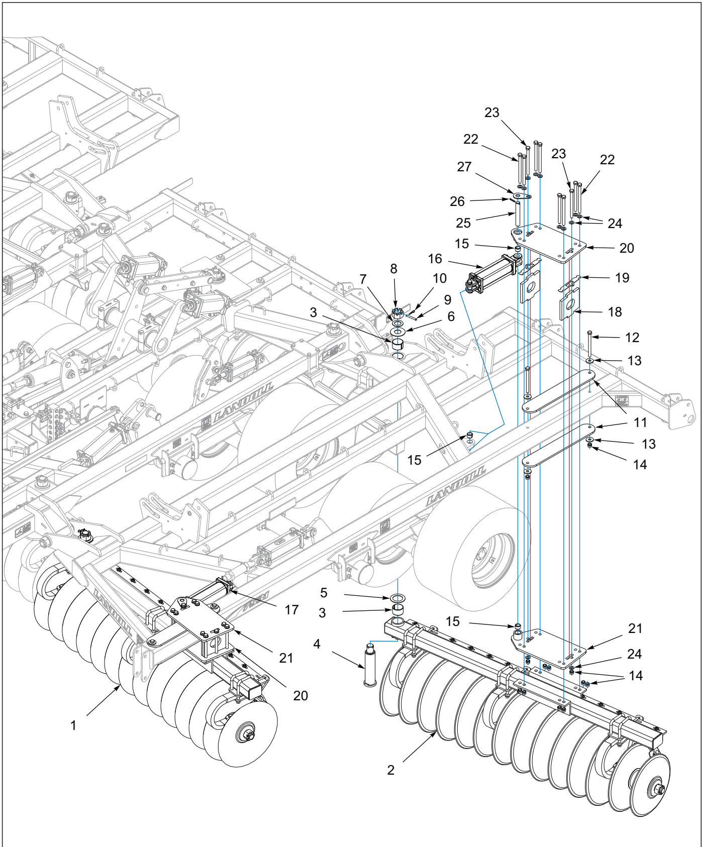
Figure 4-5: Gang Assembly Wing 7531-26'-35'
