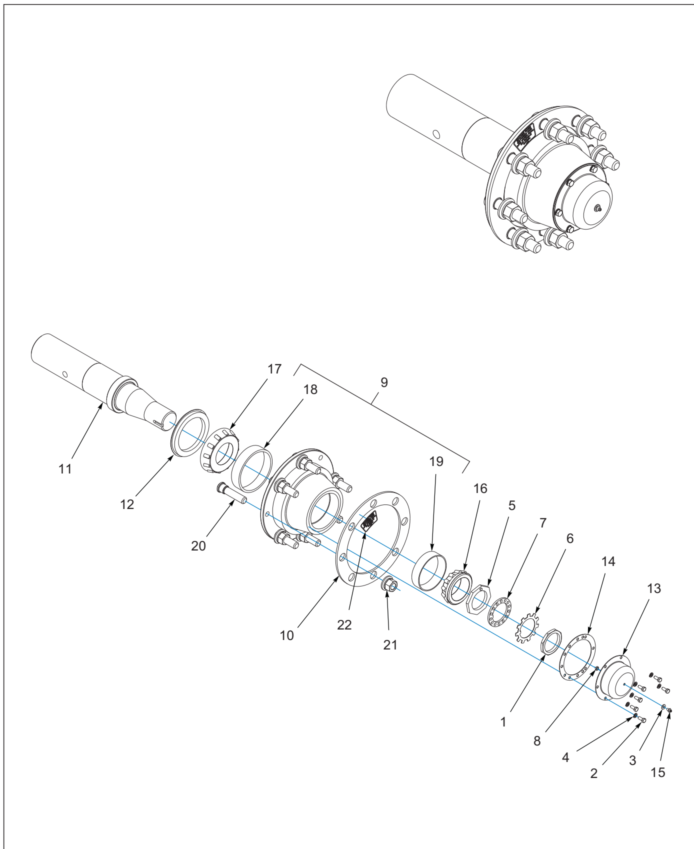
Figure 1-11: Hub/Spindle Assembly Center (Dual Wheels)
