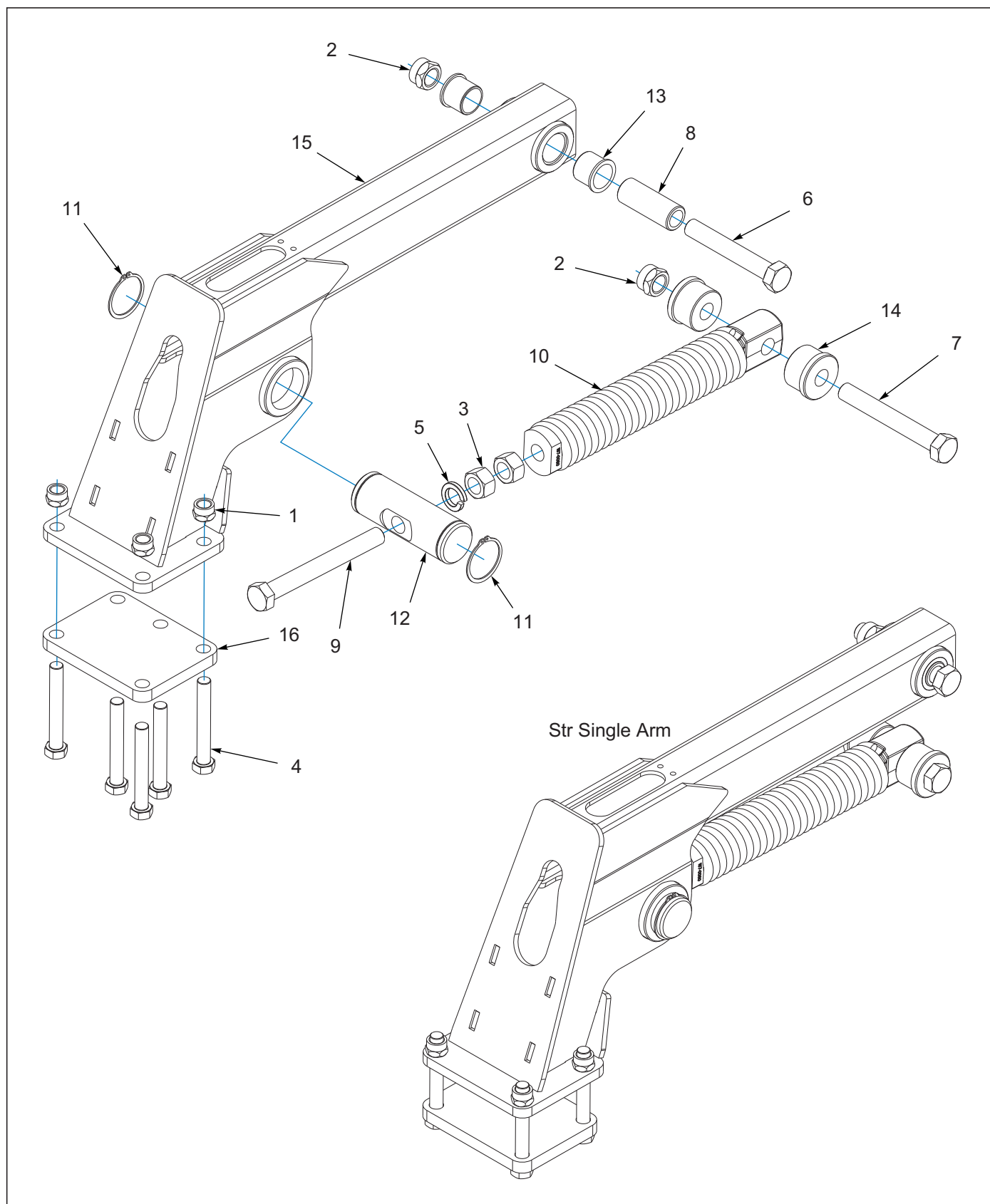
Figure 9-10: Std Single Arm Assembly
