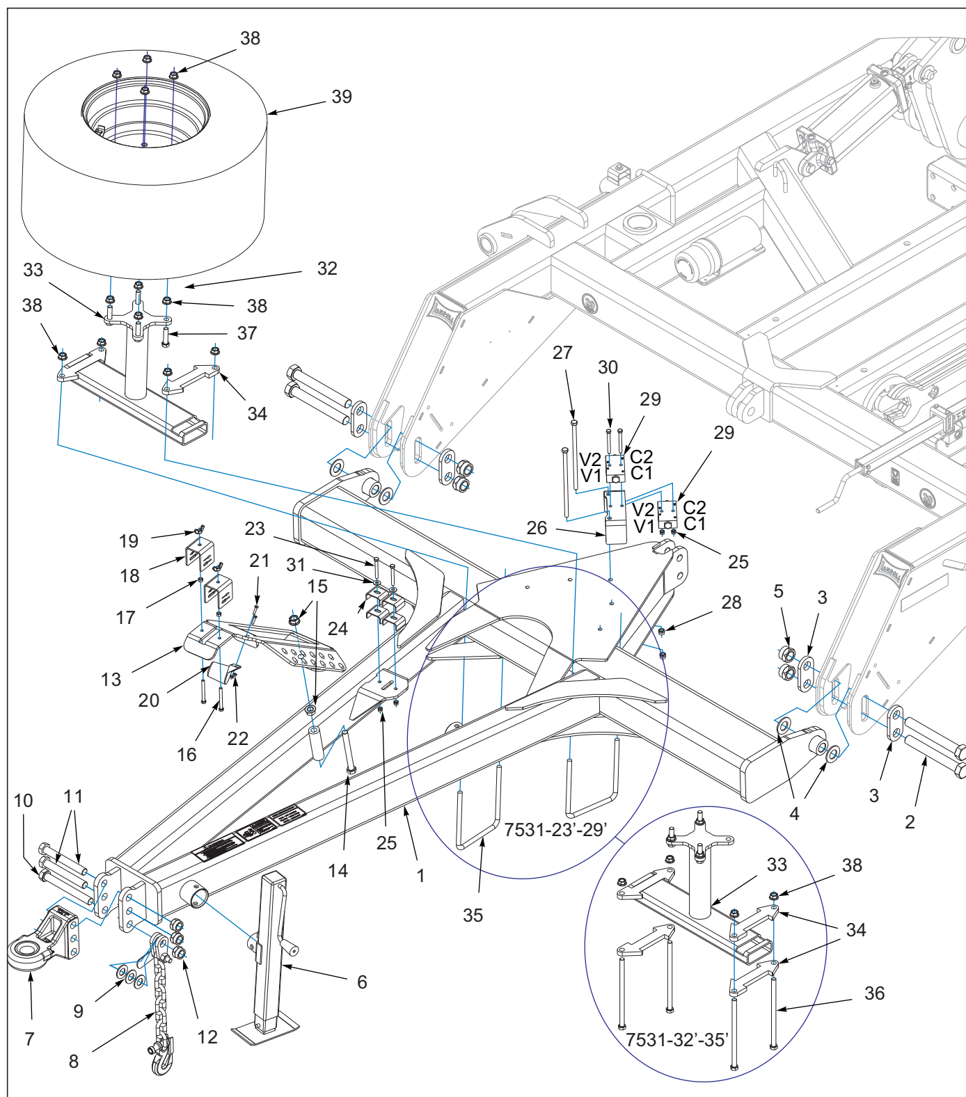
Figure 2-1: Hitch Assembly
