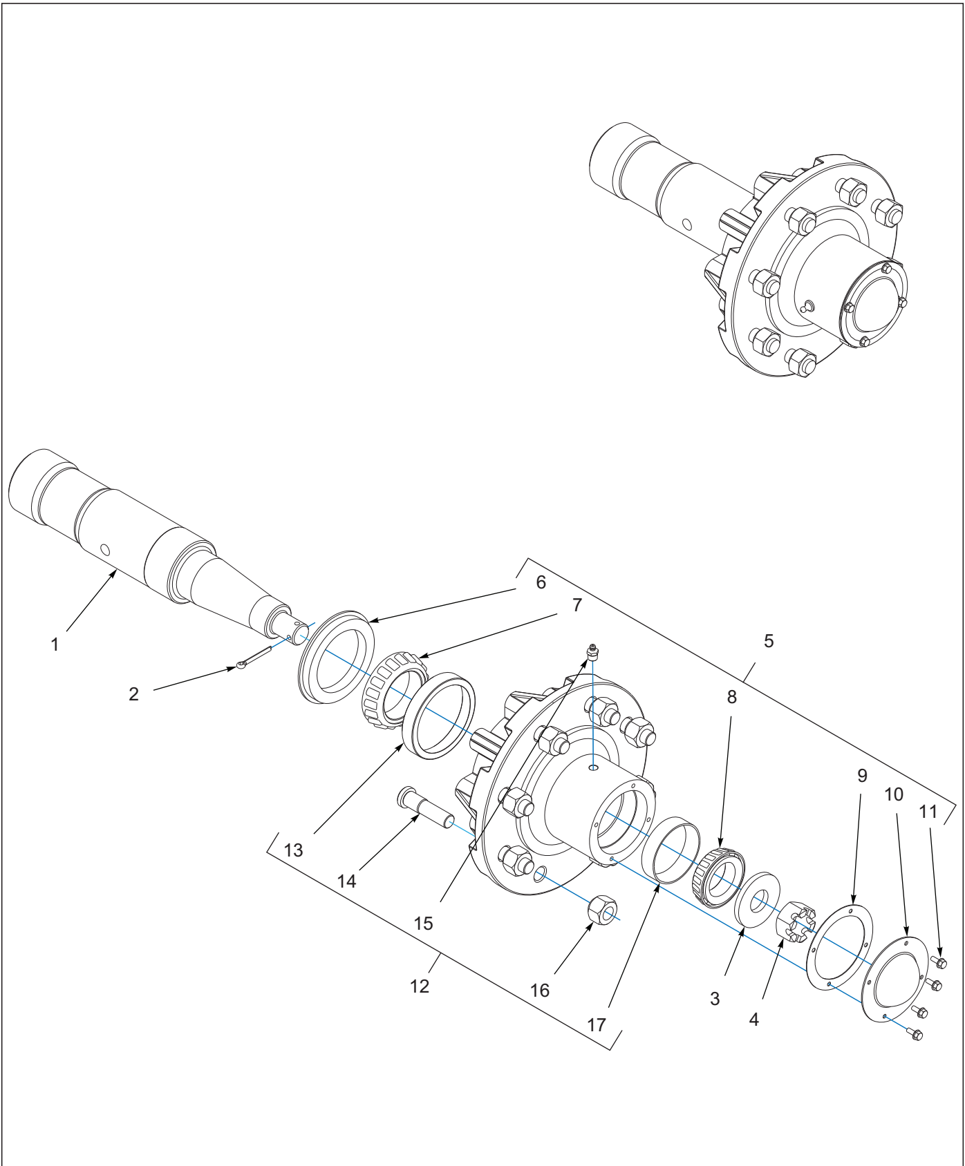
Figure 3-2: Hub/Spindle Assembly, Wings
