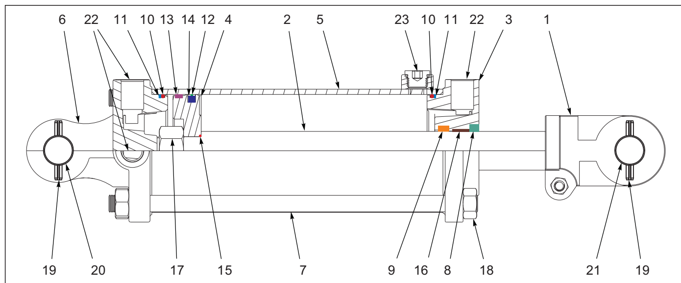
Figure 6-4: Cylinder Assembly 4-1/2 x 10 Rephase (Midway)
