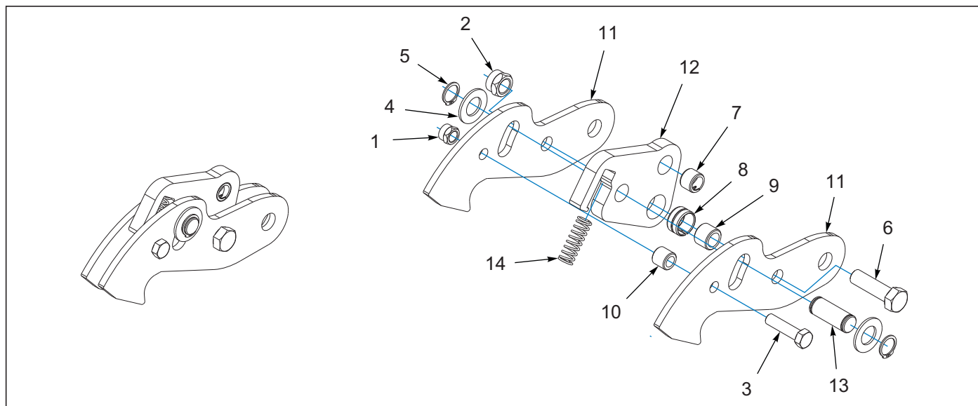
Figure 1-9: Lift Lock Assembly
