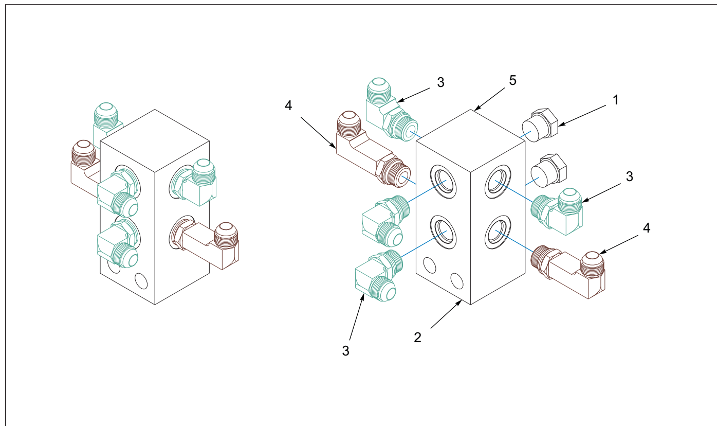
Figure 5-28: Manifold Assembly Rear 7531-32'-35' After
