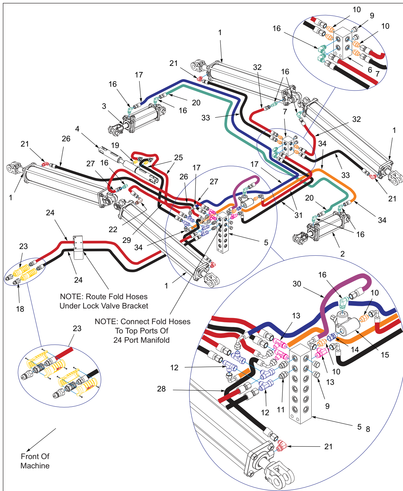
Figure 5-12: Hydraulic Assembly Fold 7531-26'-29' (After S/N 75K2501921)
