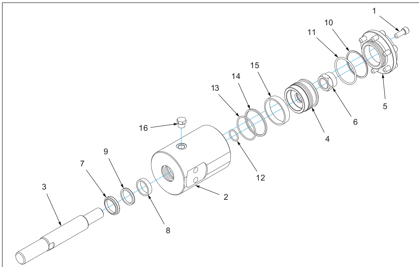
Figure 6-25: Cylinder Assembly 2-1/2 x 2-1/2
