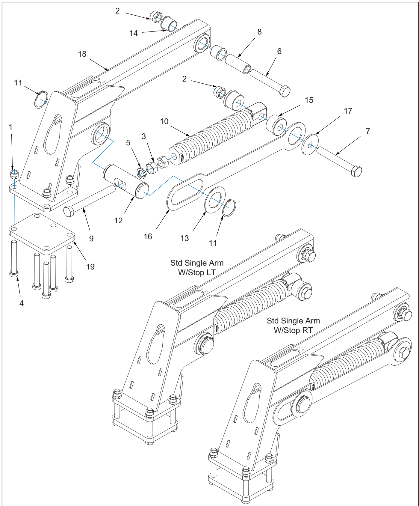
Figure 9-11: STD Single Arm W/Stop Assembly
