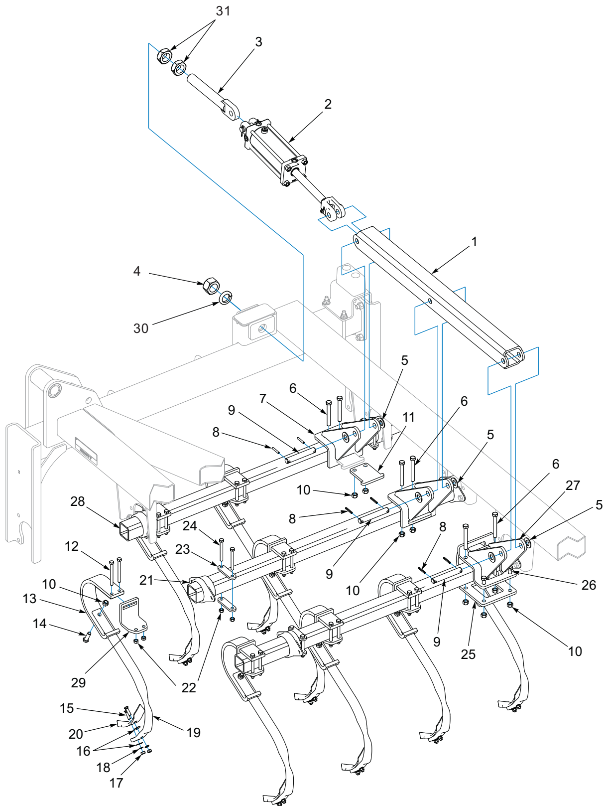
Figure 1-24: Tooth Control - Right Hand Wing
