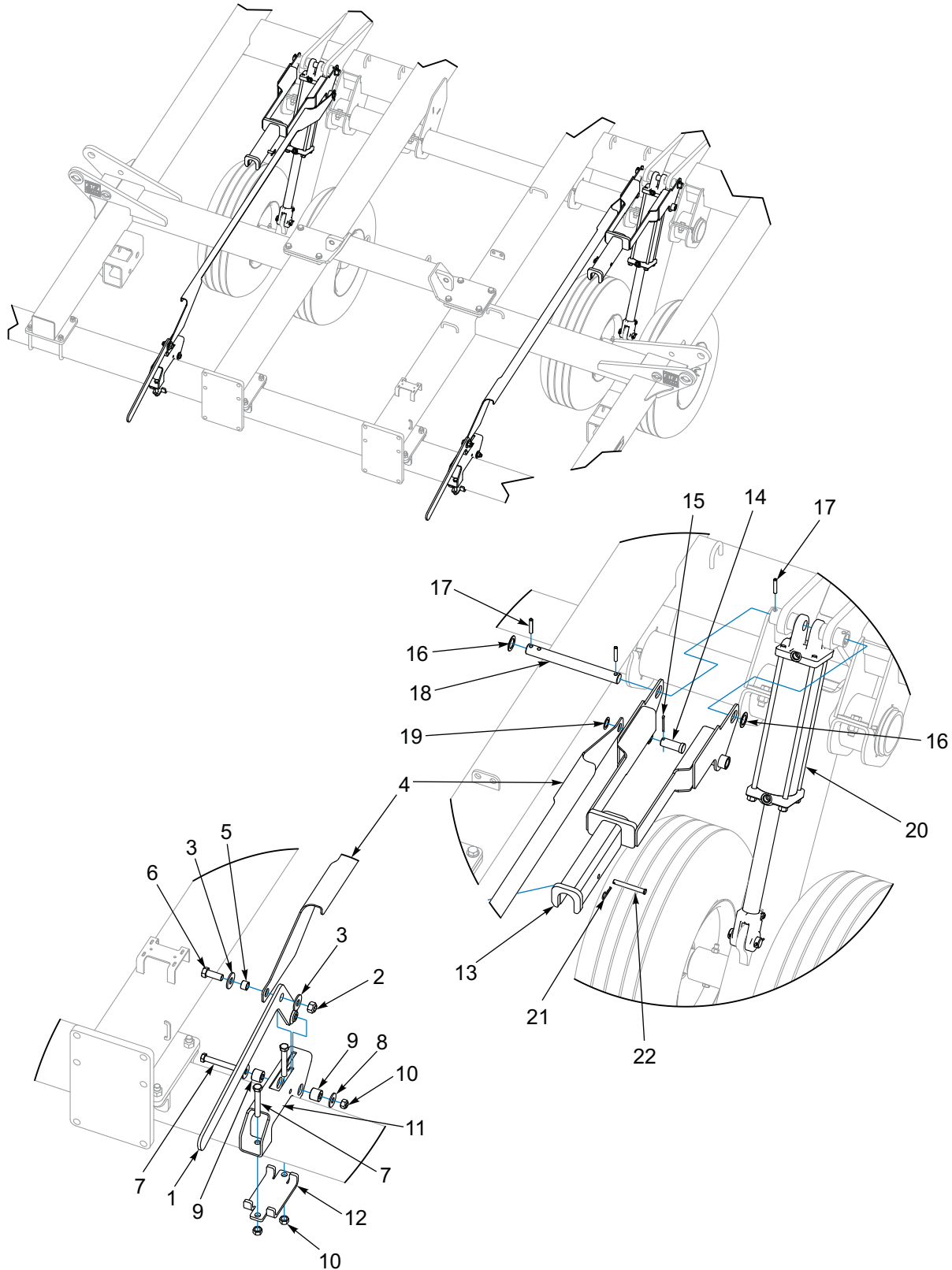
Figure 1-9: Rockshaft Cylinder Transport Lock
