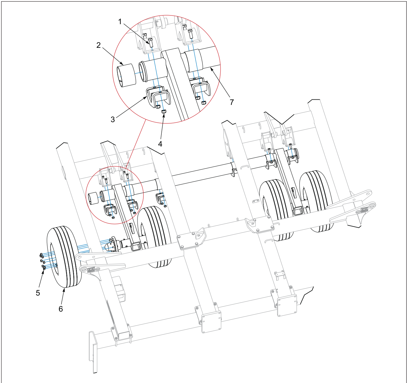
Figure 1-3: Transport Axle Mounting Components
