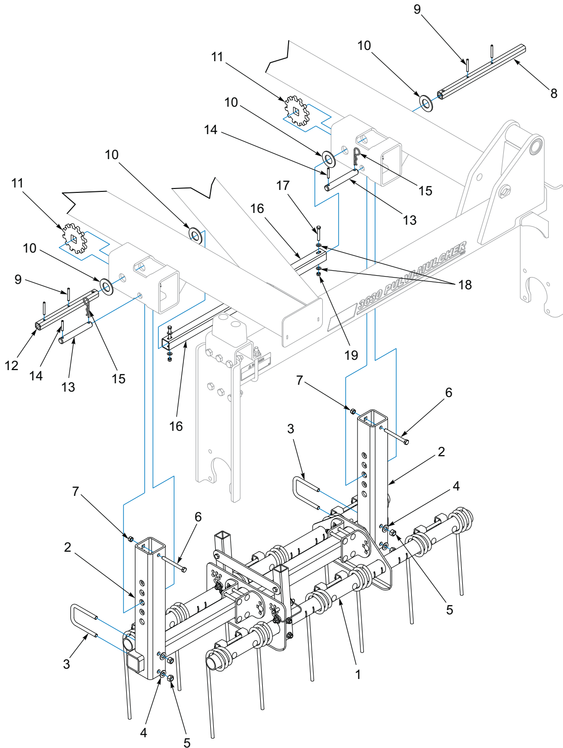
Figure 1-29: Left Hand Wing Harrow
