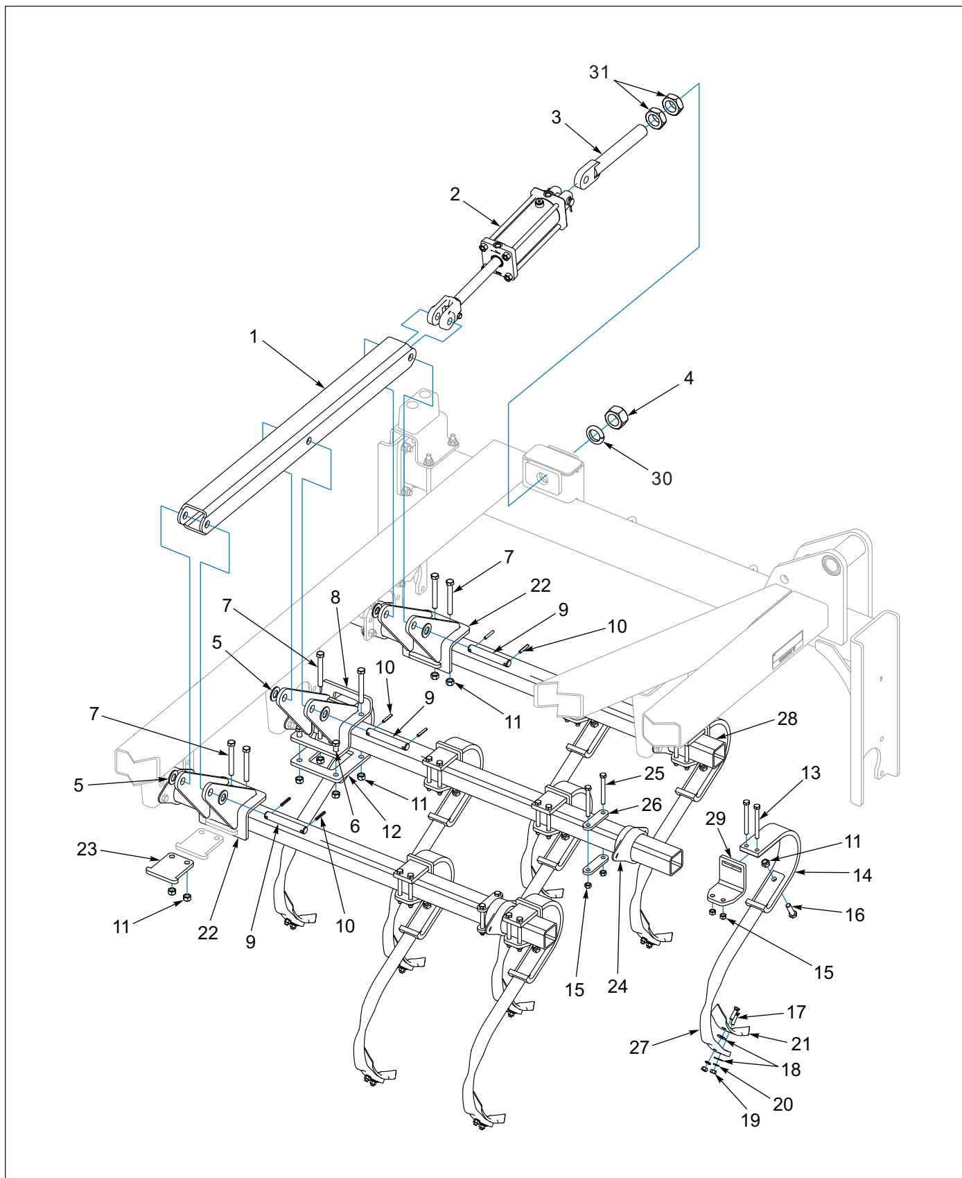
Figure 1-25: Tooth Control - Left Hand Wing
