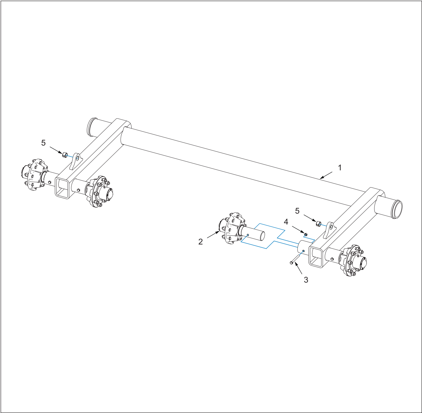
Figure 1-4: Transport Axle
