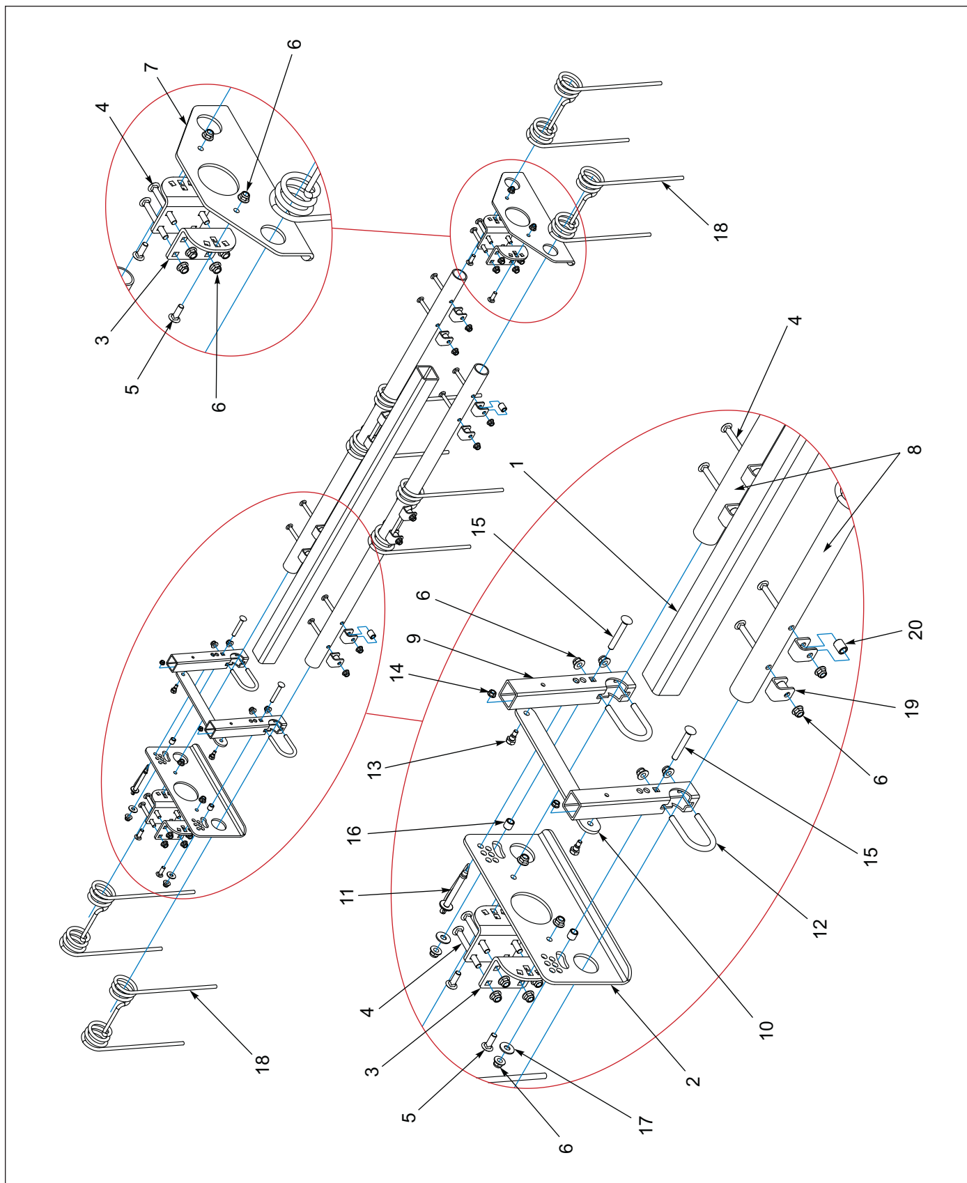
Figure 1-31: Right Hand Wing Harrow Assembly
