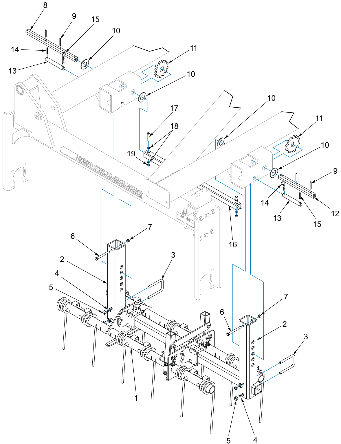
Figure 1-28: Right Hand Wing Harrow
