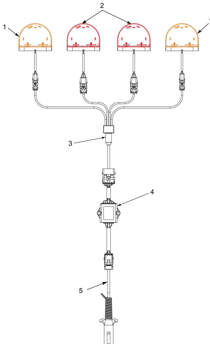
Figure 1-45: Electrical Schematic
