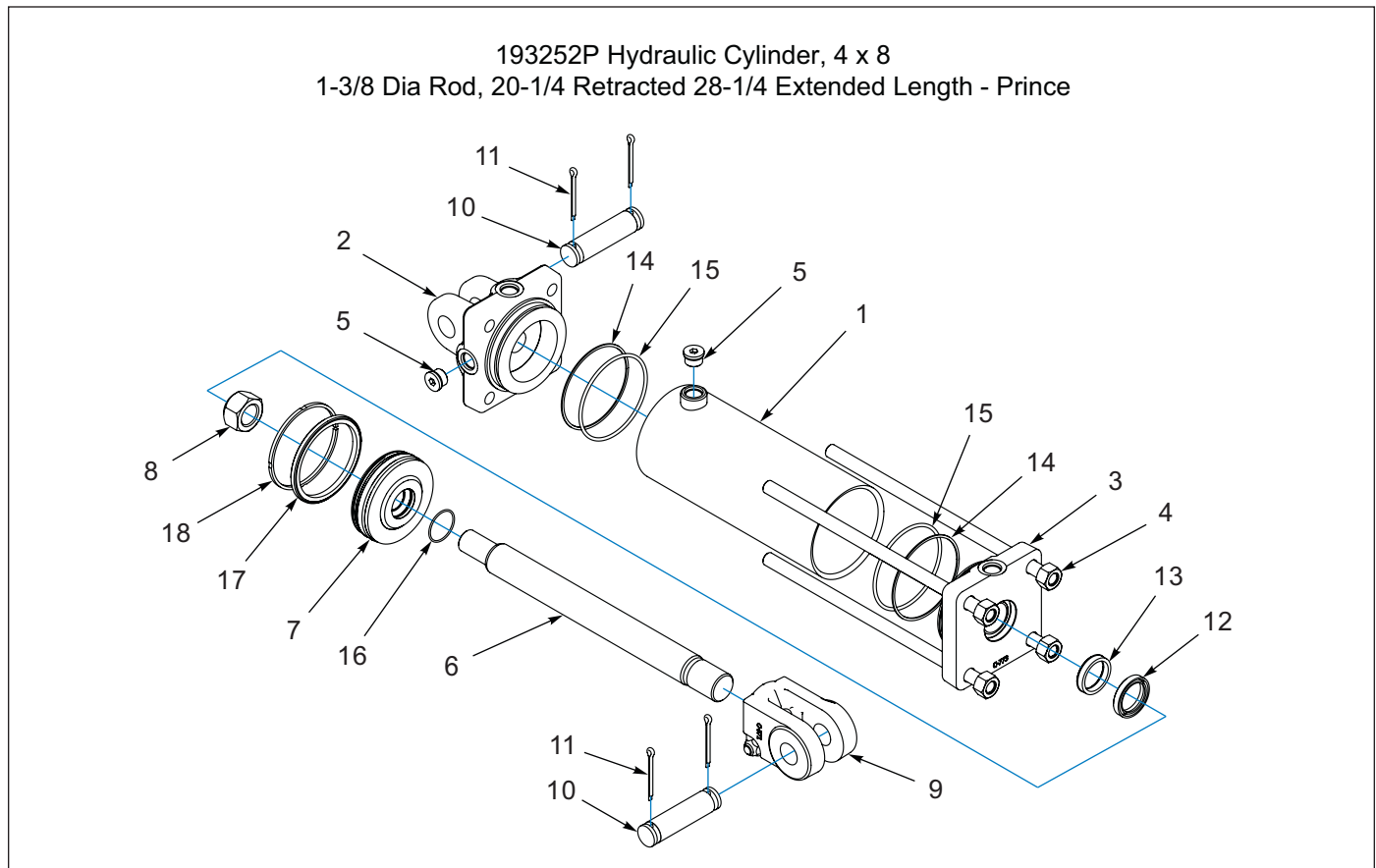
Figure 1-63: Hydraulic Cylinder, 4 x 8 Re-Phase - Prince
