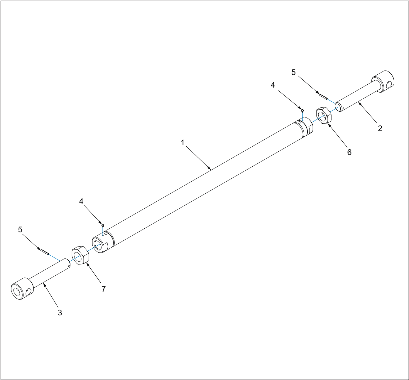
Figure 1-15: Turnbuckle
