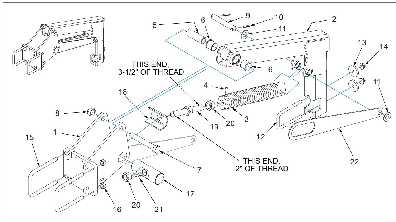
Figure 1-54: Wing Harrow Arm Assembly - Optional
