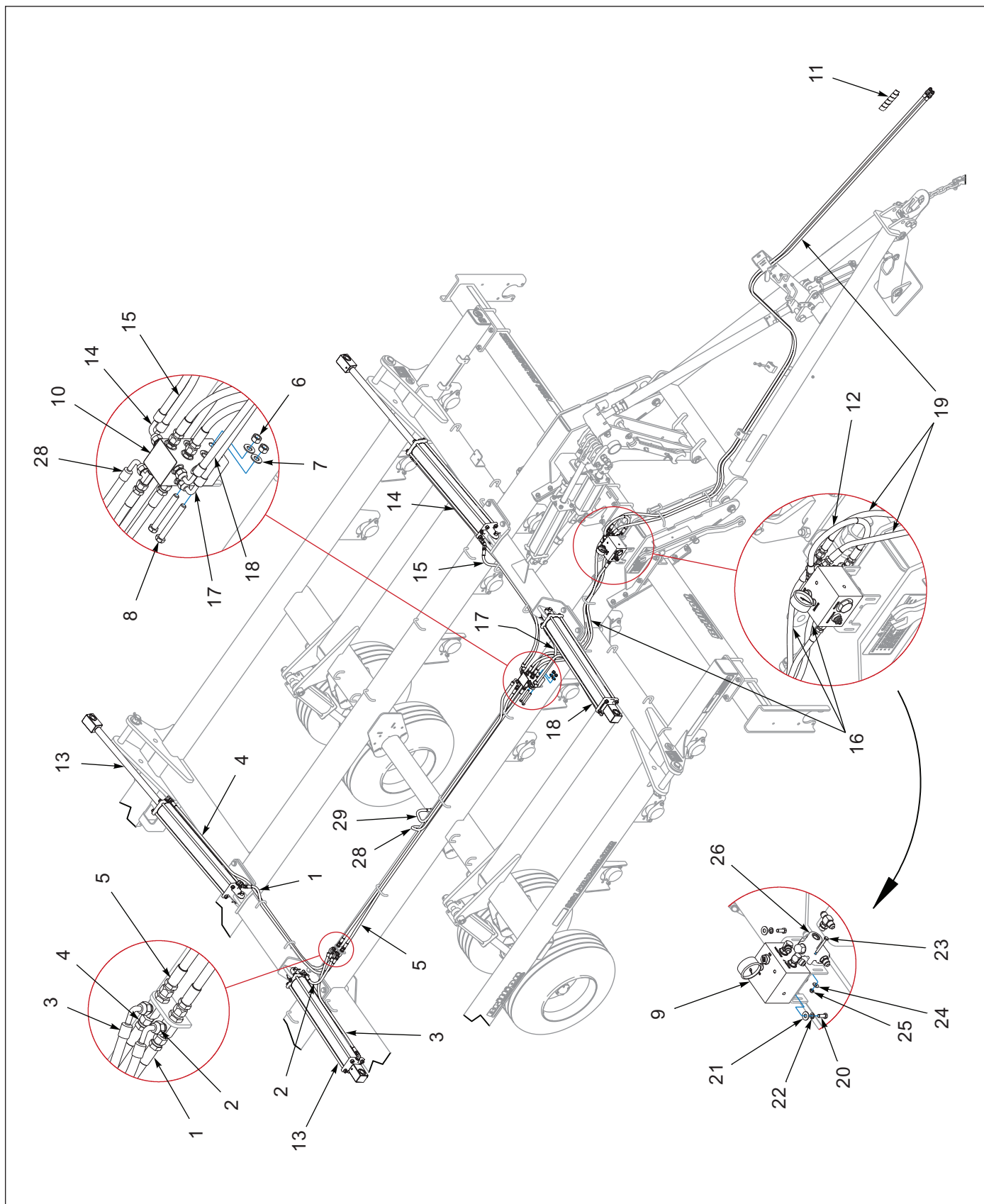
Figure 1-38: Fold and Down Pressure Hydraulic Layout
