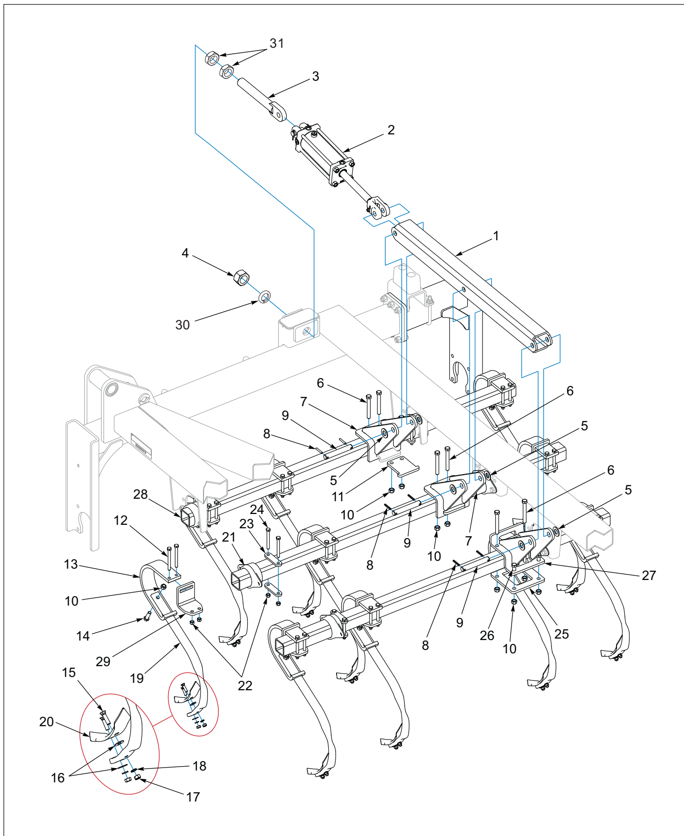
Figure 1-29: Tooth Control - Right Hand Wing
