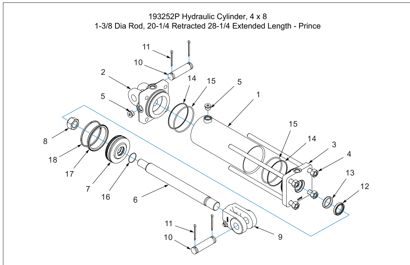
Figure 1-70: Hydraulic Cylinder, 4 x 8 Re-Phase - Prince
