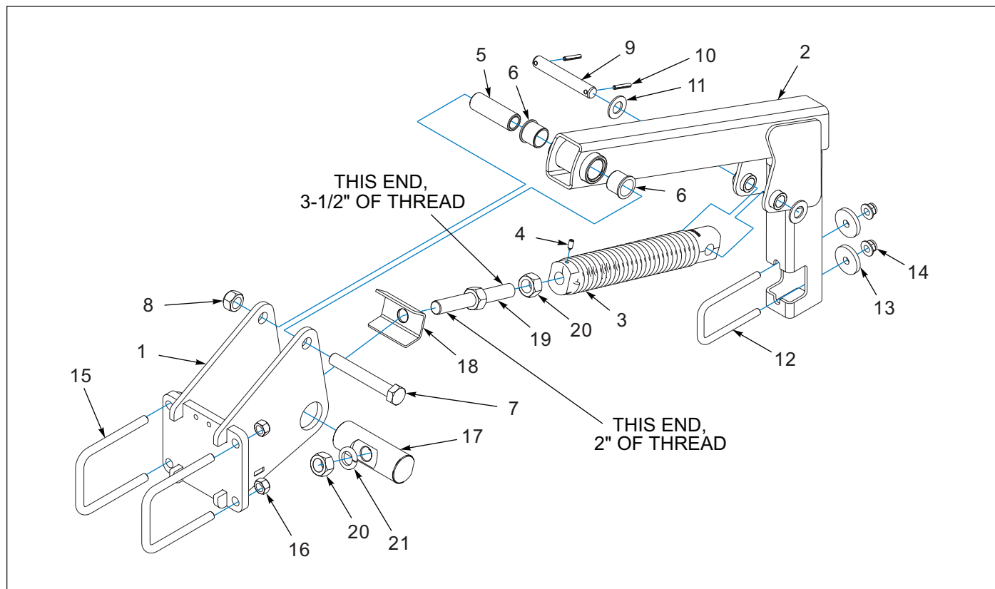
Figure 1-60: Center Harrow Arm Assembly - Optional
