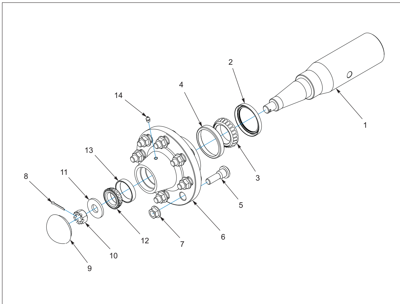
Figure 1-8: Hub and 4" Spindle Assembly
