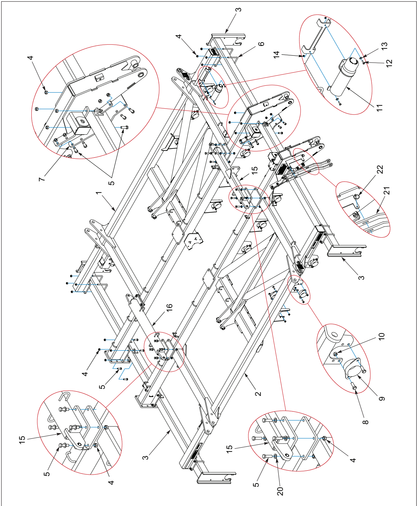
Figure 1-2: Frame (After 05/25/2022)
