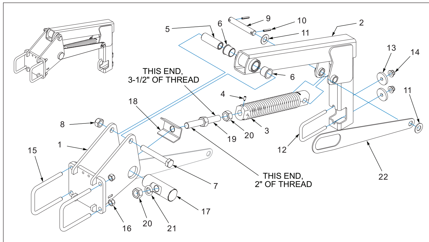
Figure 1-61: Wing Harrow Arm Assembly - Optional
