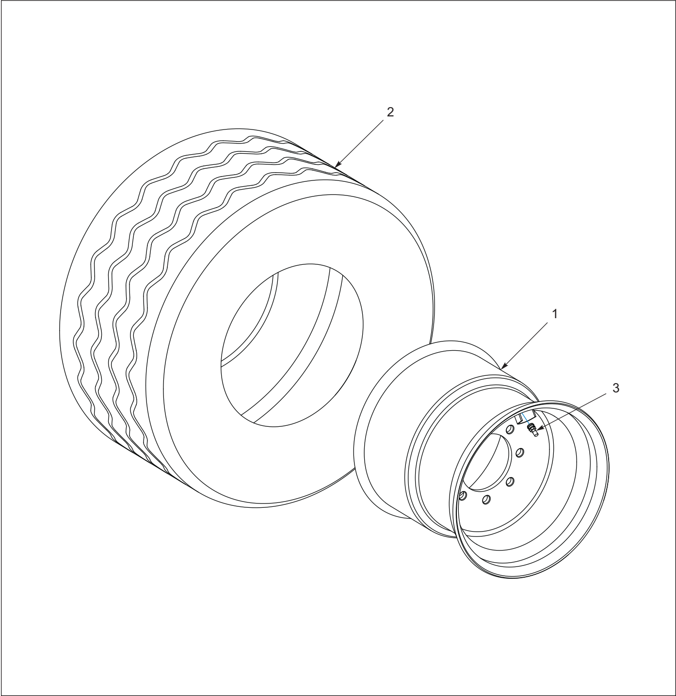
Figure 1-11: Tire and Wheel Assembly, 22156
