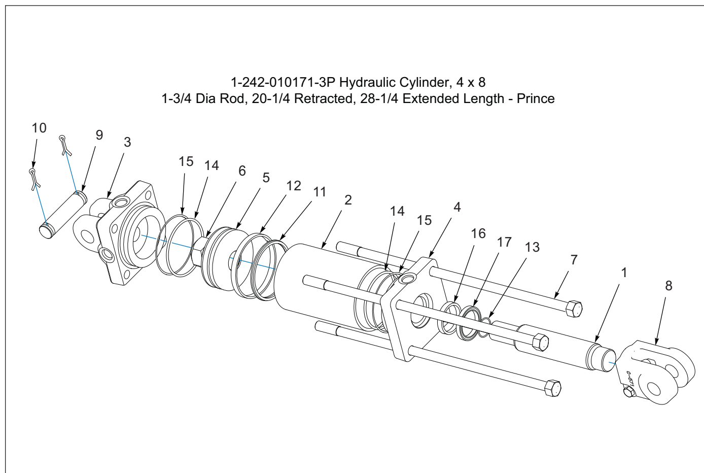
Figure 1-67: Hydraulic Cylinder, 4 x 8 - Prince
