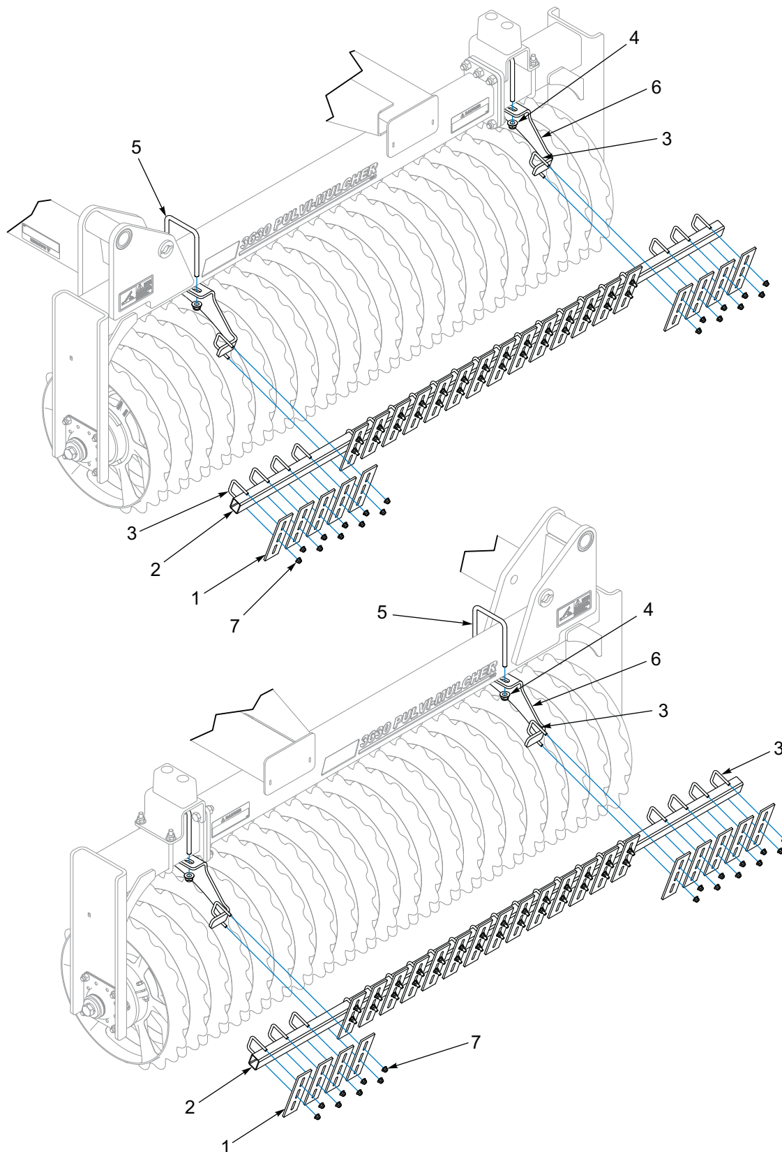
Figure 1-39: Wing Rear Scrapers
