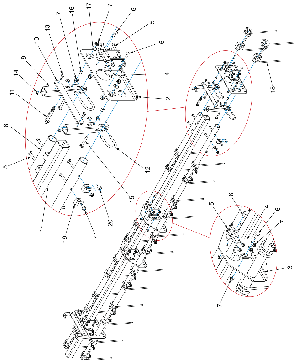
Figure 1-35: Center Harrow Assembly
