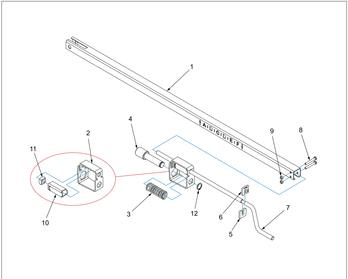
Figure 1-28: Shank Depth Control Assembly
