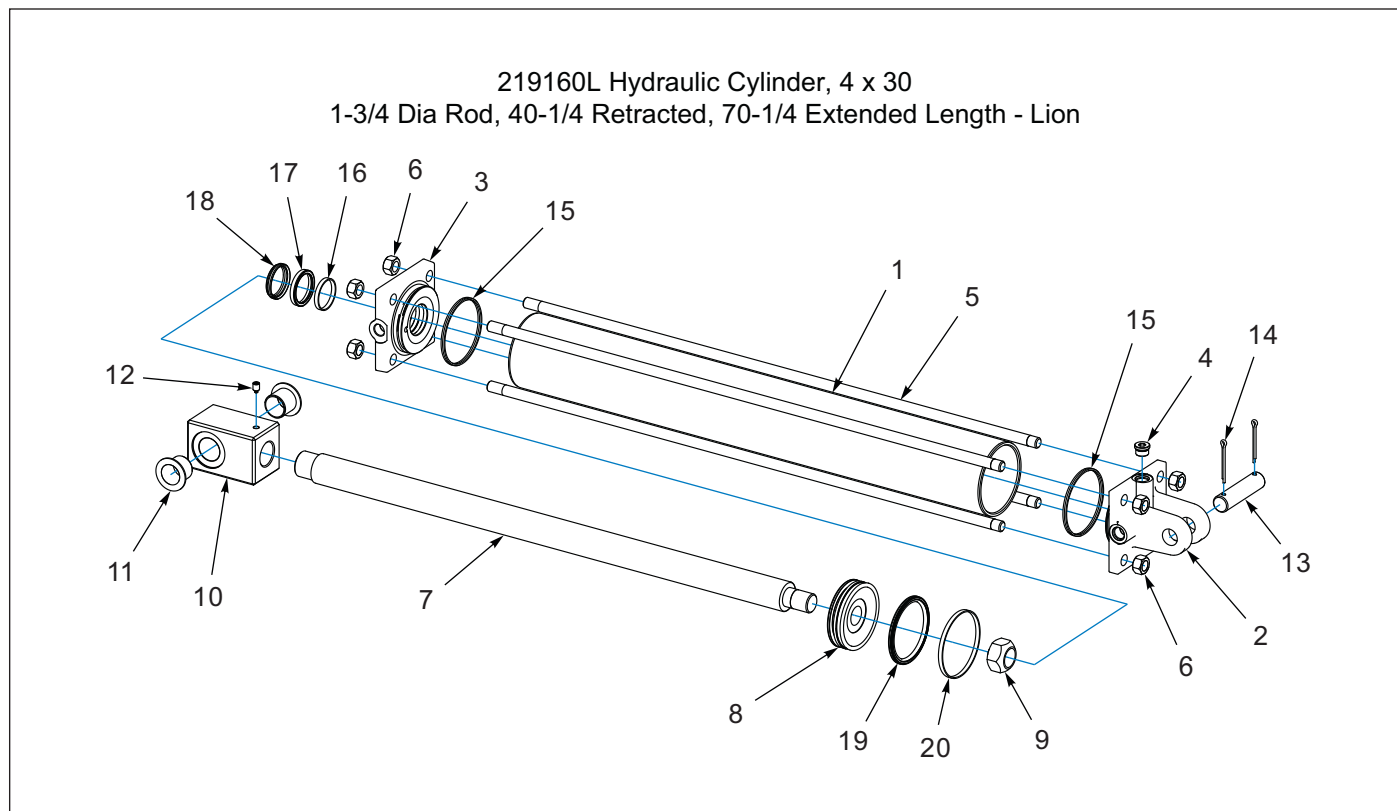
Figure 1-73: Hydraulic Cylinder, 4 x 30 - Lion
