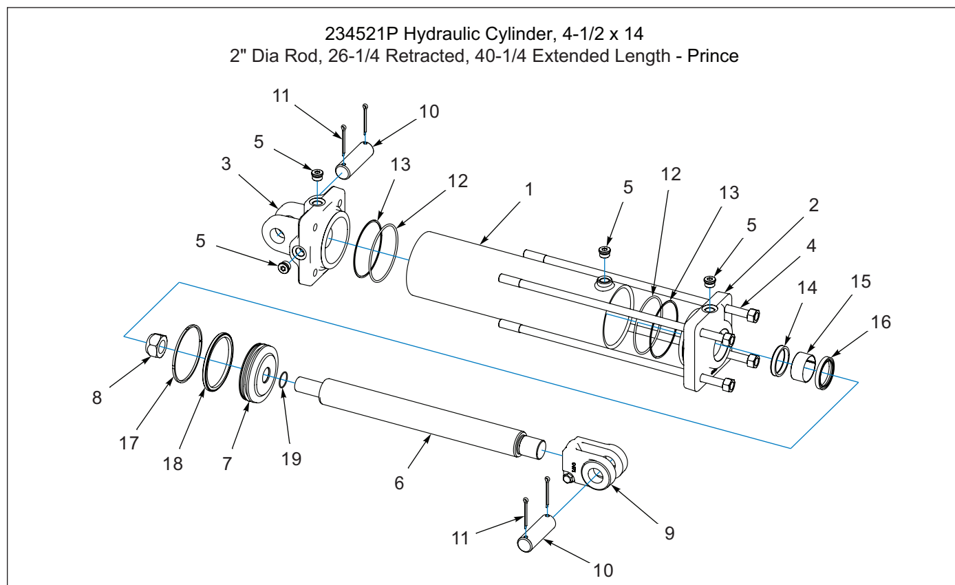
Figure 1-71: Hydraulic Cylinder, 4-1/2 x 14 Re-Phase - Prince
