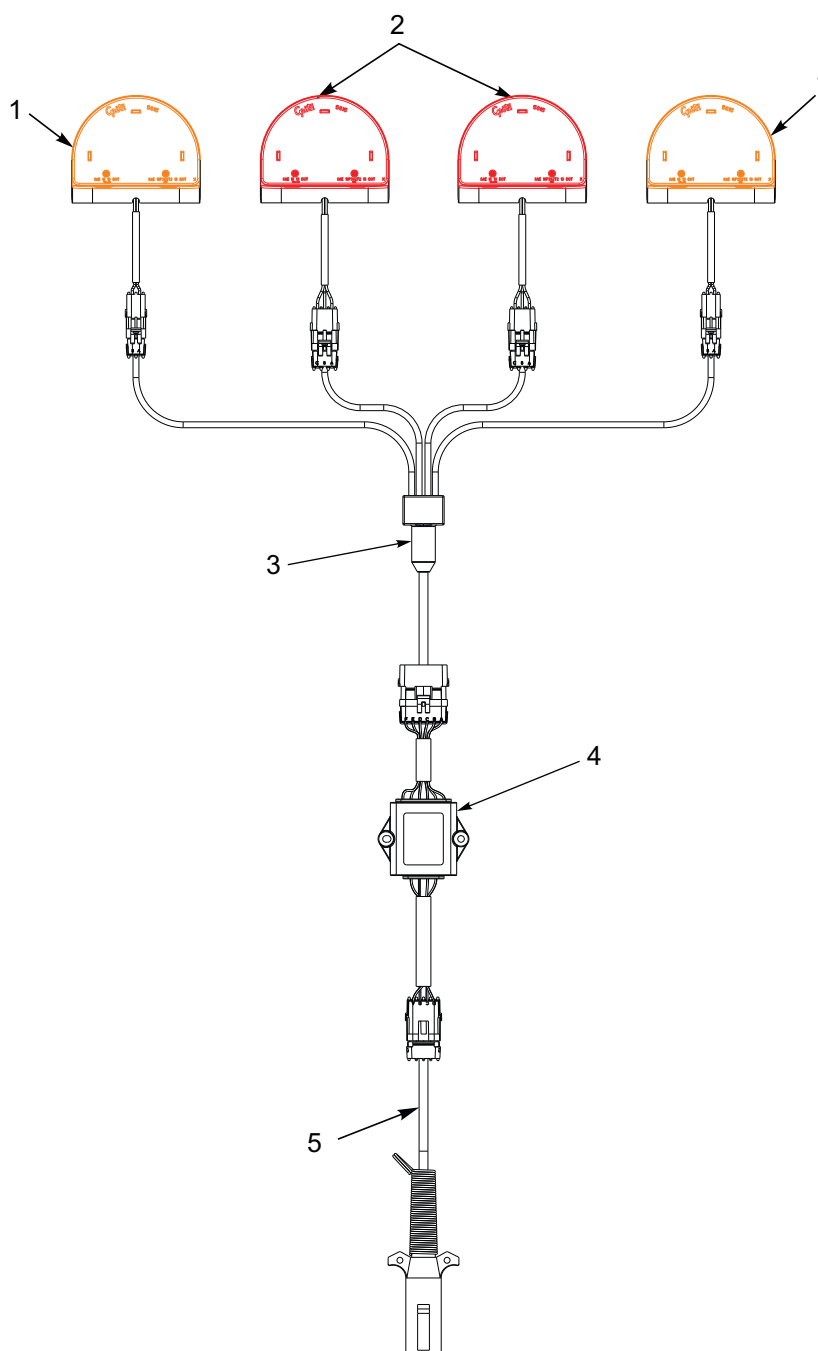
Figure 1-52: Electrical Schematic
