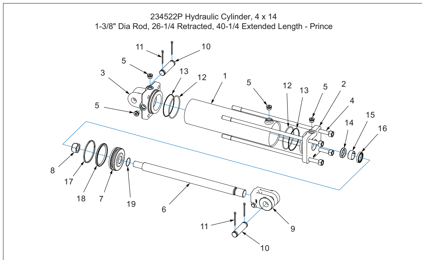
Figure 1-72: Hydraulic Cylinder, 4 x 14 Re-Phase - Prince
