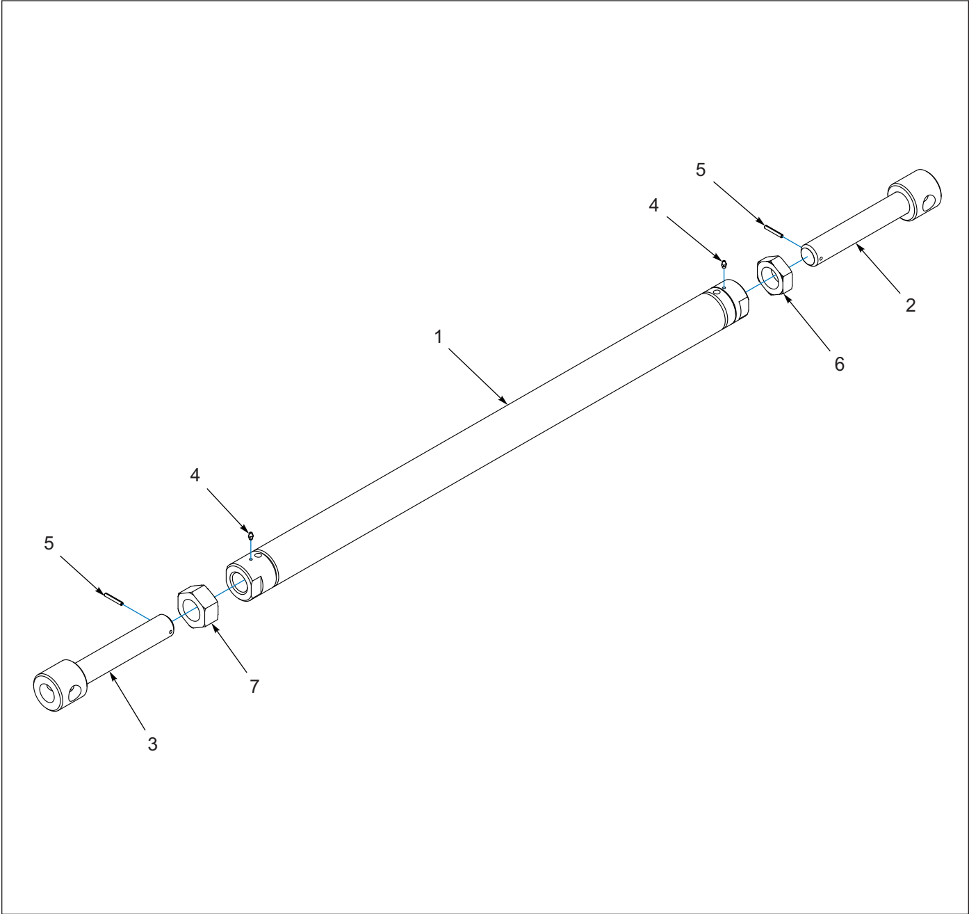
Figure 1-20: Turnbuckle
