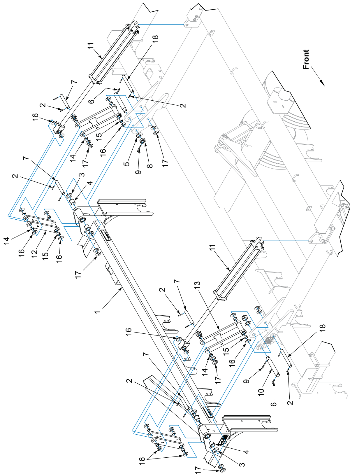
Figure 1-21: Wing Hinge
