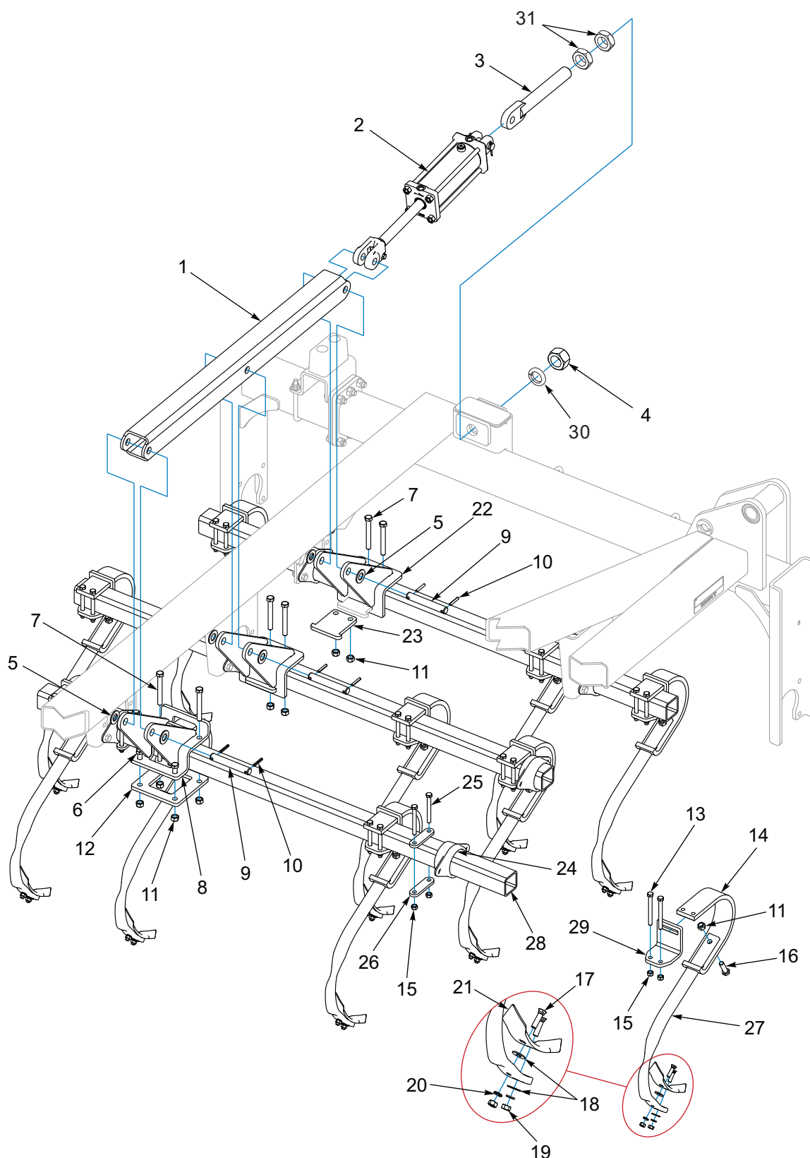
Figure 1-30: Tooth Control - Left Hand Wing
