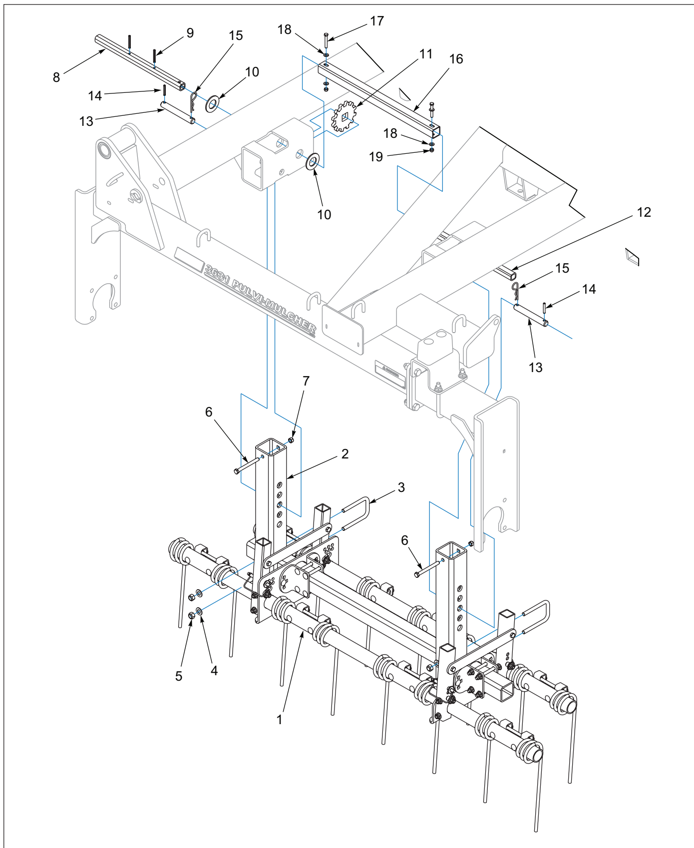
Figure 1-33: Right Hand Wing Harrow
