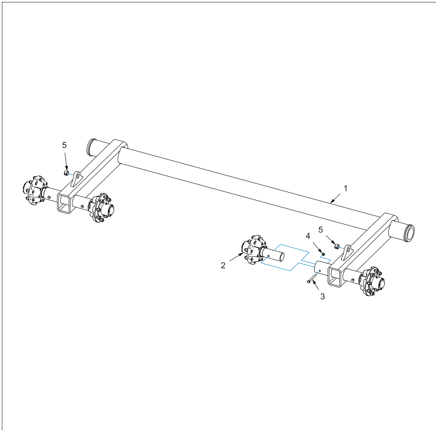
Figure 1-7: Transport Axle, 3" Spindle
