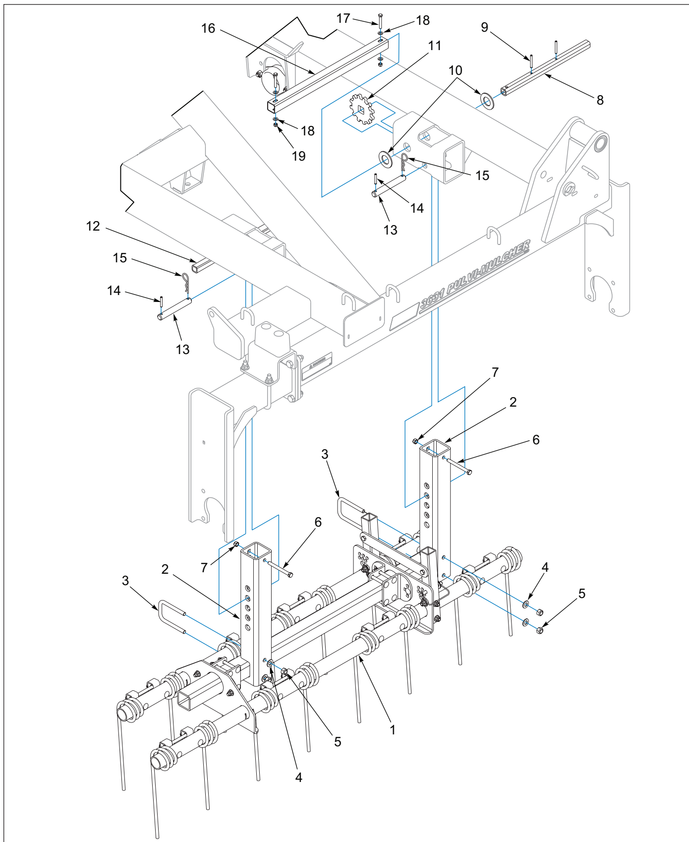
Figure 1-34: Left Hand Wing Harrow
