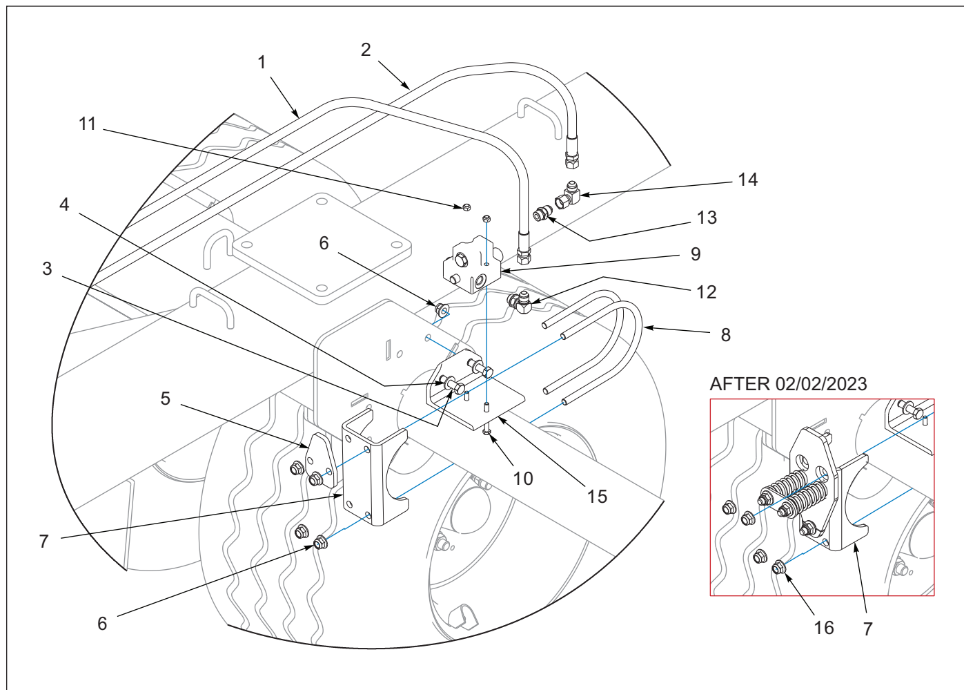
Figure 1-44: Fold and Down Pressure Limit Valve Layout
