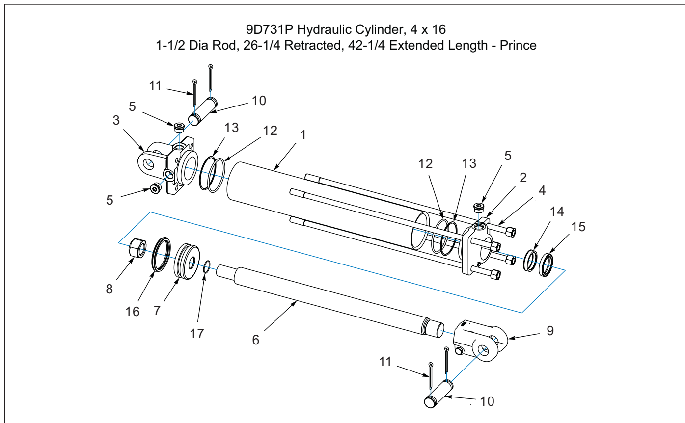
Figure 1-75: Hydraulic Cylinder, 4 x 16 - Prince
