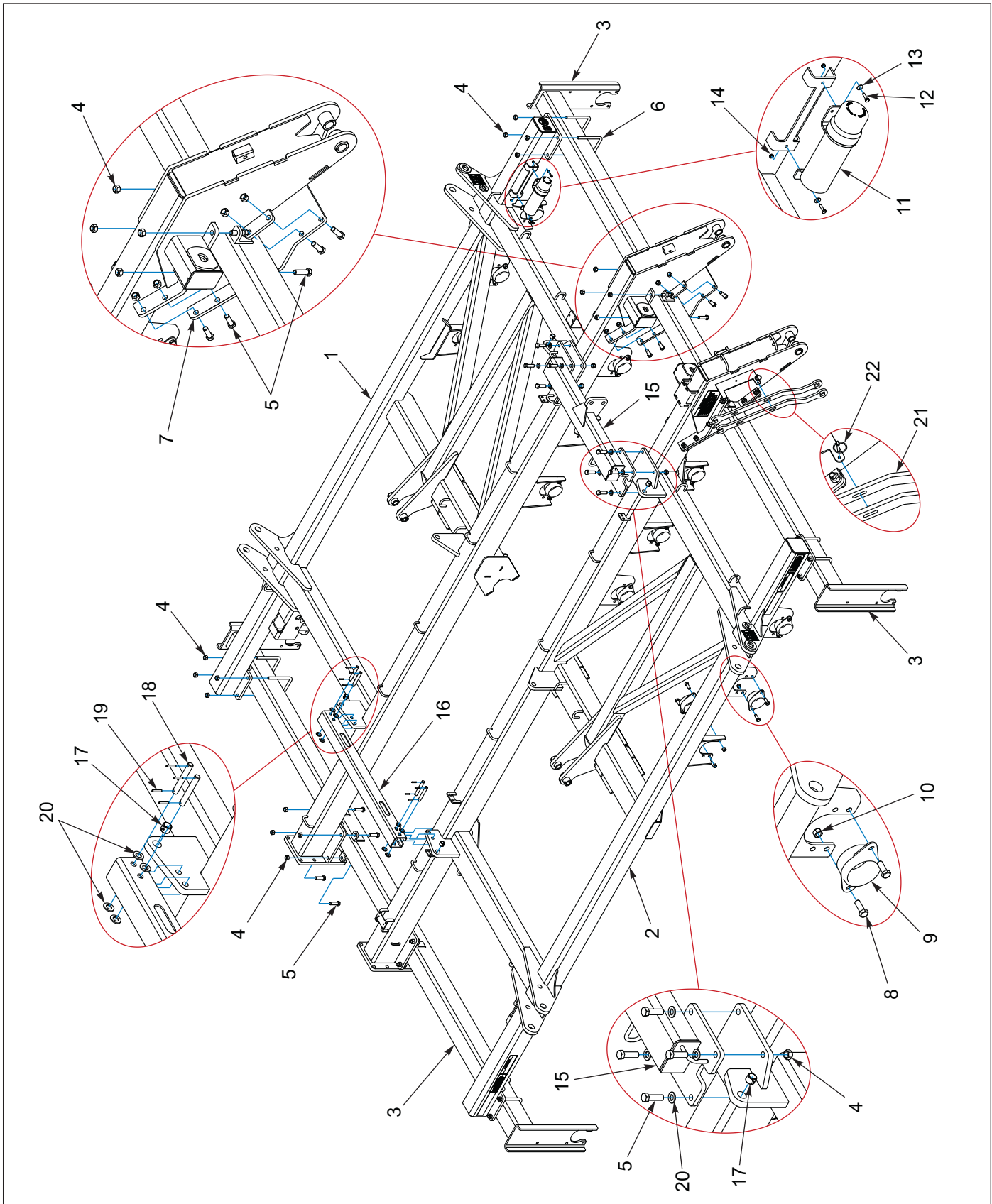
Figure 1-3: Frame (Before 05/25/2021)
