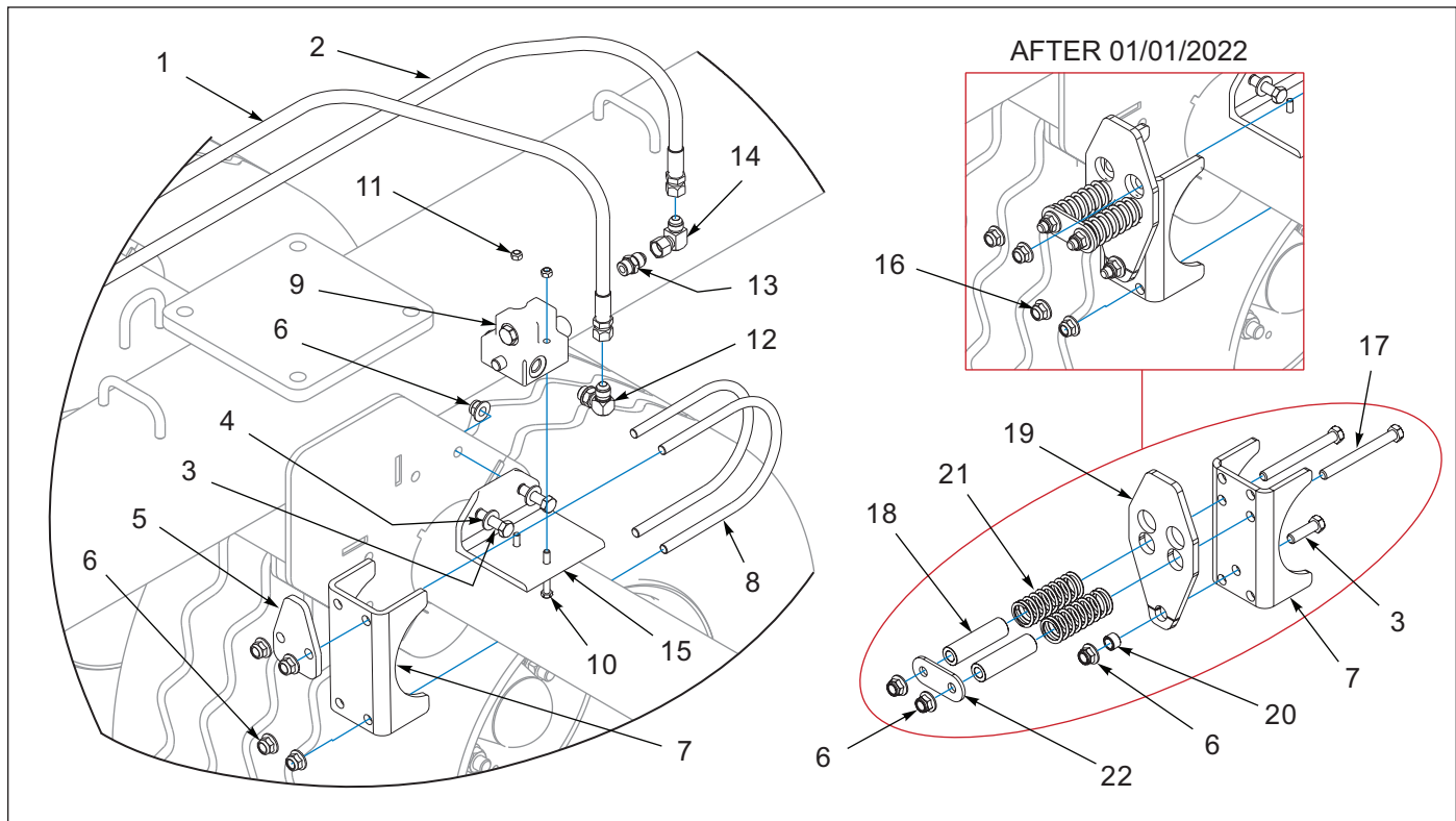
Figure 1-50: Fold and Down Pressure Limit Valve Layout
