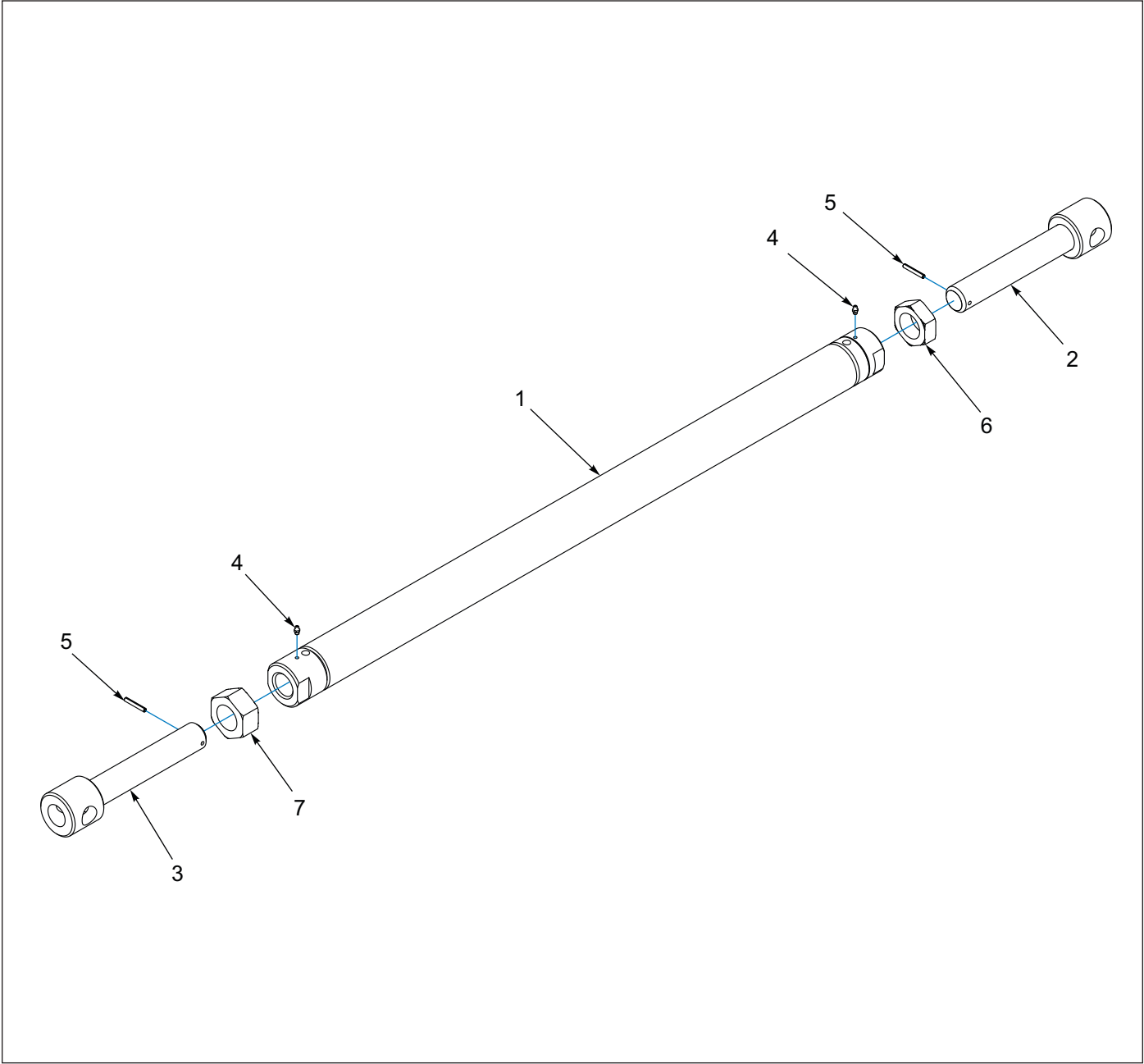
Figure 1-20: Turnbuckle
