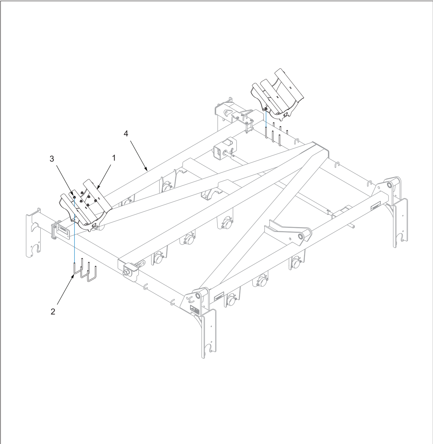
Figure 1-21: Wing Rest (After 01/01/2022)
