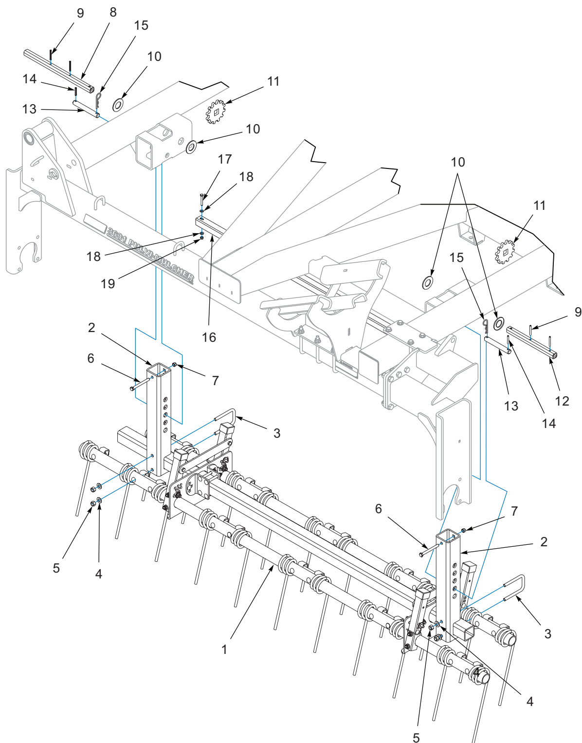
Figure 1-37: Wing Harrow - Right Hand
