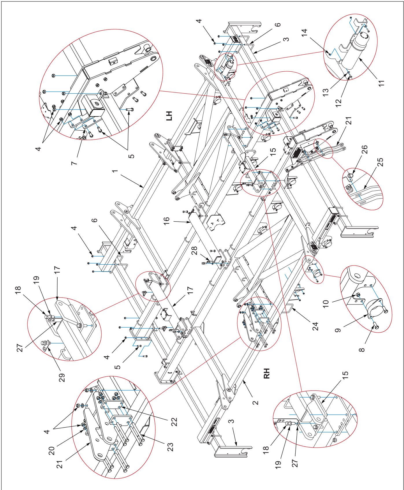
Figure 1-2: Frame (After 01/01/2022)
