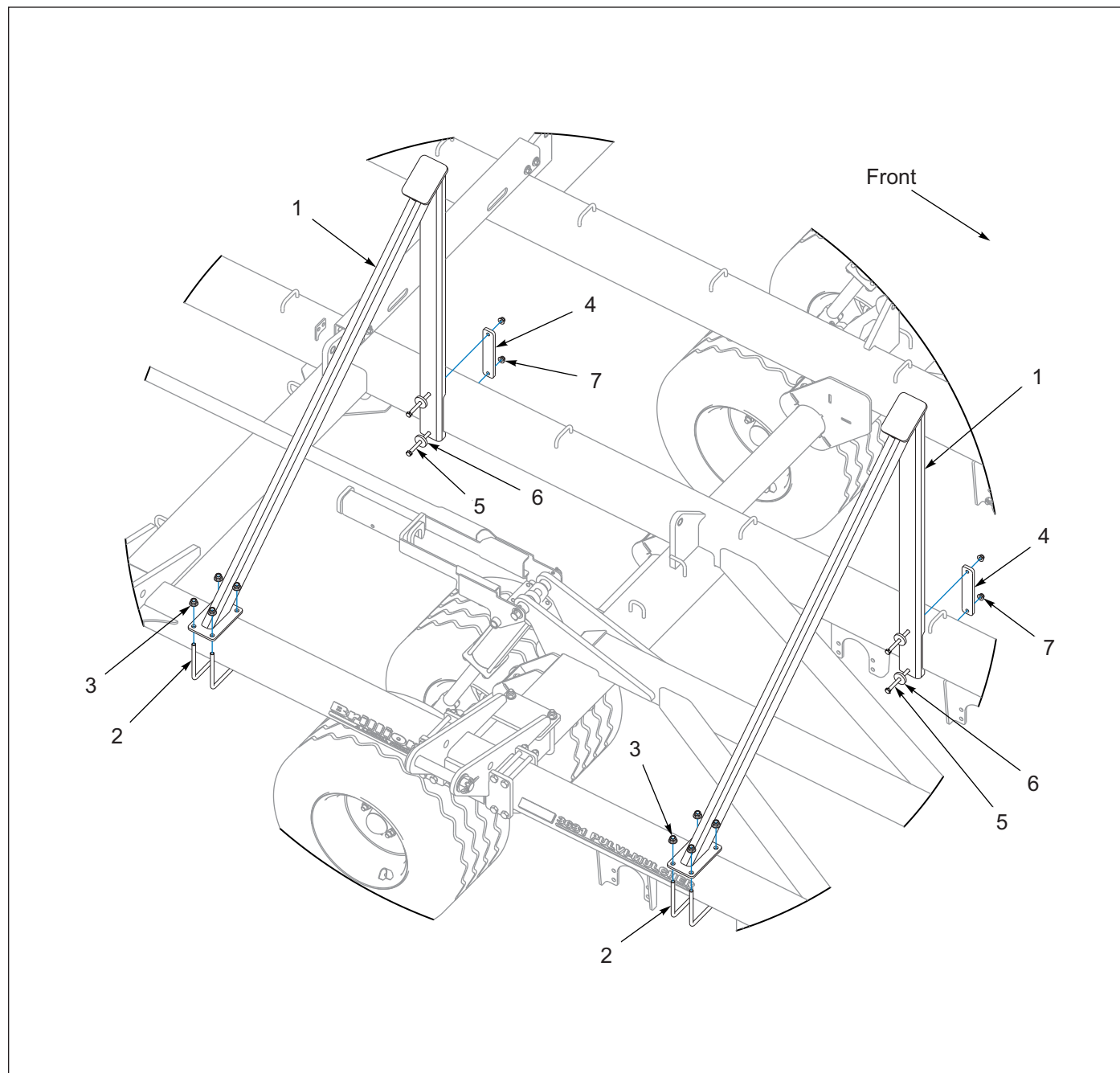
Figure 1-22: Wing Rest (Before 01/01/2022)
