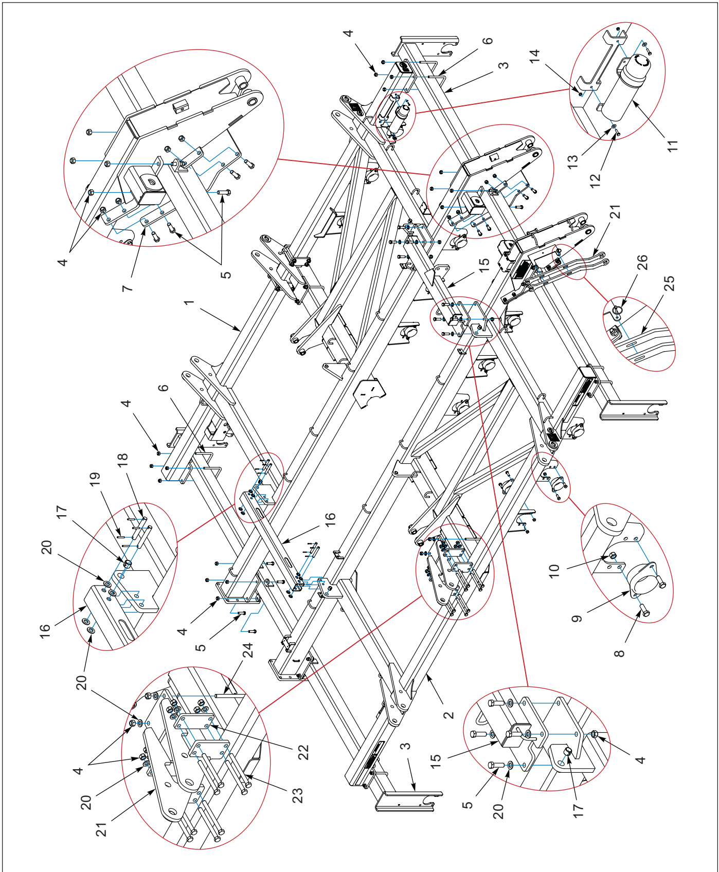
Figure 1-3: Frame (Before 01/04/2023)
