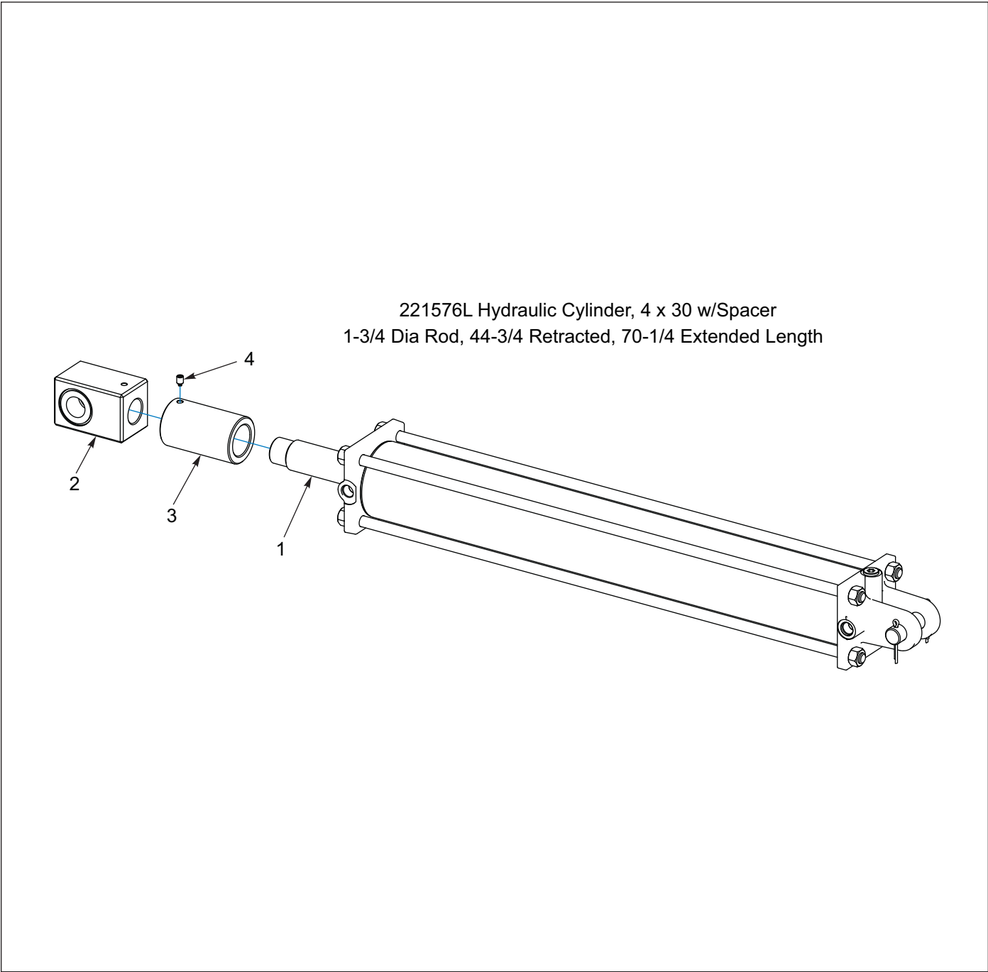
Figure 1-90: Hydraulic Cylinder, 4 x 30 with Spacer - Lion
