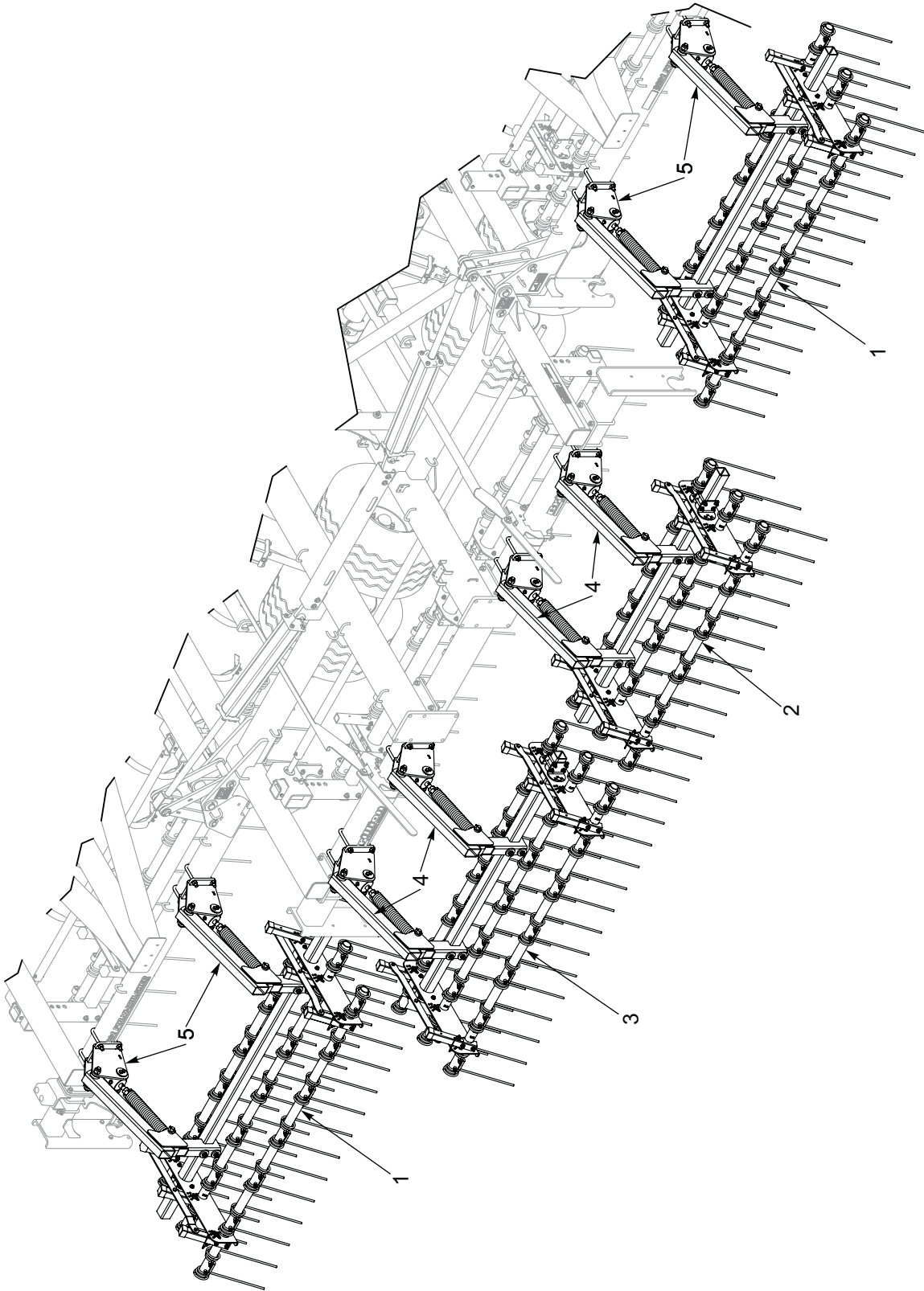
Figure 1-65: Harrow Kit, 3-Bar Coil Tine Without Lift - Optional
