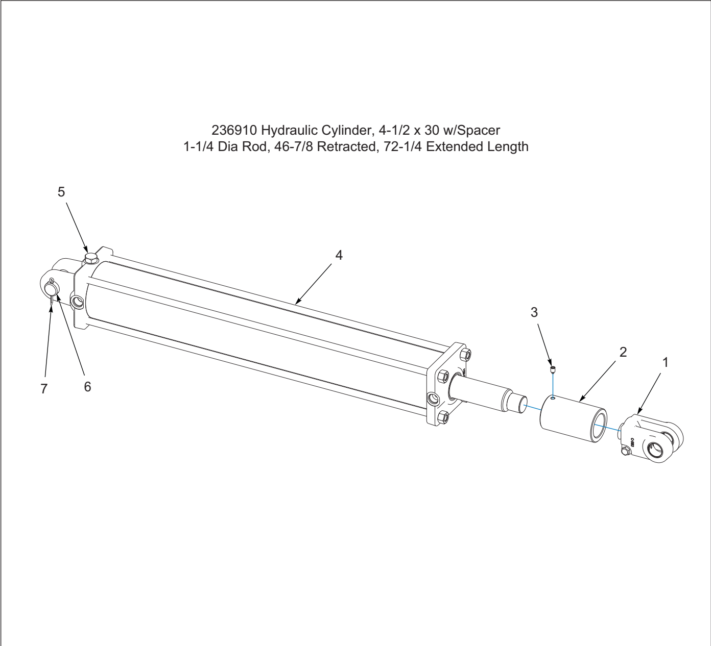
Figure 1-92: Hydraulic Cylinder, 4-1/2 x 30 with Spacer
