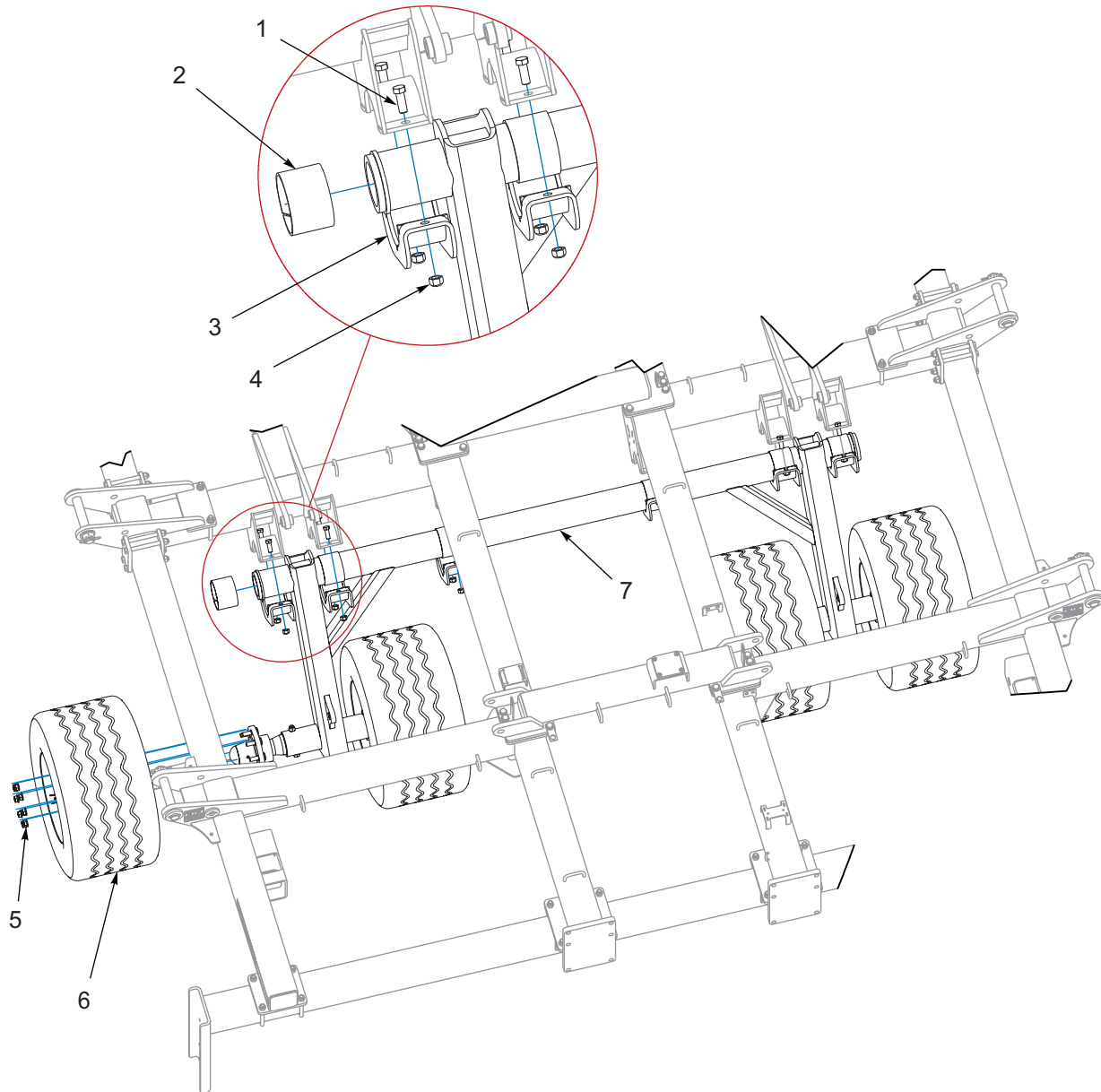
Figure 1-4: Transport Axle Mounting Components
