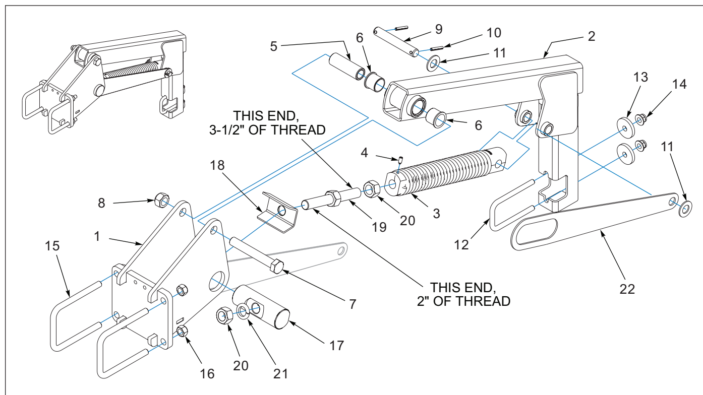
Figure 1-67: Wing Harrow Arm Assembly, Without Lift
