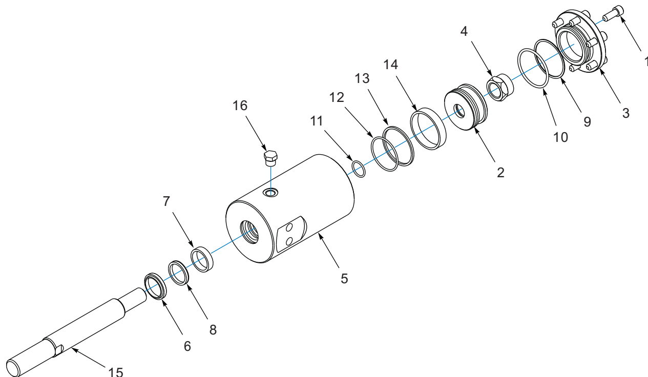
Figure 1-81: Hydraulic Cylinder, 2-1/2 x 2-1/2
