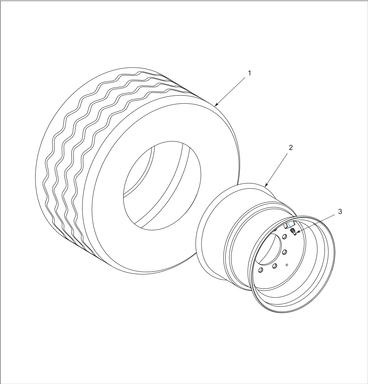
Figure 1-9: Tire and Wheel Assembly, 221526
