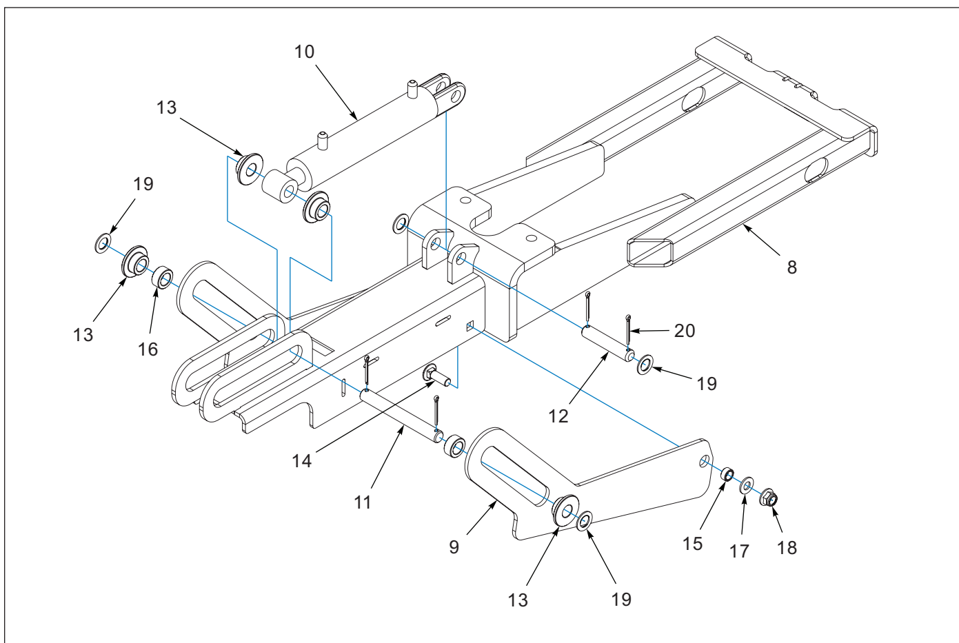
Figure 1-13: Rockshaft Cylinder Transport Lock (Automatic) - Detail
