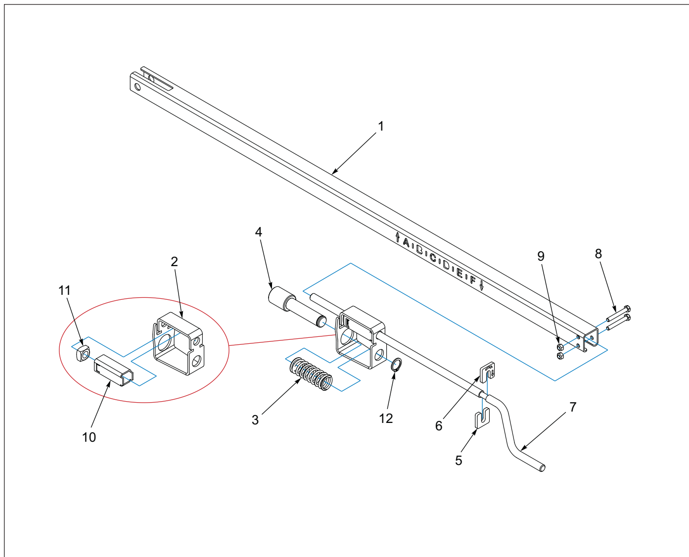
Figure 1-32: Shank Depth Control Assembly
