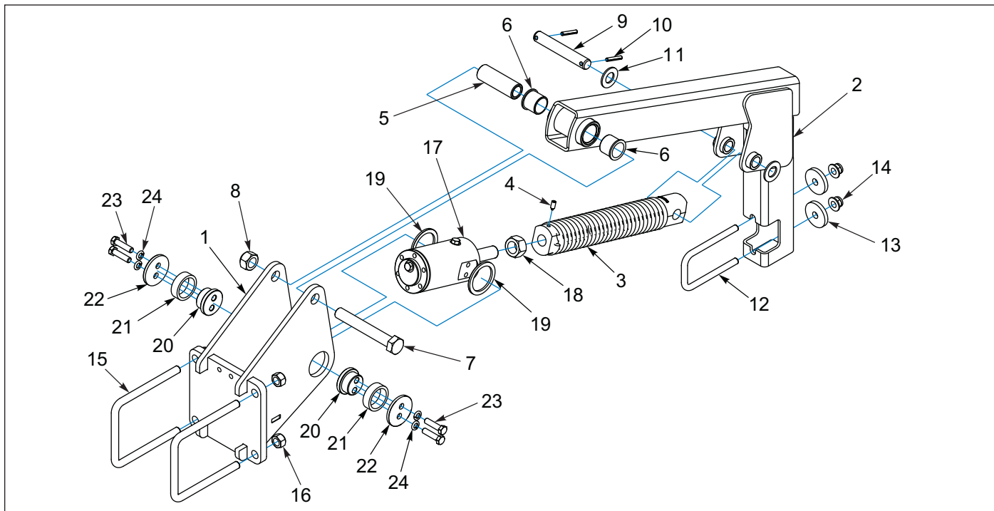
Figure 1-70: Harrow Arm Assembly, Center With Lift
