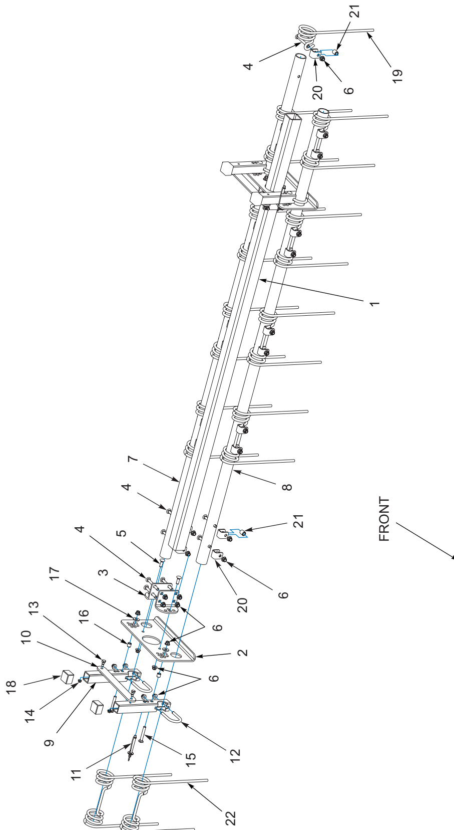
Figure 1-41: Wing Harrow Assembly - Left Hand
