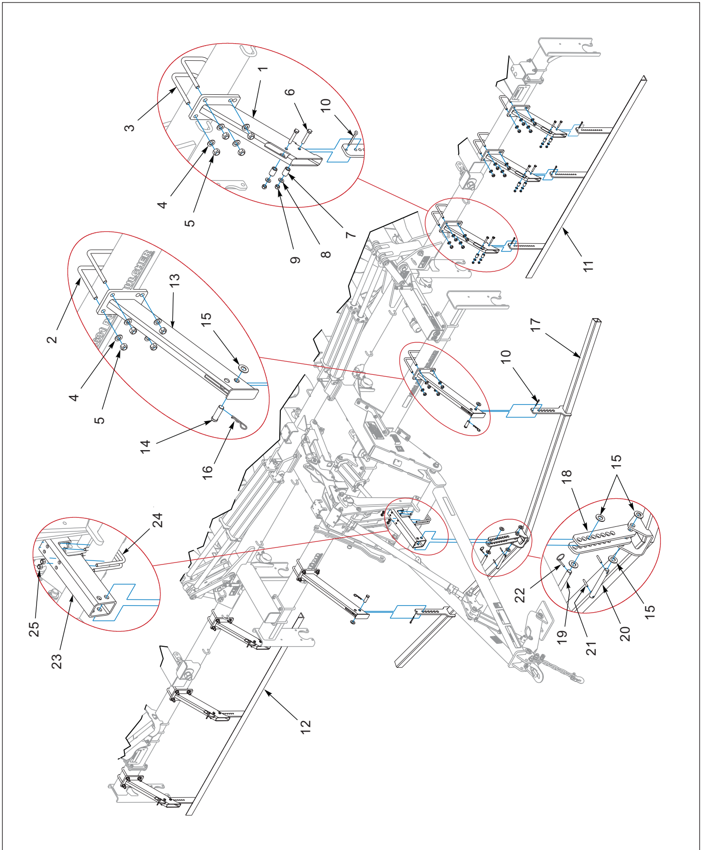
Figure 1-78: V-Leveler - Optional
