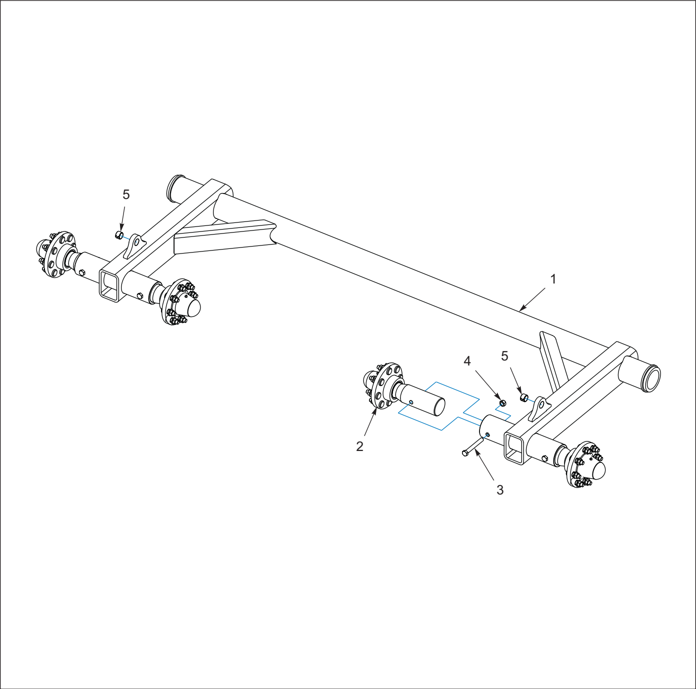
Figure 1-5: Transport Axle, 4" Spindle
