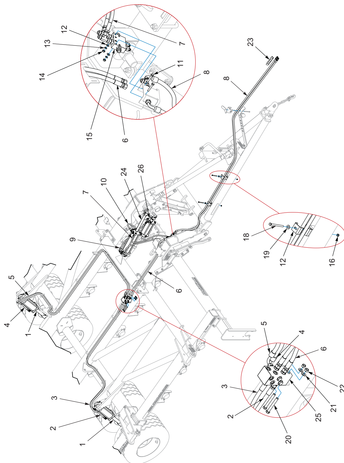
Figure 1-59: Lift Hydraulic Layout (No Wing Lift Wheels)
