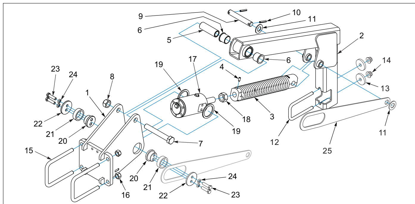
Figure 1-71: Harrow Arm Assembly, Wing With Lift
