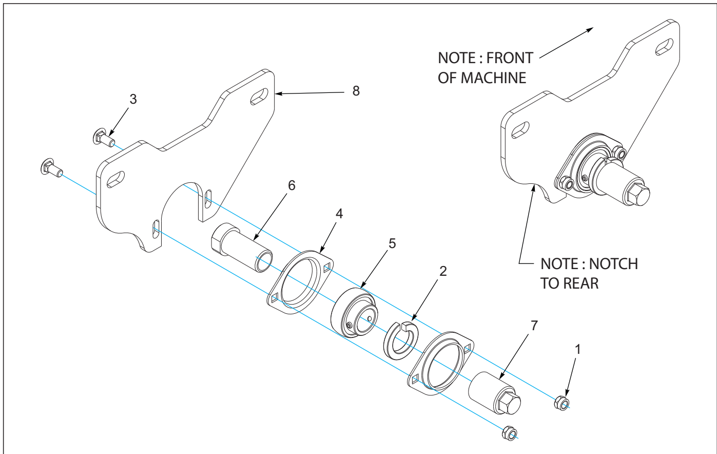
Figure 3-35: Seed Rate Adjust Assembly, Right
