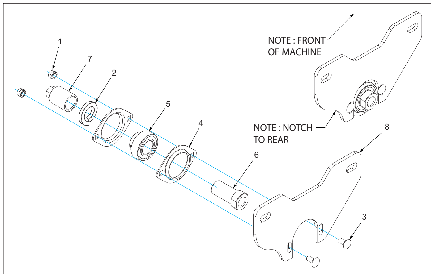
Figure 3-36: Seed Rate Adjust Assembly, Left
