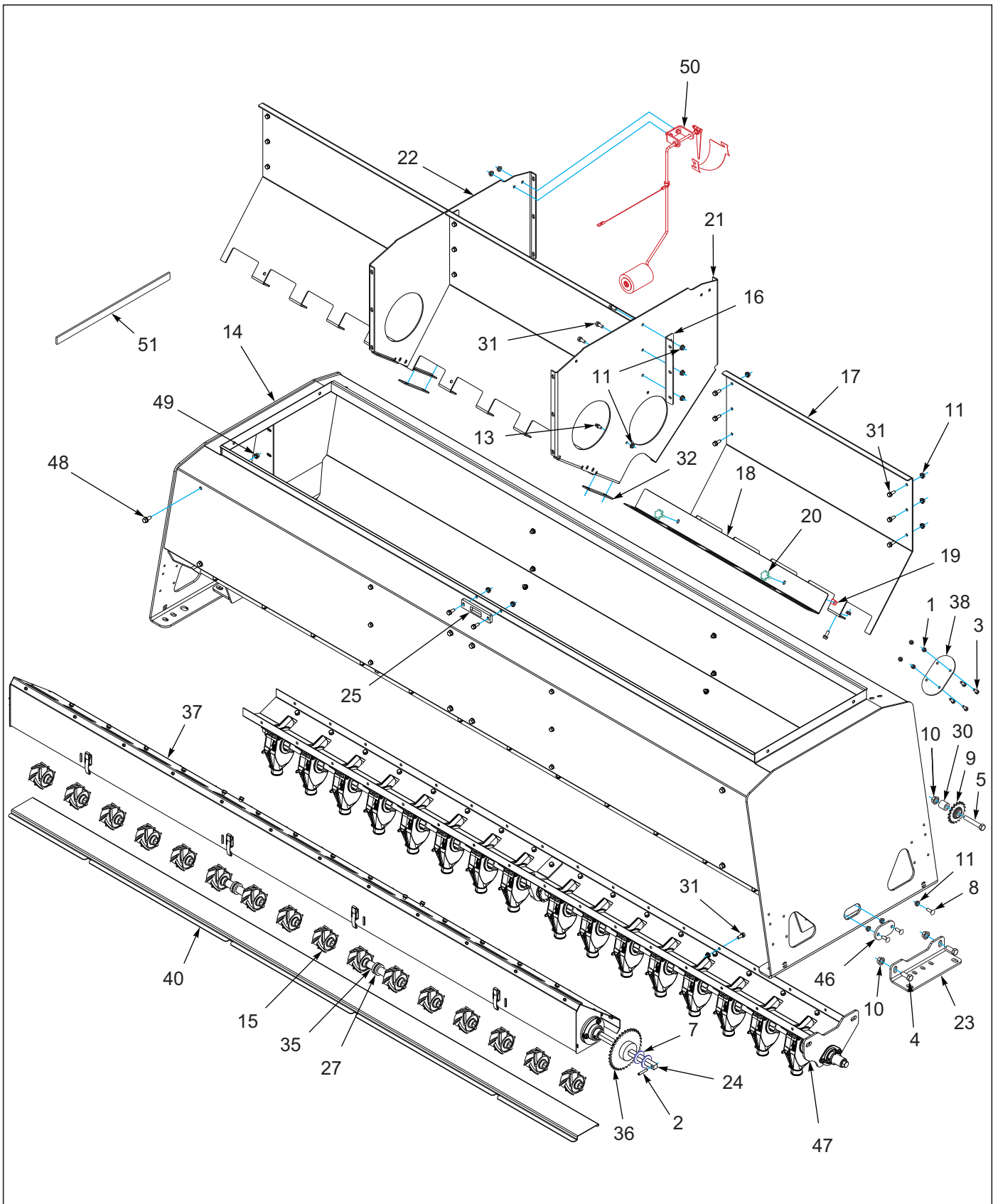
Figure 3-19: Box Assembly W/Fertilizer 5211-20' (1 of 2)
