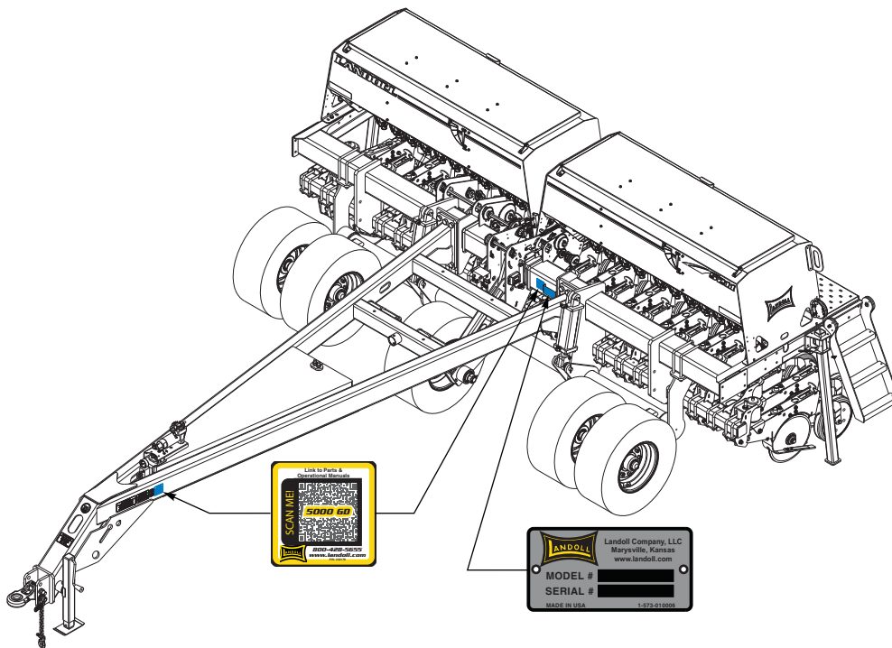
Figure 12-1: Identification Plate and Location
