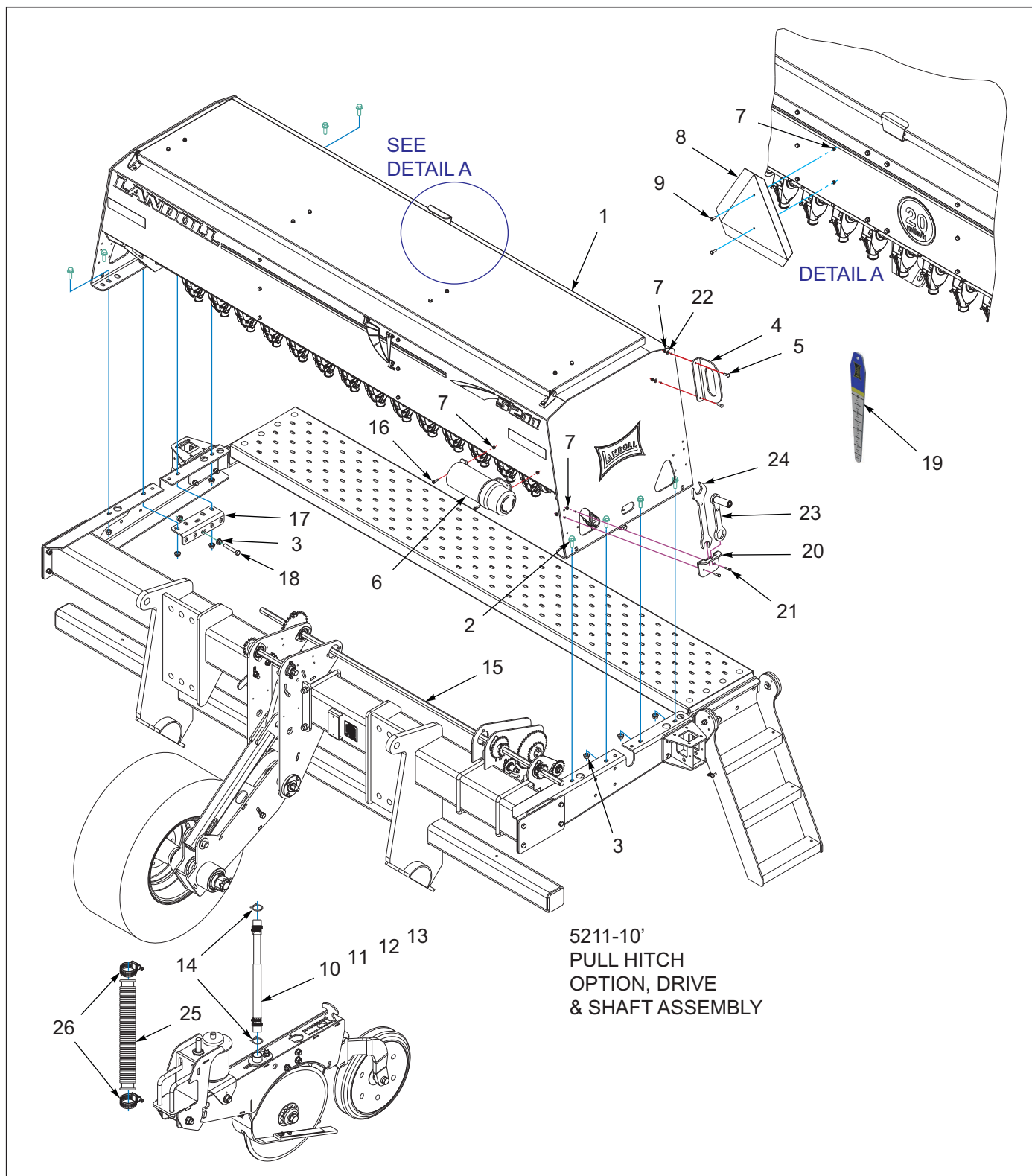
Figure 3-1: Seed Box Assembly, W/O Fertilizer 5211-10'
