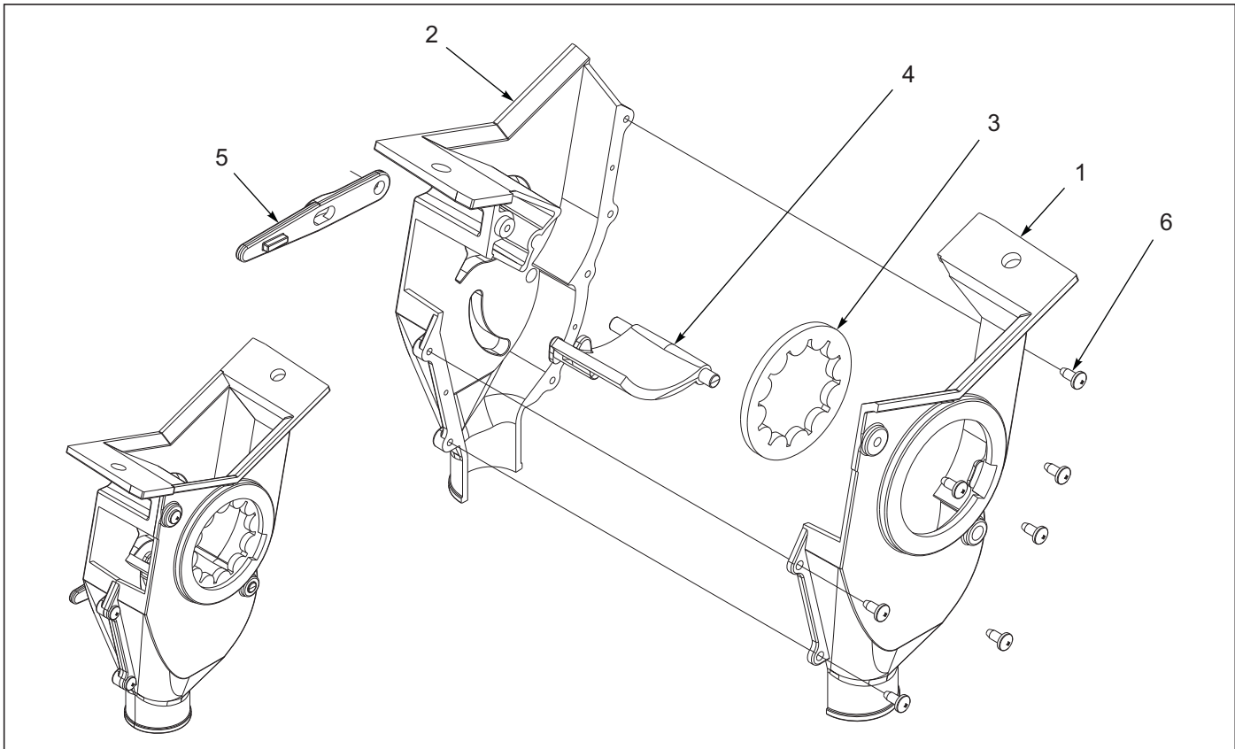
Figure 3-32: Seed Meter Housing Assembly
