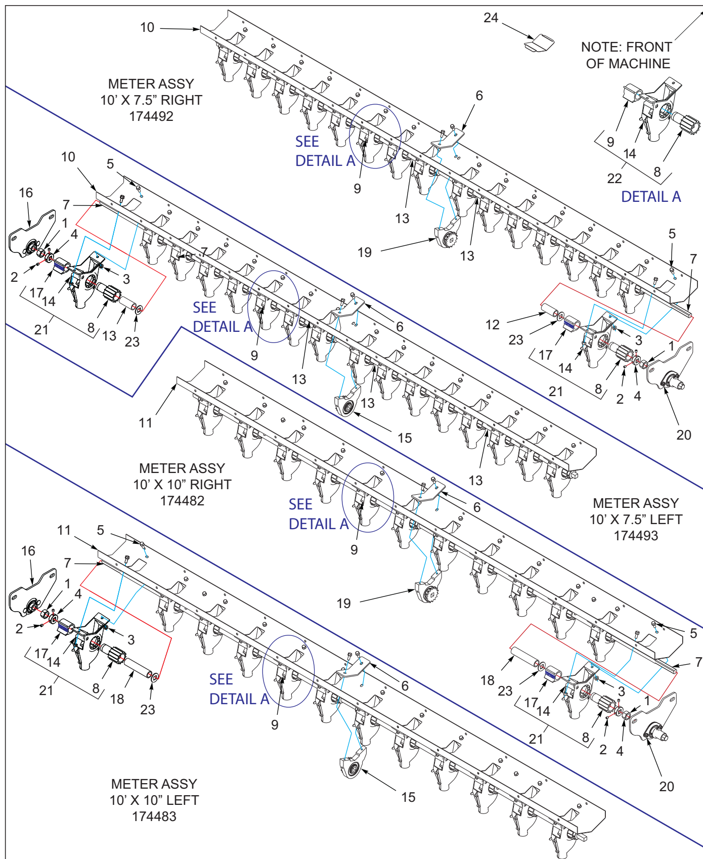
Figure 3-31: Seed Meter Assembly 5211-20'
