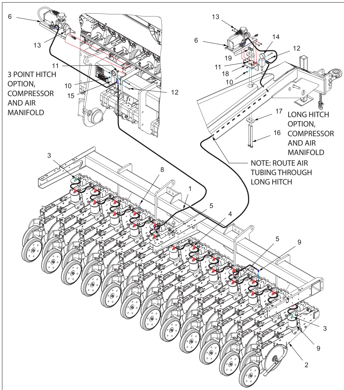
Figure 4-1: Air Opener Assembly
