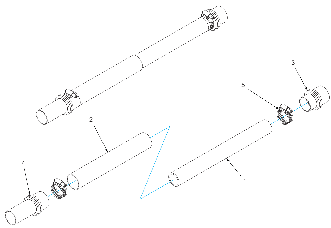
Figure 3-27: Seed Tube Assembly (Spring Opener)
