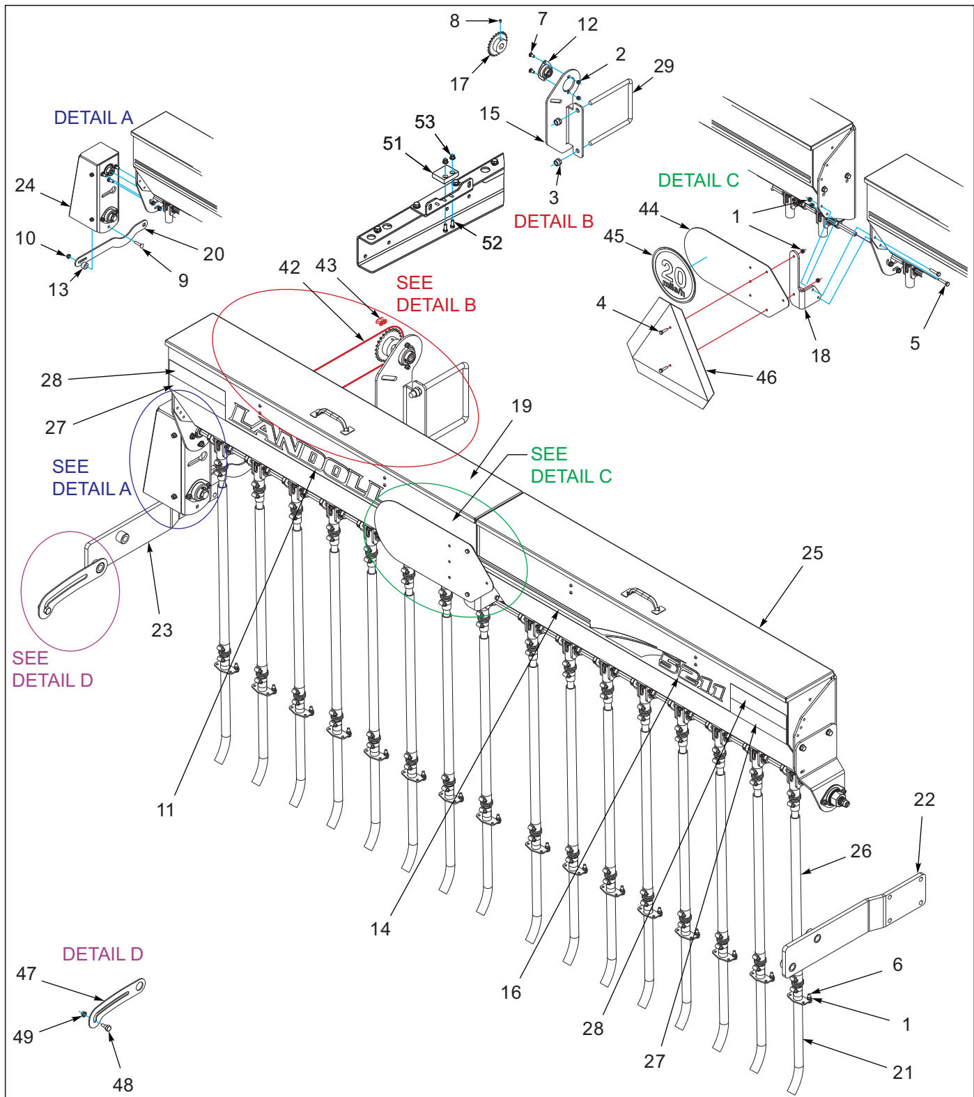
Figure 5-1: Small Seed Box Assembly 5211-10' (1 of 4)
