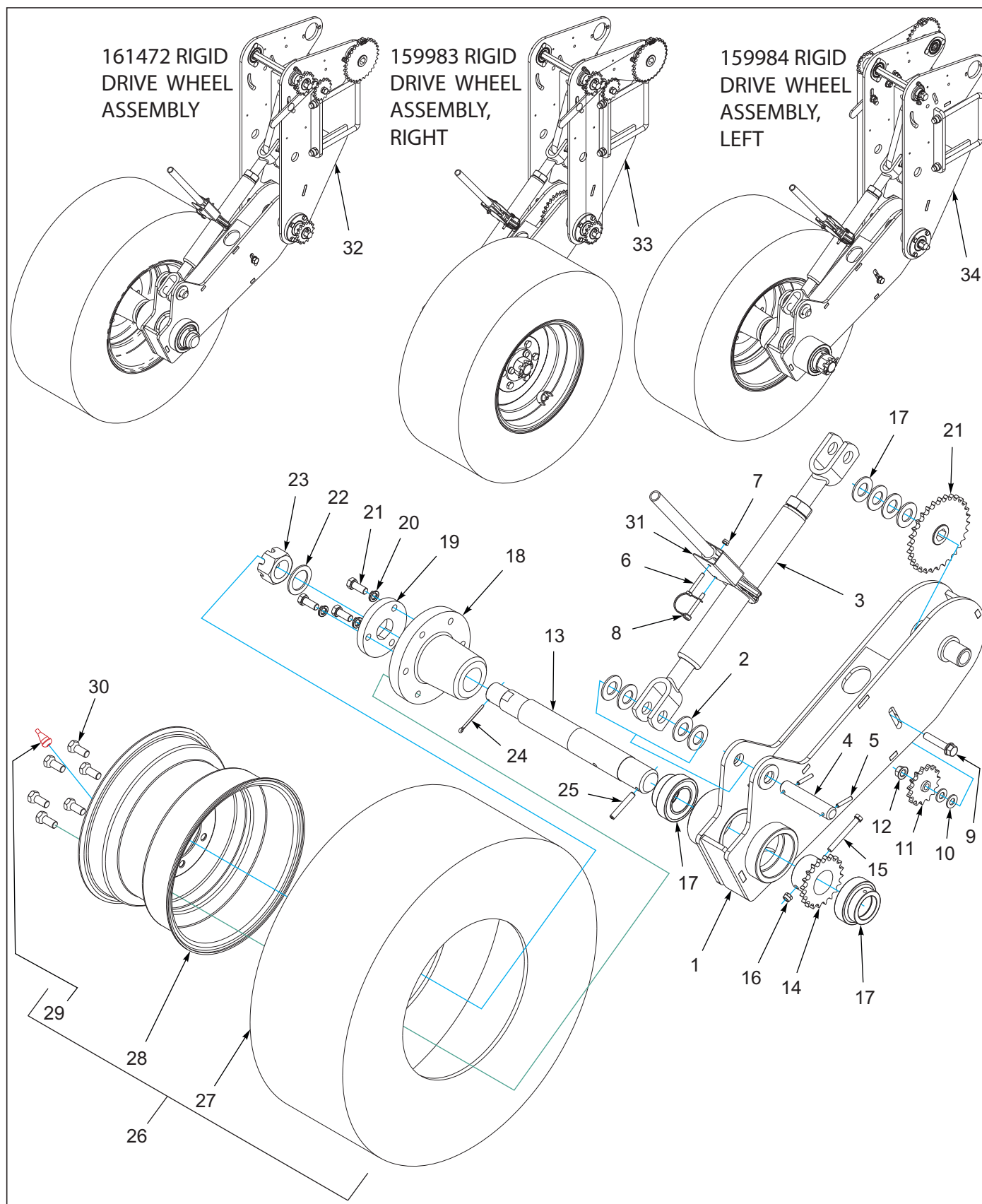
Figure 2-20: Drive Wheel Assembly, Rigid
