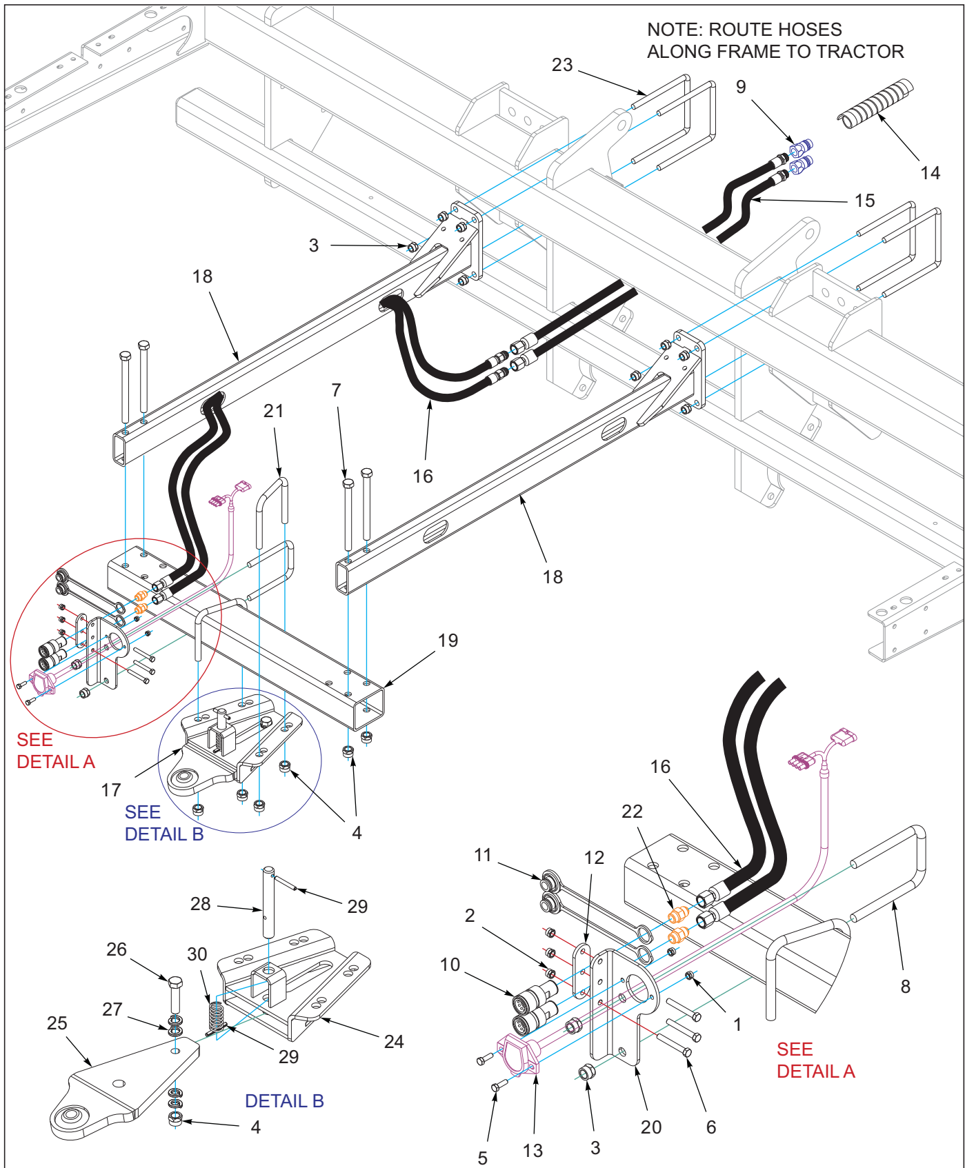
Figure 9-2: Rear Tow Hitch Assembly
