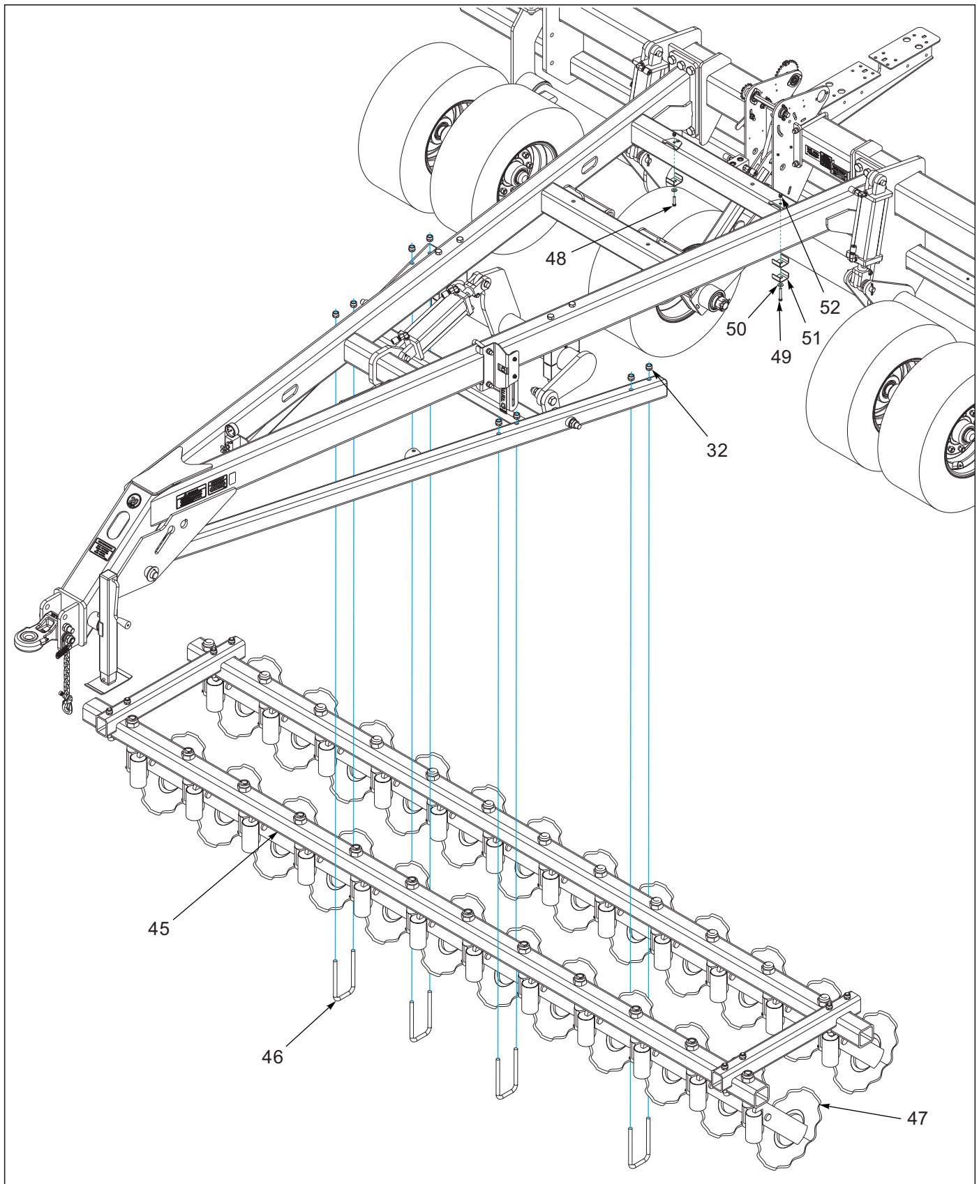
Figure 2-9: Hitch Assembly Coultter 5211-12-1/2'-15' (2 of 2)
