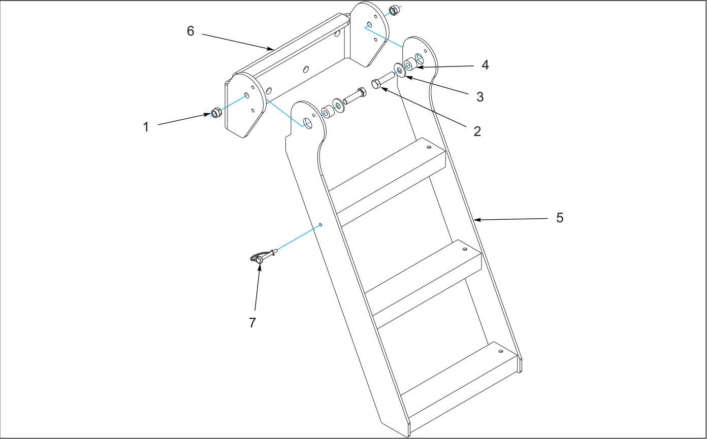
Figure 1-7: Ladder Assembly
