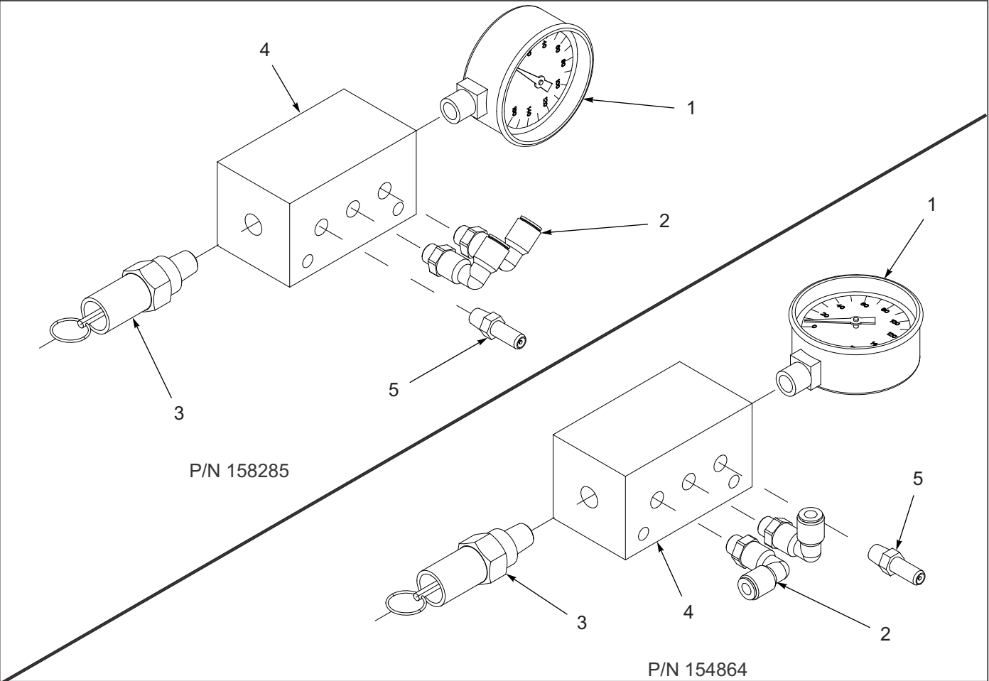
Figure 4-3: Air Manifold Assembly
