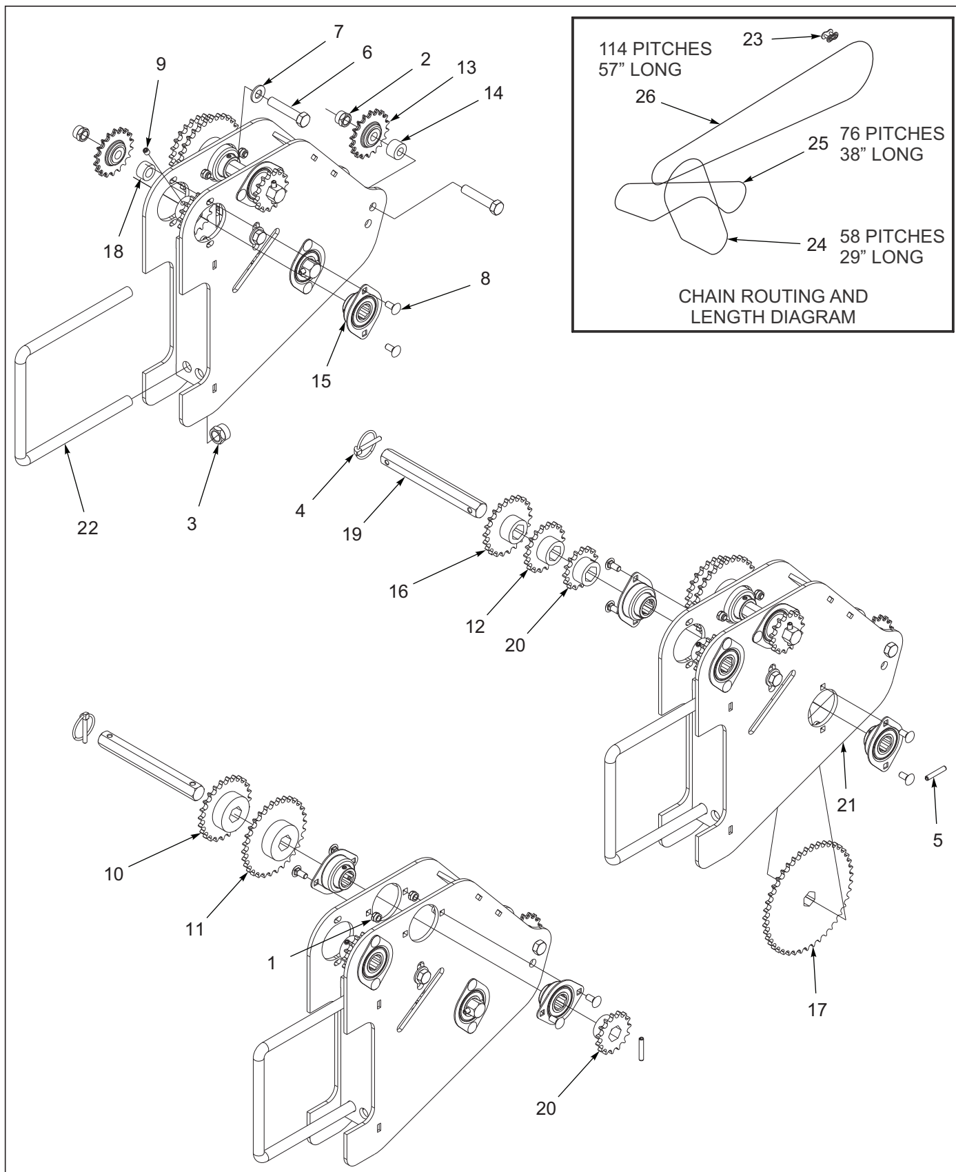
Figure 3-22: Fertilizer Drive Assembly, Left
