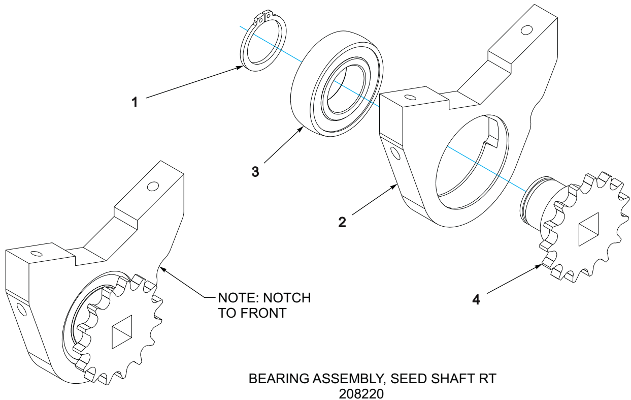
Figure 3-34: Seed Shaft Bearing Assembly (After 12-18-2018)
