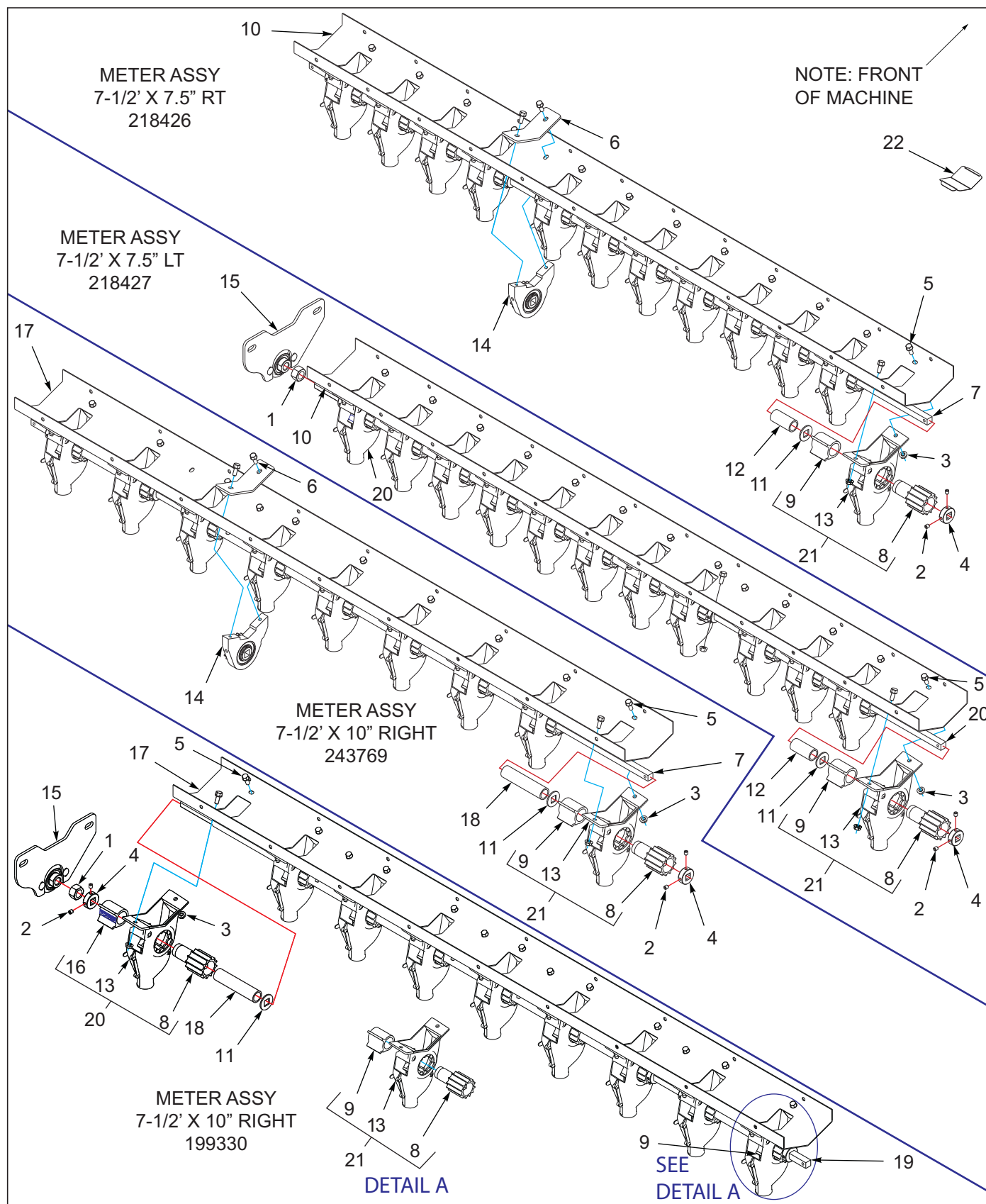
Figure 3-30: Seed Meter Assembly 5211-15'
