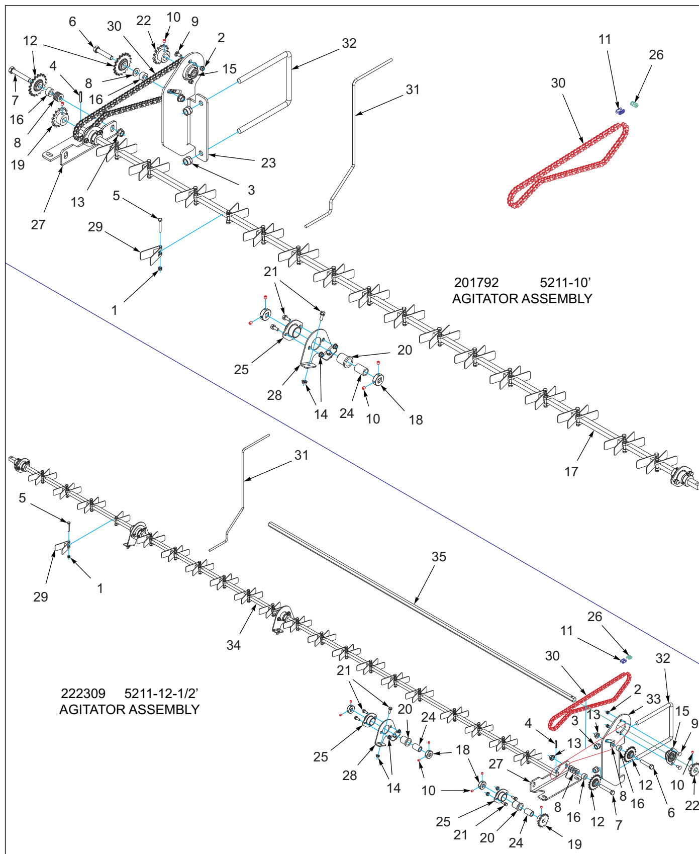
Figure 3-37: Agitator Assembly 5211-10'-12-1/2'
