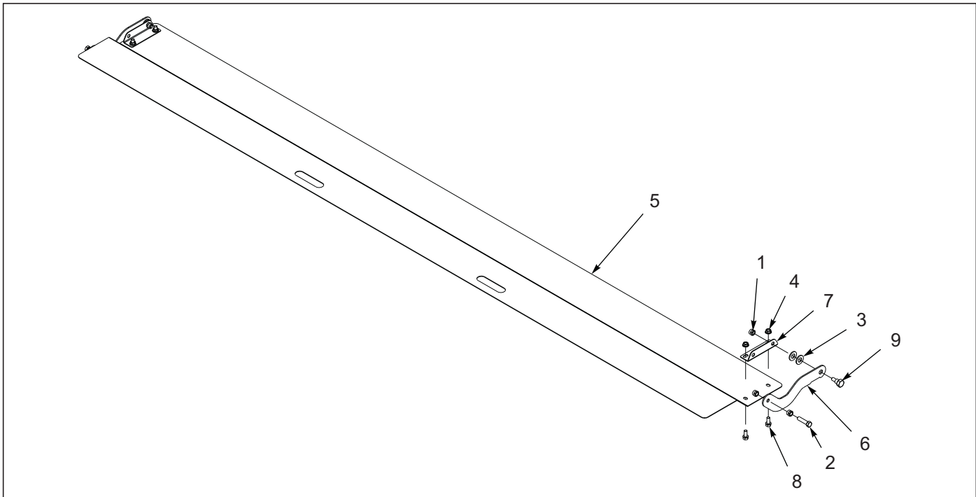
Figure 3-24: Fill Shield Assembly
