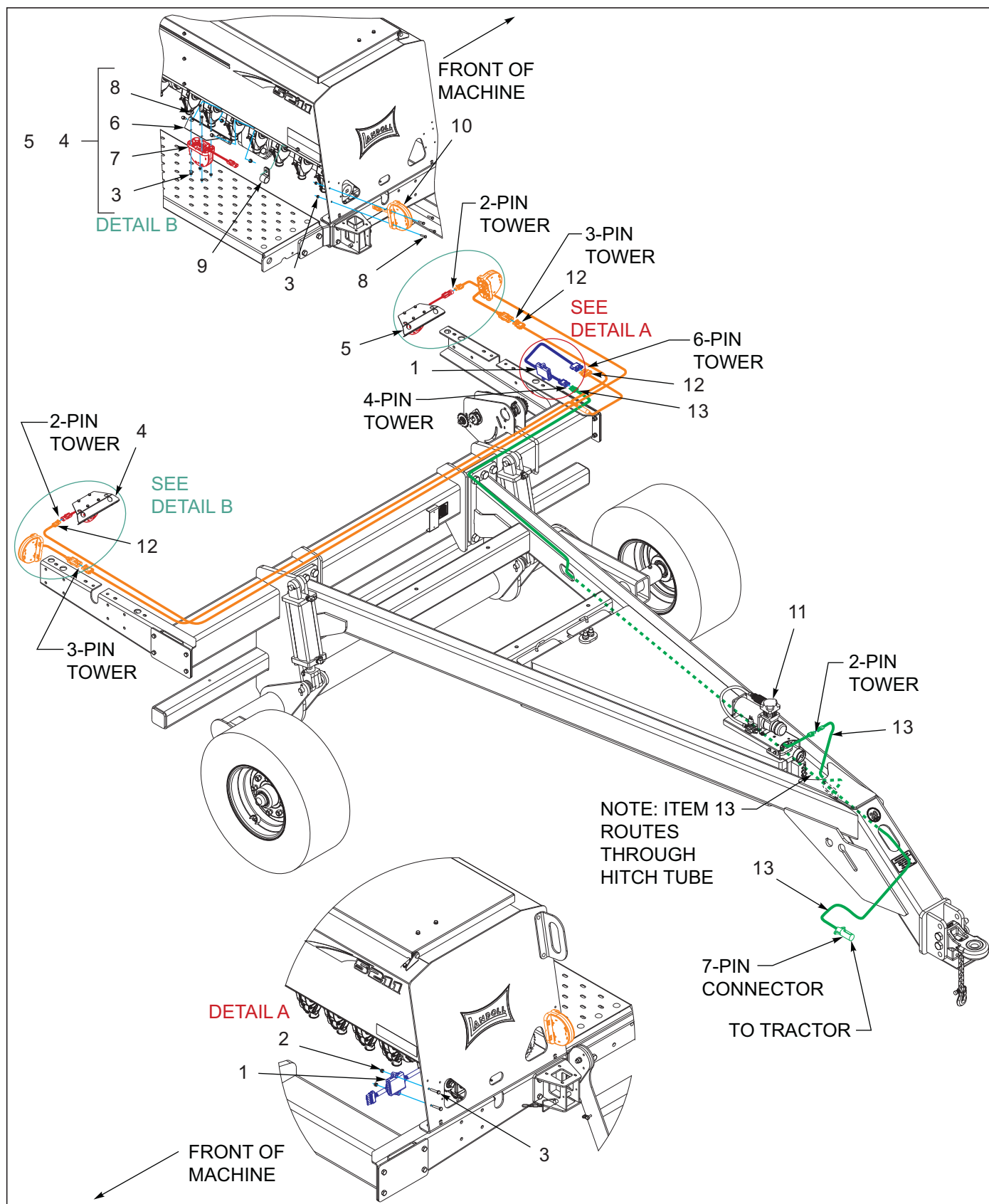
Figure 6-2: Electrical Assembly W/LED Lights 5211-10'-12-1/2' W/Long Hitch
