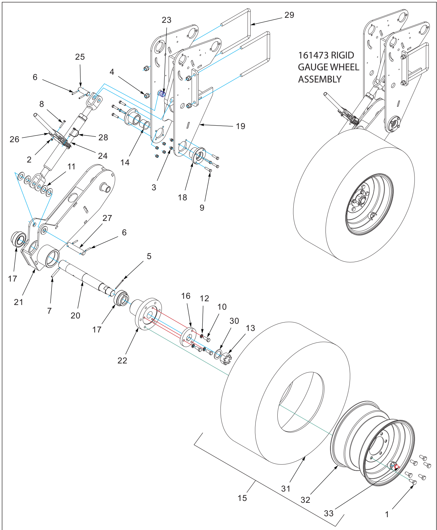
Figure 2-23: Gauge Wheel Assembly, Rigid
