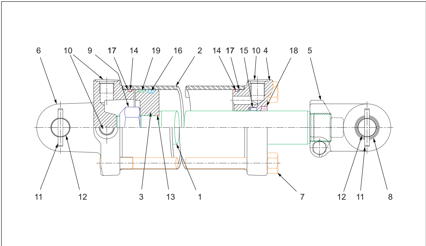
Figure 2-24: 4 x 10" Hydraulic Cylinder
