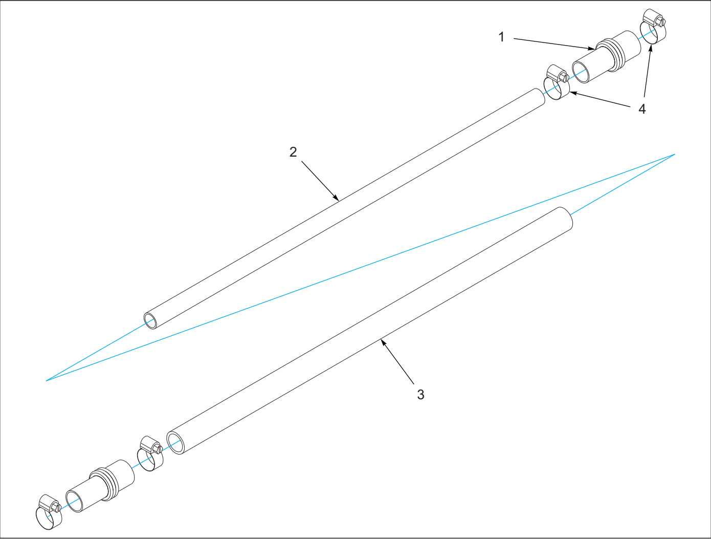
Figure 5-11: Small Tube Assembly, Small
