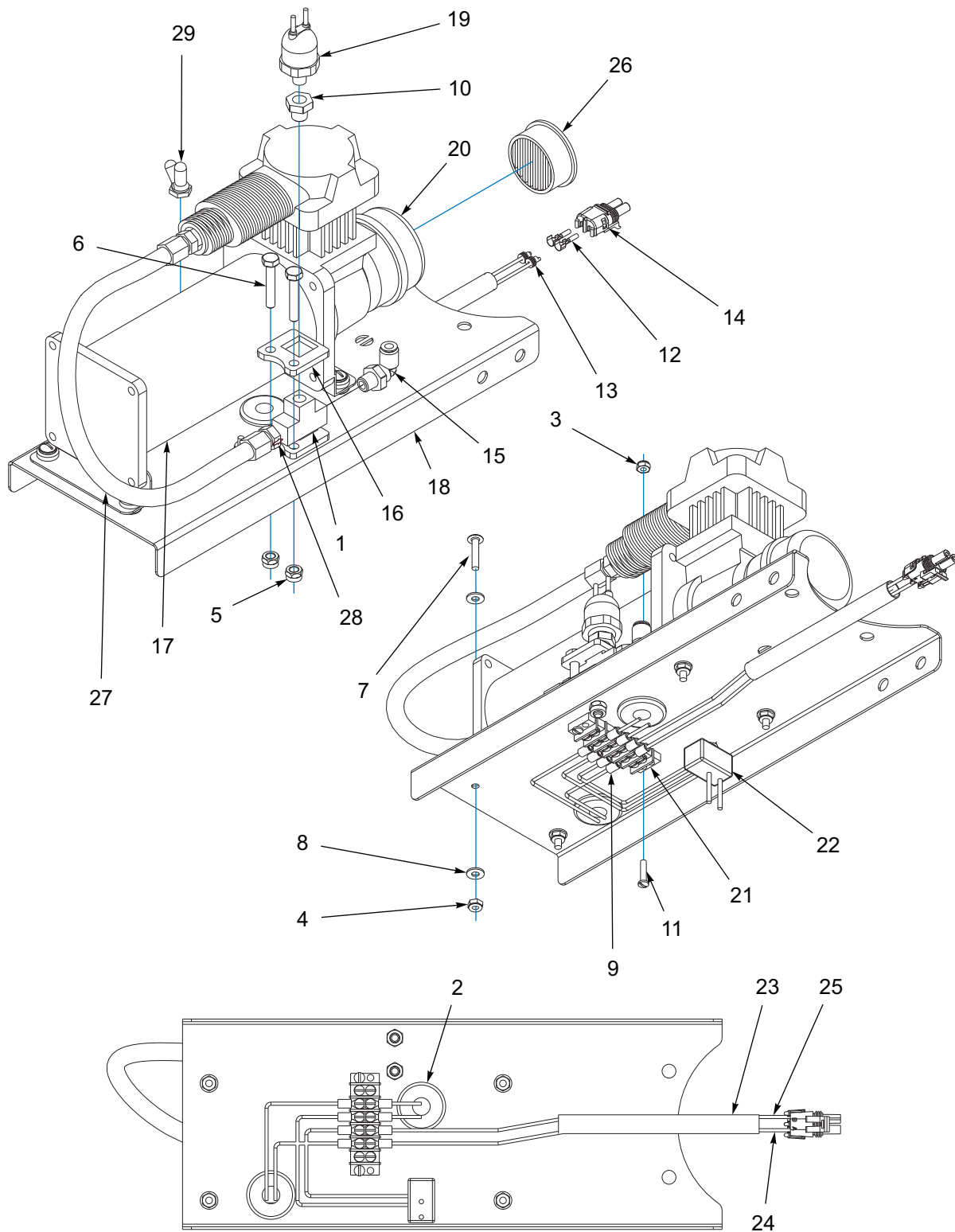
Figure 4-2: 12V Air Compressor Assembly
