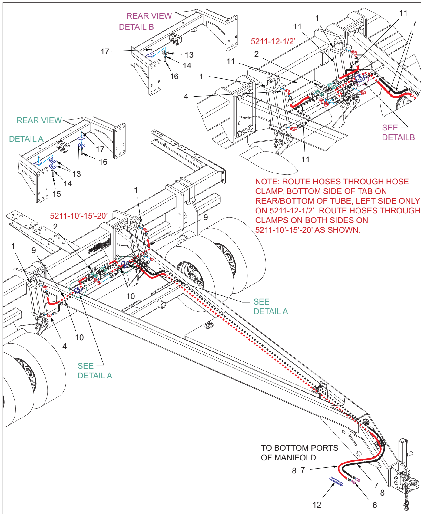
Figure 2-6: Hitch Assembly Lift Hydraulic (1 of 2)
