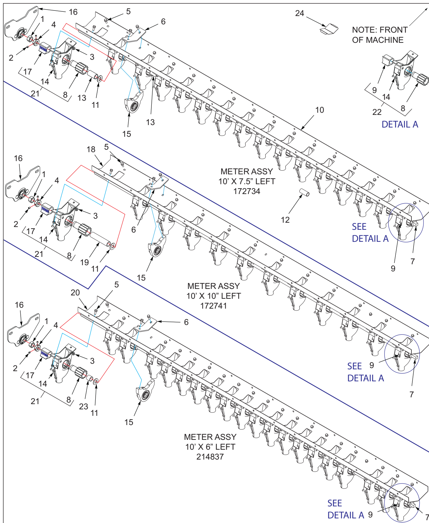
Figure 3-28: Seed Meter Assembly 5211-10'
