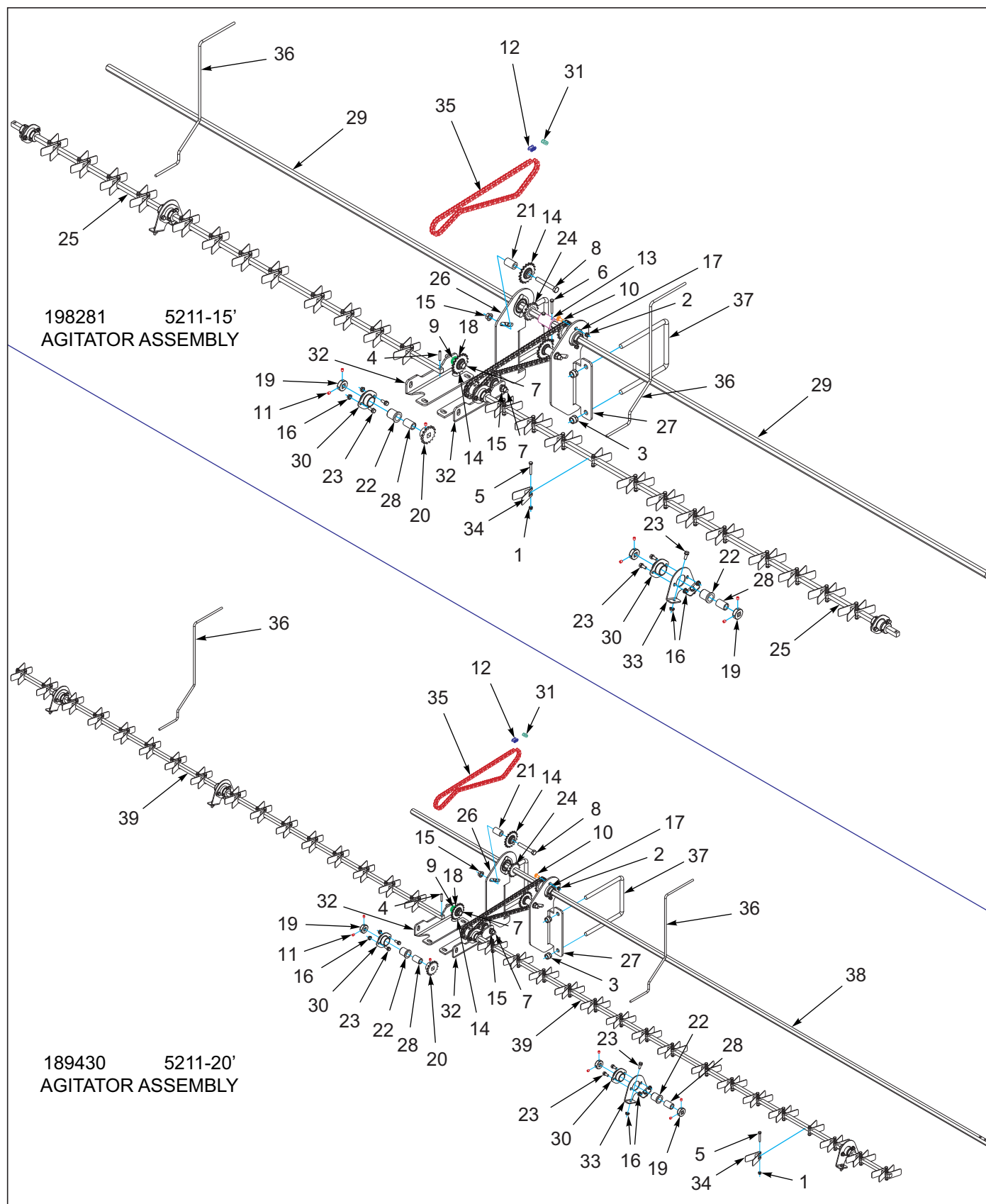
Figure 3-38: Agitator Assembly 5211-15'-20'
