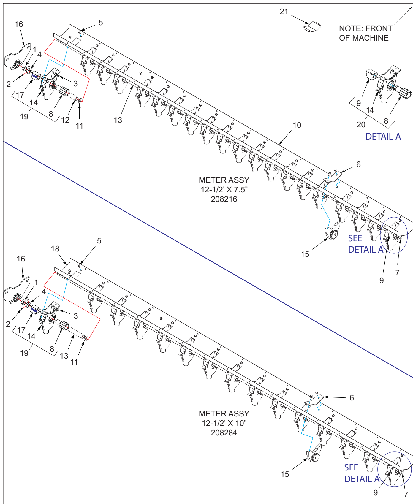
Figure 3-29: Seed Meter Assembly 5211-12-1/2'
