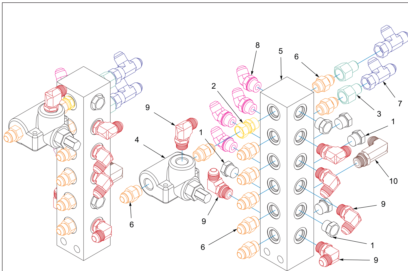
Figure 5-24: Manifold Assembly Front 7531-32'-35' (Before S/N 75K2501921)
