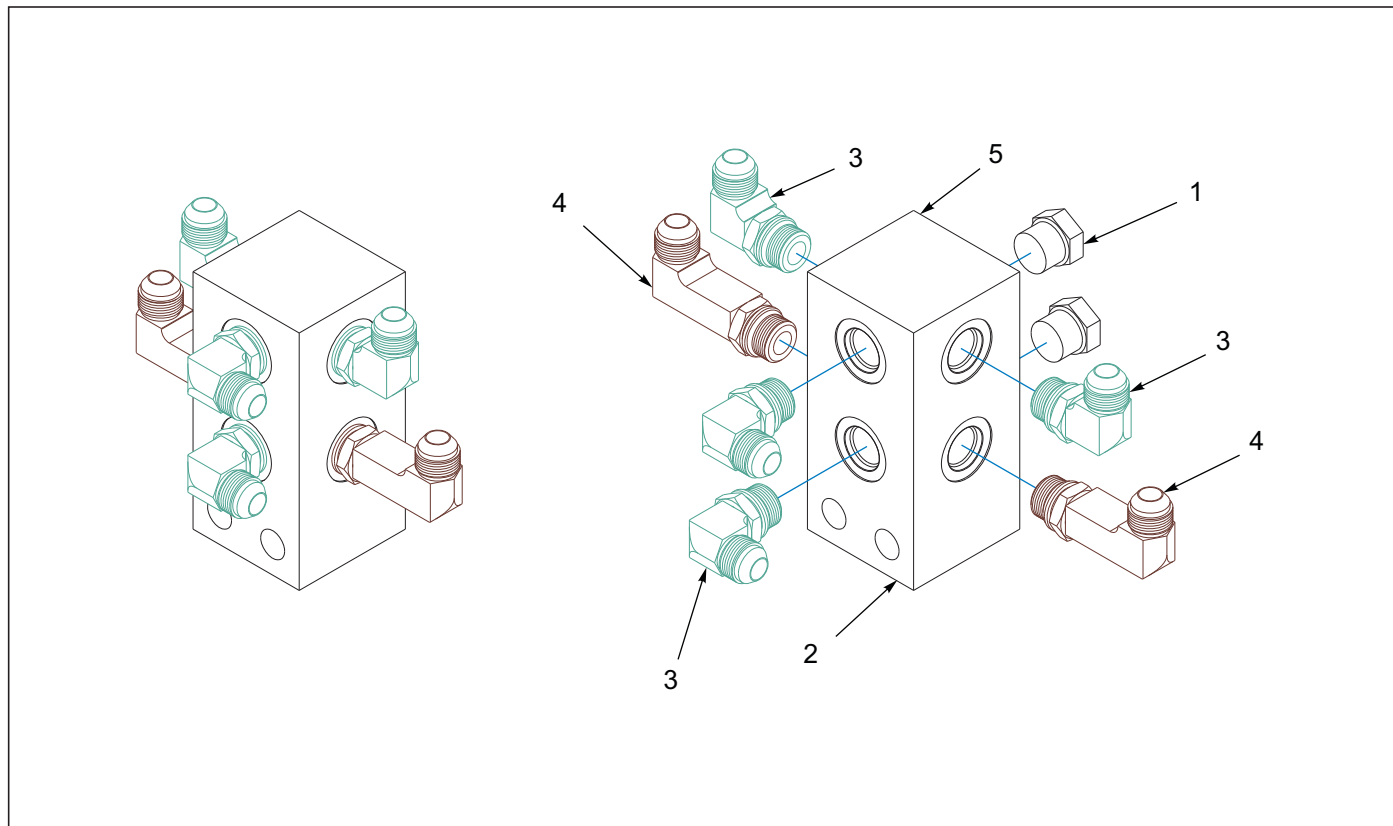
Figure 5-28: Manifold Assembly Rear 7531-32'-35' (After S/N 75K2501921)
