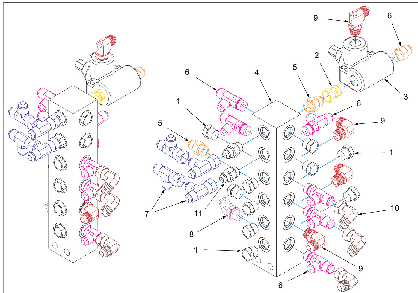
Figure 5-21: Manifold Assembly Front 7531-26'/29' (After S/N 75K2501921)
