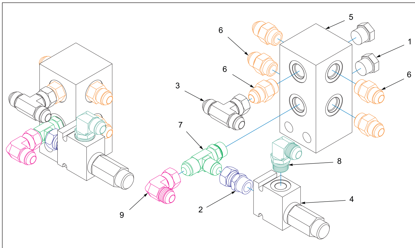
Figure 5-22: Manifold Assembly Front 7531-26'/29' (Before S/N 75K2501921)
