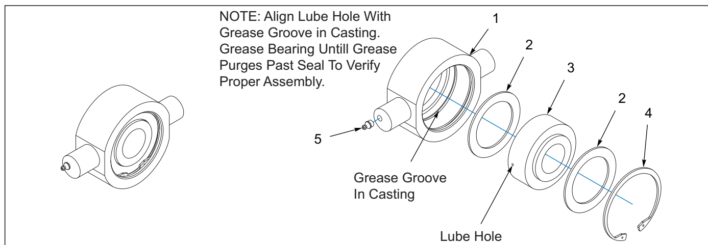
Figure 4-13: Disc Bearing Assembly
