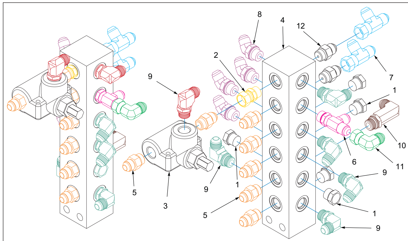
Figure 5-25: Manifold Assembly Front 7531-32'-35' (After S/N 75K2501921)
