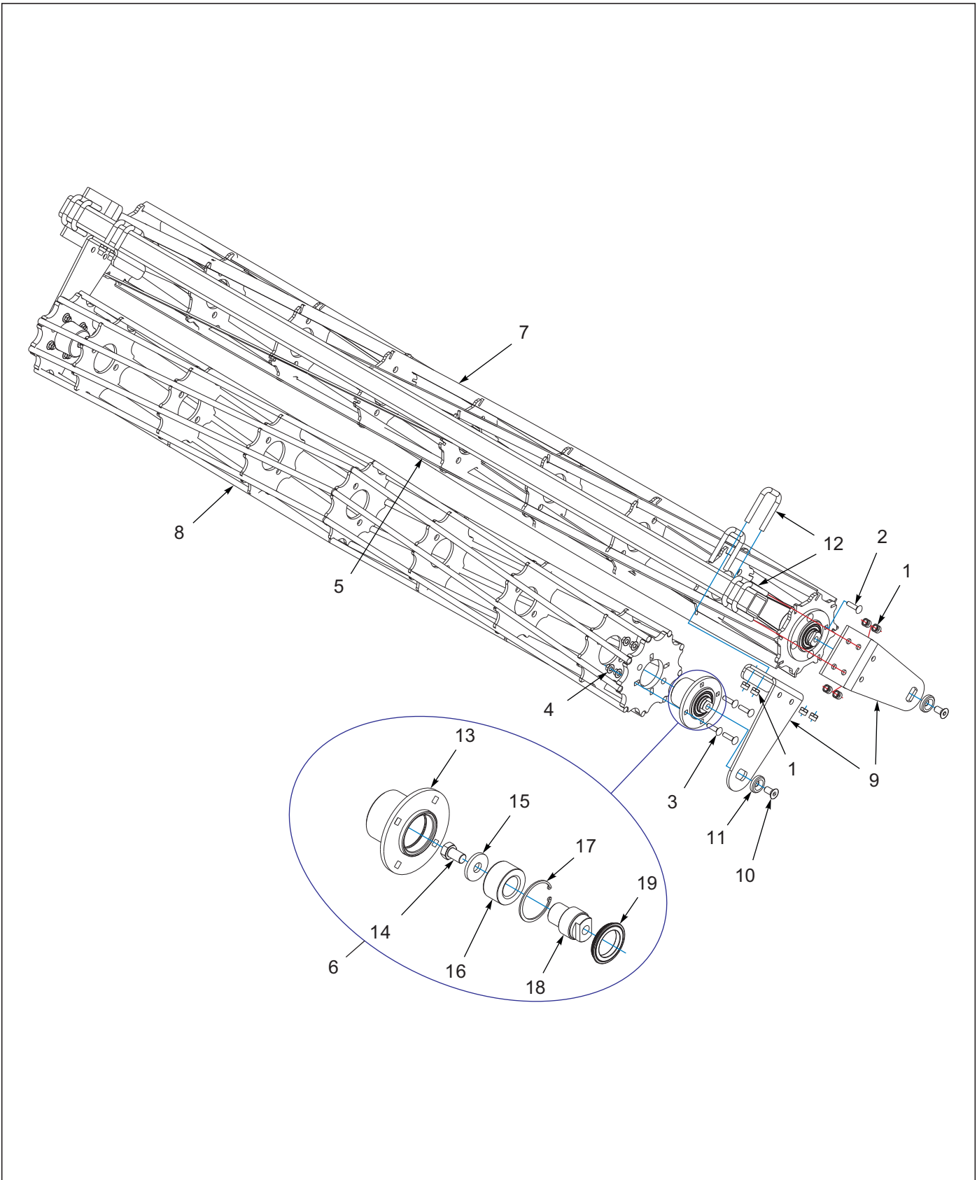
Figure 9-21: Double Flat/RD Reel Assembly 7531-23'-29' Center
