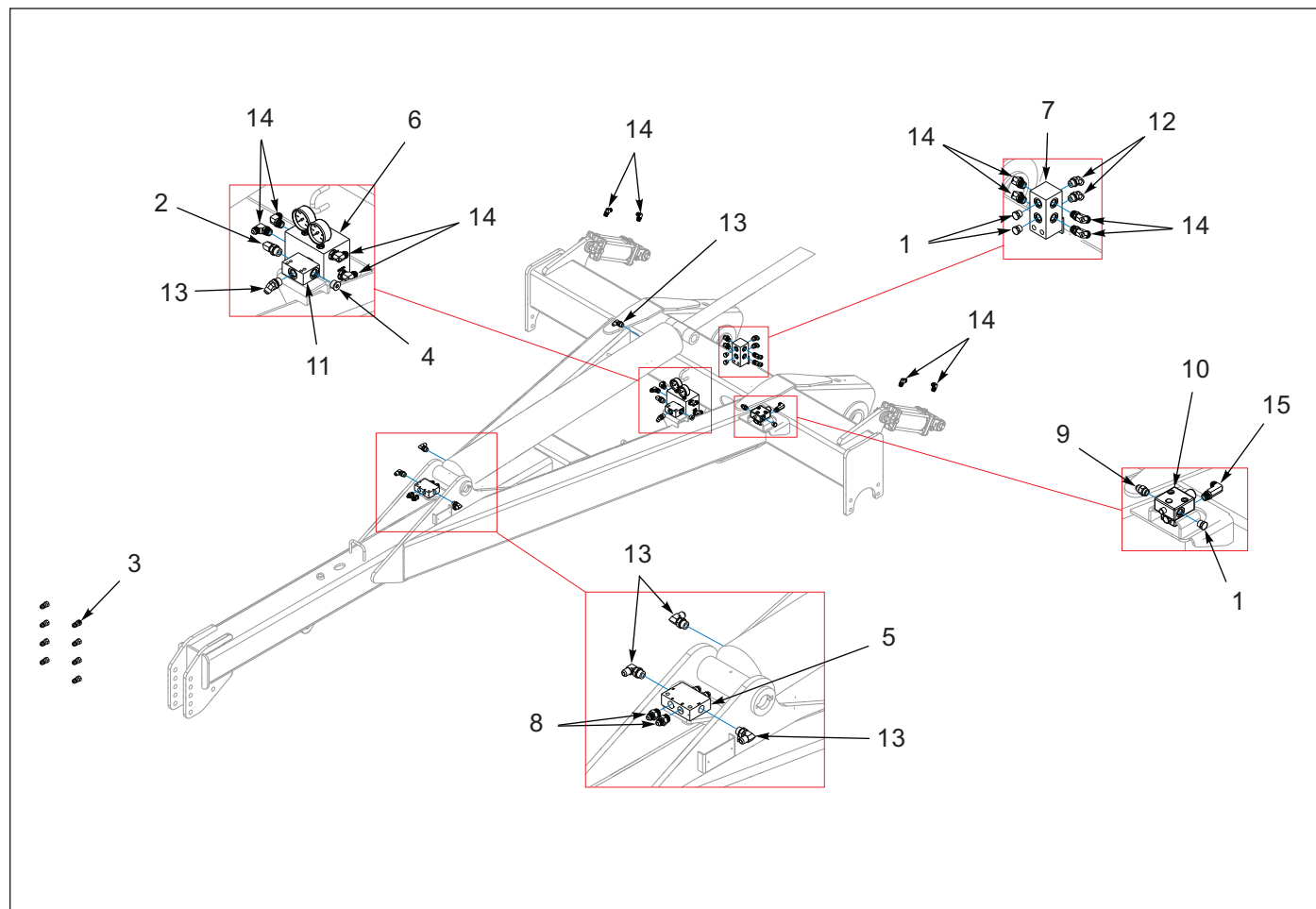
Figure 12-2: Hydraulic Hitch Kit (BEFORE 12/05/2022)
