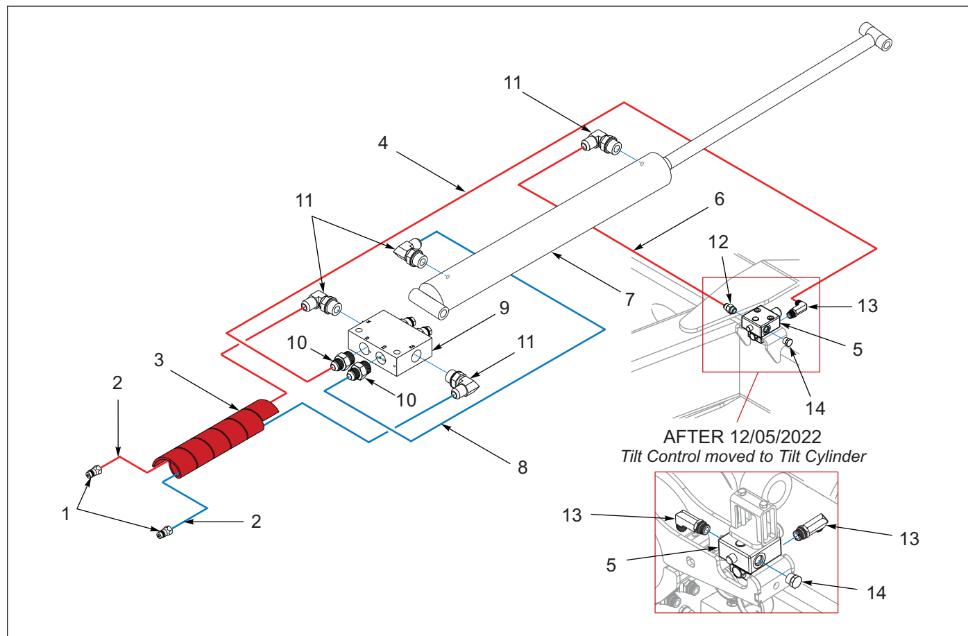
Figure 12-4: Hydraulic System - Tilt Control
