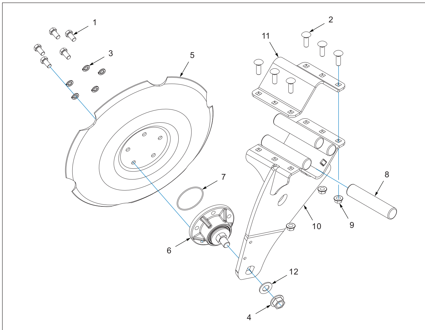
Figure 7-7: Left Disc Assembly - Hybrid
