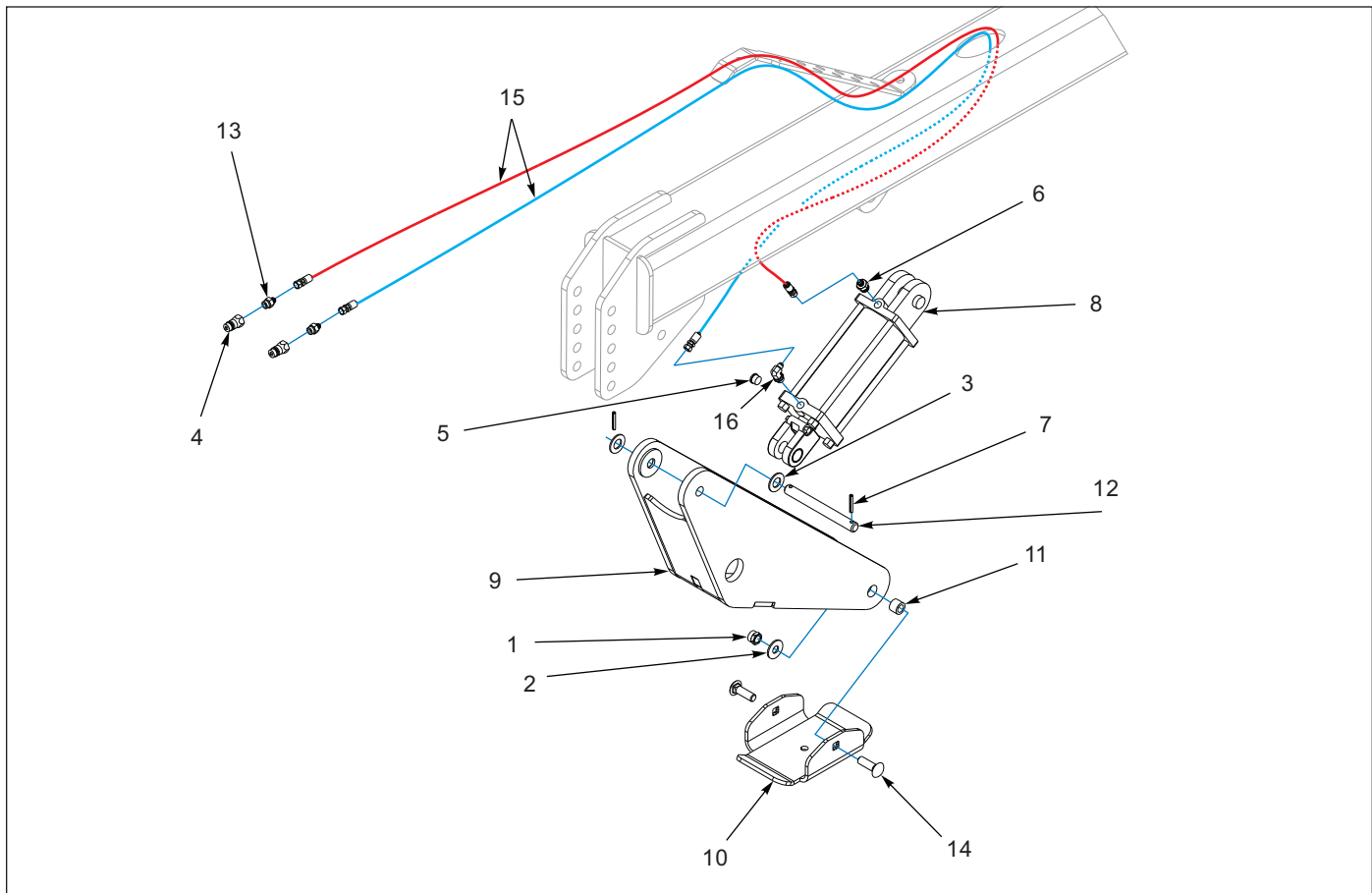
Figure 12-10: Hydraulic Jack Assembly
