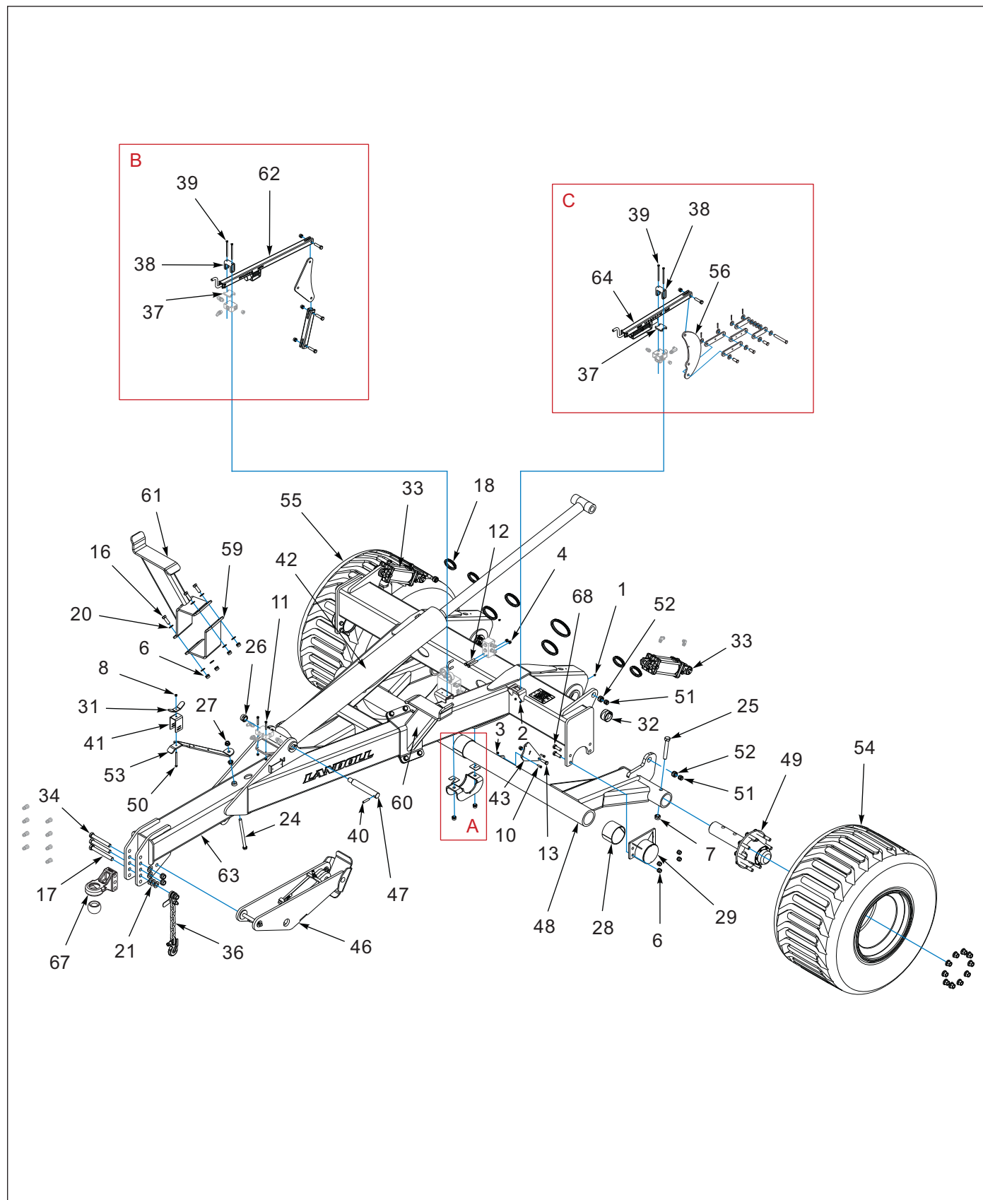
Figure 4-3: Hitch Assemblies (BEFORE 12/2022) (1 of 2)
