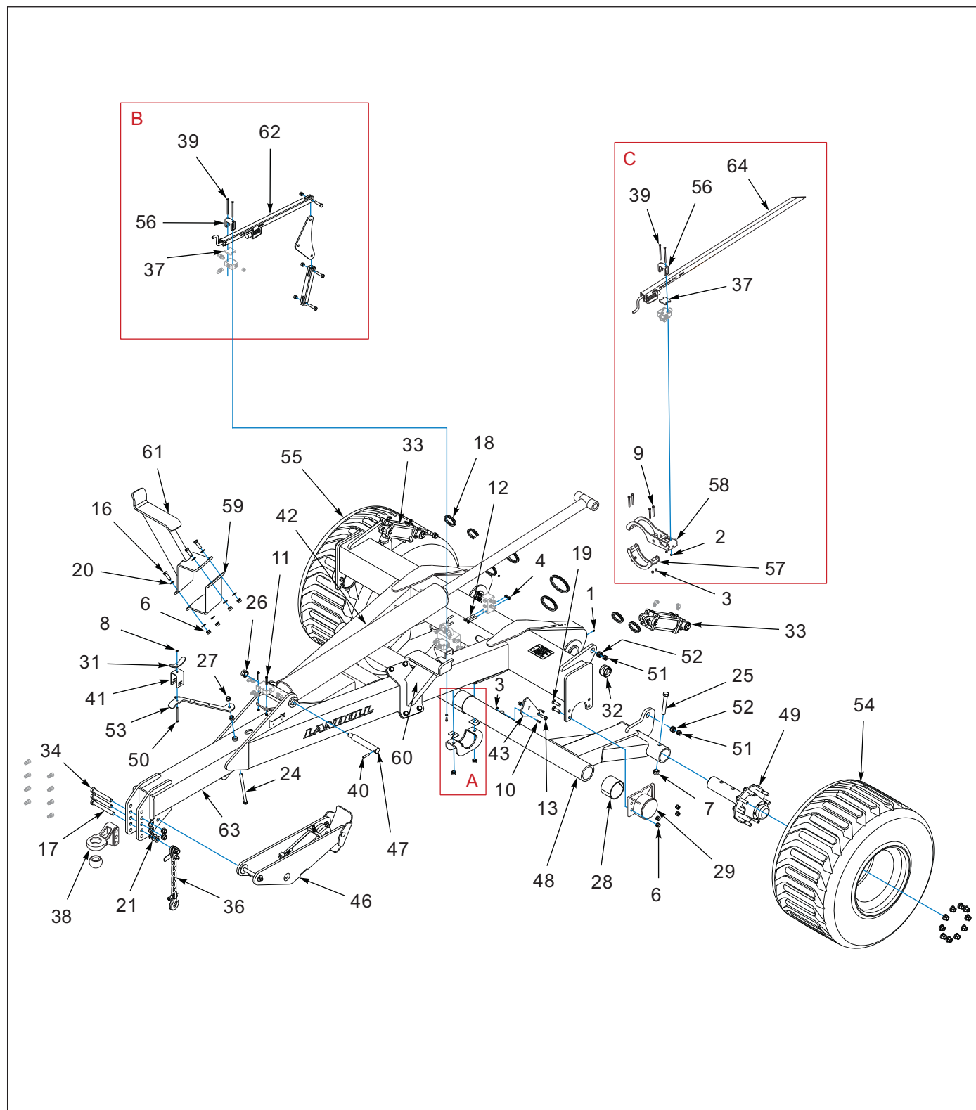
Figure 4-1: Hitch Assemblies (AFTER 12/2022) (1 of 2)
