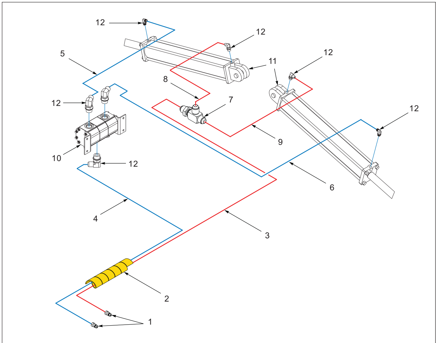
Figure 12-8: Hydraulic System - Wing Fold Down Circuit - 15'
