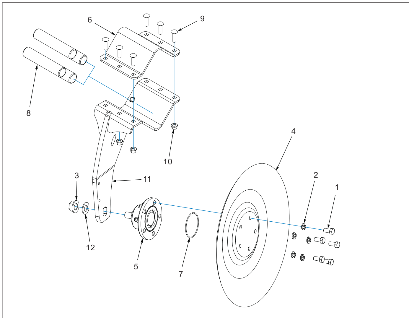
Figure 7-3: Right Disc Assembly - Rollable
