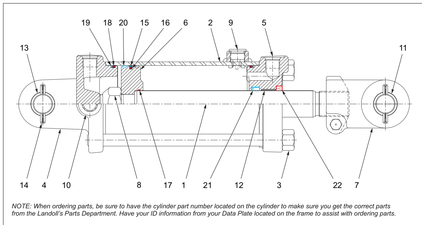
Figure 12-12: Hydraulic Cylinder, 3-3/4 x 10 - 201276
