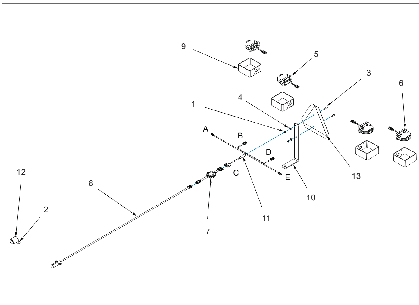
Figure 13-2: Electrical Assembly (2 of 2)
