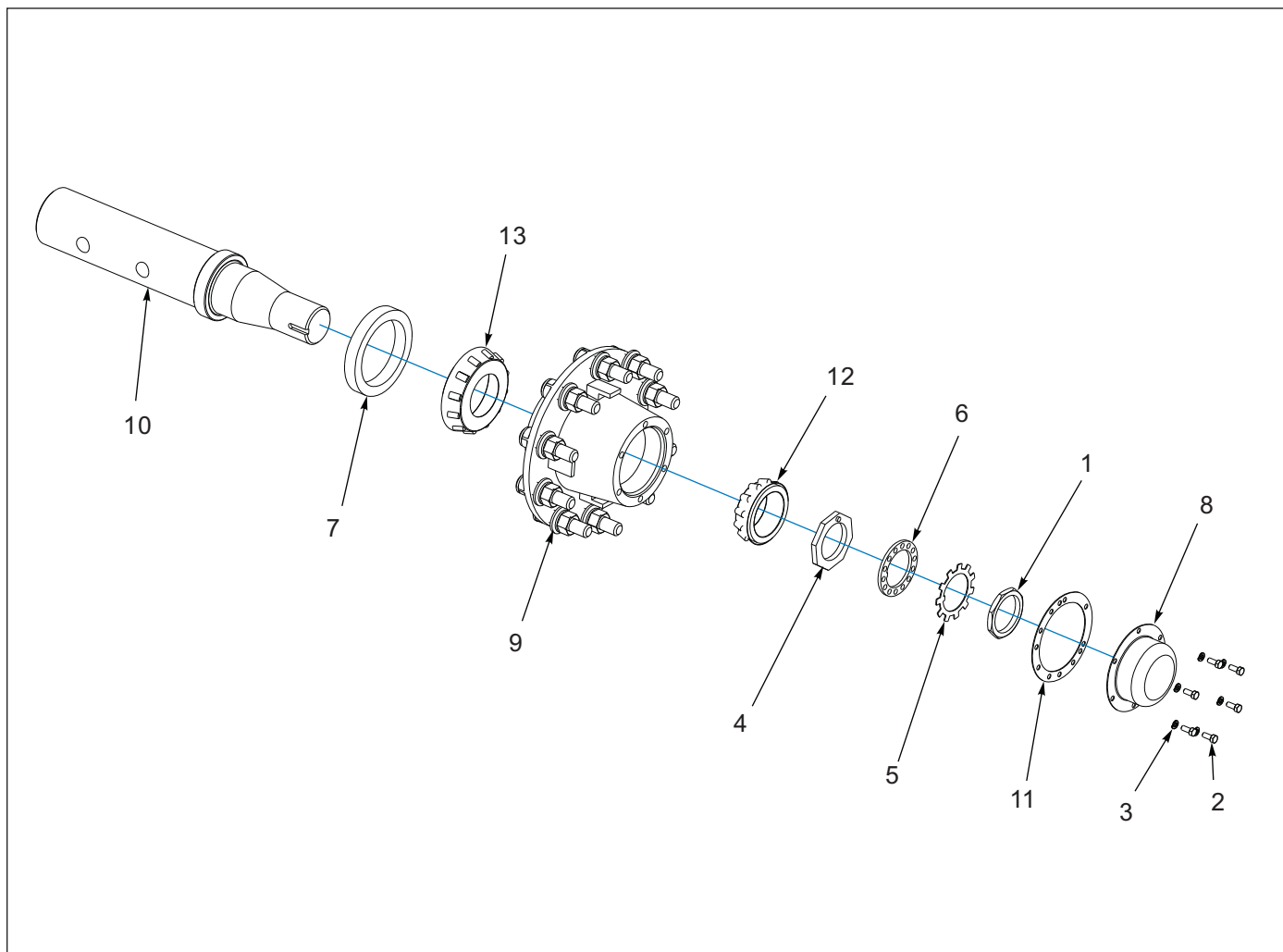
Figure 3-3: Hub and Spindle Assembly, 10 Bolt - 193814 (BEFORE 05/27/2020)
