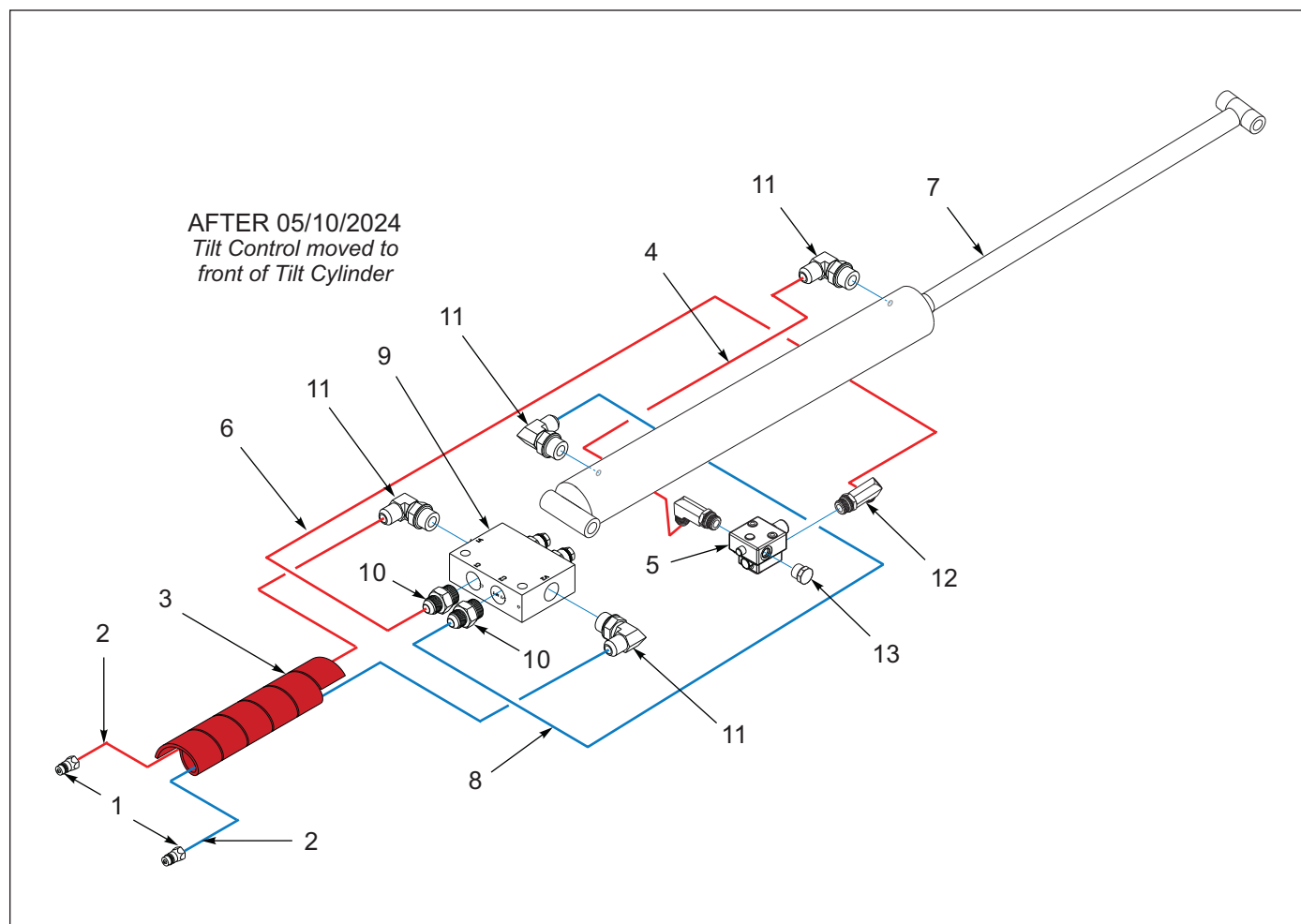
Figure 12-3: Hydraulic System - Tilt Control
