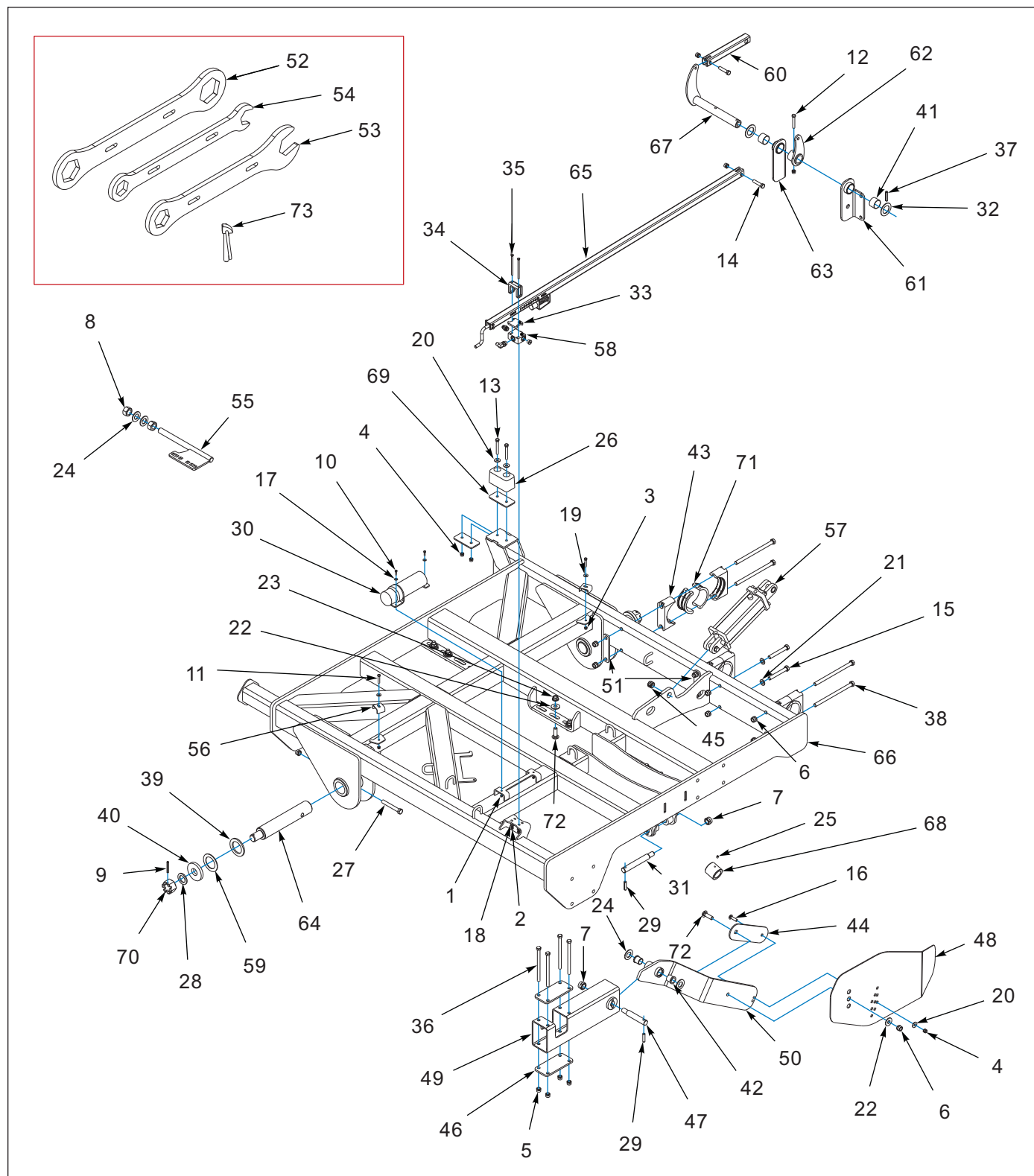
Figure 2-1: Wing Assembly - Left Hand 15'
