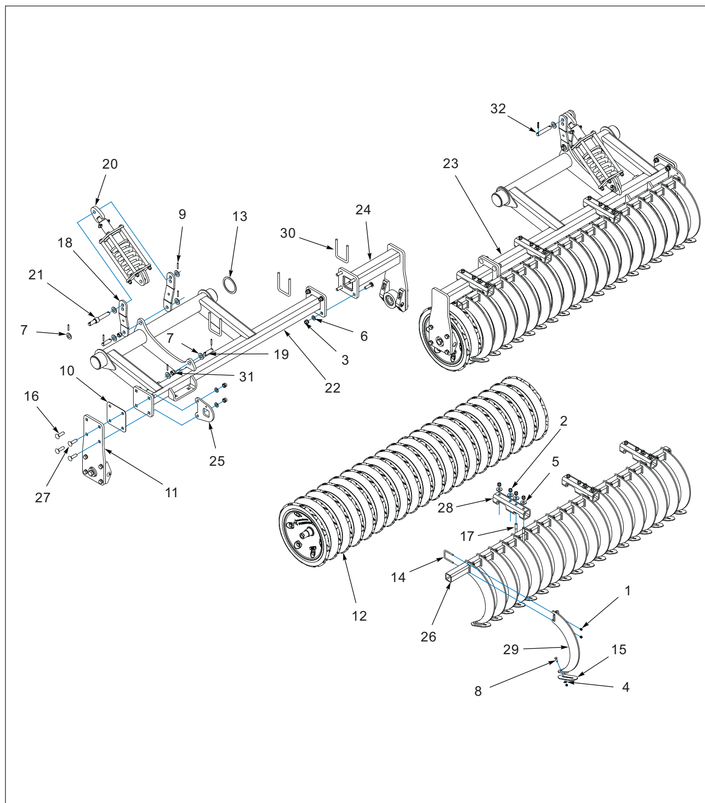
Figure 11-1: Rubber Roller Assembly - 15'
