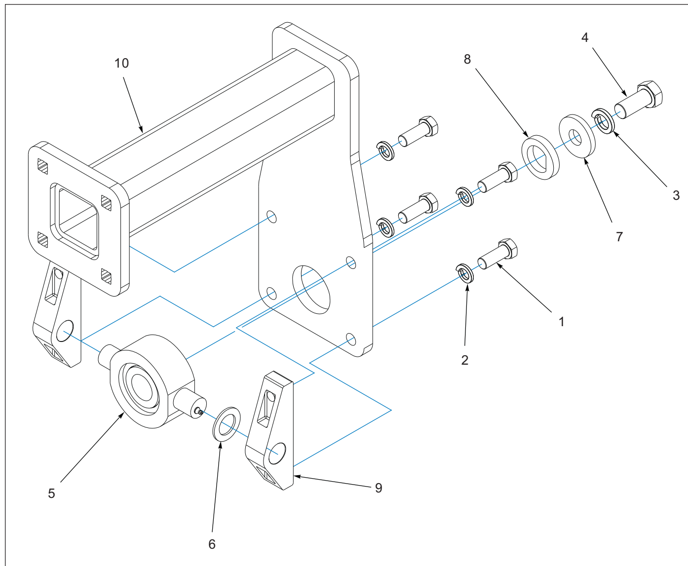
Figure 11-6: Reel Mount Extension Assembly
