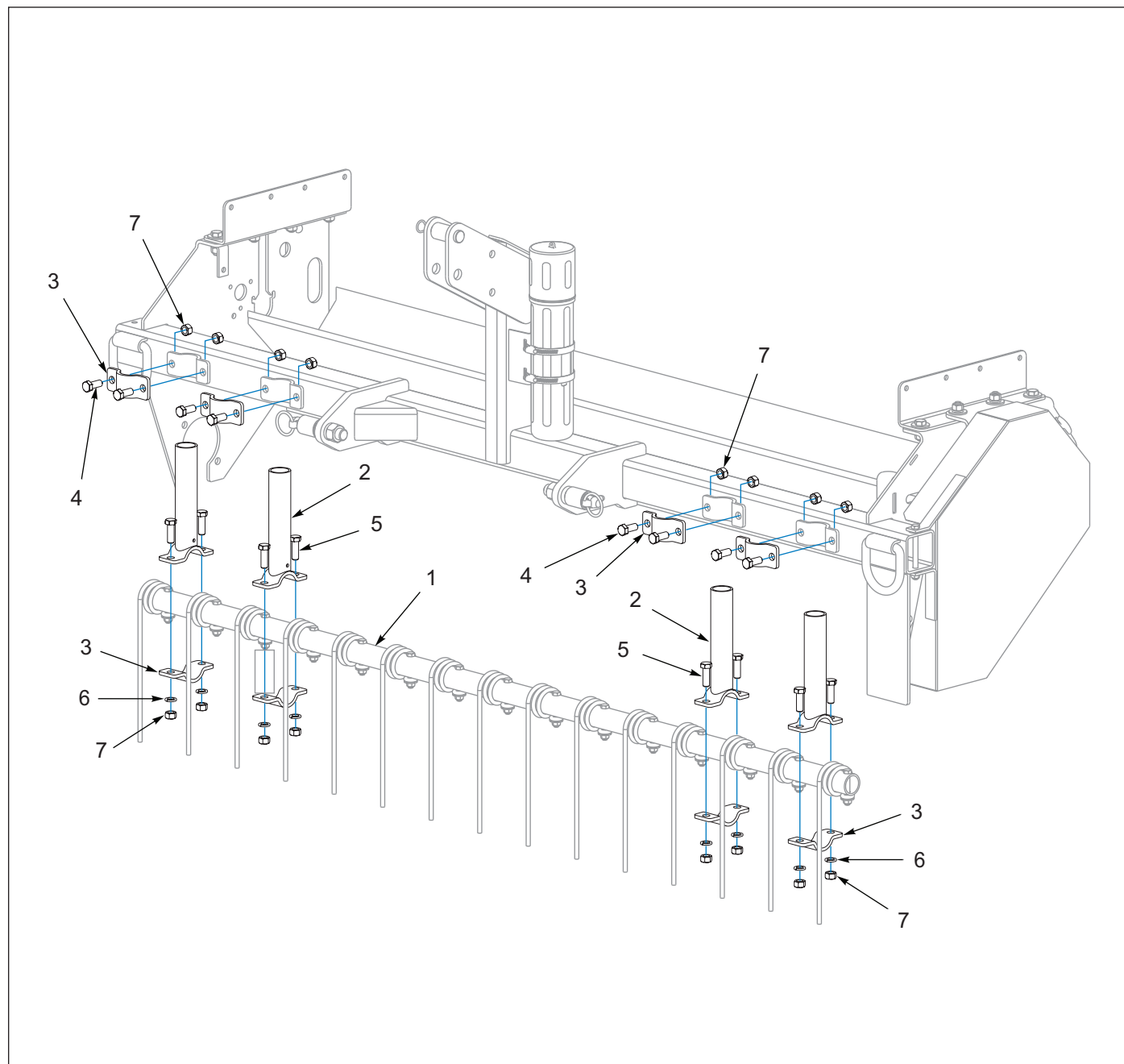
Figure 1-5: Coil Tine Harrow, 6FT (Full Width)
