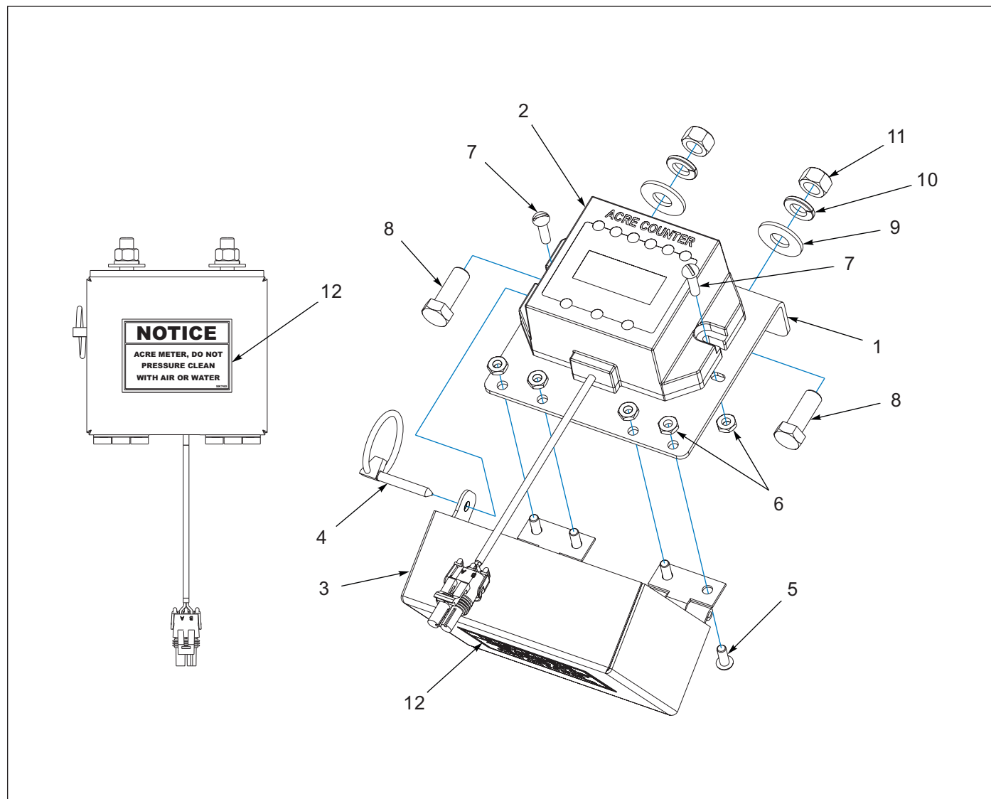
Figure 1-29: Acre Meter Assembly (05/15/2012 TO 06/01/2025)
