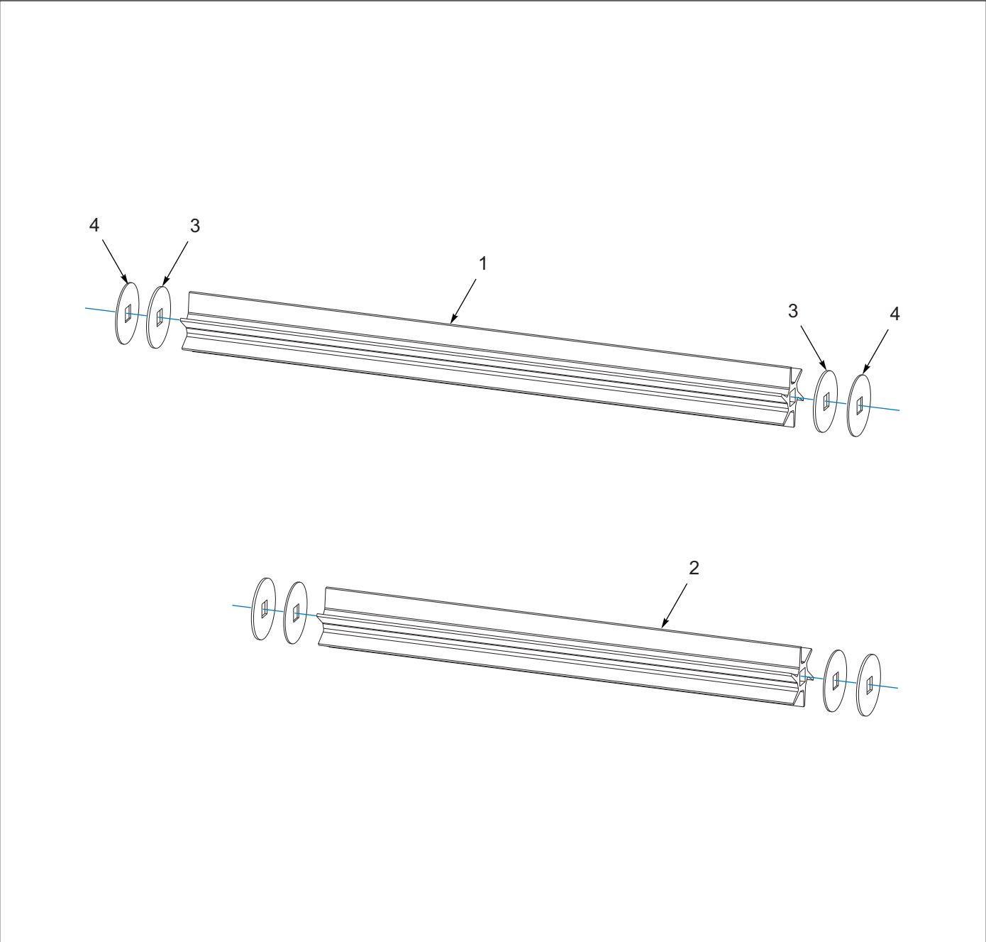
Figure 1-21: Blade Agitator Kit - Optional
