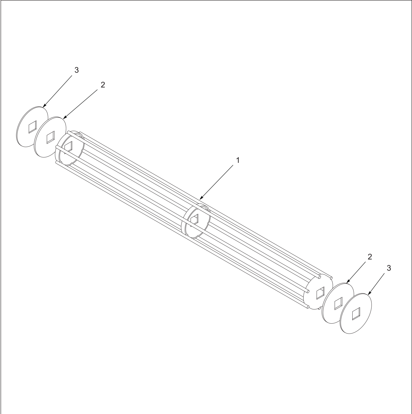
Figure 1-26: Cage Agitator - Optional
