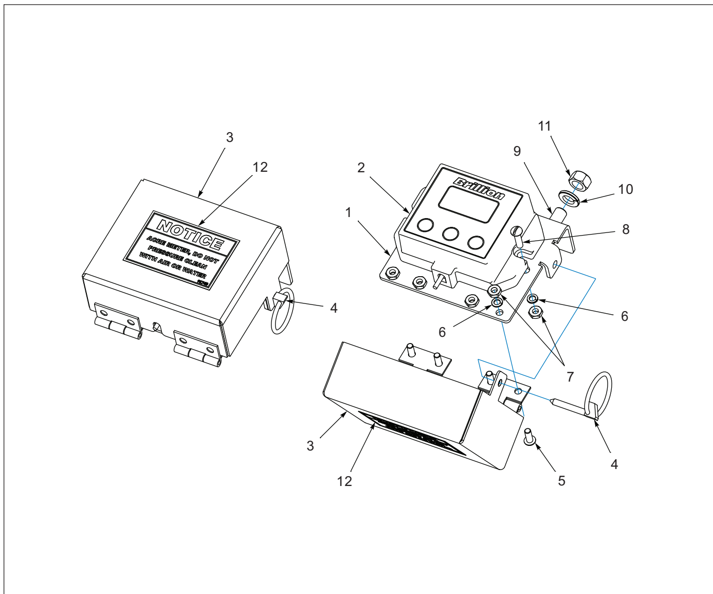
Figure 1-30: Acre Meter Assembly (Before 05/15/2012)
