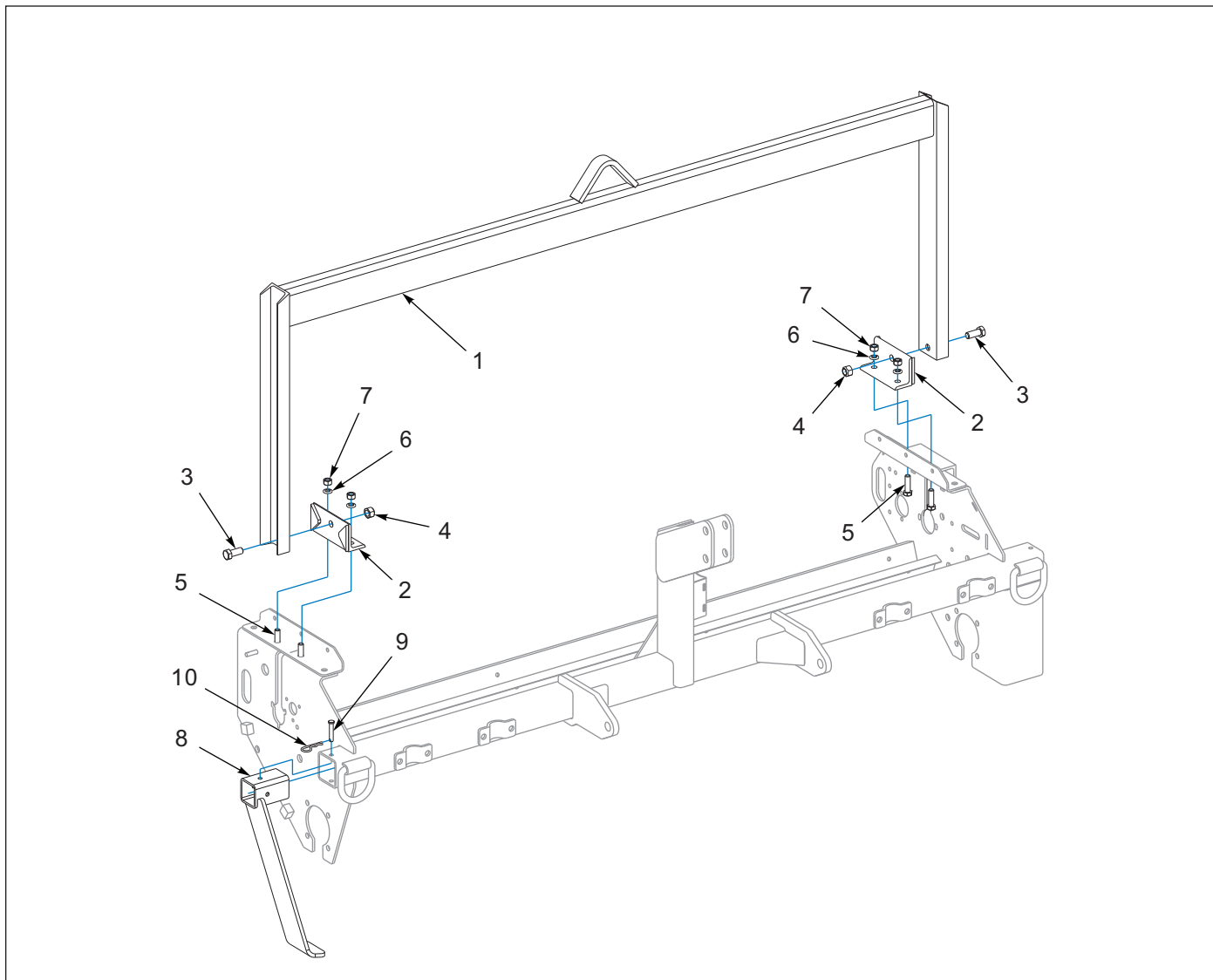
Figure 1-32: Lift Sling Kit - Optional
