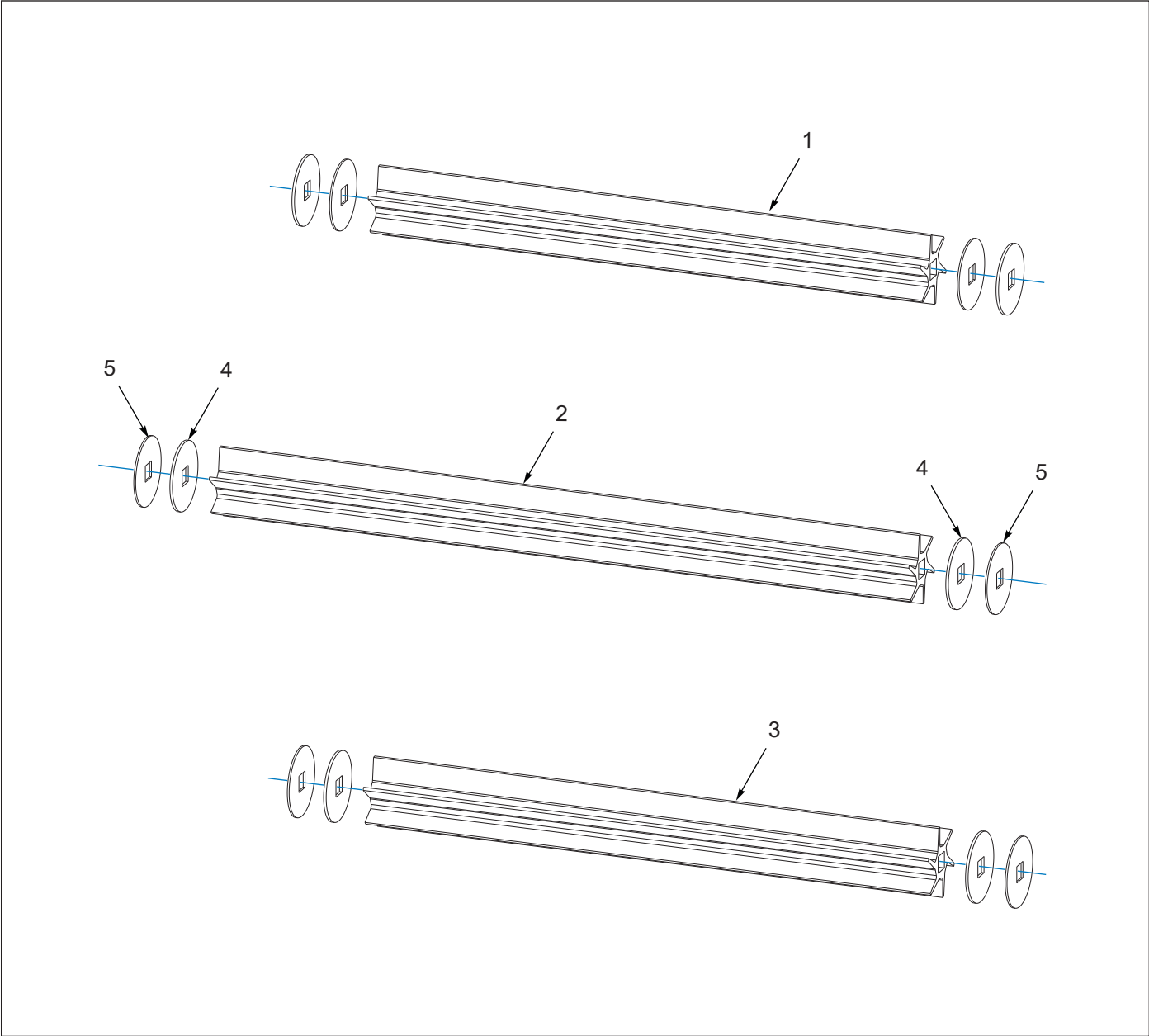
Figure 1-28: Blade Agitator Kit - Optional
