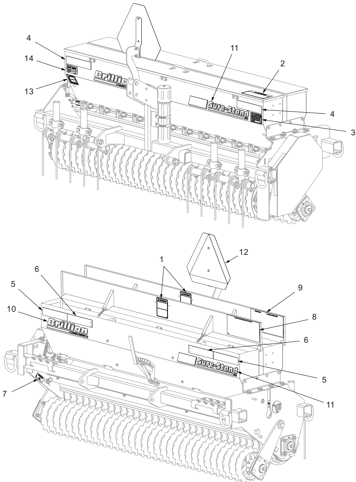
Figure 1-44: SSB6S Decal Locations (Skid Steer) (After 12/2023)
