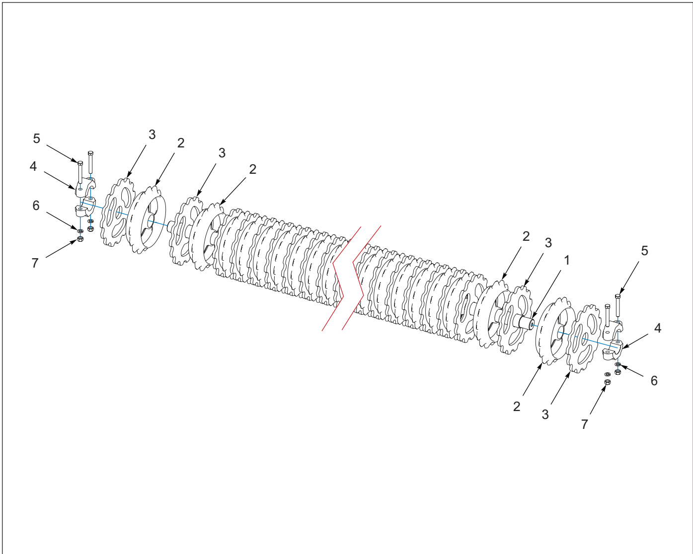
Figure 1-15: Rear Roller w/ Sprocket Assembly
