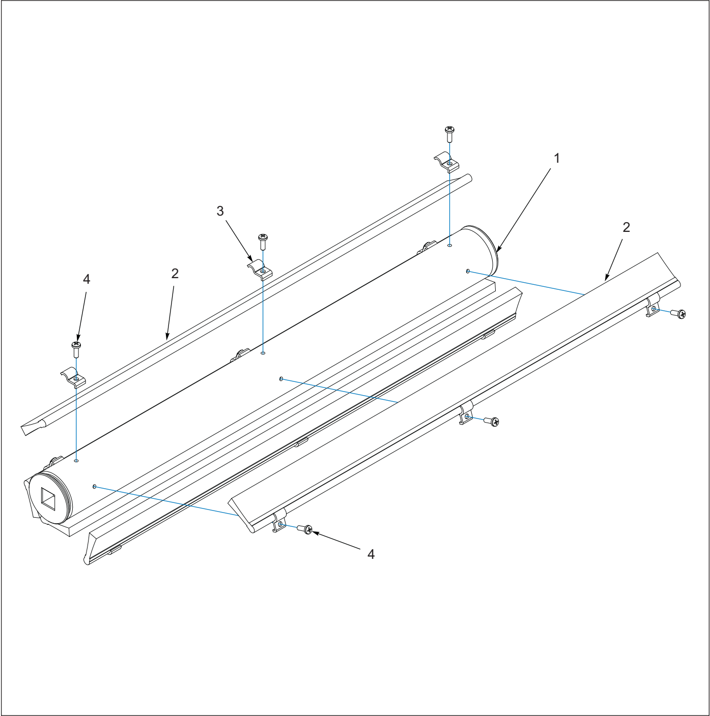
Figure 1-31: Brush Agitator Assembly - 22-1/2"
