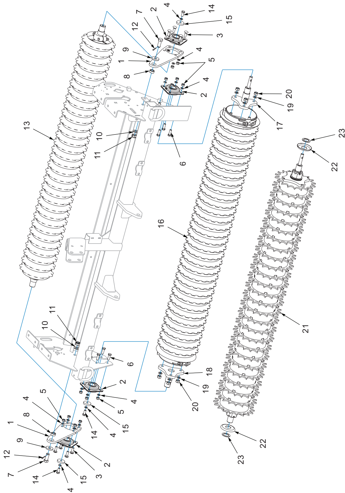
Figure 1-10: Front and Rear Roller Assemblies
