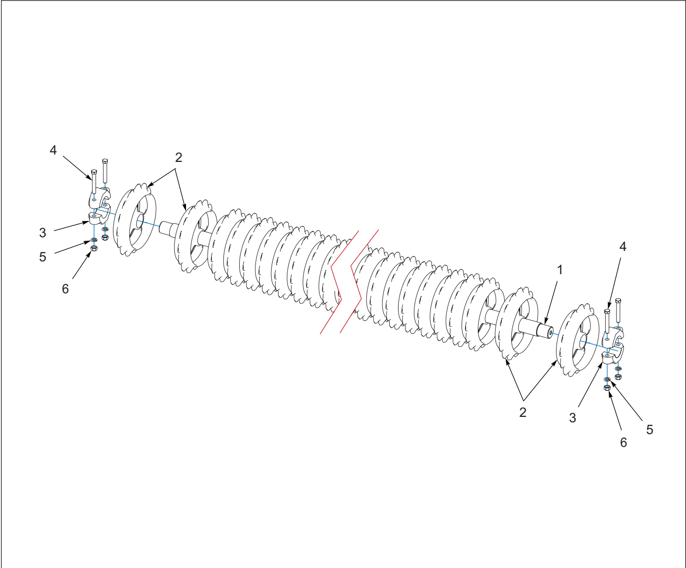
Figure 1-14: Rear Roller Assembly
