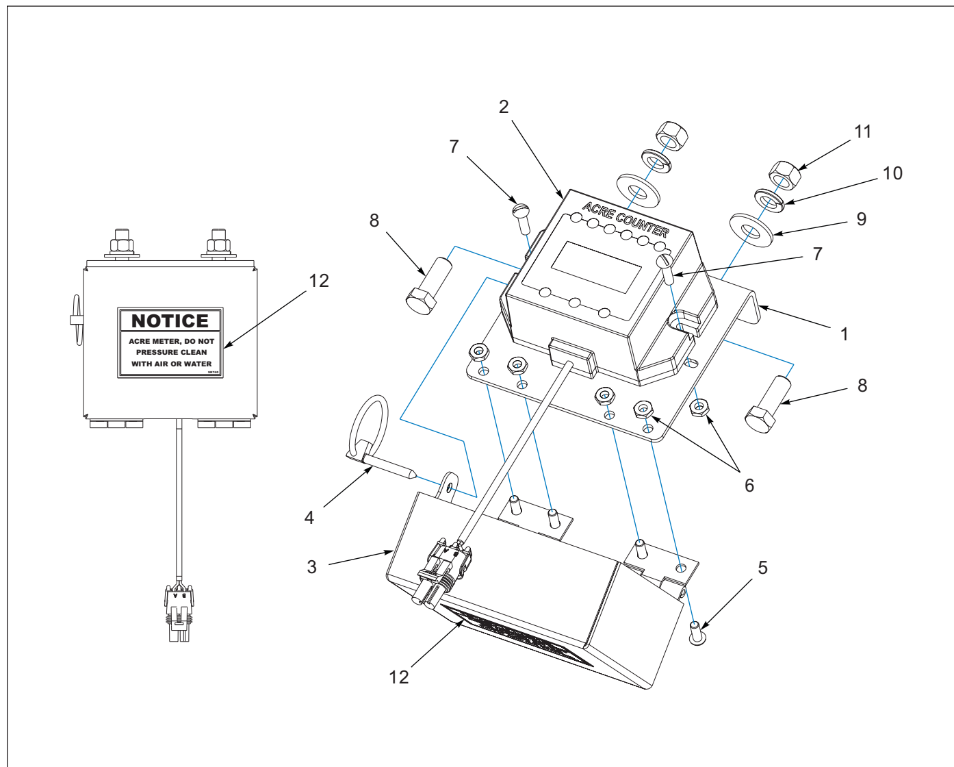
Figure 1-37: Acre Meter Assembly (05/15/2012 TO 06/01/2025)
