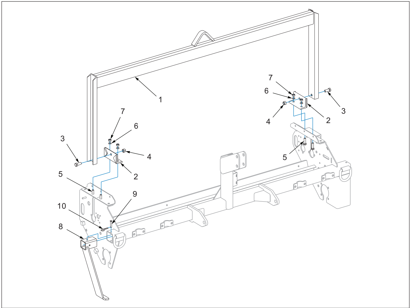
Figure 1-40: Lift Sling Kit - Optional
