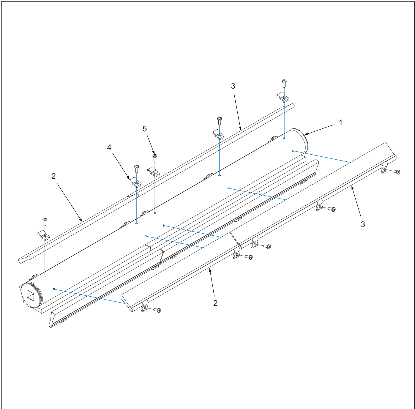
Figure 1-30: Brush Agitator Assembly - 28"
