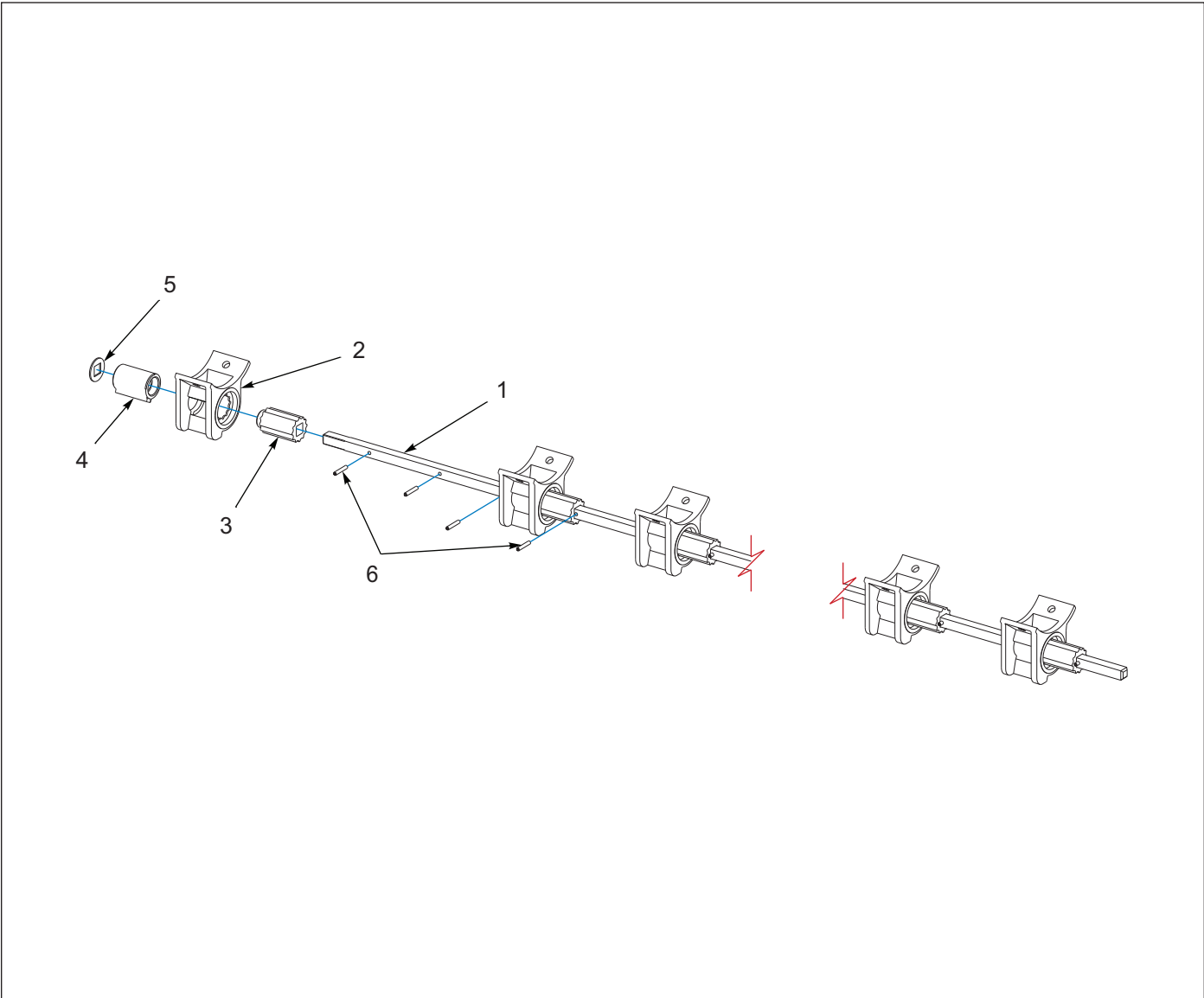
Figure 1-25: Meter Box Seed Shaft
