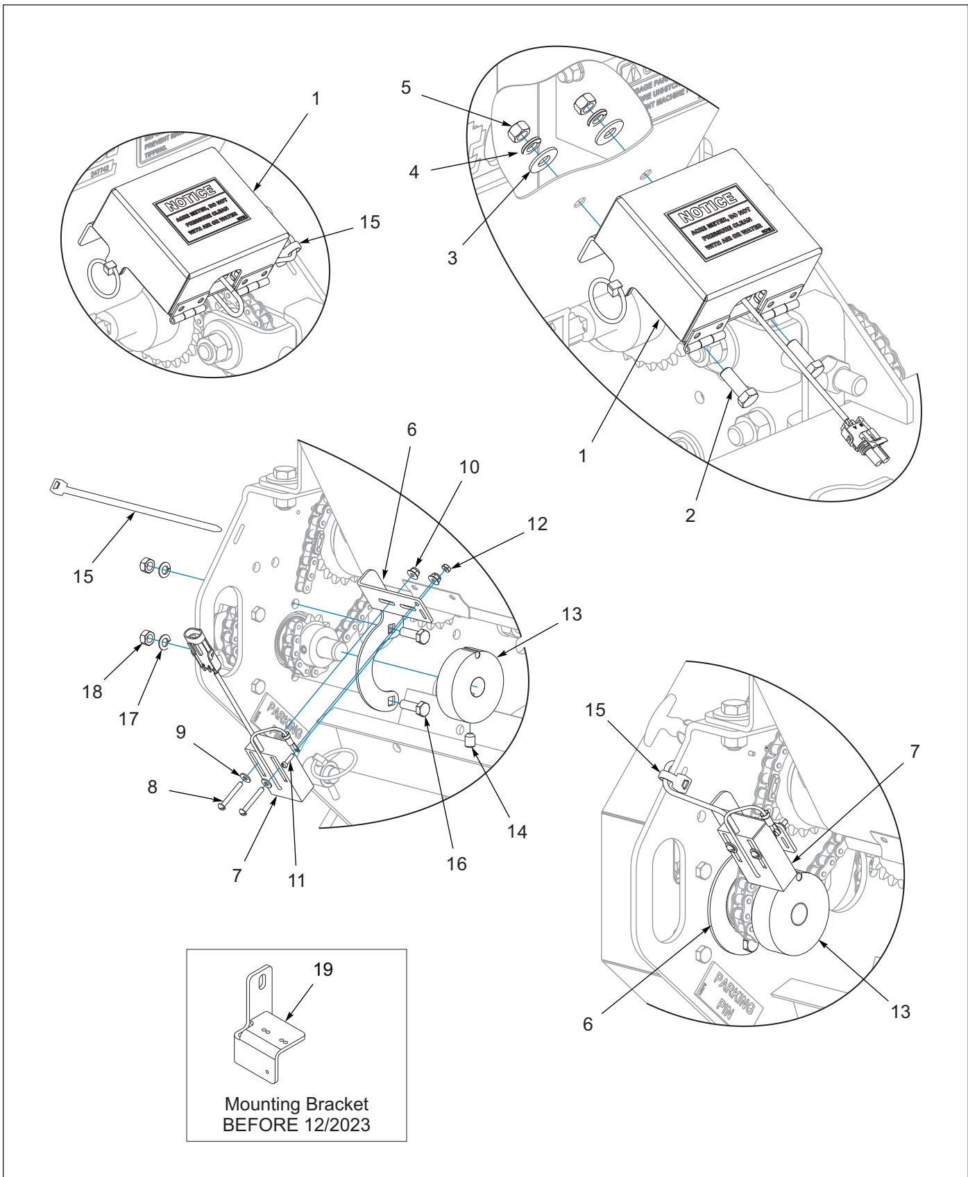
Figure 1-35: Acre Meter Kit - Optional
