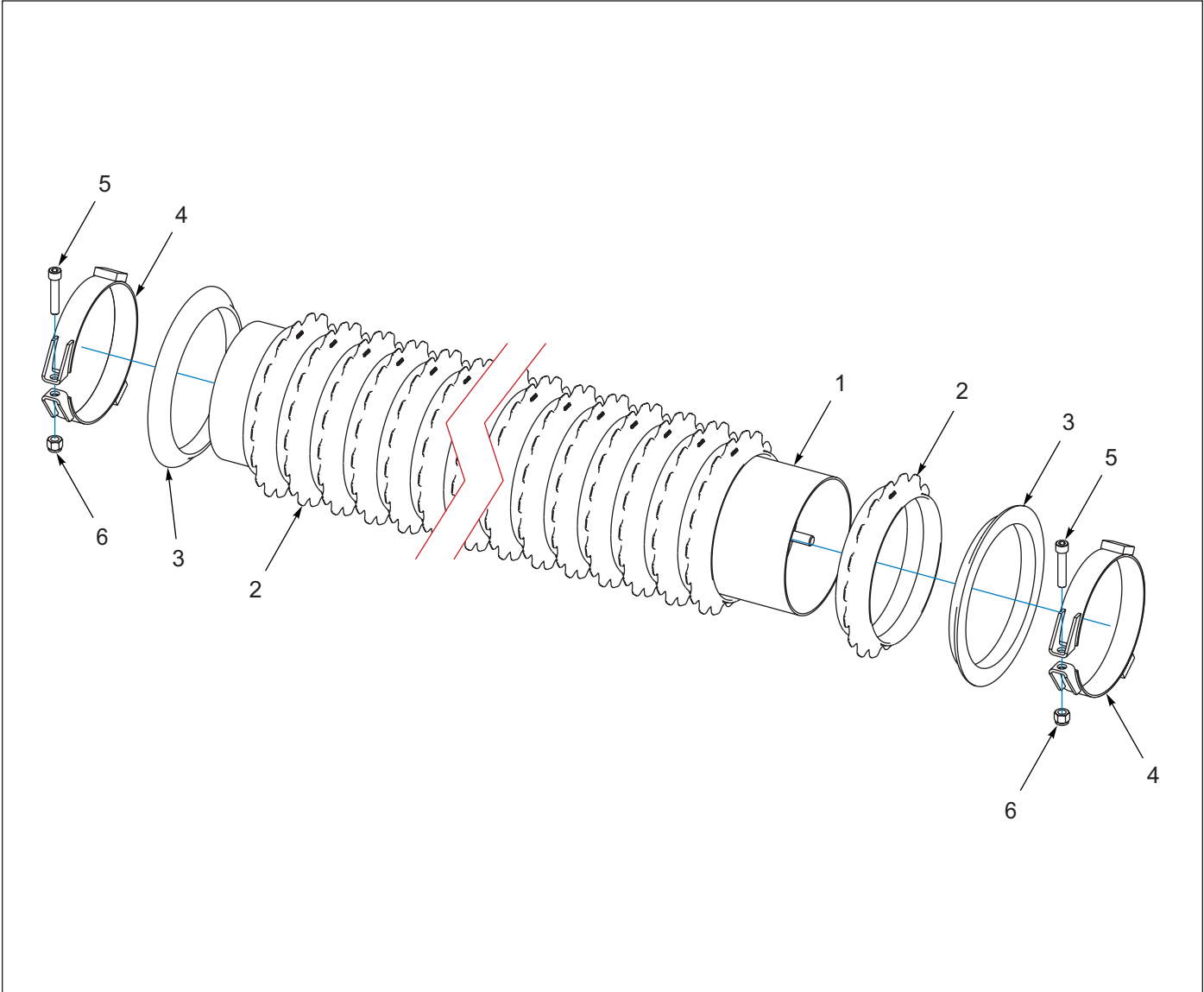
Figure 1-12: Front Roller Assembly
