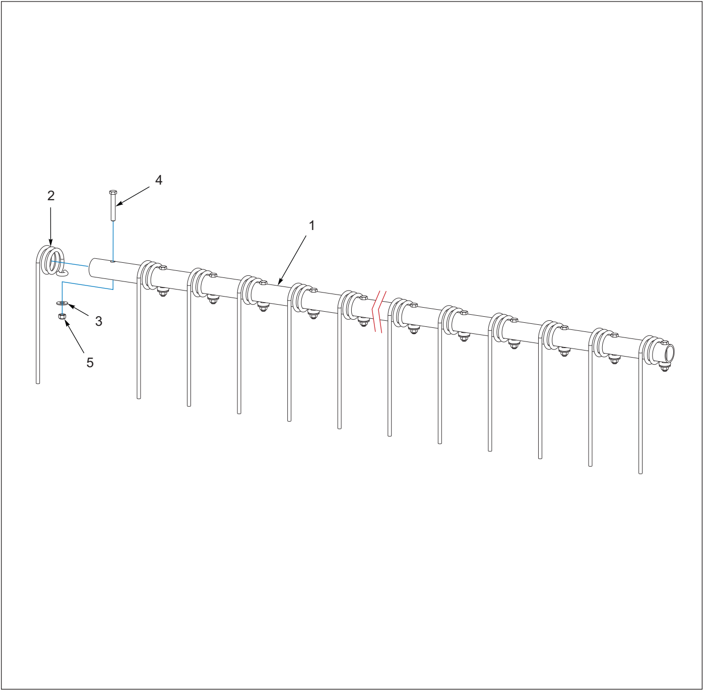
Figure 1-8: Coil Tine Harrow Assembly, 6FT (Full Width)
