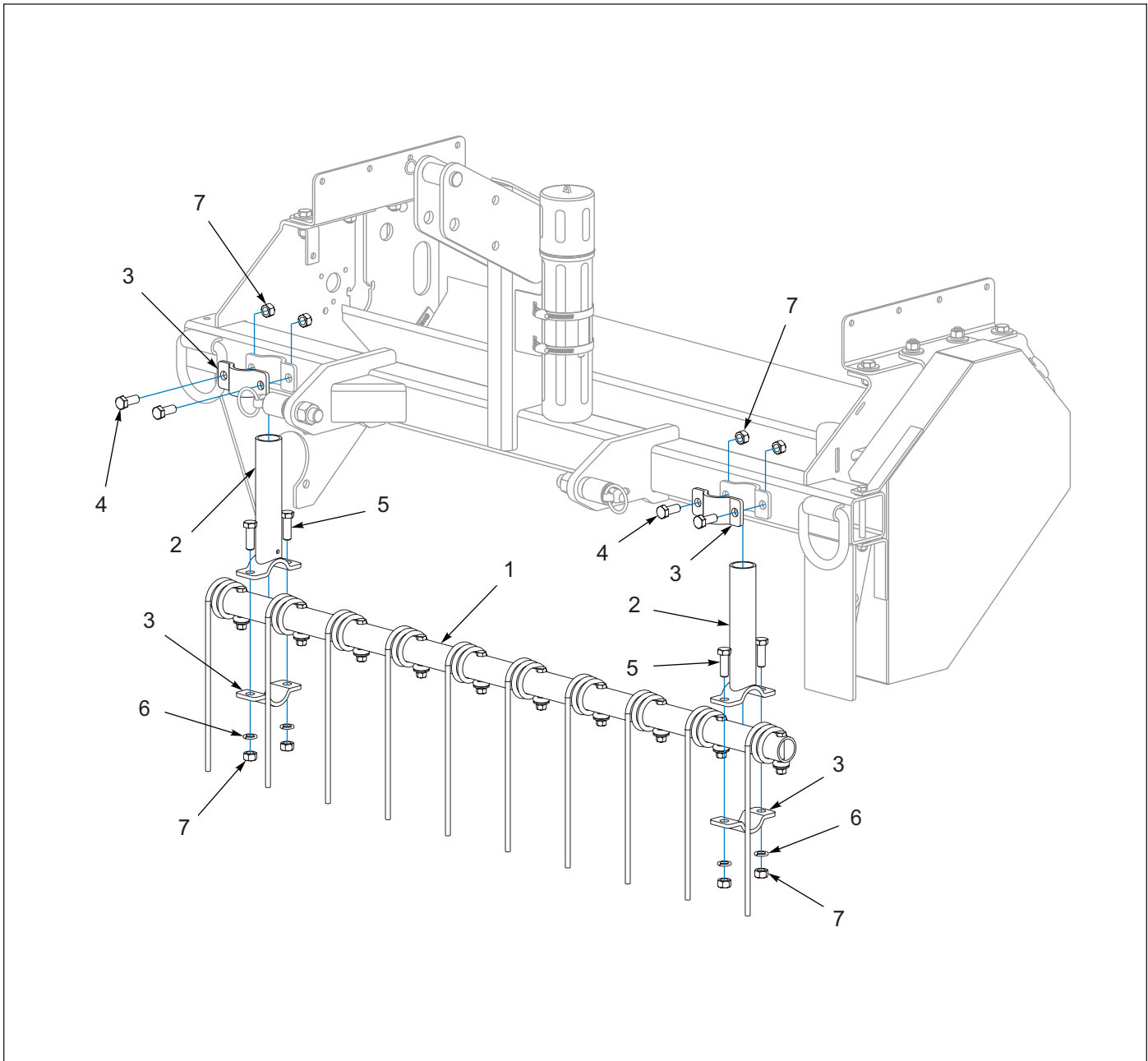
Figure 1-4: Coil Tine Harrow, 4FT & 5FT
