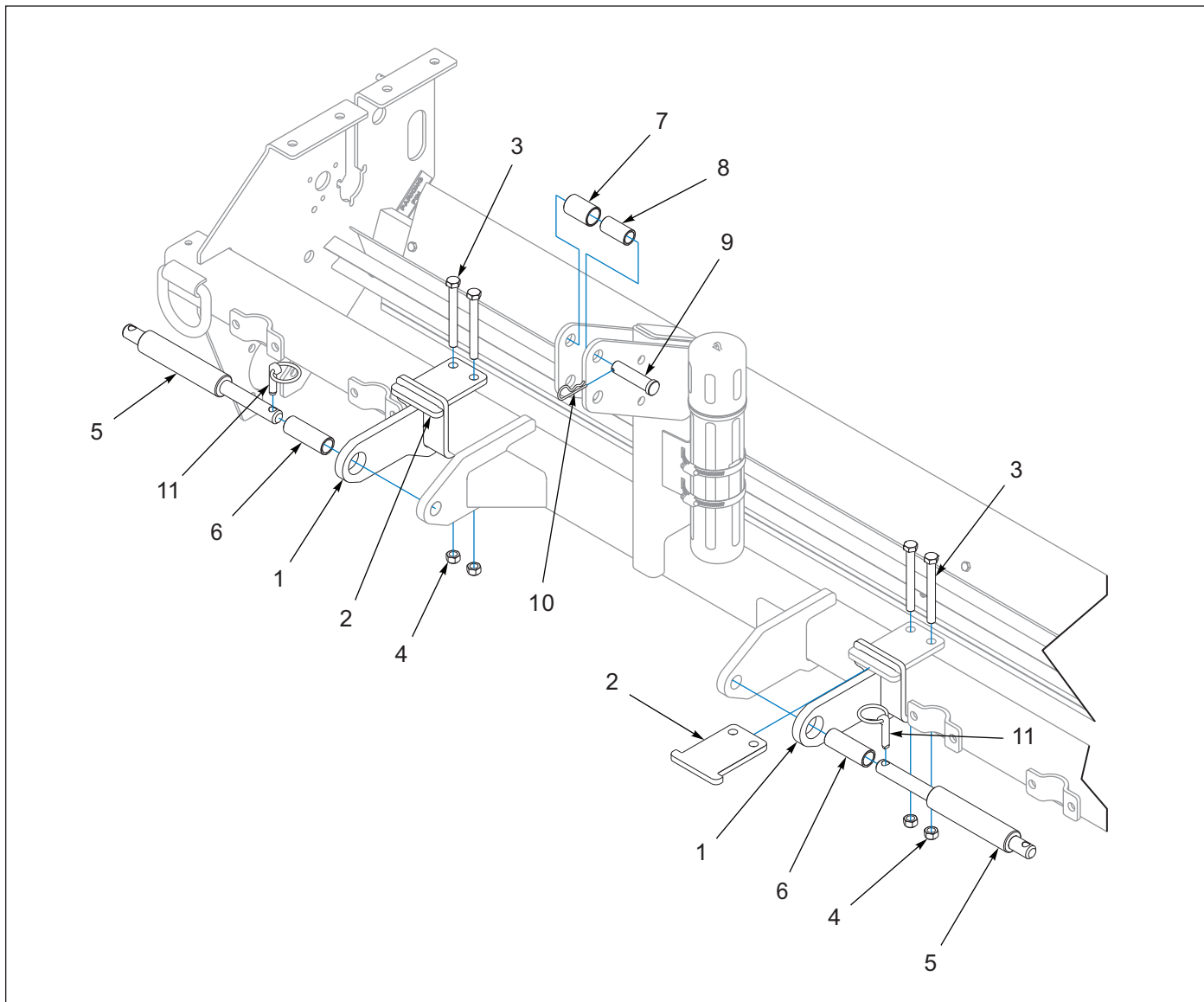
Figure 1-39: CAT2 Quick Hitch Adapter Kit - Optional
