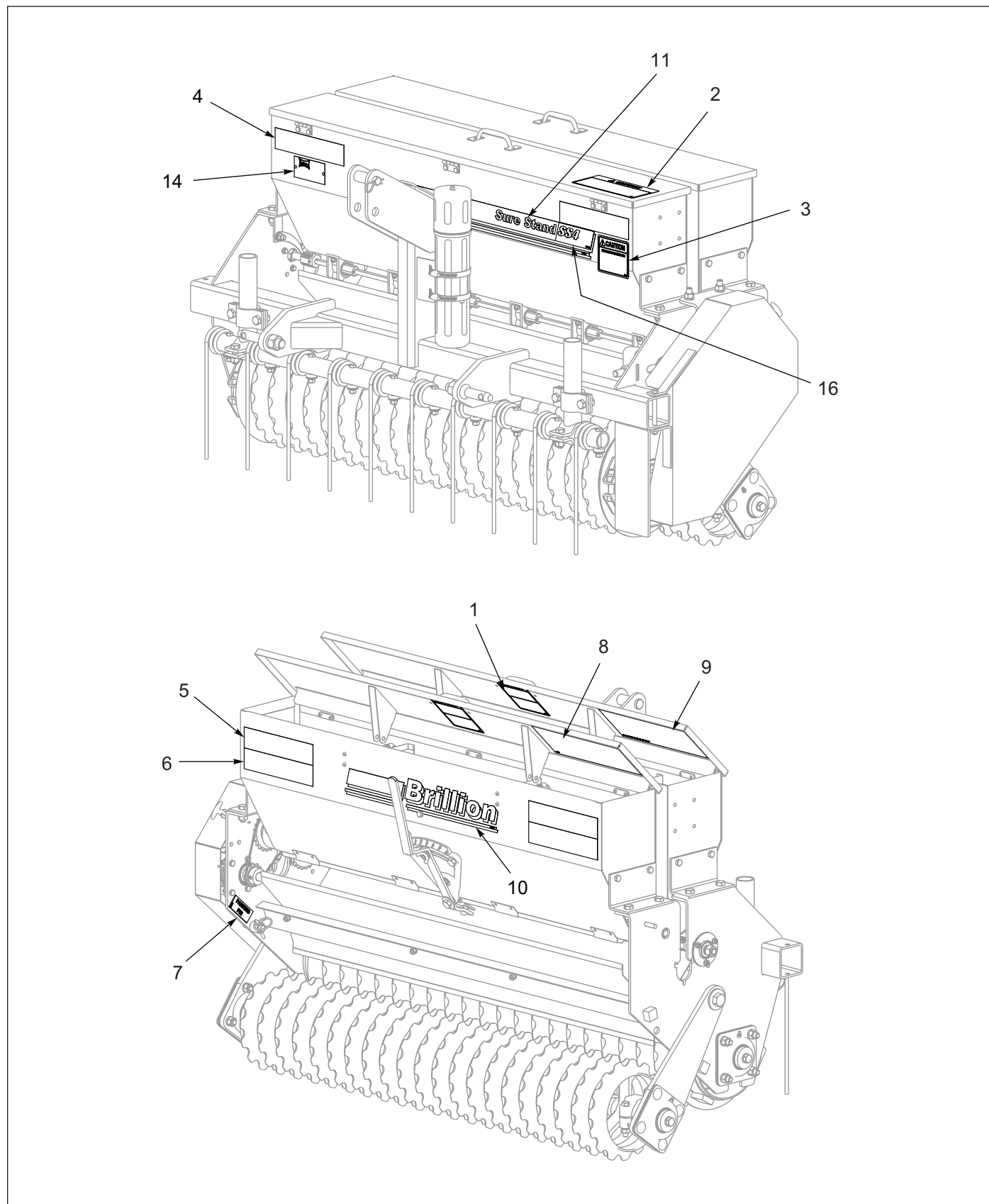
Figure 1-45: SSBP4 Decal Locations (Before 12/2023)
