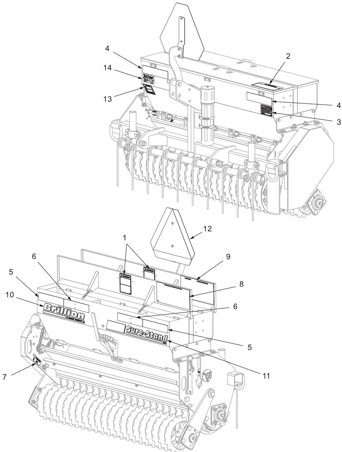
Figure 1-42: SSB4 Decal Locations (After 12/2023)
