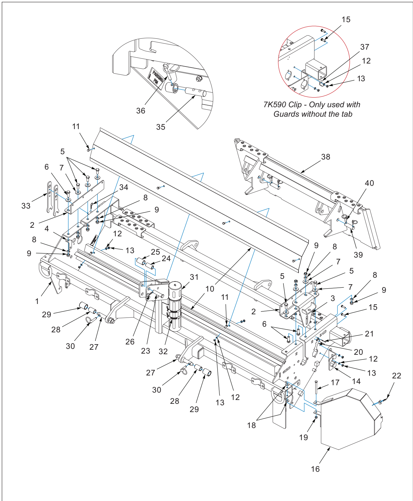
Figure 1-3: Skid Steer Frame, Quick Attach, Deflectors, Seed Box Mounts, Guards
