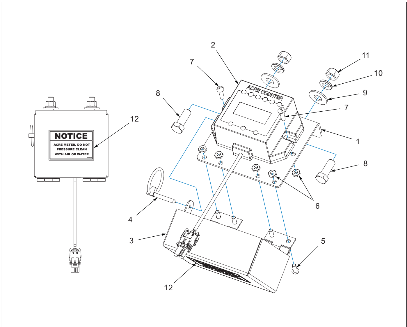
Figure 1-29: Acre Meter Assembly (Before 06/01/2025)
