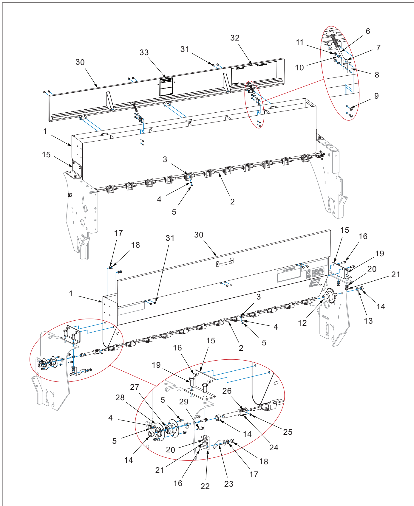
Figure 1-17: Meter Seed Box
