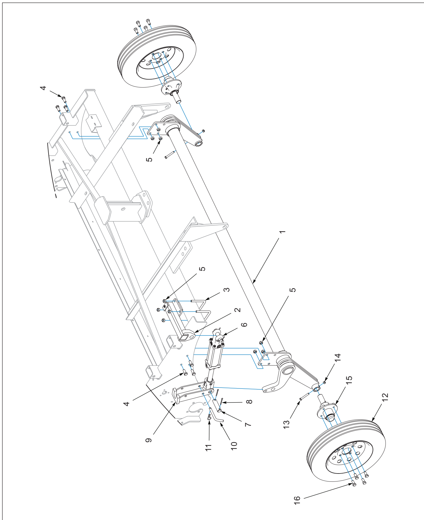
Figure 1-11: Rockshaft with Hydraulic Cylinder
