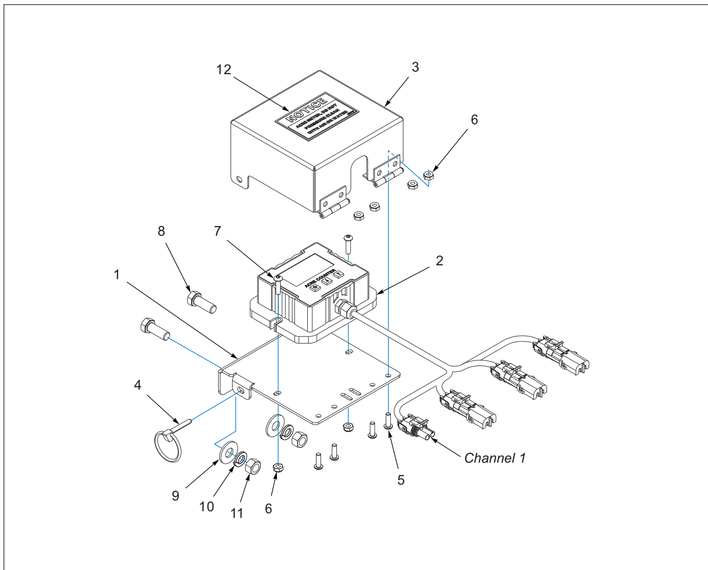
Figure 1-28: Acre Meter Assembly (After 06/01/2025)
