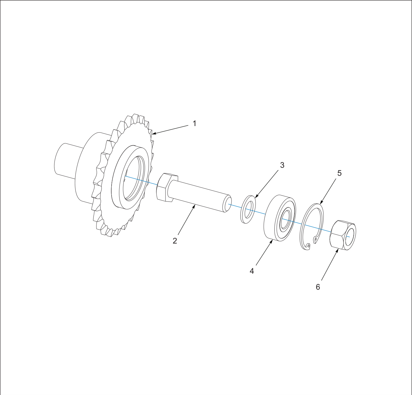
Figure 1-19: Sprocket Assembly, 26T
