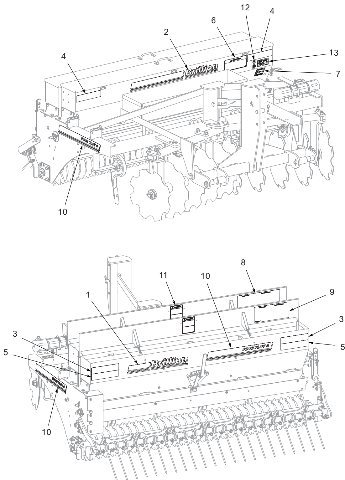
Figure 1-32: Decal Locations
