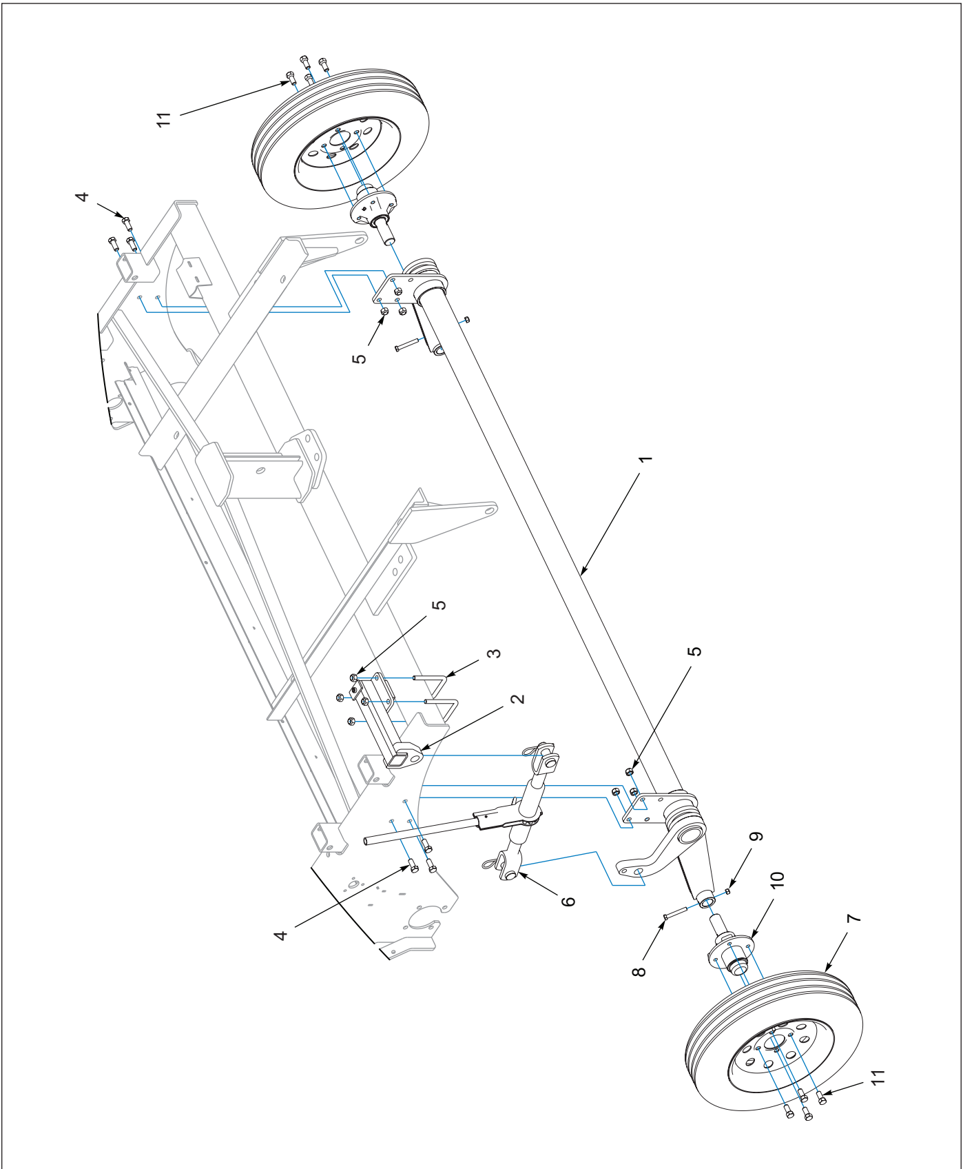
Figure 1-12: Rockshaft with Ratchet
