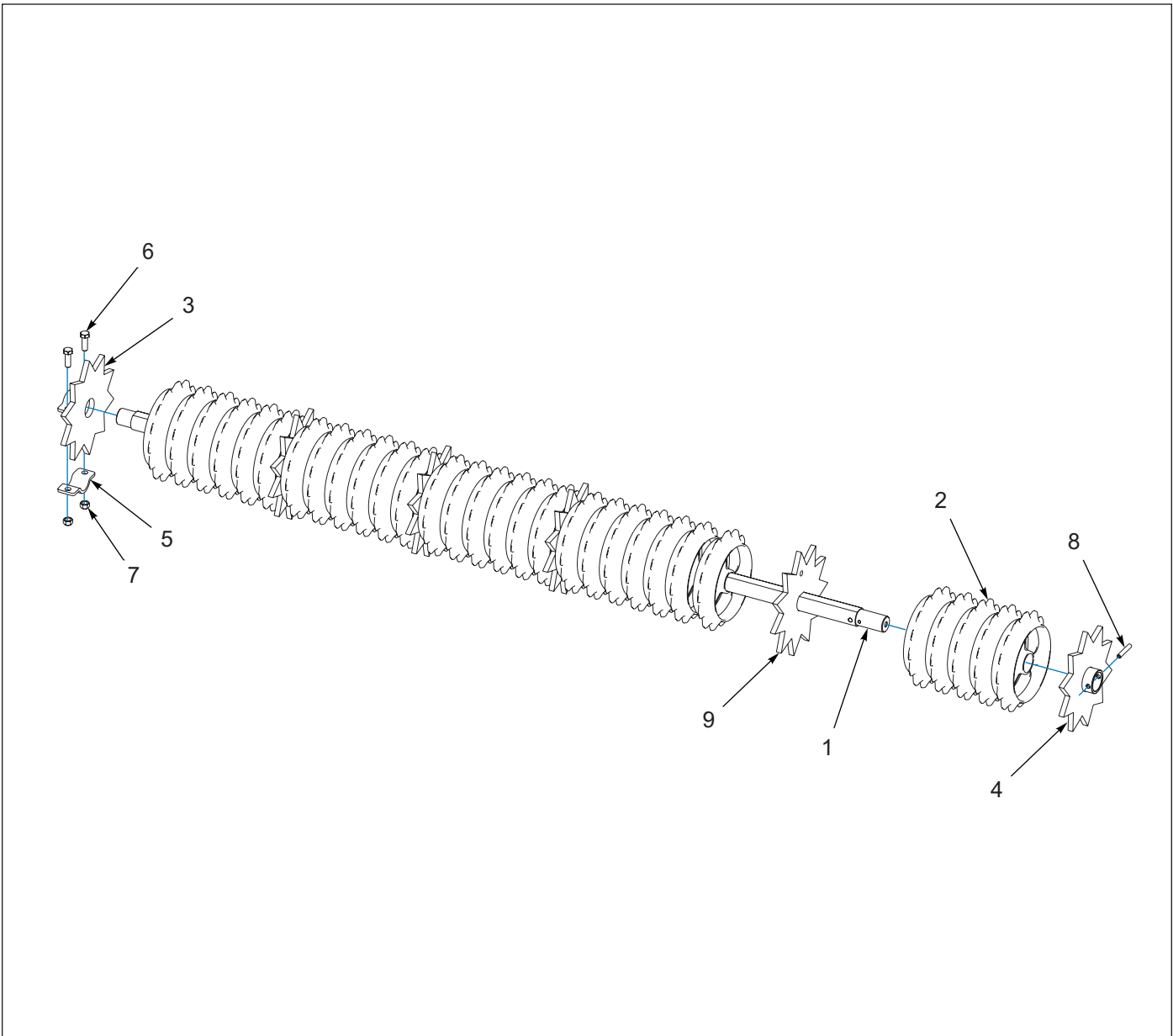
Figure 1-4: Standard Roller (AFTER 01/01/2026)
