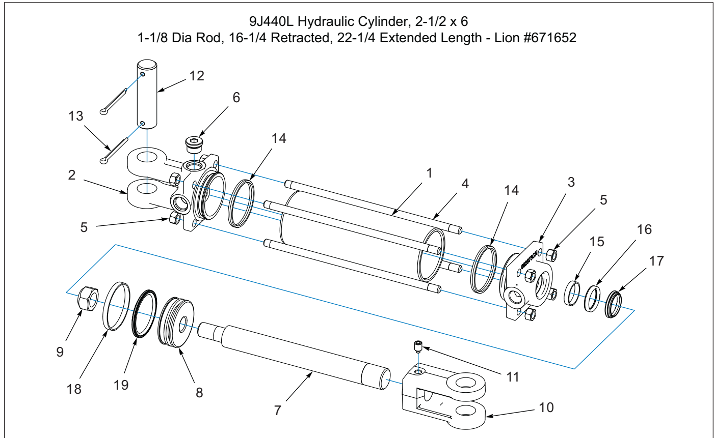
Figure 1-30: Hydraulic Cylinder, 2-1/2 x 6 - Lion - 671652
