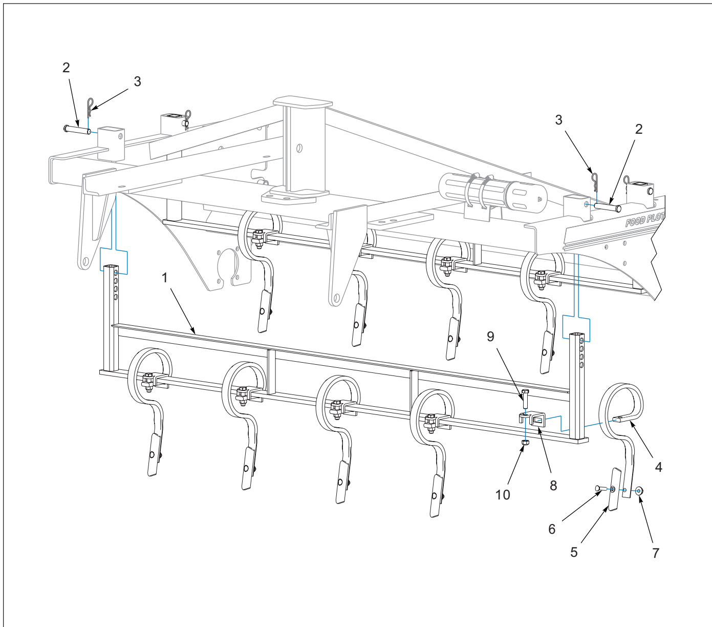
Figure 1-16: S-Tine
