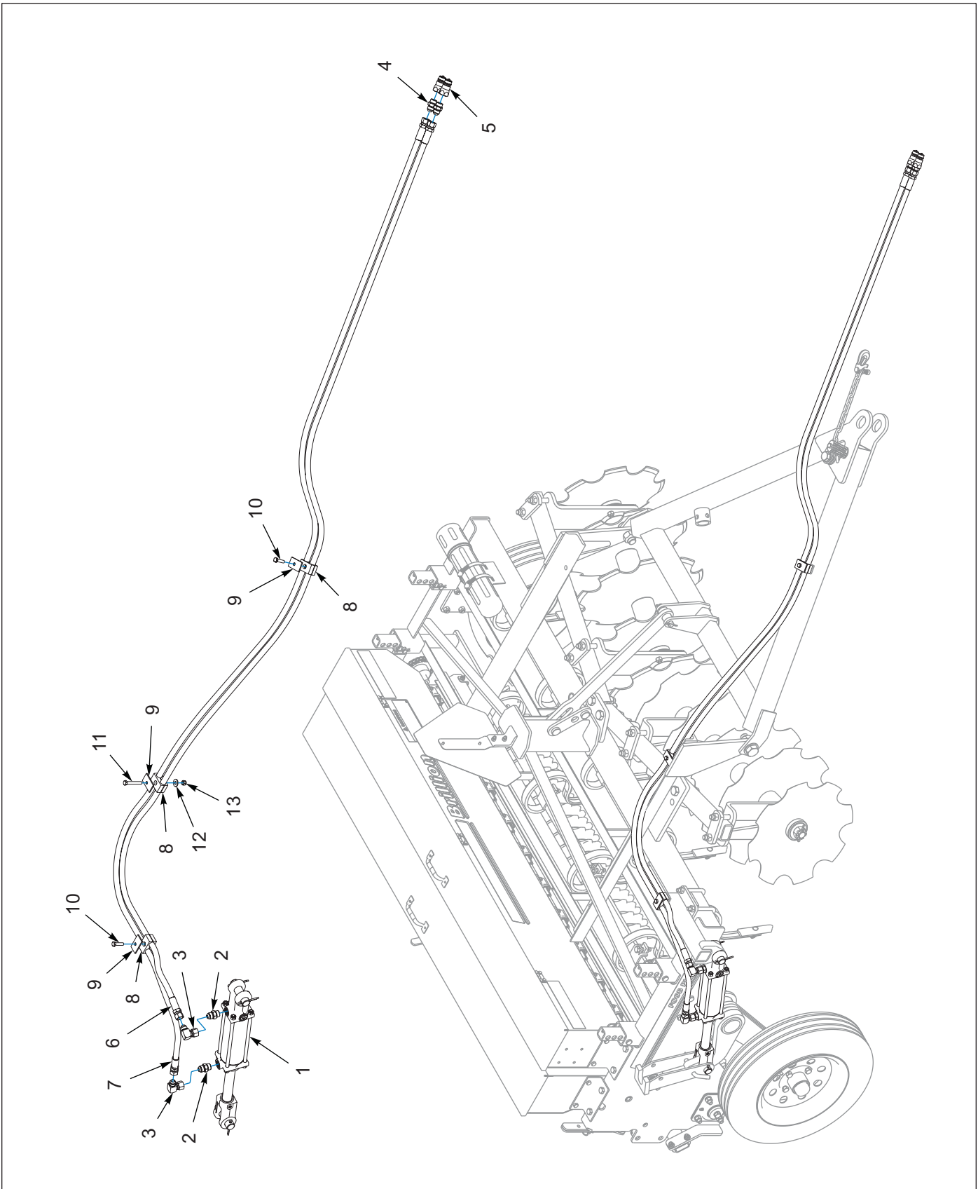
Figure 1-14: Hydraulic Layout
