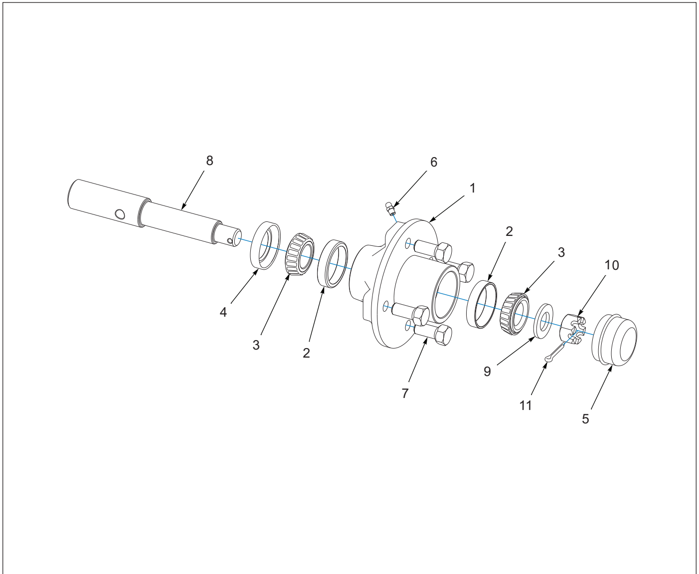
Figure 1-13: Hub and Spindle Assembly
