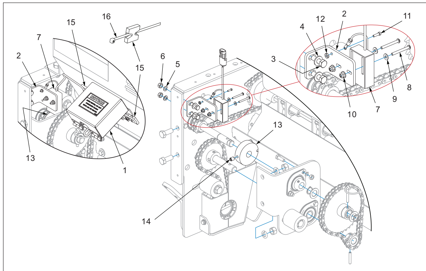
Figure 1-1: Acre Meter Kit - Optional
