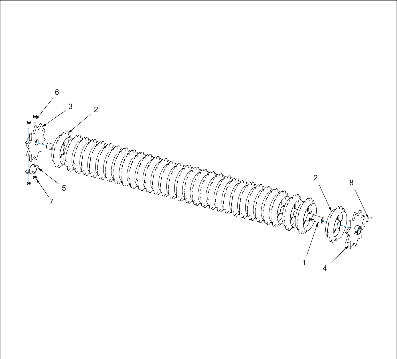
Figure 1-5: Standard Roller (BEFORE 01/01/2026)
