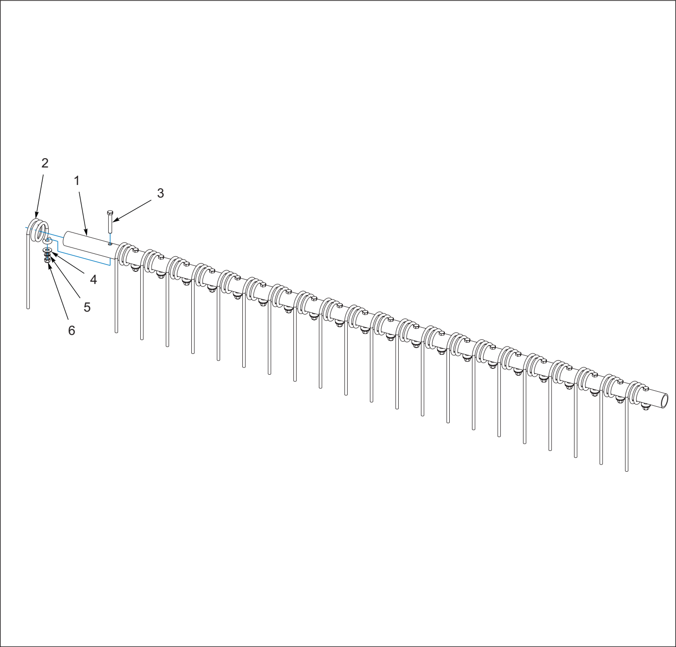
Figure 1-26: Coil Tine and Pipe Assembly
