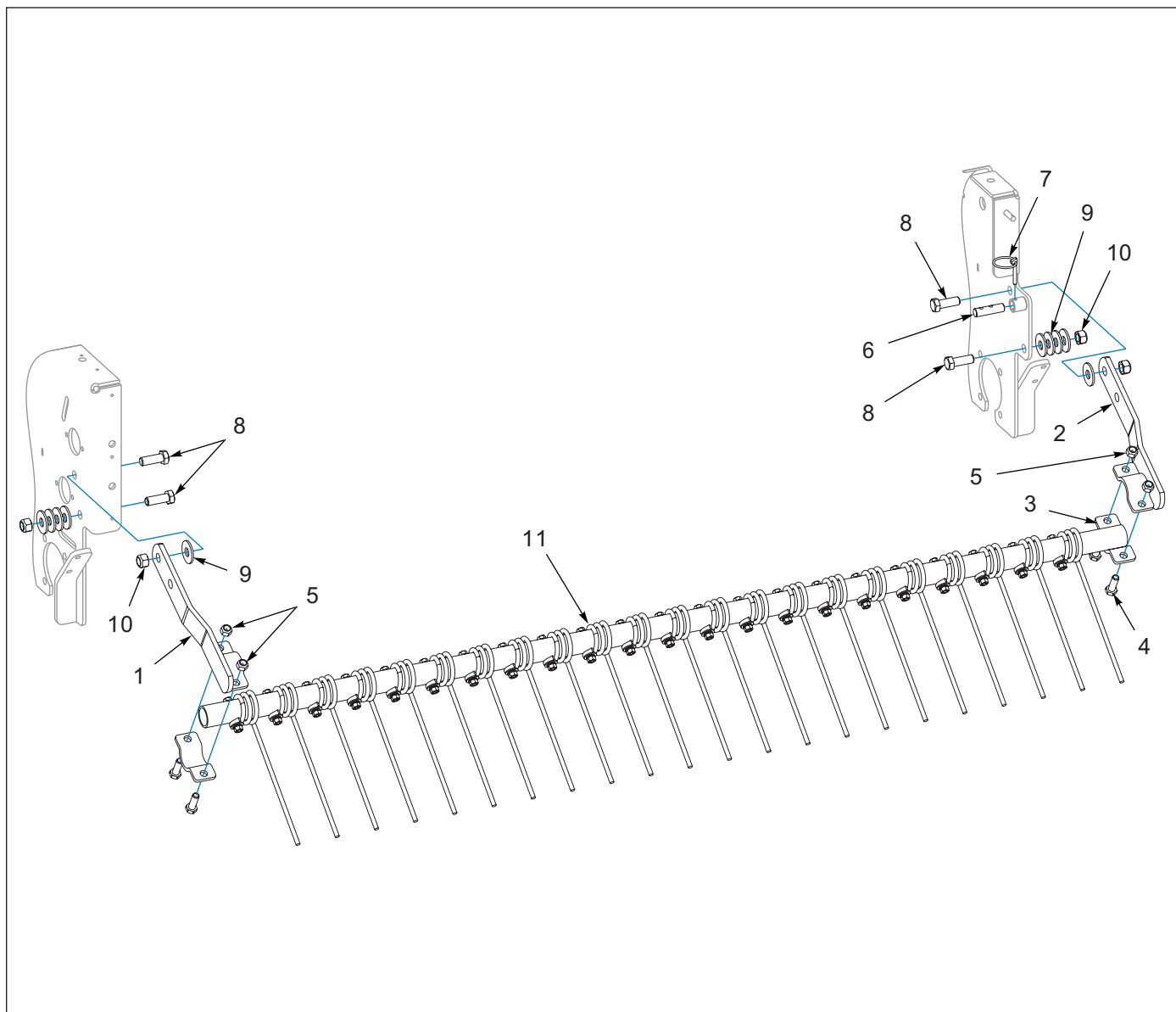
Figure 1-25: Coil Tine Assembly - Optional
