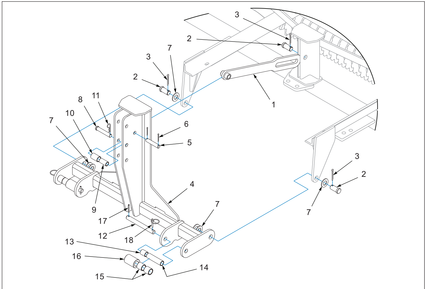
Figure 1-9: 3-PT Hitch
