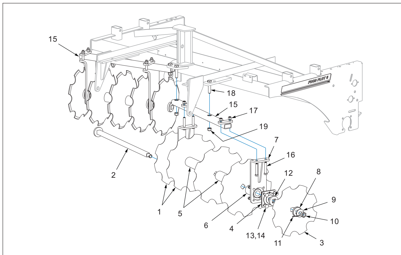
Figure 1-15: Disc Gangs
