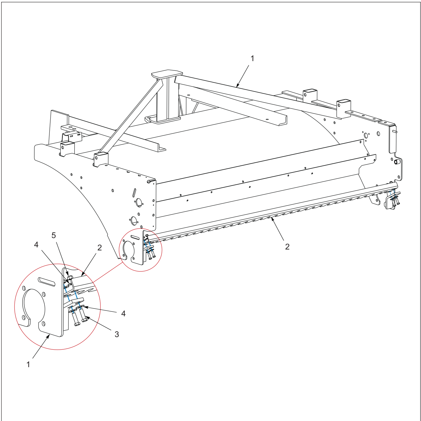
Figure 1-8: Previous Frame and Scraper
