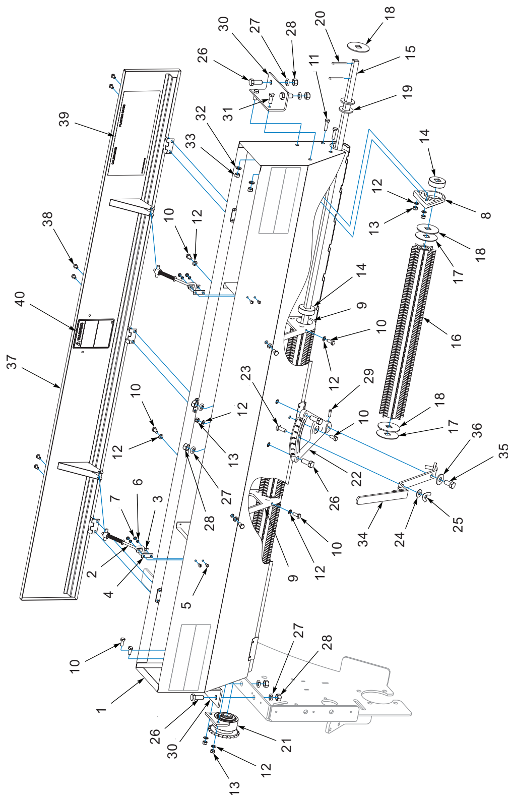
Figure 1-20: Agitator Seed Box Assembly
