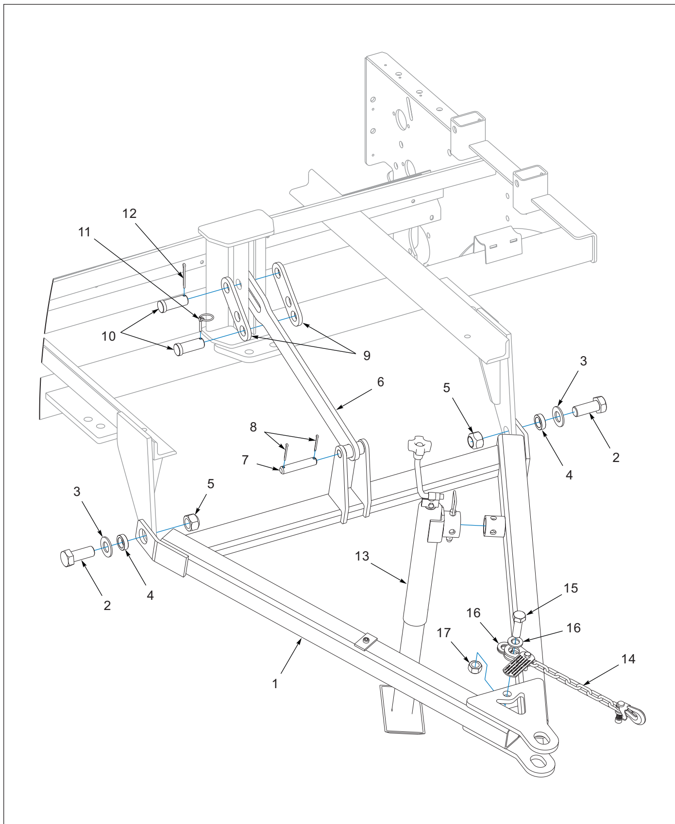
Figure 1-10: Drawbar
