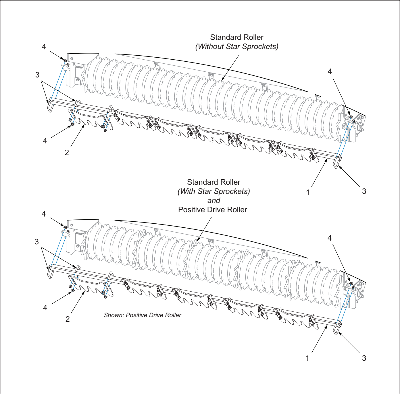
Figure 1-7: Scraper (After Serial #203912)
