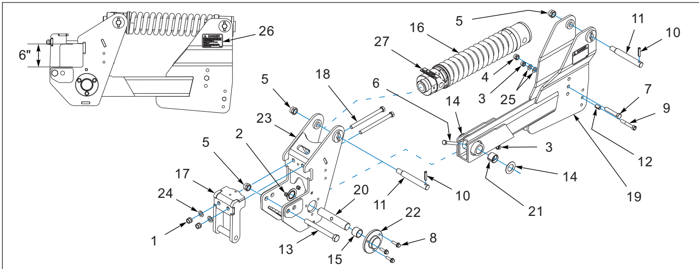
Figure 1-5: Auto Reset Shank Clamp, Spring (AFT. 01/01/2024)
