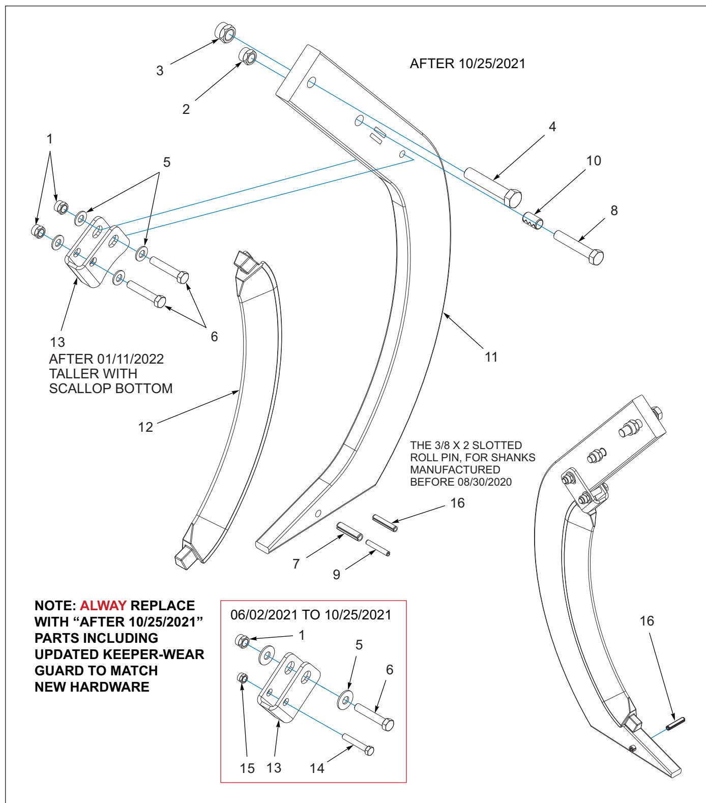
Figure 5-1: Parabolic Shank, 1-1/4
