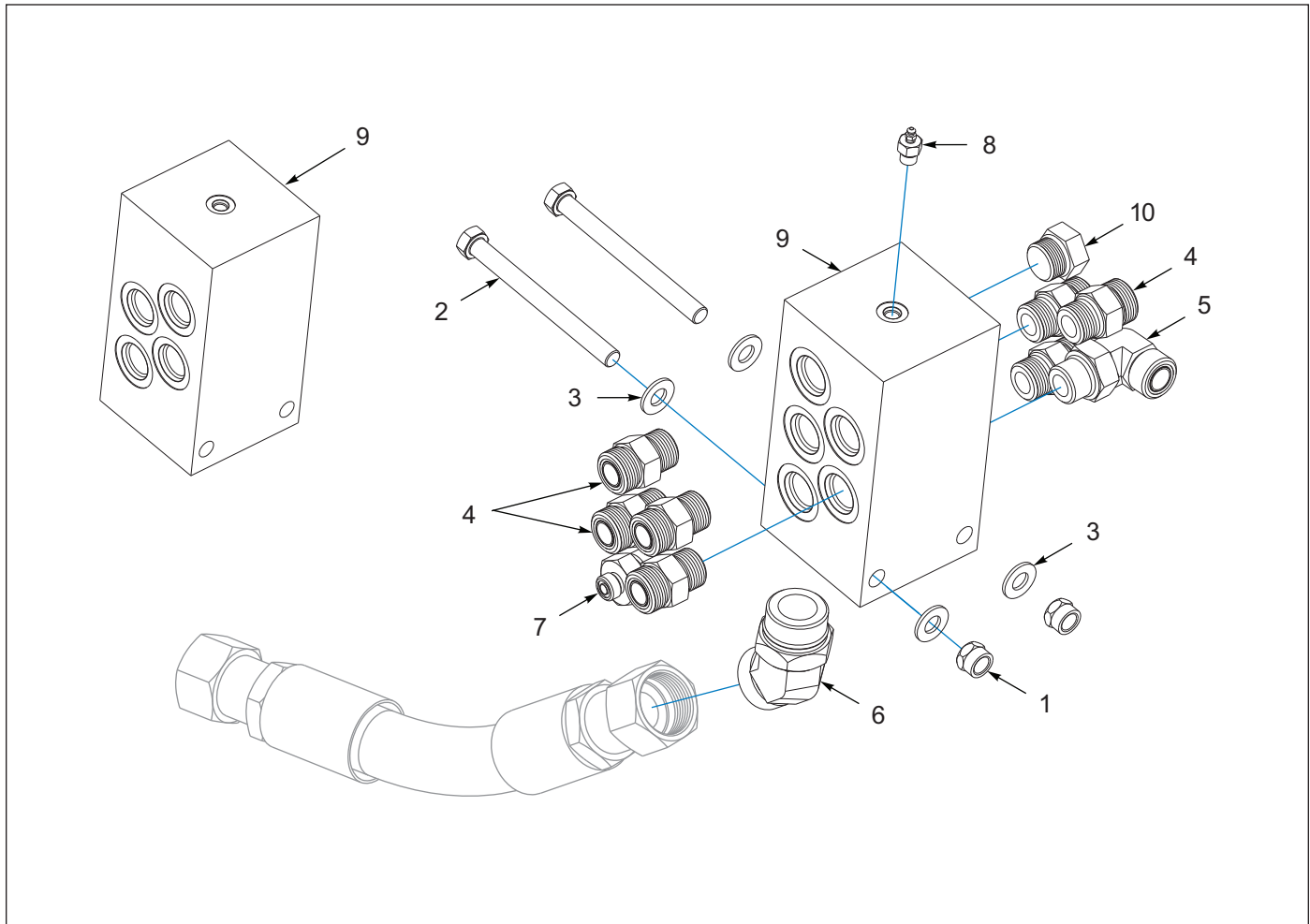
Figure 4-15: Manifold-Shank Cylinder Assembly
