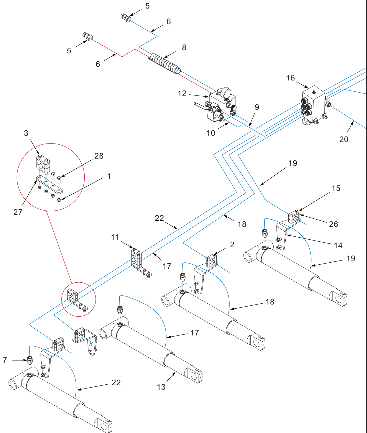
Figure 4-12: 2512 Hydraulics, 9 Shank (Folding) (1 of 2)
