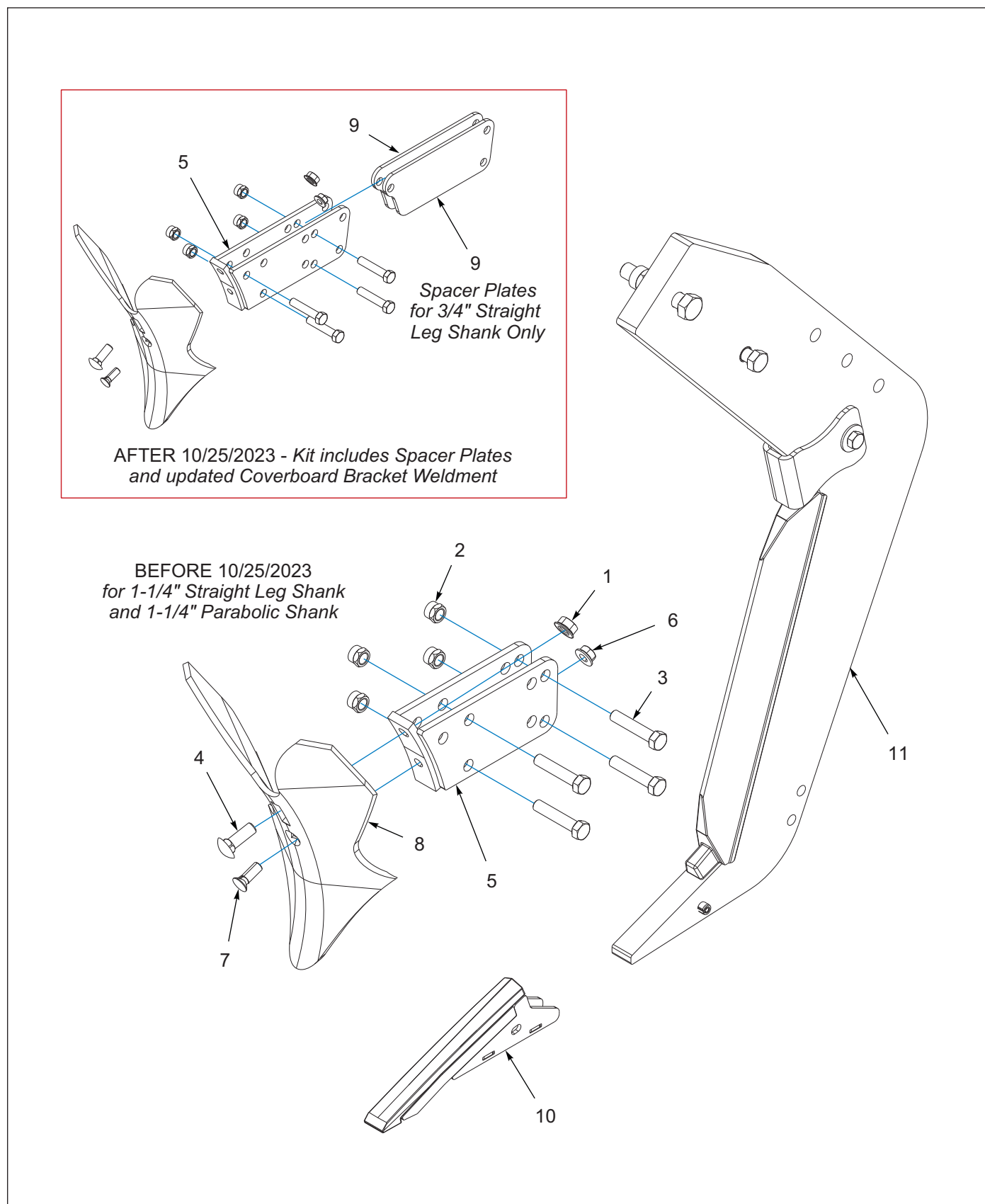
Figure 5-4: Coverboard Kit
