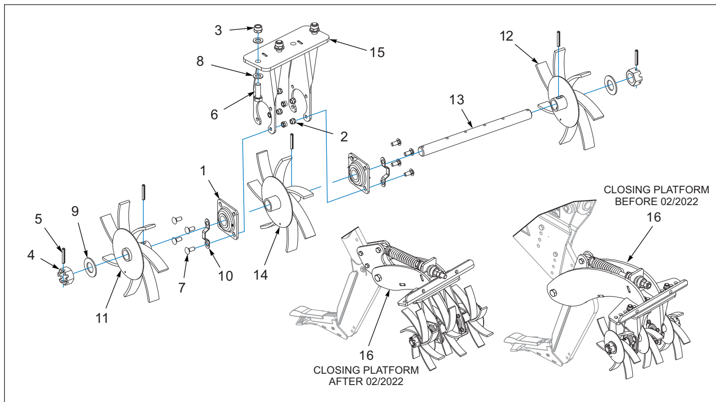
Figure 7-12: Treader
