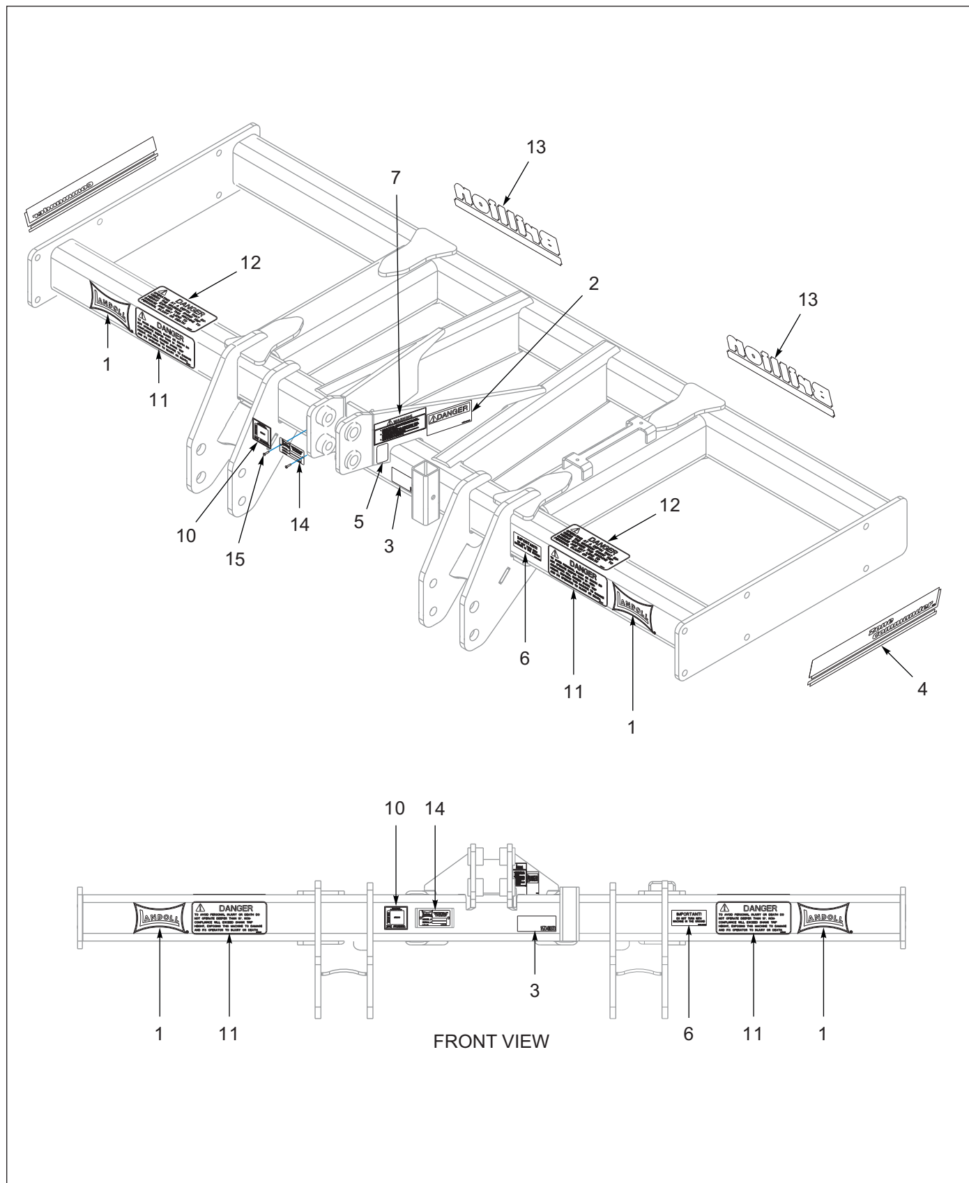
Figure 6-2: Decal Locations
