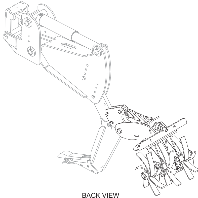
Figure 5-4: Closing Platform (02/2022 TO 04/2024) (2 of 2)
