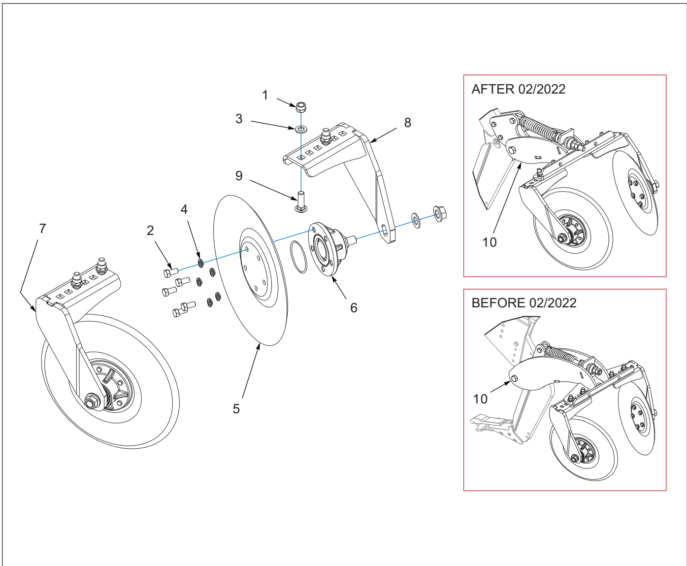
Figure 5-9: Closer Disc
