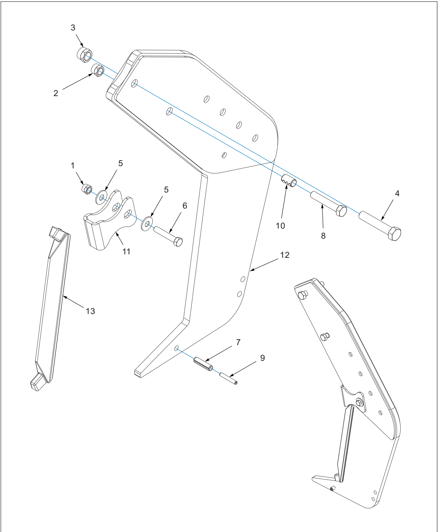
Figure 2-3: 3/4 Shanks
