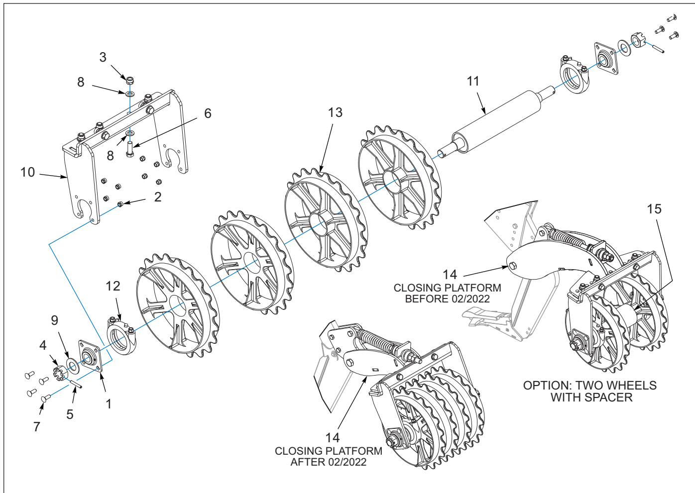
Figure 5-11: Packer Reel
