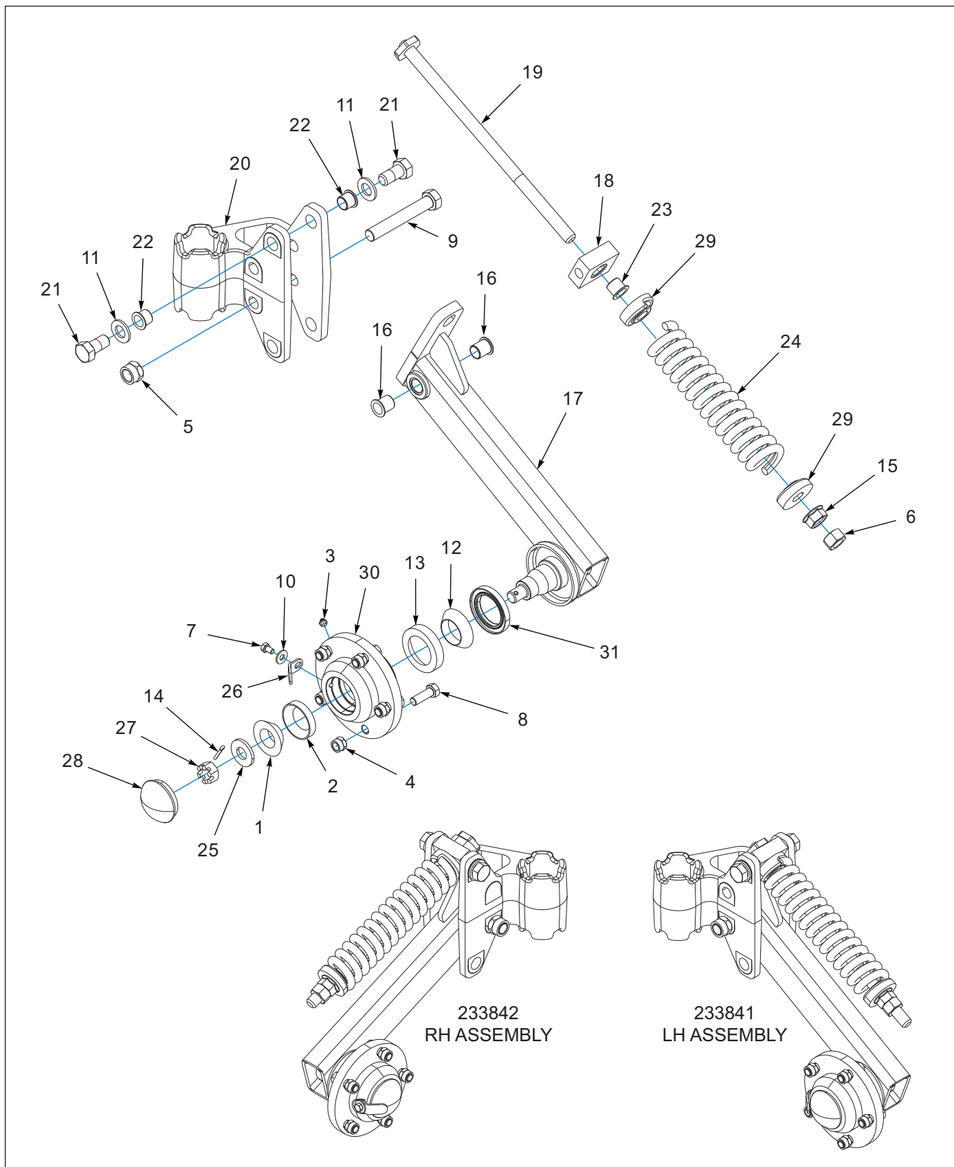
Figure 3-3: Heavy Duty Coulter (AFTER 02/2022)
