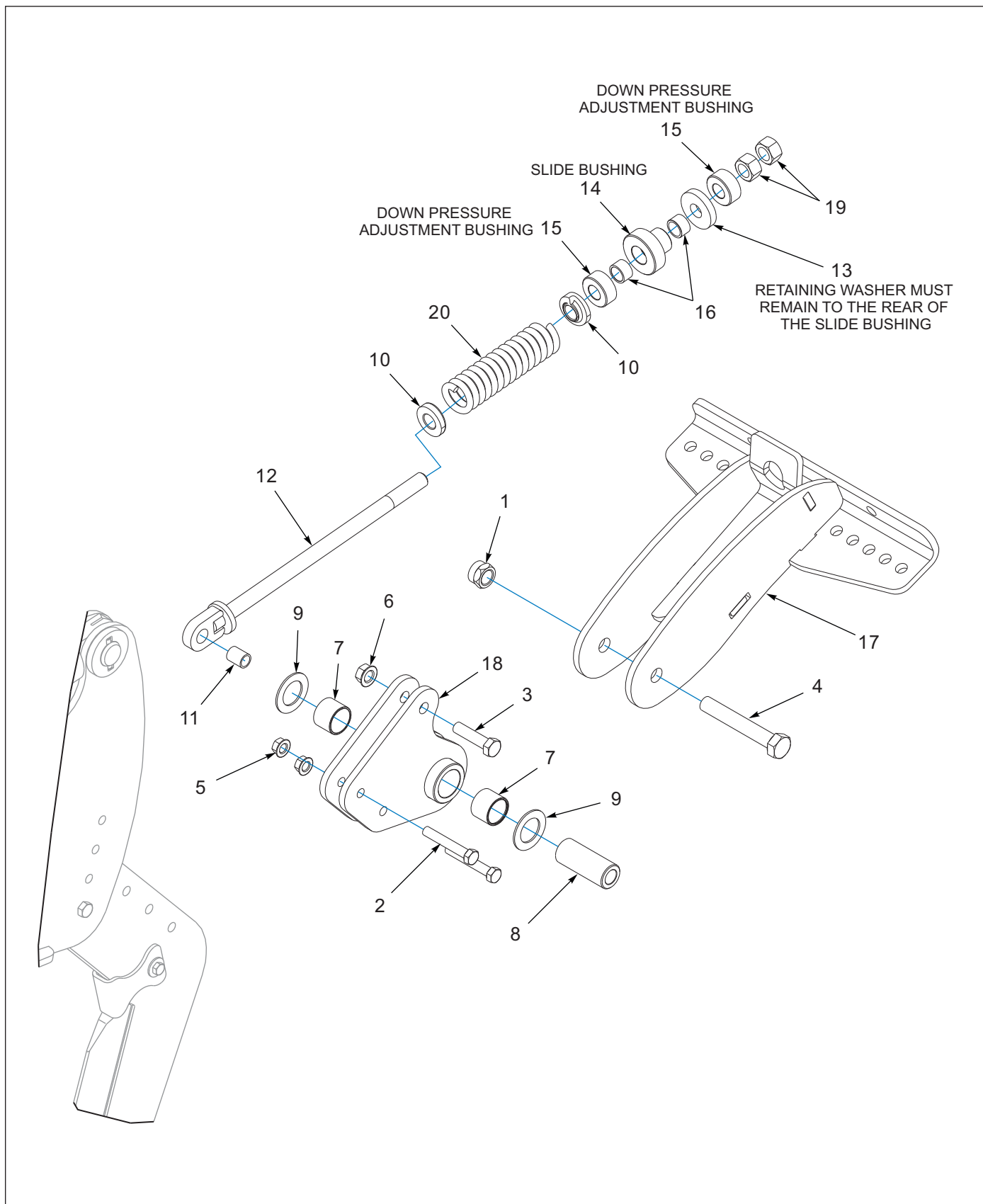
Figure 5-3: Closing Platform (02/2022 TO 04/2024) (1 of 2)
