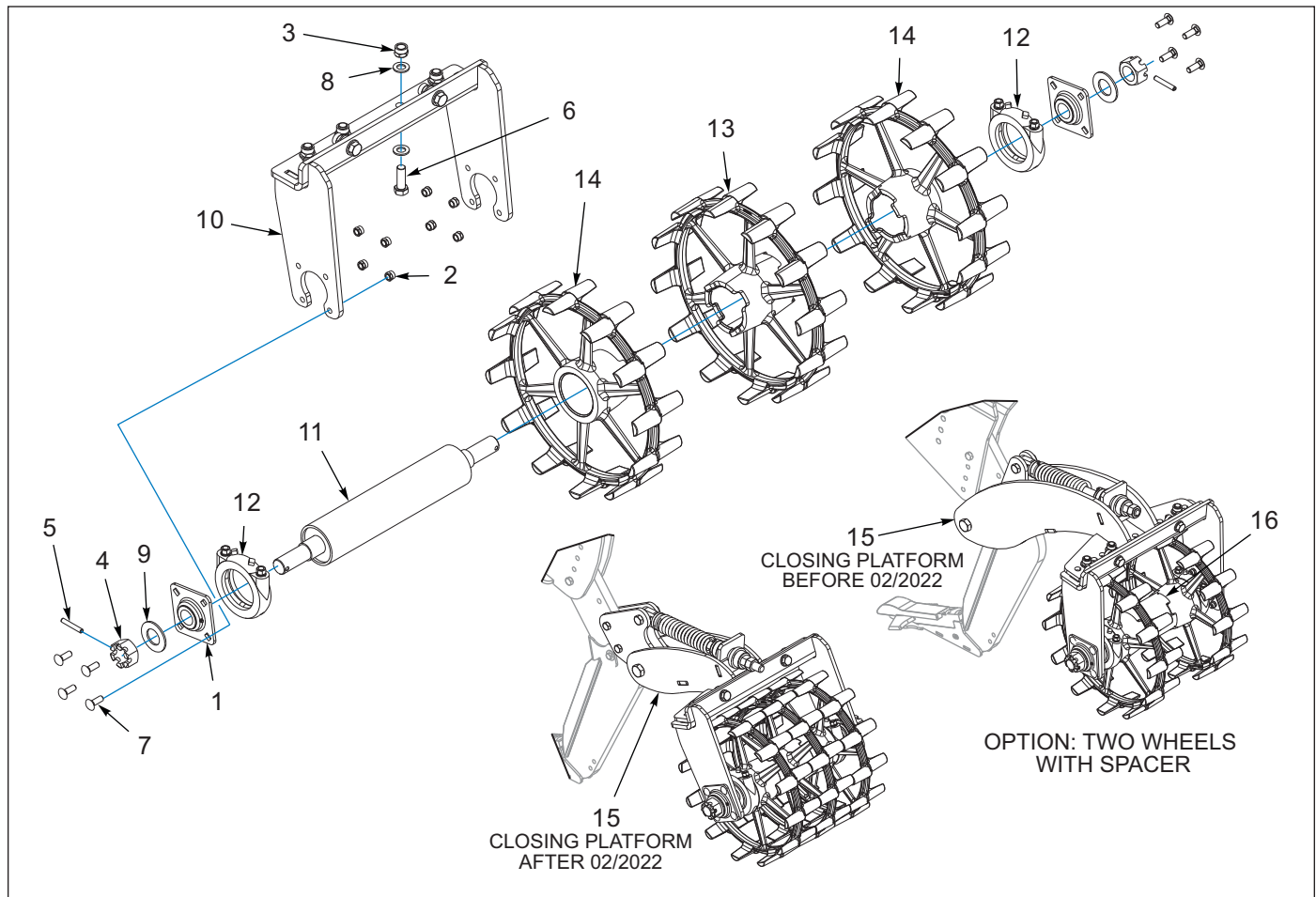
Figure 5-10: Crumbler Reel
