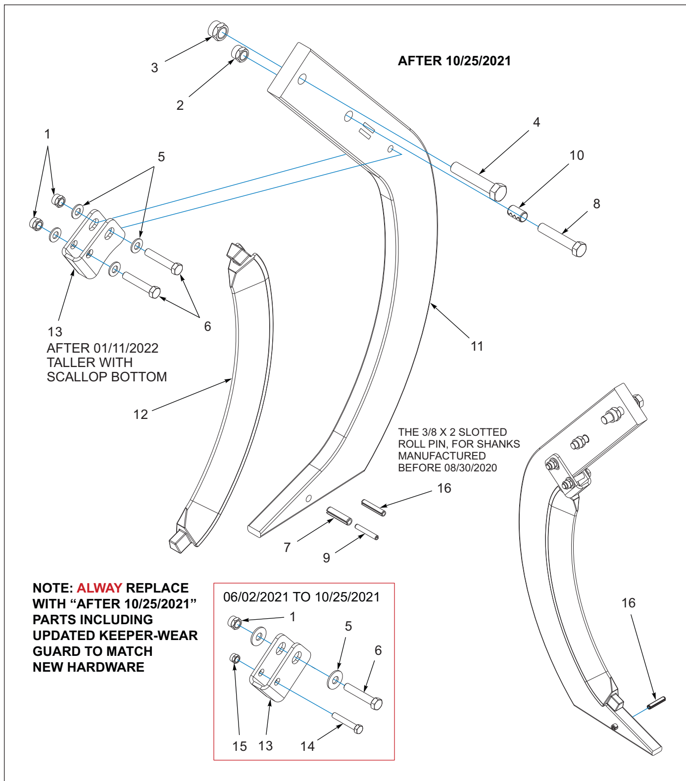
Figure 2-1: Parabolic Shank, 1-1/4
