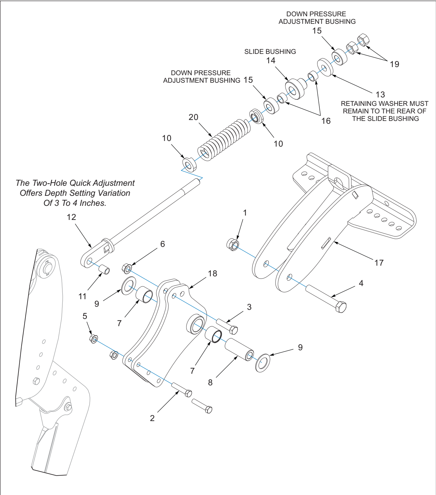
Figure 5-1: Closing Platform (AFTER 04/2024) (1 of 2)
