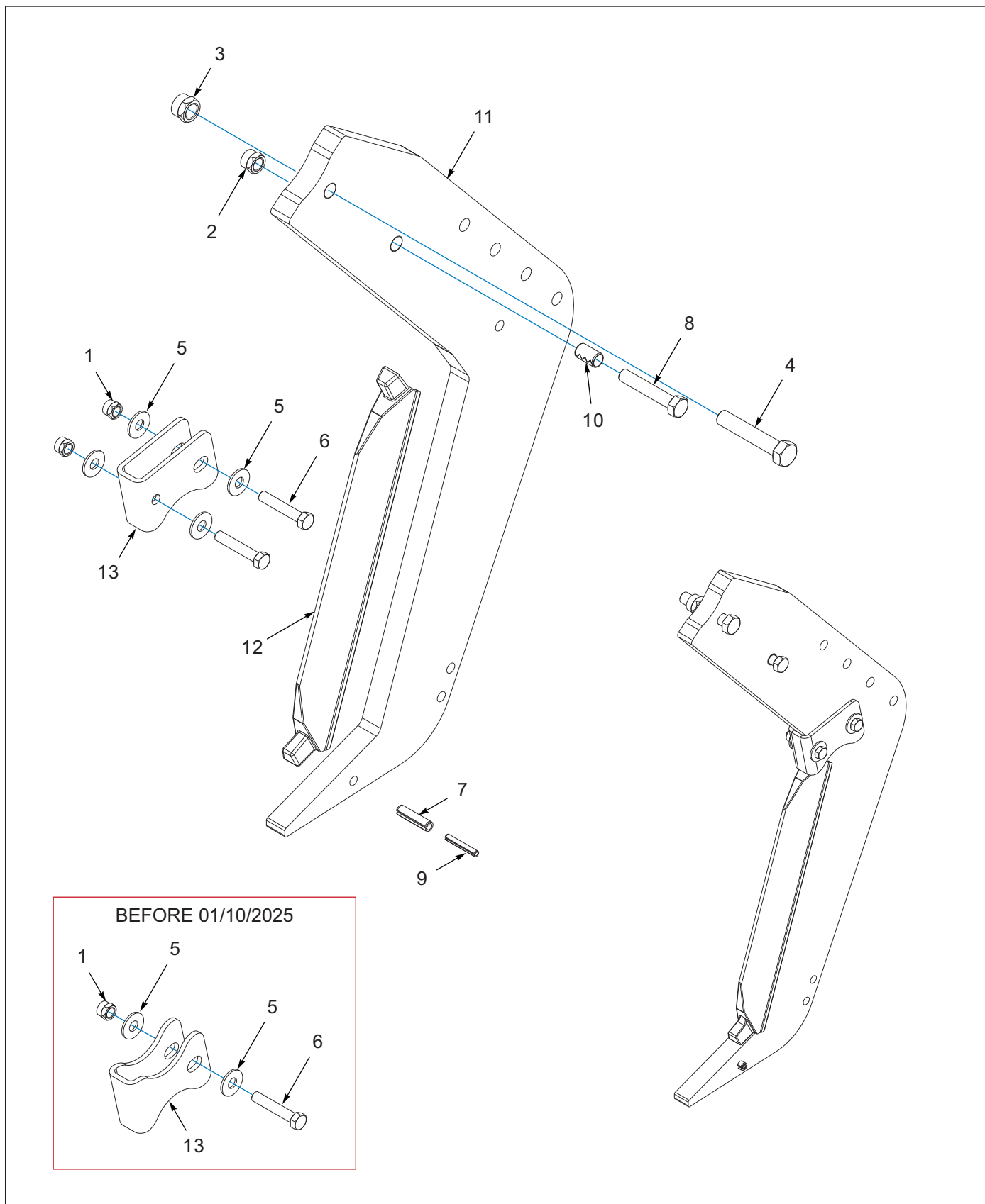
Figure 2-2: Straight Leg Shank, 1-1/4
