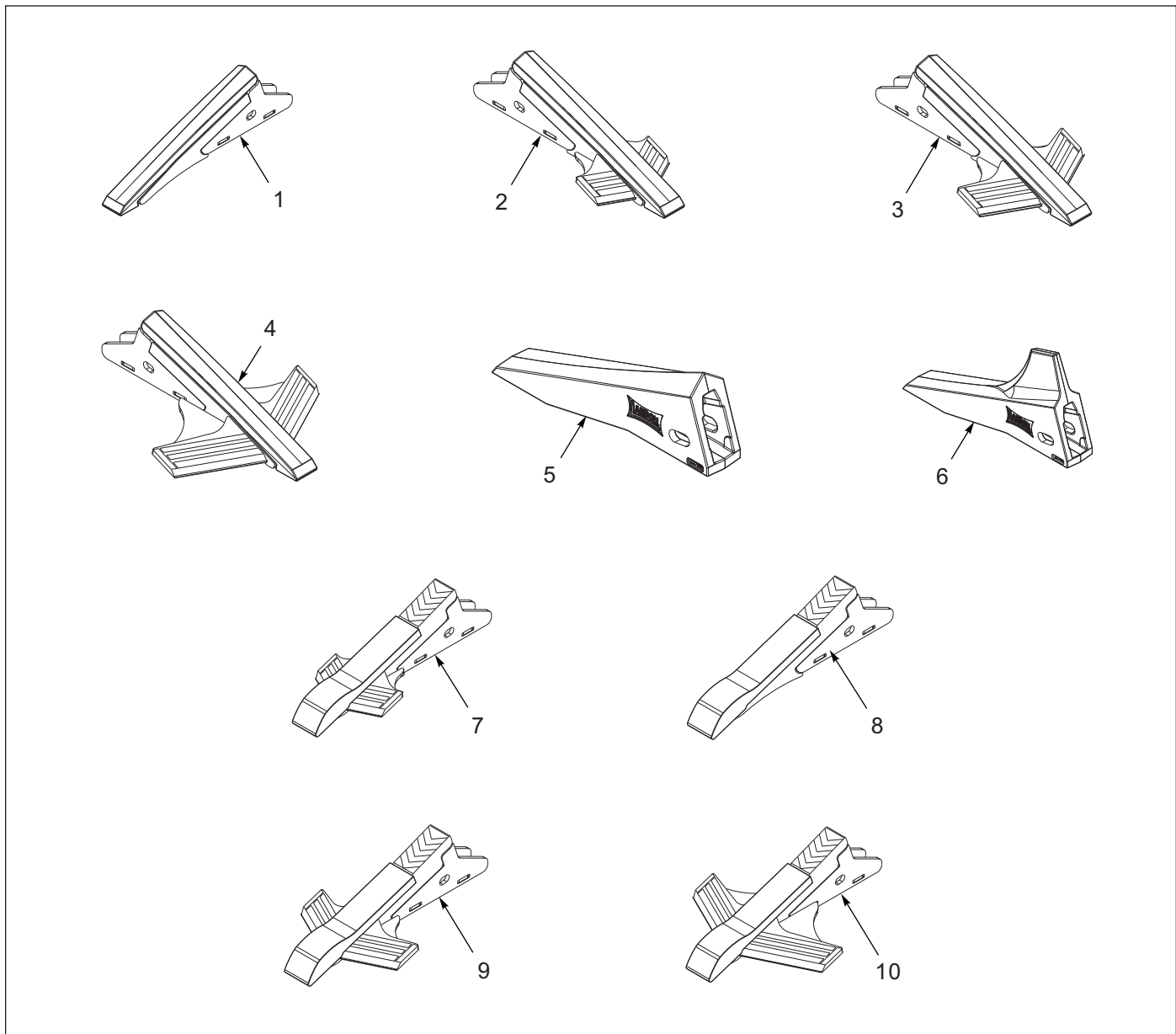
Figure 2-5: Points for 1-1/4
