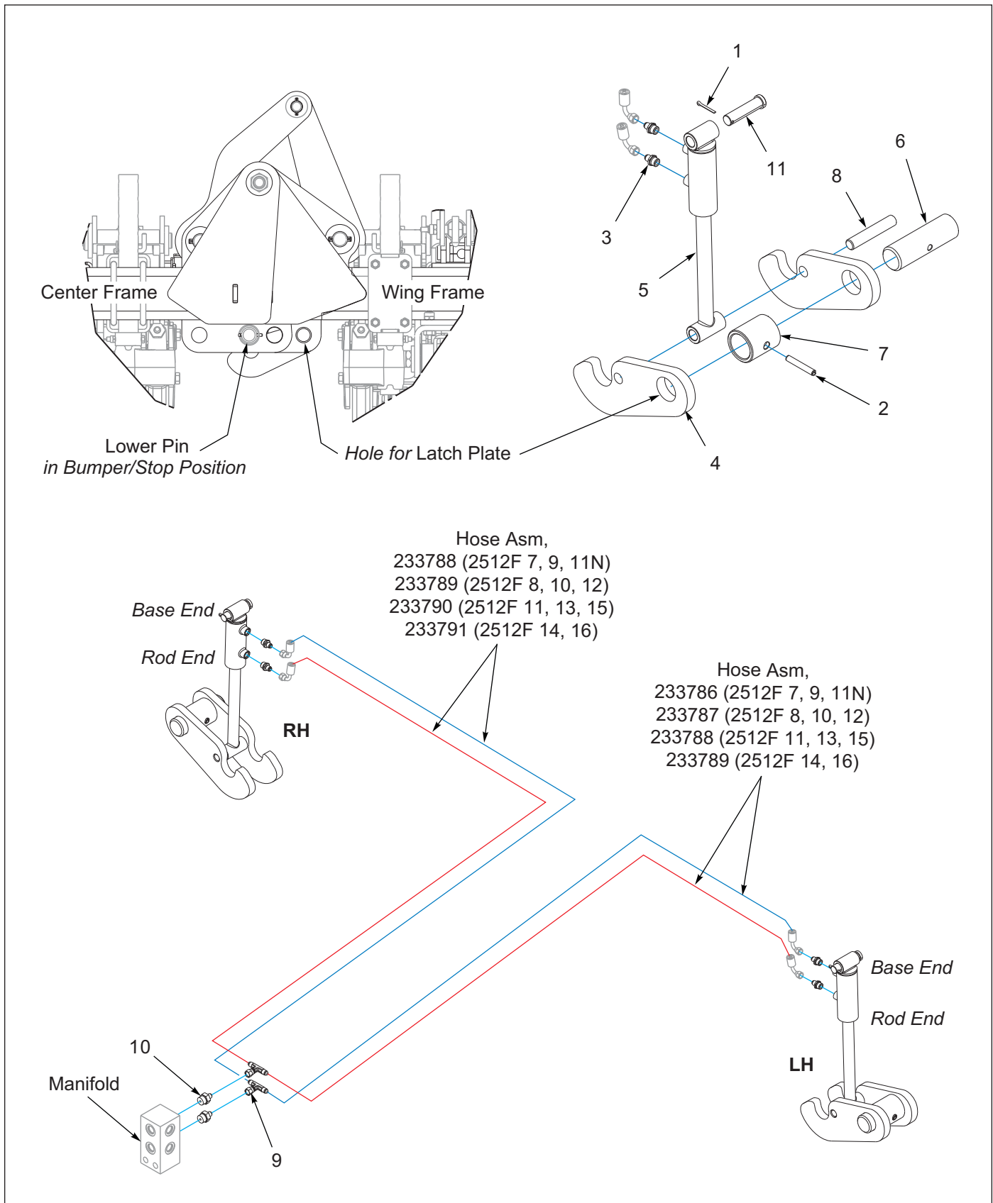
Figure 4-16: Wing Lock Kit - Optional
