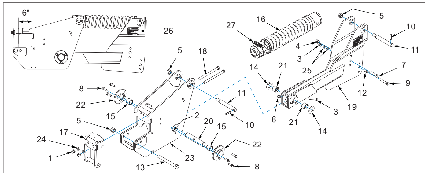
Figure 1-6: 2512 Auto Reset Shank Clamp, Spring - Setback (AFTER 01/01/2024)
