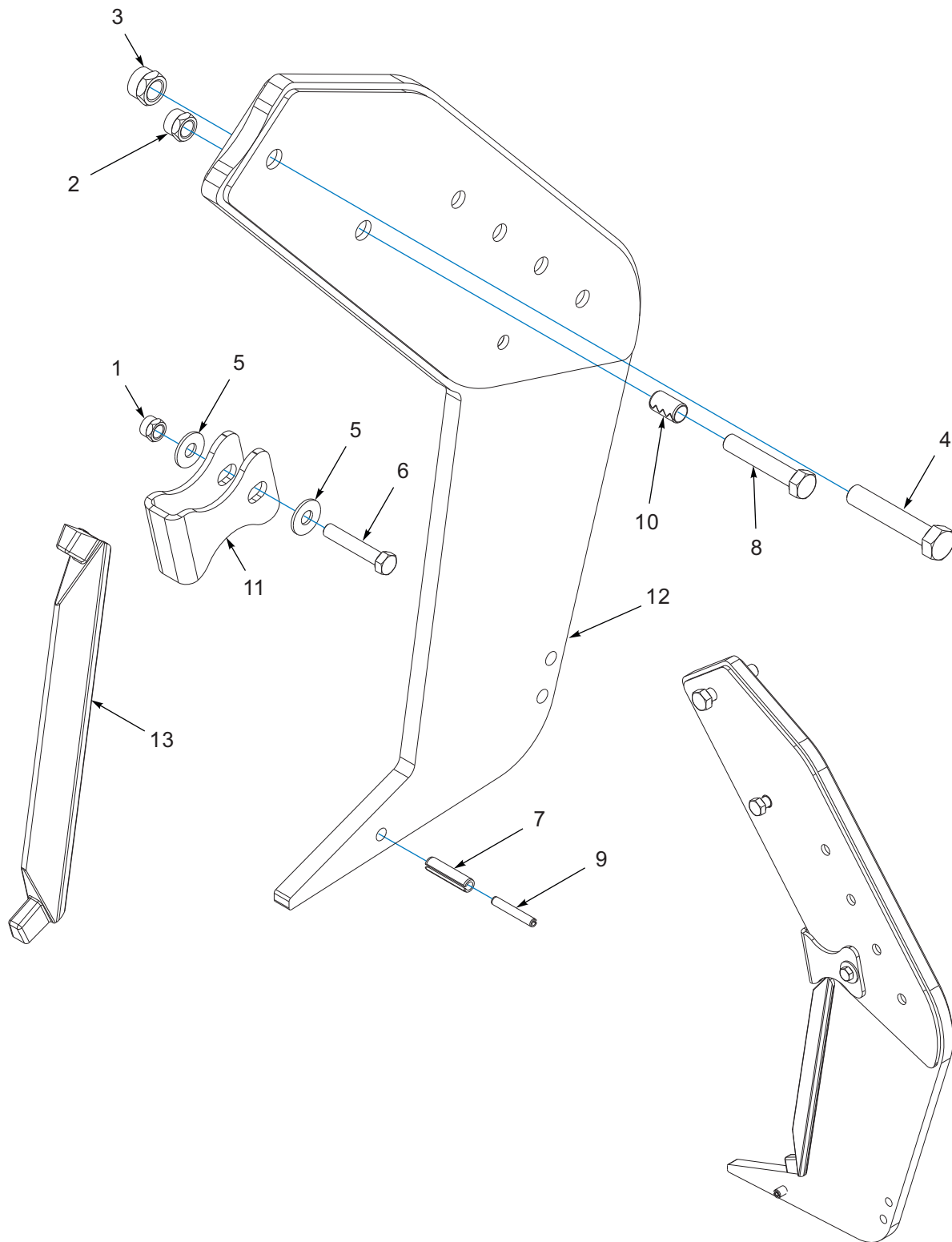
Figure 5-3: Straight Leg Shank, 3/4
