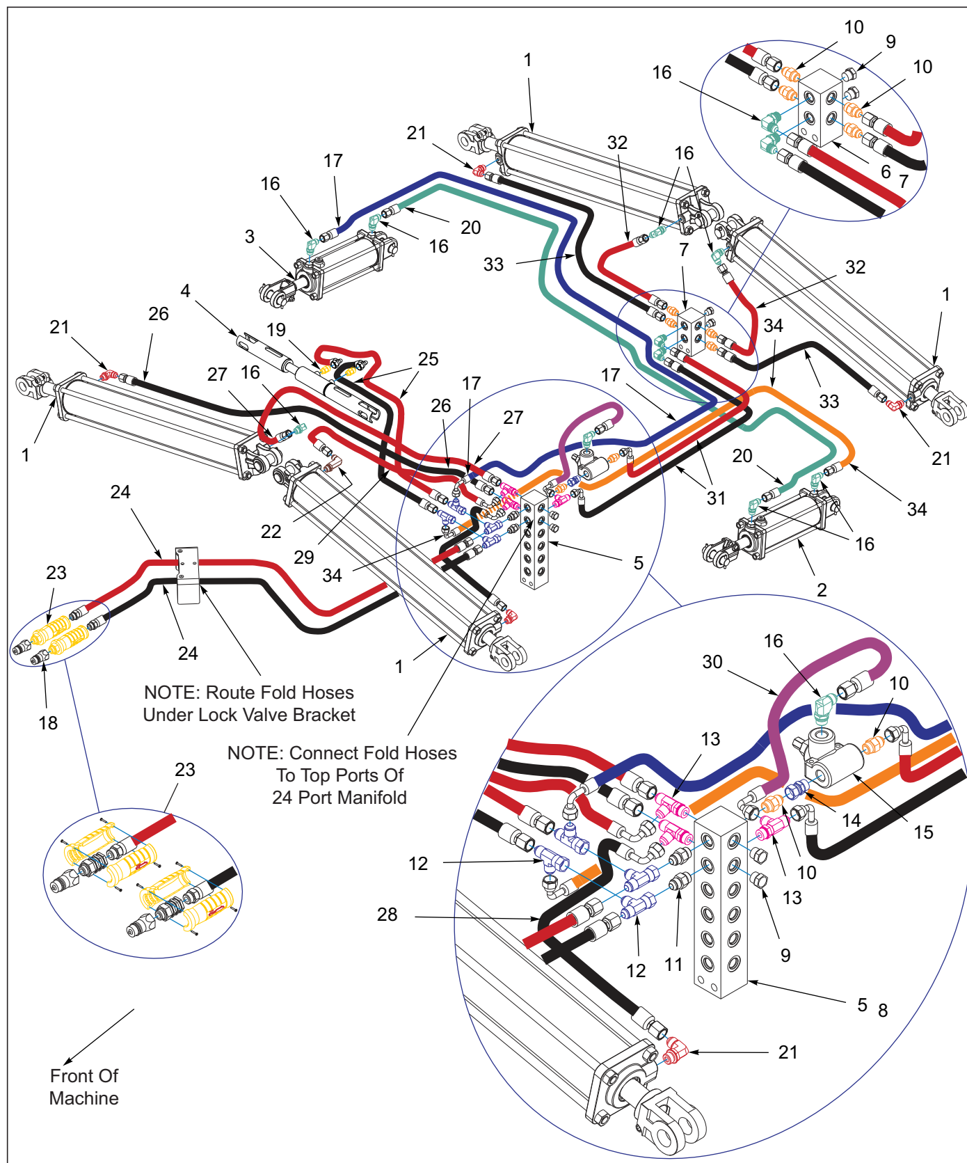
Figure 5-13: Hydraulic Assembly Fold 7531-26'-29' (After S/N 75K2501921 To S/N 75F2602020)
