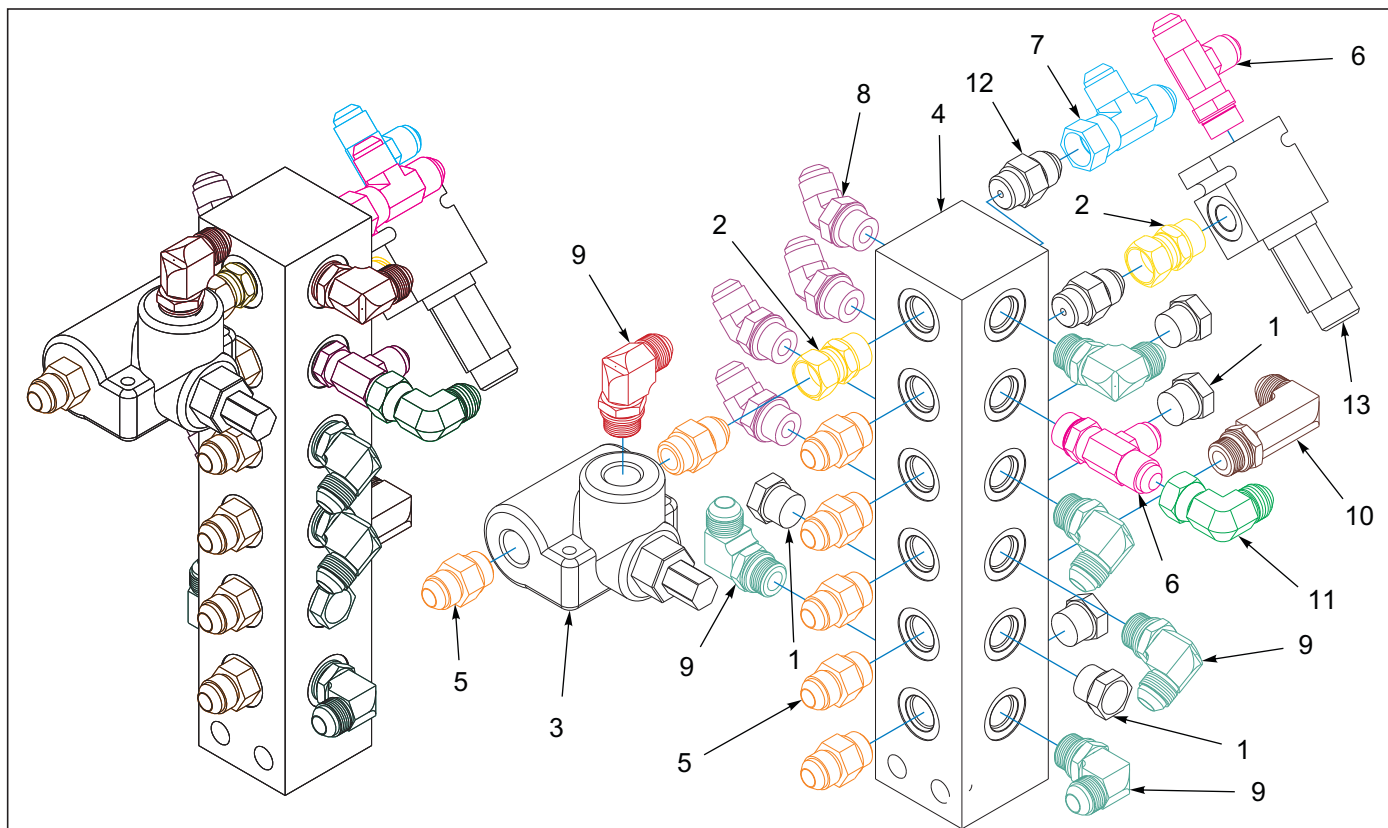
Figure 5-30: Manifold Assembly Front 7531-32'-35' (After S/N 75K2602020)
