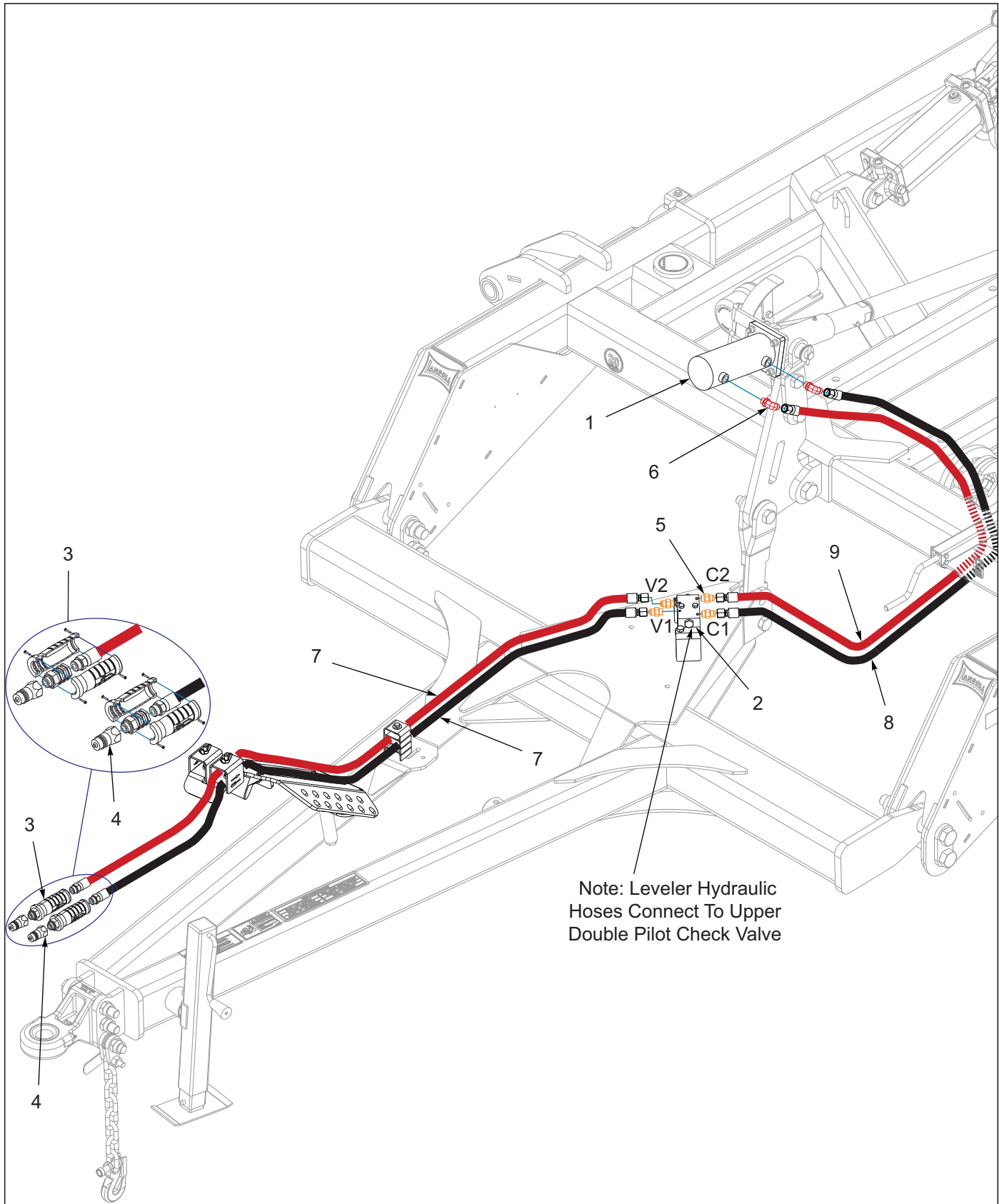
Figure 5-21: Hydraulic Assembly Leveler
