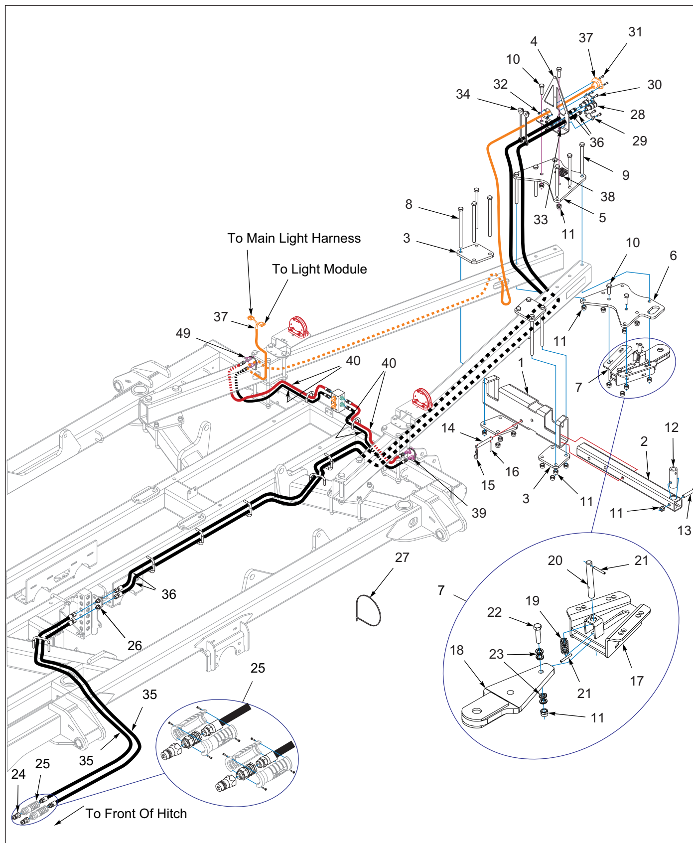
Figure 9-31: Rear Tow Assembly 7531-23'-26'-29' (2 of 2)
