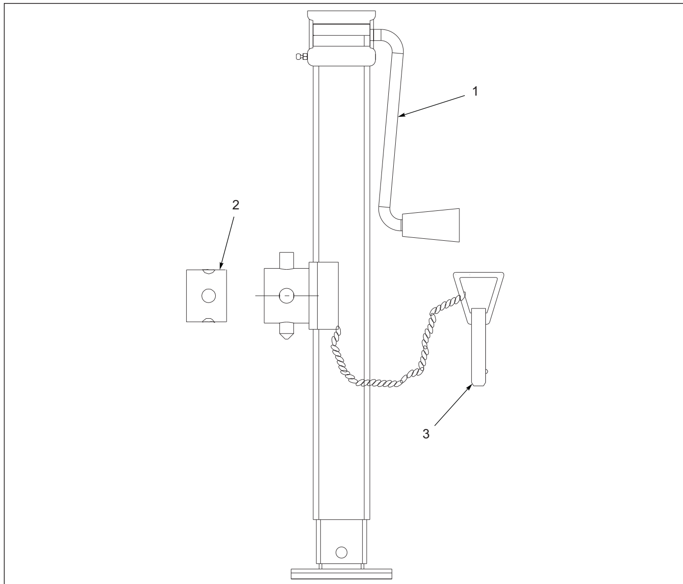
Figure 2-4: Jack Assembly
