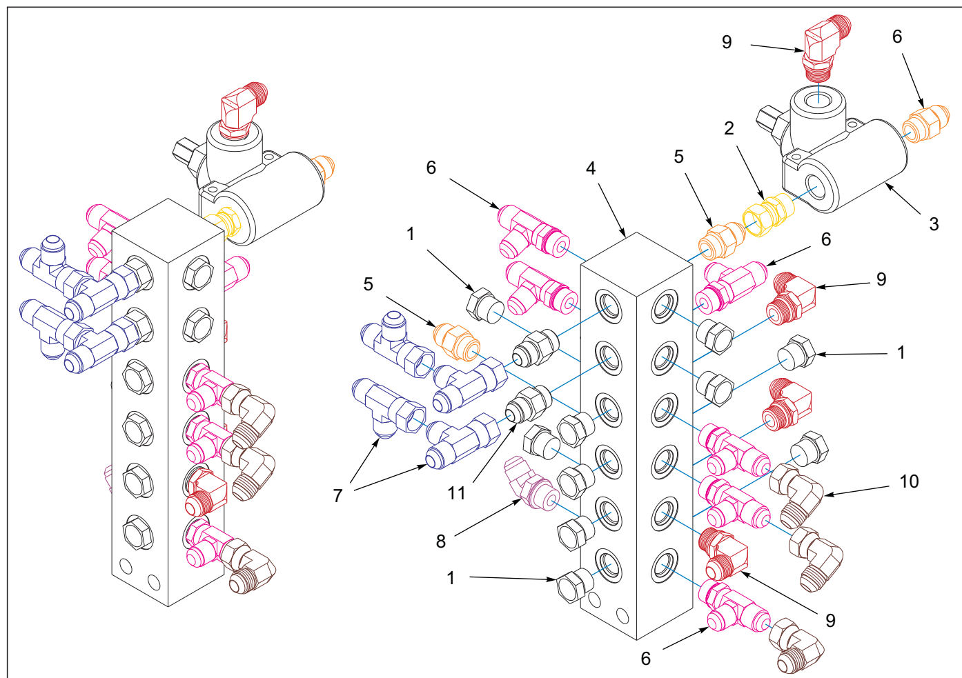
Figure 5-24: Manifold Assembly Front 7531-26'/29' (After S/N 75K2501921 To S/N 75F2602020)
