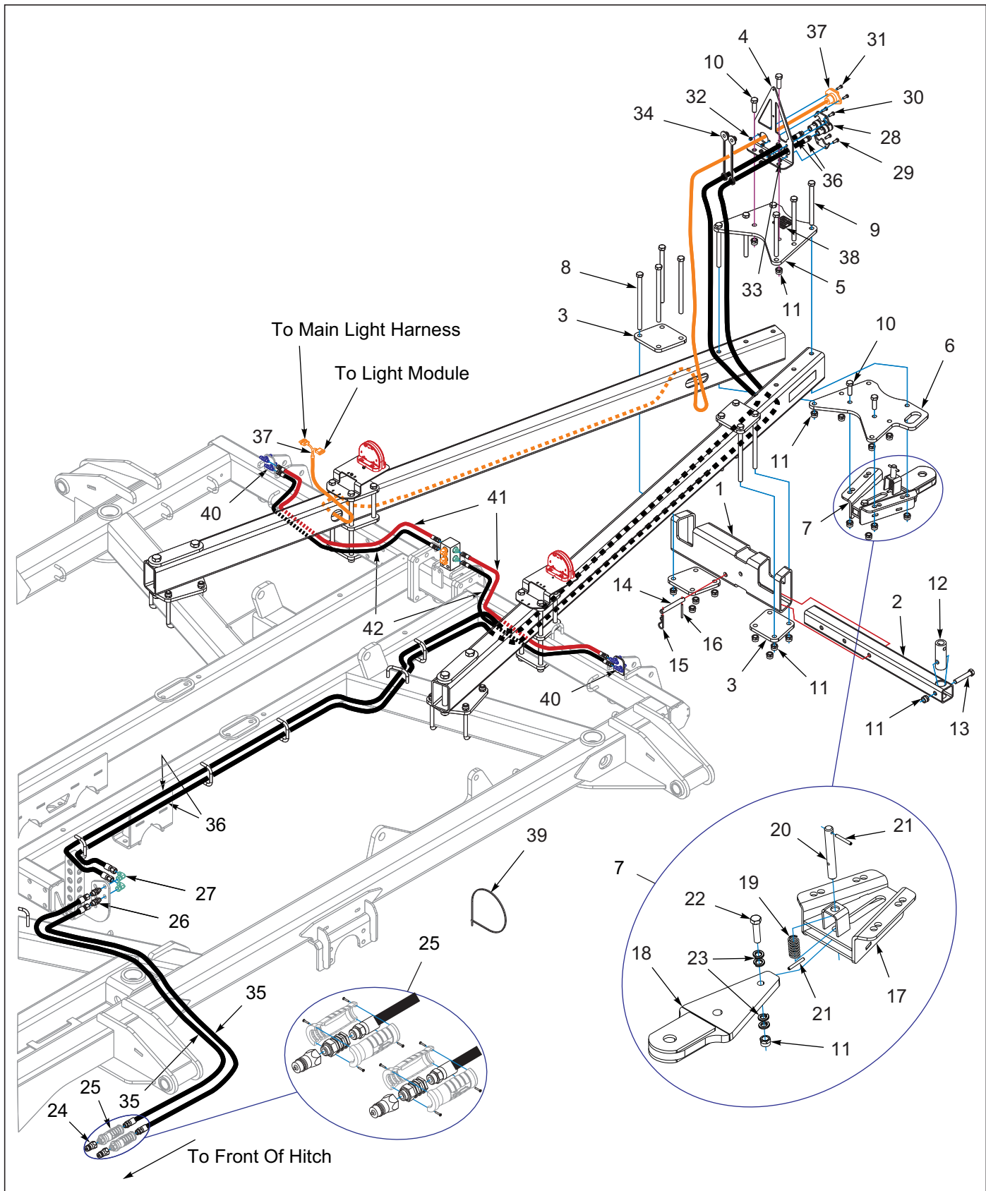
Figure 9-33: Rear Tow Assembly 7531-32'-35' (2 of 2)
