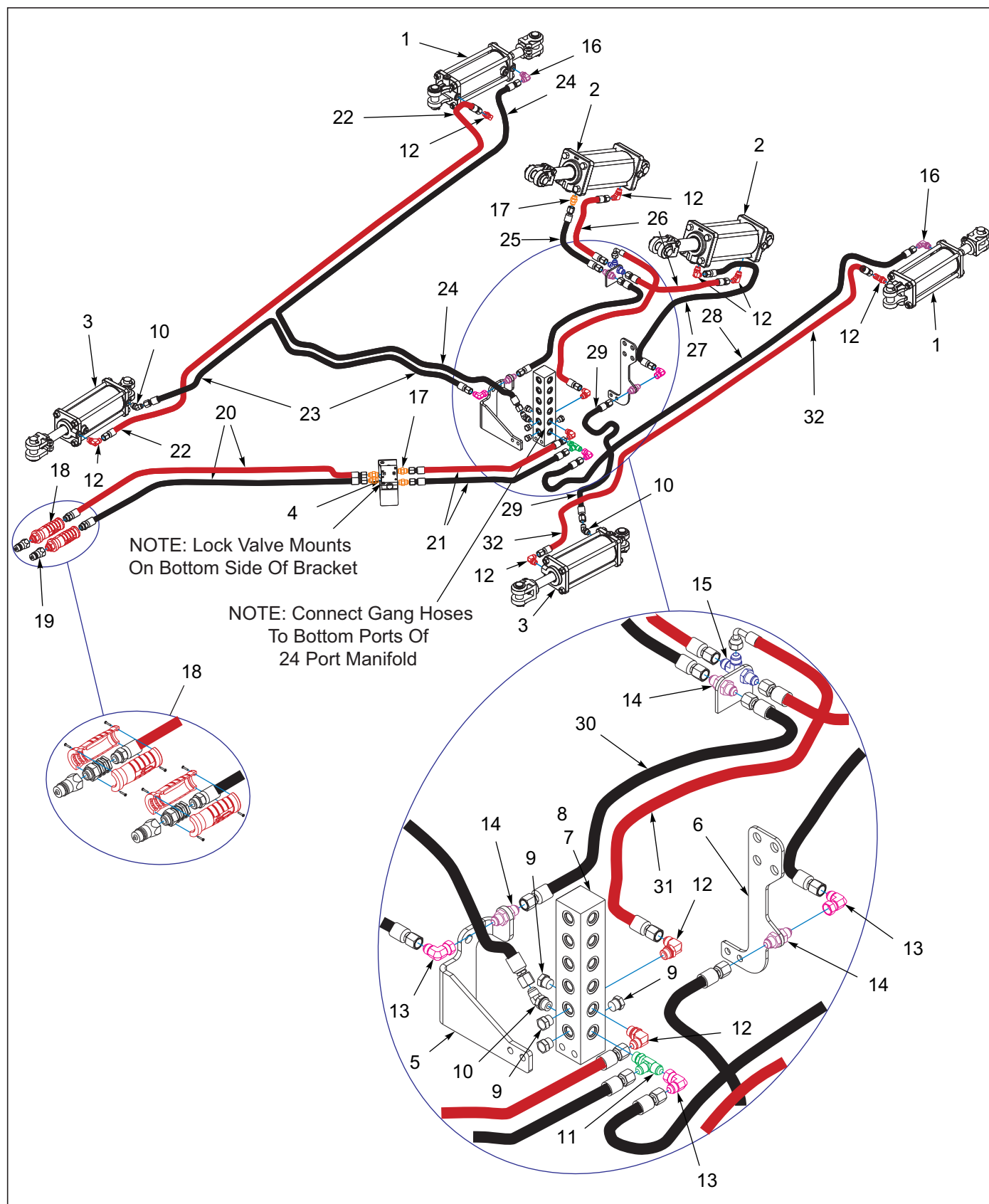
Figure 5-18: Hydraulic Assembly Gang 7531-23'
