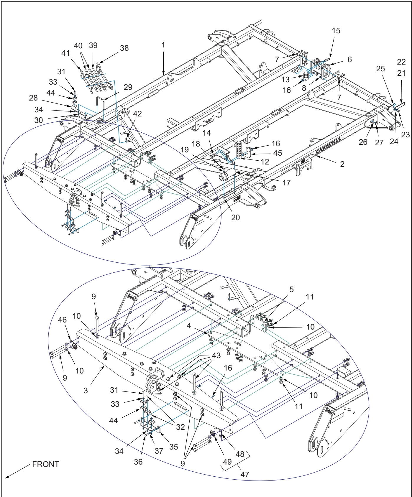
Figure 1-2: Frame Assembly 32'-35'
