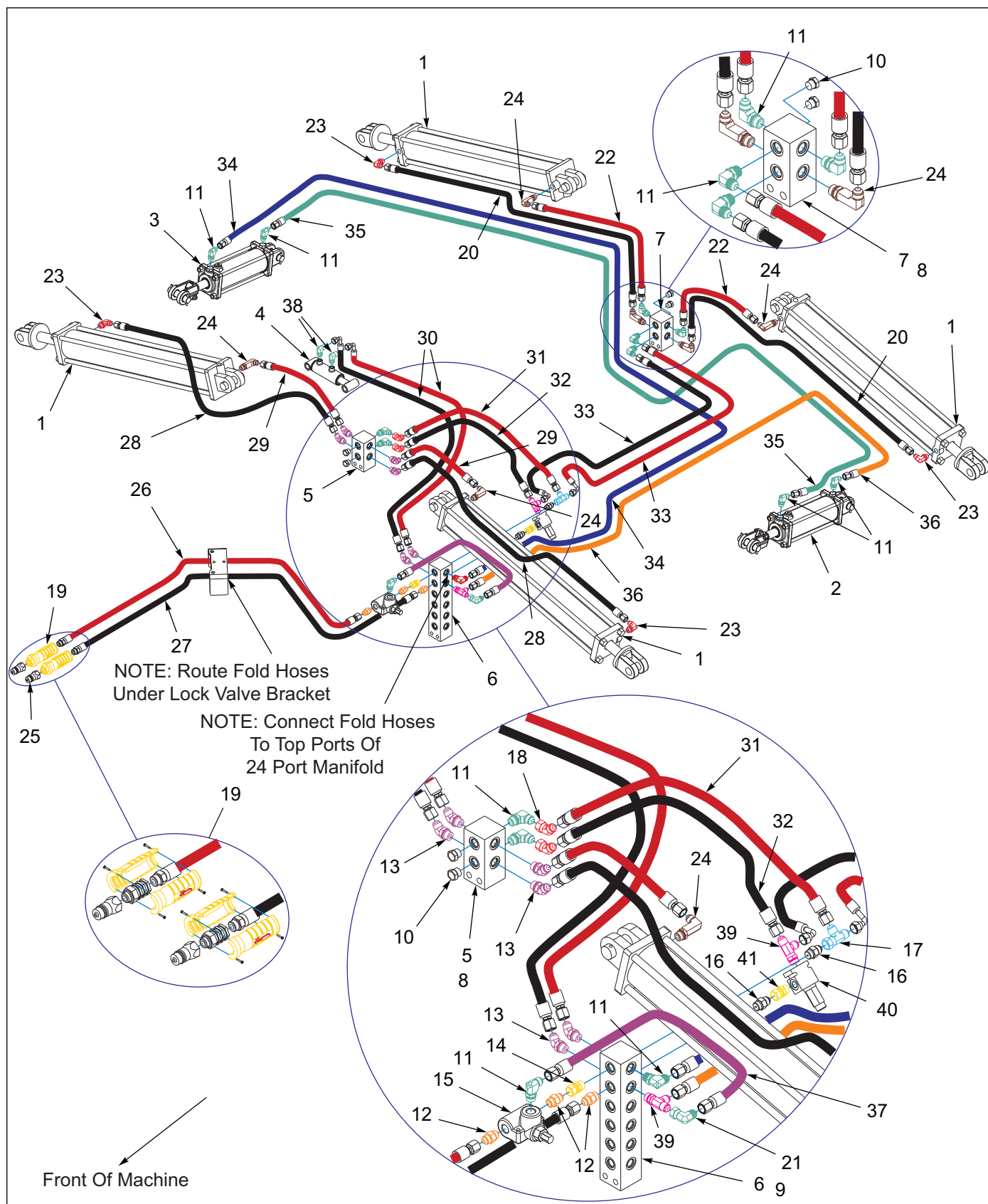
Figure 5-17: Hydraulic Assembly Fold 7531-32'-35' (After S/N 75F2602020)
