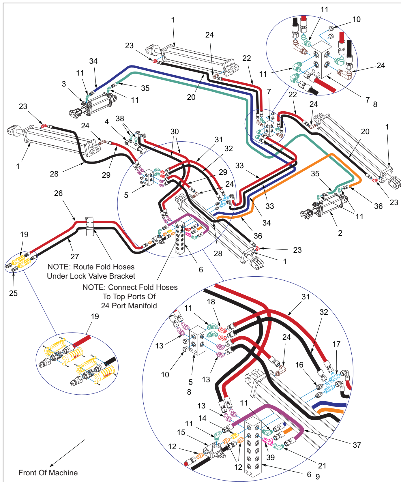
Figure 5-16: Hydraulic Assembly Fold 7531-32'-35' (After S/N75K2501921 To S/N75F2602020)
