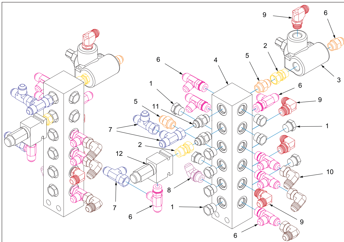
Figure 5-25: Manifold Assembly Front 7531-26'/29' (After S/N 75F2602020)
