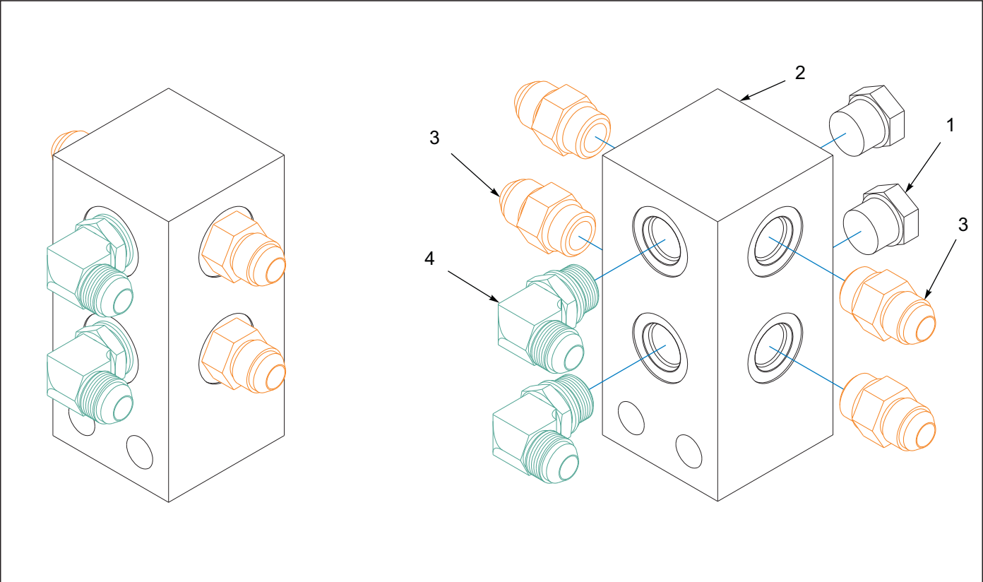
Figure 5-27: Manifold Assembly Front 7531-26’/29’ (After S/N 75K2501921)
