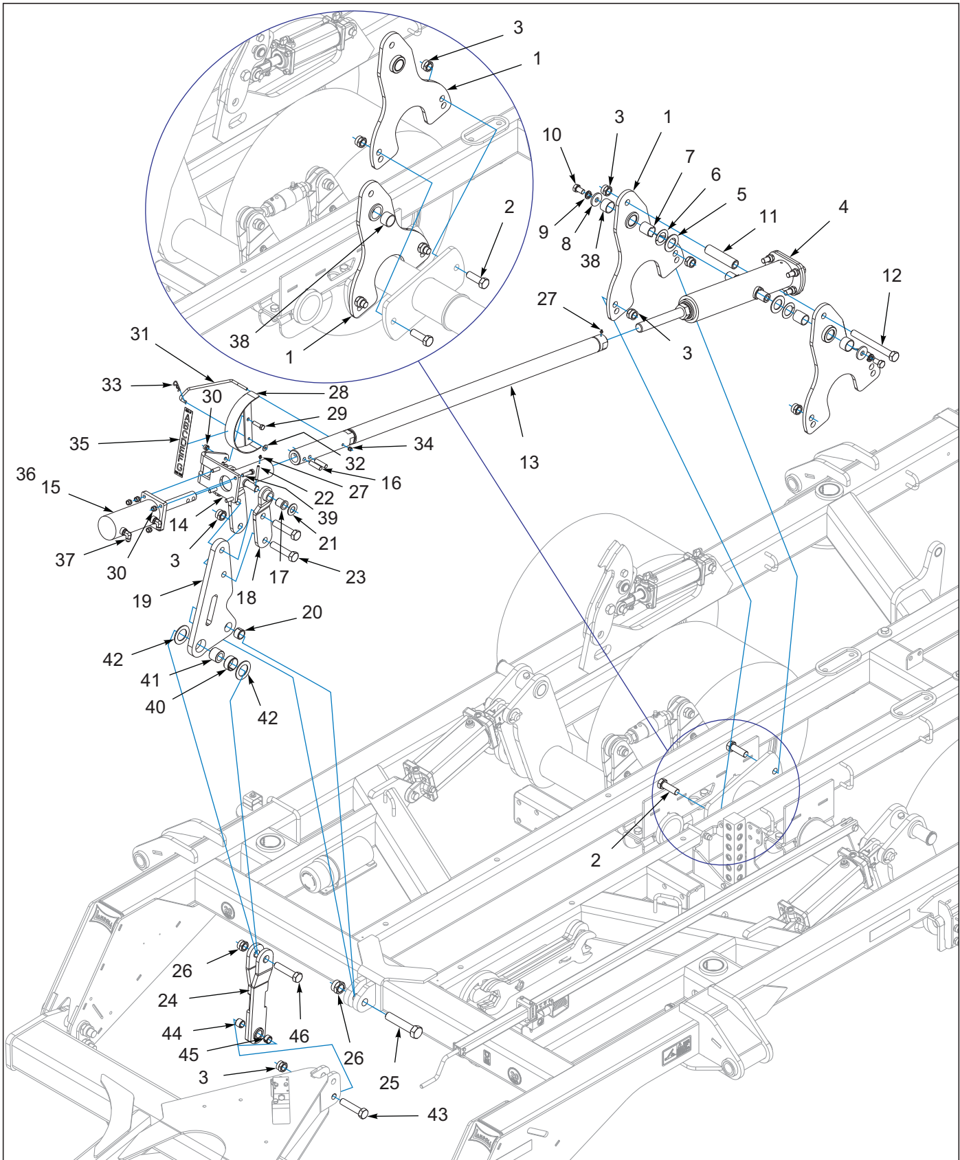
Figure 2-2: Hydraulic Leveler Assembly
