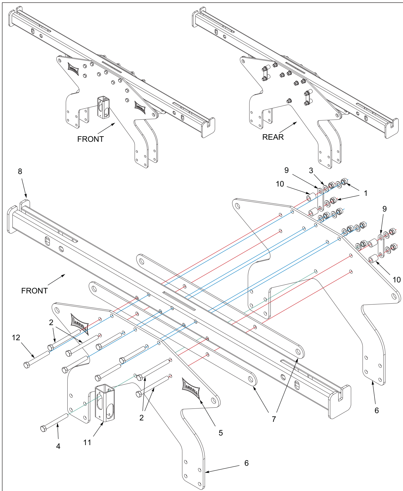
Figure 5-9: Wing Fold Stabilizer Assembly 7531-32'-35' Rear
