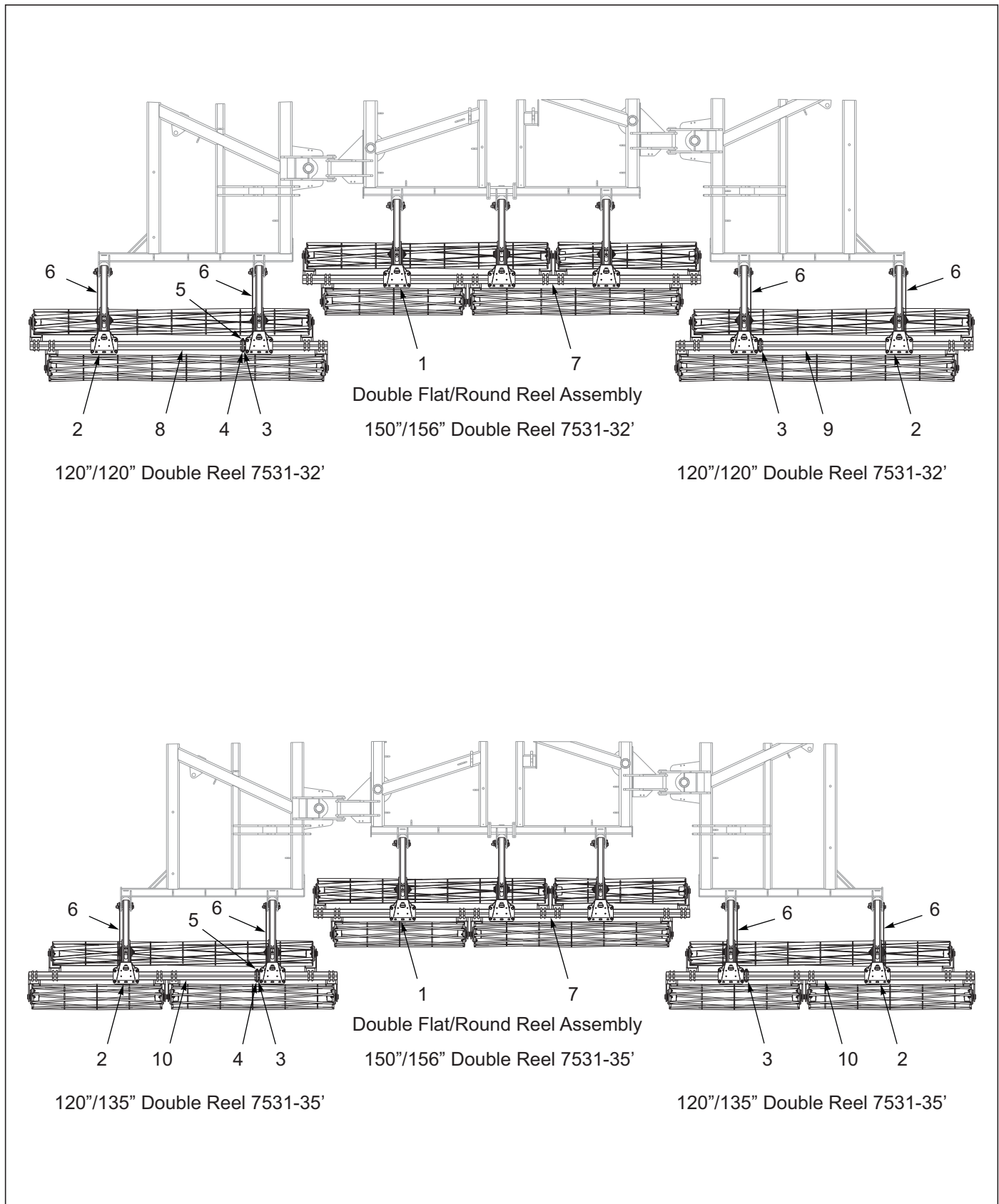
Figure 9-8: Double Flat/Round Reel Assembly 7531-32'-35'
