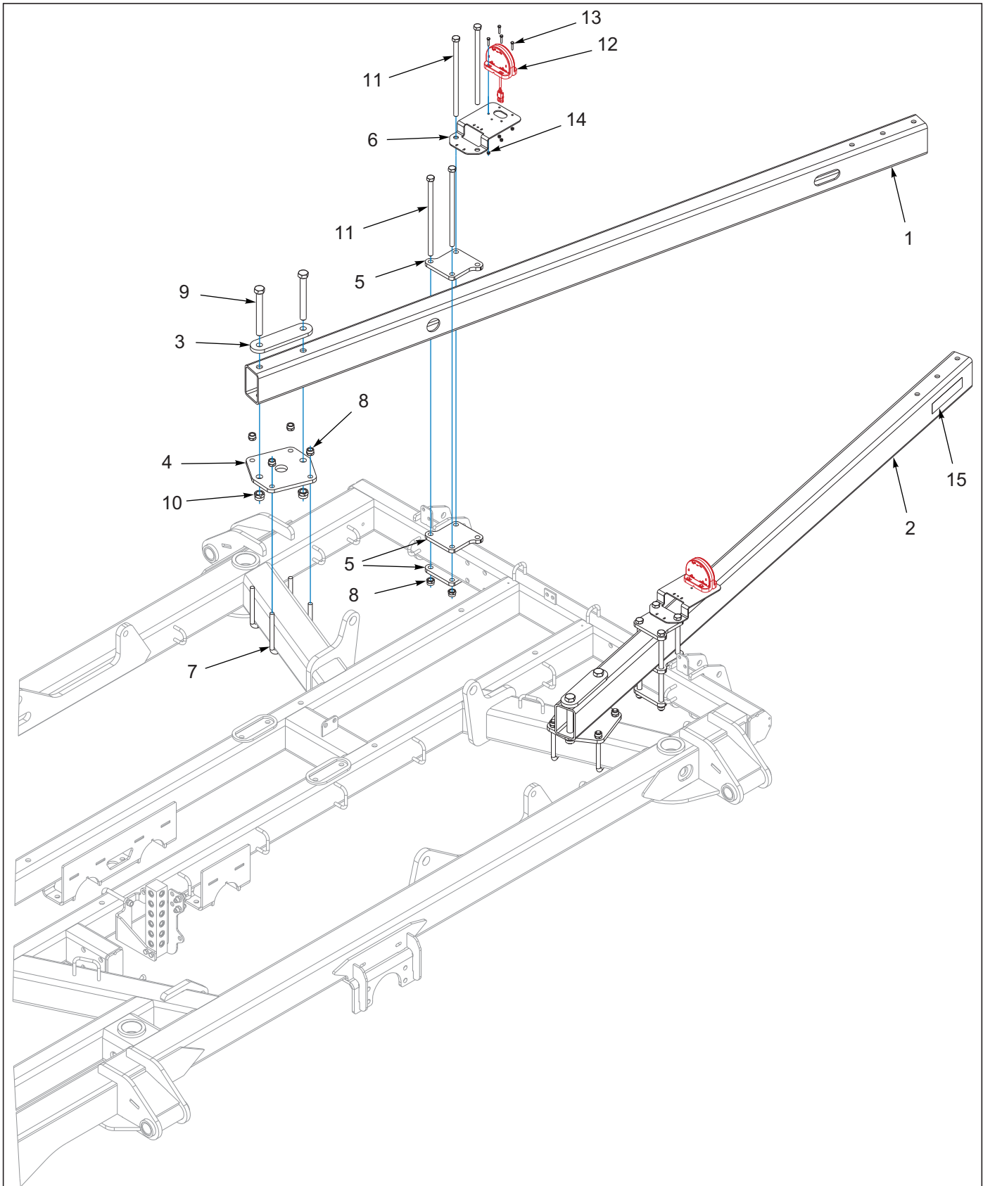
Figure 9-30: Rear Tow Assembly 8531-23'-26'-29' (1 of 2)
