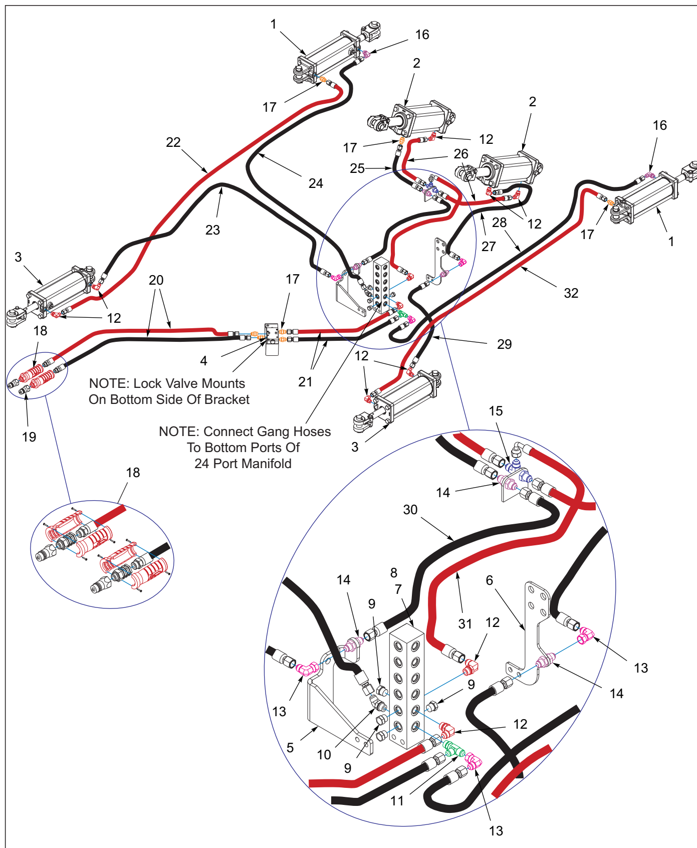
Figure 5-19: Hydraulic Assembly Gang 7531-26'-29'
