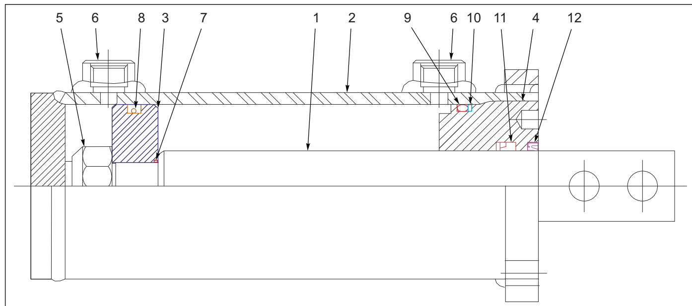
Figure 6-24: Cylinder Assembly 3-1/2 x 6
