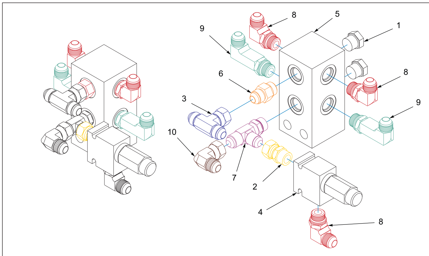
Figure 5-32: Manifold Assembly Rear 7531-32'-35' (Before S/N 75K2501921)
