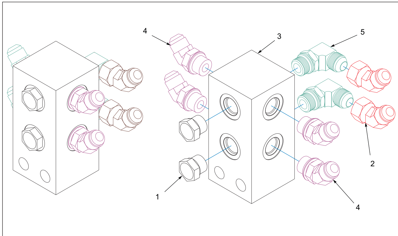
Figure 5-31: Manifold Assembly Front 7531-32'-35'
