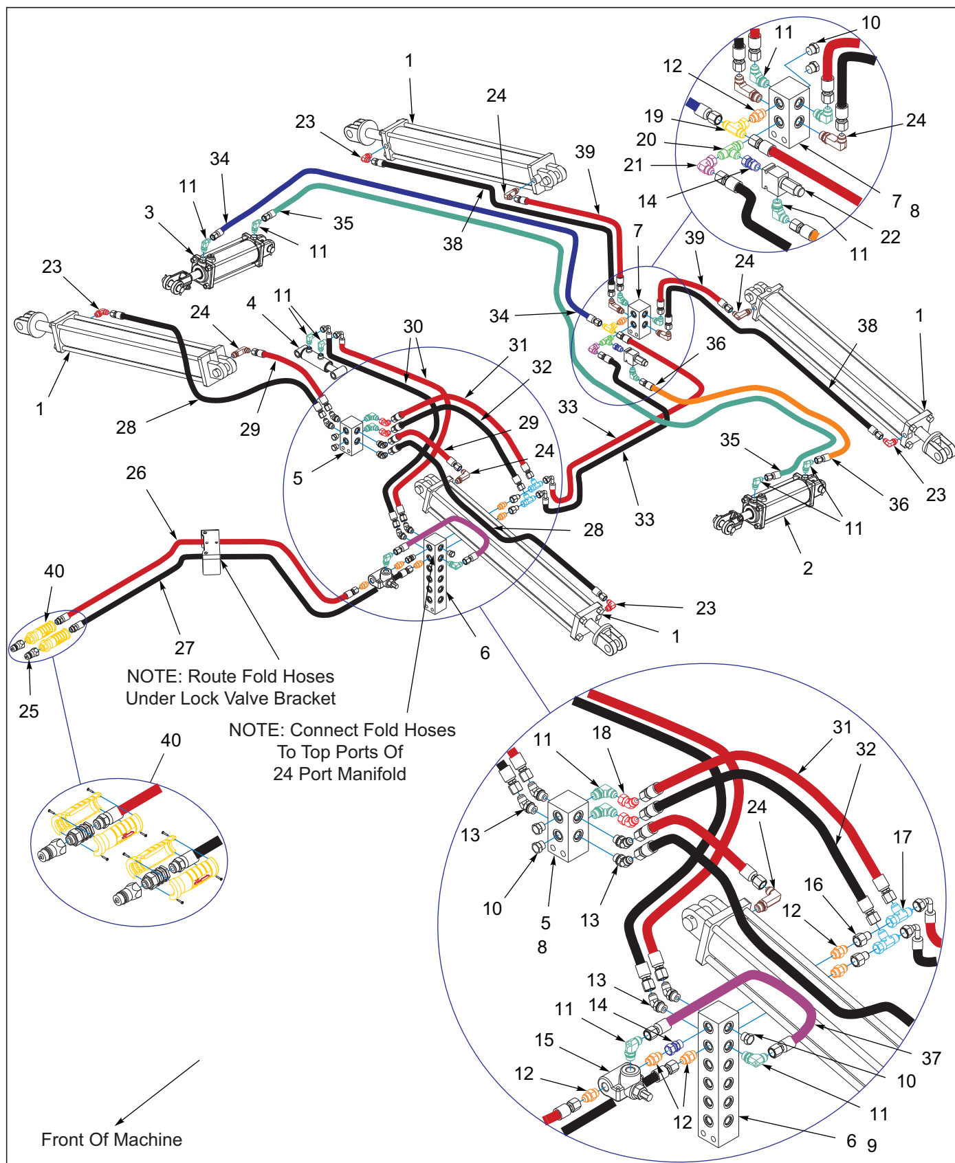
Figure 5-15: Hydraulic Assembly Fold 7531-32'-35' (Before S/N 75K2501921)
