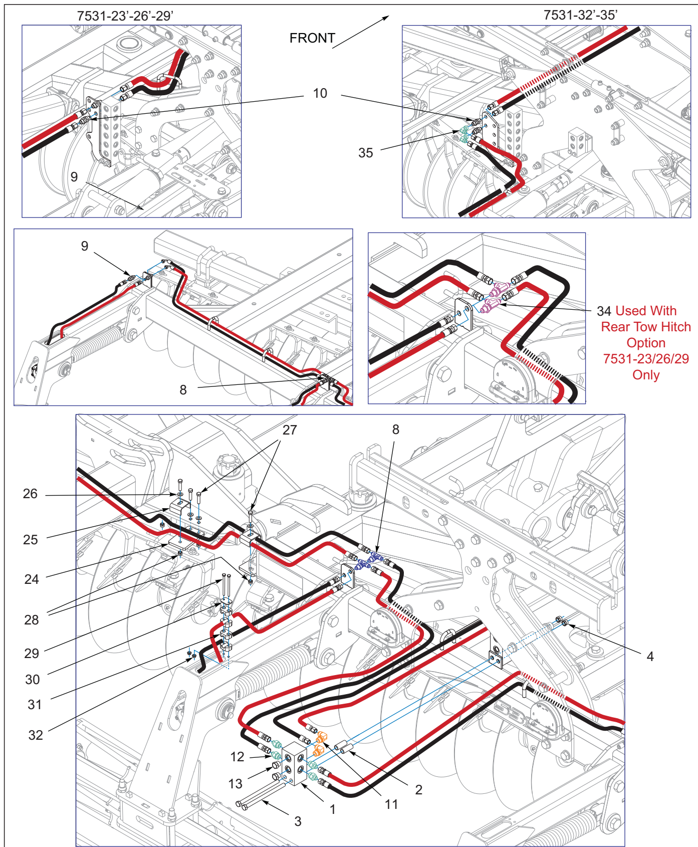
Figure 9-29: Reel Hydraulic Assembly (2 of 2)
