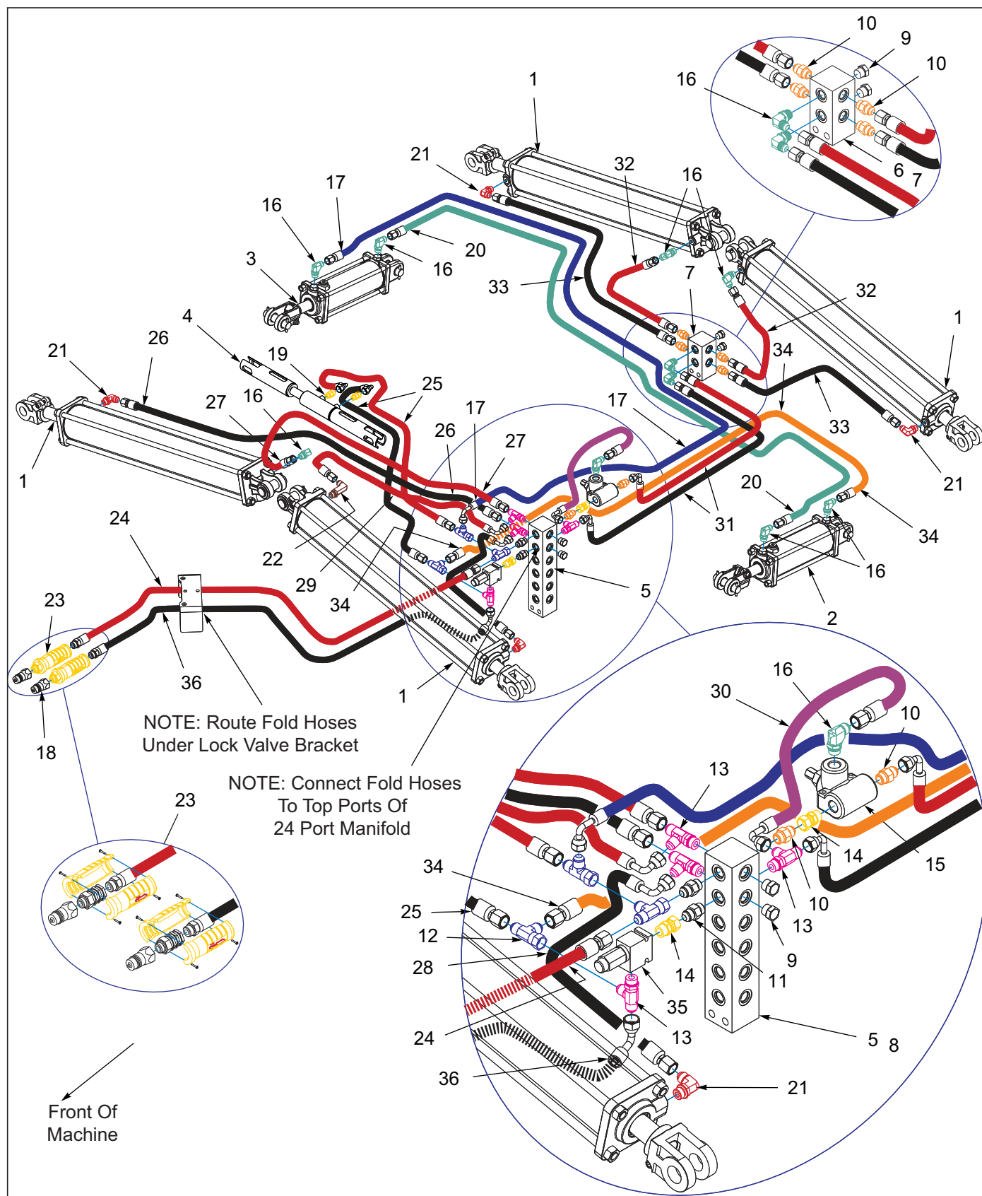
Figure 5-14: Hydraulic Assembly Fold 7531-26'-29' (After S/N 75F2602020)
