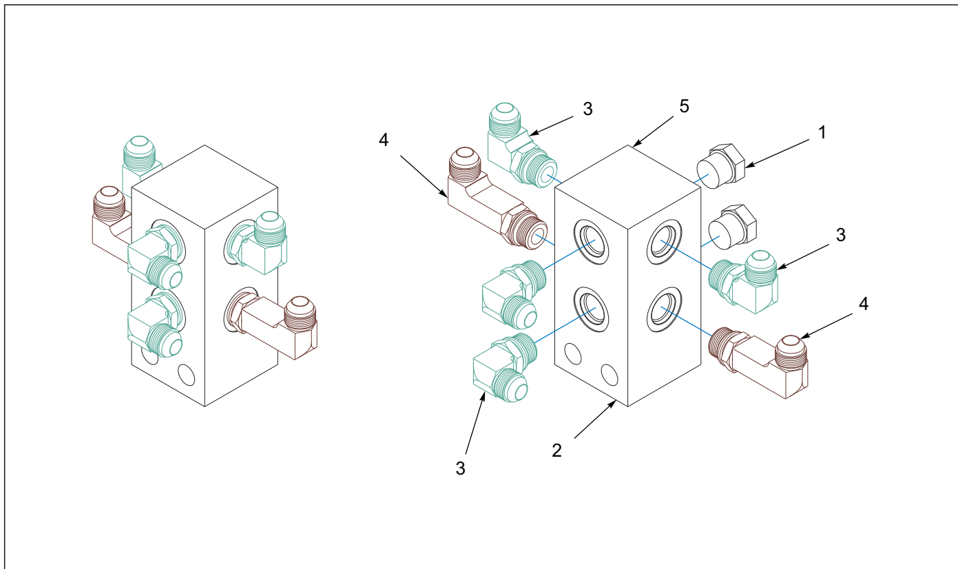
Figure 5-33: Manifold Assembly Rear 7531-32'-35' (After S/N 75K2501921)
