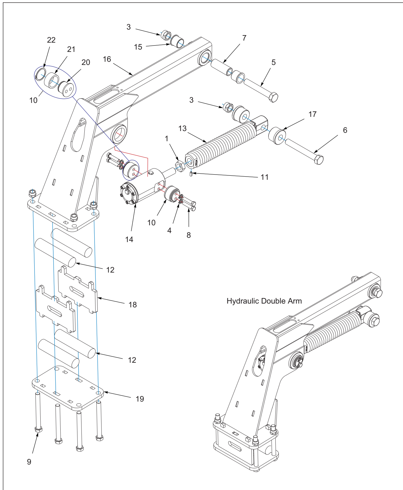
Figure 9-16: Hydraulic Double Arm Assembly
