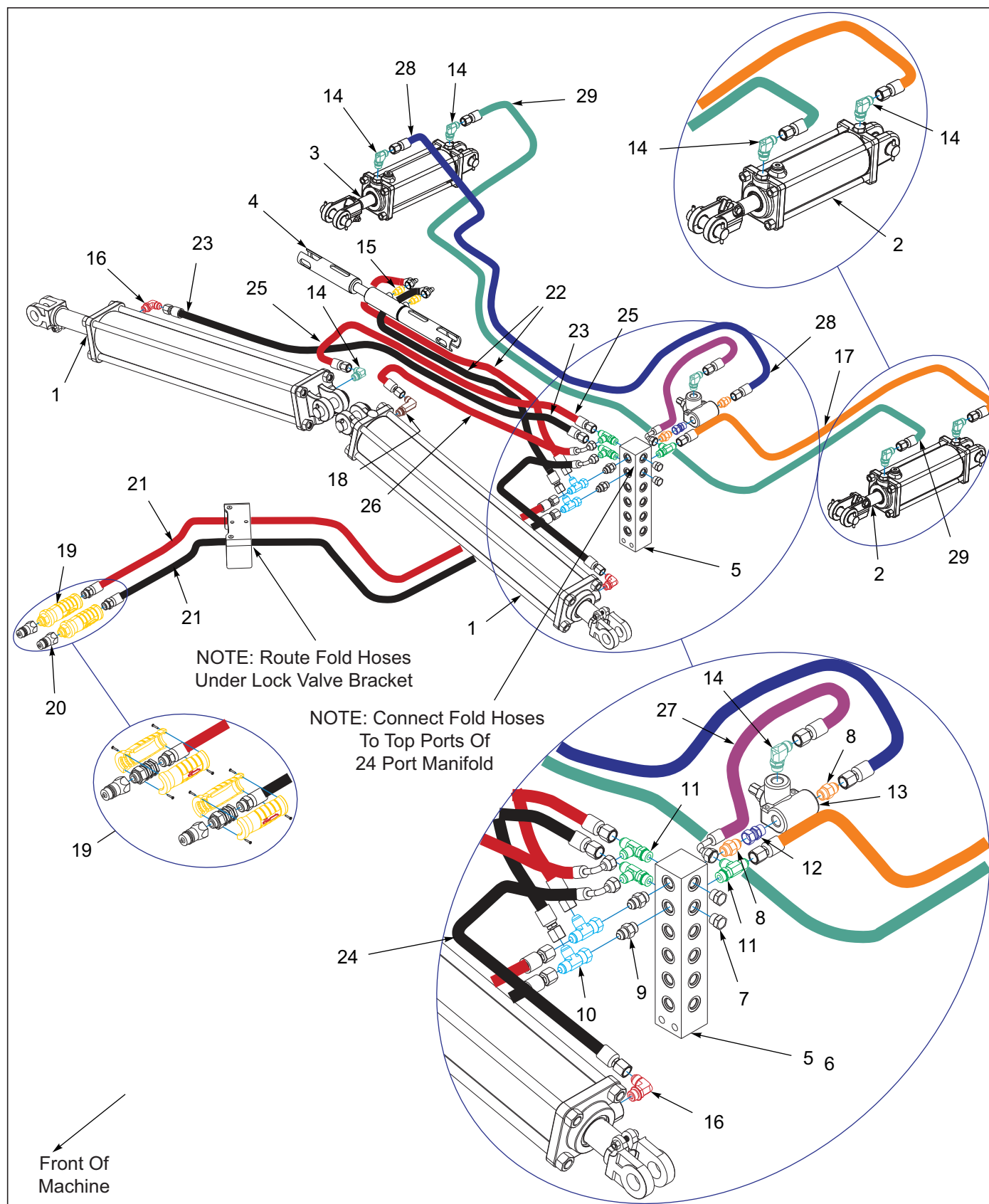
Figure 5-10: Hydraulic Assembly Fold 7531-23' (Before S/N 75F2602020)
