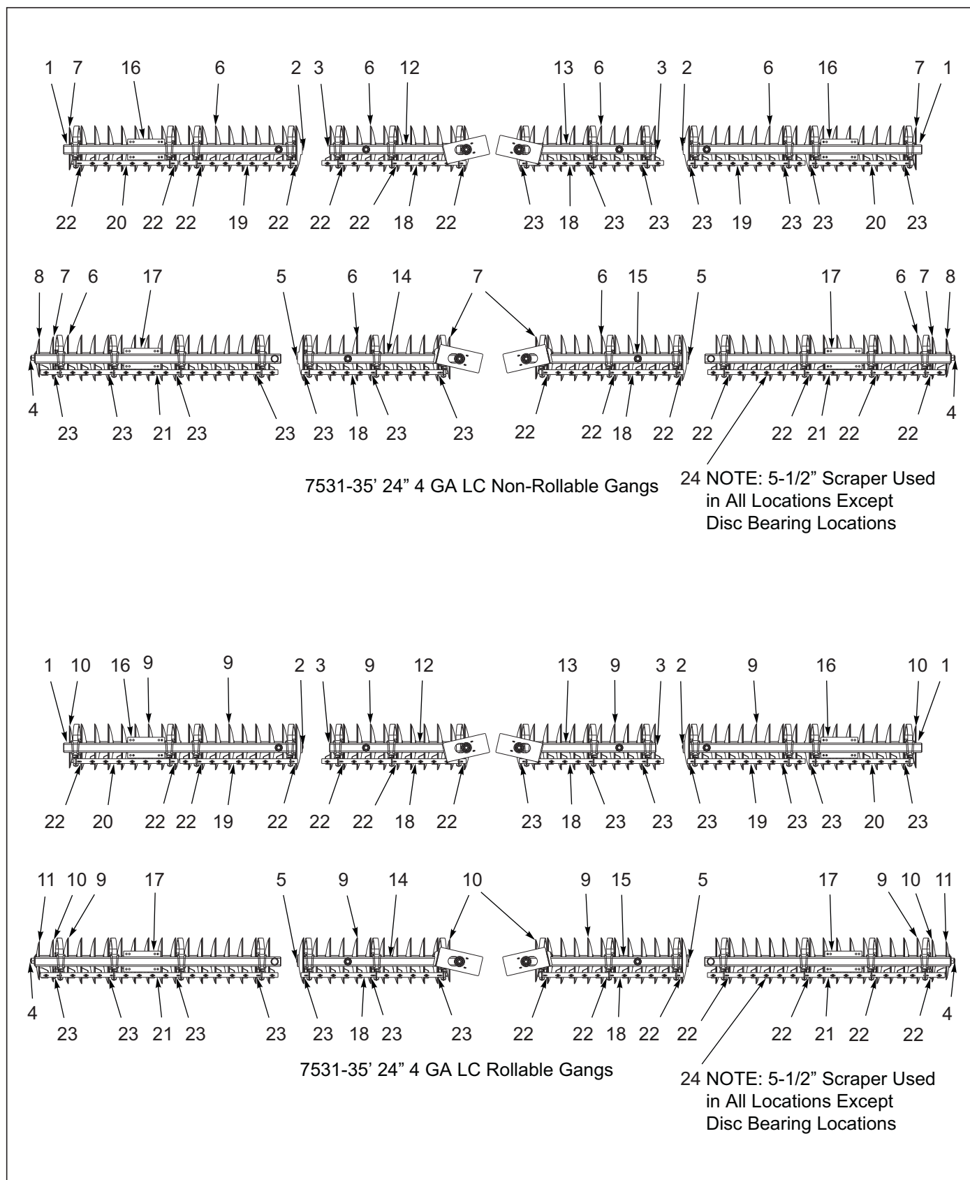
Figure 4-12: Disc Gang Assembly 7531-35'
