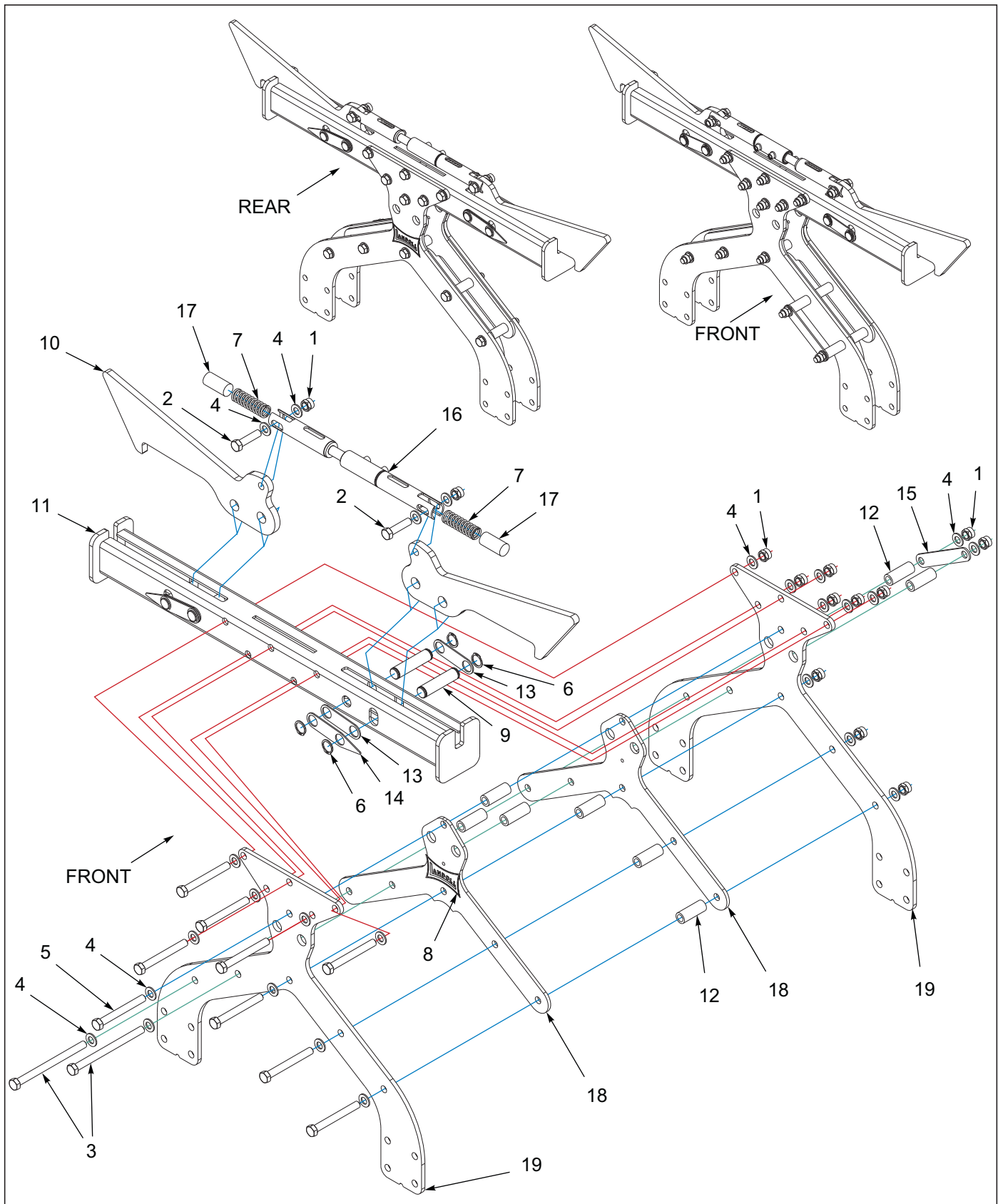
Figure 5-4: Wing Fold Stabilizer Assembly 7531-23'
