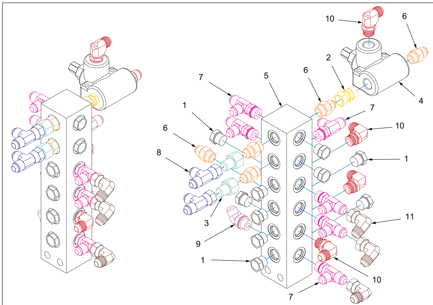
Figure 5-23: Manifold Assembly Front 7531-26'/29' (Before S/N 75K2501921)
