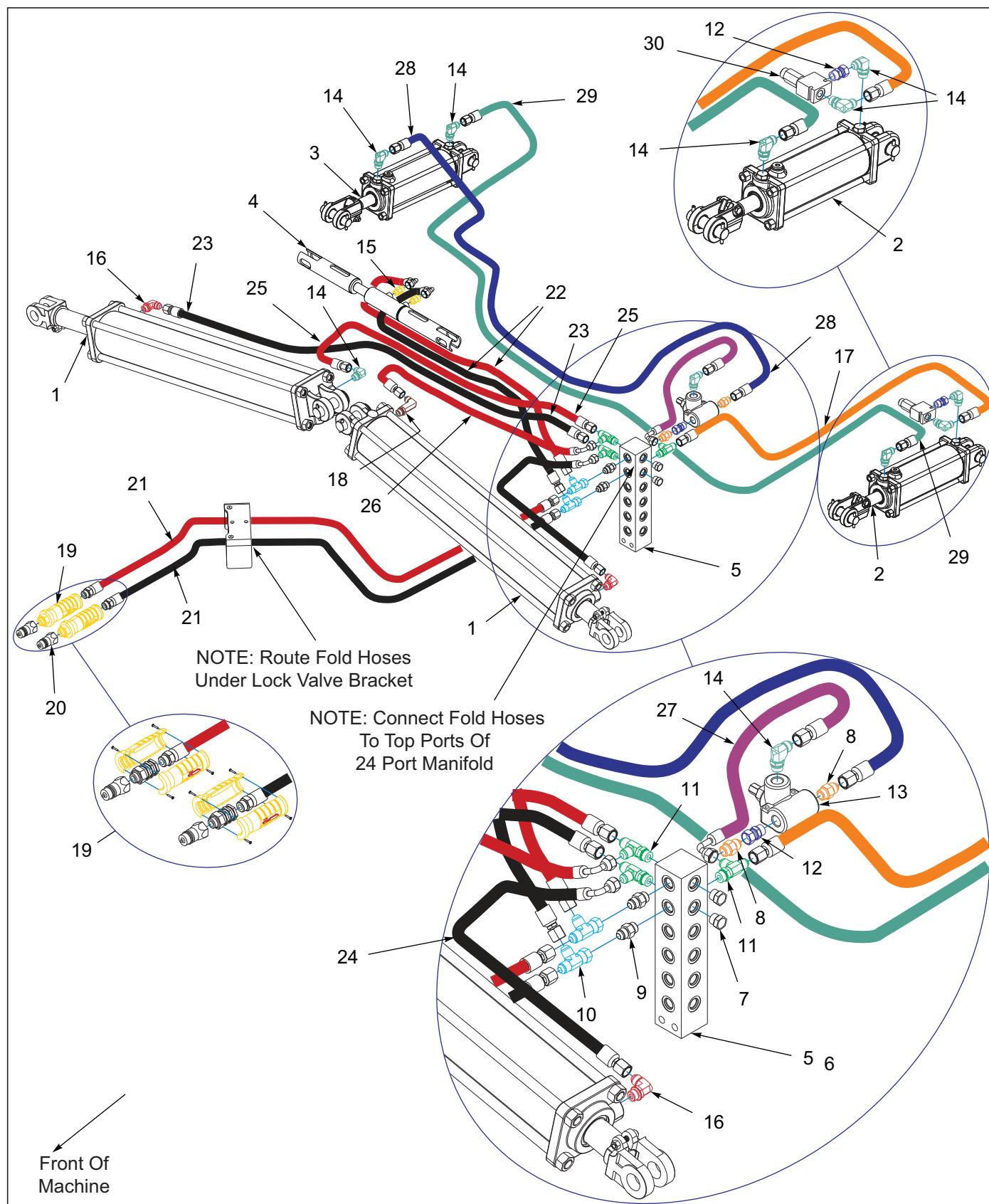
Figure 5-11: Hydraulic Assembly Fold 7531-23' (After S/N 75F2602020)
