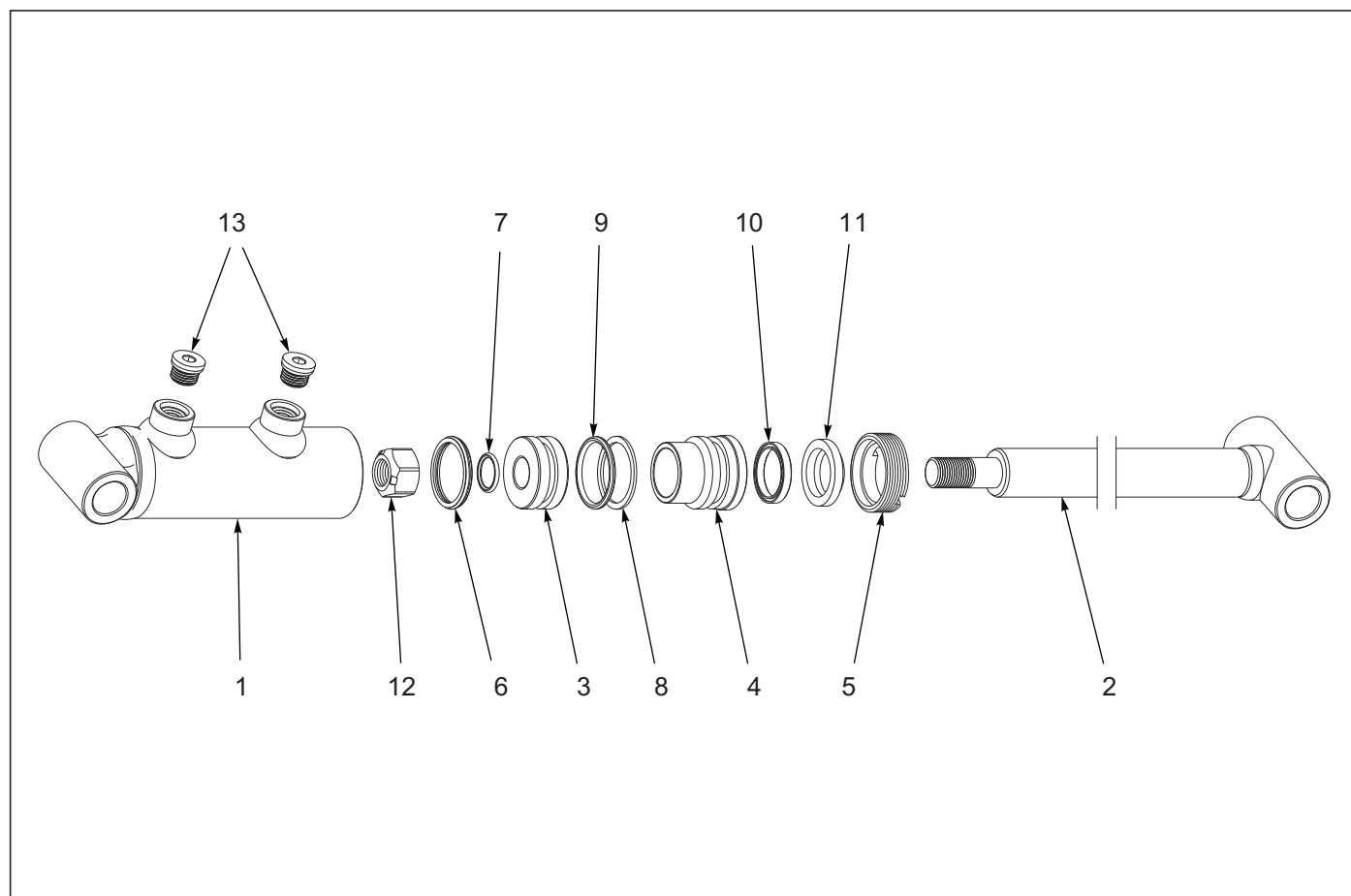
Figure 6-26: Cylinder Assembly 1-1/2 x -1-1/2
