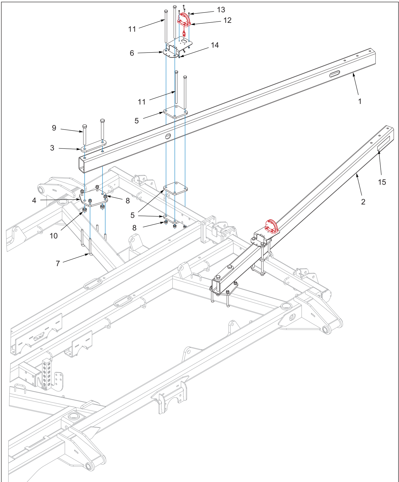
Figure 9-32: Rear Tow Assembly 7531-32'-35' (1 of 2)
