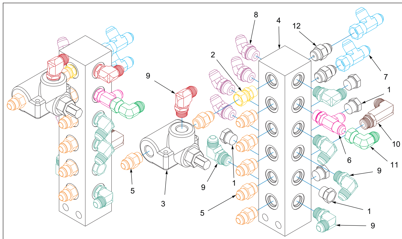
Figure 5-29: Manifold Assembly Front 7531-32'-35' (After S/N 75K2501921 To) S/N 75K2602020
