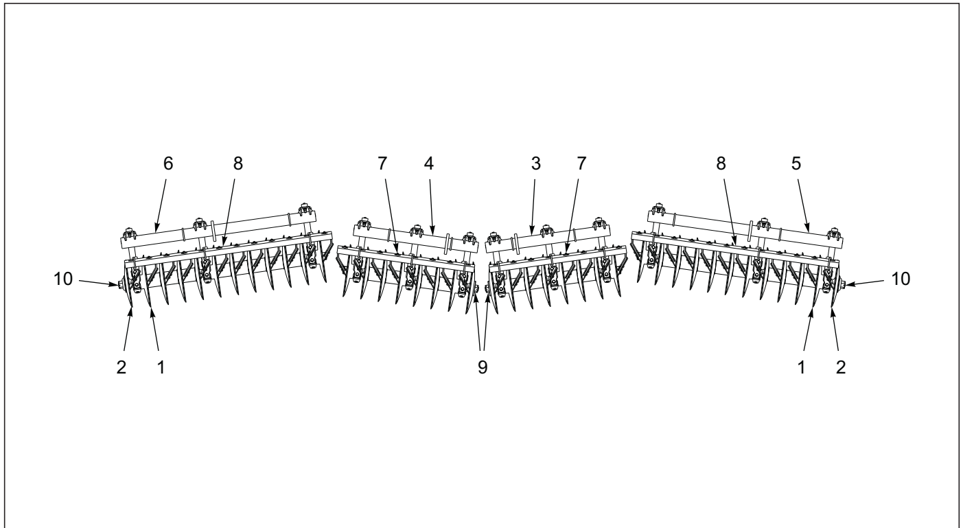
Figure 4-8: Gang Assembly 22" 4 GA 8530-25'
