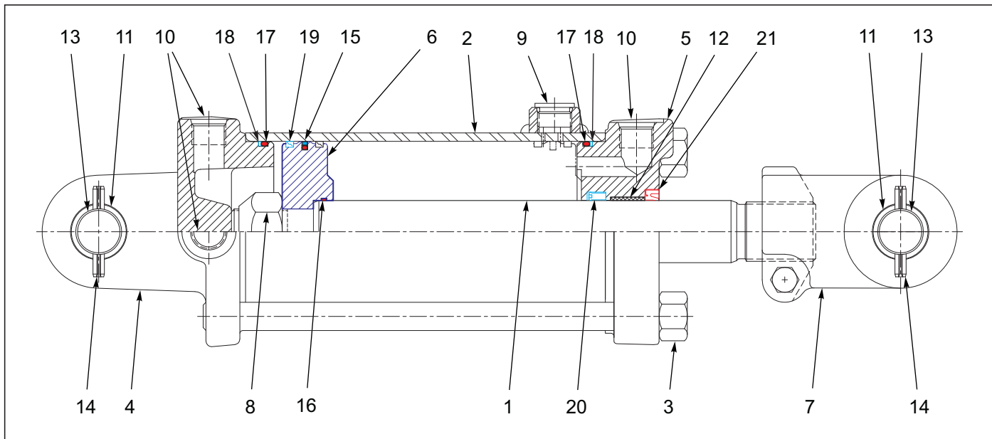
Figure 7-3: Cylinder Assembly 3-3/4 x 8, Rephase (Prince)
