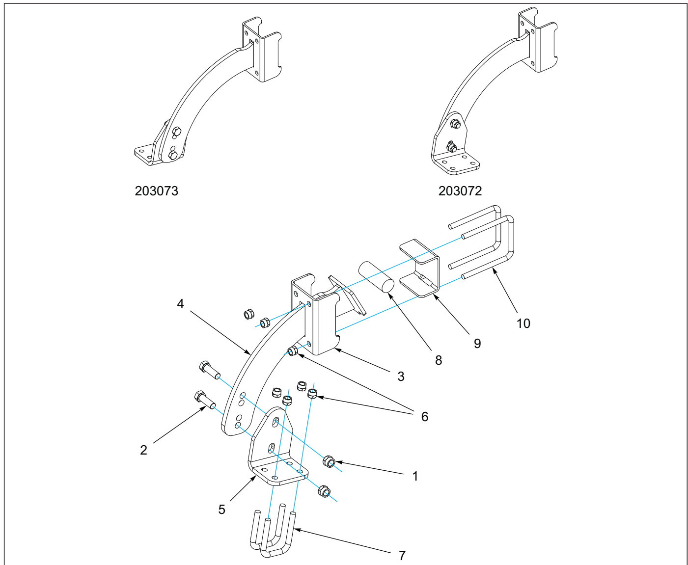
Figure 4-20: Disc Gang Reel Arm Assembly
