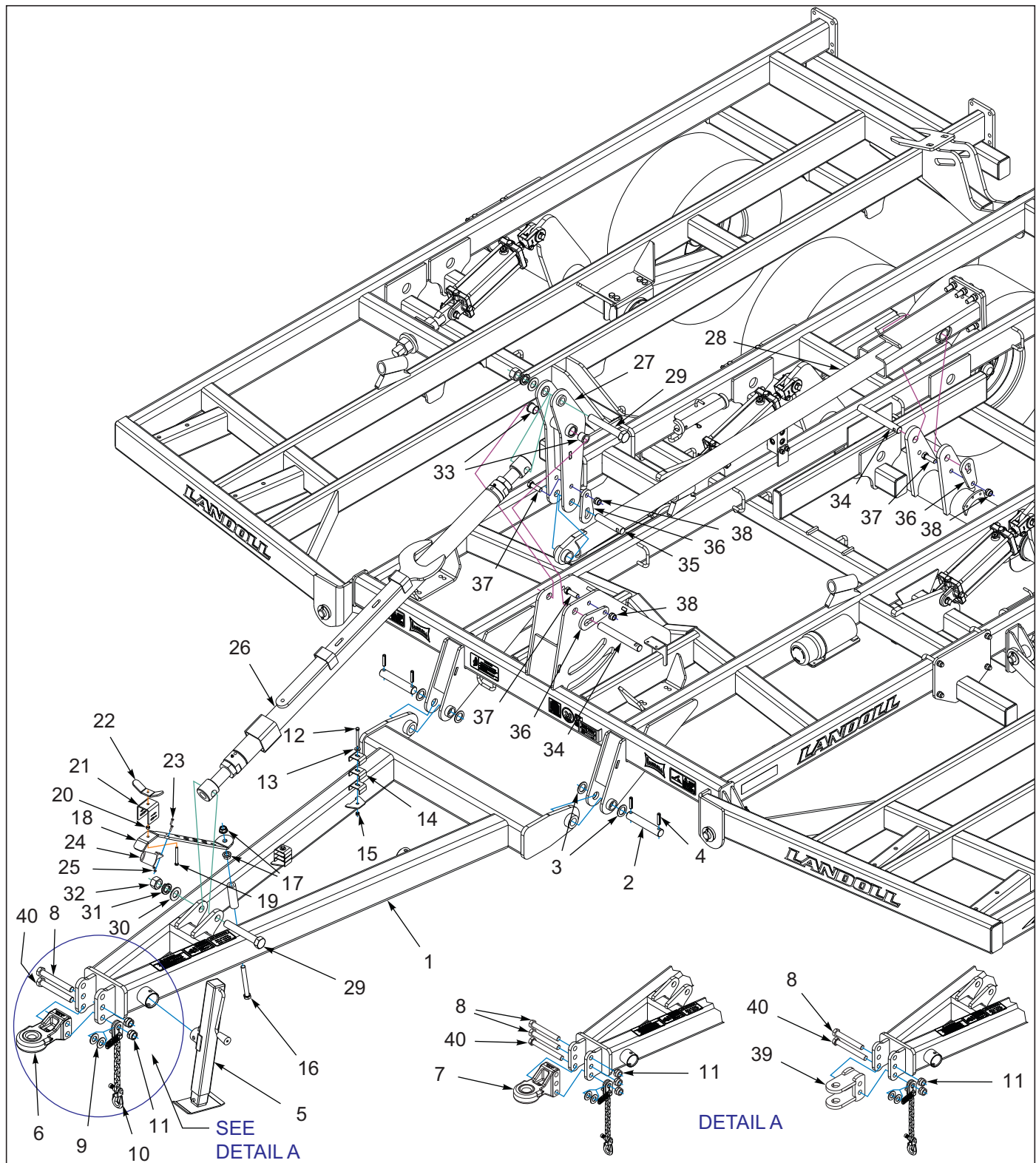
Figure 2-1: Hitch & Leveling Assembly 8530-19'-25'
