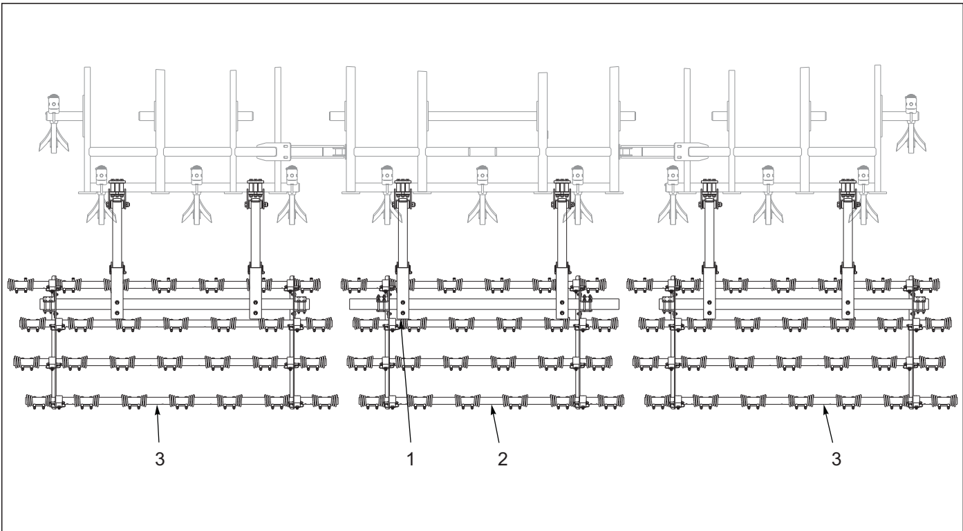
Figure 10-3: 4 Row Coil Tine Harrow Layout 8530-25'
