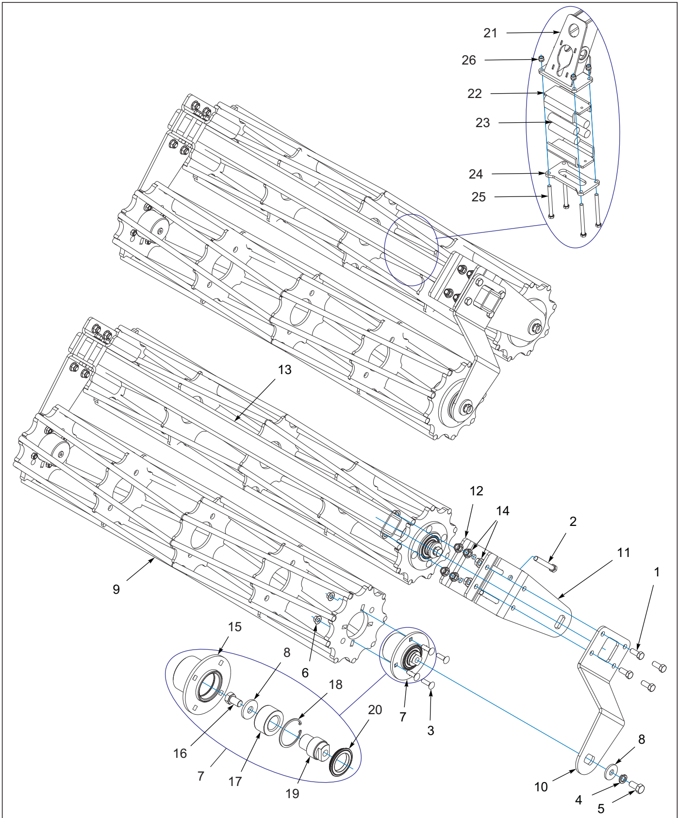
Figure 10-60: Double Conditioner Reel Assembly
