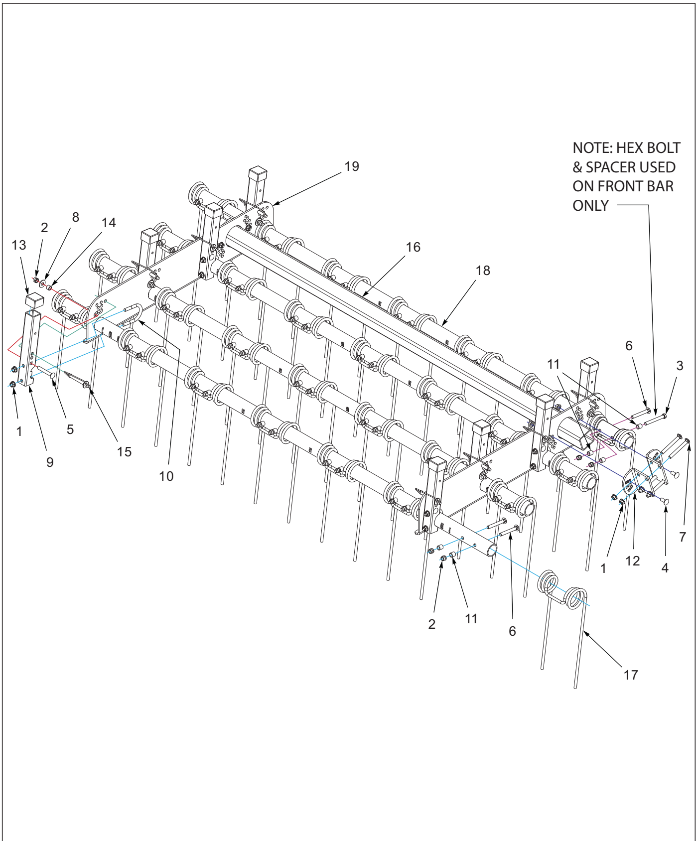
Figure 10-9: 4 Row Coil Tine Harrow Assembly
