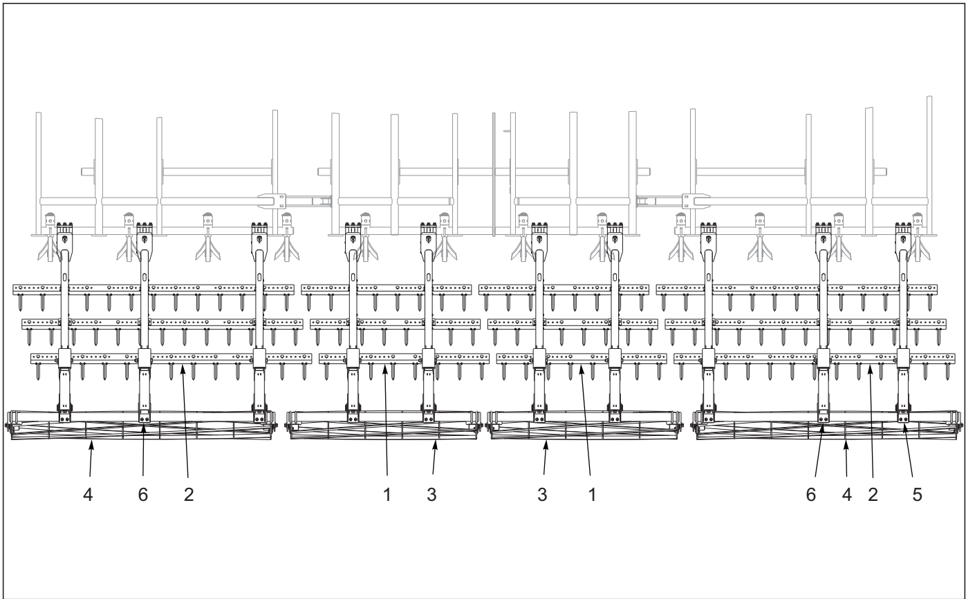
Figure 10-39: 3 Row Spike & Reel Layout 8530-30'
