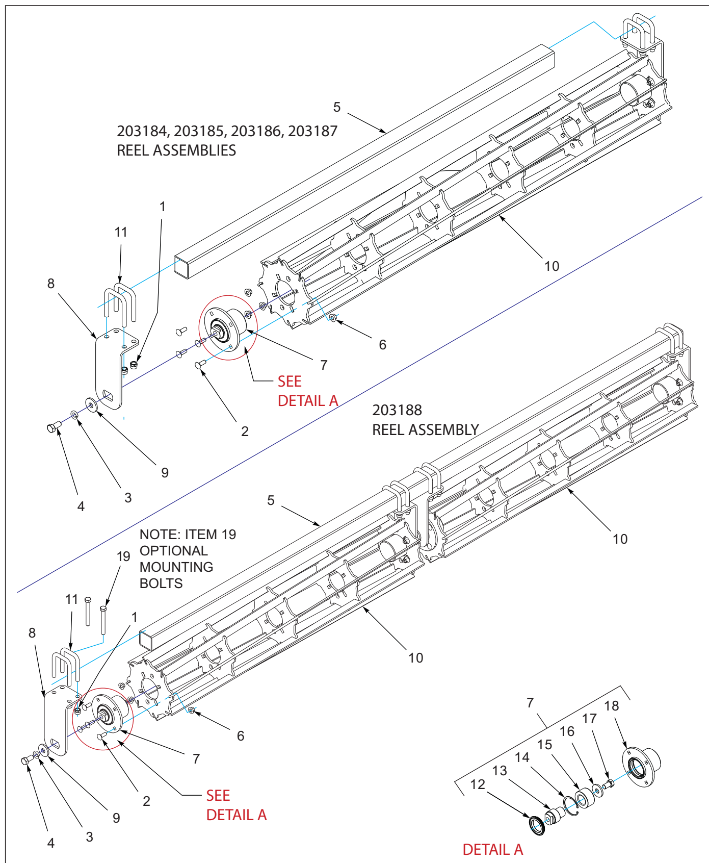
Figure 10-42: Flat Reel Assembly
