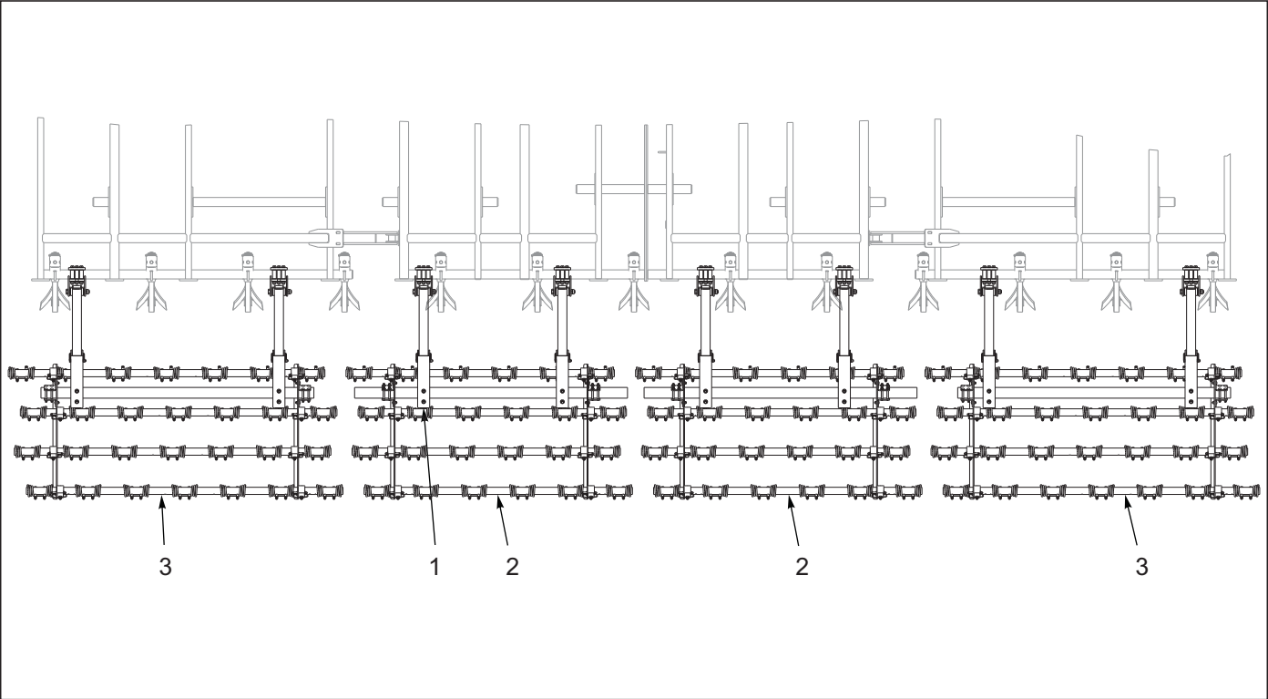
Figure 10-6: 4 Row Coil Tine Harrow Layout 8530-33'
