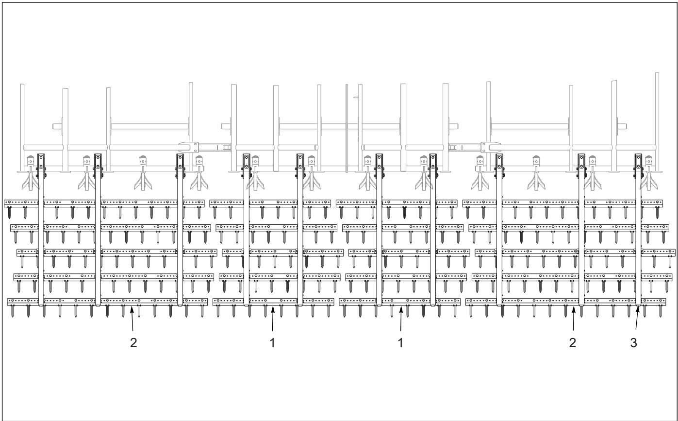
Figure 10-23: 5 Row Spike Harrow Layout 8530-30'
