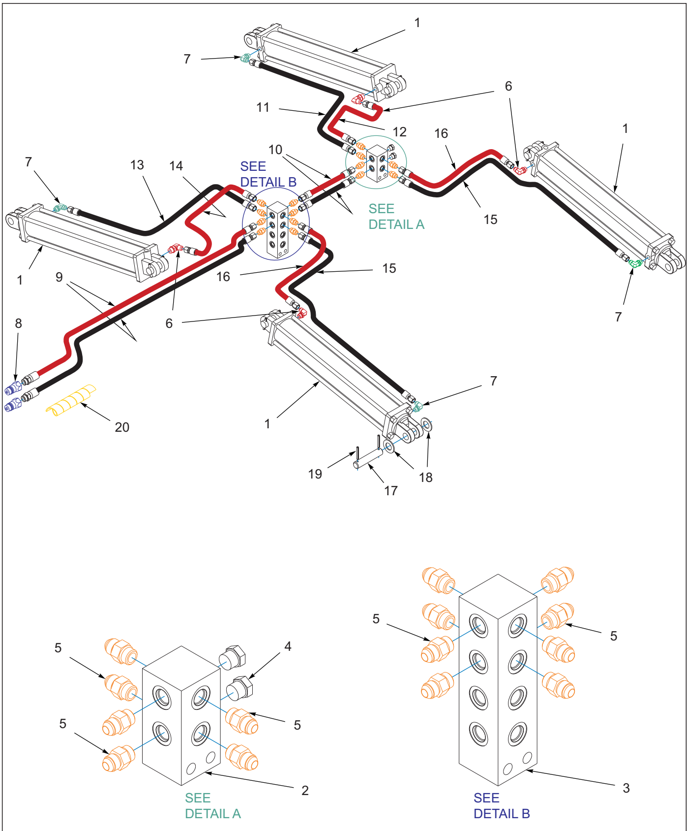
Figure 6-7: Fold Hydraulic Assembly 8530-33'-35'
