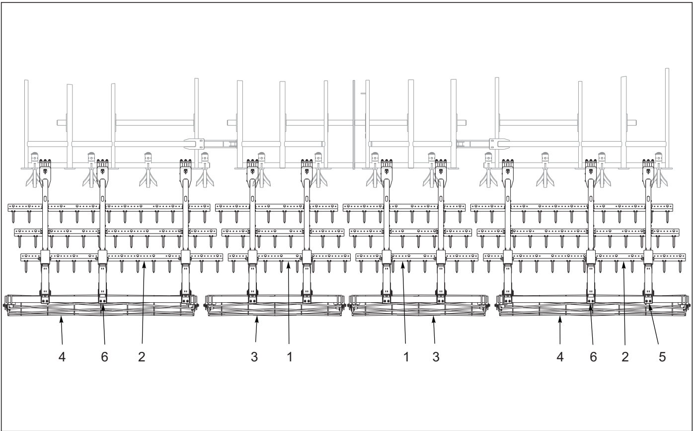
Figure 10-31: 3 Row Spike & Reel Layout 8530-30'
