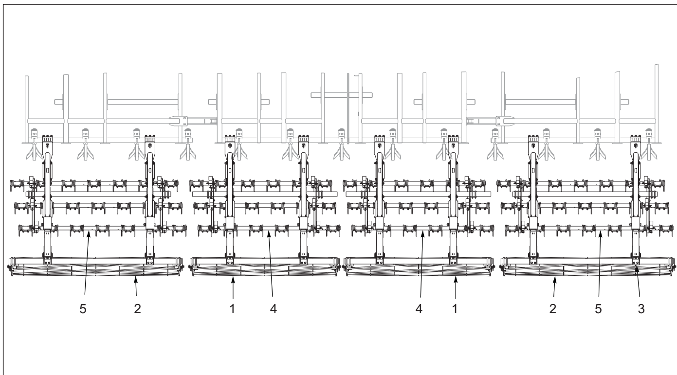
Figure 10-15: 3 Row Tine & Reel Layout 8530-33'
