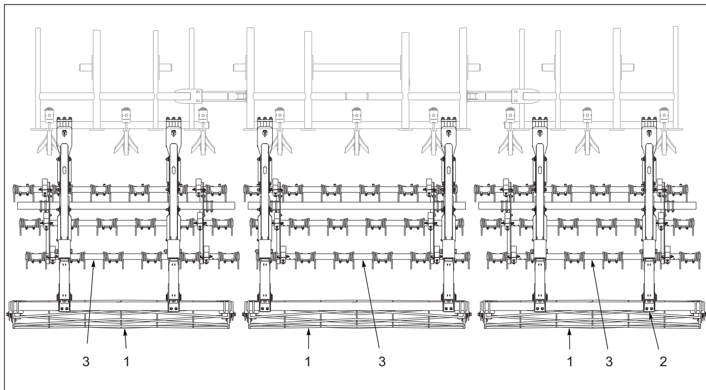
Figure 10-11: 3 Row Tine & Reel Layout 8530-22'
