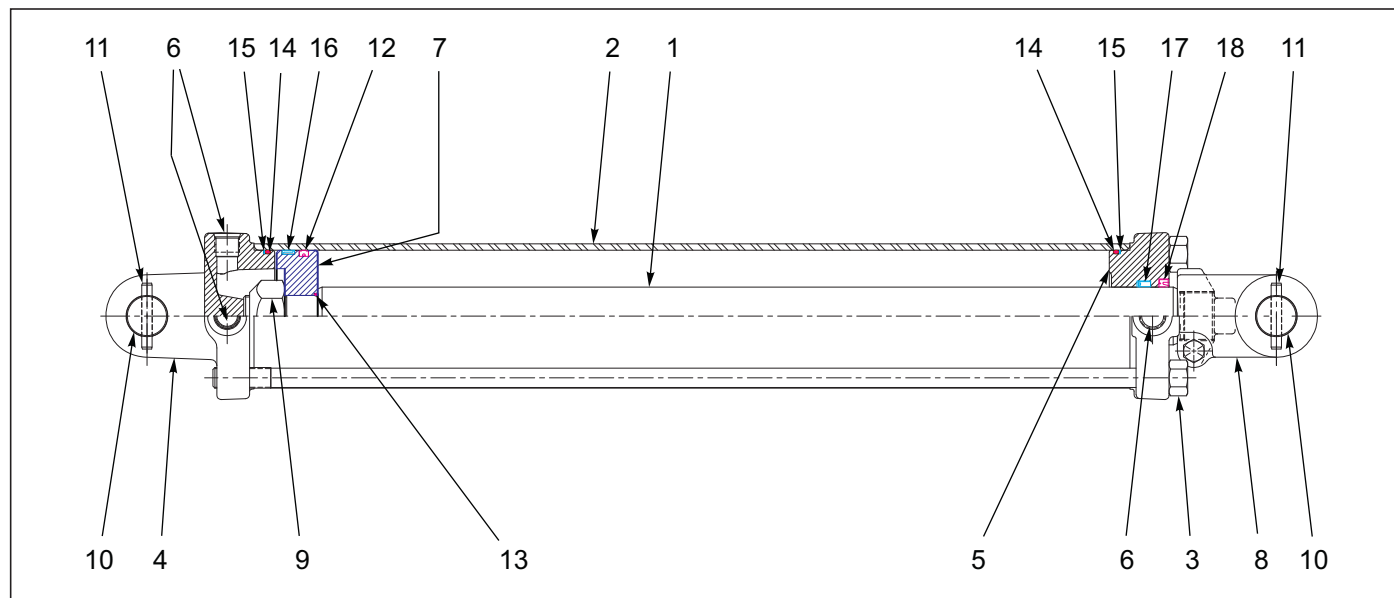
Figure 7-12: Cylinder Assembly 4-1/2 x 24
