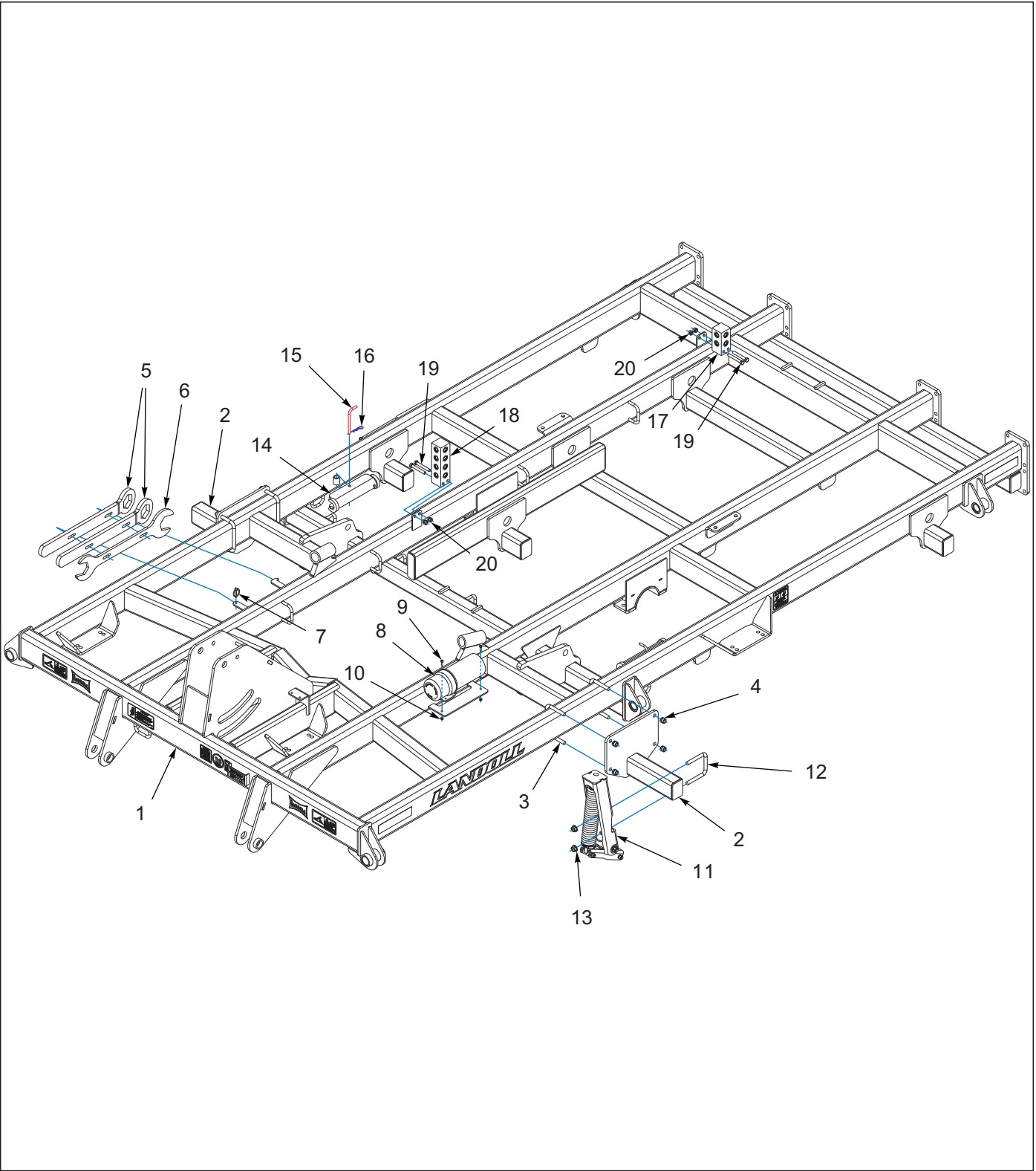
Figure 1-1: Center Frame Assembly 8530-19'-25'
