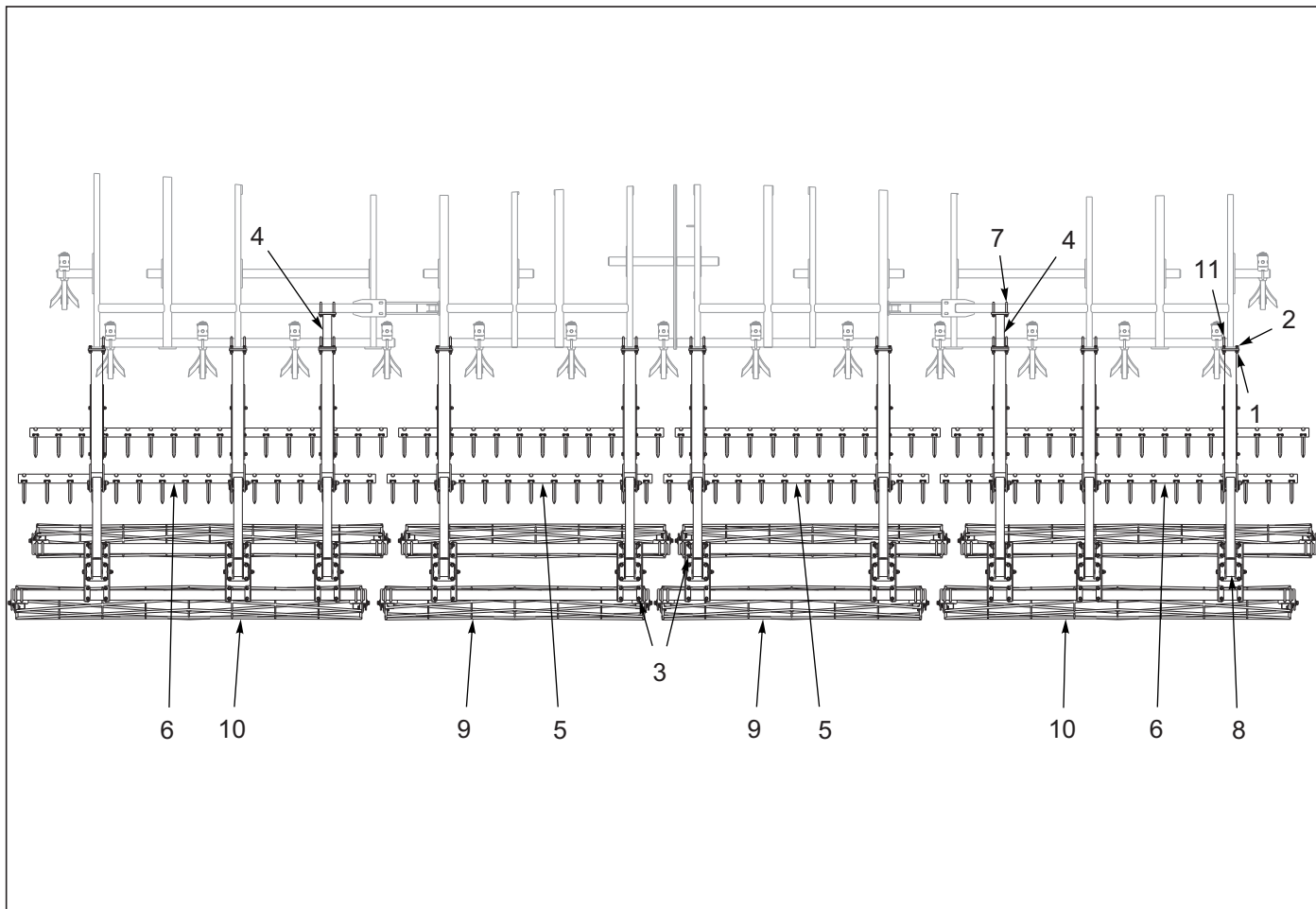
Figure 10-52: Spike & Double Reel Layout 8530-35'
