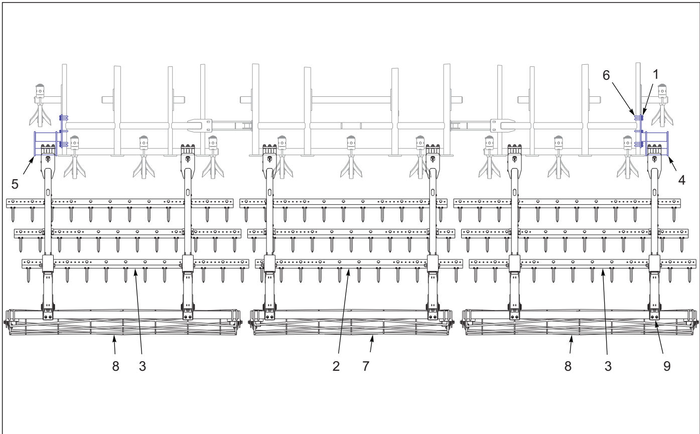
Figure 10-29: 3 Row Spike & Reel Layout 8530-25'
