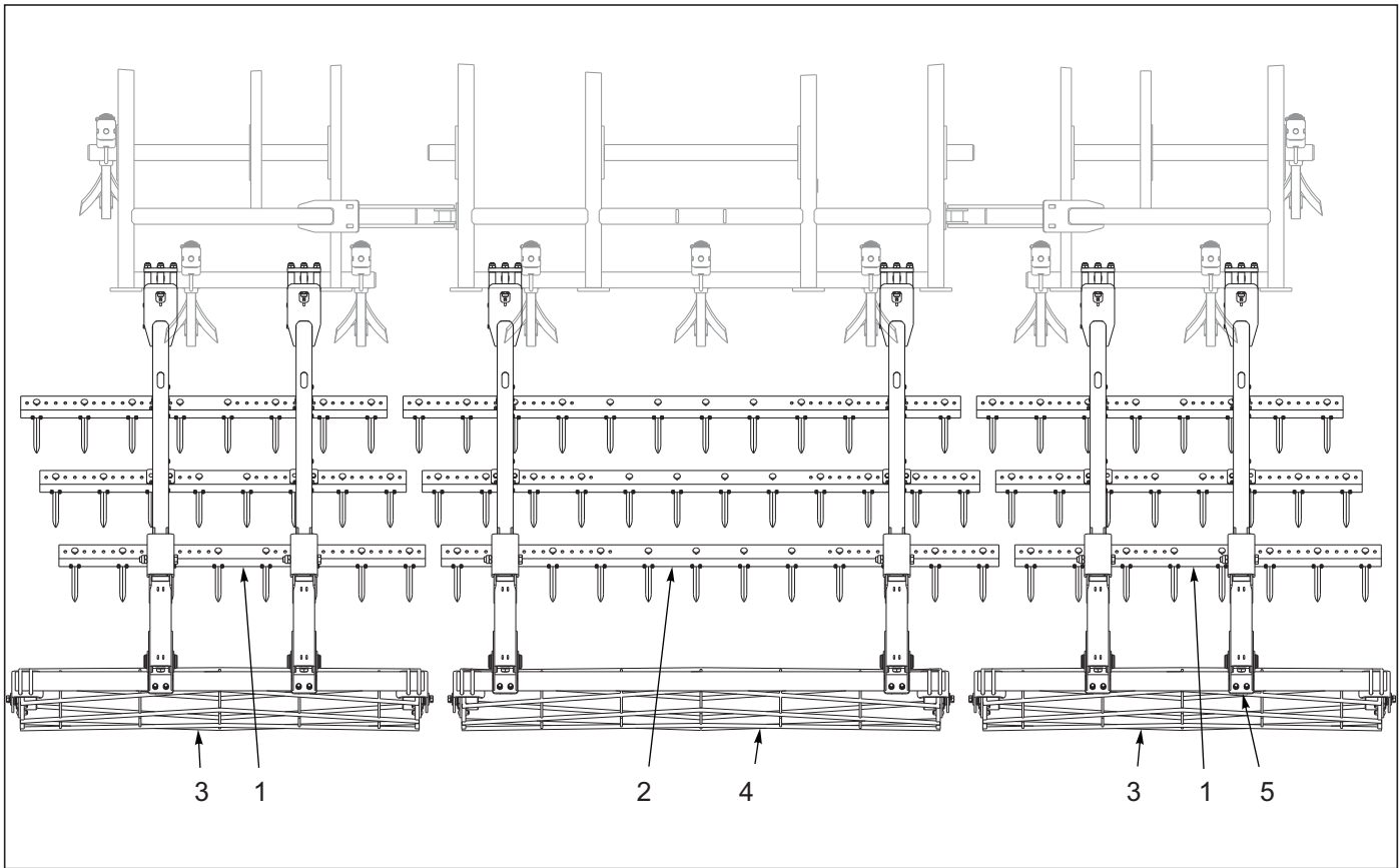
Figure 10-27: 3 Row Spike & Reel Layout 8530-19'
