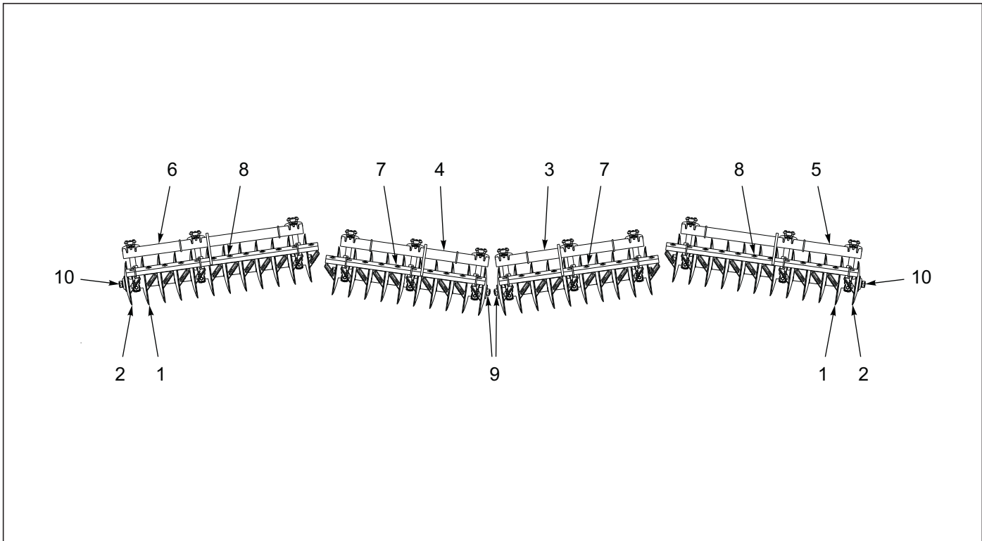
Figure 4-9: Gang Assembly 22" 4 GA 8530-27'
