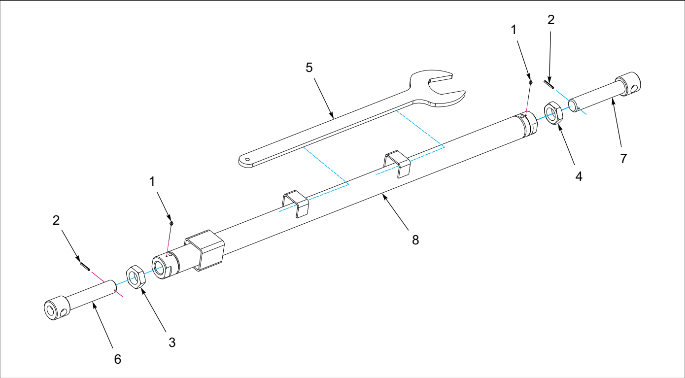
Figure 2-7: Radius Rod Assembly
