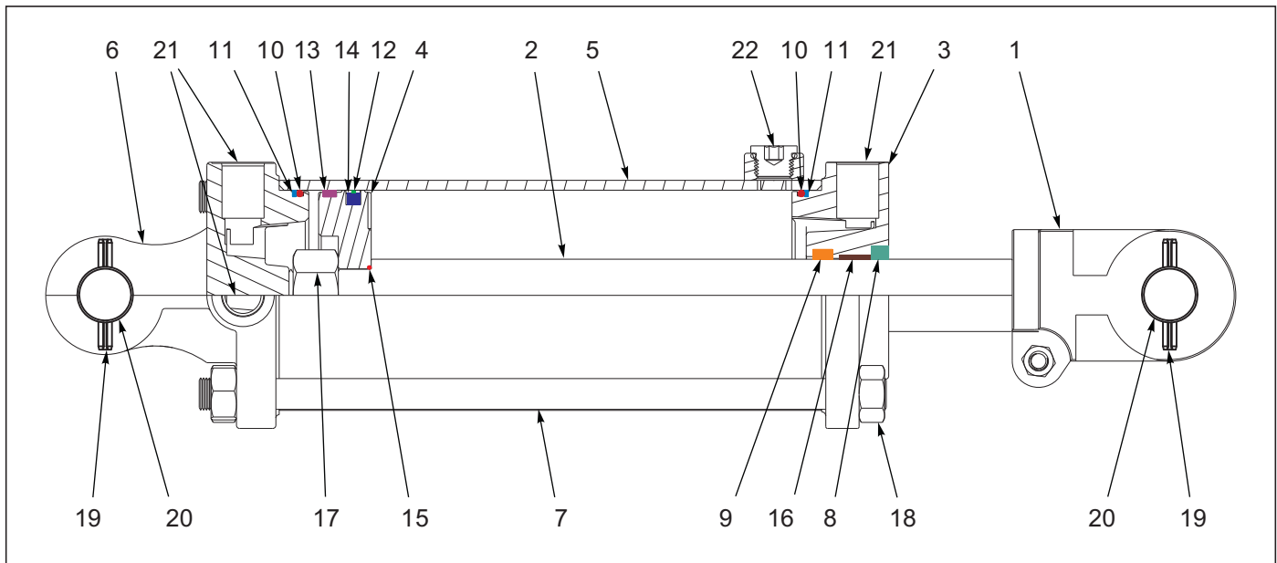
Figure 7-6: Cylinder Assembly 3-1/2 x 8, Rephase (Midway)
