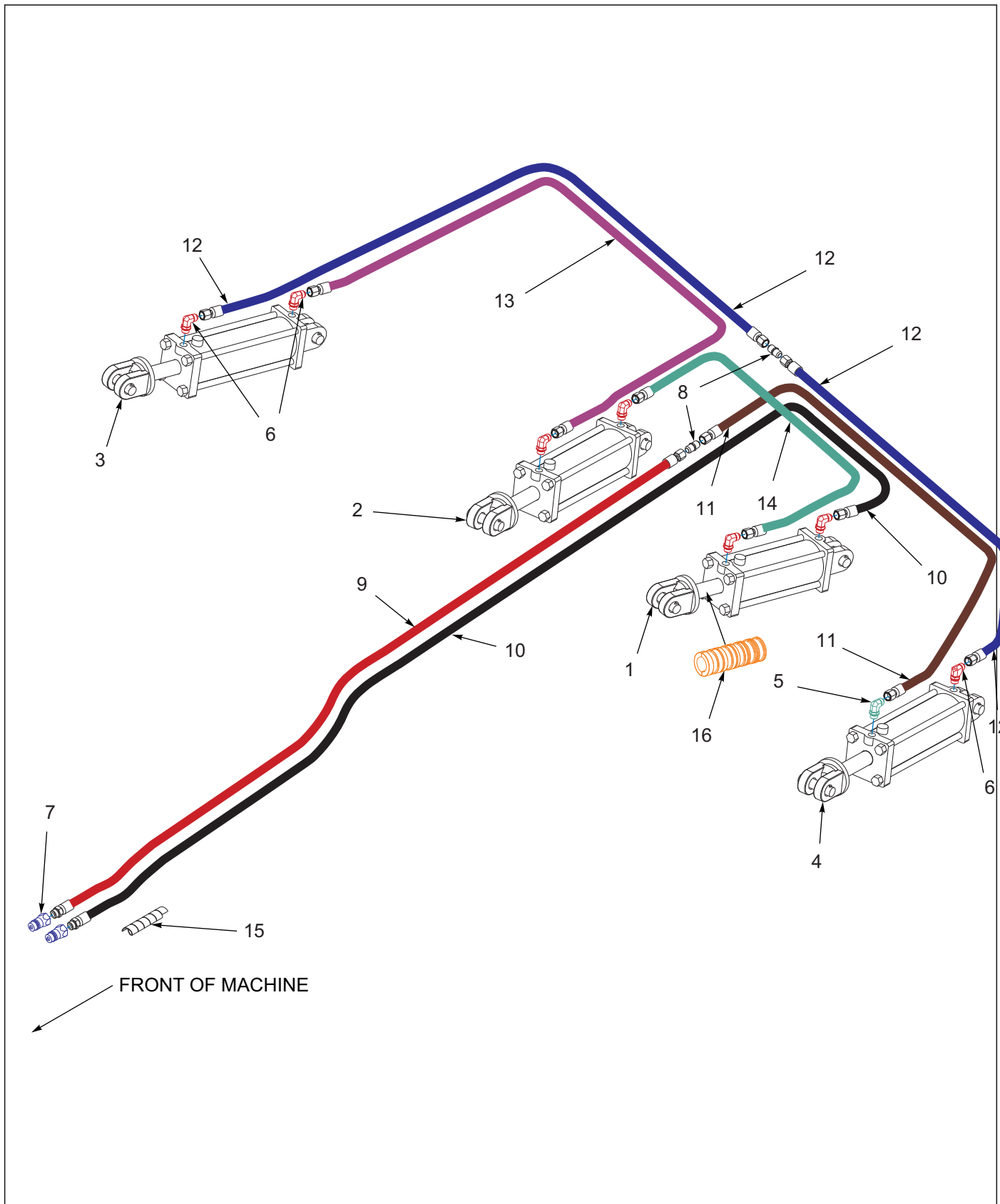
Figure 6-9: Gang Hydraulic Assembly 8530-27'-30'
