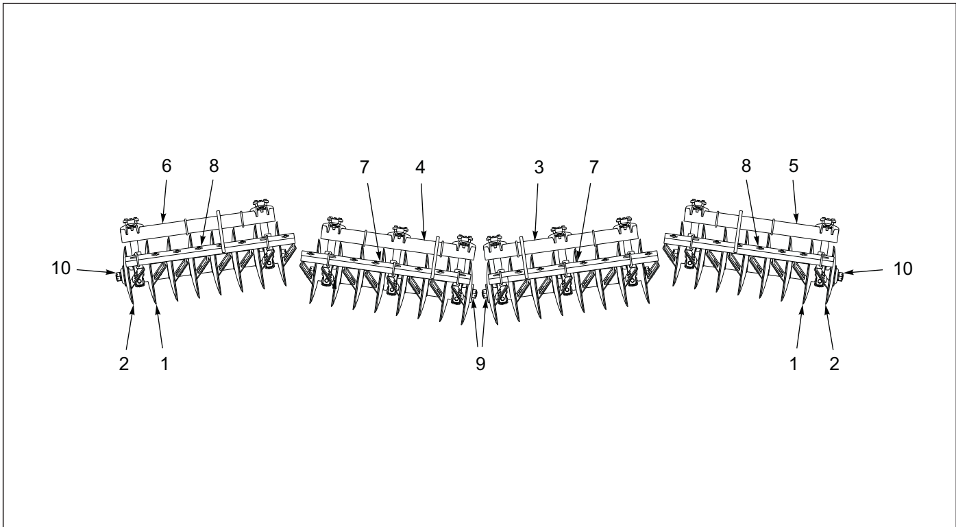
Figure 4-7: Gang Assembly 22" 4 GA 8530-22'
