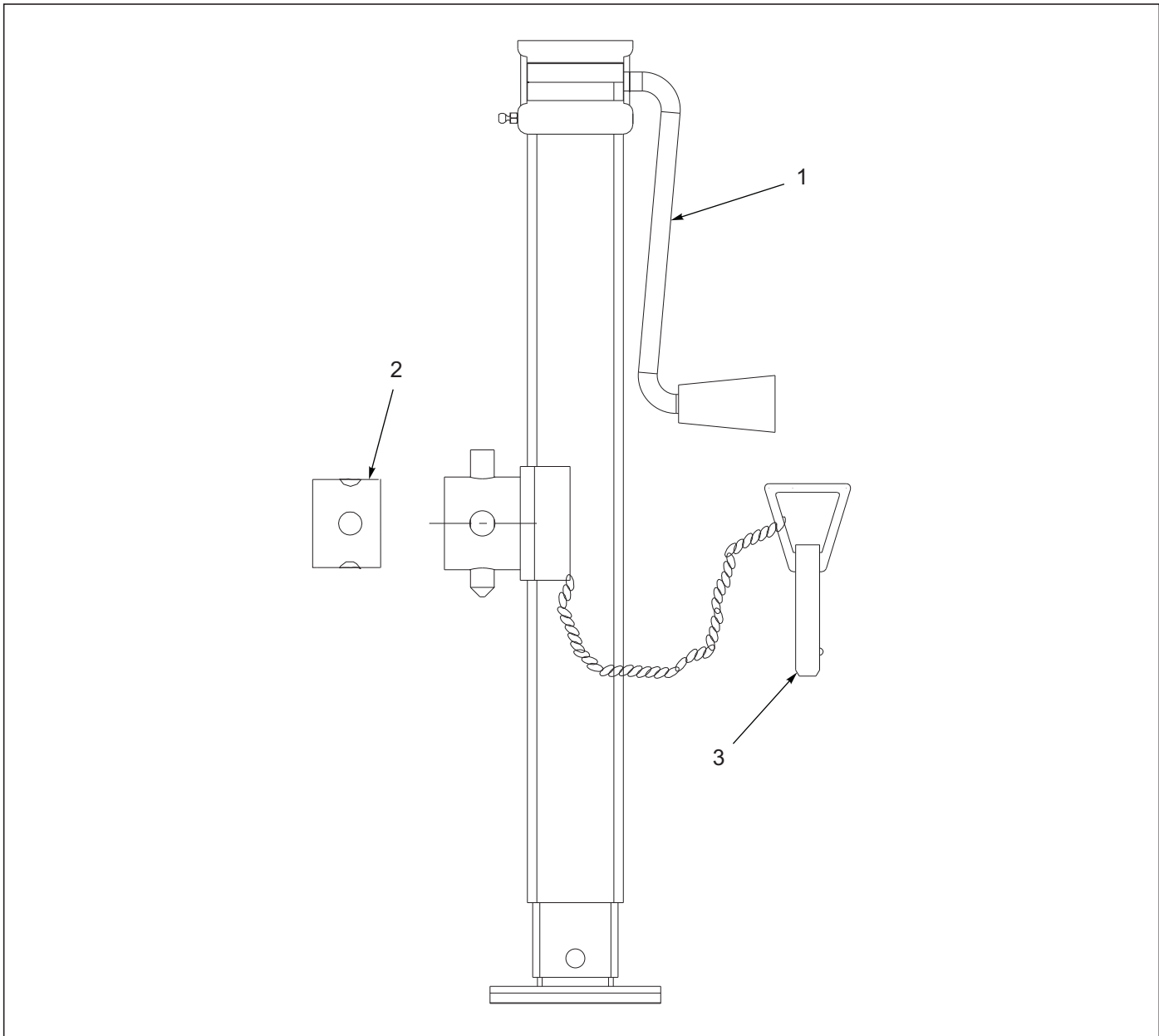
Figure 2-3: Jack Assembly 140647
