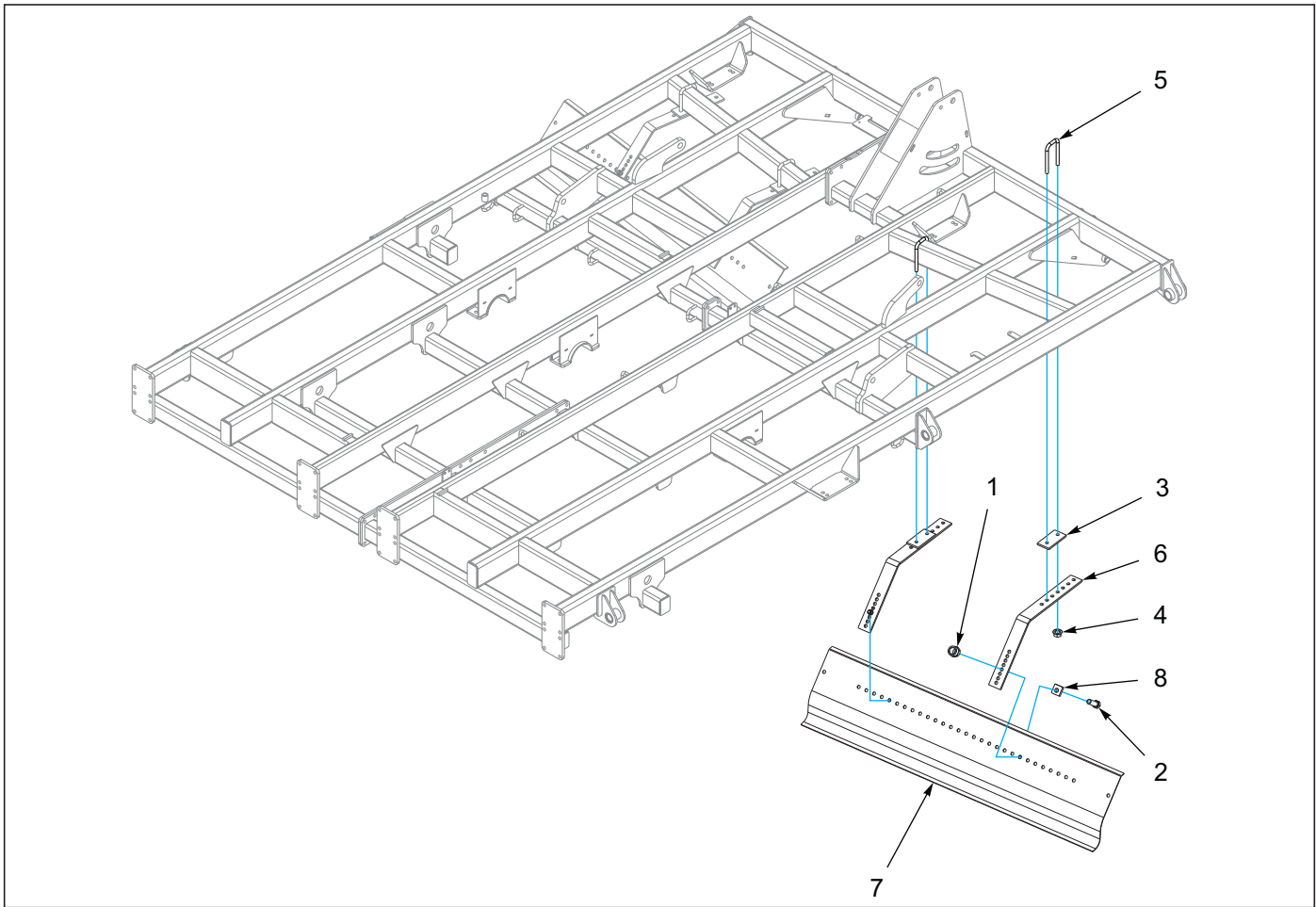
Figure 4-3: Disc Gang Shield - Center Frame 19'-30'
