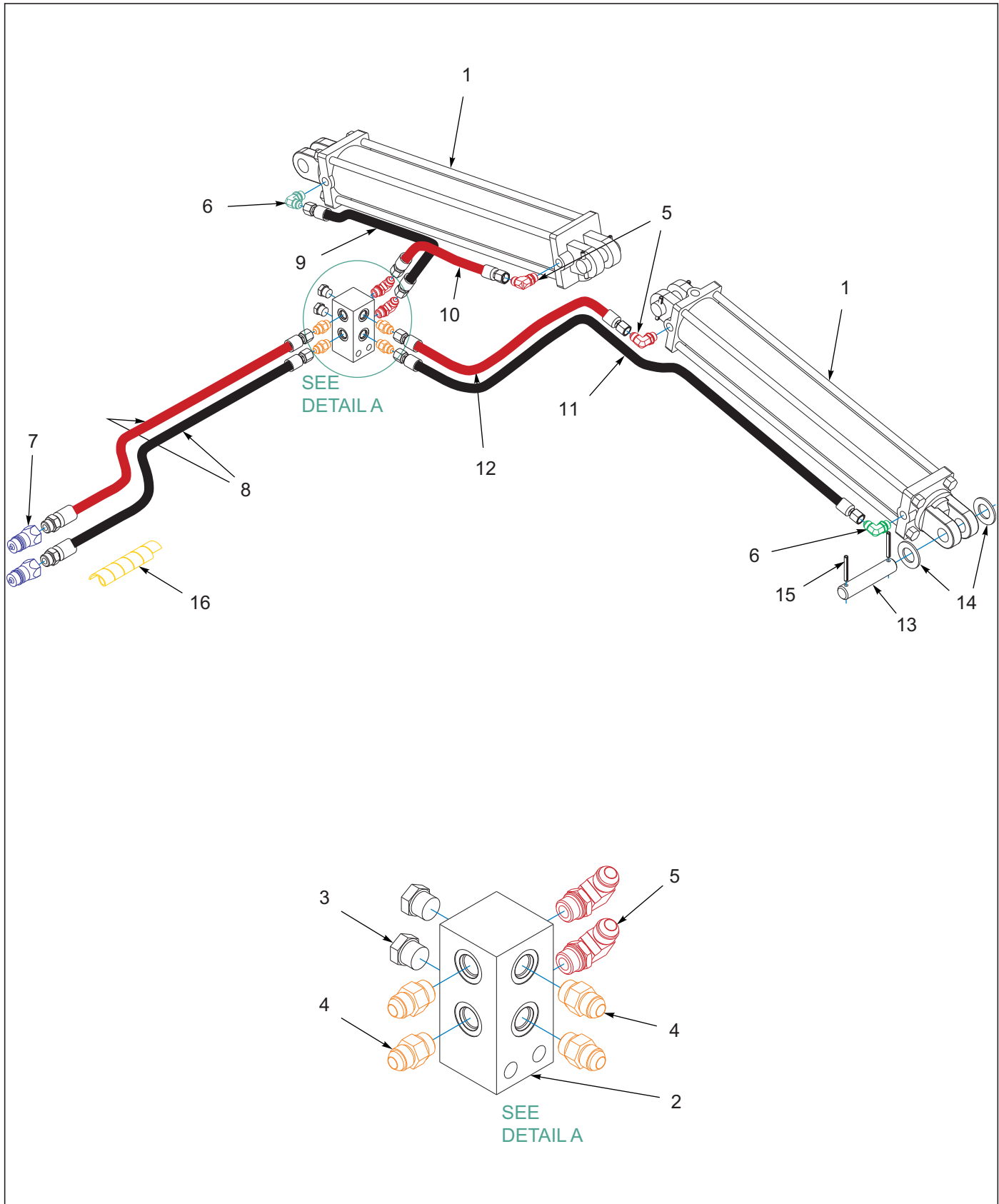
Figure 6-4: Fold Hydraulic Assembly 8530-19'
