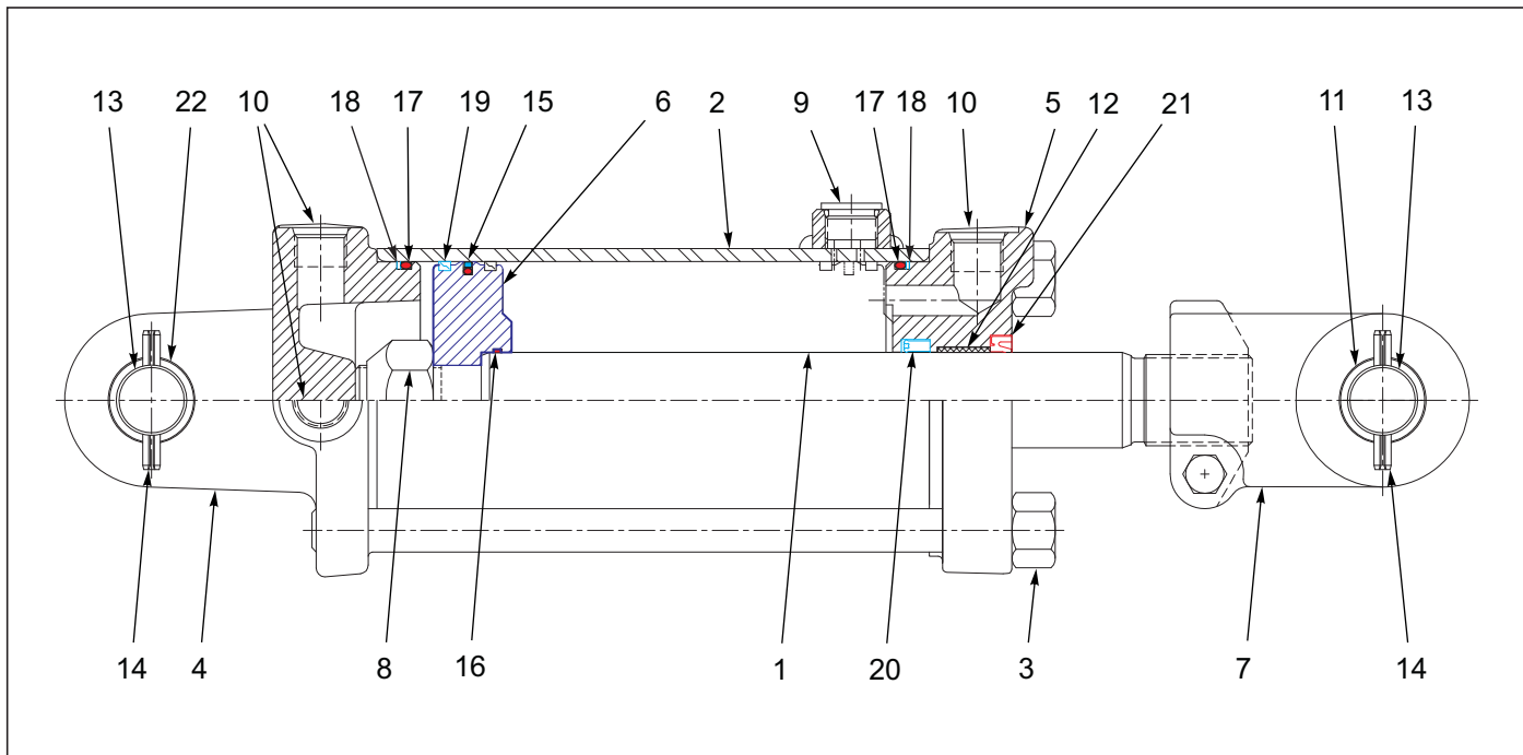
Figure 7-5: Cylinder Assembly 3-1/2 x 8, Rephase (Prince)
