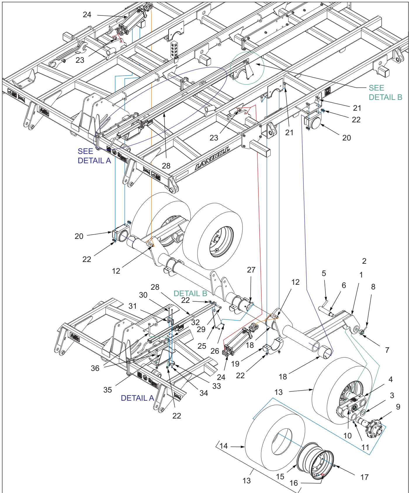
Figure 1-5: Center Lift Assembly 8530-27'-30'
