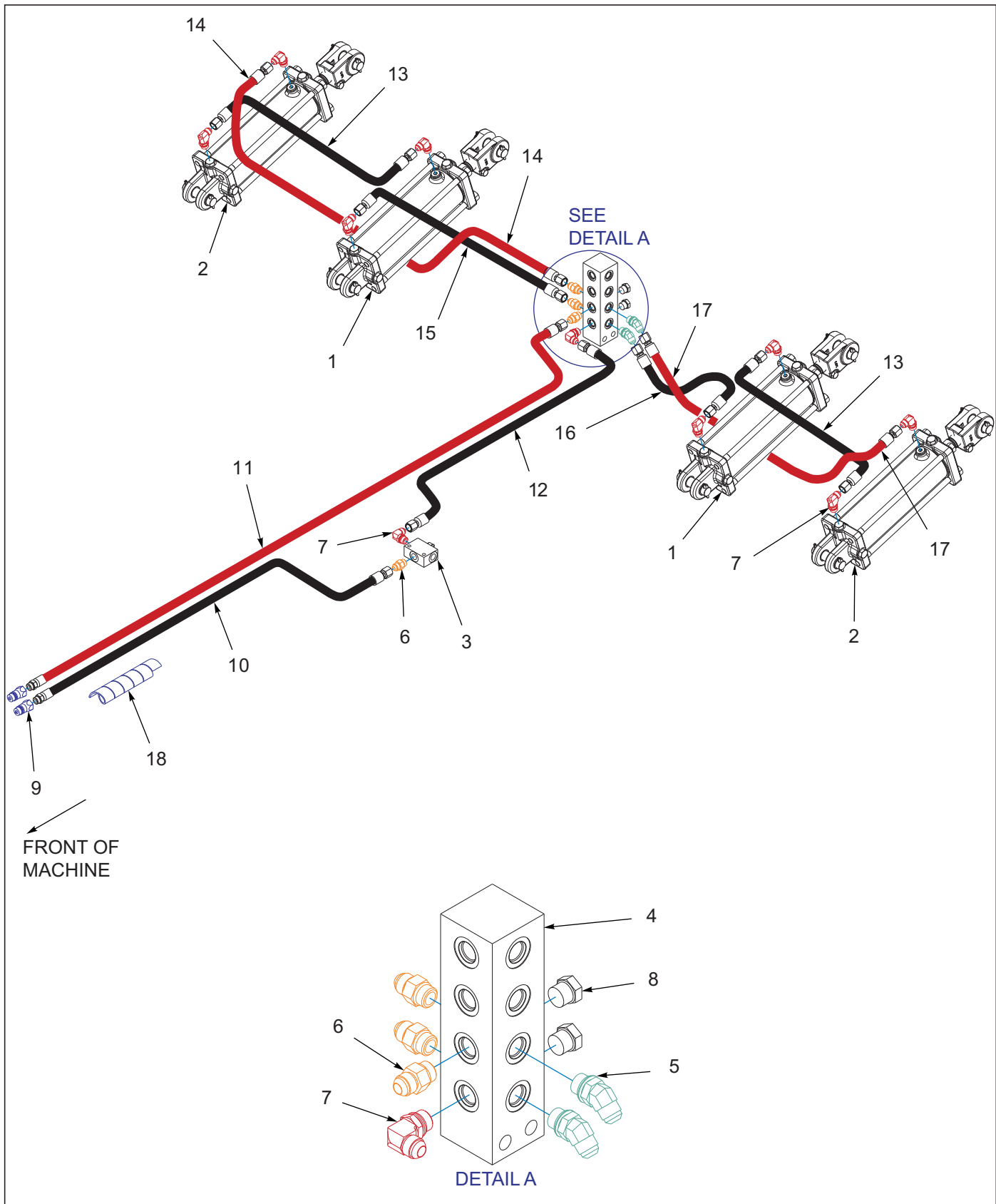
Figure 6-2: Lift Hydraulic Assembly 8530-27'-30'
