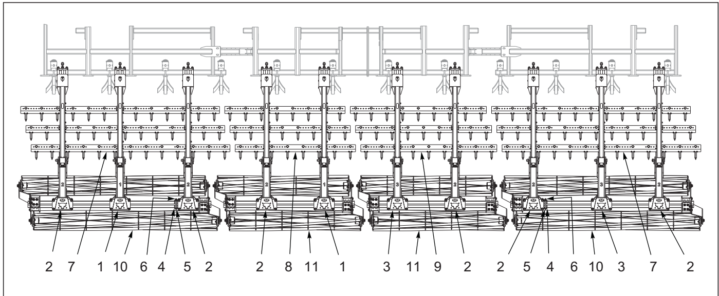
Figure 10-56: 3RS & Double Flat Reel Layout 8530-30'
