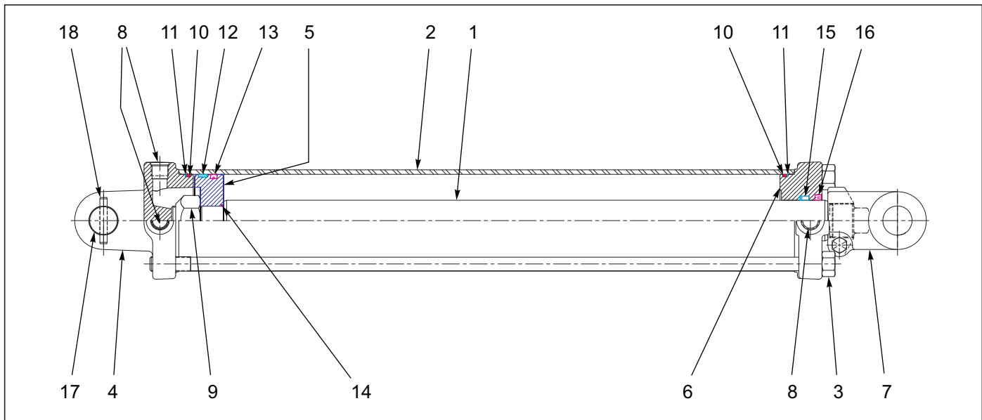
Figure 7-11: Cylinder Assembly 4 x 24
