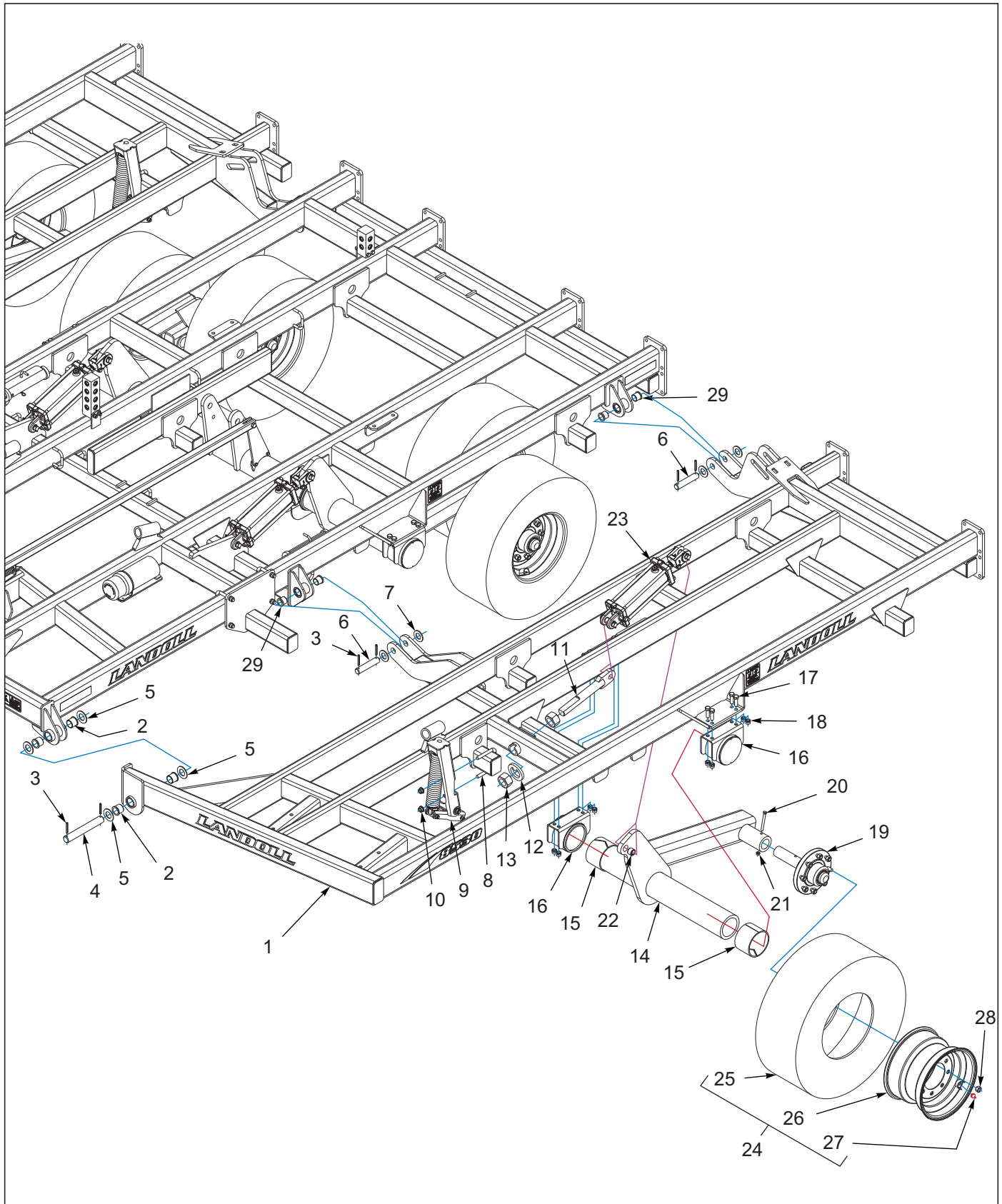
Figure 1-7: Wing Frame and Lift Assembly 8530-19'
