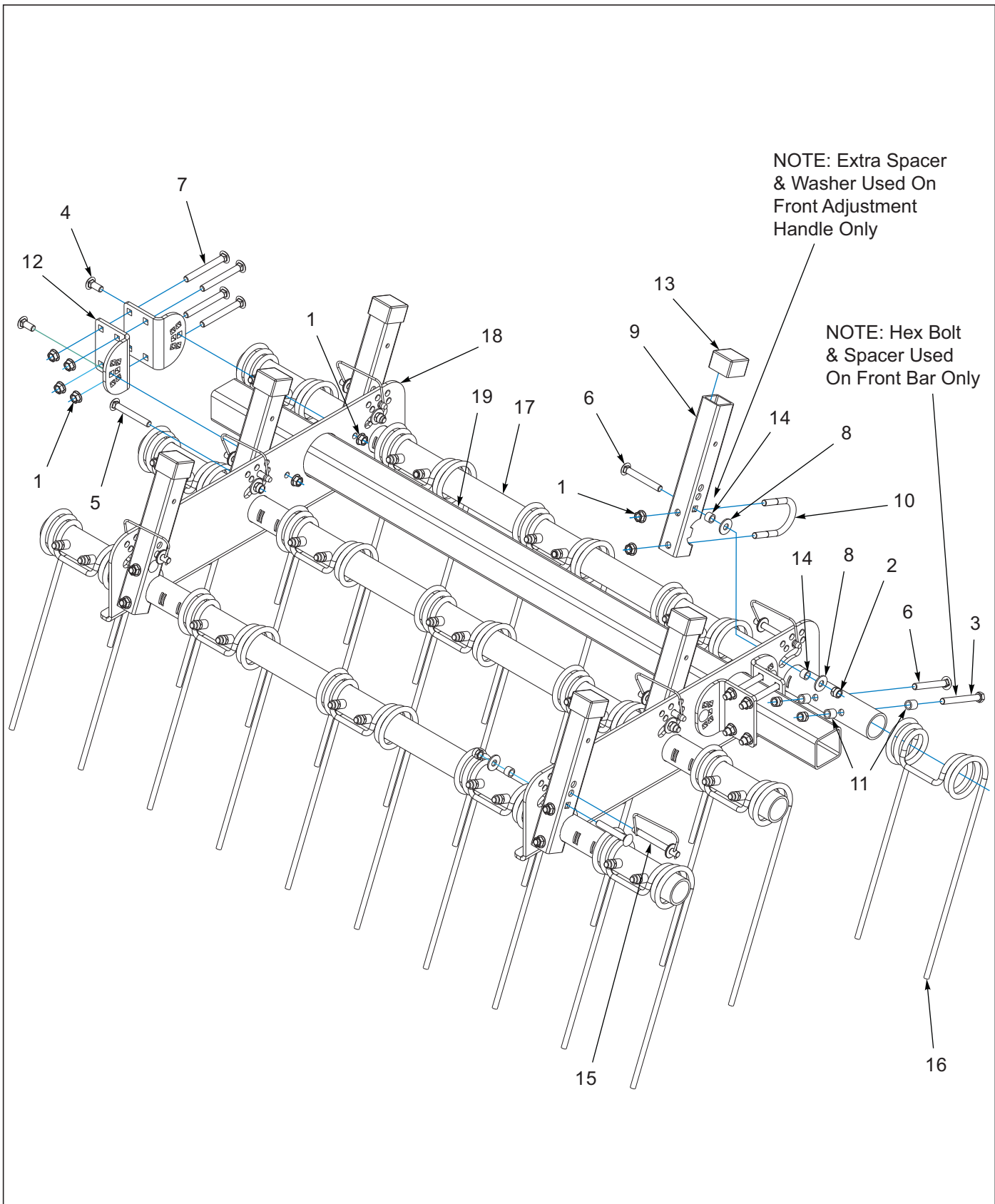
Figure 10-18: 3 Row Coil Tine Harrow Assembly
