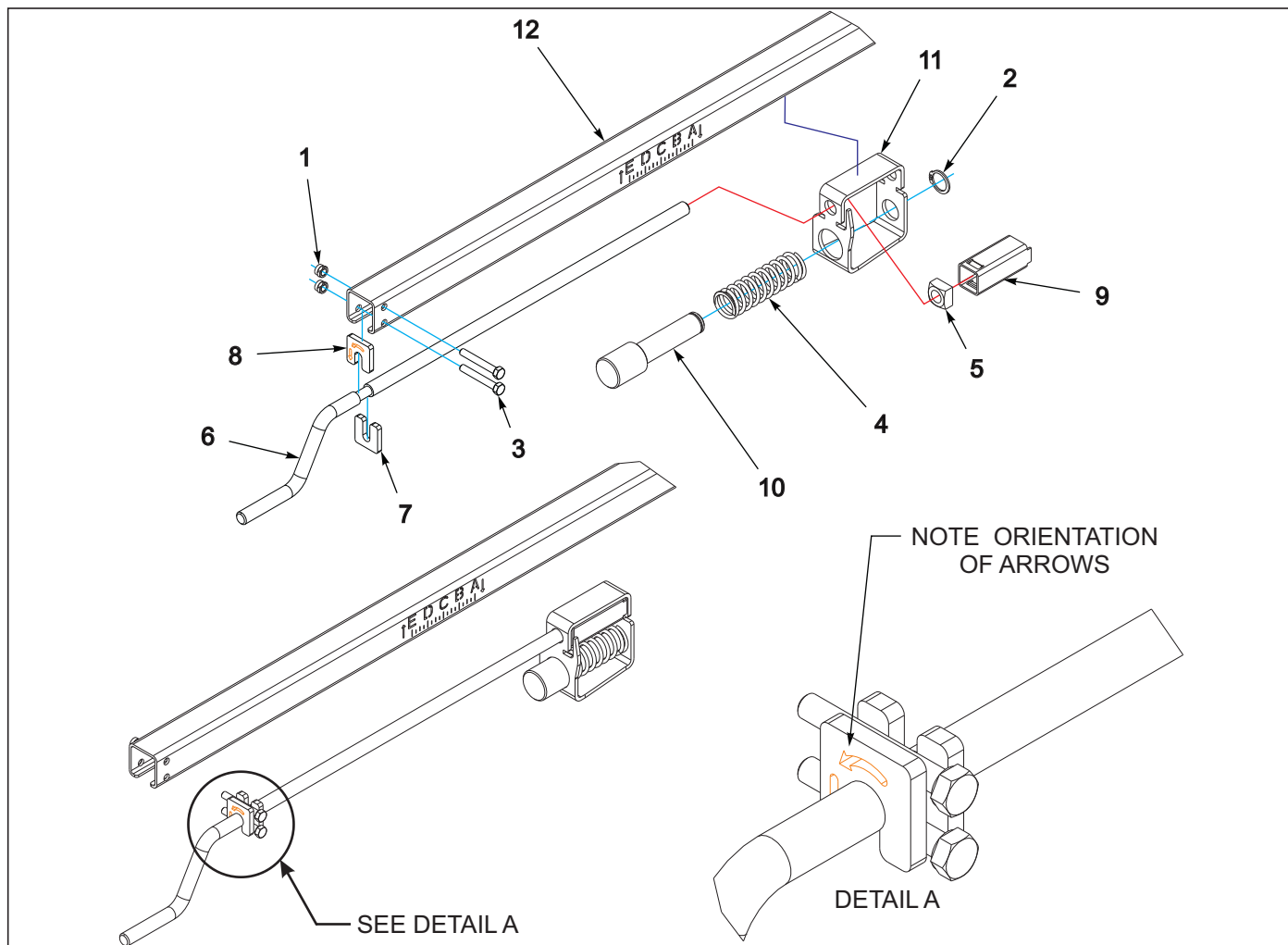
Figure 1-10: Depth Stop Tube Assembly
