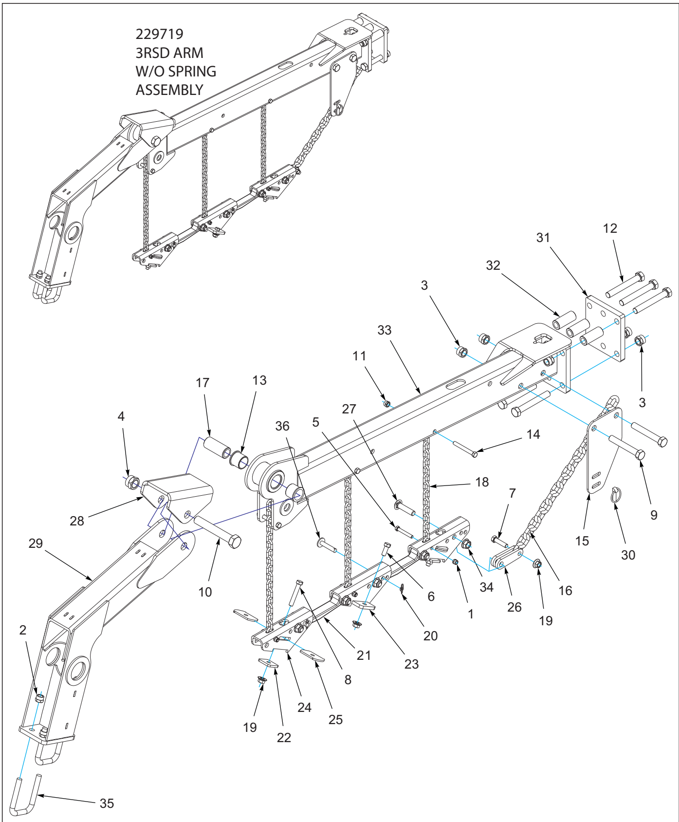
Figure 10-45: 3 RSD Arm Assembly W/O Spring
