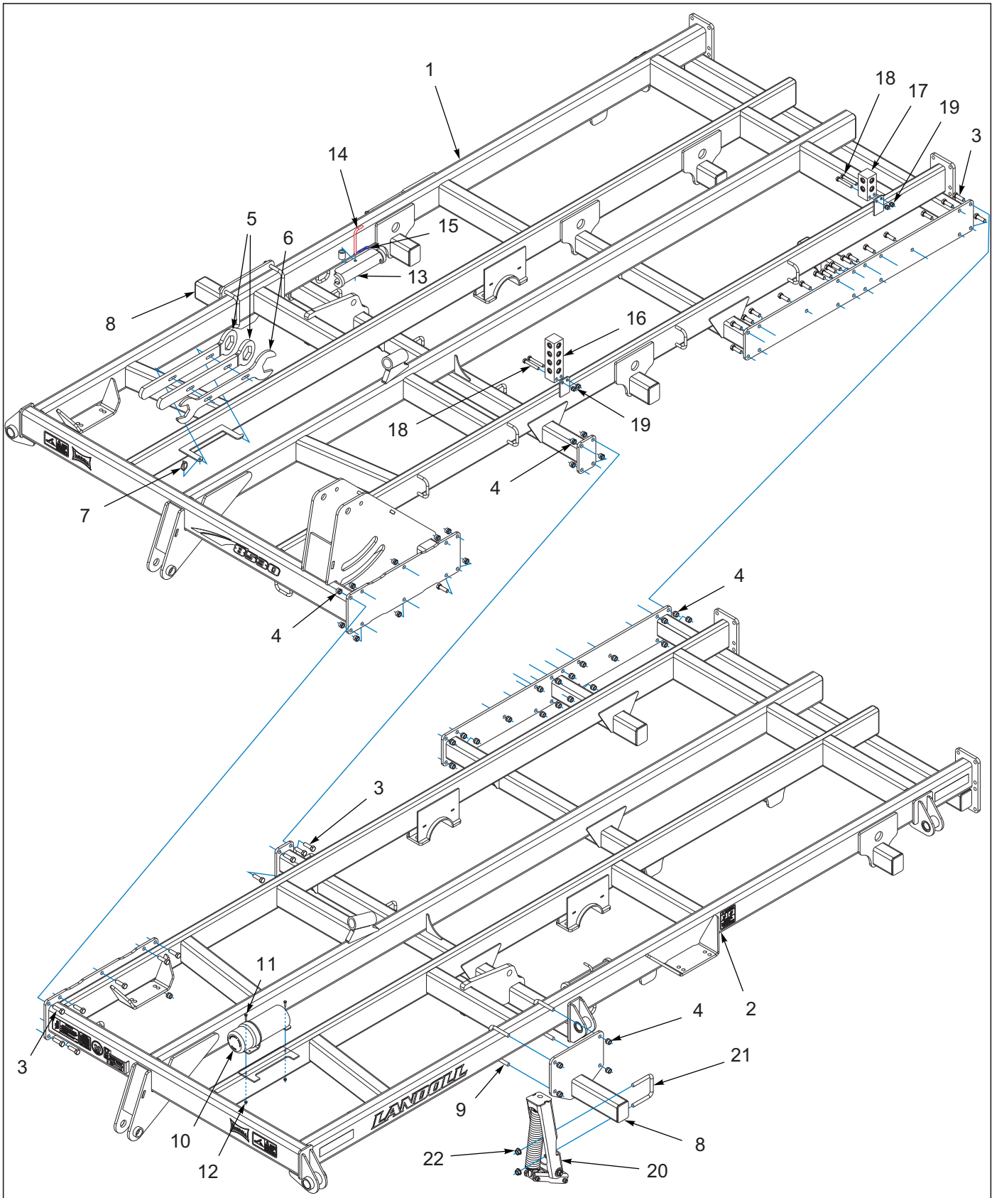
Figure 1-3: Center Frame Assembly 8530-33'-35'
