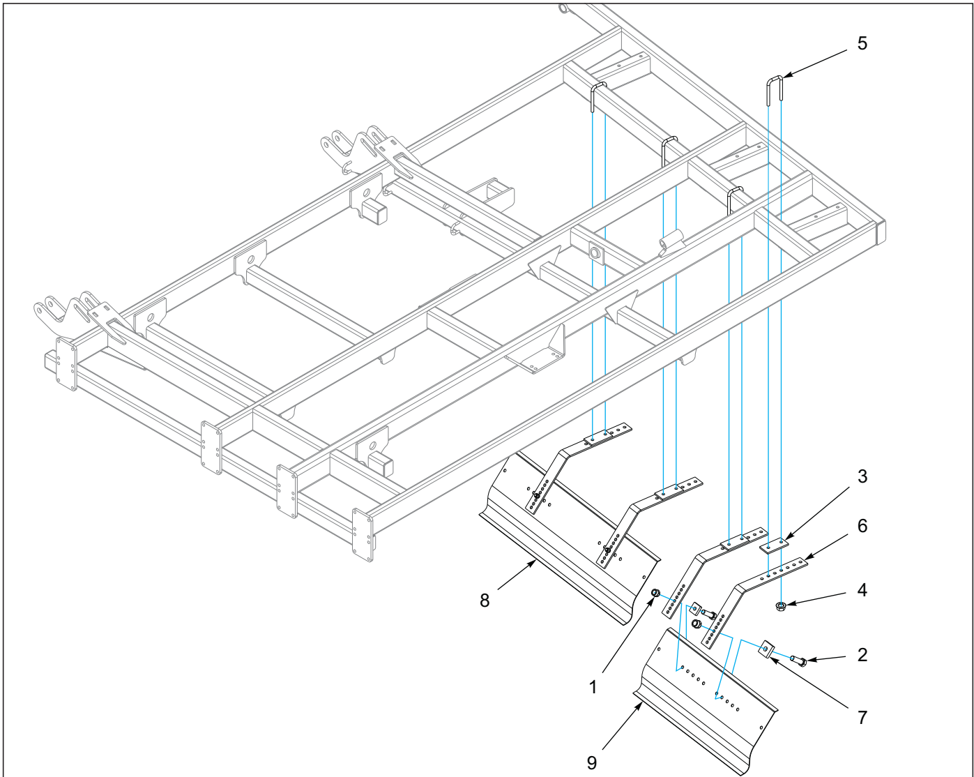
Figure 4-5: Disc Gang Shield - Wing
