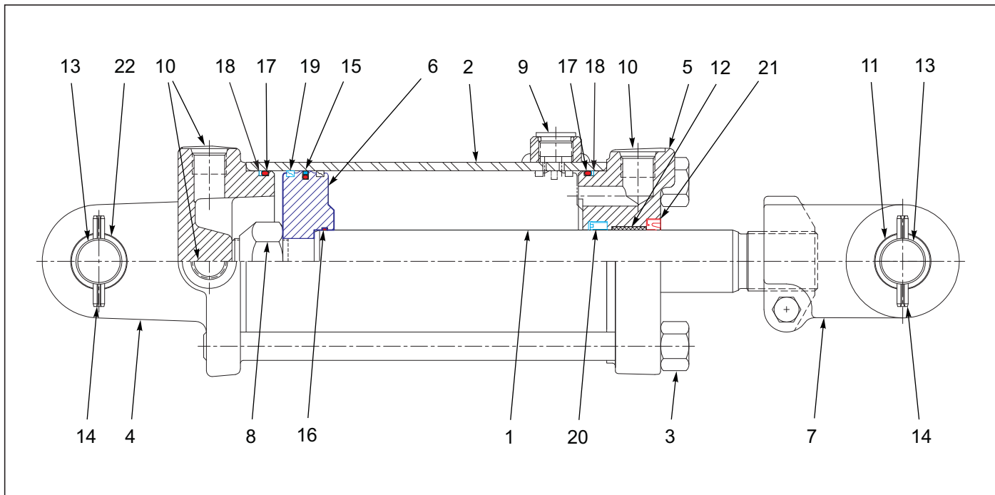
Figure 7-7: Cylinder Assembly 3-1/4 x 8, Rephase (Prince)
