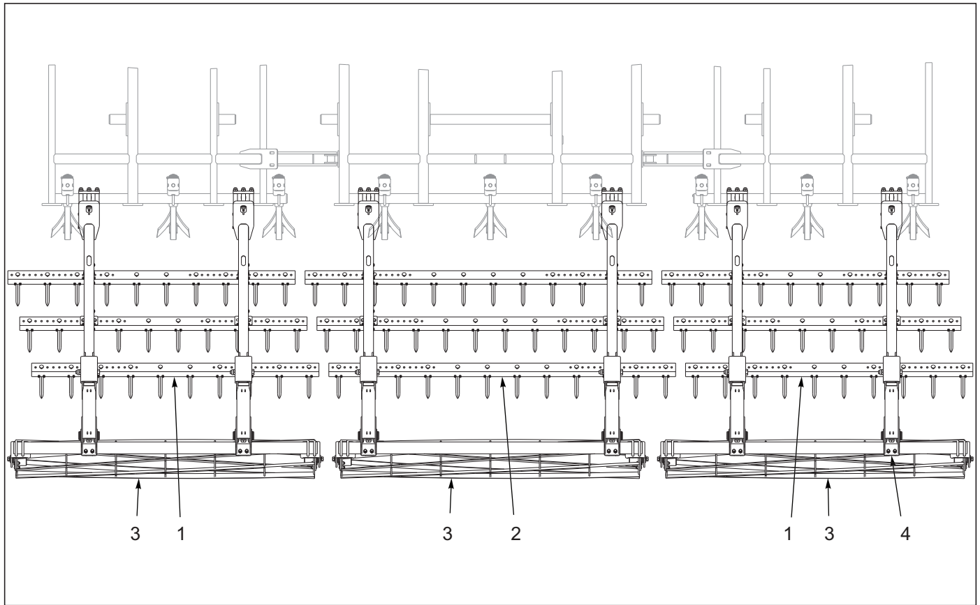
Figure 10-36: 3 Row Spike & Reel Layout 8530-22'
