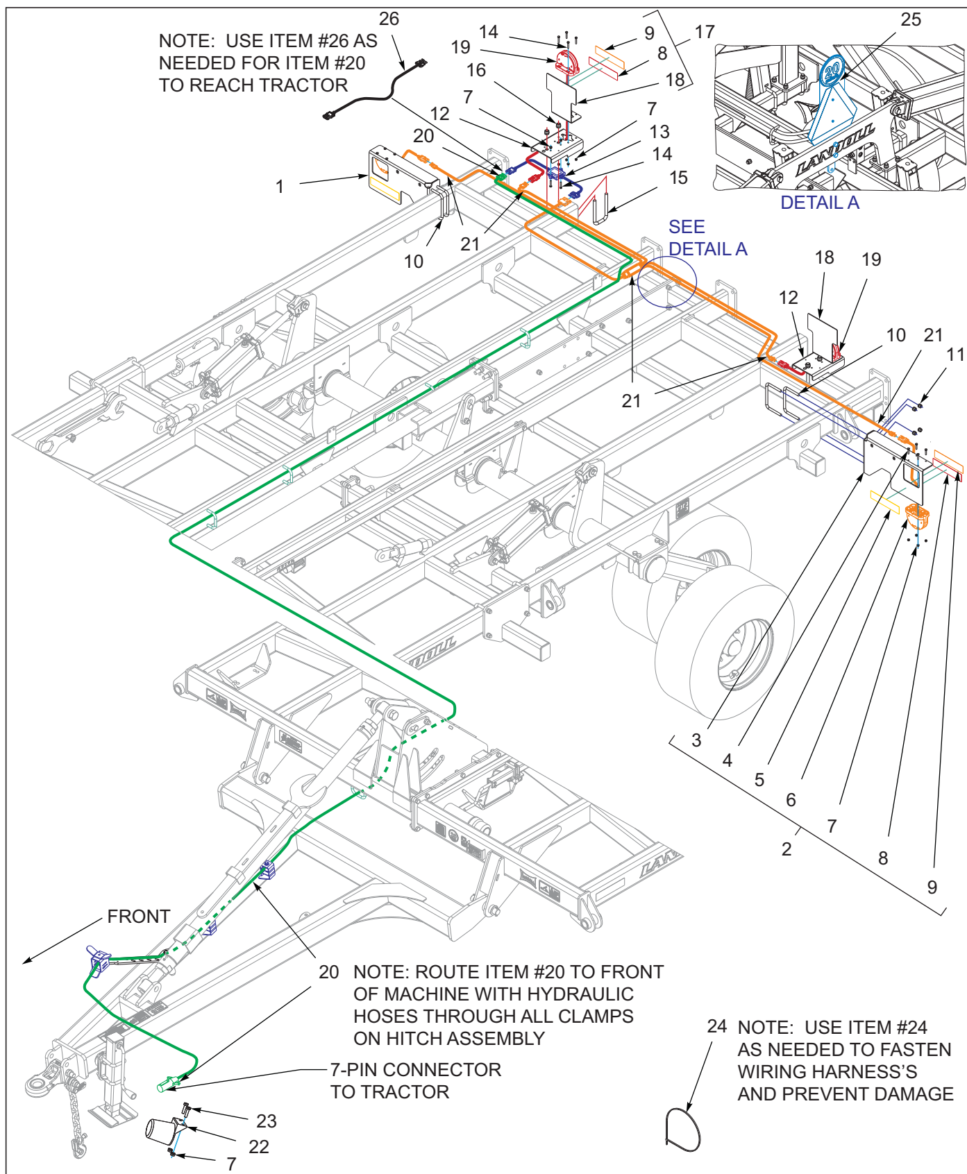
Figure 8-2: Electrical Assembly W/LED Lights (2 of 2)
