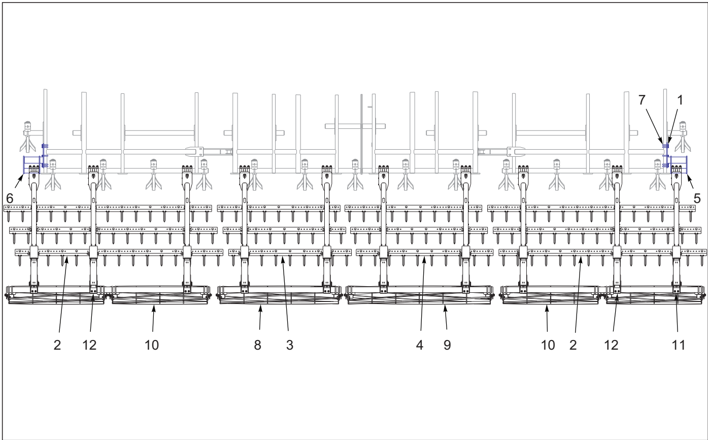
Figure 10-41: 3 Row Spike & Reel Layout 8530-35'
