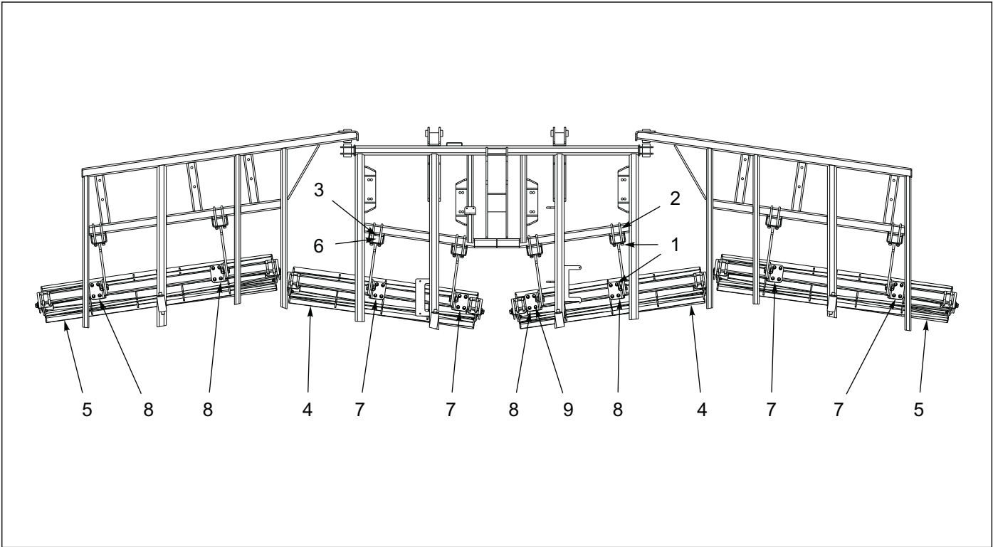
Figure 4-15: Disc Gang Reel Assembly 8530-25'
