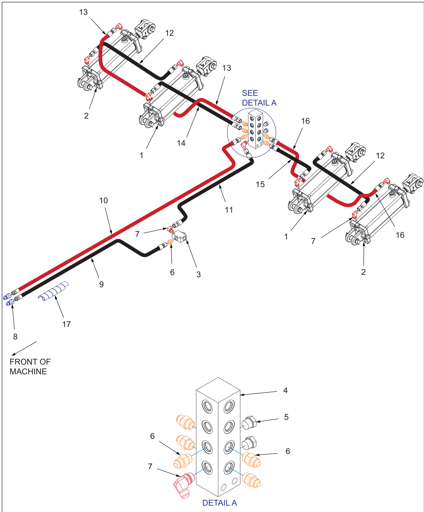
Figure 6-3: Lift Hydraulic Assembly 8530-33'-35'
