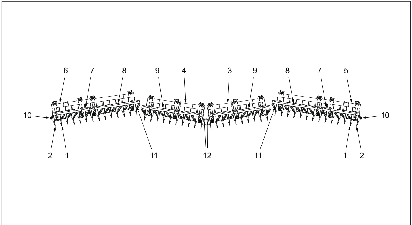
Figure 4-10: Gang Assembly 22" 4 GA 8530-30'
