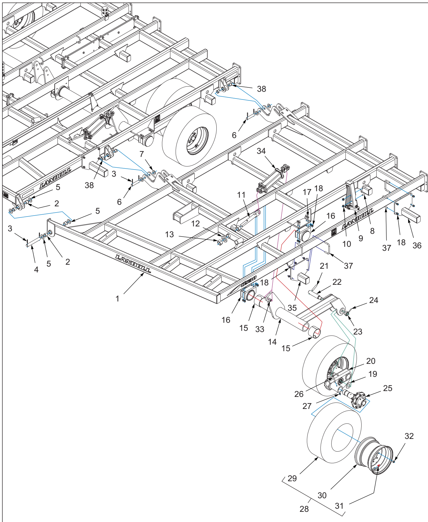
Figure 1-9: Wing Frame and Lift Assembly 8530-30'-35'
