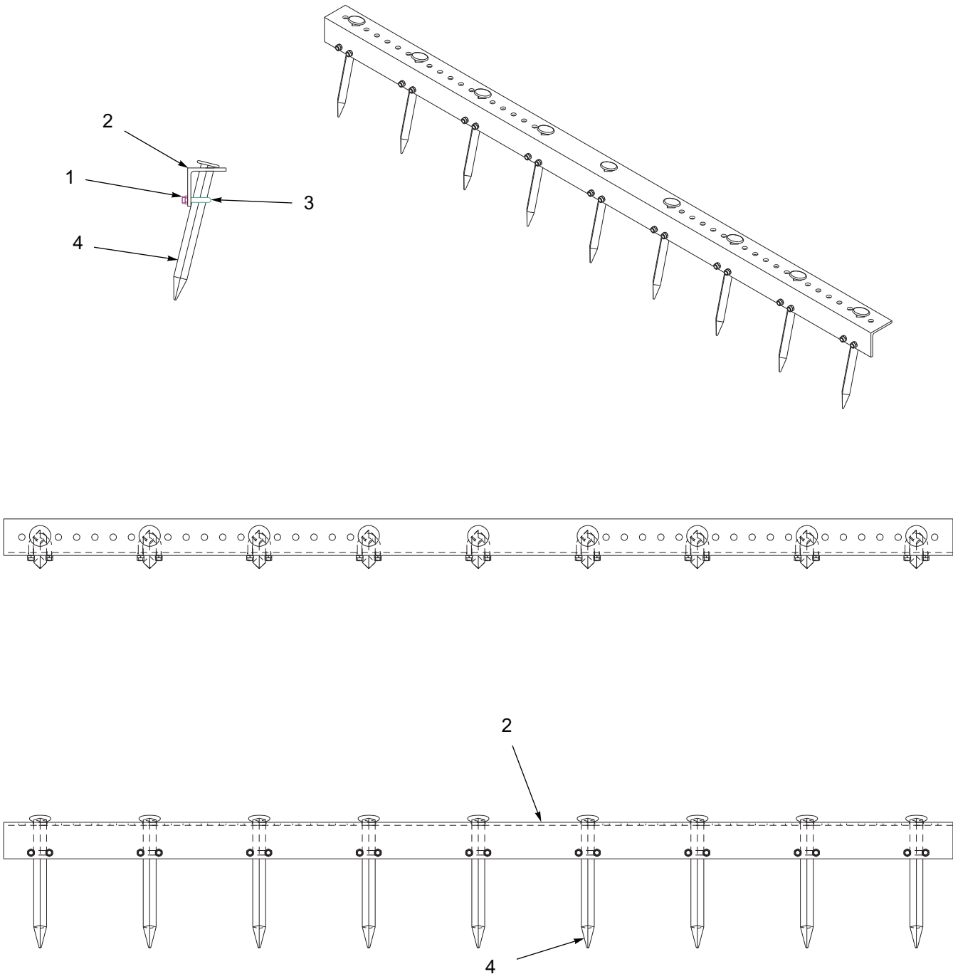
Figure 10-62: Spike Bar Assembly, 11L 9 SP
