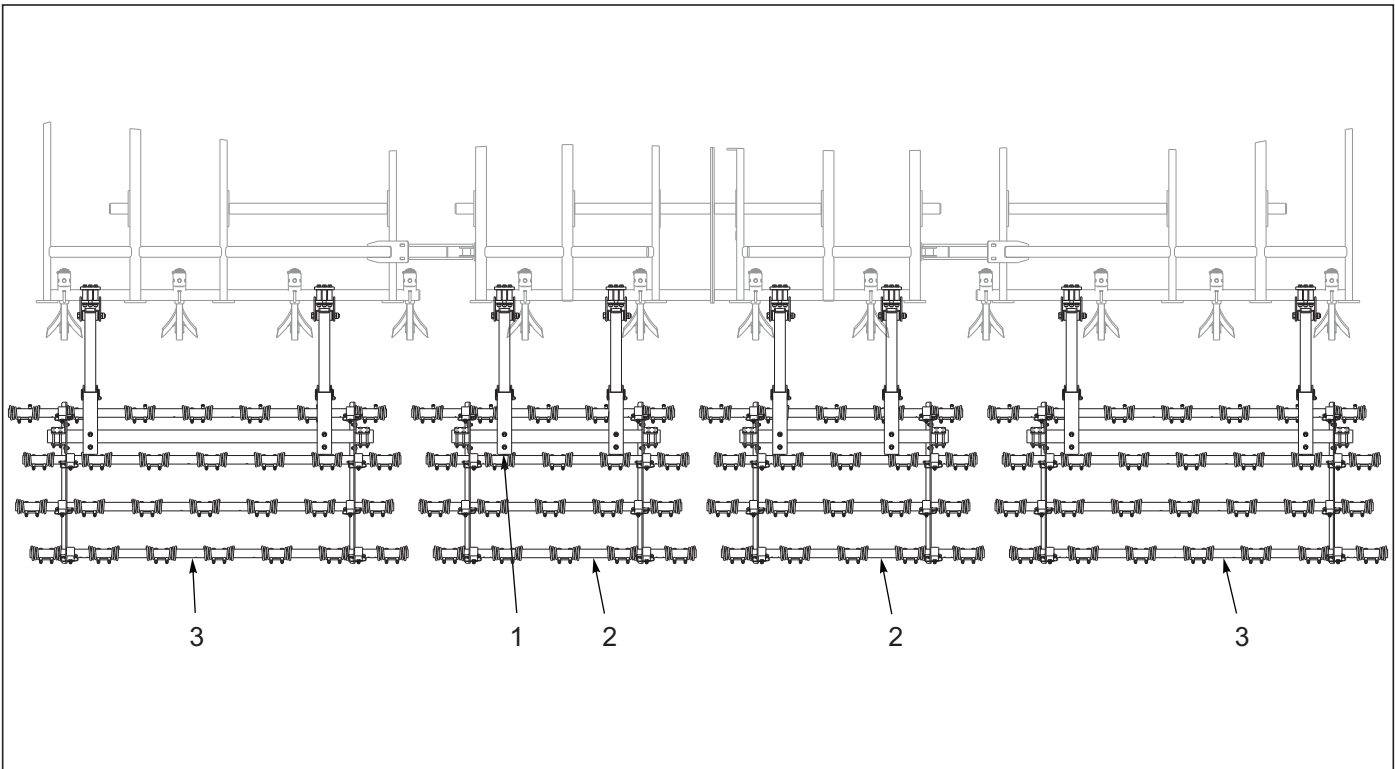
Figure 10-5: 4 Row Coil Tine Harrow Layout 8530-30'
