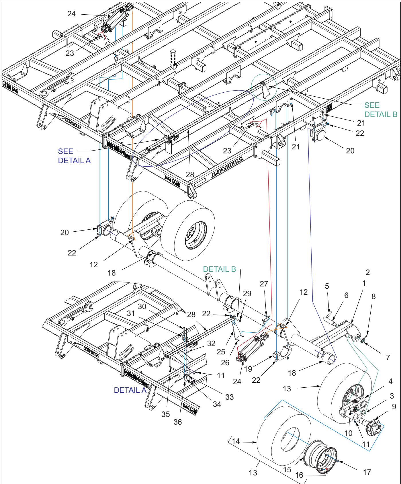
Figure 1-6: Center Lift Assembly 8530-33'-35'
