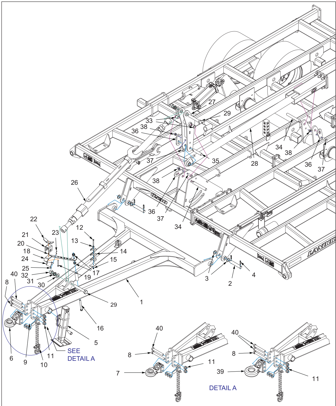
Figure 2-2: Hitch & Leveling Assembly 8530-27'-35'
