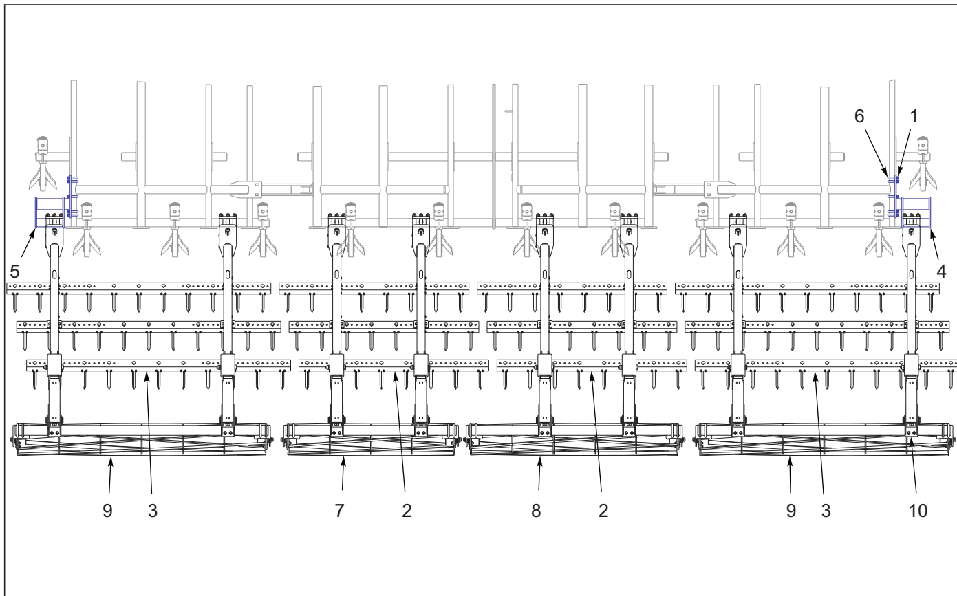
Figure 10-38: 3 Row Spike & Reel Layout 8530-27'
