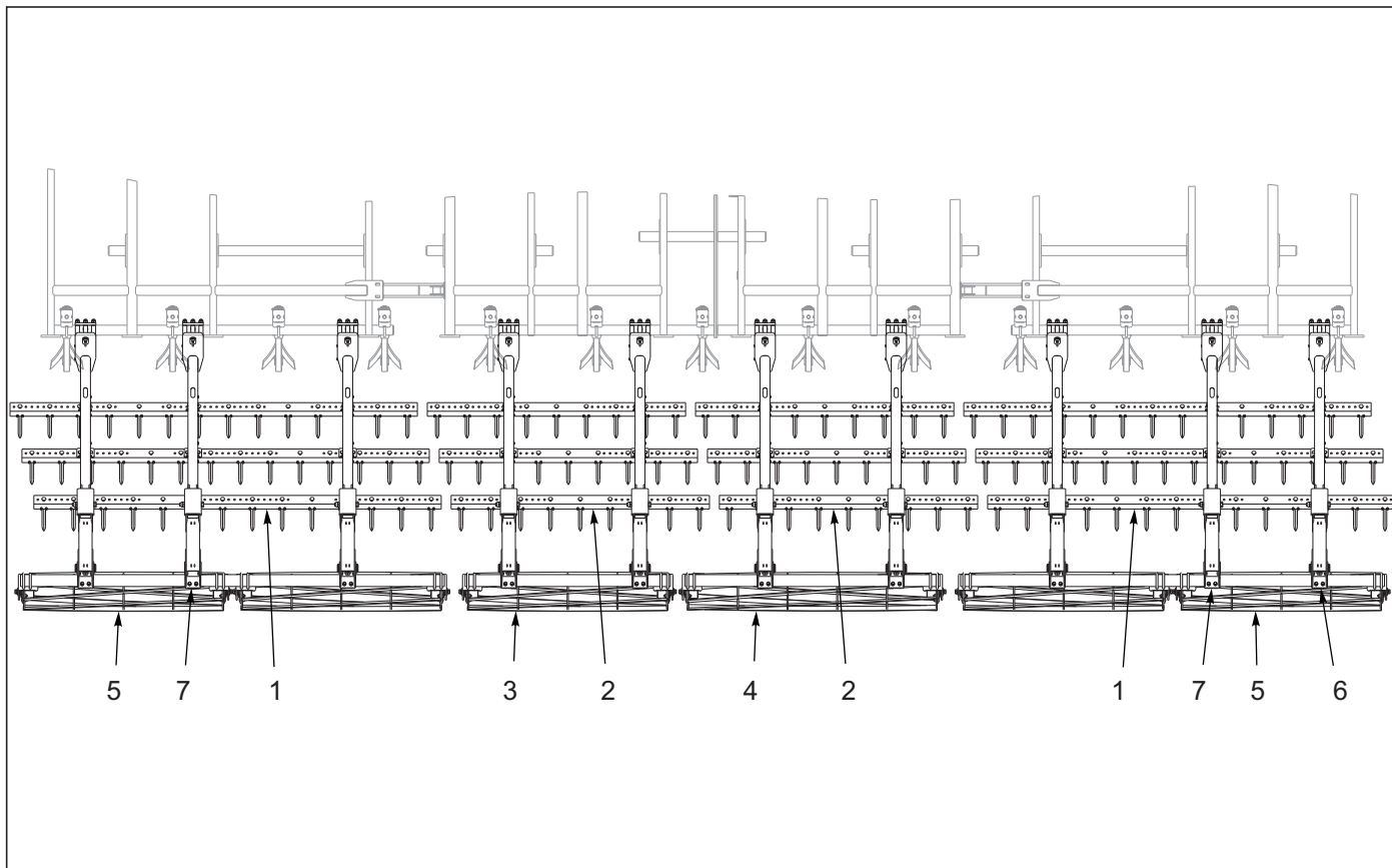
Figure 10-40: 3 Row Spike & Reel Layout 8530-33'
