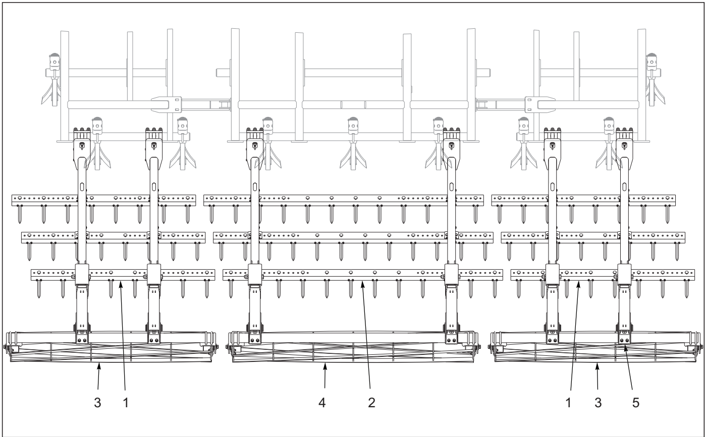
Figure 10-35: 3 Row Spike & Reel Layout 8530-19'
