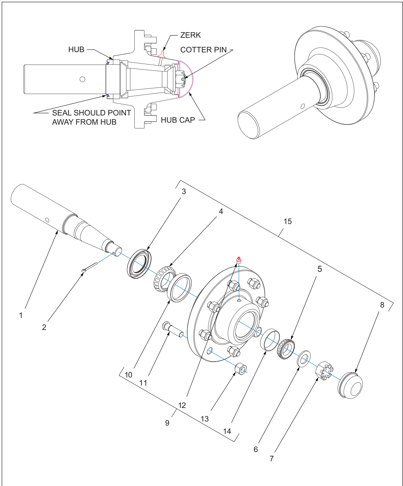
Figure 1-14: Hub and Spindle Assembly 147553
