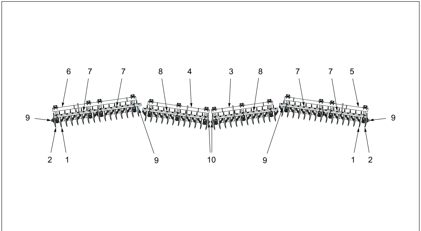
Figure 4-12: Gang Assembly 22" 4 GA 8530-35'
