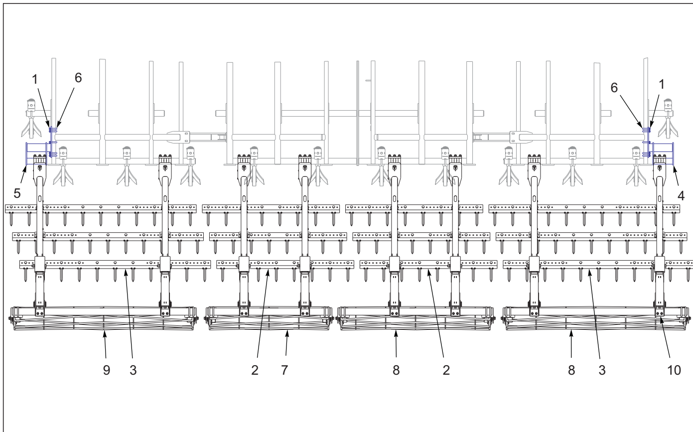
Figure 10-30: 3 Row Spike & Reel Layout 8530-27'
