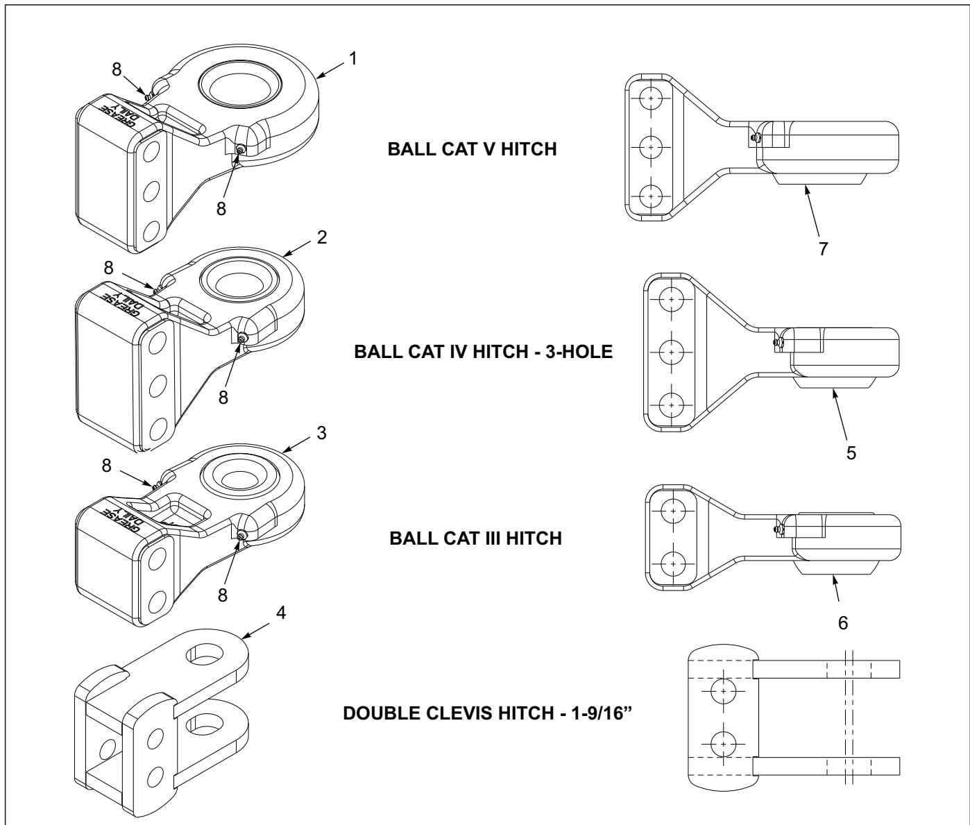
Figure 2-5: Hitch Assemblies
