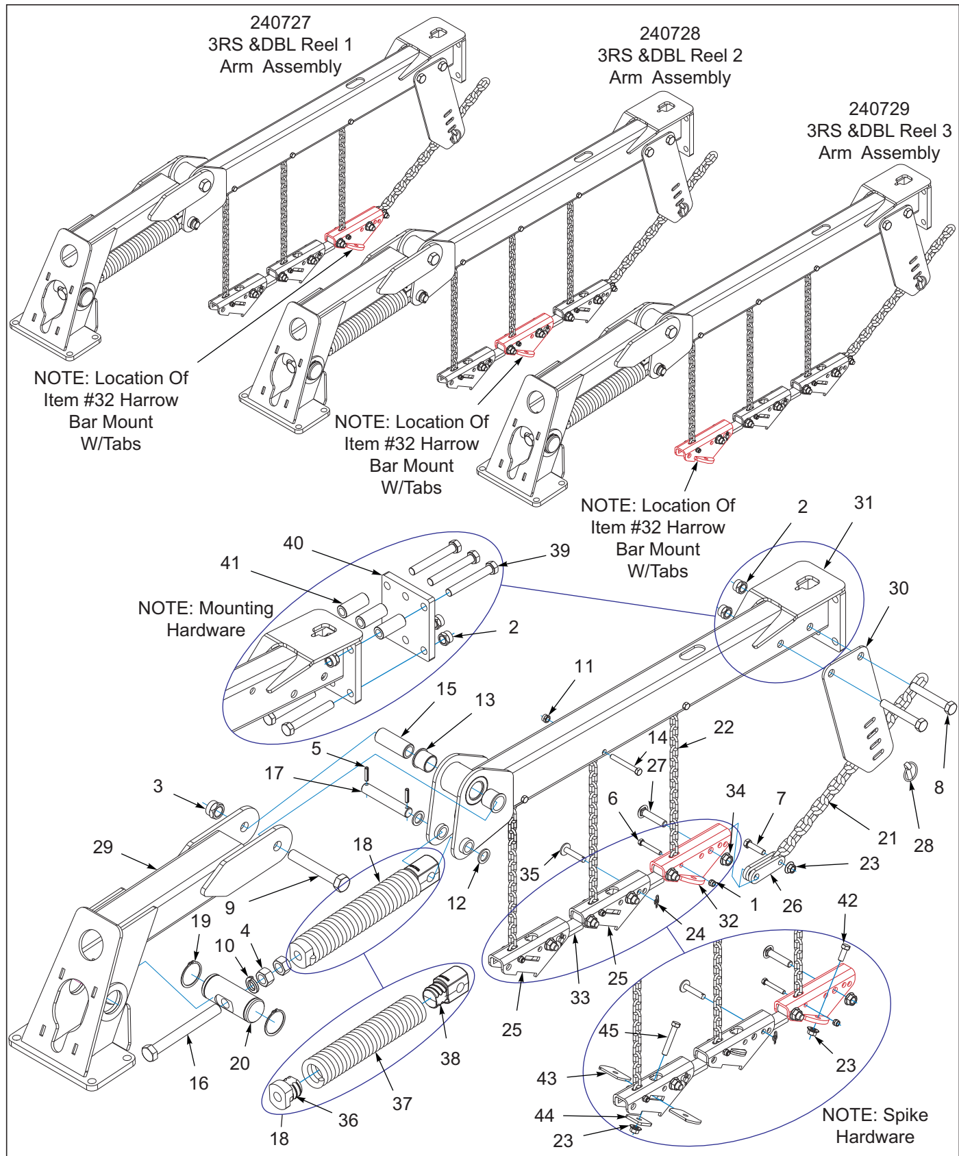
Figure 10-59: Arm Assembly 3RS and Double Reel
