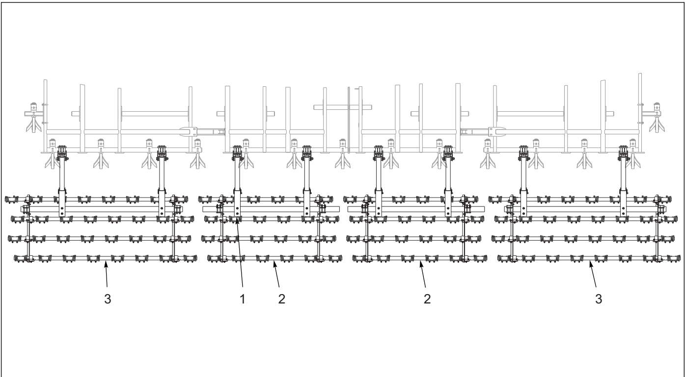
Figure 10-7: 4 Row Coil Tine Harrow Layout 8530-35'
