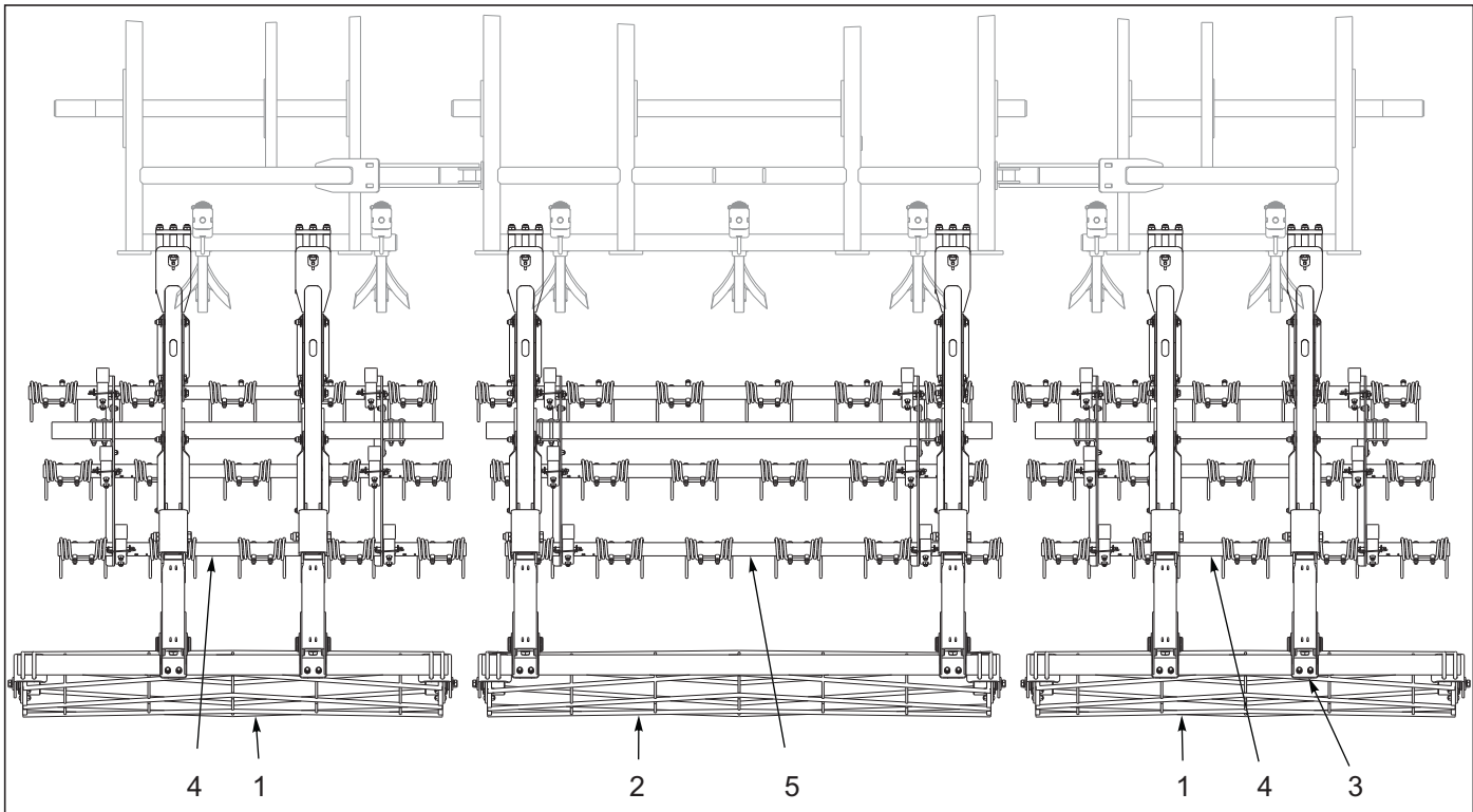
Figure 10-10: 3 Row Tine & Reel Layout 8530-19'
