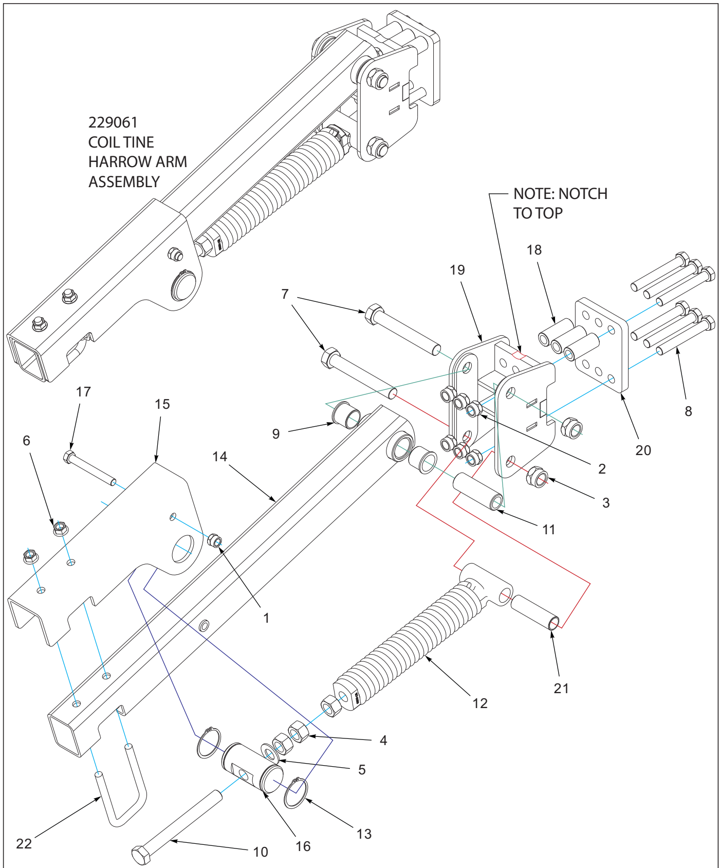
Figure 10-8: Coil Tine Harrow Arm Assembly
