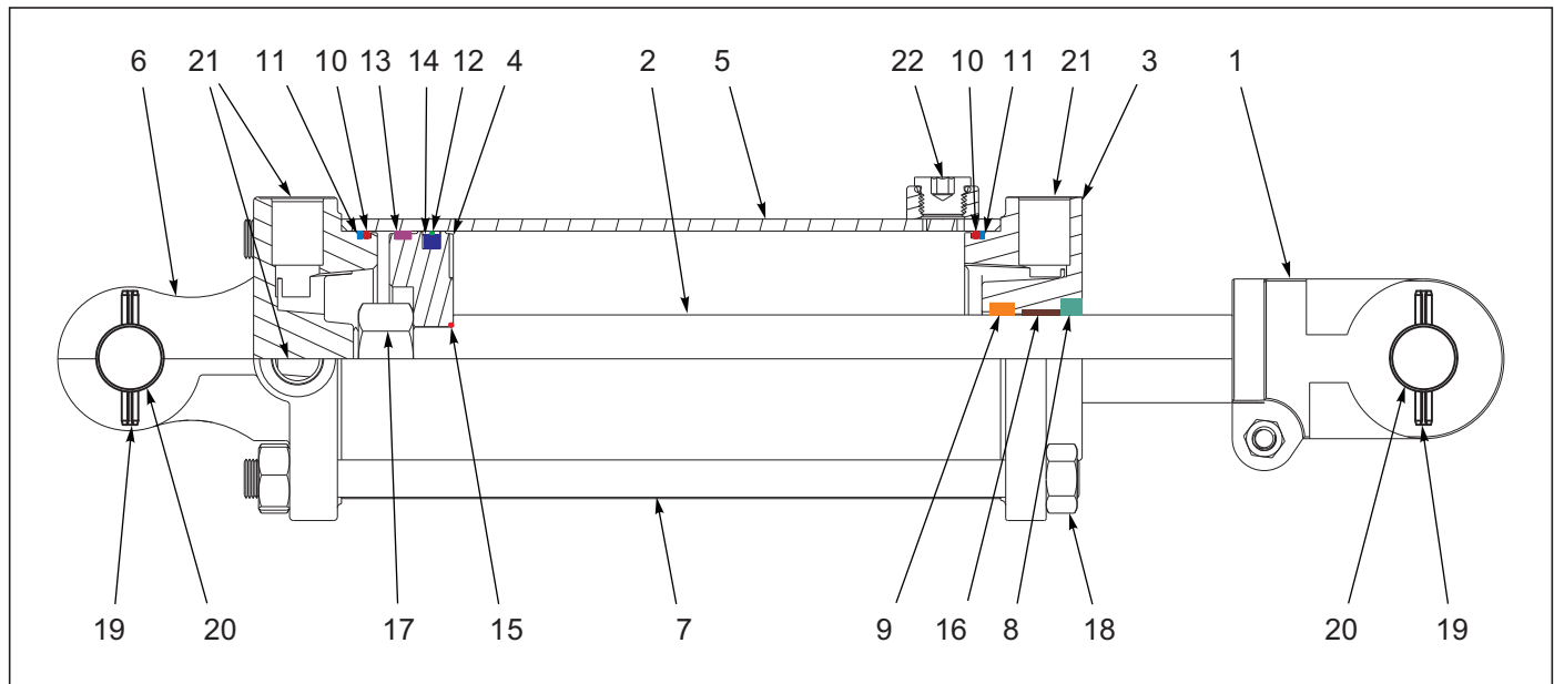
Figure 7-4: Cylinder Assembly 3-3/4 x 8, Rephase (Midway)
