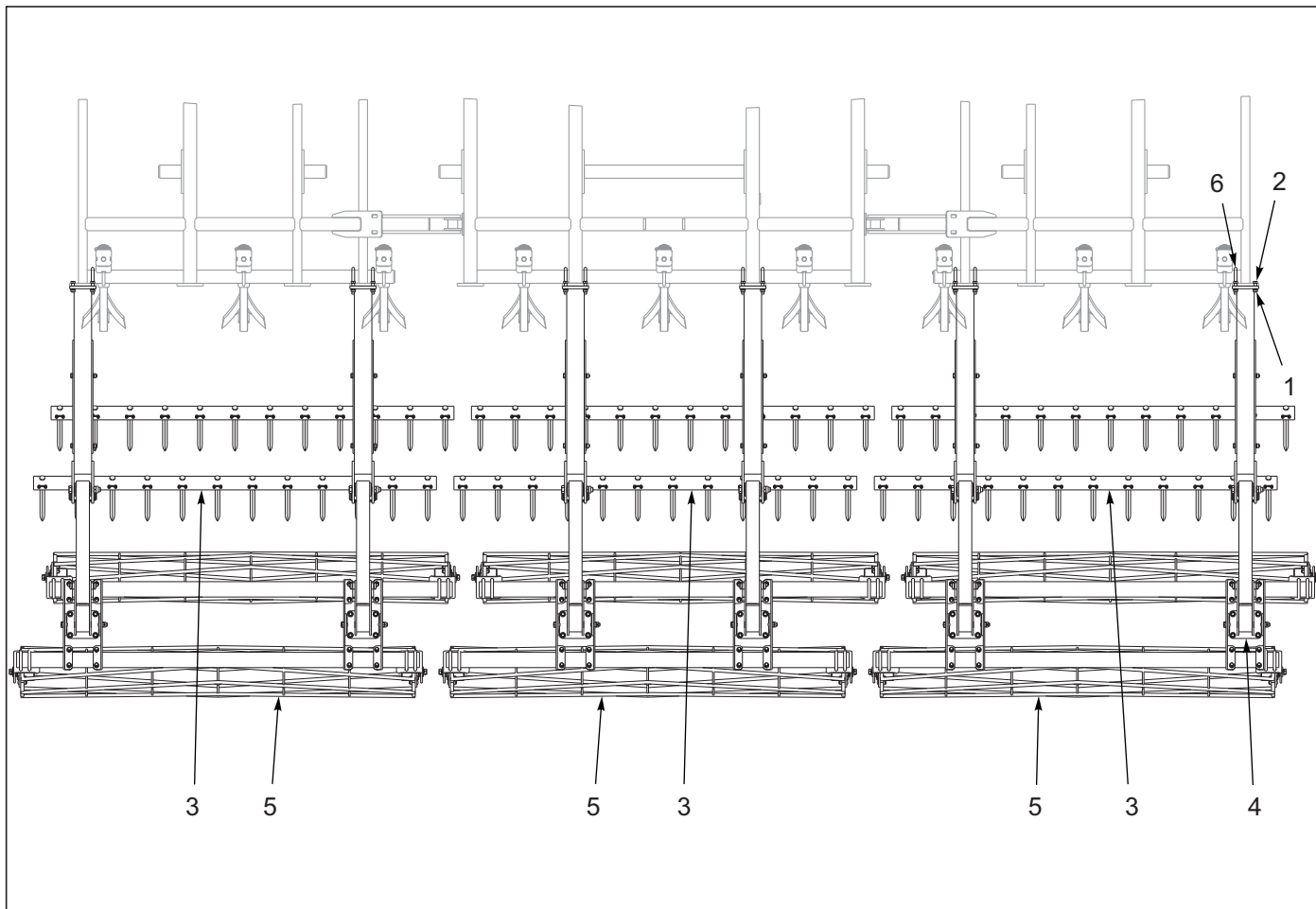
Figure 10-47: Spike & Double Reel Layout 8530-22'
