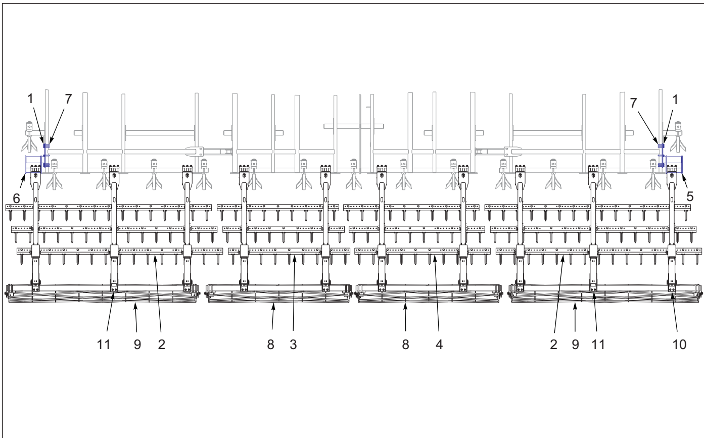
Figure 10-33: 3 Row Spike & Reel Layout 8530-35'
