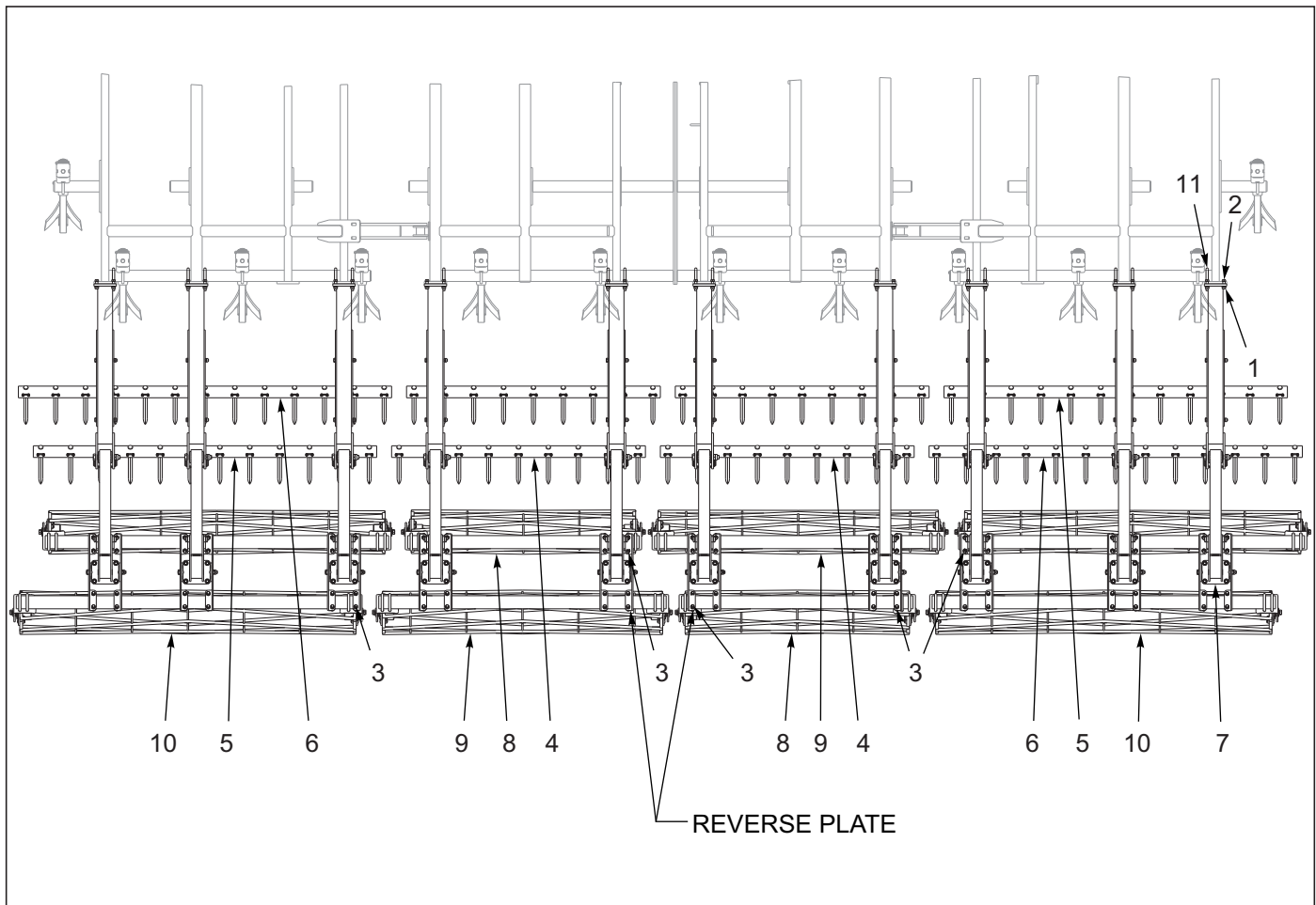
Figure 10-49: Spike & Double Reel Layout 8530-27'
