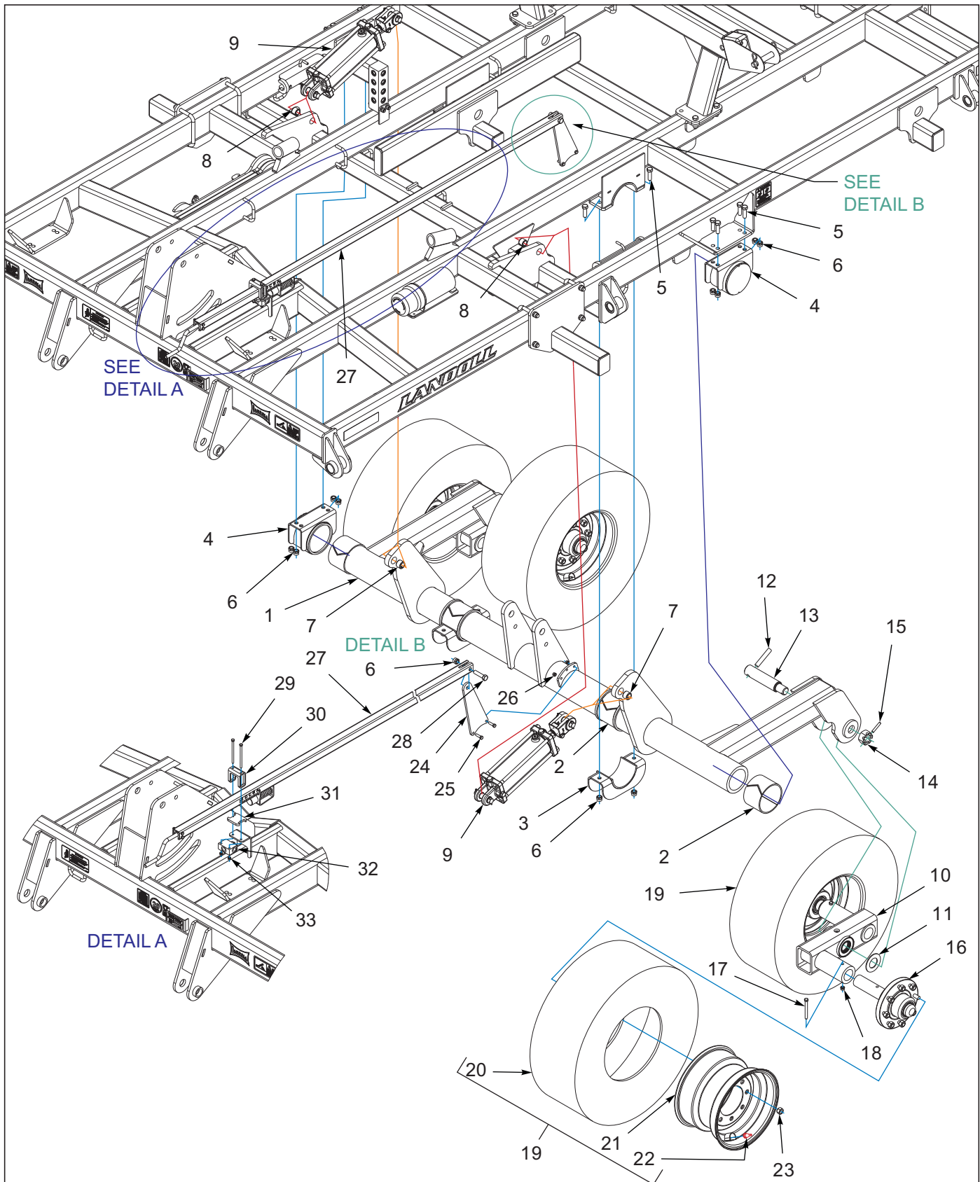
Figure 1-4: Center Lift Assembly 8530-19'-25'
