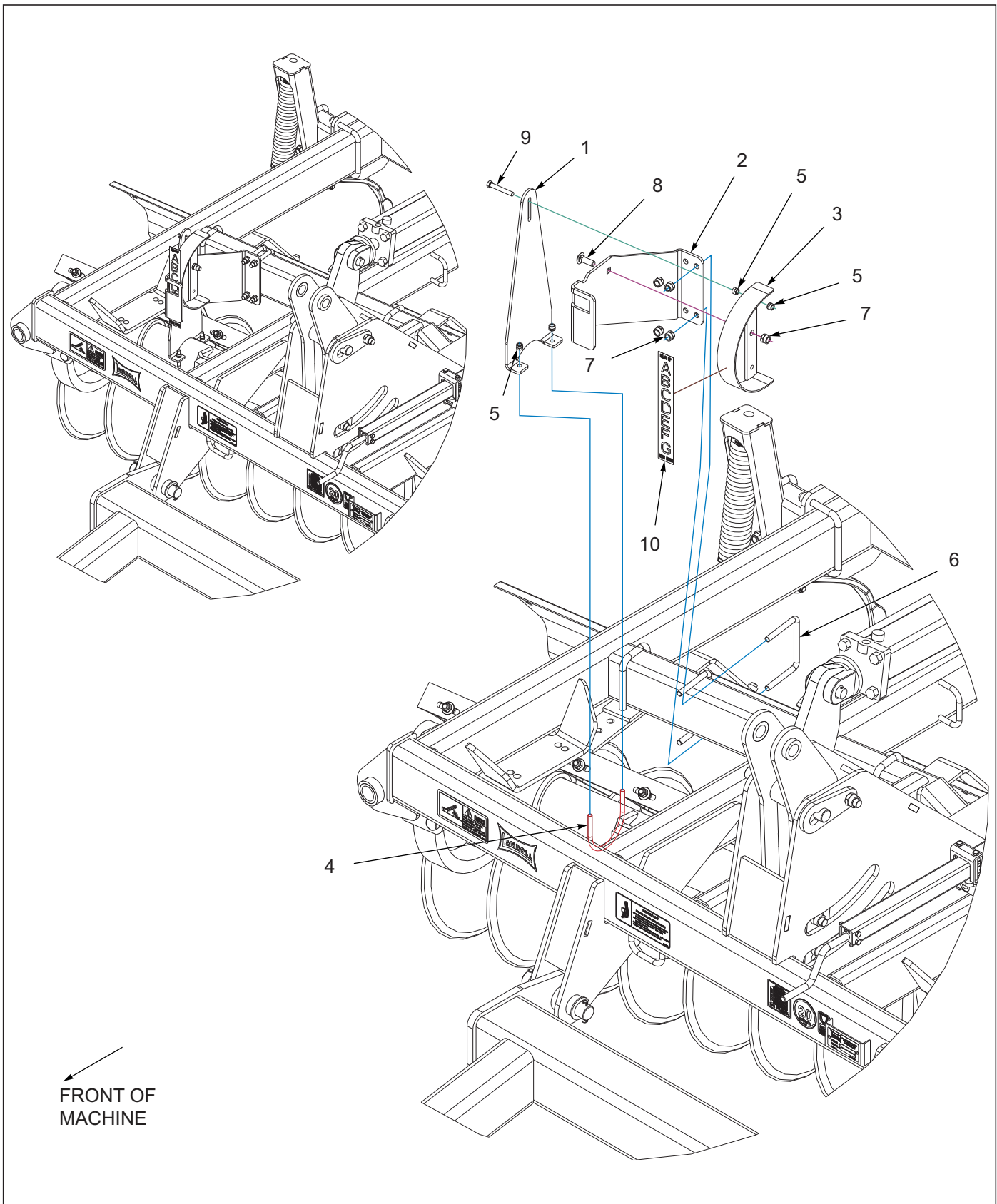
Figure 4-2: Depth Gauge Assembly
