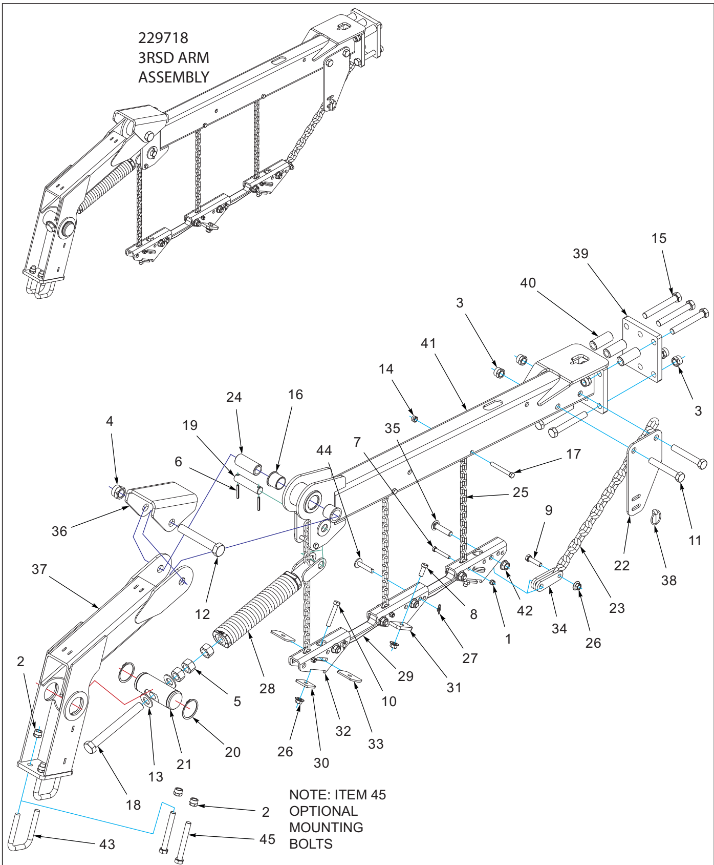
Figure 10-44: 3 RSD Arm Assembly
