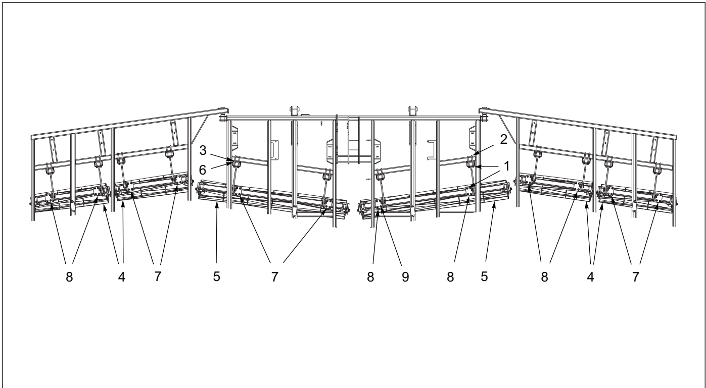
Figure 4-17: Disc Gang Reel Assembly 8530-30'
