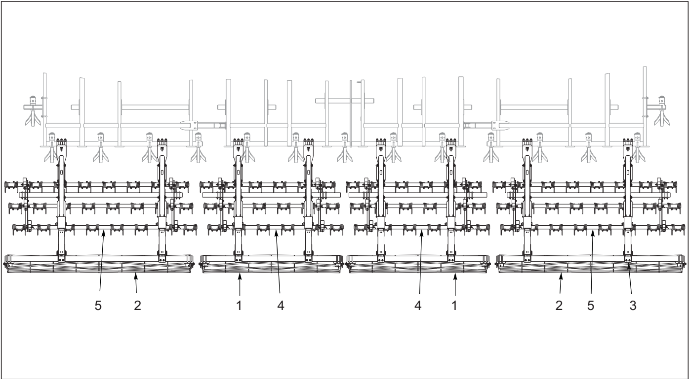
Figure 10-16: 3 Row Tine & Reel Layout 8530-35'
