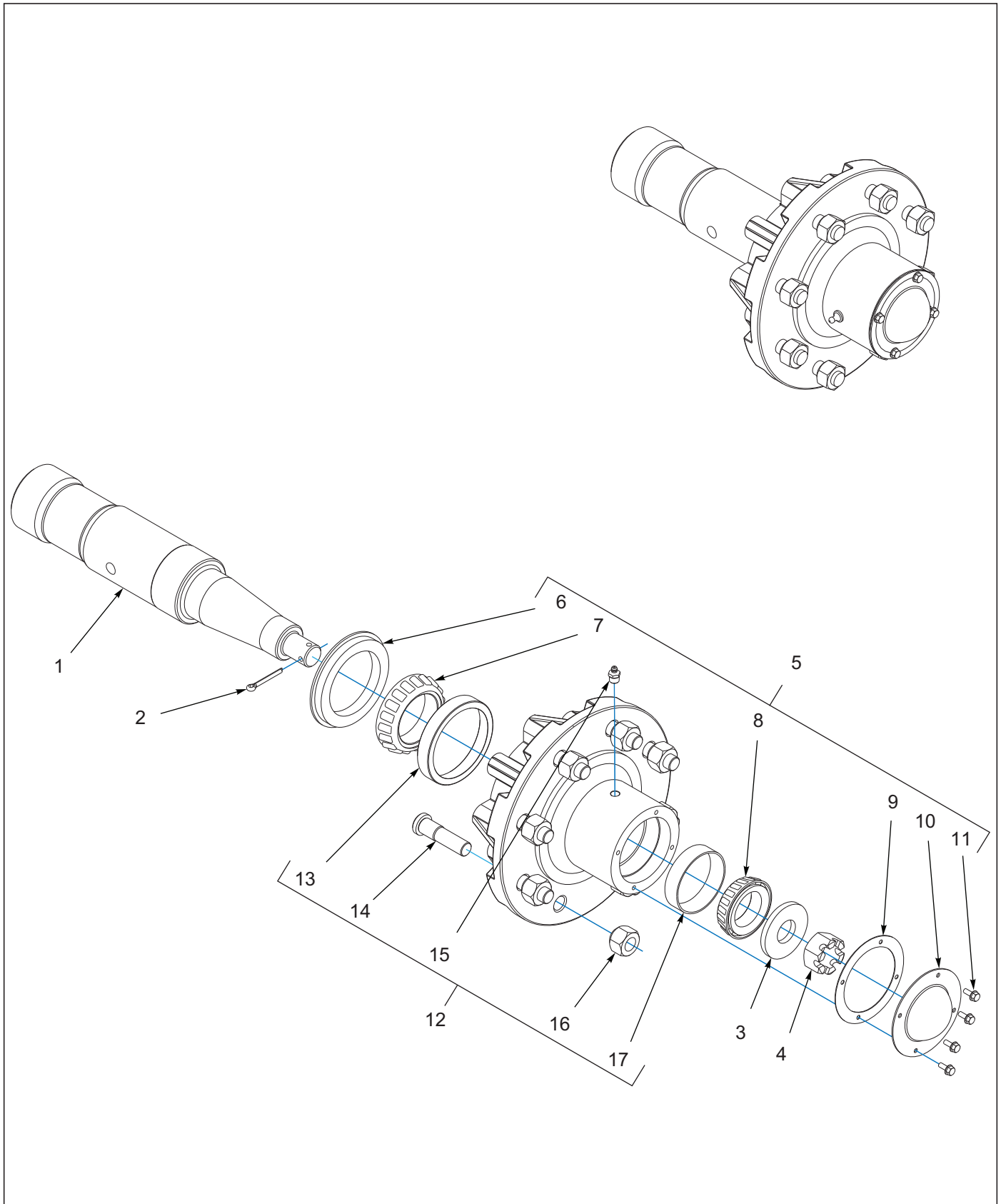
Figure 1-13: Hub and Spindle Assembly 223440
