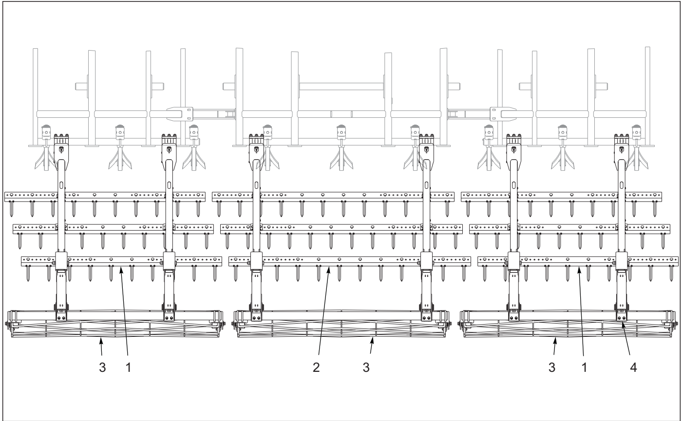
Figure 10-28: 3 Row Spike & Reel Layout 8530-22'
