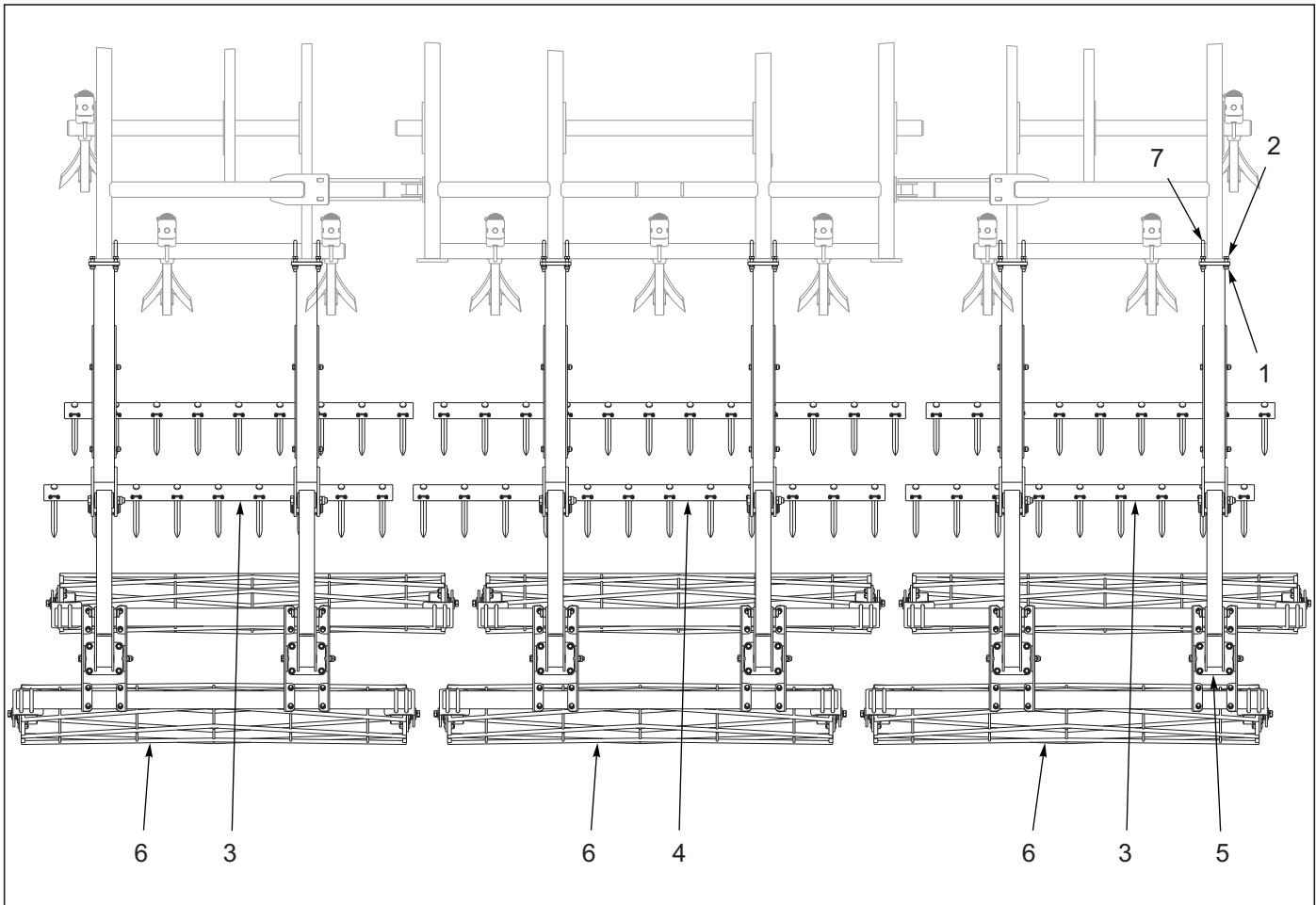
Figure 10-46: Spike & Double Reel Layout 8530-19'
