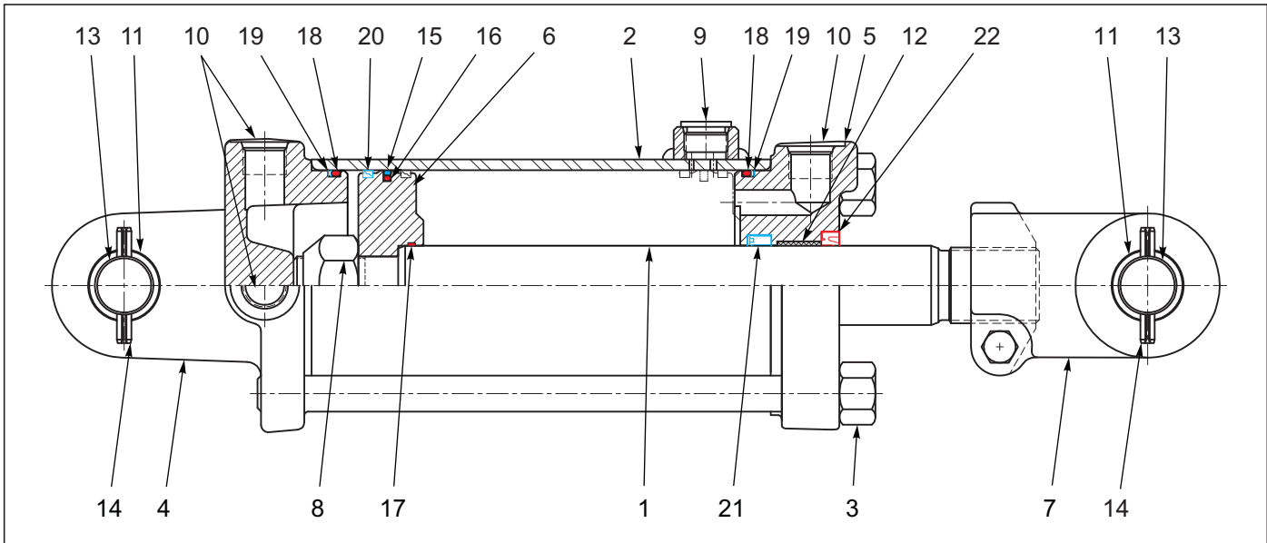
Figure 7-9: Cylinder Assembly 3-3/4 x 10, Rephase
