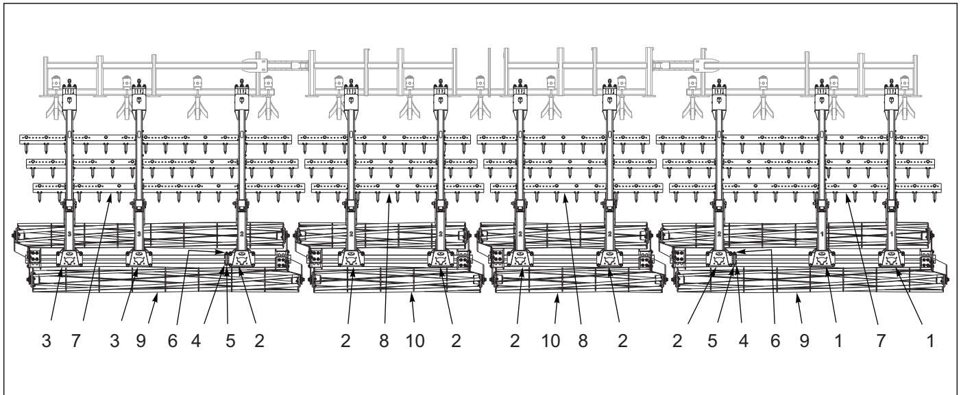
Figure 10-58: 3RS & Double Flat Reel Layout 8530-33'
