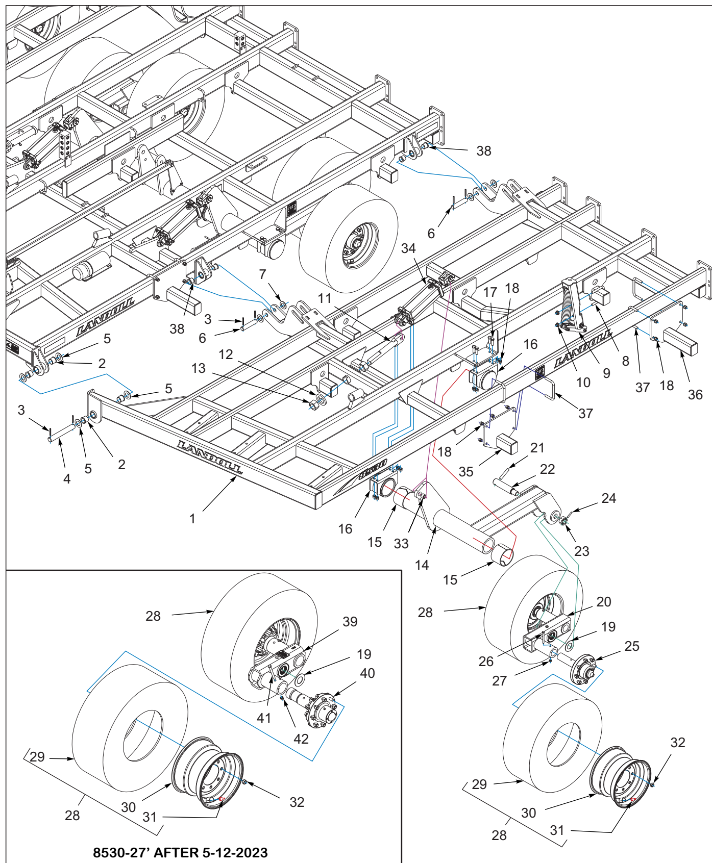
Figure 1-8: Wing Frame and Lift Assembly 8530-22'-27'
