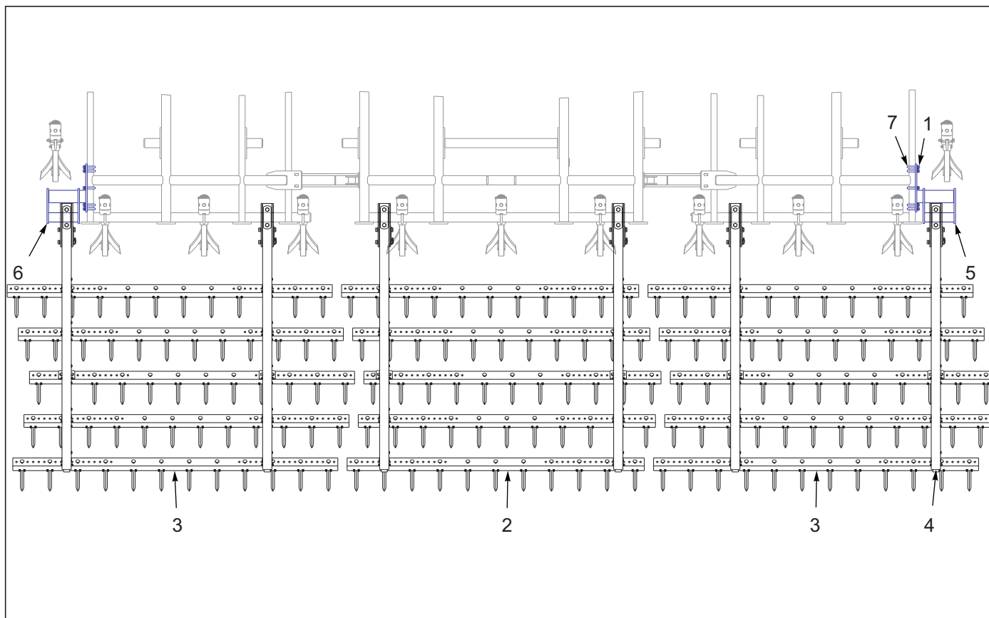
Figure 10-21: 5 Row Spike Harrow Layout 8530-25'
