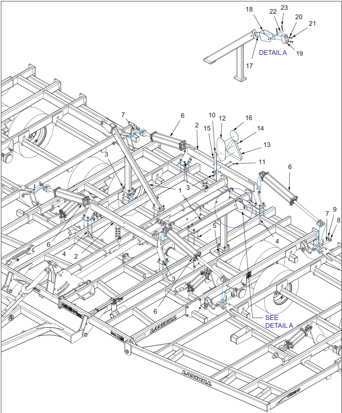
Figure 3-4: Fold Assembly 8530-33'-35'
