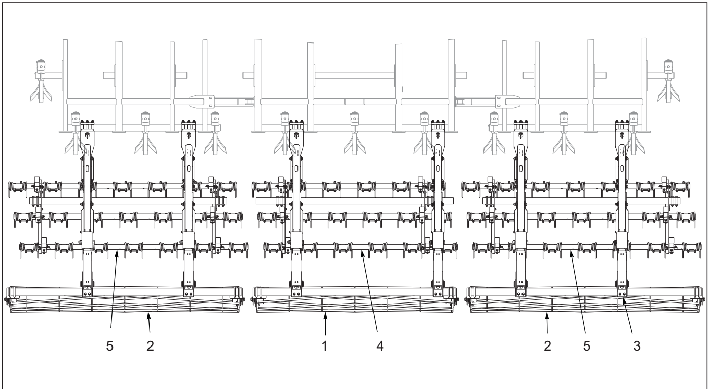
Figure 10-12: 3 Row Tine & Reel Layout 8530-25'
