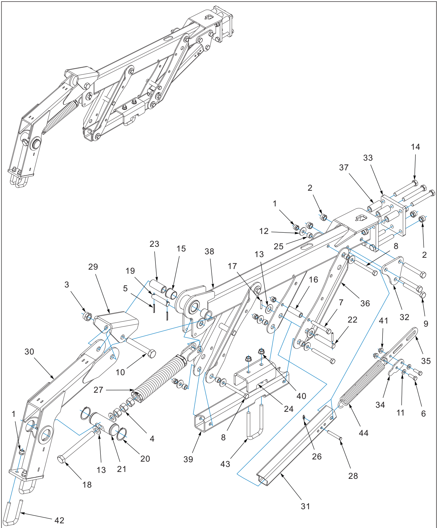
Figure 10-17: Tine & Reel Arm Assembly
