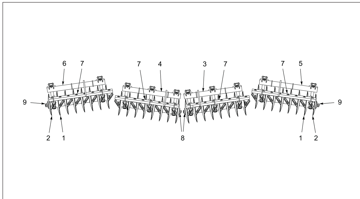
Figure 4-6: Gang Assembly 22" 4 GA 8530-19'
