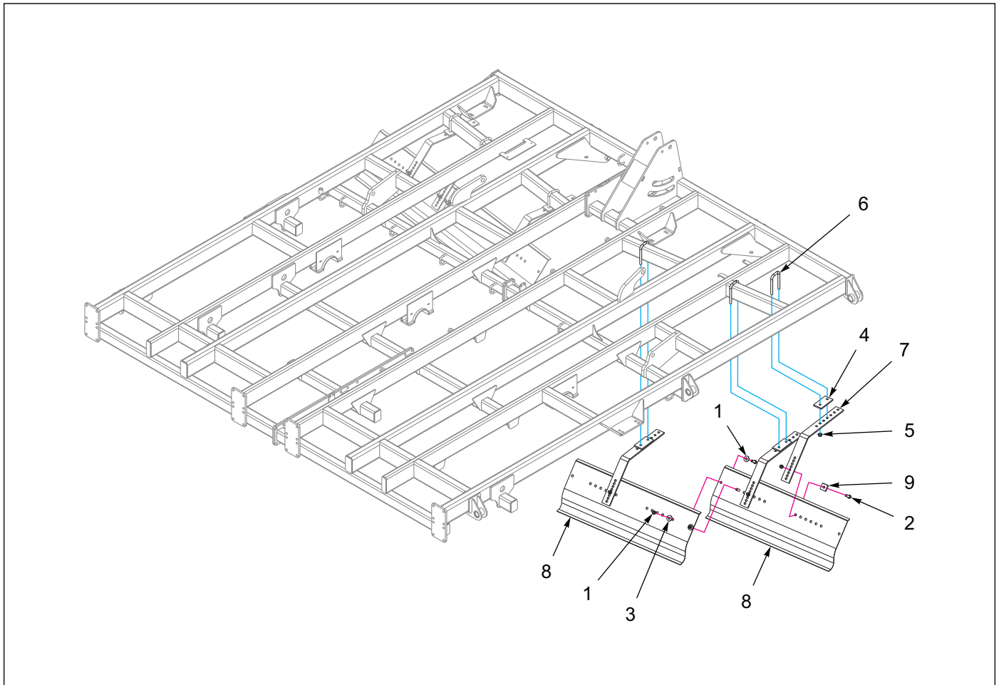
Figure 4-4: Disc Gang Shield - Center Frame 33'-35'
