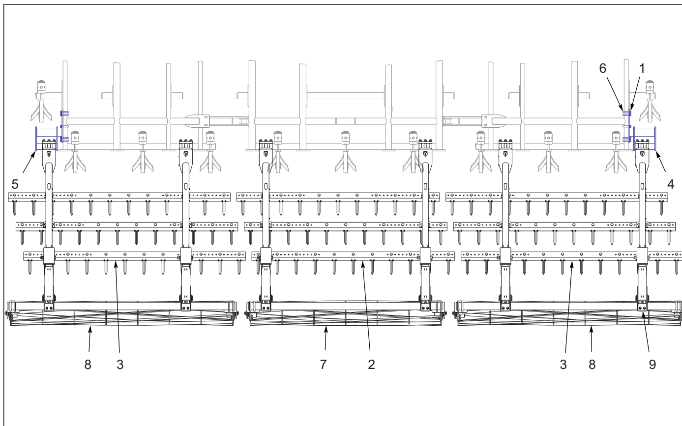
Figure 10-37: 3 Row Spike & Reel Layout 8530-25'
