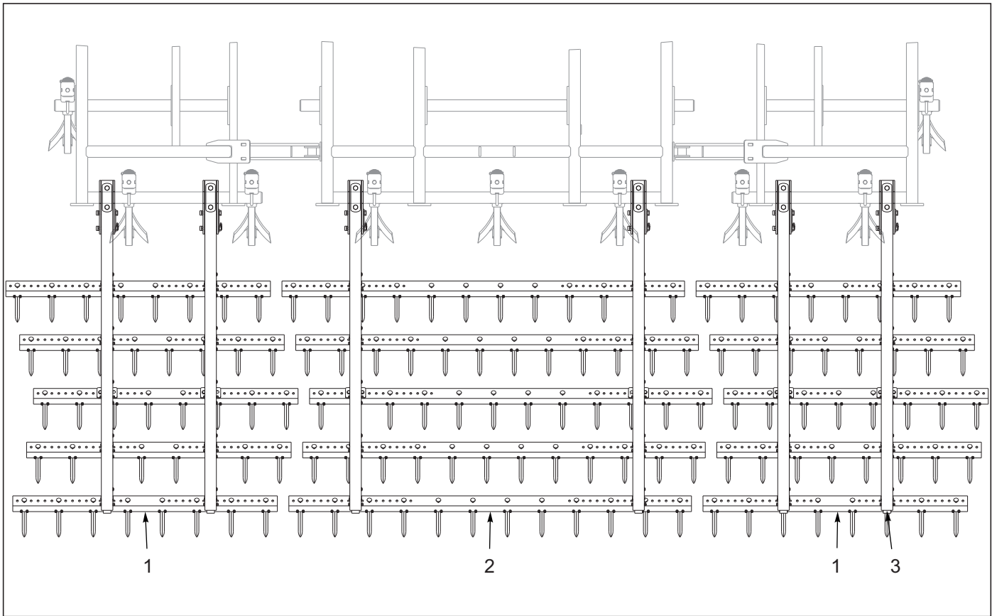
Figure 10-19: 5 Row Spike Harrow Layout 8530-19'
