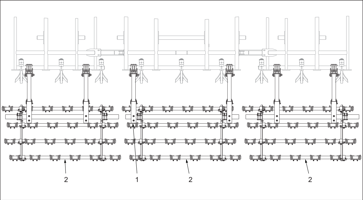
Figure 10-2: 4 Row Coil Tine Harrow Layout 8530-22'
