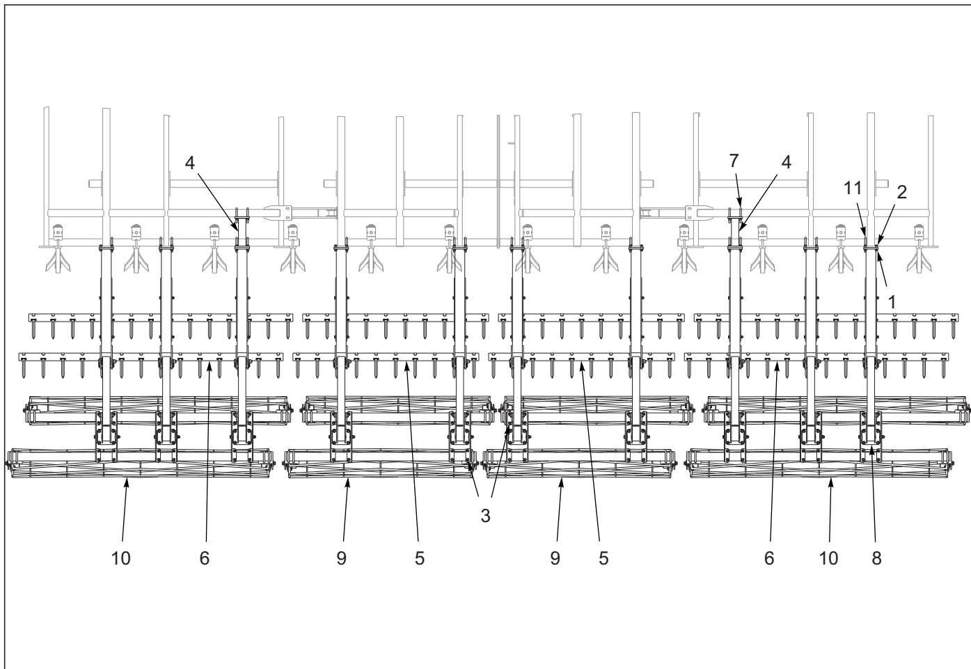
Figure 10-50: Spike & Double Reel Layout 8530-30'
