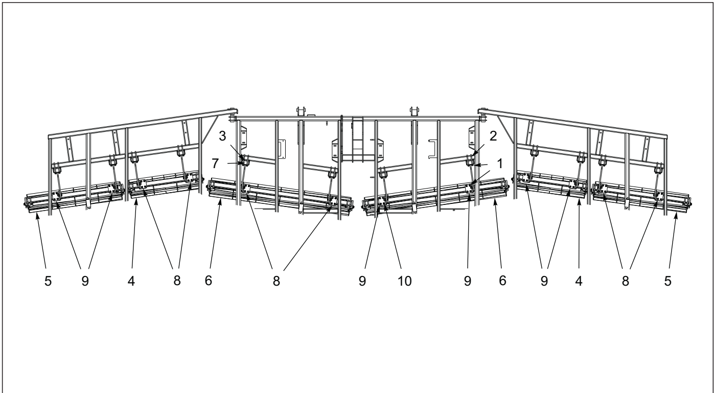
Figure 4-19: Disc Gang Reel Assembly 8530-35'
