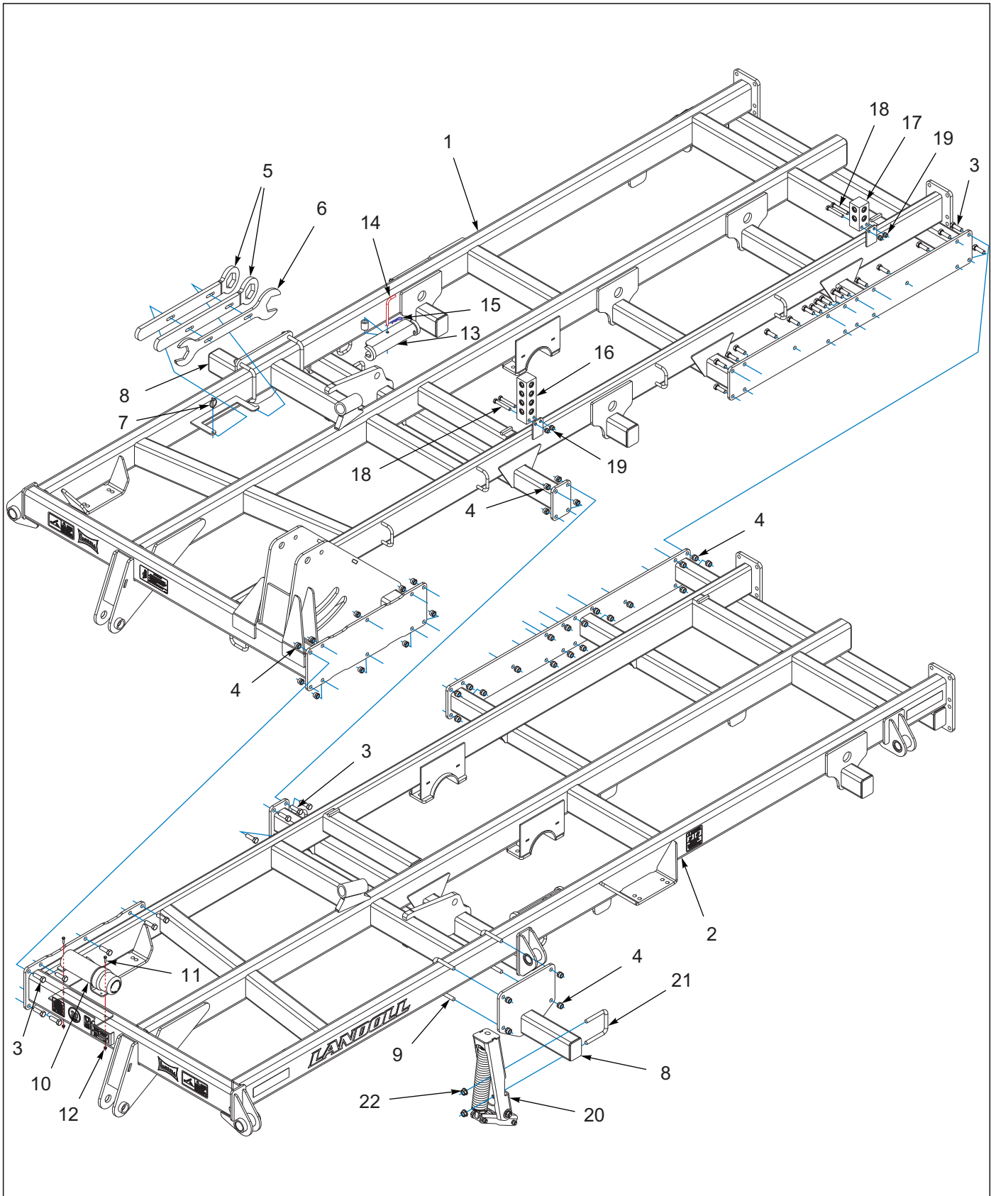
Figure 1-2: Center Frame Assembly 8530-27'-30'
