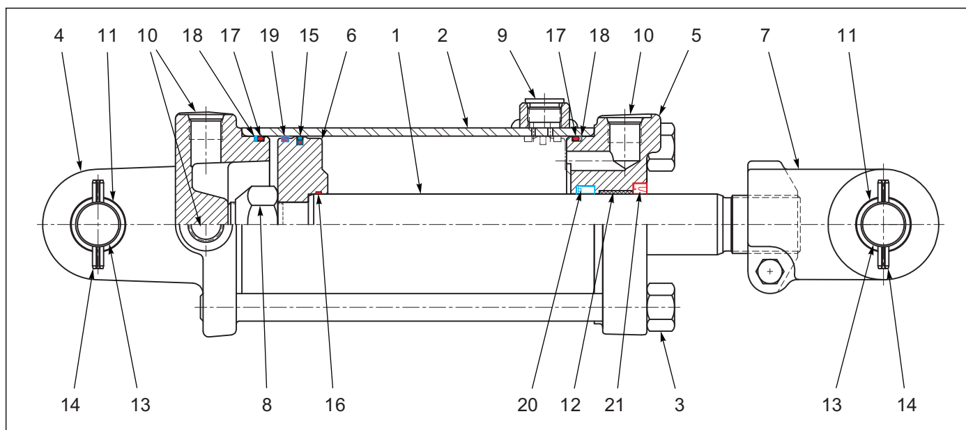
Figure 7-1: Cylinder Assembly 4 x 8, Rephase (Prince)
