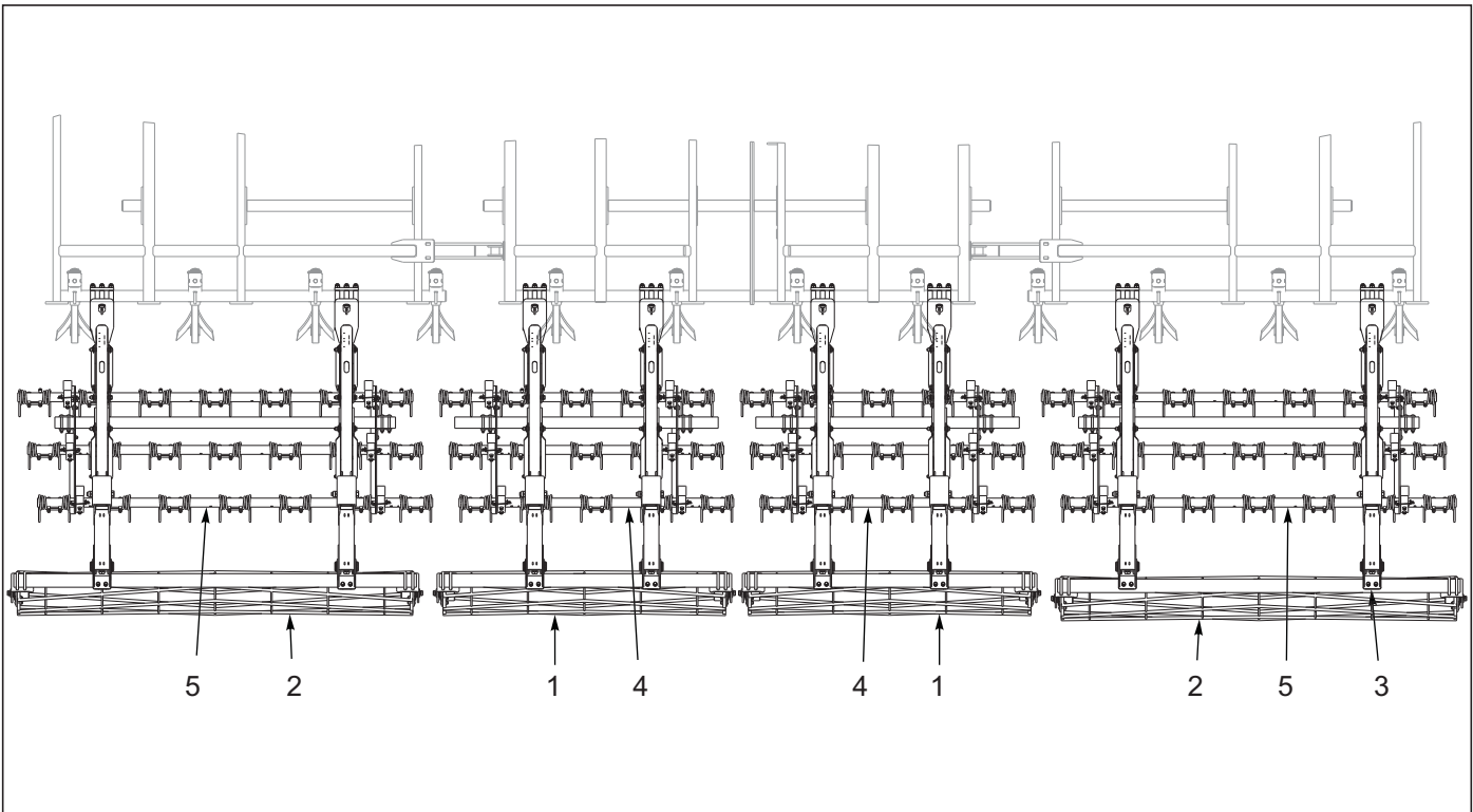
Figure 10-14: 3 Row Tine & Reel Layout 8530-30'
