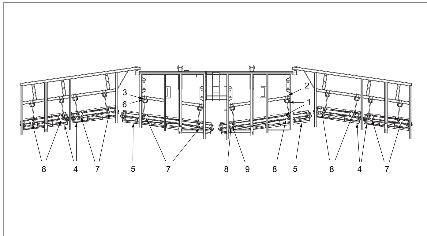
Figure 4-18: Disc Gang Reel Assembly 8530-33'
