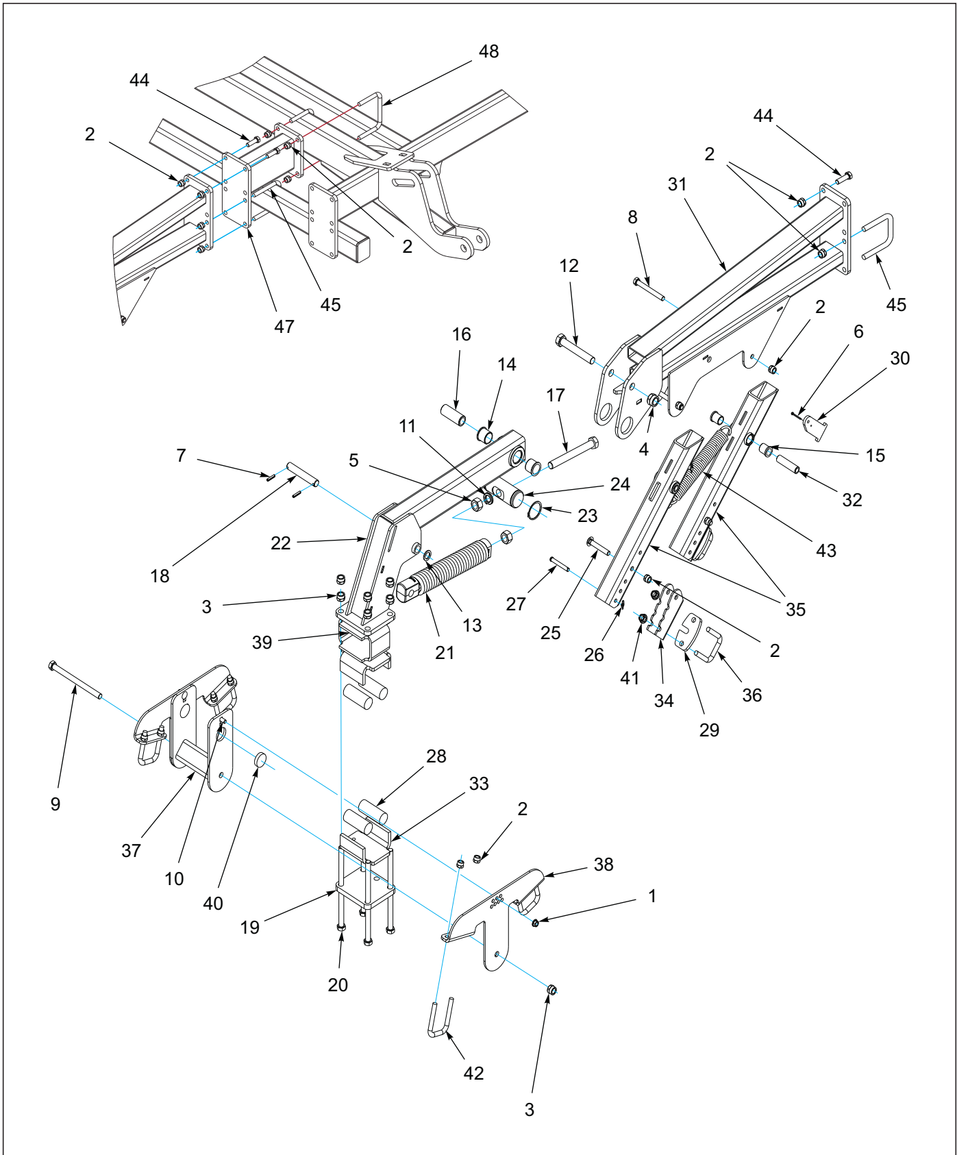
Figure 10-53: Double Reel Harrow Arm Assembly
