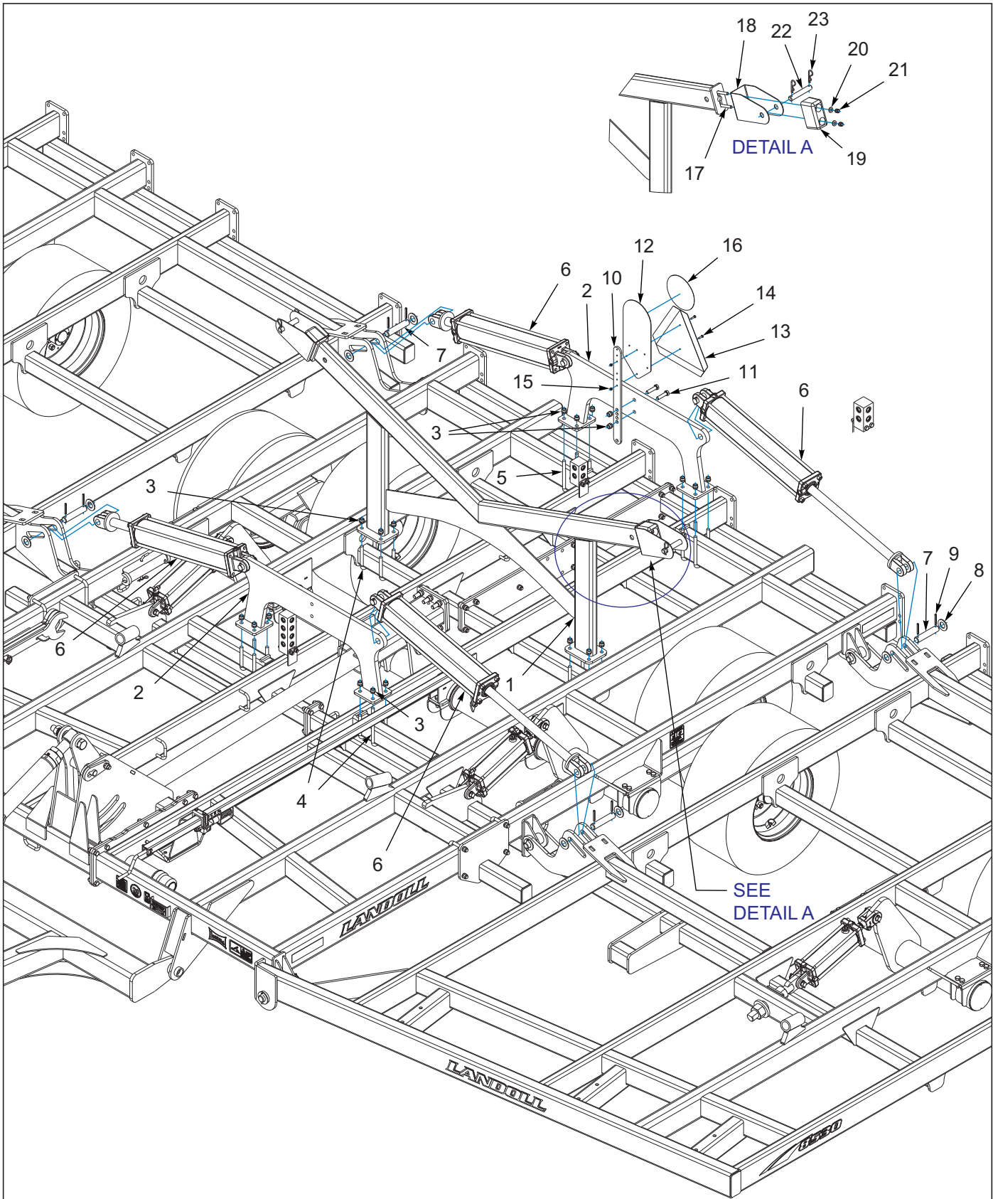
Figure 3-3: Fold Assembly 8530-27'-30'
