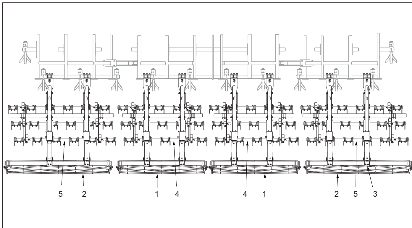
Figure 10-13: 3 Row Tine & Reel Layout 8530-27'
