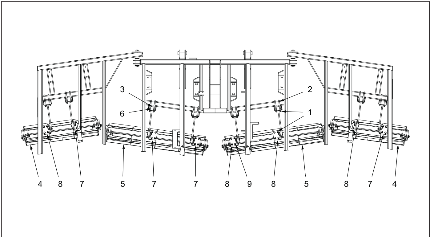
Figure 4-13: Disc Gang Reel Assembly 8530-19'
