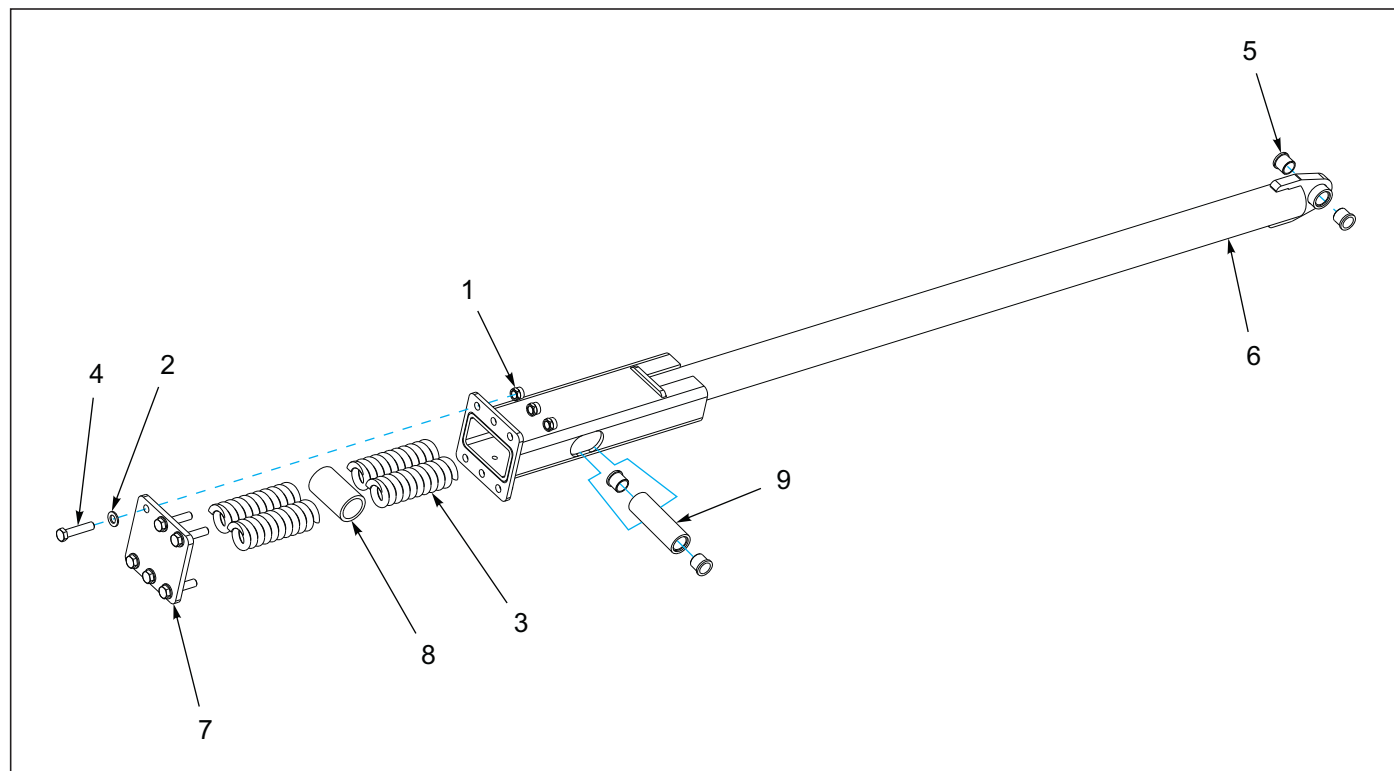
Figure 2-6: Leveler Assembly - Spring
