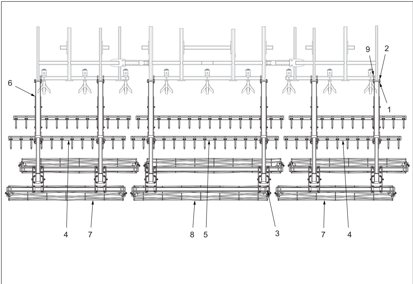
Figure 10-48: Spike & Double Reel Layout 8530-25'
