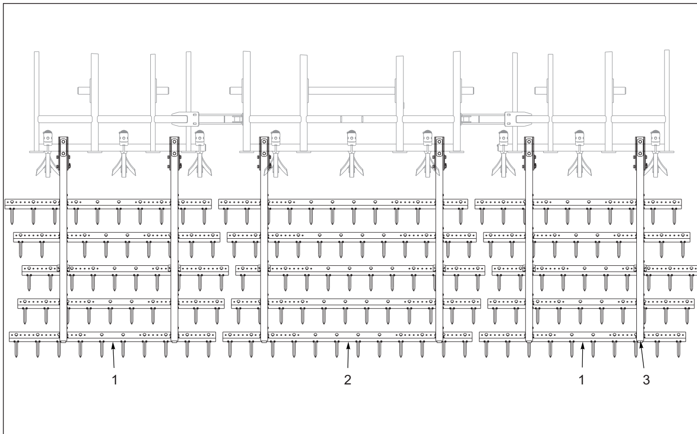
Figure 10-20: 5 Row Spike Harrow Layout 8530-22'
