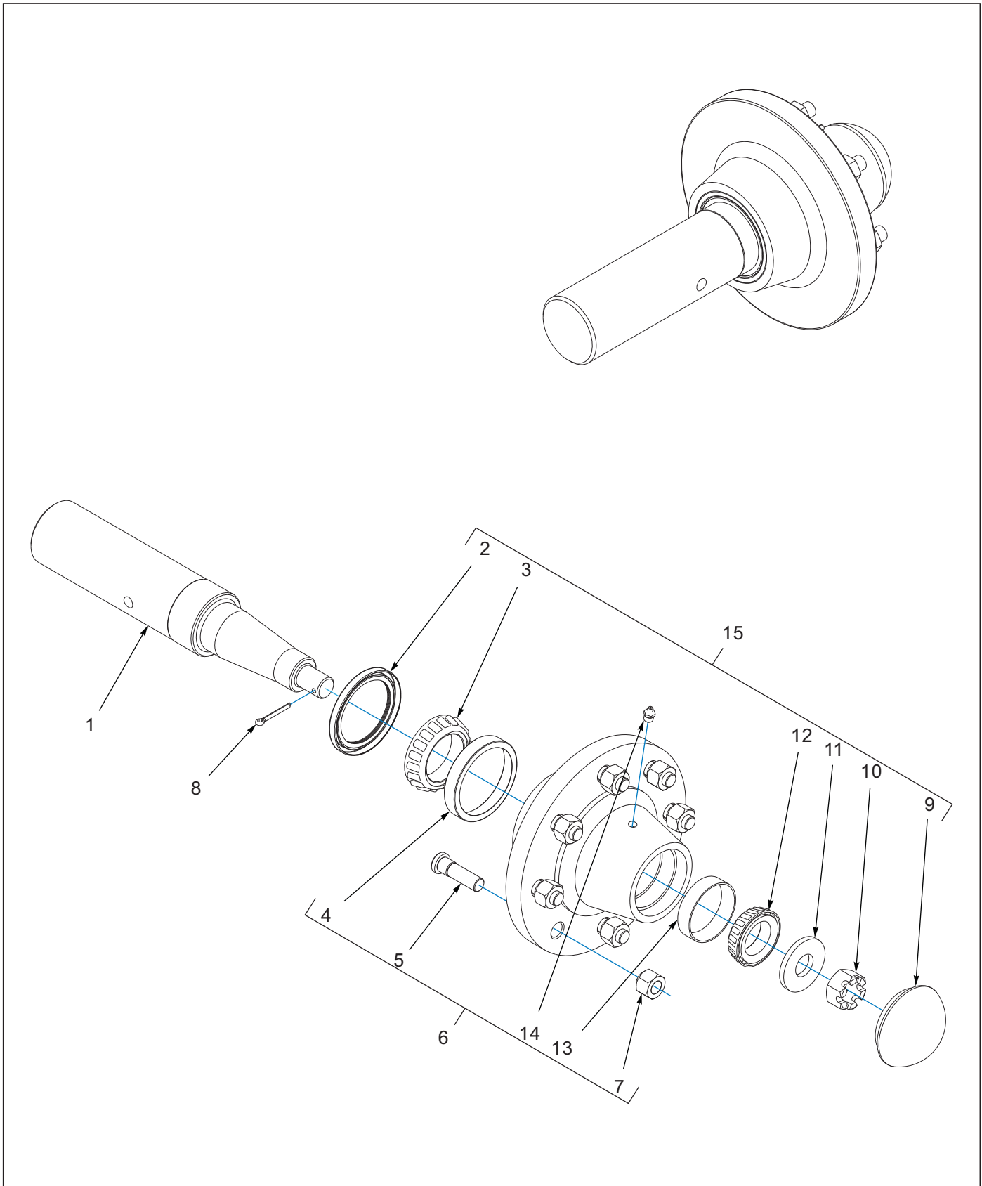
Figure 1-12: Hub and Spindle Assembly 156972
