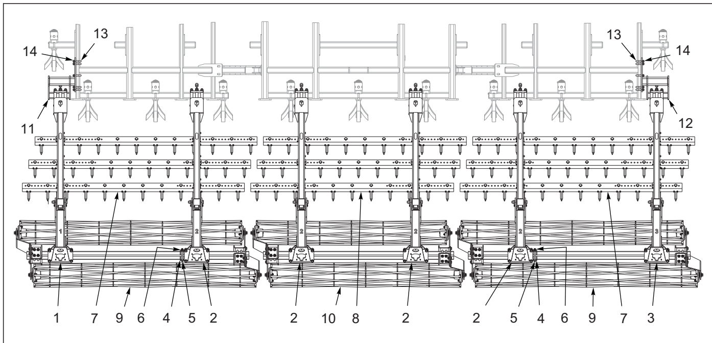
Figure 10-55: 3RS & Double Conditioner Reel Layout 8530-25'
