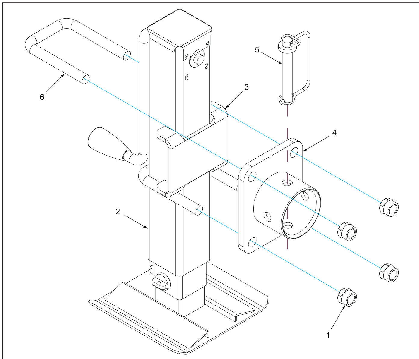
Figure 2-4: Jack Assembly 183967
