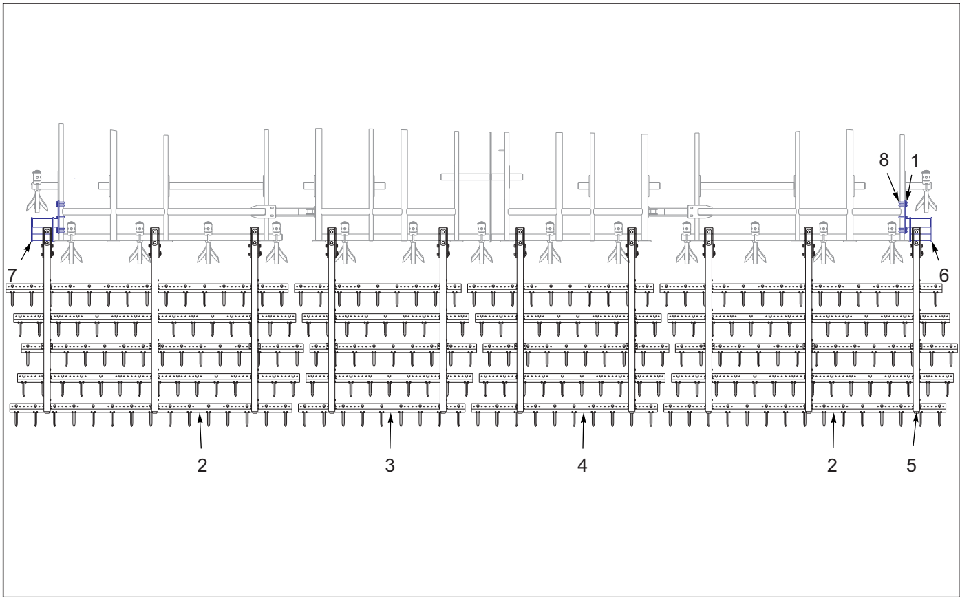
Figure 10-25: 5 Row Spike Harrow Layout 8530-35'
