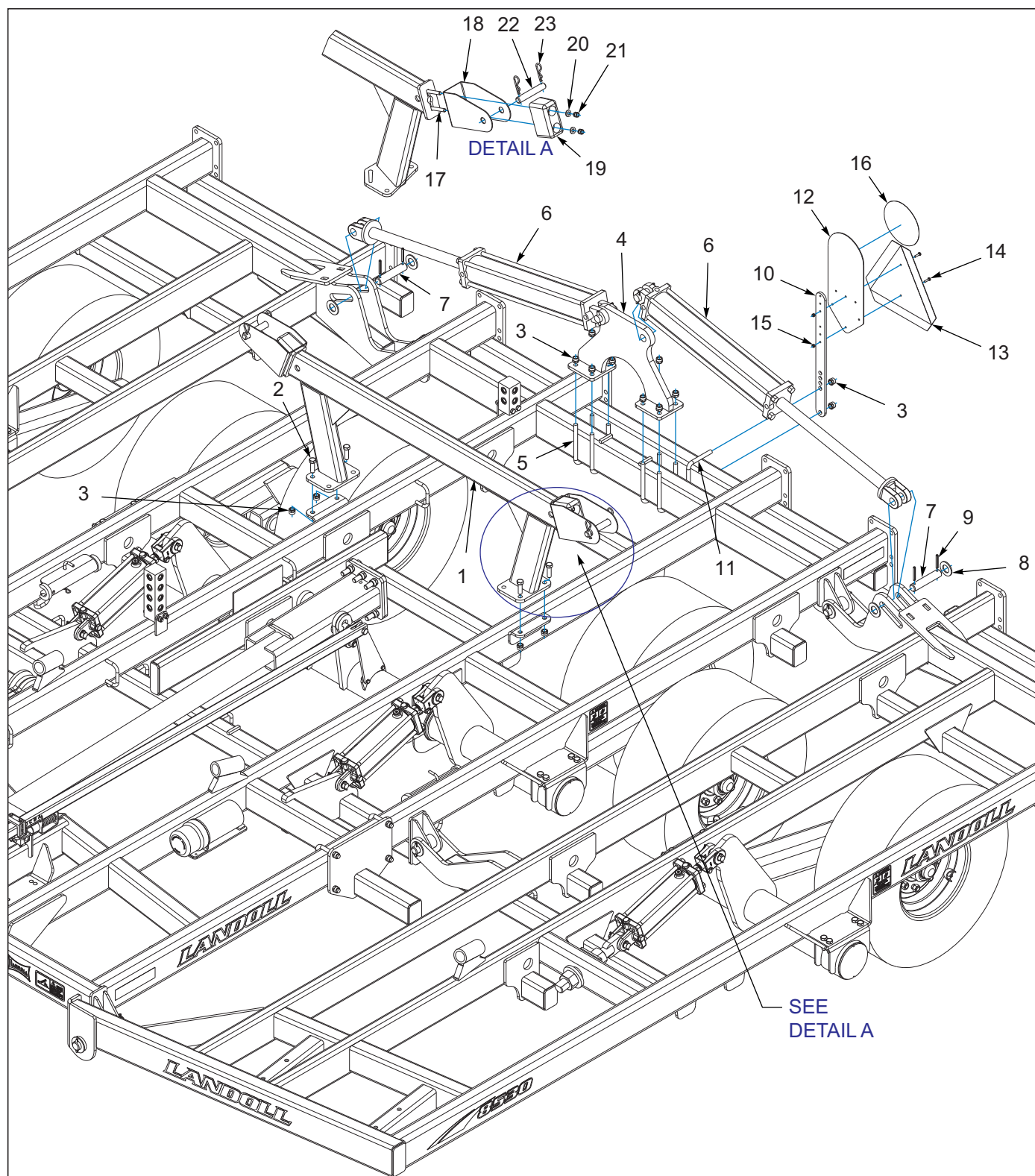
Figure 3-1: Fold Assembly 8530-19'
