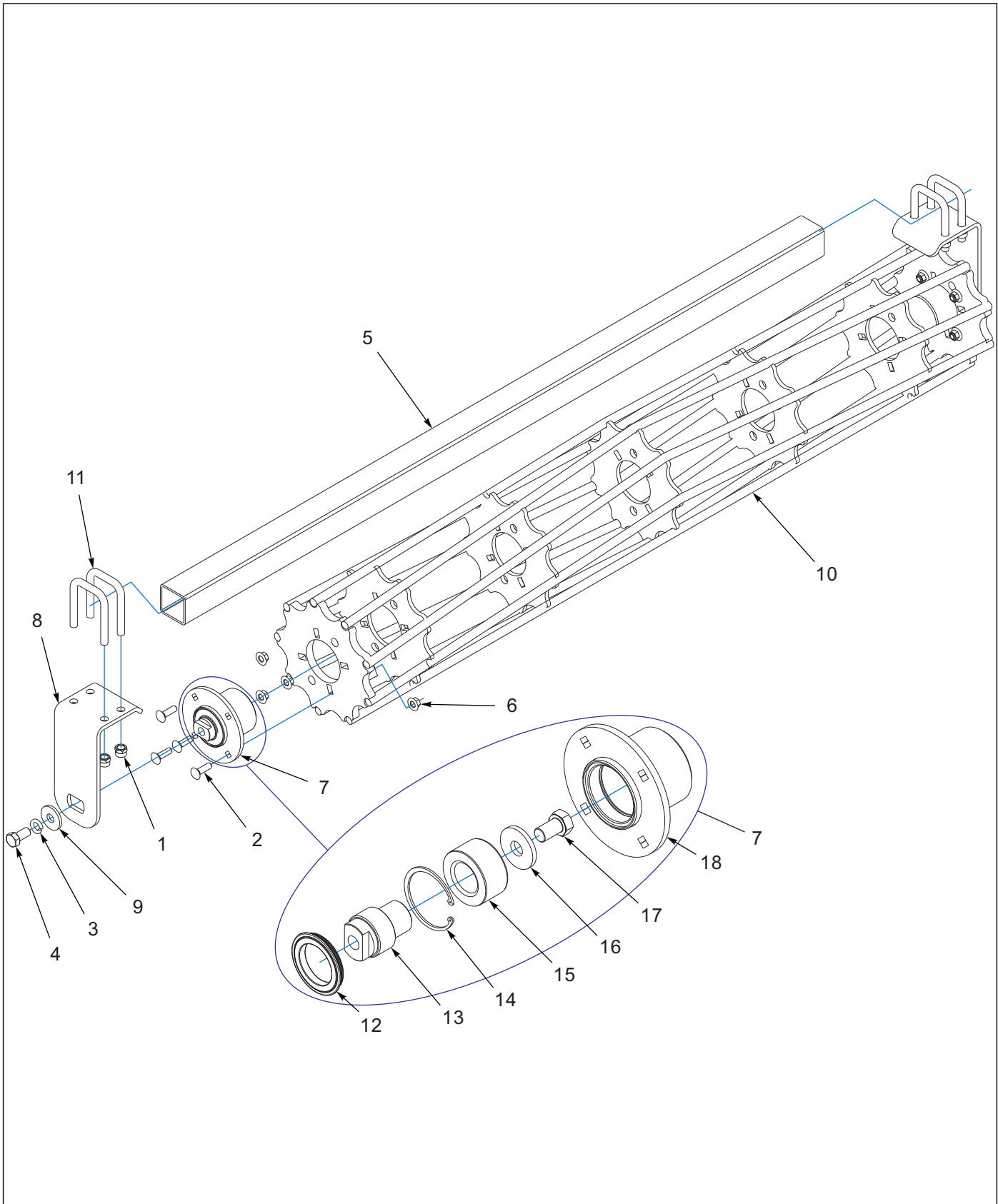
Figure 10-34: Round Bar Reel Assembly
