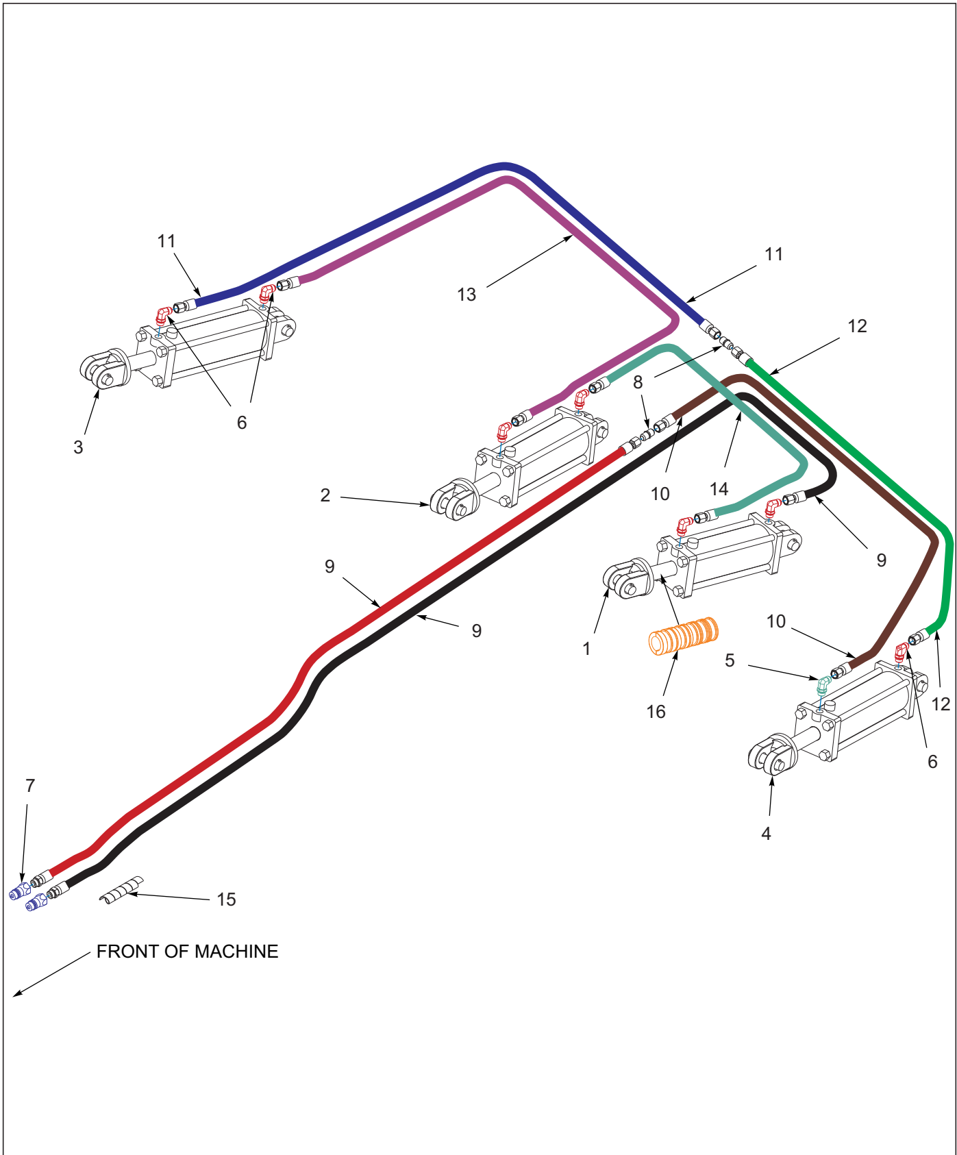
Figure 6-10: Gang Hydraulic Assembly 8530-33'-35'
