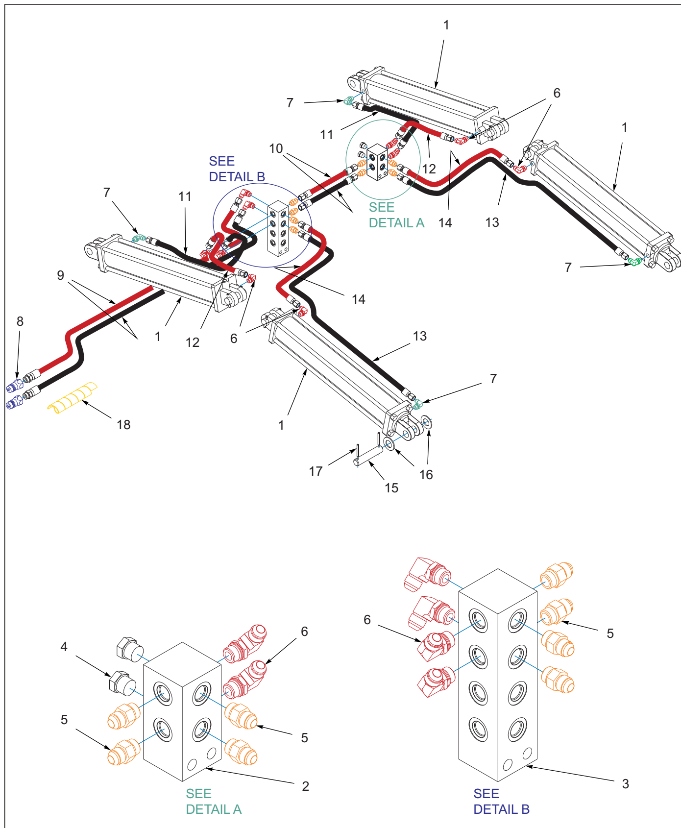
Figure 6-5: Fold Hydraulic Assembly 8530-22'-25'
