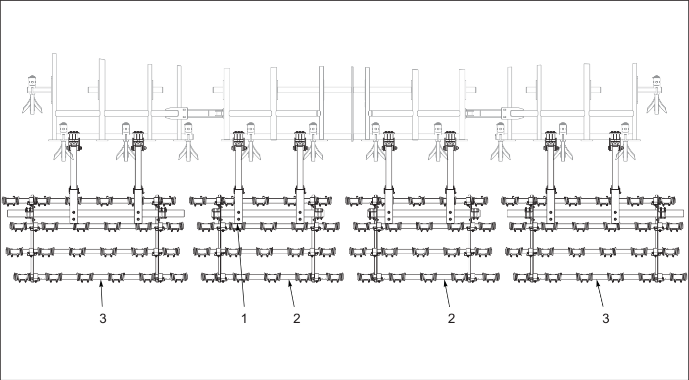
Figure 10-4: 4 Row Coil Tine Harrow Layout 8530-27'
