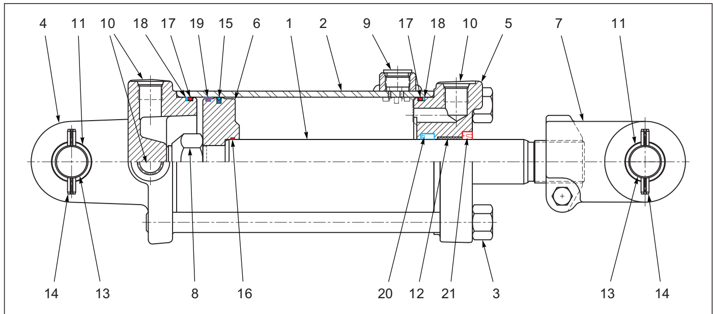
Figure 7-2: Cylinder Assembly 4 x 8, Rephase (Midway)
