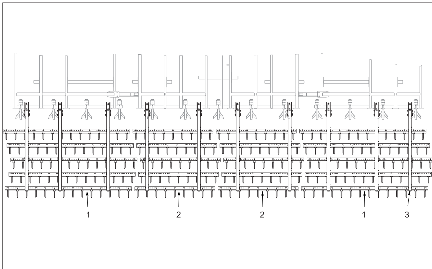
Figure 10-24: 5 Row Spike Harrow Layout 8530-33'
