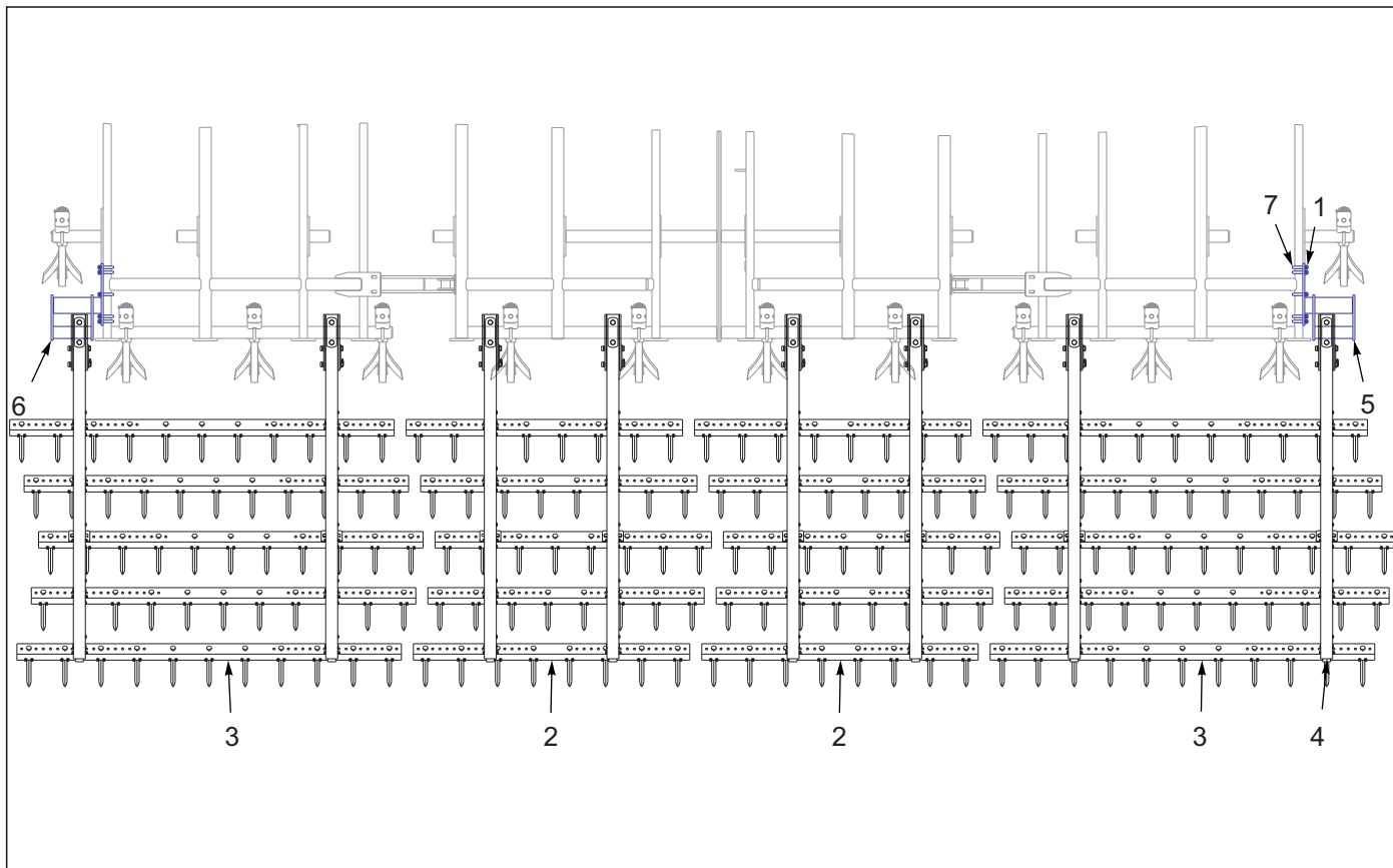
Figure 10-22: 5 Row Spike Harrow Layout 8530-27'
