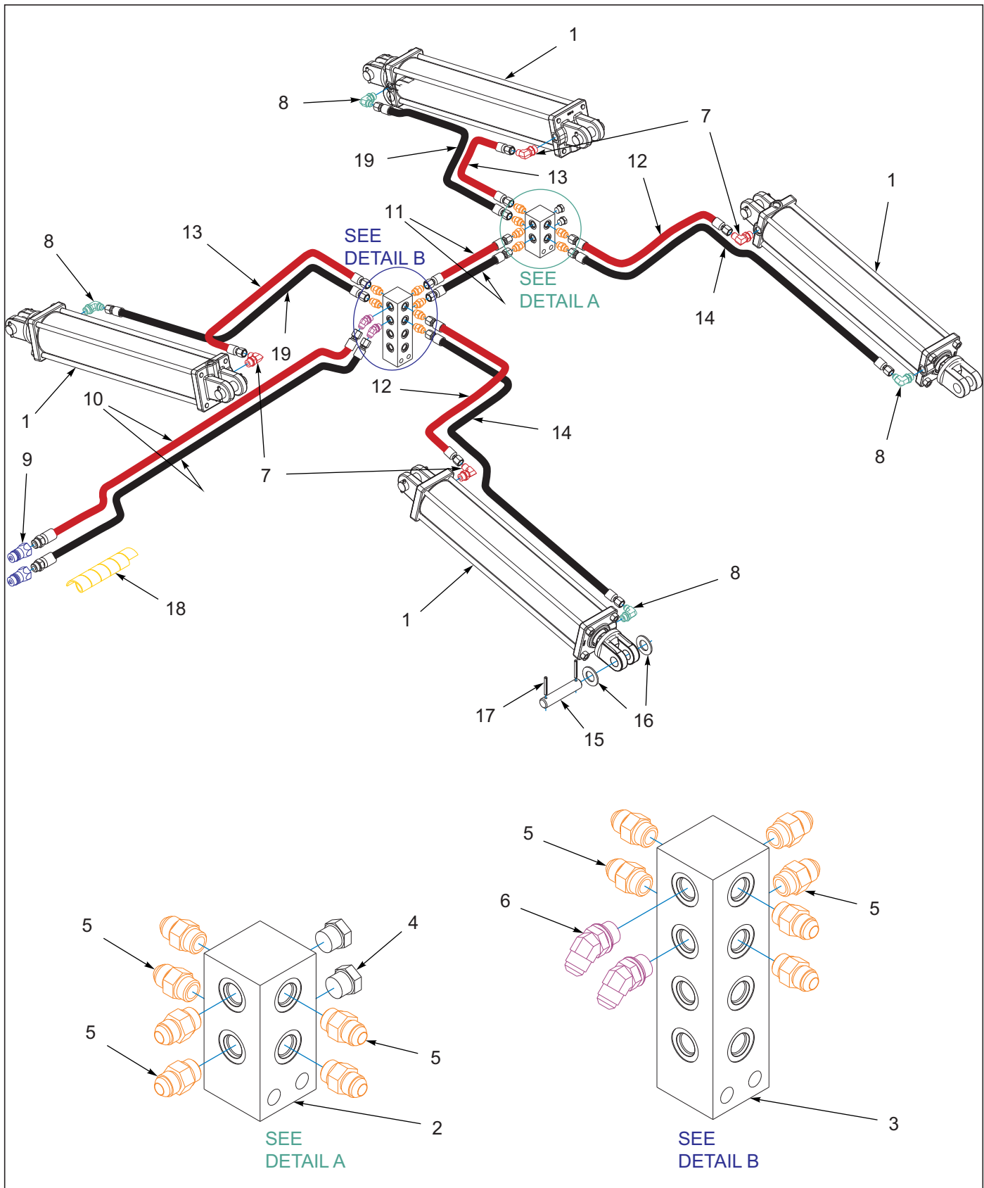
Figure 6-6: Fold Hydraulic Assembly 8530-27'-30'
