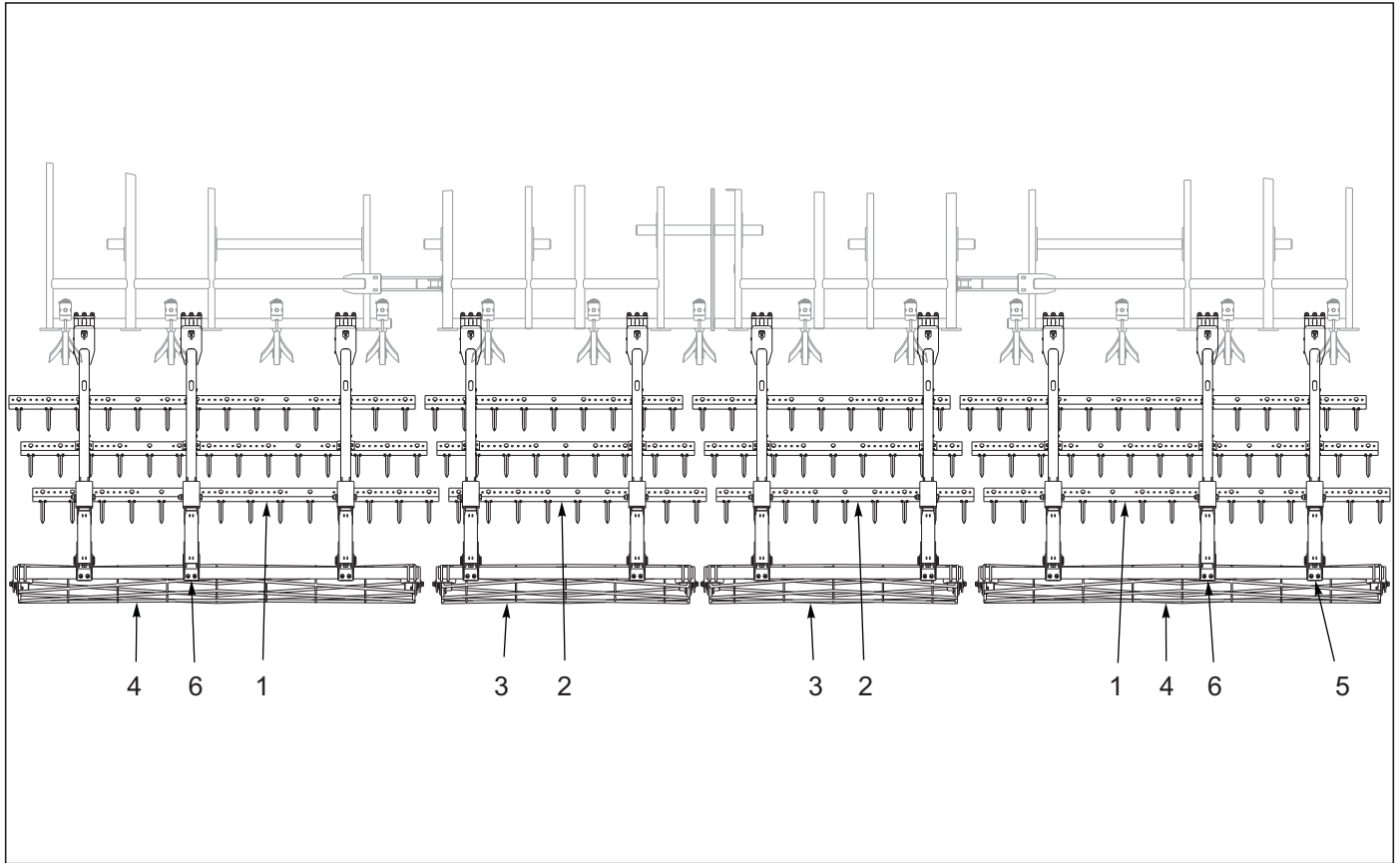
Figure 10-32: 3 Row Spike & Reel Layout 8530-33'
