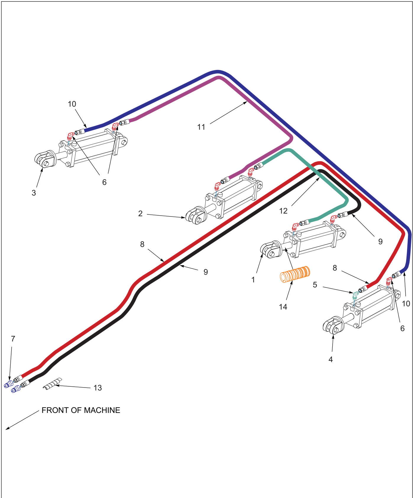
Figure 6-8: Gang Hydraulic Assembly 8530-19'-25'
