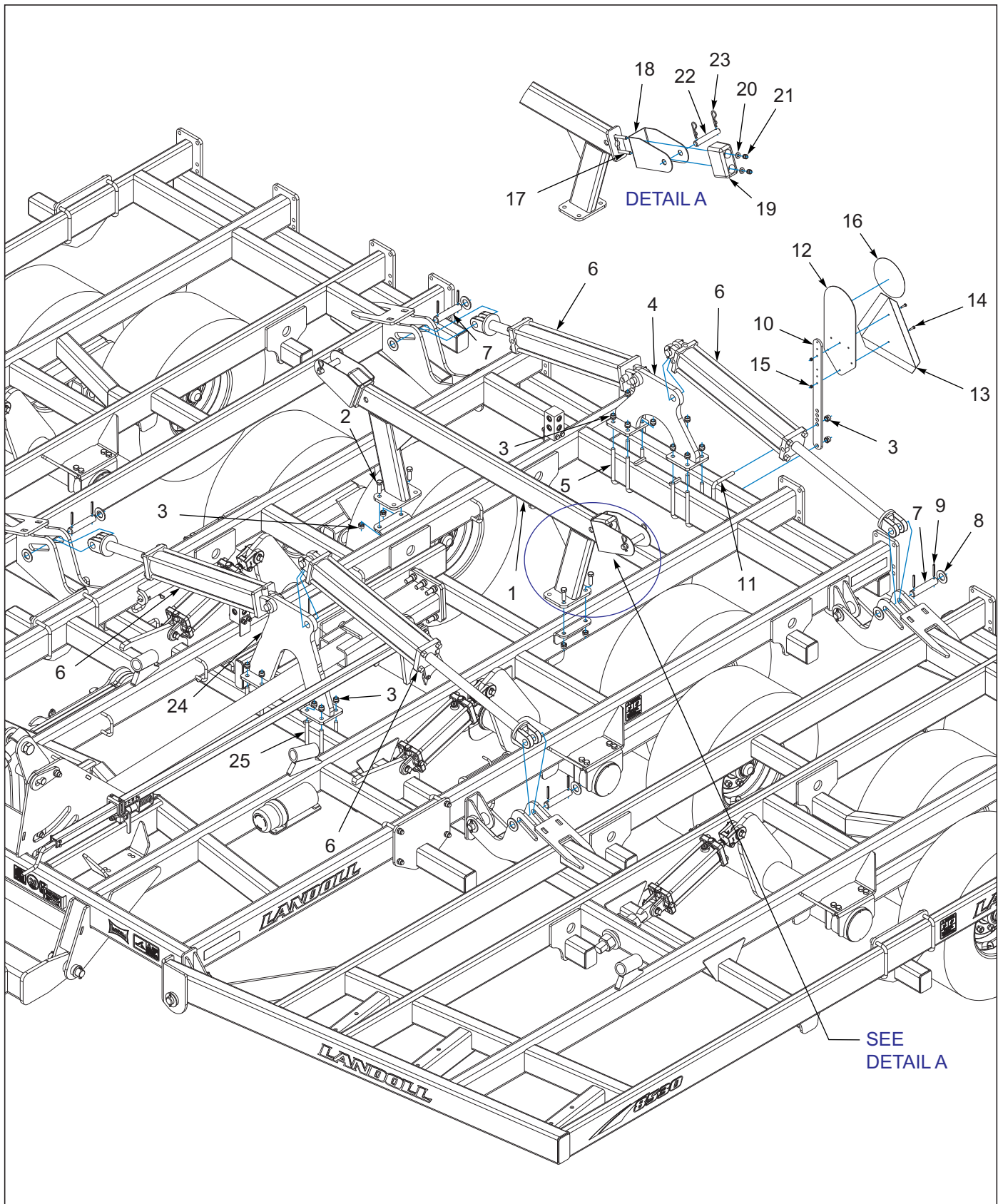
Figure 3-2: Fold Assembly 8530-22'-25'
