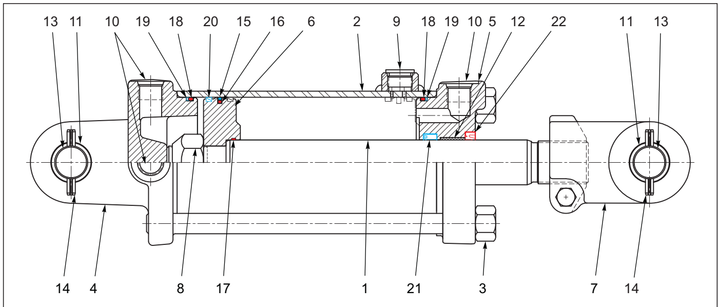
Figure 7-10: Cylinder Assembly 4 x 10, Rephase
