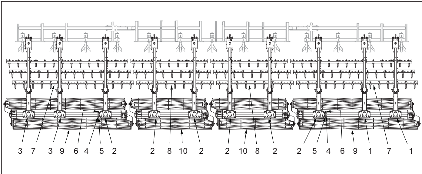
Figure 10-57: 3RS & Double Conditioner Reel Layout 8530-33'
