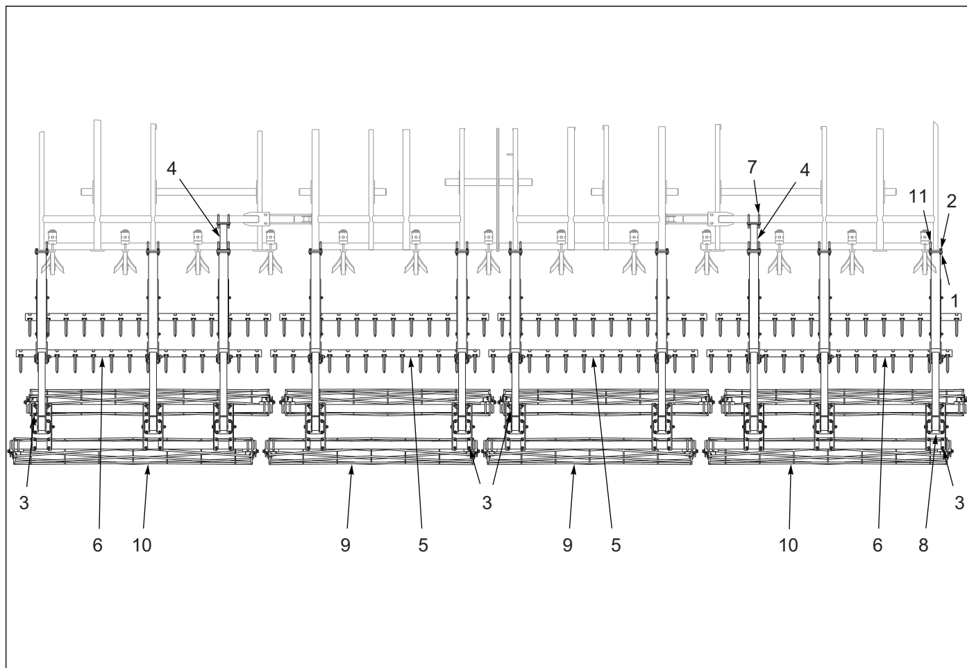
Figure 10-51: Spike & Double Reel Layout 8530-33'
