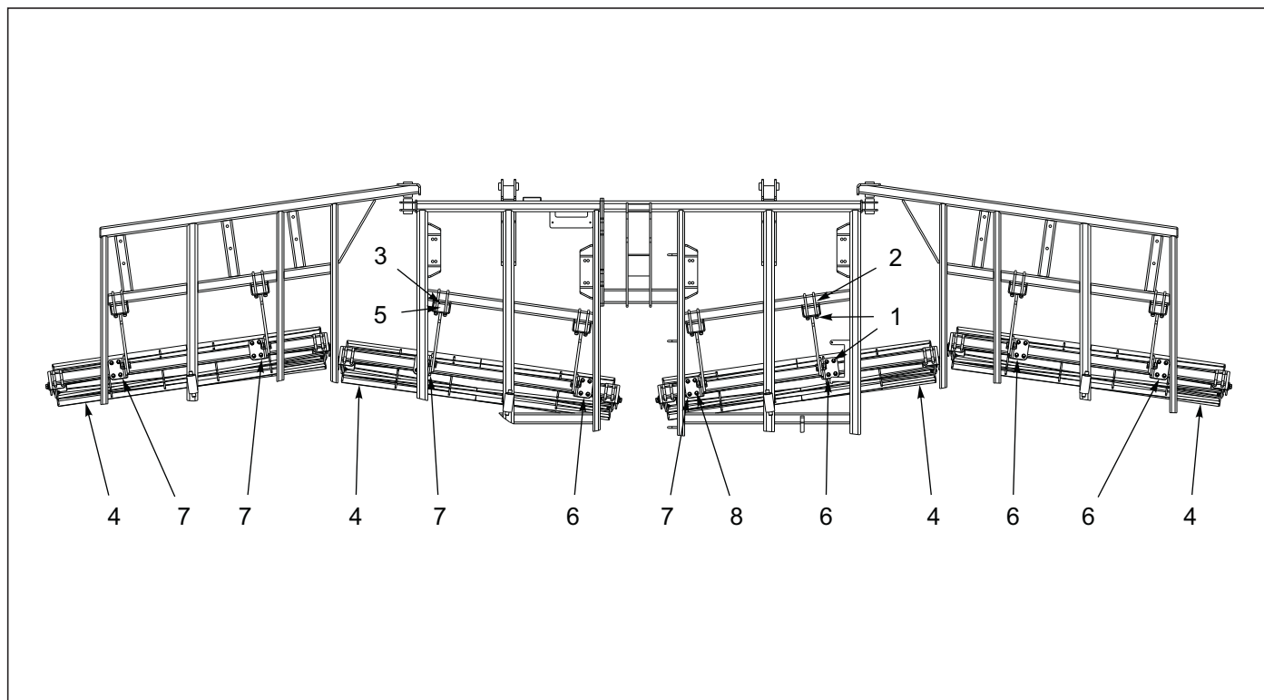
Figure 4-16: Disc Gang Reel Assembly 8530-27'
