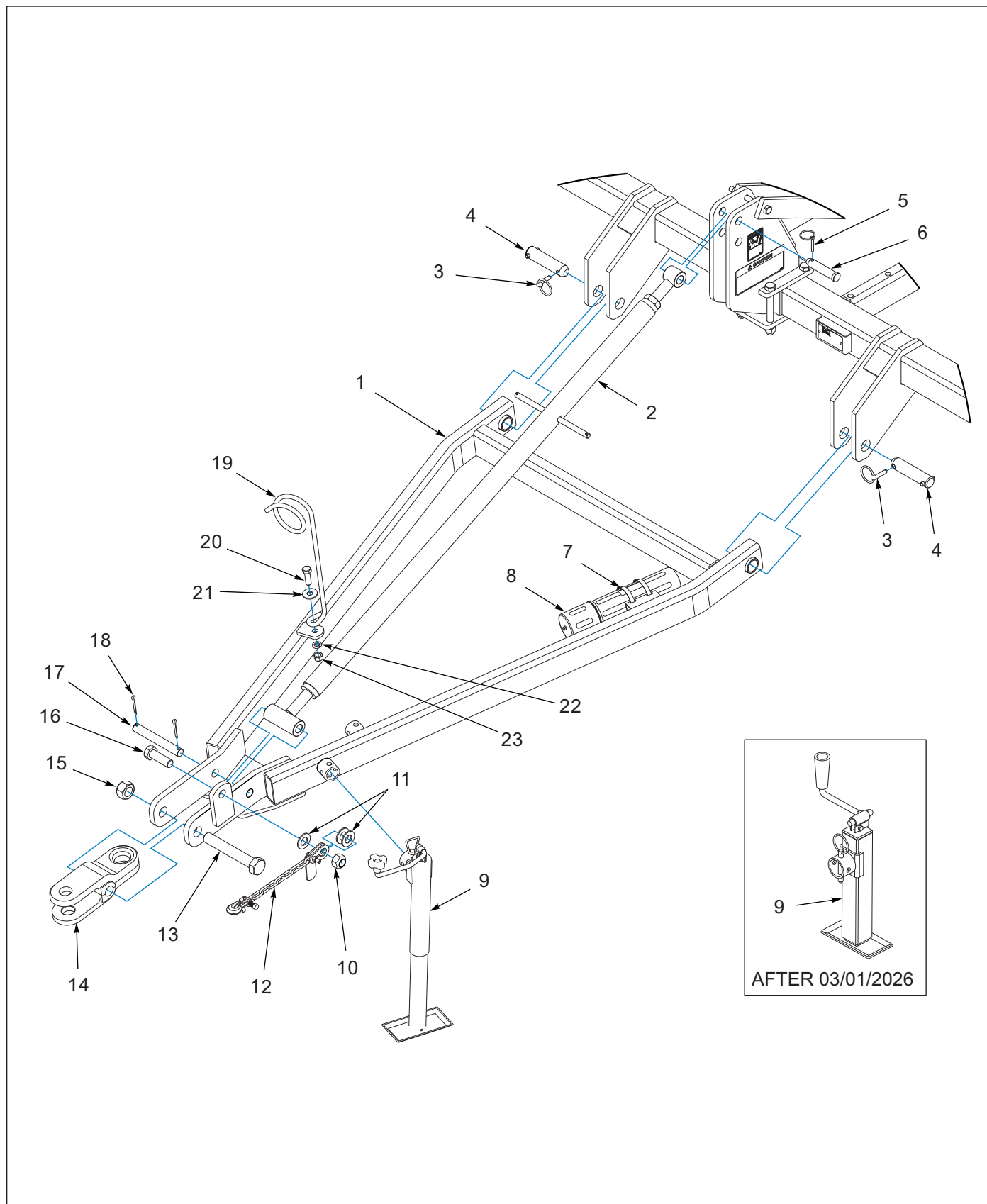
Figure 1-8: Drawbar Assembly
