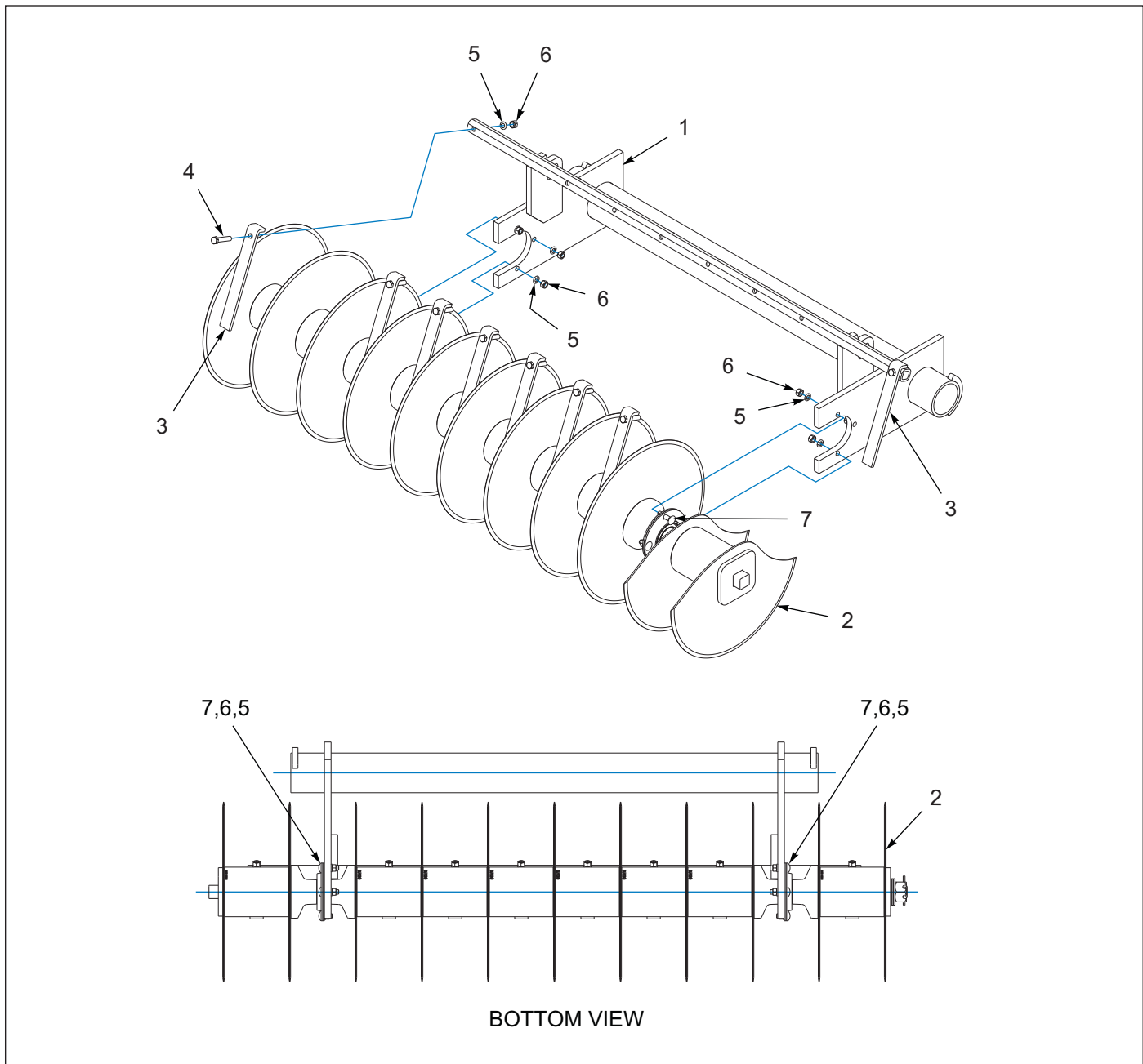
Figure 1-19: Coulter Assembly - 11 Gang
