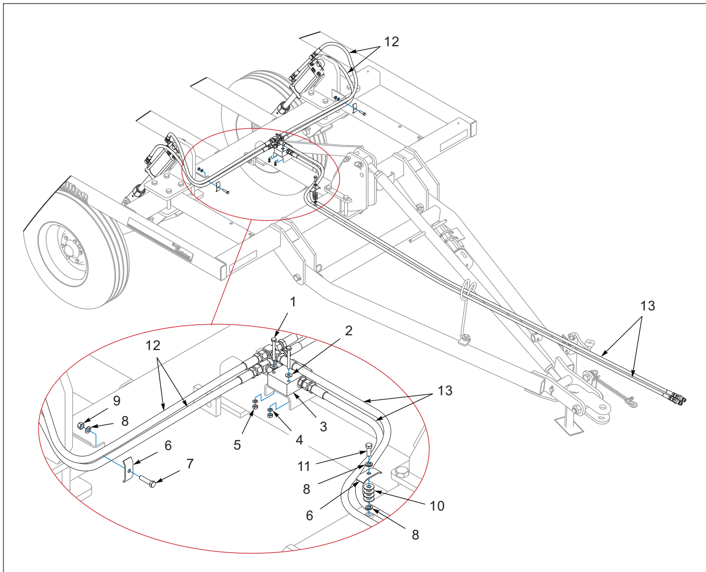
Figure 1-26: Hydraulic, Layout - 5 Shank
