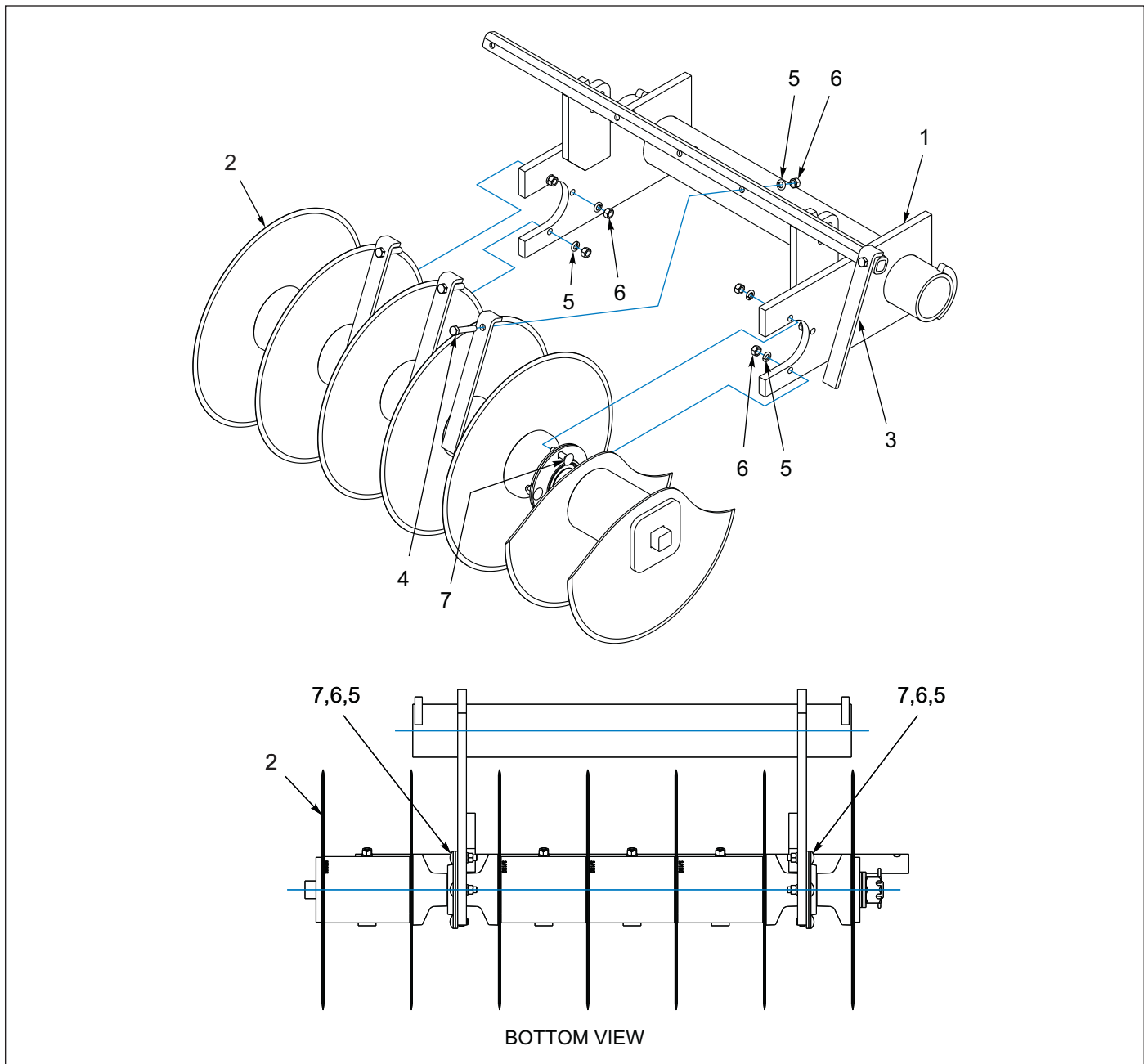
Figure 1-21: Coulter Assembly - 7 Gang
