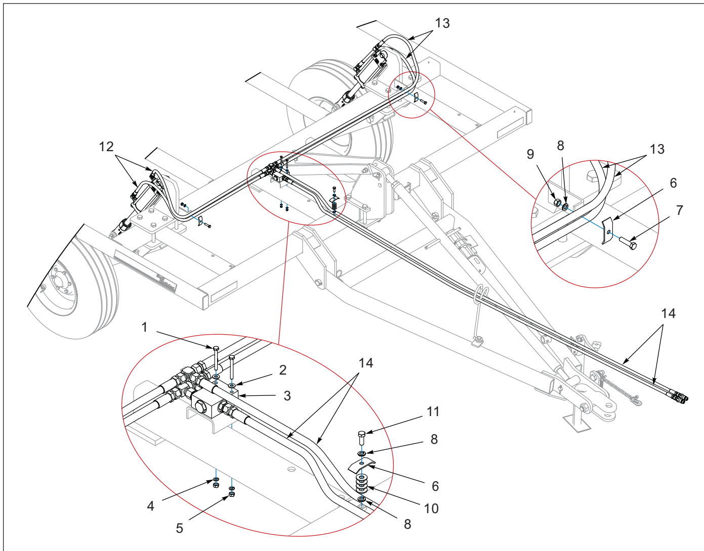
Figure 1-28: Hydraulic, Layout - 7 Shank
