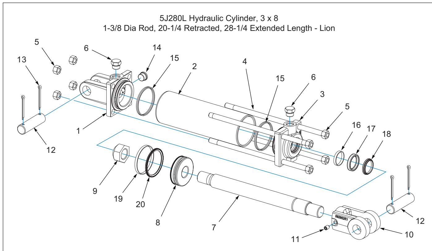
Figure 1-38: 5J280L Hydraulic Cylinder, 3 x 8 - Lion
