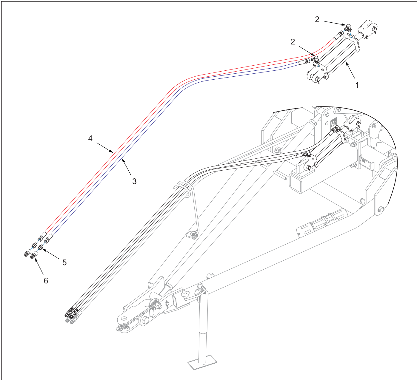
Figure 1-29: Hydraulic, Coulter Schematic/Layout - 7 Shank
