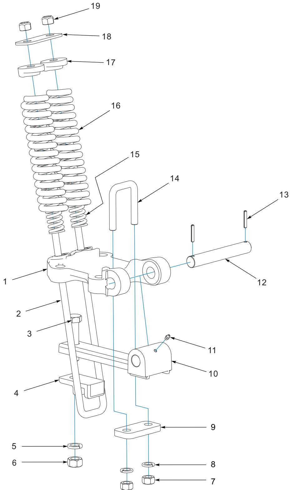
Figure 1-11: Spring Clamp Assembly
