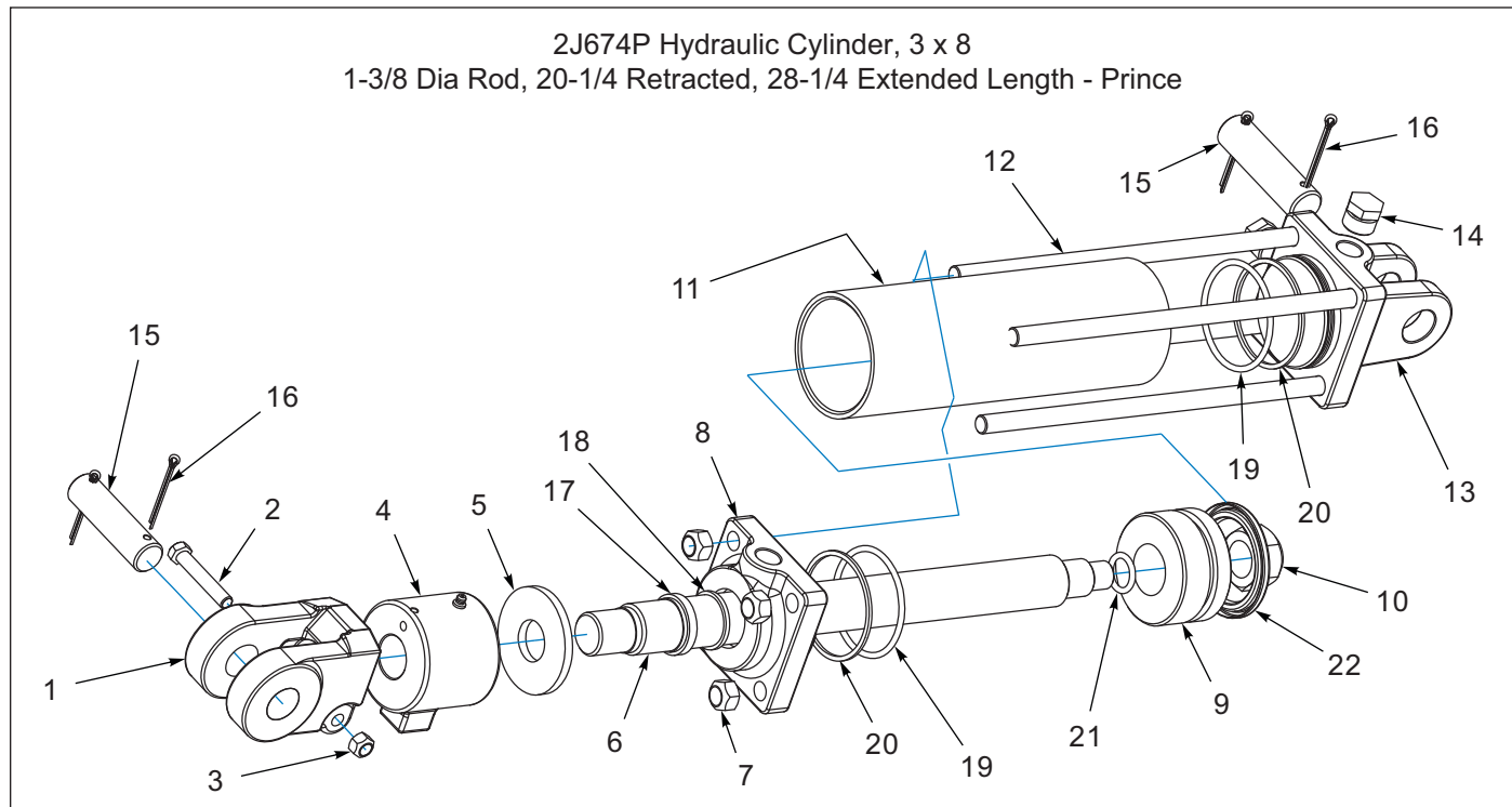
Figure 1-34: 2J674P Hydraulic Cylinder, 3 x 8 - Prince
