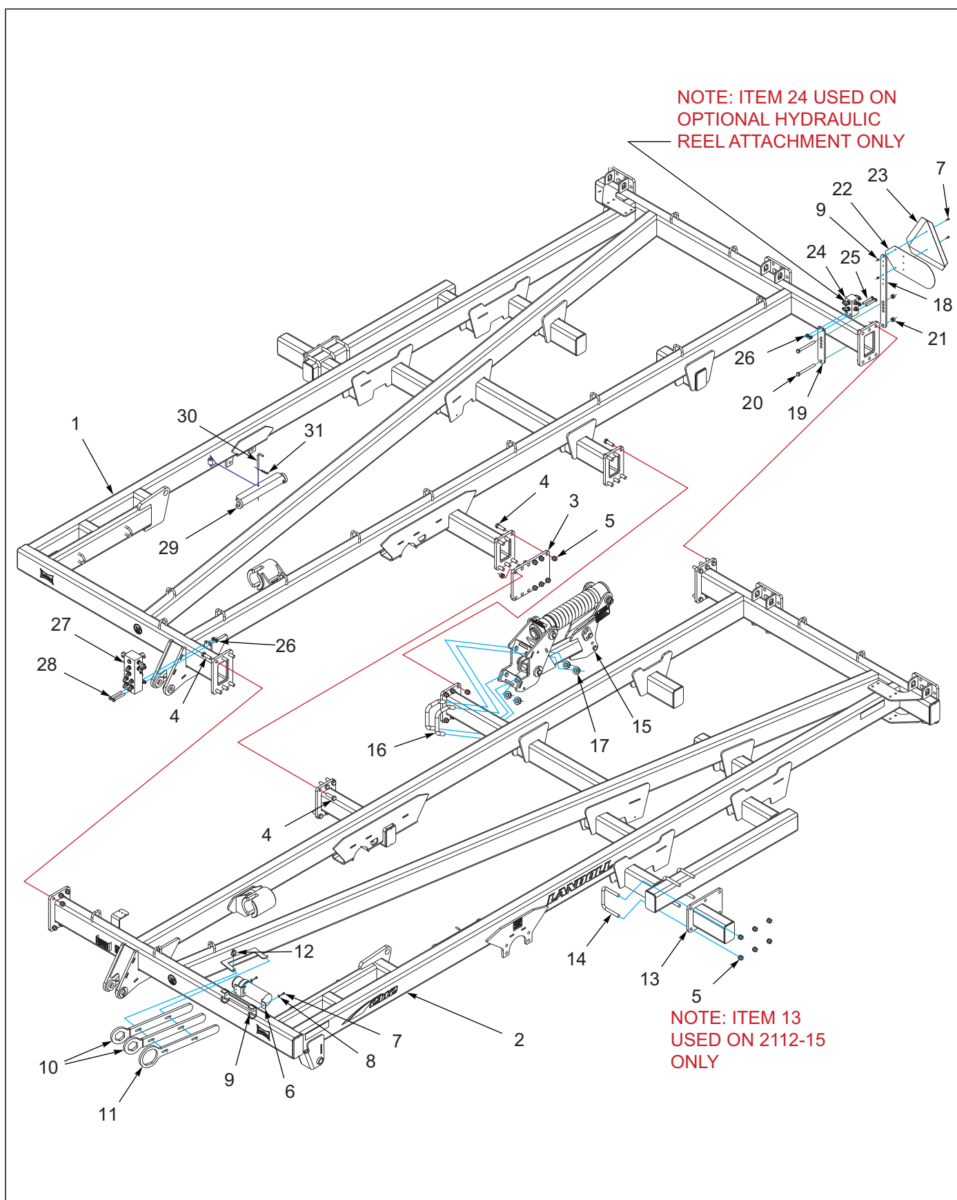
Figure 1-3: Center Frame Assembly 2112-13-15
