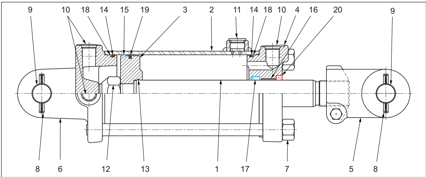
Figure 1-33: Cylinder Assembly 3-1/2 x 8 Rephase (Prince)
