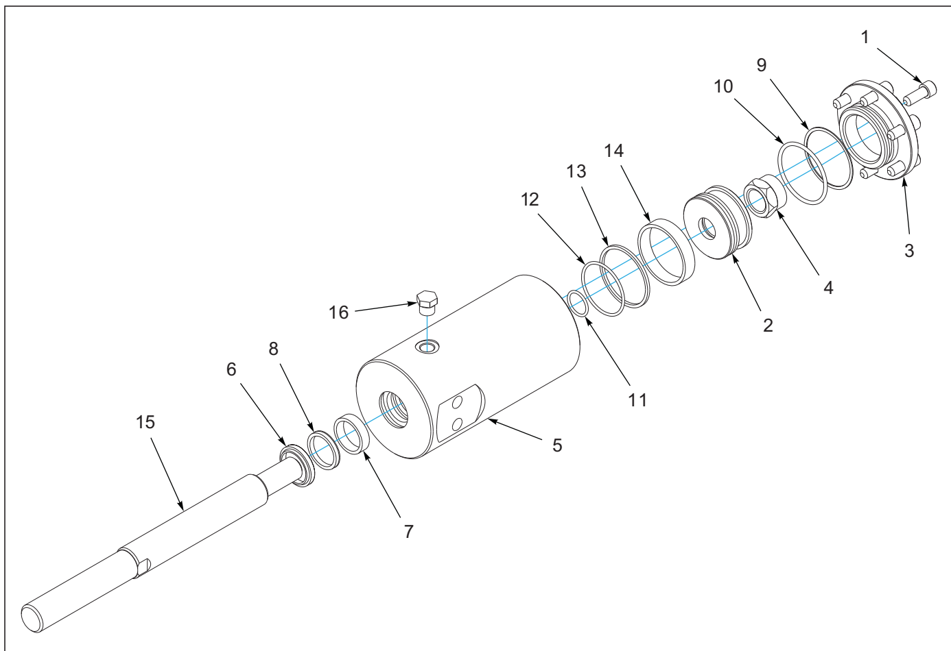
Figure 1-35: Cylinder - 2-1/2" X 3-1/2"
