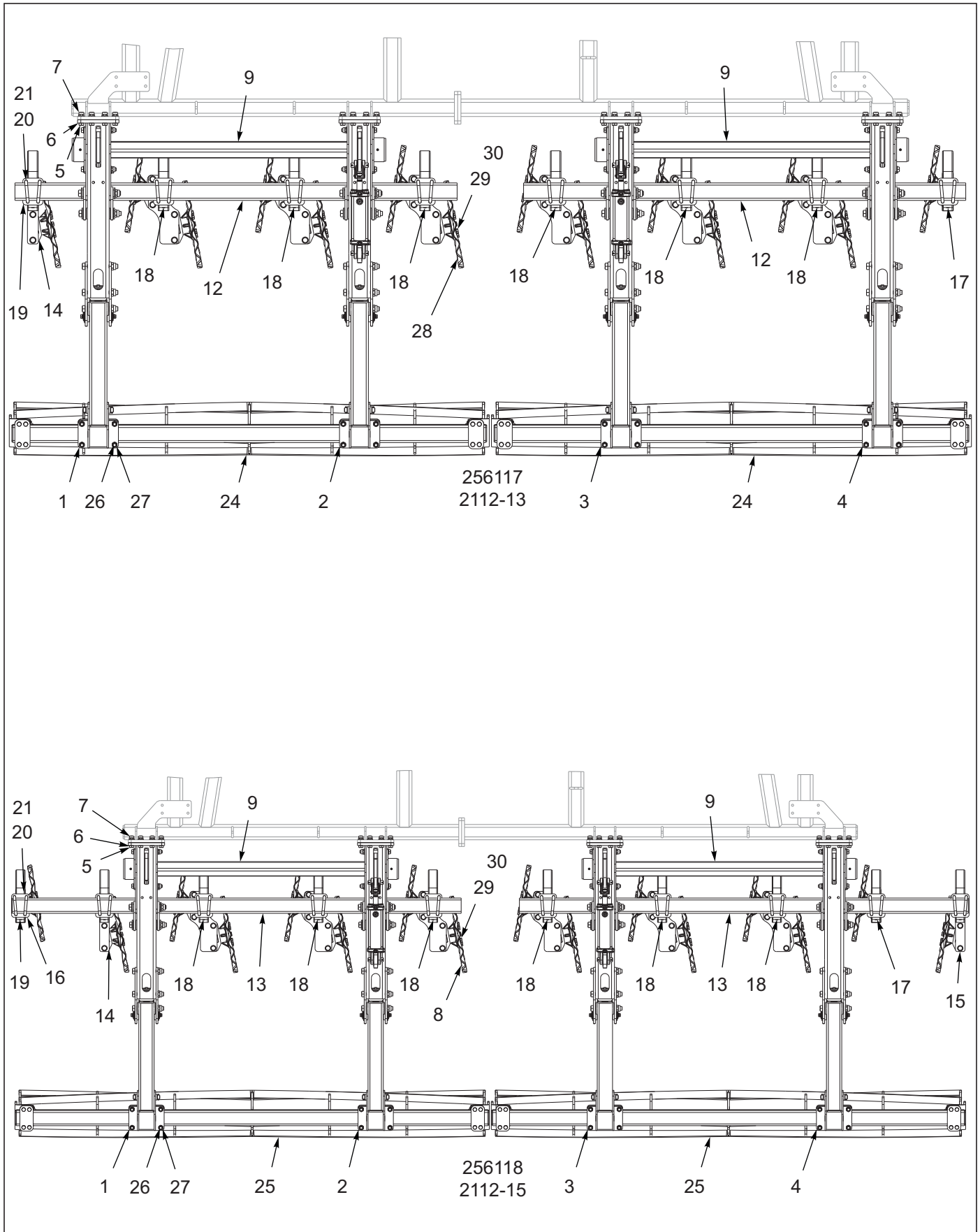
Figure 1-64: Hyd Lev/Reel Layout (2 of 2)
