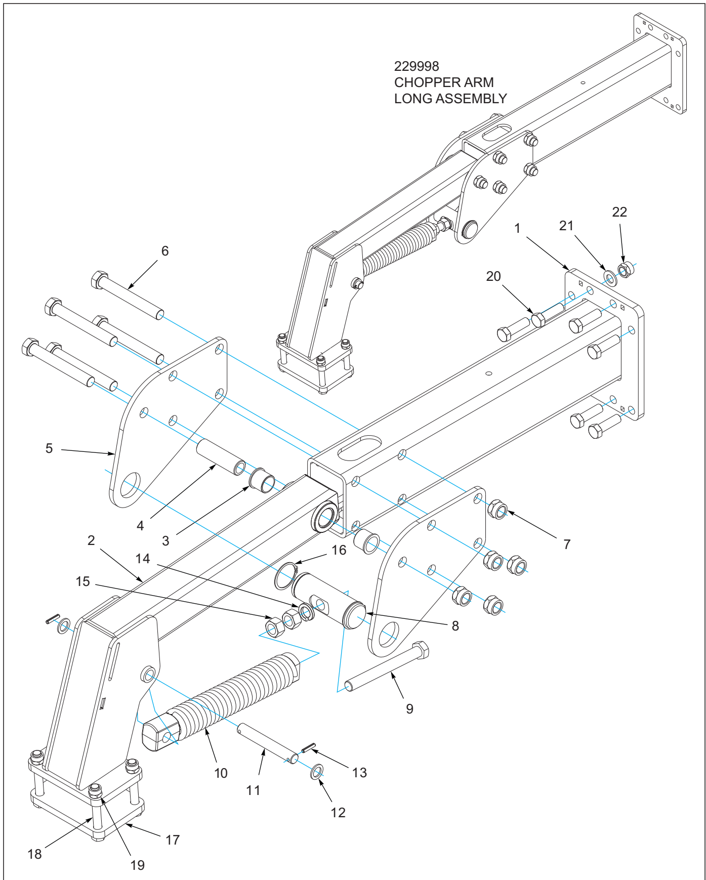
Figure 1-53: Std Chopper Arm Long Assembly
