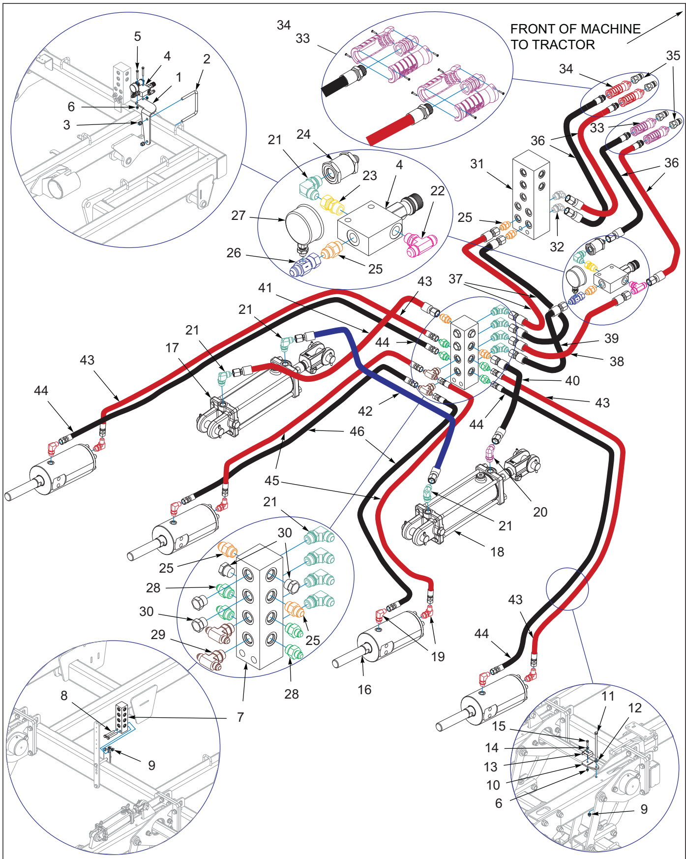
Figure 1-71: Disc Lev/Reel Hydraulic Assembly
