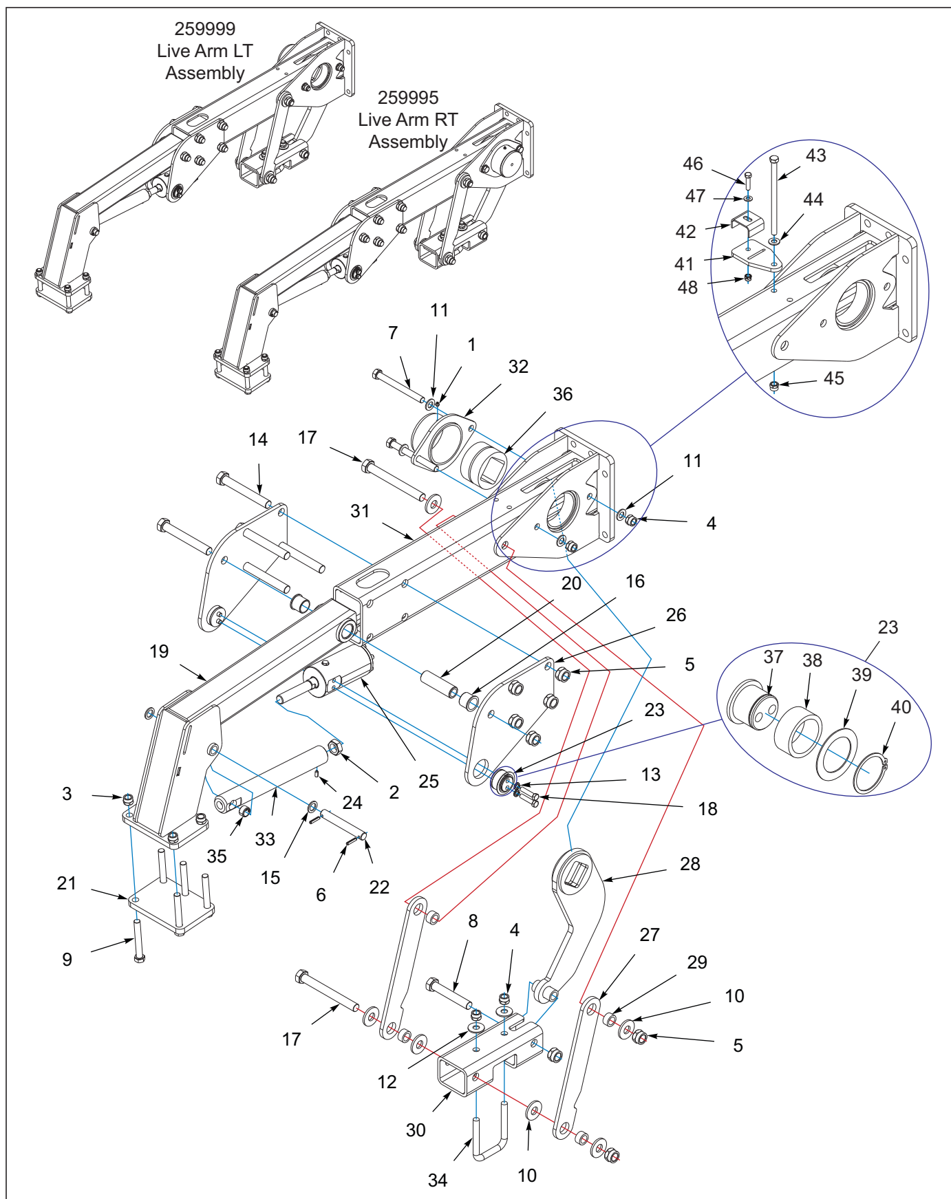
Figure 1-66: Live Arm No Hyd Assembly
