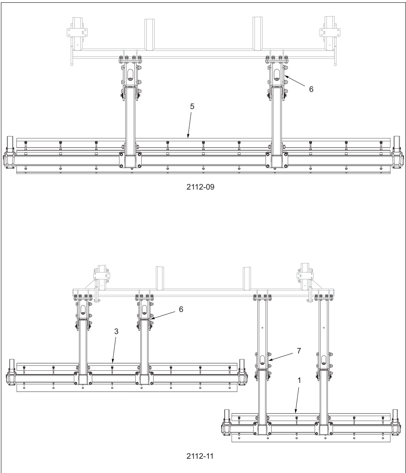
Figure 1-55: Hyd Chopper Reel Layout (1 of 2)
