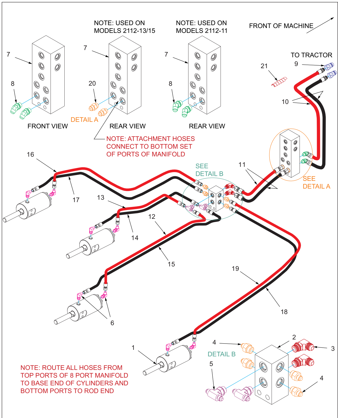
Figure 1-50: 3BCT/Chopper Hydraulic Assembly 2112-11-13-15
