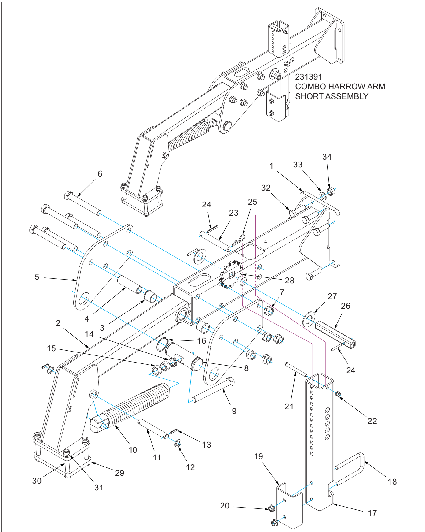
Figure 1-43: Std Combo Harrow Arm Short Assembly
