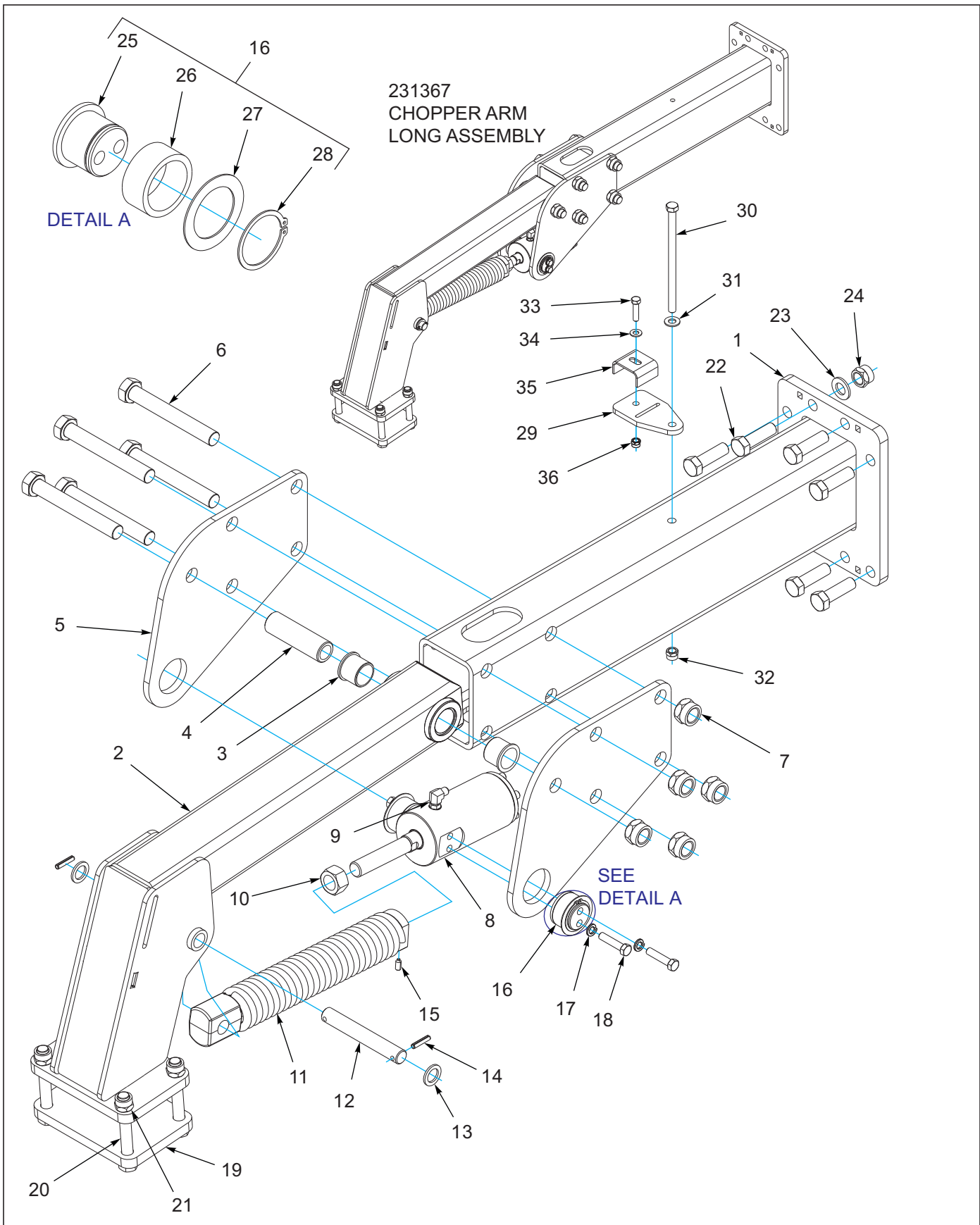
Figure 1-57: Hyd Chopper Arm Long Assembly
