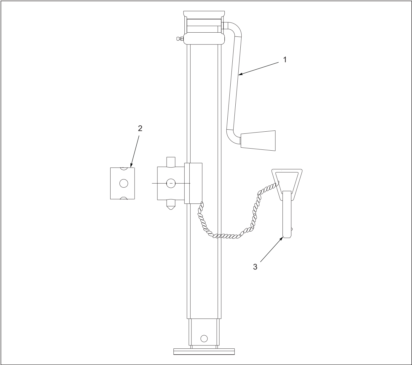
Figure 1-10: 7,000 Lb. Sidewind Jack Assembly
