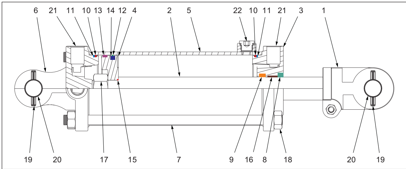
Figure 1-29: Cylinder Assembly 4 x 8 Rephase (Midway)
