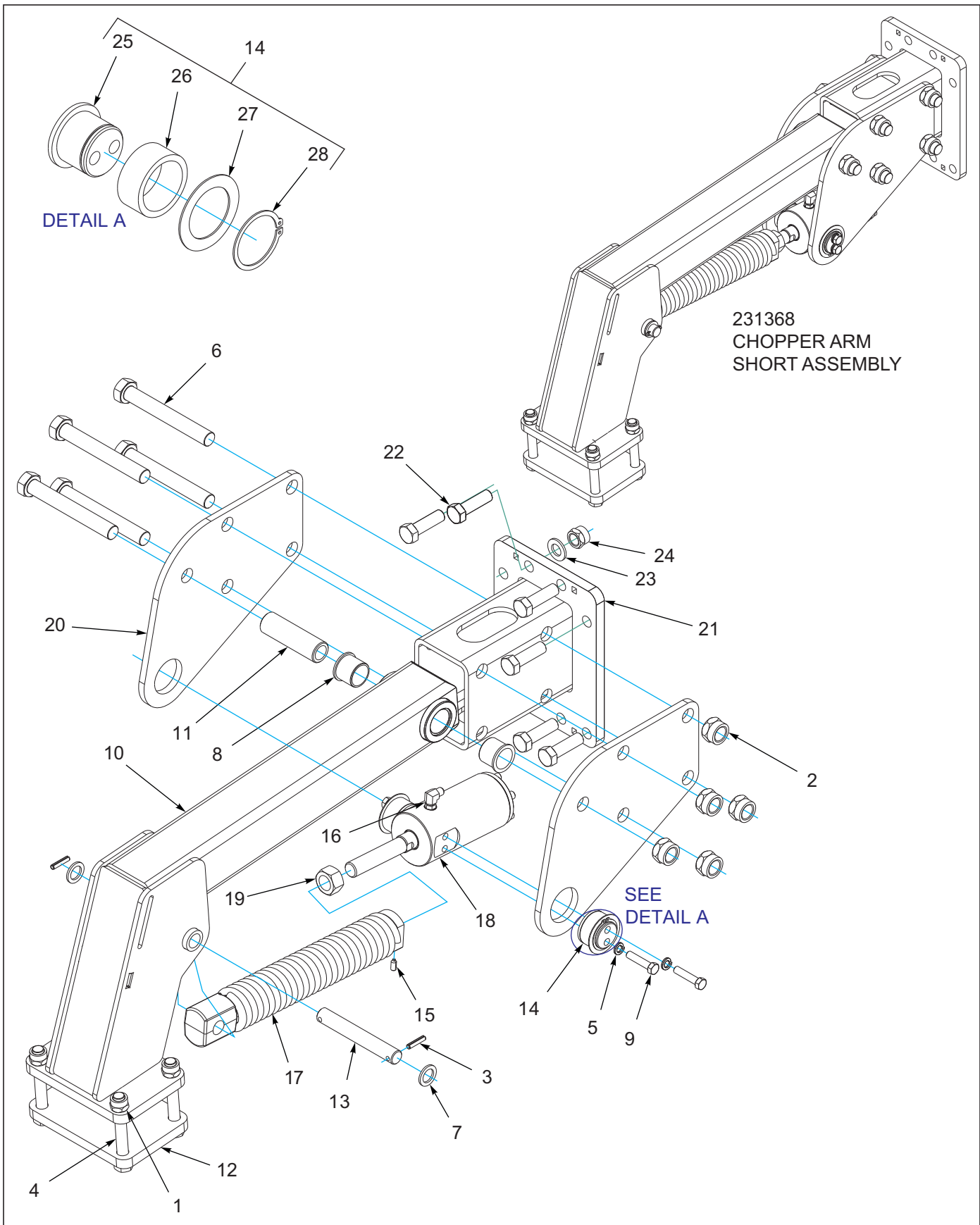
Figure 1-58: Hyd Chopper Arm Short Assembly
