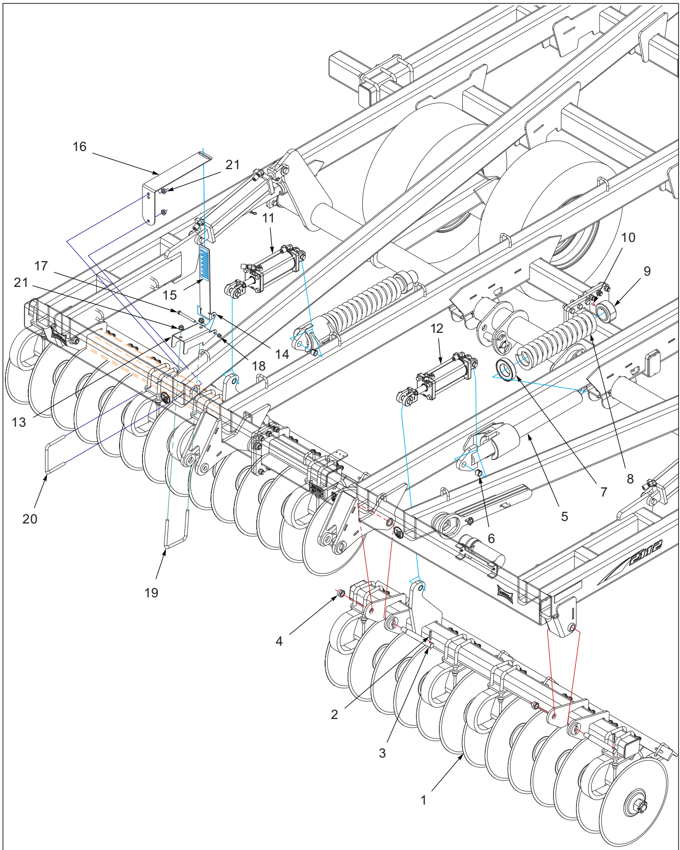
Figure 1-17: Coulter Gang To Frame Assembly
