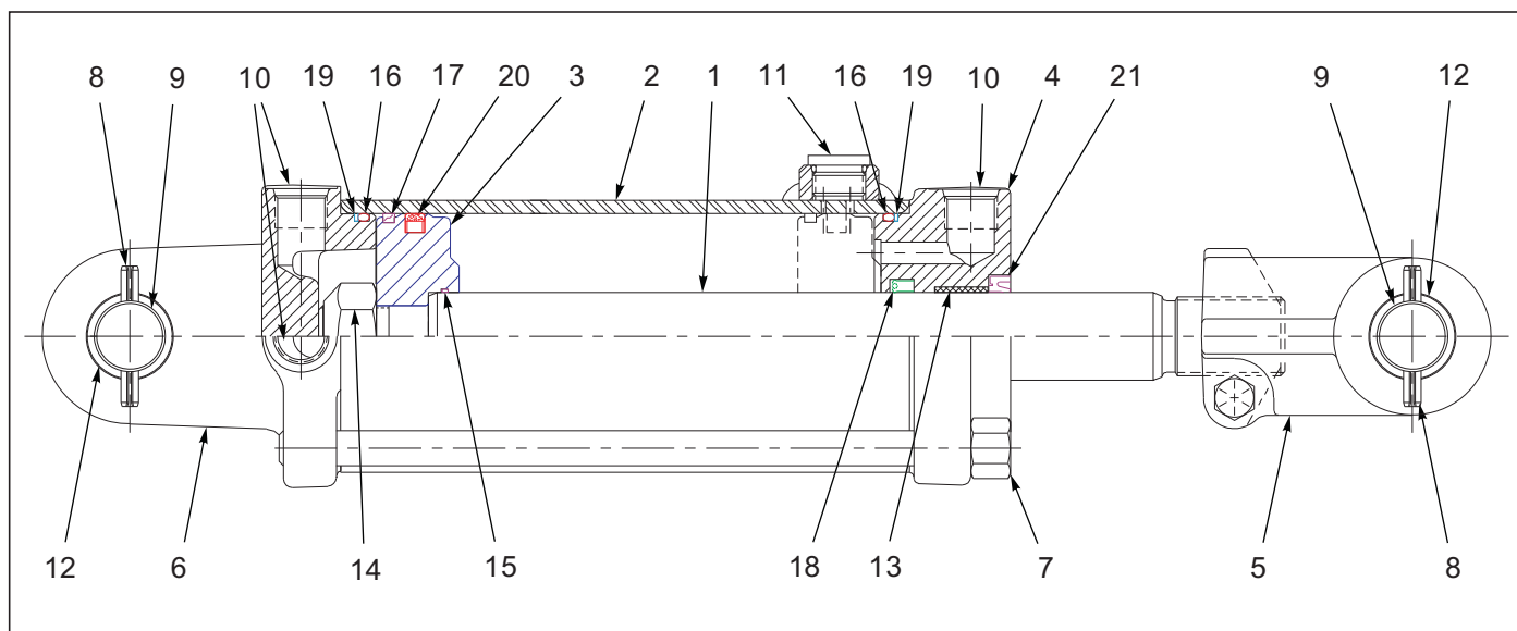
Figure 1-28: Cylinder Assembly 4 x 8 Rephase (Prince)
