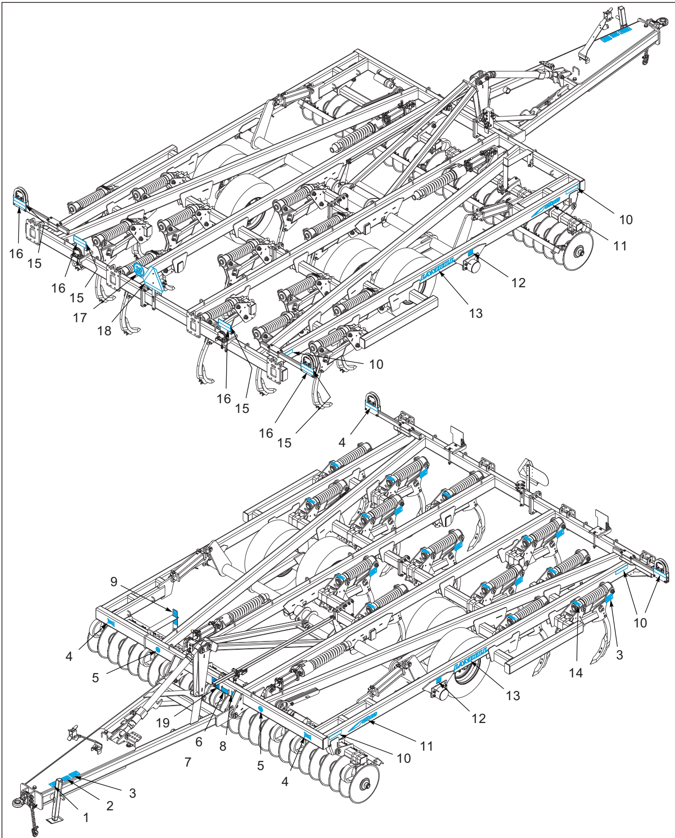
Figure 1-39: Decal Locations( 2 of 2)
