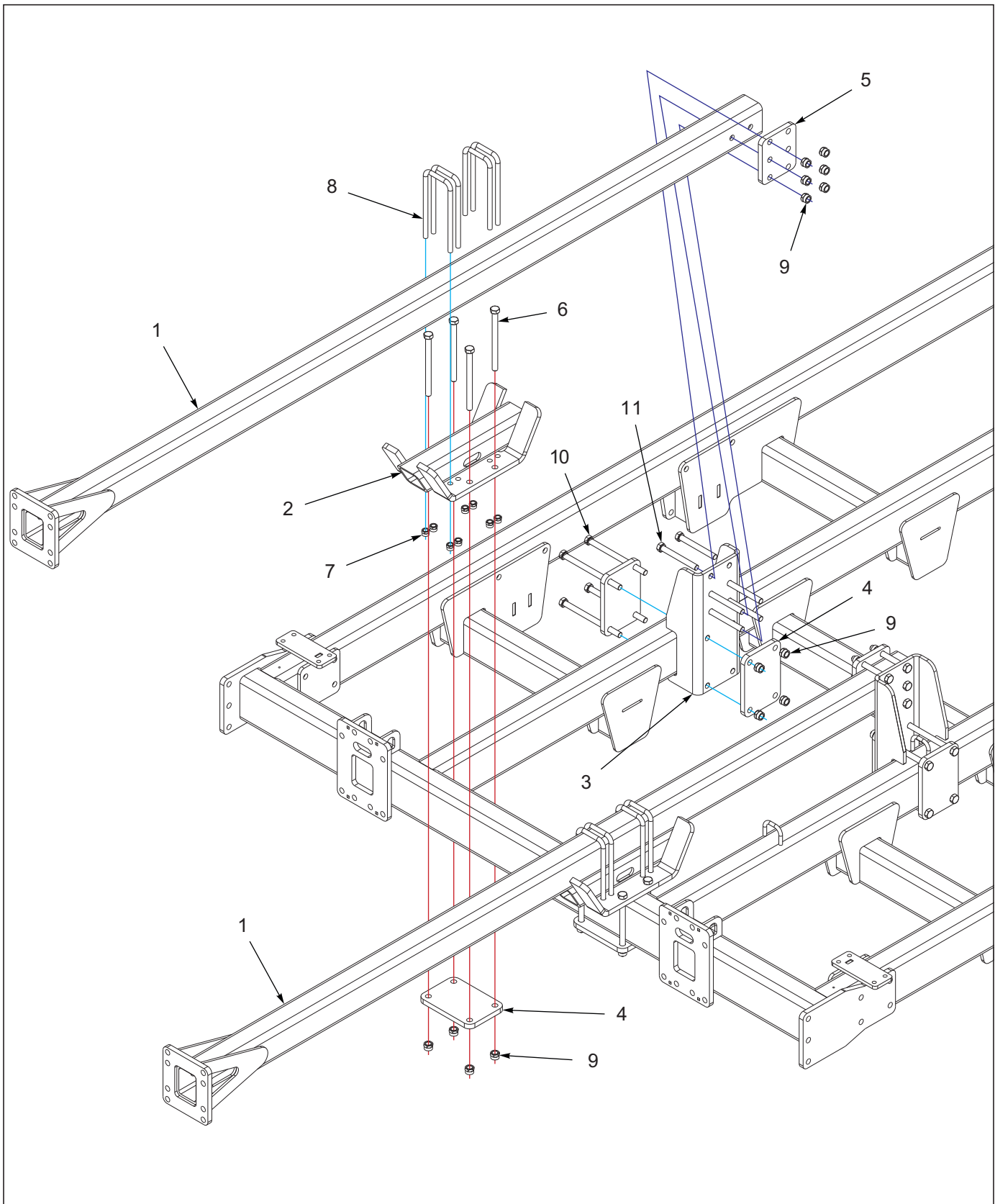
Figure 1-72: Rear Tow Hitch Assembly (1 of 2)
