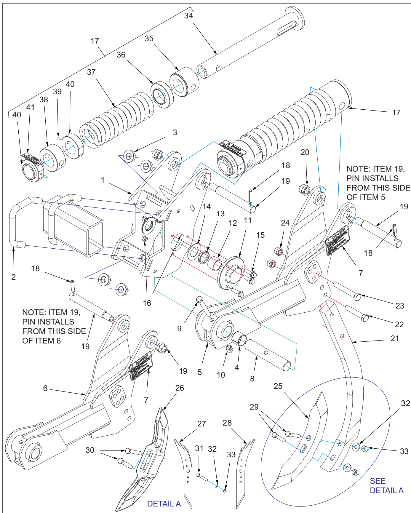
Figure 1-14: Auto Reset Clamp Assembly After 12-01-2023
