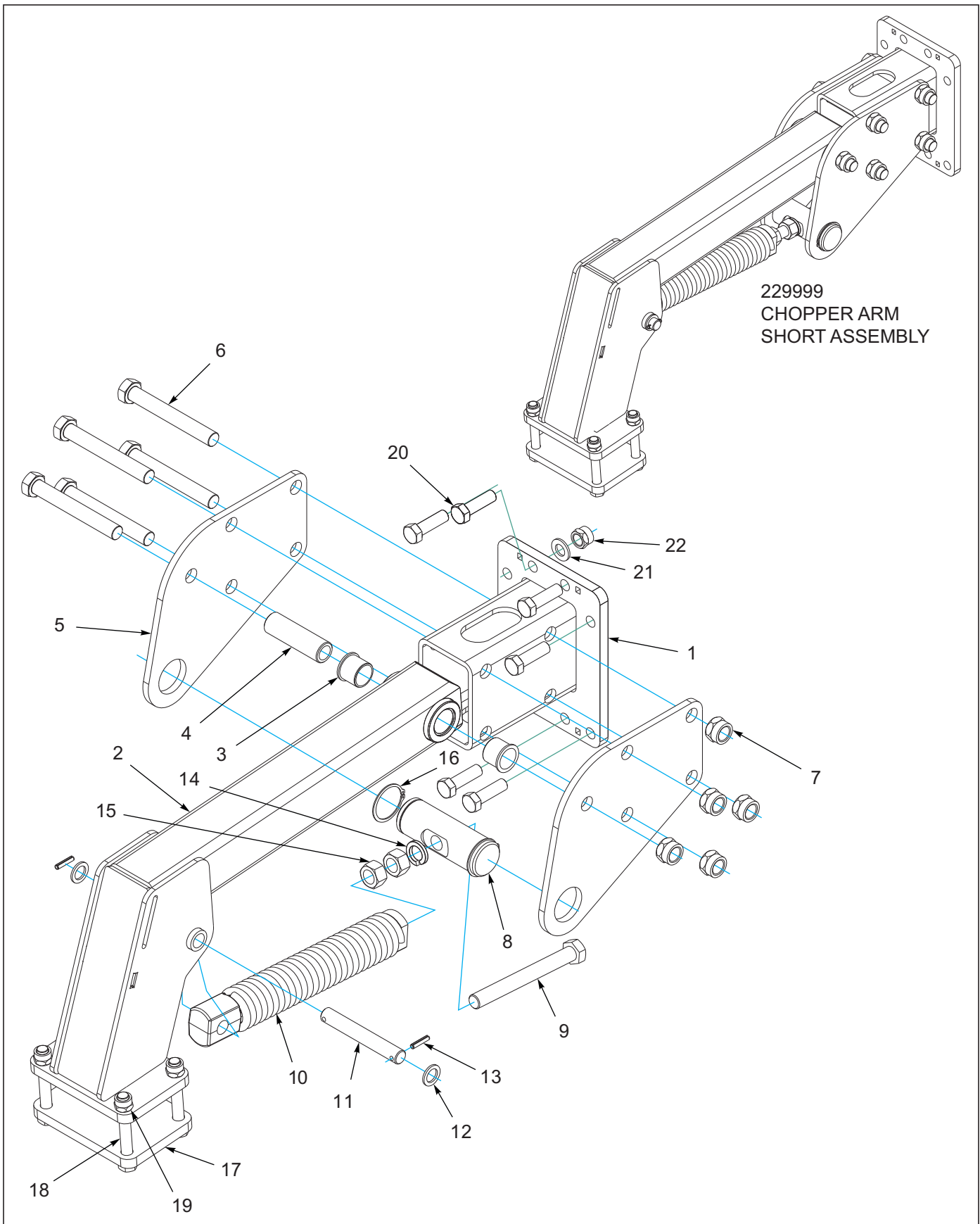
Figure 1-54: Std Chopper Arm Short Assembly
