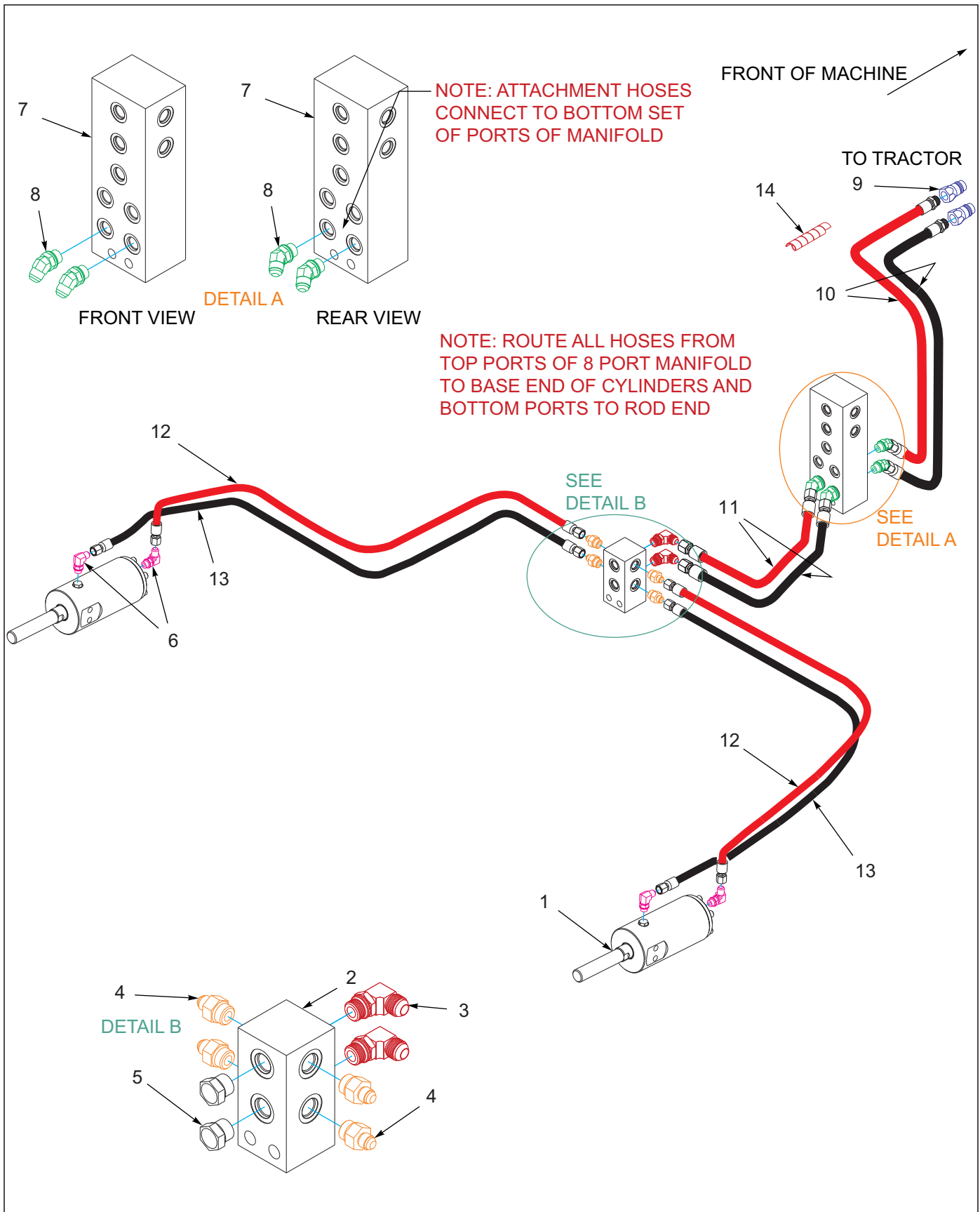
Figure 1-61: Chopper Reel Hydraulic Assembly 2112-09
