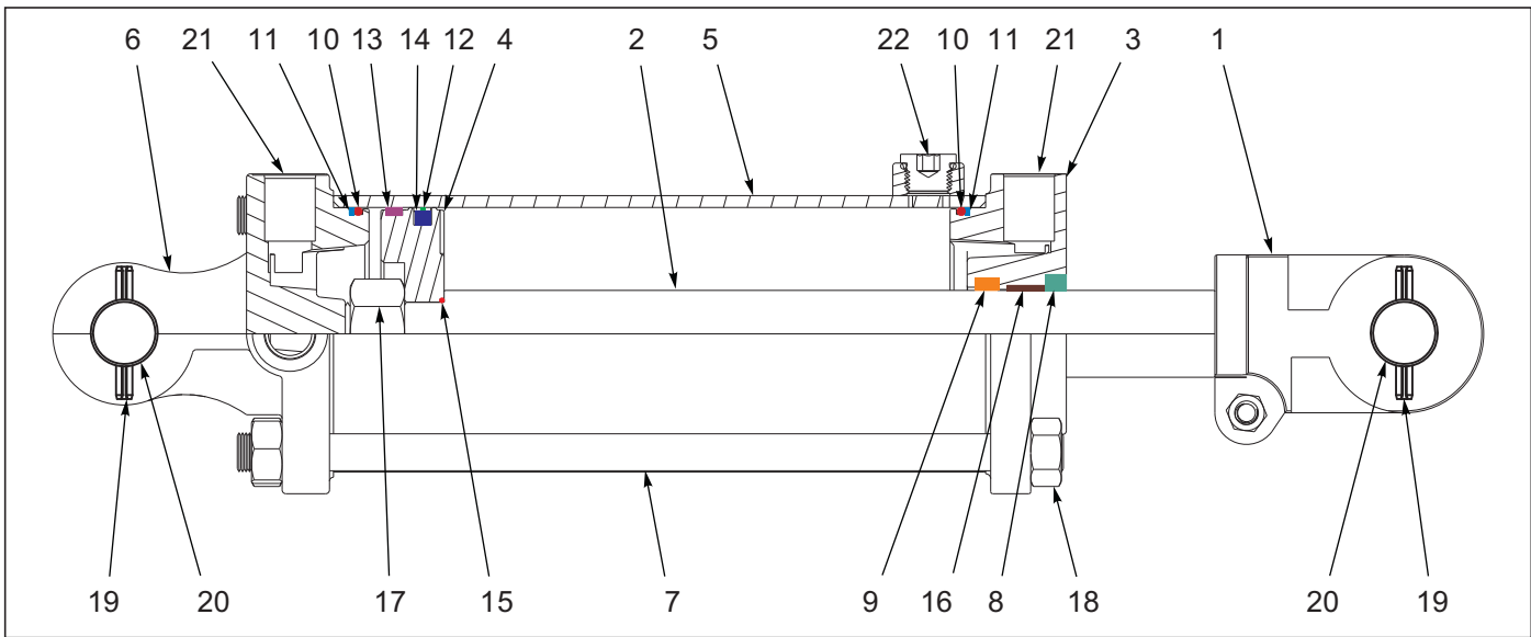
Figure 1-25: Cylinder Assembly 3-3/4 x 8 Rephase (Midway)
