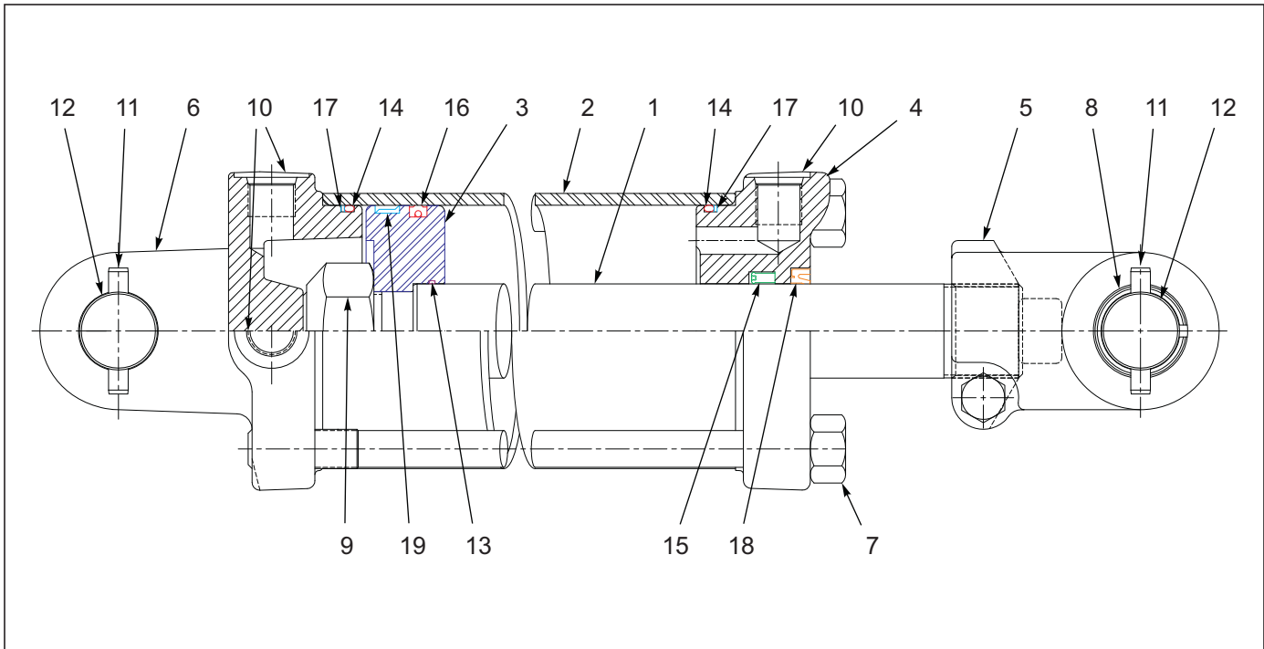
Figure 1-22: Cylinder Assembly - 4 X 16
