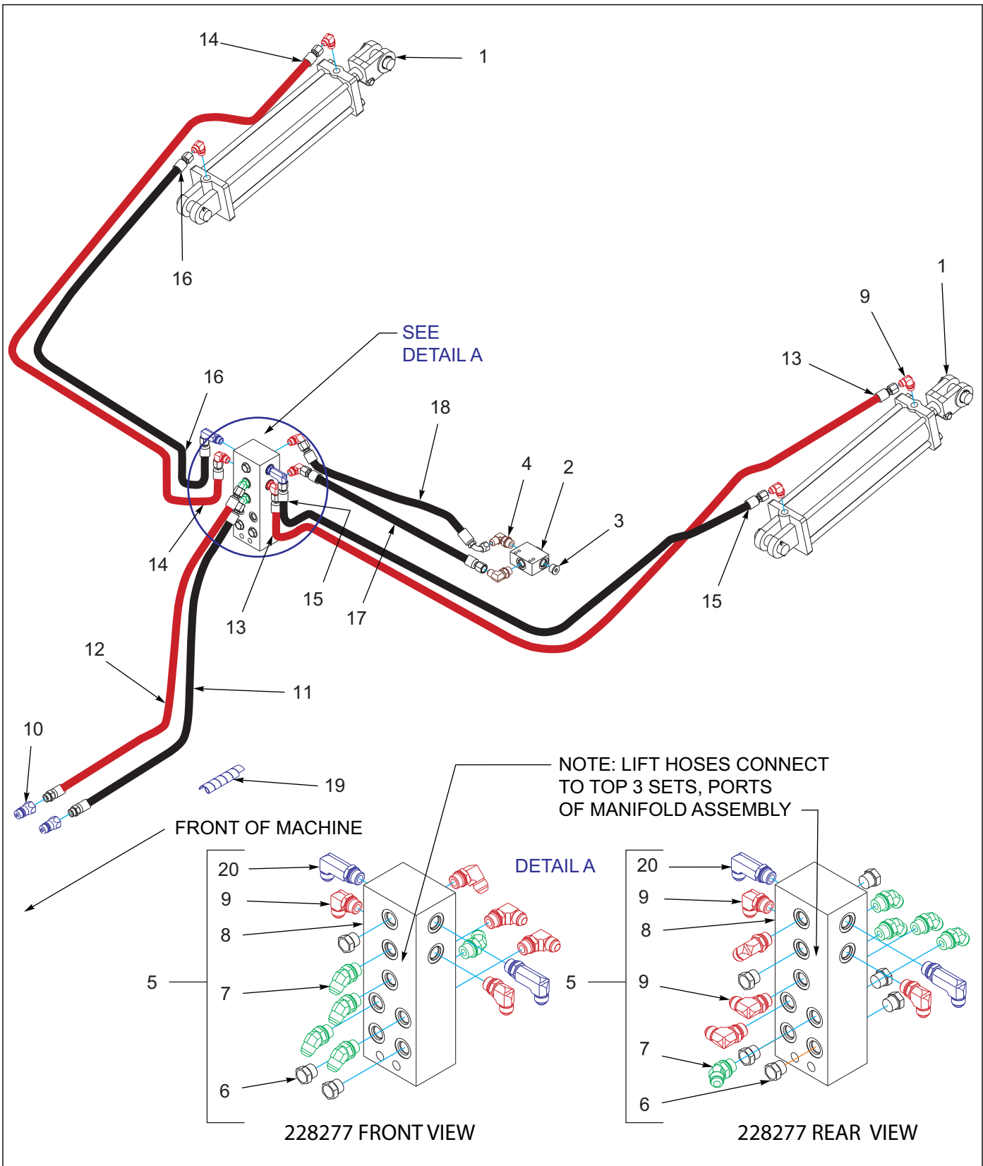
Figure 1-19: Lift Hydraulic Assembly
