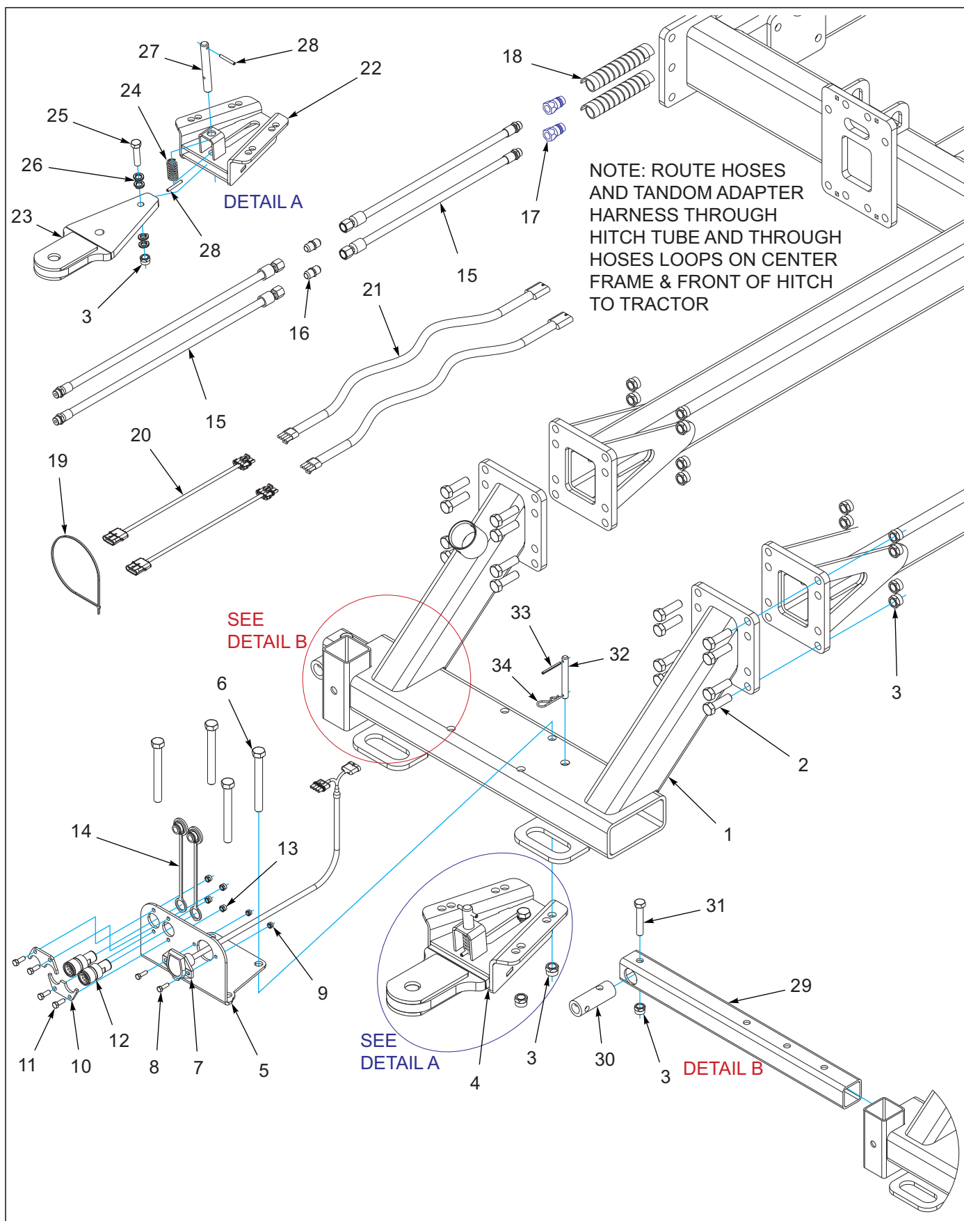
Figure 1-73: Rear Tow Hitch Assembly (2 of 2)
