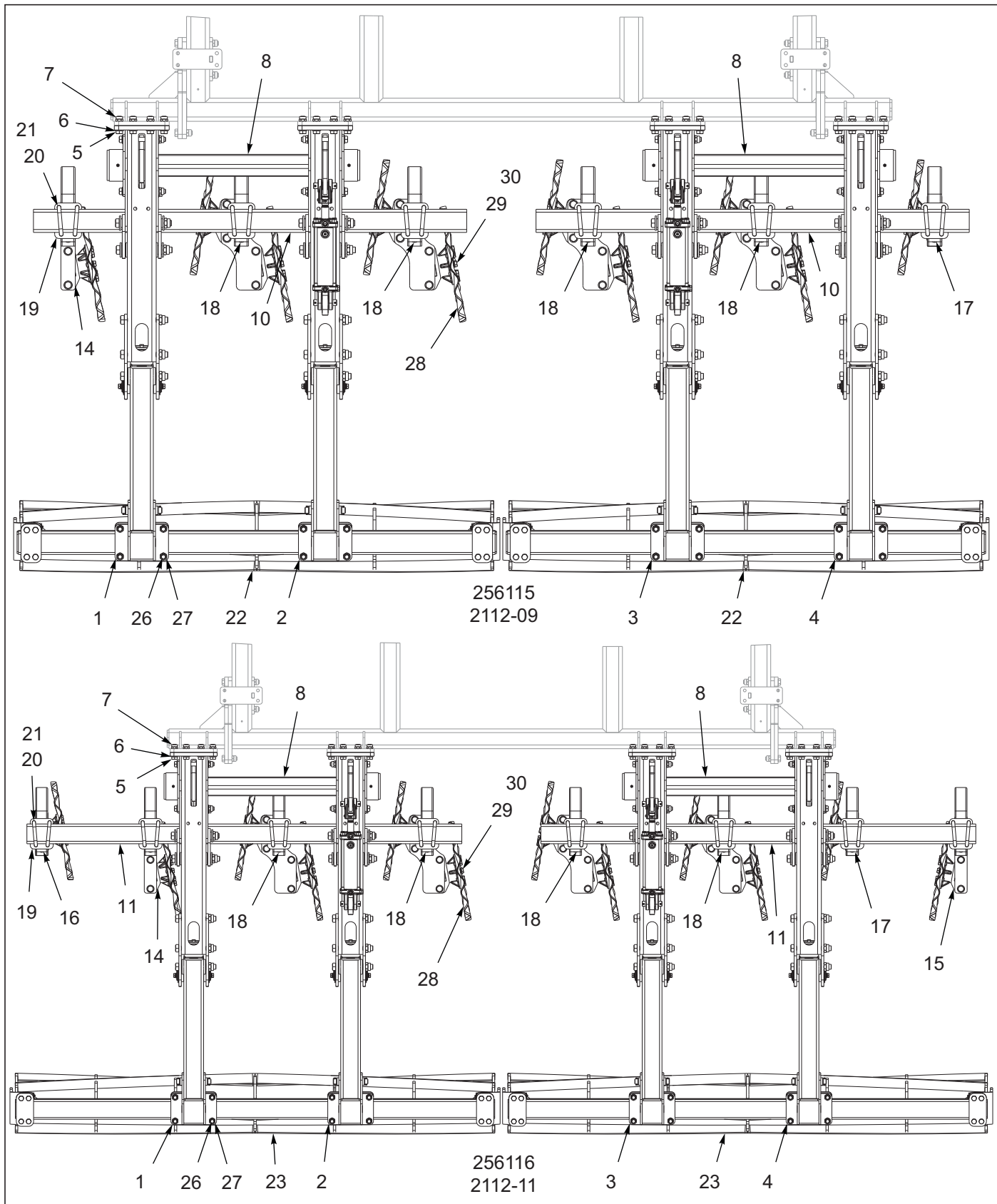
Figure 1-63: Hyd Lev/Reel Layout (1 of 2)
