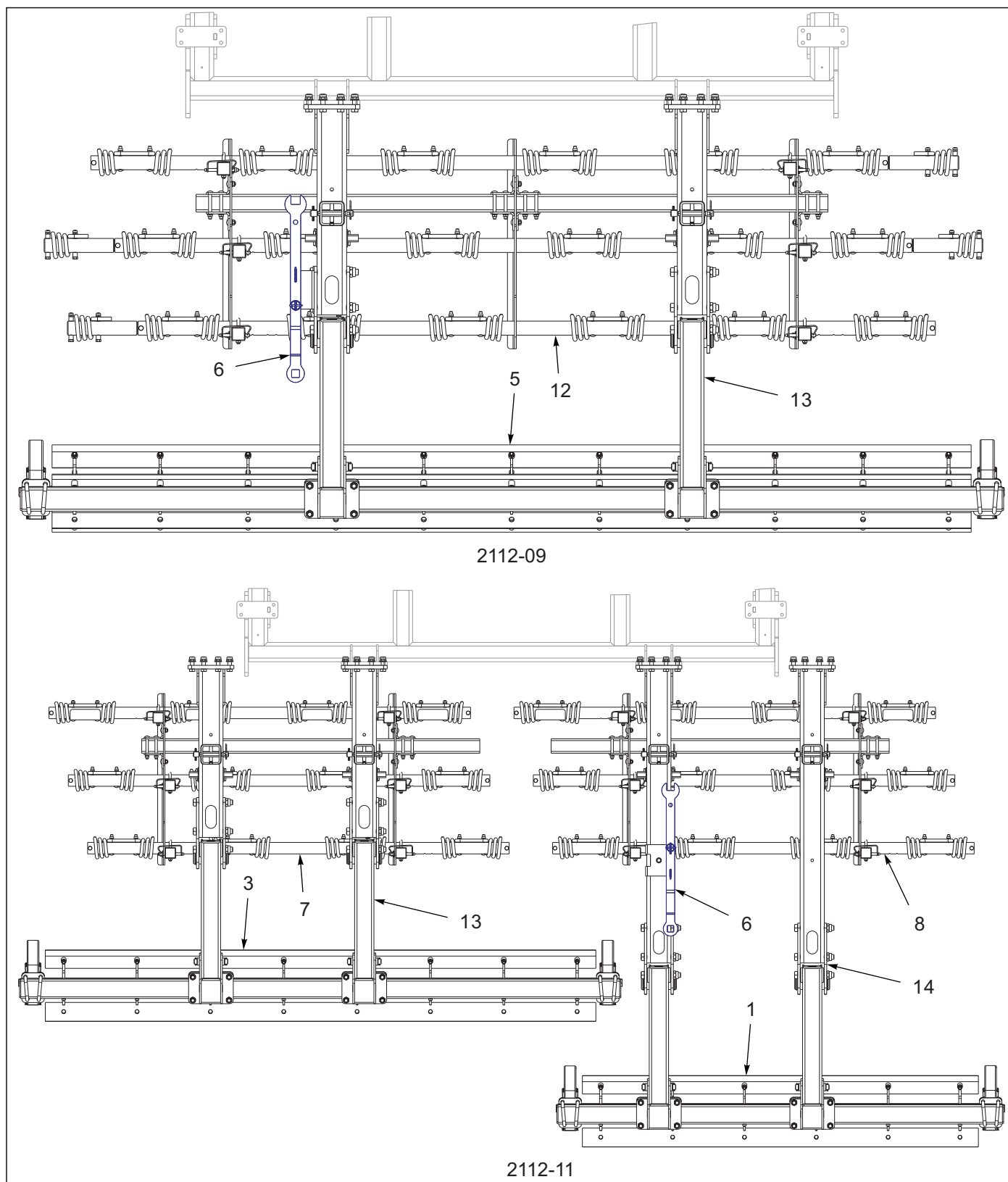
Figure 1-40: Std 3BCT/Chopper Layout (1 of 2)
