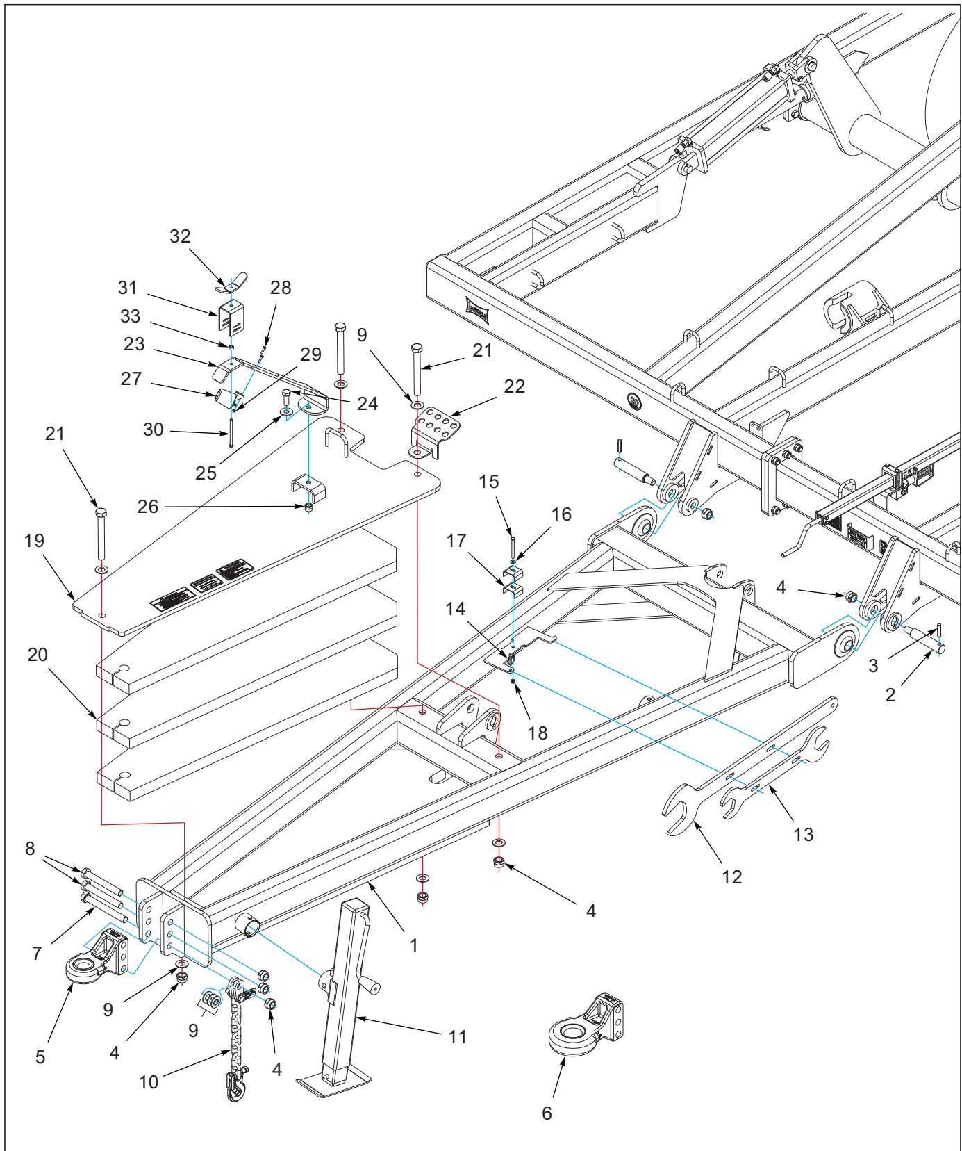
Figure 1-7: Hitch Assembly
