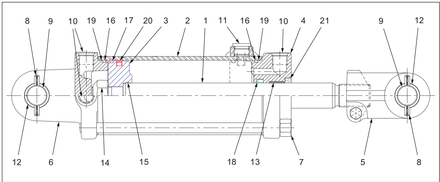
Figure 1-24: Cylinder Assembly 3-3/4 x 8 Rephase (Prince)
