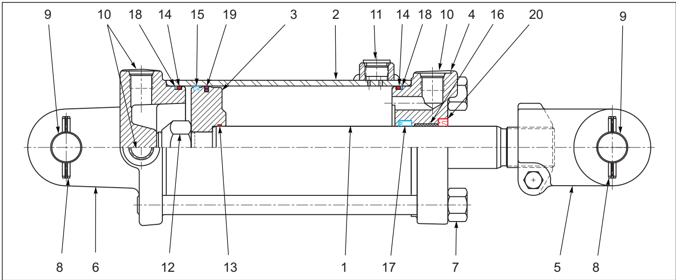
Figure 1-23: Cylinder Assembly 3-3/4 x 8 Rephase (Prince)
