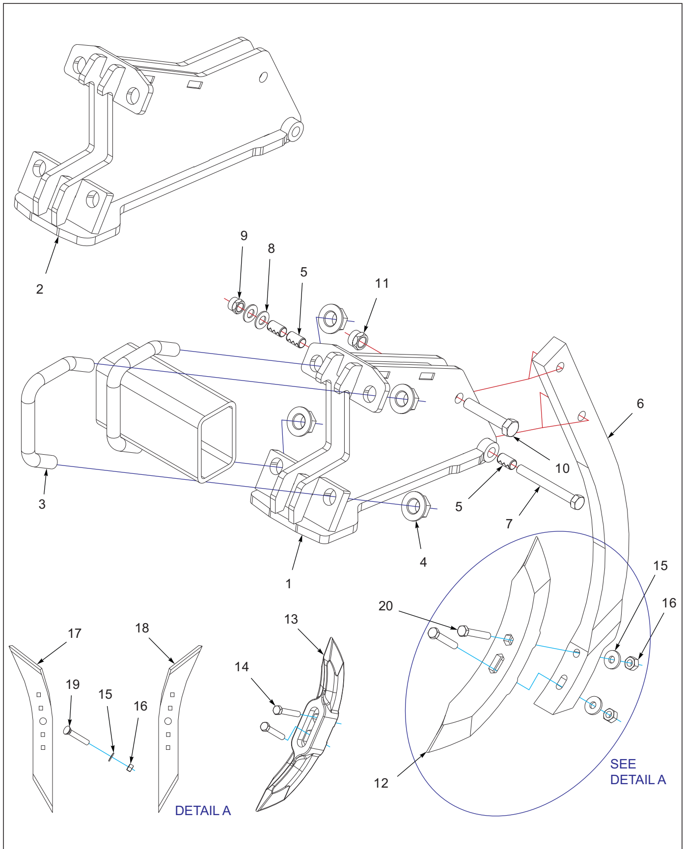
Figure 1-15: Rigid Shear Bolt Clamp Assembly
