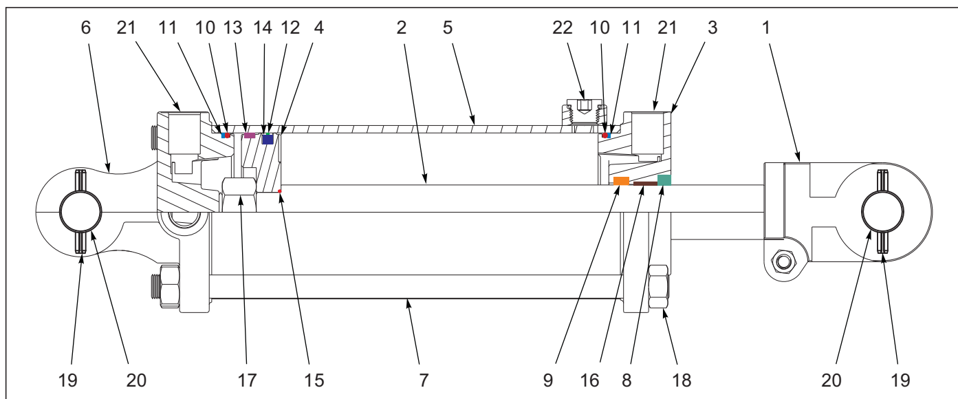
Figure 1-30: Cylinder Assembly 4 x 8 Rephase (Midway)
