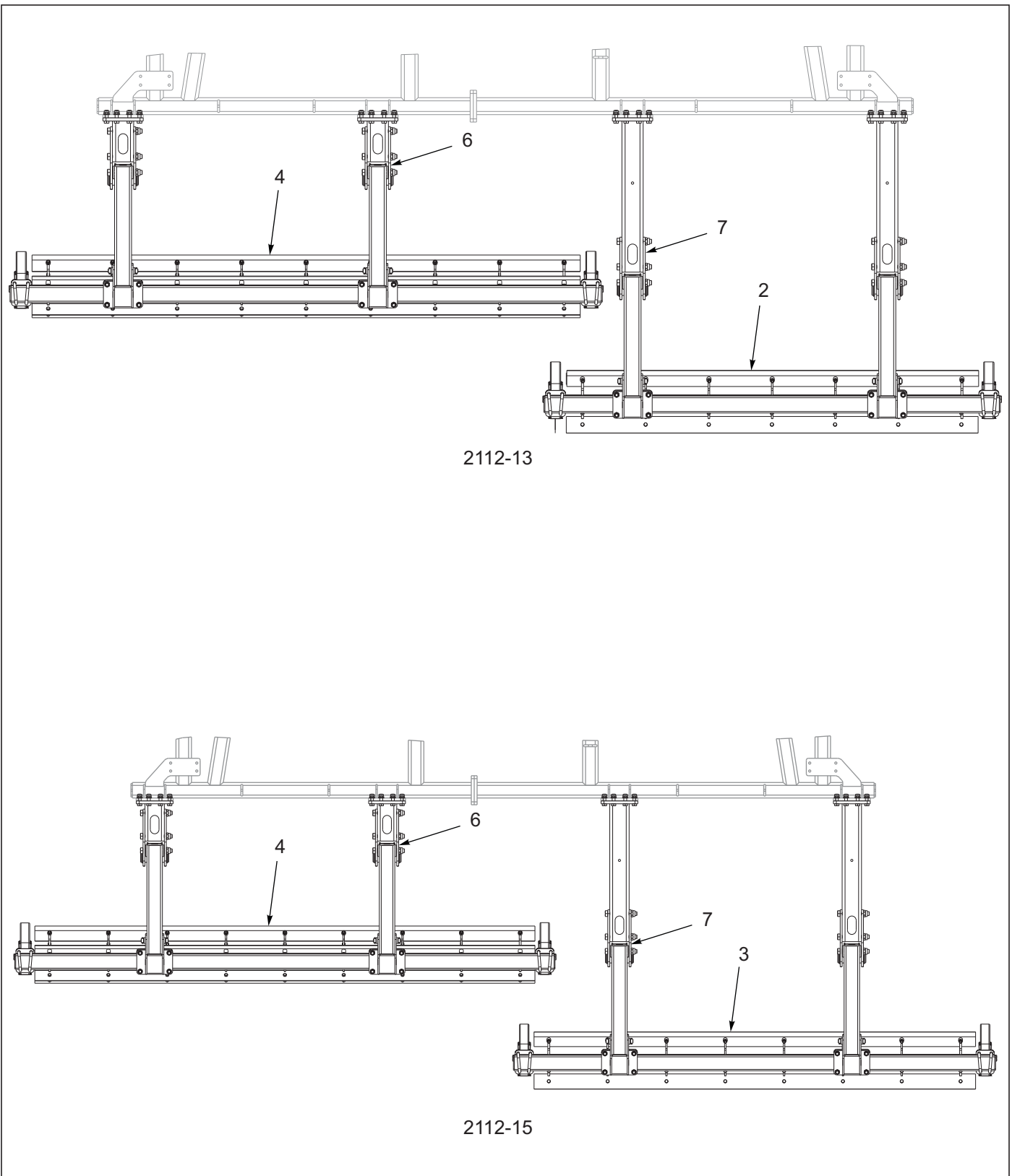
Figure 1-52: Std Chopper Reel Layout (2 of 2)
