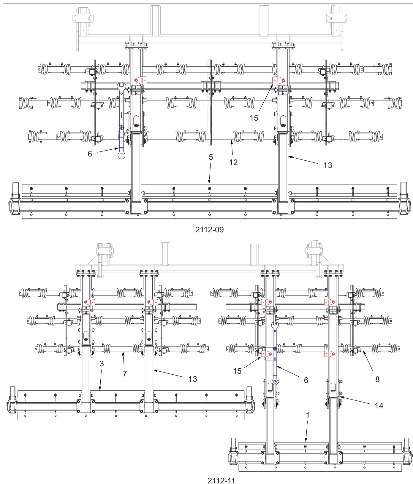
Figure 1-44: Hyd 3BCT/Chopper Layout (1 of 2)
