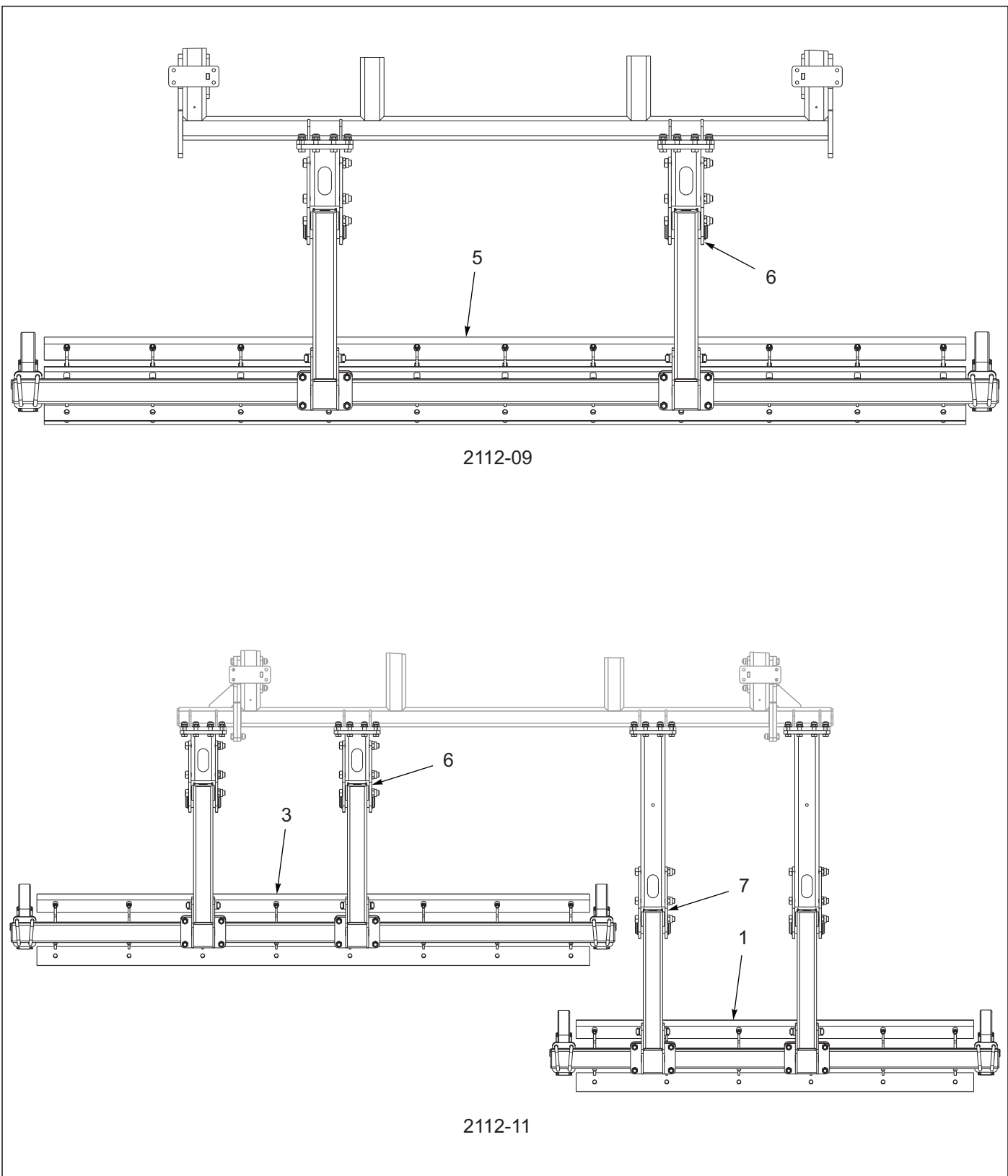
Figure 1-51: Std Chopper Reel Layout (1 of 2)
