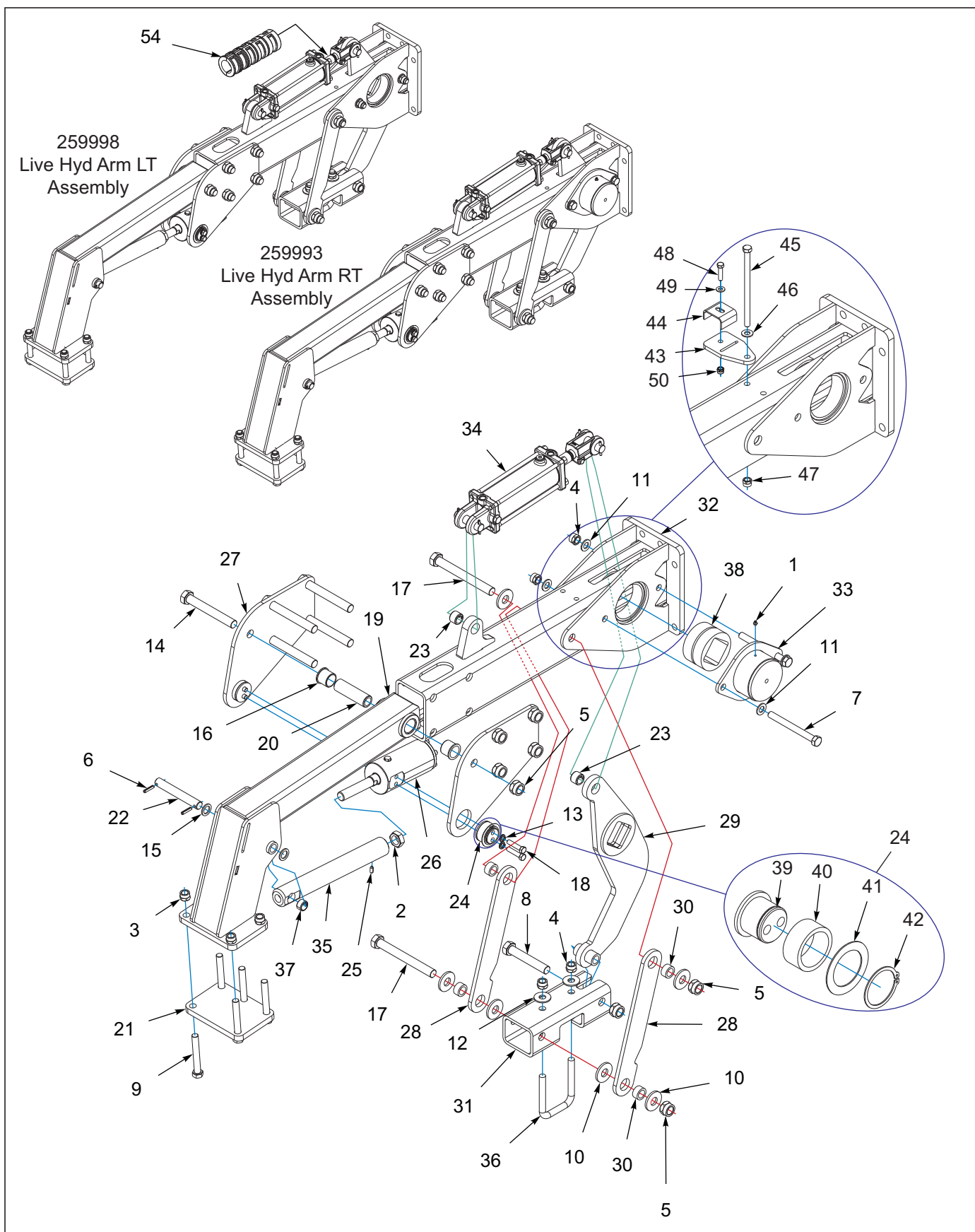
Figure 1-65: Live Hyd Arm Assembly
