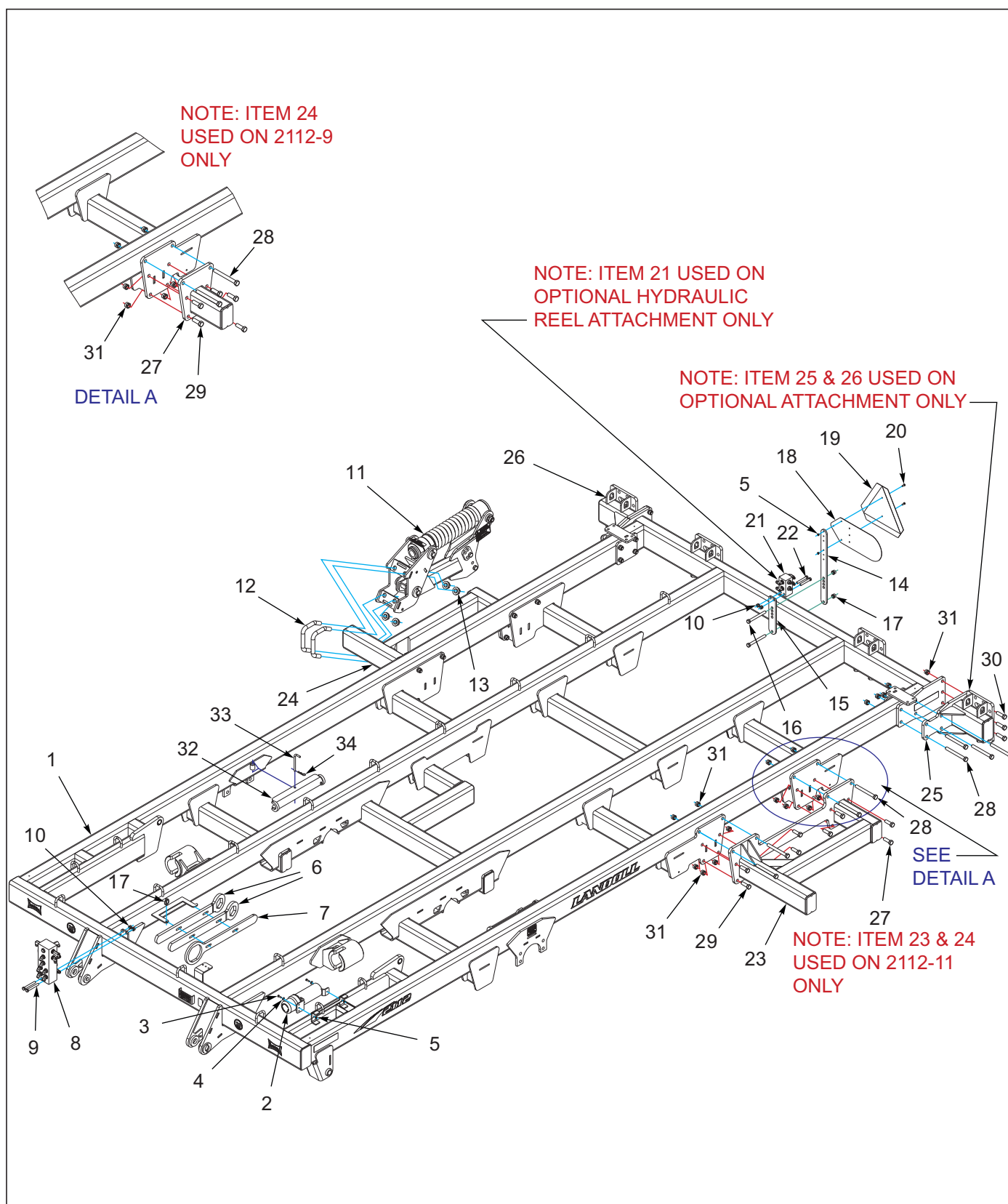
Figure 1-2: Center Frame Assembly 2112-9-11
