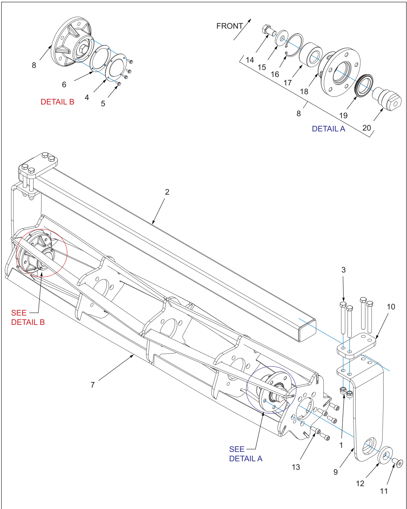
Figure 1-70: Flat Reel/Gangbar Assembly
