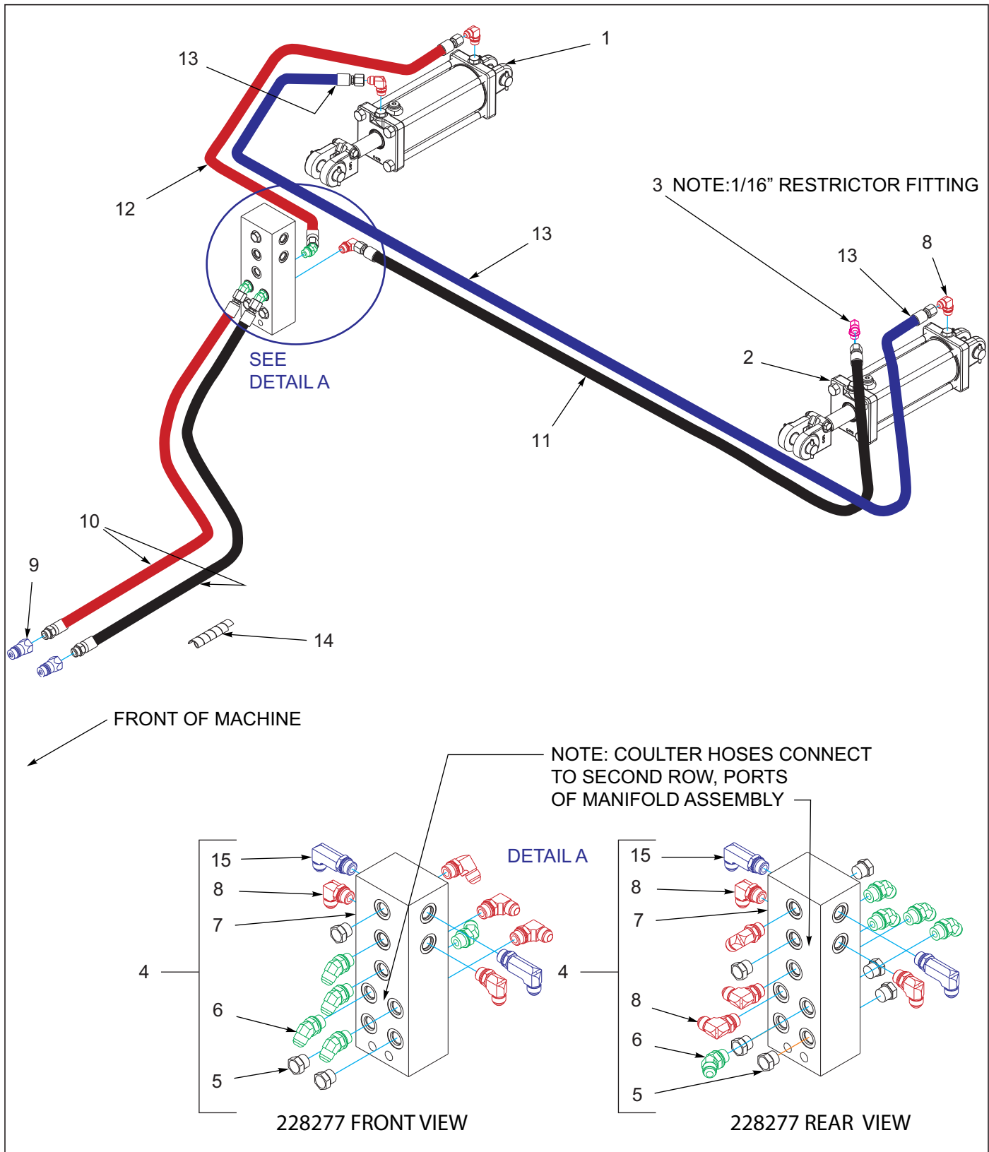
Figure 1-20: Coultter Gang Assembly
