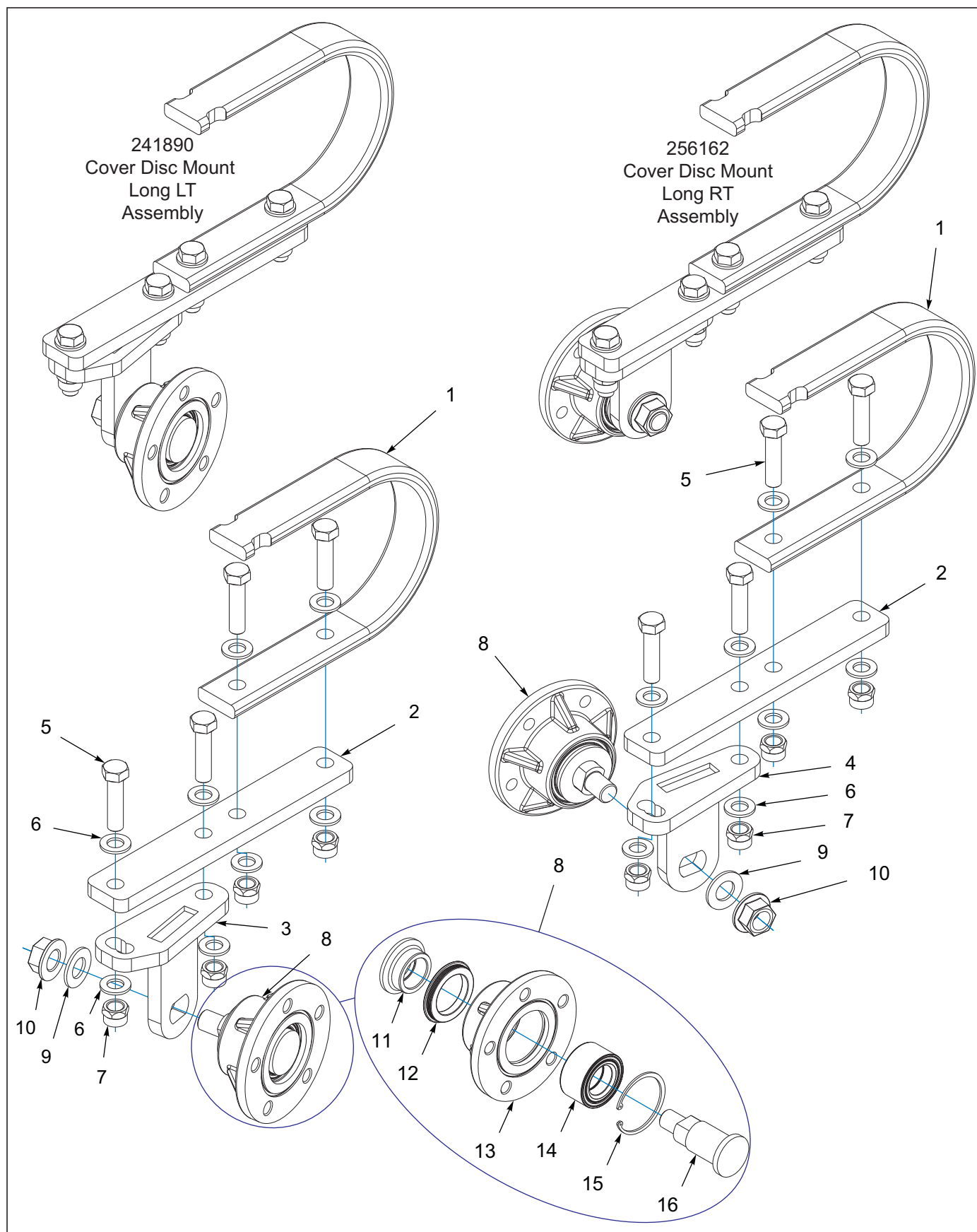
Figure 1-69: Cover Disc Mount Long Assembly
