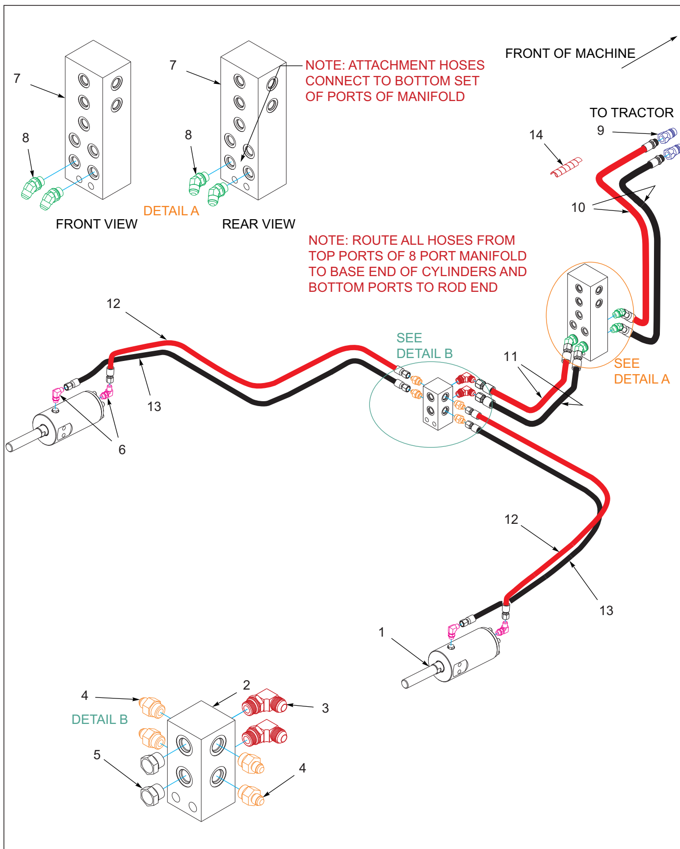
Figure 1-49: 3BCT/Chopper Hydraulic Assembly 2112-09
