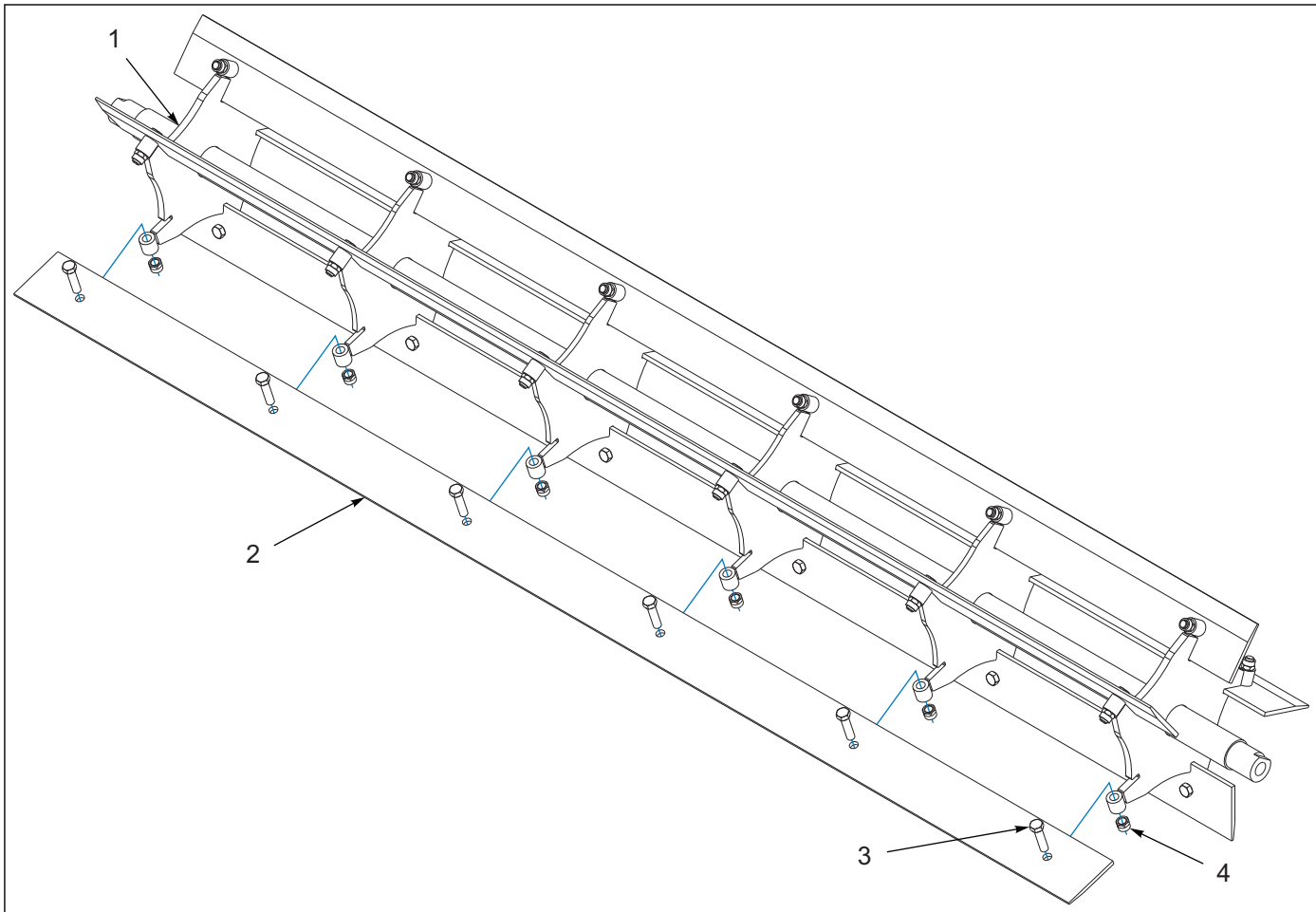
Figure 1-60: Reel Blade Assembly
