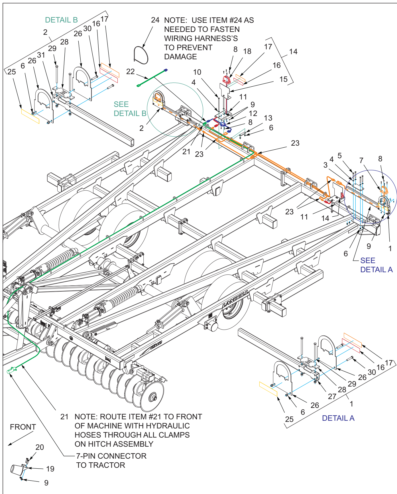
Figure 1-37: Electrical Assembly W/ LED Lights (2 of 2)
