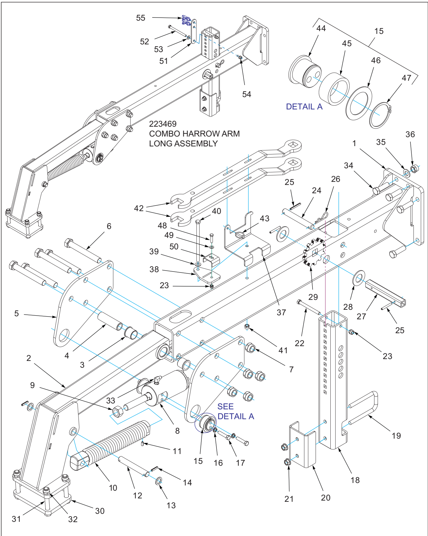
Figure 1-46: Hyd Combo Harrow Arm Long Assembly
