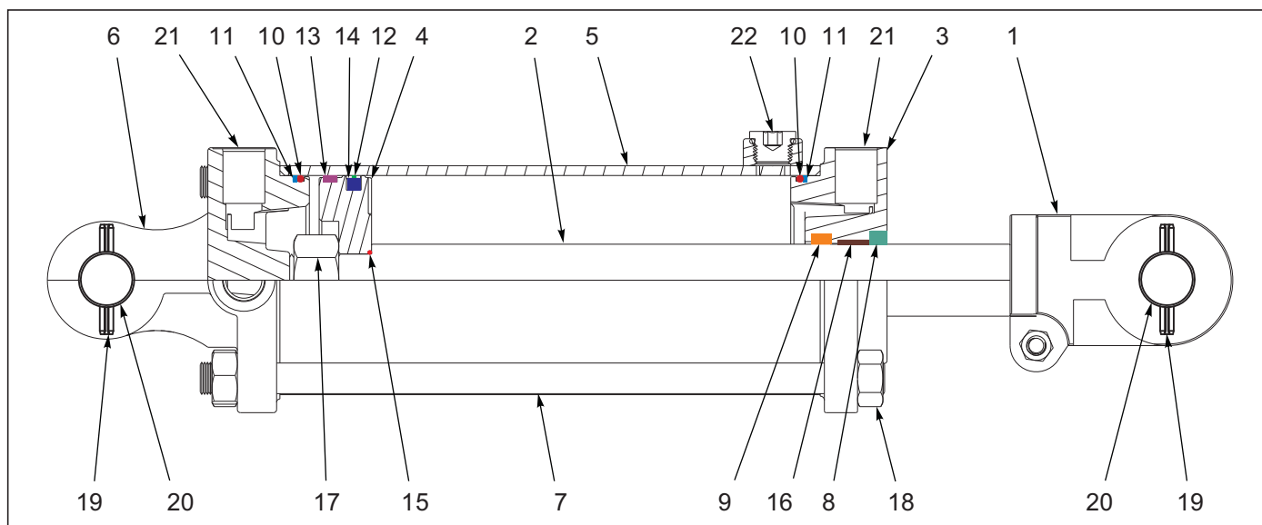
Figure 1-26: Cylinder Assembly 3-3/4 x 8 Rephase (Midway)
