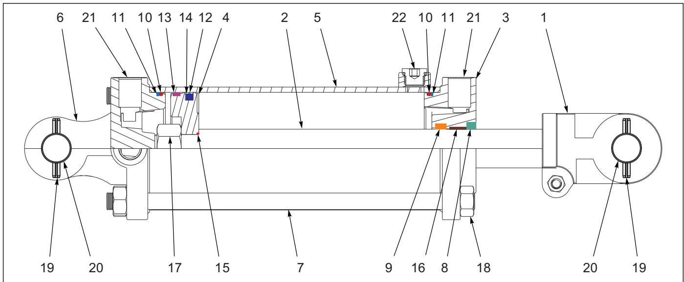
Figure 1-32: Cylinder Assembly 3-1/4 x 8 Rephase (Midway)
