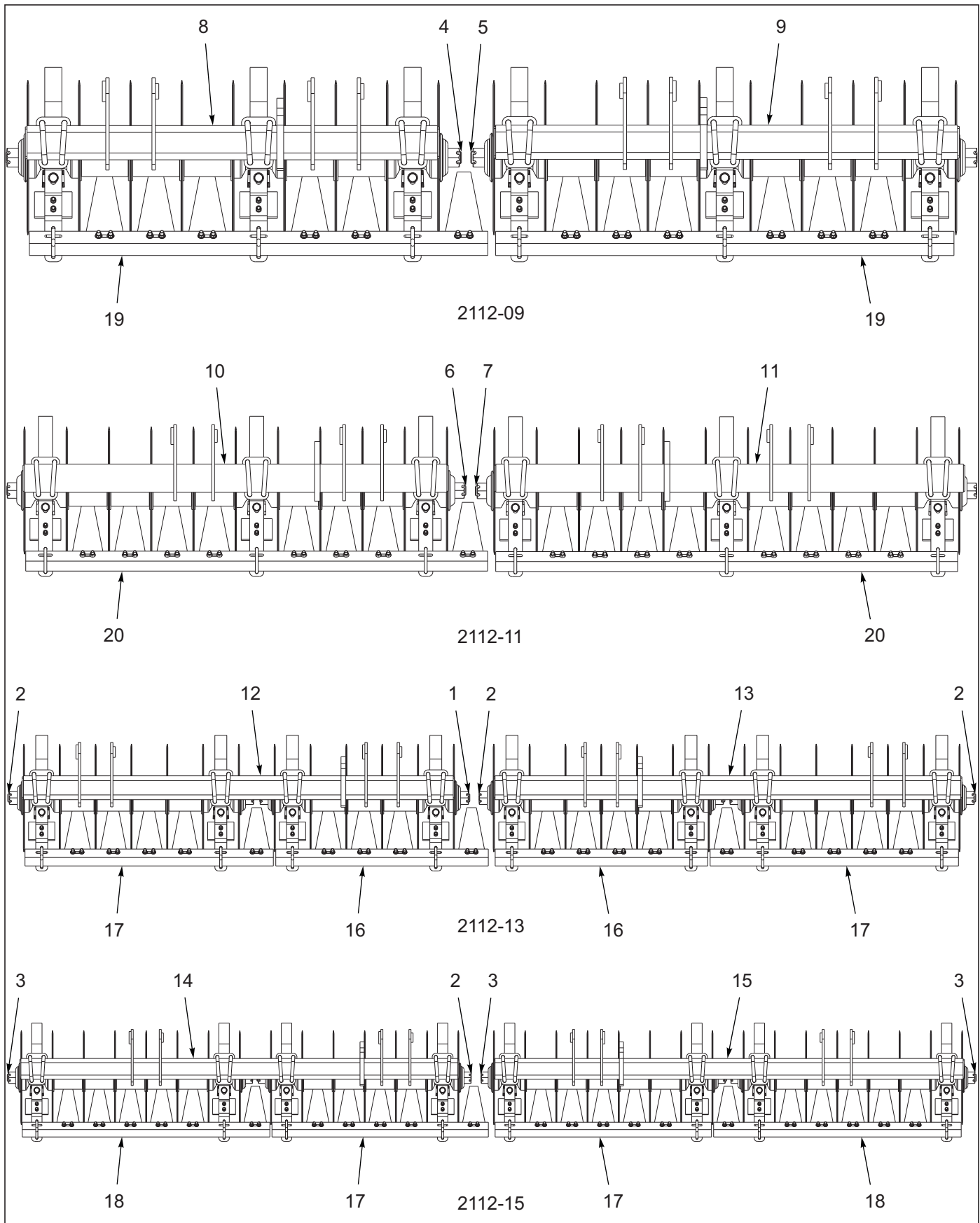
Figure 1-18: Coulter Gang Placement
