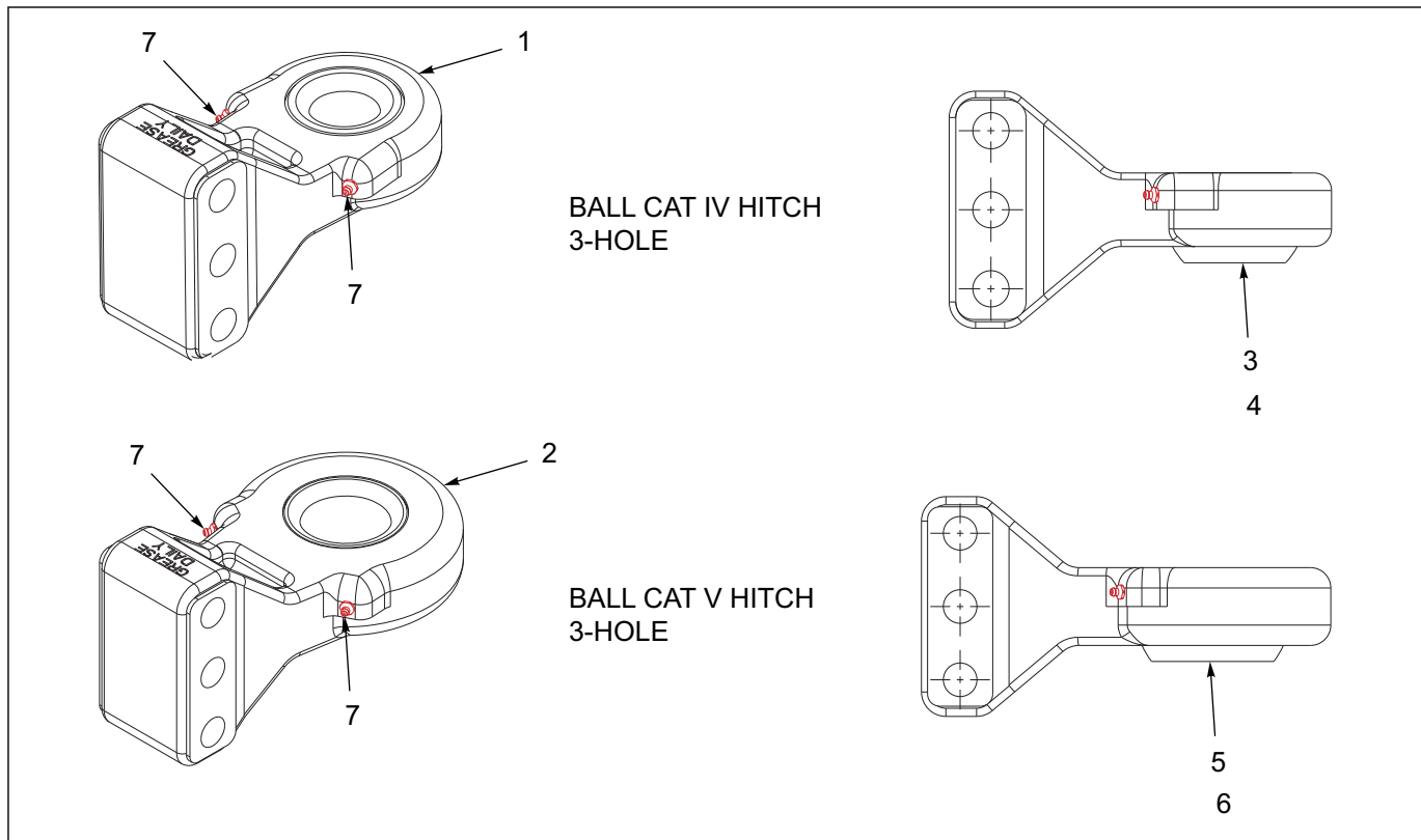
Figure 1-9: Ball &amp; Clevis Hitches
