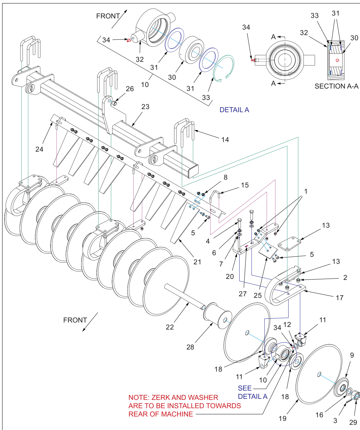
Figure 1-16: Coulter Gang Assembly
