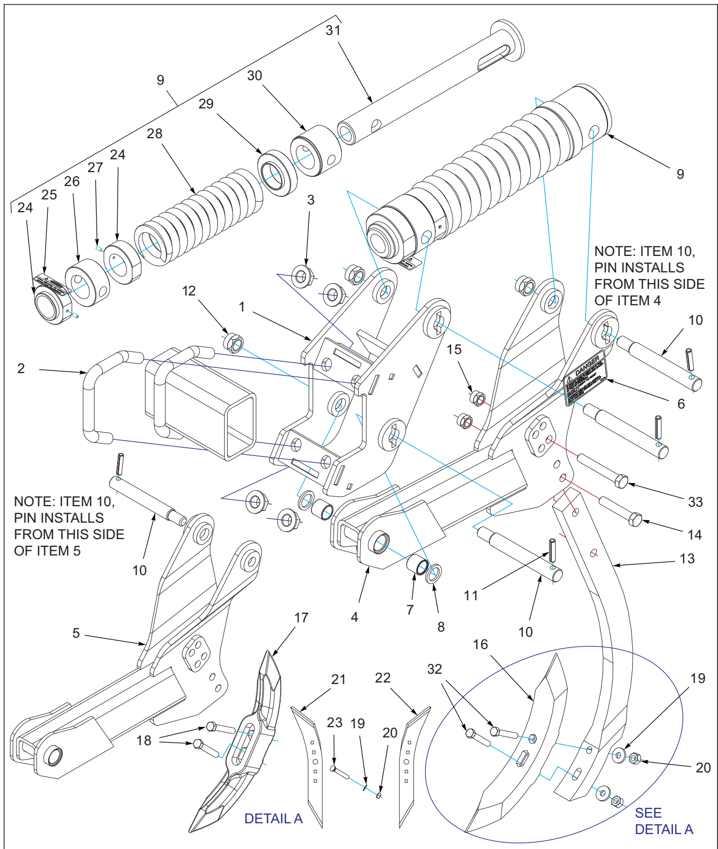
Figure 1-13: Auto Reset Clamp Assembly Before 12-01-2023
