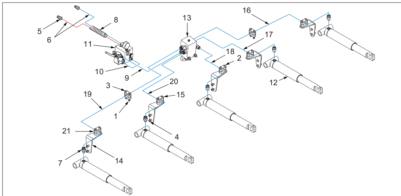
Figure 4-5: 2512 Hydraulics, 5 Shank
