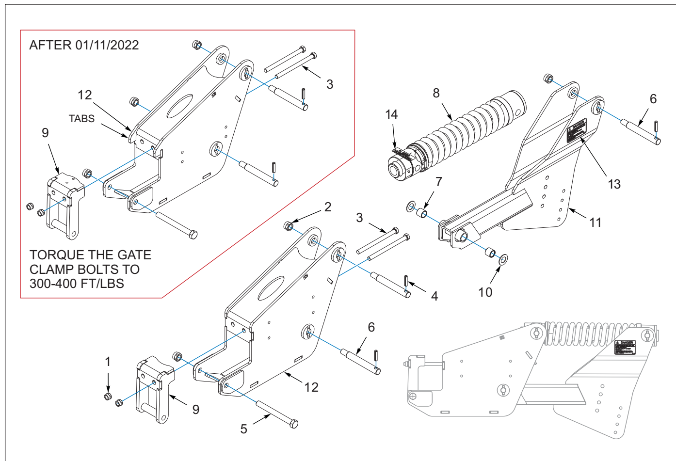
Figure 1-10: 2512 Auto Reset Shank Clamp, Spring - Setback (BEF. 01/16/2023)
