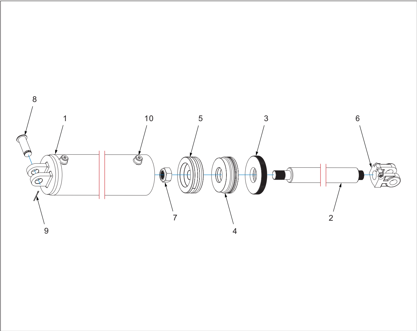
Figure 4-17: Hydraulic Cylinder, 6 x 30 - 233833
