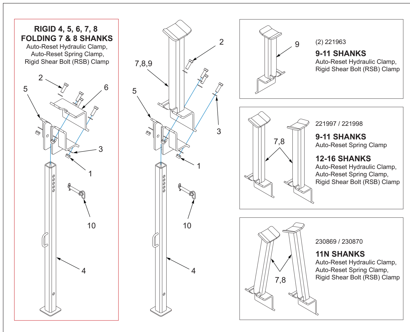
Figure 1-19: 2512 Jack Stand and Wing Rest (11/01/21 TO 06/07/23)
