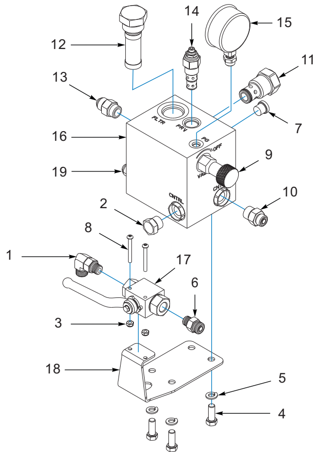
Figure 4-10: Manifold-Draft Assembly
