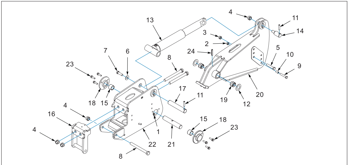
Figure 1-14: Auto Reset Shank Clamp, Hydraulic - Setback (12/12/23 TO 02/07/25)
