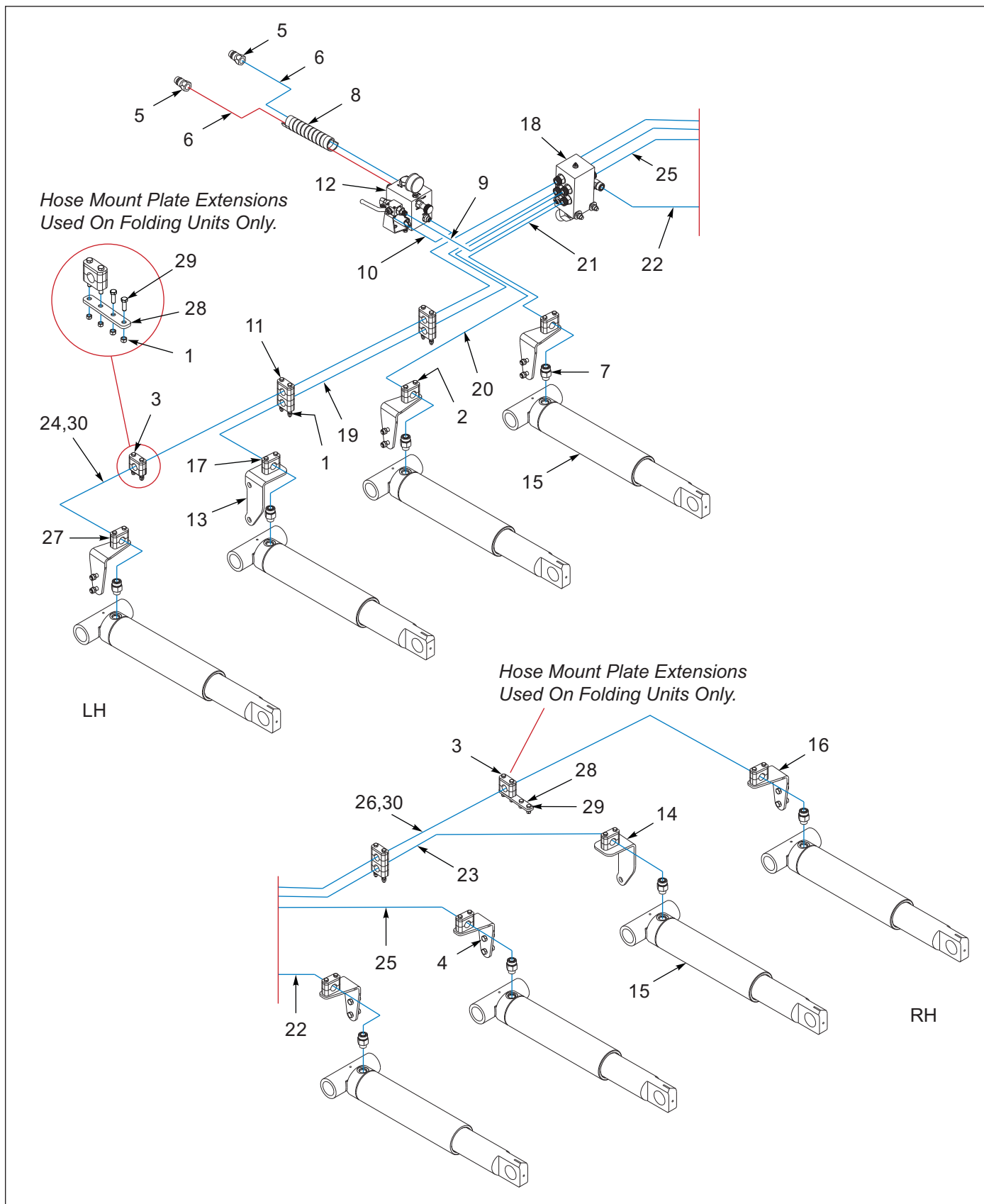
Figure 4-8: 2512 Hydraulics, 8 Shank (Rigid and Folding)
