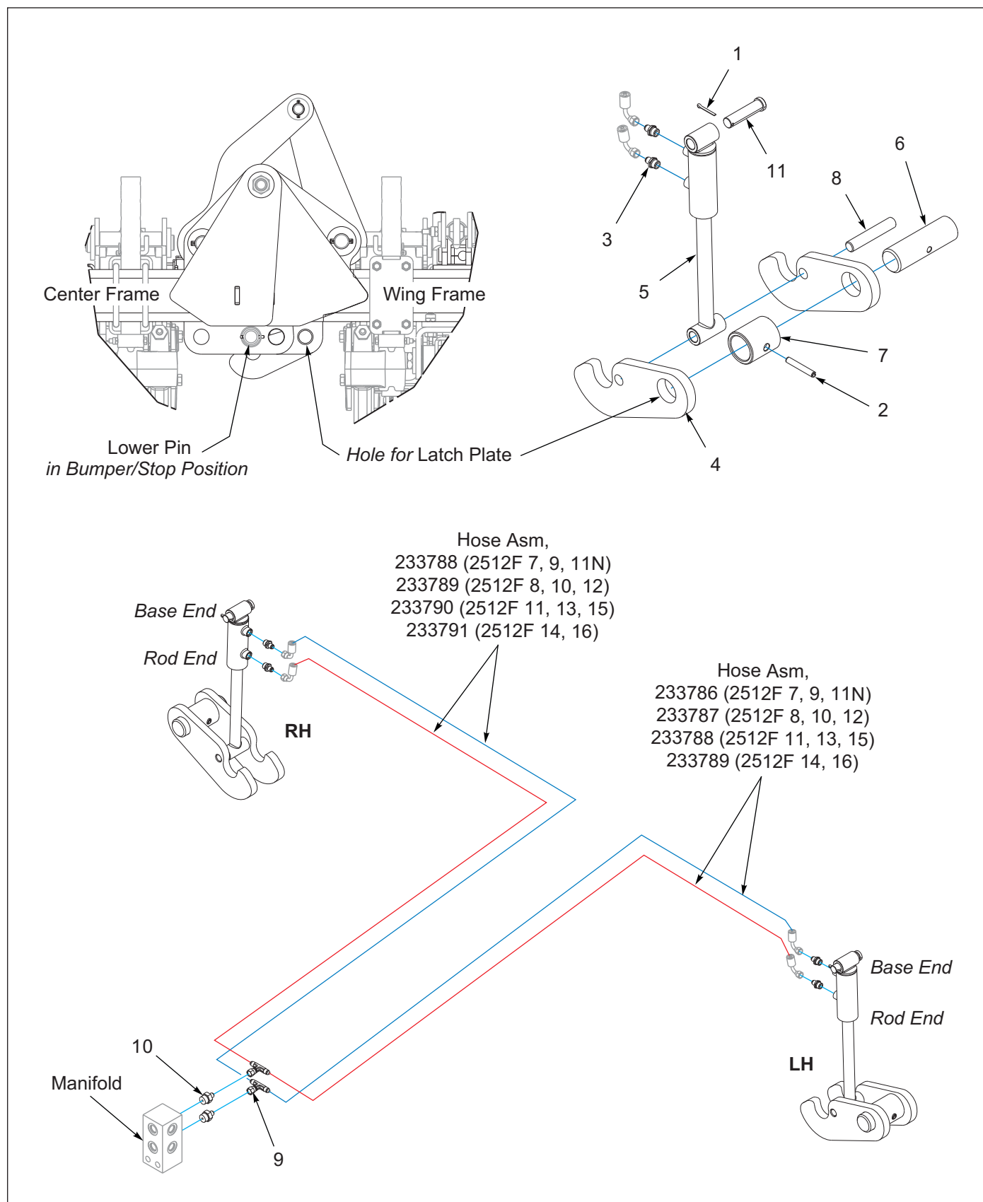
Figure 4-12: Wing Lock Kit - Optional
