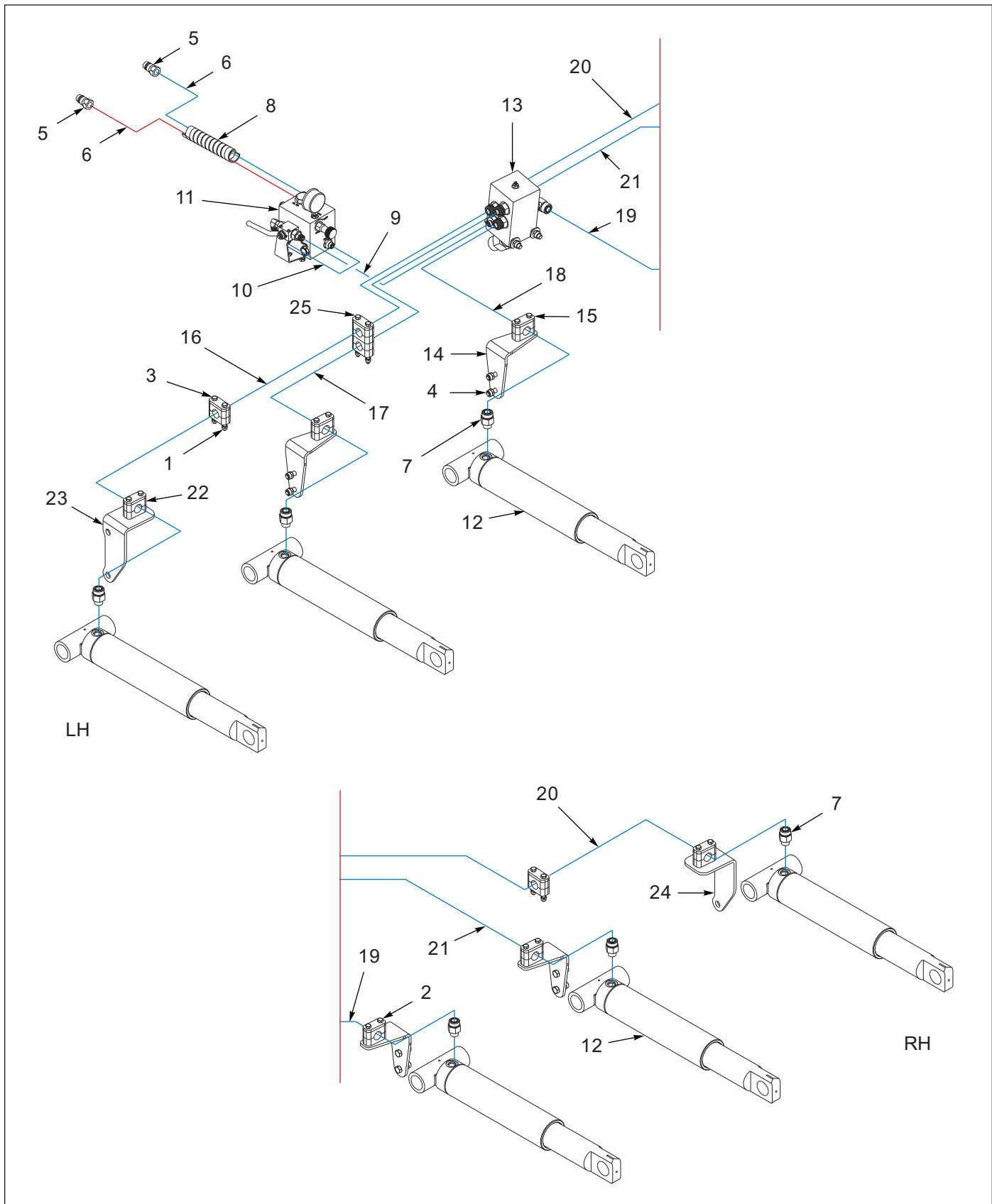
Figure 4-6: 2512 Hydraulics, 6 Shank
