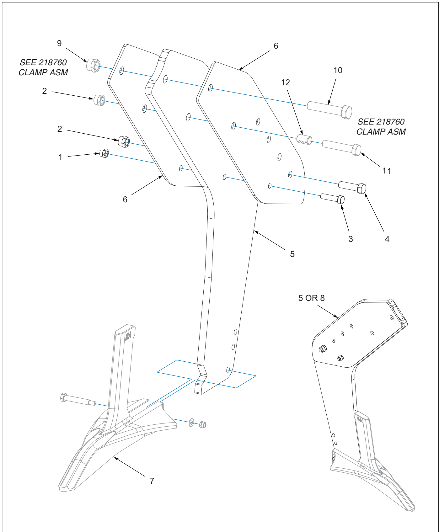
Figure 5-3: Straight Leg Shank, 3/4 (AFTER 02/2026)
