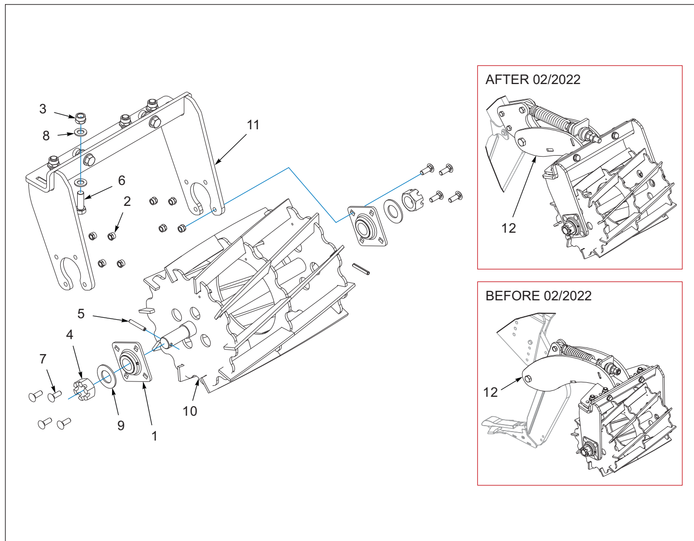
Figure 7-8: Flat Bar Basket - 20"
