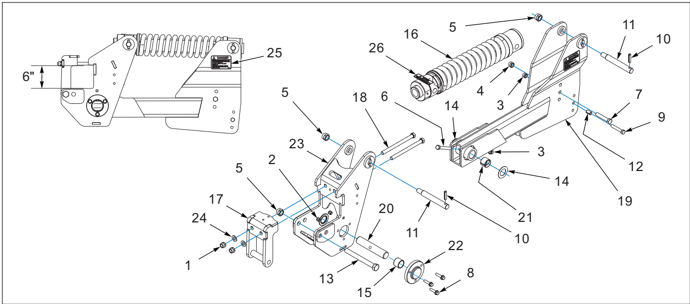
Figure 1-7: Auto Reset Shank Clamp, Spring (01/16/2023 TO 01/01/2024)
