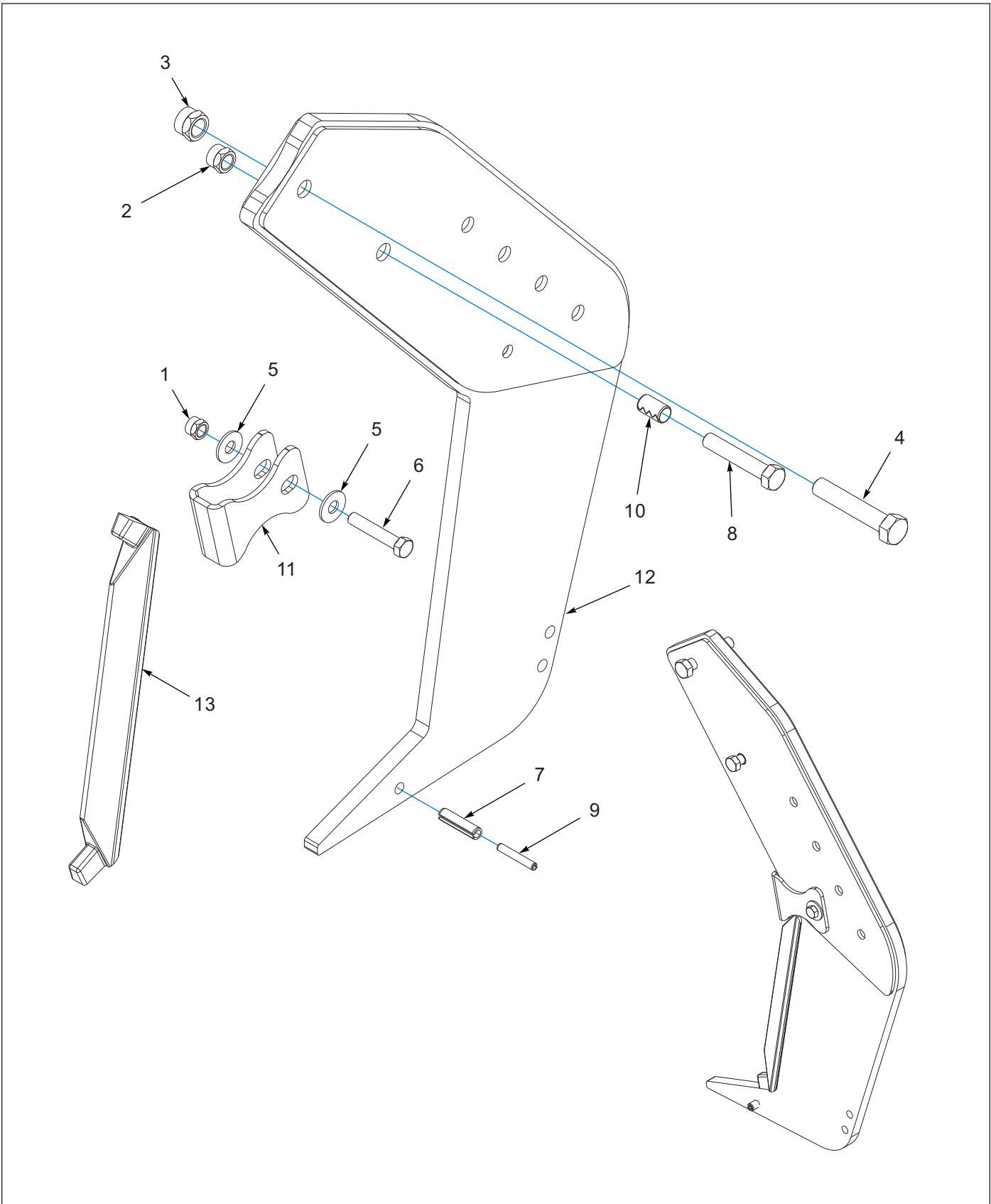
Figure 5-4: Straight Leg Shank, 3/4 (BEFORE 02/2026)
