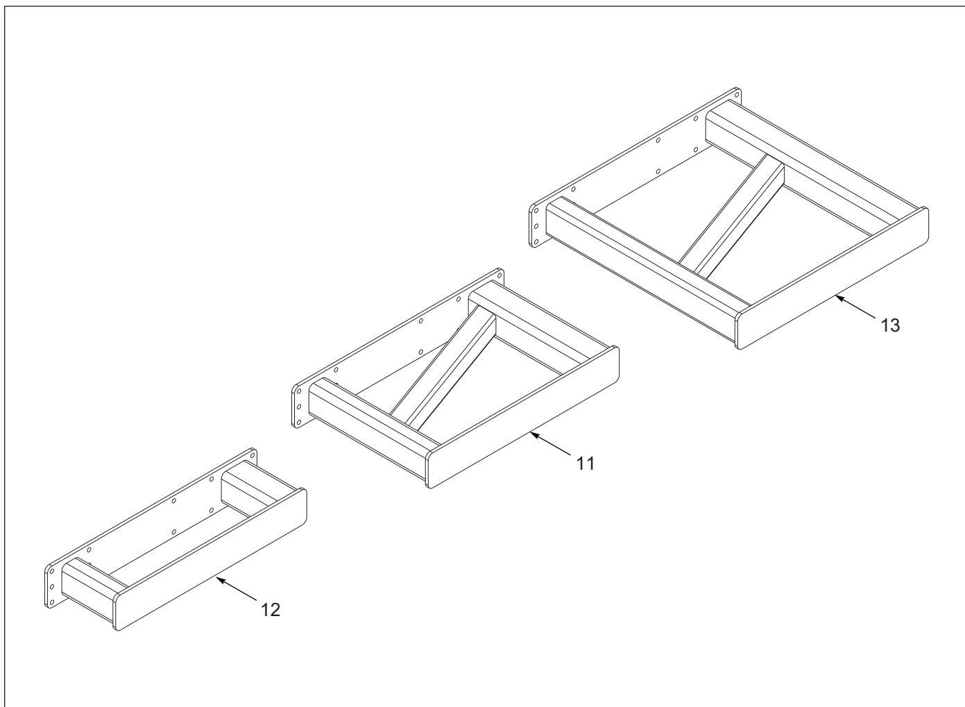
Figure 1-2: Rigid Frame (2 of 2)
