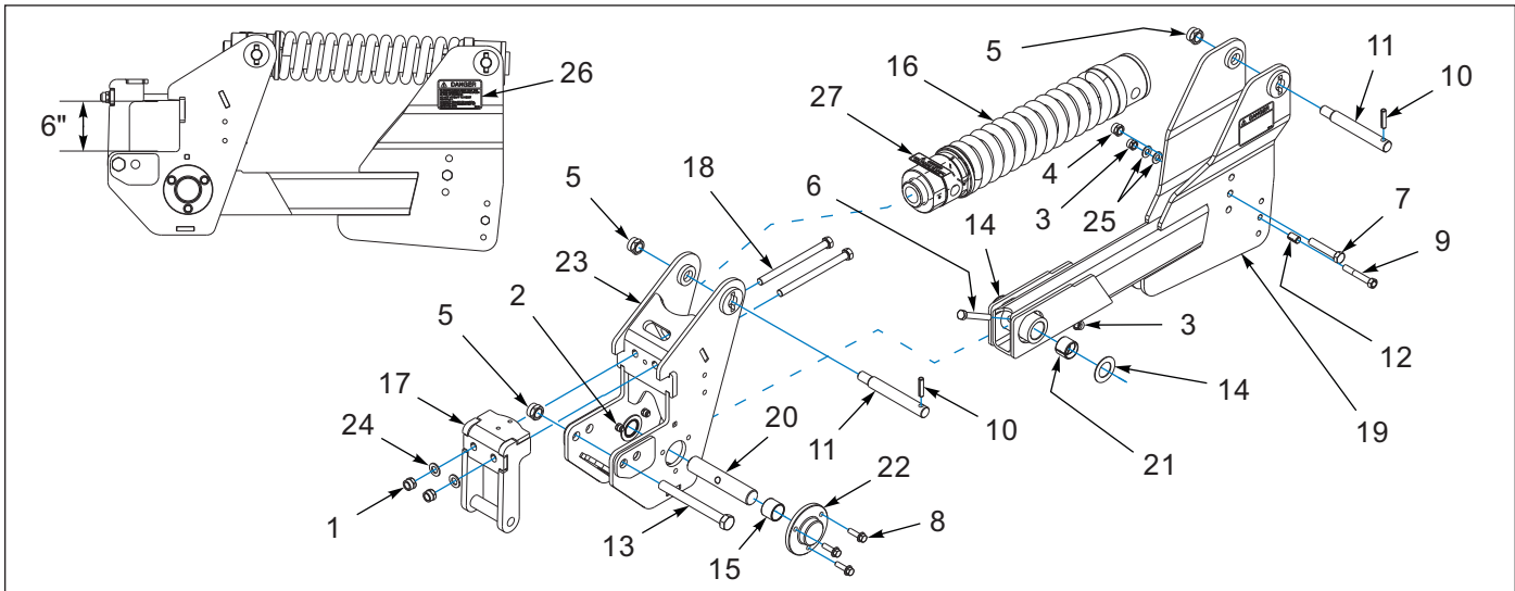
Figure 1-5: Auto Reset Shank Clamp, Spring (AFT. 01/01/2024)
