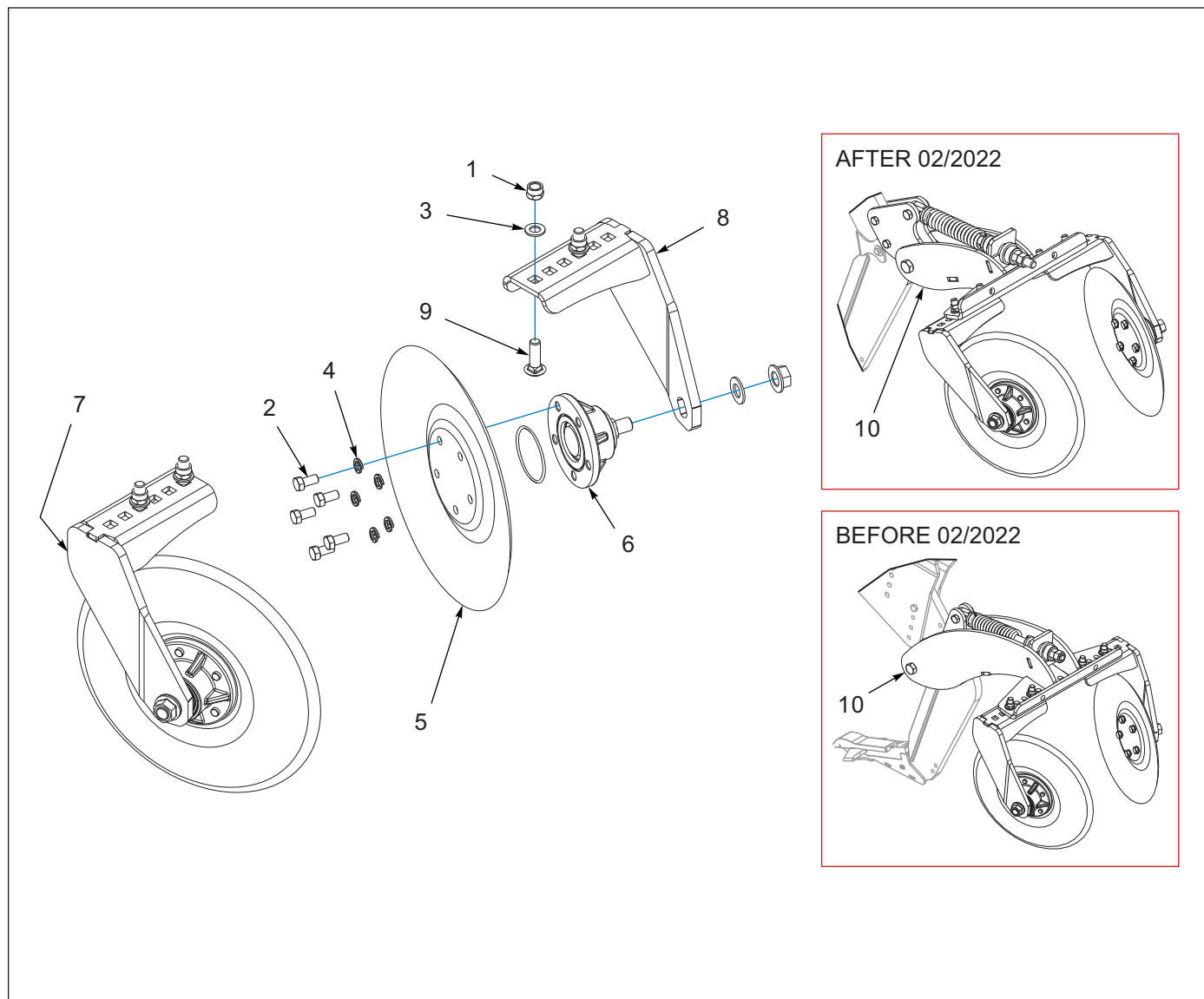
Figure 7-9: Closer Disc
