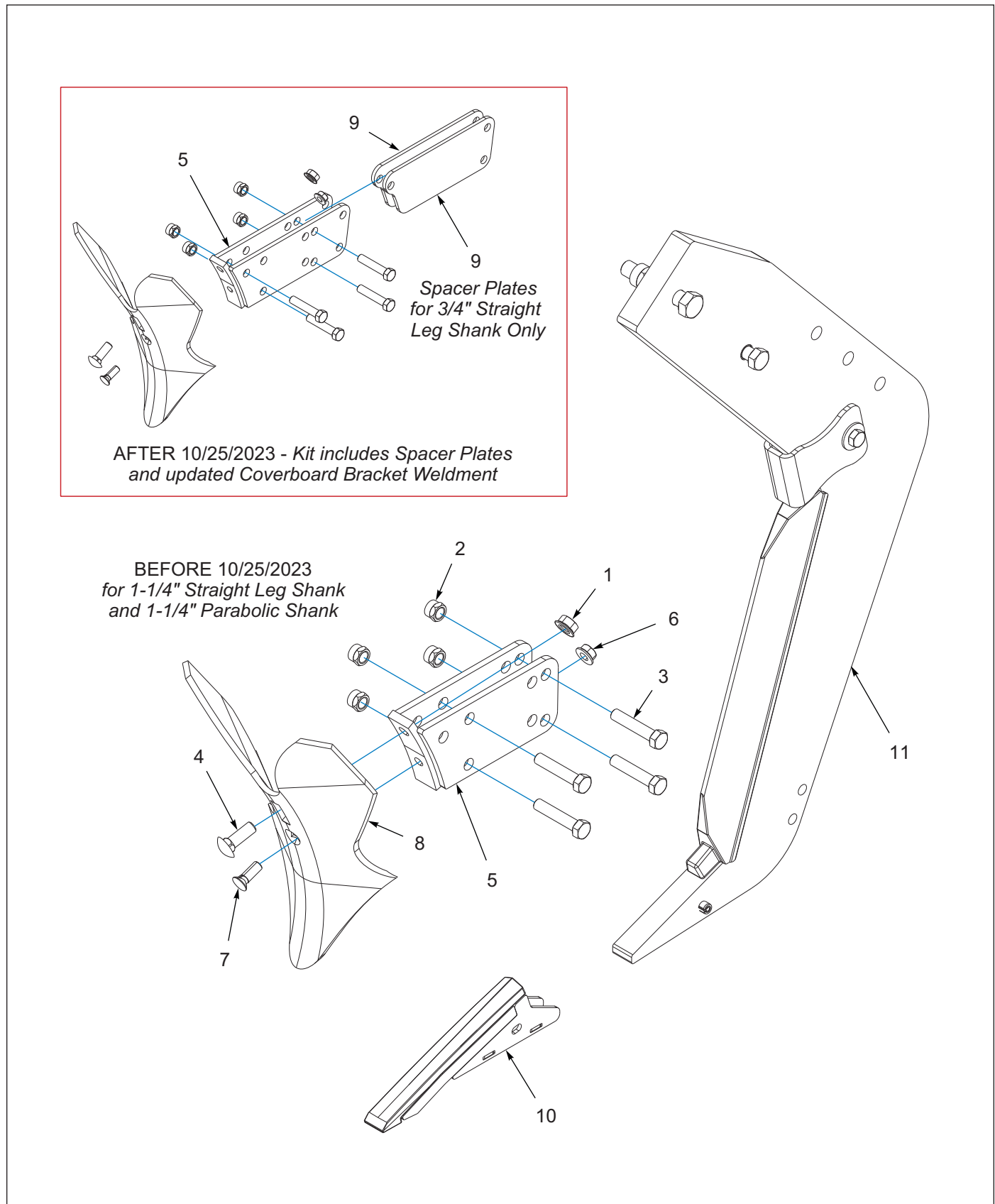
Figure 5-5: Coverboard Kit
