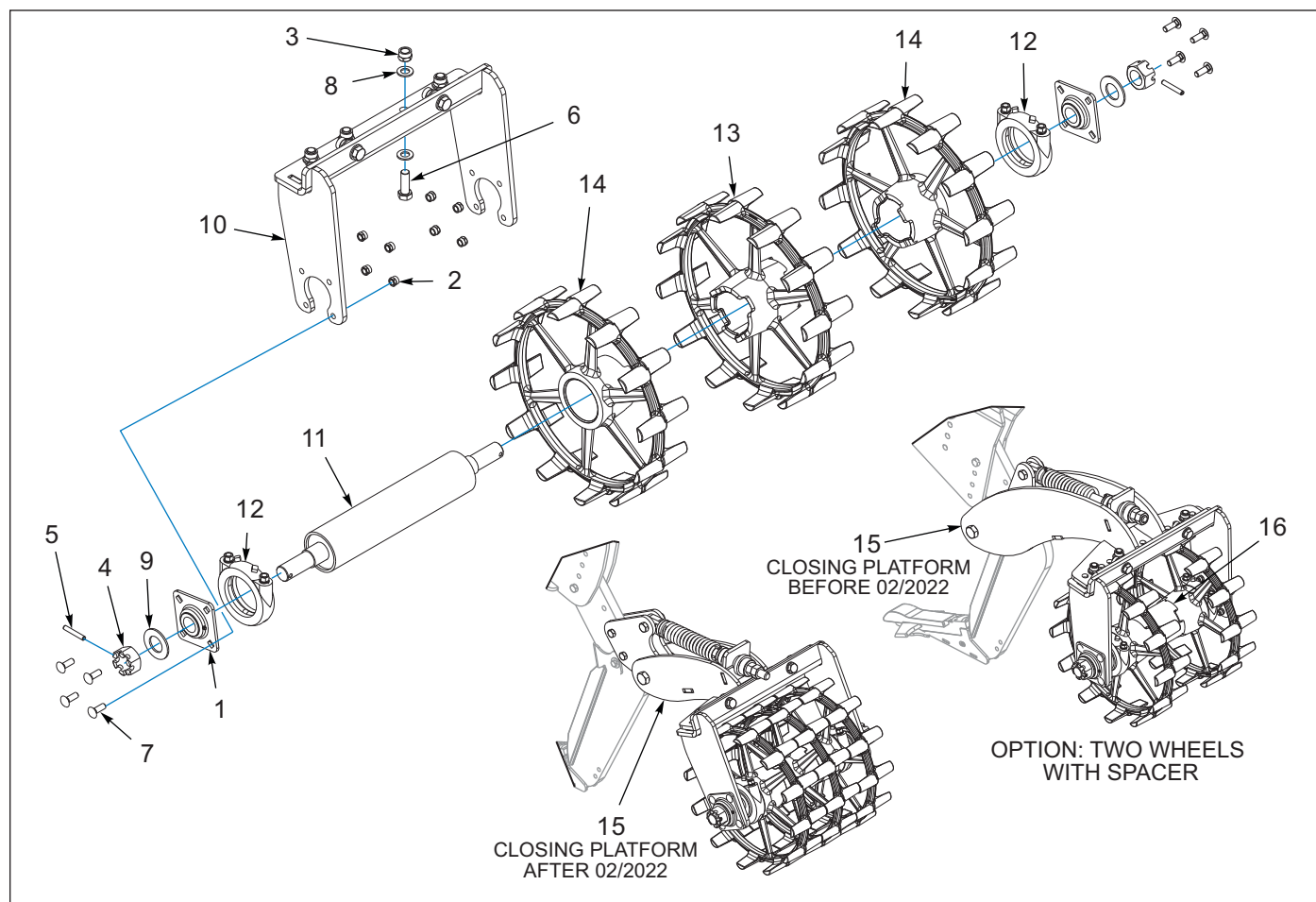
Figure 7-10: Crumbler Reel
