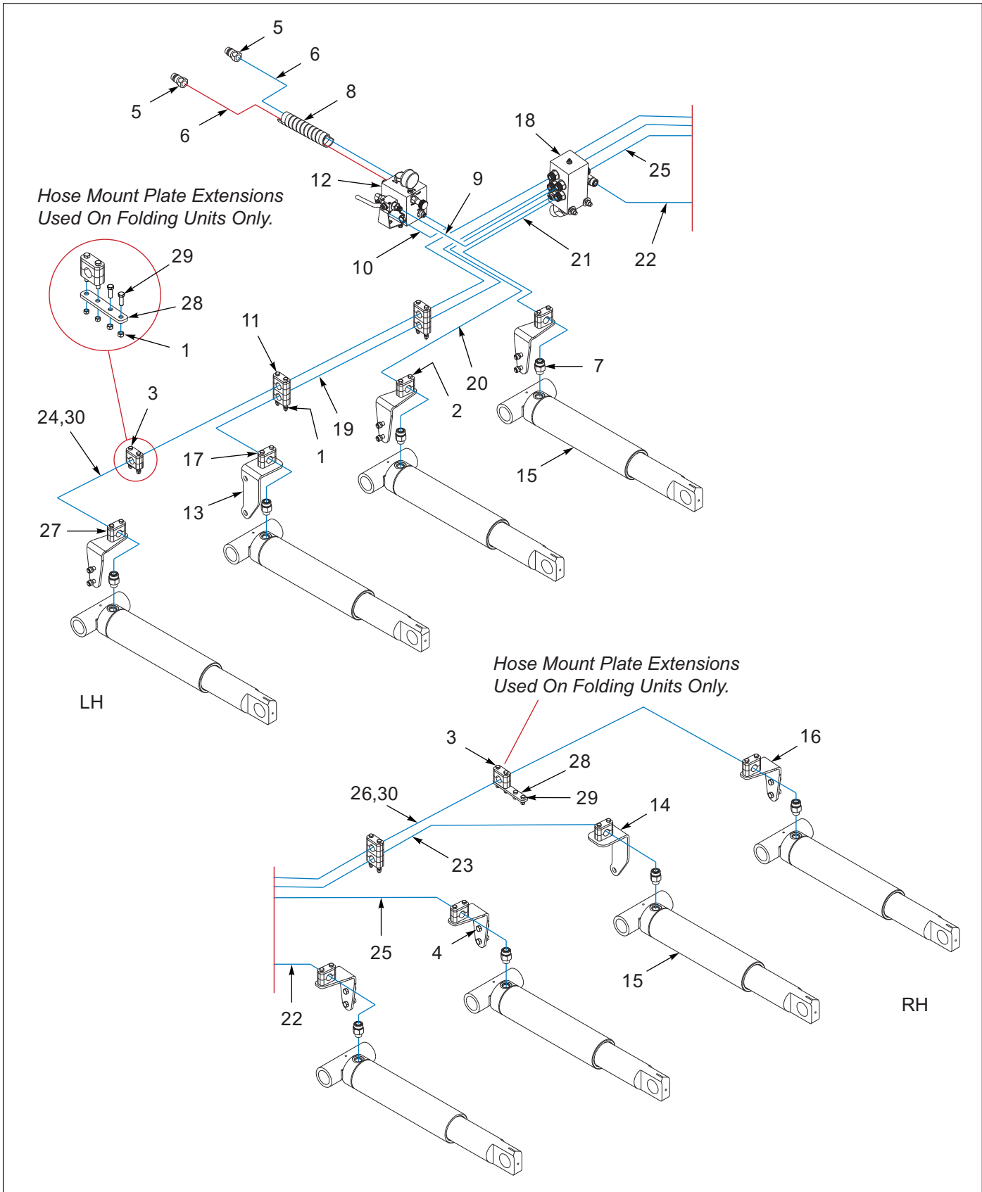
Figure 4-8: 2512 Hydraulics, 8 Shank (Rigid and Folding) (1 of 2)
