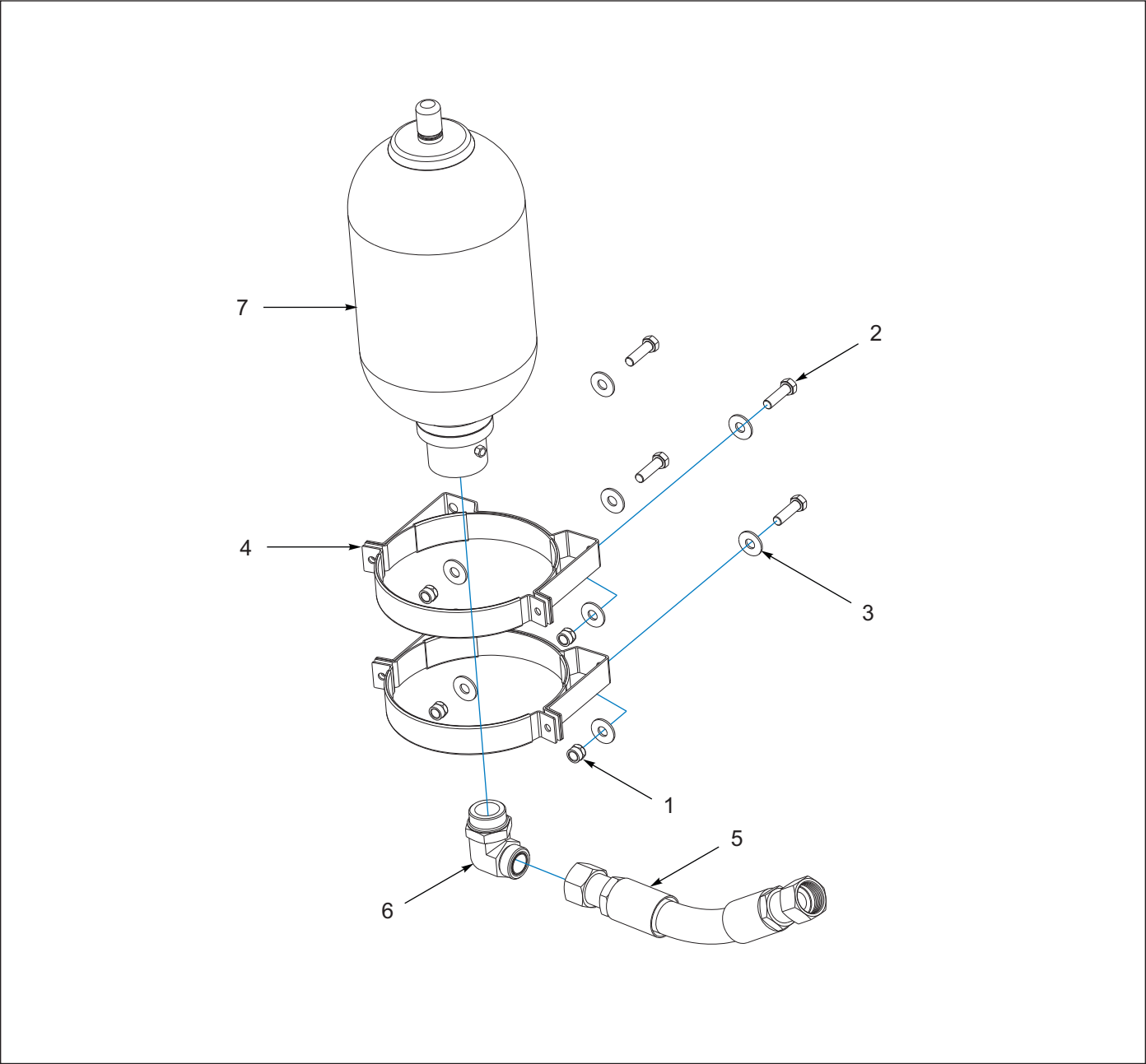
Figure 4-3: 2512 Accumulator Bladder
