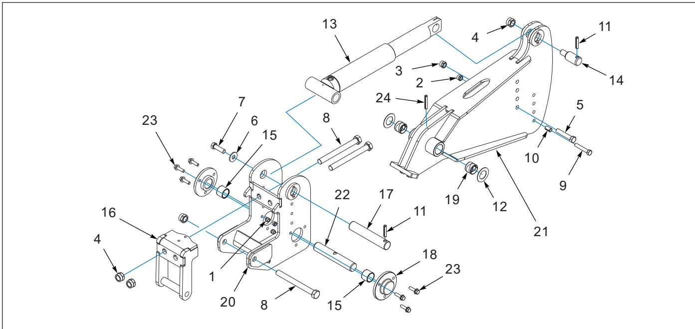
Figure 1-13: Auto Reset Shank Clamp, Hydraulic (12/12/23 TO 02/07/25)
