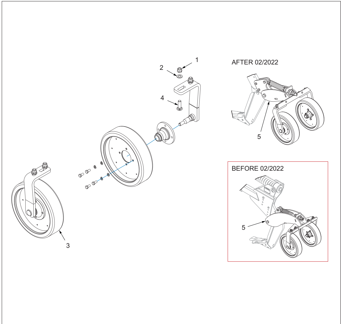
Figure 7-7: Closer Wheel
