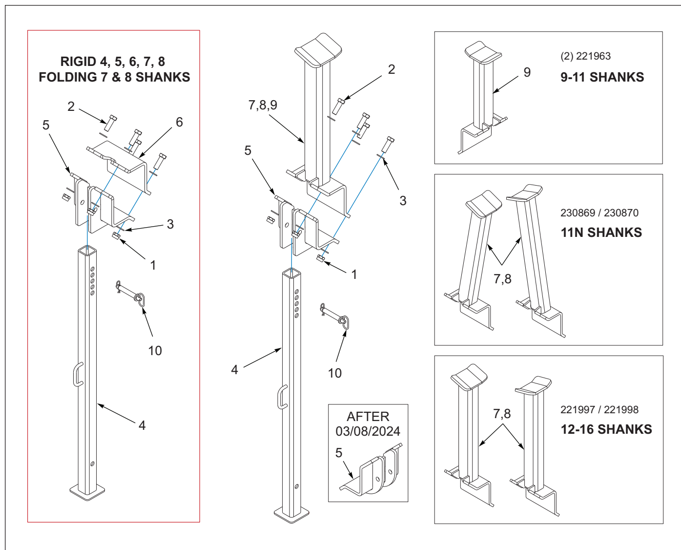
Figure 1-18: 2512 Jack Stand and Wing Rest (AFTER 06/07/2023)
