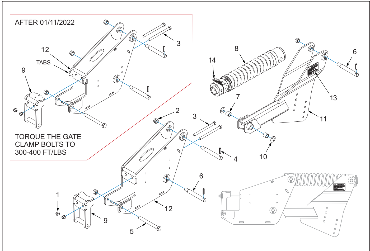
Figure 1-10: 2512 Auto Reset Shank Clamp, Spring - Setback (BEFORE 01/16/2023)
