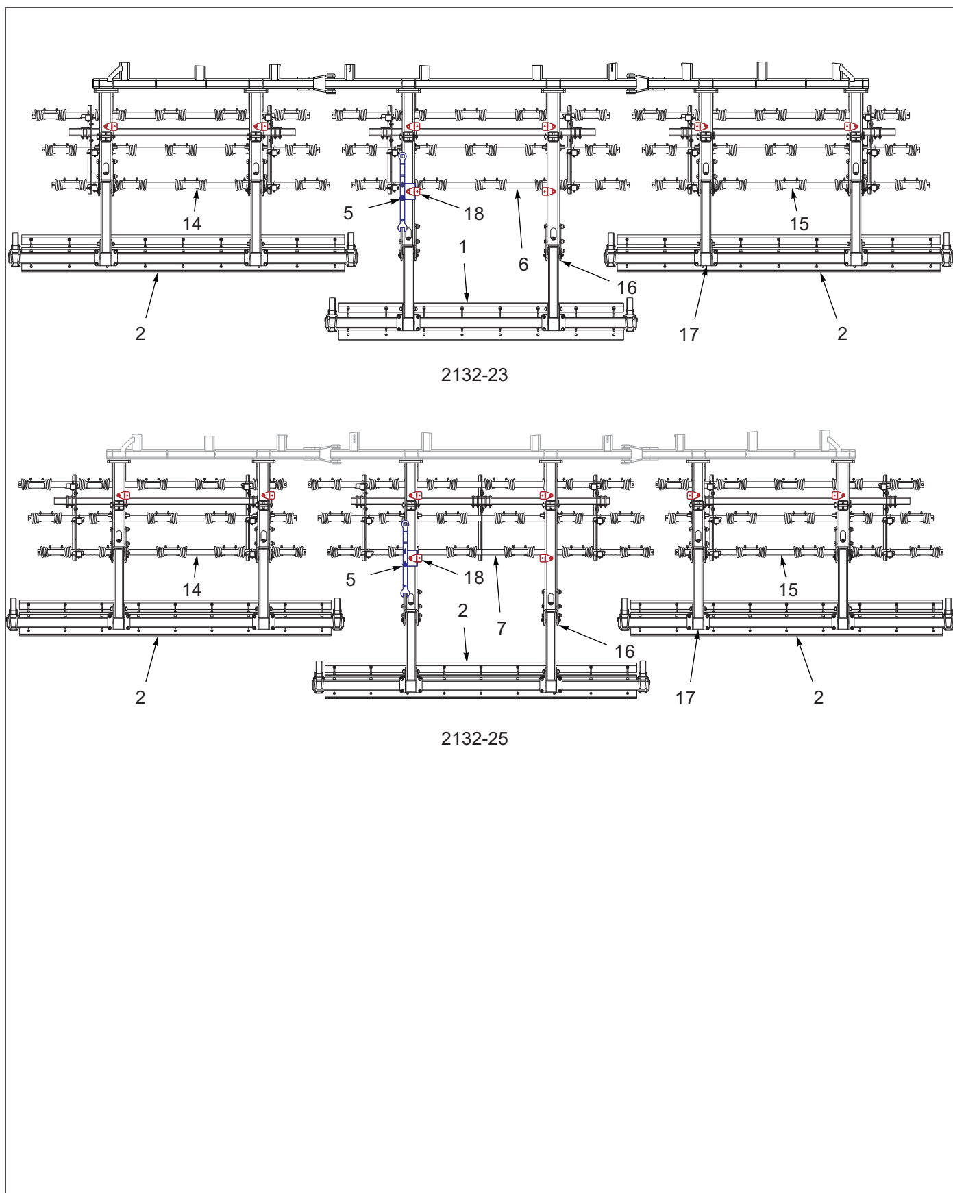
Figure 1-47: Hyd 3BCT/Chopper Layout (2 of 2)
