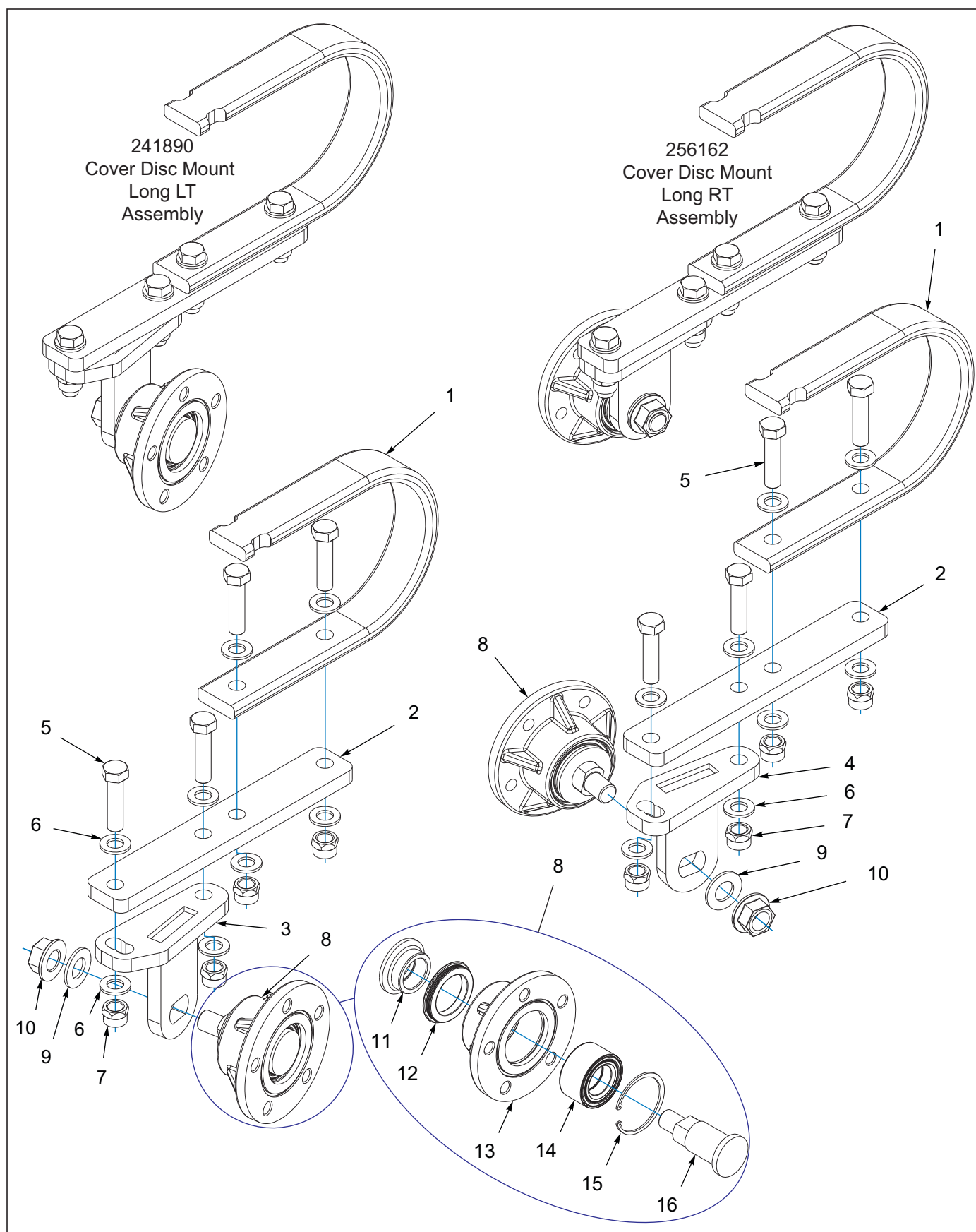
Figure 1-70: Center Disc Mount Long Assembly
