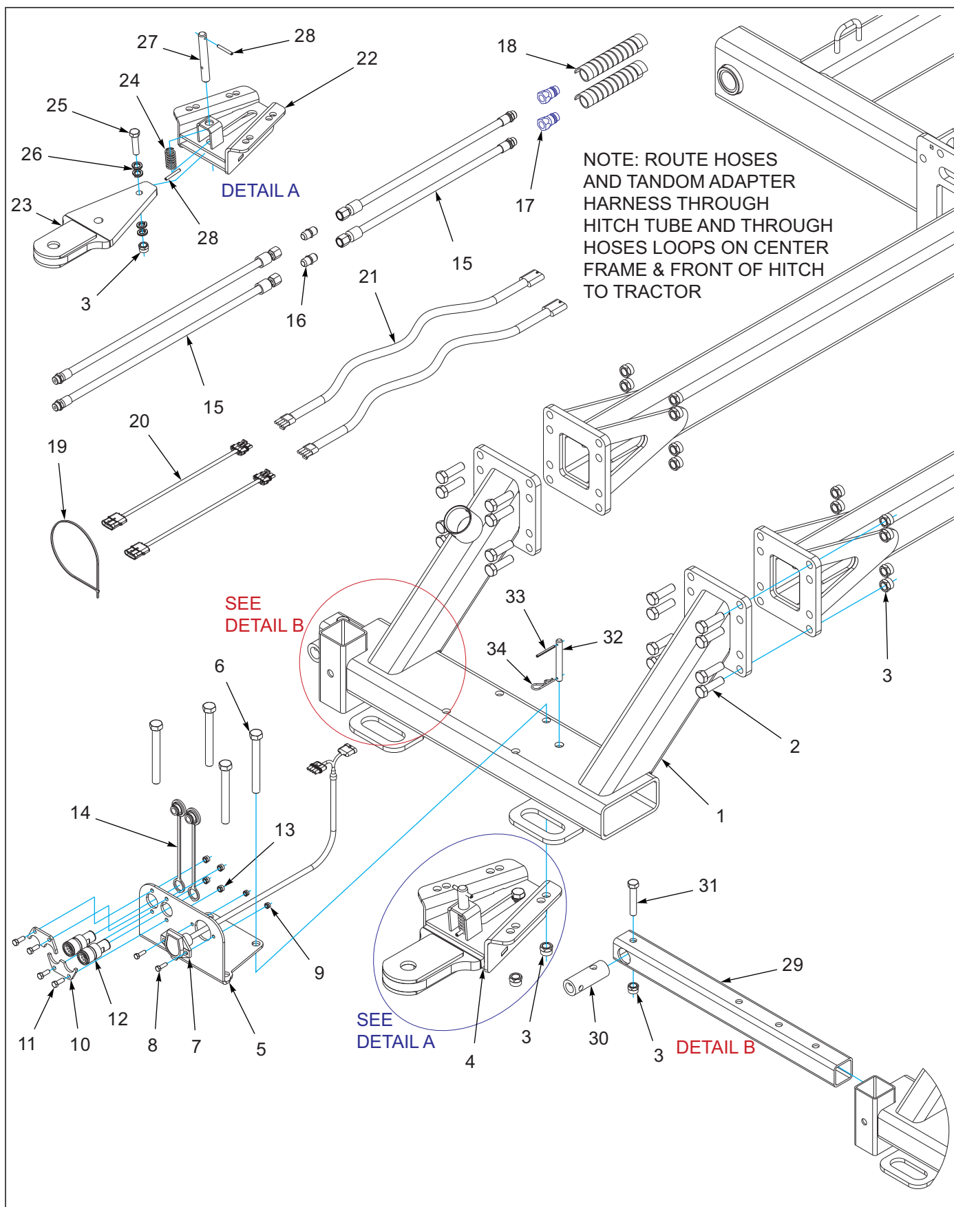
Figure 1-75: Rear Tow Hitch Assembly (2 of 2)
