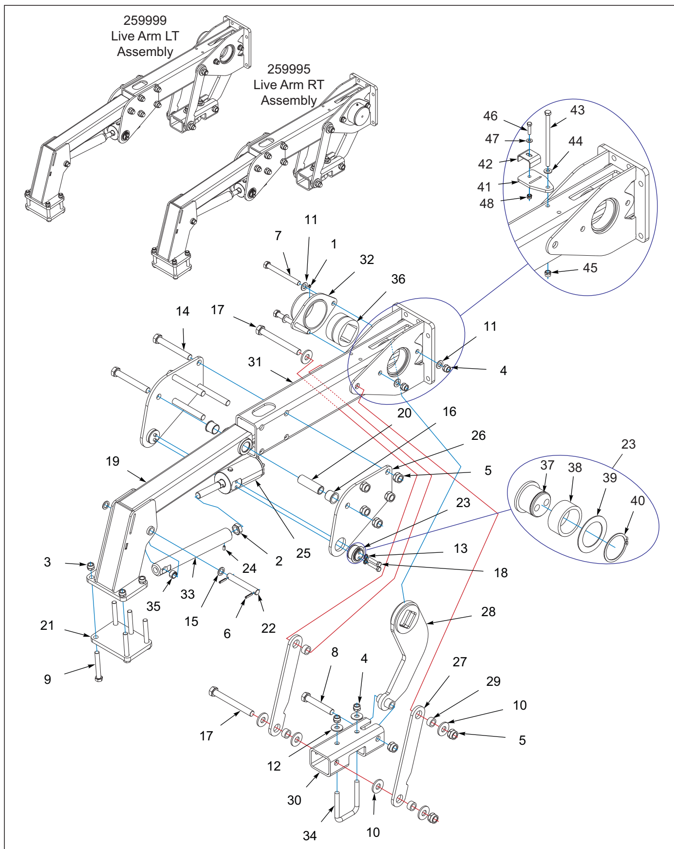
Figure 1-67: Live Hyd Arm No Hyd Assembly
