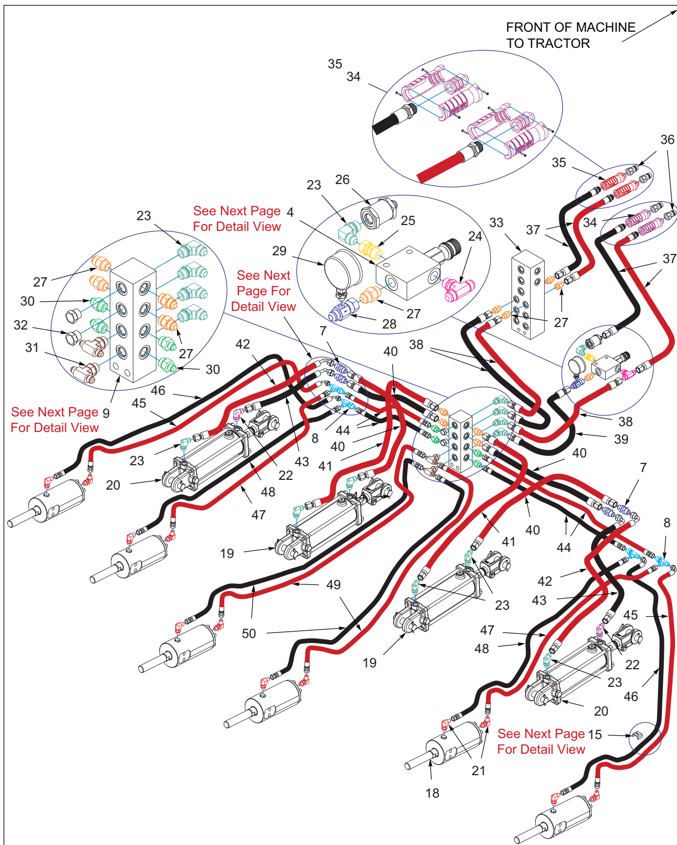
Figure 1-72: Disc Lev/Reel Hydraulic Assembly (1 of 2)
