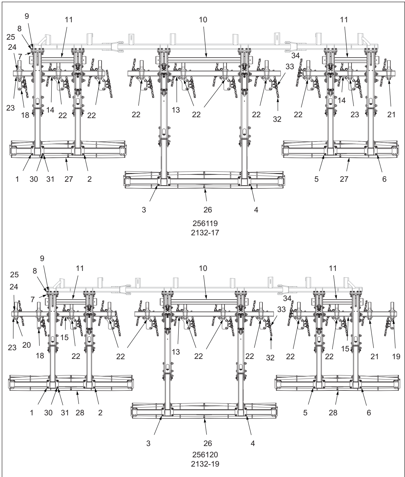
Figure 1-63: Hyd Disc Lev/Reel Layout (1 of 2)
