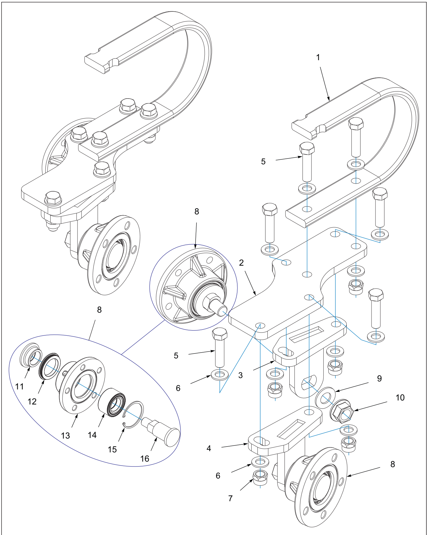
Figure 1-68: Wavy Disc Mount Center Assembly
