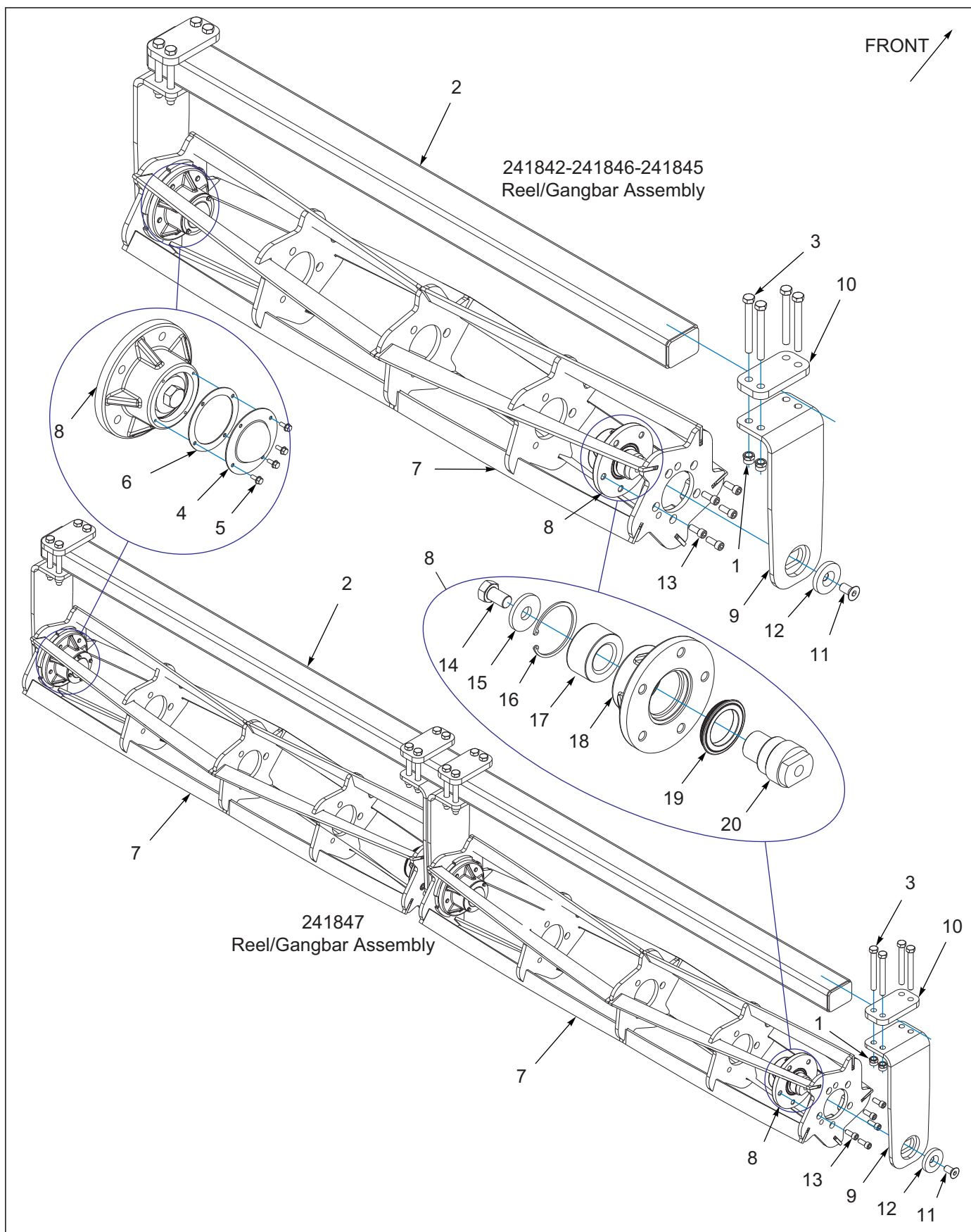
Figure 1-71: Flat Reel/Gangbar Assembly
