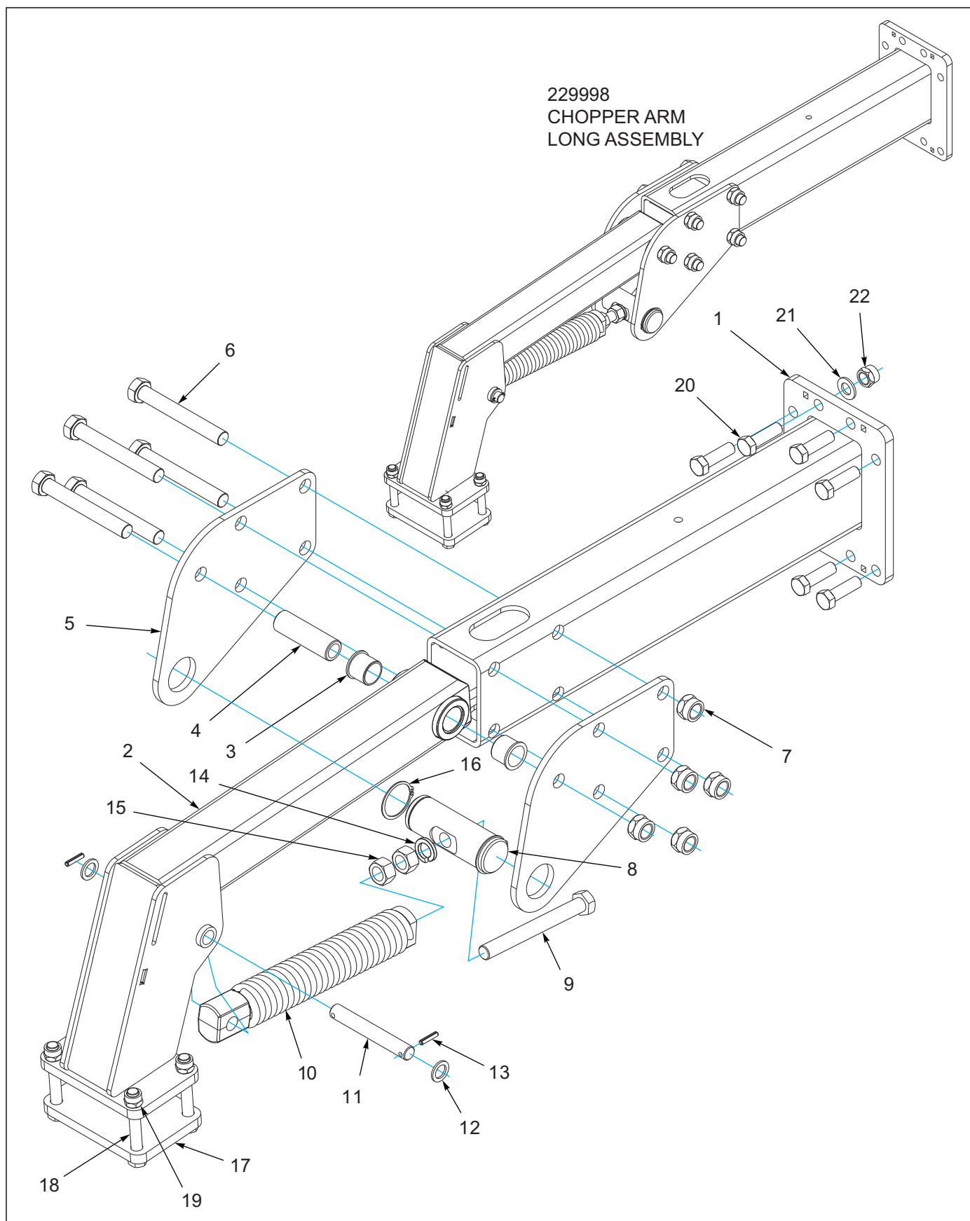
Figure 1-54: Std Chopper Arm Long Assembly
