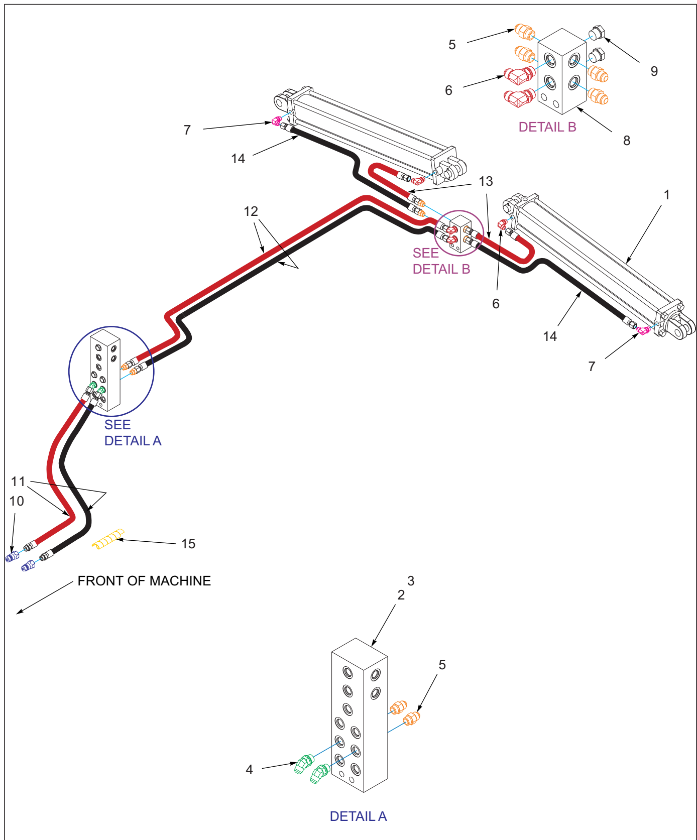
Figure 1-21: Fold Assembly 2132-17-19
