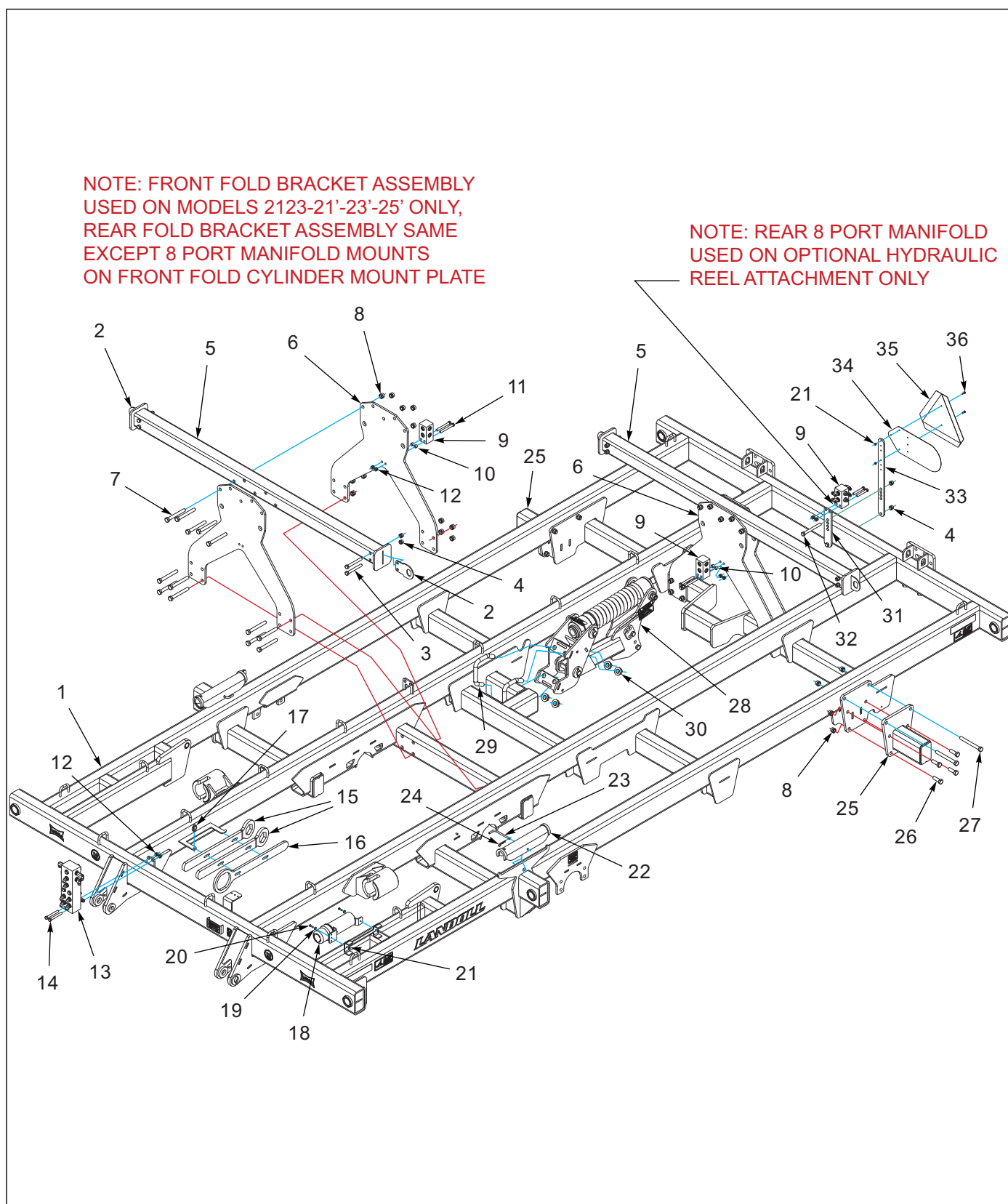
Figure 1-2: Center Frame Assembly
