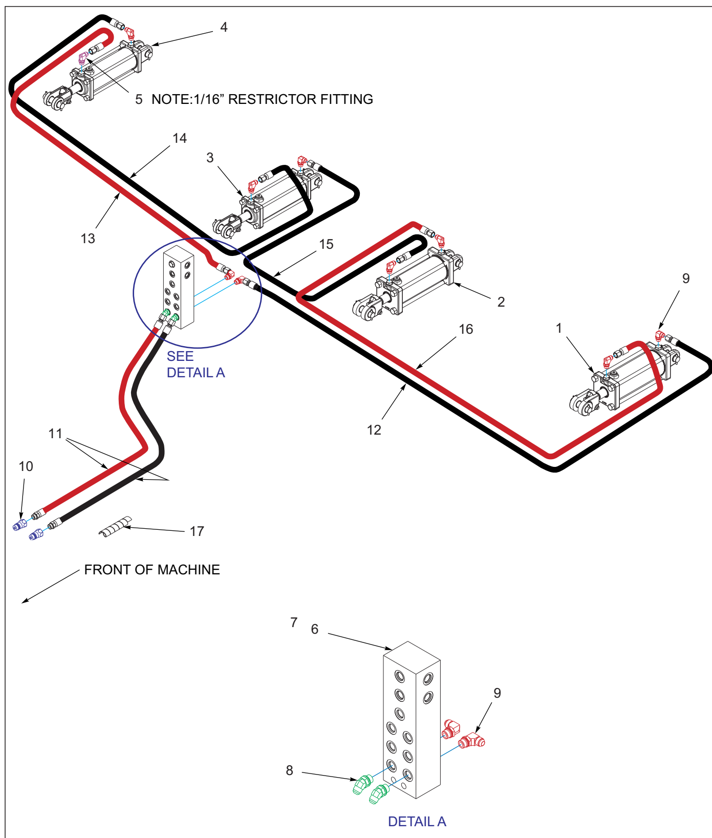
Figure 1-23: Coultter Gang Assembly
