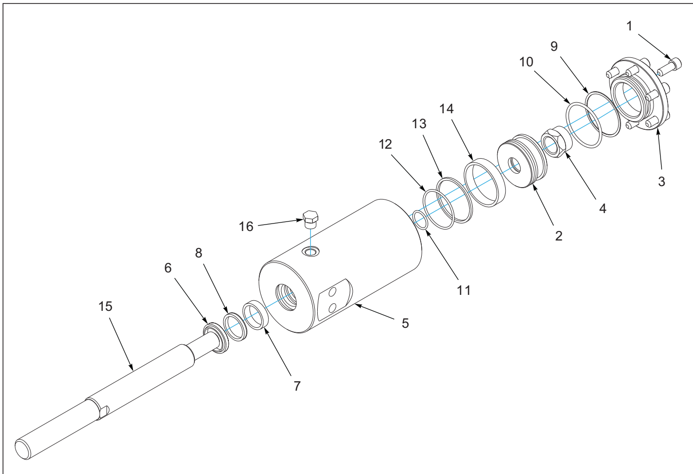
Figure 1-37: Cylinder - 2-1/2" X 3-1/2"
