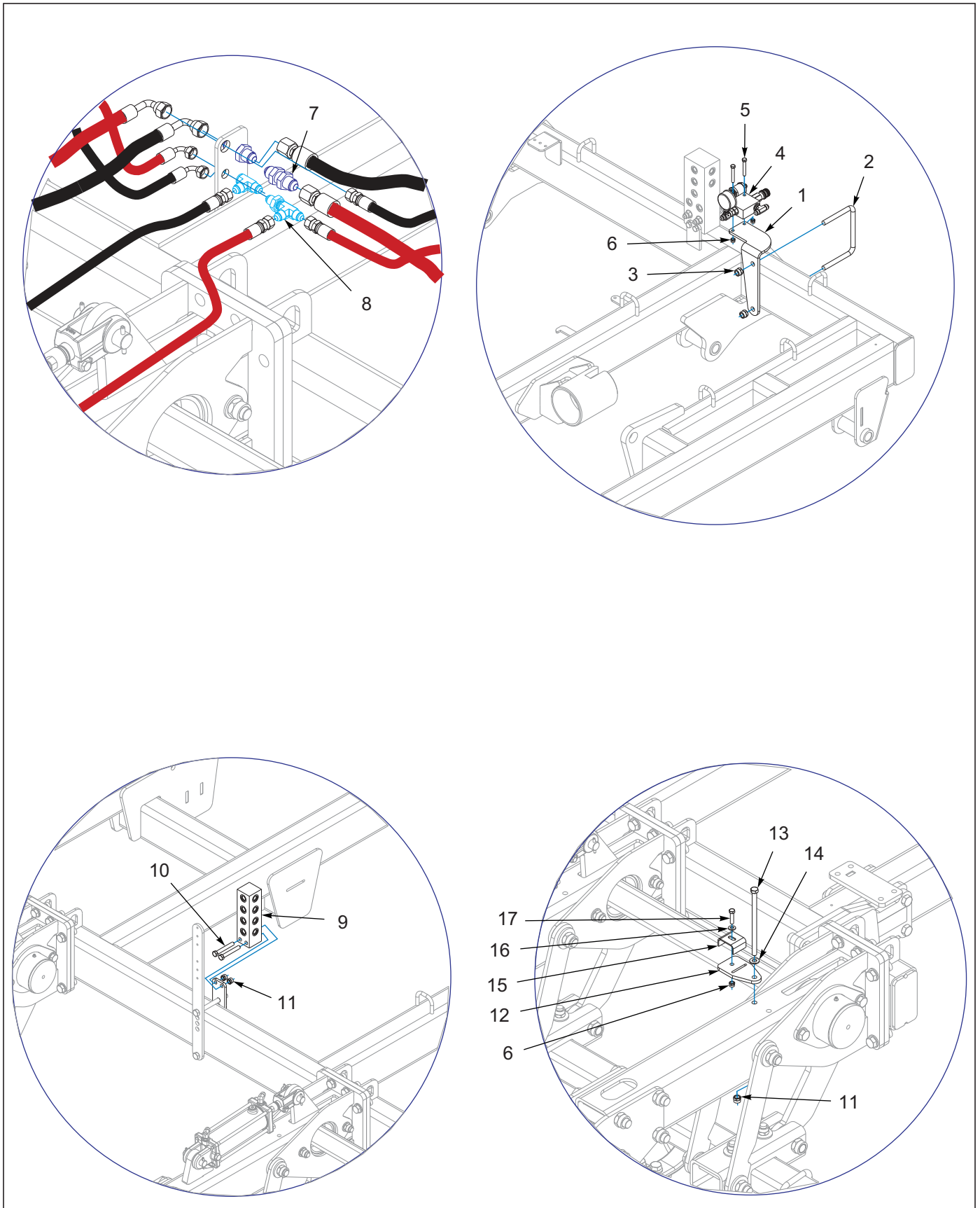
Figure 1-73: Disc Lev/Reel Hydraulic Assembly (2of 2)
