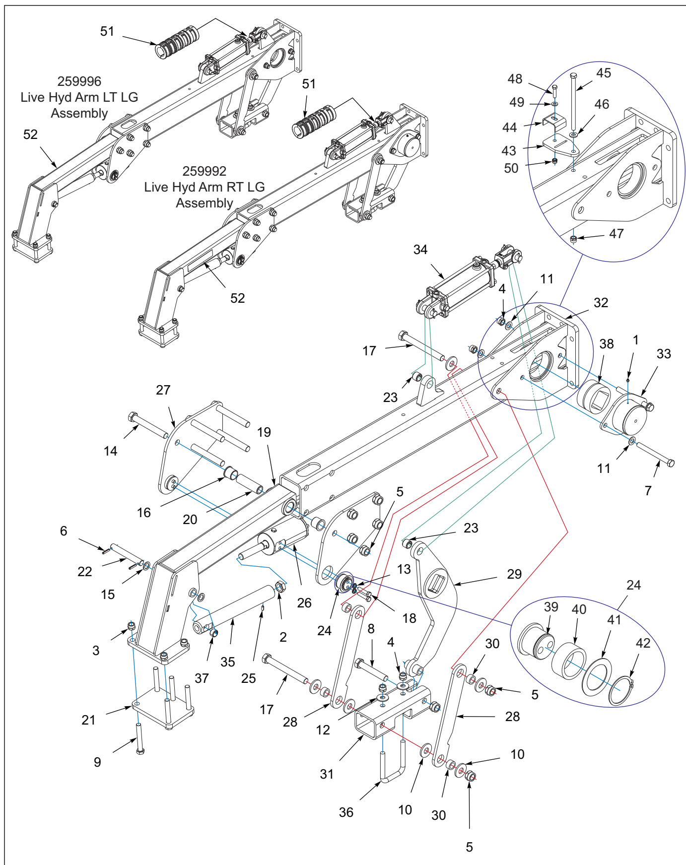
Figure 1-66: Live Hyd Arm LG Assembly
