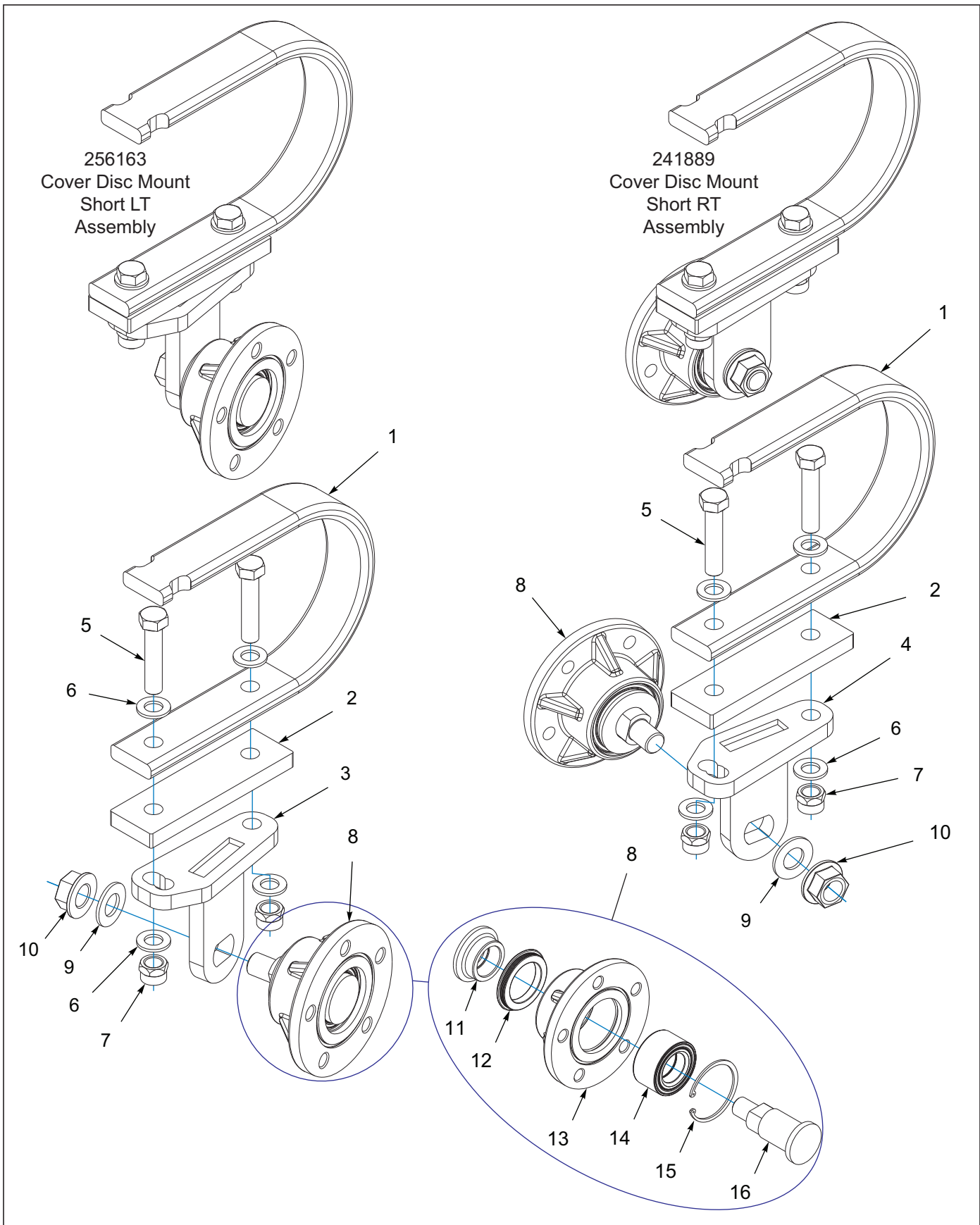
Figure 1-69: Center Disc Mount Short Assembly
