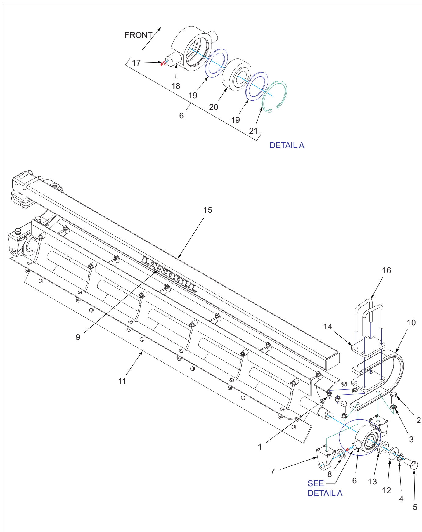
Figure 1-60: Reel/Gangbar Assembly
