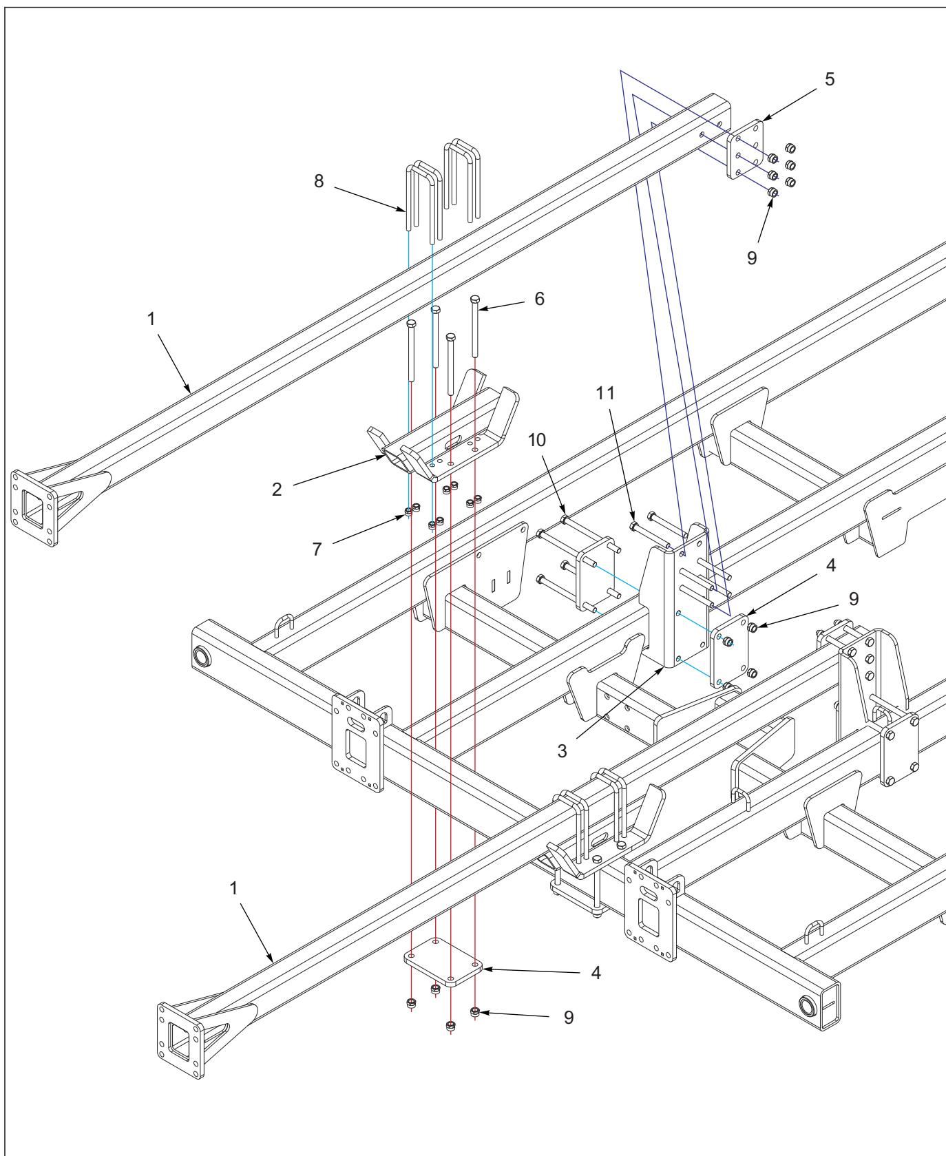
Figure 1-74: Rear Tow Hitch Assembly (1 of 2)
