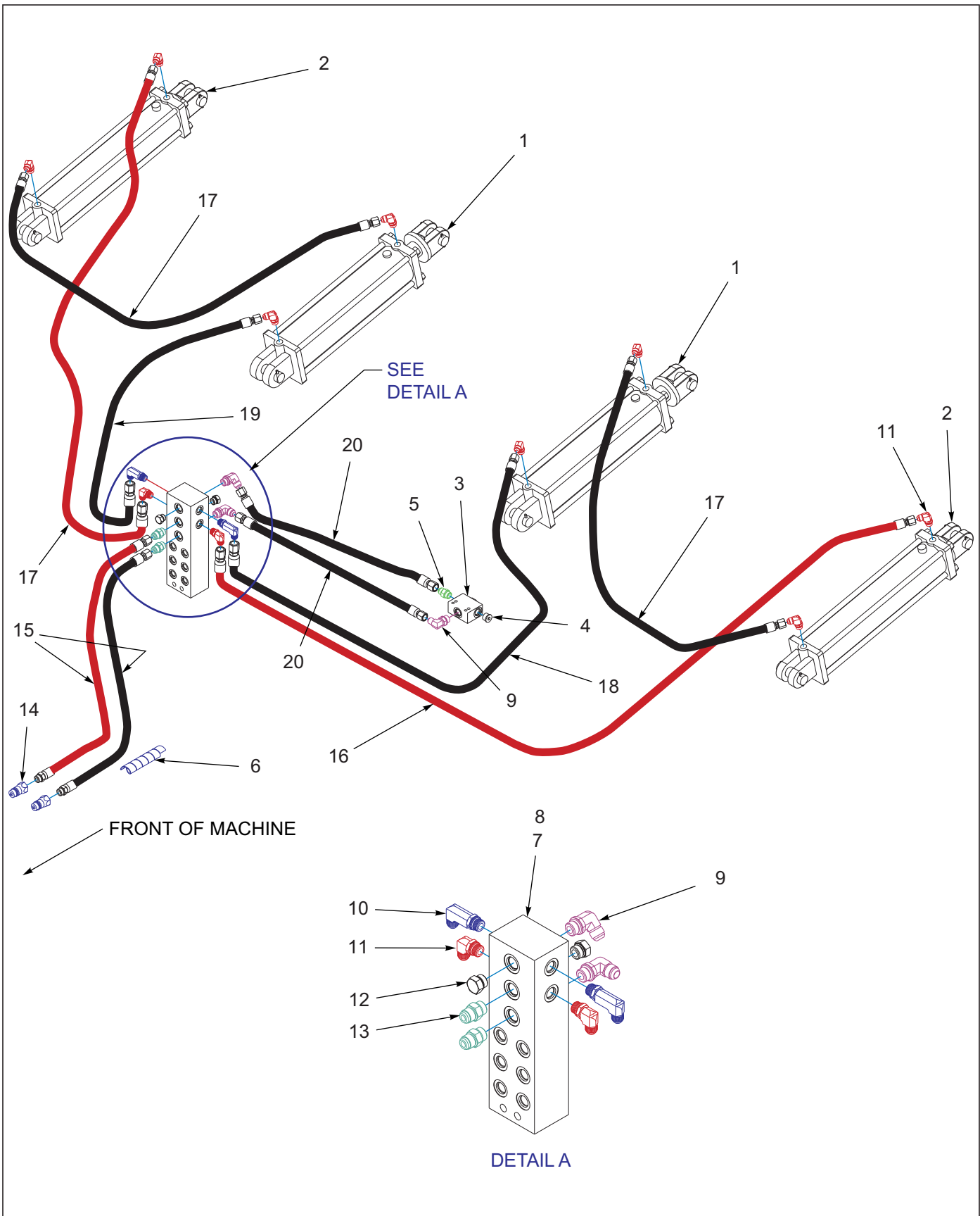
Figure 1-20: Lift Hydraulic Assembly 2132-17-19 After 01-01-2024 &amp; 21-23-25 After 10-03-2023
