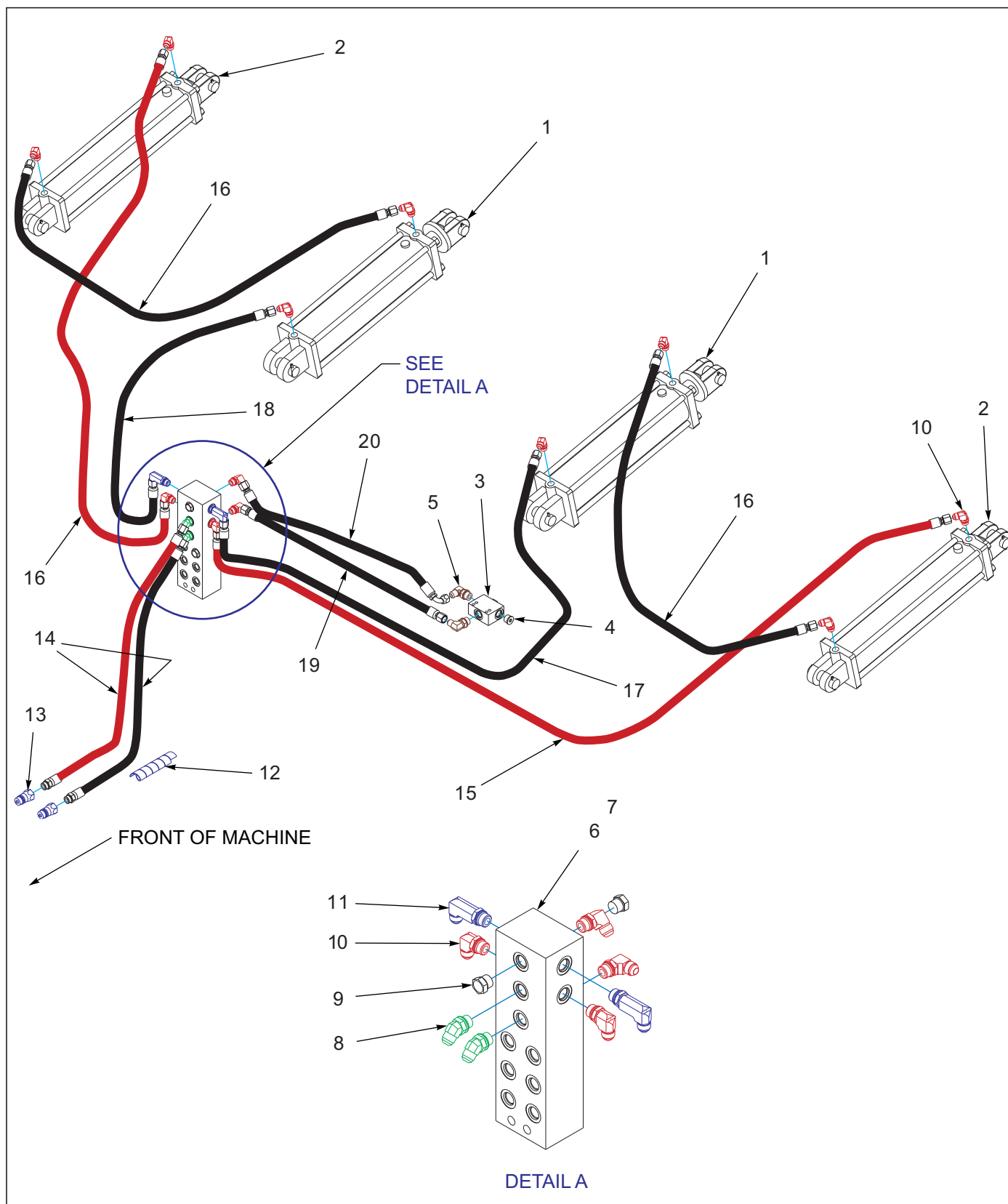
Figure 1-19: Lift Hydraulic Assembly 2132-17-19 Before 01-01-2024 & 21-23-25 Before 10-03-2023
